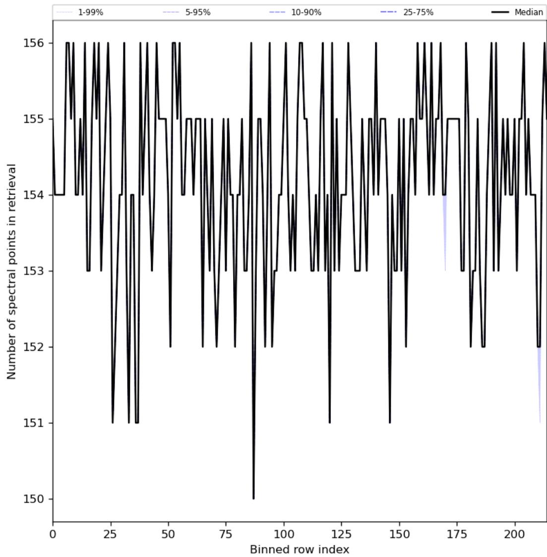
Figure 29: Along track statistics of “Number of spectral points in retrieval” for 2023-12-02 to 2023-12-04
