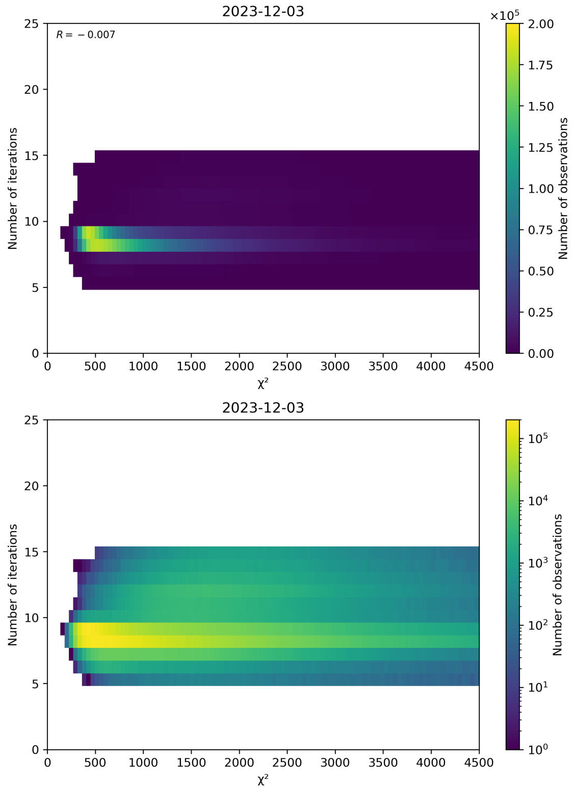
Figure 49: Scatter density plot of “ \chi^2 ” against “Number of iterations” for 2023-12-02 to 2023-12-04.
