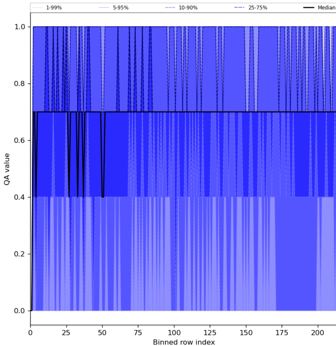
Figure 25: Along track statistics of “QA value” for 2023-12-02 to 2023-12-04
