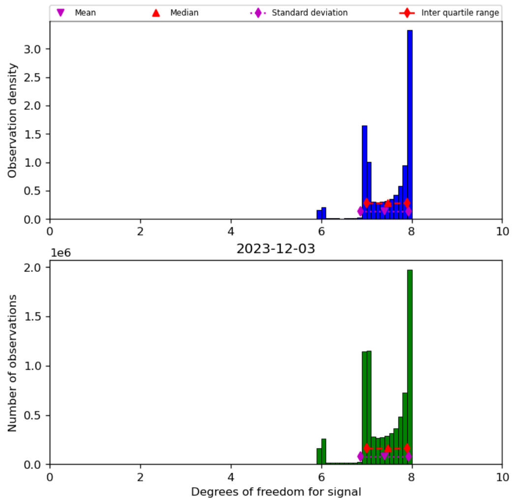
Figure 23: Histogram of “Degrees of freedom for signal” for 2023-12-02 to 2023-12-04
