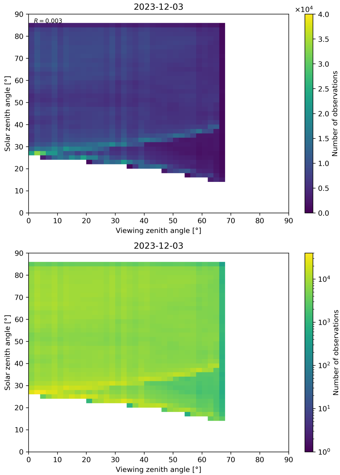
Figure 77: Scatter density plot of “Viewing zenith angle” against “Solar zenith angle” for 2023-12-02 to 2023-12-04.
