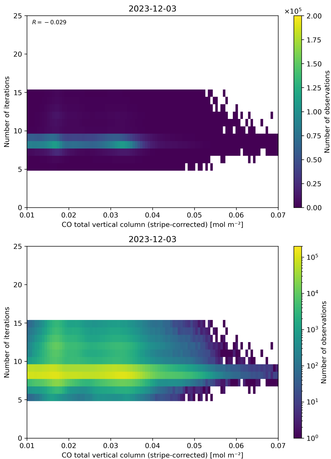
Figure 39: Scatter density plot of “CO total vertical column (stripe-corrected)” against “Number of iterations” for 2023-12-02 to 2023-12-04.
