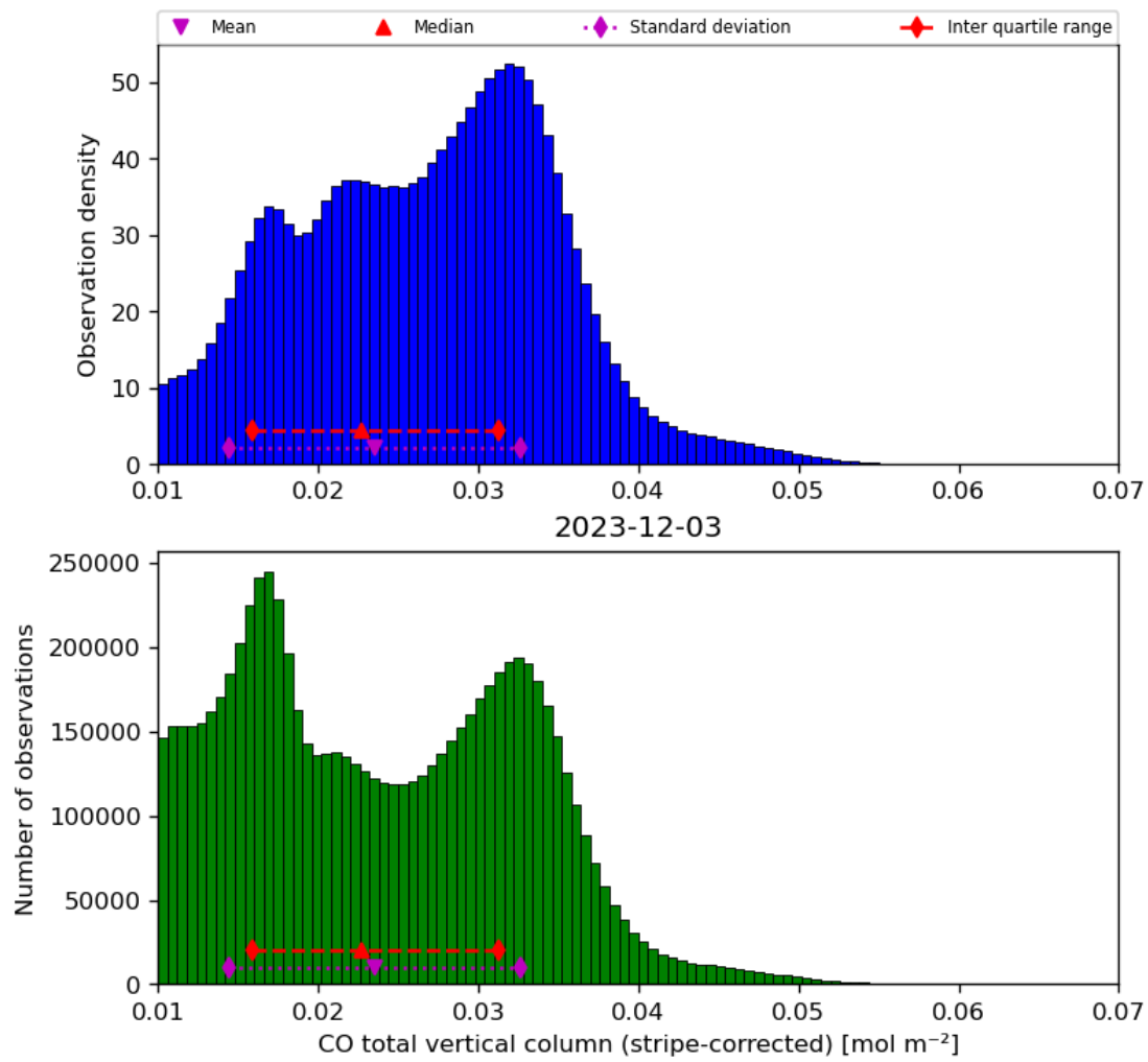
Figure 19: Histogram of “CO total vertical column (stripe-corrected)” for 2023-12-02 to 2023-12-04
