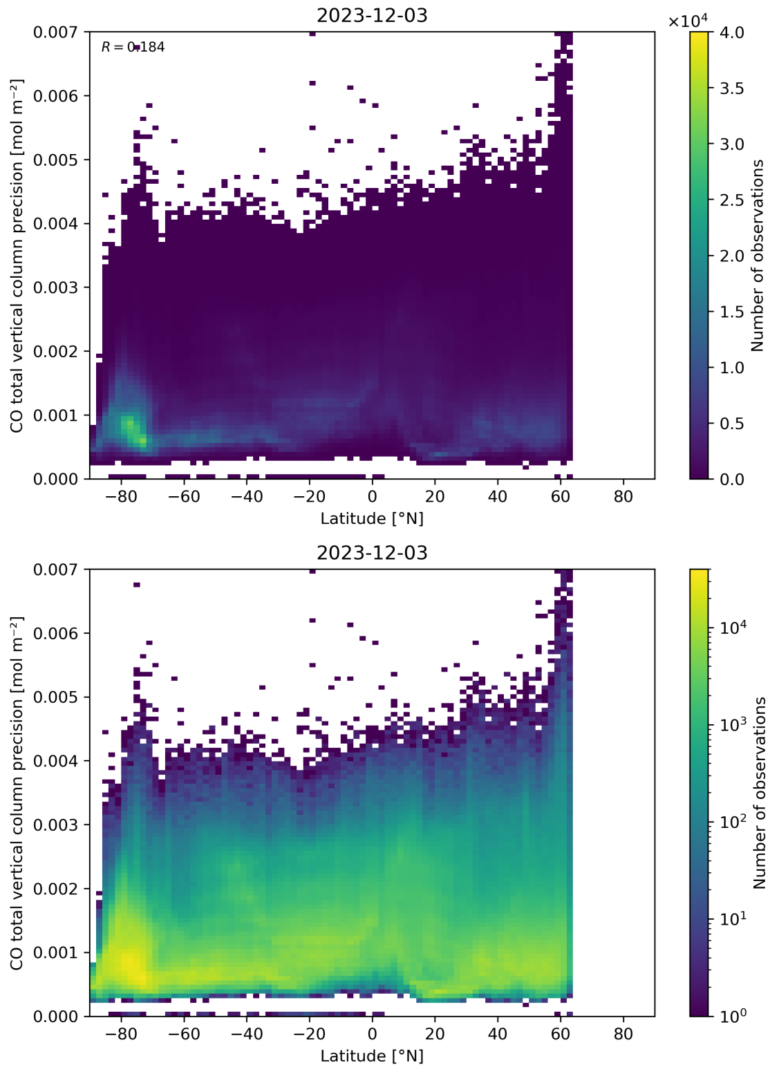
Figure 53: Scatter density plot of “Latitude” against “CO total vertical column precision” for 2023-12-02 to 2023-12-04.
