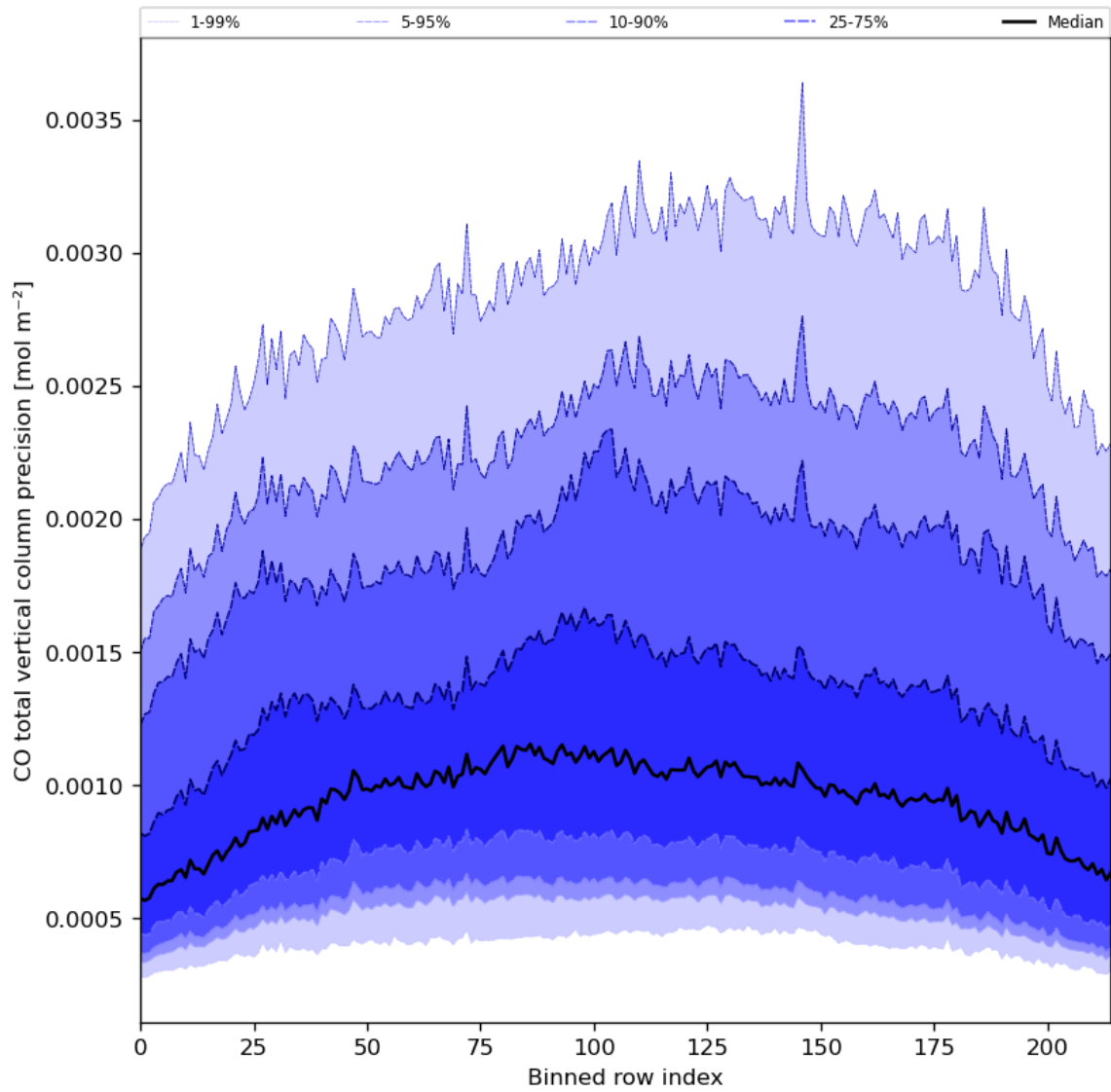
Figure 28: Along track statistics of “CO total vertical column precision” for 2023-12-02 to 2023-12-04
