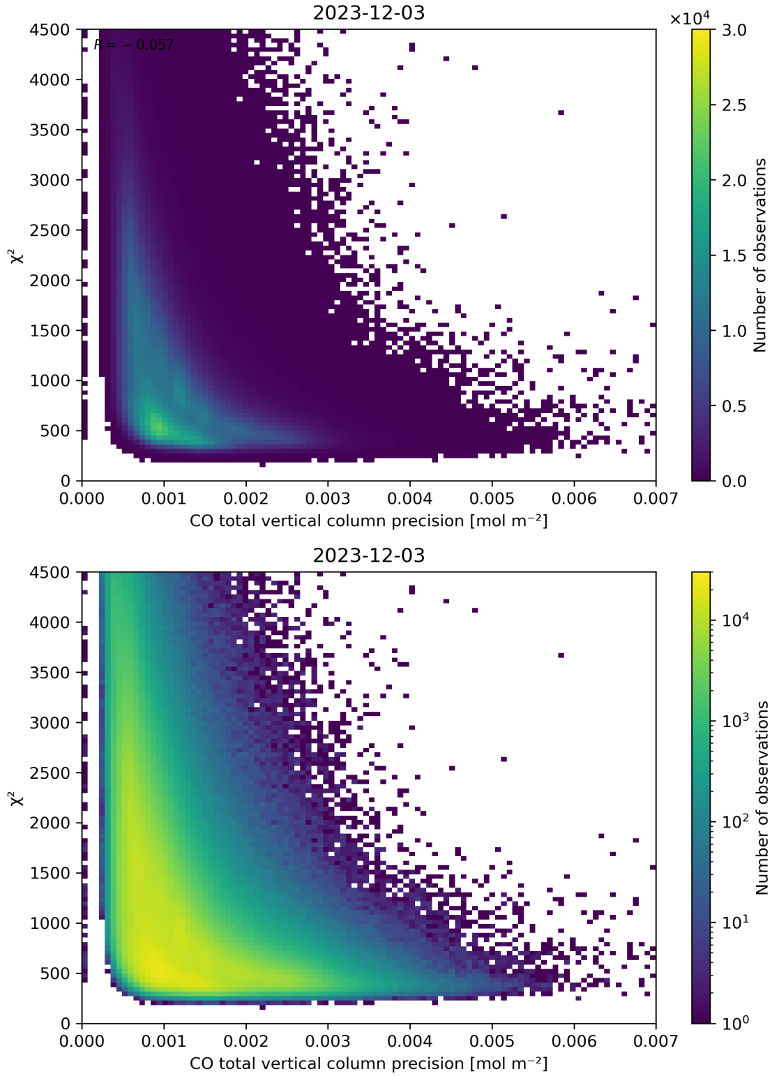
Figure 44: Scatter density plot of “CO total vertical column precision” against “ \chi^2 ” for 2023-12-02 to 2023-12-04.
