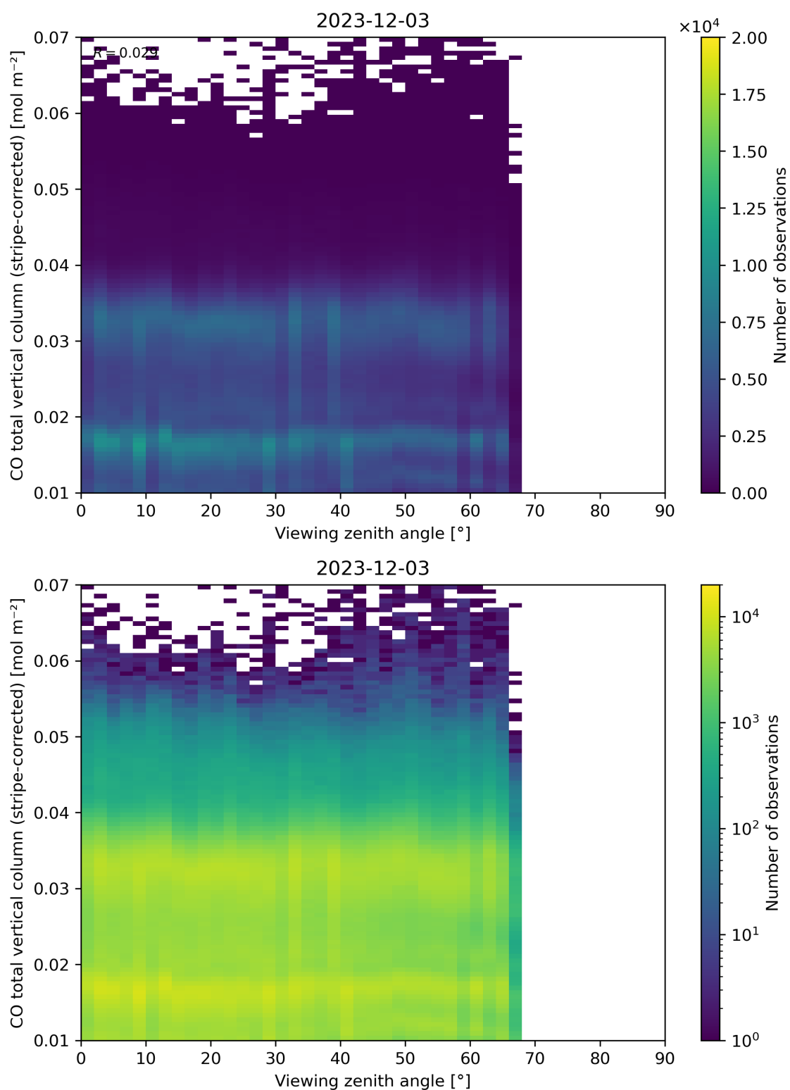
Figure 70: Scatter density plot of “Viewing zenith angle” against “CO total vertical column (stripe-corrected)” for 2023-12-02 to 2023-12-04.
