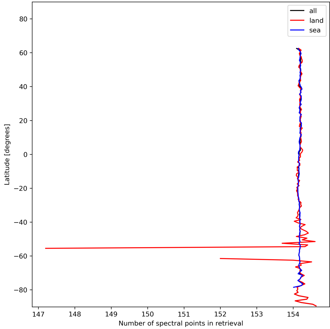
Figure 13: Zonal average of “Number of spectral points in retrieval” for 2023-12-02 to 2023-12-04.
