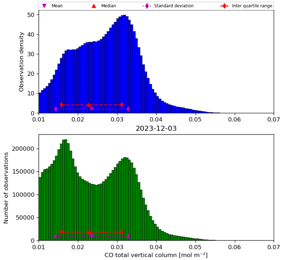
Figure 18: Histogram of “CO total vertical column” for 2023-12-02 to 2023-12-04
