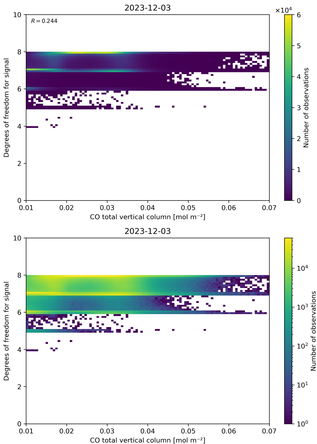
Figure 41: Scatter density plot of “CO total vertical column” against “Degrees of freedom for signal” for 2023-12-02 to 2023-12-04.
