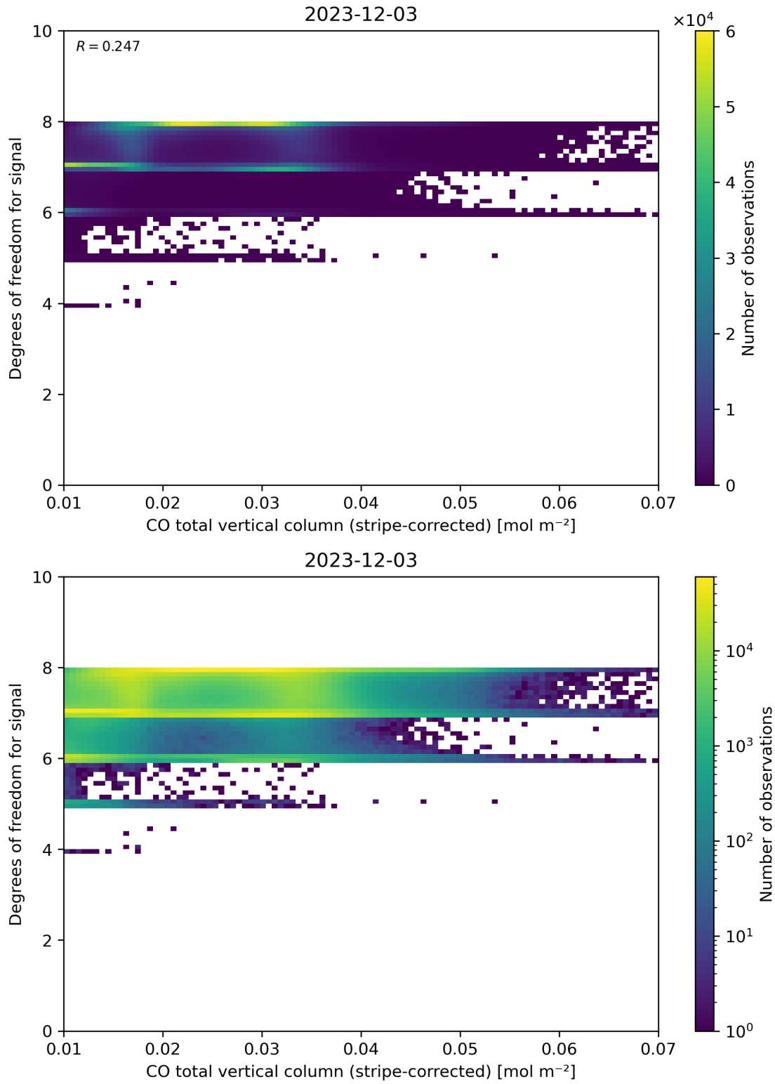
Figure 38: Scatter density plot of “CO total vertical column (stripe-corrected)” against “Degrees of freedom for signal” for 2023-12-02 to 2023-12-04.
