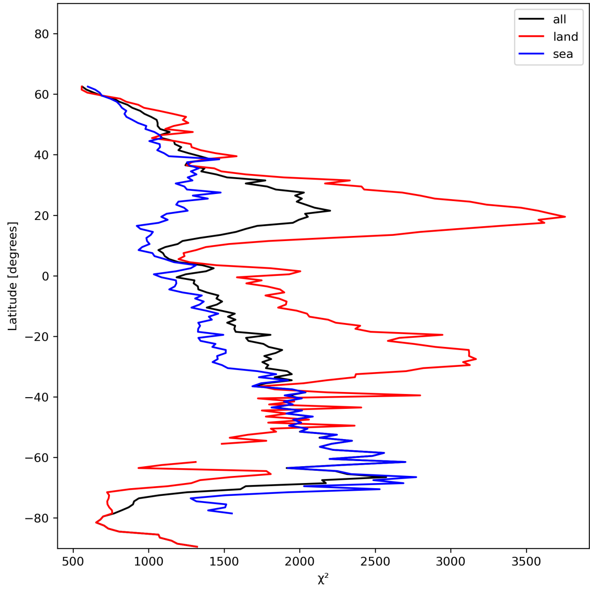
Figure 14: Zonal average of “ \chi^2 ” for 2023-12-02 to 2023-12-04.
