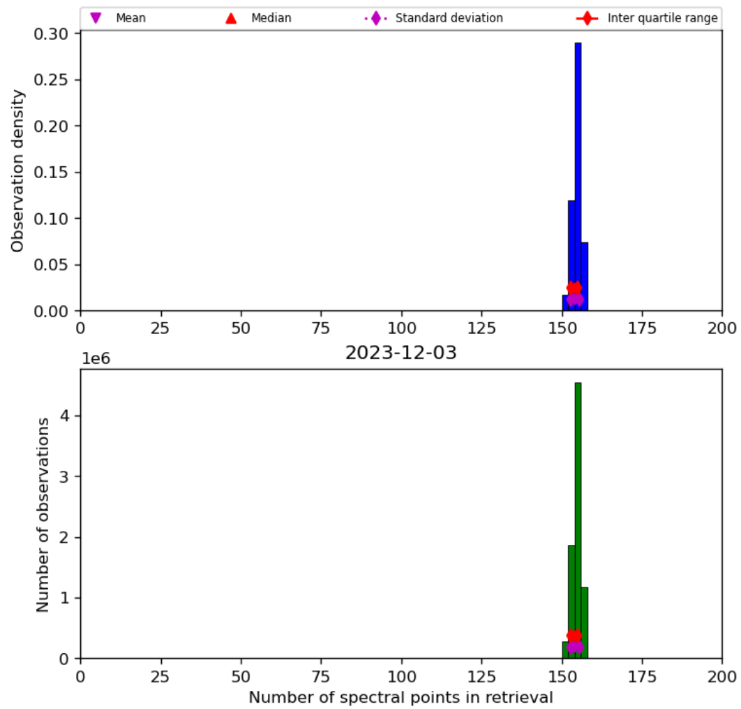
Figure 21: Histogram of "Number of spectral points in retrieval" for 2023-12-02 to 2023-12-04
