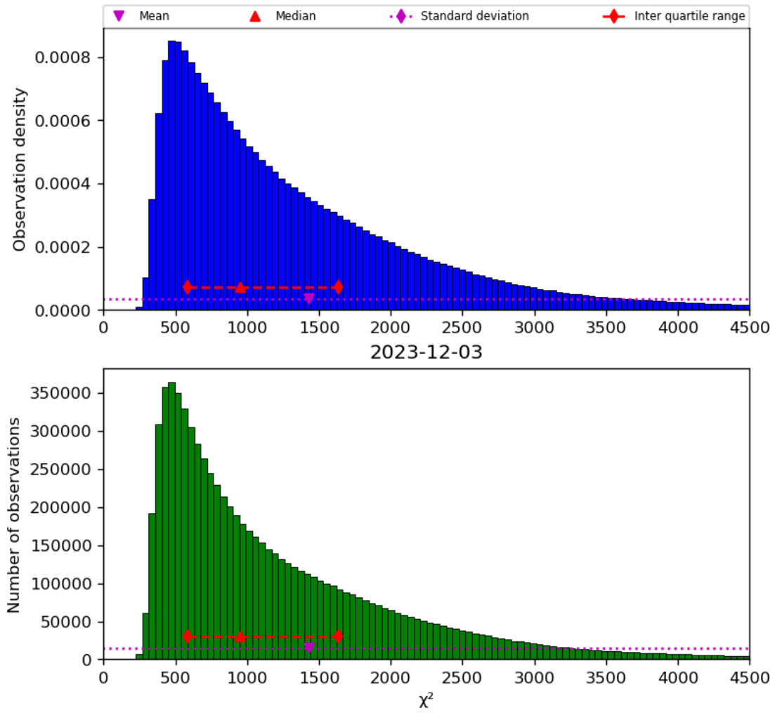
Figure 22: Histogram of " \chi^2 " for 2023-12-02 to 2023-12-04
