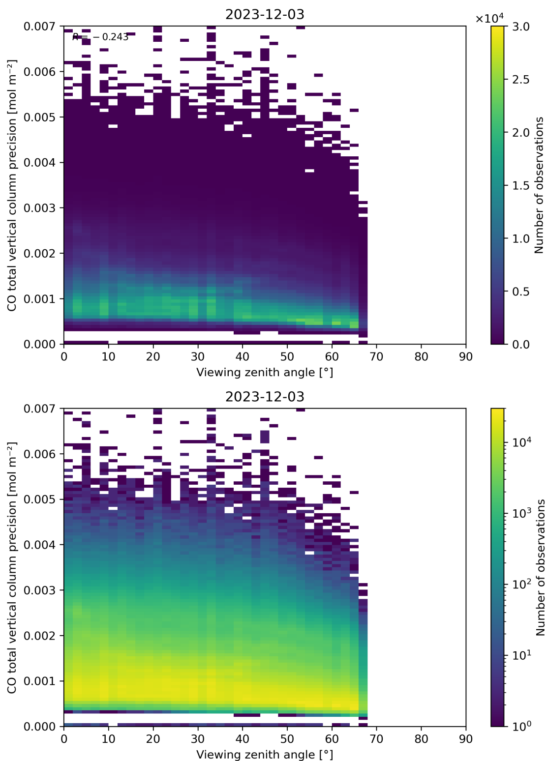
Figure 71: Scatter density plot of “Viewing zenith angle” against “CO total vertical column precision” for 2023-12-02 to 2023-12-04.
