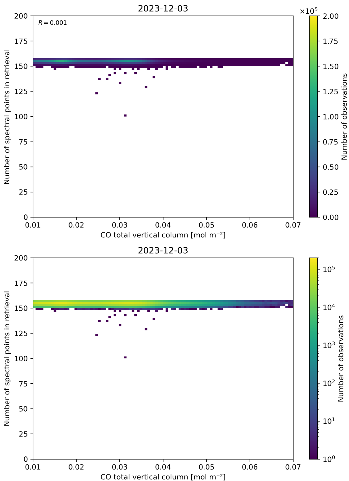
Figure 43: Scatter density plot of “CO total vertical column” against “Number of spectral points in retrieval” for 2023-12-02 to 2023-12-04.
