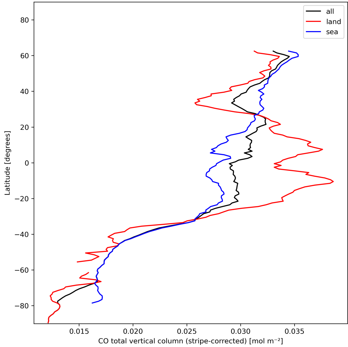
Figure 11: Zonal average of “CO total vertical column (stripe-corrected)” for 2023-12-02 to 2023-12-04.
