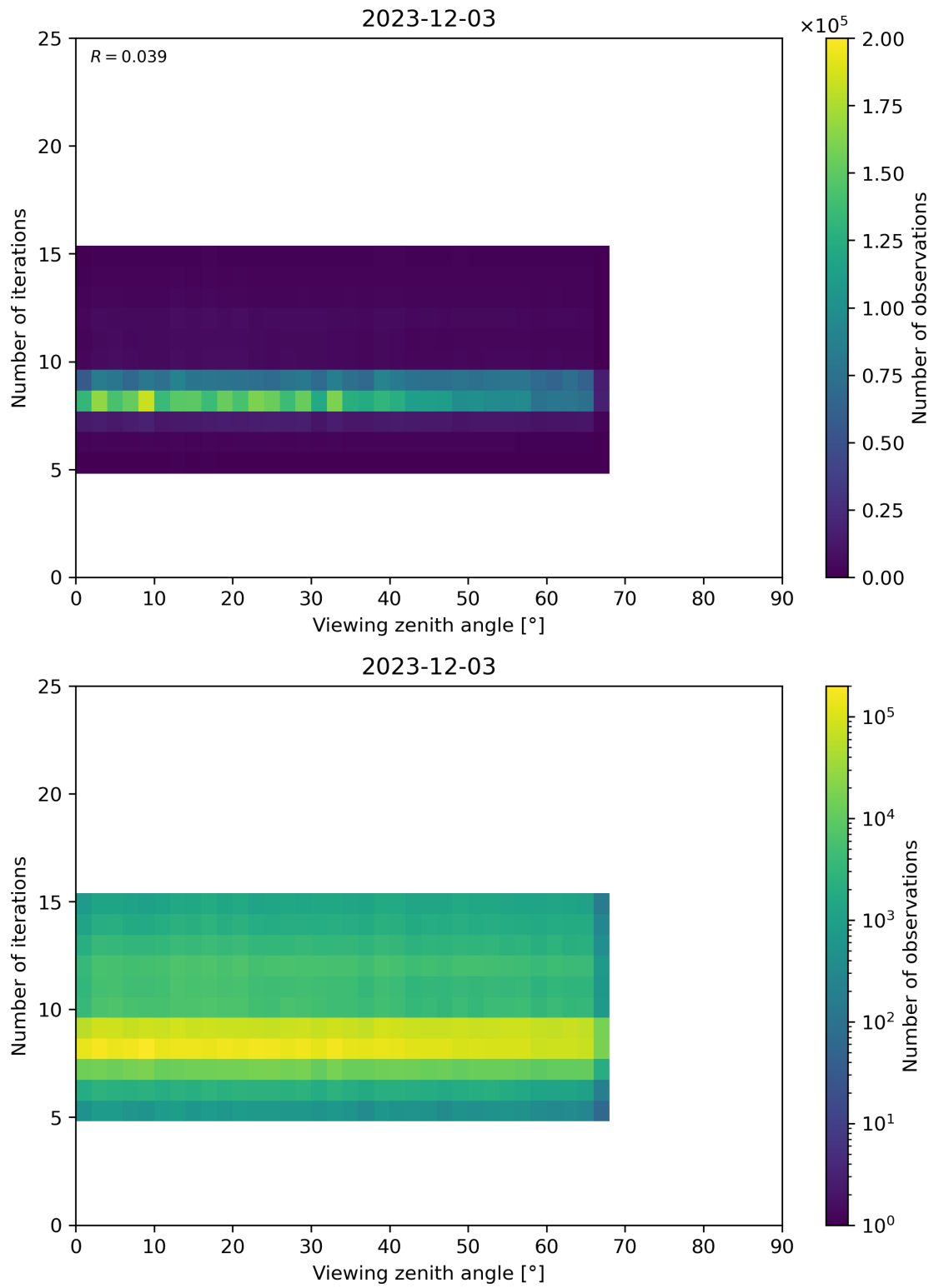
Figure 75: Scatter density plot of “Viewing zenith angle” against “Number of iterations” for 2023-12-02 to 2023-12-04.
