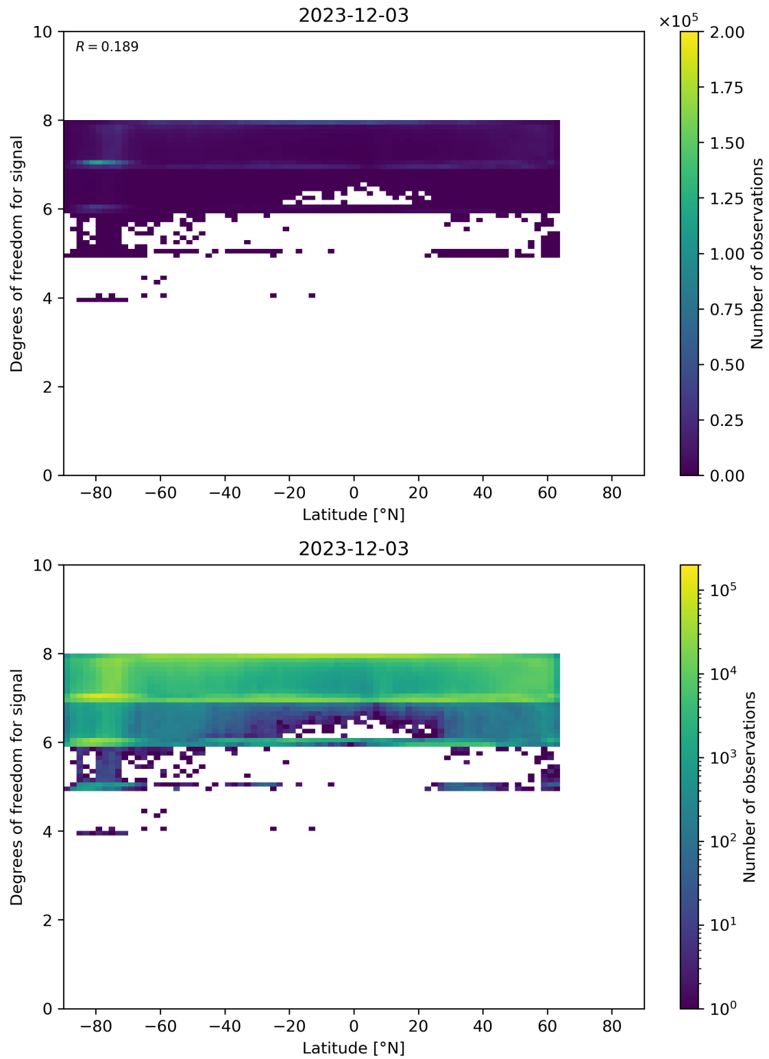
Figure 55: Scatter density plot of “Latitude” against “Degrees of freedom for signal” for 2023-12-02 to 2023-12-04.
