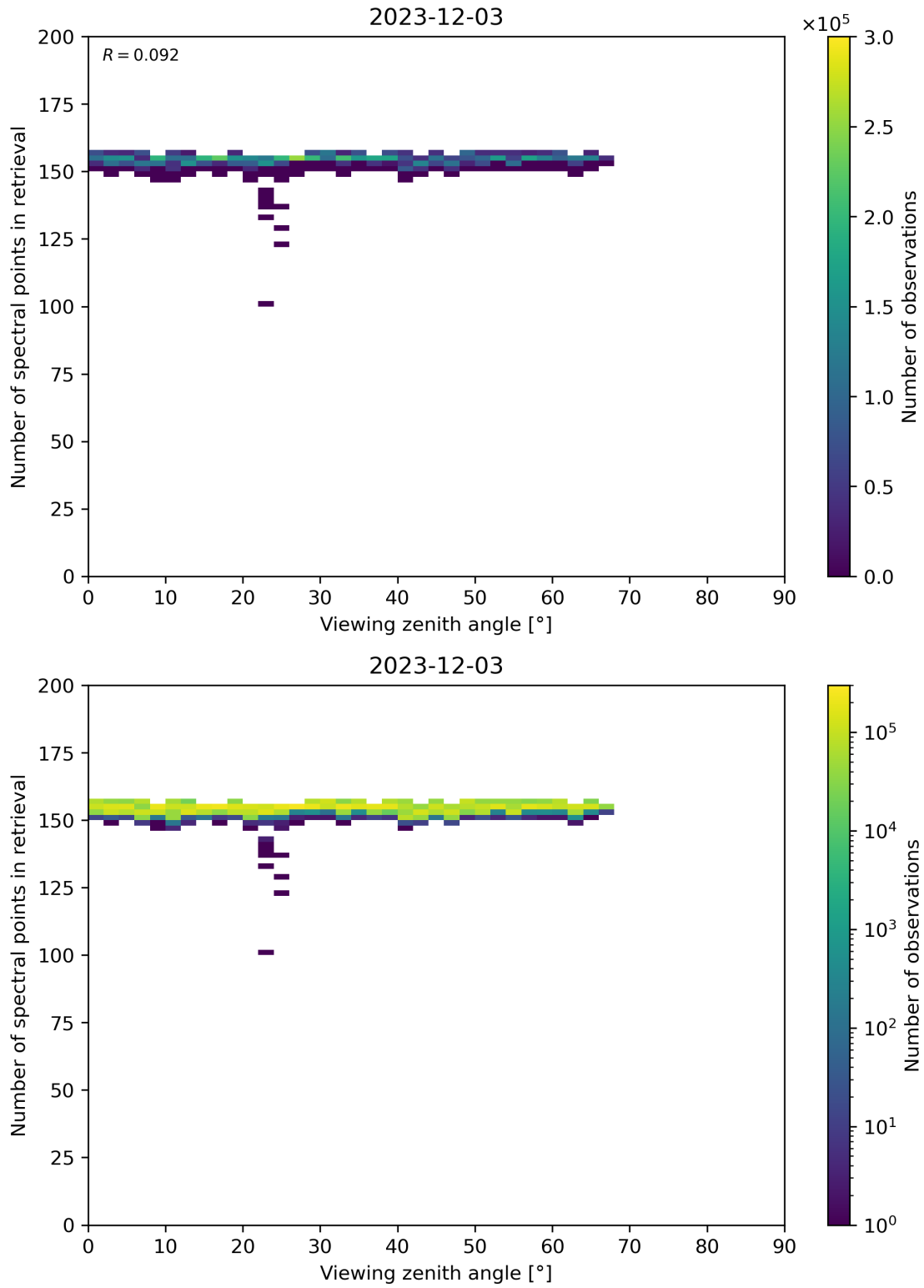
Figure 76: Scatter density plot of “Viewing zenith angle” against “Number of spectral points in retrieval” for 2023-12-02 to 2023-12-04.
