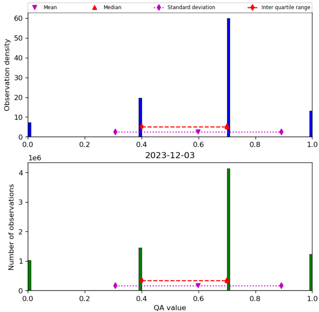
Figure 17: Histogram of “QA value” for 2023-12-02 to 2023-12-04
