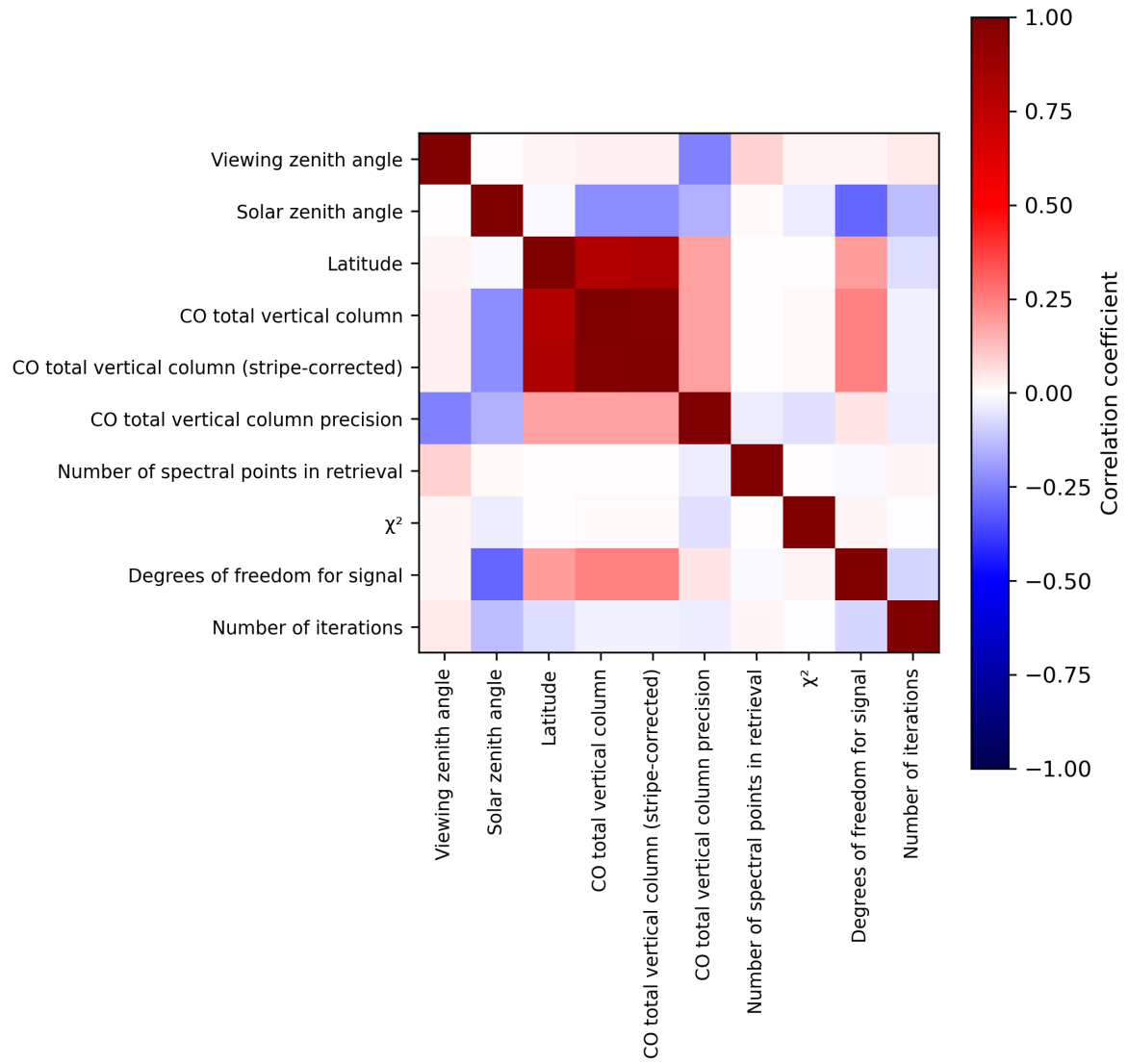
Figure 2: Map of correlation matrix for 2023-12-02 to 2023-12-04.
