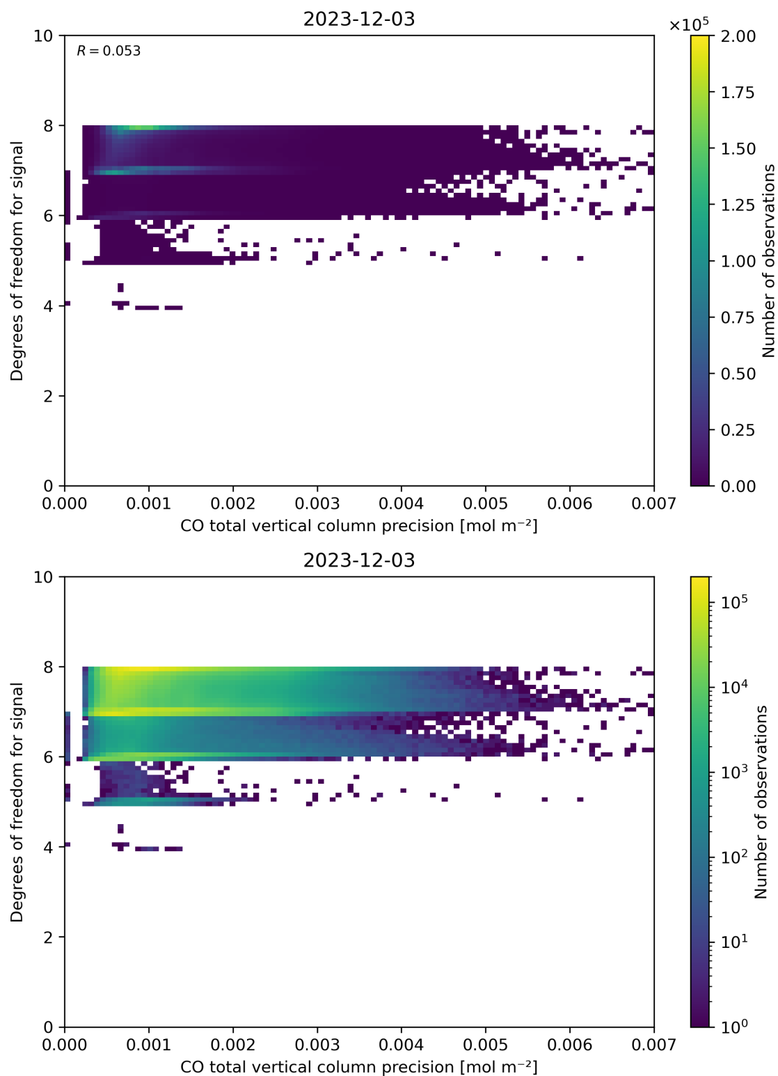
Figure 45: Scatter density plot of “CO total vertical column precision” against “Degrees of freedom for signal” for 2023-12-02 to 2023-12-04.
