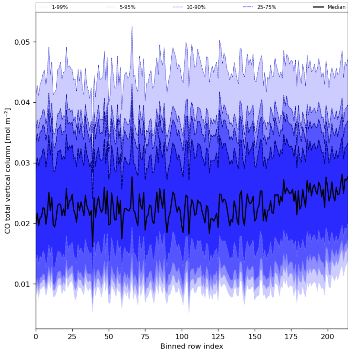
Figure 26: Along track statistics of “CO total vertical column” for 2023-12-02 to 2023-12-04
