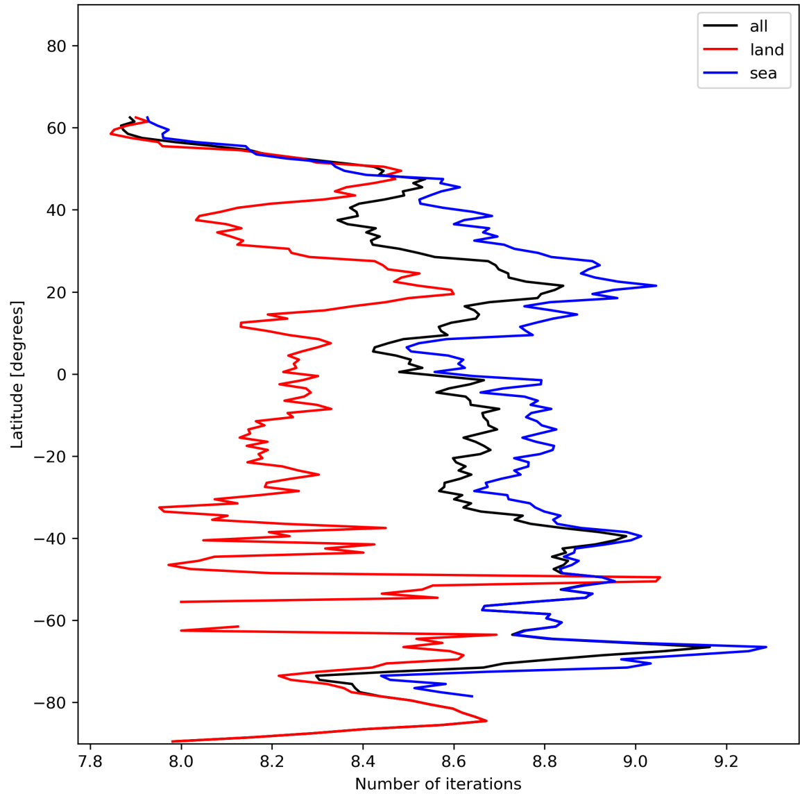
Figure 16: Zonal average of “Number of iterations” for 2023-12-02 to 2023-12-04.
