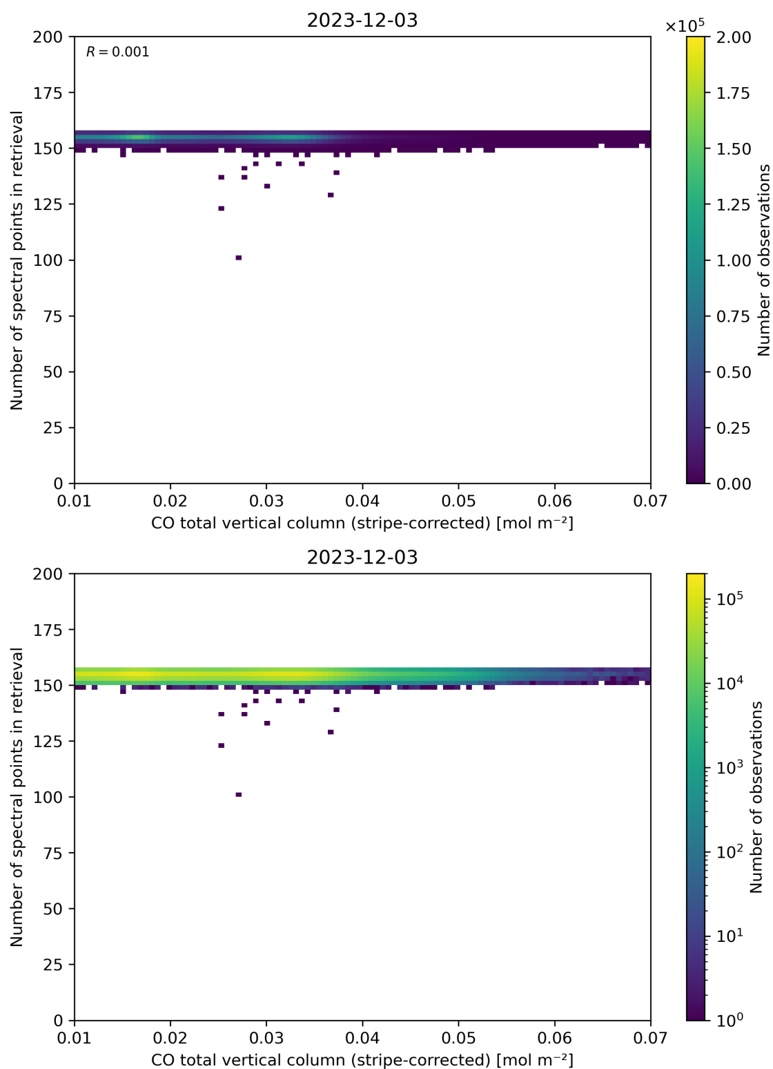
Figure 40: Scatter density plot of “CO total vertical column (stripe-corrected)” against “Number of spectral points in retrieval” for 2023-12-02 to 2023-12-04.
