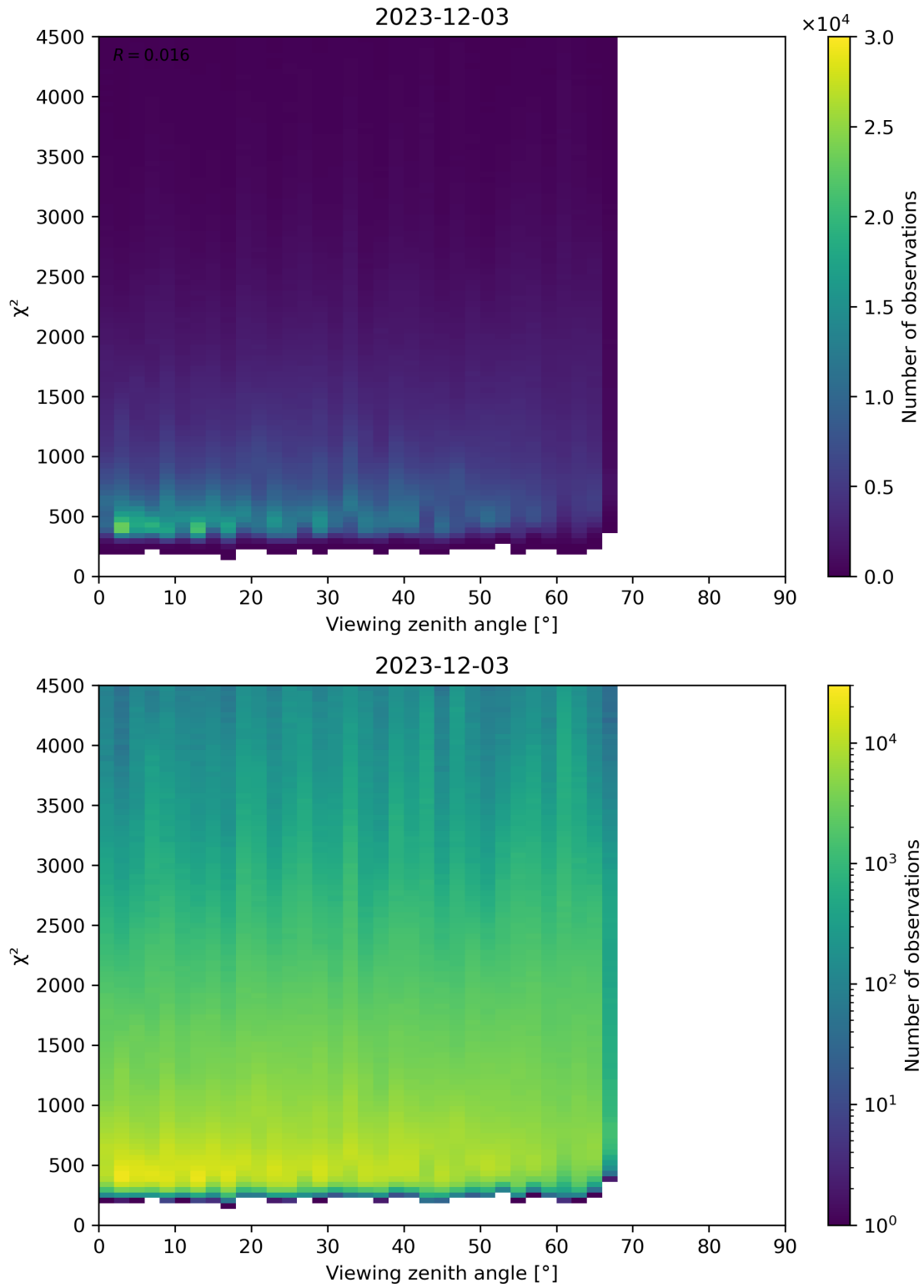
Figure 72: Scatter density plot of “Viewing zenith angle” against “ \chi^2 ” for 2023-12-02 to 2023-12-04.
