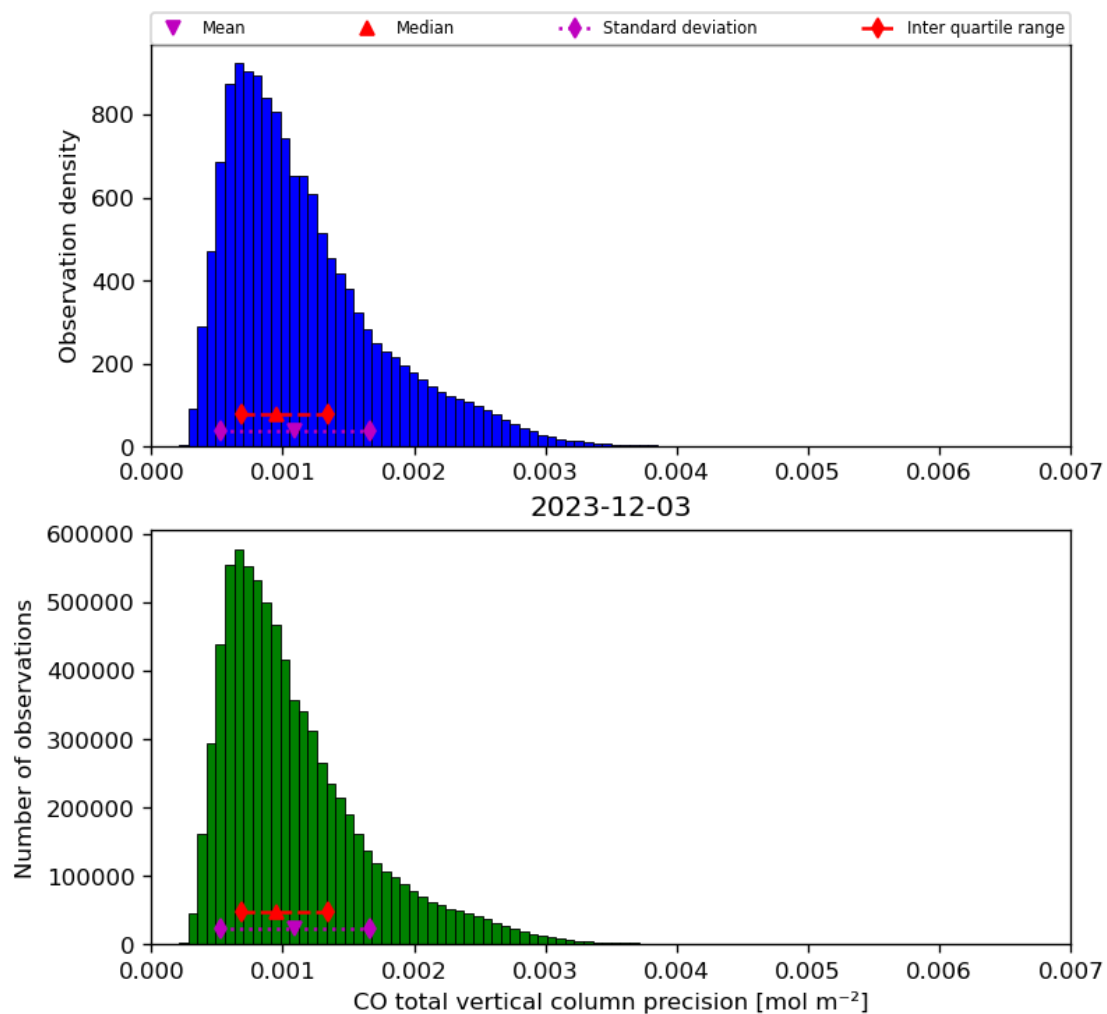
Figure 20: Histogram of “CO total vertical column precision” for 2023-12-02 to 2023-12-04
