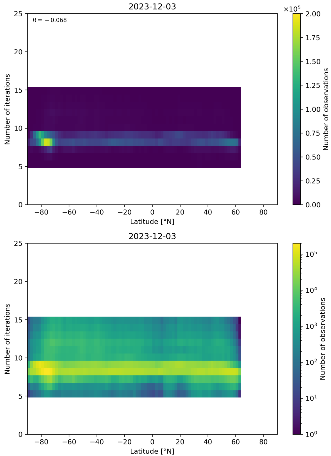
Figure 56: Scatter density plot of “Latitude” against “Number of iterations” for 2023-12-02 to 2023-12-04.
