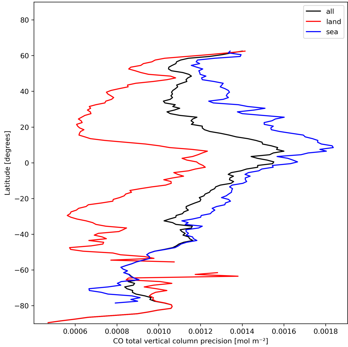
Figure 12: Zonal average of "CO total vertical column precision" for 2023-12-02 to 2023-12-04.
