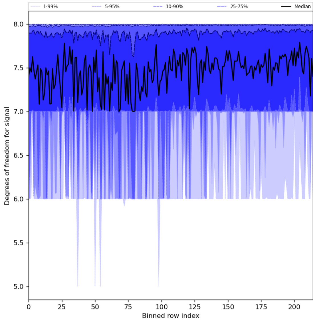
Figure 31: Along track statistics of “Degrees of freedom for signal” for 2023-12-02 to 2023-12-04
