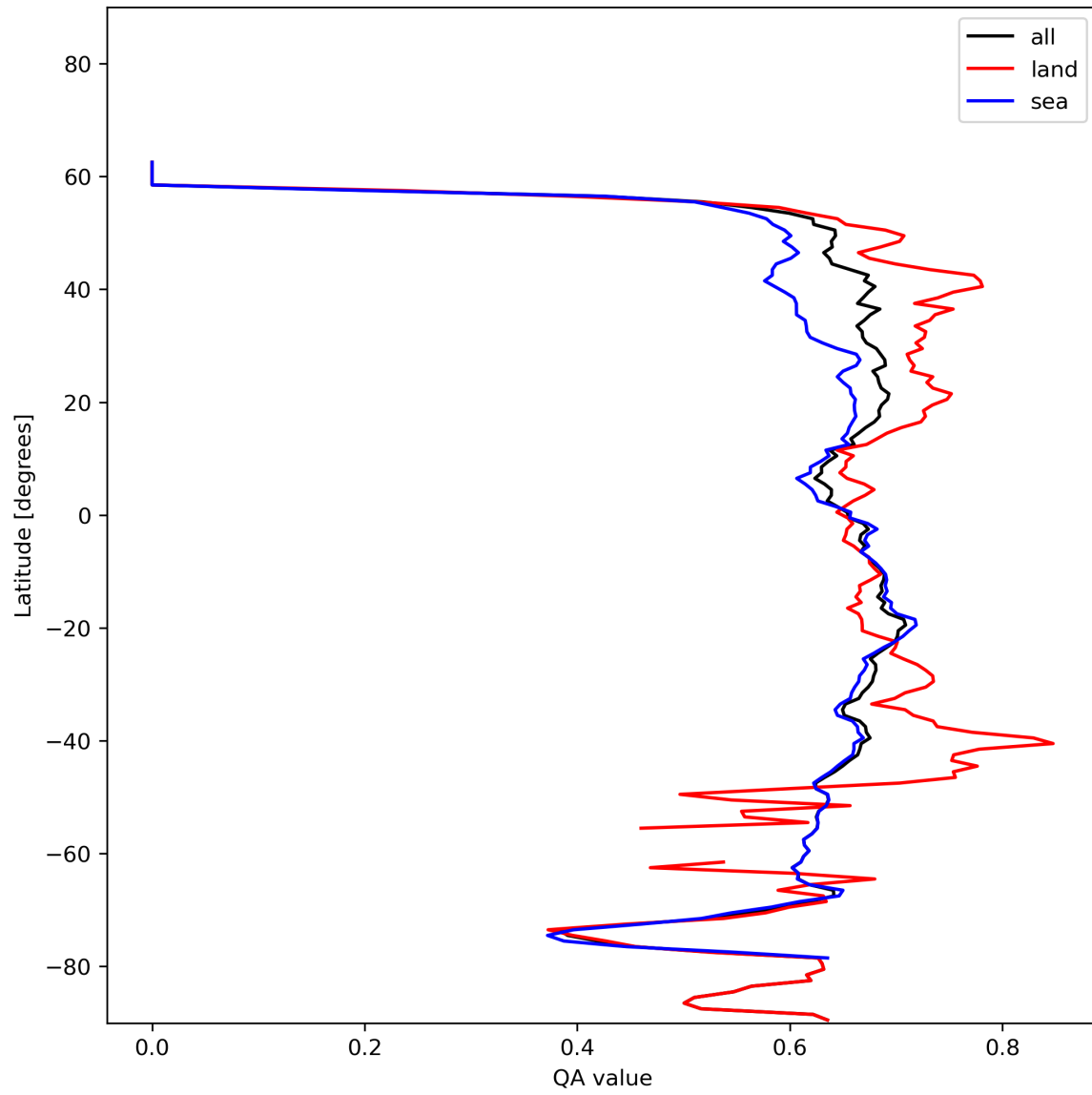
Figure 9: Zonal average of “QA value” for 2023-12-02 to 2023-12-04.
