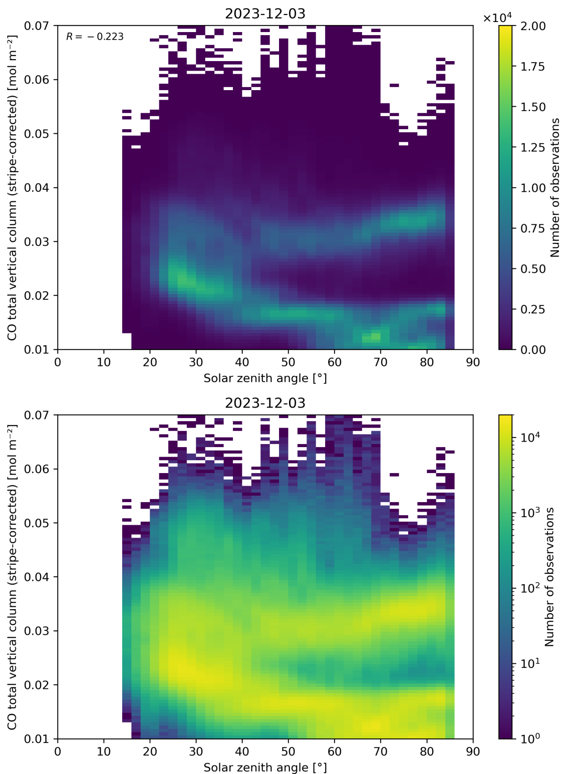
Figure 62: Scatter density plot of “Solar zenith angle” against “CO total vertical column (stripe-corrected)” for 2023-12-02 to 2023-12-04.
