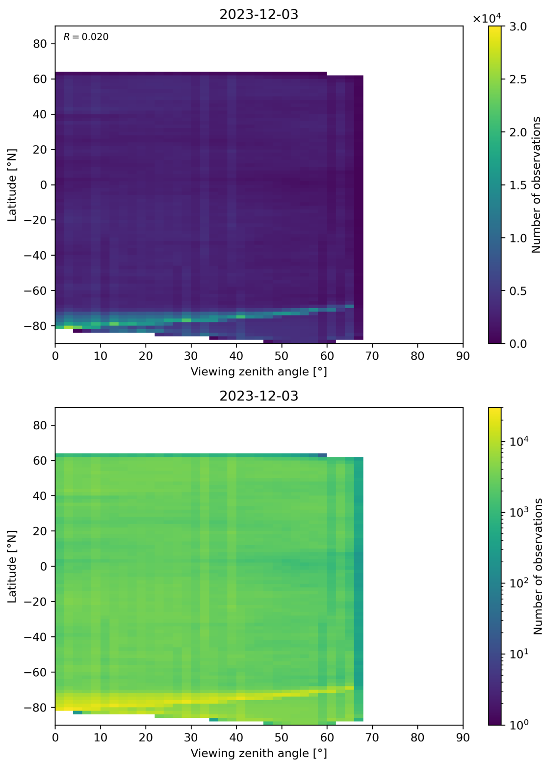
Figure 74: Scatter density plot of “Viewing zenith angle” against “Latitude” for 2023-12-02 to 2023-12-04.
