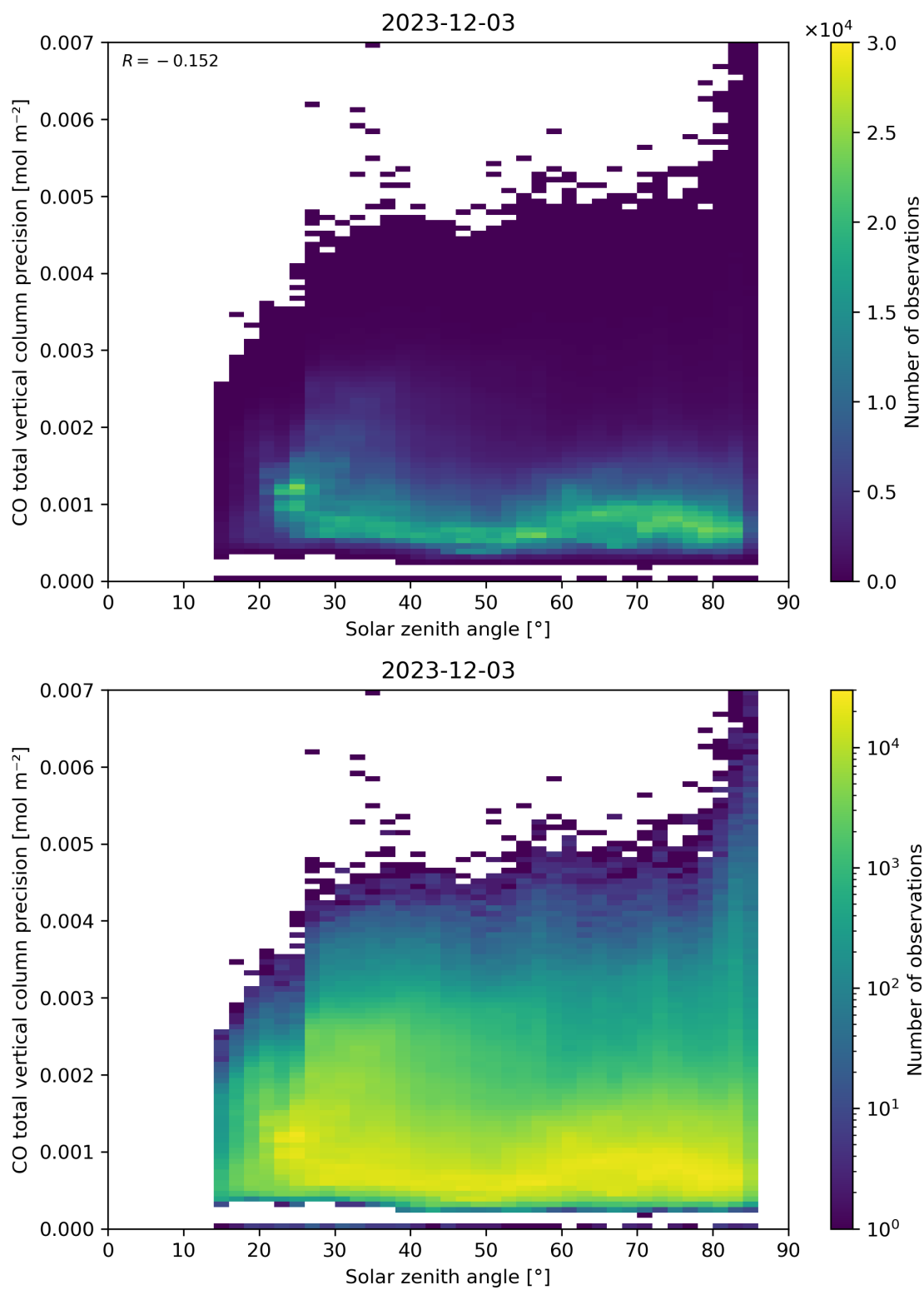
Figure 63: Scatter density plot of “Solar zenith angle” against “CO total vertical column precision” for 2023-12-02 to 2023-12-04.
