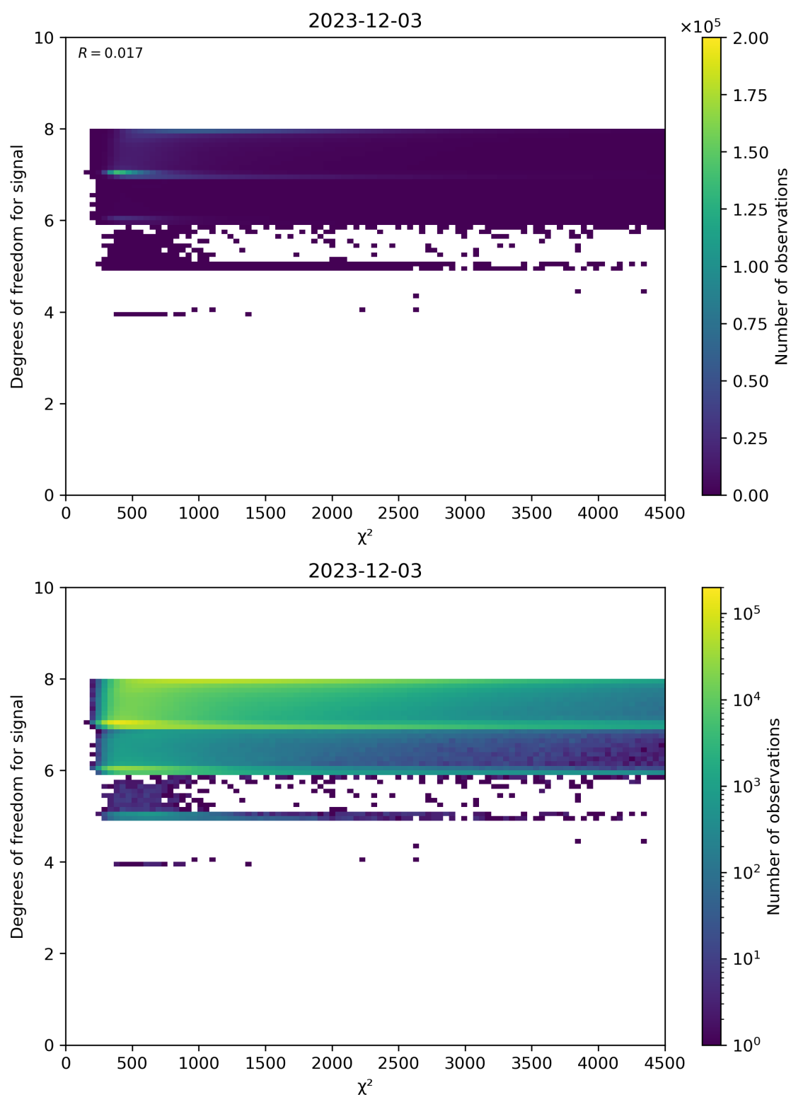
Figure 48: Scatter density plot of “ \chi^2 ” against “Degrees of freedom for signal” for 2023-12-02 to 2023-12-04.
