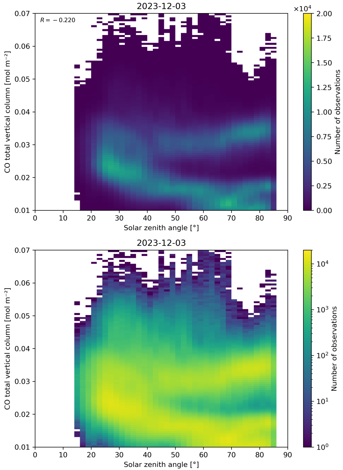
Figure 61: Scatter density plot of “Solar zenith angle” against “CO total vertical column” for 2023-12-02 to 2023-12-04.
