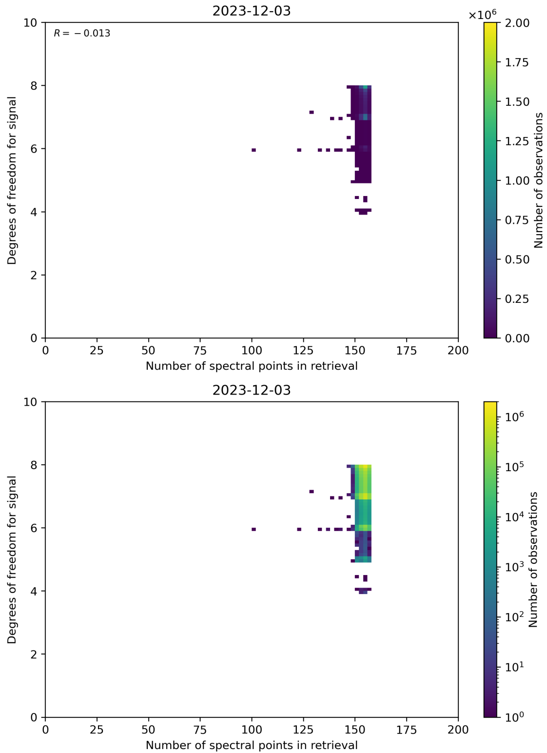
Figure 59: Scatter density plot of “Number of spectral points in retrieval” against “Degrees of freedom for signal” for 2023-12-02 to 2023-12-04.
