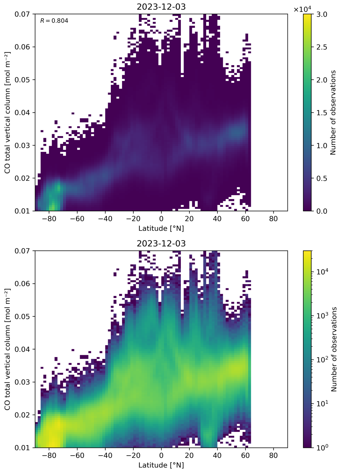
Figure 51: Scatter density plot of “Latitude” against “CO total vertical column” for 2023-12-02 to 2023-12-04.
