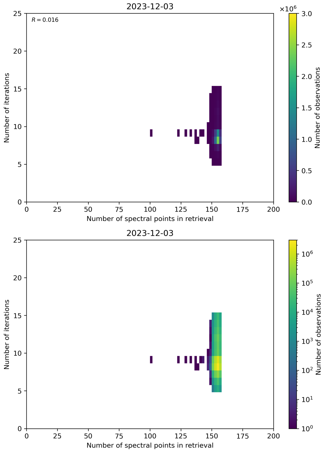
Figure 60: Scatter density plot of “Number of spectral points in retrieval” against “Number of iterations” for 2023-12-02 to 2023-12-04.
