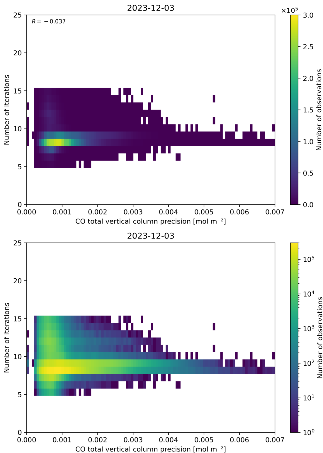
Figure 46: Scatter density plot of “CO total vertical column precision” against “Number of iterations” for 2023-12-02 to 2023-12-04.
