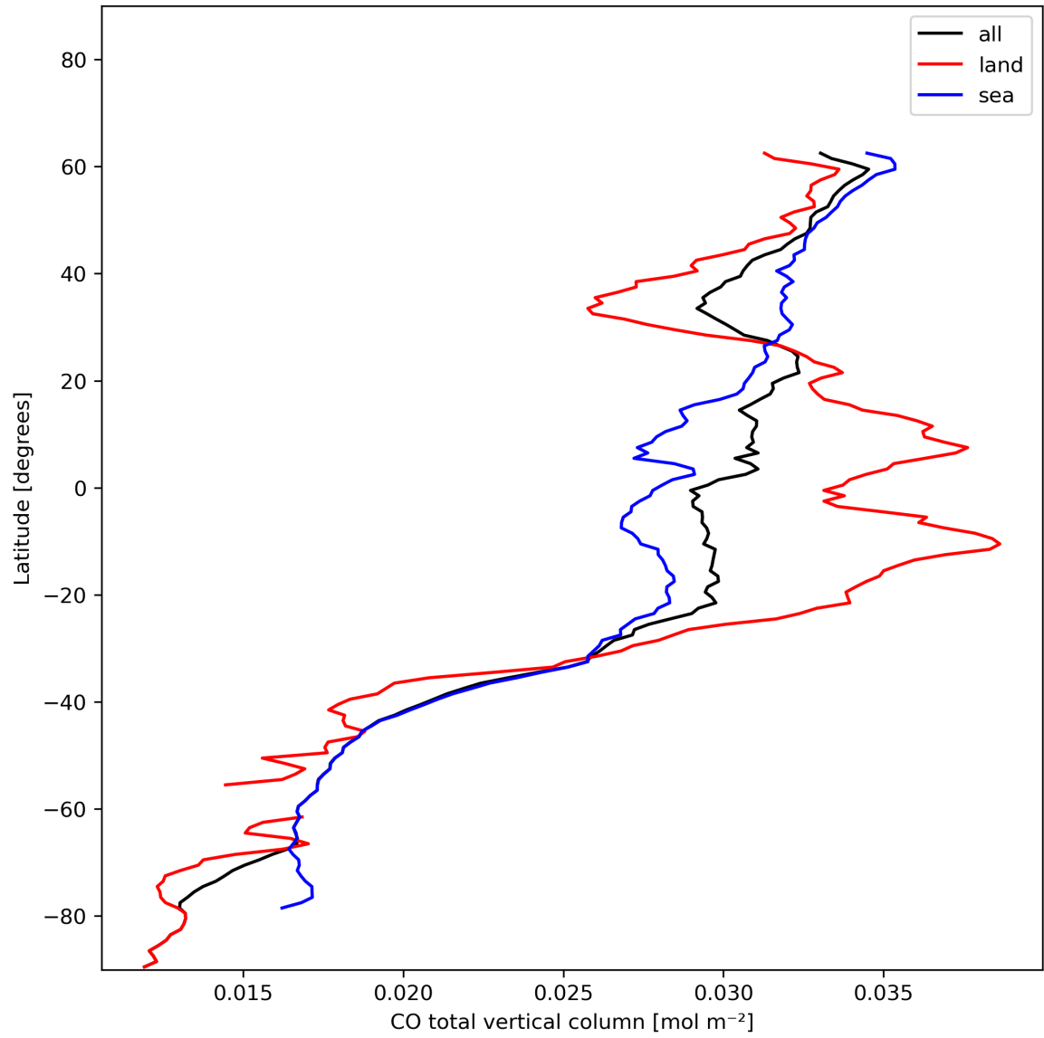
Figure 10: Zonal average of “CO total vertical column” for 2023-12-02 to 2023-12-04.
