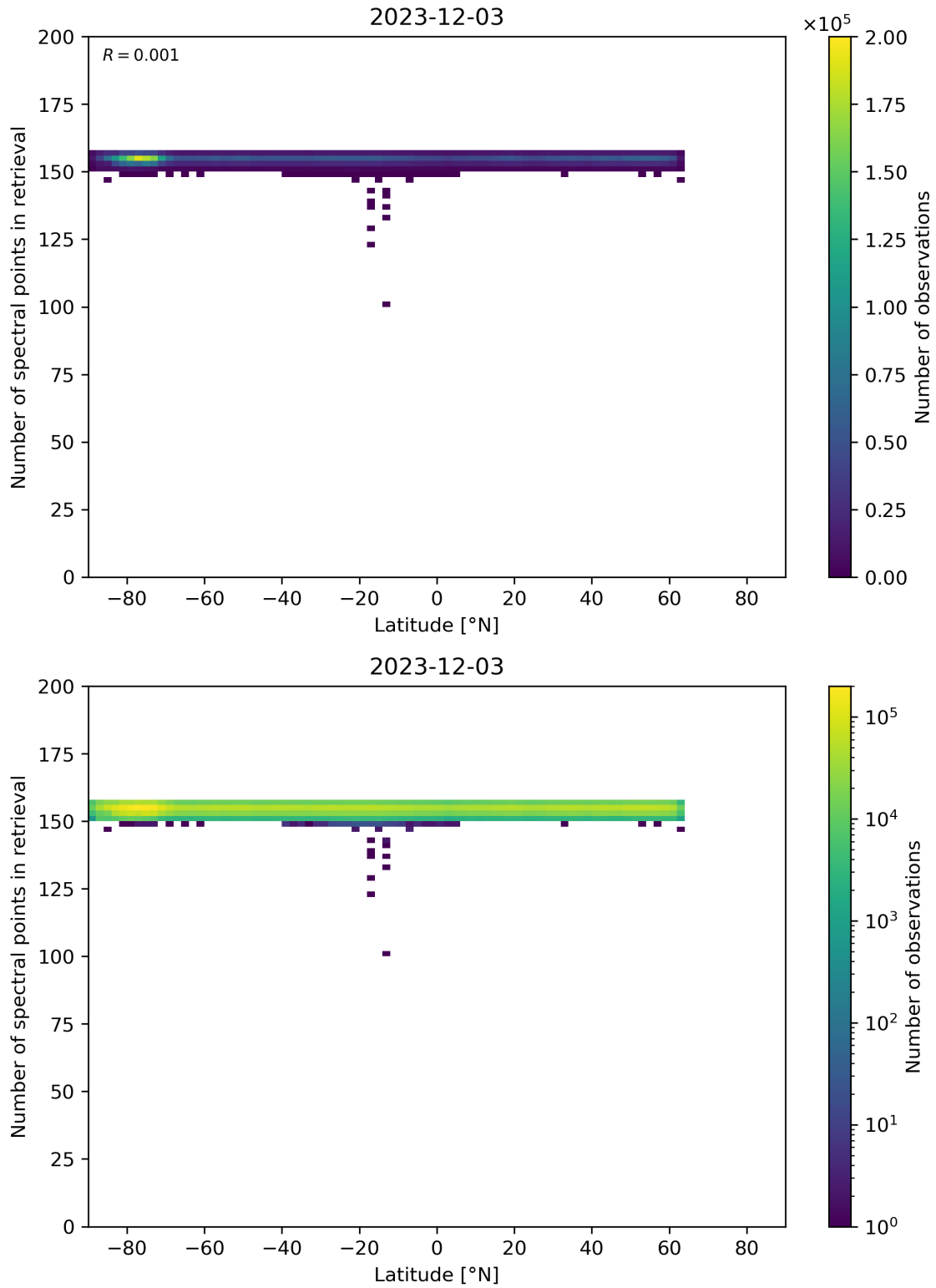
Figure 57: Scatter density plot of “Latitude” against “Number of spectral points in retrieval” for 2023-12-02 to 2023-12-04.
