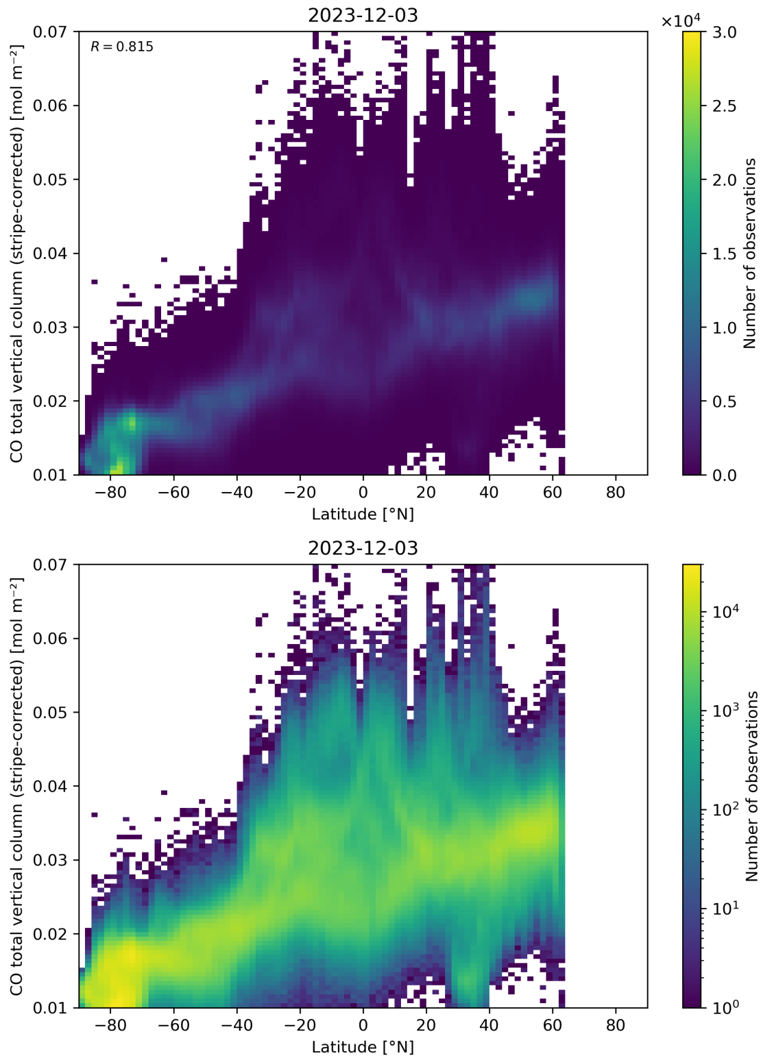
Figure 52: Scatter density plot of “Latitude” against “CO total vertical column (stripe-corrected)” for 2023-12-02 to 2023-12-04.
