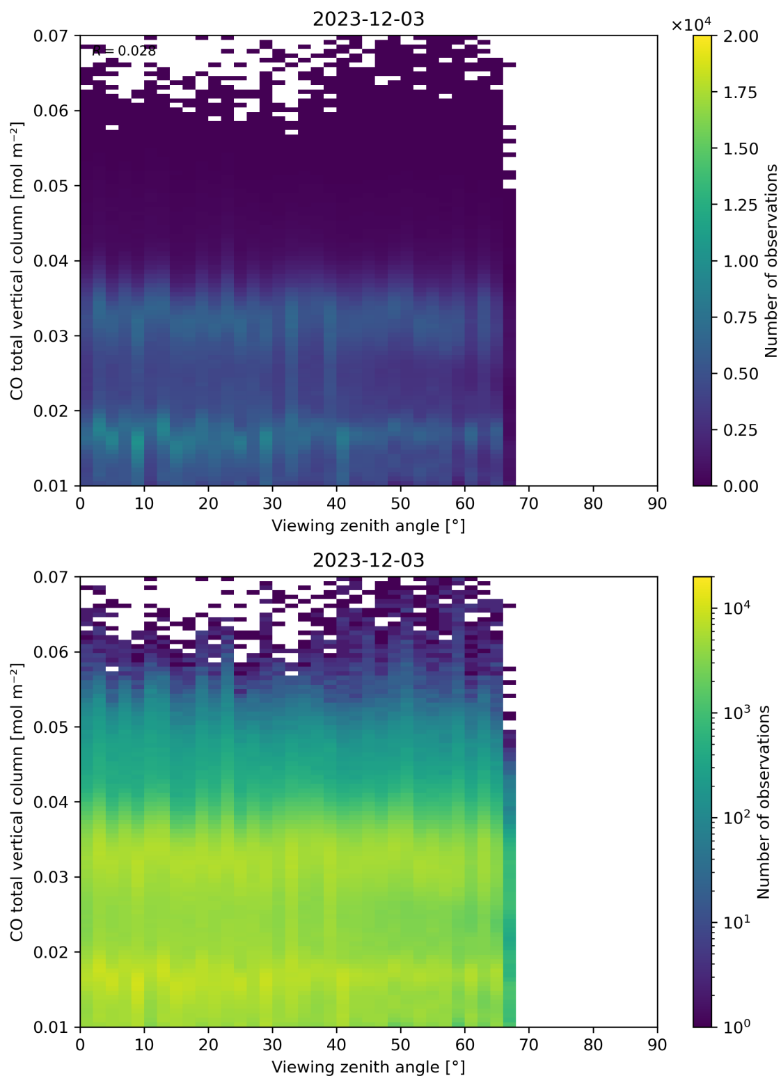
Figure 69: Scatter density plot of “Viewing zenith angle” against “CO total vertical column” for 2023-12-02 to 2023-12-04.
