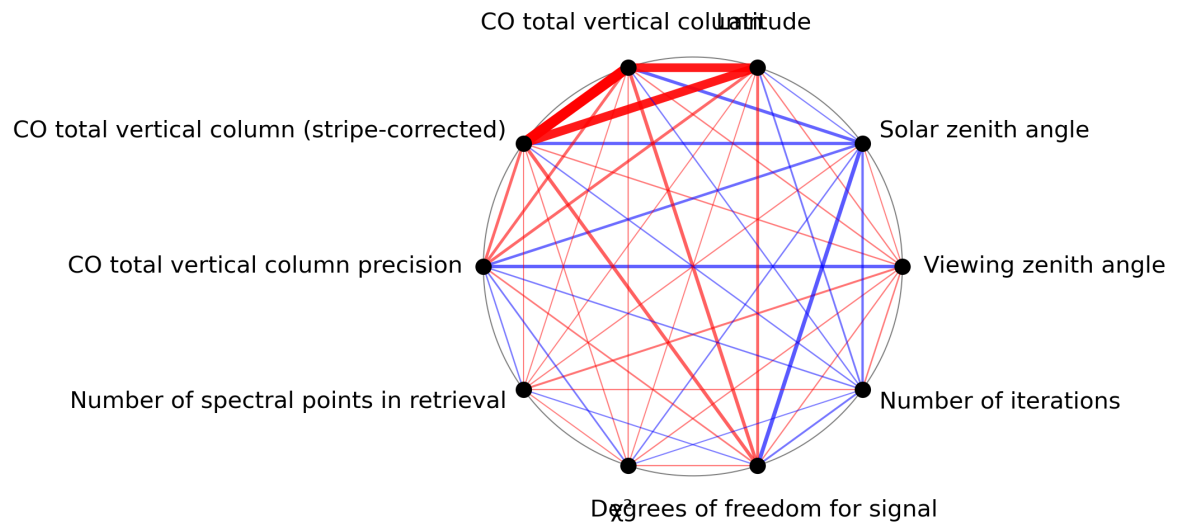
Figure 1: Map of correlation graph for 2023-12-02 to 2023-12-04.
