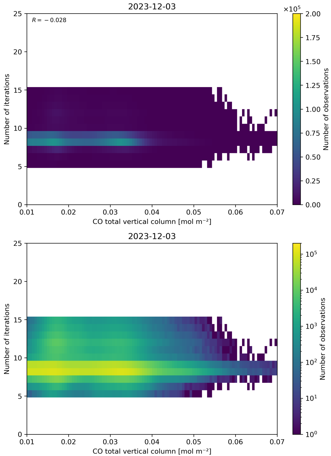
Figure 42: Scatter density plot of “CO total vertical column” against “Number of iterations” for 2023-12-02 to 2023-12-04.
