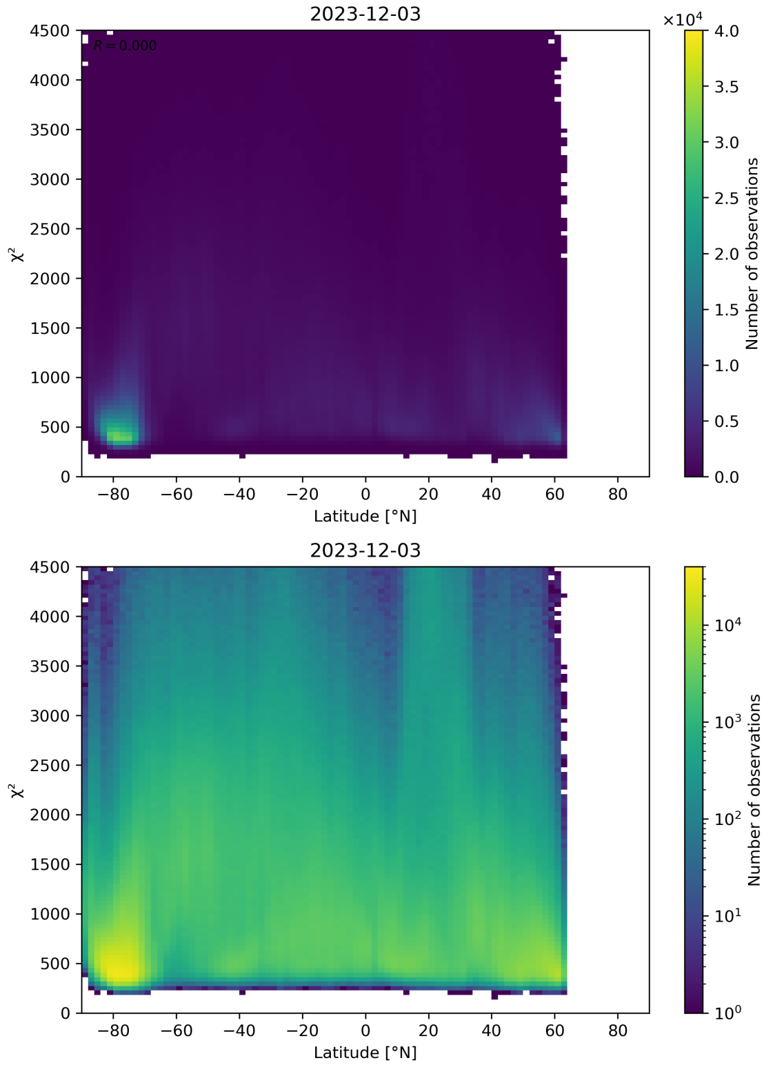
Figure 54: Scatter density plot of “Latitude” against “ \chi^2 ” for 2023-12-02 to 2023-12-04.
