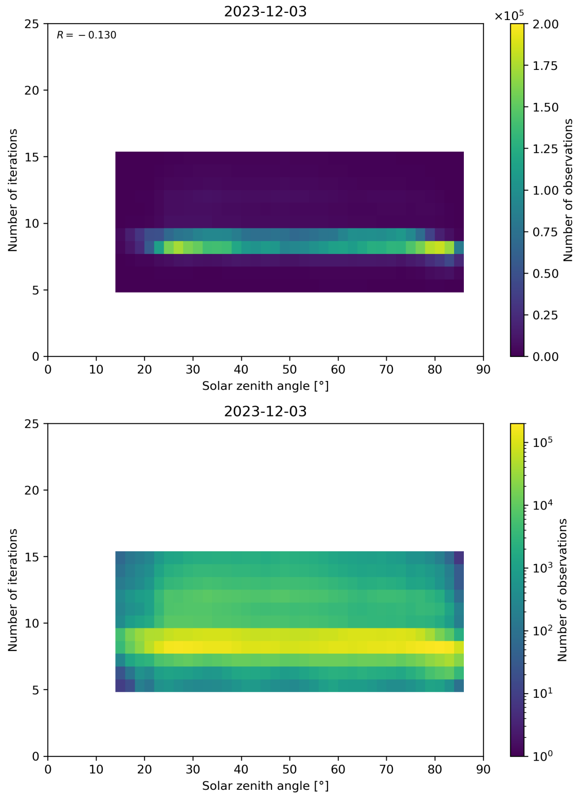
Figure 67: Scatter density plot of “Solar zenith angle” against “Number of iterations” for 2023-12-02 to 2023-12-04.
