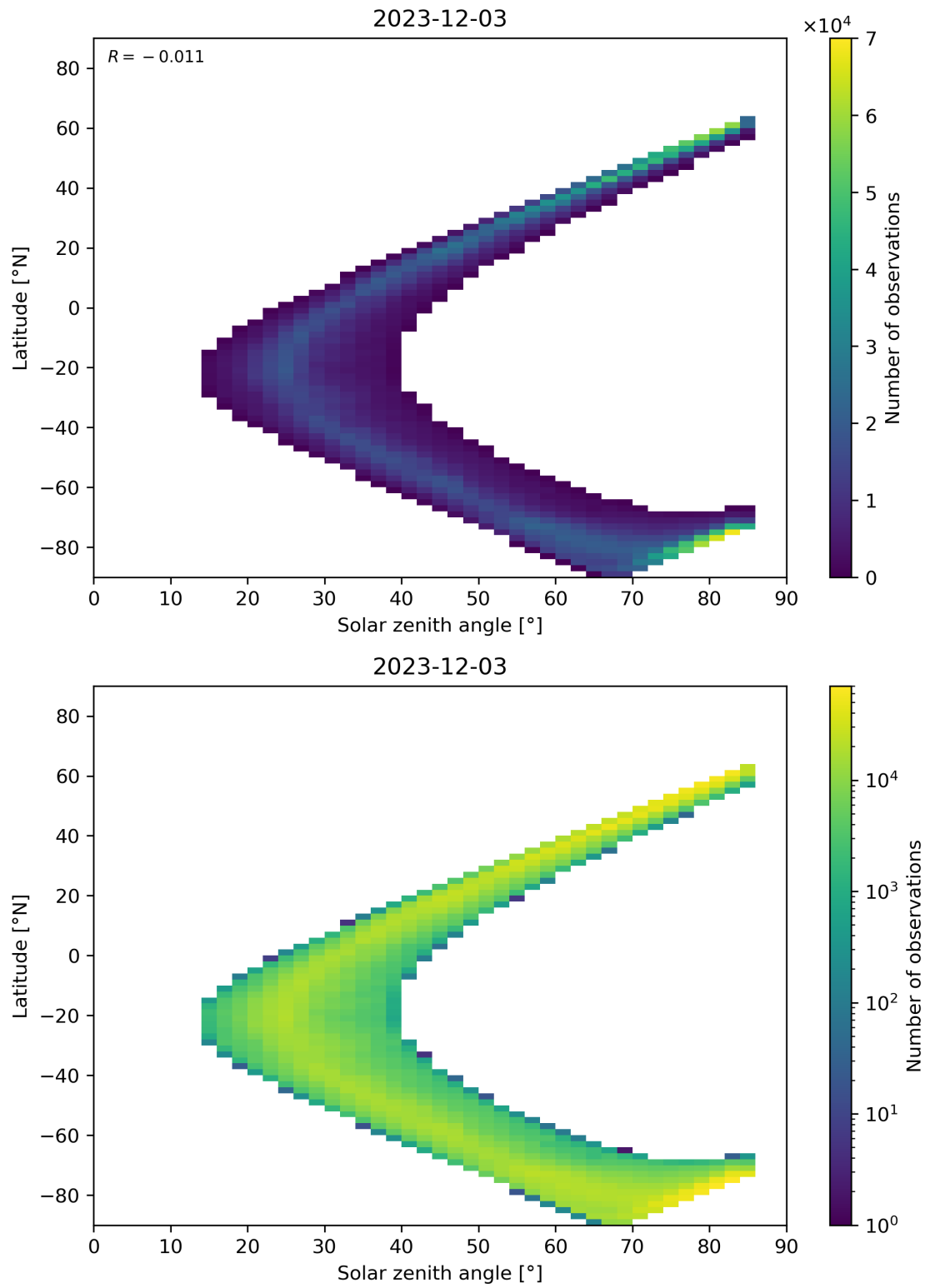
Figure 66: Scatter density plot of “Solar zenith angle” against “Latitude” for 2023-12-02 to 2023-12-04.
