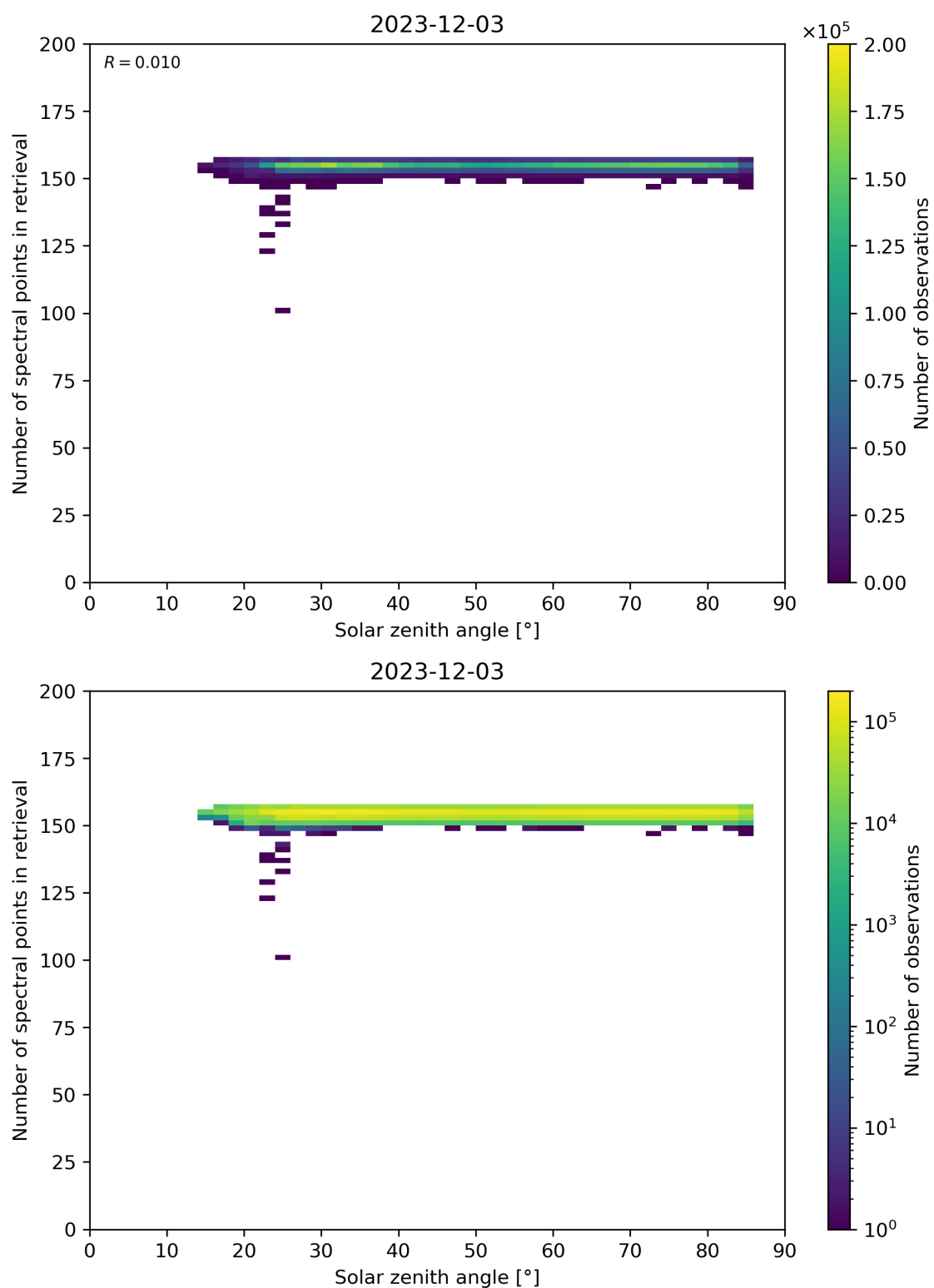
Figure 68: Scatter density plot of “Solar zenith angle” against “Number of spectral points in retrieval” for 2023-12-02 to 2023-12-04.
