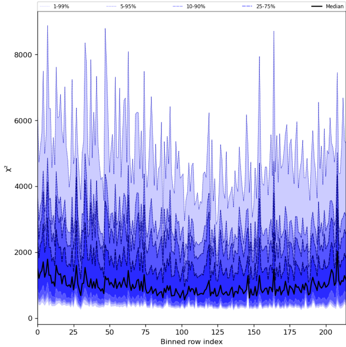
Figure 30: Along track statistics of “ \chi^2 ” for 2023-12-02 to 2023-12-04
