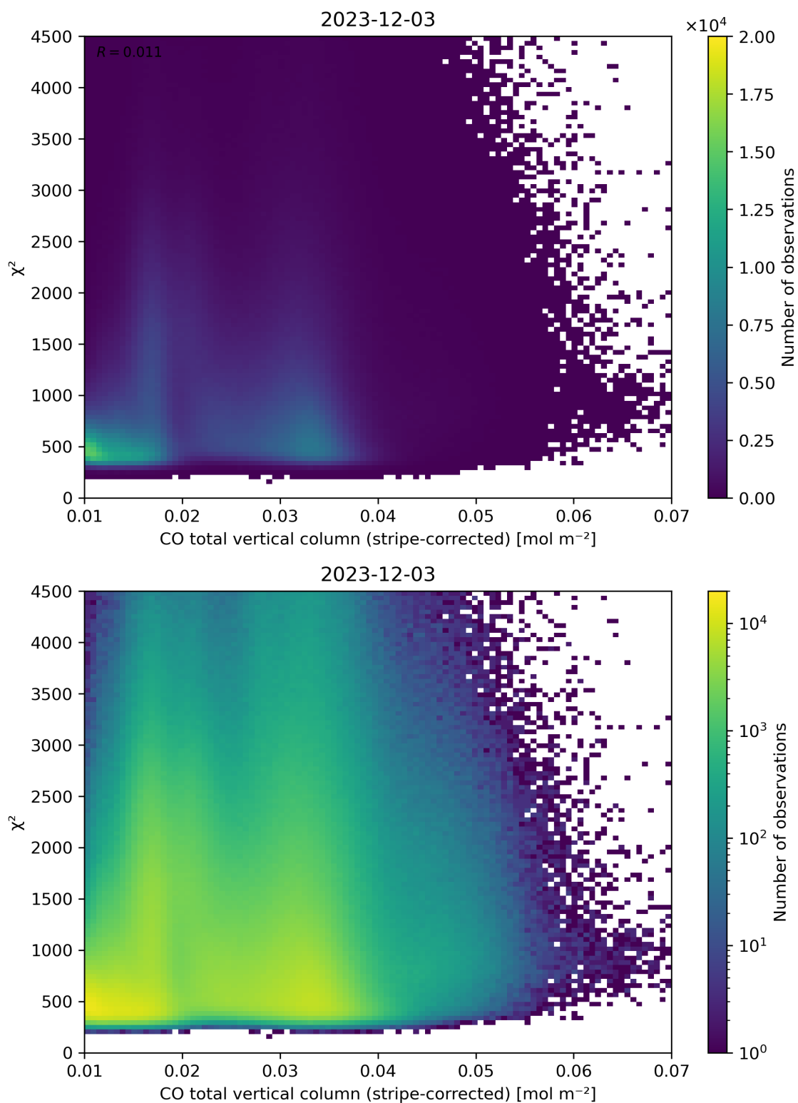
Figure 37: Scatter density plot of “CO total vertical column (stripe-corrected)” against “ \chi^2 ” for 2023-12-02 to 2023-12-04.
