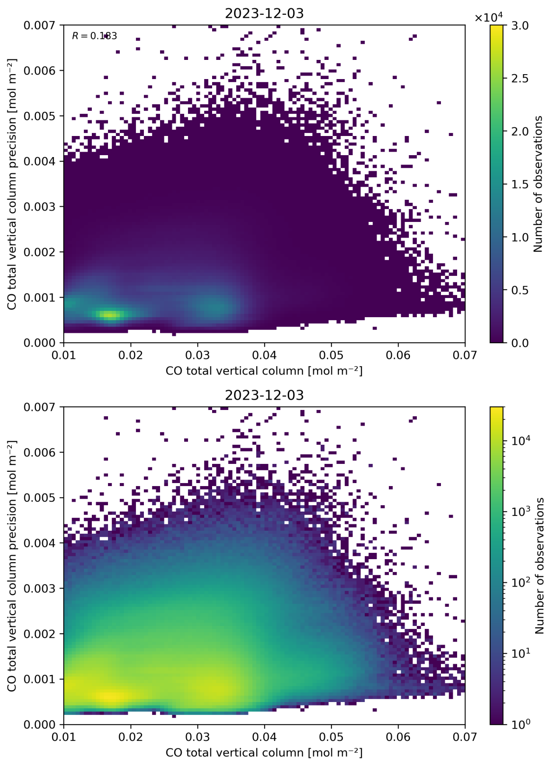
Figure 34: Scatter density plot of “CO total vertical column” against “CO total vertical column precision” for 2023-12-02 to 2023-12-04.
