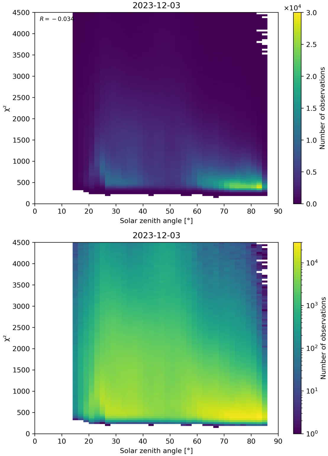
Figure 64: Scatter density plot of “Solar zenith angle” against “ \chi^2 ” for 2023-12-02 to 2023-12-04.
