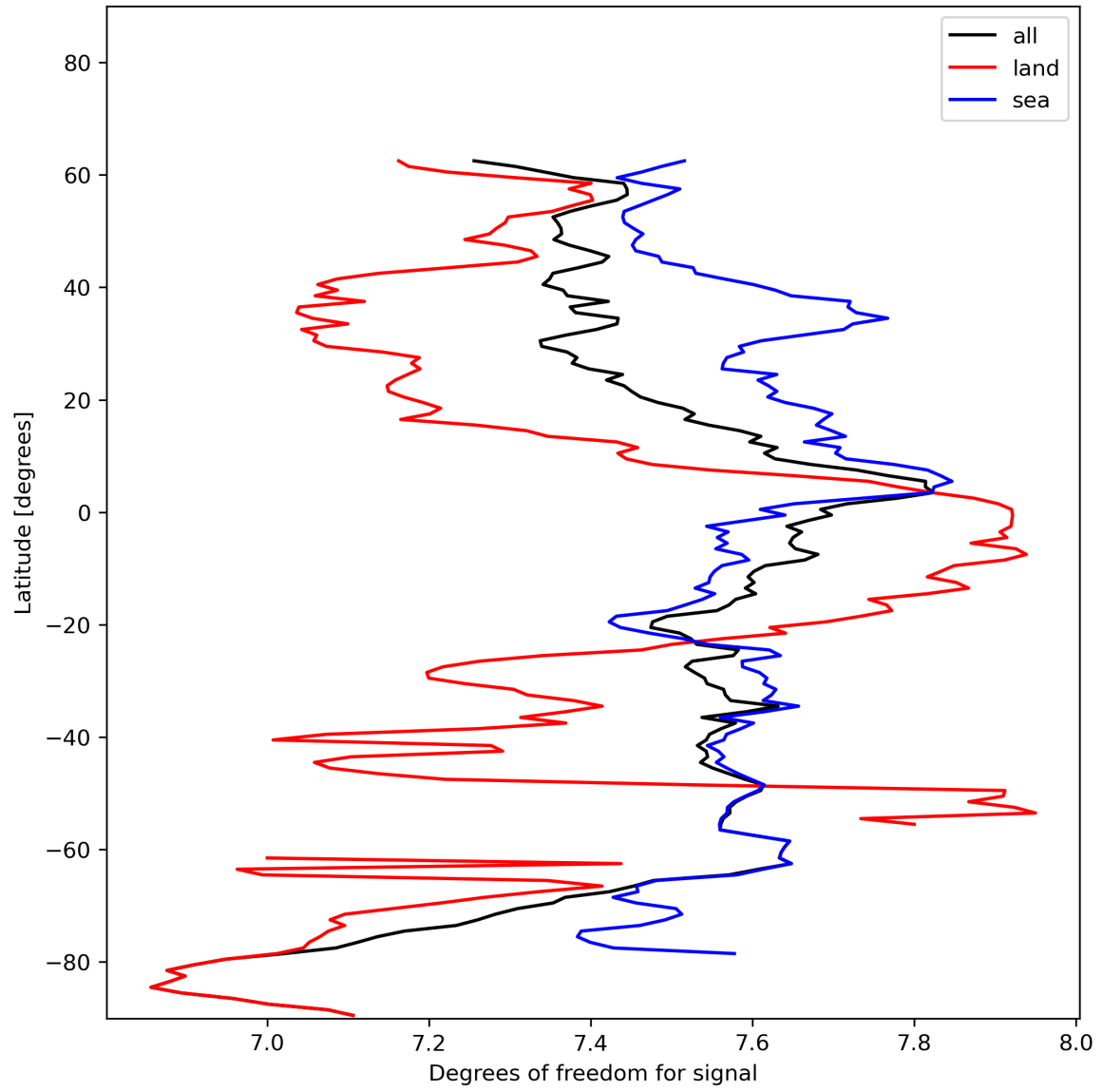
Figure 15: Zonal average of “Degrees of freedom for signal” for 2023-12-02 to 2023-12-04.
