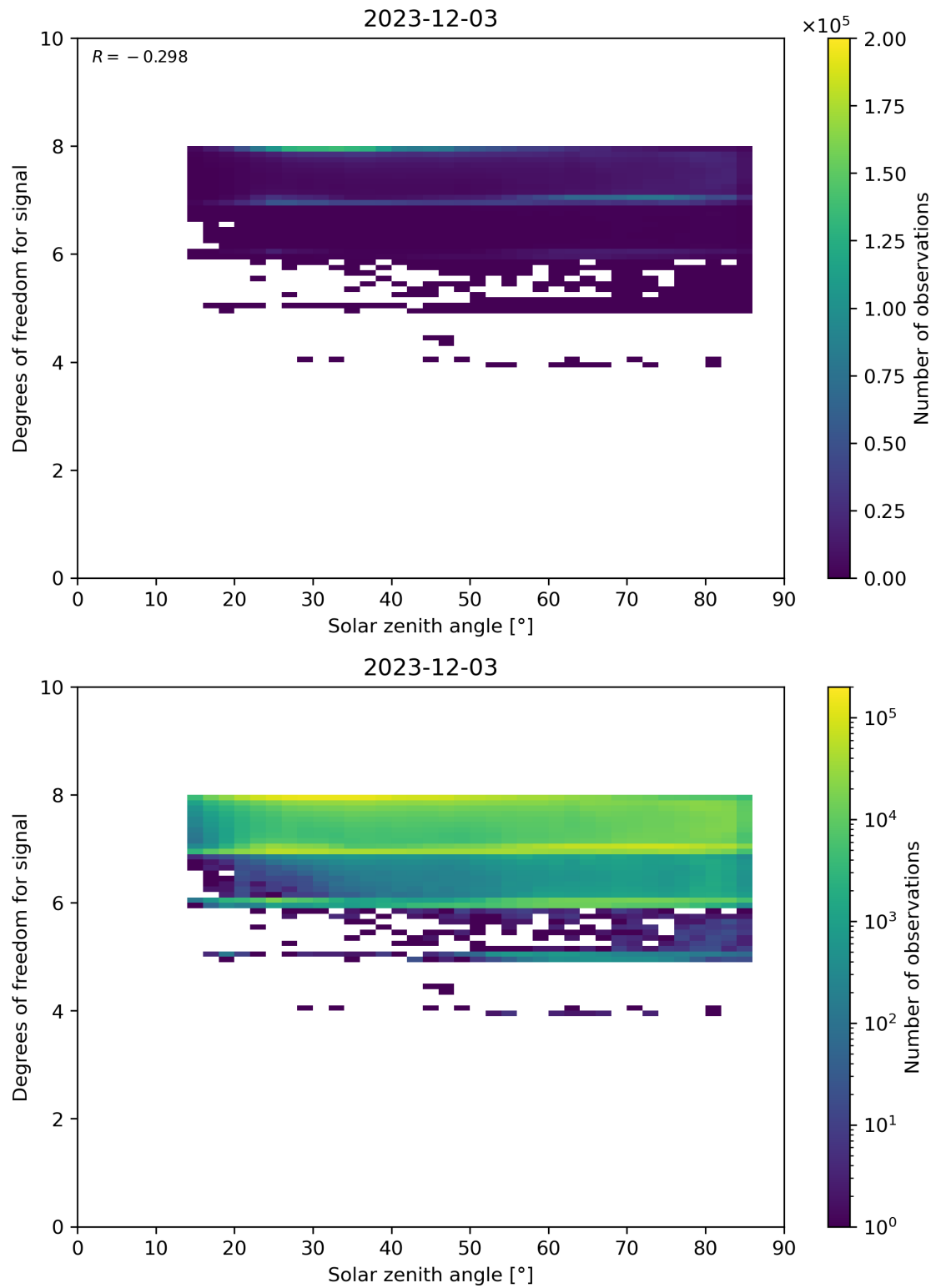
Figure 65: Scatter density plot of “Solar zenith angle” against “Degrees of freedom for signal” for 2023-12-02 to 2023-12-04.
