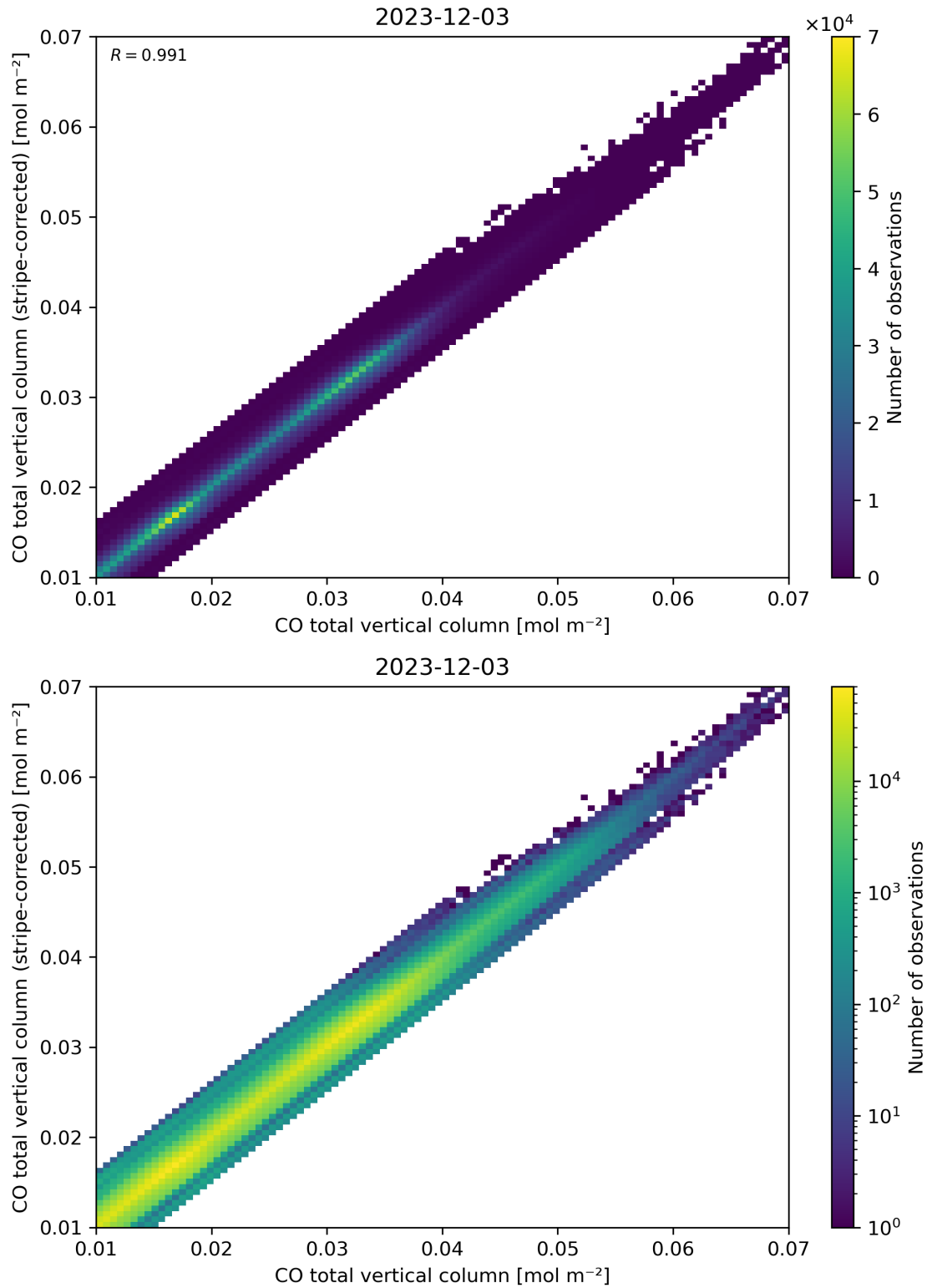
Figure 33: Scatter density plot of “CO total vertical column” against “CO total vertical column (stripe-corrected)” for 2023-12-02 to 2023-12-04.
