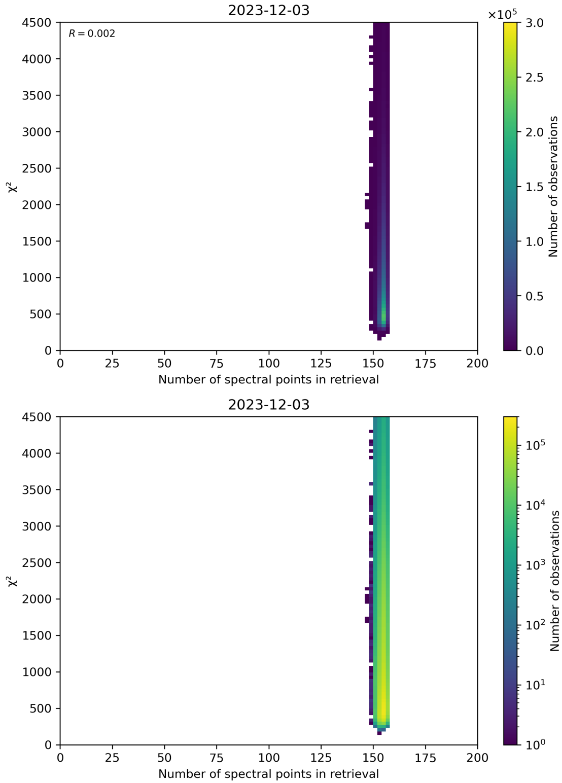
Figure 58: Scatter density plot of “Number of spectral points in retrieval” against “ \chi^2 ” for 2023-12-02 to 2023-12-04.
