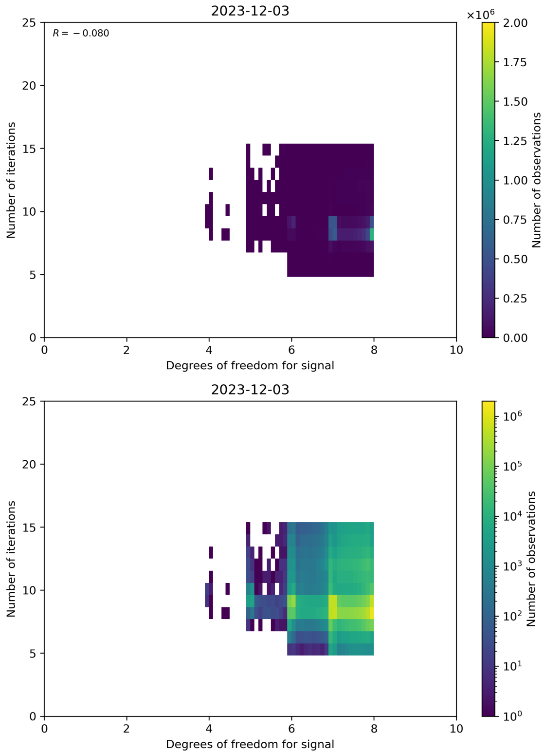
Figure 50: Scatter density plot of “Degrees of freedom for signal” against “Number of iterations” for 2023-12-02 to 2023-12-04.
