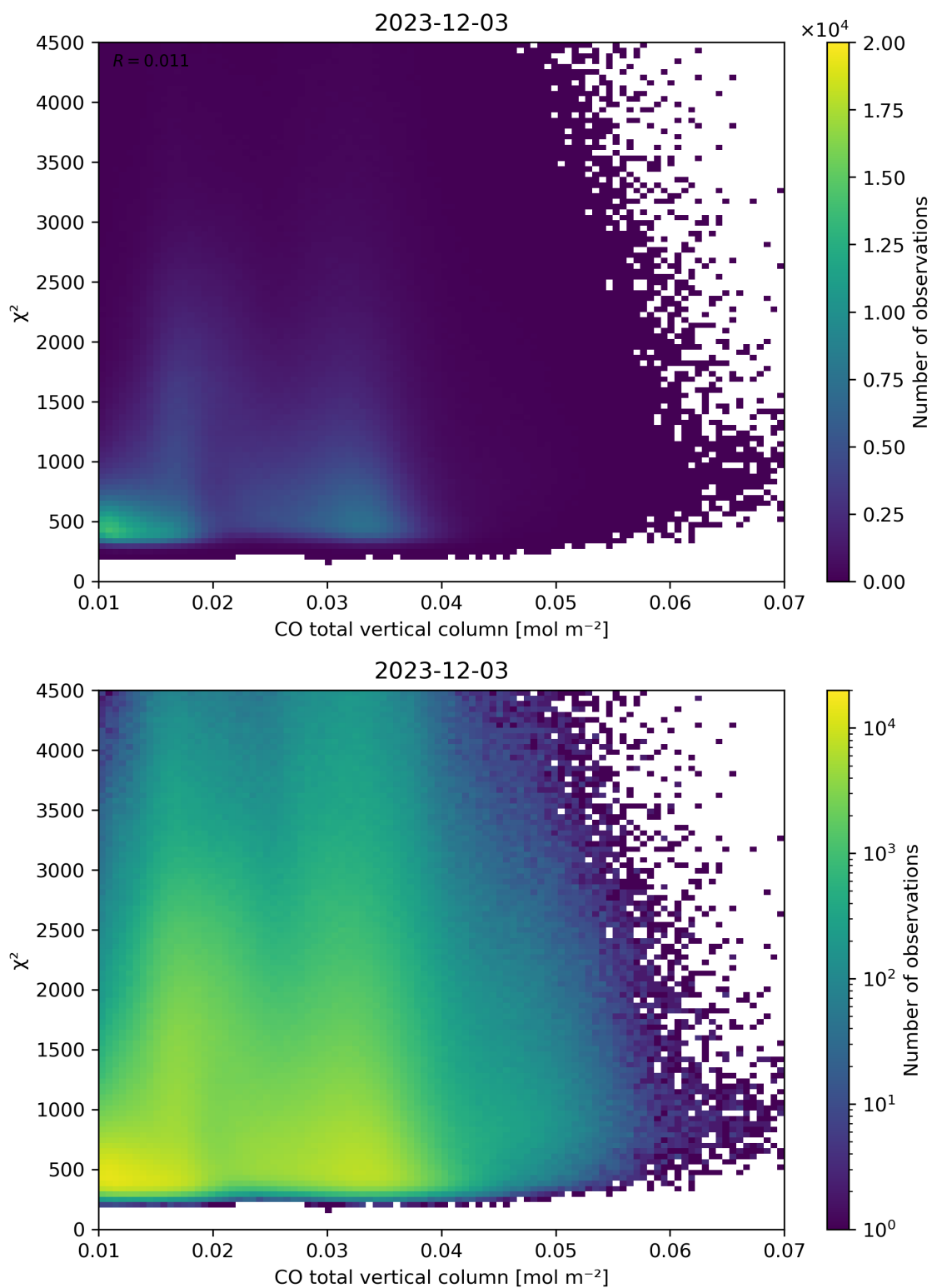
Figure 35: Scatter density plot of “CO total vertical column” against “ \chi^2 ” for 2023-12-02 to 2023-12-04.
