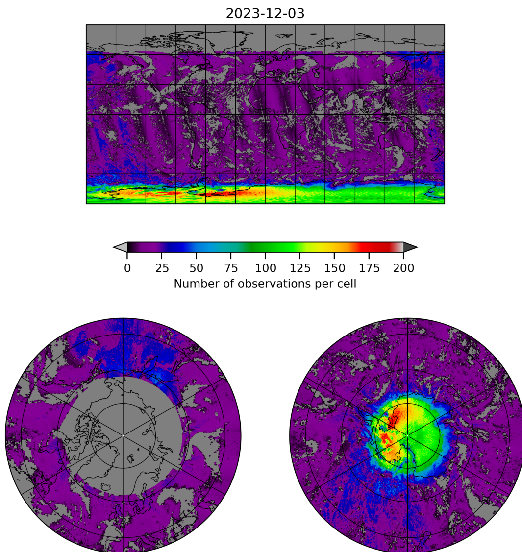
Figure 8: Map of the number of observations for 2023-12-02 to 2023-12-04
