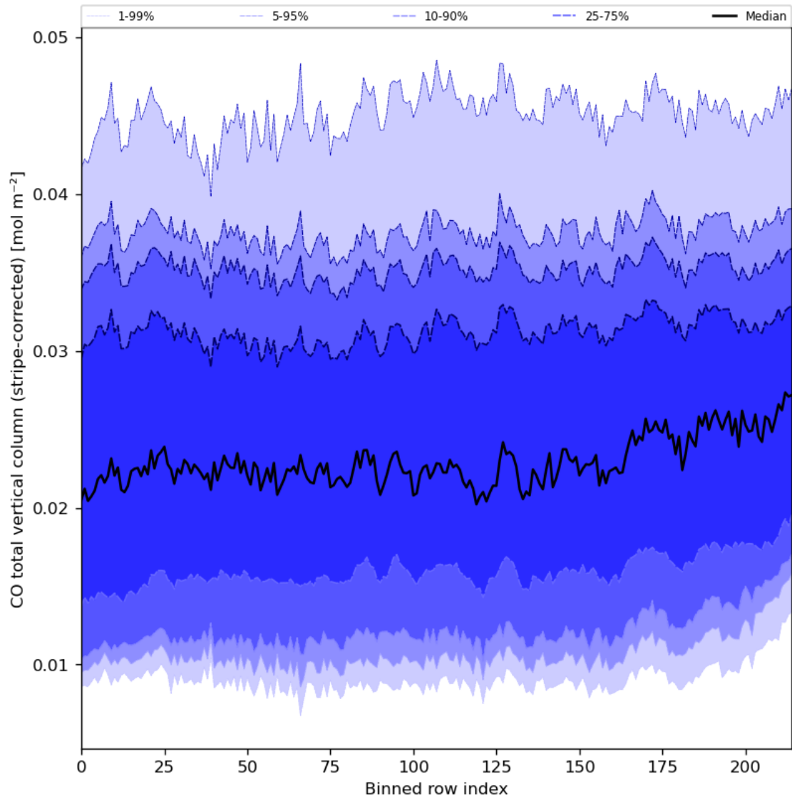
Figure 27: Along track statistics of “CO total vertical column (stripe-corrected)” for 2023-12-02 to 2023-12-04
