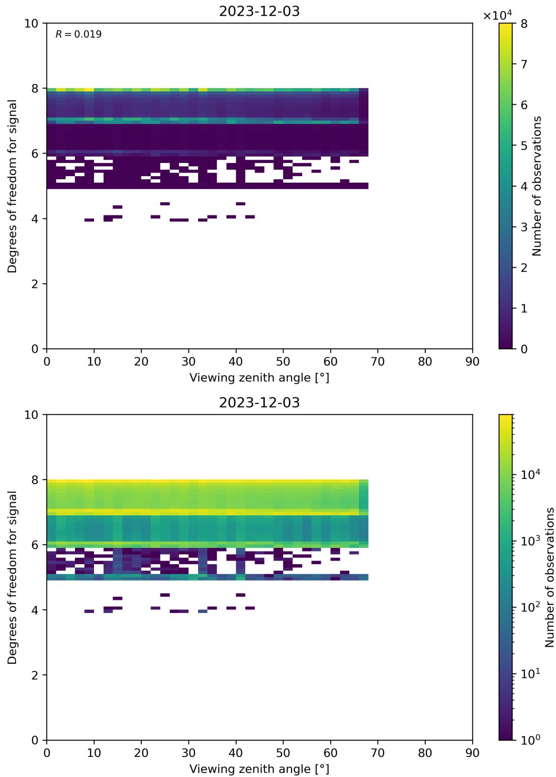
Figure 73: Scatter density plot of “Viewing zenith angle” against “Degrees of freedom for signal” for 2023-12-02 to 2023-12-04.
