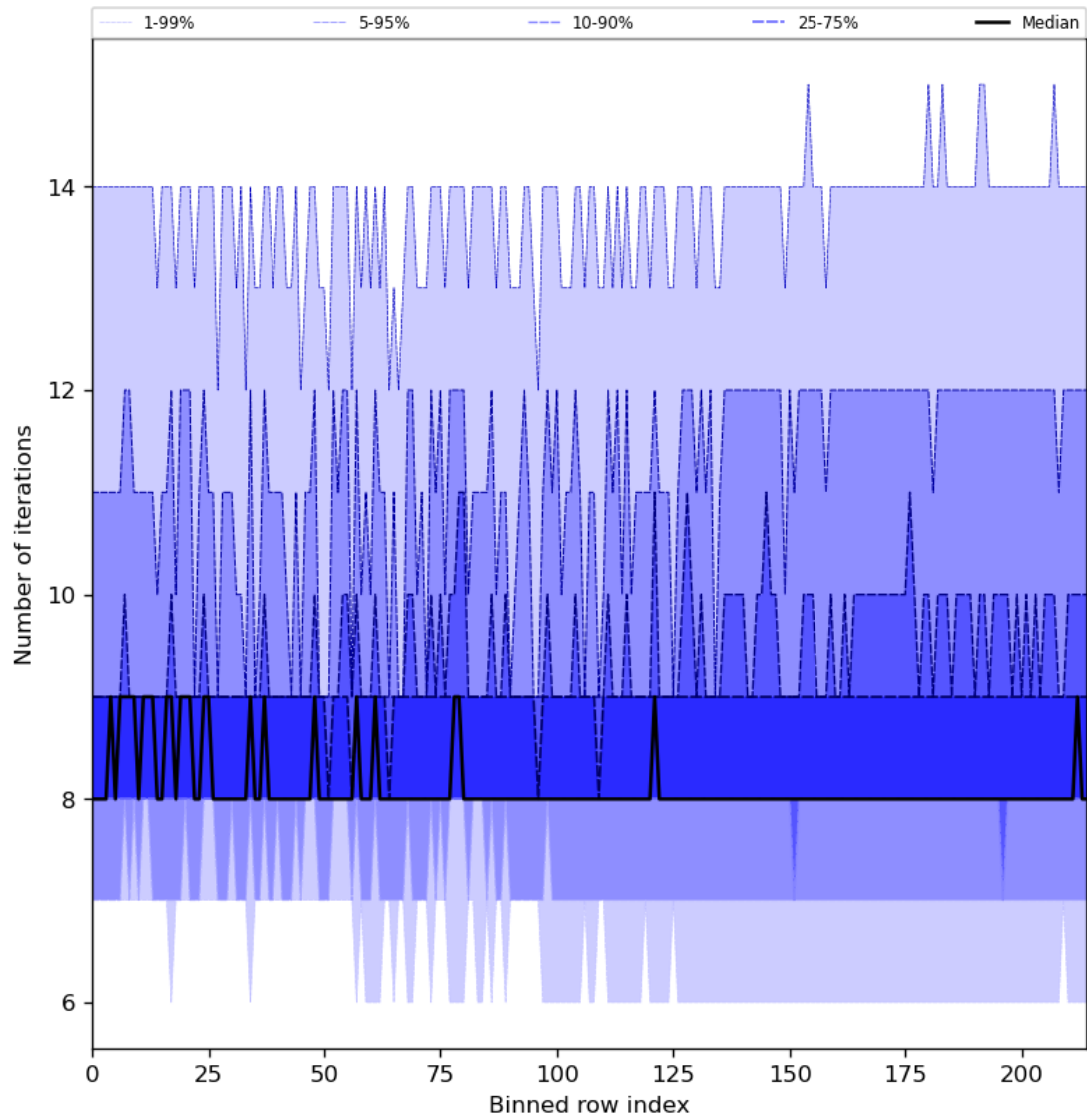
Figure 32: Along track statistics of “Number of iterations” for 2023-12-02 to 2023-12-04
