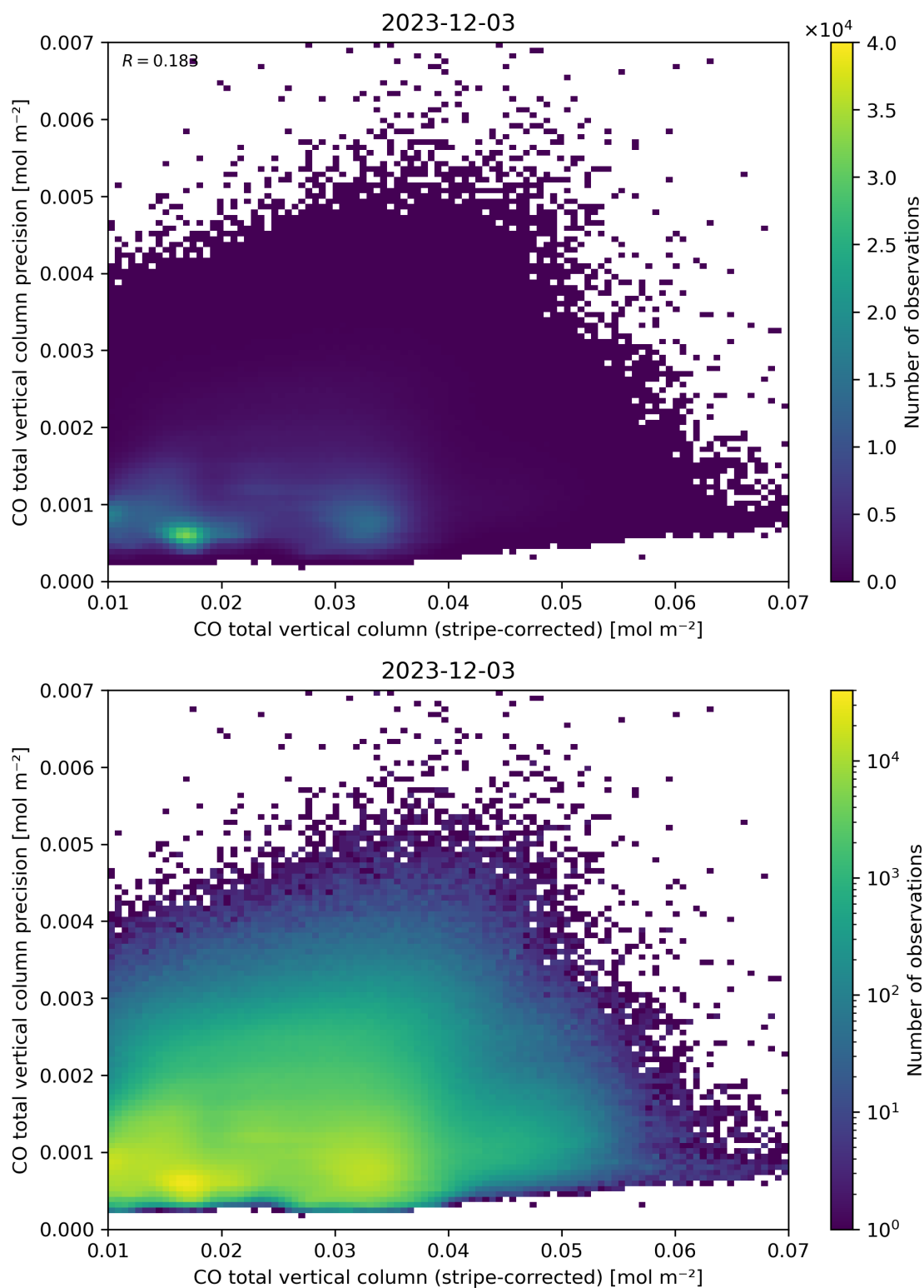
Figure 36: Scatter density plot of “CO total vertical column (stripe-corrected)” against “CO total vertical column precision” for 2023-12-02 to 2023-12-04.
