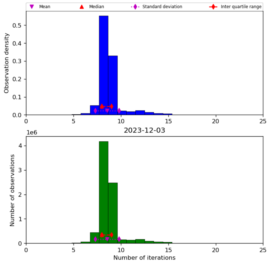
Figure 24: Histogram of “Number of iterations” for 2023-12-02 to 2023-12-04
