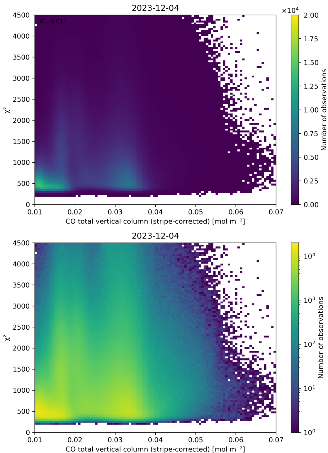
Figure 37: Scatter density plot of “CO total vertical column (stripe-corrected)” against “ \chi^2 ” for 2023-12-04 to 2023-12-05.
