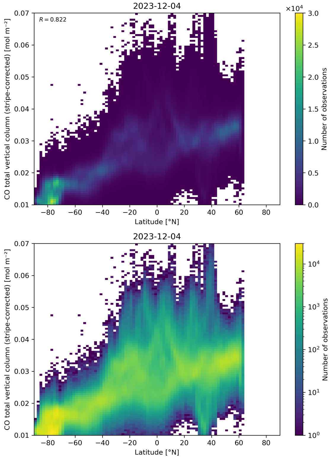
Figure 52: Scatter density plot of “Latitude” against “CO total vertical column (stripe-corrected)” for 2023-12-04 to 2023-12-05.
