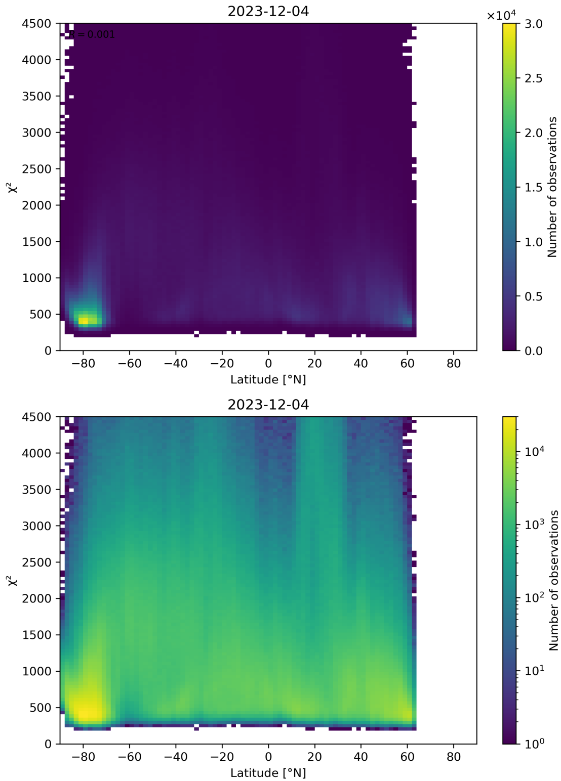
Figure 54: Scatter density plot of “Latitude” against “ \chi^2 ” for 2023-12-04 to 2023-12-05.
