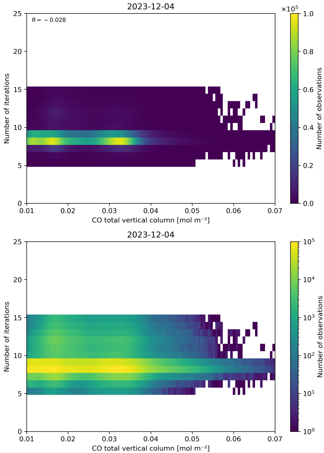
Figure 42: Scatter density plot of “CO total vertical column” against “Number of iterations” for 2023-12-04 to 2023-12-05.
