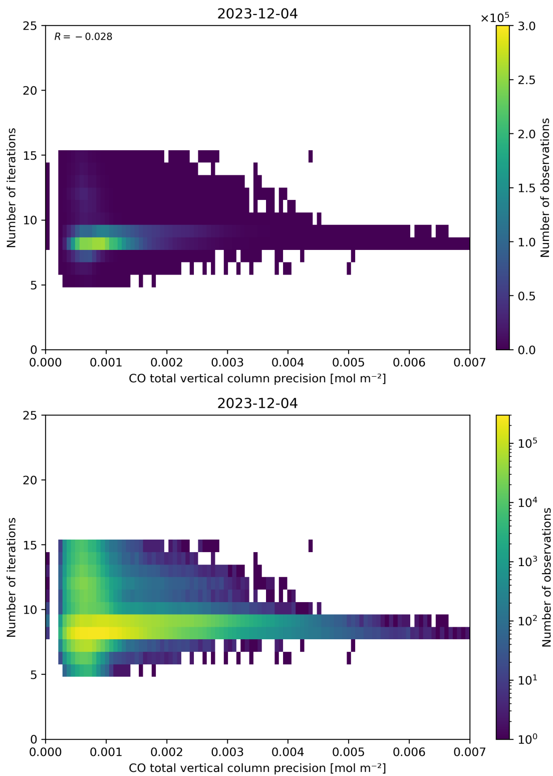
Figure 46: Scatter density plot of “CO total vertical column precision” against “Number of iterations” for 2023-12-04 to 2023-12-05.
