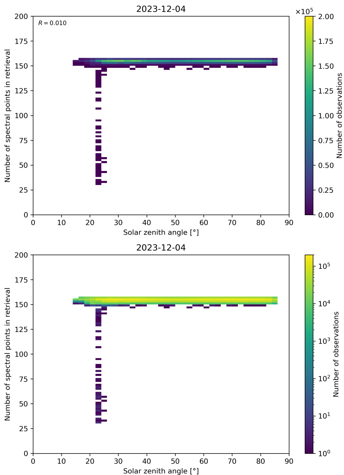
Figure 68: Scatter density plot of “Solar zenith angle” against “Number of spectral points in retrieval” for 2023-12-04 to 2023-12-05.
