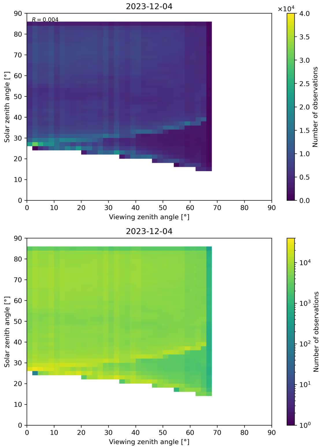
Figure 77: Scatter density plot of “Viewing zenith angle” against “Solar zenith angle” for 2023-12-04 to 2023-12-05.
