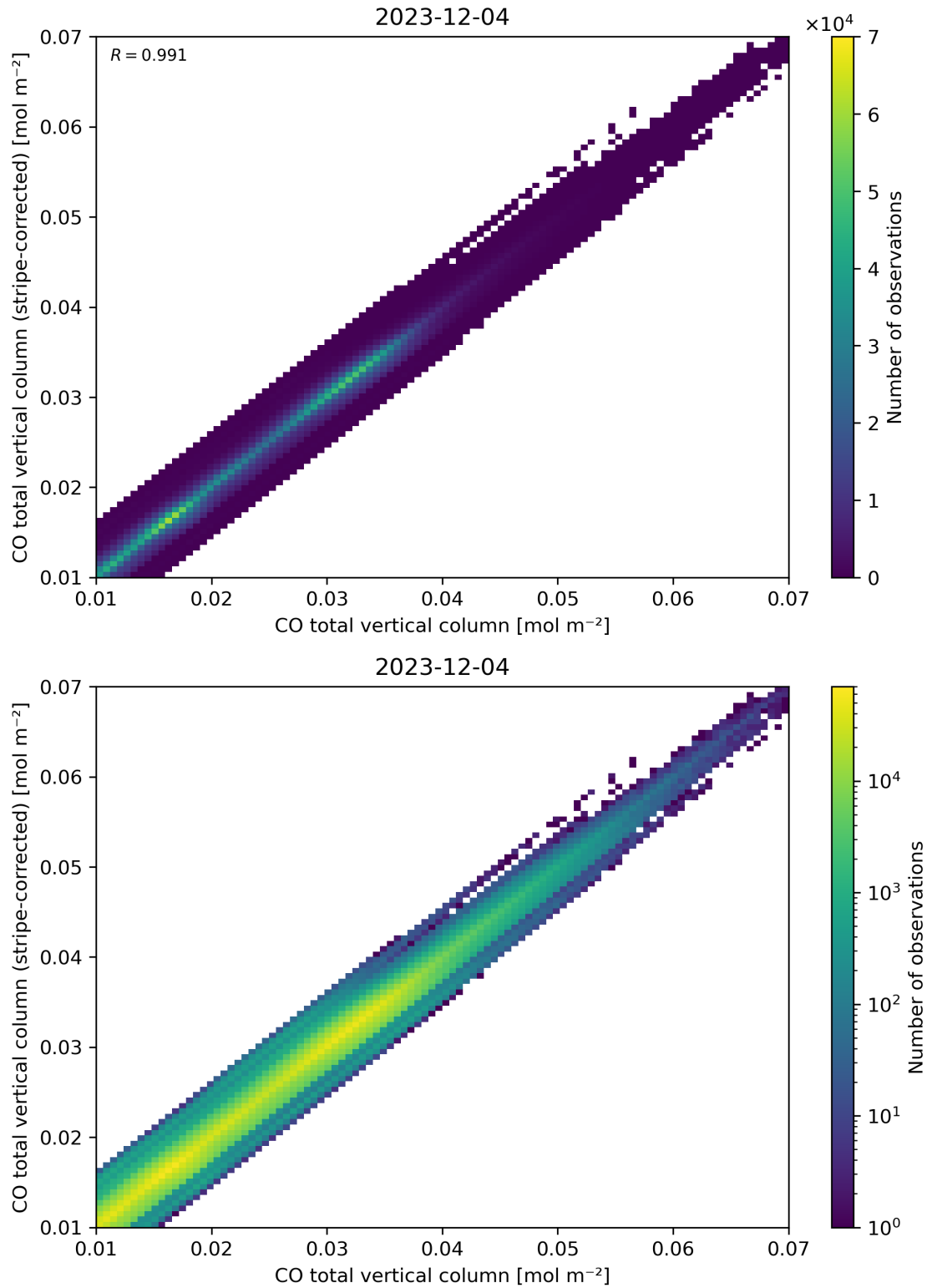
Figure 33: Scatter density plot of “CO total vertical column” against “CO total vertical column (stripe-corrected)” for 2023-12-04 to 2023-12-05.
