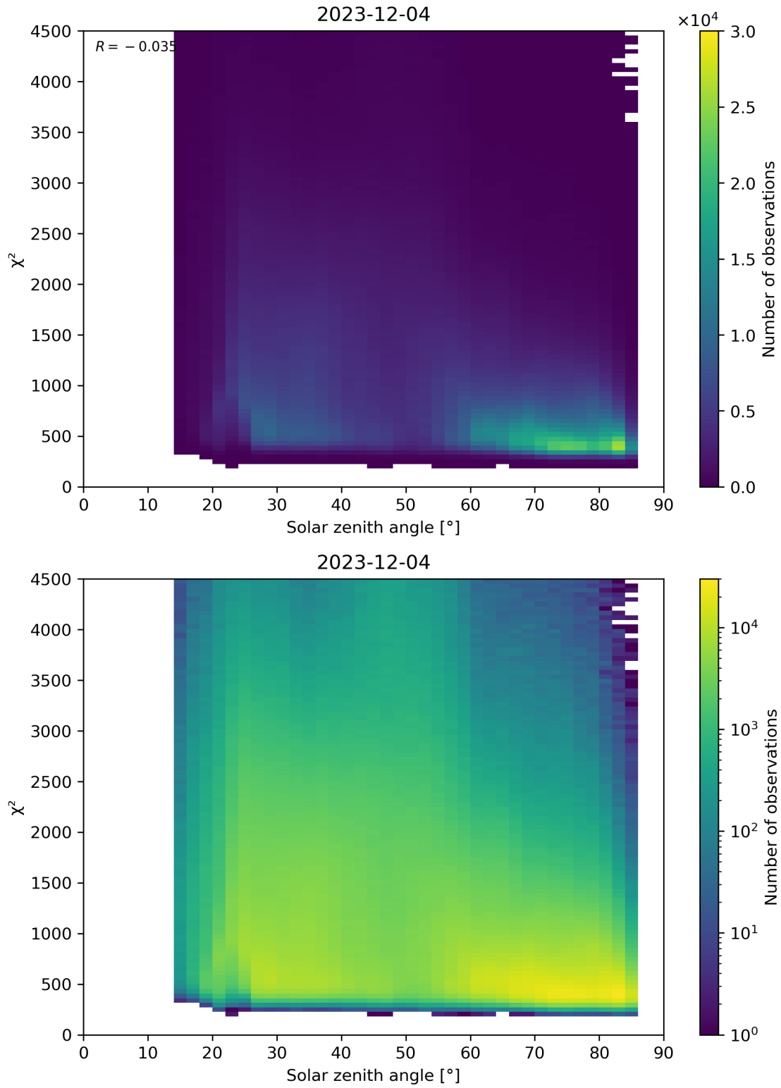
Figure 64: Scatter density plot of “Solar zenith angle” against “ \chi^2 ” for 2023-12-04 to 2023-12-05.
