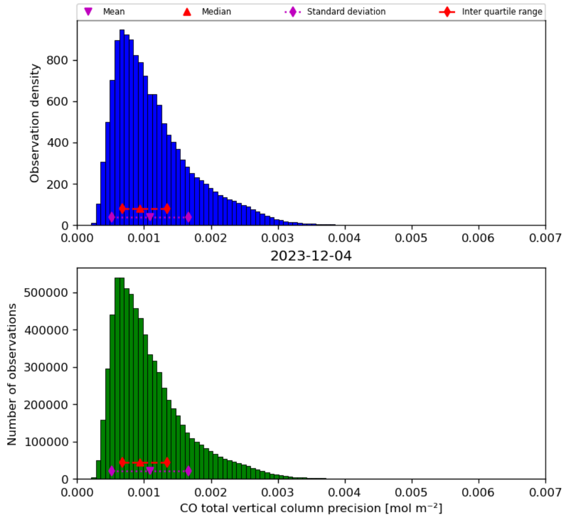
Figure 20: Histogram of “CO total vertical column precision” for 2023-12-04 to 2023-12-05
