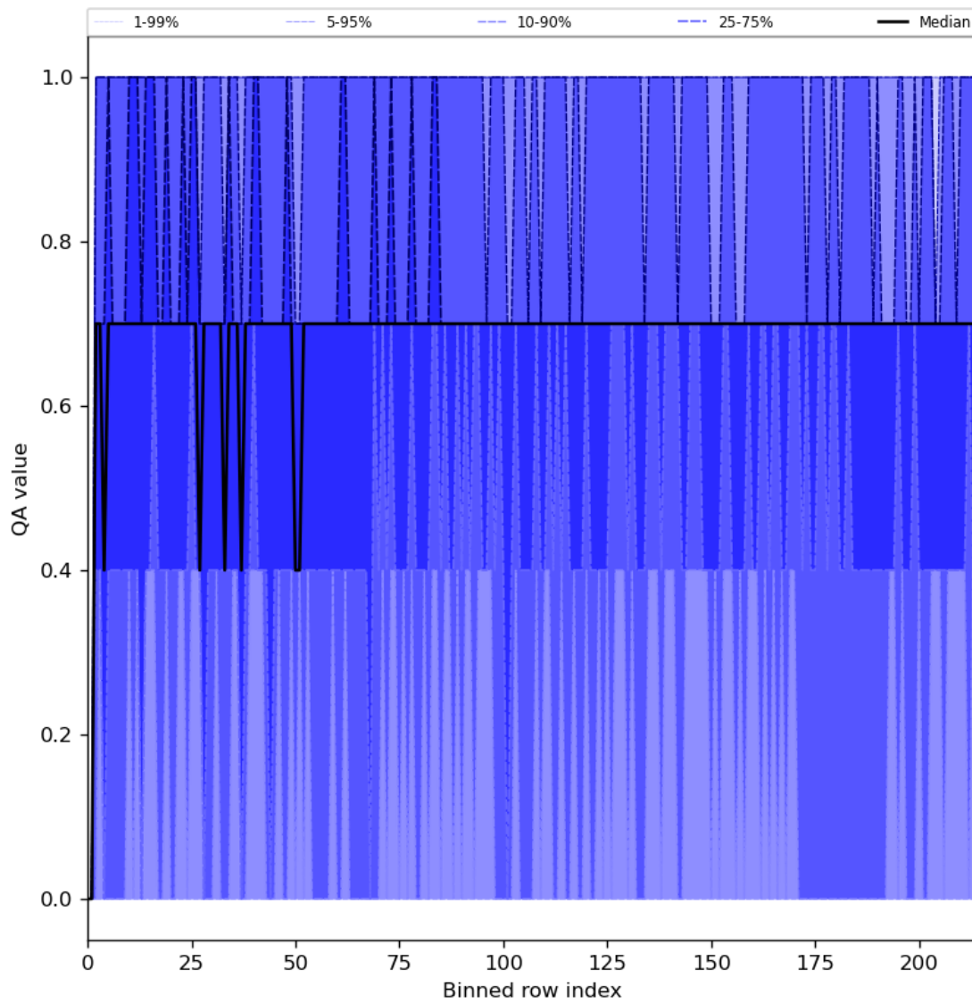
Figure 25: Along track statistics of “QA value” for 2023-12-04 to 2023-12-05
