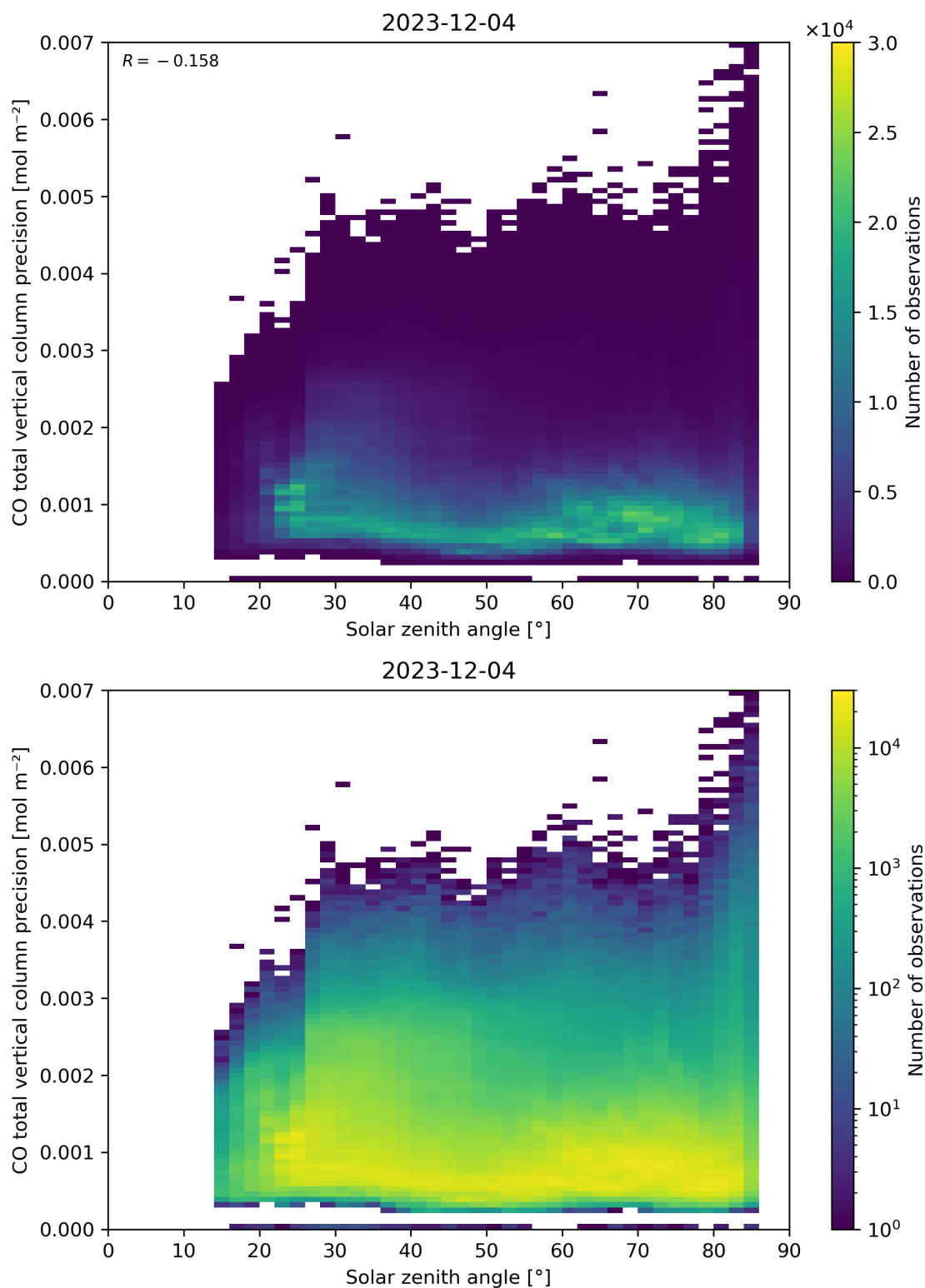
Figure 63: Scatter density plot of “Solar zenith angle” against “CO total vertical column precision” for 2023-12-04 to 2023-12-05.
