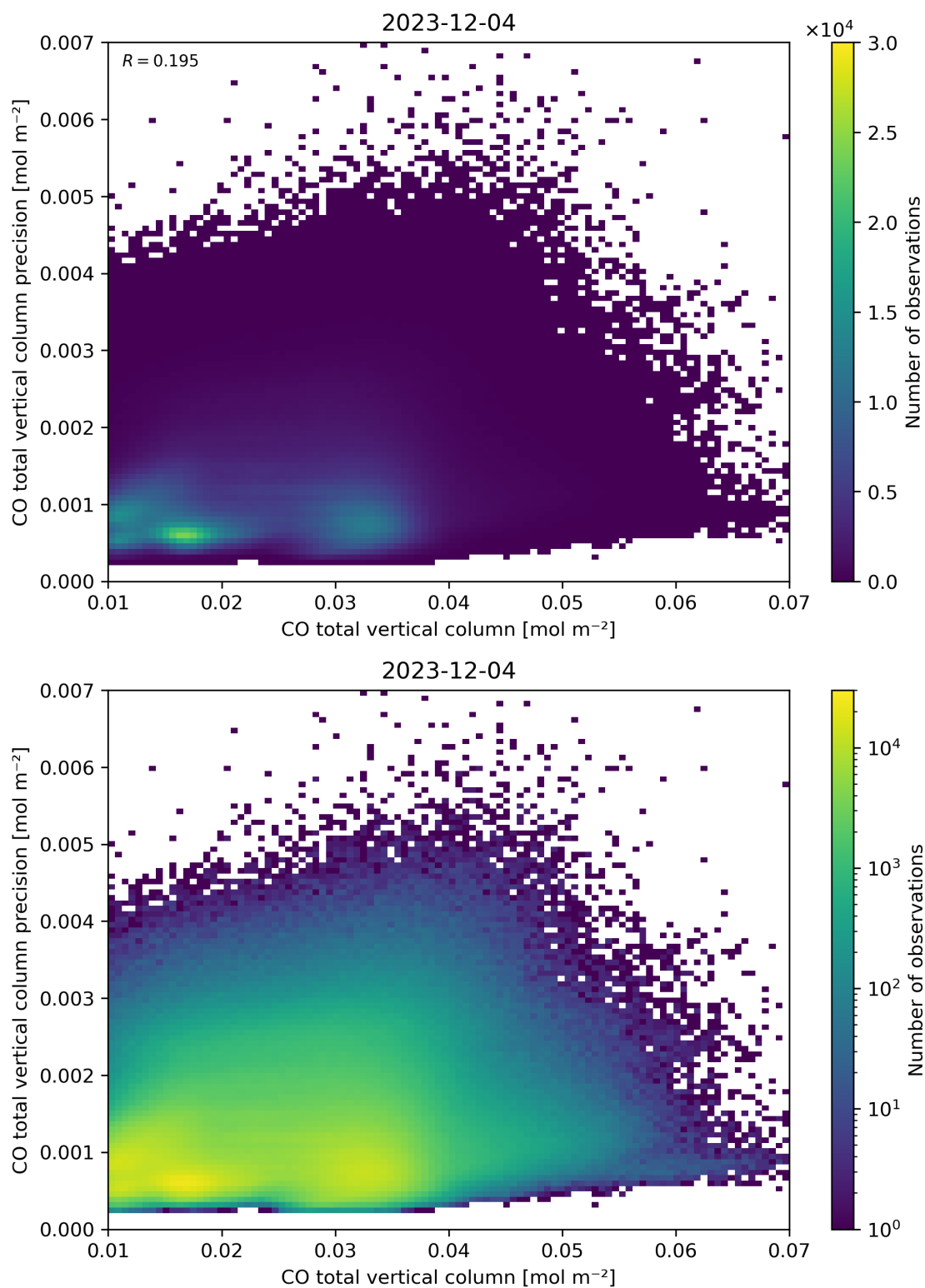
Figure 34: Scatter density plot of “CO total vertical column” against “CO total vertical column precision” for 2023-12-04 to 2023-12-05.
