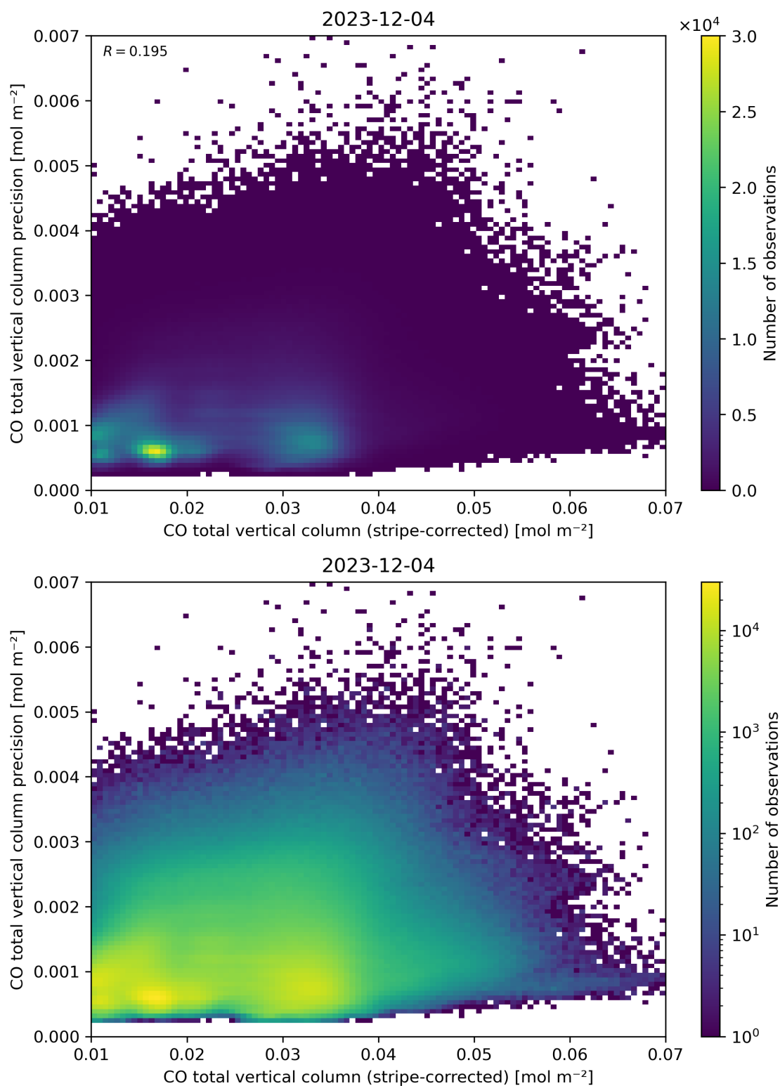
Figure 36: Scatter density plot of “CO total vertical column (stripe-corrected)” against “CO total vertical column precision” for 2023-12-04 to 2023-12-05.
