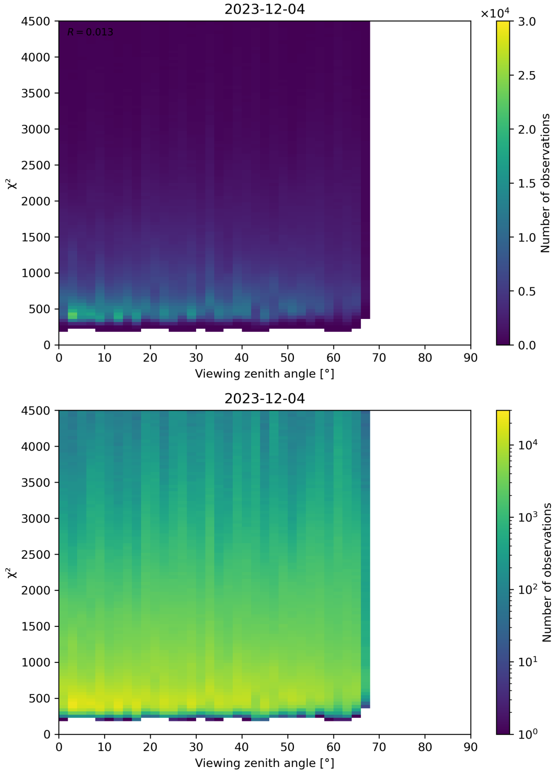
Figure 72: Scatter density plot of “Viewing zenith angle” against “ \chi^2 ” for 2023-12-04 to 2023-12-05.
