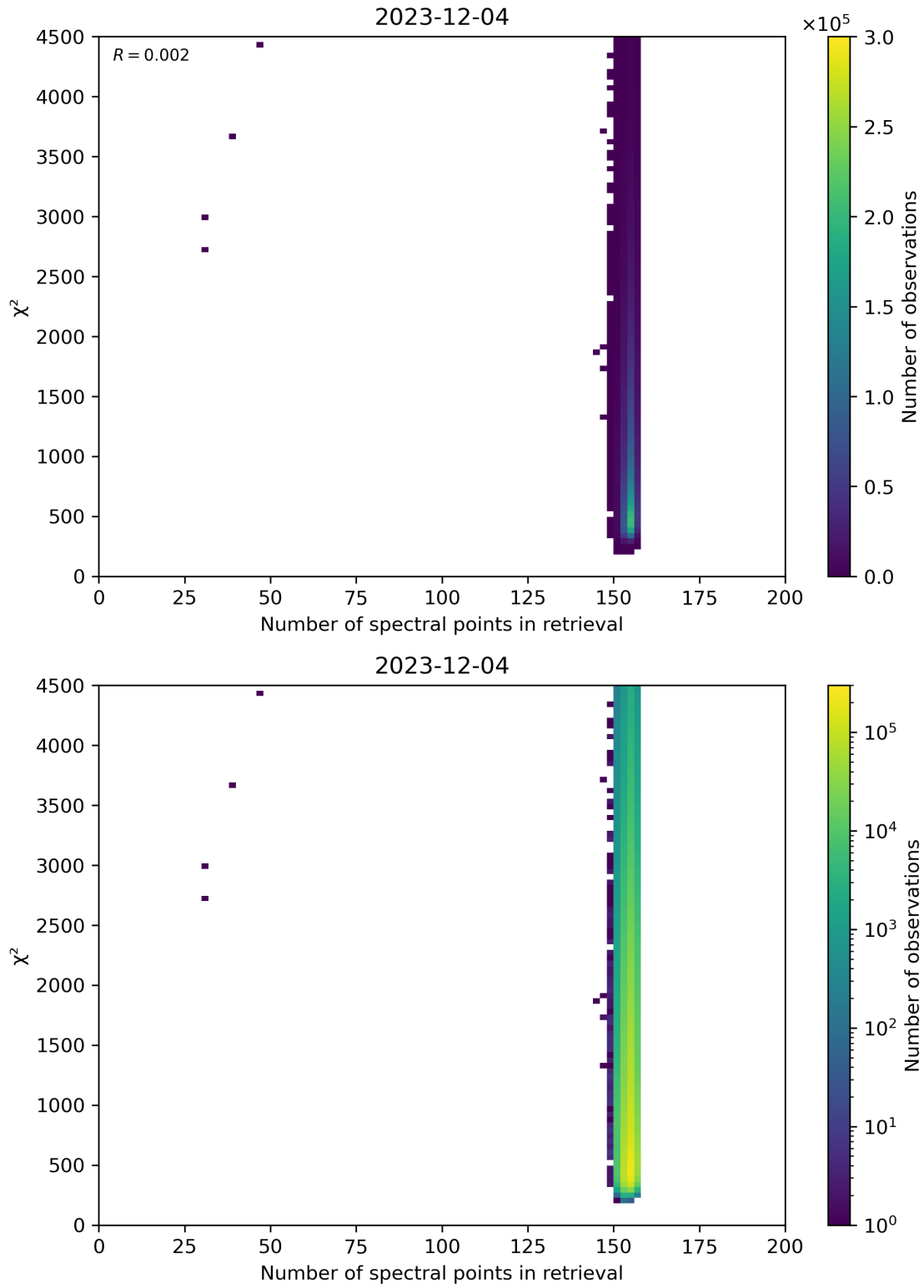
Figure 58: Scatter density plot of “Number of spectral points in retrieval” against “ \chi^2 ” for 2023-12-04 to 2023-12-05.
