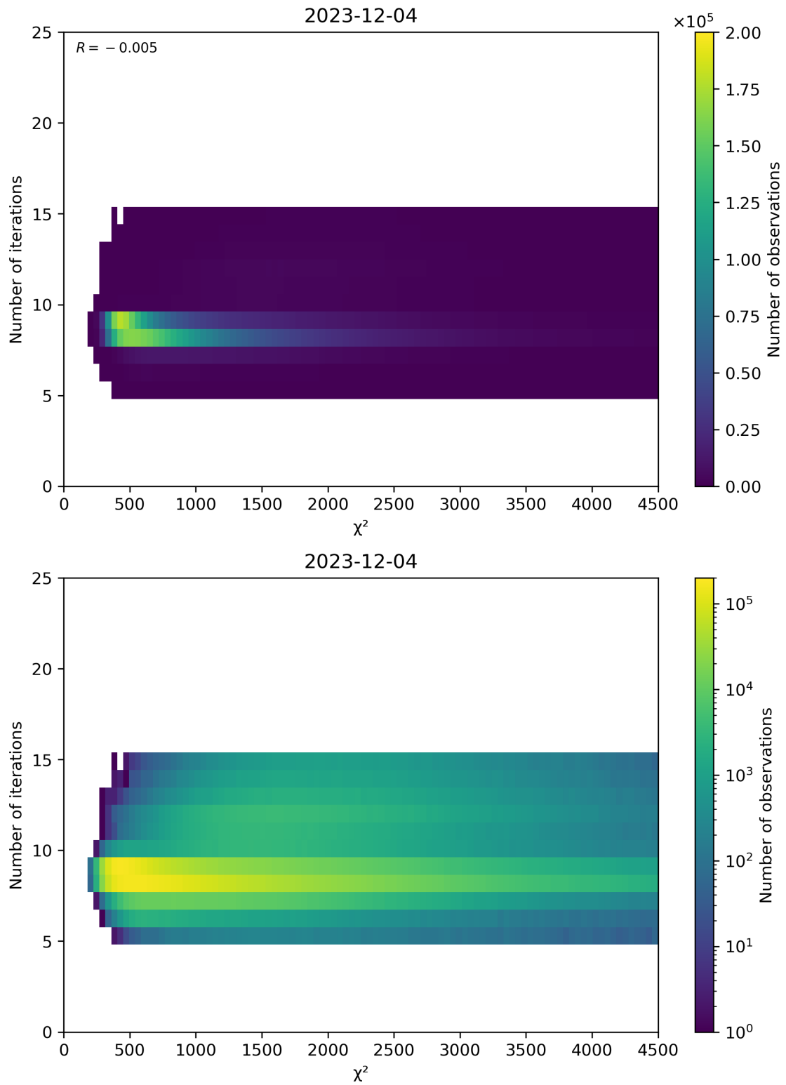
Figure 49: Scatter density plot of “ \chi^2 ” against “Number of iterations” for 2023-12-04 to 2023-12-05.
