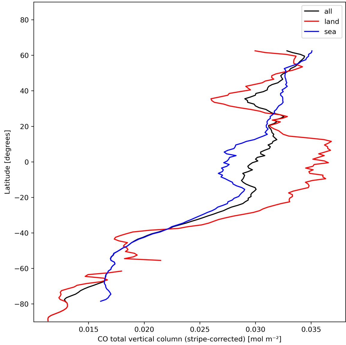
Figure 11: Zonal average of “CO total vertical column (stripe-corrected)” for 2023-12-04 to 2023-12-05.
