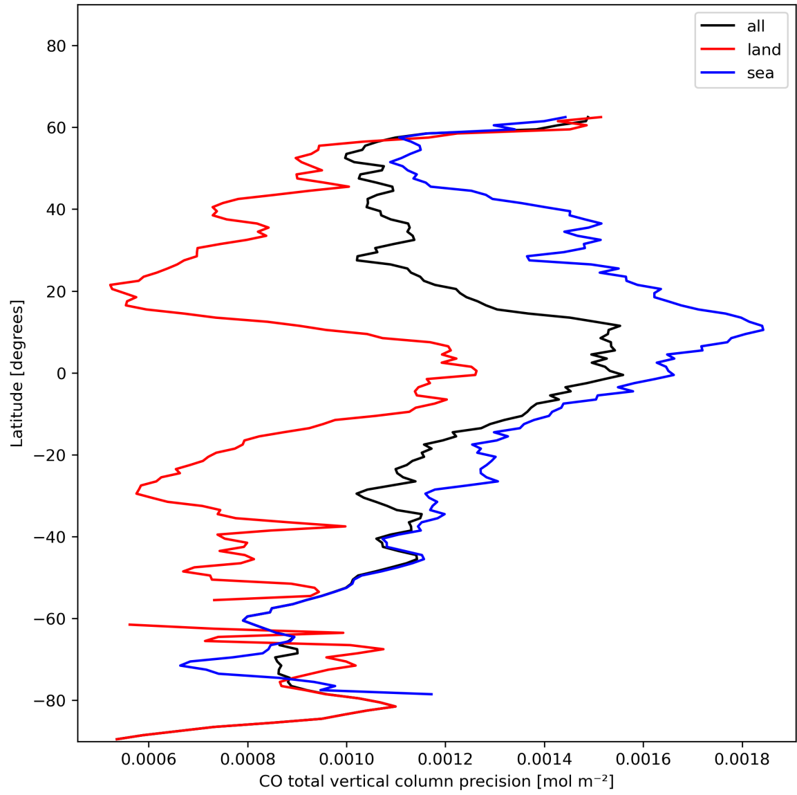
Figure 12: Zonal average of “CO total vertical column precision” for 2023-12-04 to 2023-12-05.
