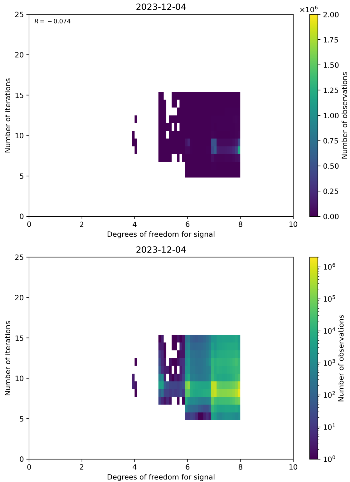
Figure 50: Scatter density plot of “Degrees of freedom for signal” against “Number of iterations” for 2023-12-04 to 2023-12-05.
