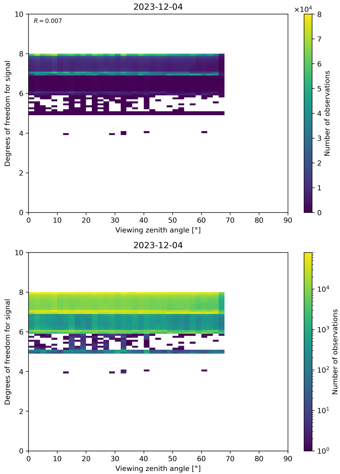
Figure 73: Scatter density plot of “Viewing zenith angle” against “Degrees of freedom for signal” for 2023-12-04 to 2023-12-05.
