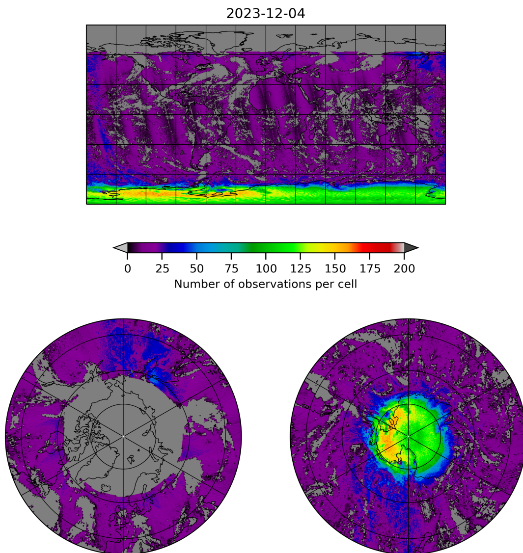
Figure 8: Map of the number of observations for 2023-12-04 to 2023-12-05
