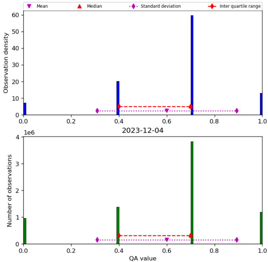
Figure 17: Histogram of “QA value” for 2023-12-04 to 2023-12-05
