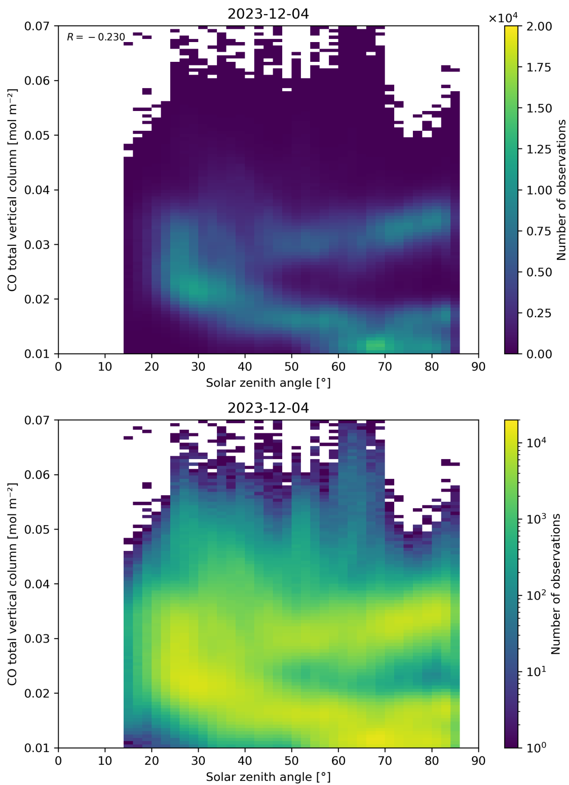
Figure 61: Scatter density plot of “Solar zenith angle” against “CO total vertical column” for 2023-12-04 to 2023-12-05.
