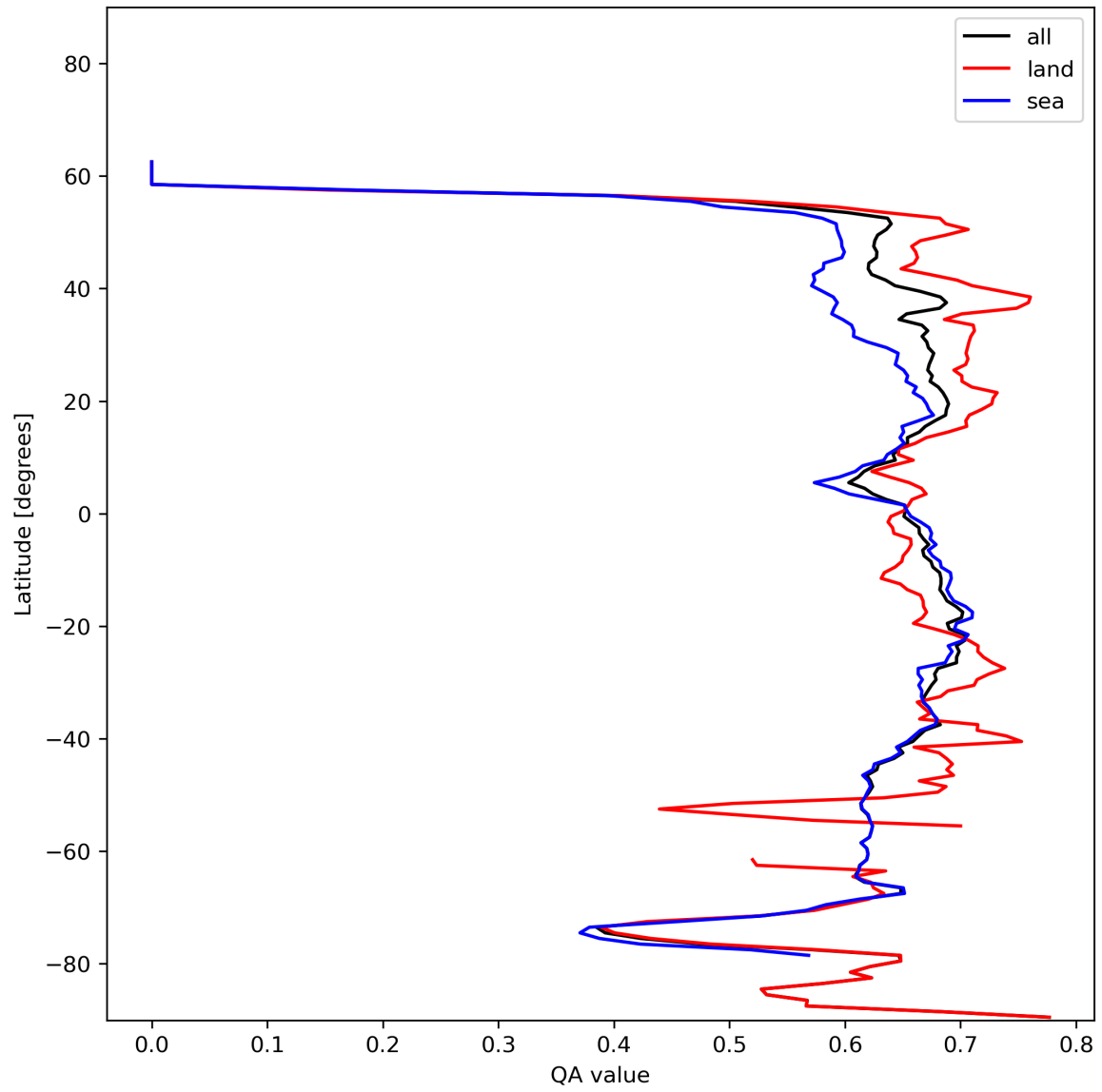
Figure 9: Zonal average of “QA value” for 2023-12-04 to 2023-12-05.
