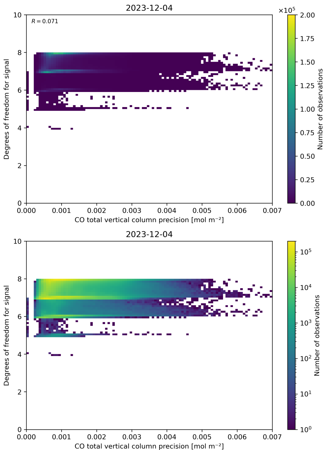
Figure 45: Scatter density plot of “CO total vertical column precision” against “Degrees of freedom for signal” for 2023-12-04 to 2023-12-05.
