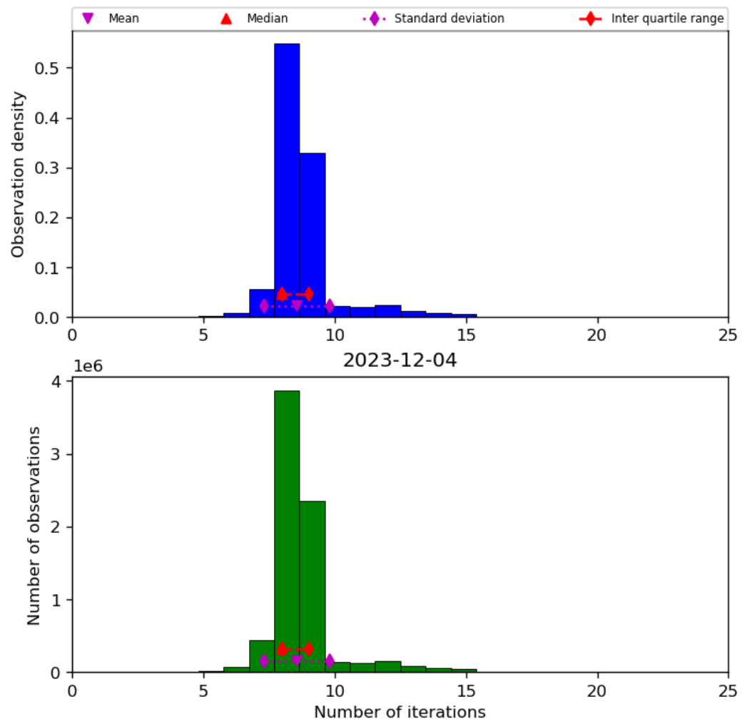
Figure 24: Histogram of “Number of iterations” for 2023-12-04 to 2023-12-05
