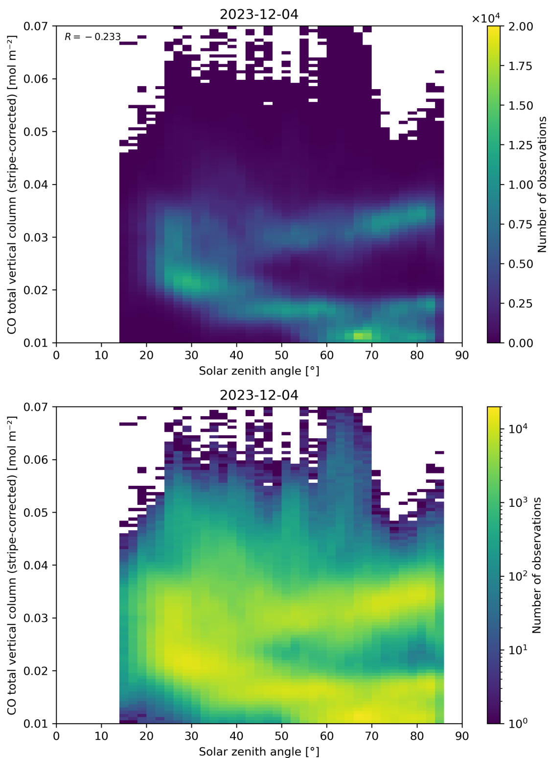
Figure 62: Scatter density plot of “Solar zenith angle” against “CO total vertical column (stripe-corrected)” for 2023-12-04 to 2023-12-05.
