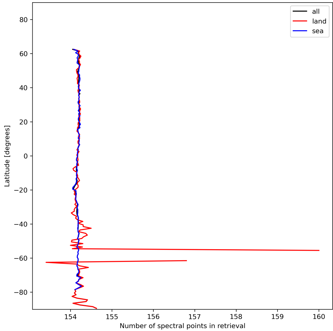
Figure 13: Zonal average of “Number of spectral points in retrieval” for 2023-12-04 to 2023-12-05.
