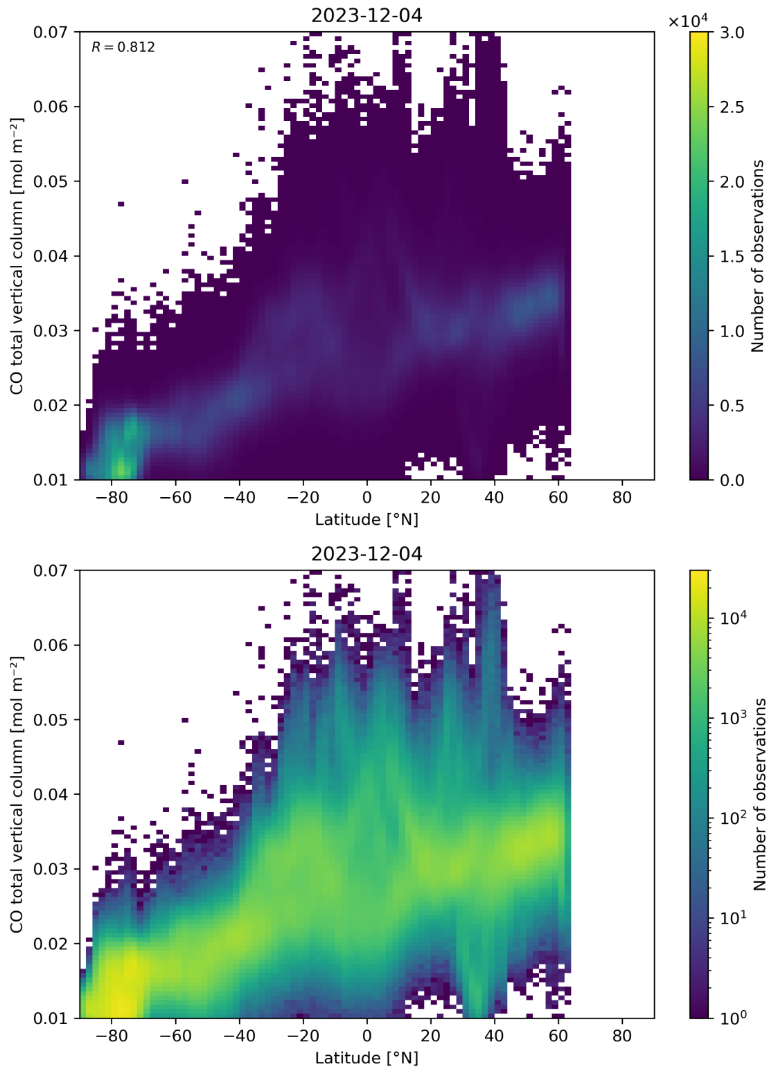
Figure 51: Scatter density plot of “Latitude” against “CO total vertical column” for 2023-12-04 to 2023-12-05.
