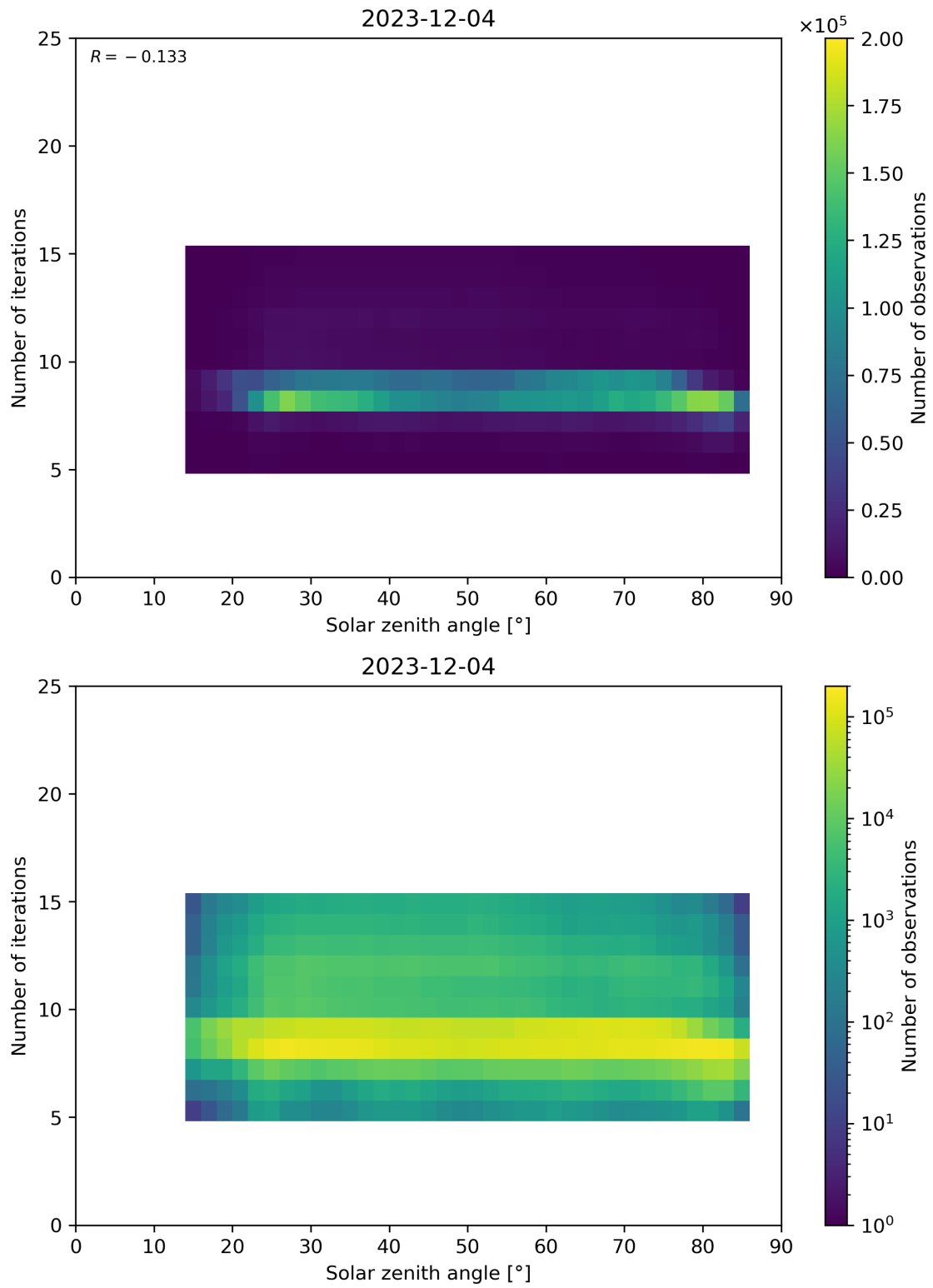
Figure 67: Scatter density plot of “Solar zenith angle” against “Number of iterations” for 2023-12-04 to 2023-12-05.
