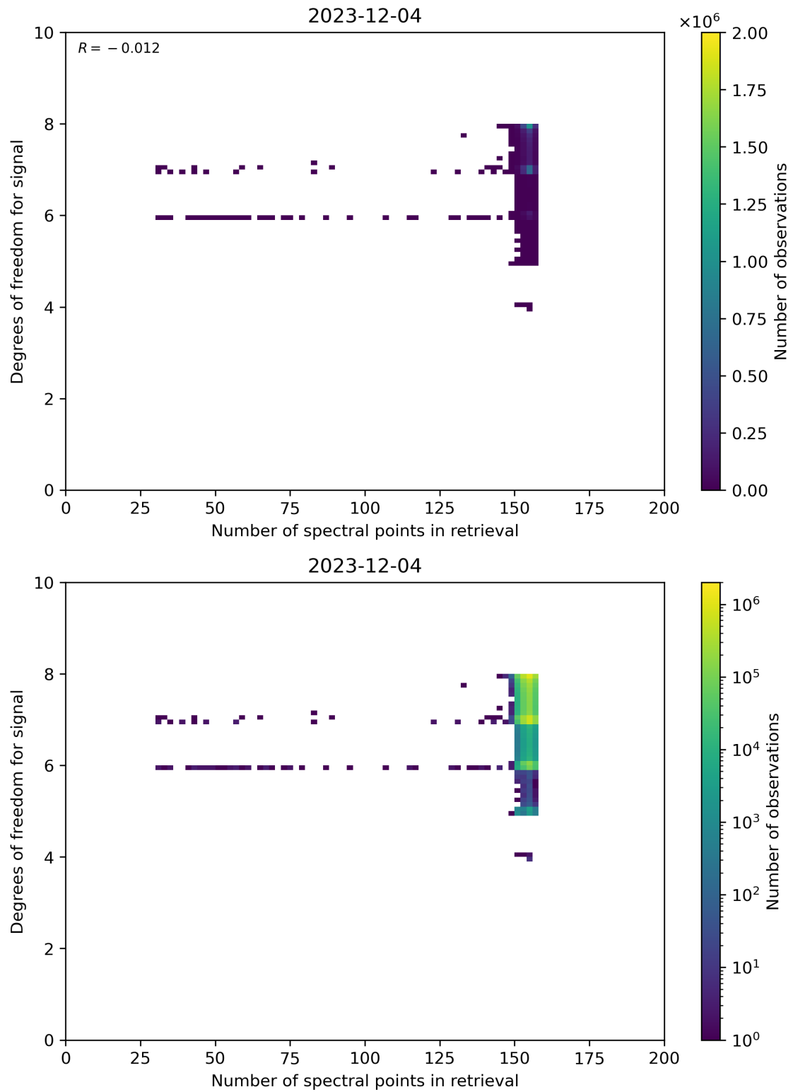
Figure 59: Scatter density plot of “Number of spectral points in retrieval” against “Degrees of freedom for signal” for 2023-12-04 to 2023-12-05.
