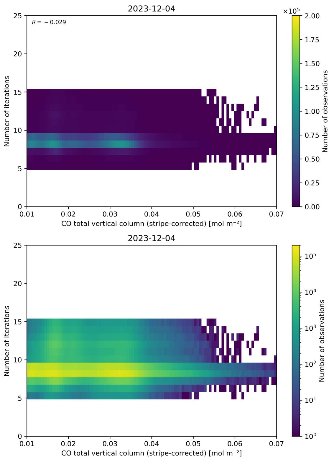
Figure 39: Scatter density plot of “CO total vertical column (stripe-corrected)” against “Number of iterations” for 2023-12-04 to 2023-12-05.
