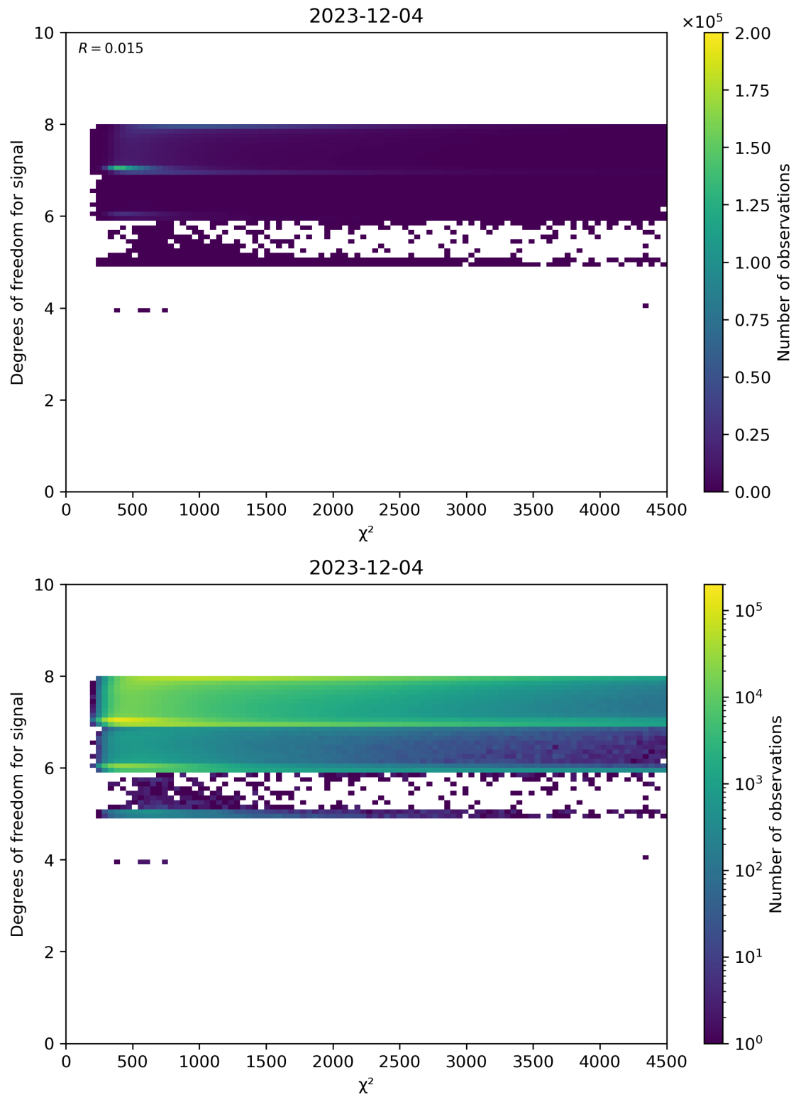
Figure 48: Scatter density plot of “ \chi^2 ” against “Degrees of freedom for signal” for 2023-12-04 to 2023-12-05.
