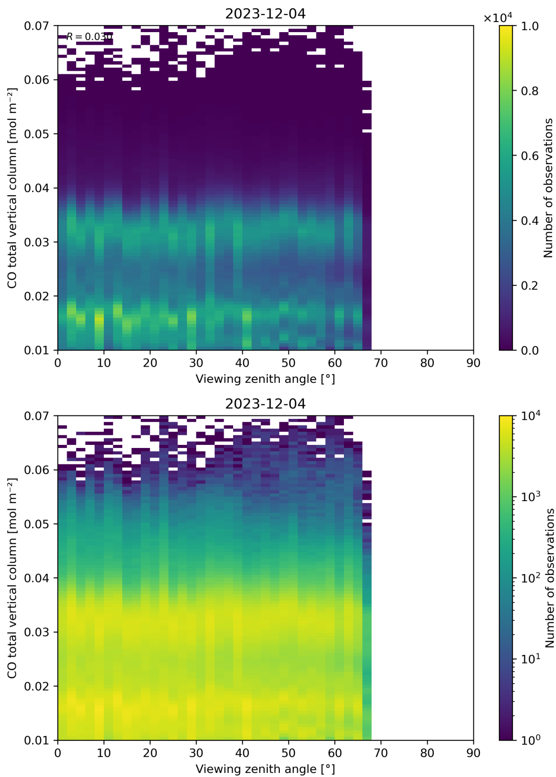
Figure 69: Scatter density plot of “Viewing zenith angle” against “CO total vertical column” for 2023-12-04 to 2023-12-05.
