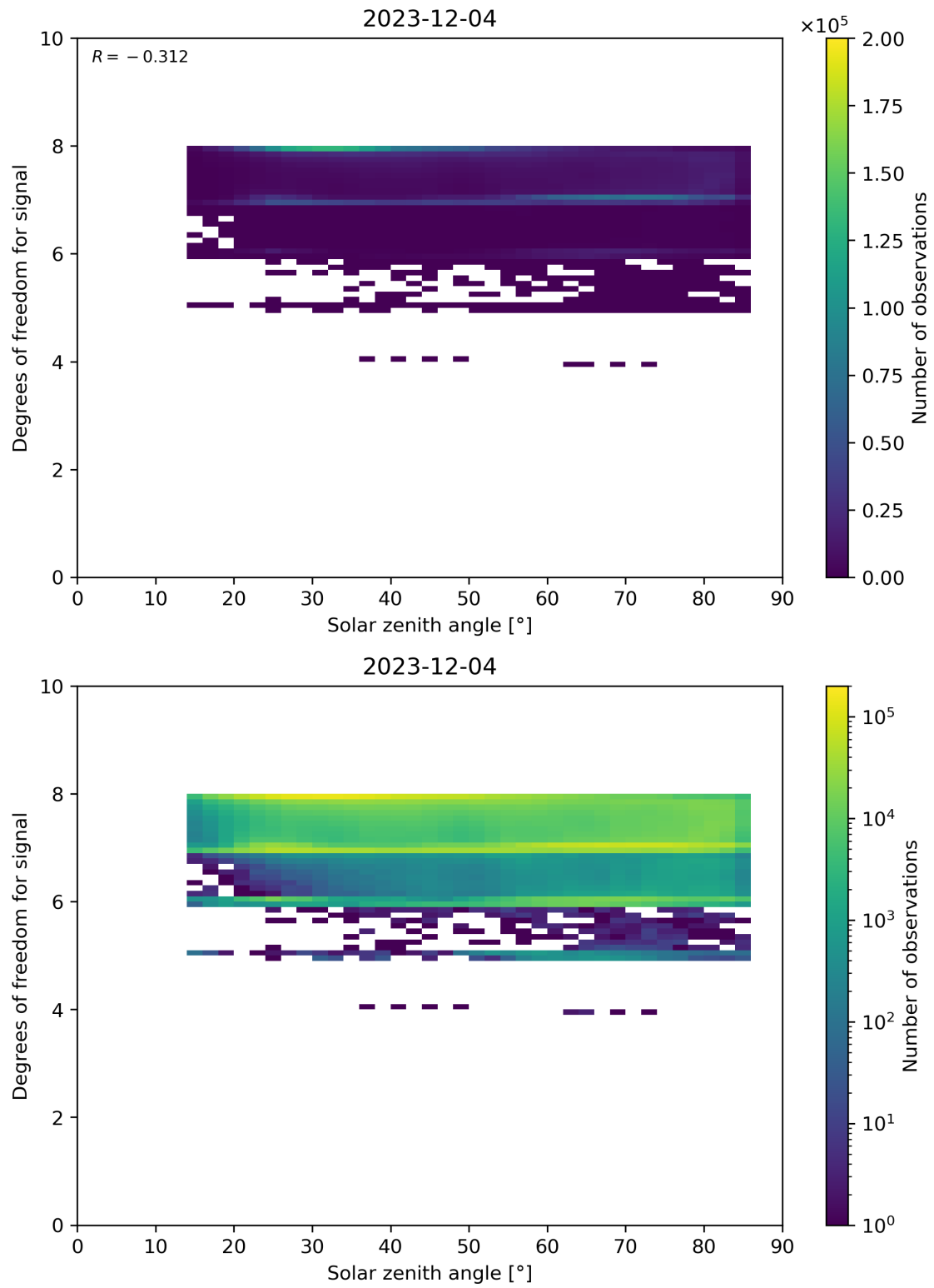
Figure 65: Scatter density plot of “Solar zenith angle” against “Degrees of freedom for signal” for 2023-12-04 to 2023-12-05.
