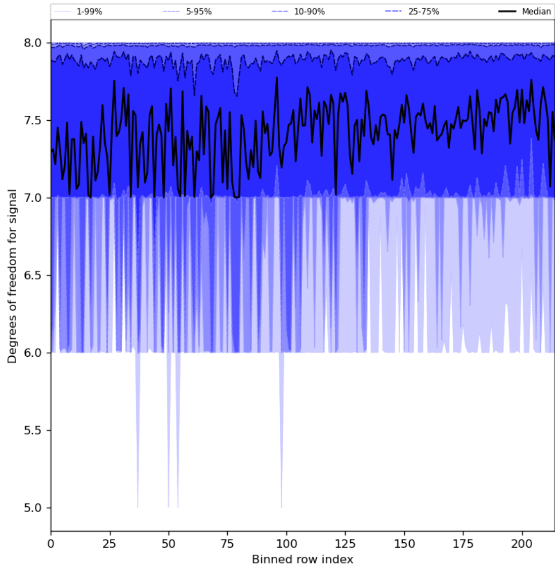
Figure 31: Along track statistics of “Degrees of freedom for signal” for 2023-12-04 to 2023-12-05
