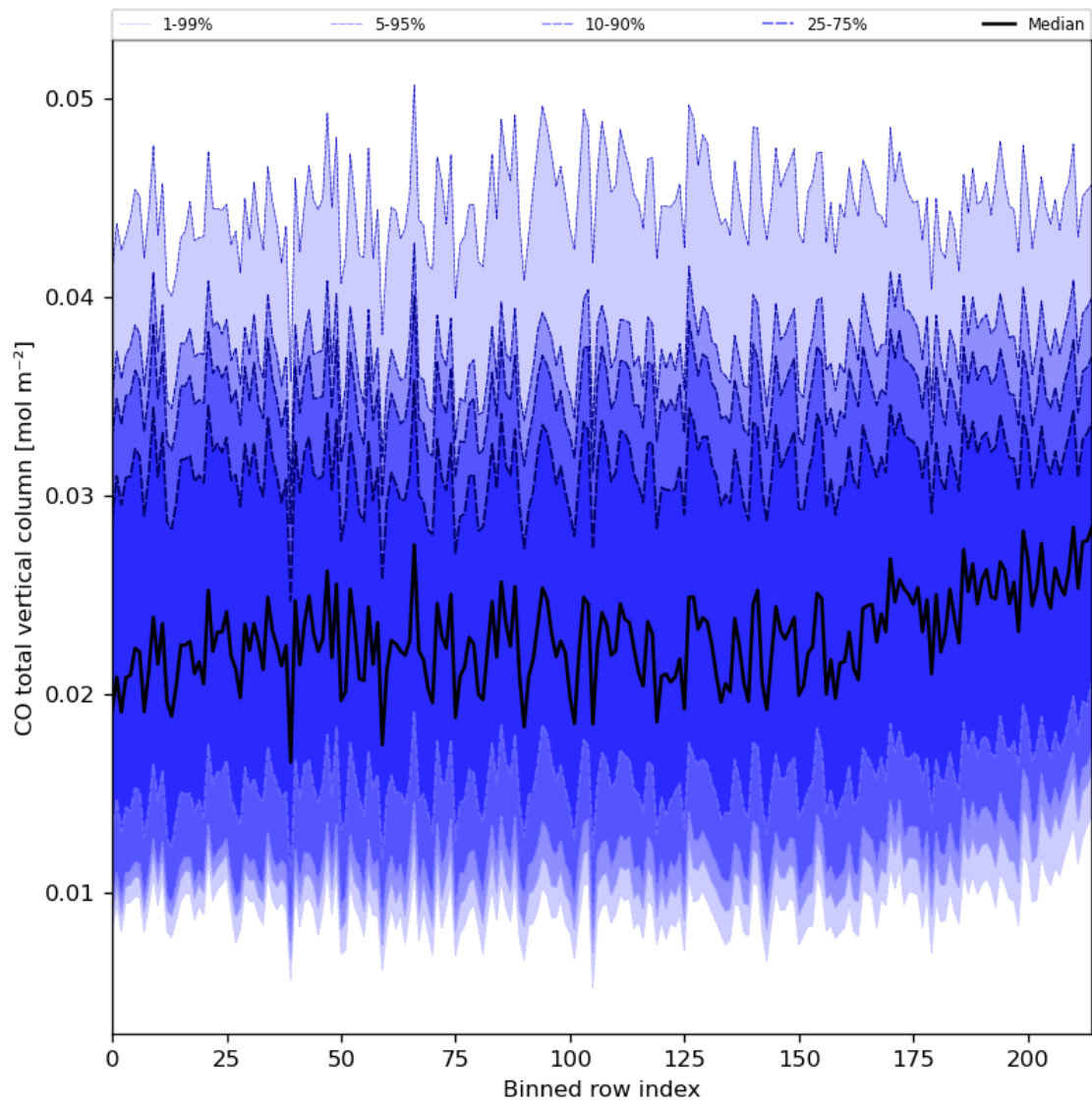
Figure 26: Along track statistics of “CO total vertical column” for 2023-12-04 to 2023-12-05
