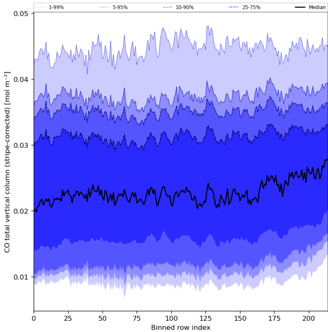
Figure 27: Along track statistics of “CO total vertical column (stripe-corrected)” for 2023-12-04 to 2023-12-05
