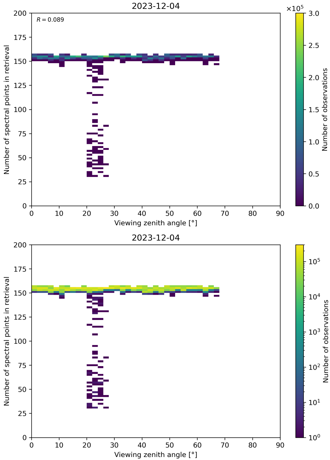
Figure 76: Scatter density plot of “Viewing zenith angle” against “Number of spectral points in retrieval” for 2023-12-04 to 2023-12-05.
