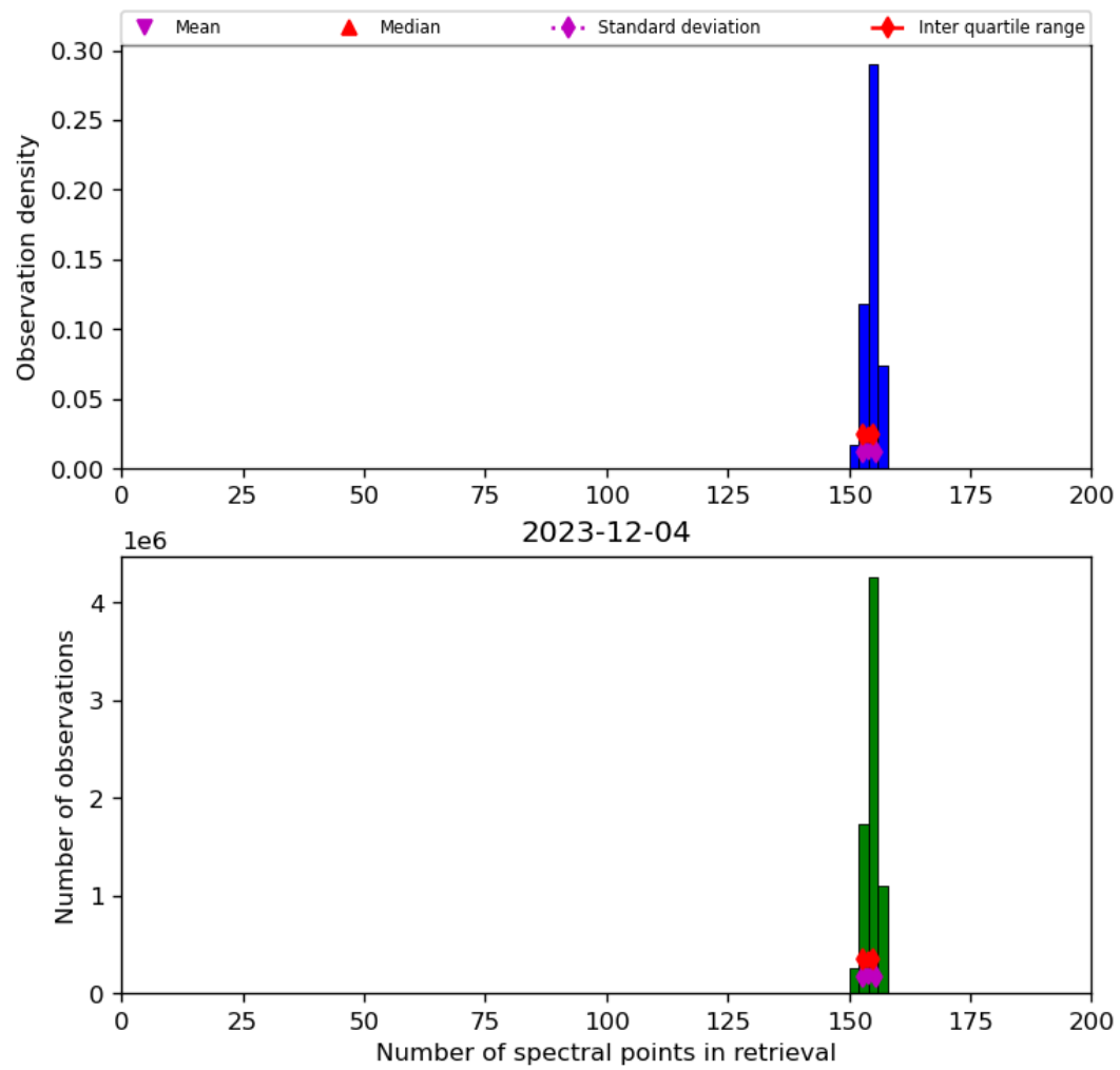
Figure 21: Histogram of “Number of spectral points in retrieval” for 2023-12-04 to 2023-12-05
