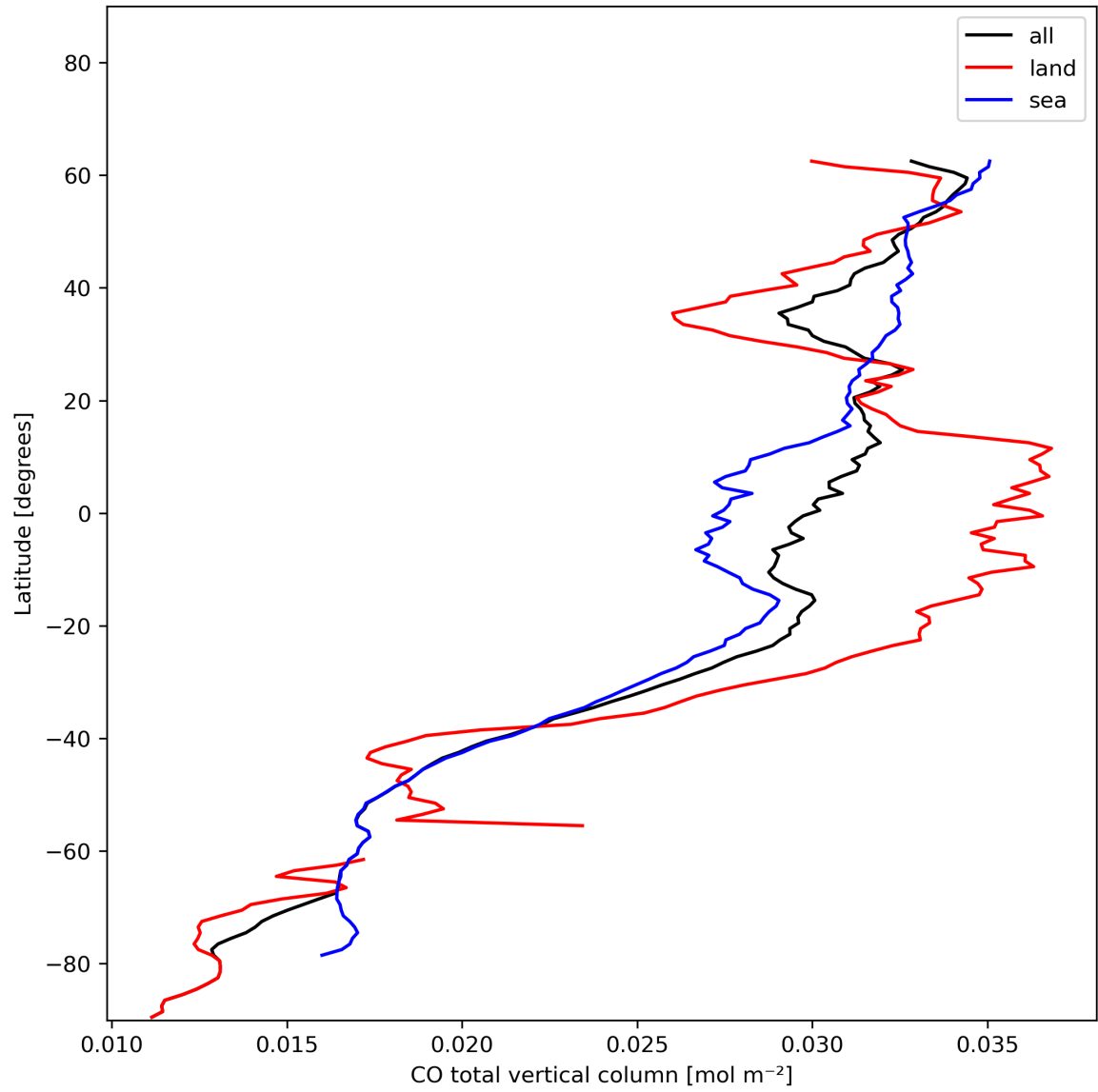
Figure 10: Zonal average of “CO total vertical column” for 2023-12-04 to 2023-12-05.
