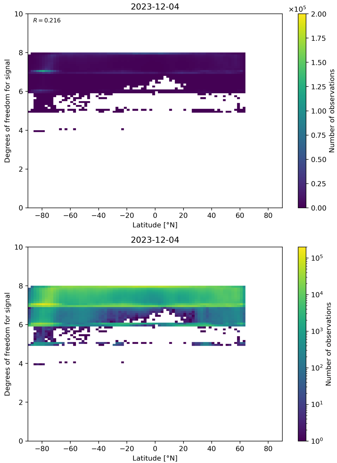
Figure 55: Scatter density plot of “Latitude” against “Degrees of freedom for signal” for 2023-12-04 to 2023-12-05.
