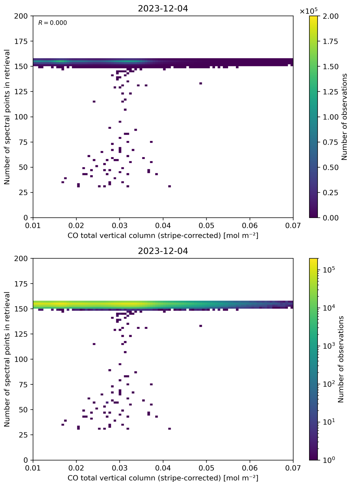
Figure 40: Scatter density plot of “CO total vertical column (stripe-corrected)” against “Number of spectral points in retrieval” for 2023-12-04 to 2023-12-05.
