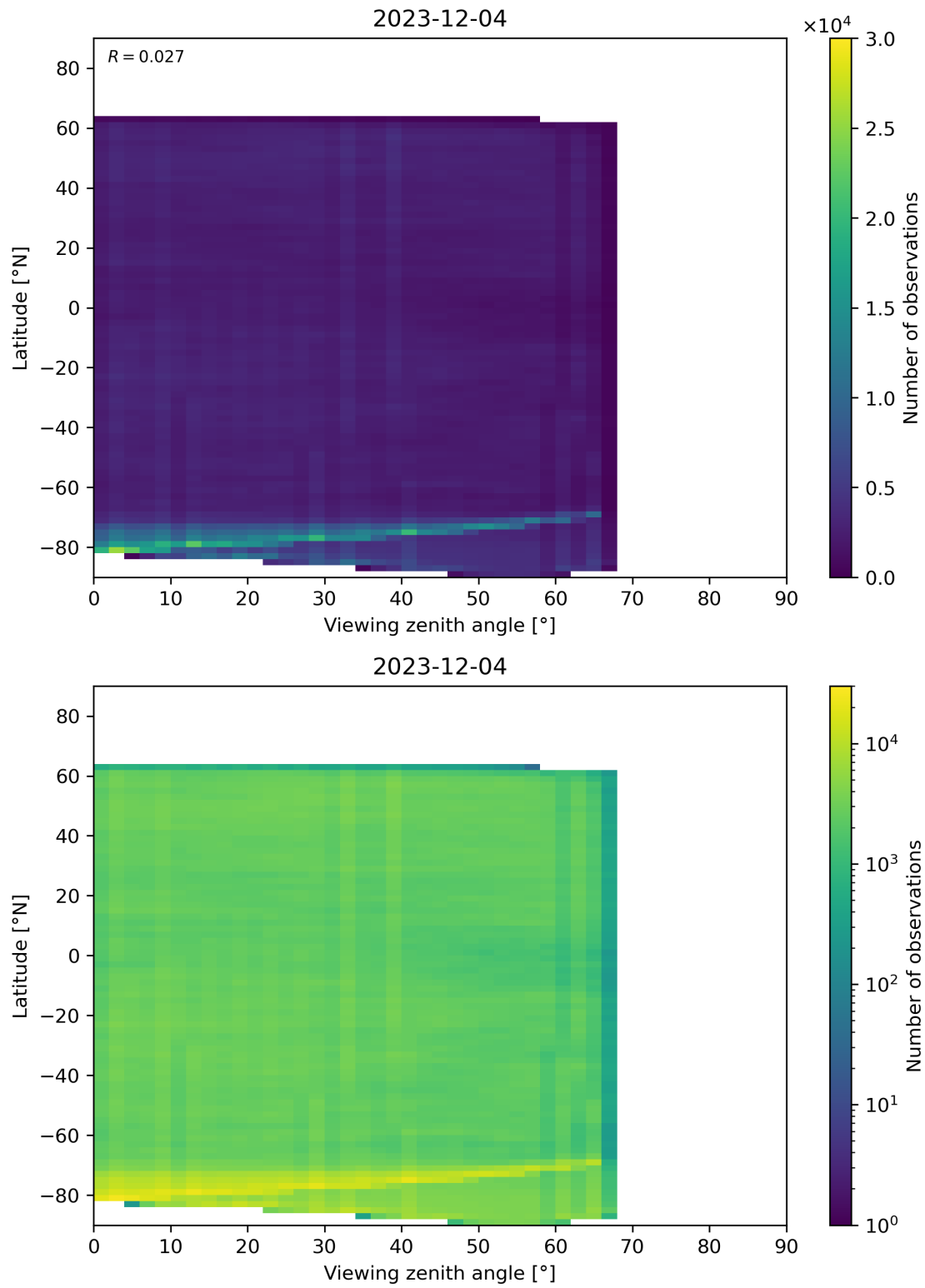
Figure 74: Scatter density plot of “Viewing zenith angle” against “Latitude” for 2023-12-04 to 2023-12-05.
