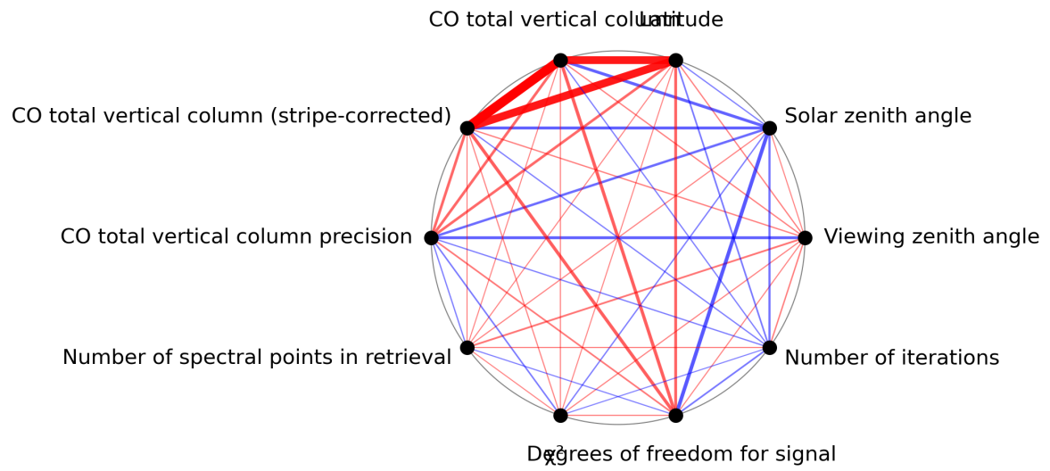
Figure 1: Map of correlation graph for 2023-12-04 to 2023-12-05.
