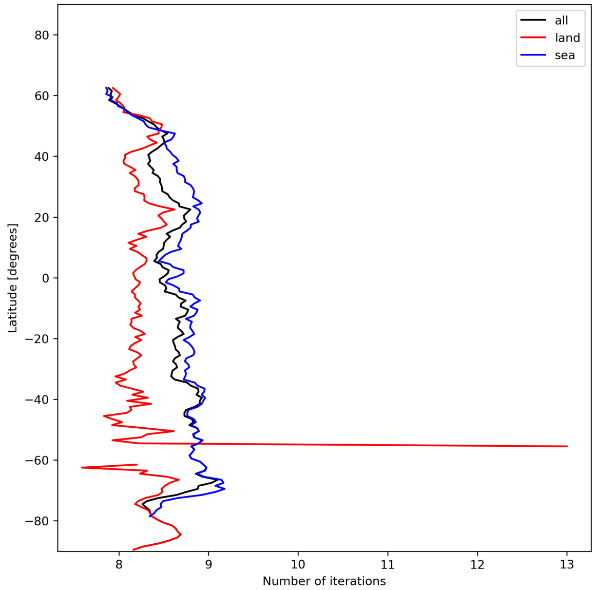
Figure 16: Zonal average of “Number of iterations” for 2023-12-04 to 2023-12-05.
