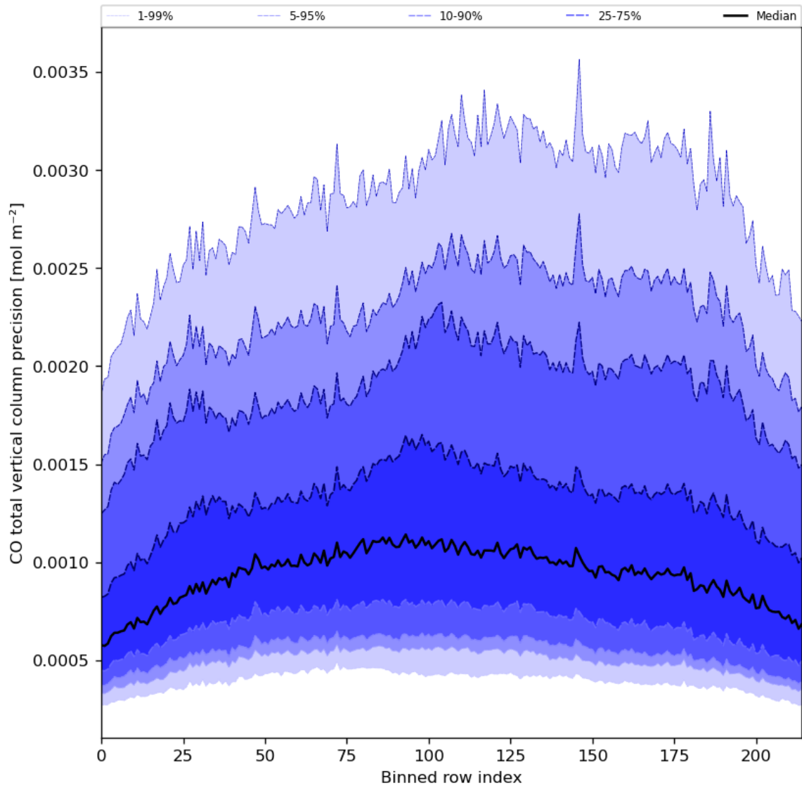
Figure 28: Along track statistics of “CO total vertical column precision” for 2023-12-04 to 2023-12-05
