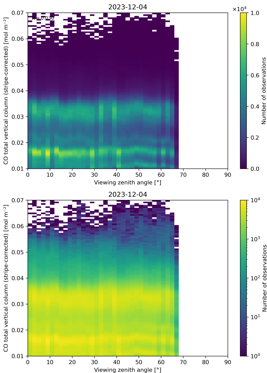
Figure 70: Scatter density plot of “Viewing zenith angle” against “CO total vertical column (stripe-corrected)” for 2023-12-04 to 2023-12-05.
