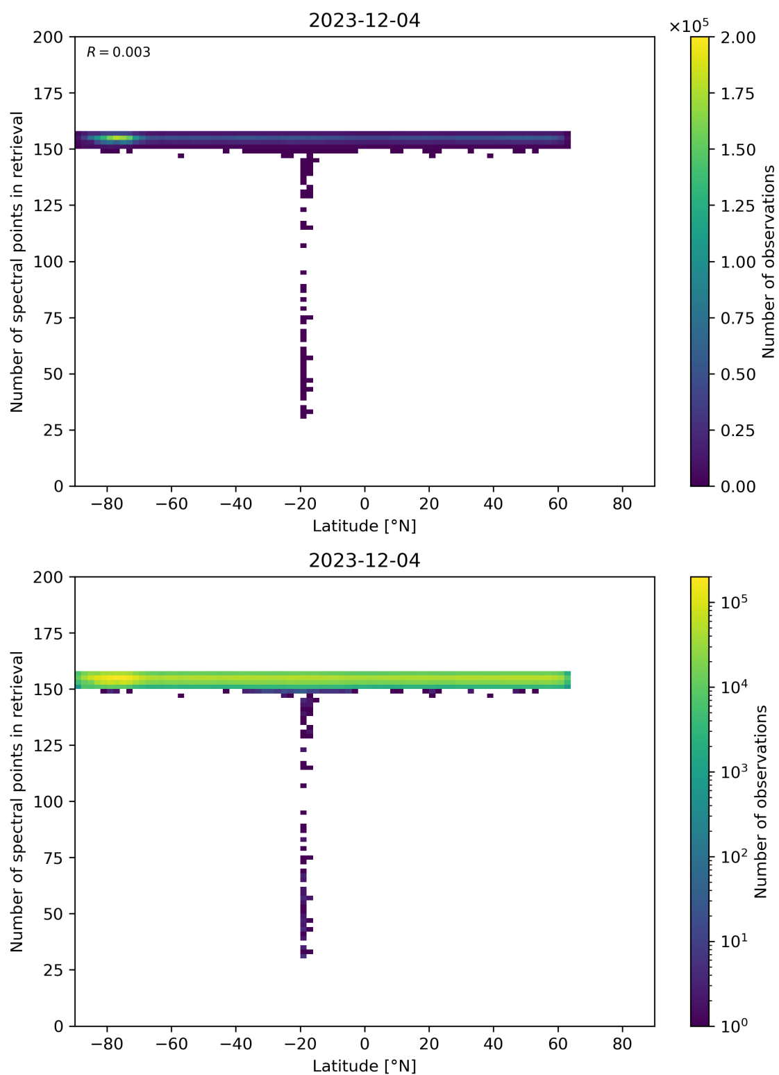
Figure 57: Scatter density plot of “Latitude” against “Number of spectral points in retrieval” for 2023-12-04 to 2023-12-05.
