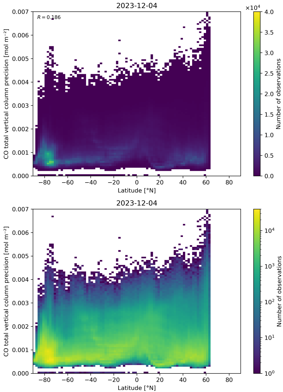
Figure 53: Scatter density plot of “Latitude” against “CO total vertical column precision” for 2023-12-04 to 2023-12-05.
