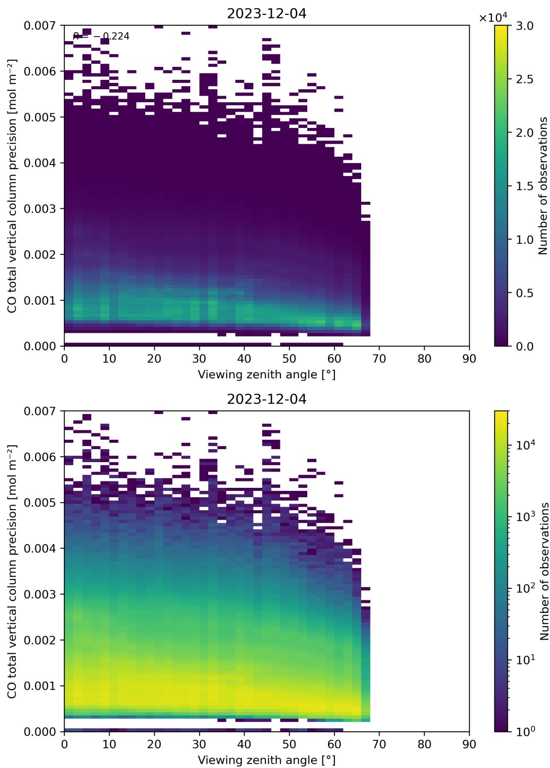
Figure 71: Scatter density plot of “Viewing zenith angle” against “CO total vertical column precision” for 2023-12-04 to 2023-12-05.
