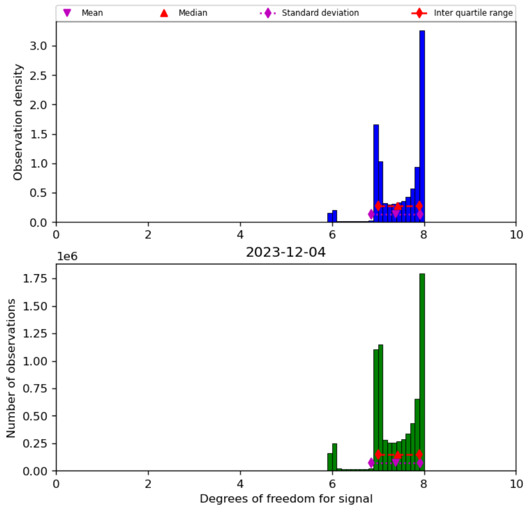
Figure 23: Histogram of “Degrees of freedom for signal” for 2023-12-04 to 2023-12-05
