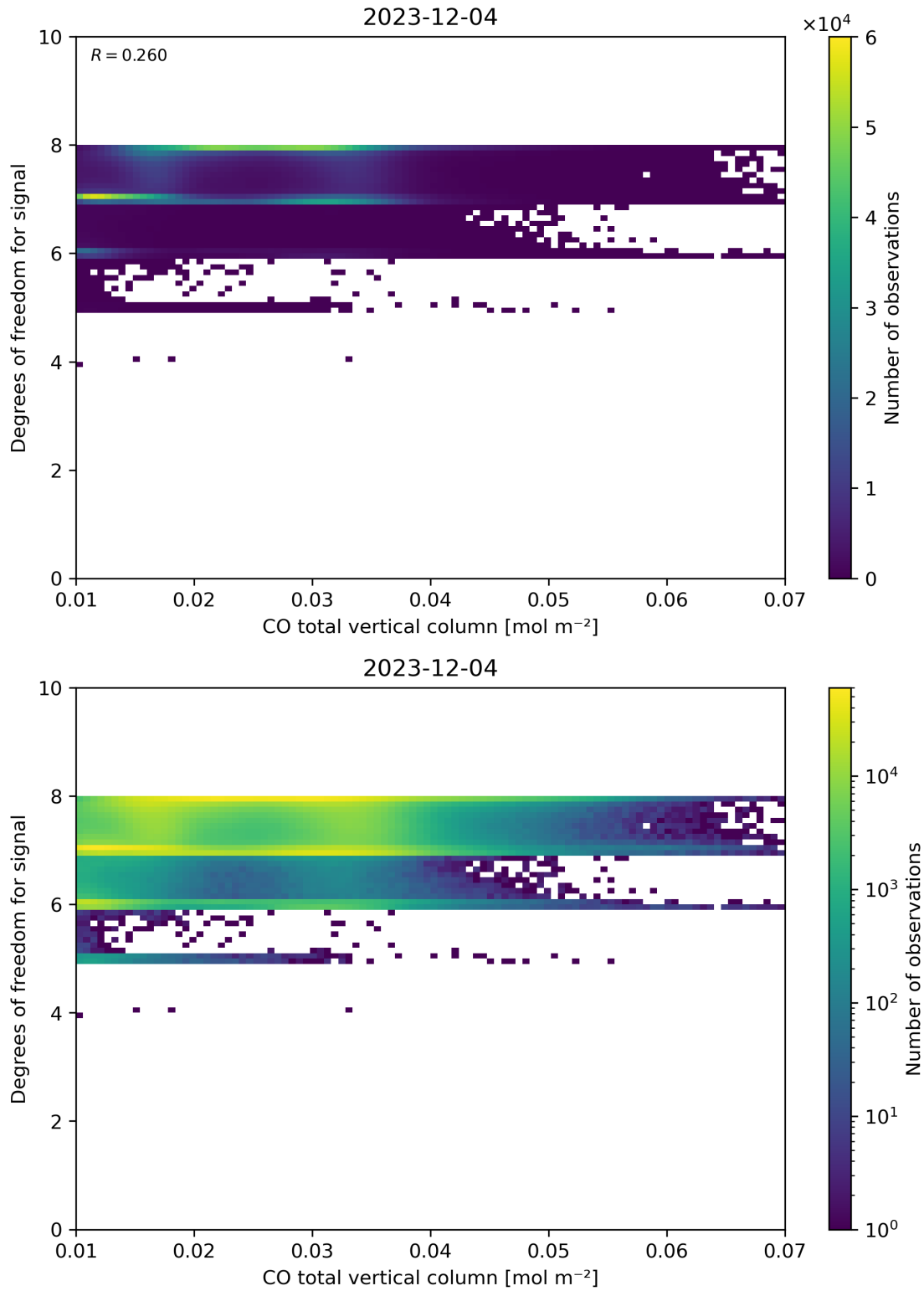
Figure 41: Scatter density plot of “CO total vertical column” against “Degrees of freedom for signal” for 2023-12-04 to 2023-12-05.
