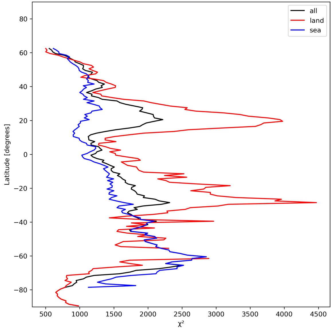
Figure 14: Zonal average of “ \chi^2 ” for 2023-12-04 to 2023-12-05.
