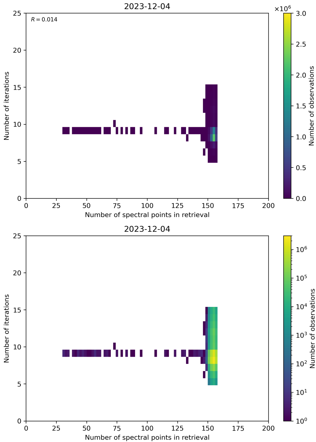
Figure 60: Scatter density plot of “Number of spectral points in retrieval” against “Number of iterations” for 2023-12-04 to 2023-12-05.
