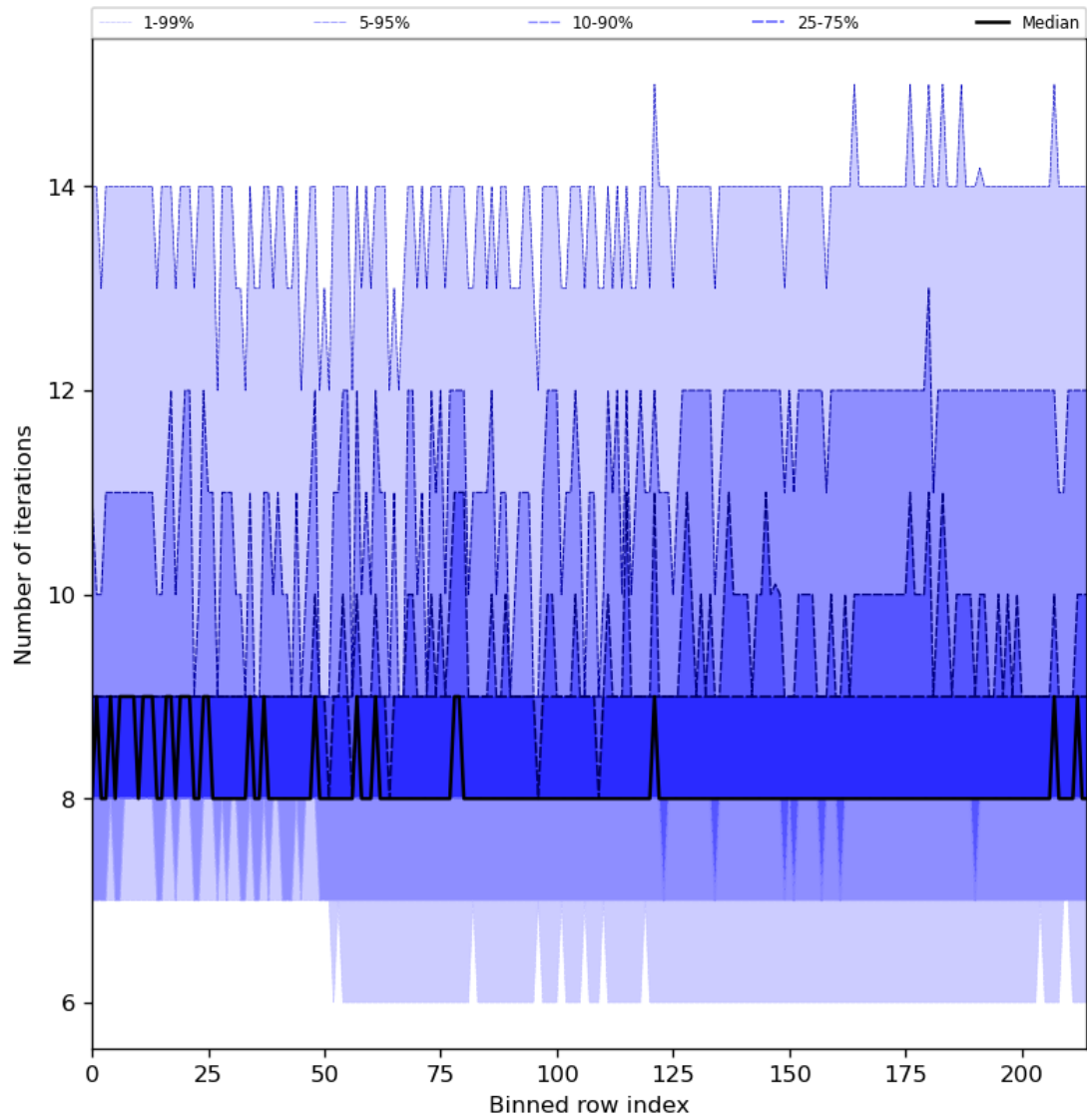
Figure 32: Along track statistics of “Number of iterations” for 2023-12-04 to 2023-12-05
