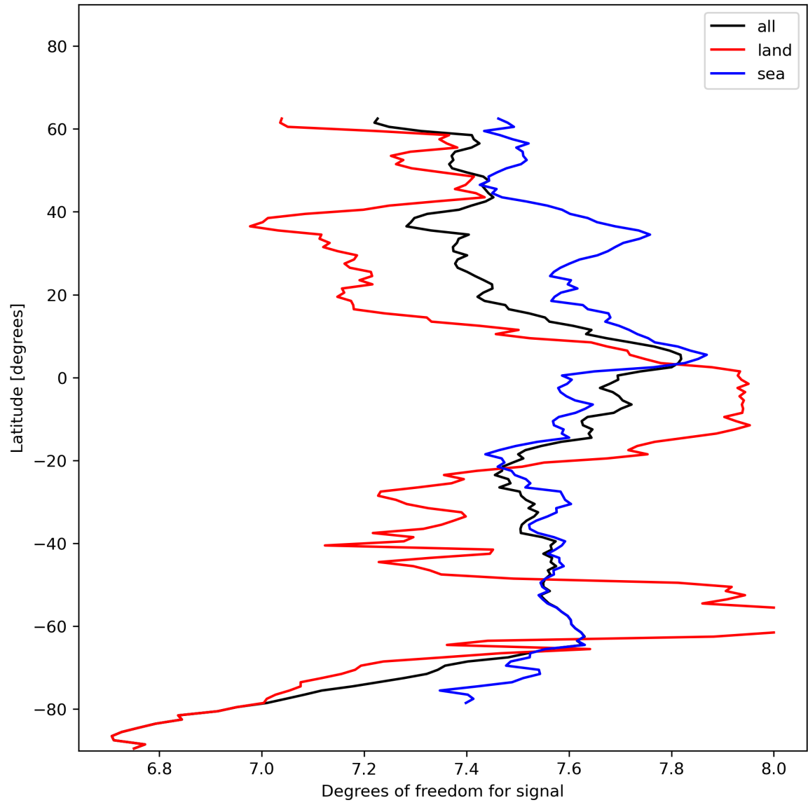
Figure 15: Zonal average of “Degrees of freedom for signal” for 2023-12-04 to 2023-12-05.
