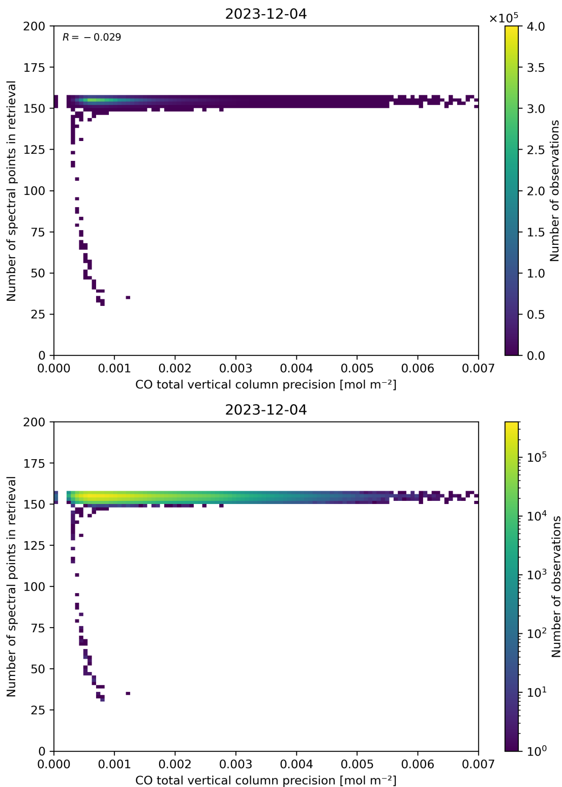
Figure 47: Scatter density plot of “CO total vertical column precision” against “Number of spectral points in retrieval” for 2023-12-04 to 2023-12-05.
