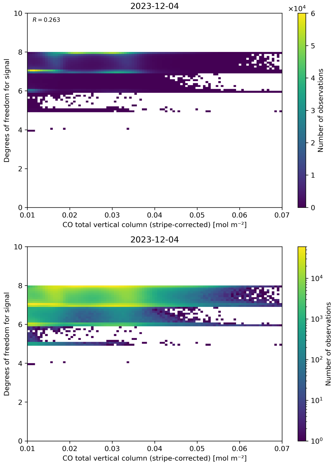
Figure 38: Scatter density plot of “CO total vertical column (stripe-corrected)” against “Degrees of freedom for signal” for 2023-12-04 to 2023-12-05.
