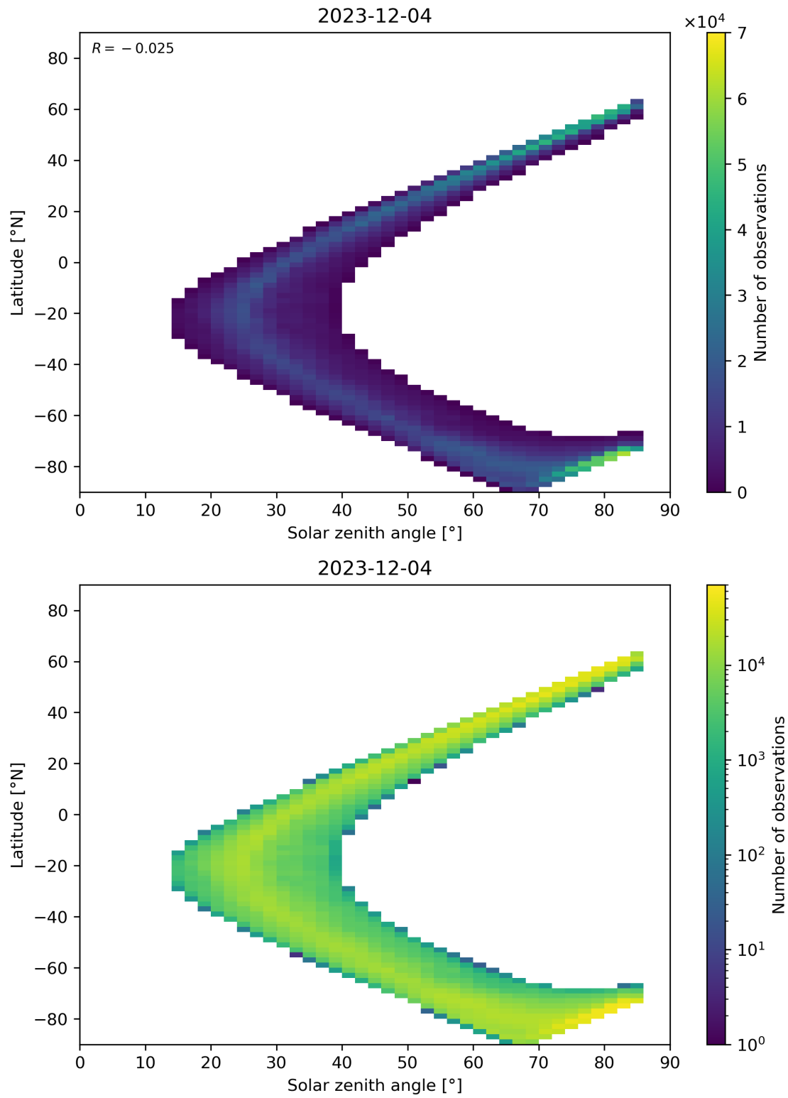
Figure 66: Scatter density plot of “Solar zenith angle” against “Latitude” for 2023-12-04 to 2023-12-05.
