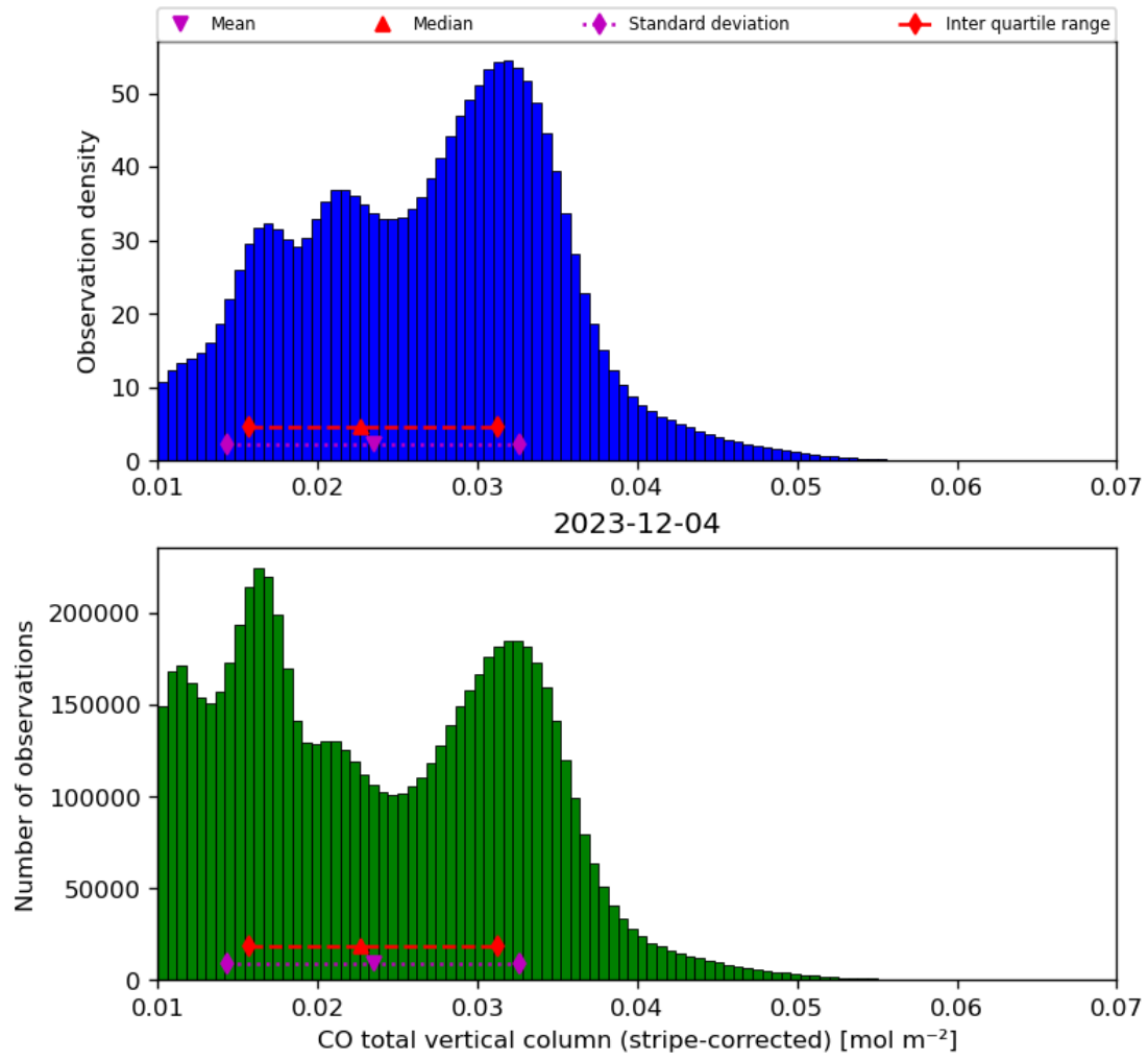
Figure 19: Histogram of “CO total vertical column (stripe-corrected)” for 2023-12-04 to 2023-12-05
