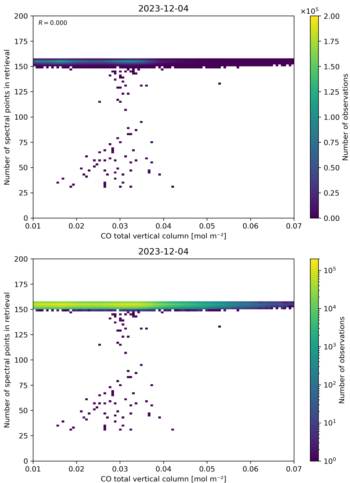
Figure 43: Scatter density plot of “CO total vertical column” against “Number of spectral points in retrieval” for 2023-12-04 to 2023-12-05.
