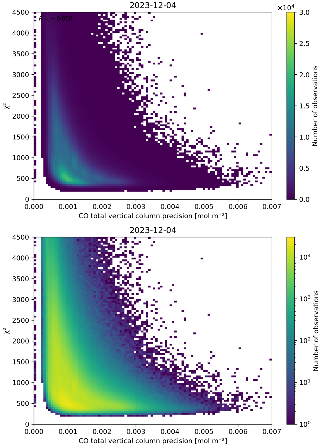
Figure 44: Scatter density plot of “CO total vertical column precision” against “ \chi^2 ” for 2023-12-04 to 2023-12-05.
