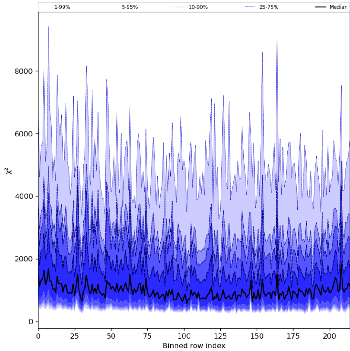
Figure 30: Along track statistics of “ \chi^2 ” for 2023-12-04 to 2023-12-05
