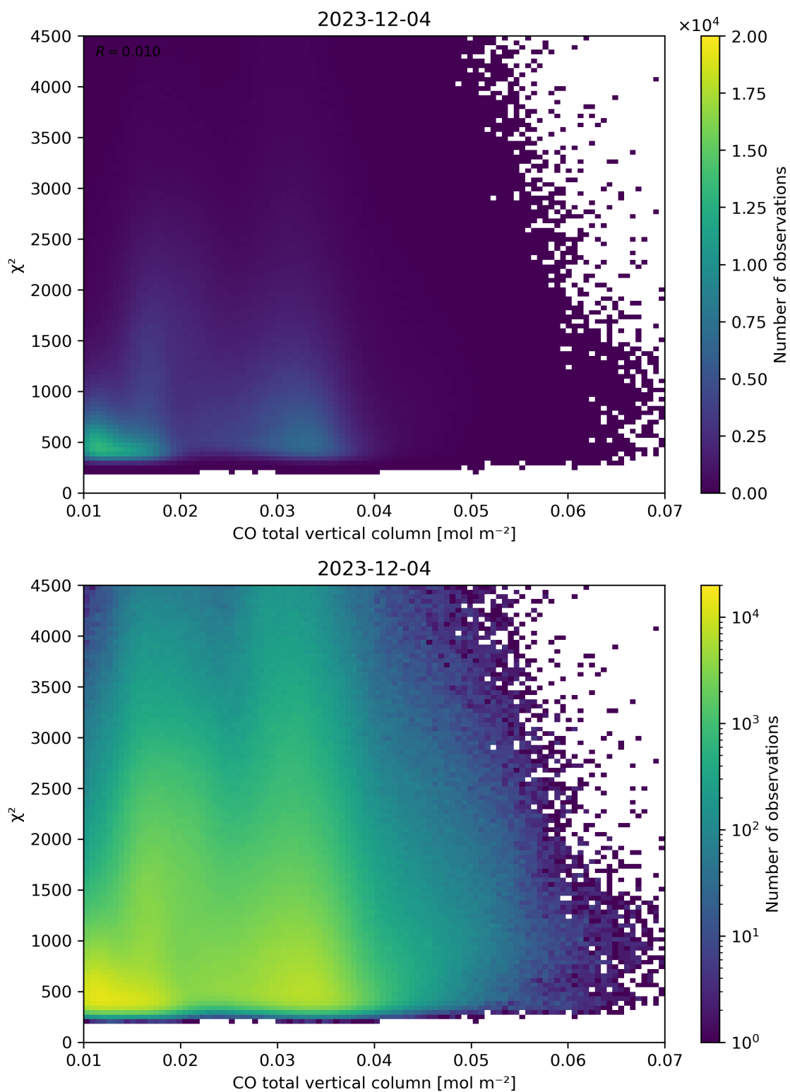
Figure 35: Scatter density plot of “CO total vertical column” against “ \chi^2 ” for 2023-12-04 to 2023-12-05.
