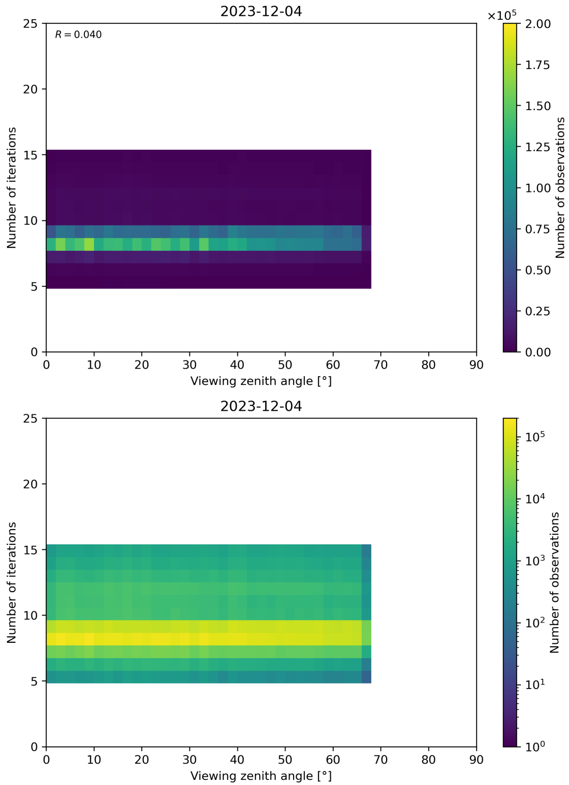
Figure 75: Scatter density plot of “Viewing zenith angle” against “Number of iterations” for 2023-12-04 to 2023-12-05.
