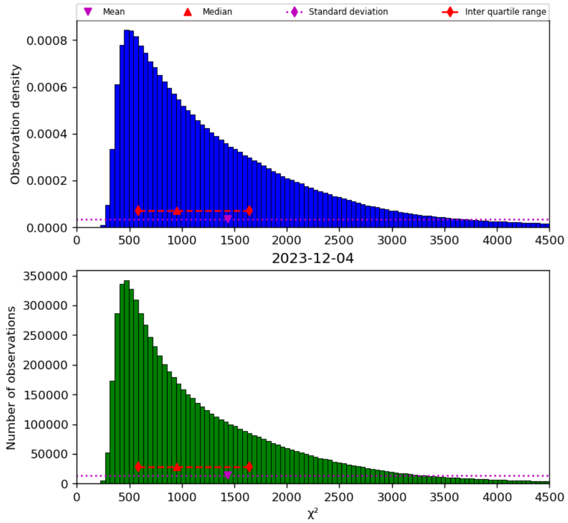
Figure 22: Histogram of “ \chi^2 ” for 2023-12-04 to 2023-12-05
