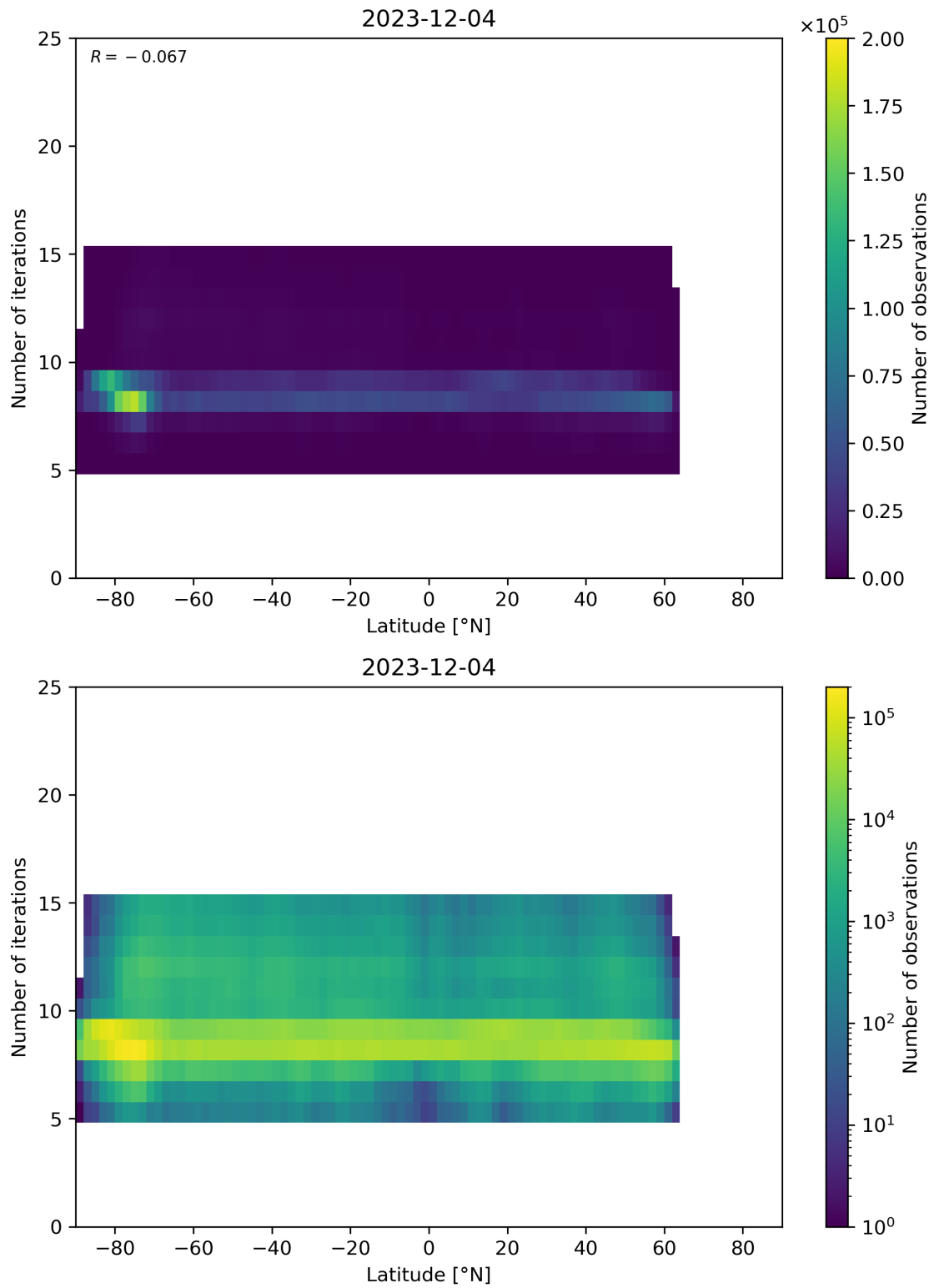
Figure 56: Scatter density plot of “Latitude” against “Number of iterations” for 2023-12-04 to 2023-12-05.
