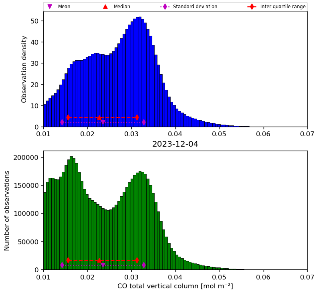
Figure 18: Histogram of “CO total vertical column” for 2023-12-04 to 2023-12-05
