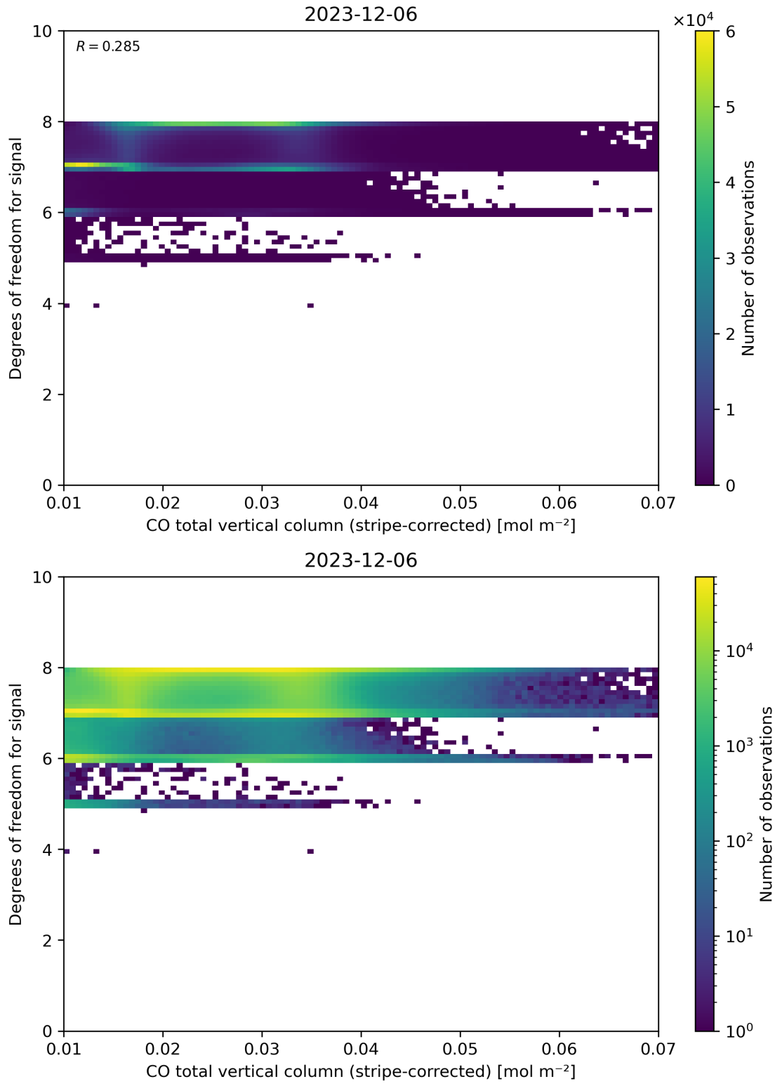
Figure 38: Scatter density plot of “CO total vertical column (stripe-corrected)” against “Degrees of freedom for signal” for 2023-12-05 to 2023-12-07.
