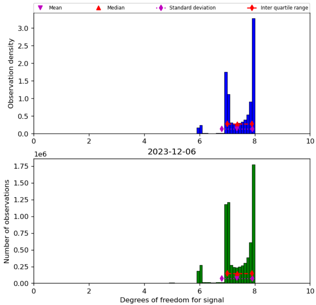
Figure 23: Histogram of “Degrees of freedom for signal” for 2023-12-05 to 2023-12-07
