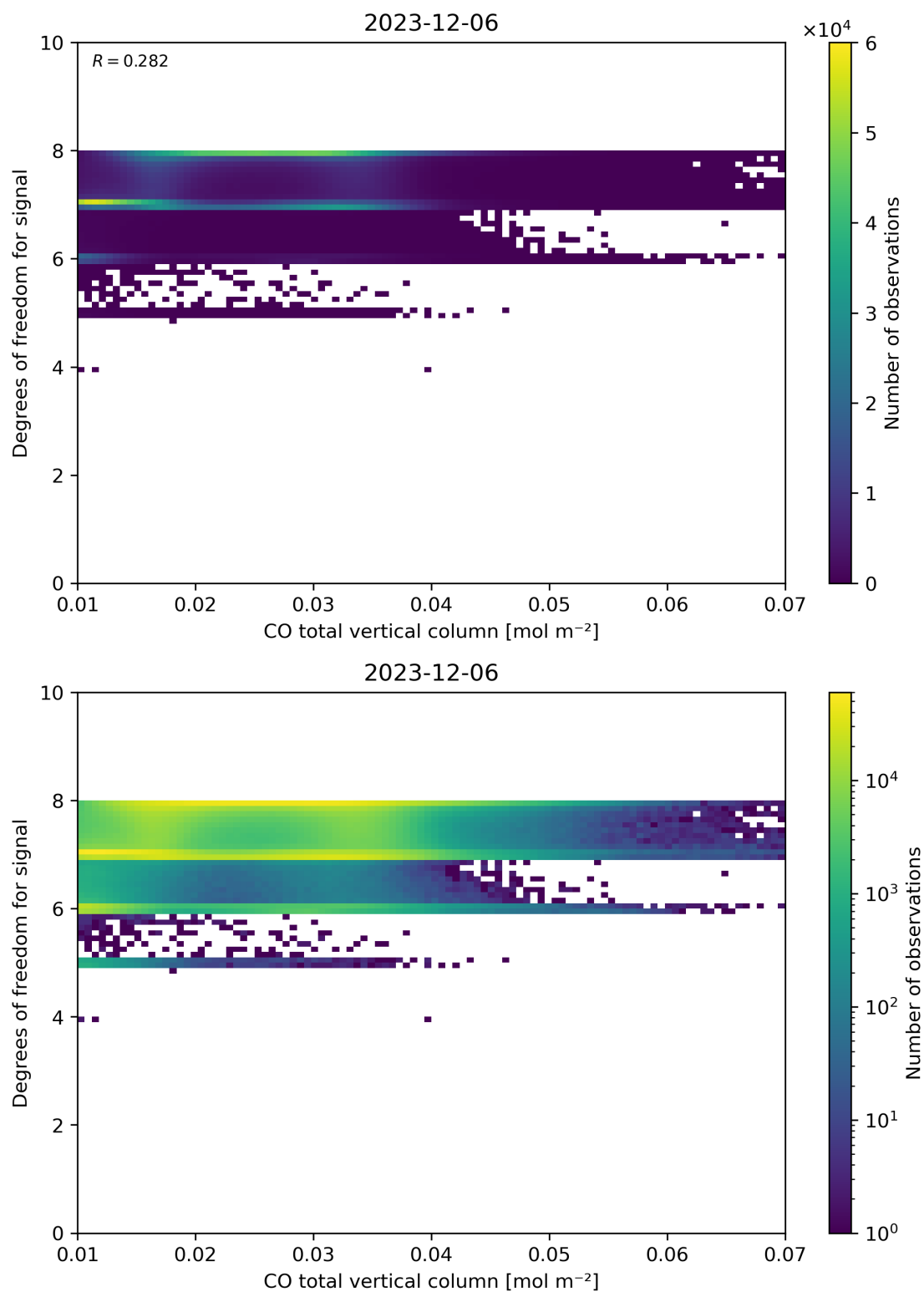
Figure 41: Scatter density plot of “CO total vertical column” against “Degrees of freedom for signal” for 2023-12-05 to 2023-12-07.
