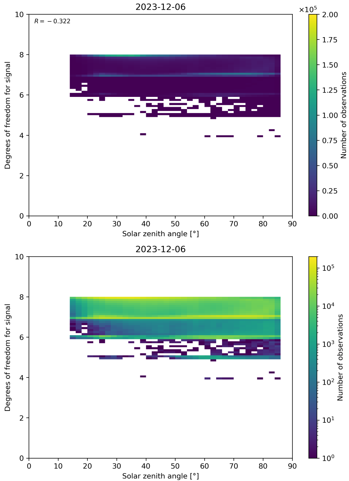
Figure 65: Scatter density plot of “Solar zenith angle” against “Degrees of freedom for signal” for 2023-12-05 to 2023-12-07.
