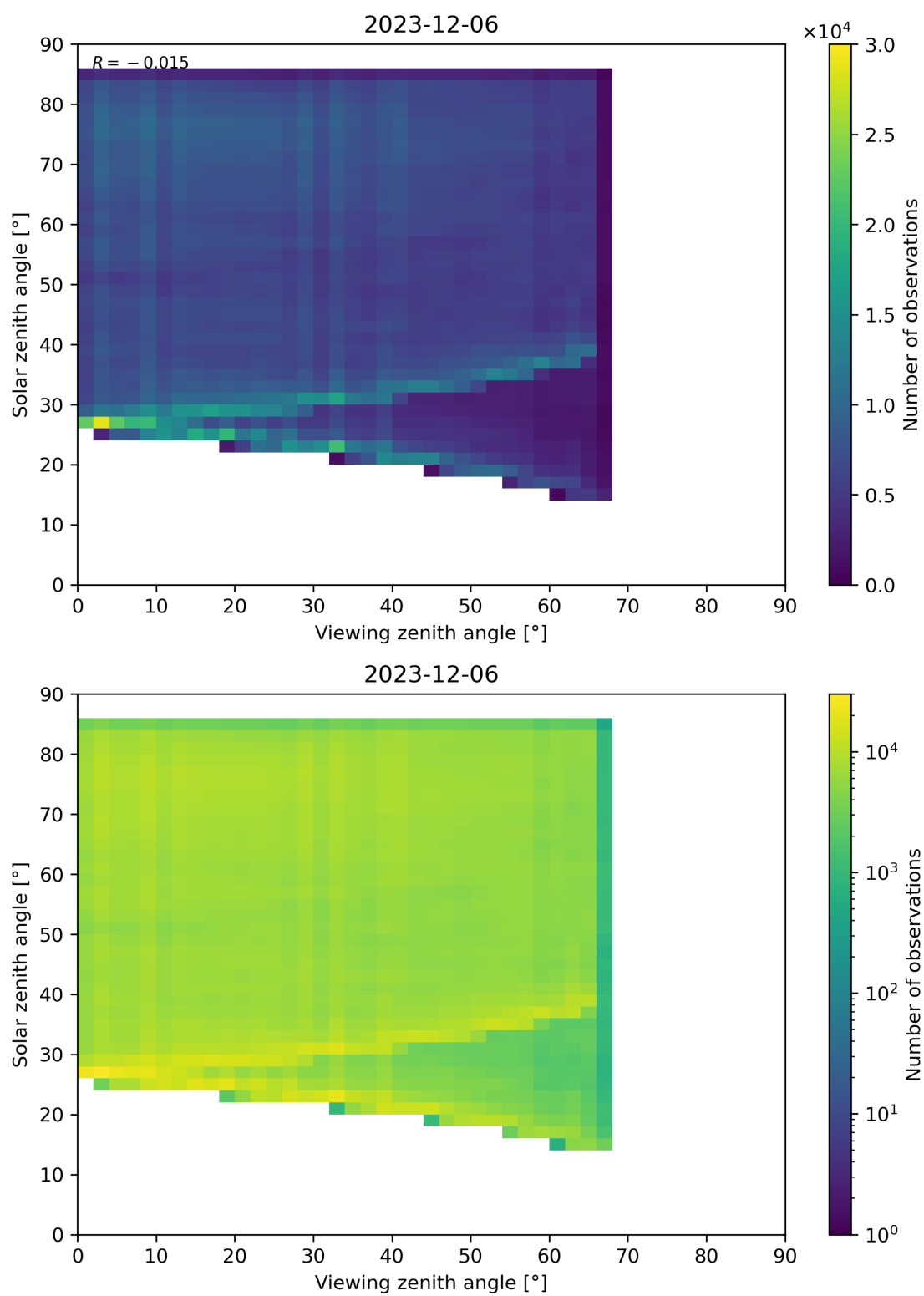
Figure 77: Scatter density plot of “Viewing zenith angle” against “Solar zenith angle” for 2023-12-05 to 2023-12-07.
