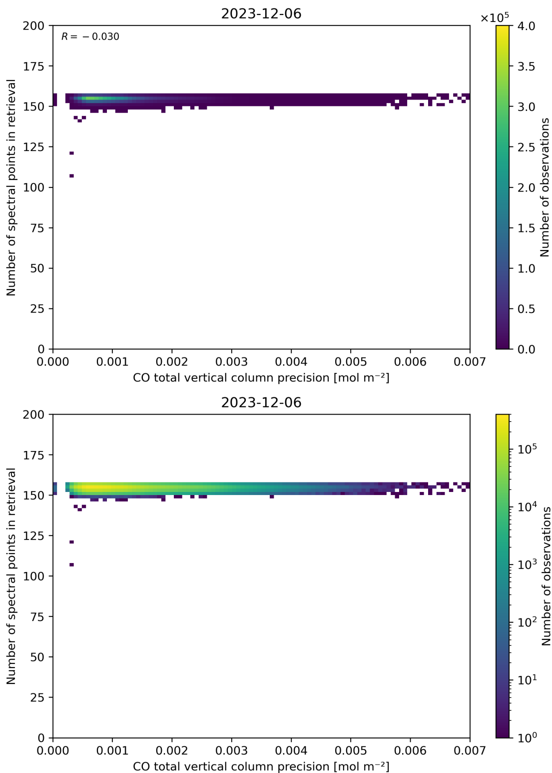
Figure 47: Scatter density plot of “CO total vertical column precision” against “Number of spectral points in retrieval” for 2023-12-05 to 2023-12-07.
