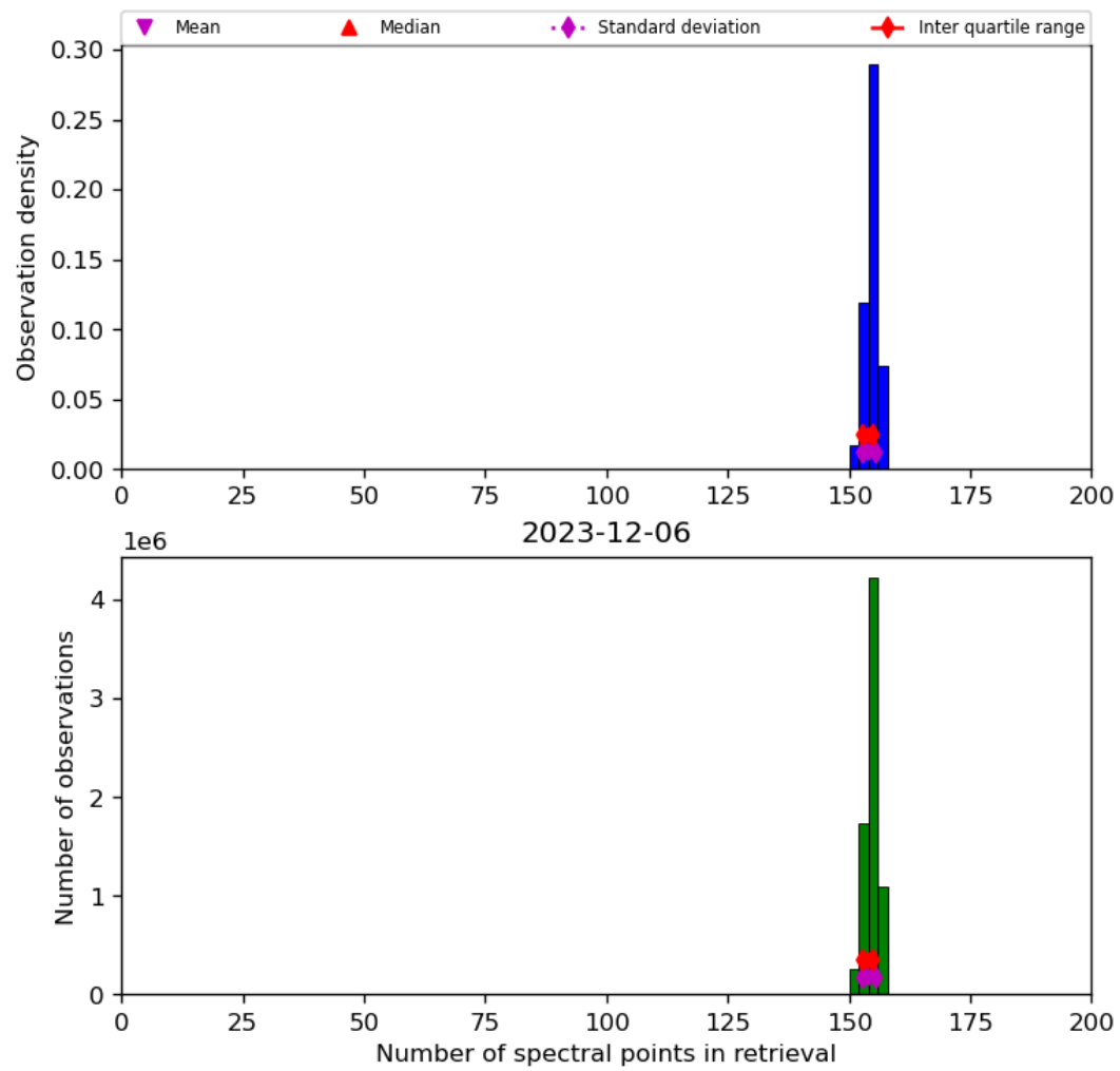
Figure 21: Histogram of “Number of spectral points in retrieval” for 2023-12-05 to 2023-12-07
