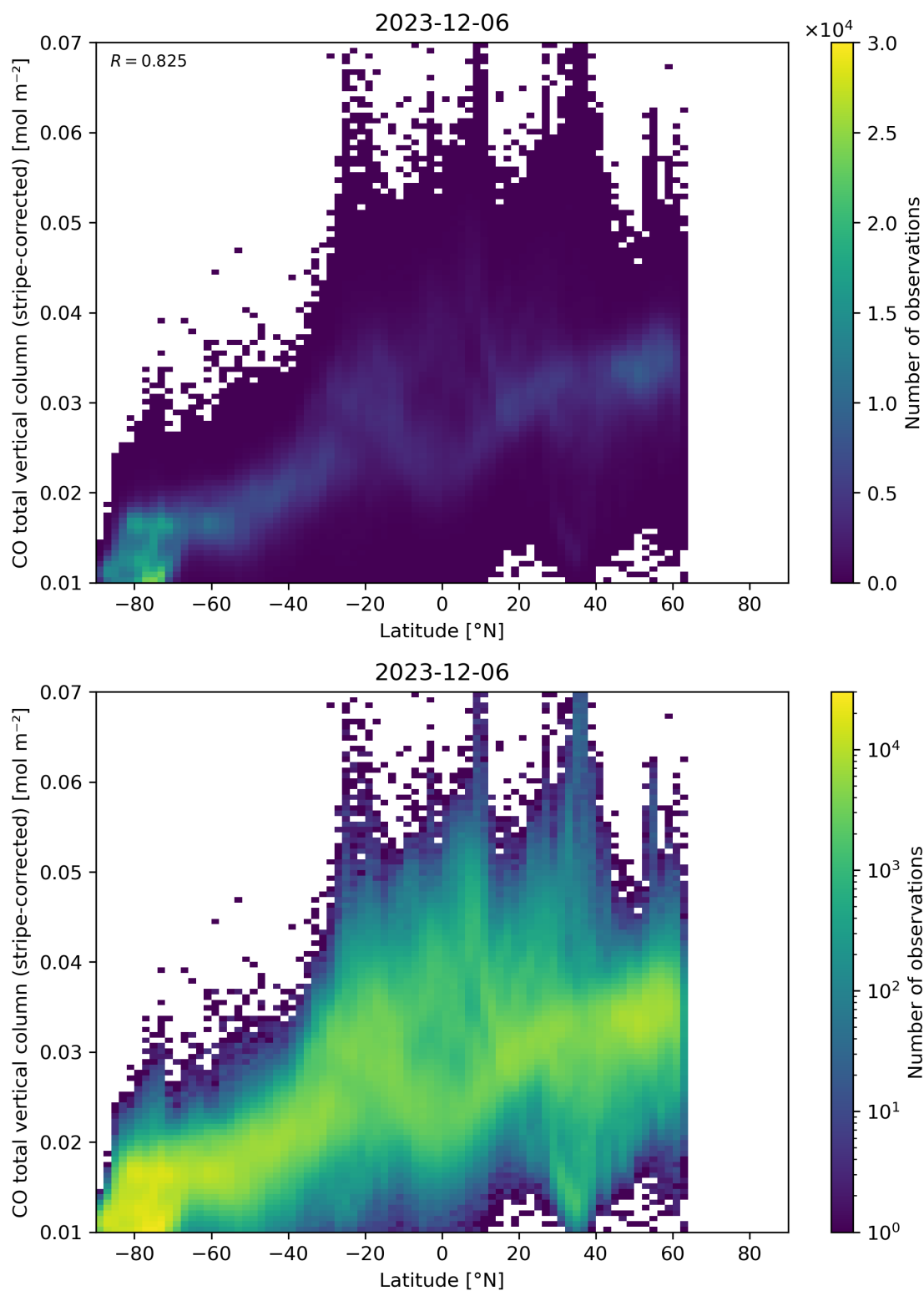
Figure 52: Scatter density plot of “Latitude” against “CO total vertical column (stripe-corrected)” for 2023-12-05 to 2023-12-07.
