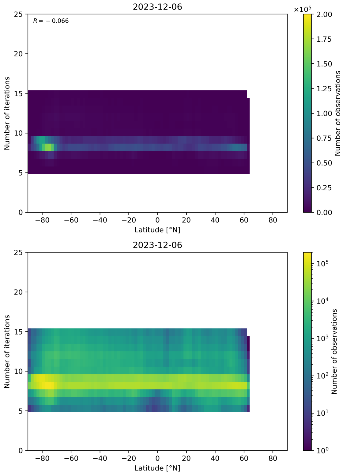
Figure 56: Scatter density plot of “Latitude” against “Number of iterations” for 2023-12-05 to 2023-12-07.
