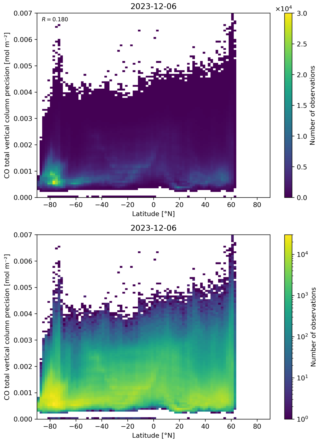
Figure 53: Scatter density plot of “Latitude” against “CO total vertical column precision” for 2023-12-05 to 2023-12-07.
