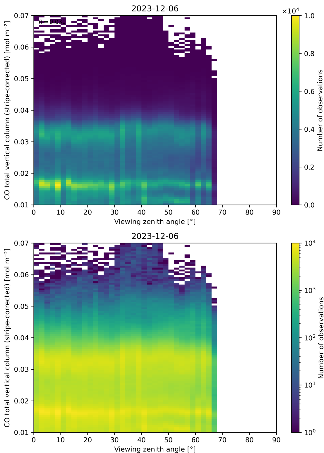
Figure 70: Scatter density plot of “Viewing zenith angle” against “CO total vertical column (stripe-corrected)” for 2023-12-05 to 2023-12-07.
