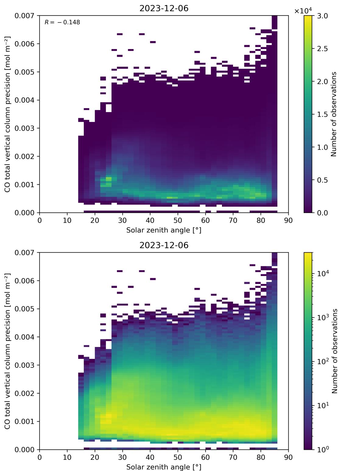
Figure 63: Scatter density plot of “Solar zenith angle” against “CO total vertical column precision” for 2023-12-05 to 2023-12-07.
