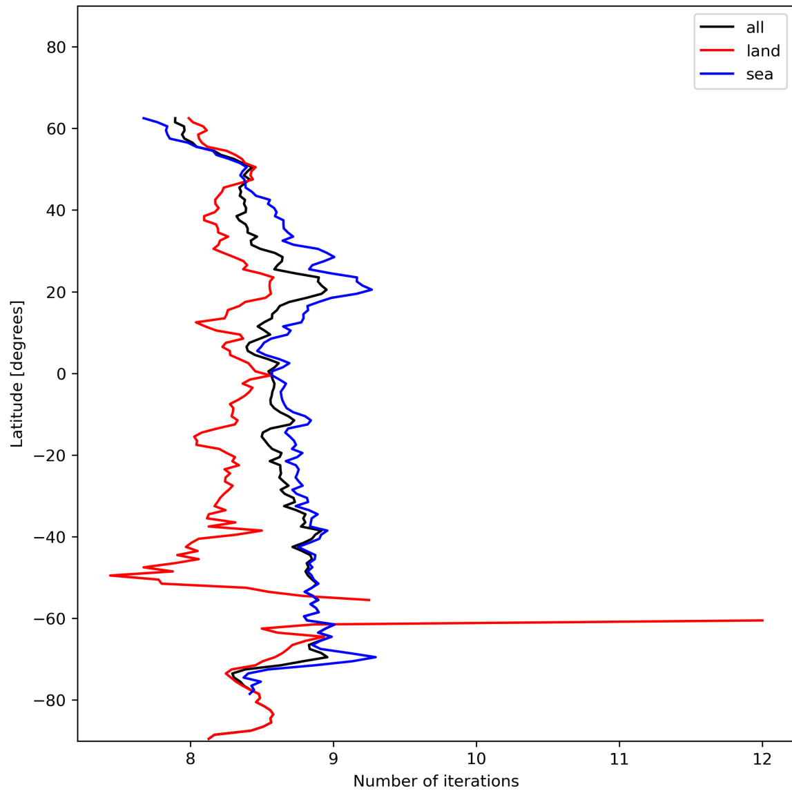
Figure 16: Zonal average of “Number of iterations” for 2023-12-05 to 2023-12-07.
