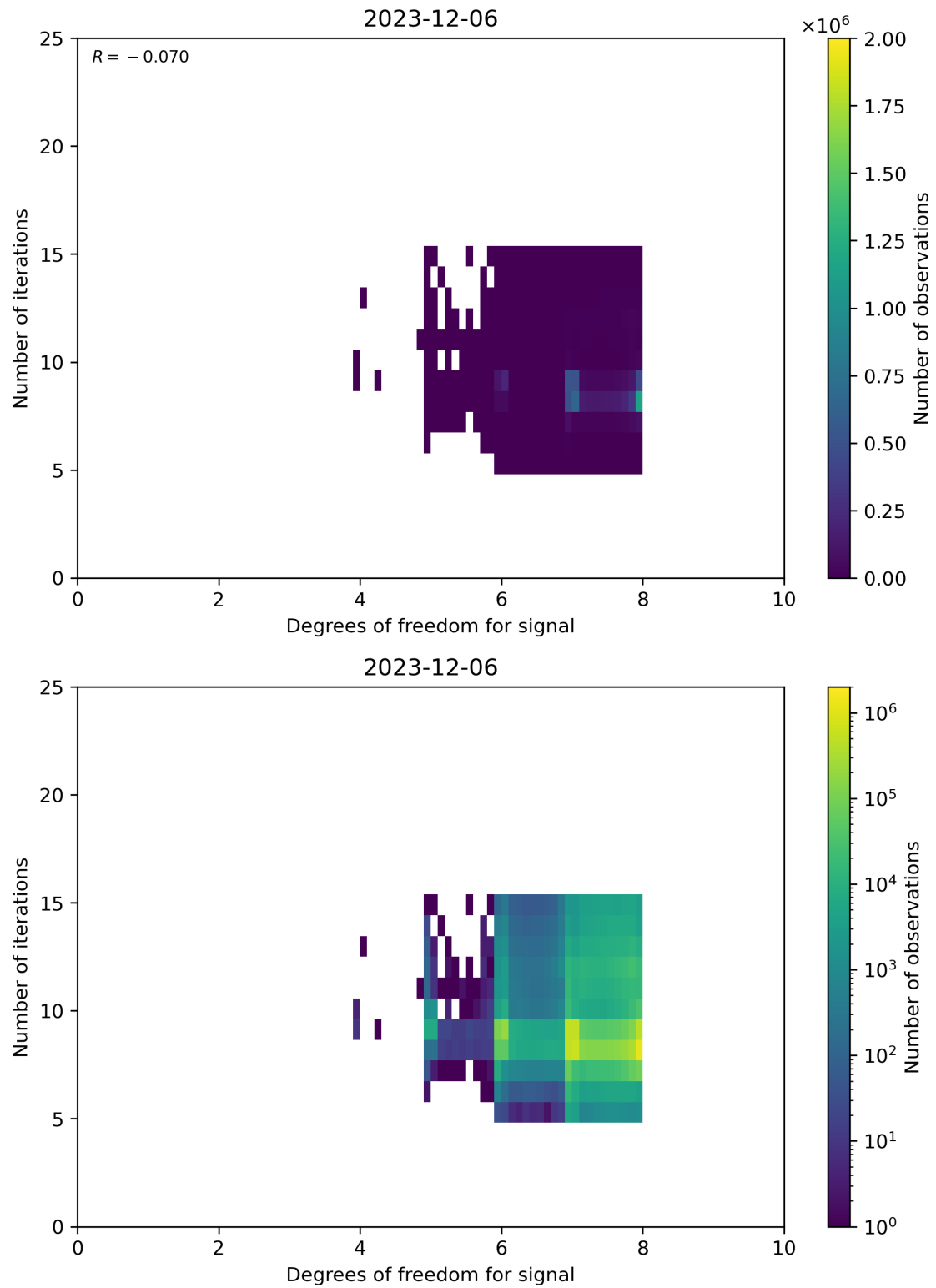
Figure 50: Scatter density plot of “Degrees of freedom for signal” against “Number of iterations” for 2023-12-05 to 2023-12-07.
