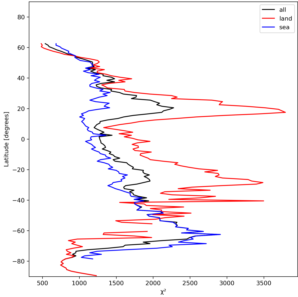
Figure 14: Zonal average of “ \chi^2 ” for 2023-12-05 to 2023-12-07.
