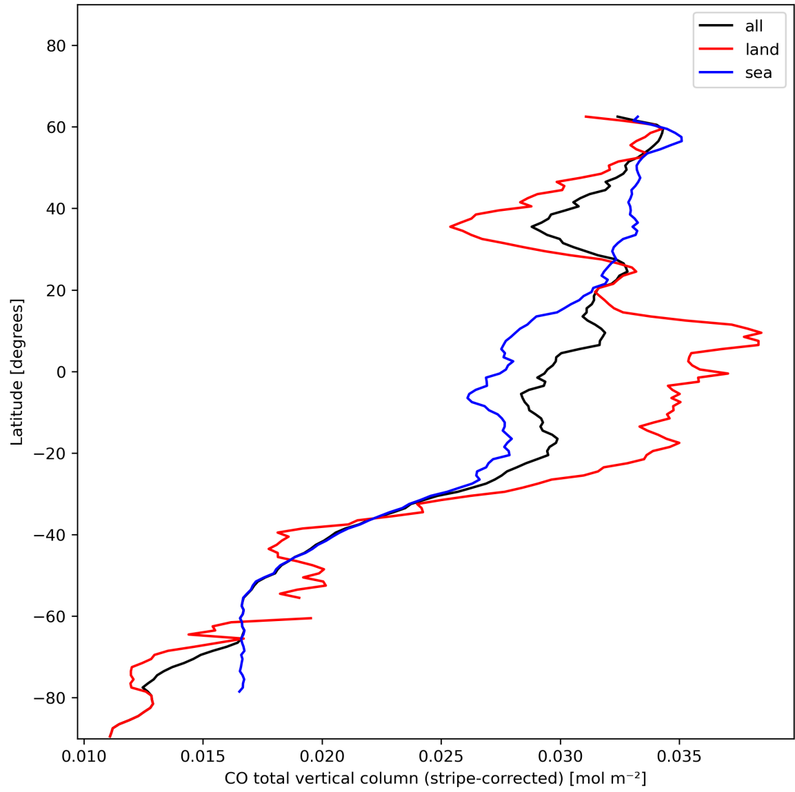
Figure 11: Zonal average of “CO total vertical column (stripe-corrected)” for 2023-12-05 to 2023-12-07.
