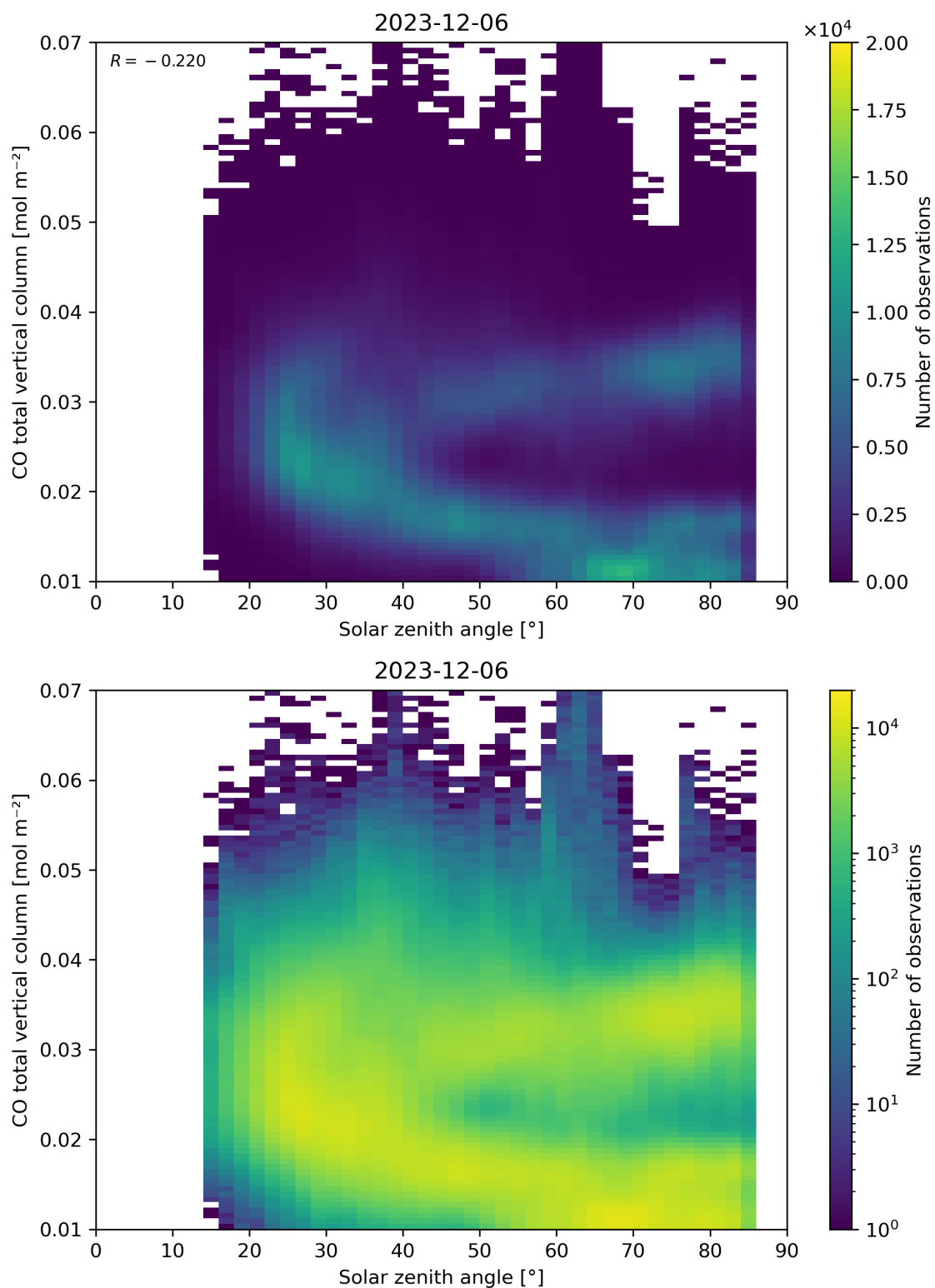
Figure 61: Scatter density plot of “Solar zenith angle” against “CO total vertical column” for 2023-12-05 to 2023-12-07.
