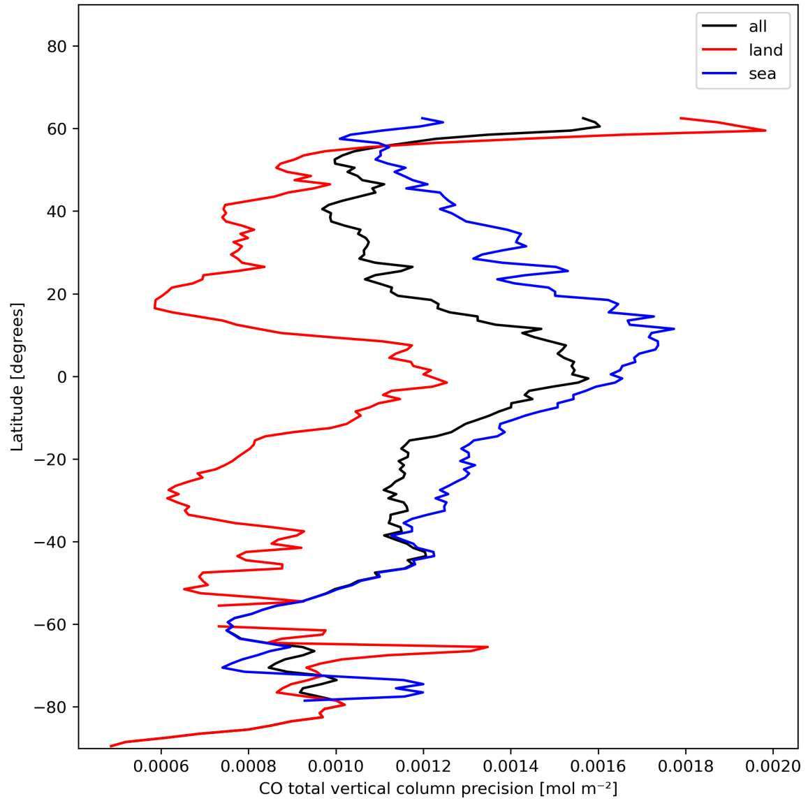
Figure 12: Zonal average of “CO total vertical column precision” for 2023-12-05 to 2023-12-07.
