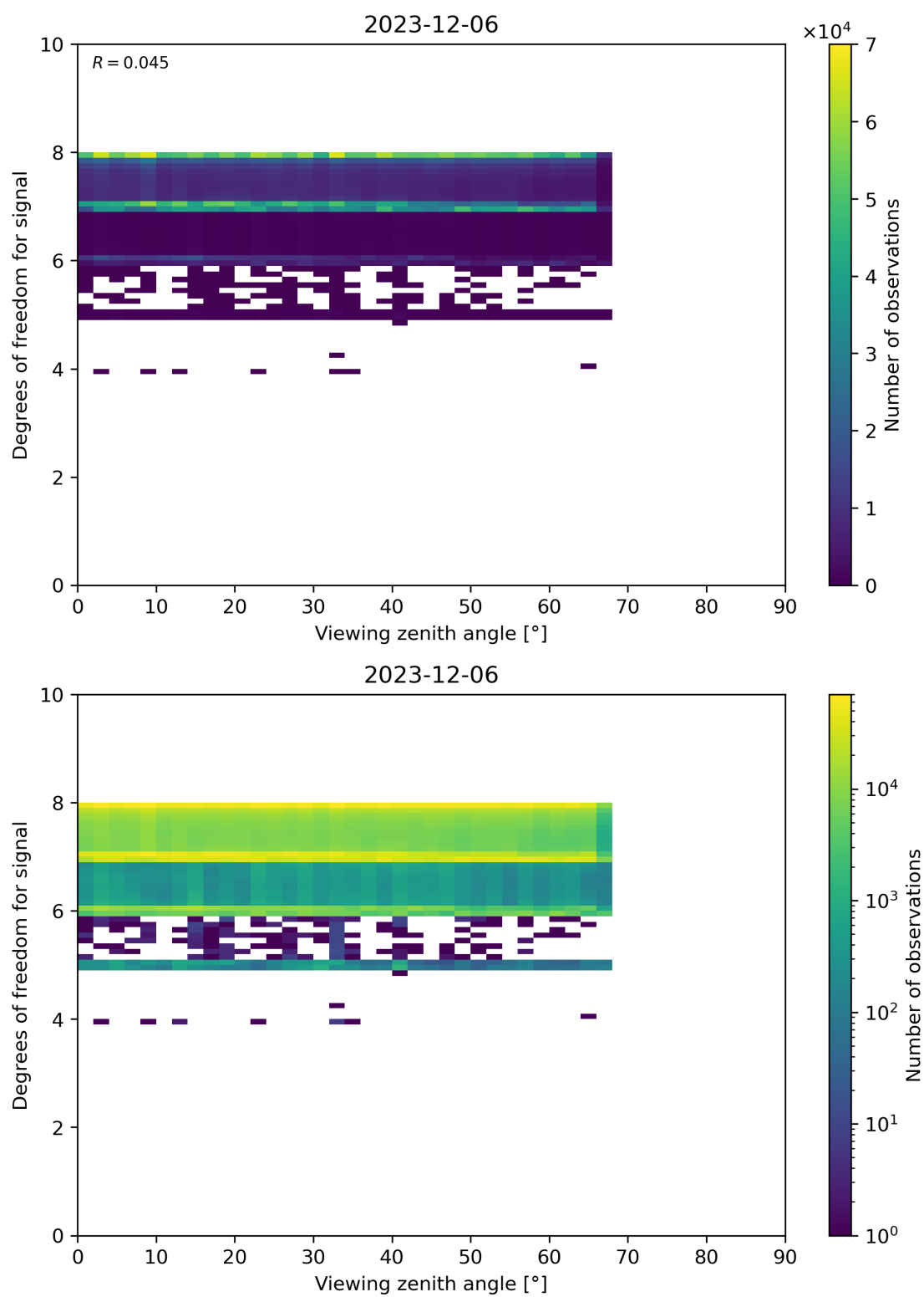
Figure 73: Scatter density plot of “Viewing zenith angle” against “Degrees of freedom for signal” for 2023-12-05 to 2023-12-07.
