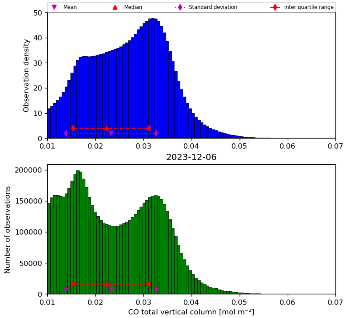
Figure 18: Histogram of “CO total vertical column” for 2023-12-05 to 2023-12-07
