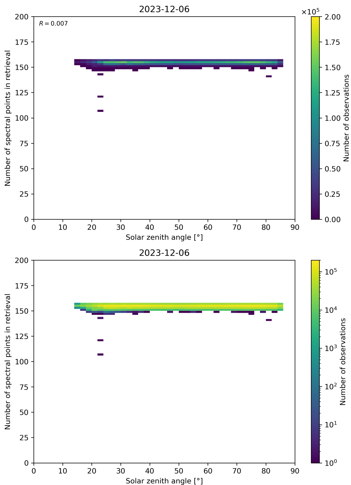
Figure 68: Scatter density plot of “Solar zenith angle” against “Number of spectral points in retrieval” for 2023-12-05 to 2023-12-07.
