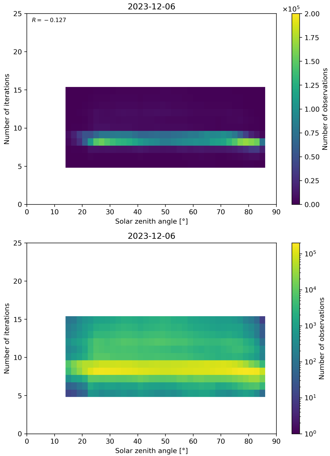
Figure 67: Scatter density plot of “Solar zenith angle” against “Number of iterations” for 2023-12-05 to 2023-12-07.
