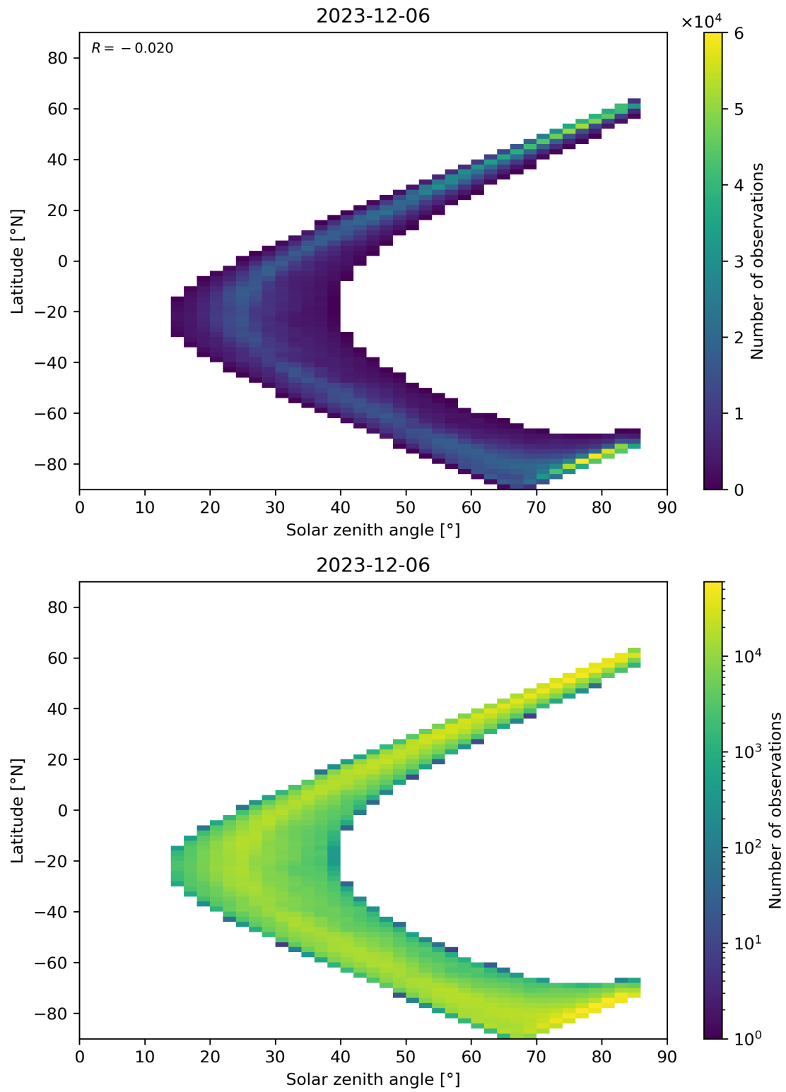
Figure 66: Scatter density plot of “Solar zenith angle” against “Latitude” for 2023-12-05 to 2023-12-07.
