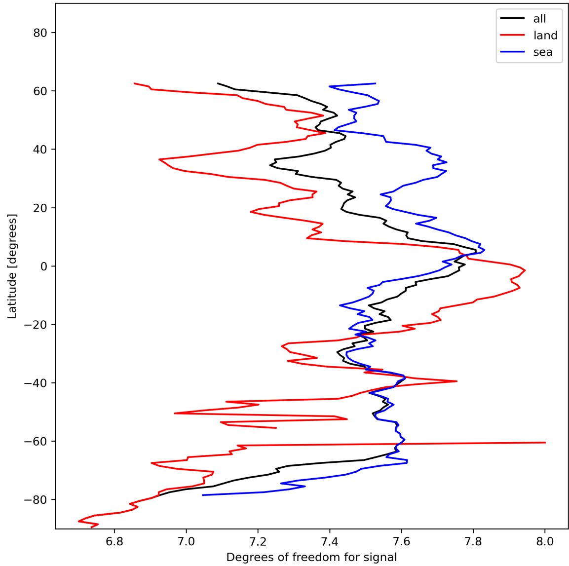
Figure 15: Zonal average of “Degrees of freedom for signal” for 2023-12-05 to 2023-12-07.
