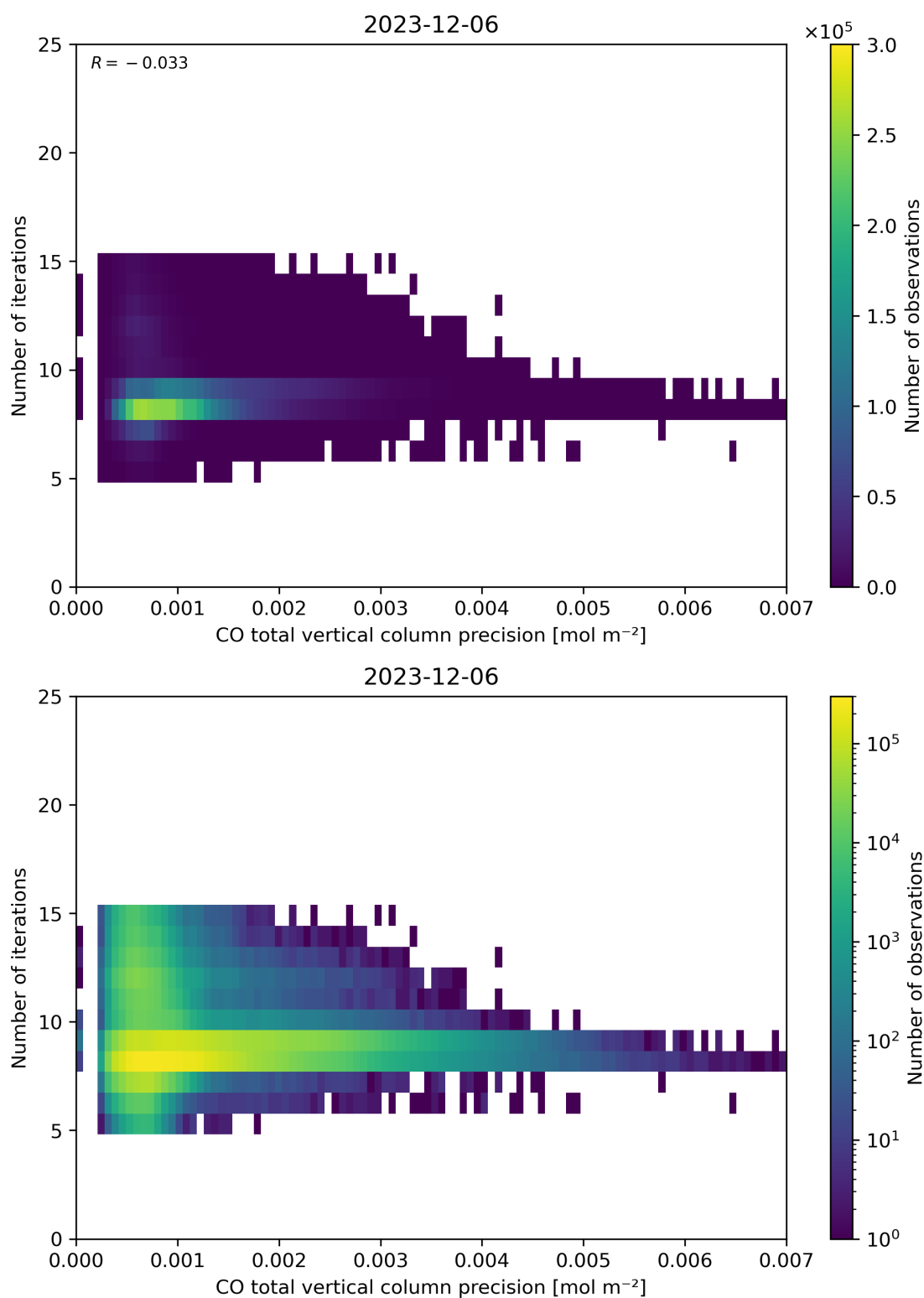
Figure 46: Scatter density plot of “CO total vertical column precision” against “Number of iterations” for 2023-12-05 to 2023-12-07.
