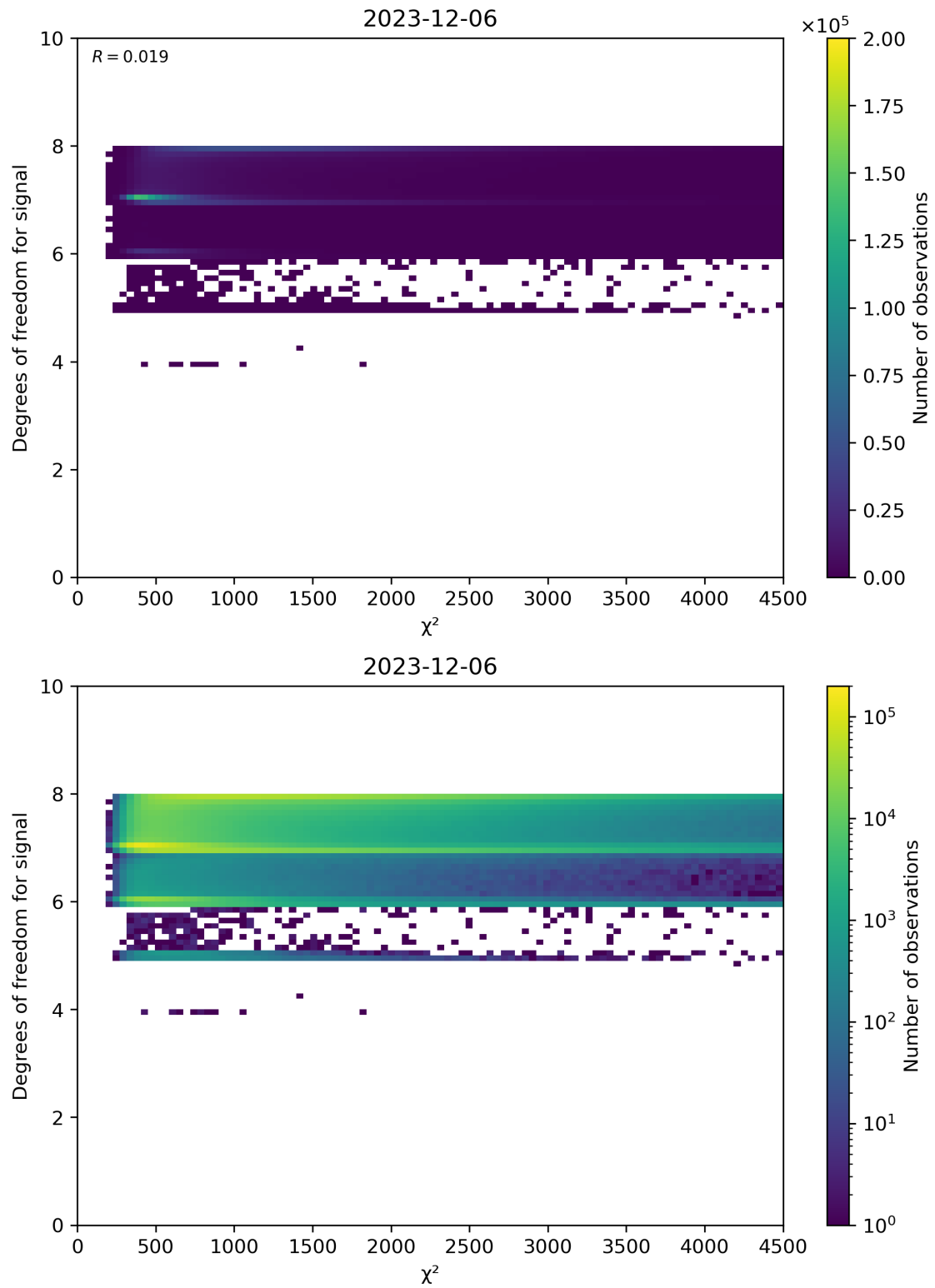
Figure 48: Scatter density plot of “ \chi^2 ” against “Degrees of freedom for signal” for 2023-12-05 to 2023-12-07.
