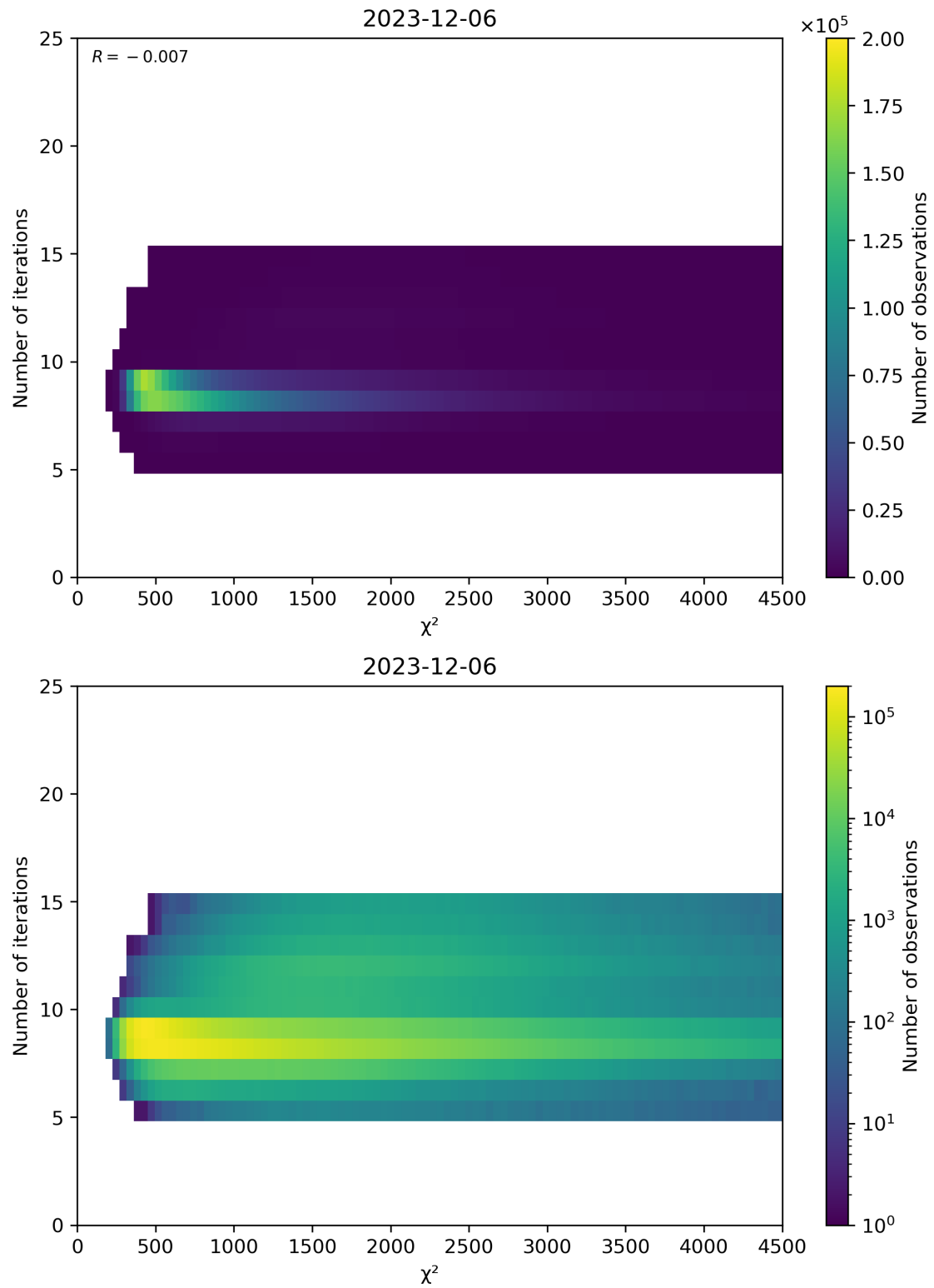
Figure 49: Scatter density plot of “ \chi^2 ” against “Number of iterations” for 2023-12-05 to 2023-12-07.
