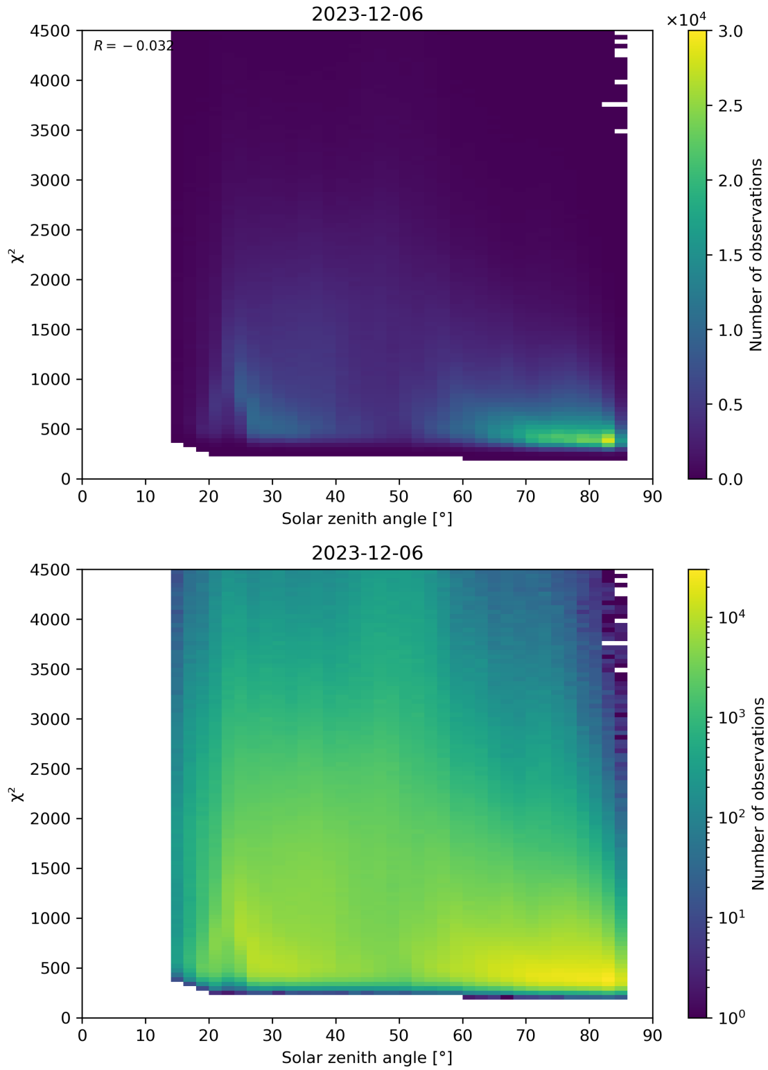
Figure 64: Scatter density plot of “Solar zenith angle” against “ \chi^2 ” for 2023-12-05 to 2023-12-07.
