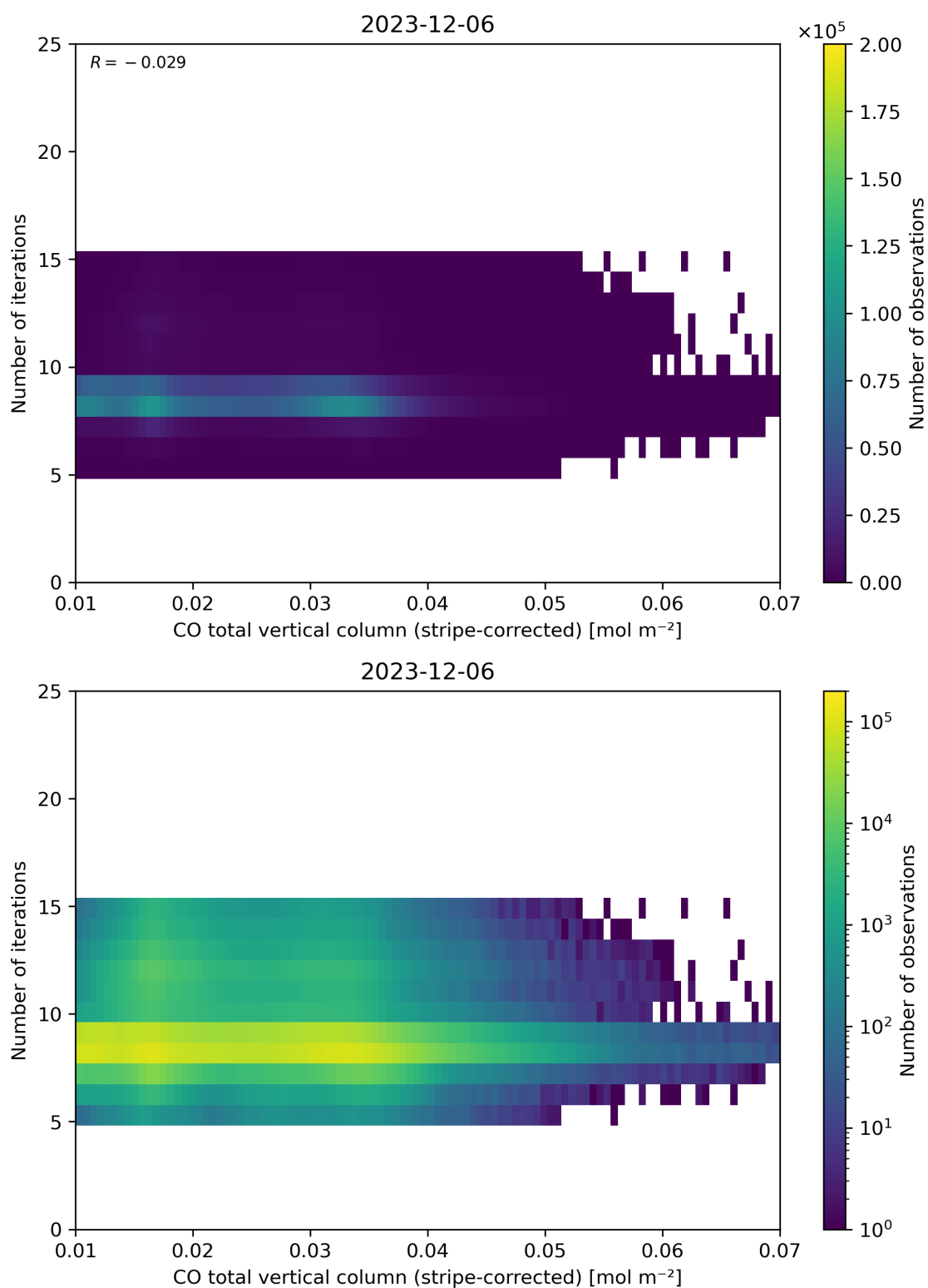
Figure 39: Scatter density plot of “CO total vertical column (stripe-corrected)” against “Number of iterations” for 2023-12-05 to 2023-12-07.
