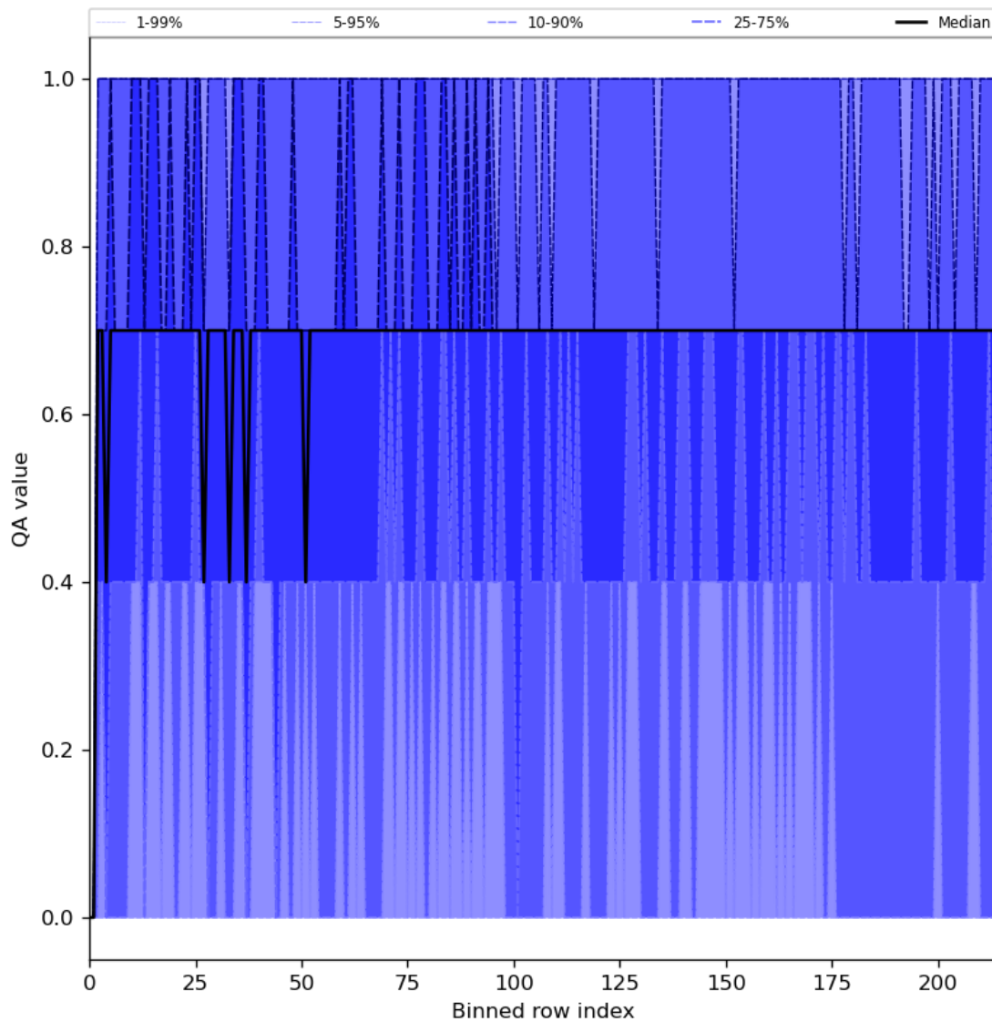
Figure 25: Along track statistics of “QA value” for 2023-12-05 to 2023-12-07
