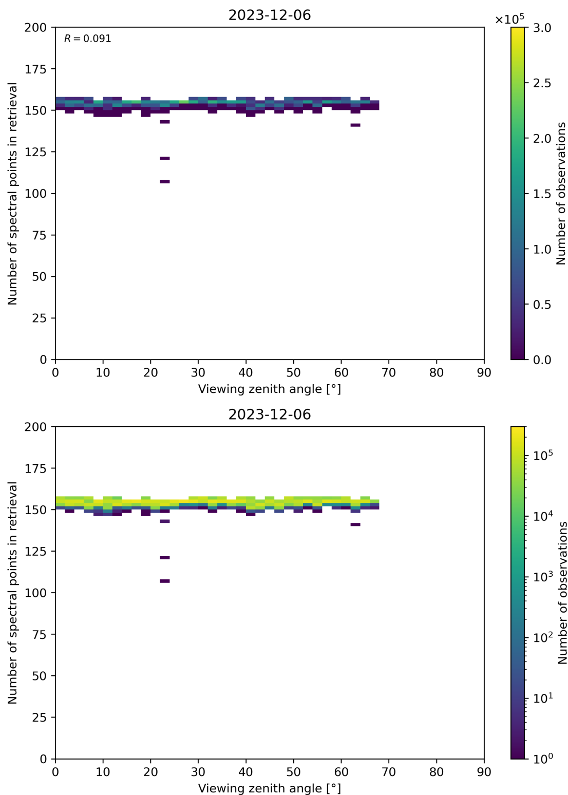
Figure 76: Scatter density plot of “Viewing zenith angle” against “Number of spectral points in retrieval” for 2023-12-05 to 2023-12-07.
