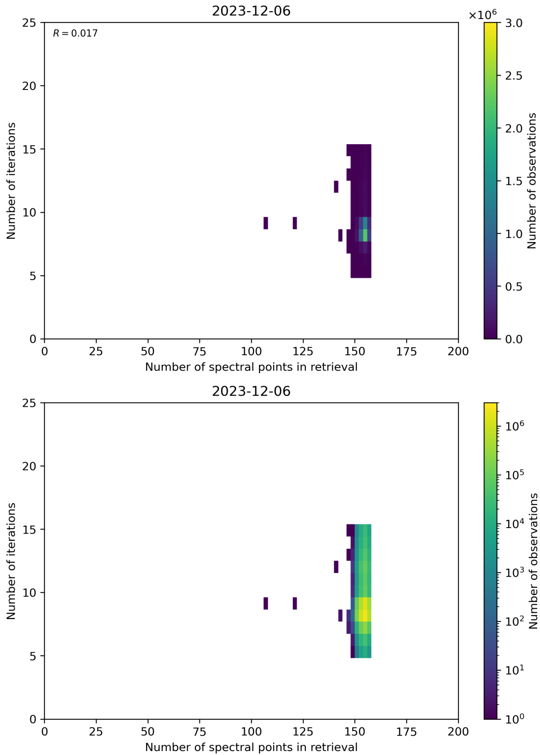
Figure 60: Scatter density plot of “Number of spectral points in retrieval” against “Number of iterations” for 2023-12-05 to 2023-12-07.
