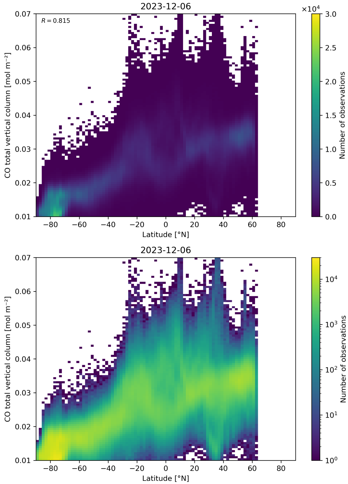
Figure 51: Scatter density plot of “Latitude” against “CO total vertical column” for 2023-12-05 to 2023-12-07.
