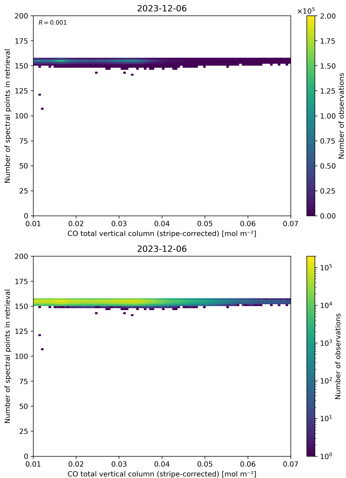
Figure 40: Scatter density plot of “CO total vertical column (stripe-corrected)” against “Number of spectral points in retrieval” for 2023-12-05 to 2023-12-07.
