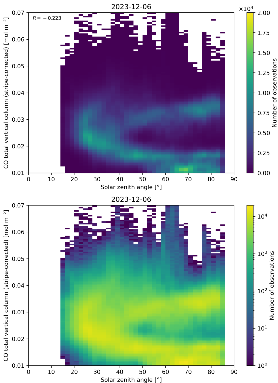
Figure 62: Scatter density plot of “Solar zenith angle” against “CO total vertical column (stripe-corrected)” for 2023-12-05 to 2023-12-07.
