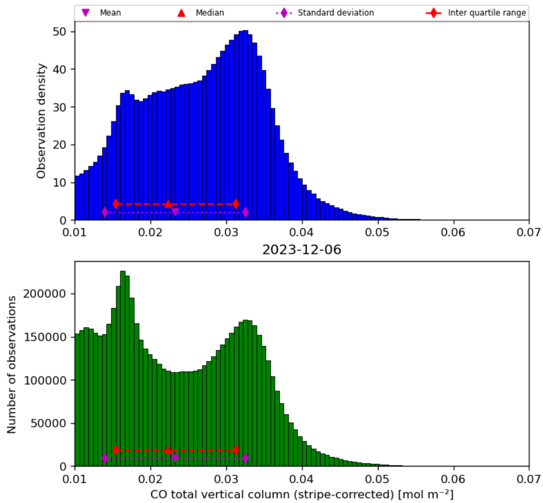
Figure 19: Histogram of “CO total vertical column (stripe-corrected)” for 2023-12-05 to 2023-12-07
