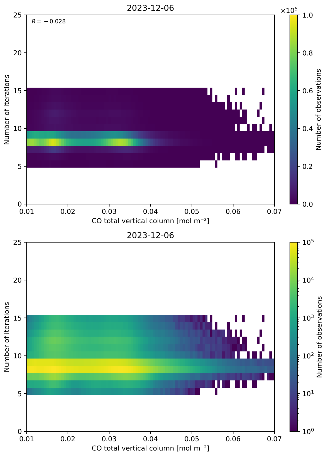
Figure 42: Scatter density plot of “CO total vertical column” against “Number of iterations” for 2023-12-05 to 2023-12-07.
