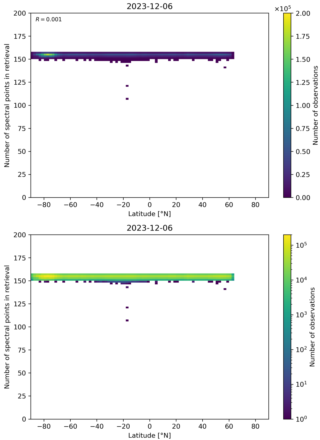
Figure 57: Scatter density plot of “Latitude” against “Number of spectral points in retrieval” for 2023-12-05 to 2023-12-07.
