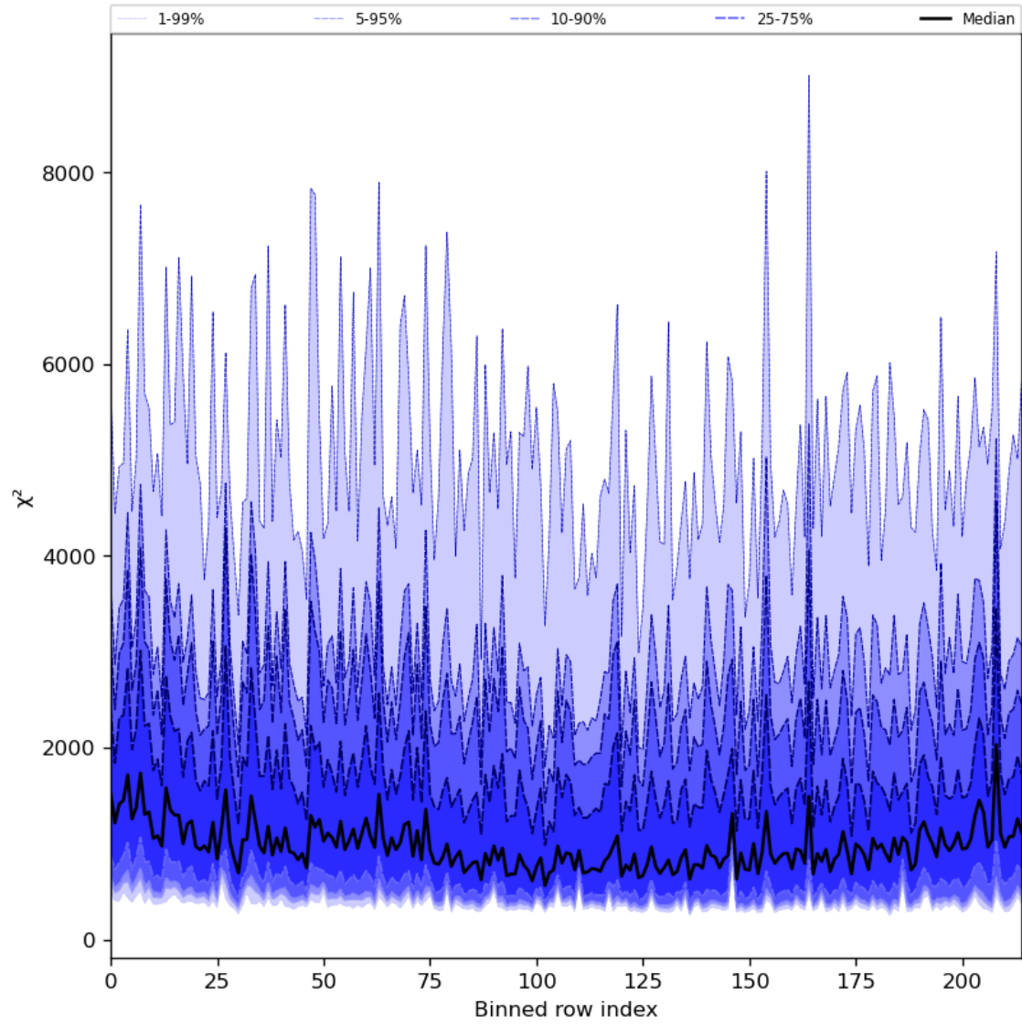
Figure 30: Along track statistics of “ \chi^2 ” for 2023-12-05 to 2023-12-07
