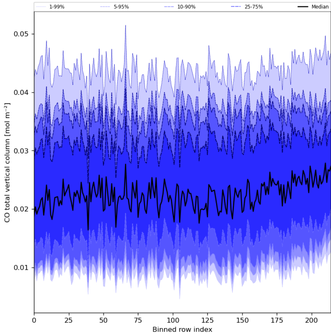
Figure 26: Along track statistics of “CO total vertical column” for 2023-12-05 to 2023-12-07
