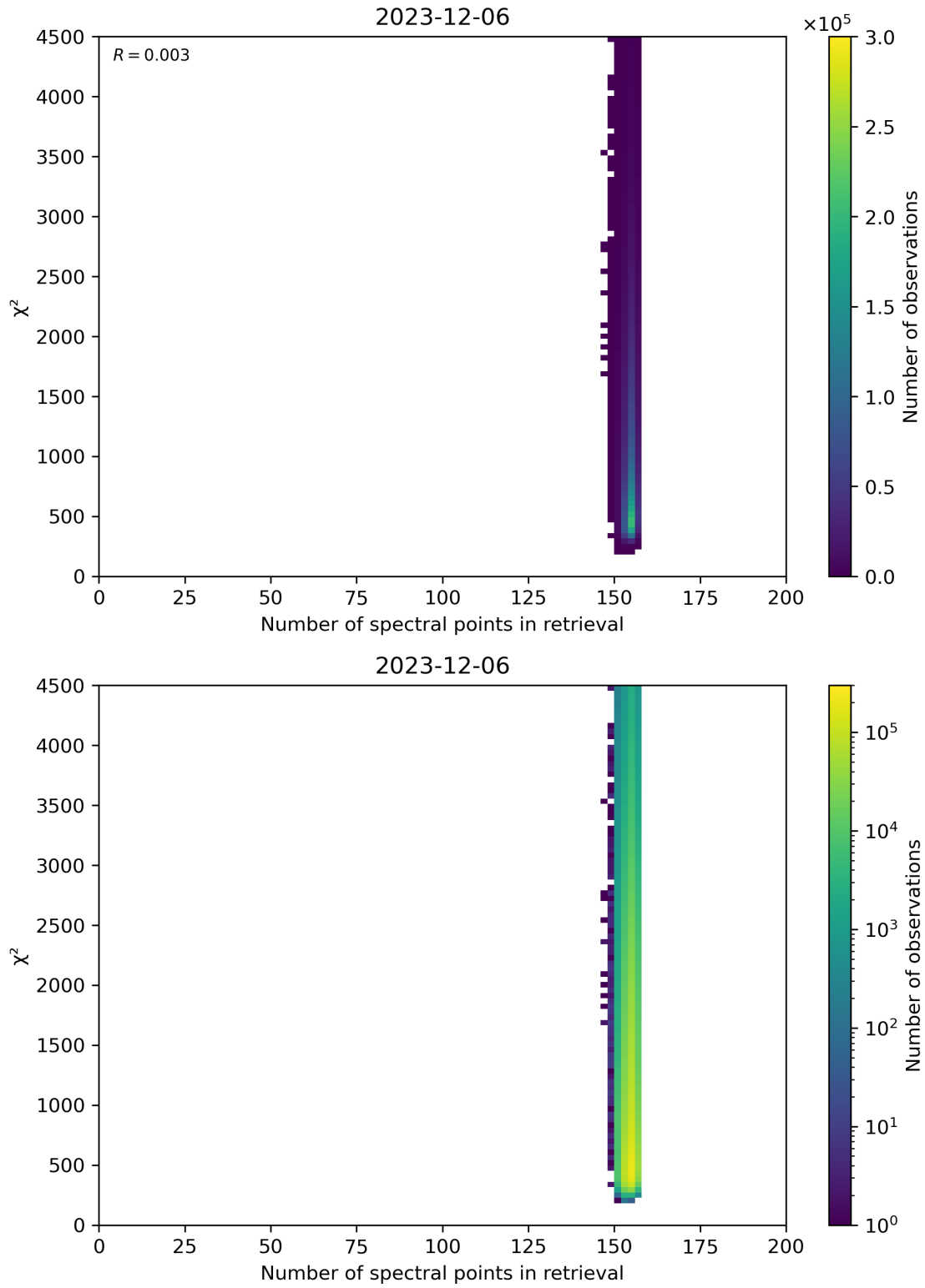
Figure 58: Scatter density plot of “Number of spectral points in retrieval” against “ \chi^2 ” for 2023-12-05 to 2023-12-07.
