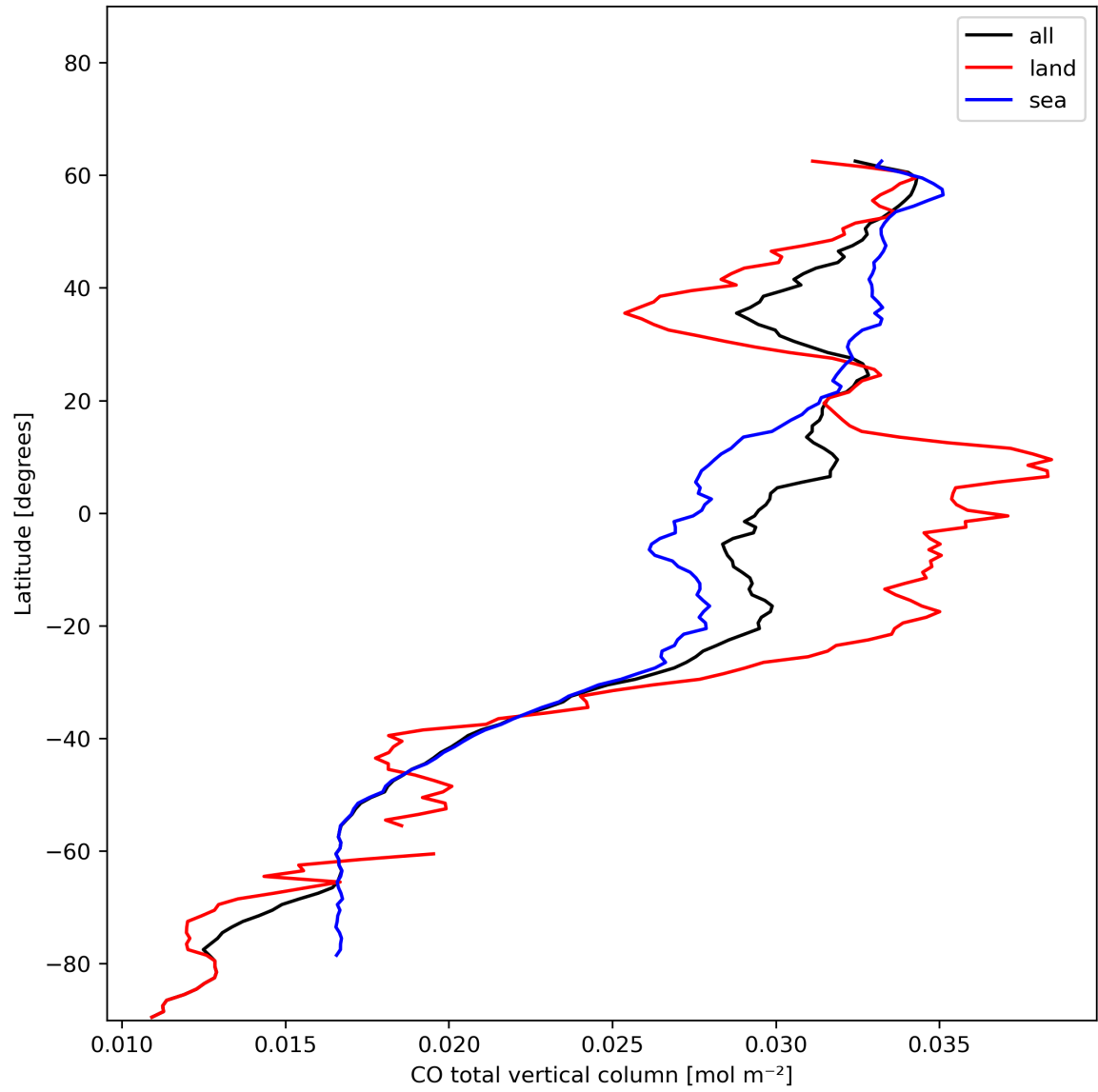
Figure 10: Zonal average of “CO total vertical column” for 2023-12-05 to 2023-12-07.
