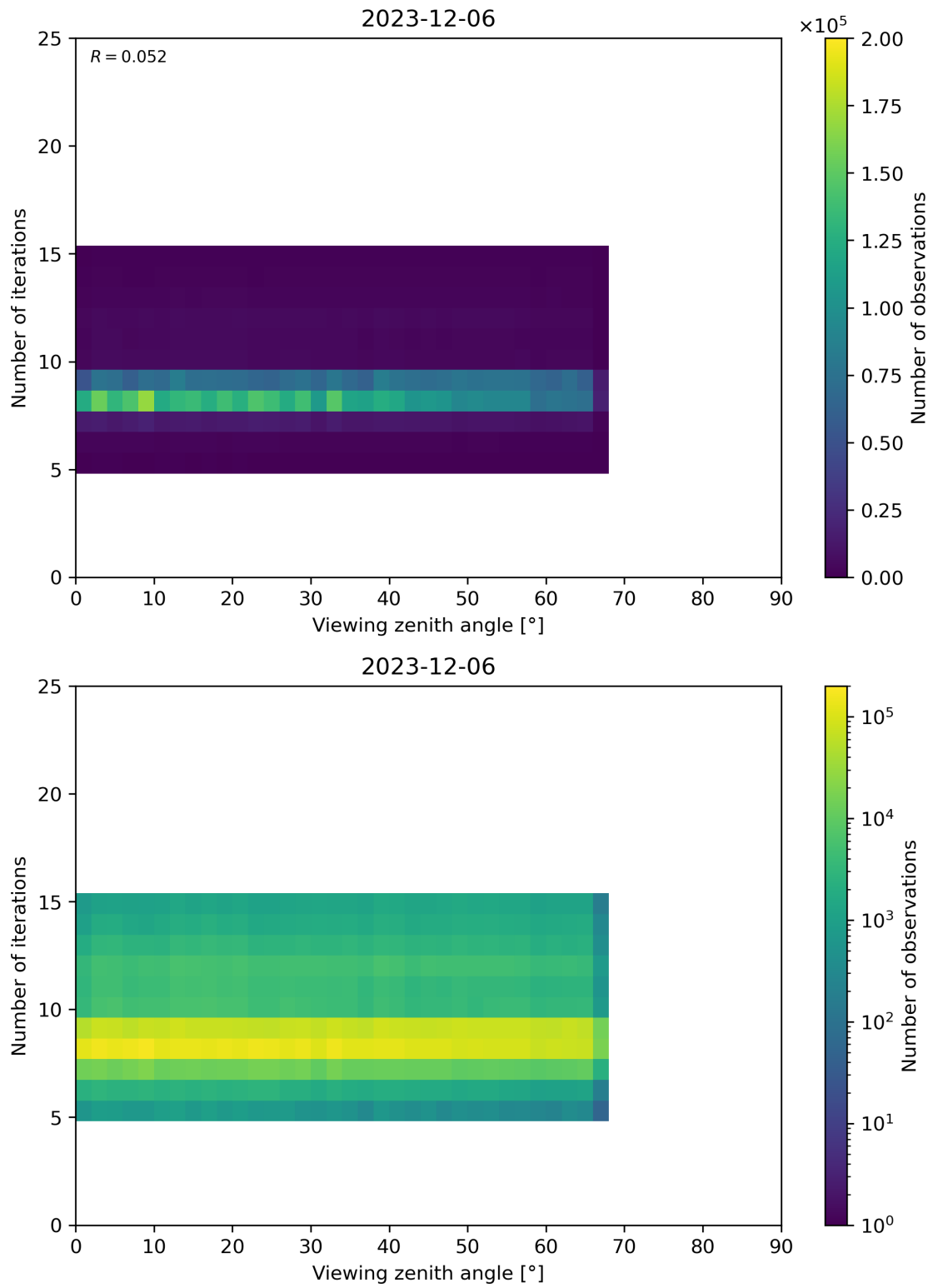
Figure 75: Scatter density plot of “Viewing zenith angle” against “Number of iterations” for 2023-12-05 to 2023-12-07.
