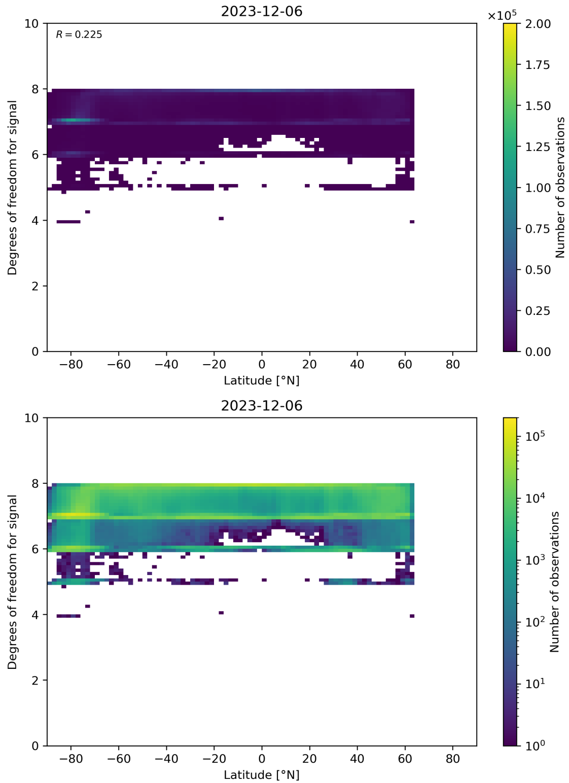
Figure 55: Scatter density plot of “Latitude” against “Degrees of freedom for signal” for 2023-12-05 to 2023-12-07.
