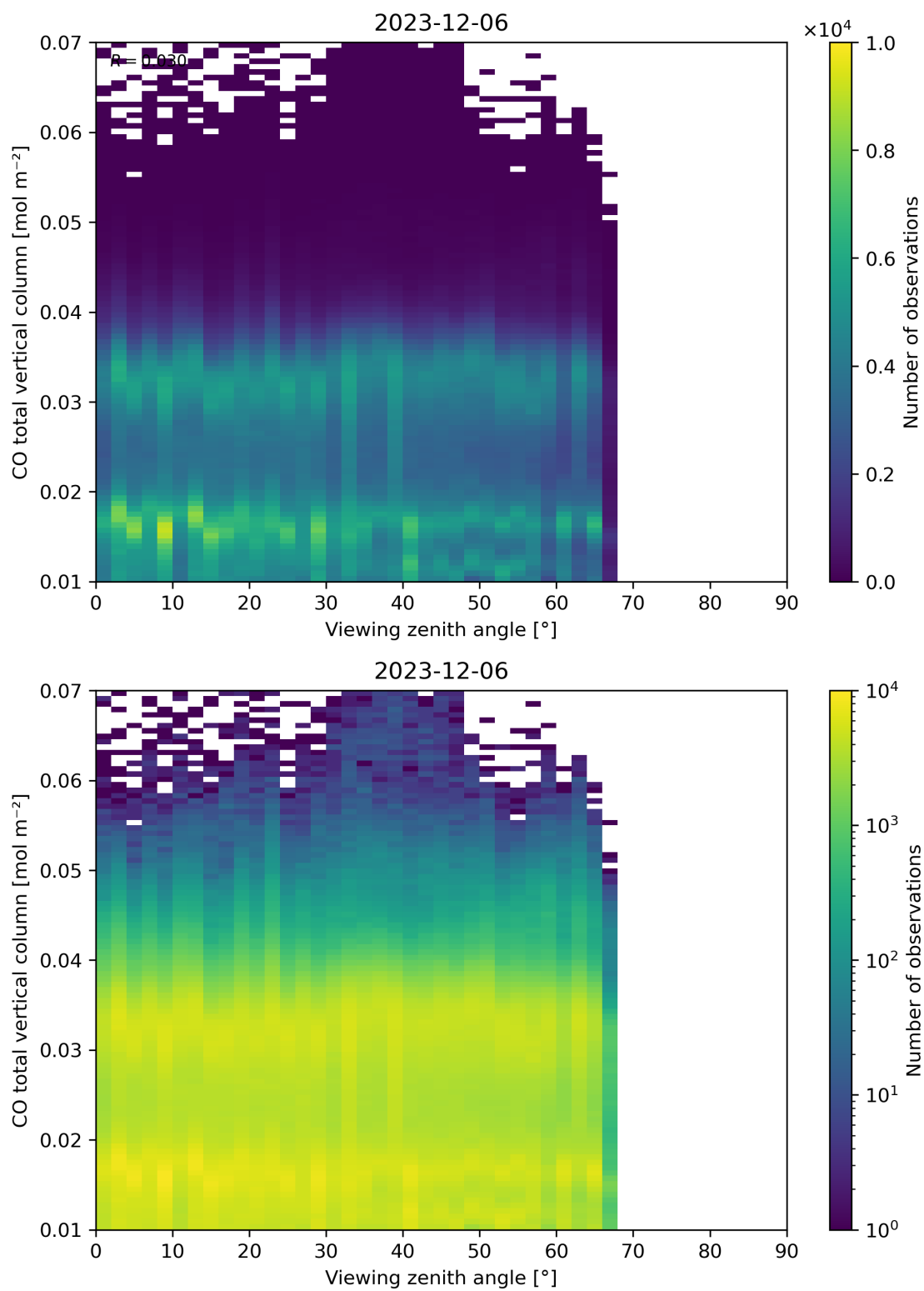
Figure 69: Scatter density plot of “Viewing zenith angle” against “CO total vertical column” for 2023-12-05 to 2023-12-07.
