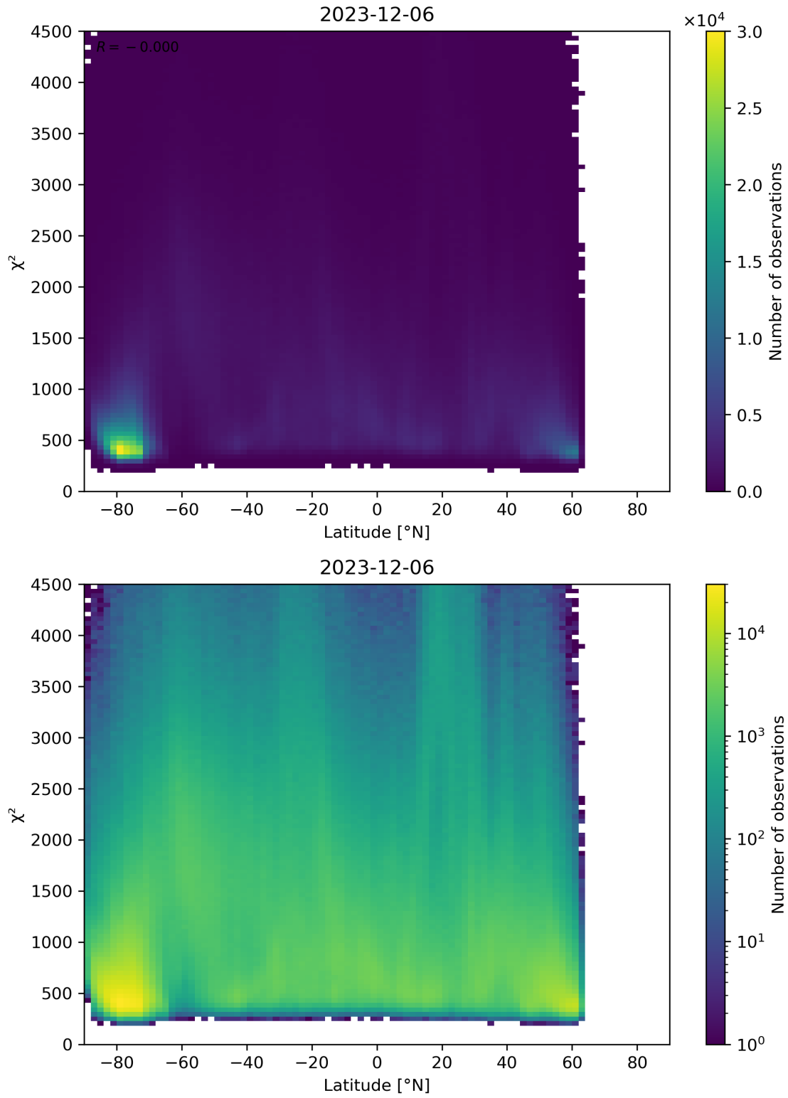
Figure 54: Scatter density plot of “Latitude” against “ \chi^2 ” for 2023-12-05 to 2023-12-07.
