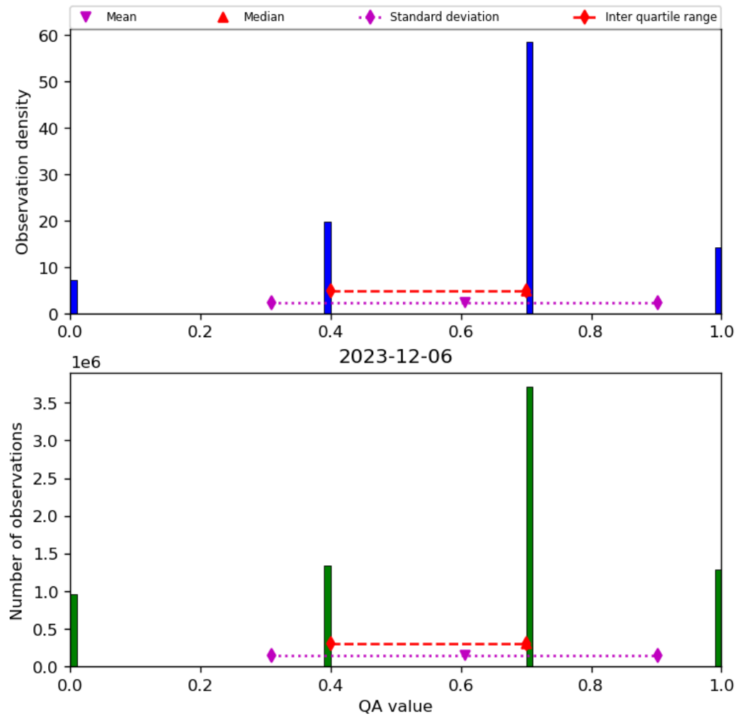
Figure 17: Histogram of “QA value” for 2023-12-05 to 2023-12-07
