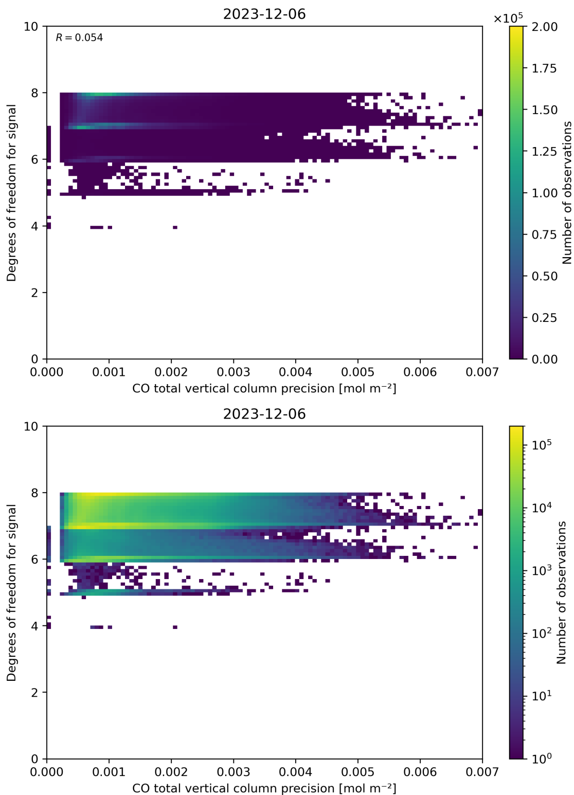
Figure 45: Scatter density plot of “CO total vertical column precision” against “Degrees of freedom for signal” for 2023-12-05 to 2023-12-07.
