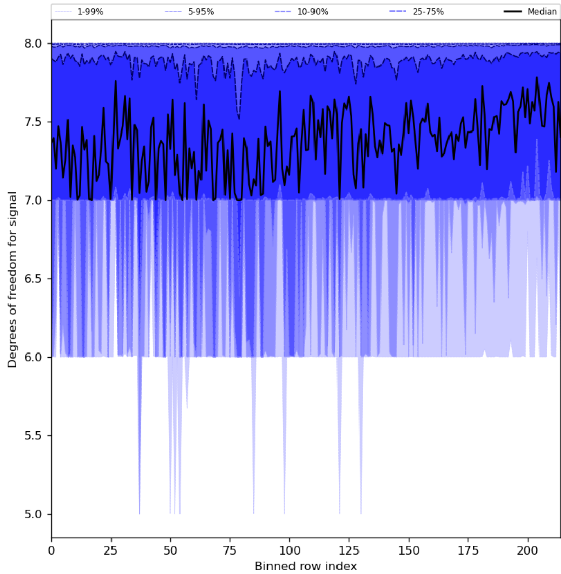
Figure 31: Along track statistics of “Degrees of freedom for signal” for 2023-12-05 to 2023-12-07
