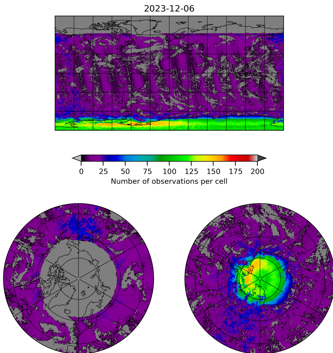
Figure 8: Map of the number of observations for 2023-12-05 to 2023-12-07
