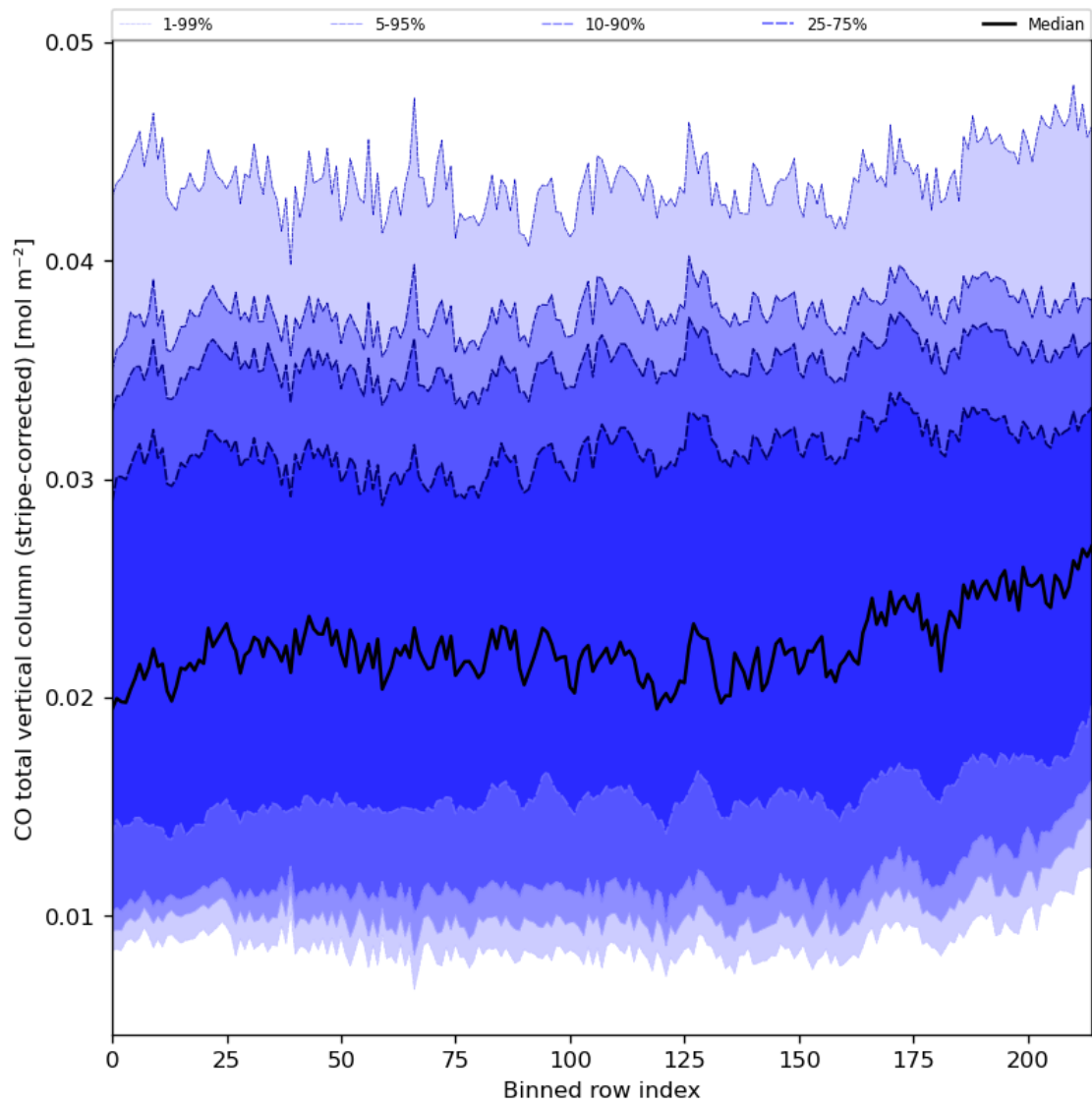
Figure 27: Along track statistics of “CO total vertical column (stripe-corrected)” for 2023-12-05 to 2023-12-07
