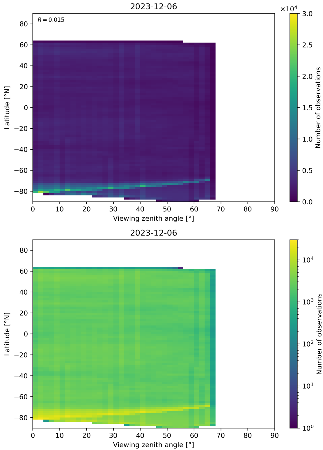
Figure 74: Scatter density plot of “Viewing zenith angle” against “Latitude” for 2023-12-05 to 2023-12-07.
