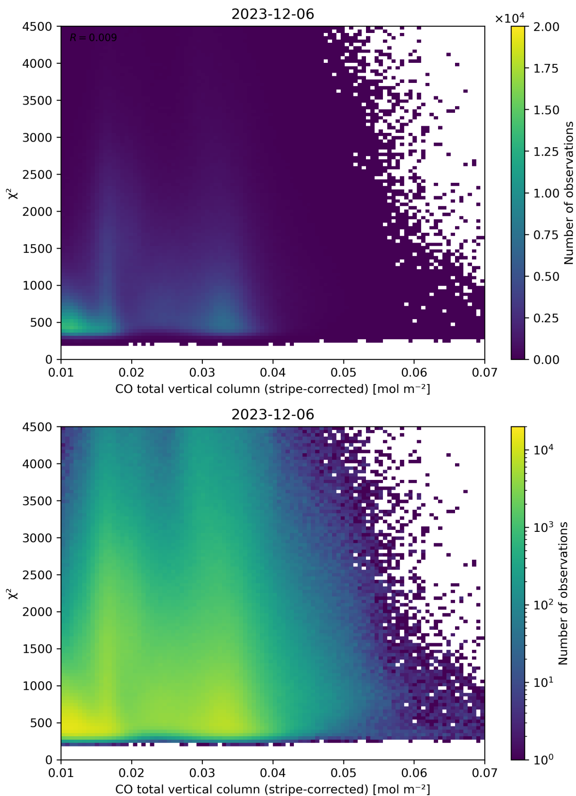
Figure 37: Scatter density plot of “CO total vertical column (stripe-corrected)” against “ \chi^2 ” for 2023-12-05 to 2023-12-07.
