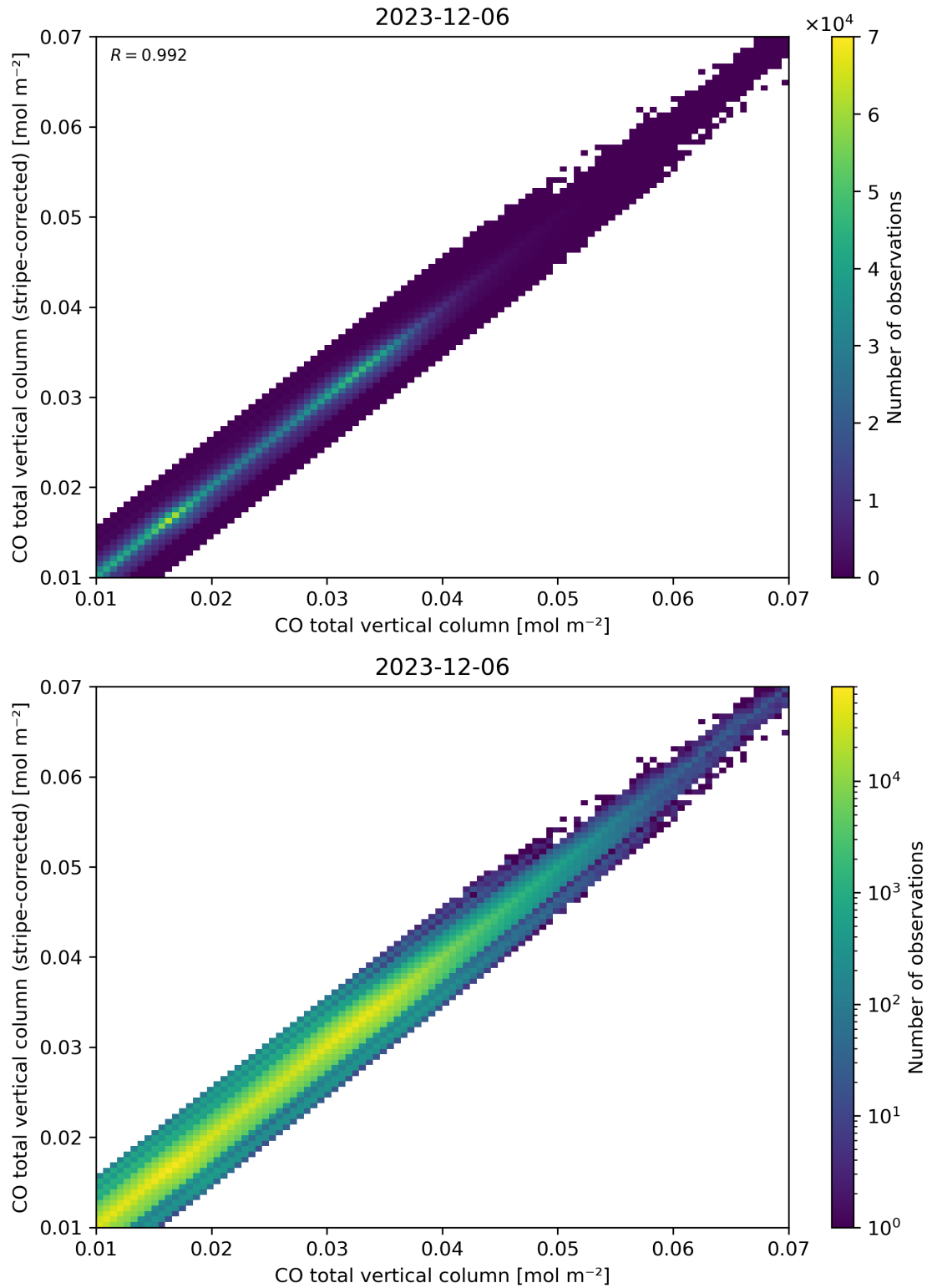
Figure 33: Scatter density plot of “CO total vertical column” against “CO total vertical column (stripe-corrected)” for 2023-12-05 to 2023-12-07.
