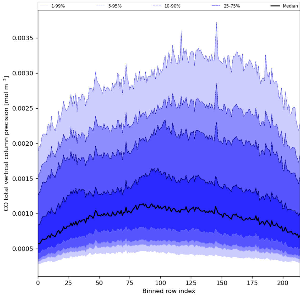
Figure 28: Along track statistics of “CO total vertical column precision” for 2023-12-05 to 2023-12-07
