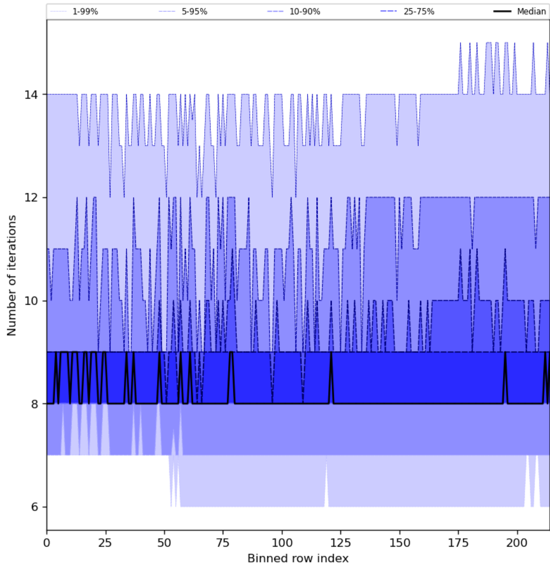
Figure 32: Along track statistics of “Number of iterations” for 2023-12-05 to 2023-12-07
