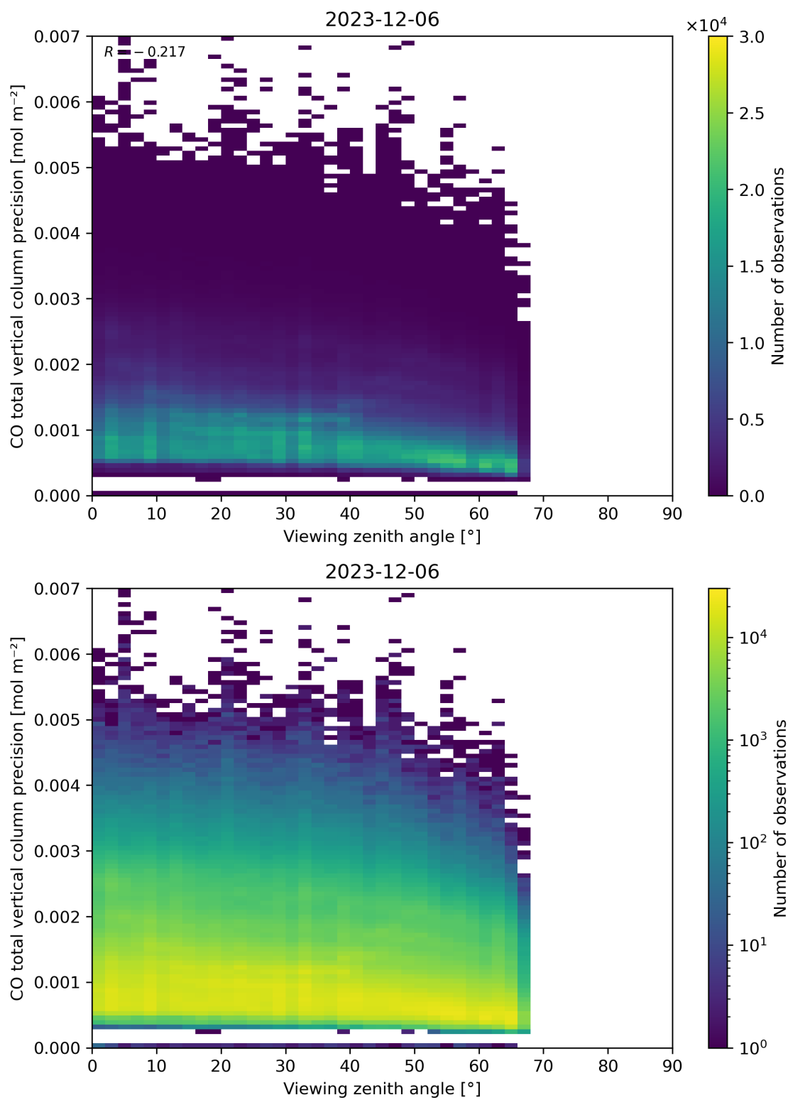
Figure 71: Scatter density plot of “Viewing zenith angle” against “CO total vertical column precision” for 2023-12-05 to 2023-12-07.
