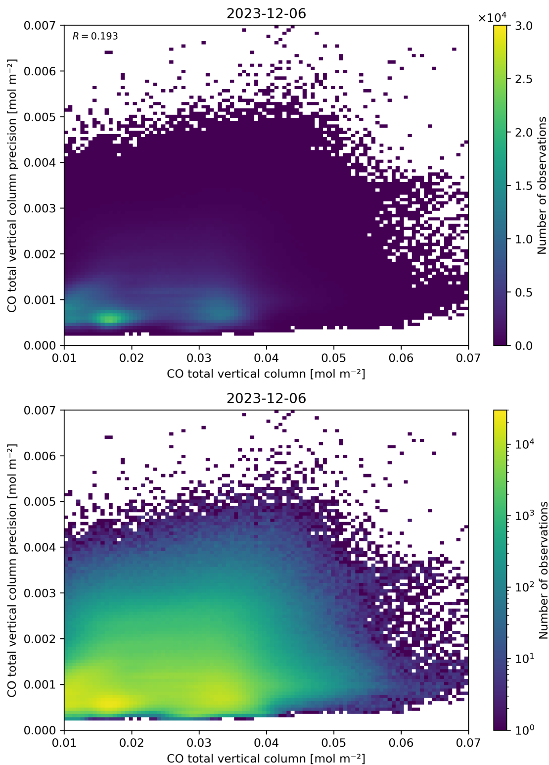
Figure 34: Scatter density plot of “CO total vertical column” against “CO total vertical column precision” for 2023-12-05 to 2023-12-07.
