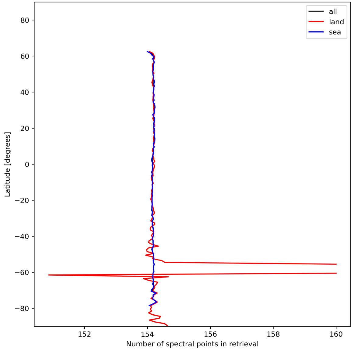
Figure 13: Zonal average of “Number of spectral points in retrieval” for 2023-12-05 to 2023-12-07.
