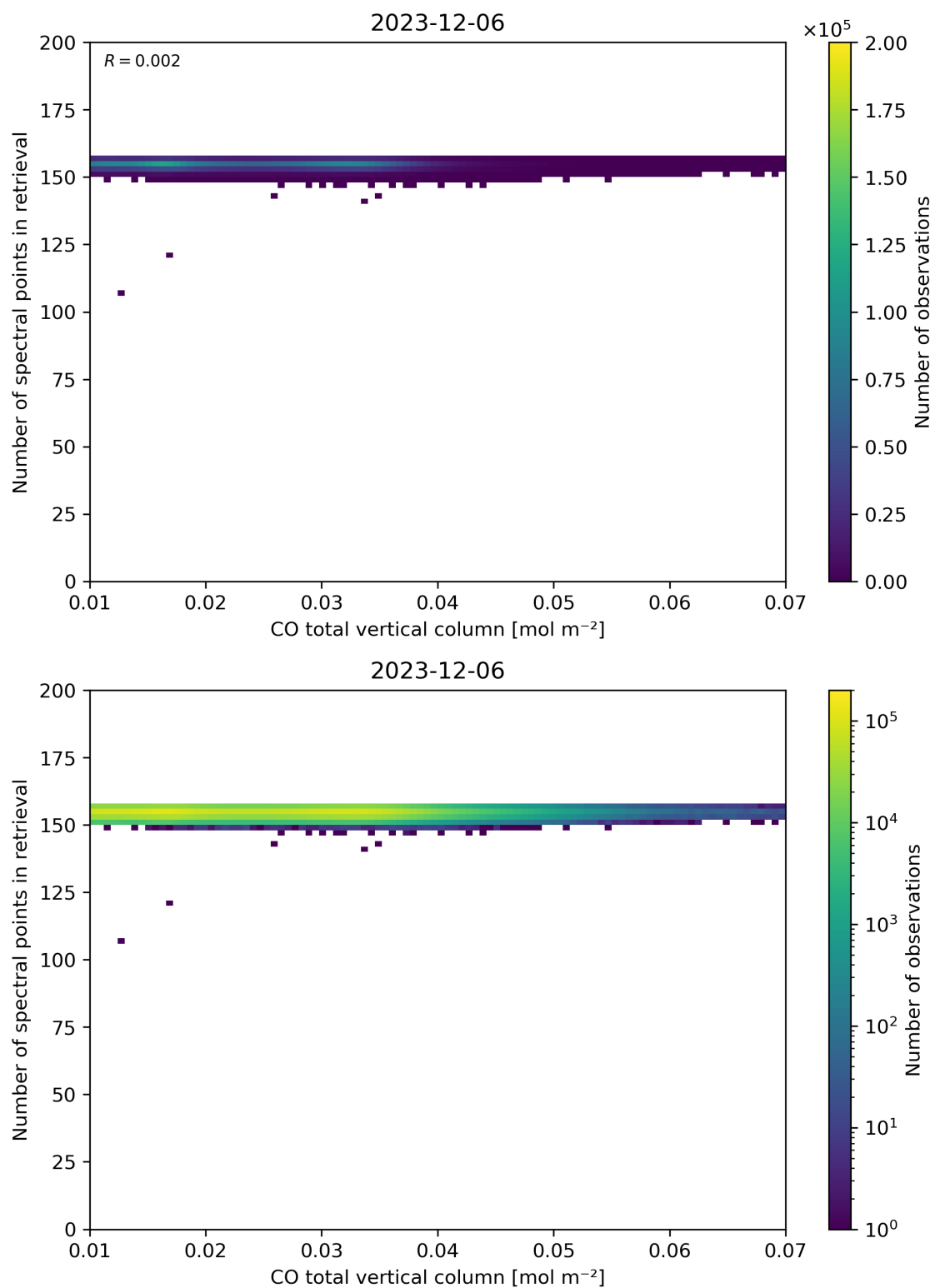
Figure 43: Scatter density plot of “CO total vertical column” against “Number of spectral points in retrieval” for 2023-12-05 to 2023-12-07.
