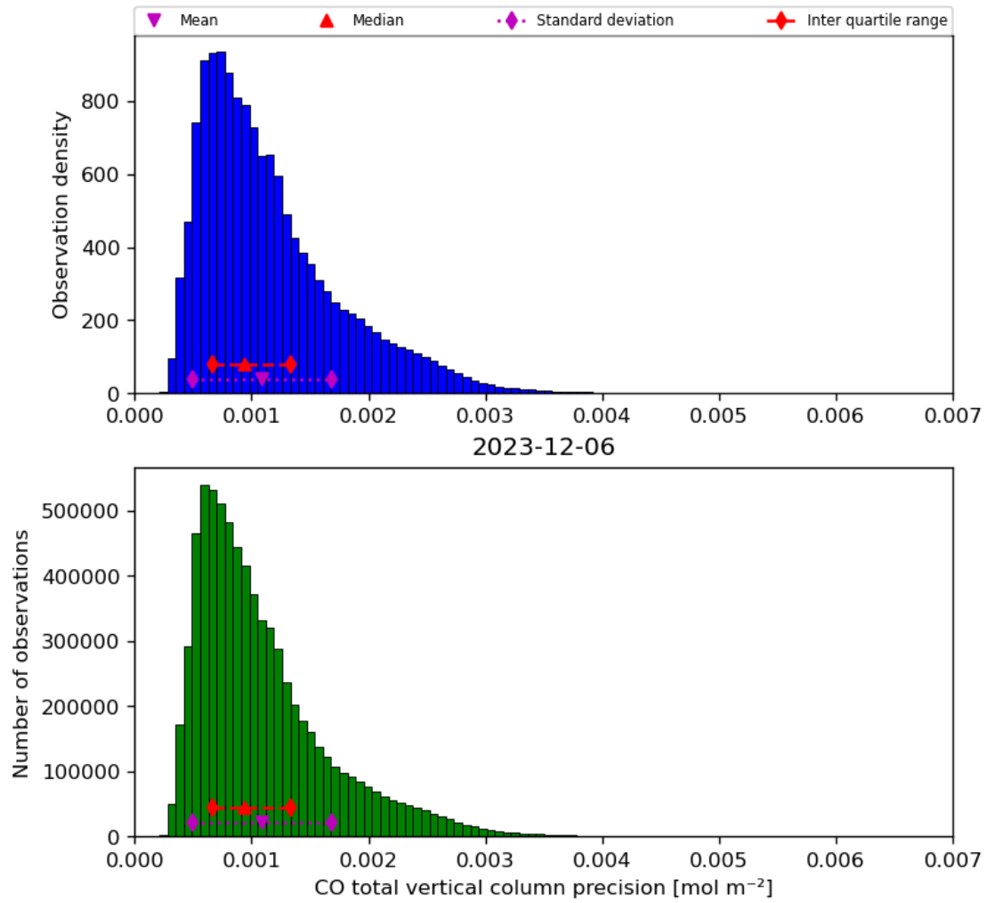
Figure 20: Histogram of “CO total vertical column precision” for 2023-12-05 to 2023-12-07
