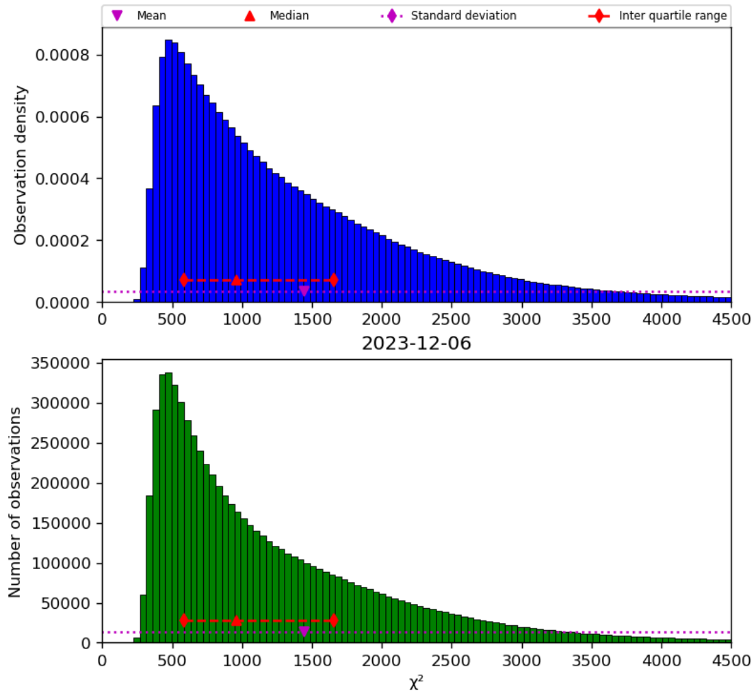
Figure 22: Histogram of “ \chi^2 ” for 2023-12-05 to 2023-12-07
