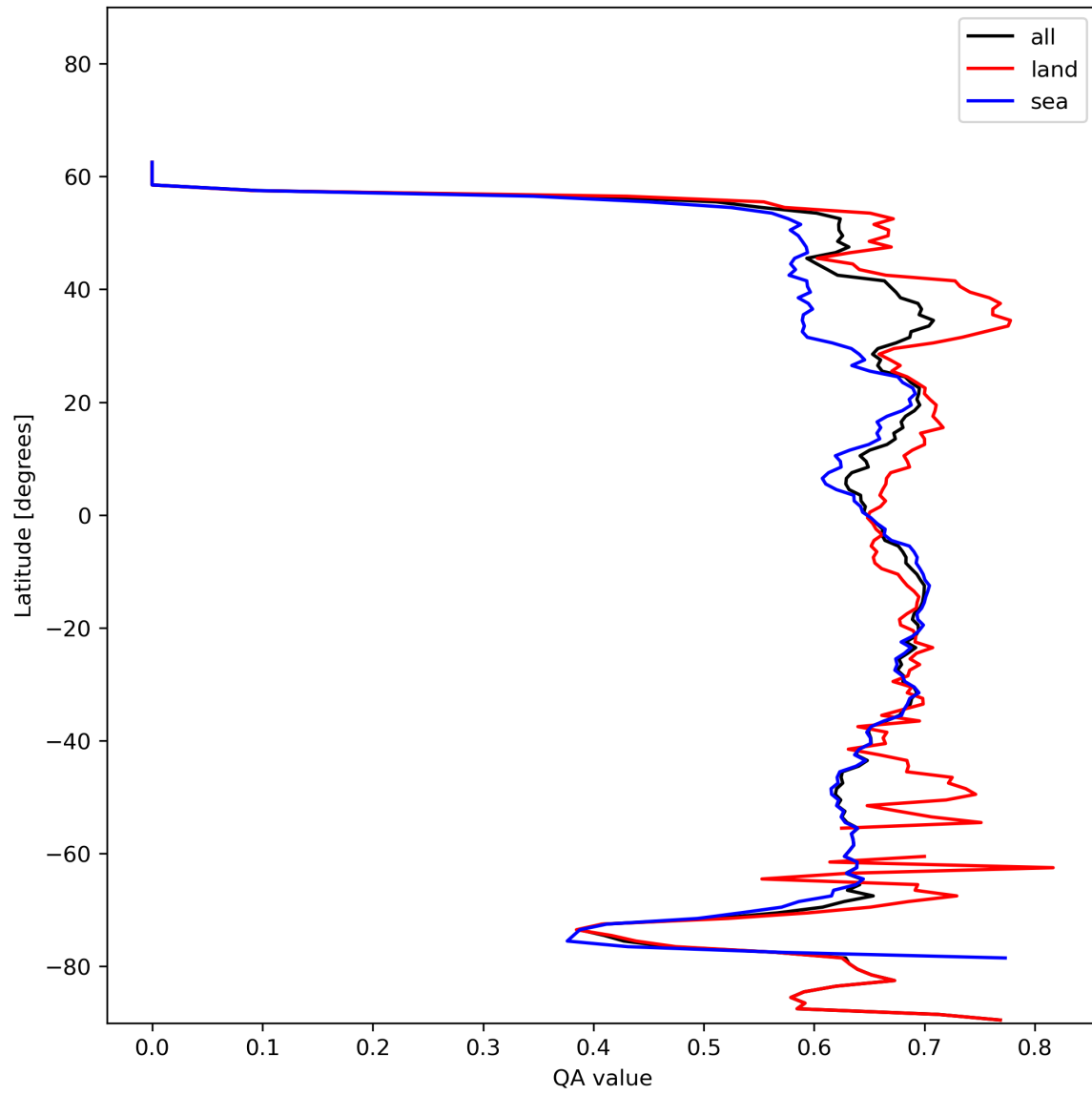
Figure 9: Zonal average of “QA value” for 2023-12-05 to 2023-12-07.
