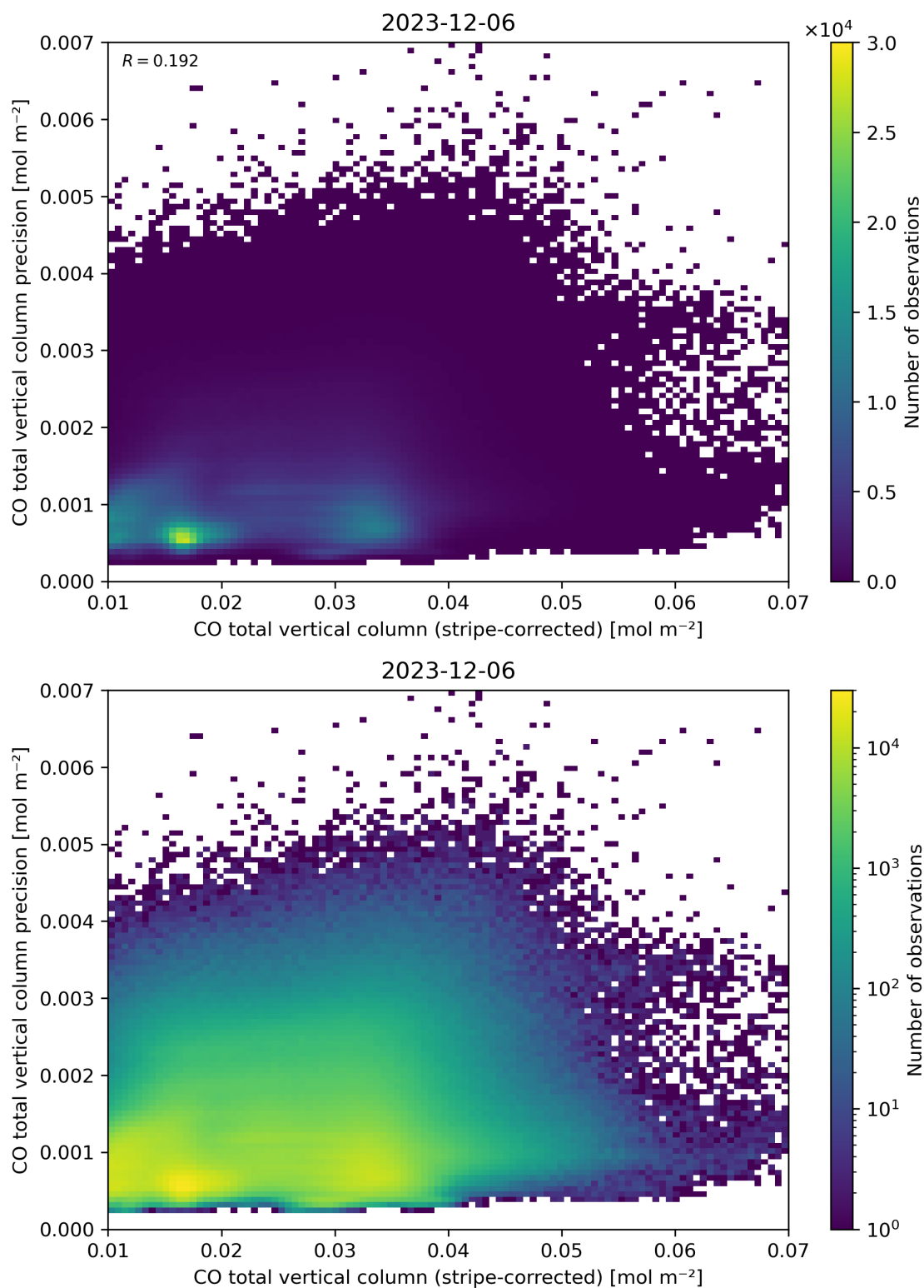
Figure 36: Scatter density plot of “CO total vertical column (stripe-corrected)” against “CO total vertical column precision” for 2023-12-05 to 2023-12-07.
