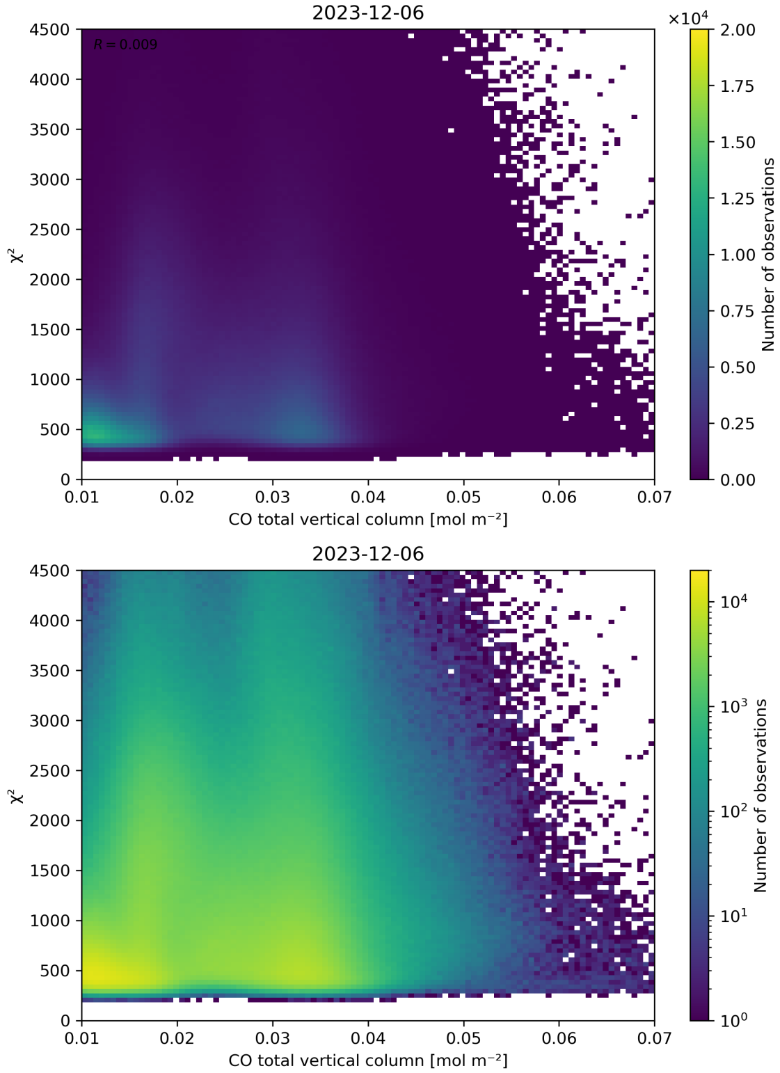
Figure 35: Scatter density plot of “CO total vertical column” against “ \chi^2 ” for 2023-12-05 to 2023-12-07.
