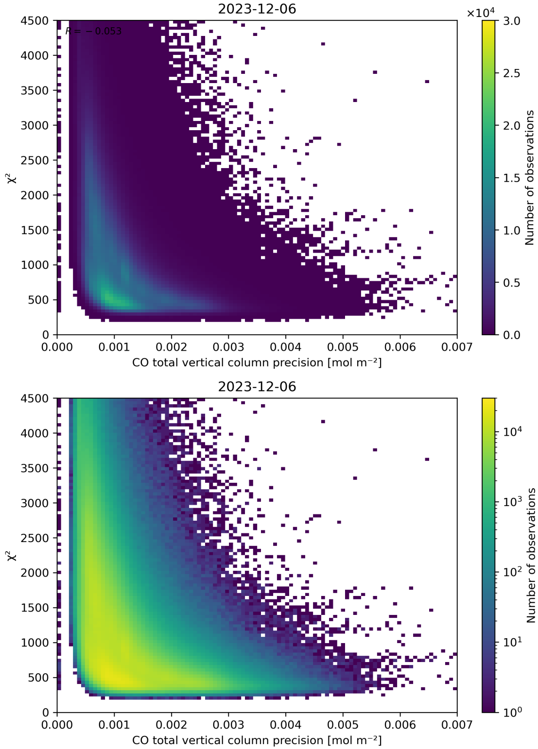
Figure 44: Scatter density plot of “CO total vertical column precision” against “ \chi^2 ” for 2023-12-05 to 2023-12-07.
