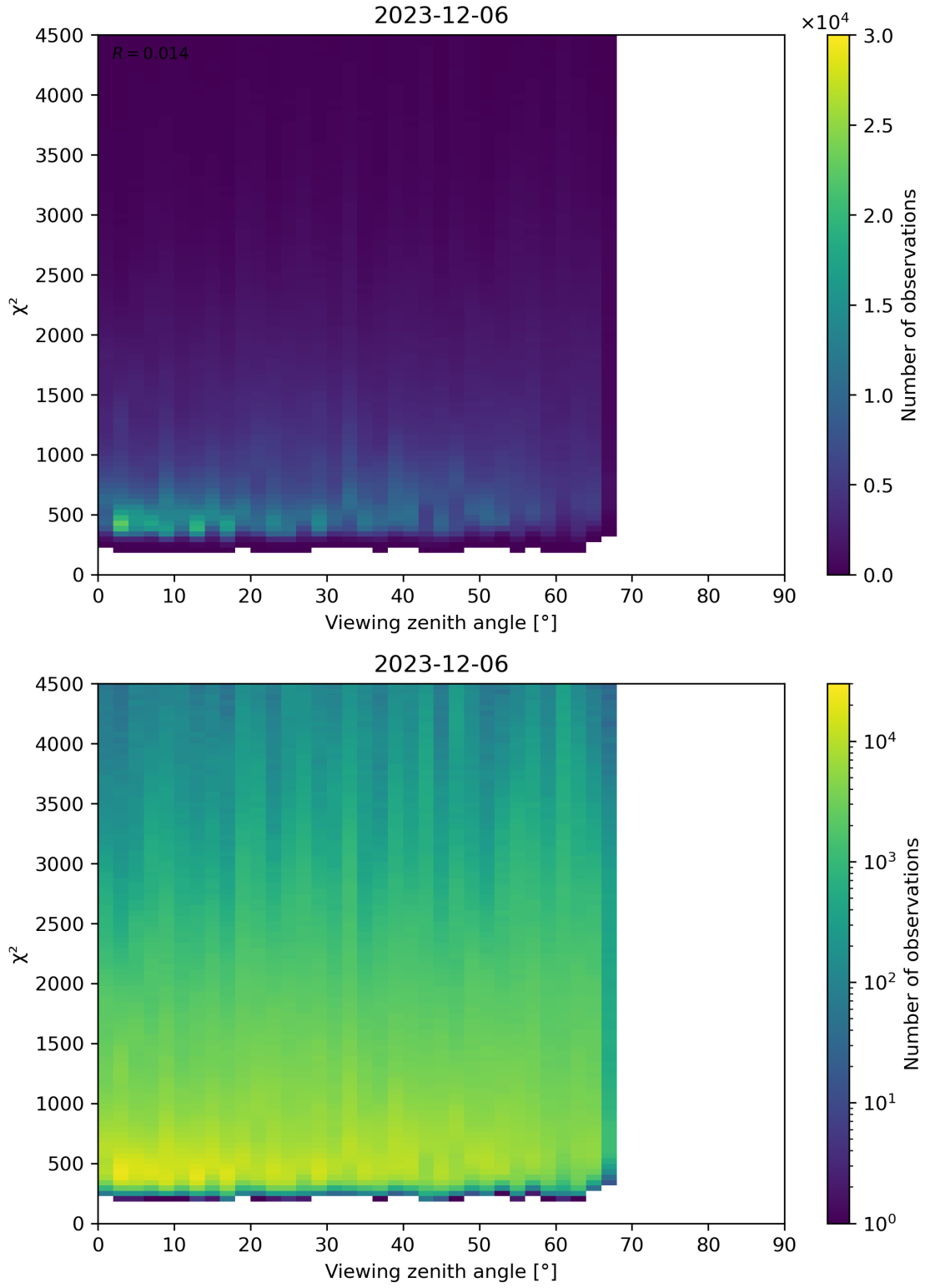
Figure 72: Scatter density plot of “Viewing zenith angle” against “ \chi^2 ” for 2023-12-05 to 2023-12-07.
