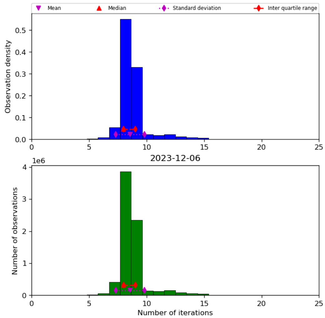
Figure 24: Histogram of “Number of iterations” for 2023-12-05 to 2023-12-07
