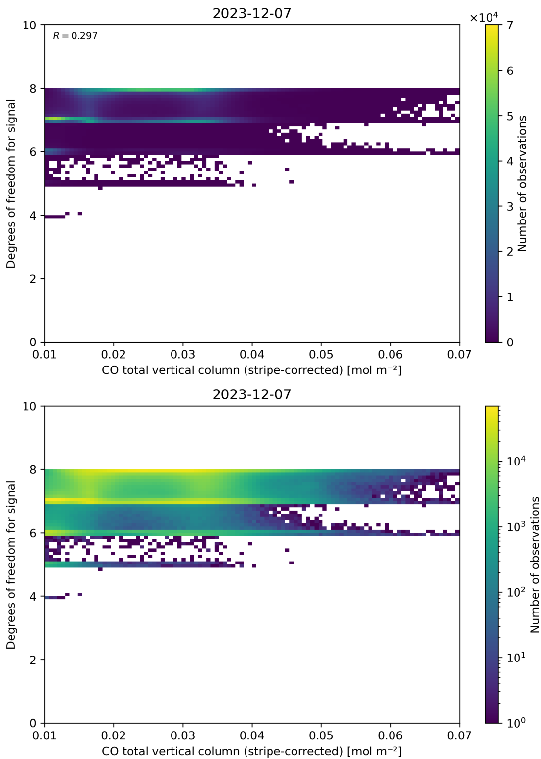
Figure 38: Scatter density plot of “CO total vertical column (stripe-corrected)” against “Degrees of freedom for signal” for 2023-12-06 to 2023-12-08.
