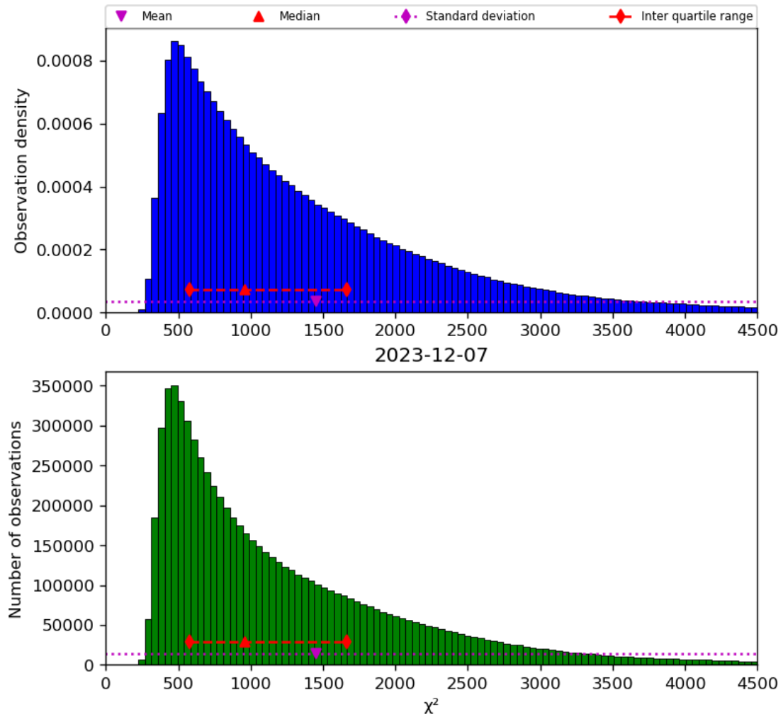
Figure 22: Histogram of “ \chi^2 ” for 2023-12-06 to 2023-12-08
