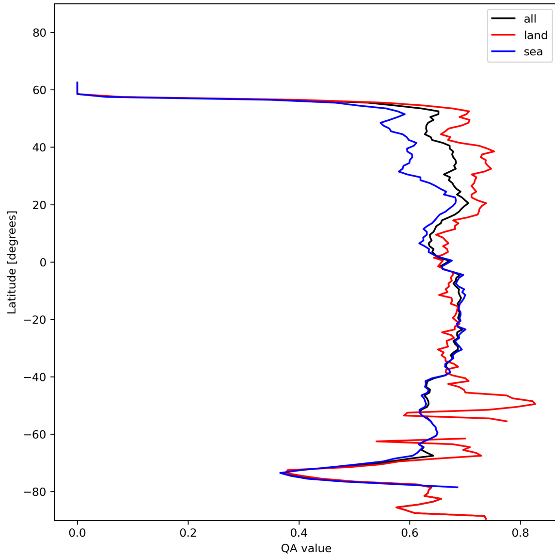
Figure 9: Zonal average of “QA value” for 2023-12-06 to 2023-12-08.
