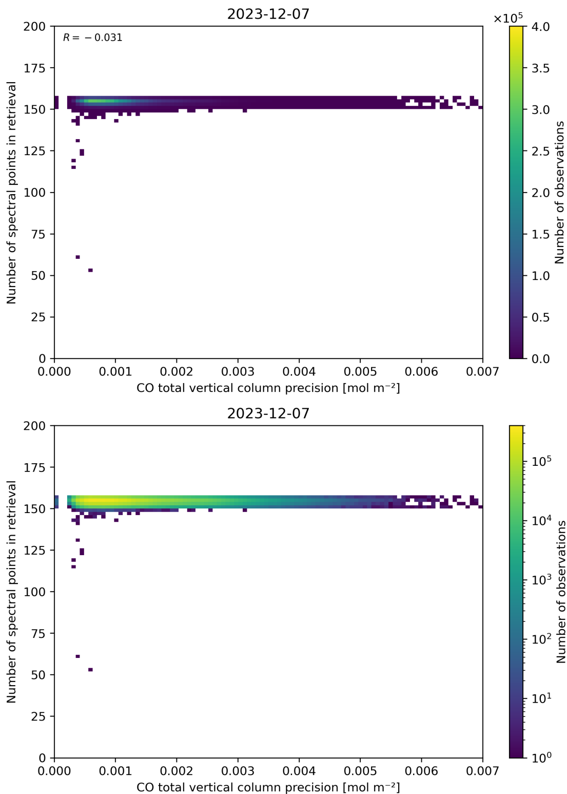
Figure 47: Scatter density plot of “CO total vertical column precision” against “Number of spectral points in retrieval” for 2023-12-06 to 2023-12-08.
