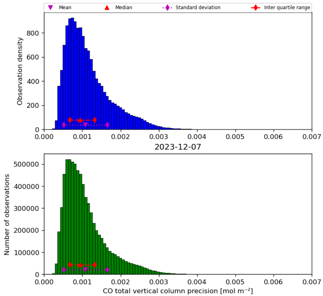
Figure 20: Histogram of “CO total vertical column precision” for 2023-12-06 to 2023-12-08
