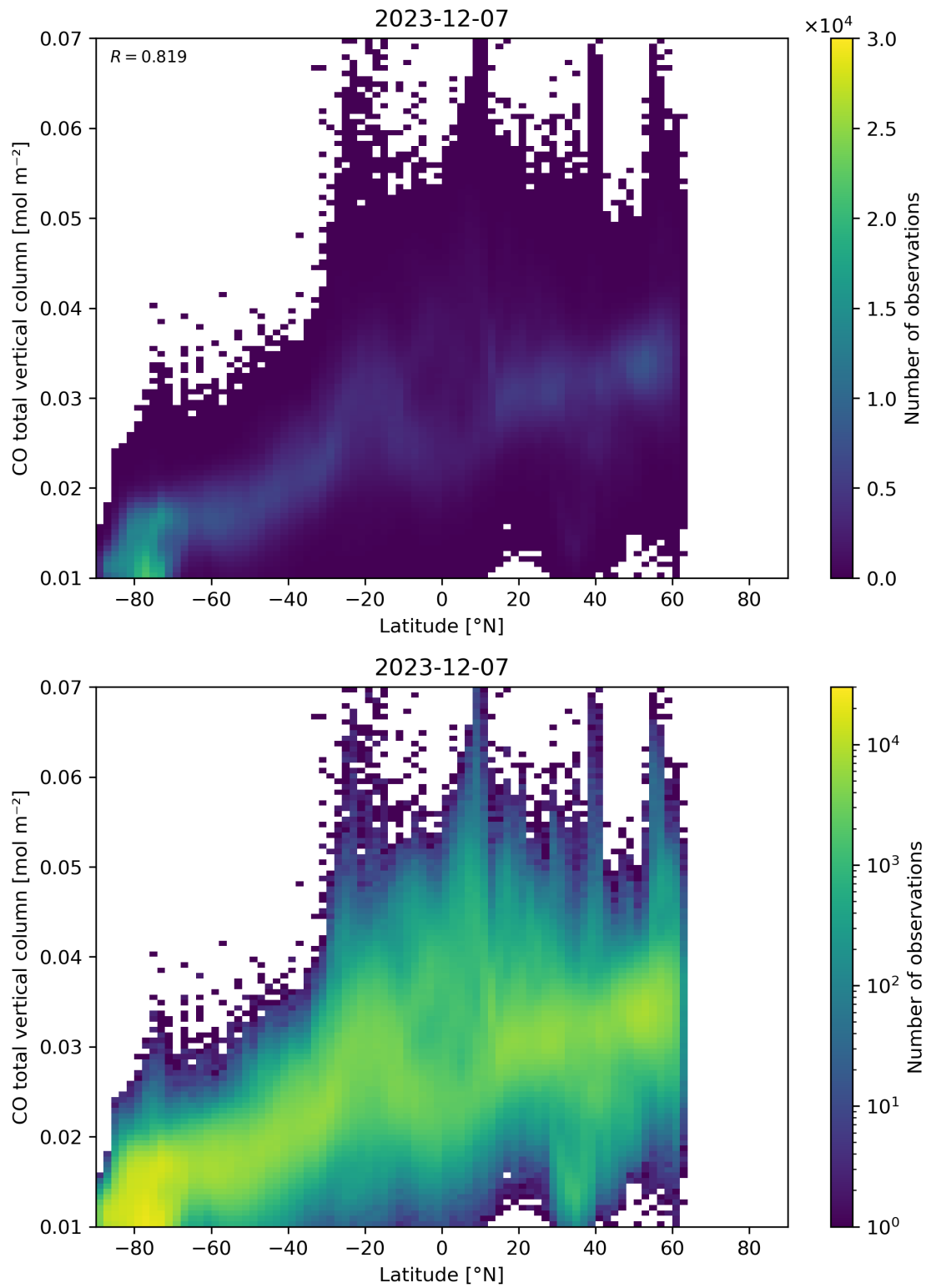
Figure 51: Scatter density plot of “Latitude” against “CO total vertical column” for 2023-12-06 to 2023-12-08.
