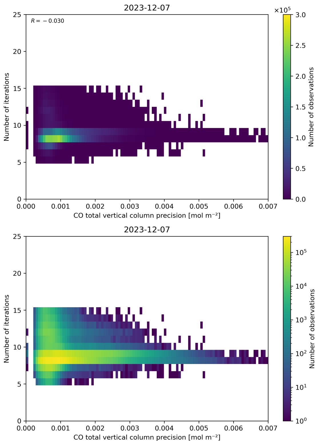
Figure 46: Scatter density plot of “CO total vertical column precision” against “Number of iterations” for 2023-12-06 to 2023-12-08.
