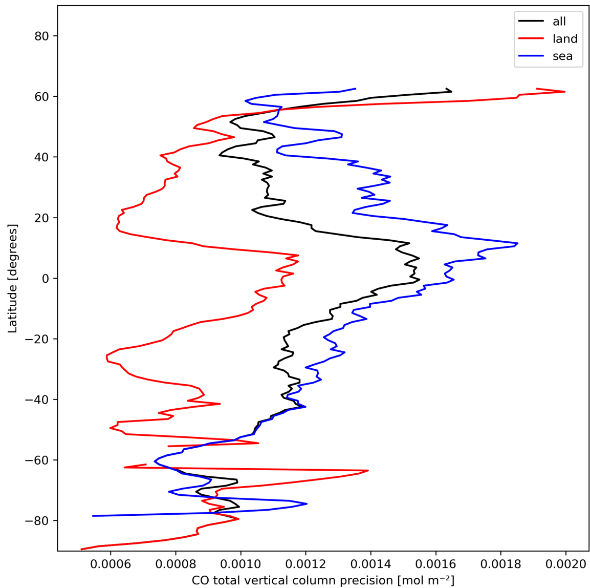
Figure 12: Zonal average of “CO total vertical column precision” for 2023-12-06 to 2023-12-08.
