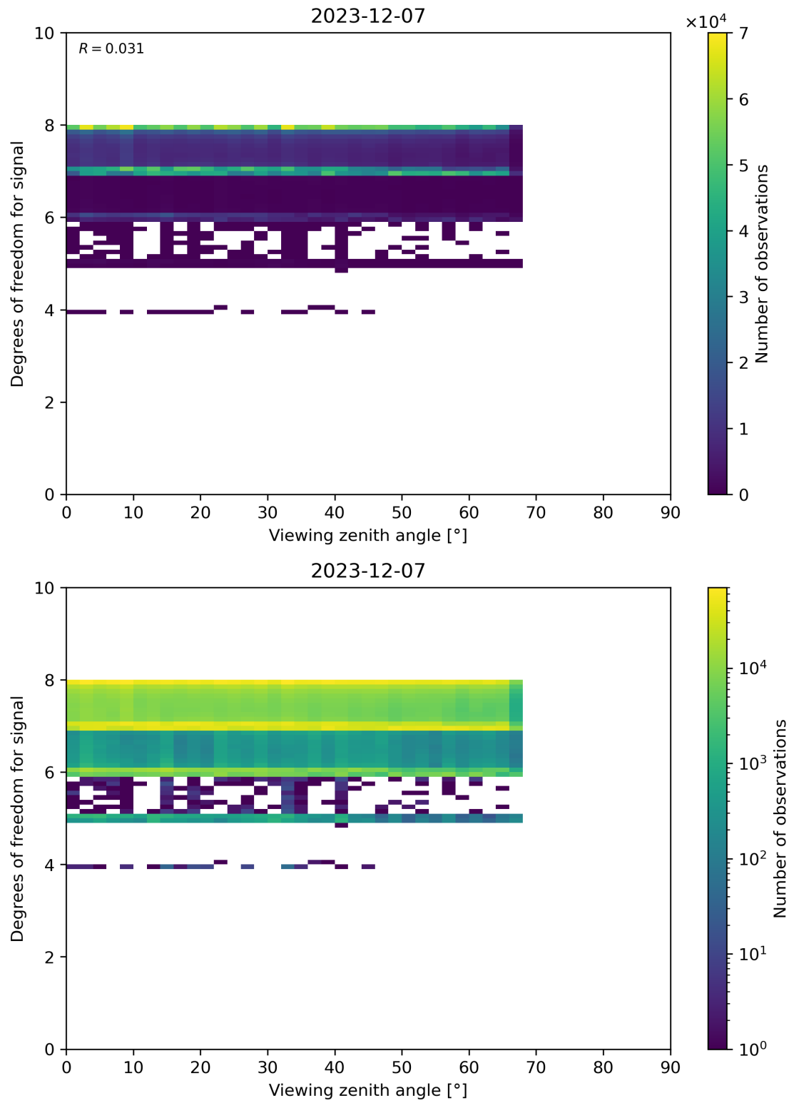
Figure 73: Scatter density plot of “Viewing zenith angle” against “Degrees of freedom for signal” for 2023-12-06 to 2023-12-08.
