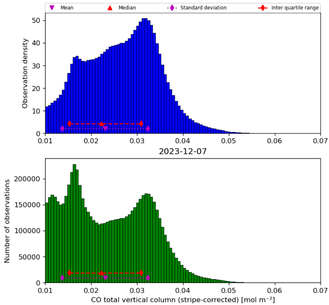
Figure 19: Histogram of “CO total vertical column (stripe-corrected)” for 2023-12-06 to 2023-12-08
