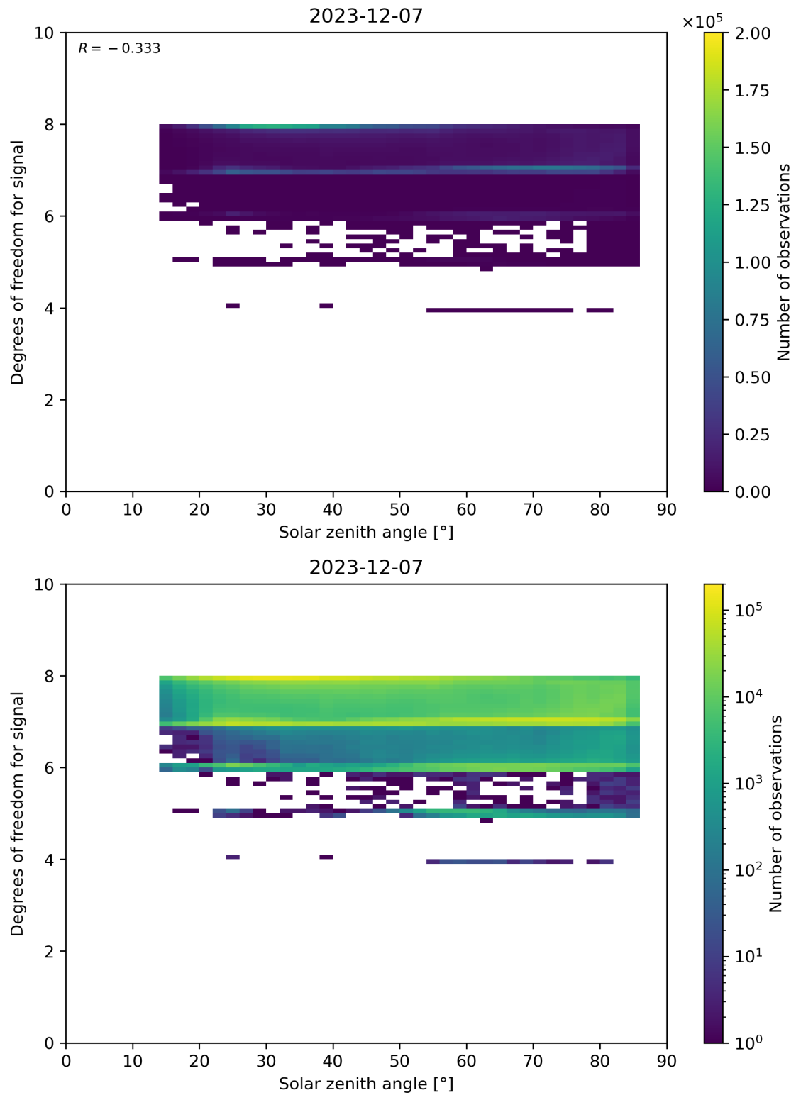
Figure 65: Scatter density plot of “Solar zenith angle” against “Degrees of freedom for signal” for 2023-12-06 to 2023-12-08.
