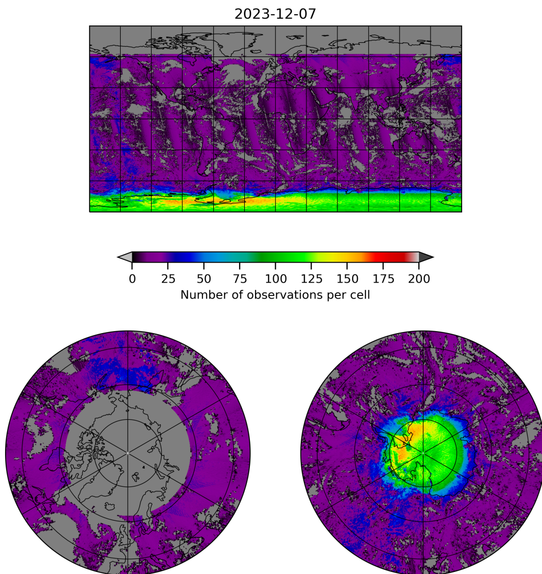
Figure 8: Map of the number of observations for 2023-12-06 to 2023-12-08
