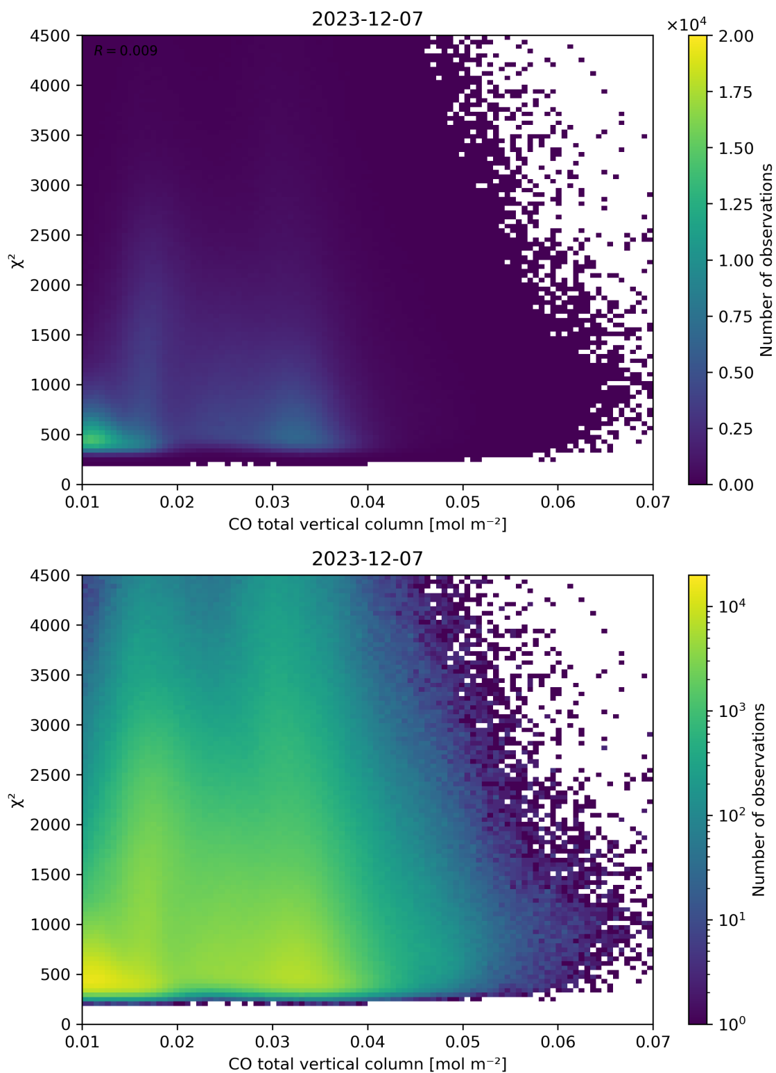
Figure 35: Scatter density plot of “CO total vertical column” against “ \chi^2 ” for 2023-12-06 to 2023-12-08.
