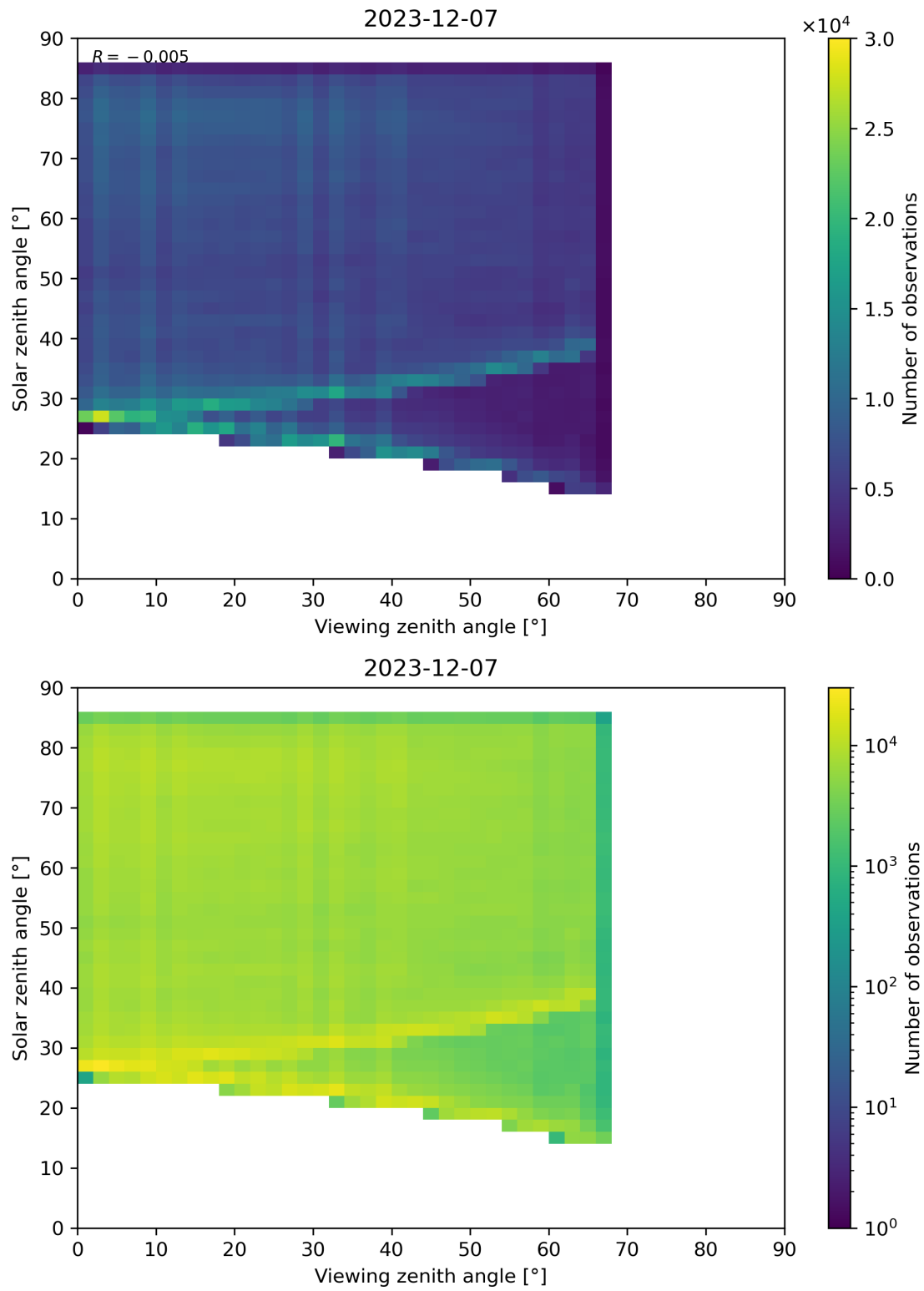
Figure 77: Scatter density plot of “Viewing zenith angle” against “Solar zenith angle” for 2023-12-06 to 2023-12-08.
