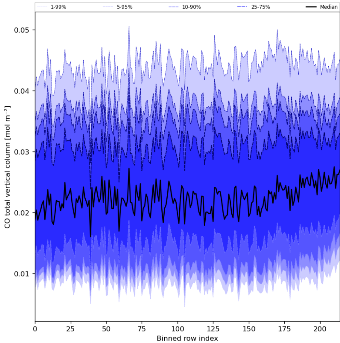
Figure 26: Along track statistics of “CO total vertical column” for 2023-12-06 to 2023-12-08
