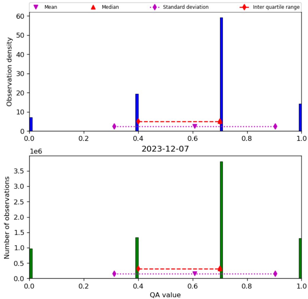
Figure 17: Histogram of “QA value” for 2023-12-06 to 2023-12-08
