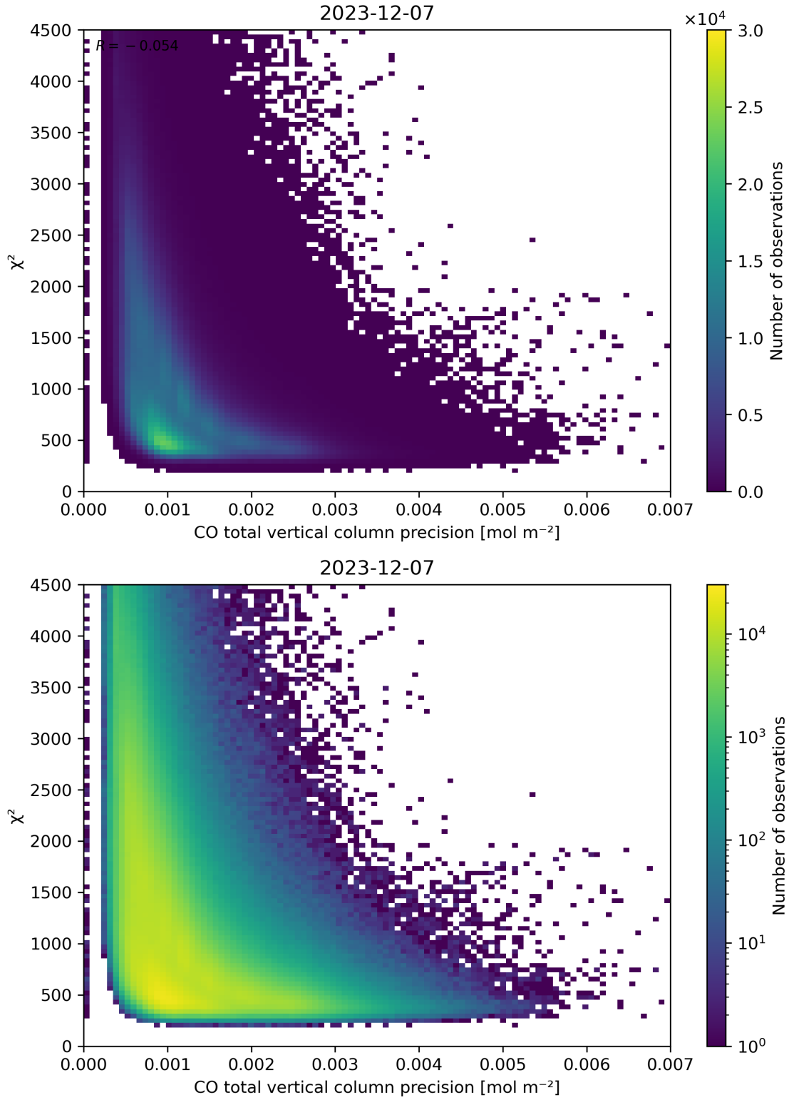
Figure 44: Scatter density plot of “CO total vertical column precision” against “ \chi^2 ” for 2023-12-06 to 2023-12-08.
