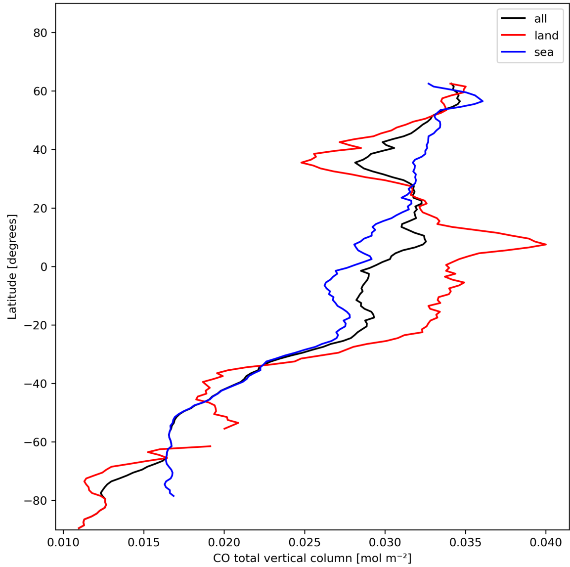
Figure 10: Zonal average of “CO total vertical column” for 2023-12-06 to 2023-12-08.
