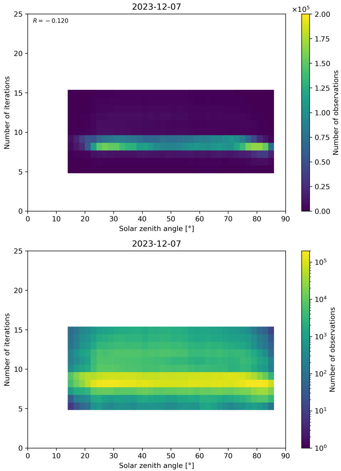
Figure 67: Scatter density plot of “Solar zenith angle” against “Number of iterations” for 2023-12-06 to 2023-12-08.
