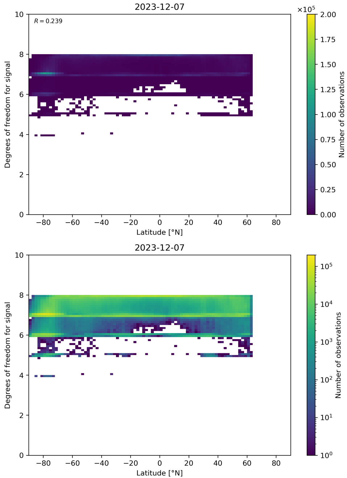
Figure 55: Scatter density plot of “Latitude” against “Degrees of freedom for signal” for 2023-12-06 to 2023-12-08.
