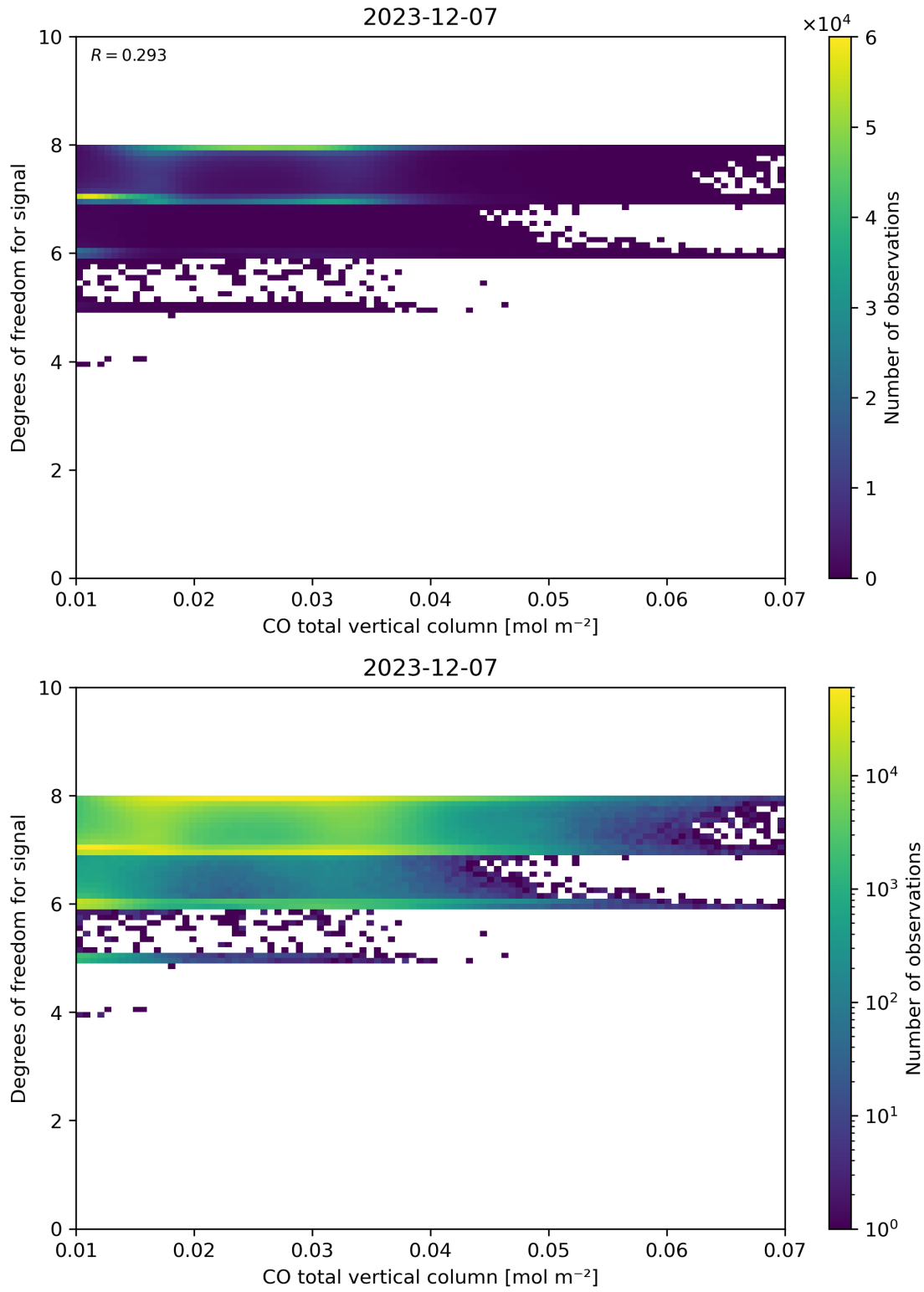
Figure 41: Scatter density plot of “CO total vertical column” against “Degrees of freedom for signal” for 2023-12-06 to 2023-12-08.
