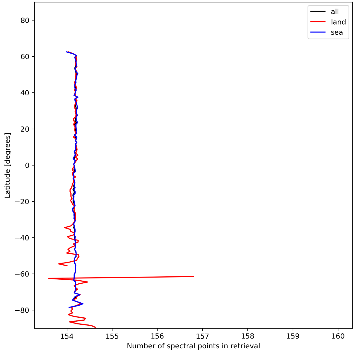
Figure 13: Zonal average of “Number of spectral points in retrieval” for 2023-12-06 to 2023-12-08.
