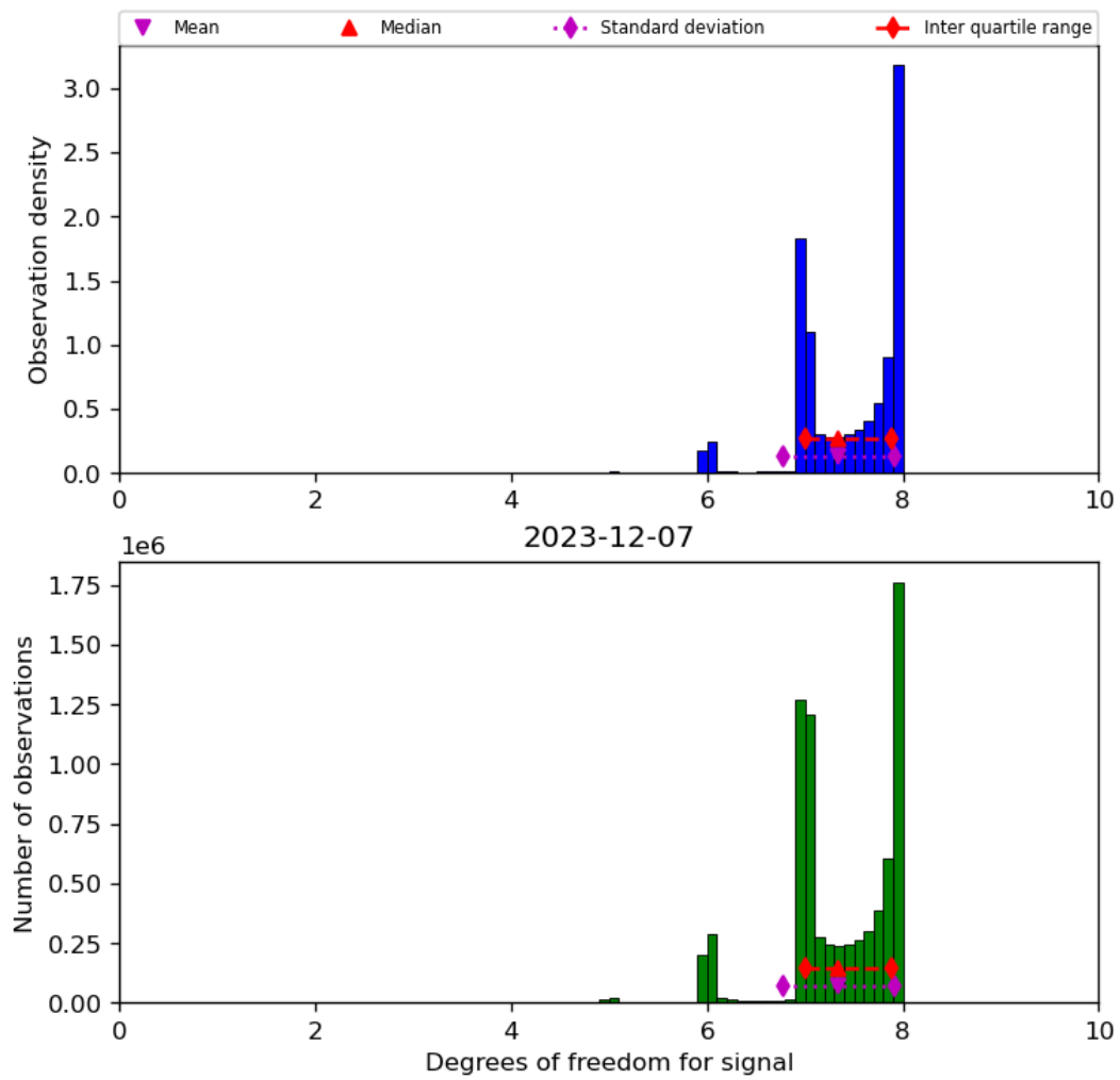
Figure 23: Histogram of “Degrees of freedom for signal” for 2023-12-06 to 2023-12-08
