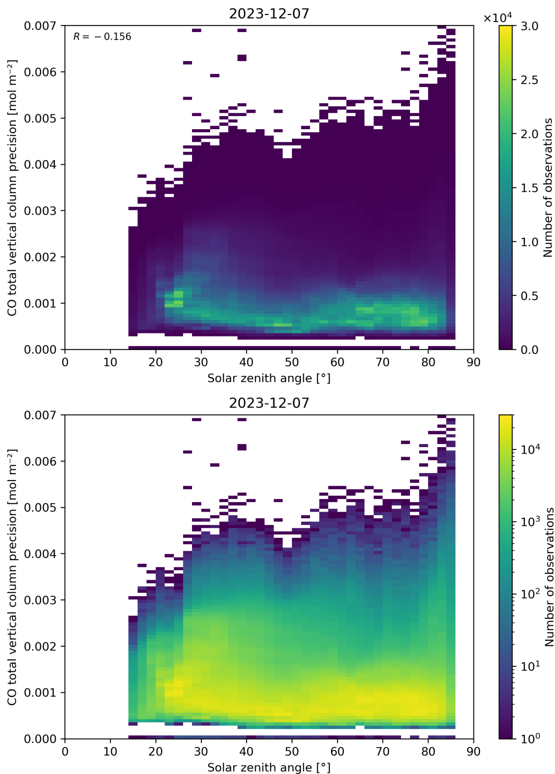
Figure 63: Scatter density plot of “Solar zenith angle” against “CO total vertical column precision” for 2023-12-06 to 2023-12-08.
