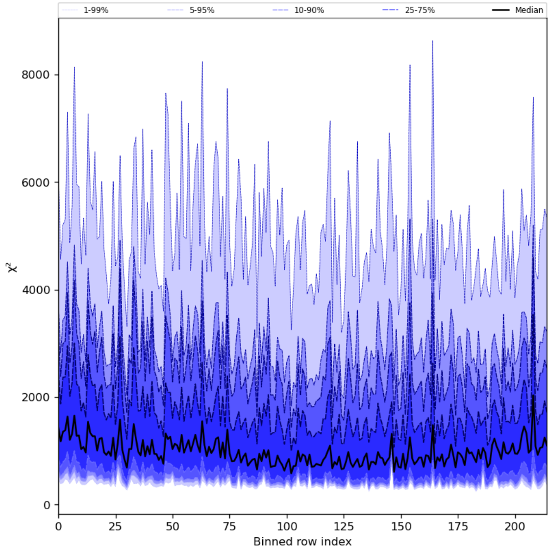
Figure 30: Along track statistics of “ \chi^2 ” for 2023-12-06 to 2023-12-08
