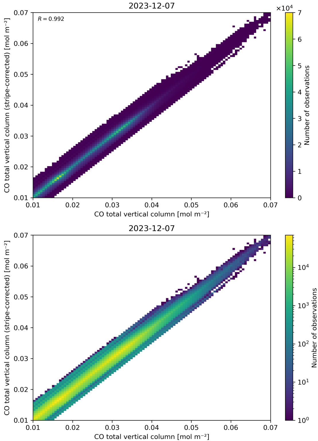
Figure 33: Scatter density plot of “CO total vertical column” against “CO total vertical column (stripe-corrected)” for 2023-12-06 to 2023-12-08.
