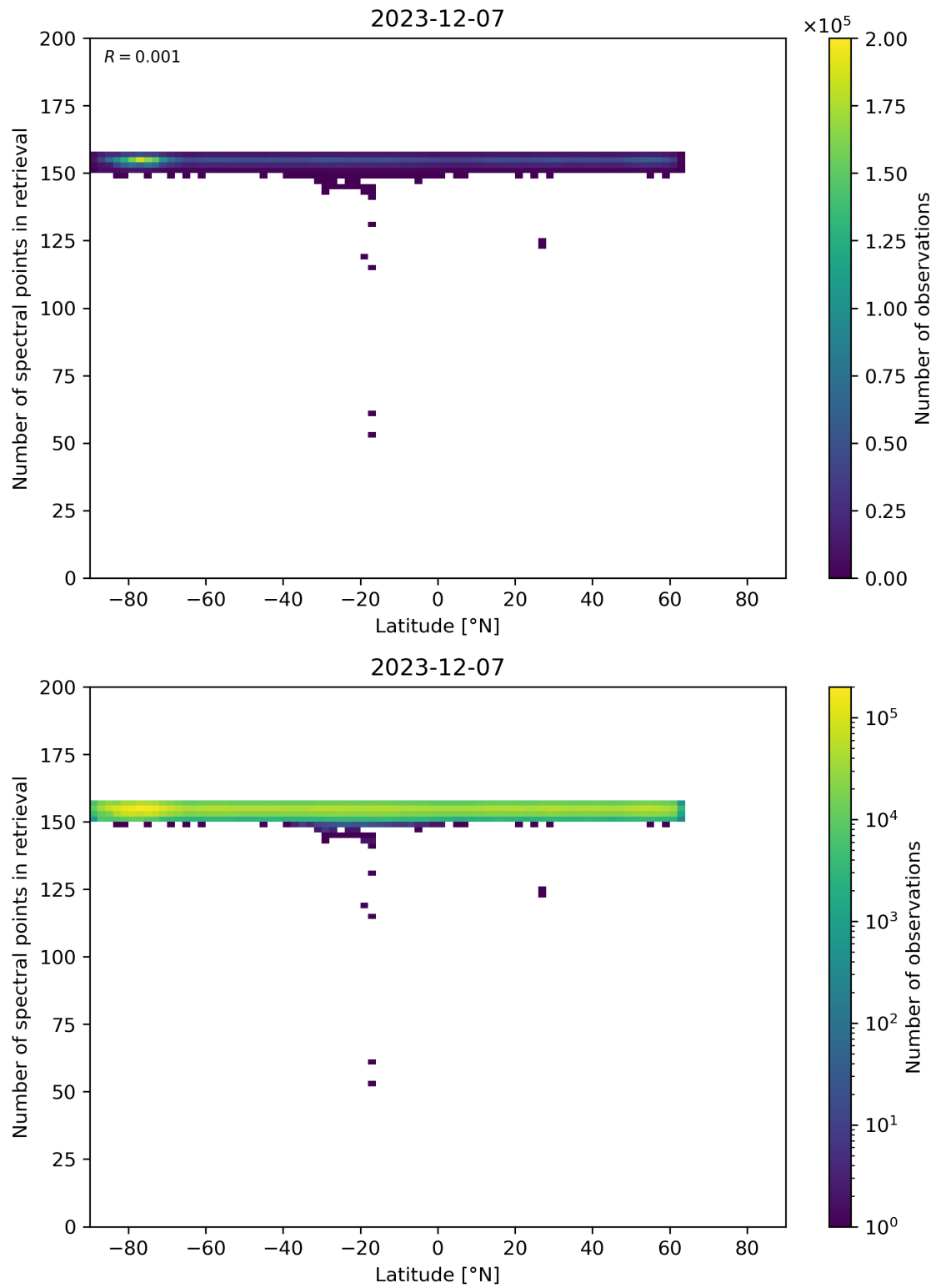
Figure 57: Scatter density plot of “Latitude” against “Number of spectral points in retrieval” for 2023-12-06 to 2023-12-08.
