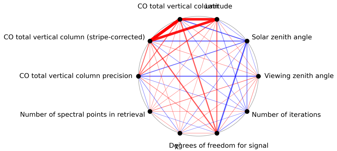
Figure 1: Map of correlation graph for 2023-12-06 to 2023-12-08.
