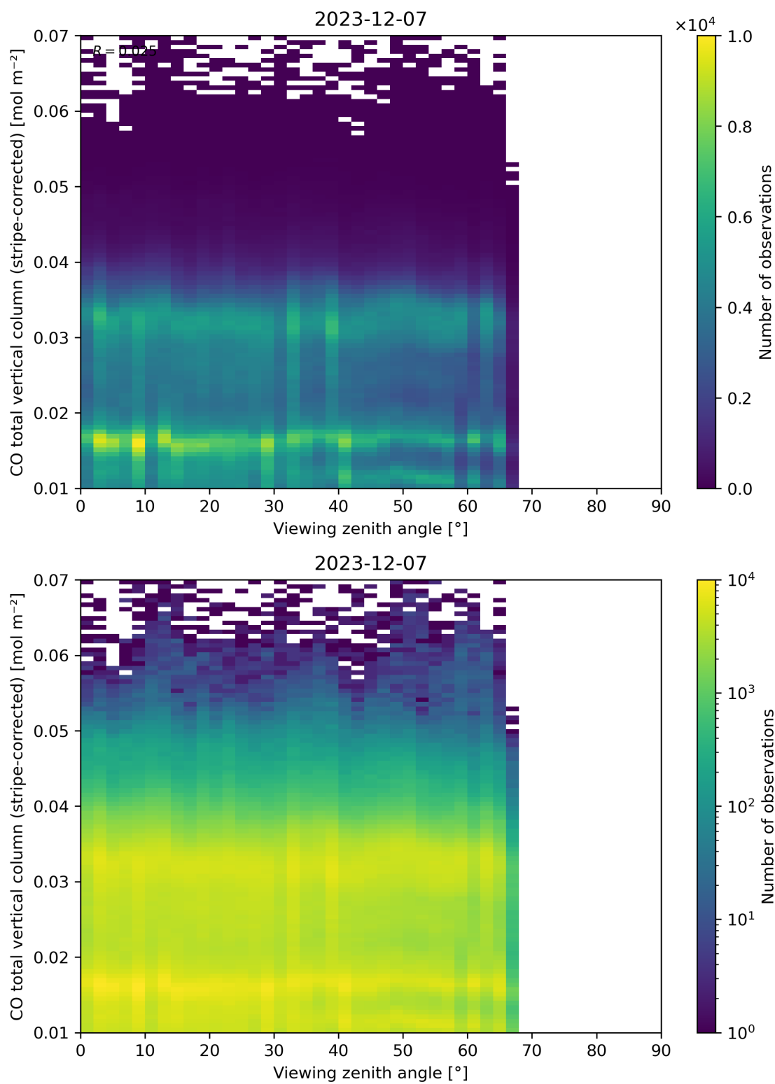
Figure 70: Scatter density plot of “Viewing zenith angle” against “CO total vertical column (stripe-corrected)” for 2023-12-06 to 2023-12-08.
