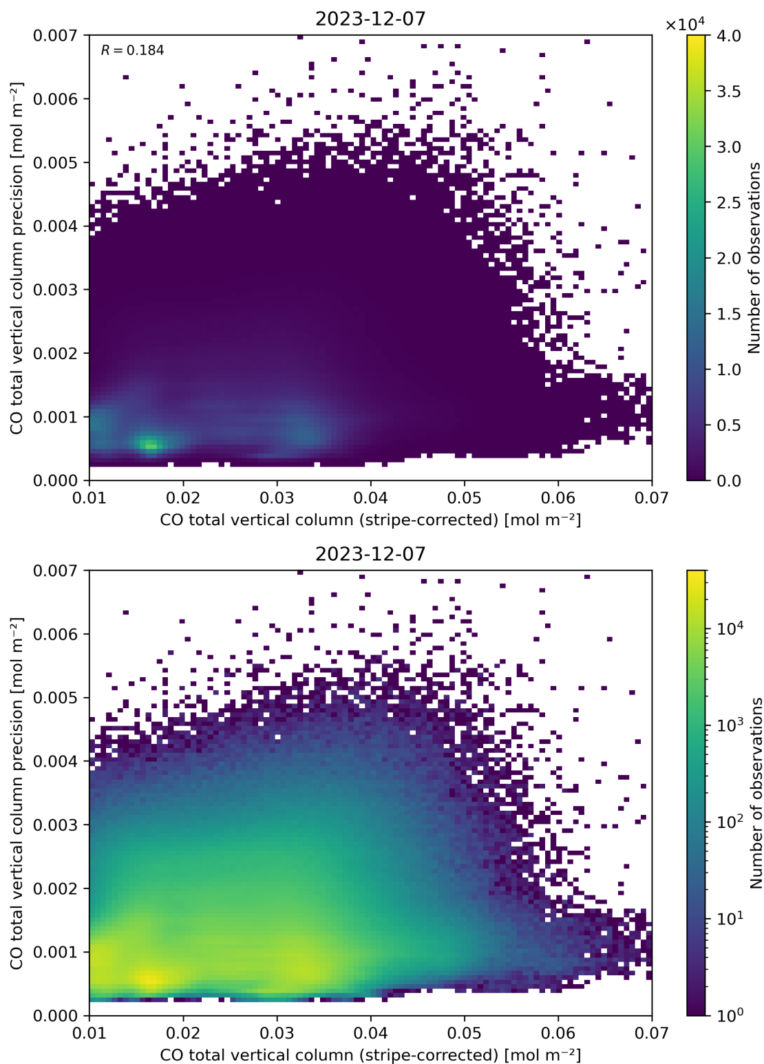
Figure 36: Scatter density plot of “CO total vertical column (stripe-corrected)” against “CO total vertical column precision” for 2023-12-06 to 2023-12-08.
