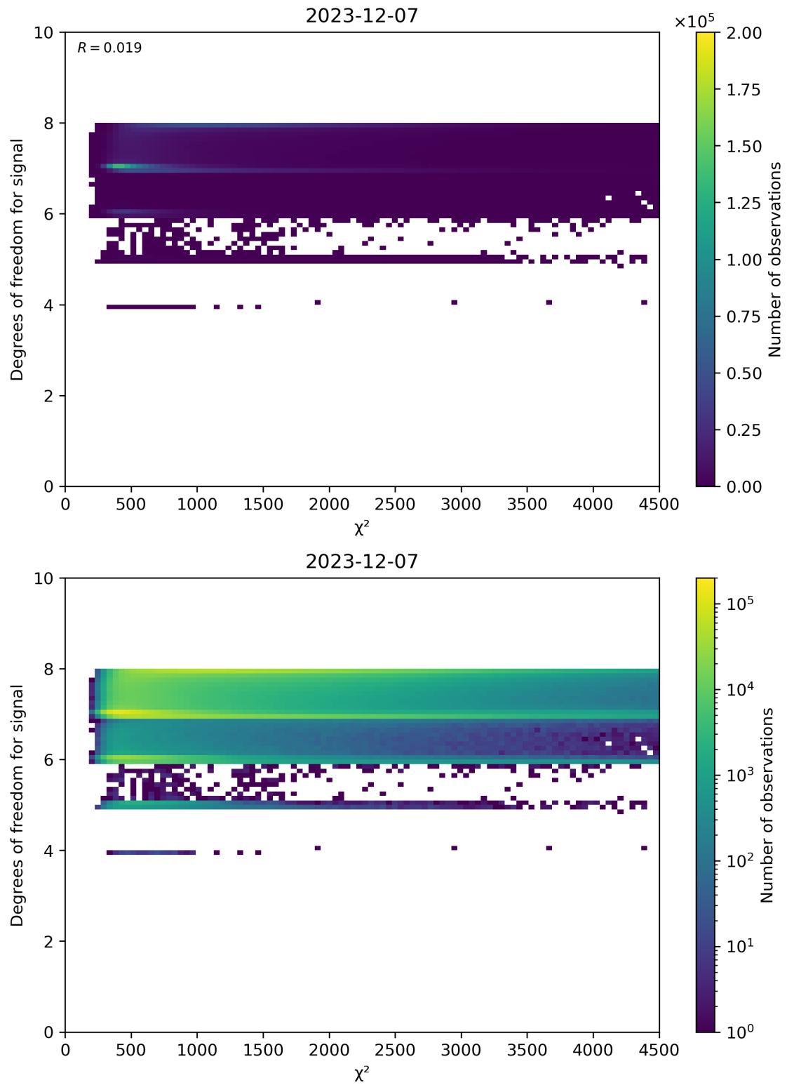
Figure 48: Scatter density plot of “ \chi^2 ” against “Degrees of freedom for signal” for 2023-12-06 to 2023-12-08.
