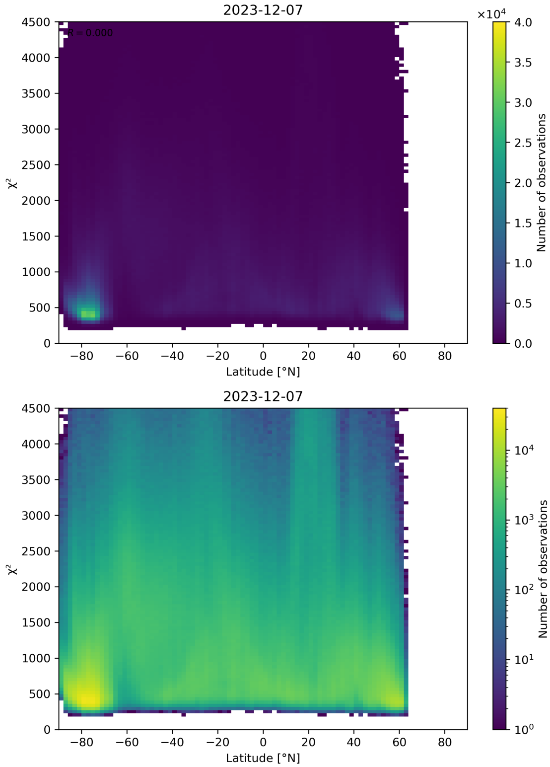
Figure 54: Scatter density plot of “Latitude” against “ \chi^2 ” for 2023-12-06 to 2023-12-08.
