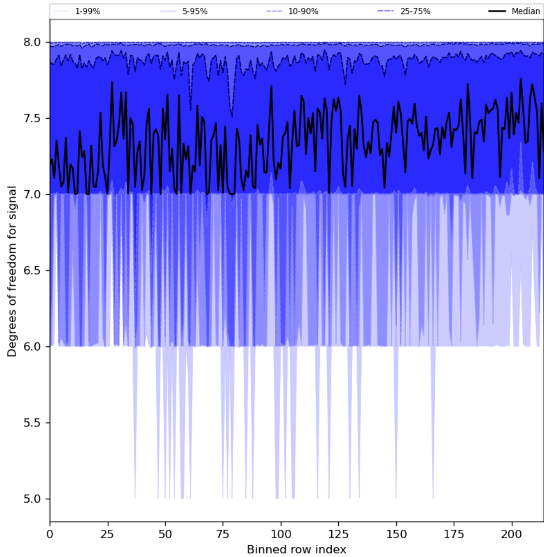
Figure 31: Along track statistics of “Degrees of freedom for signal” for 2023-12-06 to 2023-12-08
