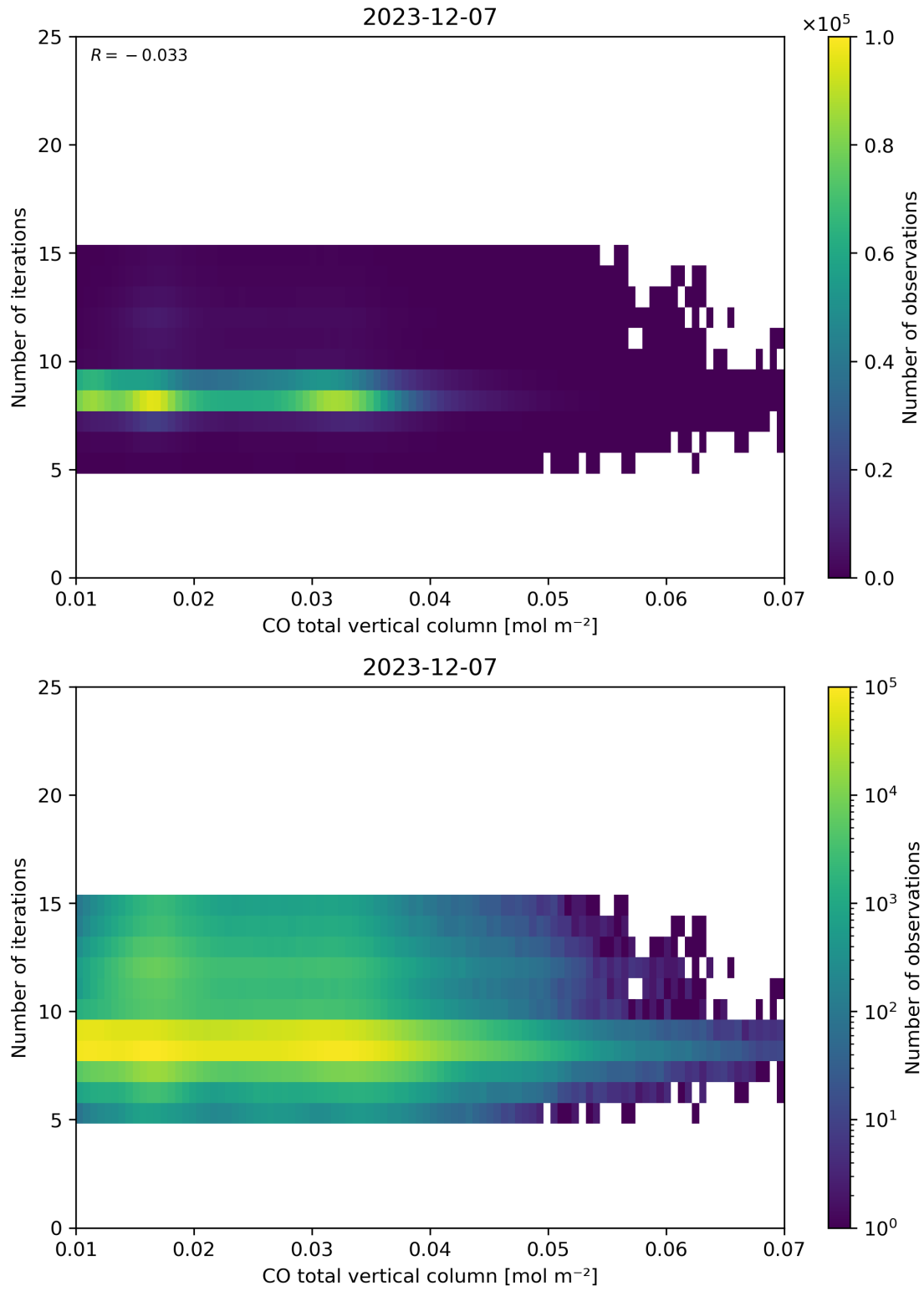
Figure 42: Scatter density plot of “CO total vertical column” against “Number of iterations” for 2023-12-06 to 2023-12-08.
