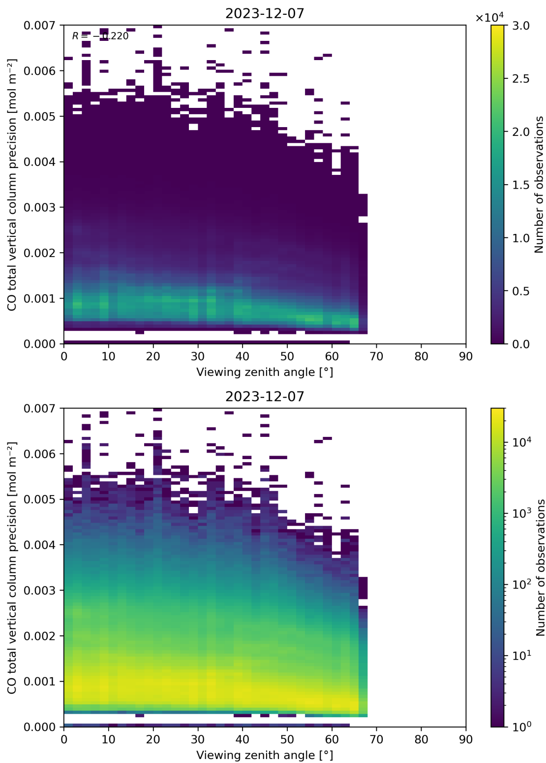
Figure 71: Scatter density plot of “Viewing zenith angle” against “CO total vertical column precision” for 2023-12-06 to 2023-12-08.
