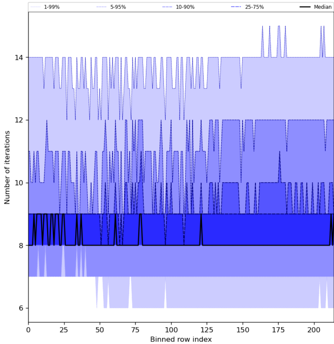
Figure 32: Along track statistics of “Number of iterations” for 2023-12-06 to 2023-12-08
