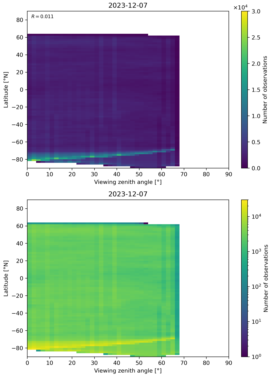
Figure 74: Scatter density plot of “Viewing zenith angle” against “Latitude” for 2023-12-06 to 2023-12-08.
