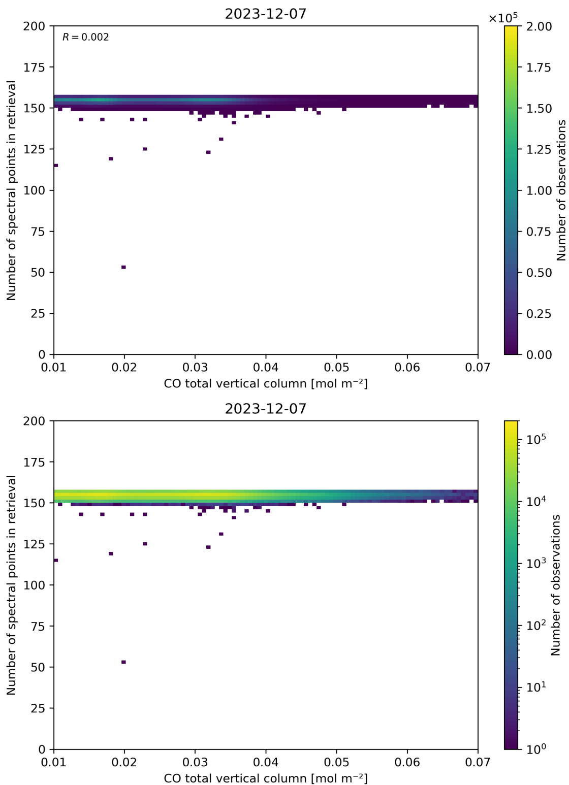
Figure 43: Scatter density plot of “CO total vertical column” against “Number of spectral points in retrieval” for 2023-12-06 to 2023-12-08.
