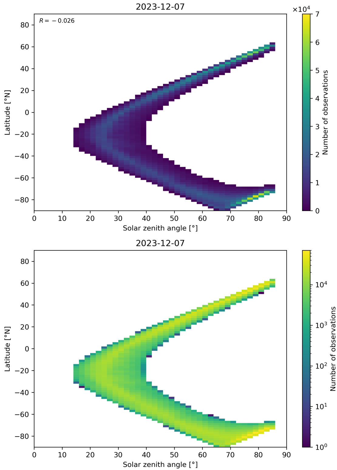
Figure 66: Scatter density plot of “Solar zenith angle” against “Latitude” for 2023-12-06 to 2023-12-08.
