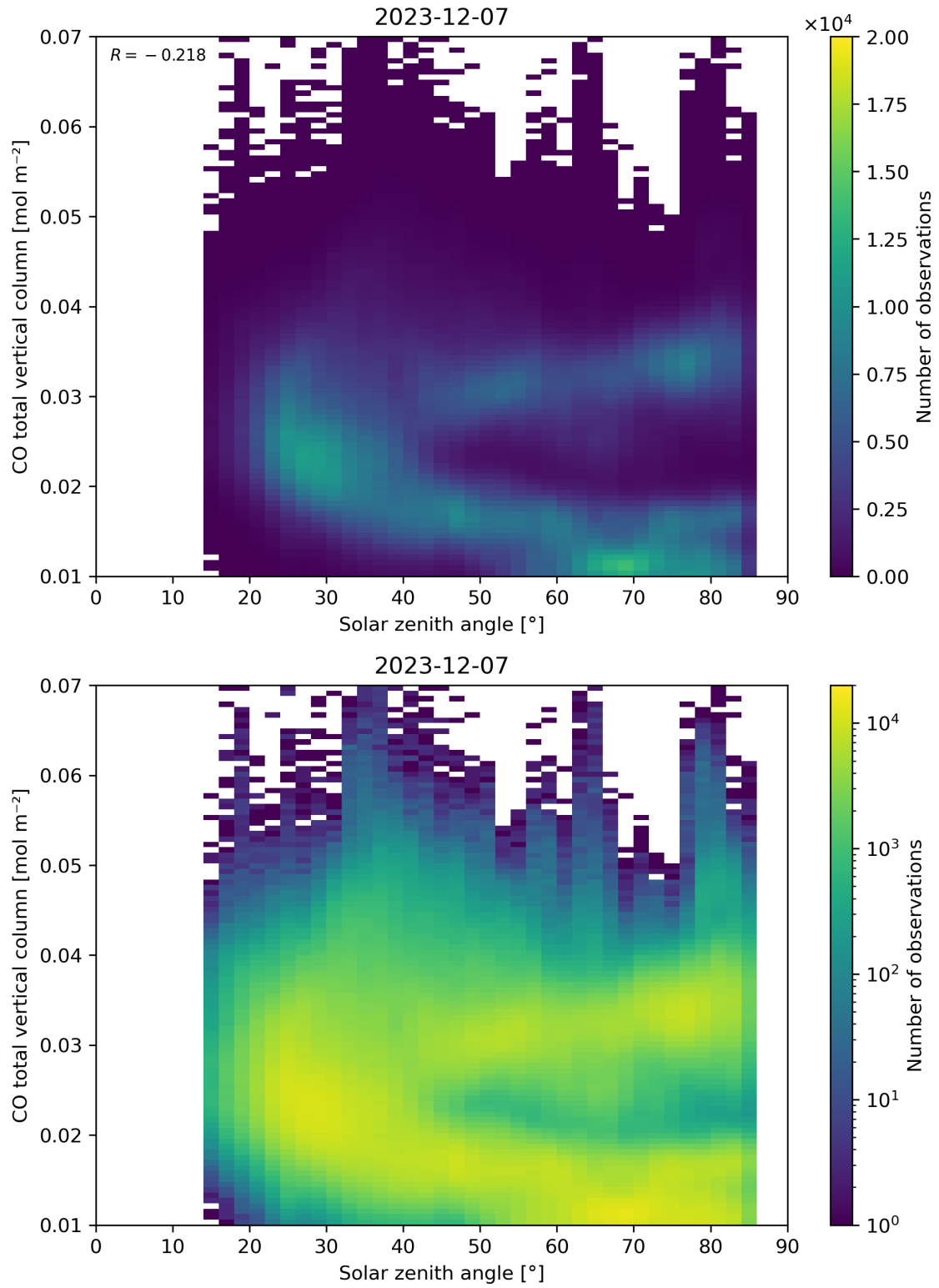
Figure 61: Scatter density plot of “Solar zenith angle” against “CO total vertical column” for 2023-12-06 to 2023-12-08.
