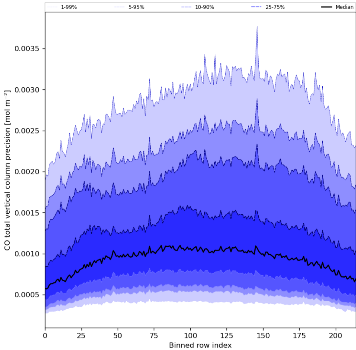
Figure 28: Along track statistics of “CO total vertical column precision” for 2023-12-06 to 2023-12-08
