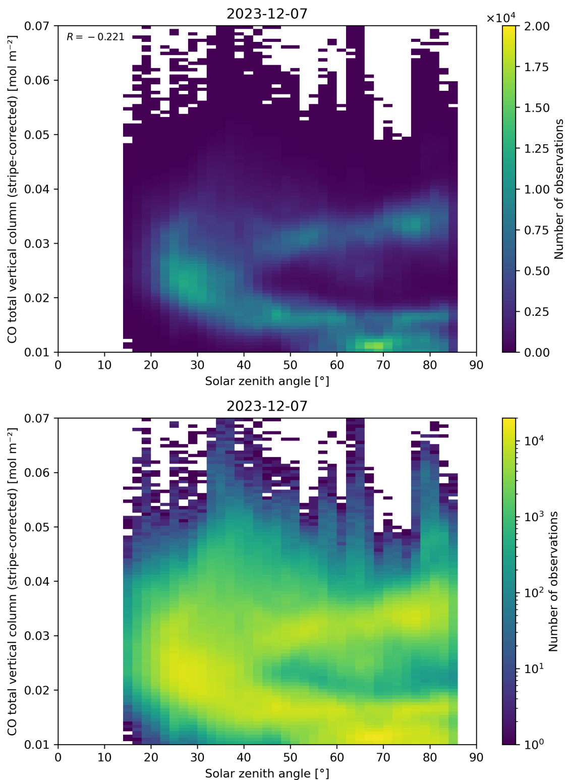
Figure 62: Scatter density plot of “Solar zenith angle” against “CO total vertical column (stripe-corrected)” for 2023-12-06 to 2023-12-08.
