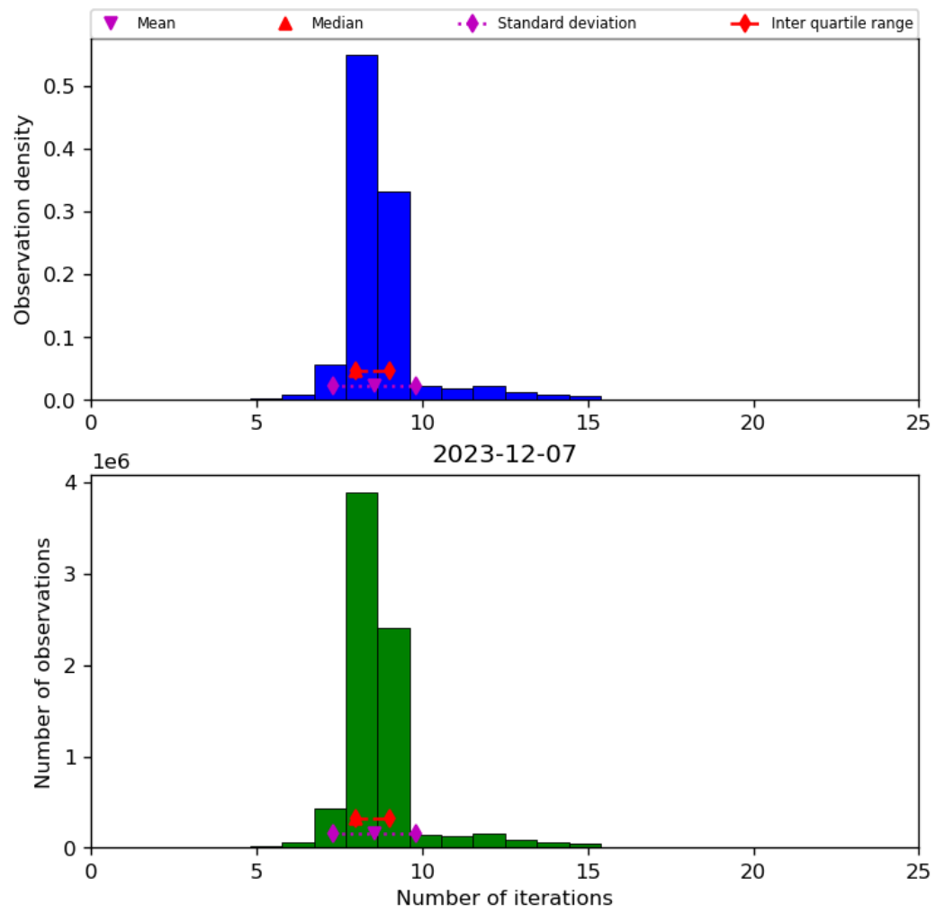
Figure 24: Histogram of “Number of iterations” for 2023-12-06 to 2023-12-08
