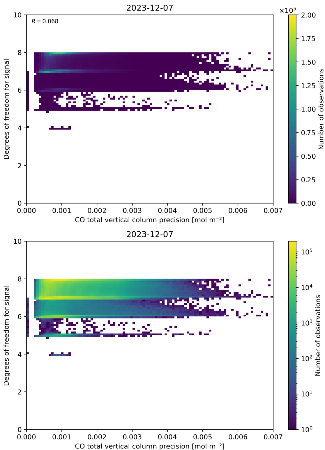
Figure 45: Scatter density plot of “CO total vertical column precision” against “Degrees of freedom for signal” for 2023-12-06 to 2023-12-08.
