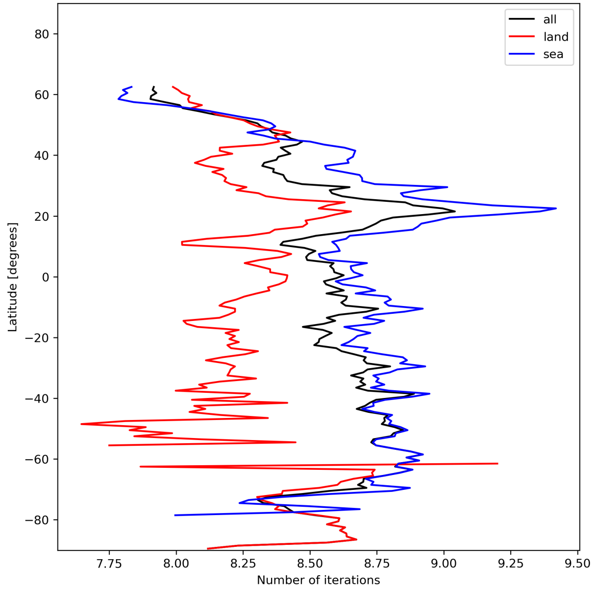
Figure 16: Zonal average of “Number of iterations” for 2023-12-06 to 2023-12-08.
