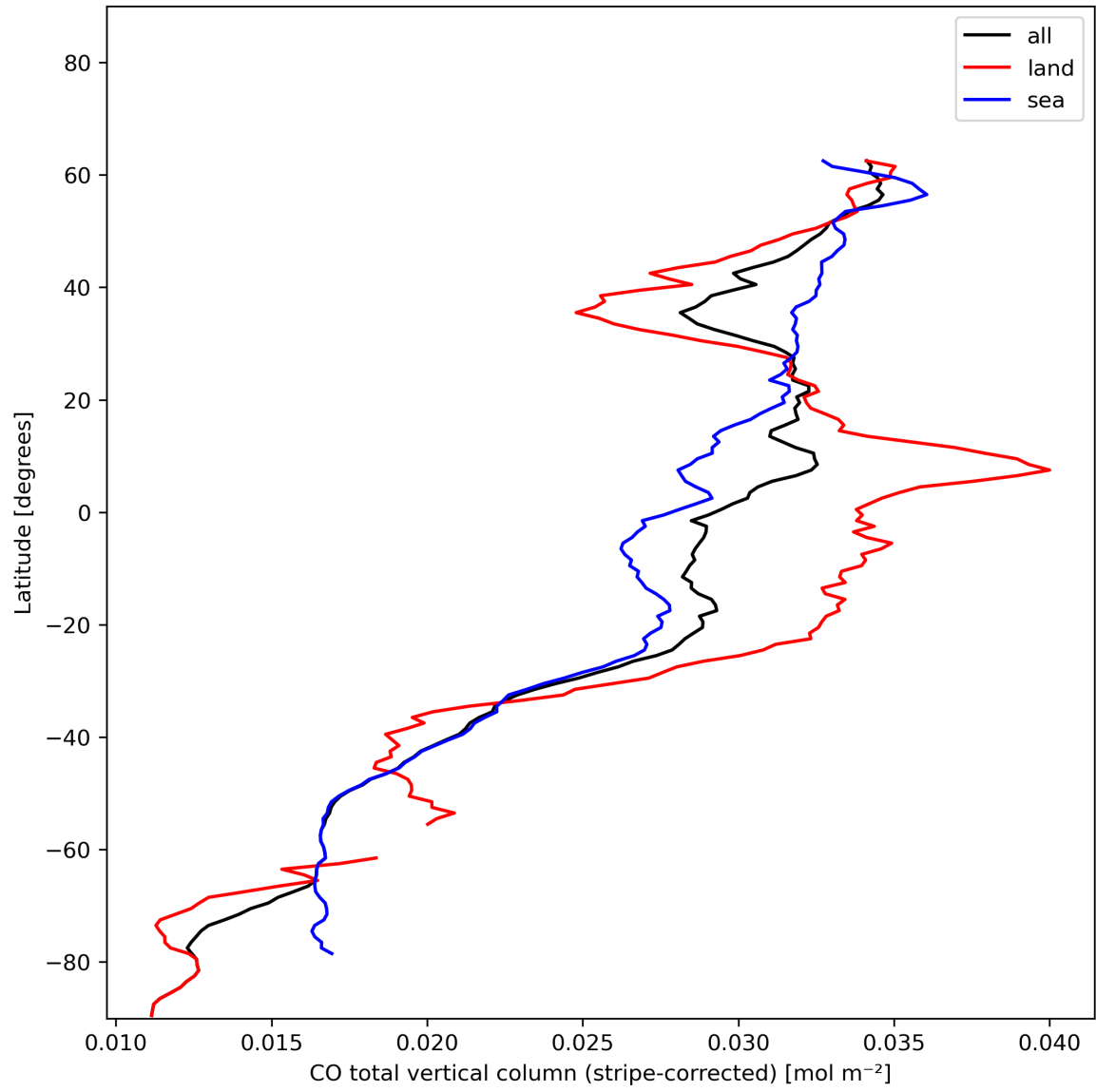
Figure 11: Zonal average of “CO total vertical column (stripe-corrected)” for 2023-12-06 to 2023-12-08.
