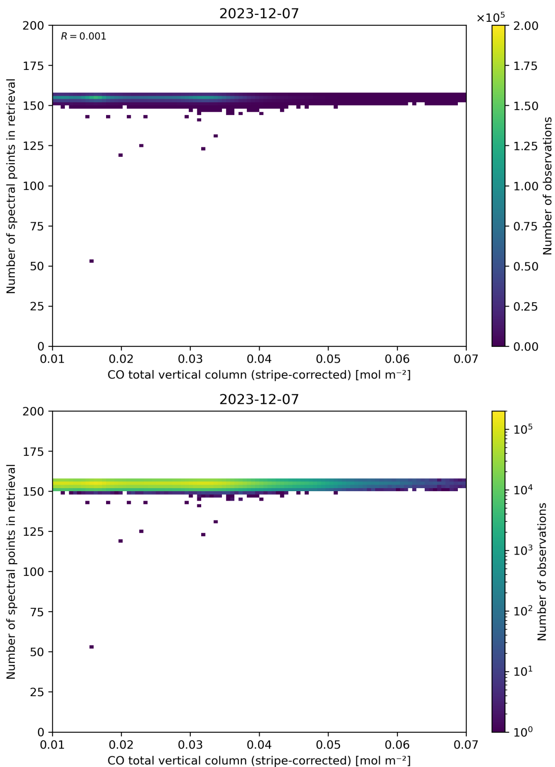
Figure 40: Scatter density plot of “CO total vertical column (stripe-corrected)” against “Number of spectral points in retrieval” for 2023-12-06 to 2023-12-08.
