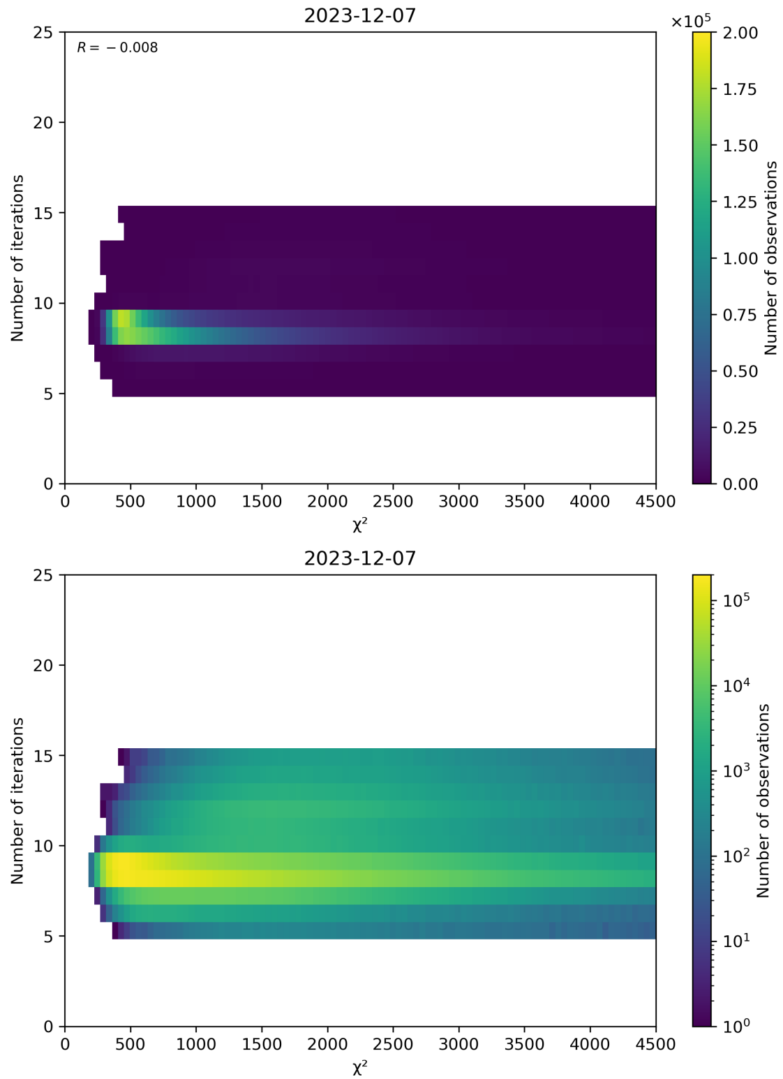
Figure 49: Scatter density plot of “ \chi^2 ” against “Number of iterations” for 2023-12-06 to 2023-12-08.
