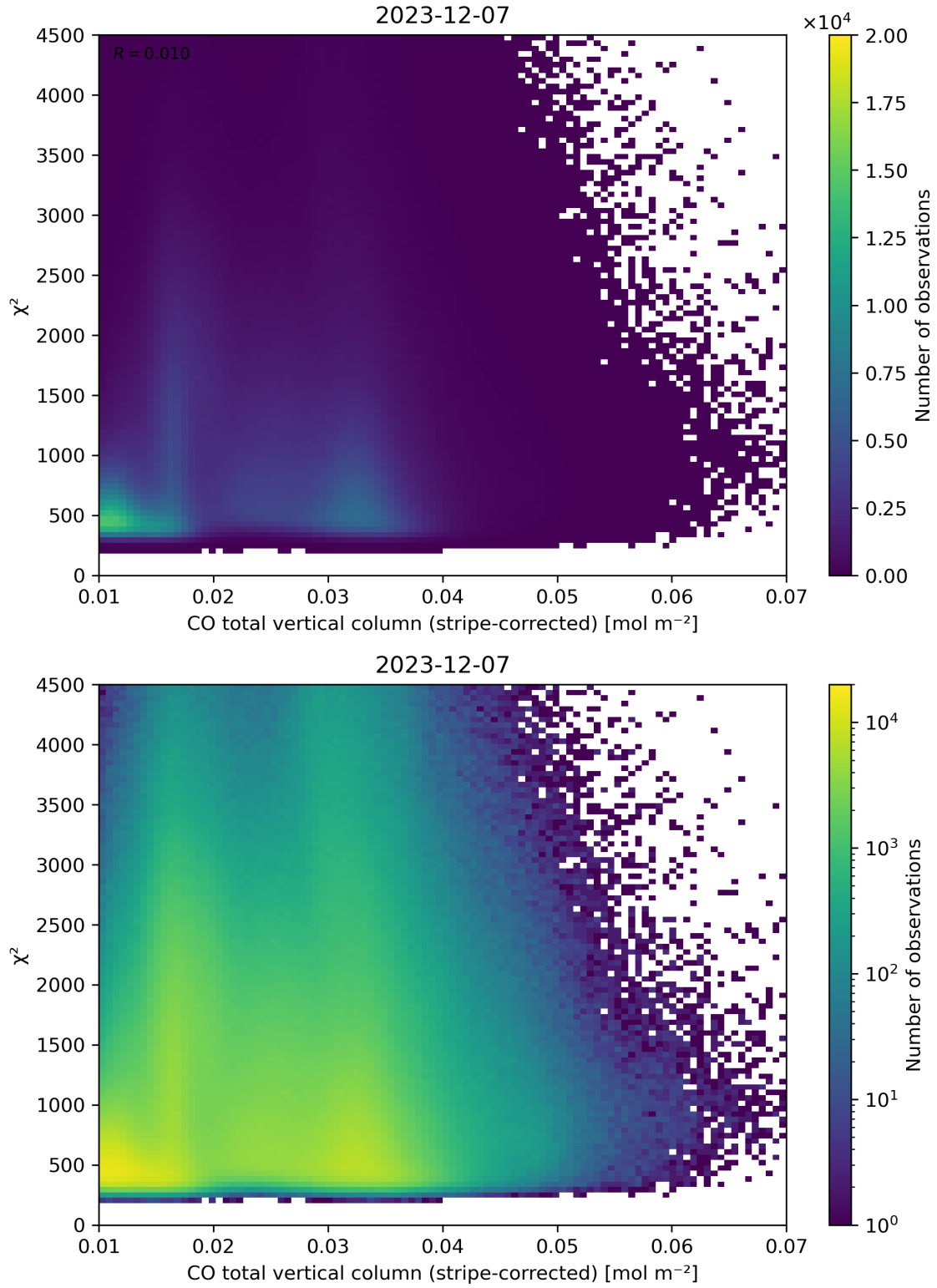
Figure 37: Scatter density plot of “CO total vertical column (stripe-corrected)” against “ \chi^2 ” for 2023-12-06 to 2023-12-08.
