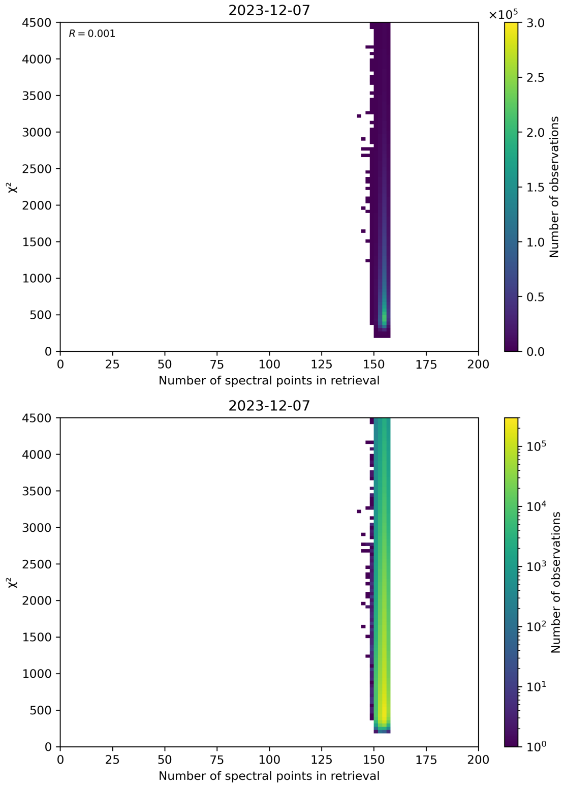
Figure 58: Scatter density plot of “Number of spectral points in retrieval” against “ \chi^2 ” for 2023-12-06 to 2023-12-08.
