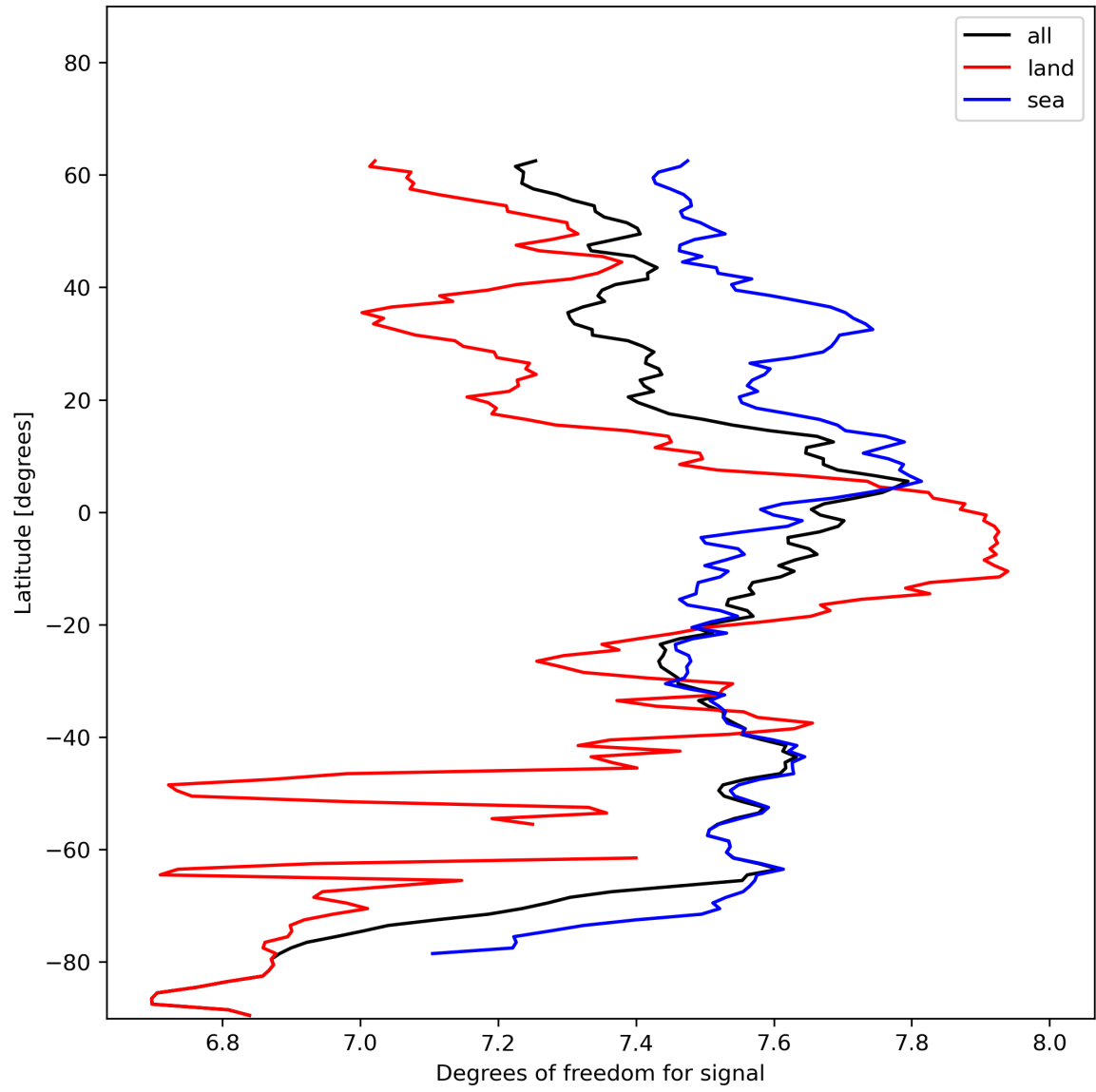
Figure 15: Zonal average of “Degrees of freedom for signal” for 2023-12-06 to 2023-12-08.
