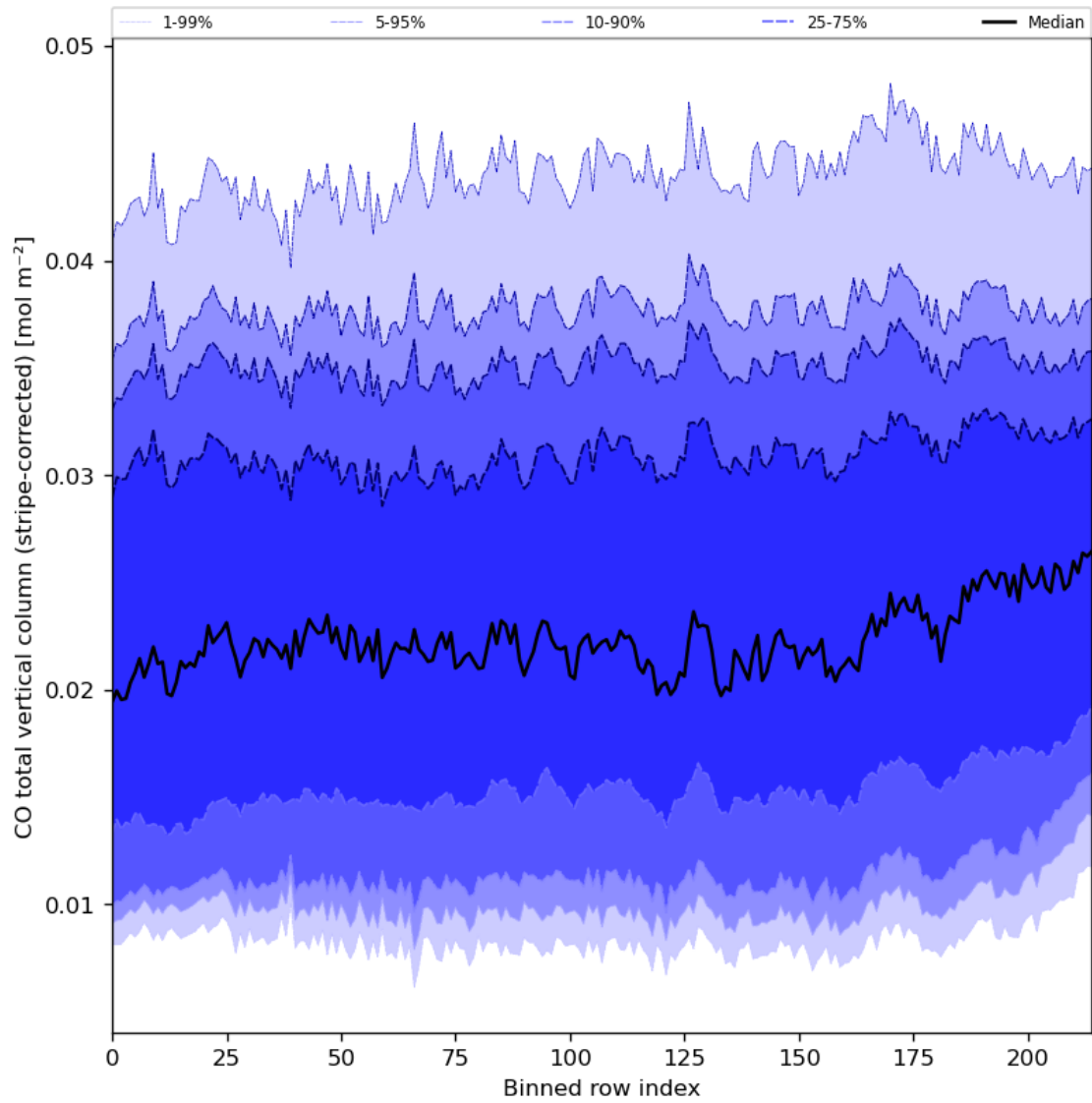
Figure 27: Along track statistics of “CO total vertical column (stripe-corrected)” for 2023-12-06 to 2023-12-08
