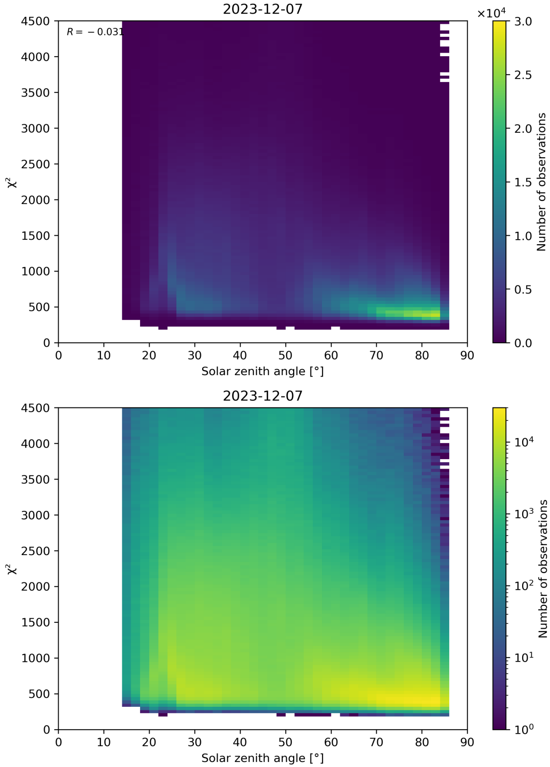
Figure 64: Scatter density plot of “Solar zenith angle” against “ \chi^2 ” for 2023-12-06 to 2023-12-08.
