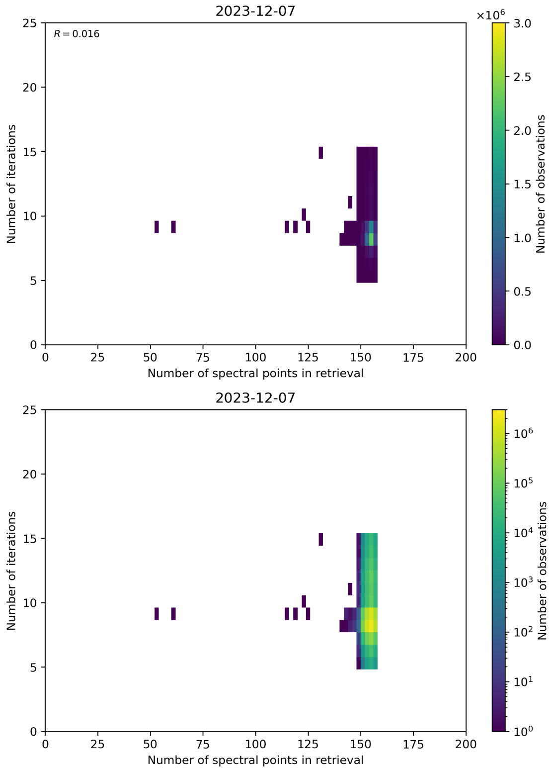
Figure 60: Scatter density plot of “Number of spectral points in retrieval” against “Number of iterations” for 2023-12-06 to 2023-12-08.
