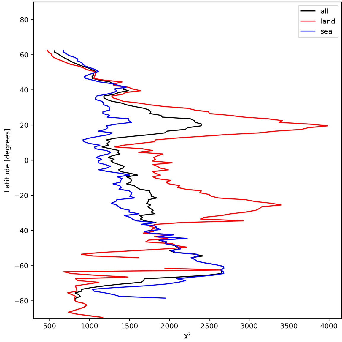
Figure 14: Zonal average of “ \chi^2 ” for 2023-12-06 to 2023-12-08.
