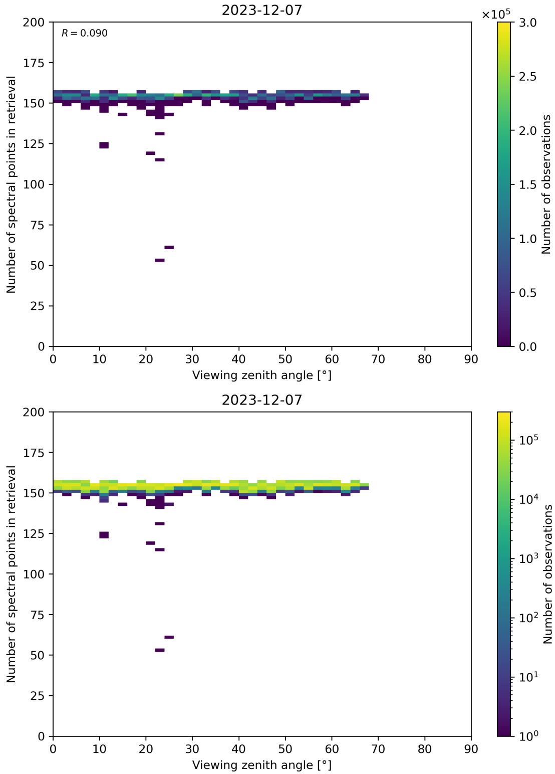
Figure 76: Scatter density plot of “Viewing zenith angle” against “Number of spectral points in retrieval” for 2023-12-06 to 2023-12-08.
