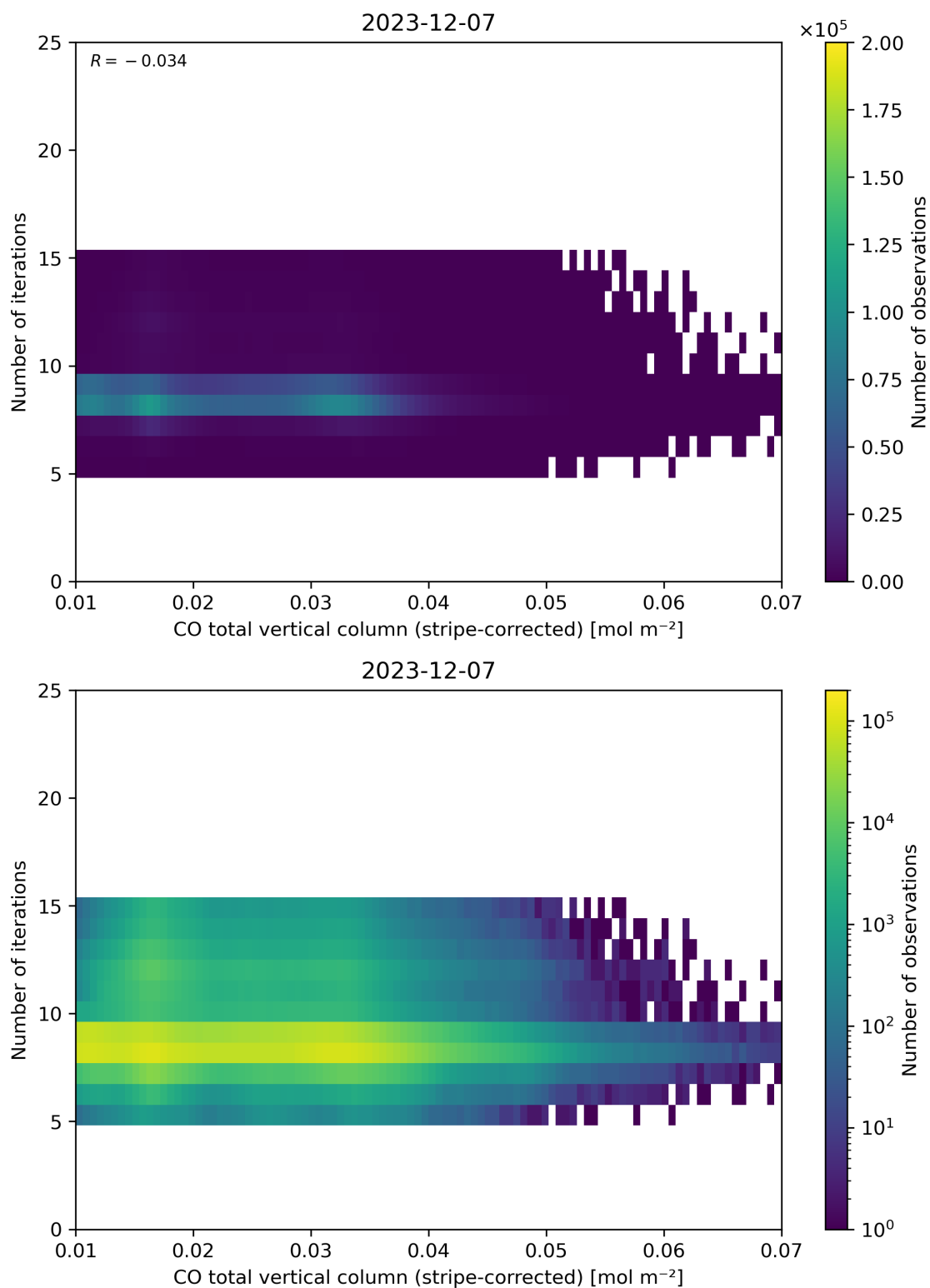
Figure 39: Scatter density plot of “CO total vertical column (stripe-corrected)” against “Number of iterations” for 2023-12-06 to 2023-12-08.
