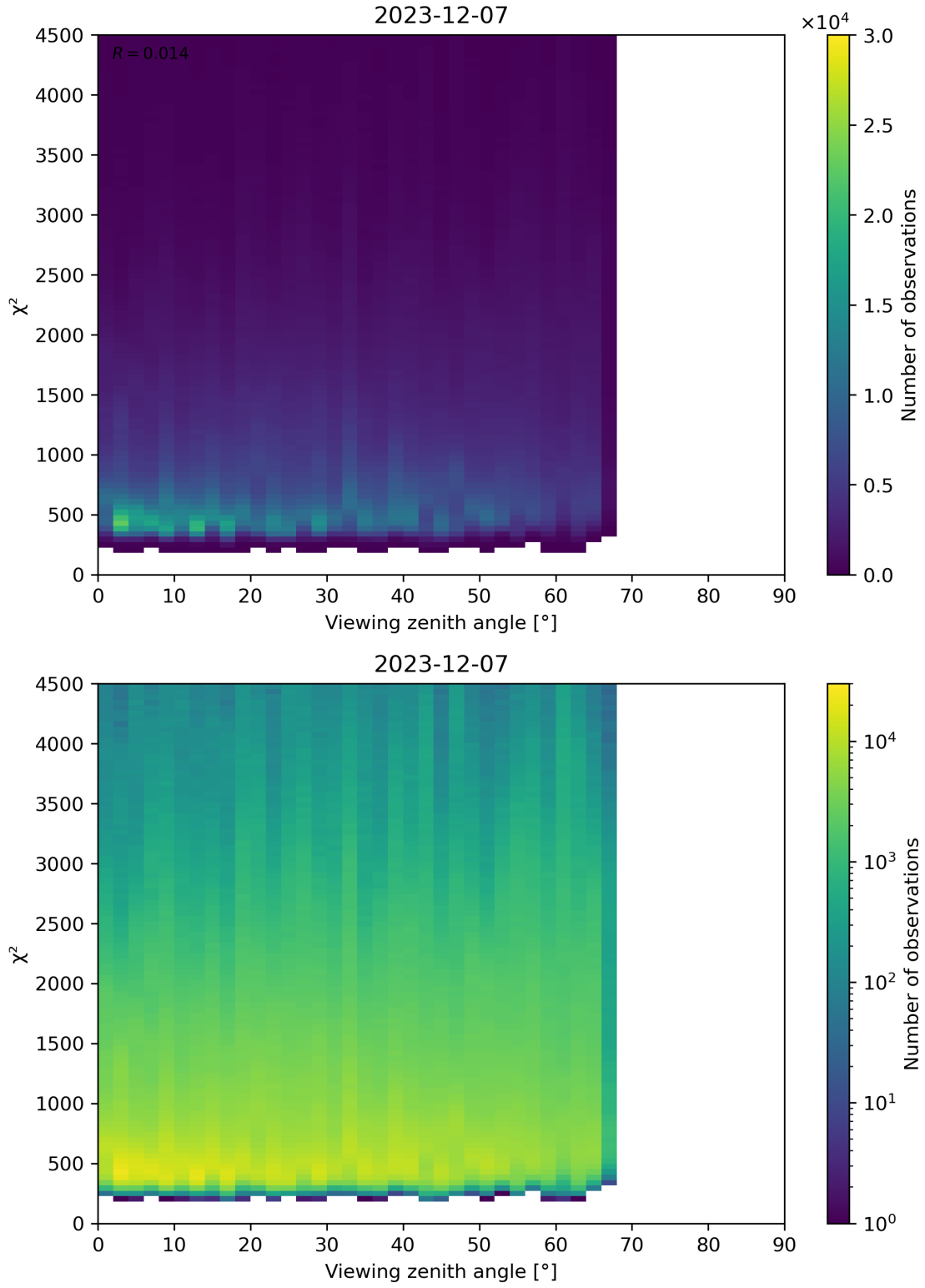
Figure 72: Scatter density plot of “Viewing zenith angle” against “ \chi^2 ” for 2023-12-06 to 2023-12-08.
