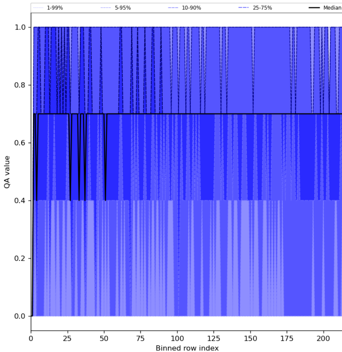
Figure 25: Along track statistics of “QA value” for 2023-12-06 to 2023-12-08
