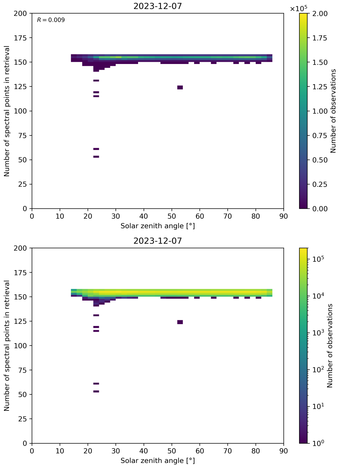
Figure 68: Scatter density plot of “Solar zenith angle” against “Number of spectral points in retrieval” for 2023-12-06 to 2023-12-08.
