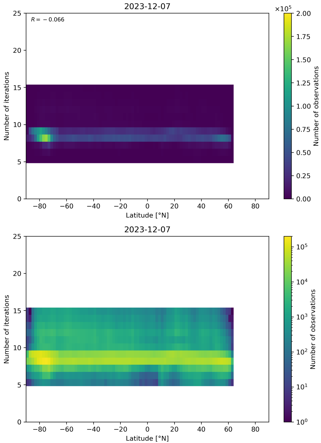
Figure 56: Scatter density plot of “Latitude” against “Number of iterations” for 2023-12-06 to 2023-12-08.
