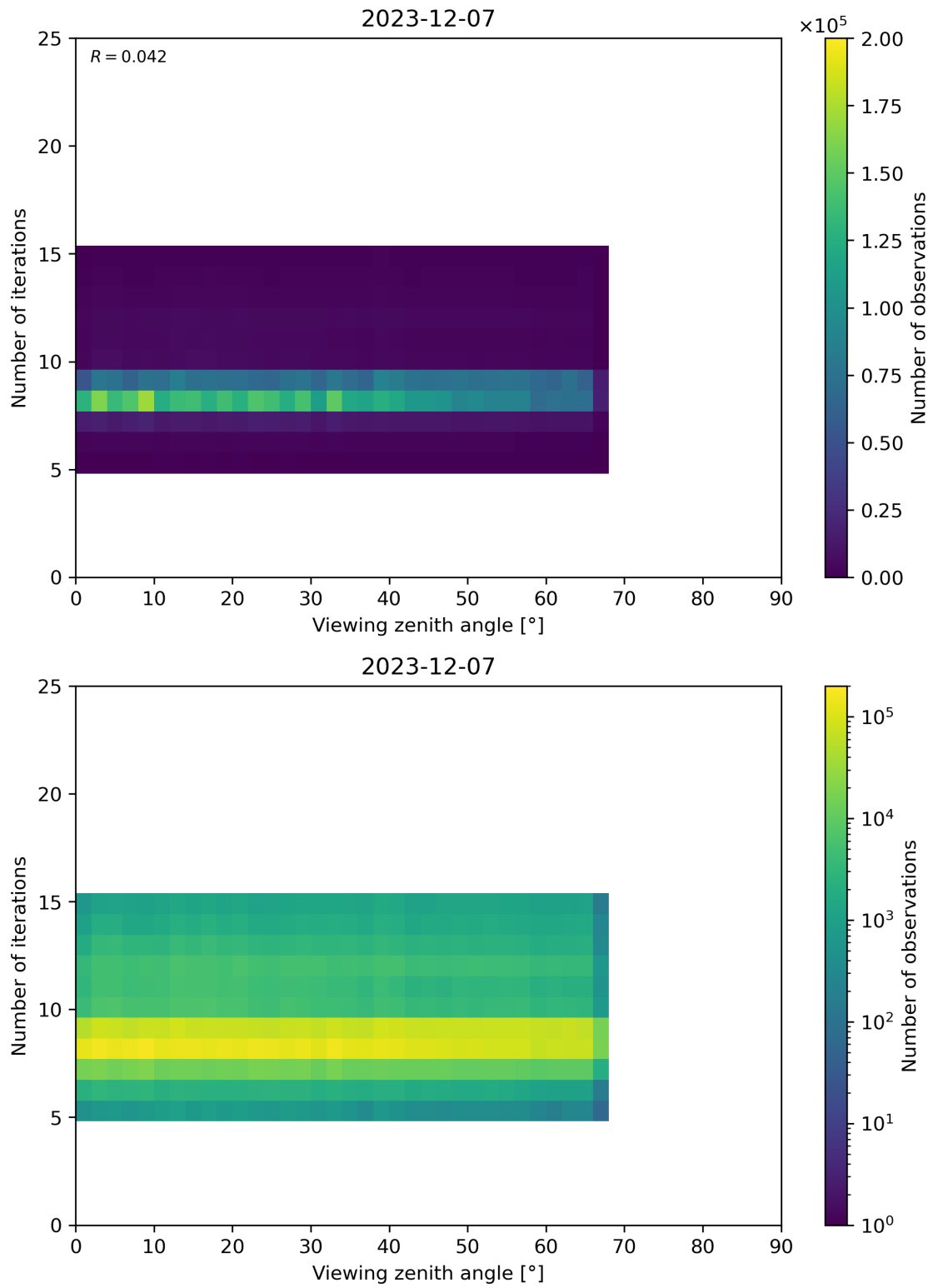
Figure 75: Scatter density plot of “Viewing zenith angle” against “Number of iterations” for 2023-12-06 to 2023-12-08.
