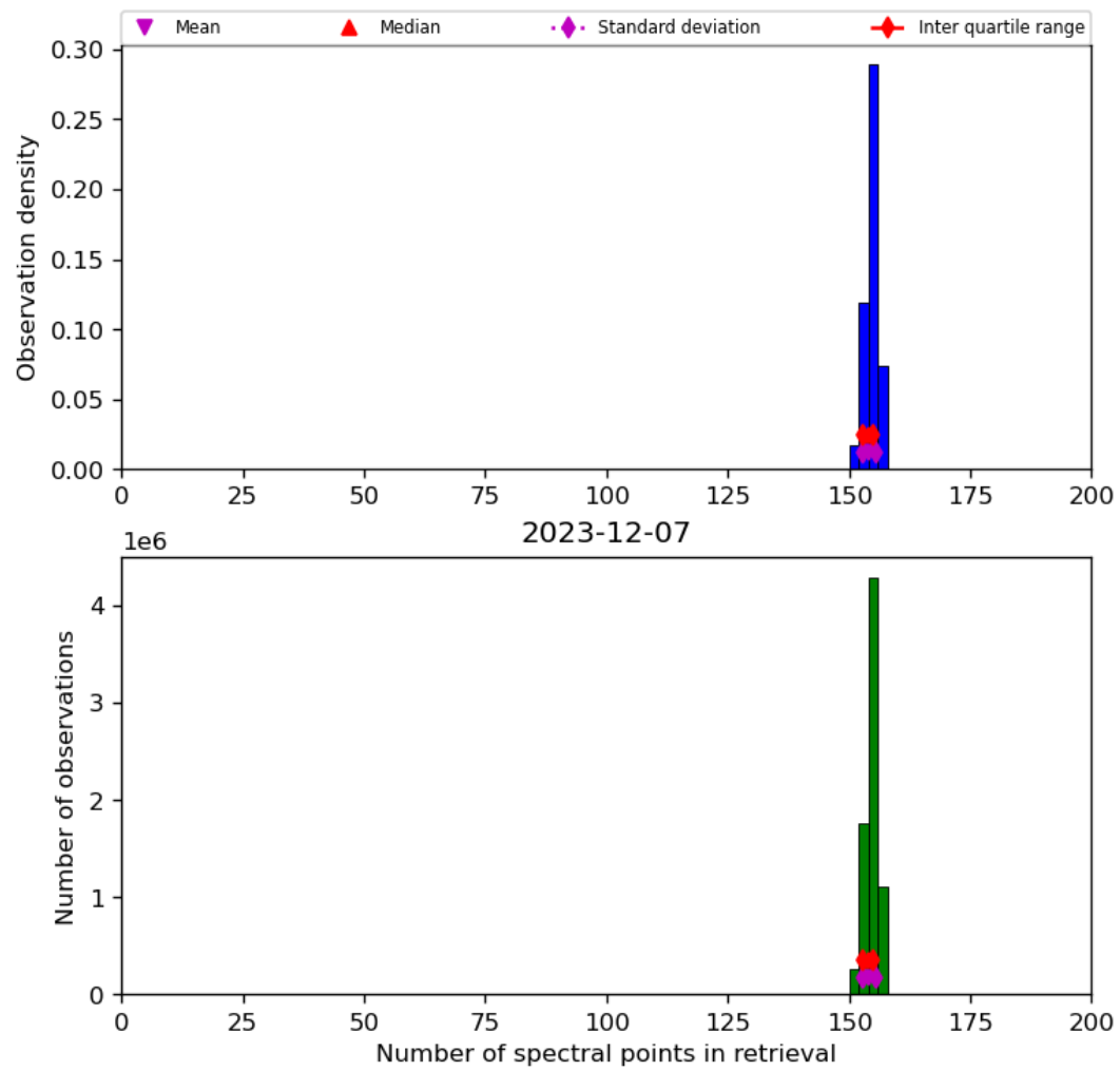
Figure 21: Histogram of “Number of spectral points in retrieval” for 2023-12-06 to 2023-12-08
