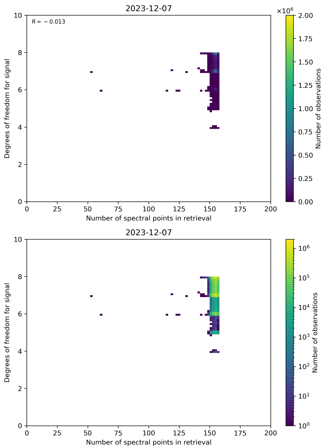
Figure 59: Scatter density plot of “Number of spectral points in retrieval” against “Degrees of freedom for signal” for 2023-12-06 to 2023-12-08.
