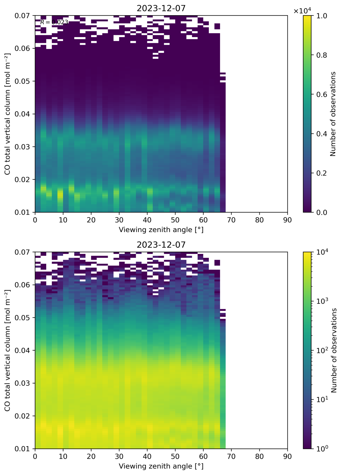
Figure 69: Scatter density plot of “Viewing zenith angle” against “CO total vertical column” for 2023-12-06 to 2023-12-08.
