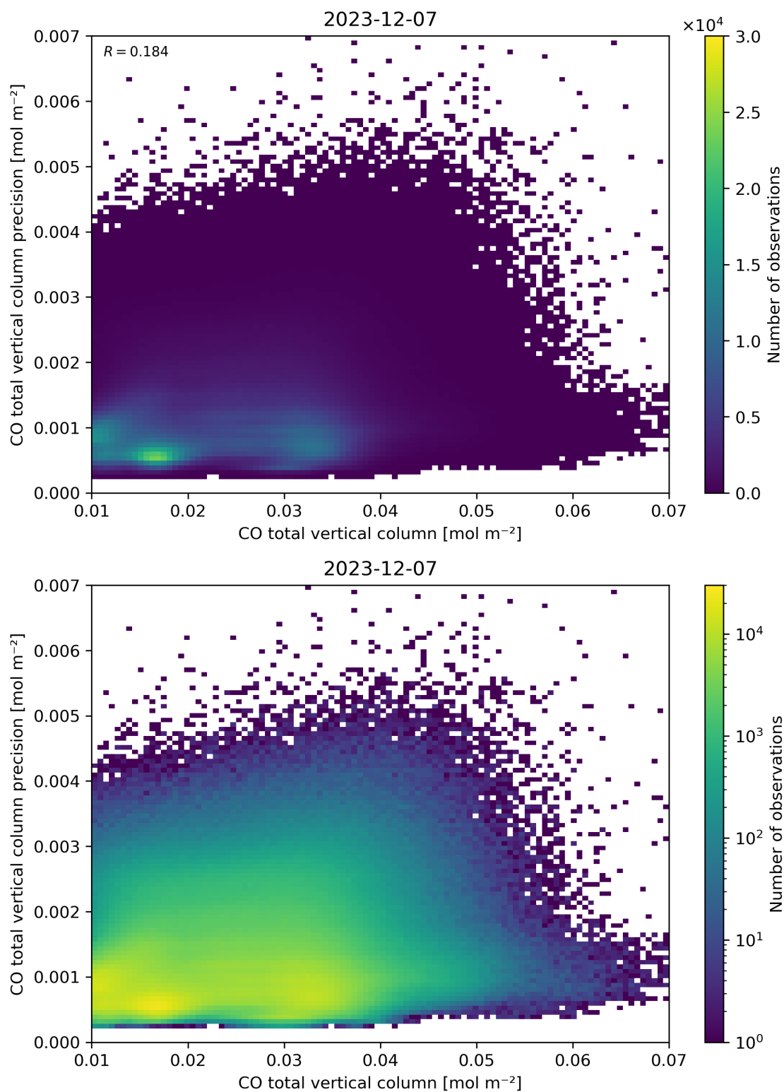
Figure 34: Scatter density plot of “CO total vertical column” against “CO total vertical column precision” for 2023-12-06 to 2023-12-08.
