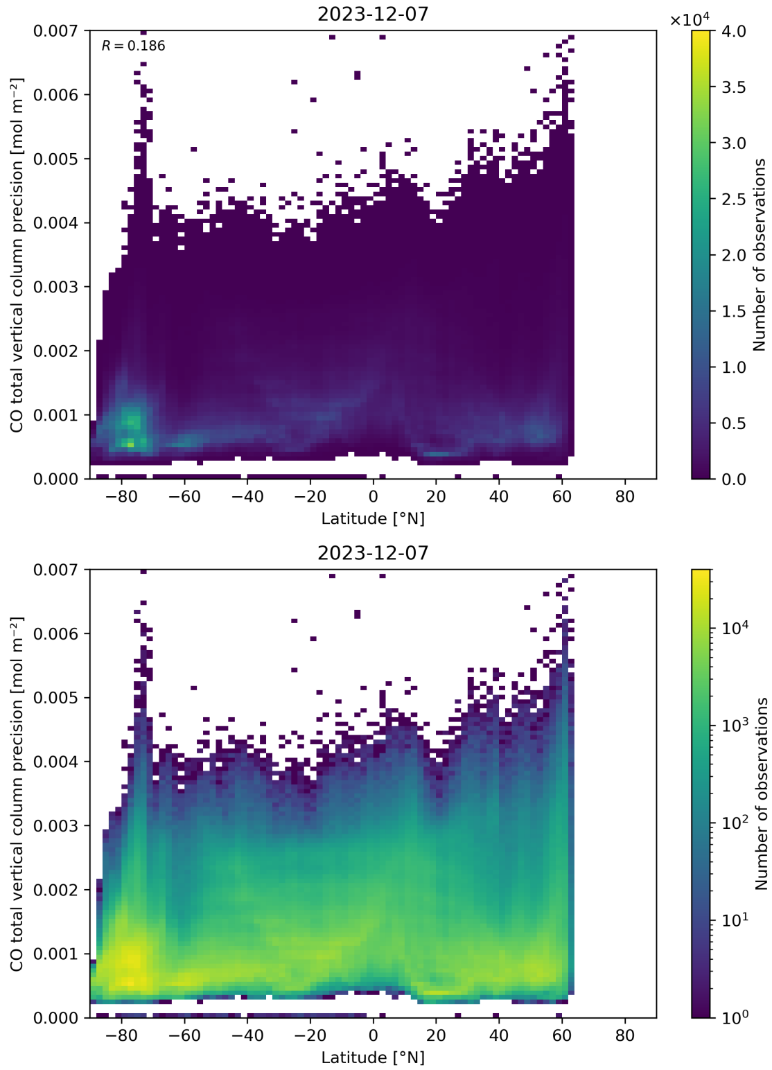
Figure 53: Scatter density plot of “Latitude” against “CO total vertical column precision” for 2023-12-06 to 2023-12-08.
