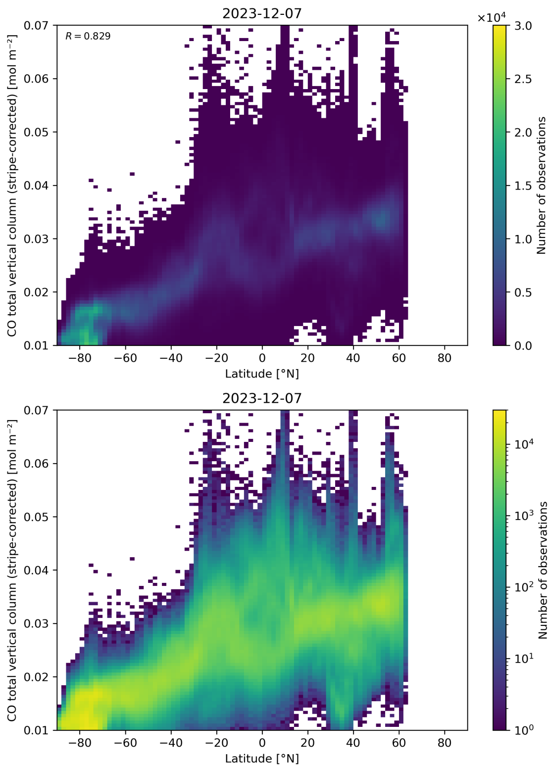
Figure 52: Scatter density plot of “Latitude” against “CO total vertical column (stripe-corrected)” for 2023-12-06 to 2023-12-08.
