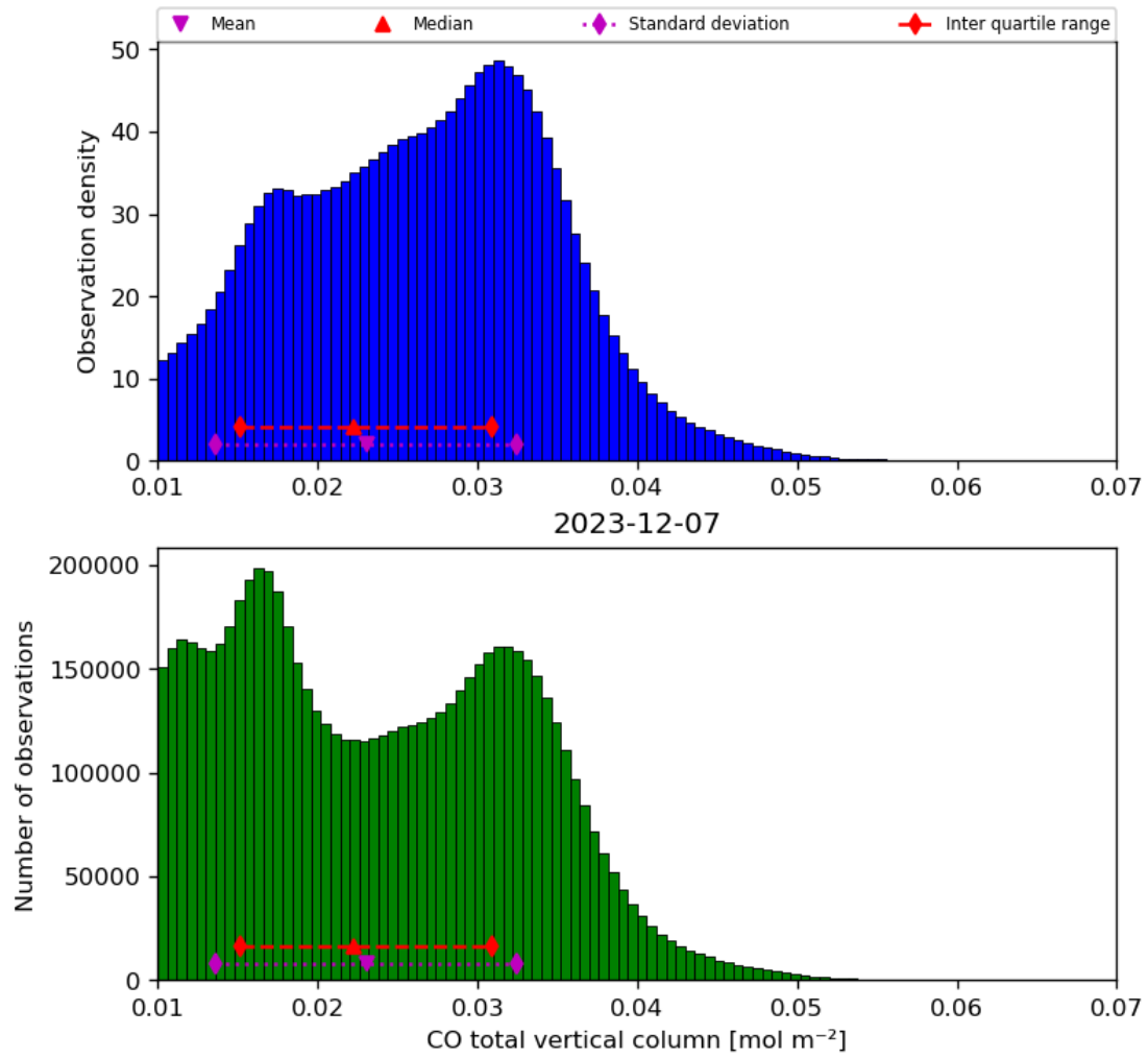
Figure 18: Histogram of “CO total vertical column” for 2023-12-06 to 2023-12-08
