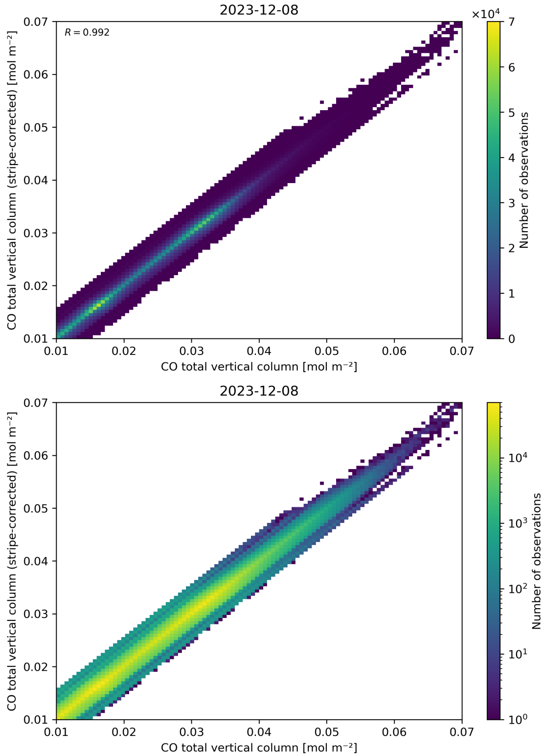
Figure 33: Scatter density plot of “CO total vertical column” against “CO total vertical column (stripe-corrected)” for 2023-12-07 to 2023-12-09.
