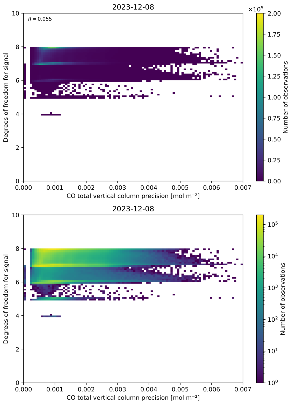
Figure 45: Scatter density plot of “CO total vertical column precision” against “Degrees of freedom for signal” for 2023-12-07 to 2023-12-09.
