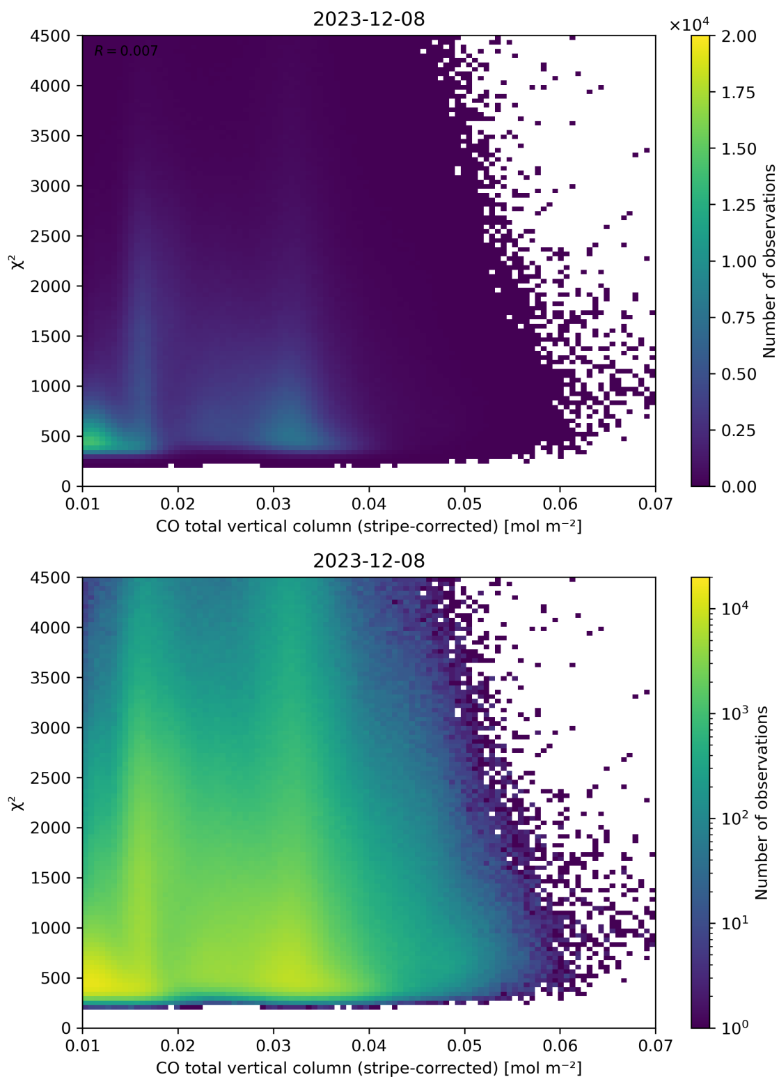
Figure 37: Scatter density plot of “CO total vertical column (stripe-corrected)” against “ \chi^2 ” for 2023-12-07 to 2023-12-09.
