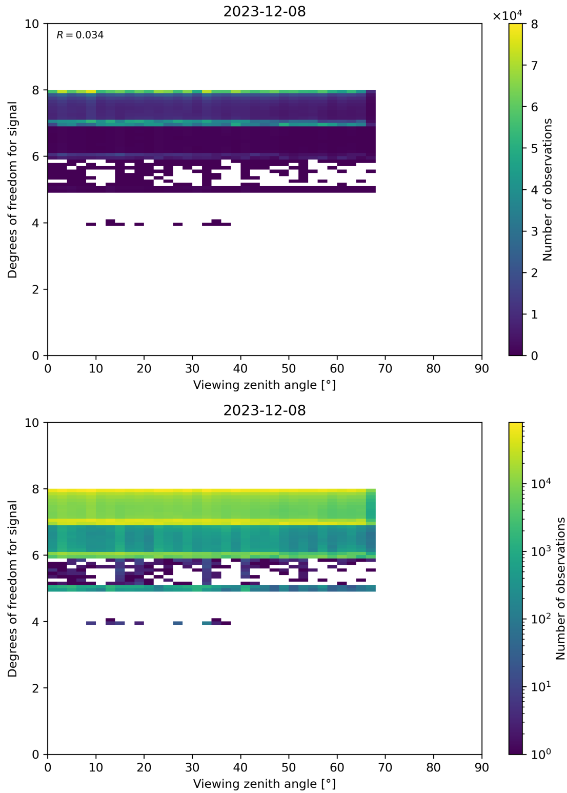
Figure 73: Scatter density plot of “Viewing zenith angle” against “Degrees of freedom for signal” for 2023-12-07 to 2023-12-09.
