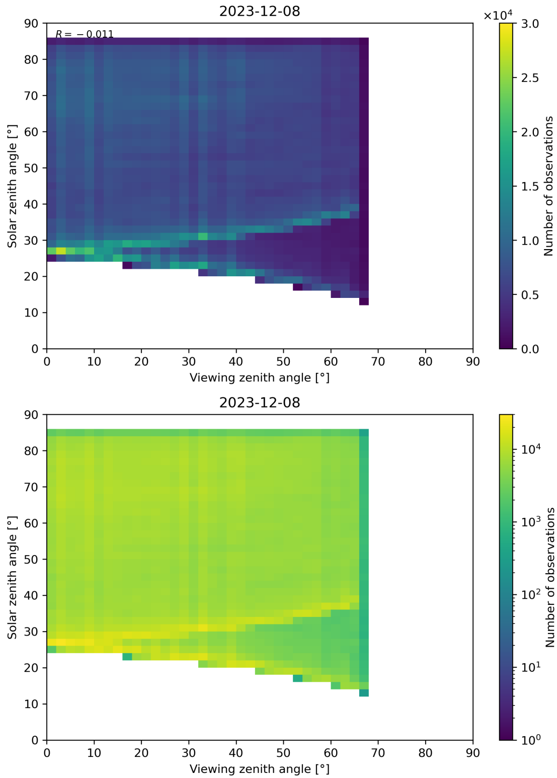
Figure 77: Scatter density plot of “Viewing zenith angle” against “Solar zenith angle” for 2023-12-07 to 2023-12-09.
