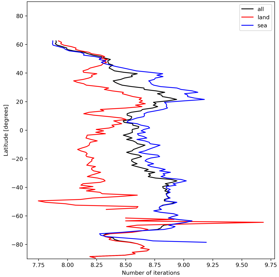
Figure 16: Zonal average of “Number of iterations” for 2023-12-07 to 2023-12-09.
