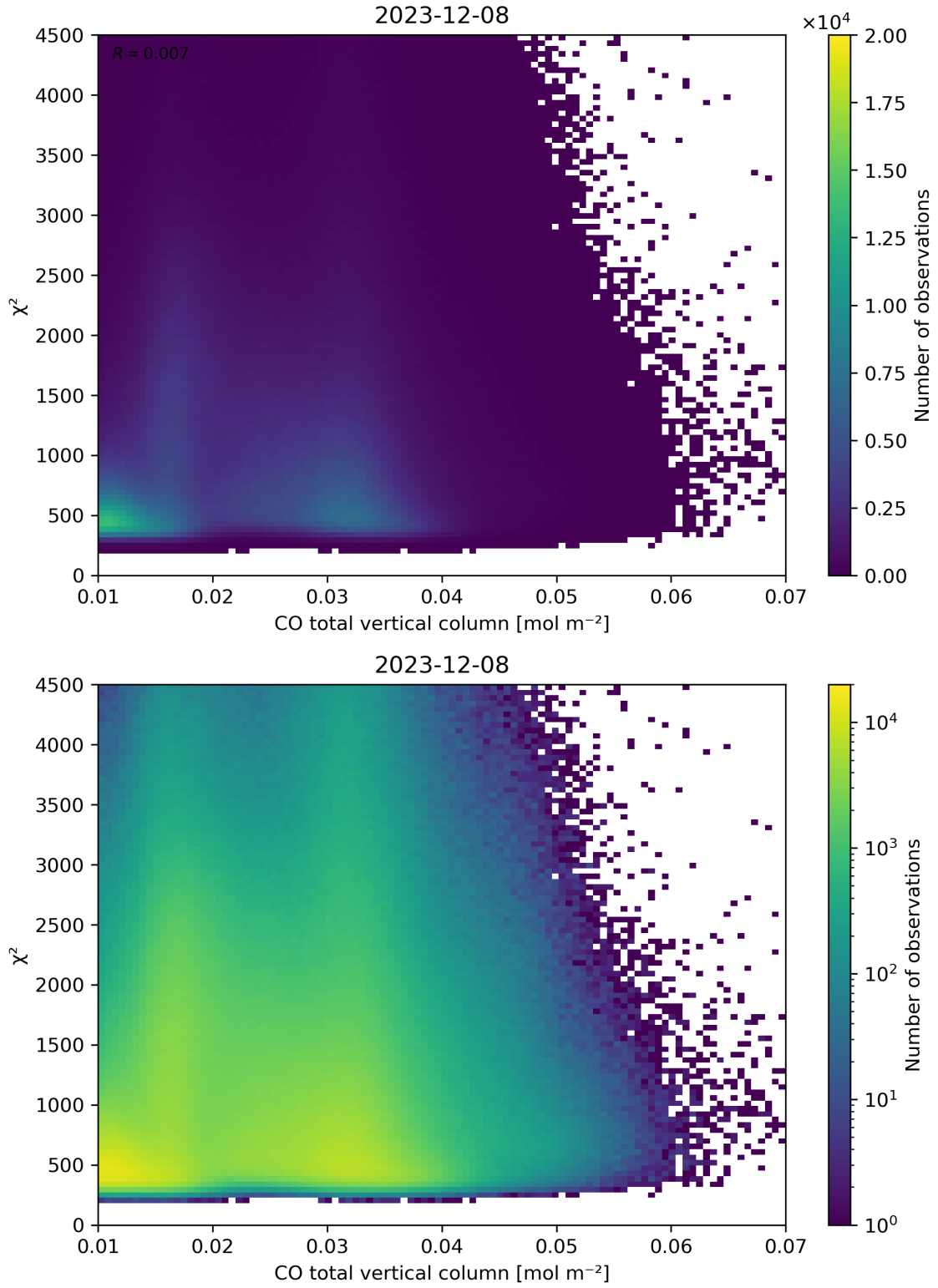
Figure 35: Scatter density plot of “CO total vertical column” against “ \chi^2 ” for 2023-12-07 to 2023-12-09.
