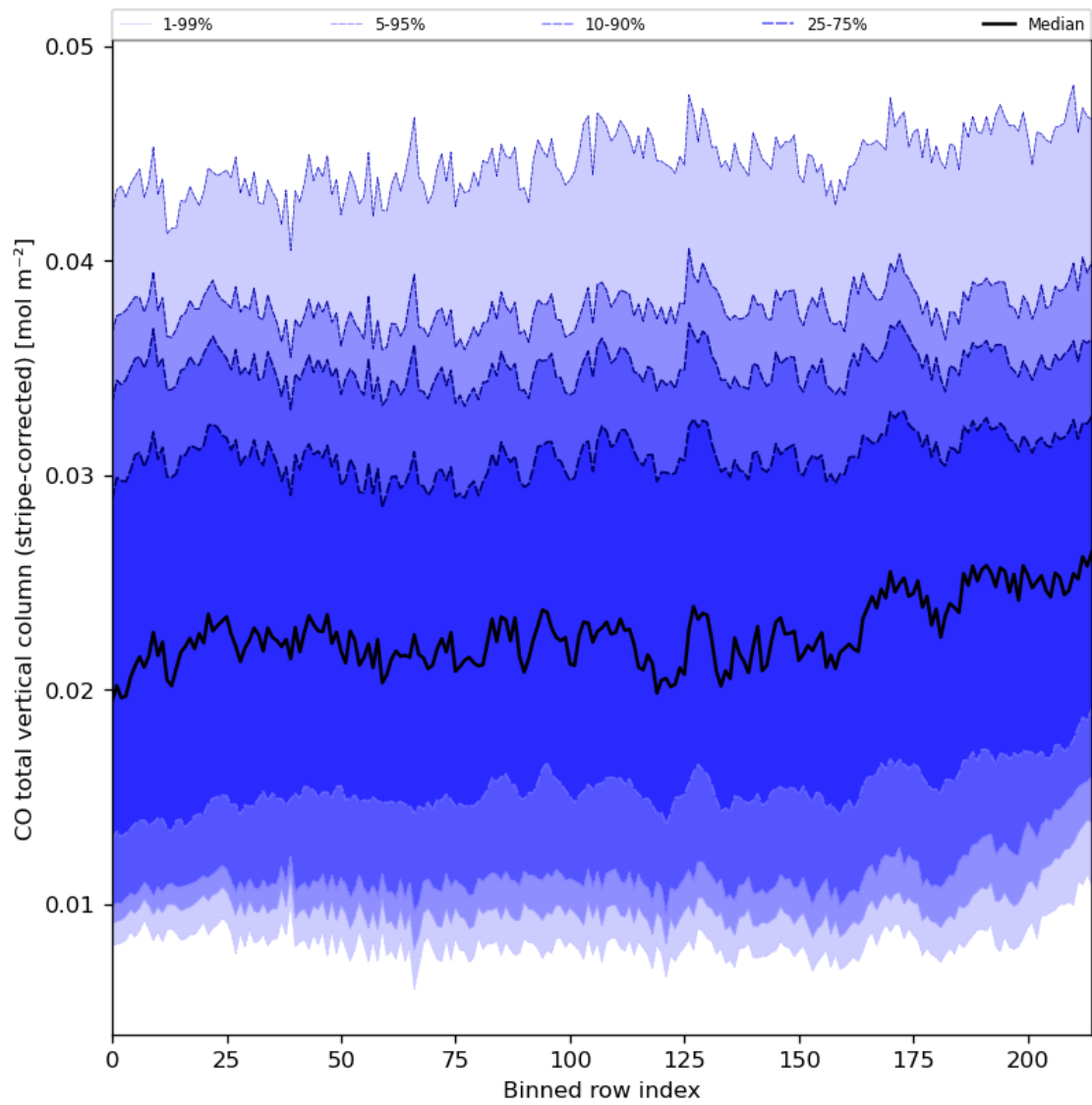
Figure 27: Along track statistics of “CO total vertical column (stripe-corrected)” for 2023-12-07 to 2023-12-09
