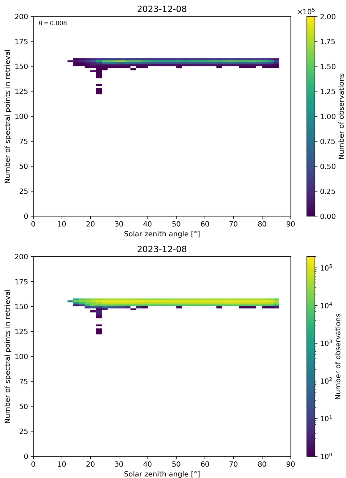
Figure 68: Scatter density plot of “Solar zenith angle” against “Number of spectral points in retrieval” for 2023-12-07 to 2023-12-09.
