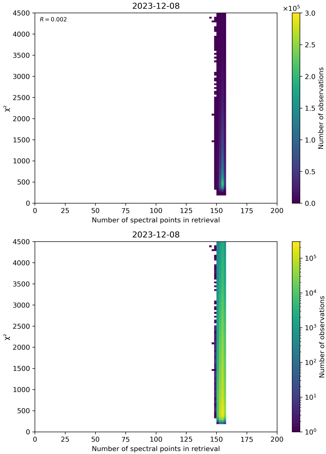
Figure 58: Scatter density plot of “Number of spectral points in retrieval” against “ \chi^2 ” for 2023-12-07 to 2023-12-09.
