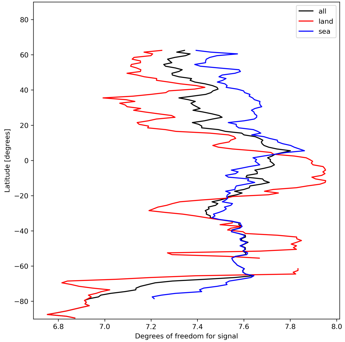
Figure 15: Zonal average of “Degrees of freedom for signal” for 2023-12-07 to 2023-12-09.
