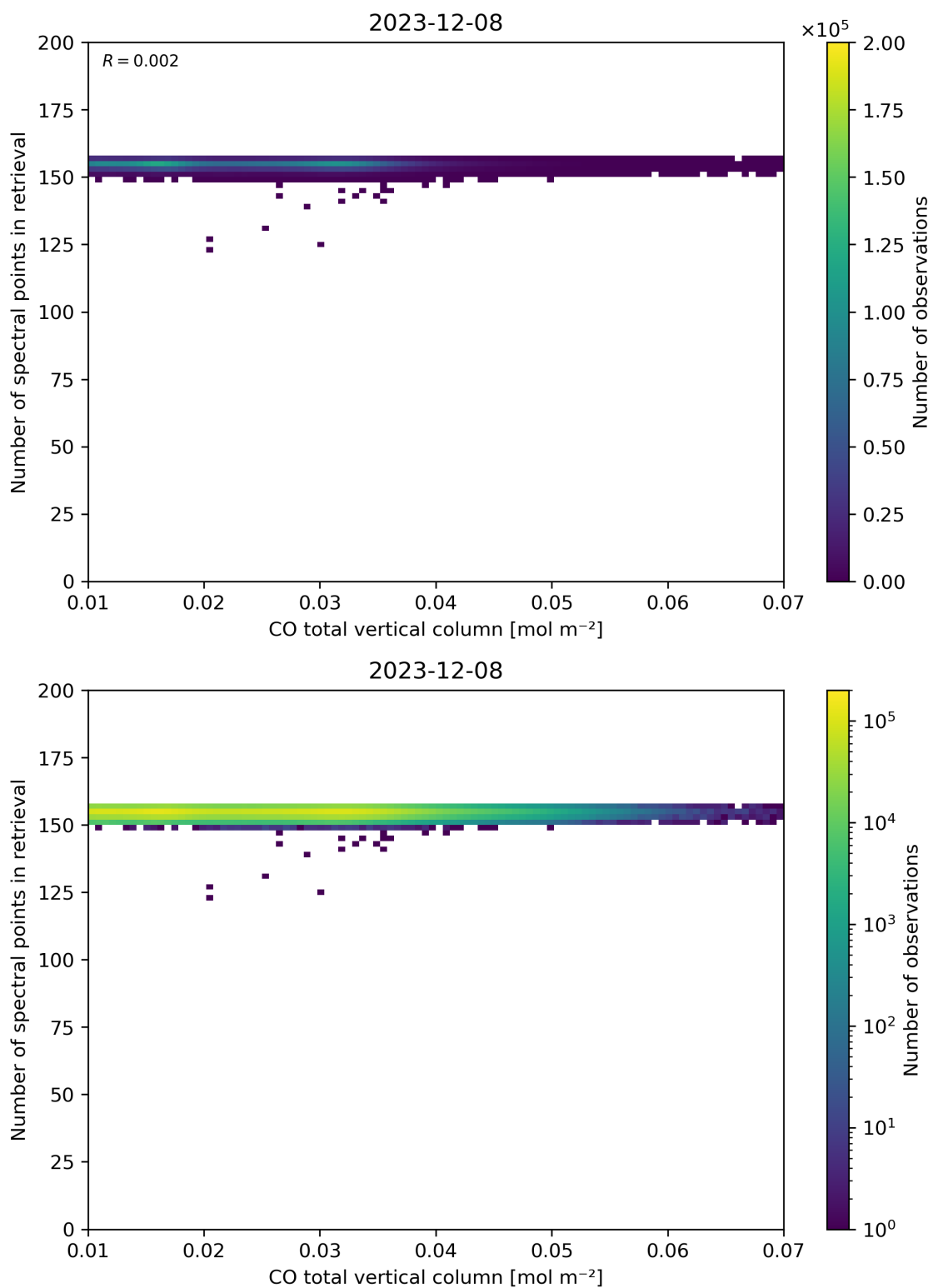
Figure 43: Scatter density plot of “CO total vertical column” against “Number of spectral points in retrieval” for 2023-12-07 to 2023-12-09.
