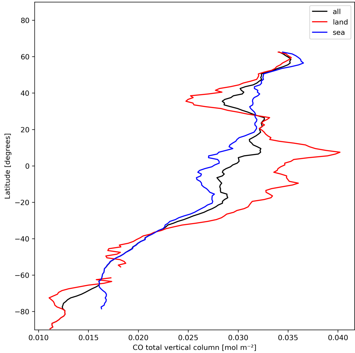
Figure 10: Zonal average of “CO total vertical column” for 2023-12-07 to 2023-12-09.
