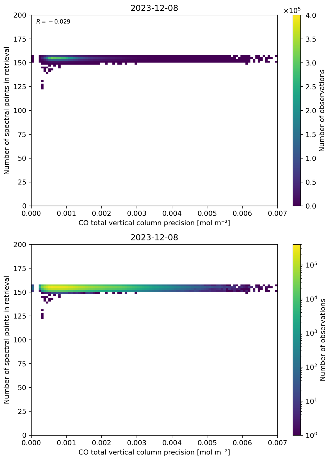
Figure 47: Scatter density plot of “CO total vertical column precision” against “Number of spectral points in retrieval” for 2023-12-07 to 2023-12-09.
