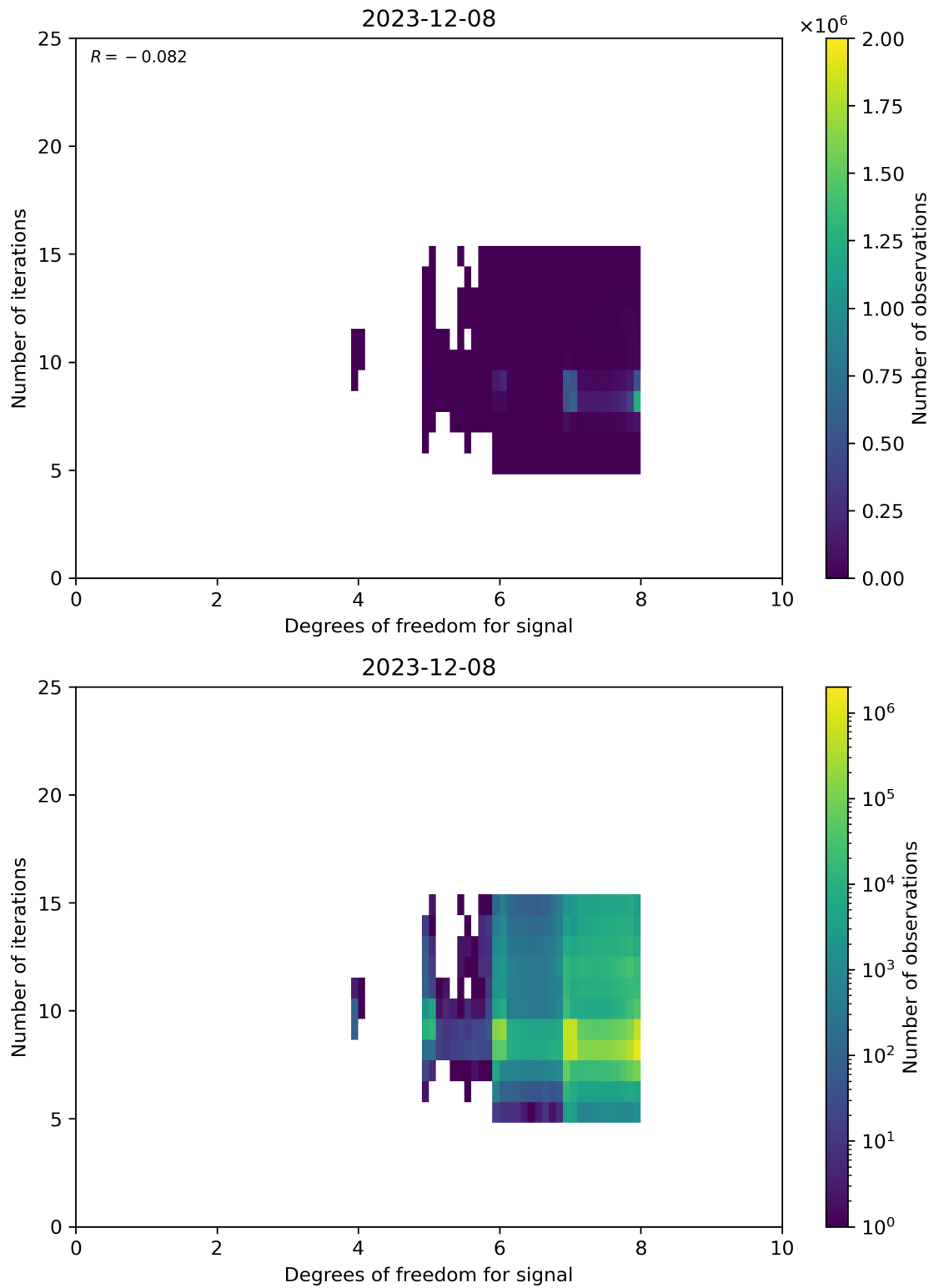
Figure 50: Scatter density plot of “Degrees of freedom for signal” against “Number of iterations” for 2023-12-07 to 2023-12-09.
