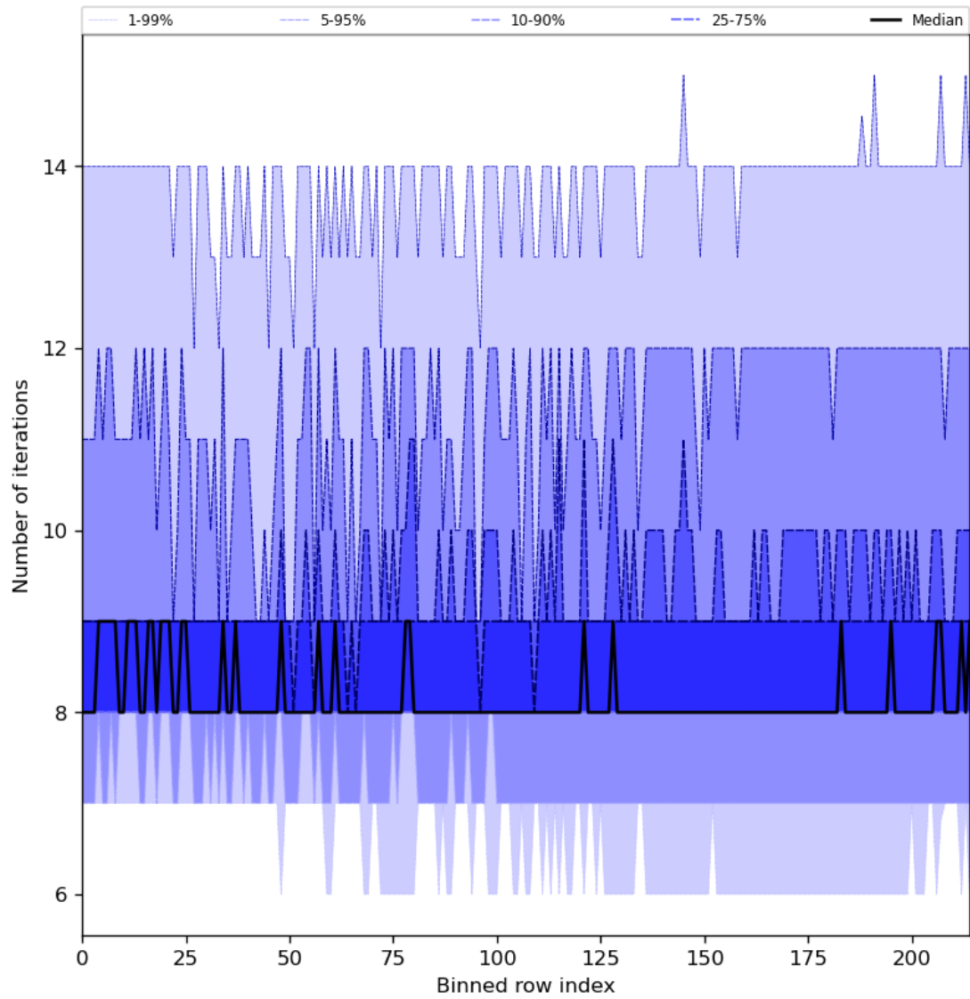
Figure 32: Along track statistics of “Number of iterations” for 2023-12-07 to 2023-12-09
