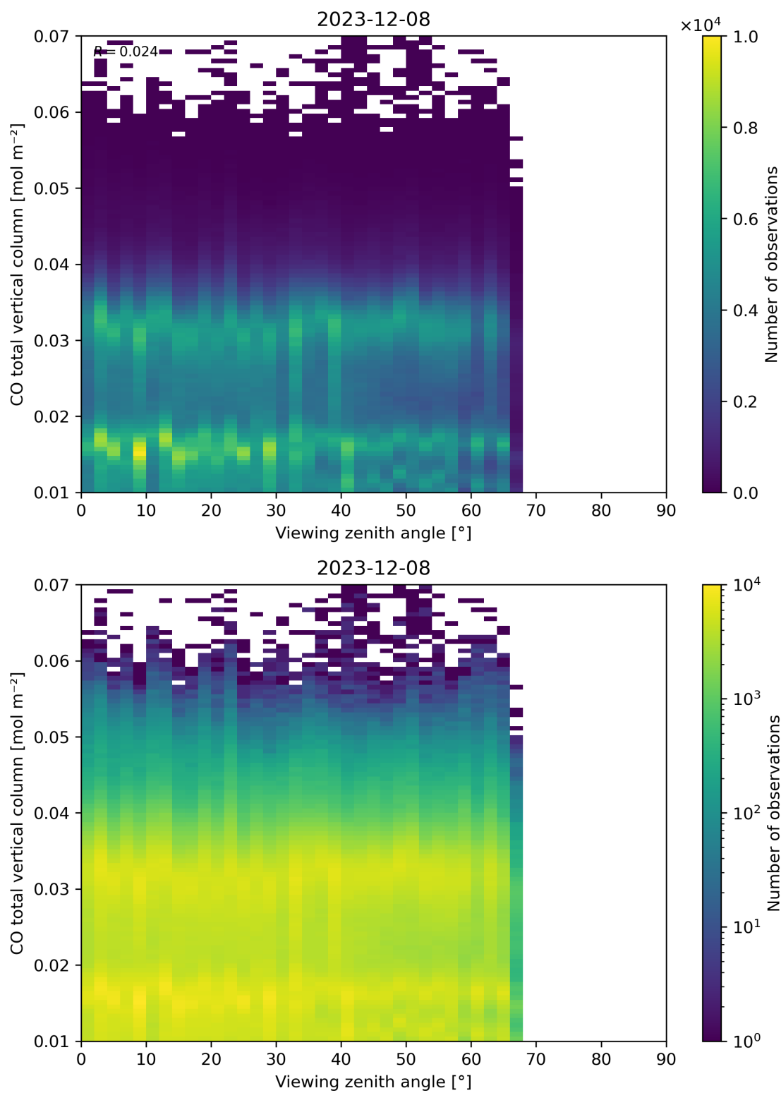
Figure 69: Scatter density plot of “Viewing zenith angle” against “CO total vertical column” for 2023-12-07 to 2023-12-09.
