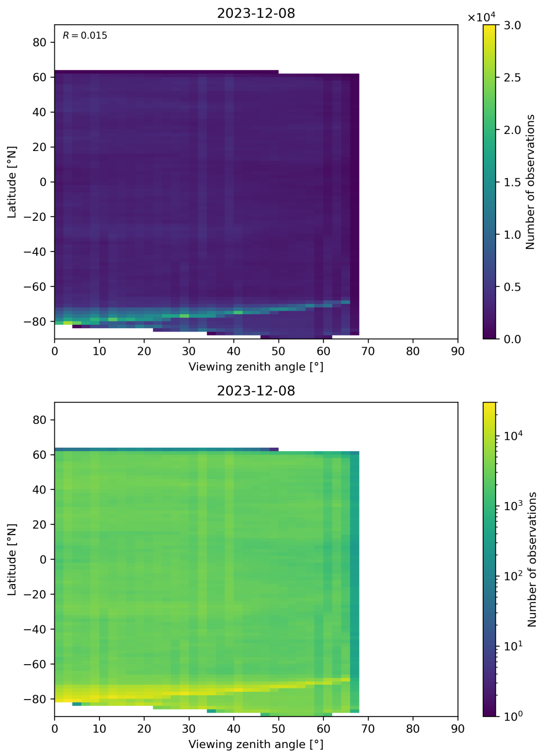
Figure 74: Scatter density plot of “Viewing zenith angle” against “Latitude” for 2023-12-07 to 2023-12-09.
