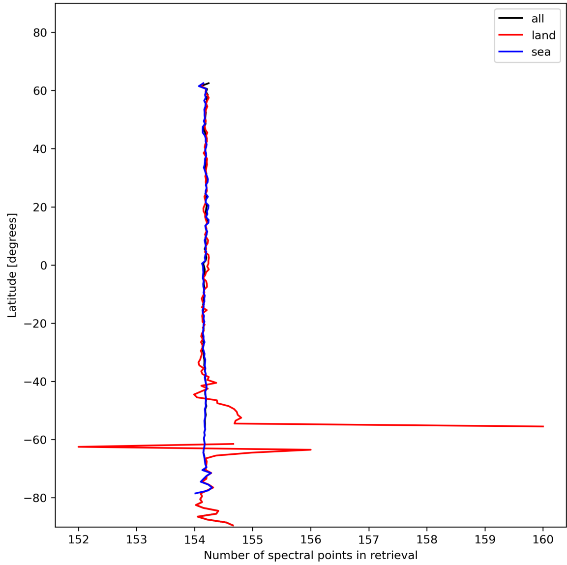
Figure 13: Zonal average of “Number of spectral points in retrieval” for 2023-12-07 to 2023-12-09.
