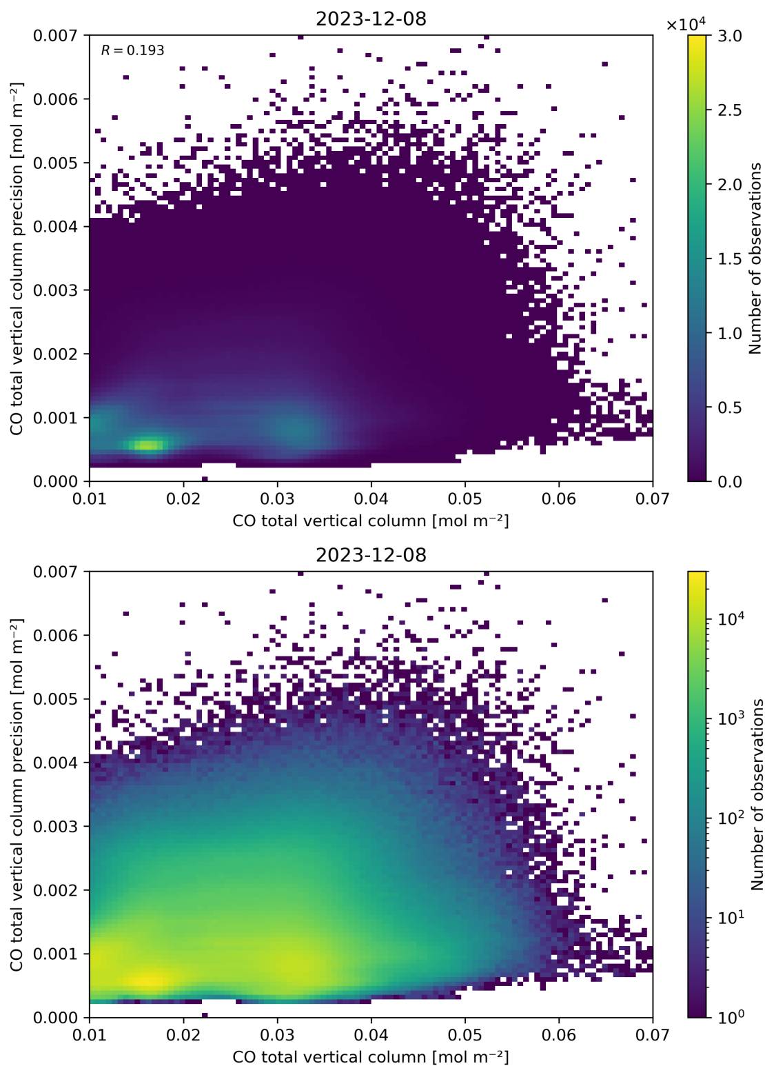
Figure 34: Scatter density plot of “CO total vertical column” against “CO total vertical column precision” for 2023-12-07 to 2023-12-09.
