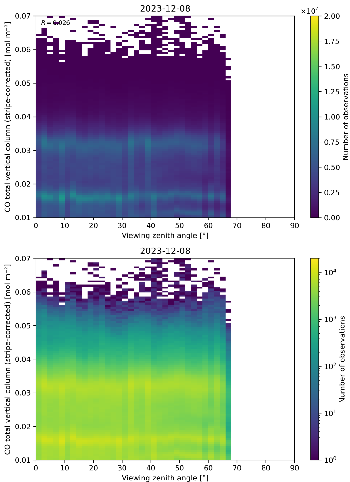
Figure 70: Scatter density plot of “Viewing zenith angle” against “CO total vertical column (stripe-corrected)” for 2023-12-07 to 2023-12-09.
