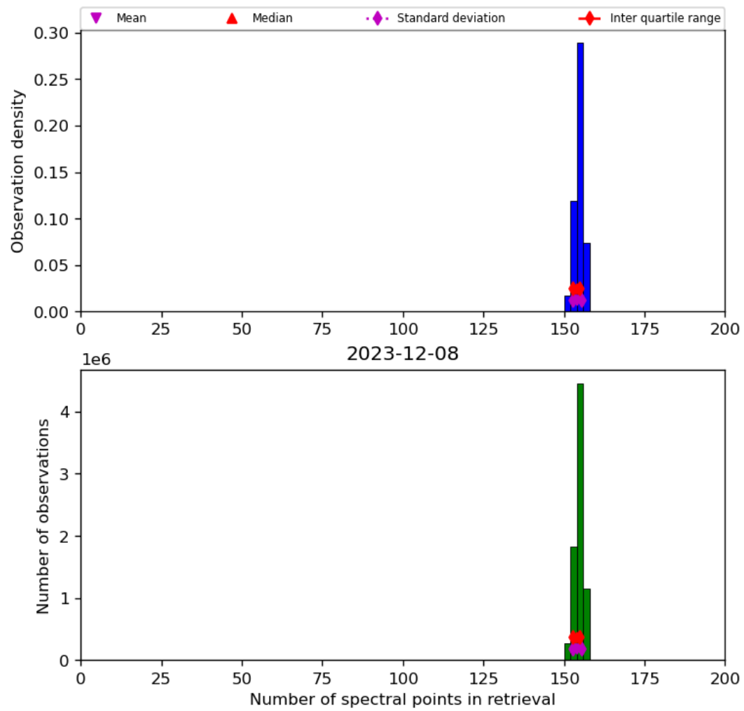
Figure 21: Histogram of “Number of spectral points in retrieval” for 2023-12-07 to 2023-12-09
