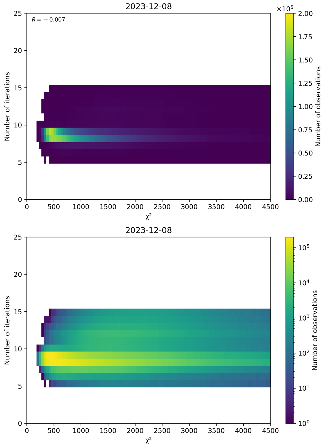
Figure 49: Scatter density plot of “ \chi^2 ” against “Number of iterations” for 2023-12-07 to 2023-12-09.
