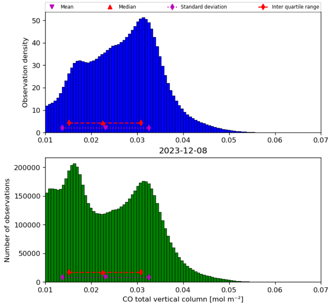
Figure 18: Histogram of “CO total vertical column” for 2023-12-07 to 2023-12-09
