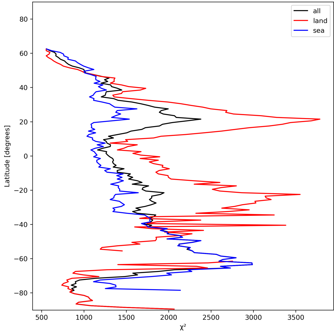
Figure 14: Zonal average of “ \chi^2 ” for 2023-12-07 to 2023-12-09.
