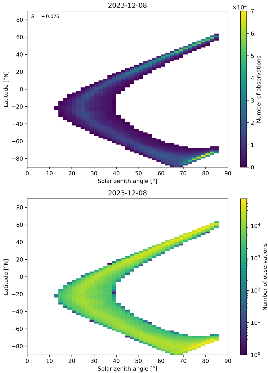
Figure 66: Scatter density plot of “Solar zenith angle” against “Latitude” for 2023-12-07 to 2023-12-09.
