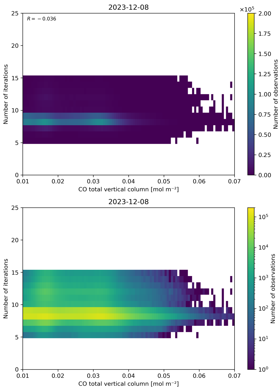
Figure 42: Scatter density plot of “CO total vertical column” against “Number of iterations” for 2023-12-07 to 2023-12-09.
