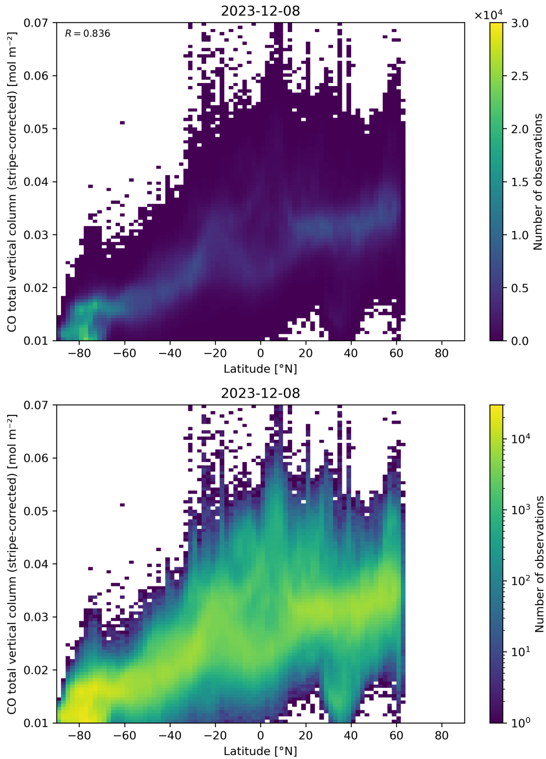
Figure 52: Scatter density plot of “Latitude” against “CO total vertical column (stripe-corrected)” for 2023-12-07 to 2023-12-09.
