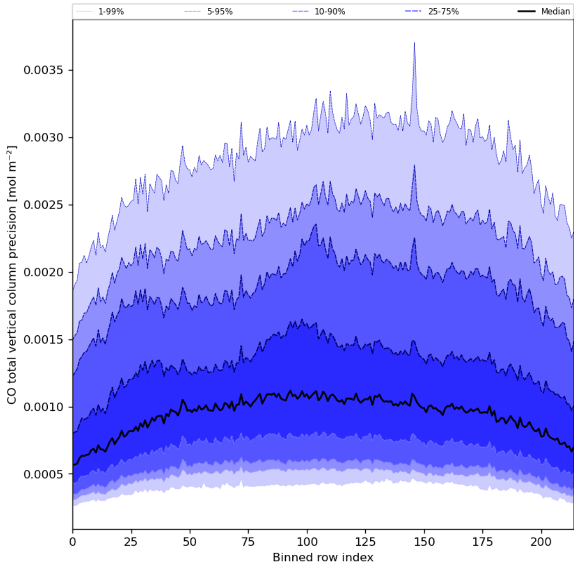
Figure 28: Along track statistics of “CO total vertical column precision” for 2023-12-07 to 2023-12-09
