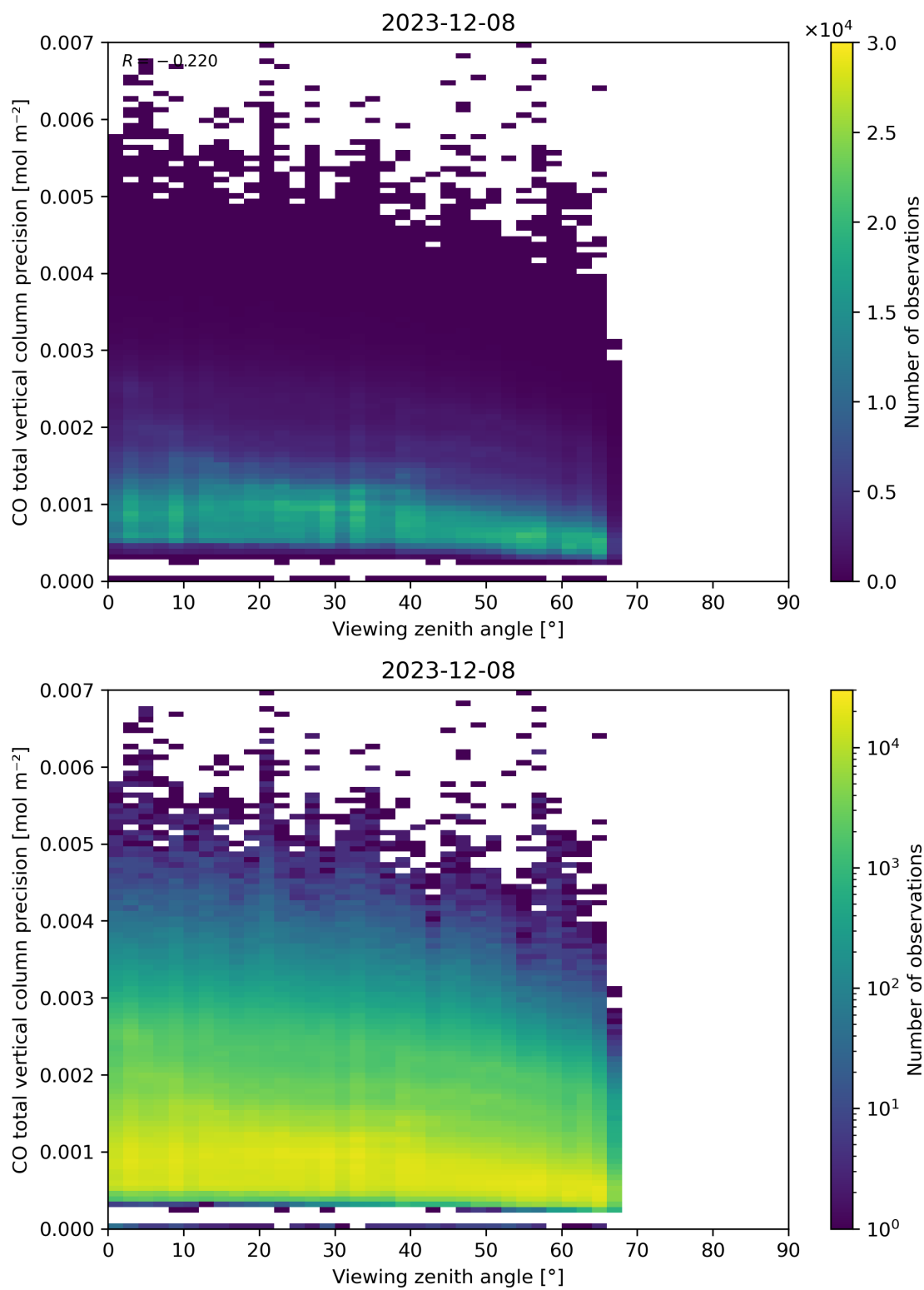
Figure 71: Scatter density plot of “Viewing zenith angle” against “CO total vertical column precision” for 2023-12-07 to 2023-12-09.
