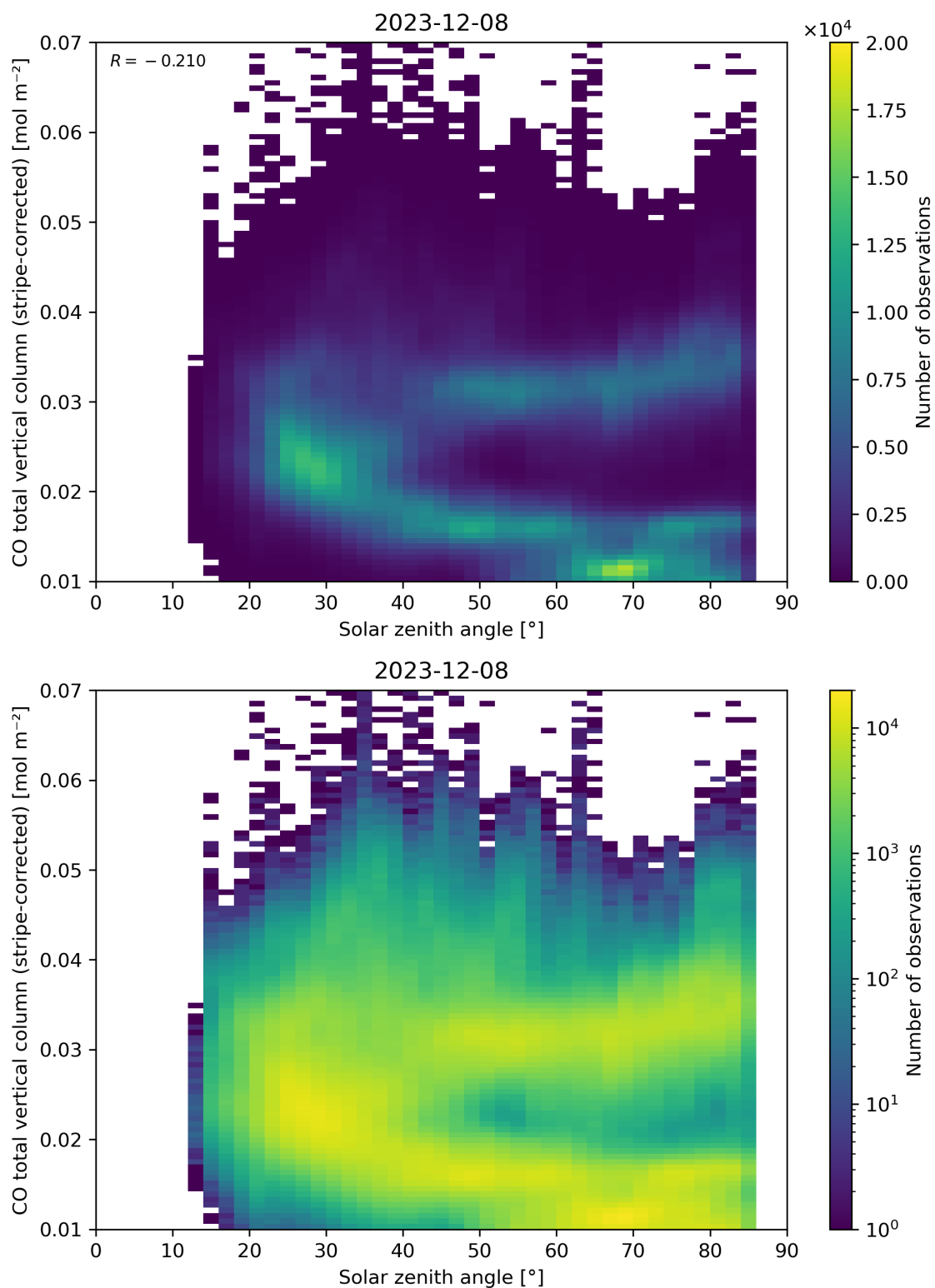
Figure 62: Scatter density plot of “Solar zenith angle” against “CO total vertical column (stripe-corrected)” for 2023-12-07 to 2023-12-09.
