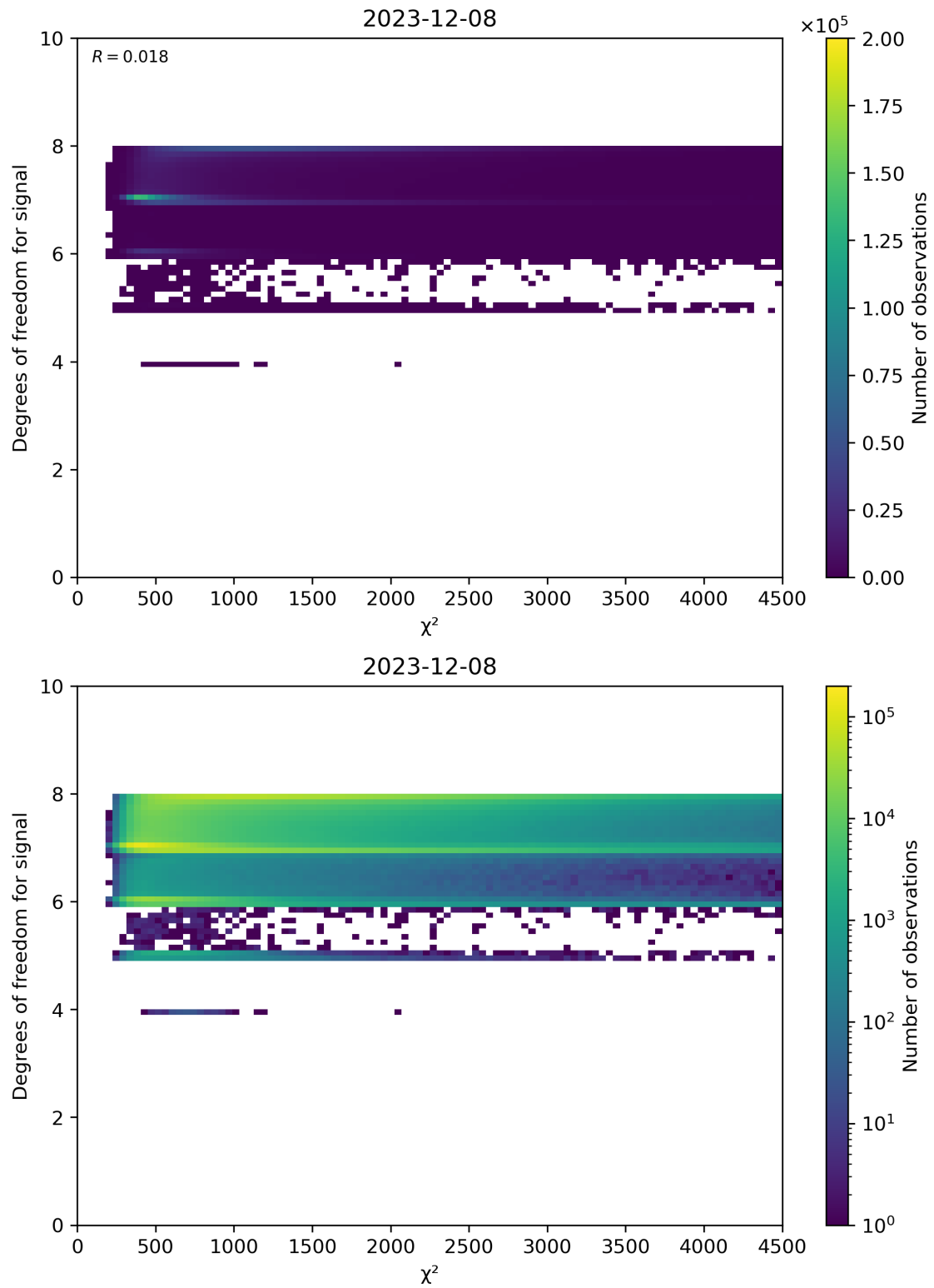
Figure 48: Scatter density plot of “ \chi^2 ” against “Degrees of freedom for signal” for 2023-12-07 to 2023-12-09.
