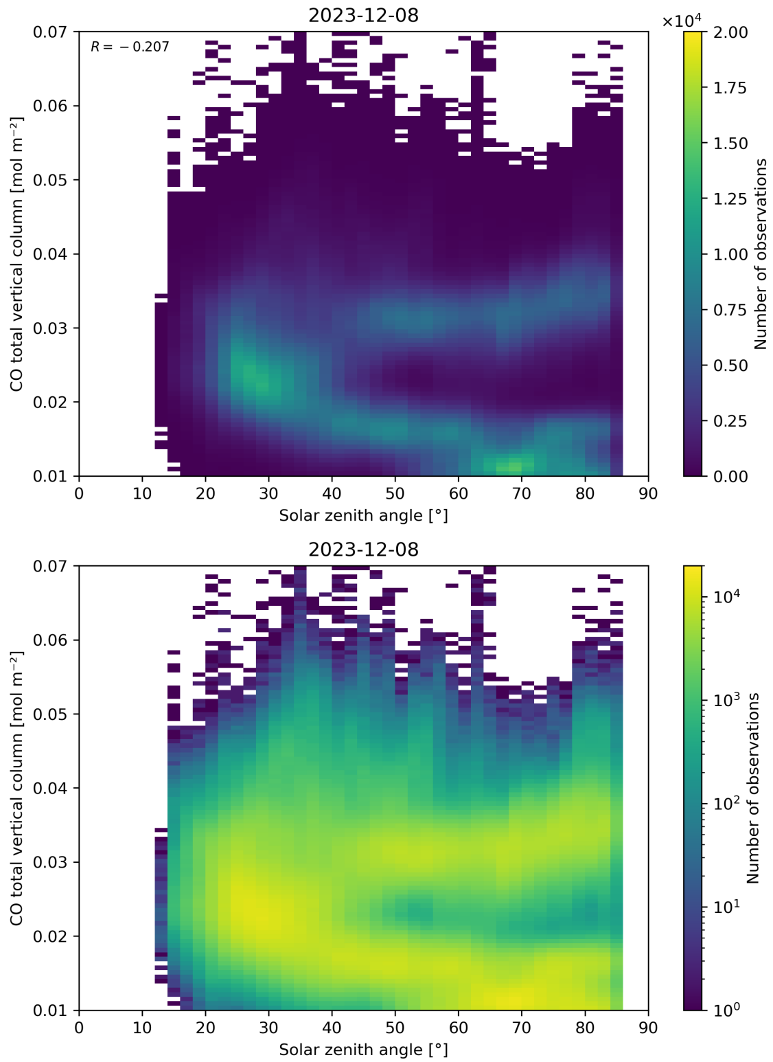
Figure 61: Scatter density plot of “Solar zenith angle” against “CO total vertical column” for 2023-12-07 to 2023-12-09.
