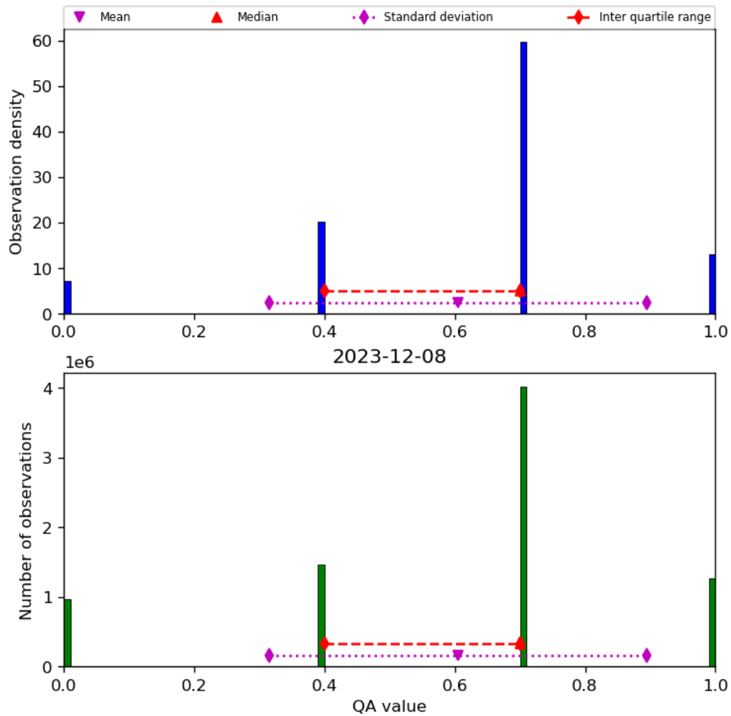
Figure 17: Histogram of “QA value” for 2023-12-07 to 2023-12-09
