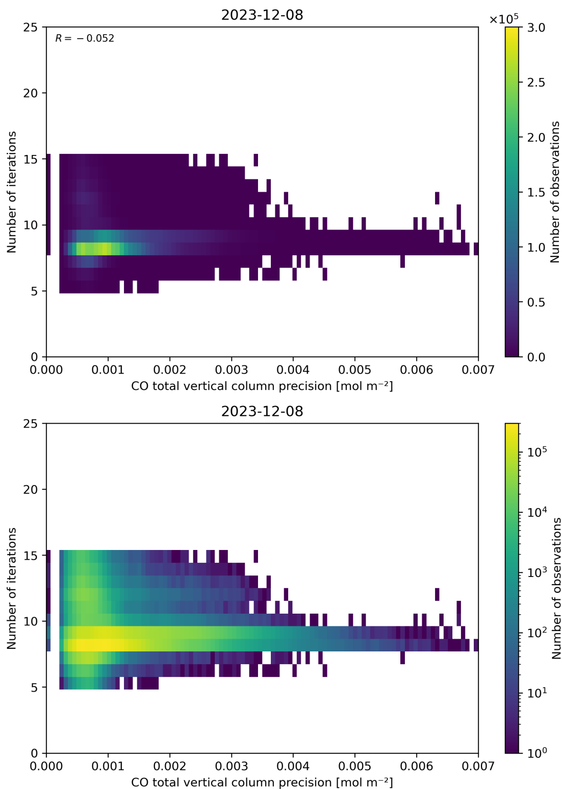
Figure 46: Scatter density plot of “CO total vertical column precision” against “Number of iterations” for 2023-12-07 to 2023-12-09.
