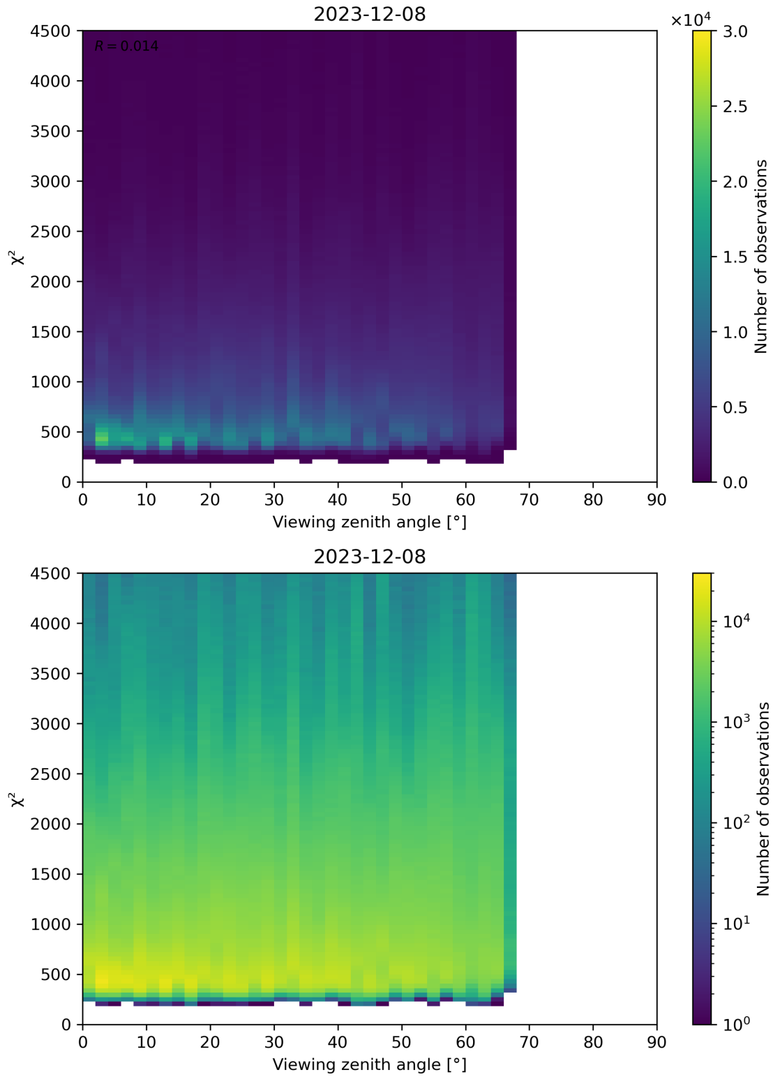
Figure 72: Scatter density plot of “Viewing zenith angle” against “ \chi^2 ” for 2023-12-07 to 2023-12-09.
