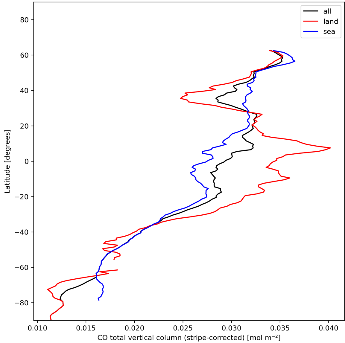
Figure 11: Zonal average of “CO total vertical column (stripe-corrected)” for 2023-12-07 to 2023-12-09.
