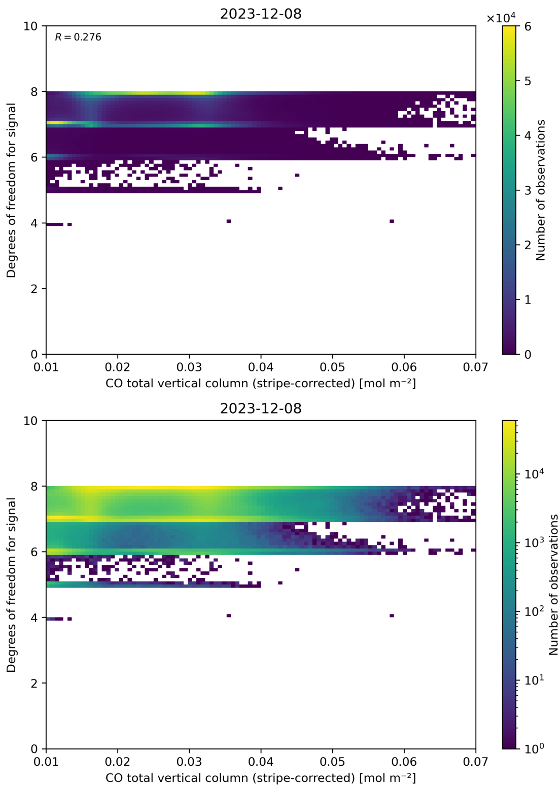
Figure 38: Scatter density plot of “CO total vertical column (stripe-corrected)” against “Degrees of freedom for signal” for 2023-12-07 to 2023-12-09.
