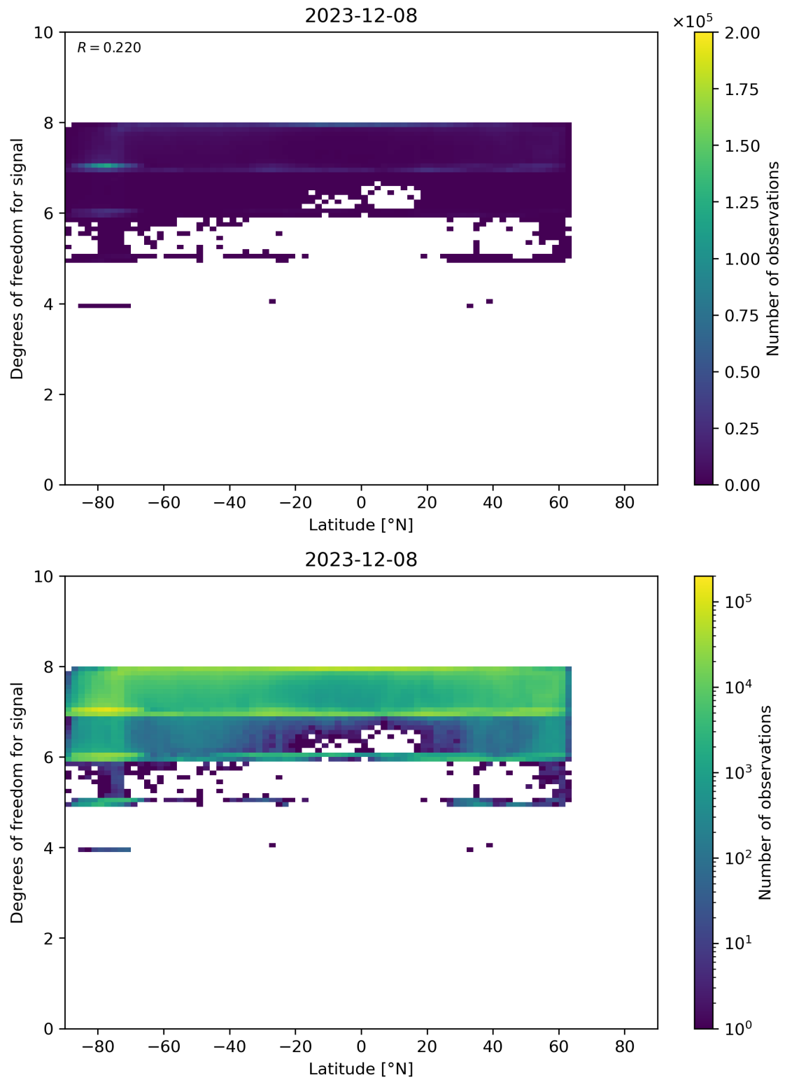
Figure 55: Scatter density plot of “Latitude” against “Degrees of freedom for signal” for 2023-12-07 to 2023-12-09.
