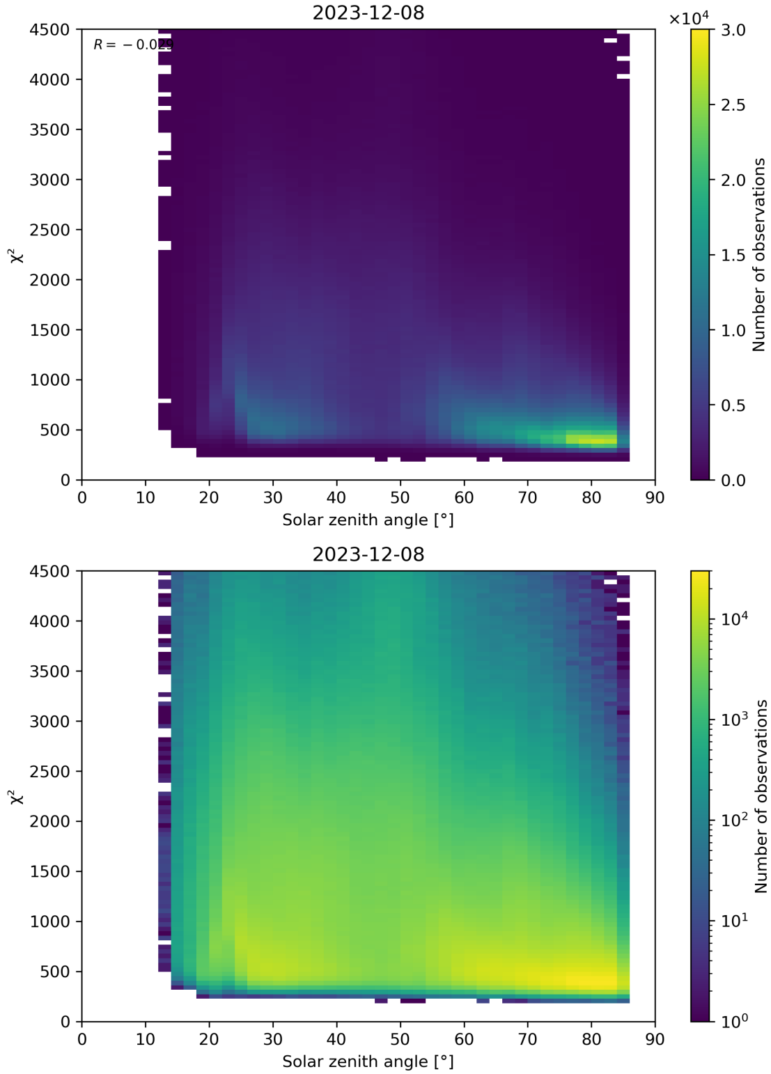
Figure 64: Scatter density plot of “Solar zenith angle” against “ \chi^2 ” for 2023-12-07 to 2023-12-09.
