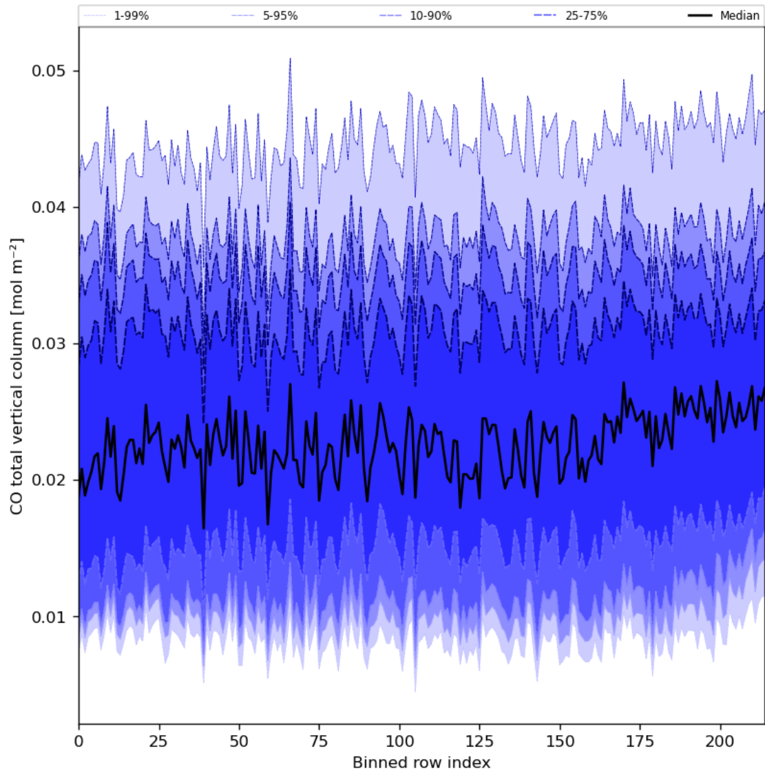
Figure 26: Along track statistics of “CO total vertical column” for 2023-12-07 to 2023-12-09
