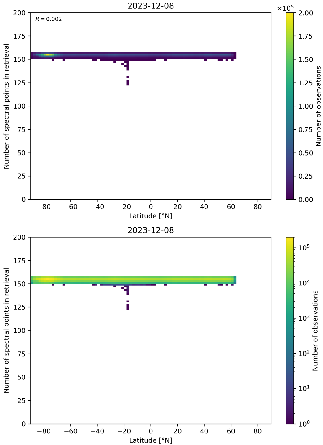
Figure 57: Scatter density plot of “Latitude” against “Number of spectral points in retrieval” for 2023-12-07 to 2023-12-09.
