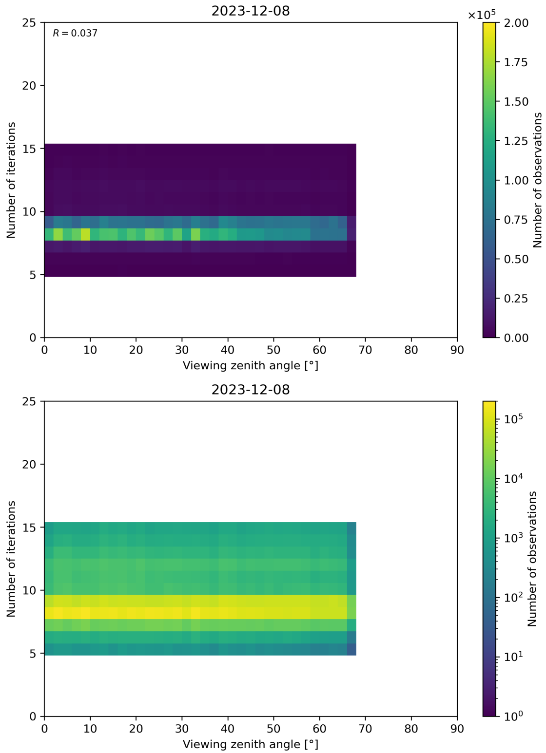
Figure 75: Scatter density plot of “Viewing zenith angle” against “Number of iterations” for 2023-12-07 to 2023-12-09.
