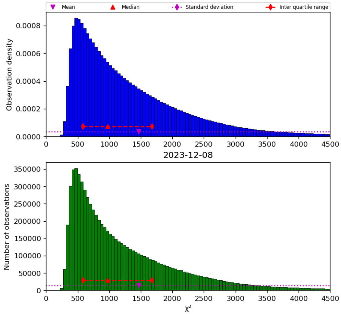
Figure 22: Histogram of “ \chi^2 ” for 2023-12-07 to 2023-12-09
