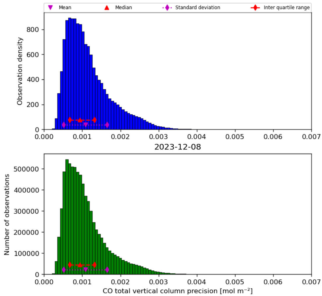
Figure 20: Histogram of “CO total vertical column precision” for 2023-12-07 to 2023-12-09
