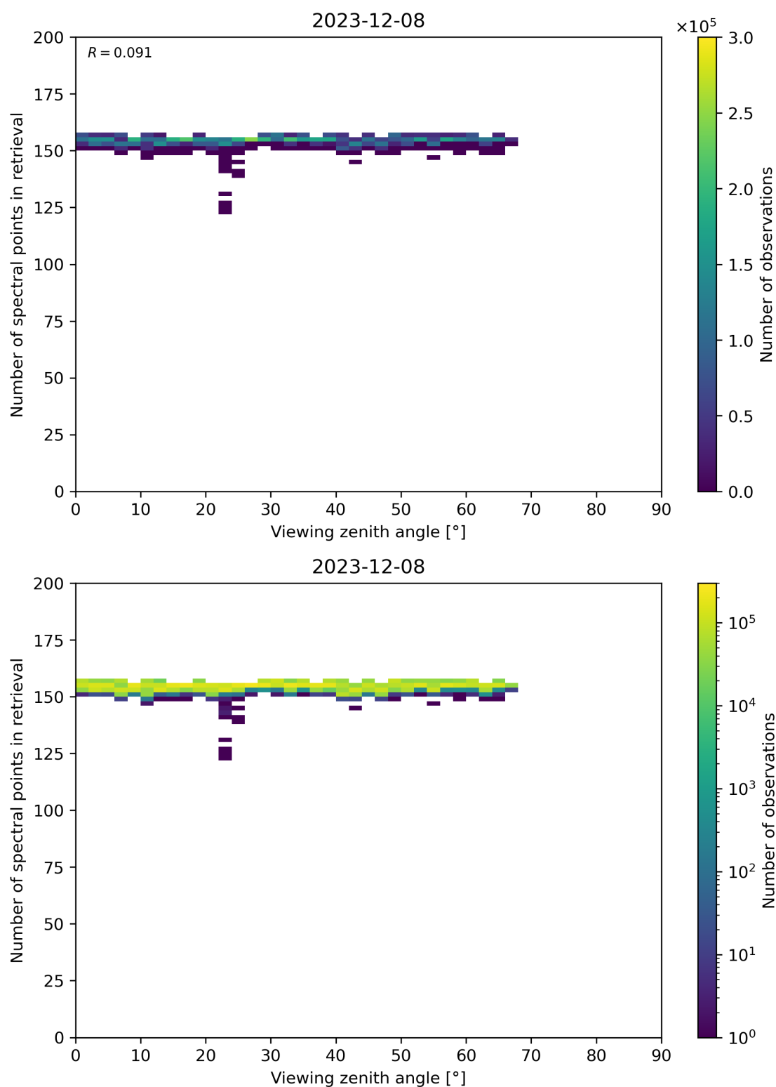
Figure 76: Scatter density plot of “Viewing zenith angle” against “Number of spectral points in retrieval” for 2023-12-07 to 2023-12-09.
