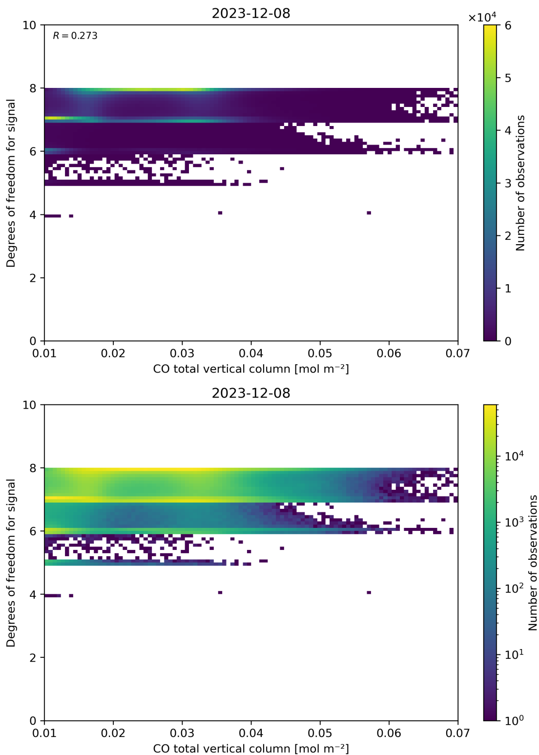
Figure 41: Scatter density plot of “CO total vertical column” against “Degrees of freedom for signal” for 2023-12-07 to 2023-12-09.
