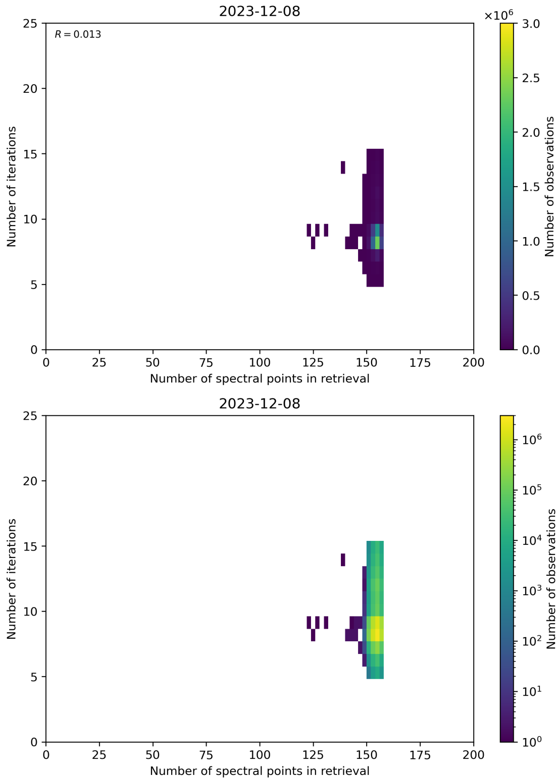
Figure 60: Scatter density plot of “Number of spectral points in retrieval” against “Number of iterations” for 2023-12-07 to 2023-12-09.
