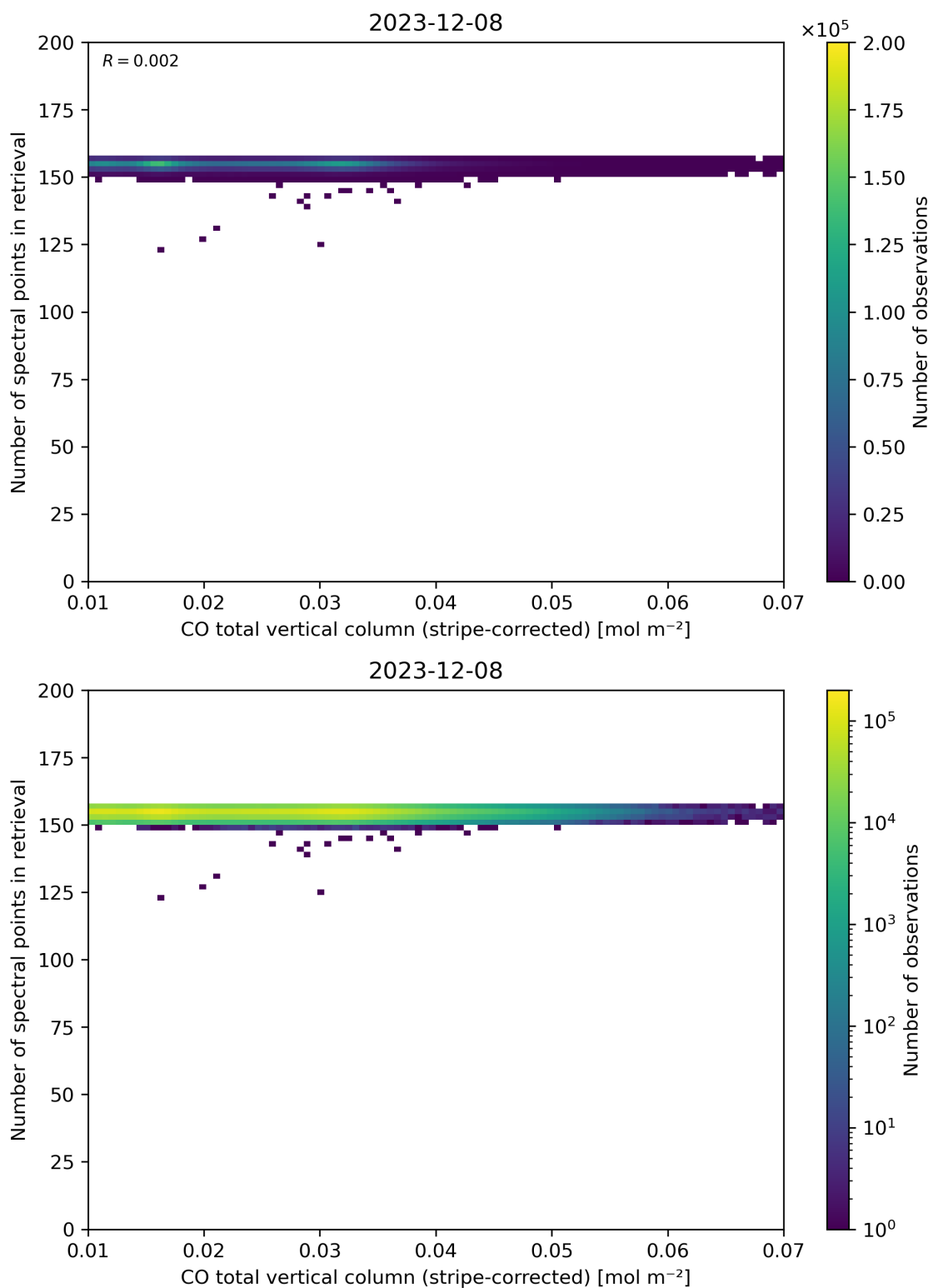
Figure 40: Scatter density plot of “CO total vertical column (stripe-corrected)” against “Number of spectral points in retrieval” for 2023-12-07 to 2023-12-09.
