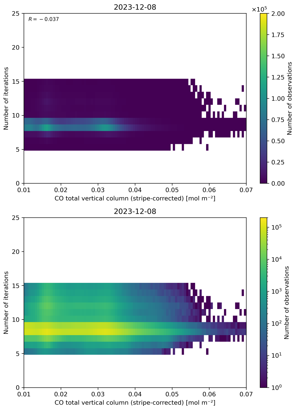
Figure 39: Scatter density plot of “CO total vertical column (stripe-corrected)” against “Number of iterations” for 2023-12-07 to 2023-12-09.
