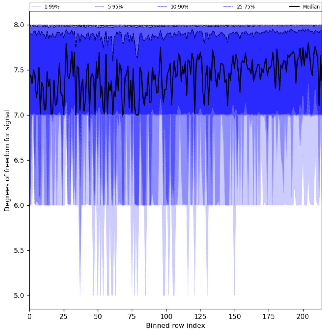
Figure 31: Along track statistics of “Degrees of freedom for signal” for 2023-12-07 to 2023-12-09
