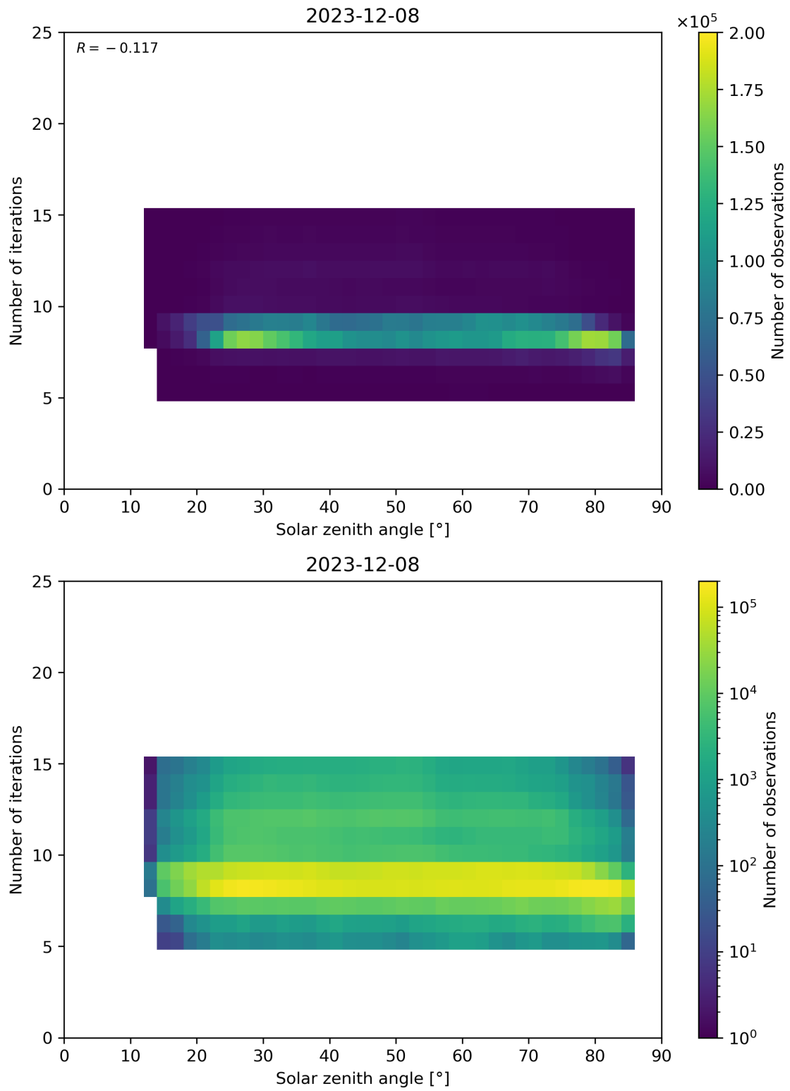
Figure 67: Scatter density plot of “Solar zenith angle” against “Number of iterations” for 2023-12-07 to 2023-12-09.
