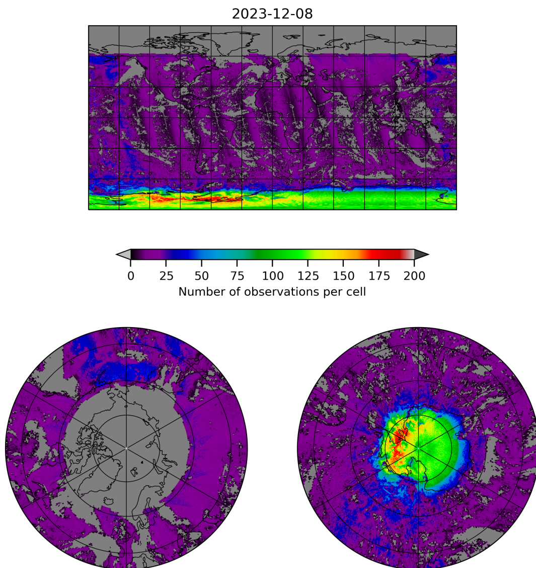
Figure 8: Map of the number of observations for 2023-12-07 to 2023-12-09
