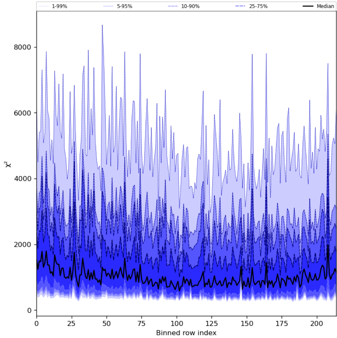
Figure 30: Along track statistics of “ \chi^2 ” for 2023-12-07 to 2023-12-09
