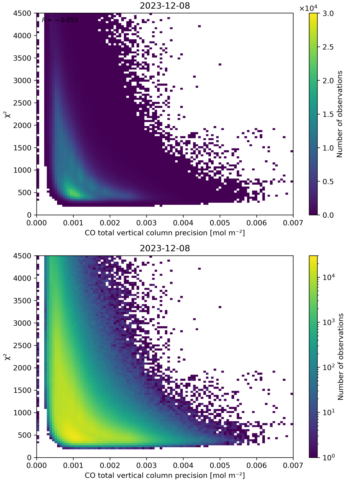
Figure 44: Scatter density plot of “CO total vertical column precision” against “ \chi^2 ” for 2023-12-07 to 2023-12-09.
