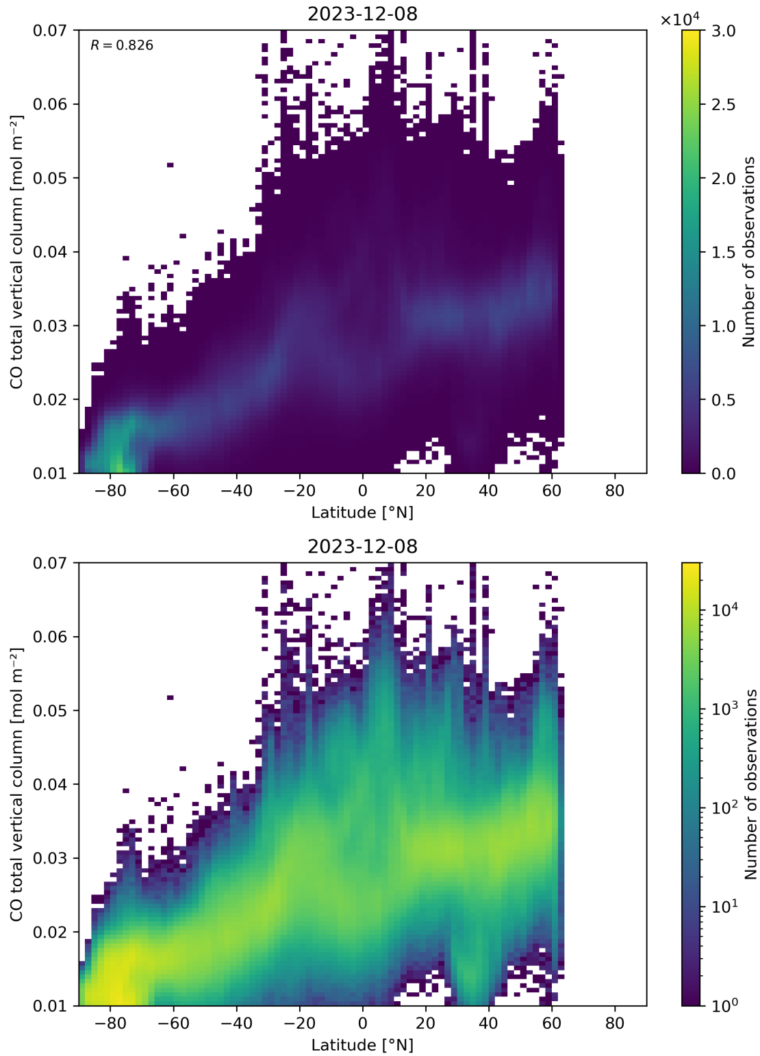
Figure 51: Scatter density plot of “Latitude” against “CO total vertical column” for 2023-12-07 to 2023-12-09.
