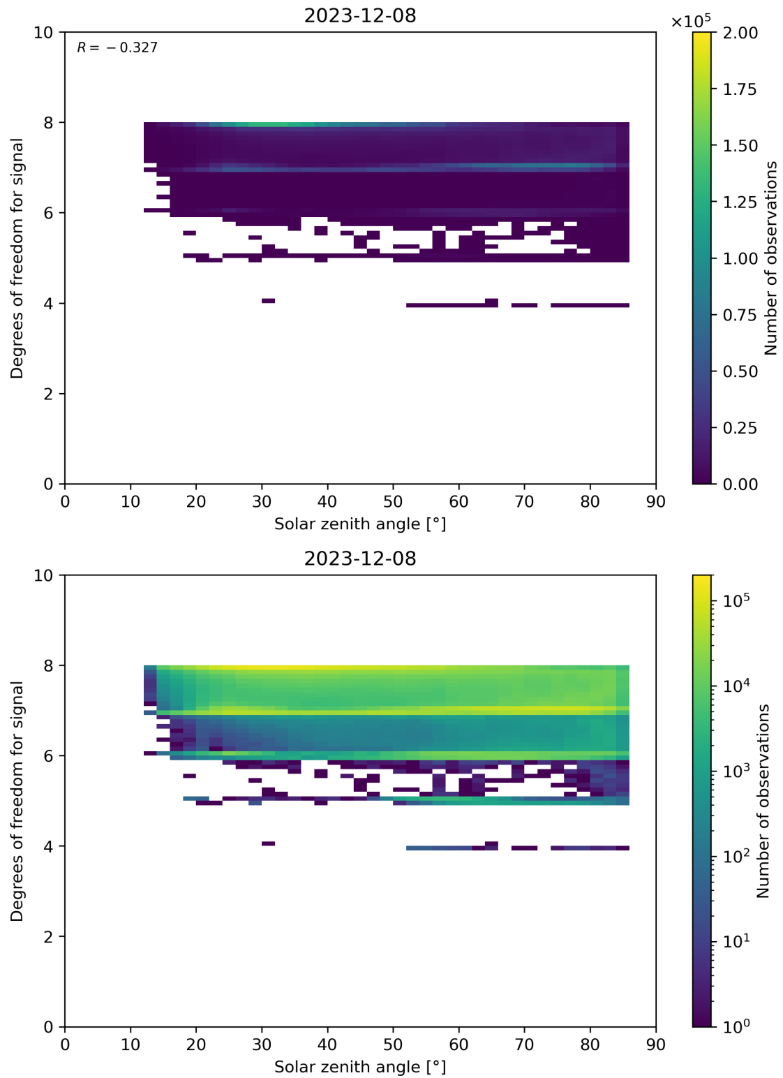
Figure 65: Scatter density plot of “Solar zenith angle” against “Degrees of freedom for signal” for 2023-12-07 to 2023-12-09.
