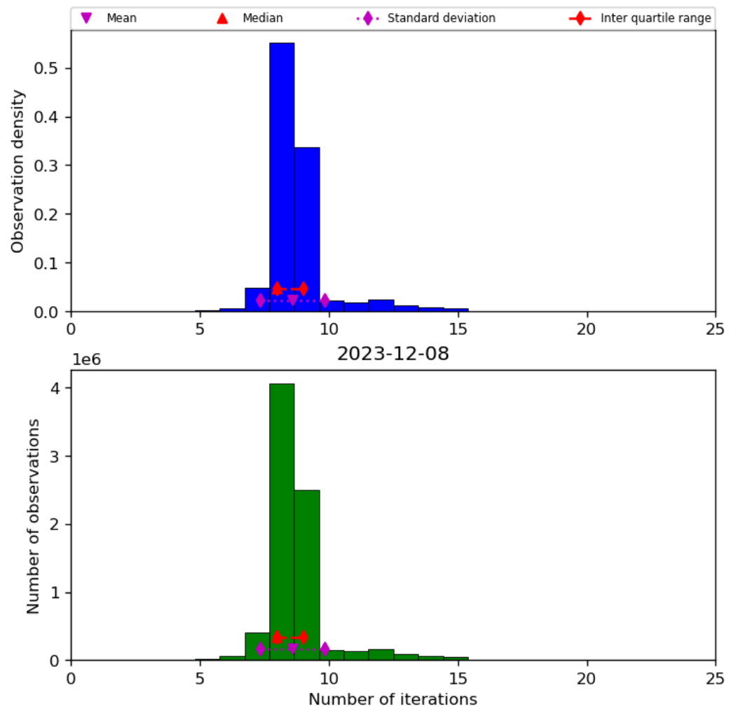
Figure 24: Histogram of “Number of iterations” for 2023-12-07 to 2023-12-09
