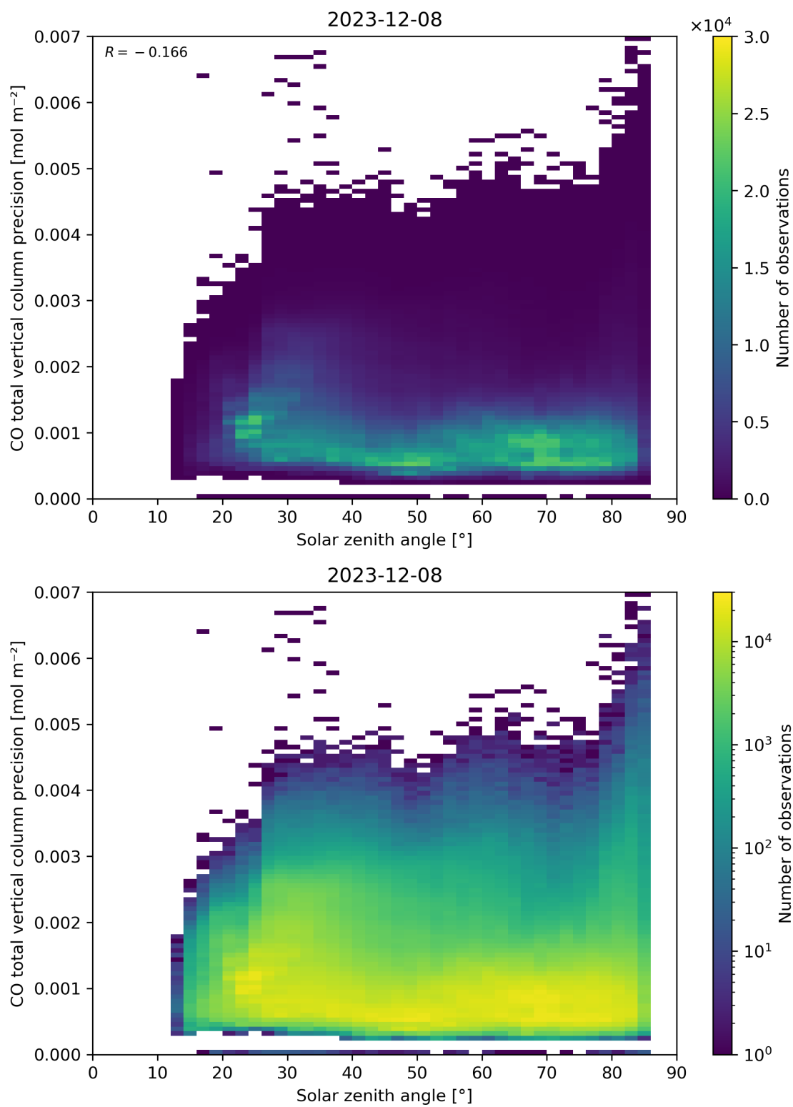
Figure 63: Scatter density plot of “Solar zenith angle” against “CO total vertical column precision” for 2023-12-07 to 2023-12-09.
