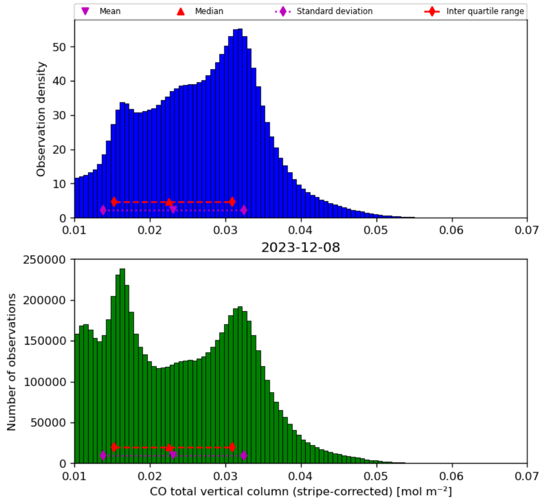
Figure 19: Histogram of “CO total vertical column (stripe-corrected)” for 2023-12-07 to 2023-12-09
