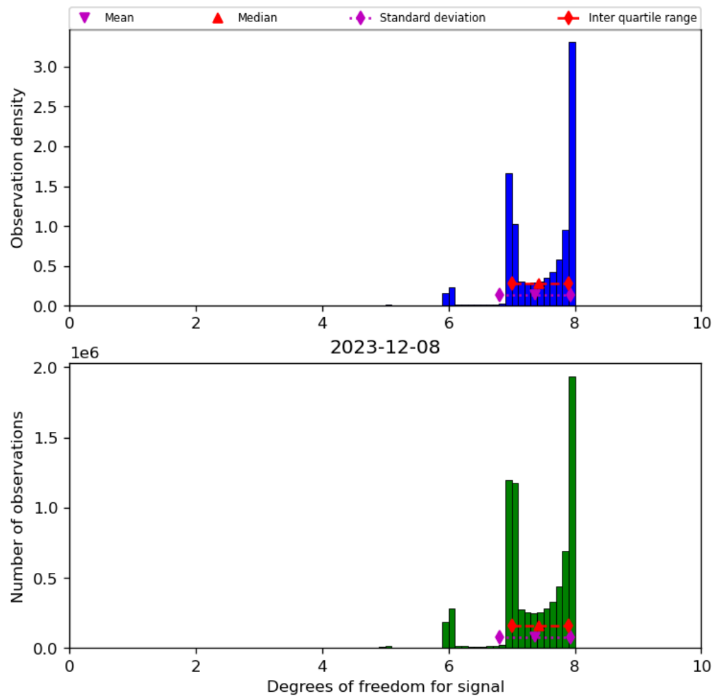
Figure 23: Histogram of “Degrees of freedom for signal” for 2023-12-07 to 2023-12-09
