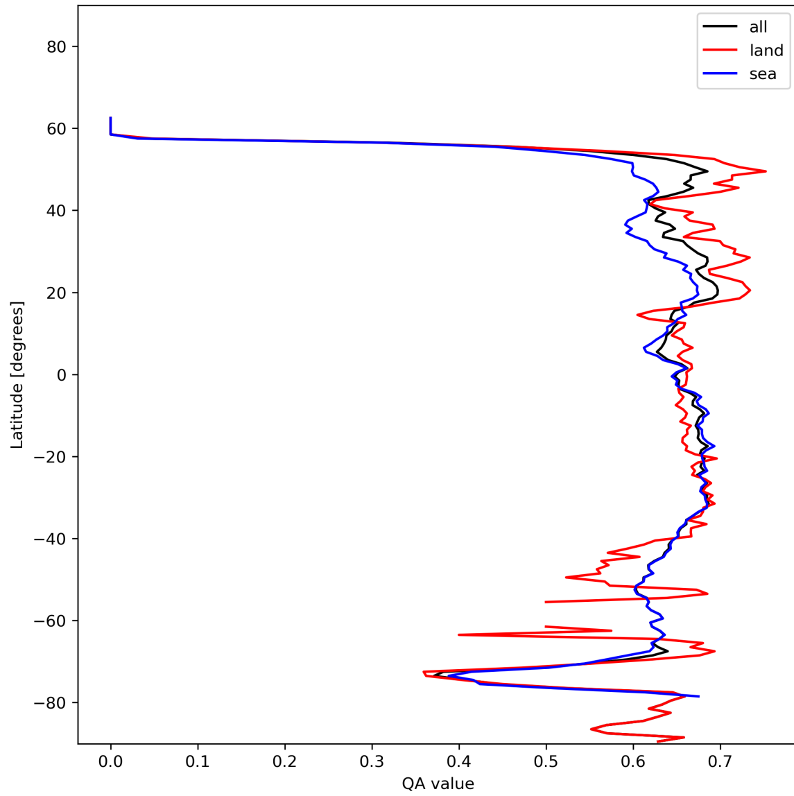
Figure 9: Zonal average of “QA value” for 2023-12-07 to 2023-12-09.
