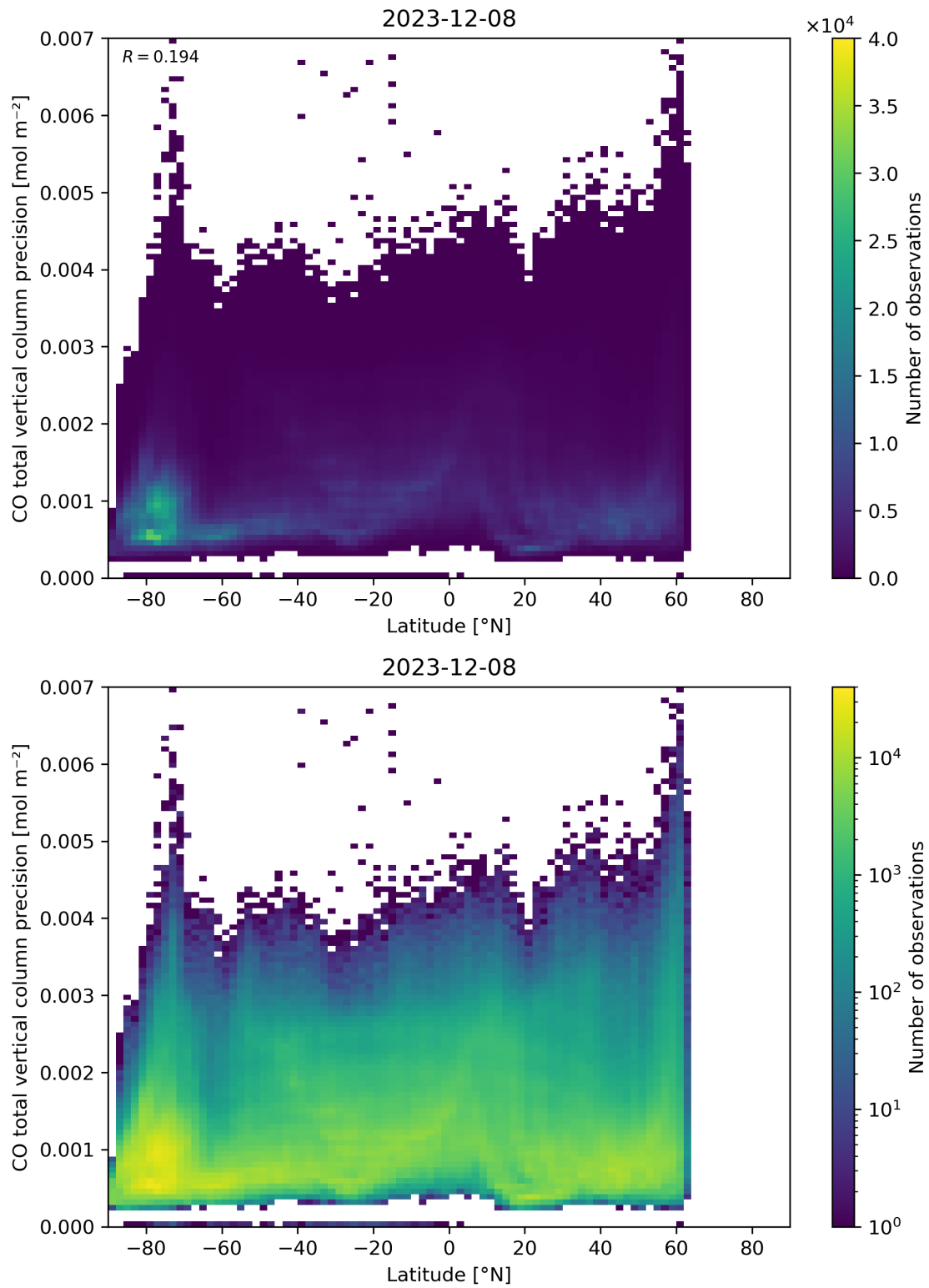
Figure 53: Scatter density plot of “Latitude” against “CO total vertical column precision” for 2023-12-07 to 2023-12-09.
