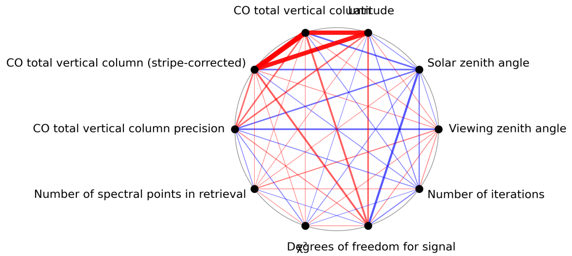
Figure 1: Map of correlation graph for 2023-12-07 to 2023-12-09.
