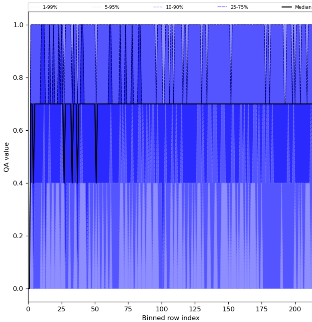
Figure 25: Along track statistics of “QA value” for 2023-12-07 to 2023-12-09
