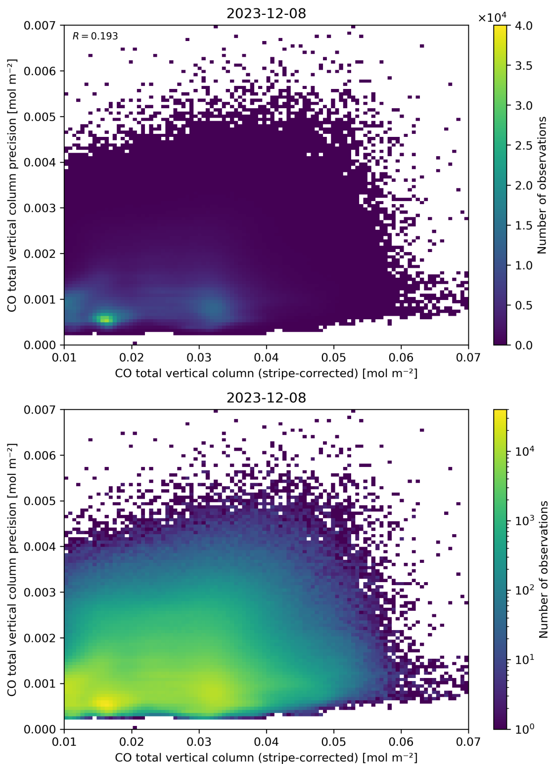
Figure 36: Scatter density plot of “CO total vertical column (stripe-corrected)” against “CO total vertical column precision” for 2023-12-07 to 2023-12-09.
