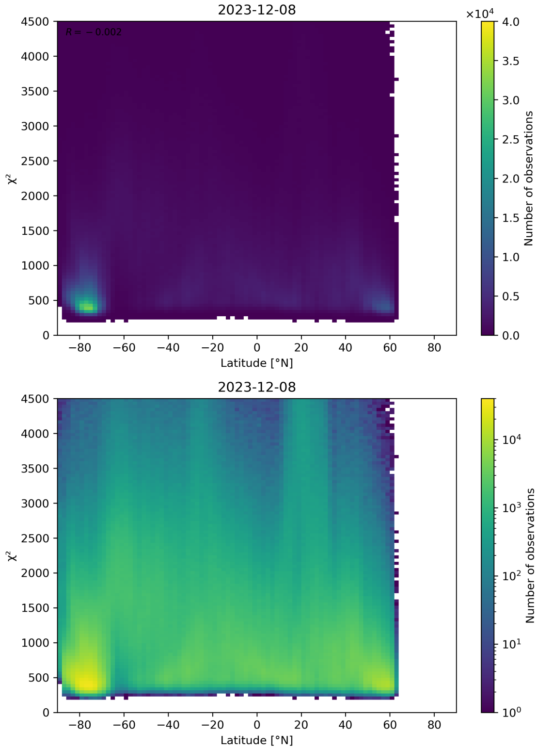
Figure 54: Scatter density plot of “Latitude” against “ \chi^2 ” for 2023-12-07 to 2023-12-09.
