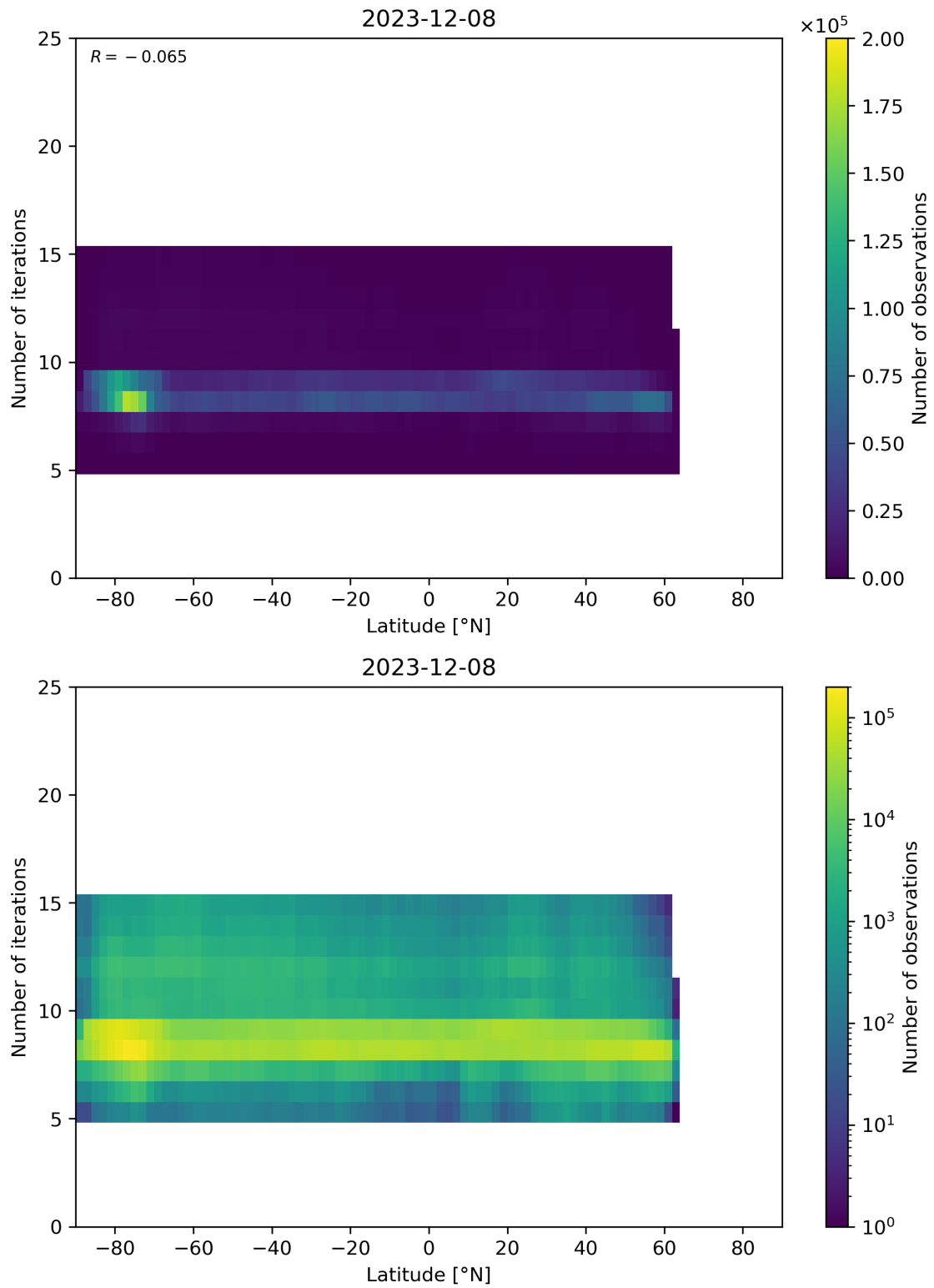
Figure 56: Scatter density plot of “Latitude” against “Number of iterations” for 2023-12-07 to 2023-12-09.
