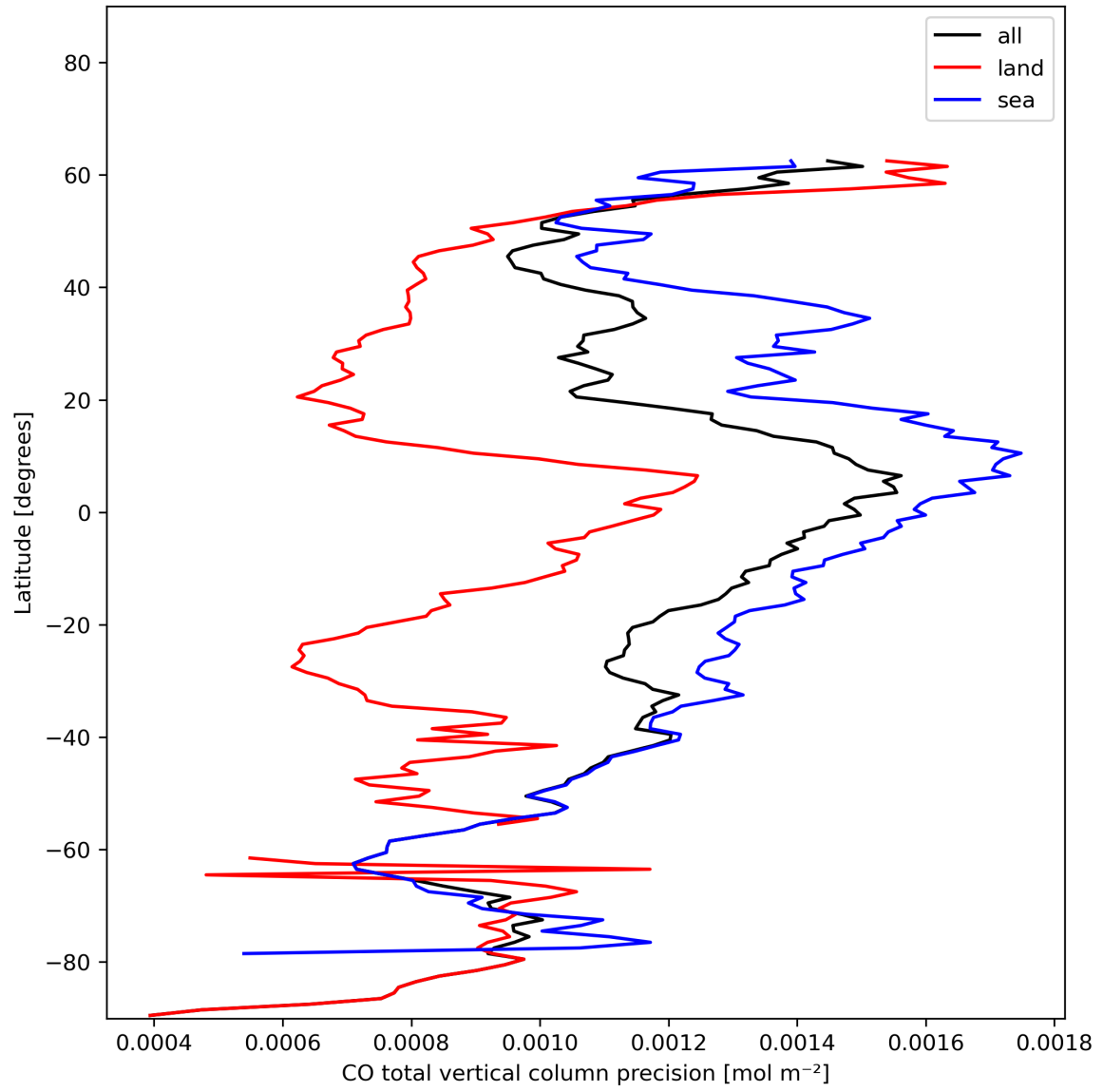
Figure 12: Zonal average of “CO total vertical column precision” for 2023-12-07 to 2023-12-09.
