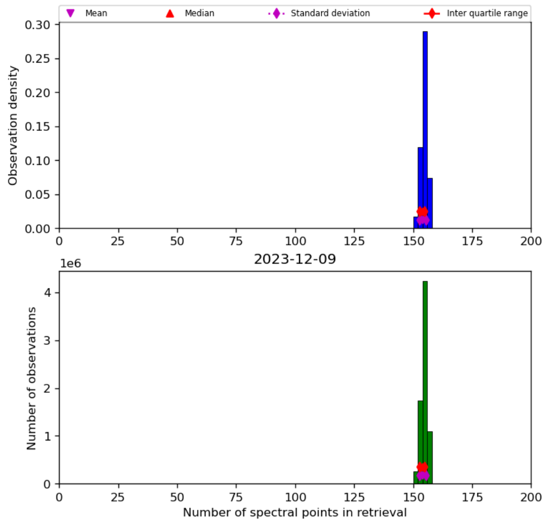
Figure 21: Histogram of “Number of spectral points in retrieval” for 2023-12-09 to 2023-12-10
