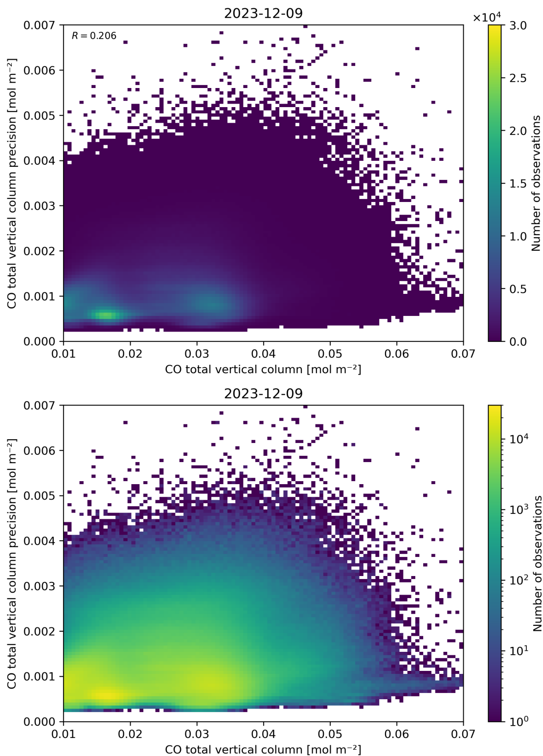
Figure 34: Scatter density plot of “CO total vertical column” against “CO total vertical column precision” for 2023-12-09 to 2023-12-10.
