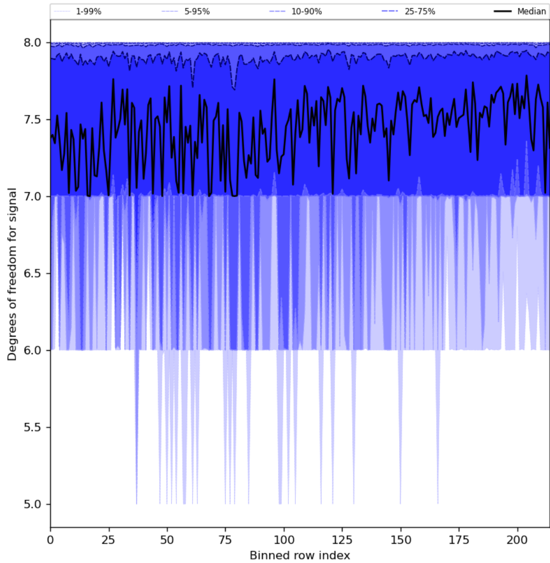
Figure 31: Along track statistics of “Degrees of freedom for signal” for 2023-12-09 to 2023-12-10
