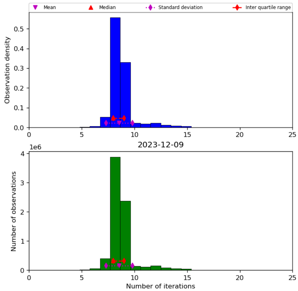
Figure 24: Histogram of “Number of iterations” for 2023-12-09 to 2023-12-10
