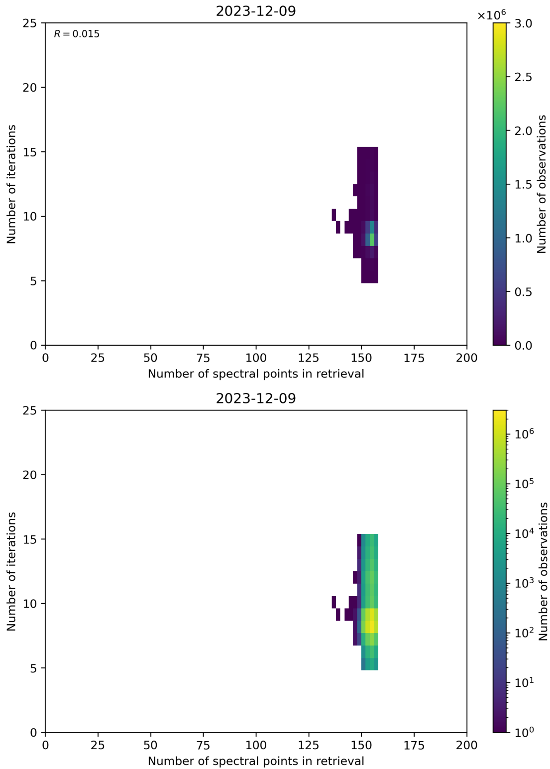
Figure 60: Scatter density plot of “Number of spectral points in retrieval” against “Number of iterations” for 2023-12-09 to 2023-12-10.
