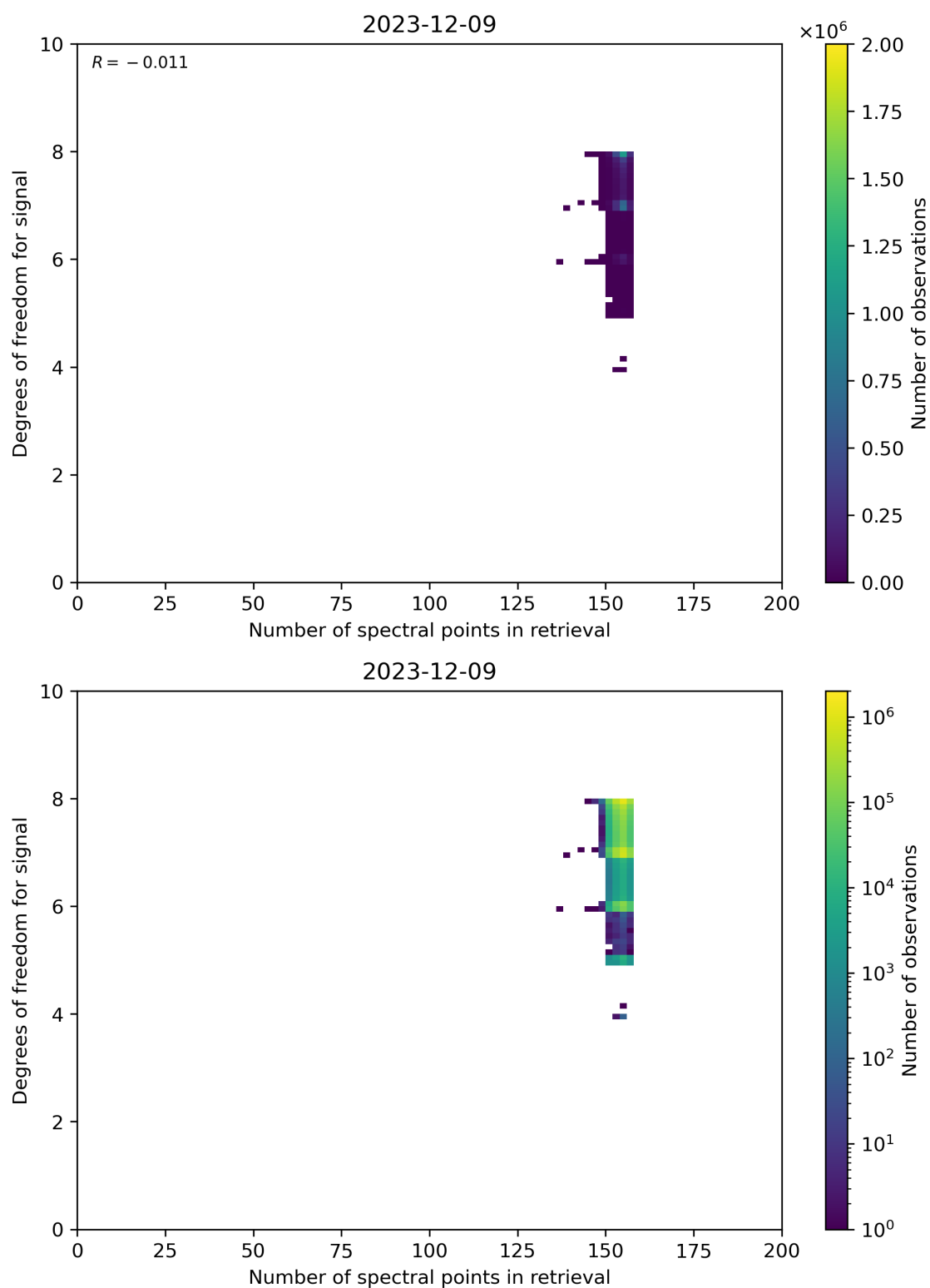
Figure 59: Scatter density plot of “Number of spectral points in retrieval” against “Degrees of freedom for signal” for 2023-12-09 to 2023-12-10.
