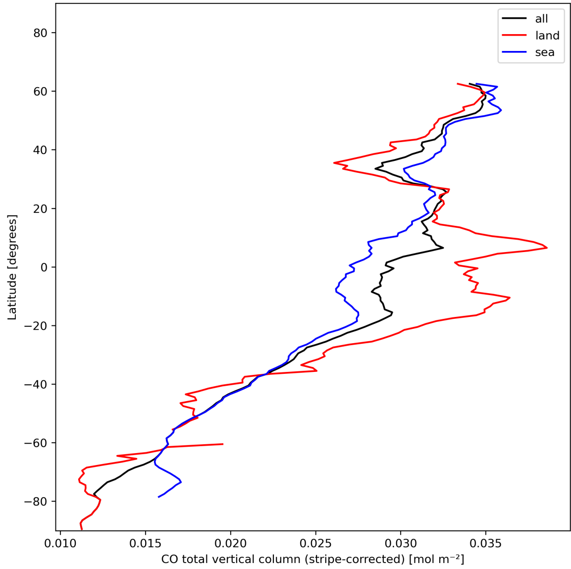
Figure 11: Zonal average of “CO total vertical column (stripe-corrected)” for 2023-12-09 to 2023-12-10.
