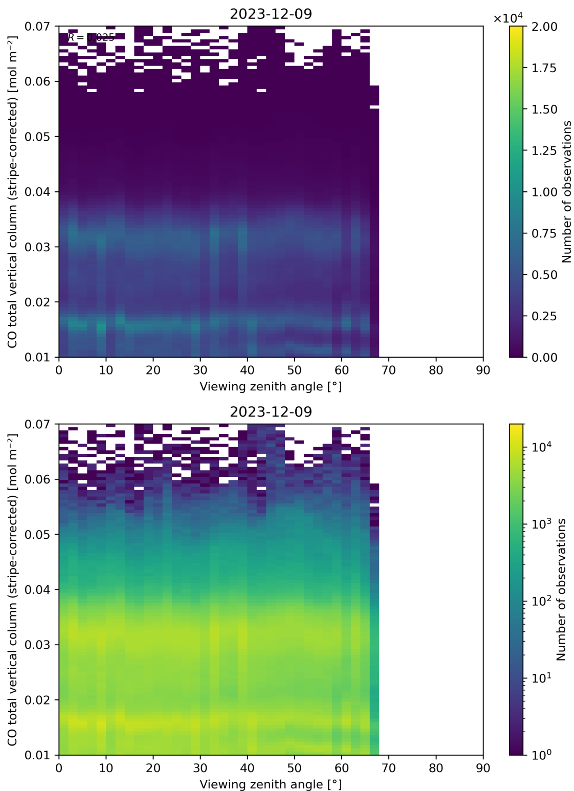
Figure 70: Scatter density plot of “Viewing zenith angle” against “CO total vertical column (stripe-corrected)” for 2023-12-09 to 2023-12-10.
