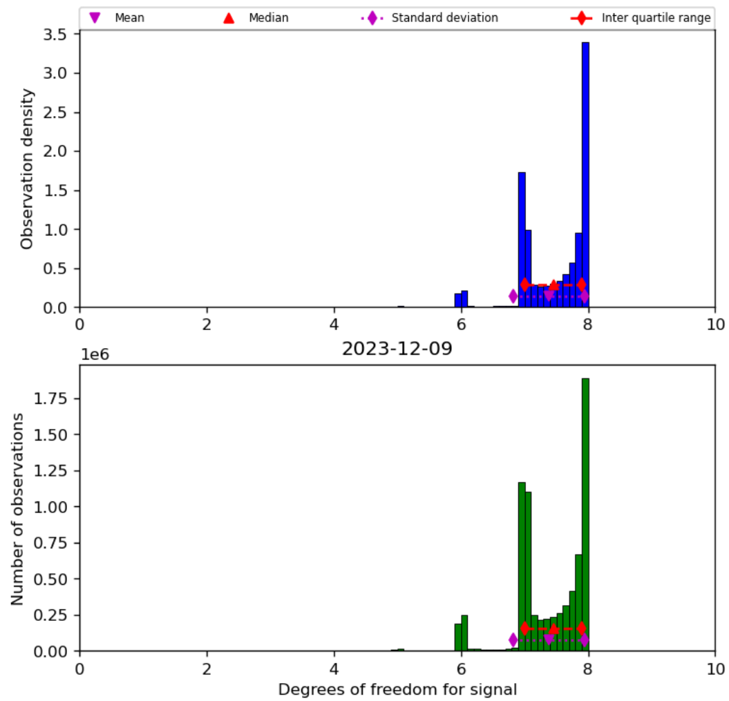
Figure 23: Histogram of “Degrees of freedom for signal” for 2023-12-09 to 2023-12-10
