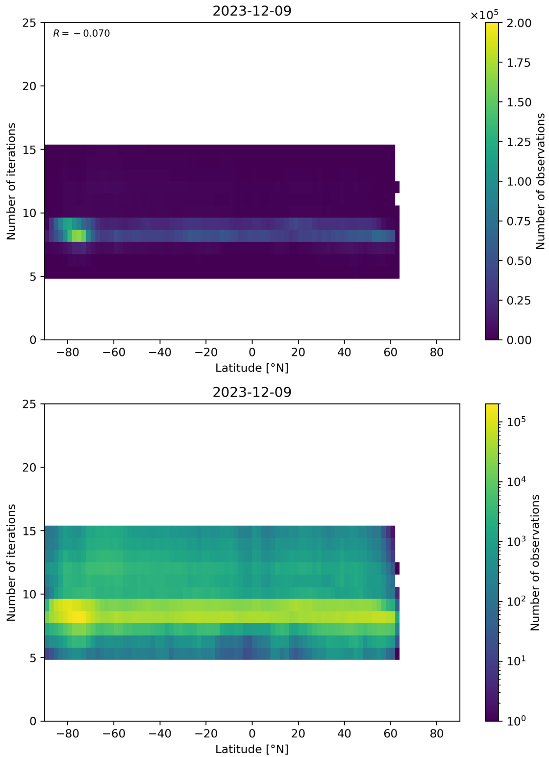
Figure 56: Scatter density plot of “Latitude” against “Number of iterations” for 2023-12-09 to 2023-12-10.
