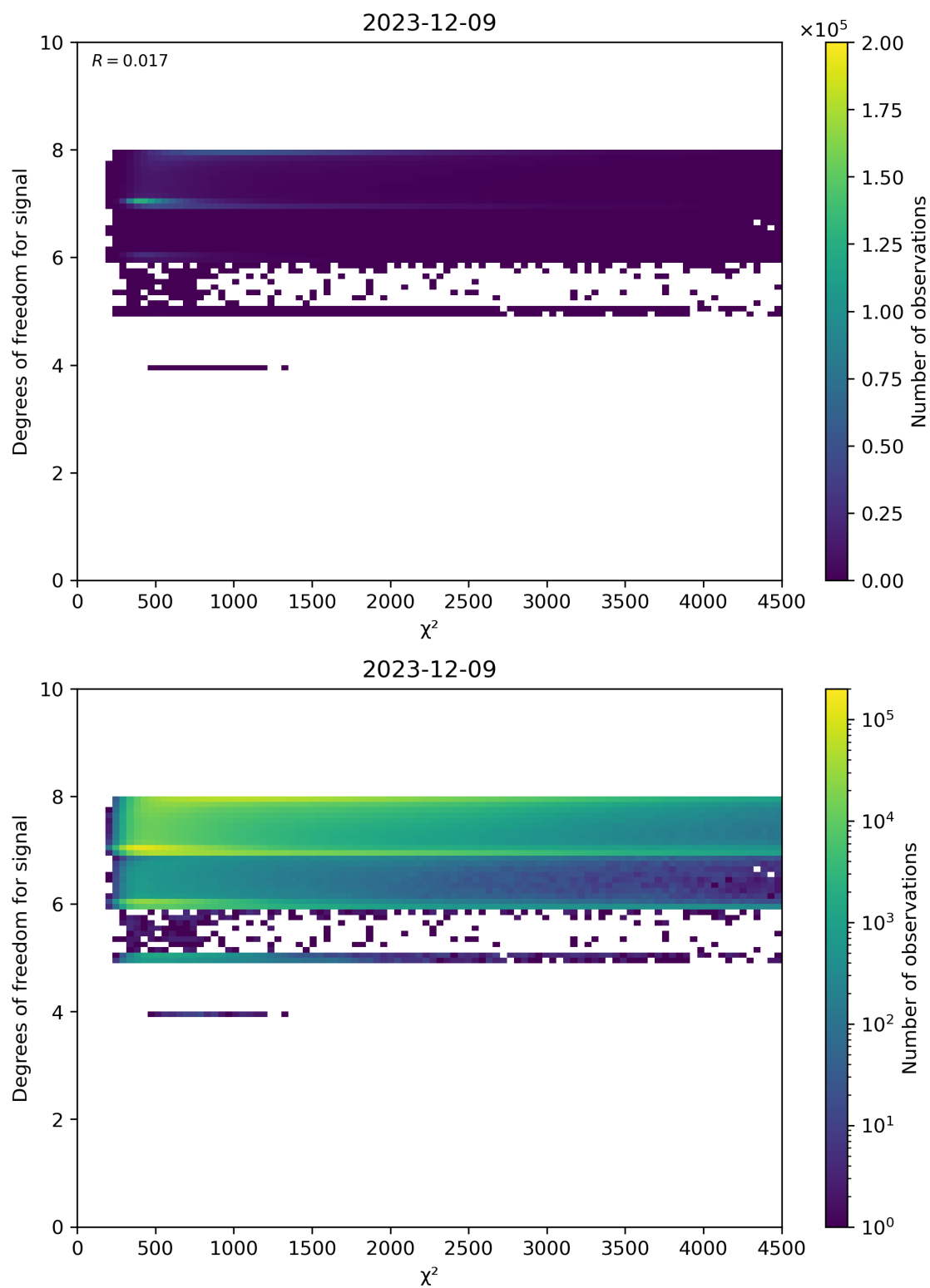
Figure 48: Scatter density plot of “ \chi^2 ” against “Degrees of freedom for signal” for 2023-12-09 to 2023-12-10.
