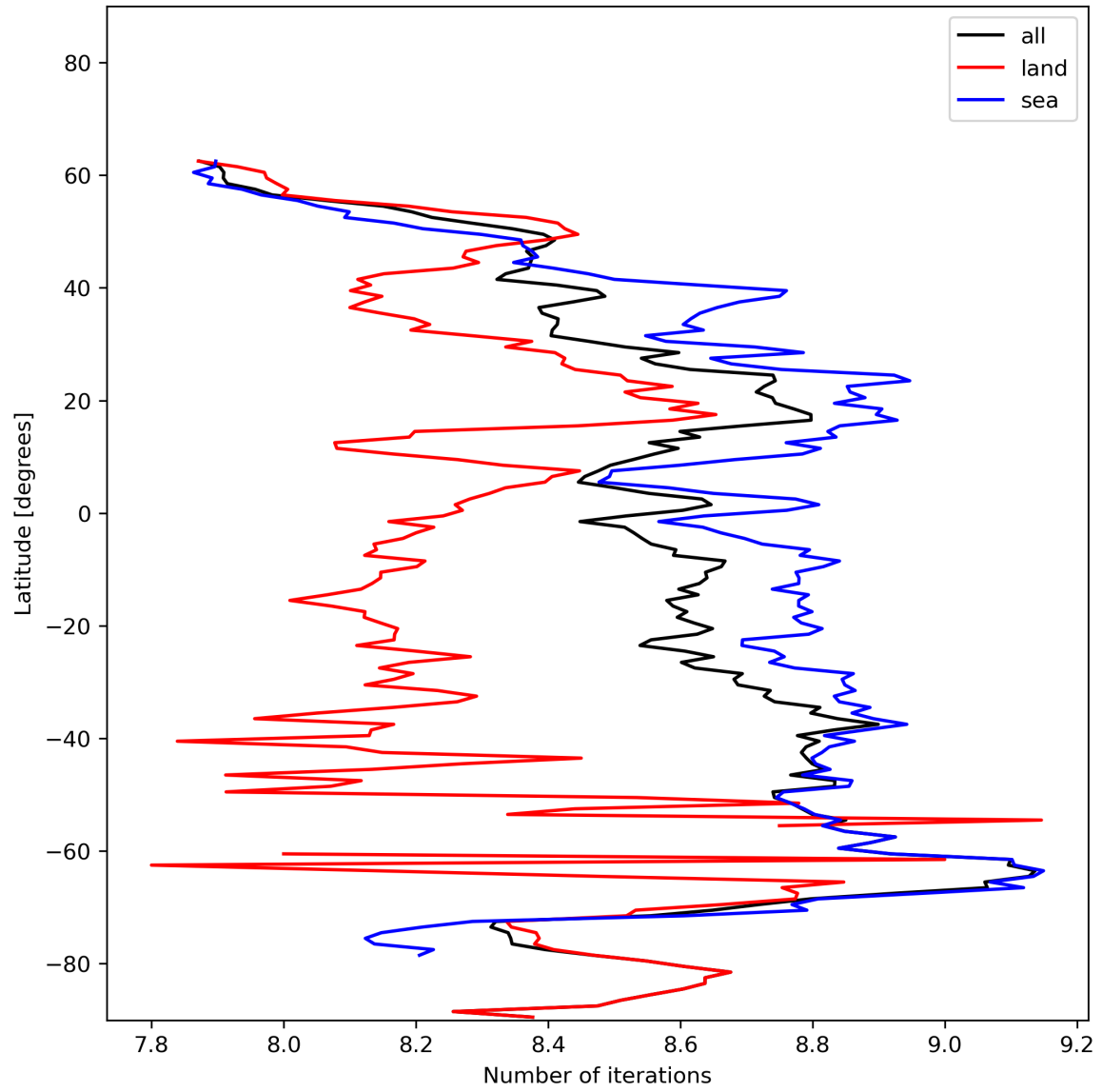
Figure 16: Zonal average of “Number of iterations” for 2023-12-09 to 2023-12-10.
