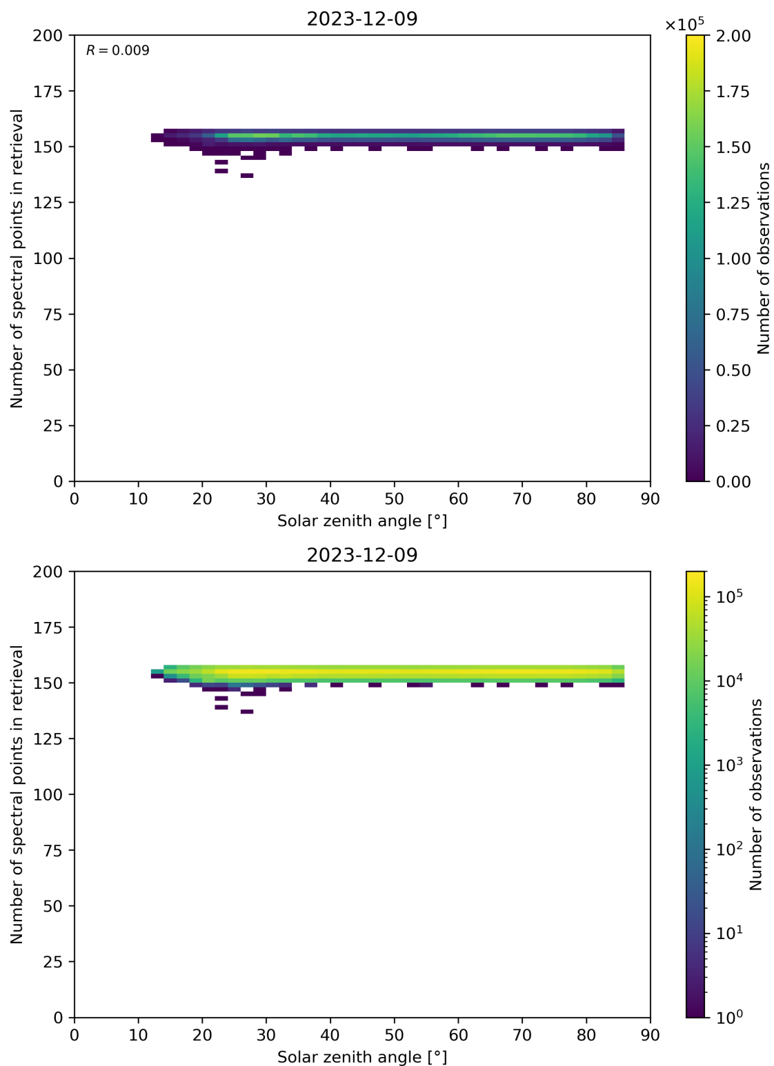
Figure 68: Scatter density plot of “Solar zenith angle” against “Number of spectral points in retrieval” for 2023-12-09 to 2023-12-10.
