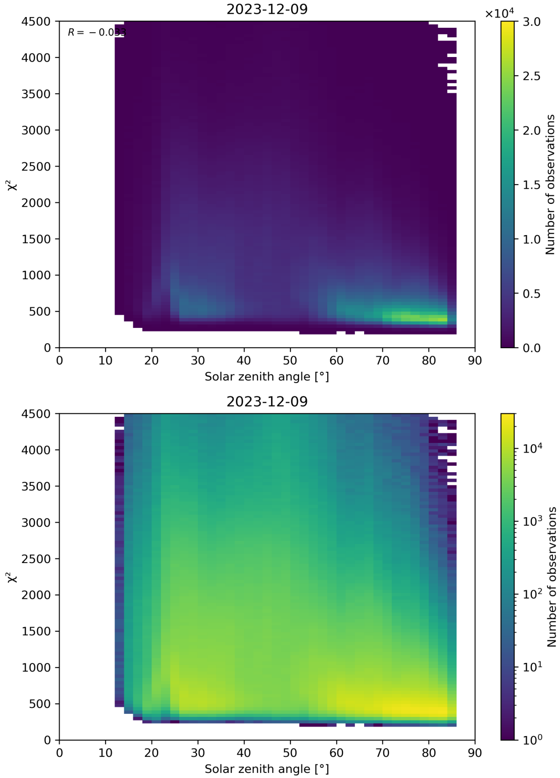
Figure 64: Scatter density plot of “Solar zenith angle” against “ \chi^2 ” for 2023-12-09 to 2023-12-10.
