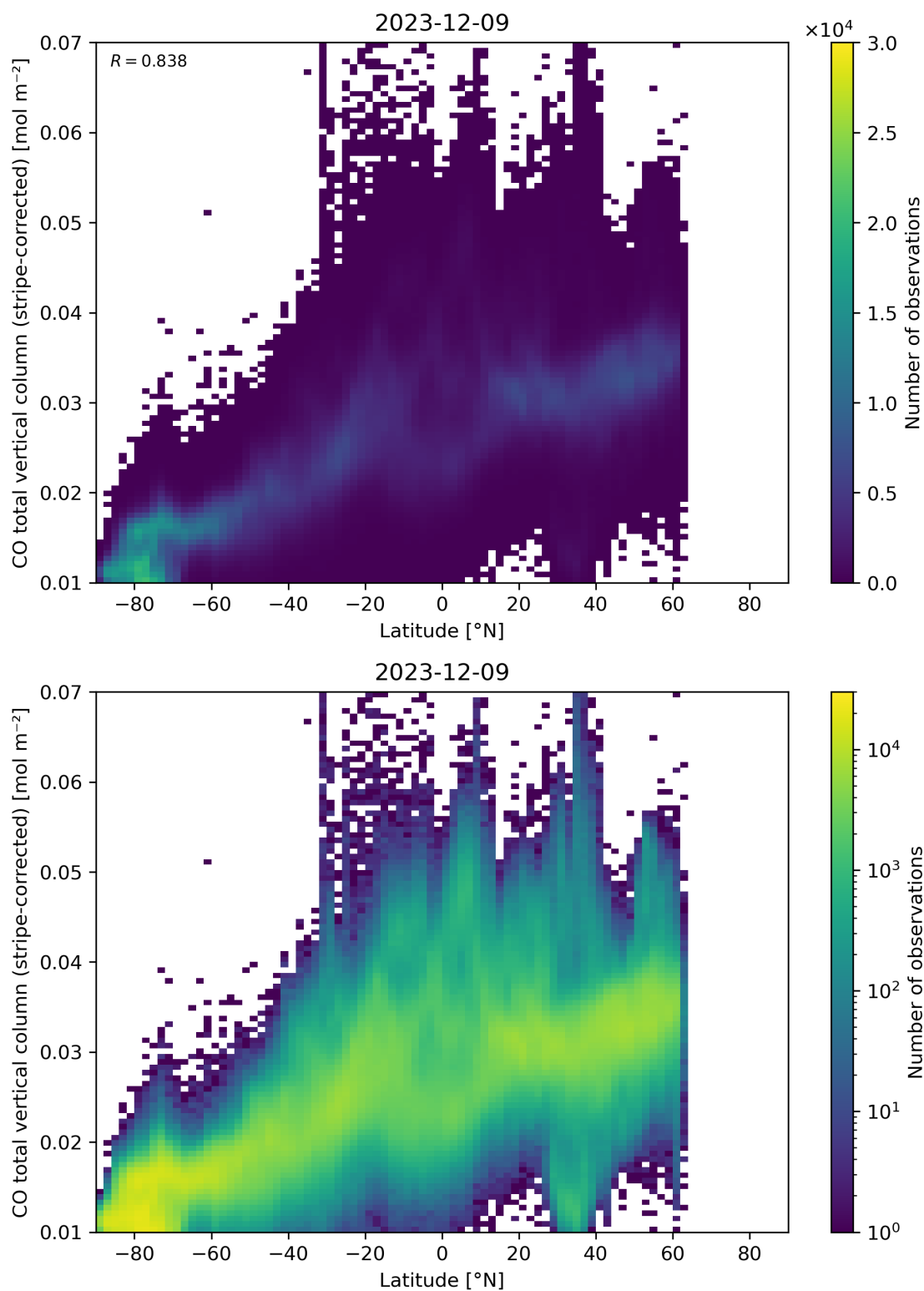
Figure 52: Scatter density plot of “Latitude” against “CO total vertical column (stripe-corrected)” for 2023-12-09 to 2023-12-10.
