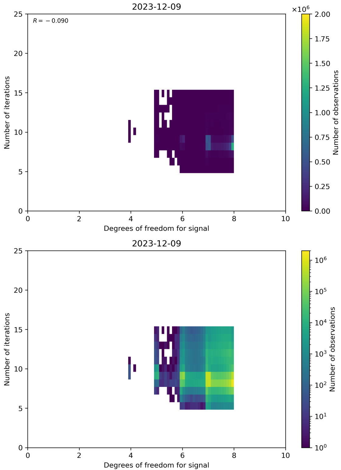
Figure 50: Scatter density plot of “Degrees of freedom for signal” against “Number of iterations” for 2023-12-09 to 2023-12-10.
