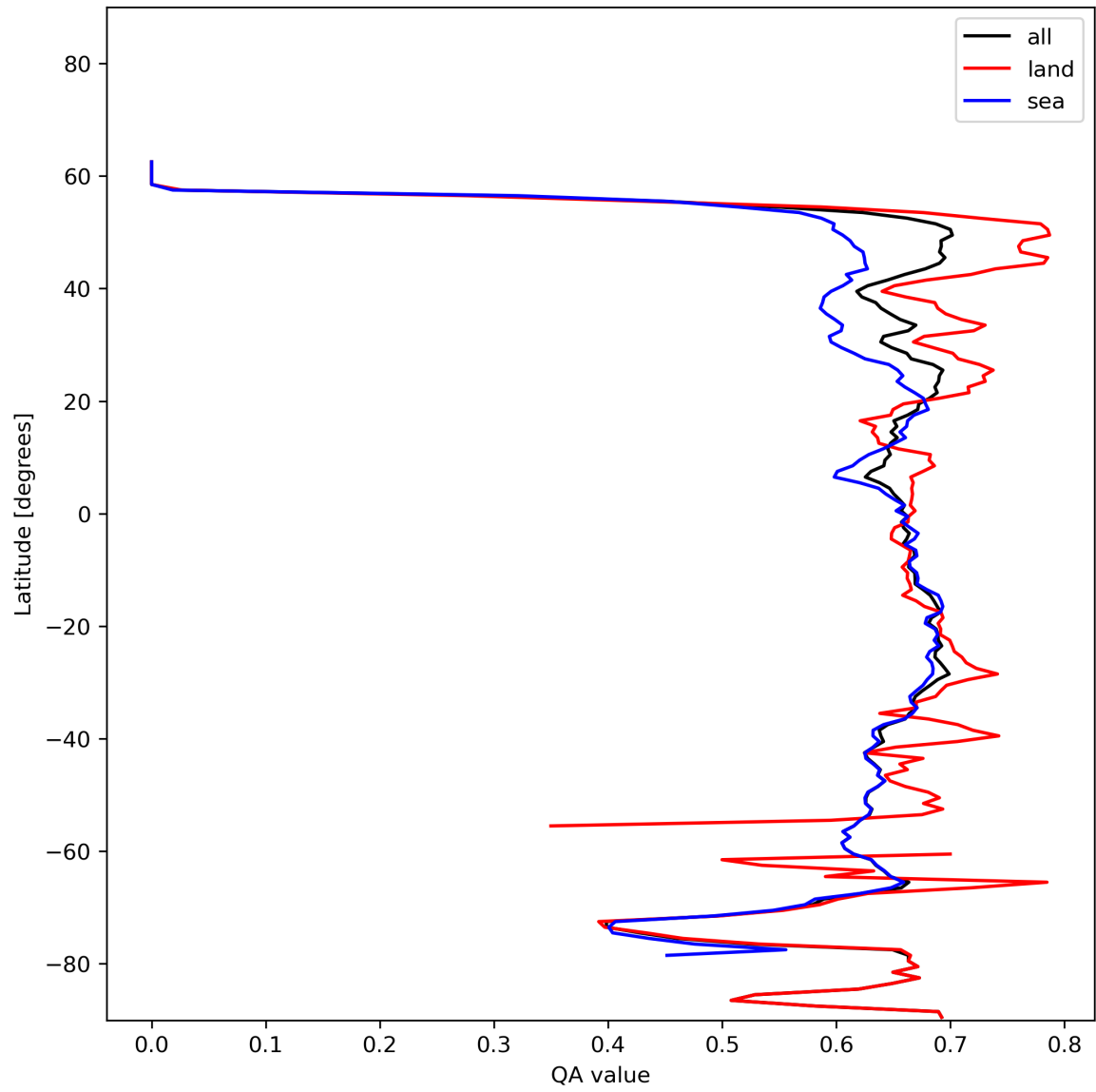
Figure 9: Zonal average of “QA value” for 2023-12-09 to 2023-12-10.
