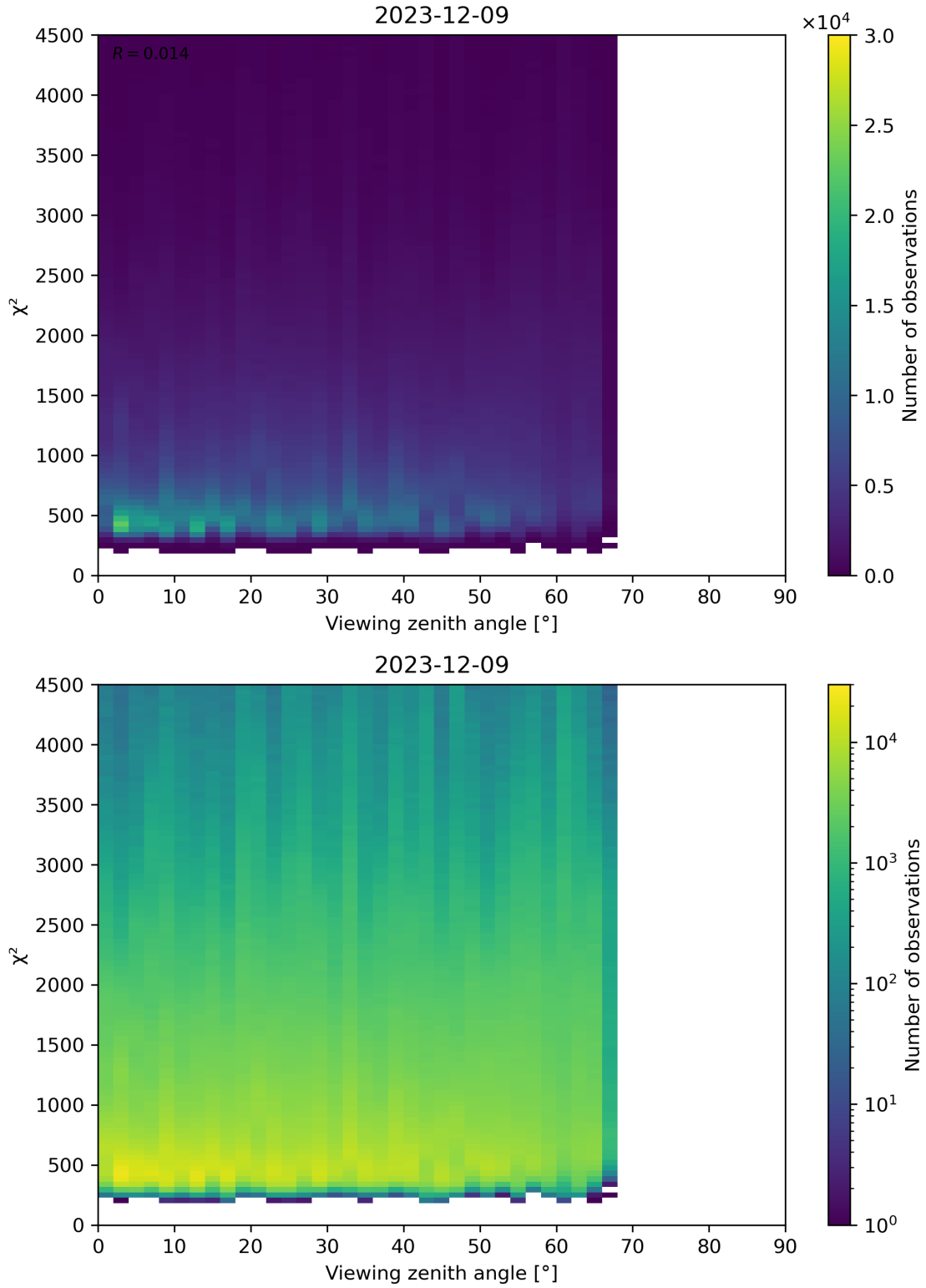
Figure 72: Scatter density plot of “Viewing zenith angle” against “ \chi^2 ” for 2023-12-09 to 2023-12-10.
