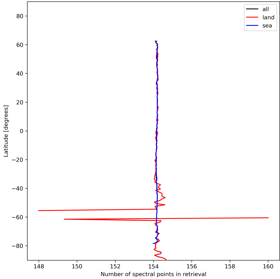
Figure 13: Zonal average of “Number of spectral points in retrieval” for 2023-12-09 to 2023-12-10.
