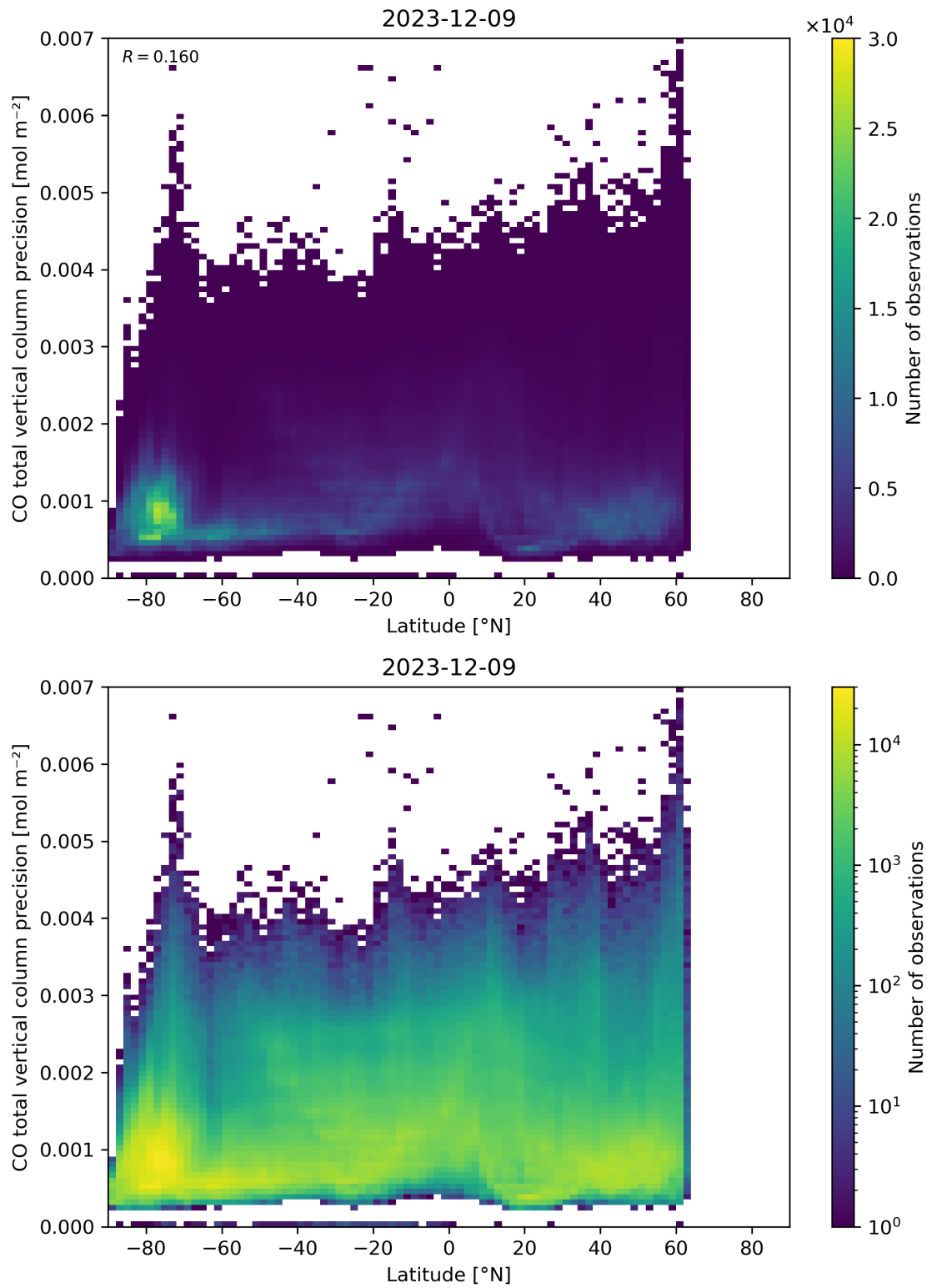
Figure 53: Scatter density plot of “Latitude” against “CO total vertical column precision” for 2023-12-09 to 2023-12-10.
