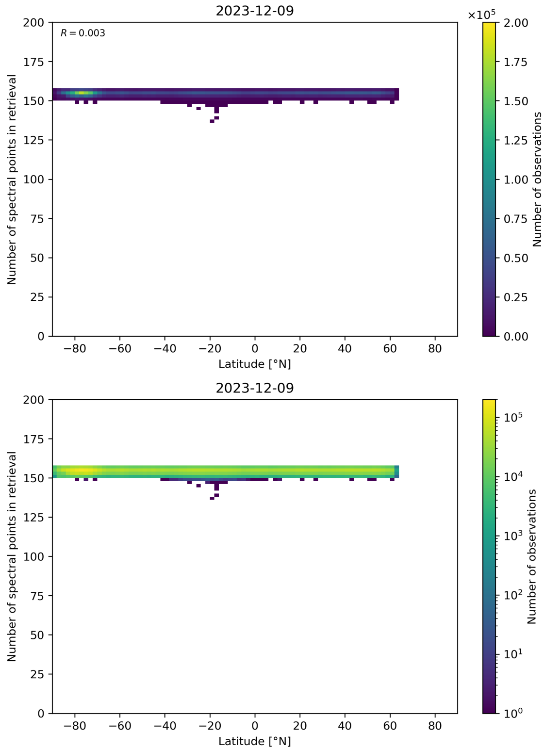
Figure 57: Scatter density plot of “Latitude” against “Number of spectral points in retrieval” for 2023-12-09 to 2023-12-10.
