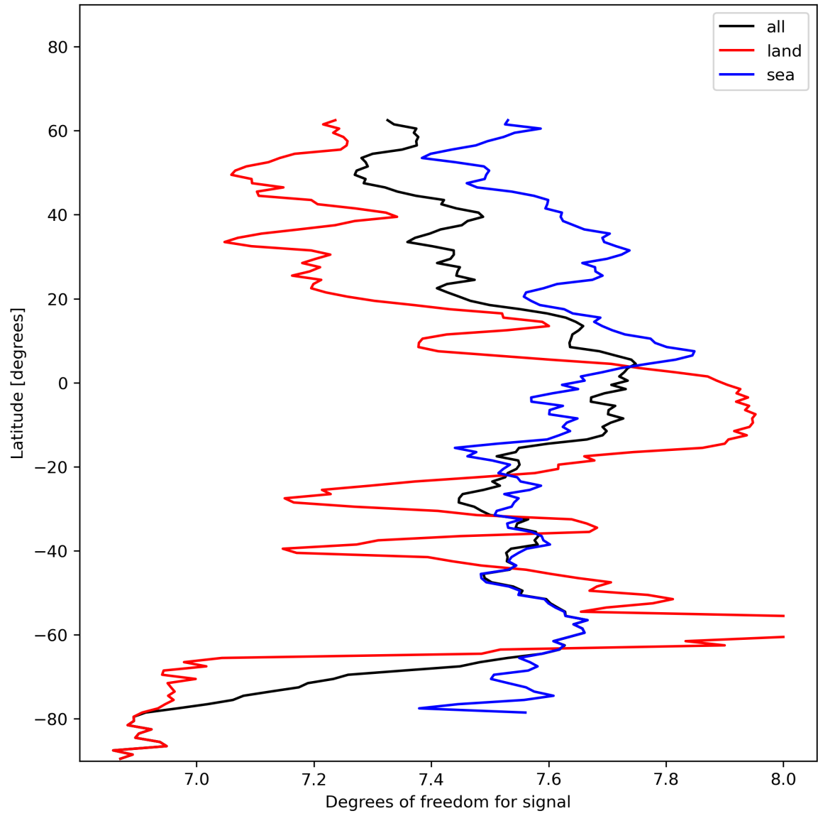
Figure 15: Zonal average of “Degrees of freedom for signal” for 2023-12-09 to 2023-12-10.
