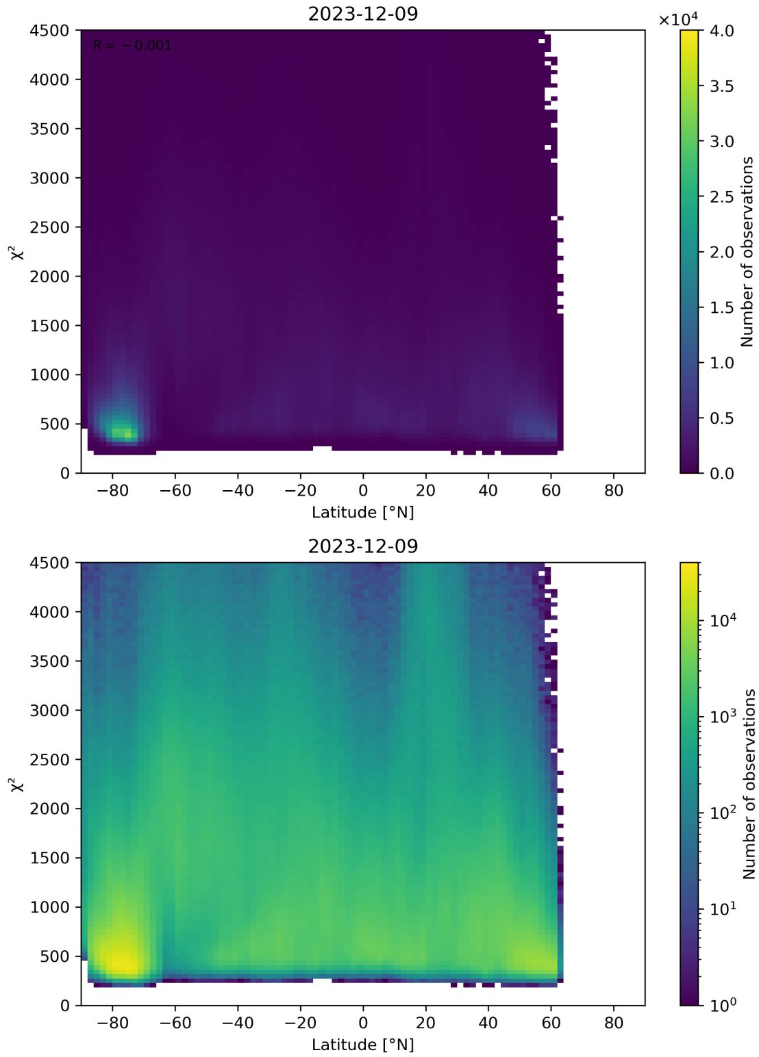
Figure 54: Scatter density plot of “Latitude” against “ \chi^2 ” for 2023-12-09 to 2023-12-10.
