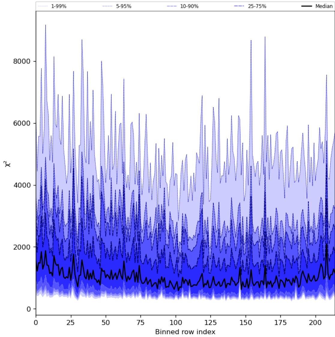
Figure 30: Along track statistics of “ \chi^2 ” for 2023-12-09 to 2023-12-10
