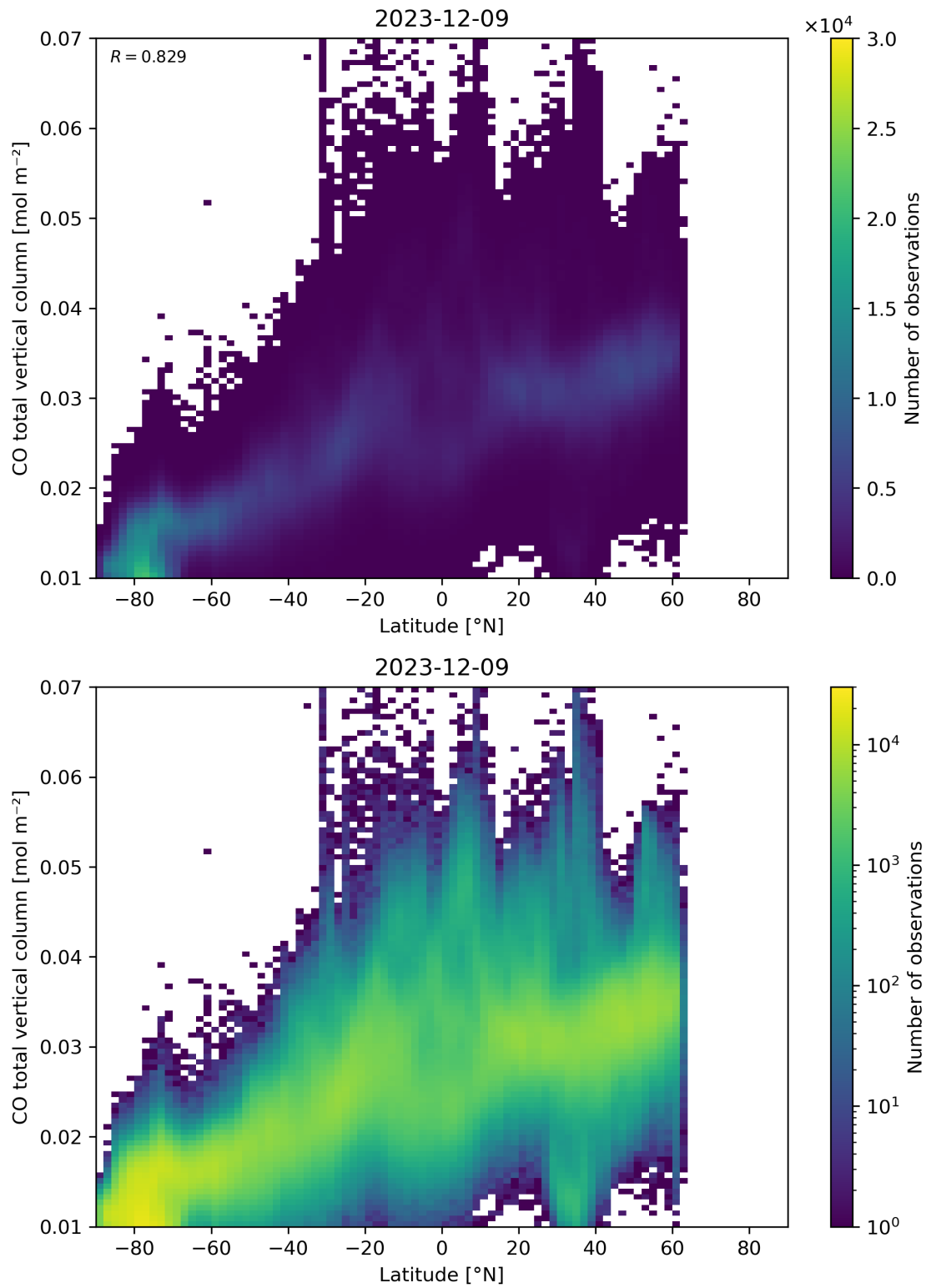
Figure 51: Scatter density plot of “Latitude” against “CO total vertical column” for 2023-12-09 to 2023-12-10.
