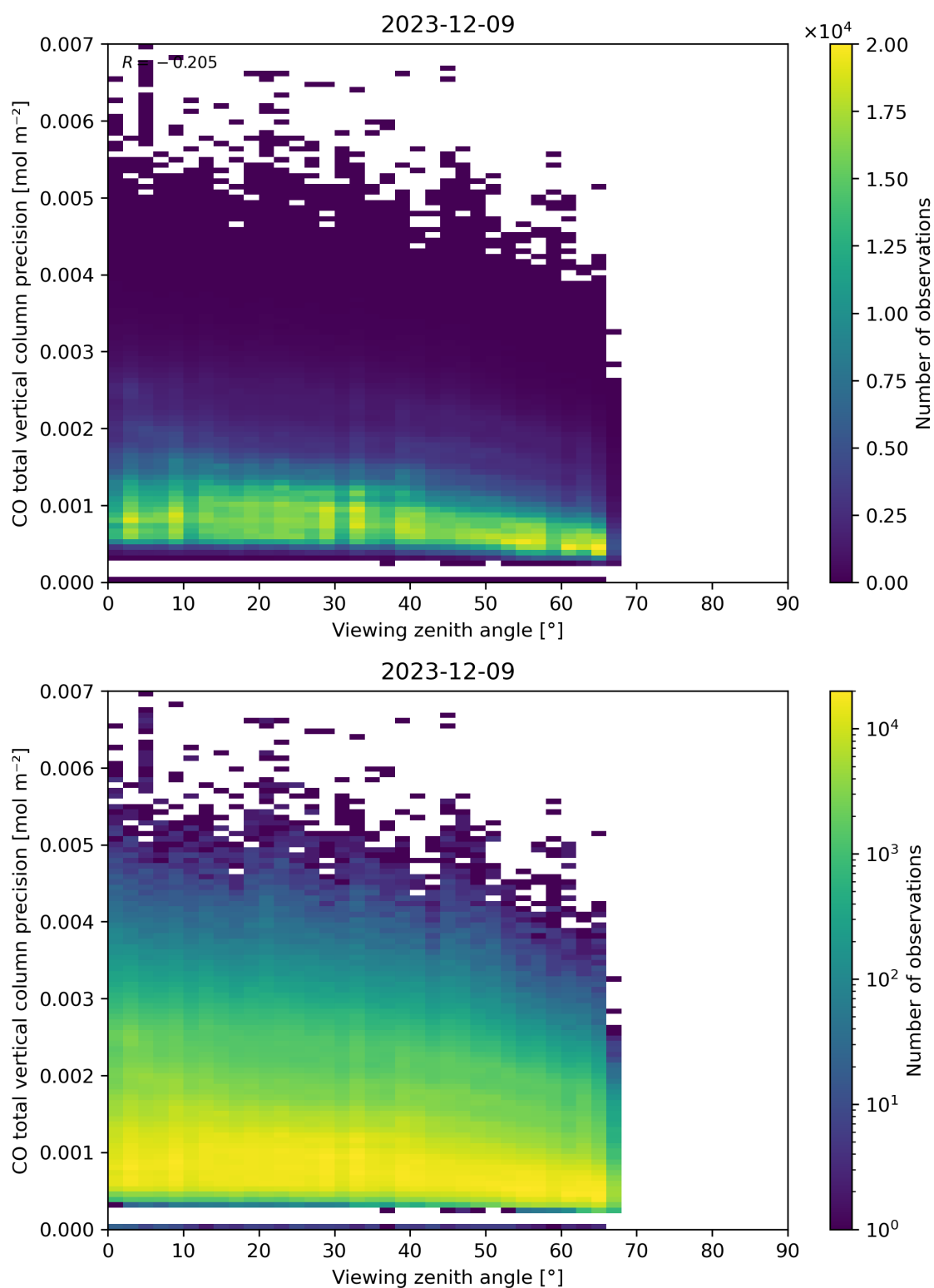
Figure 71: Scatter density plot of “Viewing zenith angle” against “CO total vertical column precision” for 2023-12-09 to 2023-12-10.
