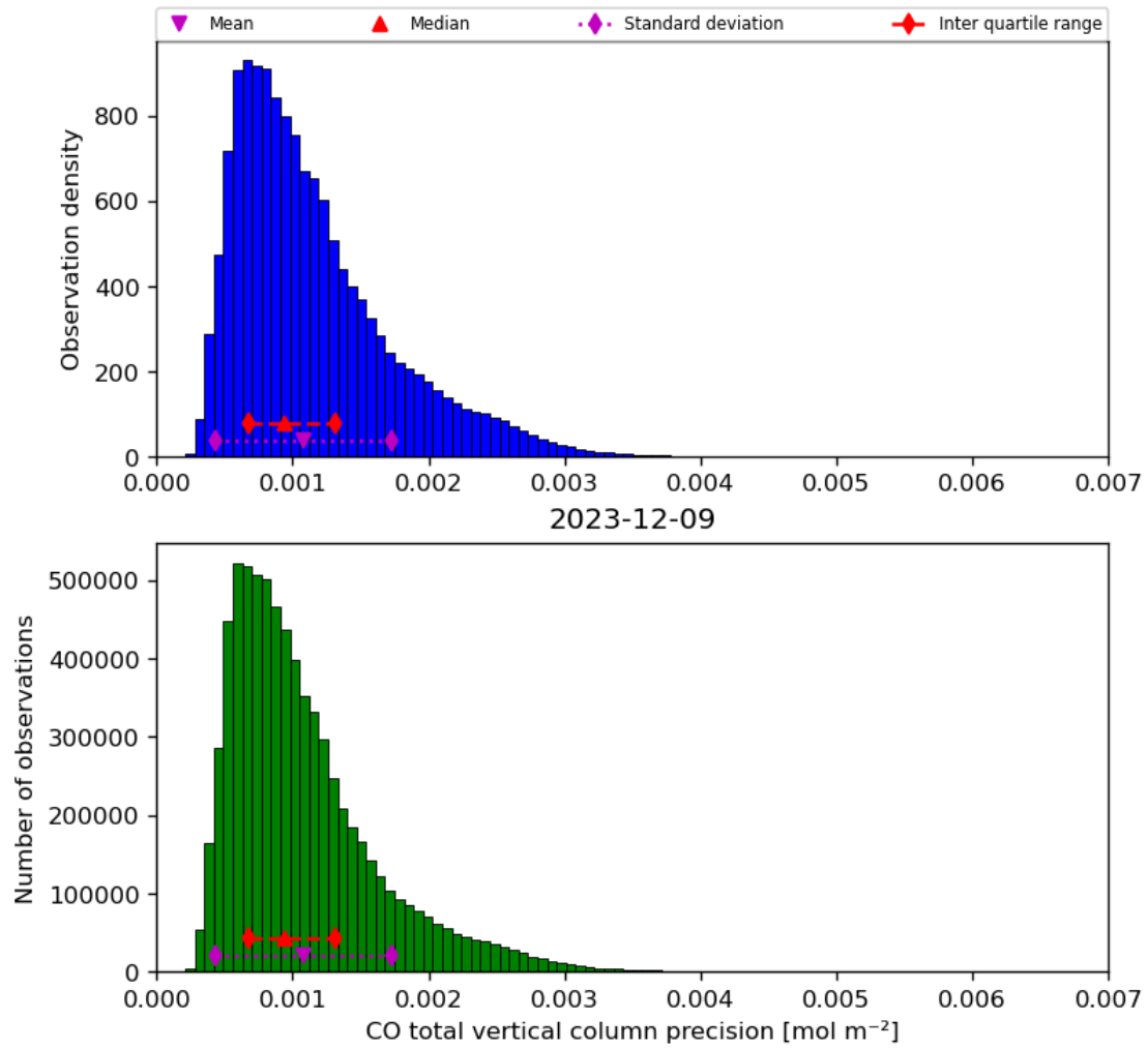
Figure 20: Histogram of “CO total vertical column precision” for 2023-12-09 to 2023-12-10
