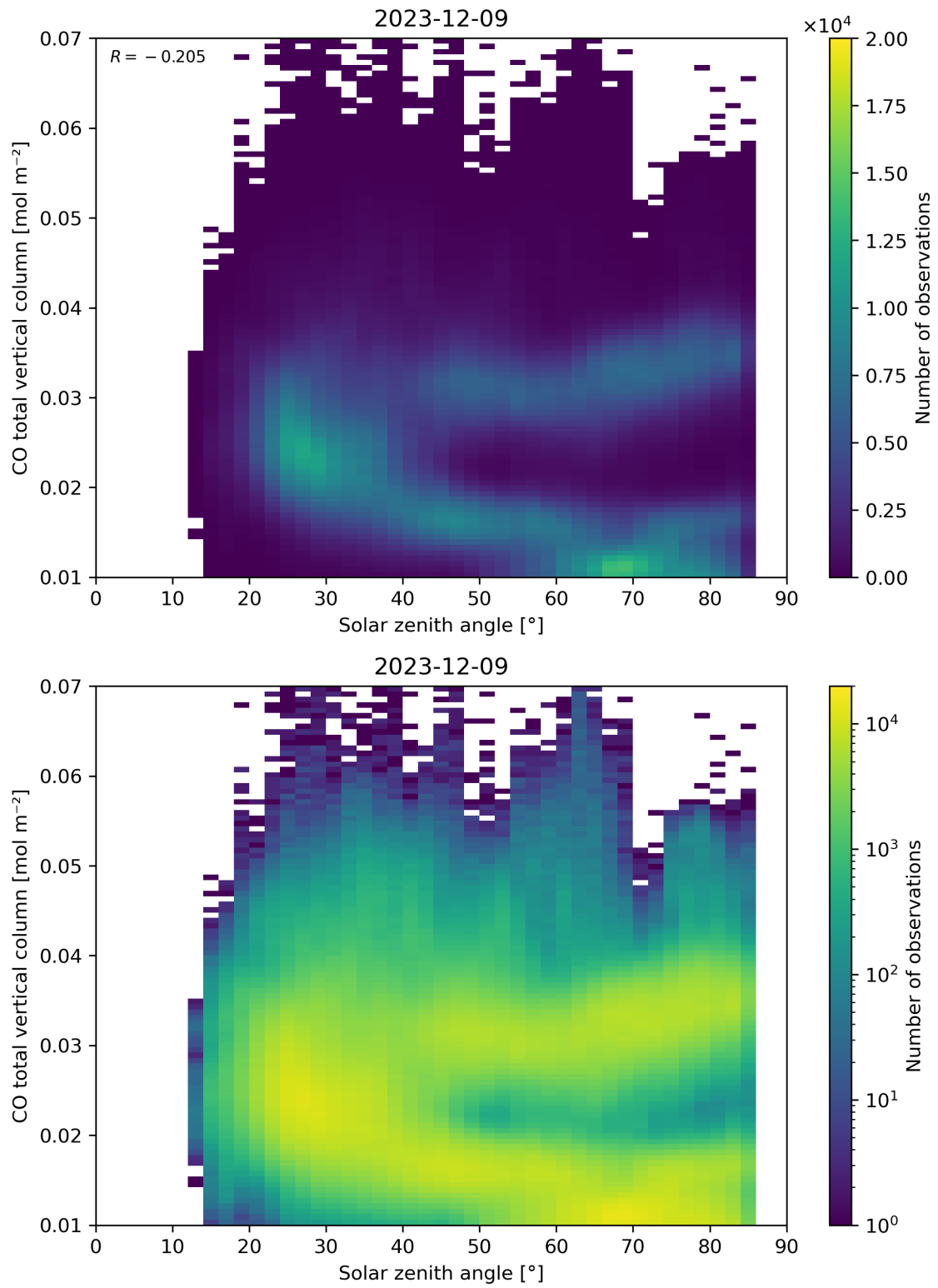
Figure 61: Scatter density plot of “Solar zenith angle” against “CO total vertical column” for 2023-12-09 to 2023-12-10.
