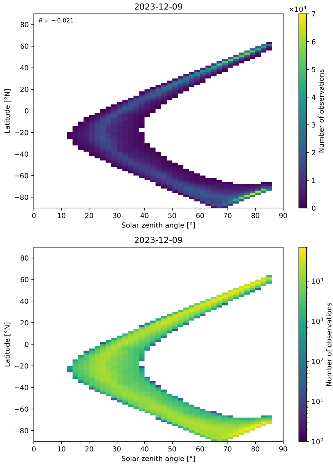
Figure 66: Scatter density plot of “Solar zenith angle” against “Latitude” for 2023-12-09 to 2023-12-10.
