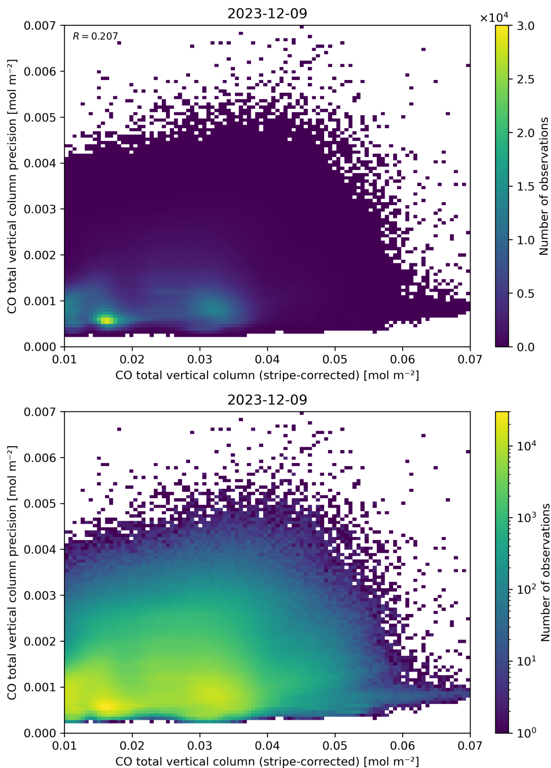
Figure 36: Scatter density plot of “CO total vertical column (stripe-corrected)” against “CO total vertical column precision” for 2023-12-09 to 2023-12-10.
