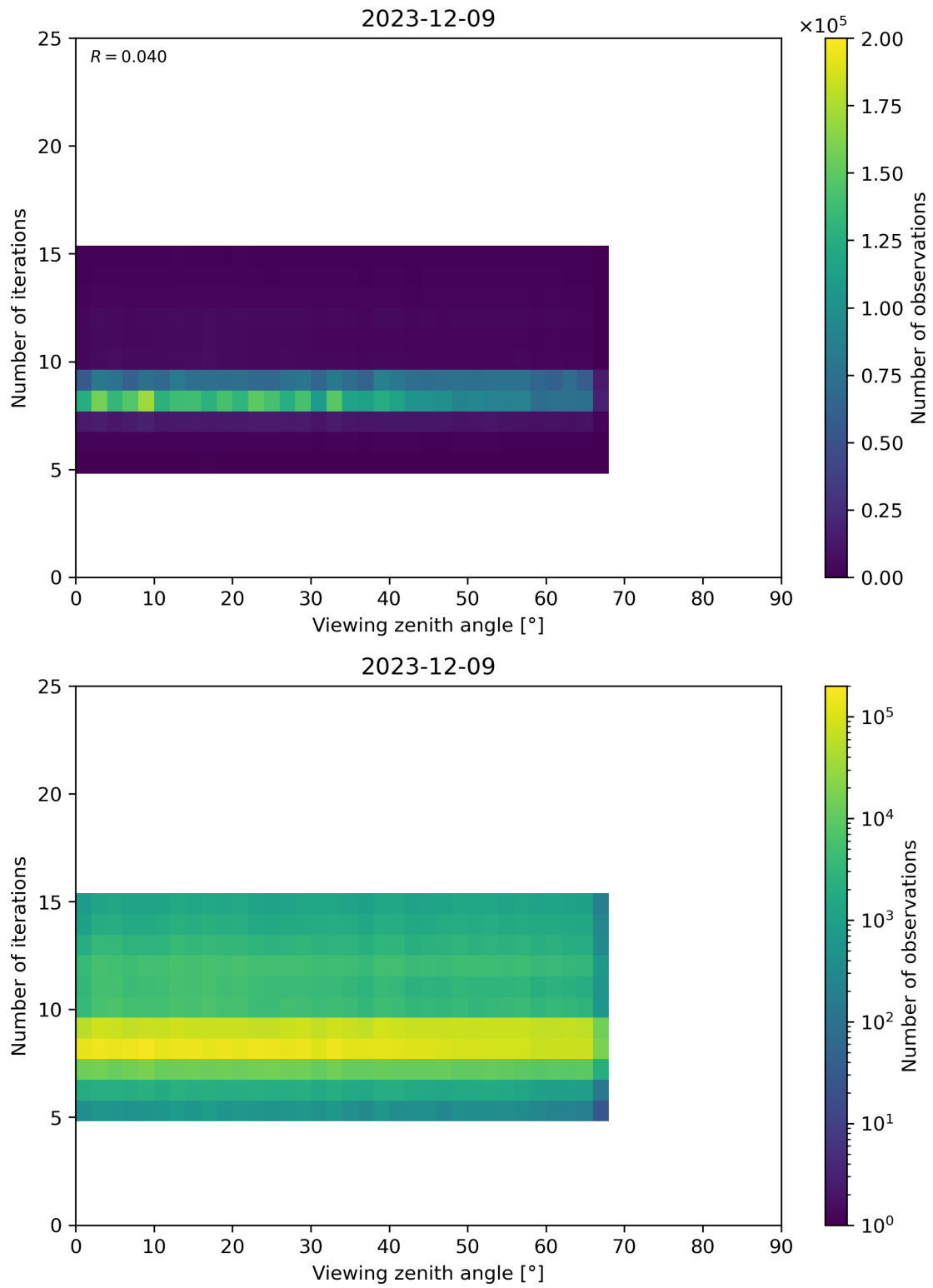
Figure 75: Scatter density plot of “Viewing zenith angle” against “Number of iterations” for 2023-12-09 to 2023-12-10.
