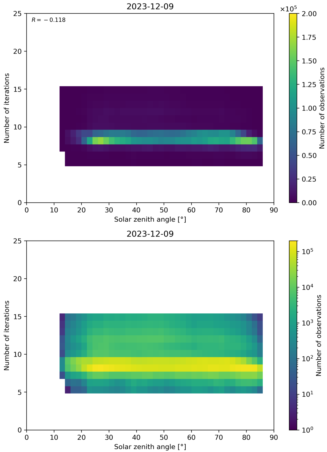
Figure 67: Scatter density plot of “Solar zenith angle” against “Number of iterations” for 2023-12-09 to 2023-12-10.
