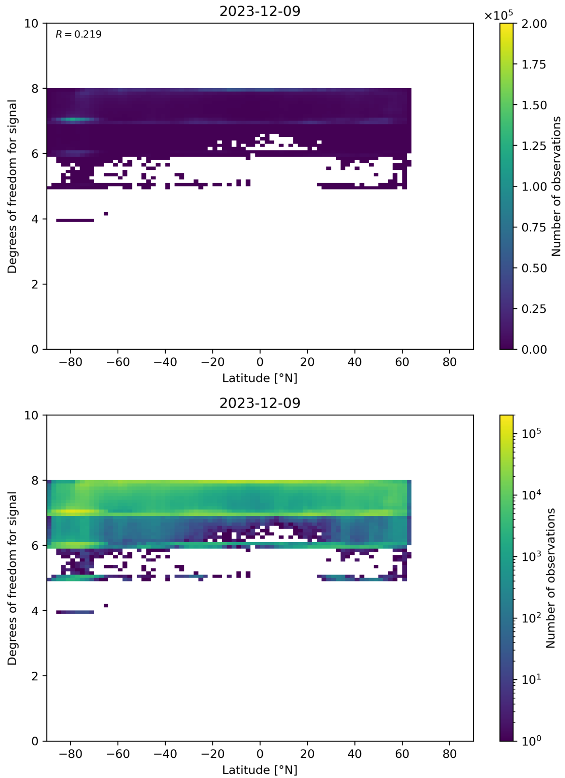
Figure 55: Scatter density plot of “Latitude” against “Degrees of freedom for signal” for 2023-12-09 to 2023-12-10.
