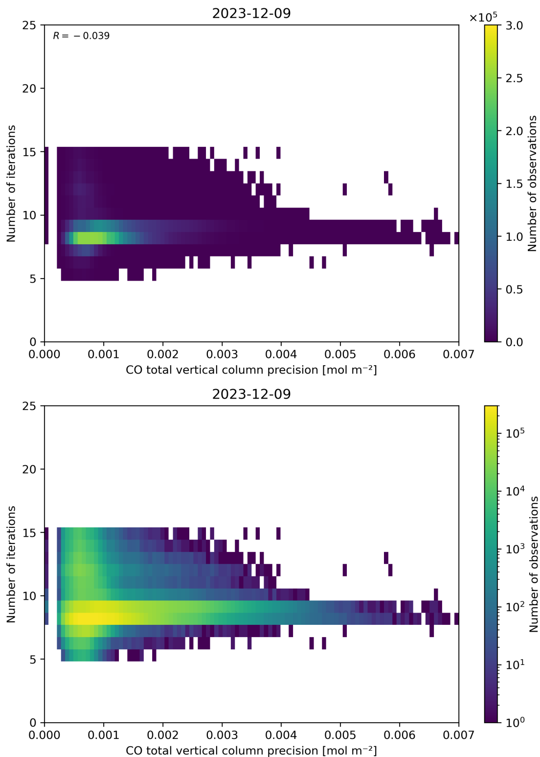
Figure 46: Scatter density plot of “CO total vertical column precision” against “Number of iterations” for 2023-12-09 to 2023-12-10.
