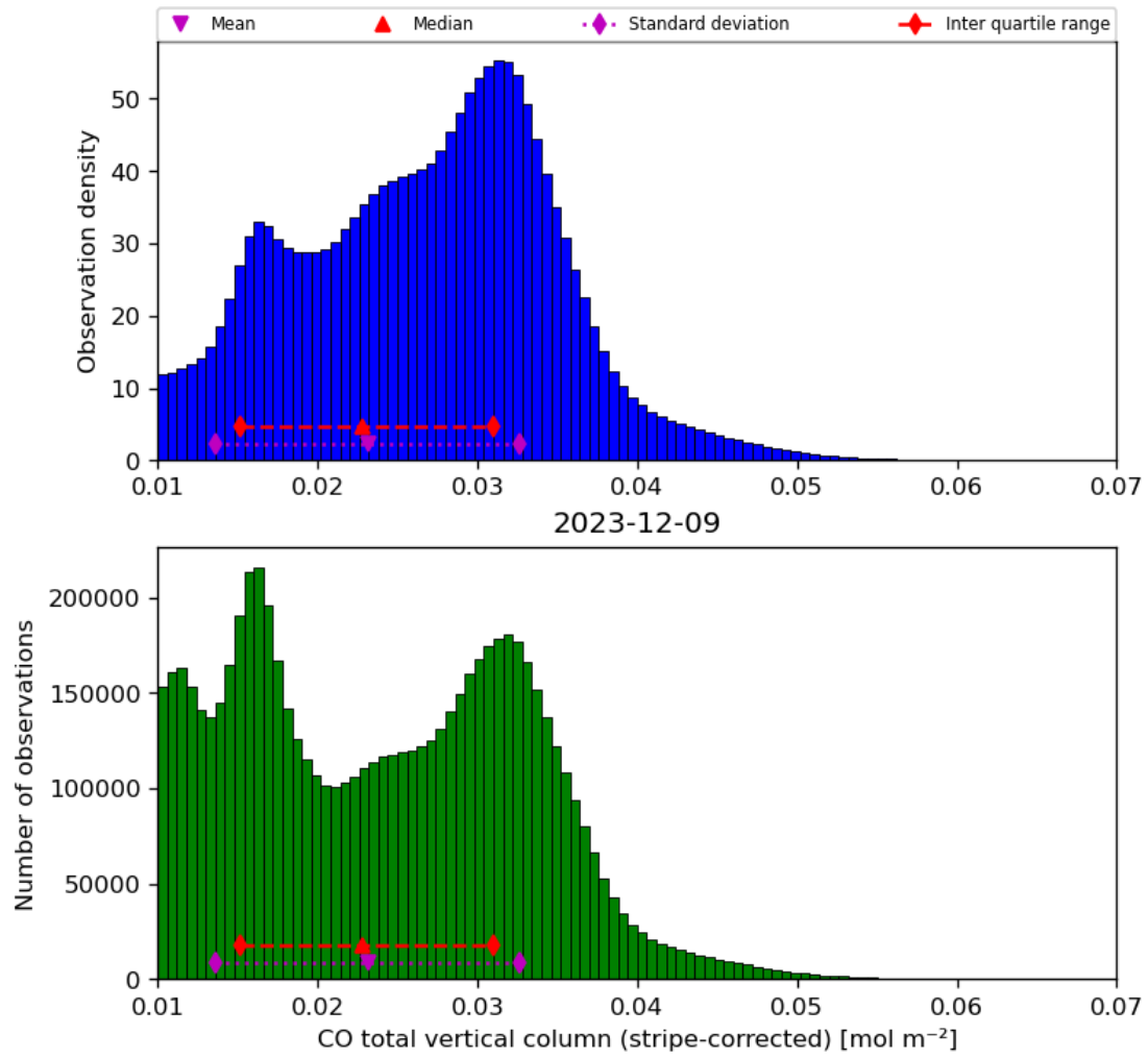
Figure 19: Histogram of “CO total vertical column (stripe-corrected)” for 2023-12-09 to 2023-12-10
