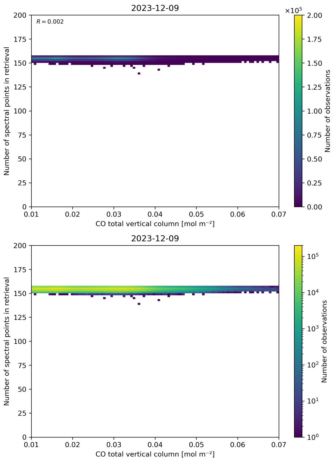
Figure 43: Scatter density plot of “CO total vertical column” against “Number of spectral points in retrieval” for 2023-12-09 to 2023-12-10.
