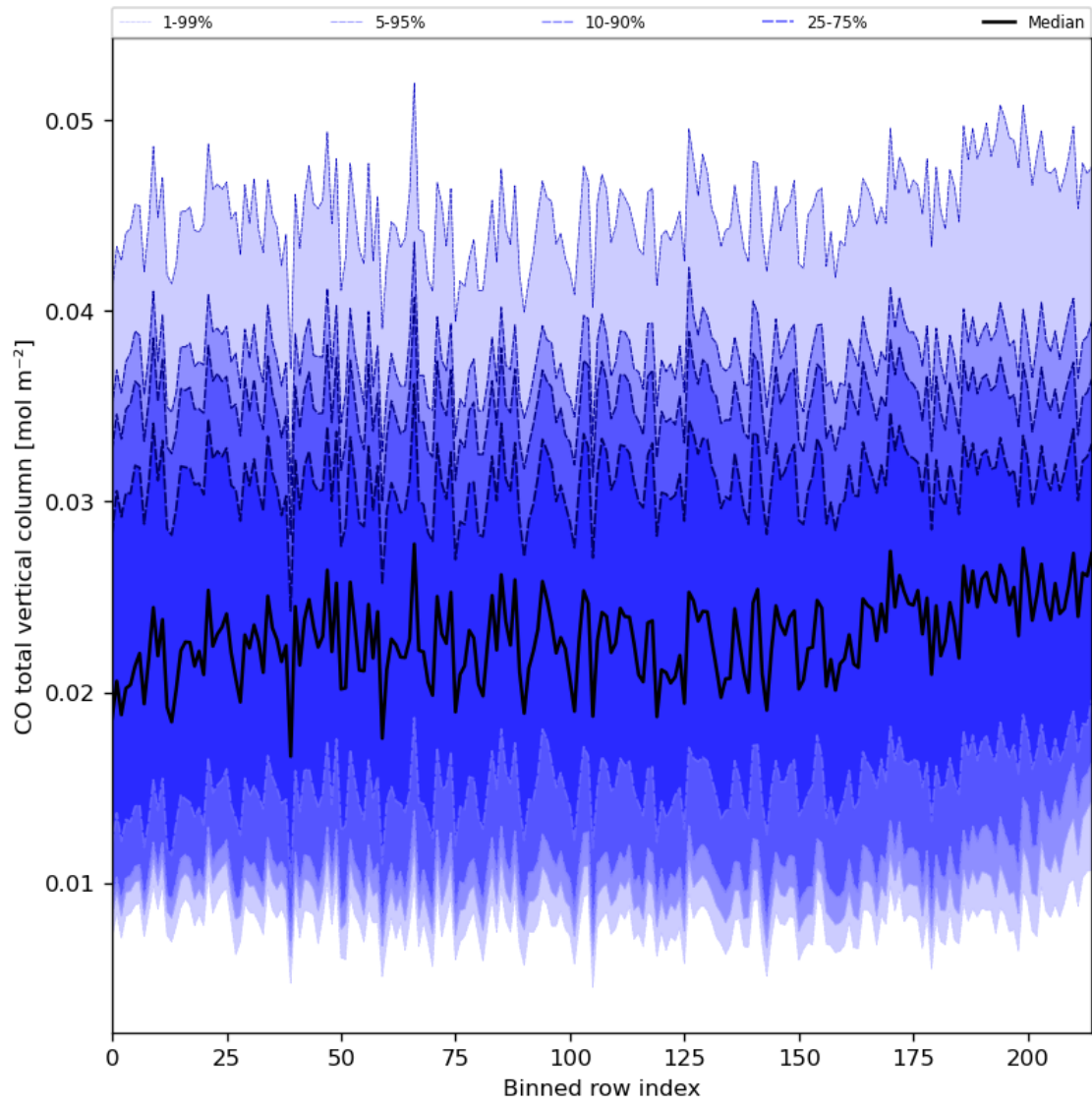
Figure 26: Along track statistics of “CO total vertical column” for 2023-12-09 to 2023-12-10
