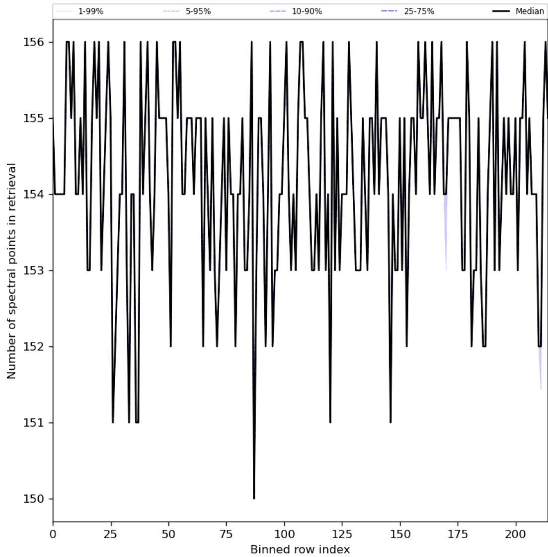
Figure 29: Along track statistics of “Number of spectral points in retrieval” for 2023-12-09 to 2023-12-10
