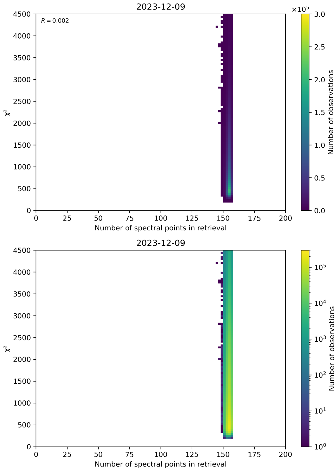
Figure 58: Scatter density plot of “Number of spectral points in retrieval” against “ \chi^2 ” for 2023-12-09 to 2023-12-10.
