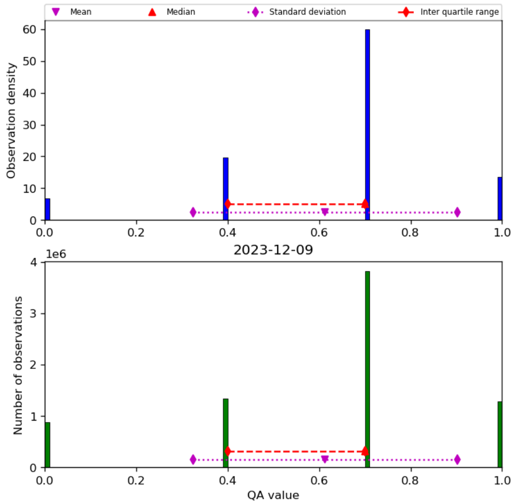
Figure 17: Histogram of “QA value” for 2023-12-09 to 2023-12-10
