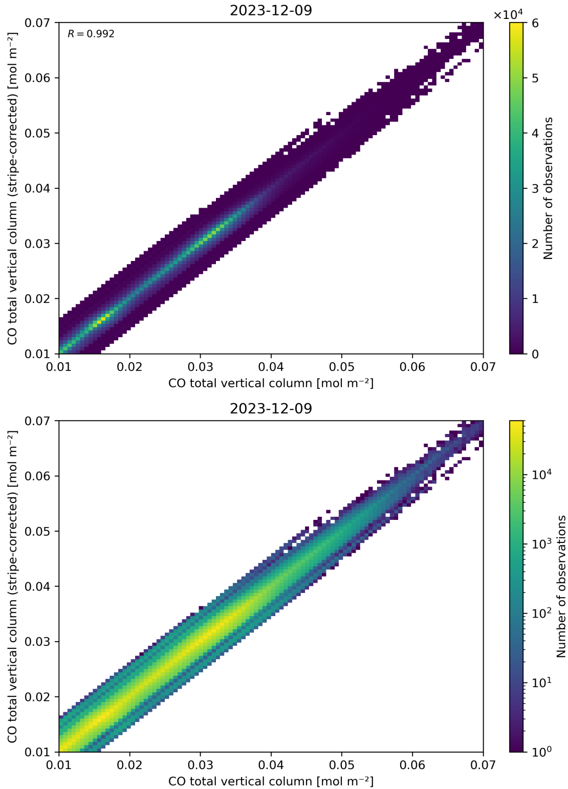
Figure 33: Scatter density plot of “CO total vertical column” against “CO total vertical column (stripe-corrected)” for 2023-12-09 to 2023-12-10.
