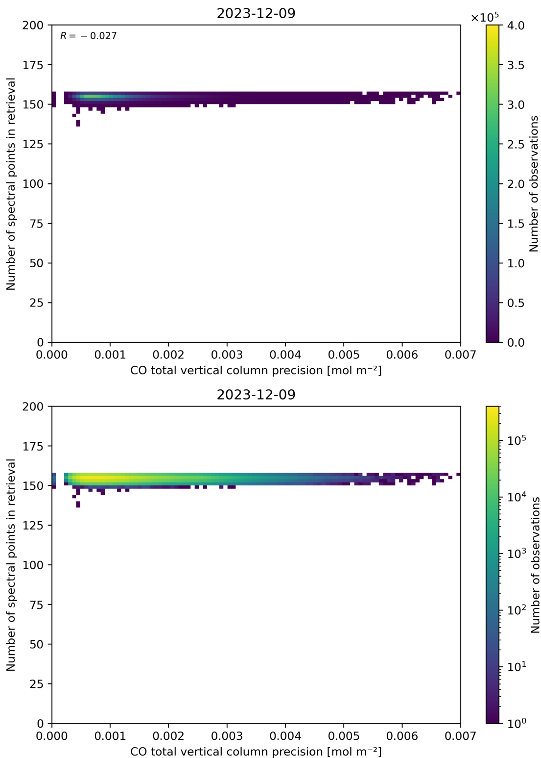
Figure 47: Scatter density plot of “CO total vertical column precision” against “Number of spectral points in retrieval” for 2023-12-09 to 2023-12-10.
