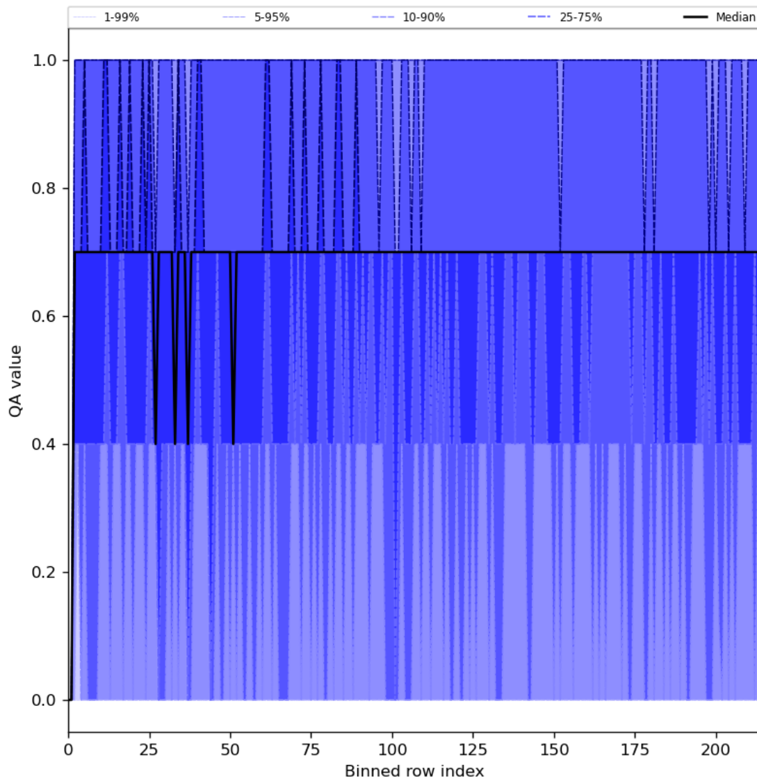
Figure 25: Along track statistics of “QA value” for 2023-12-09 to 2023-12-10
