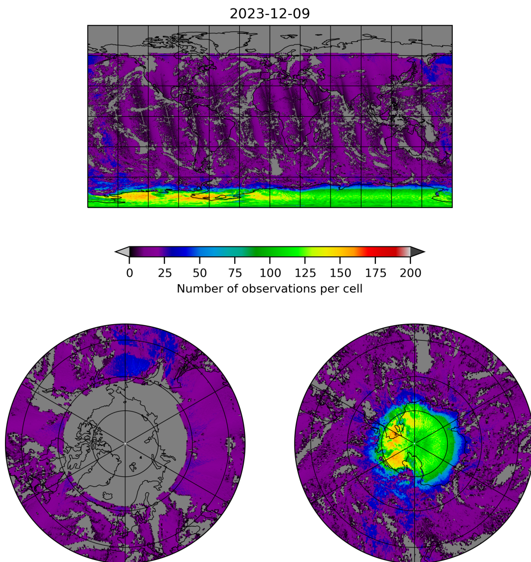
Figure 8: Map of the number of observations for 2023-12-09 to 2023-12-10
