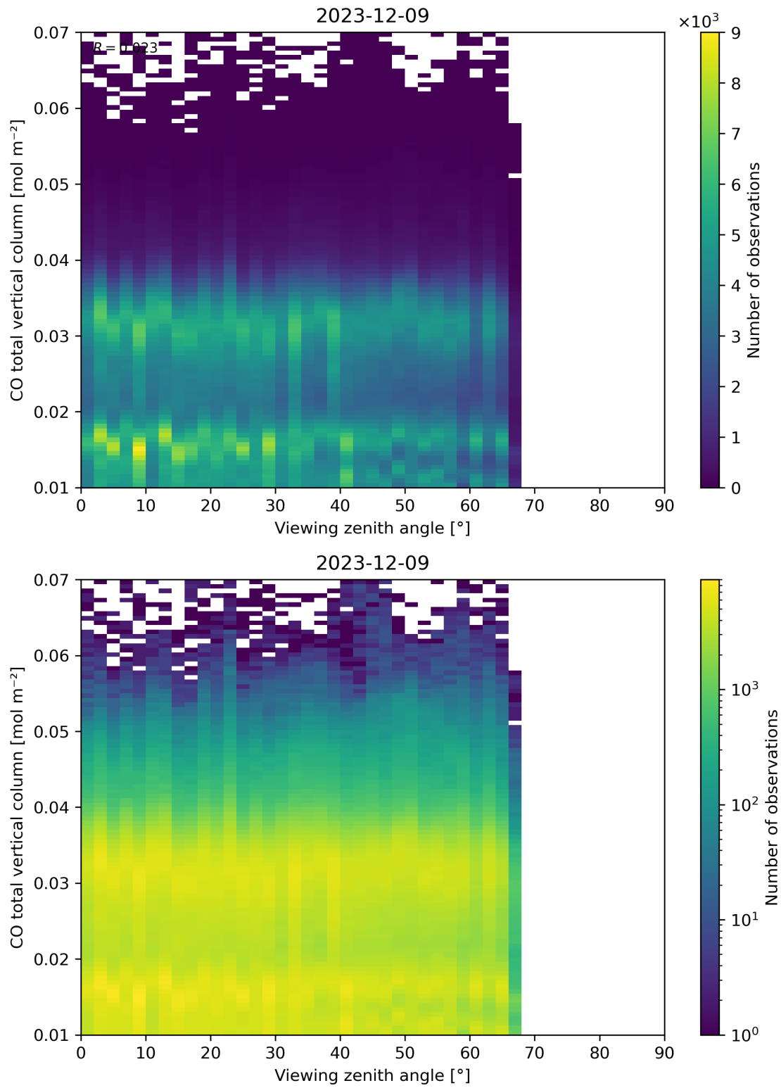
Figure 69: Scatter density plot of “Viewing zenith angle” against “CO total vertical column” for 2023-12-09 to 2023-12-10.
