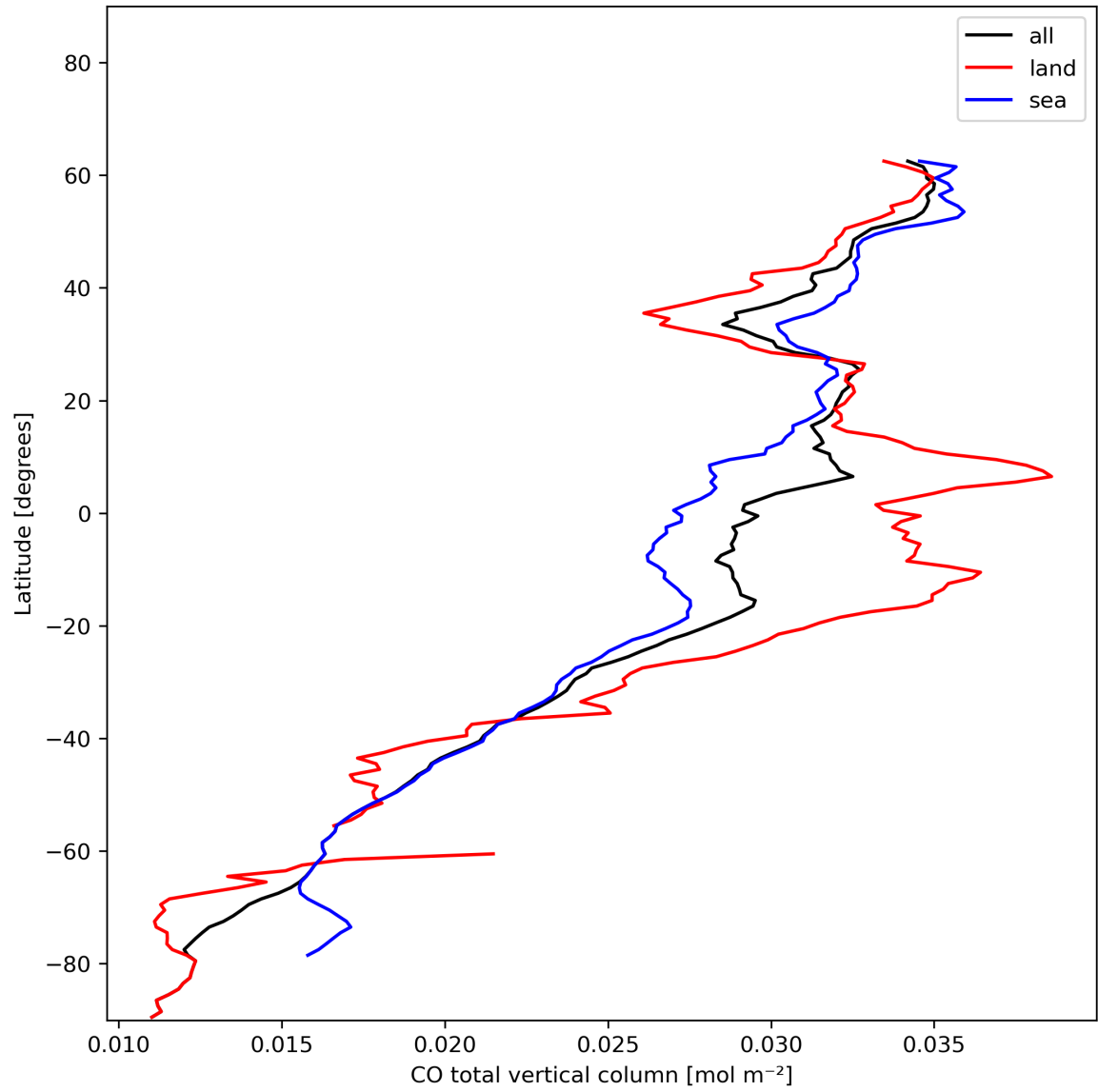
Figure 10: Zonal average of “CO total vertical column” for 2023-12-09 to 2023-12-10.
