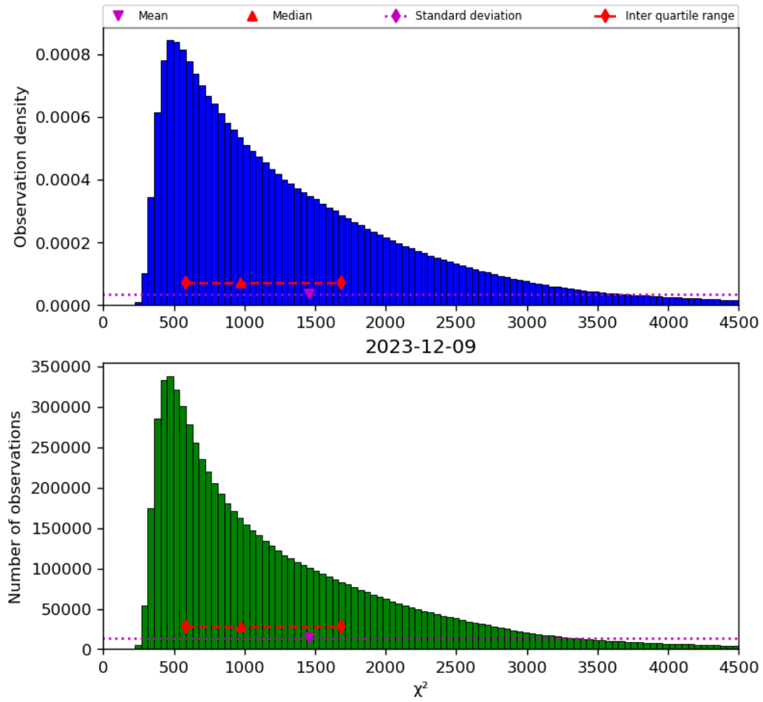
Figure 22: Histogram of “ \chi^2 ” for 2023-12-09 to 2023-12-10
