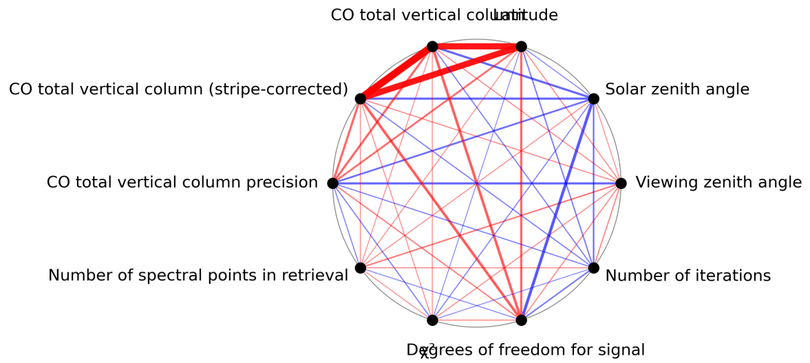
Figure 1: Map of correlation graph for 2023-12-09 to 2023-12-10.
