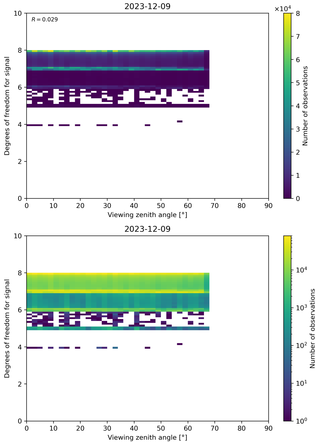
Figure 73: Scatter density plot of “Viewing zenith angle” against “Degrees of freedom for signal” for 2023-12-09 to 2023-12-10.
