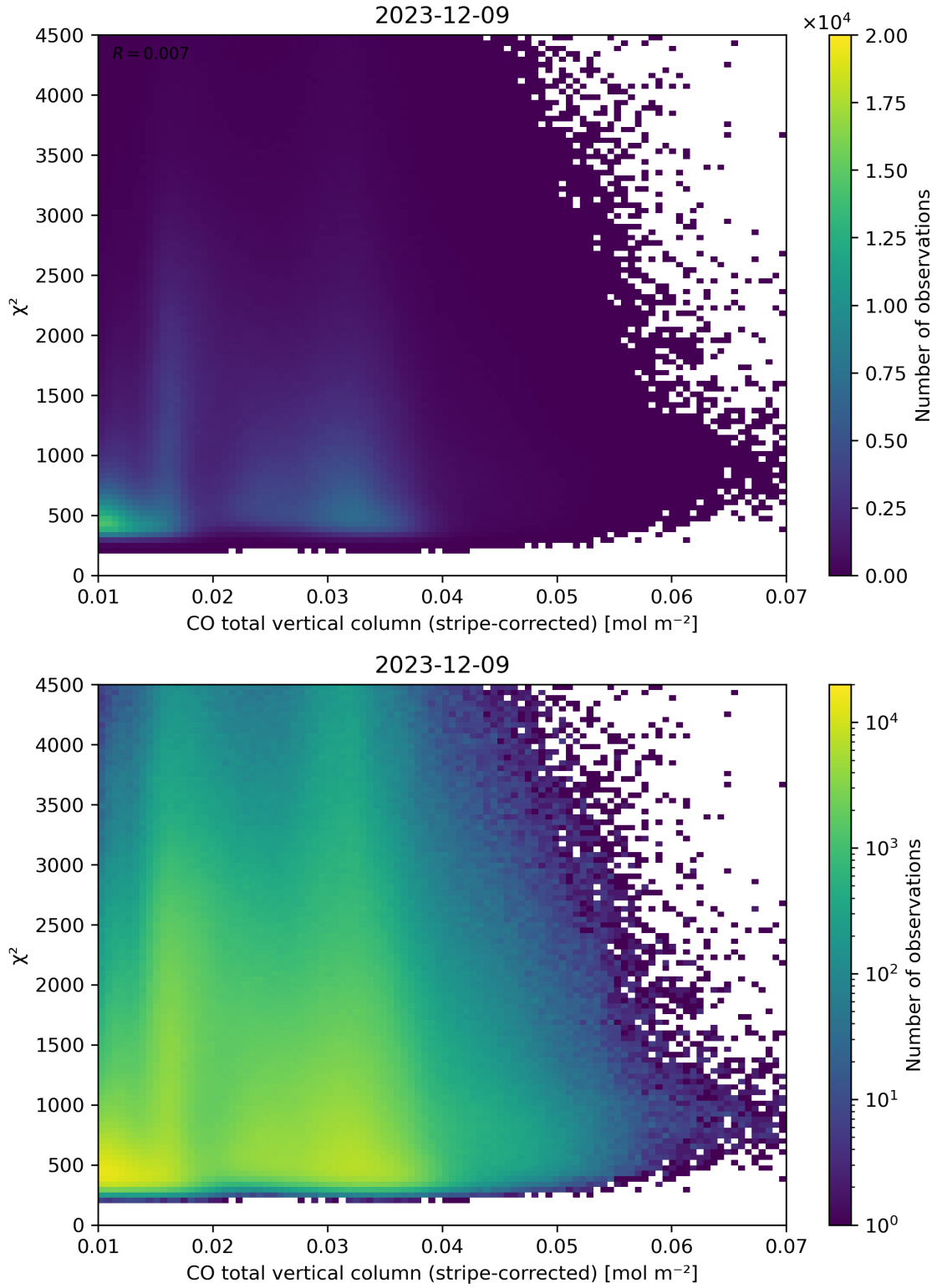
Figure 37: Scatter density plot of “CO total vertical column (stripe-corrected)” against “ \chi^2 ” for 2023-12-09 to 2023-12-10.
