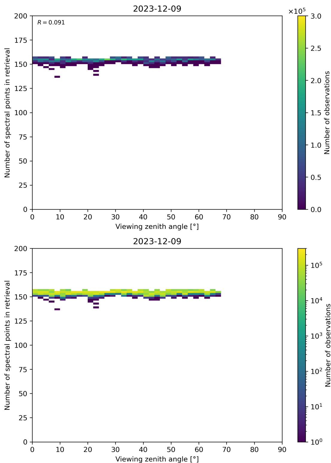
Figure 76: Scatter density plot of “Viewing zenith angle” against “Number of spectral points in retrieval” for 2023-12-09 to 2023-12-10.
