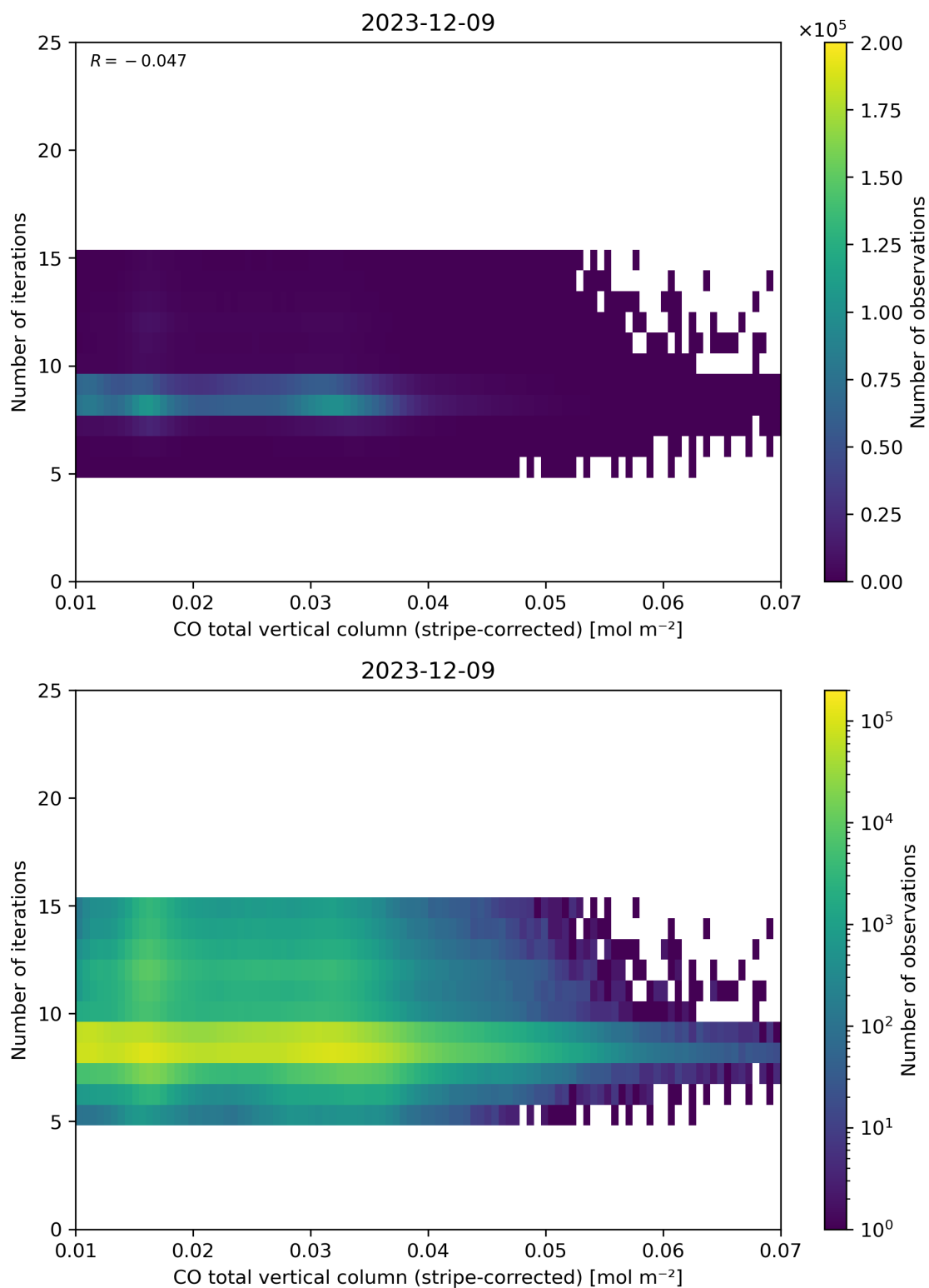
Figure 39: Scatter density plot of “CO total vertical column (stripe-corrected)” against “Number of iterations” for 2023-12-09 to 2023-12-10.
