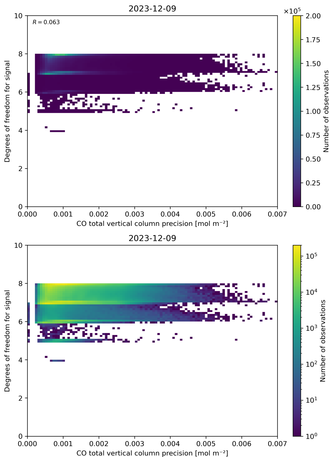
Figure 45: Scatter density plot of “CO total vertical column precision” against “Degrees of freedom for signal” for 2023-12-09 to 2023-12-10.
