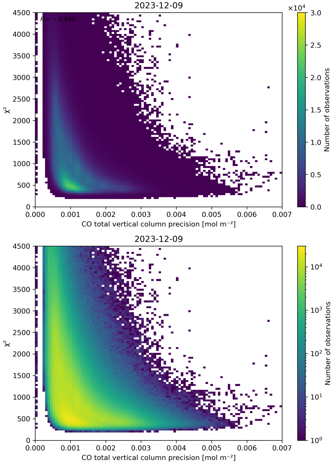
Figure 44: Scatter density plot of “CO total vertical column precision” against “ \chi^2 ” for 2023-12-09 to 2023-12-10.
