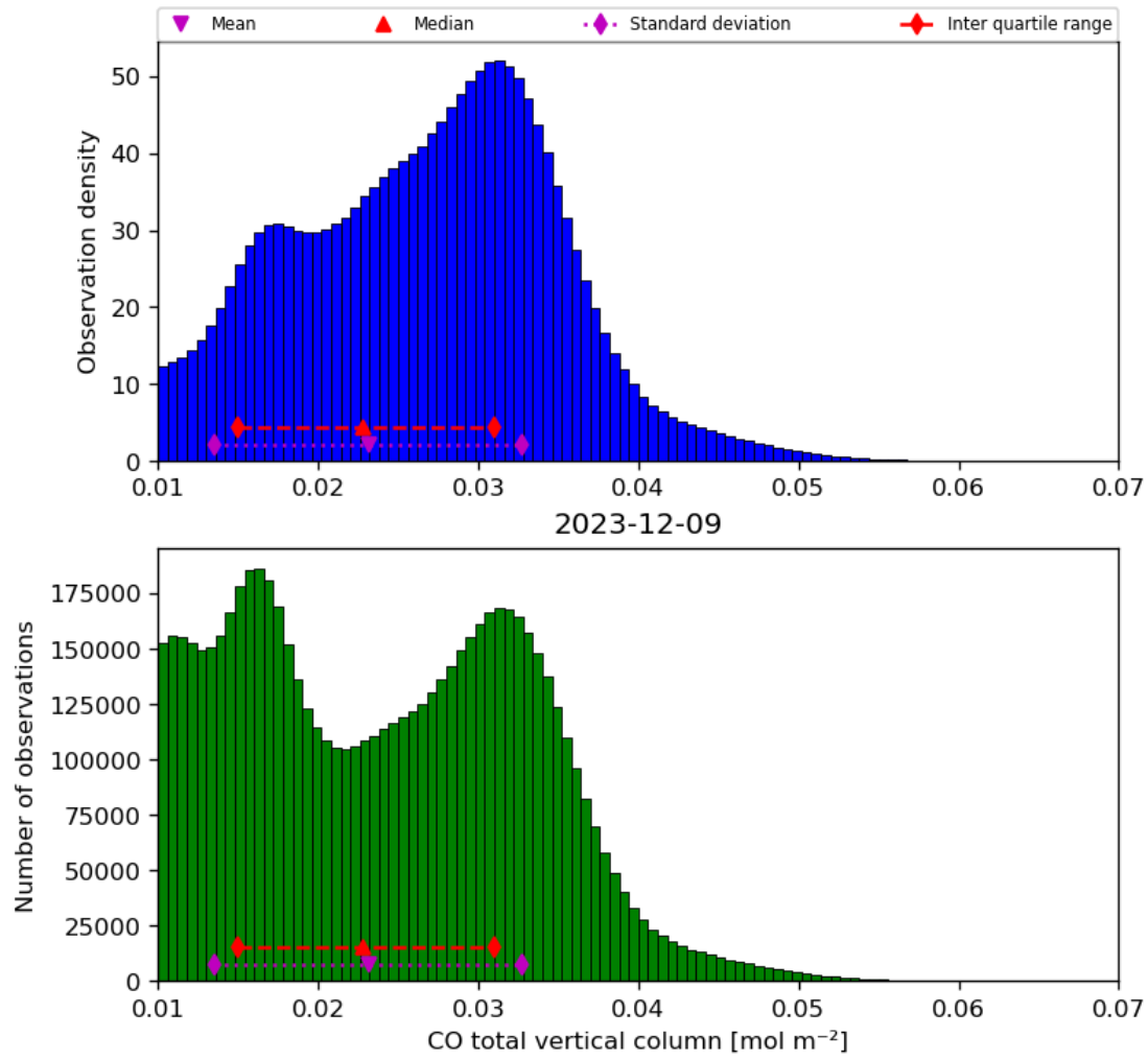
Figure 18: Histogram of “CO total vertical column” for 2023-12-09 to 2023-12-10
