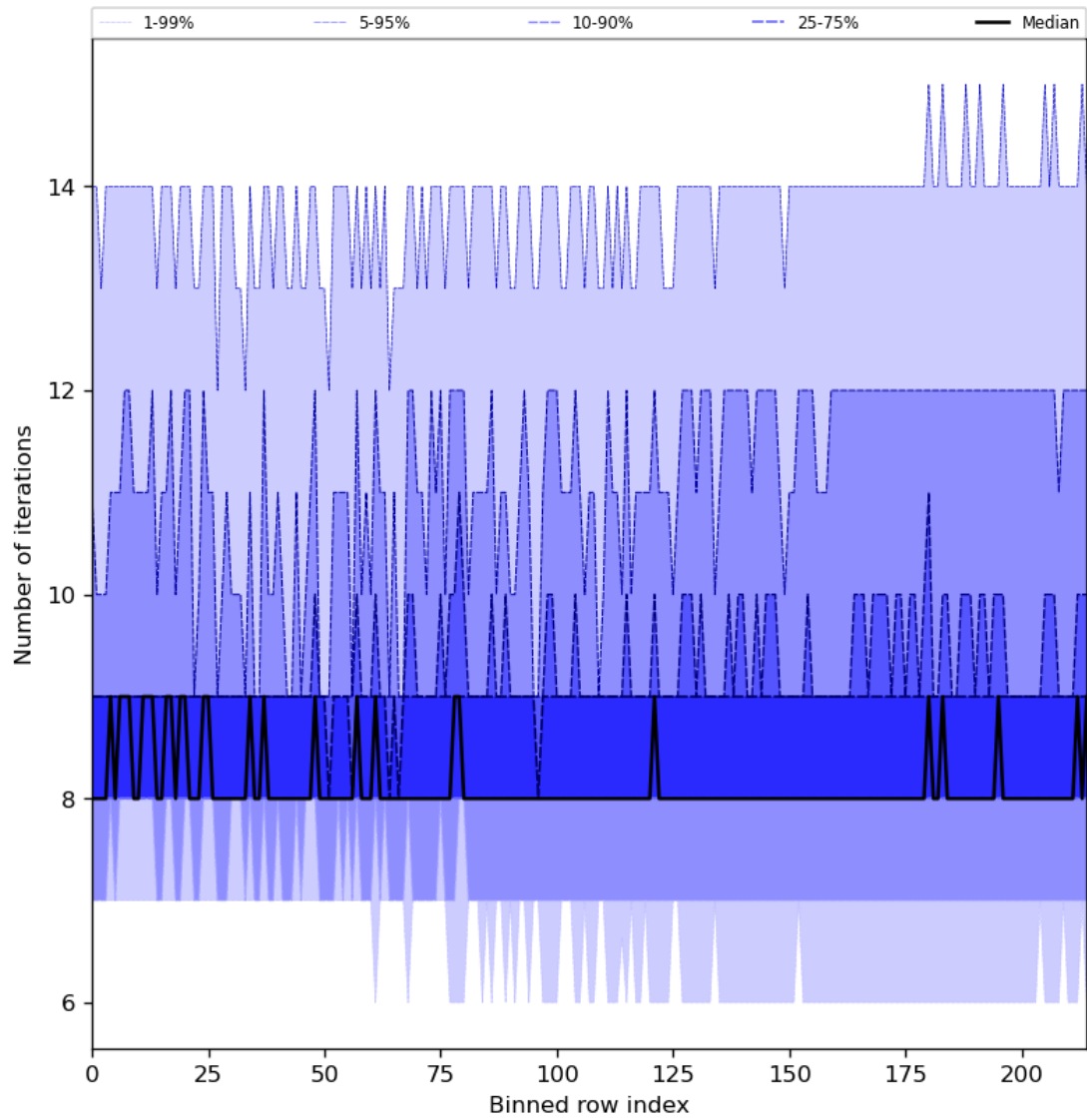
Figure 32: Along track statistics of “Number of iterations” for 2023-12-09 to 2023-12-10
