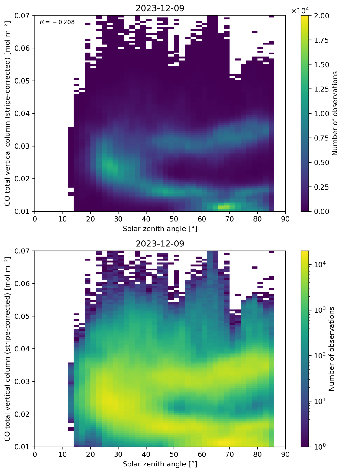
Figure 62: Scatter density plot of “Solar zenith angle” against “CO total vertical column (stripe-corrected)” for 2023-12-09 to 2023-12-10.
