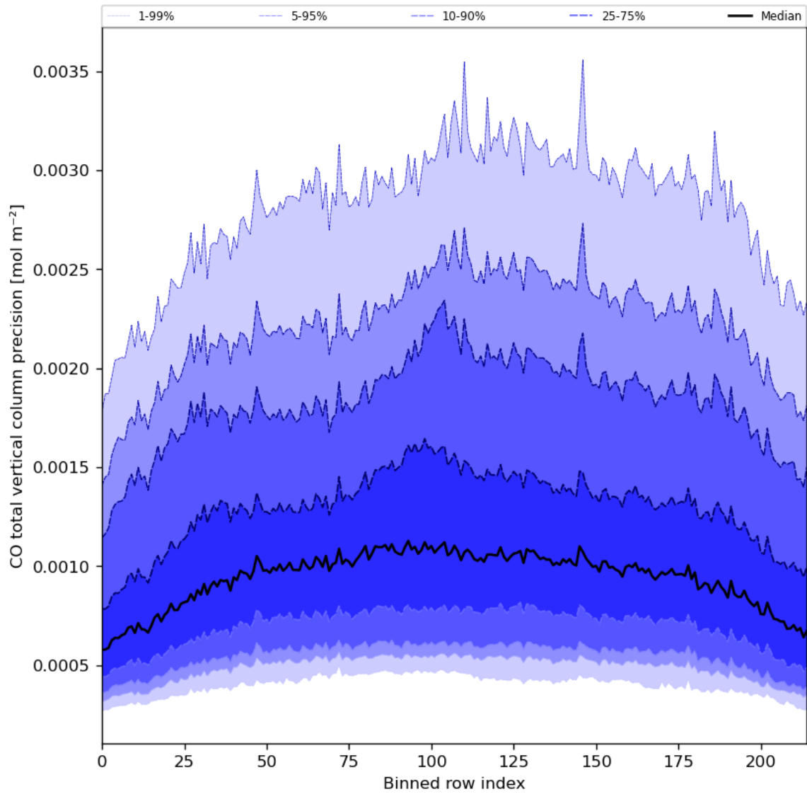
Figure 28: Along track statistics of “CO total vertical column precision” for 2023-12-09 to 2023-12-10
