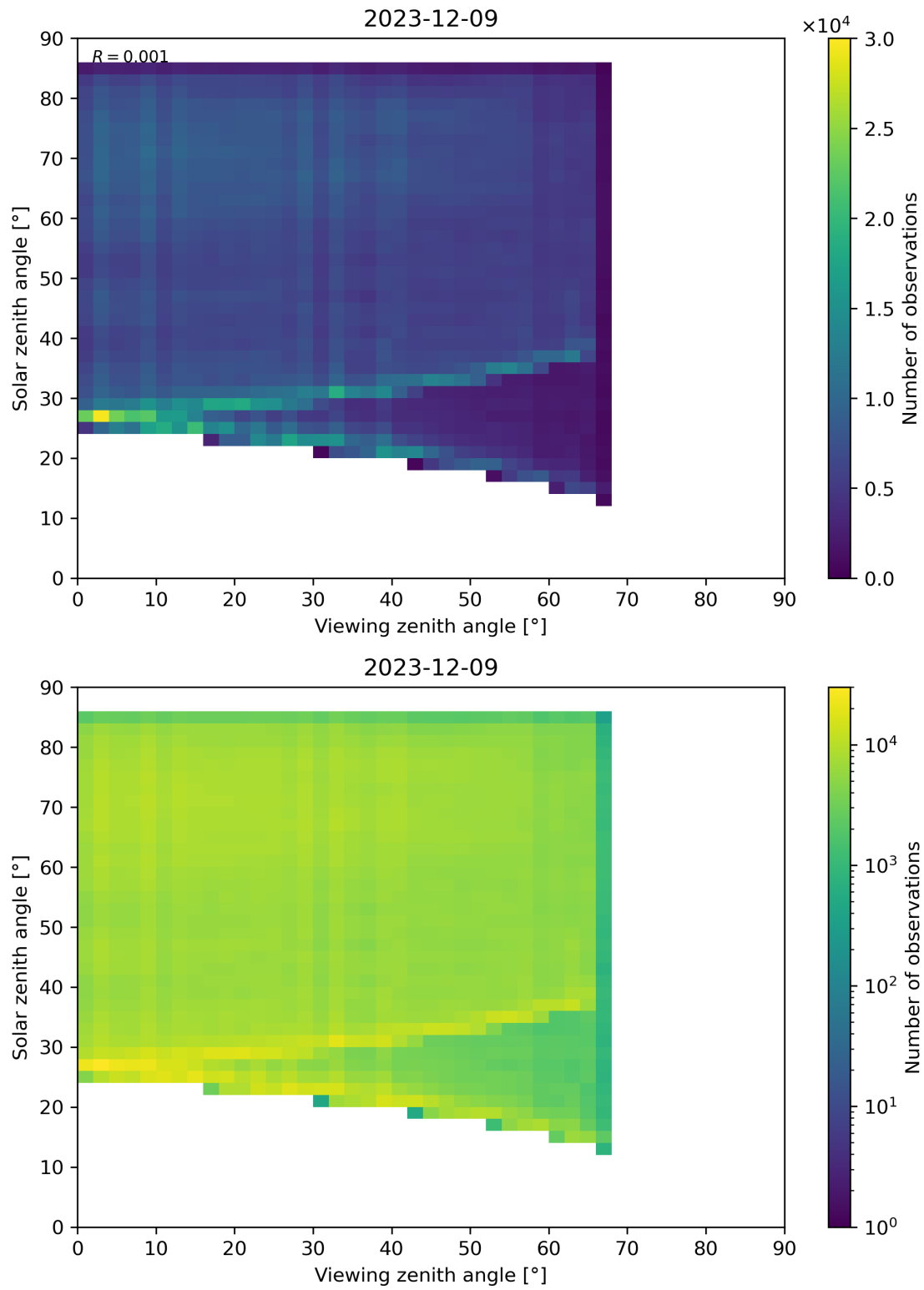
Figure 77: Scatter density plot of “Viewing zenith angle” against “Solar zenith angle” for 2023-12-09 to 2023-12-10.
