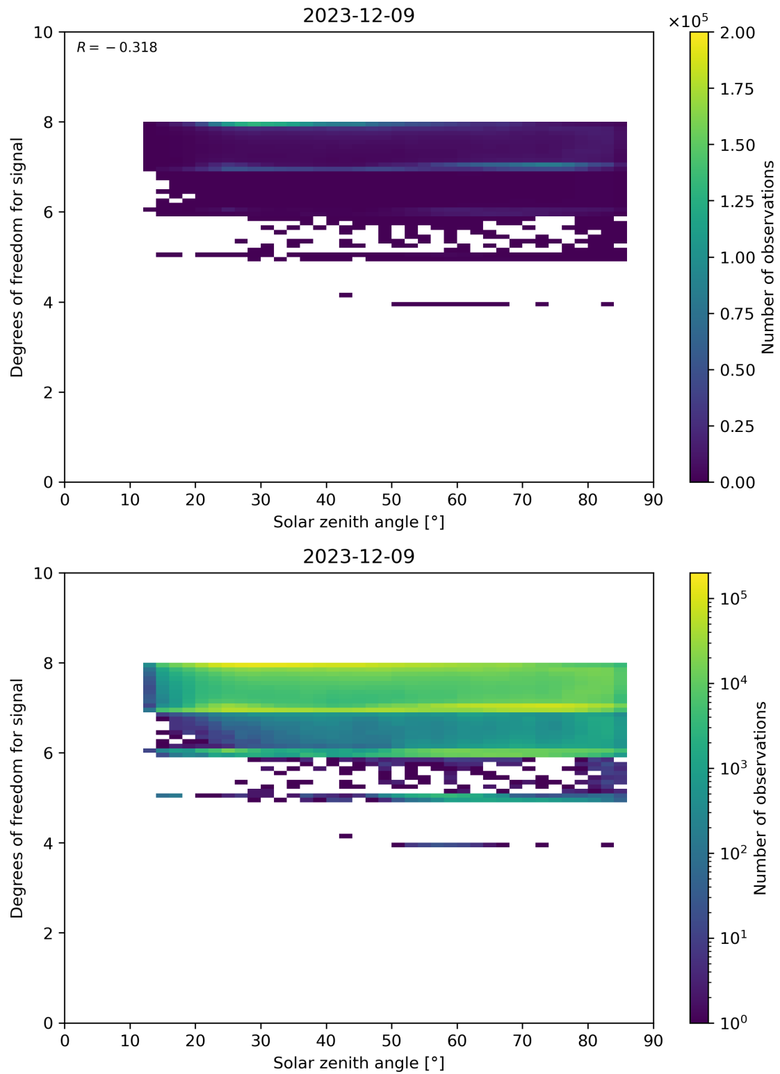
Figure 65: Scatter density plot of “Solar zenith angle” against “Degrees of freedom for signal” for 2023-12-09 to 2023-12-10.
