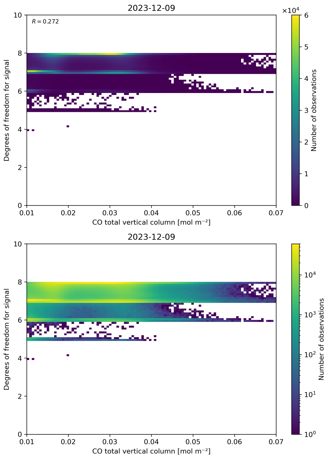
Figure 41: Scatter density plot of “CO total vertical column” against “Degrees of freedom for signal” for 2023-12-09 to 2023-12-10.
