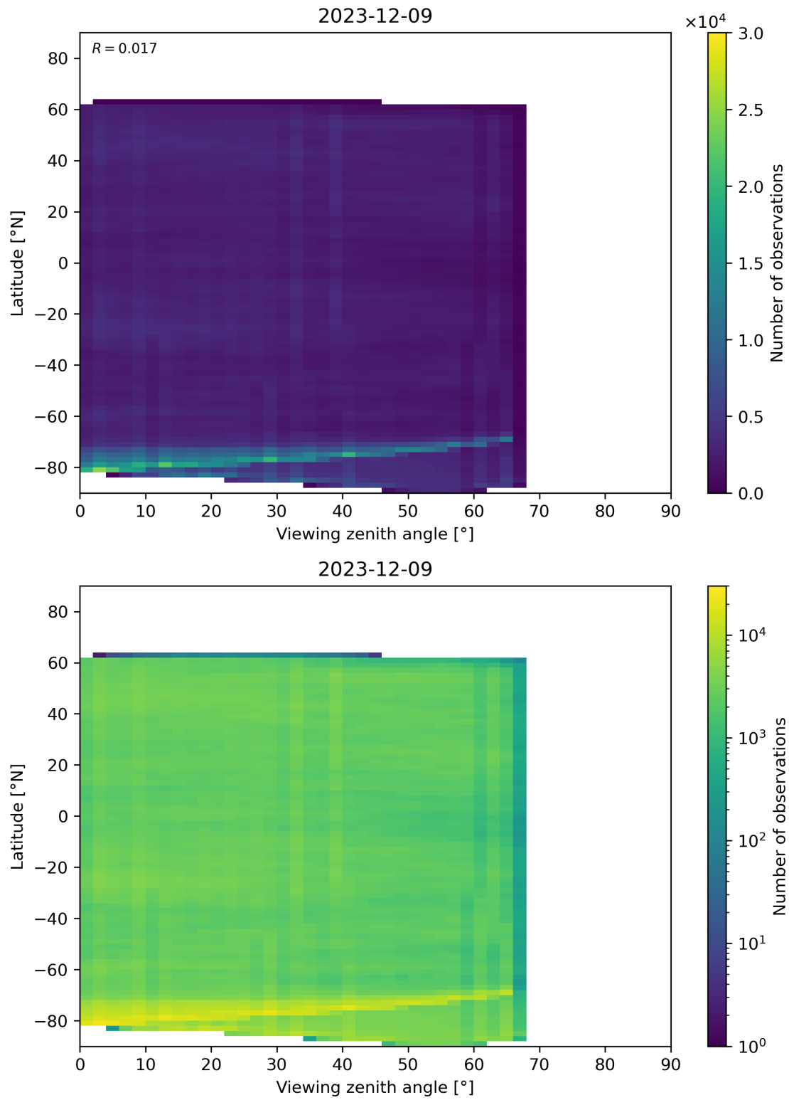
Figure 74: Scatter density plot of “Viewing zenith angle” against “Latitude” for 2023-12-09 to 2023-12-10.
