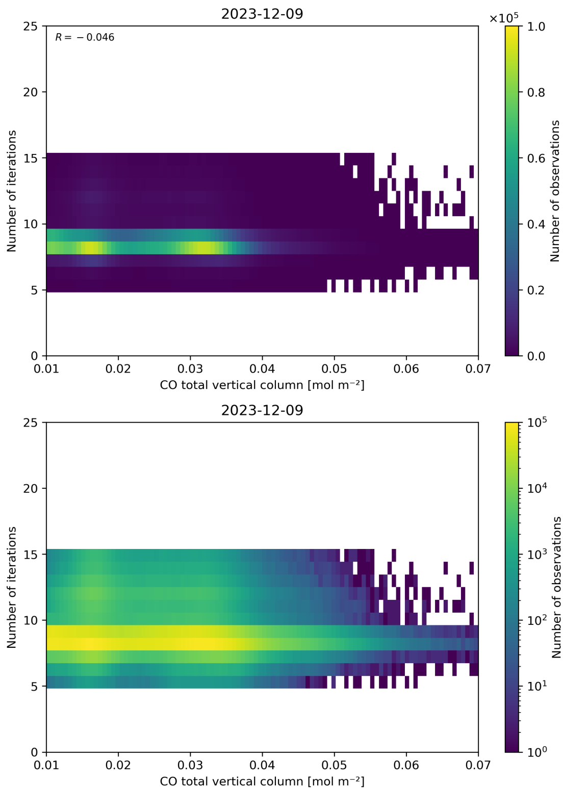
Figure 42: Scatter density plot of “CO total vertical column” against “Number of iterations” for 2023-12-09 to 2023-12-10.
