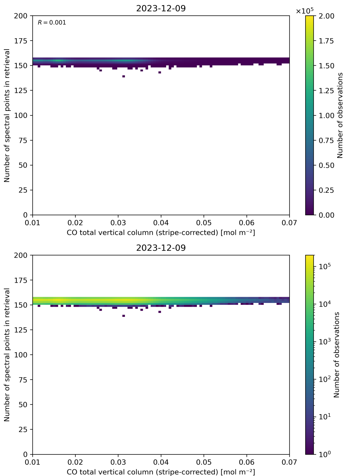
Figure 40: Scatter density plot of “CO total vertical column (stripe-corrected)” against “Number of spectral points in retrieval” for 2023-12-09 to 2023-12-10.
