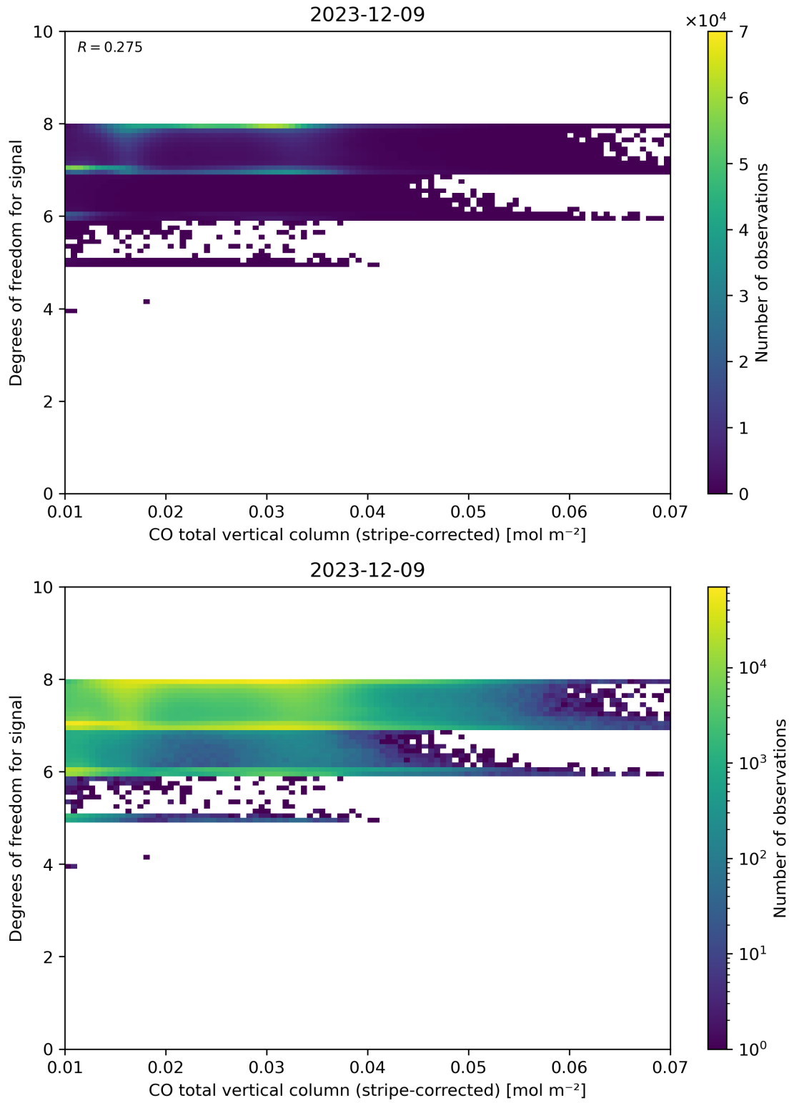
Figure 38: Scatter density plot of “CO total vertical column (stripe-corrected)” against “Degrees of freedom for signal” for 2023-12-09 to 2023-12-10.
