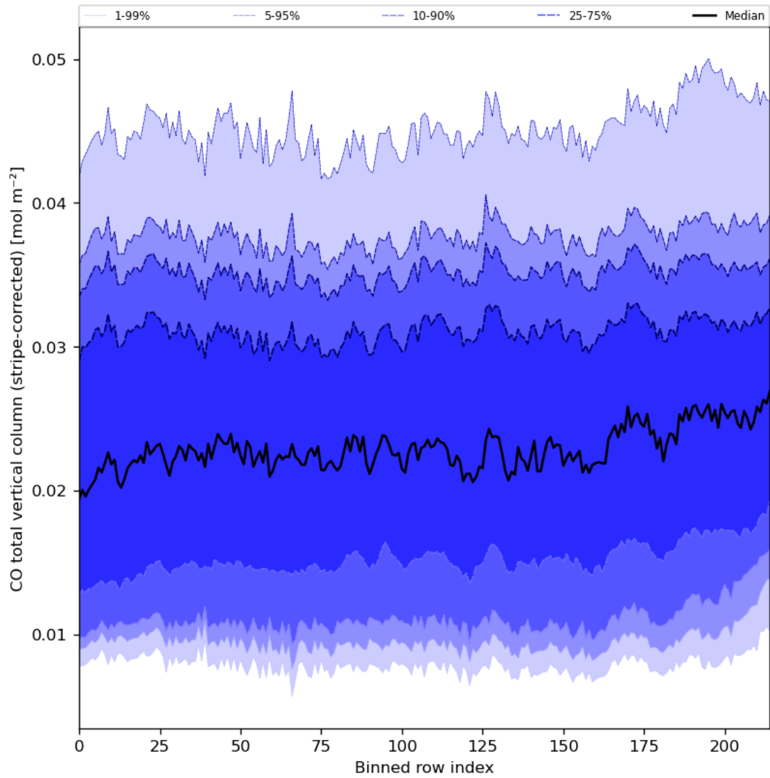
Figure 27: Along track statistics of “CO total vertical column (stripe-corrected)” for 2023-12-09 to 2023-12-10
