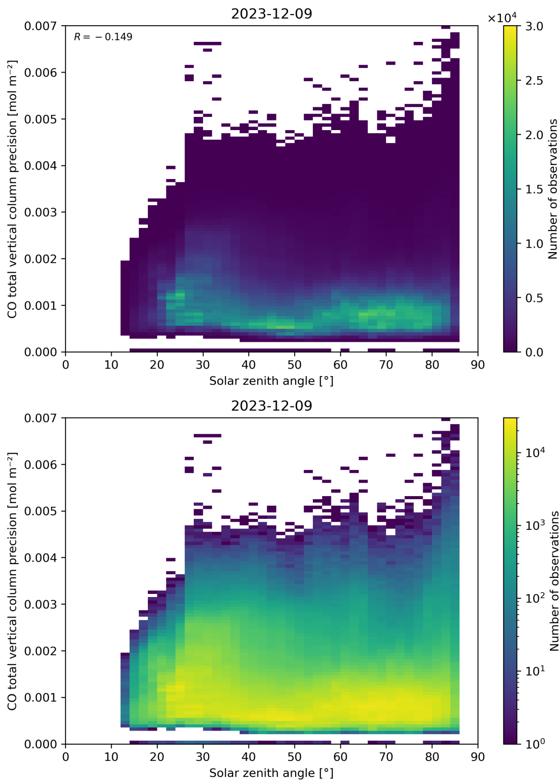
Figure 63: Scatter density plot of “Solar zenith angle” against “CO total vertical column precision” for 2023-12-09 to 2023-12-10.
