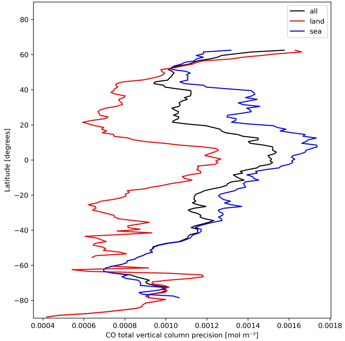
Figure 12: Zonal average of “CO total vertical column precision” for 2023-12-09 to 2023-12-10.
