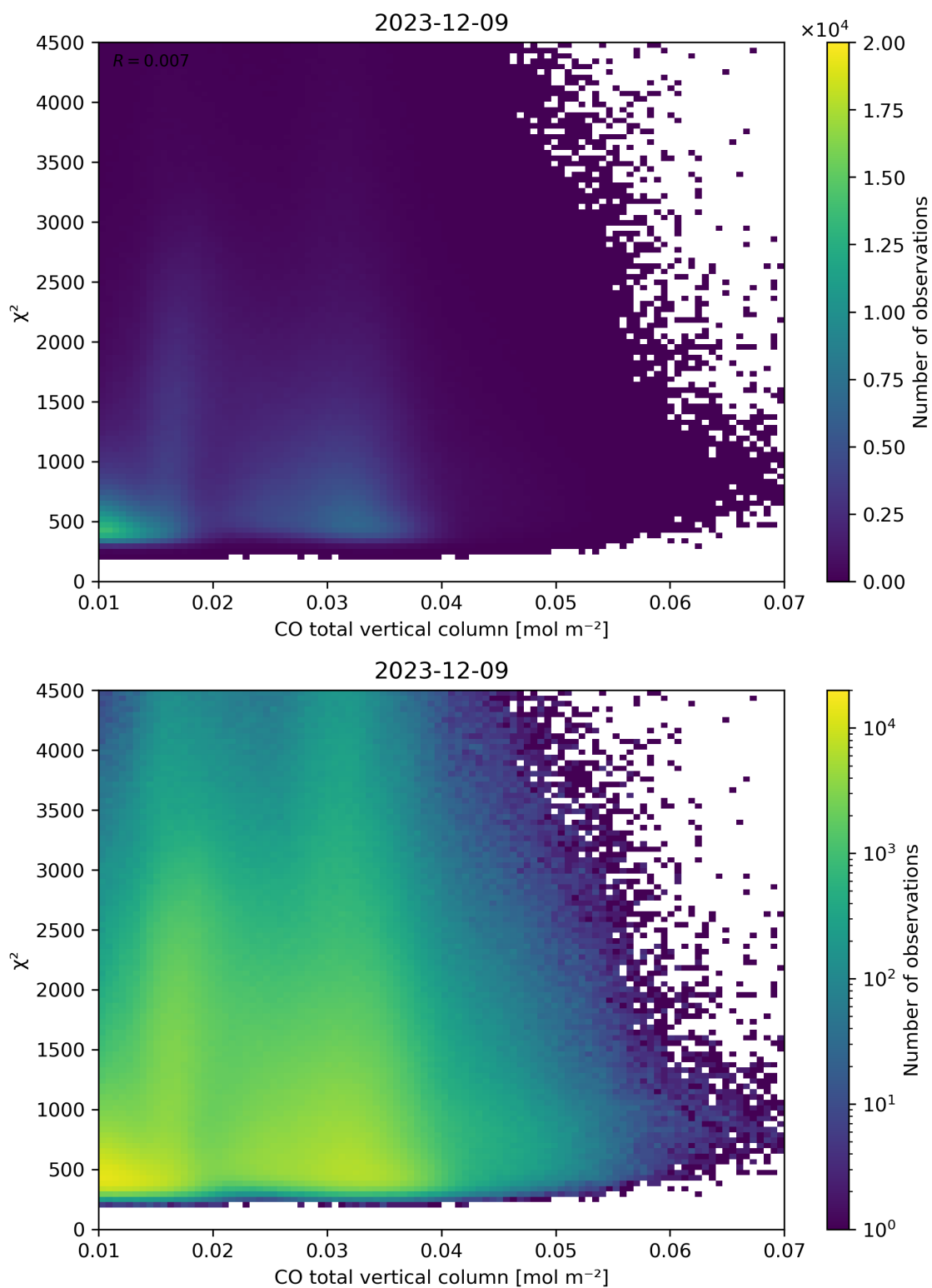
Figure 35: Scatter density plot of “CO total vertical column” against “ \chi^2 ” for 2023-12-09 to 2023-12-10.
