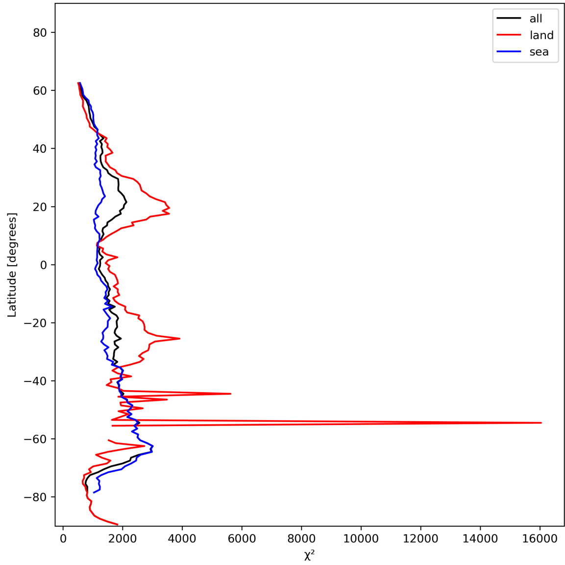
Figure 14: Zonal average of “ \chi^2 ” for 2023-12-09 to 2023-12-10.
