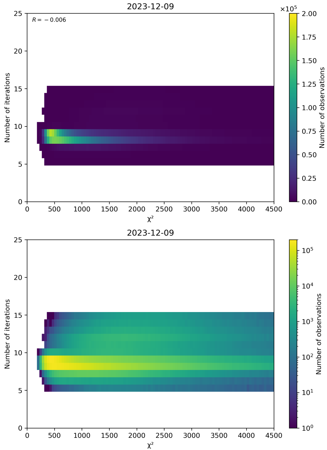
Figure 49: Scatter density plot of “ \chi^2 ” against “Number of iterations” for 2023-12-09 to 2023-12-10.
