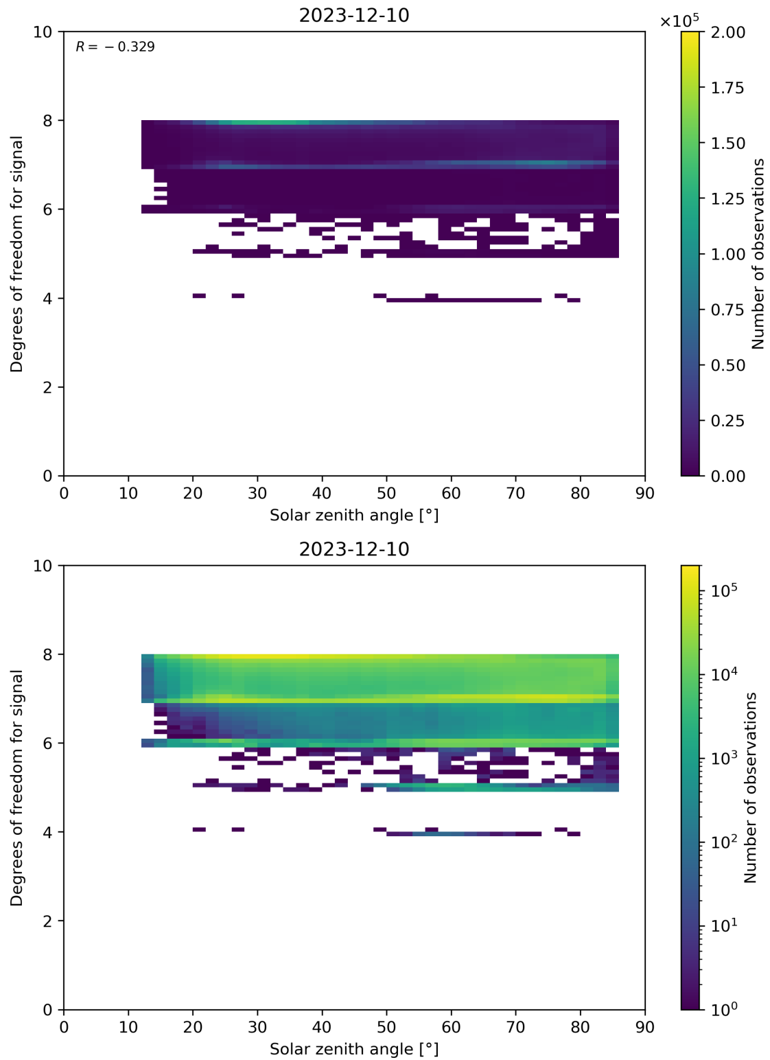
Figure 65: Scatter density plot of “Solar zenith angle” against “Degrees of freedom for signal” for 2023-12-09 to 2023-12-11.
