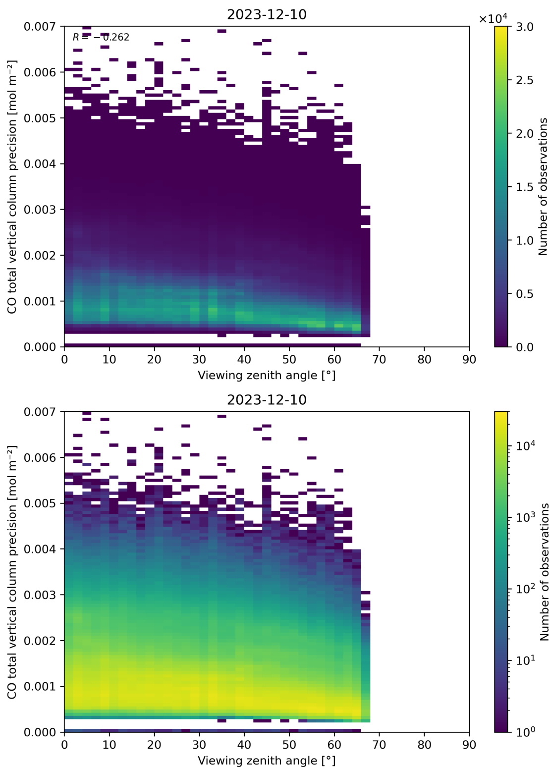
Figure 71: Scatter density plot of “Viewing zenith angle” against “CO total vertical column precision” for 2023-12-09 to 2023-12-11.
