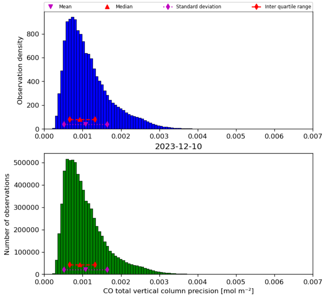
Figure 20: Histogram of “CO total vertical column precision” for 2023-12-09 to 2023-12-11
