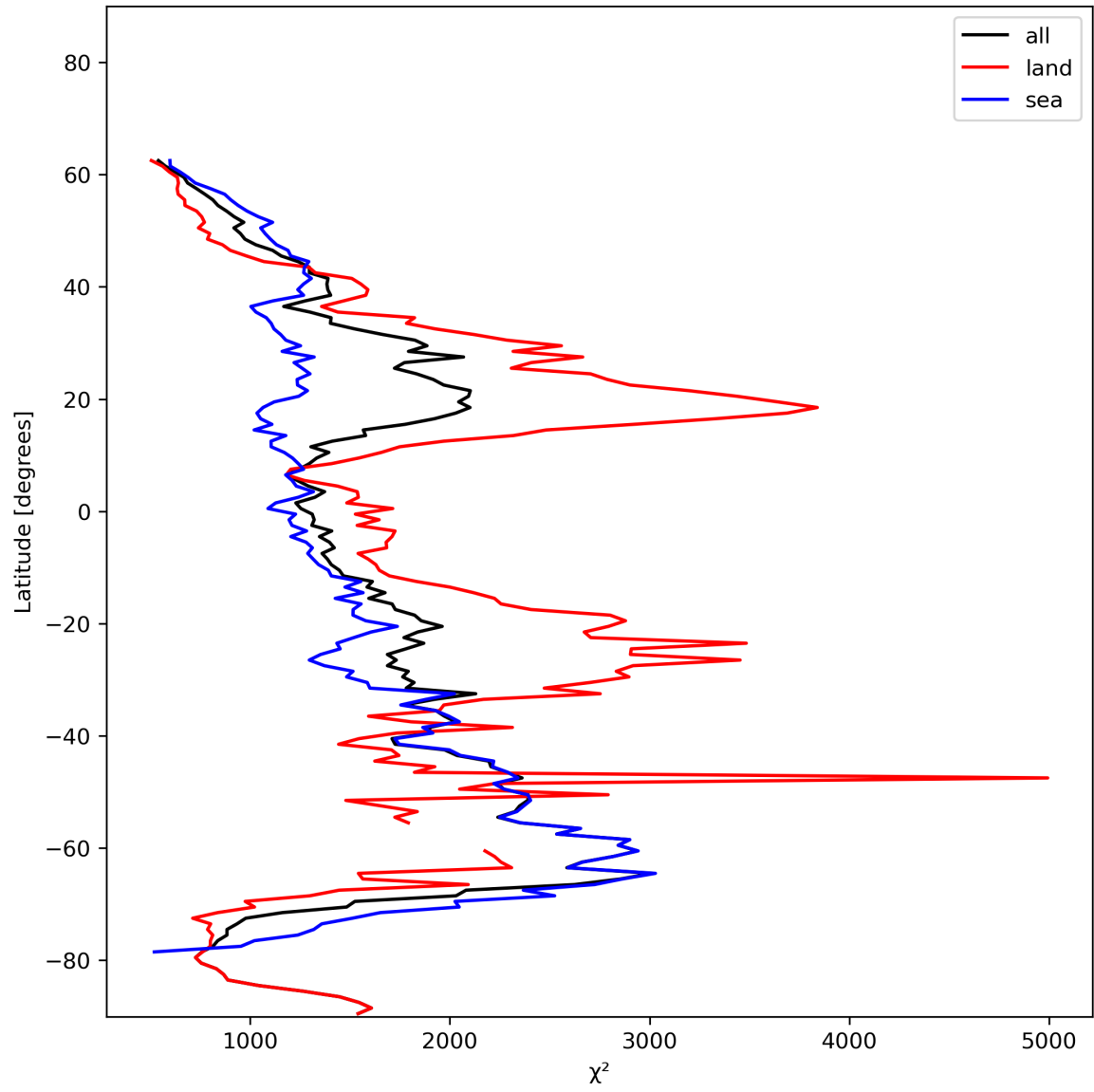
Figure 14: Zonal average of “ \chi^2 ” for 2023-12-09 to 2023-12-11.
