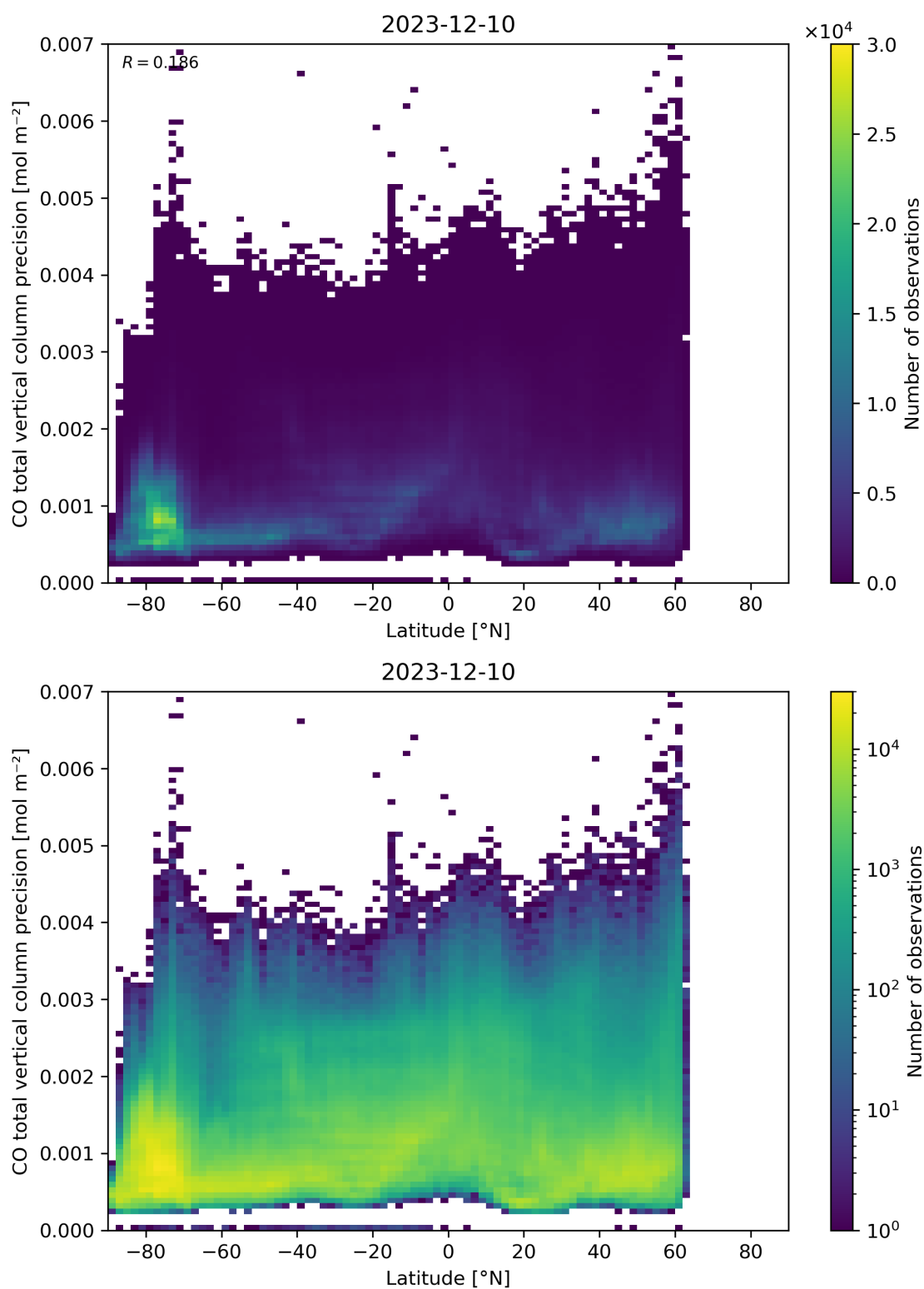
Figure 53: Scatter density plot of “Latitude” against “CO total vertical column precision” for 2023-12-09 to 2023-12-11.
