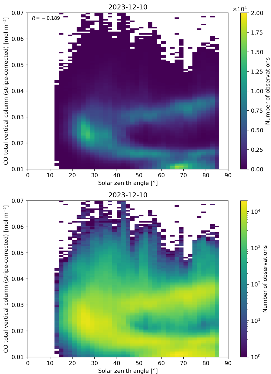
Figure 62: Scatter density plot of “Solar zenith angle” against “CO total vertical column (stripe-corrected)” for 2023-12-09 to 2023-12-11.
