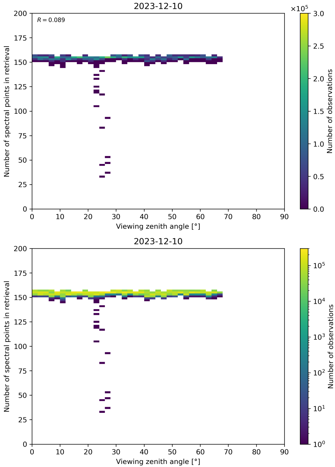
Figure 76: Scatter density plot of “Viewing zenith angle” against “Number of spectral points in retrieval” for 2023-12-09 to 2023-12-11.
