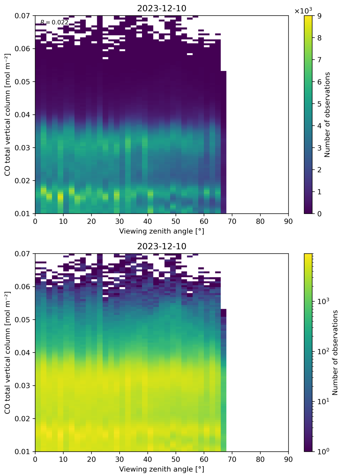
Figure 69: Scatter density plot of “Viewing zenith angle” against “CO total vertical column” for 2023-12-09 to 2023-12-11.
