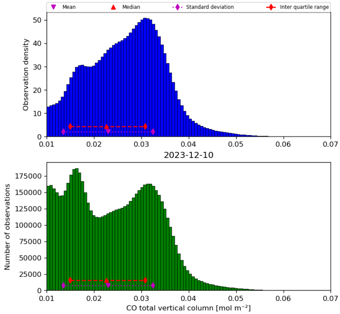
Figure 18: Histogram of “CO total vertical column” for 2023-12-09 to 2023-12-11
