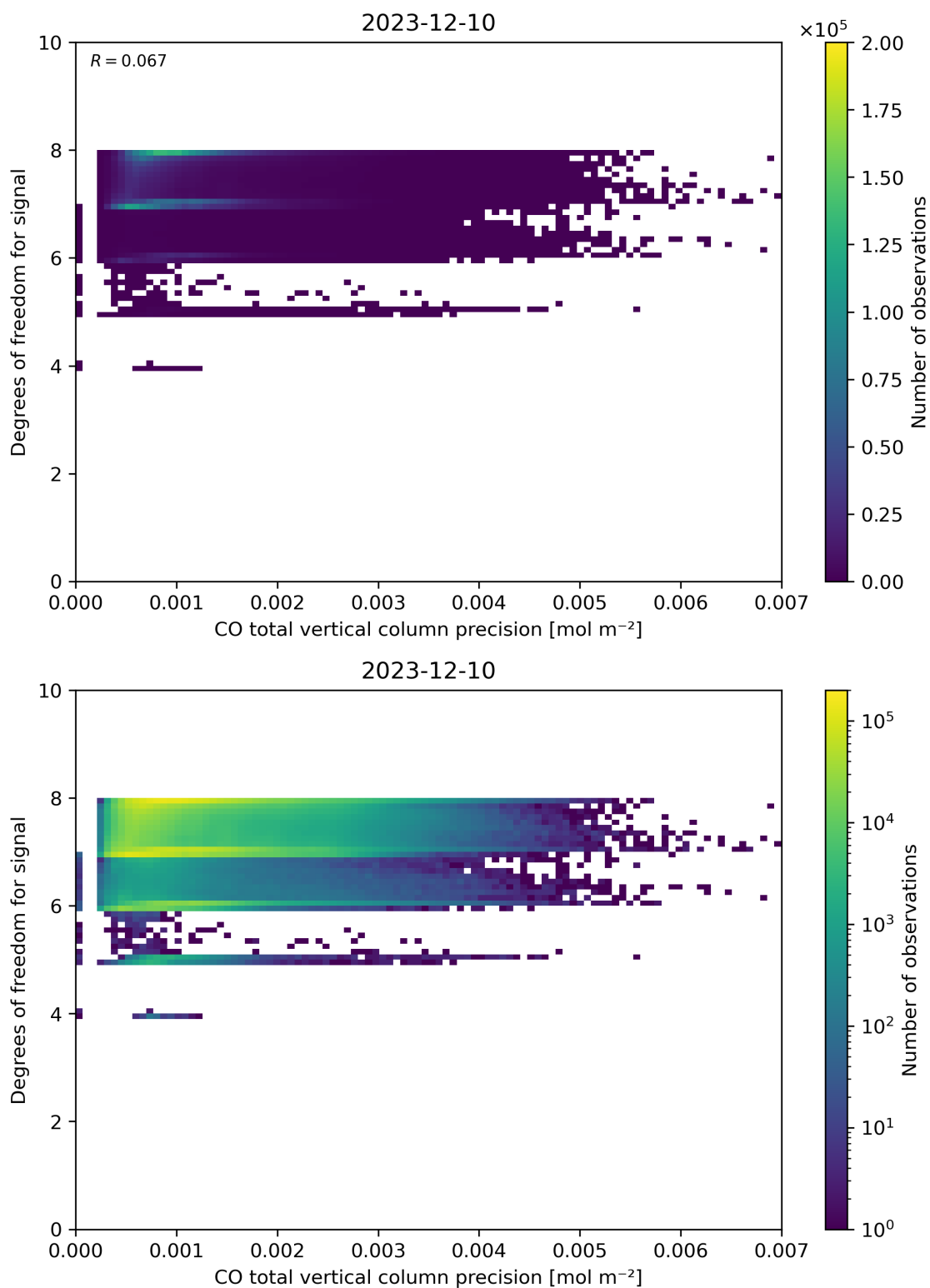
Figure 45: Scatter density plot of “CO total vertical column precision” against “Degrees of freedom for signal” for 2023-12-09 to 2023-12-11.
