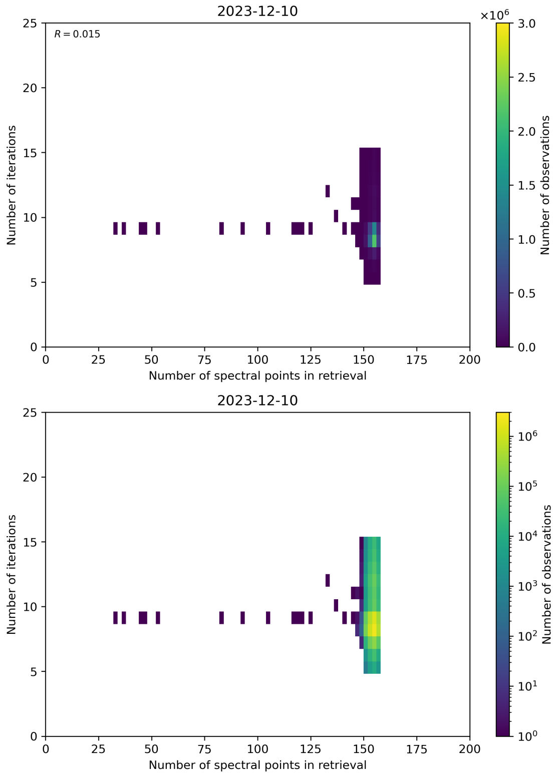
Figure 60: Scatter density plot of “Number of spectral points in retrieval” against “Number of iterations” for 2023-12-09 to 2023-12-11.
