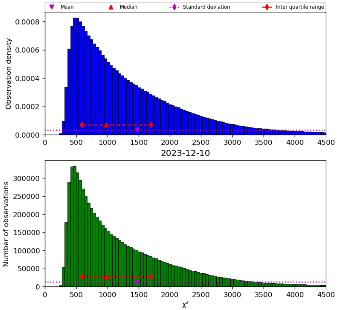
Figure 22: Histogram of “ \chi^2 ” for 2023-12-09 to 2023-12-11
