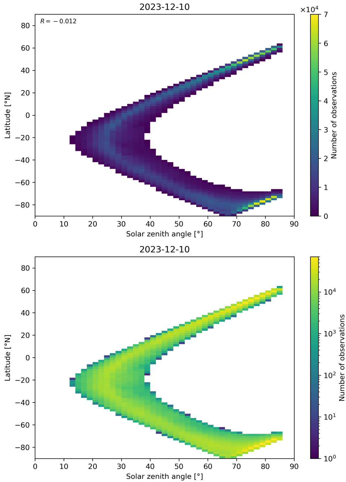
Figure 66: Scatter density plot of “Solar zenith angle” against “Latitude” for 2023-12-09 to 2023-12-11.
