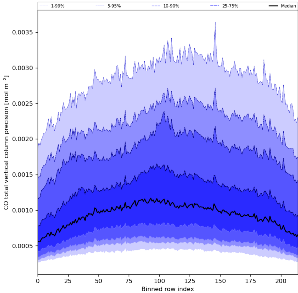
Figure 28: Along track statistics of “CO total vertical column precision” for 2023-12-09 to 2023-12-11
