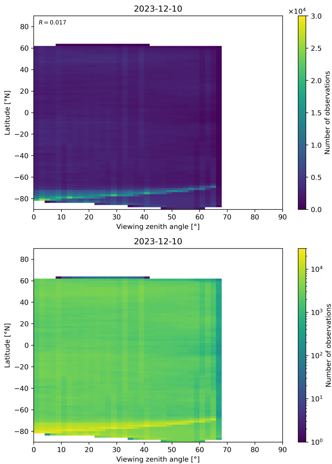
Figure 74: Scatter density plot of “Viewing zenith angle” against “Latitude” for 2023-12-09 to 2023-12-11.
