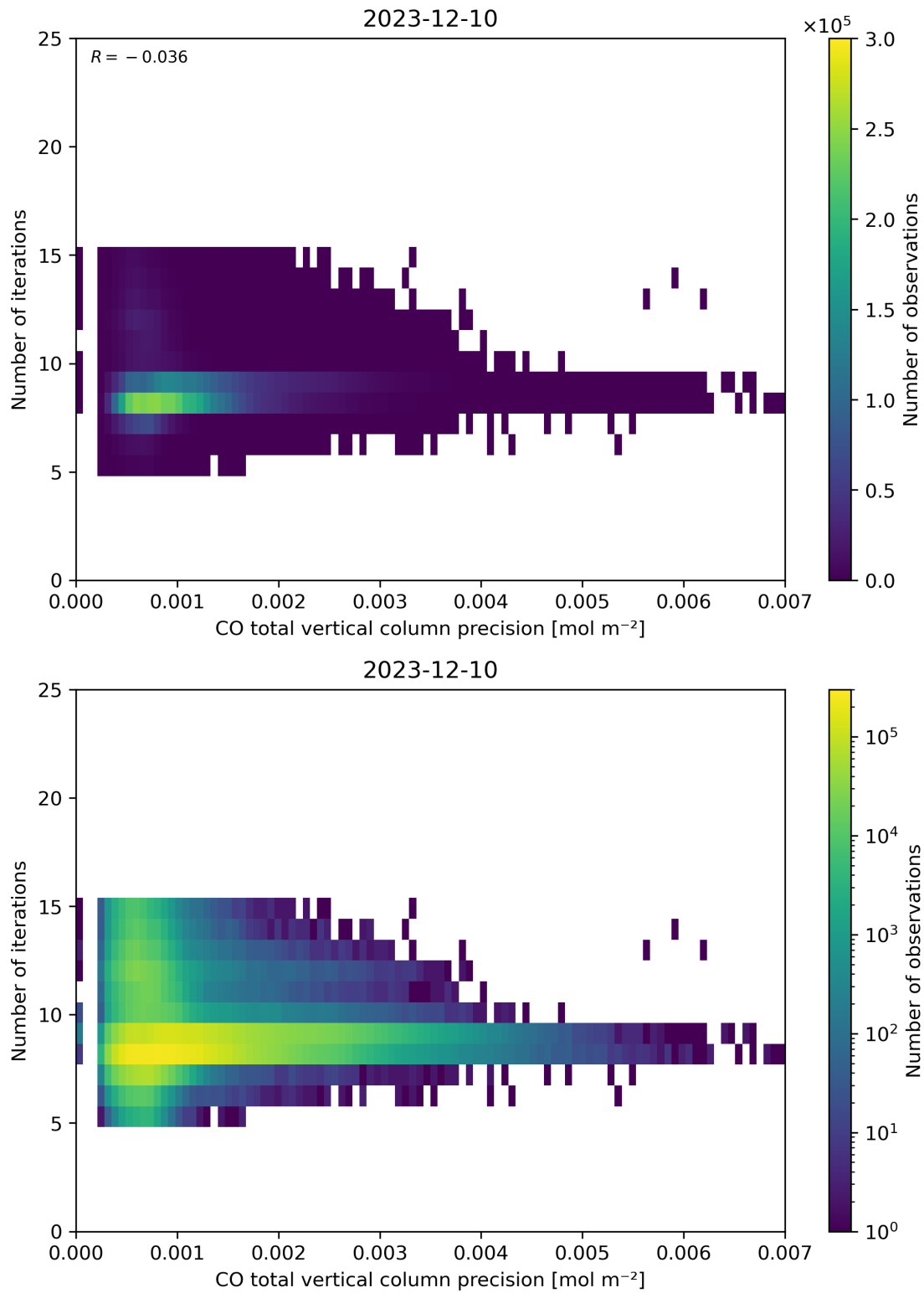
Figure 46: Scatter density plot of “CO total vertical column precision” against “Number of iterations” for 2023-12-09 to 2023-12-11.
