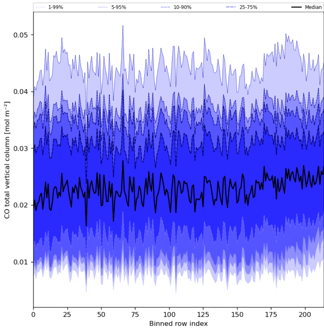
Figure 26: Along track statistics of “CO total vertical column” for 2023-12-09 to 2023-12-11
