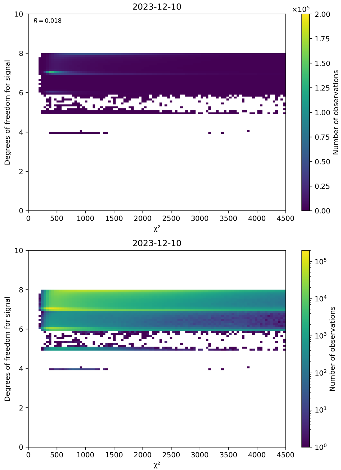
Figure 48: Scatter density plot of “ \chi^2 ” against “Degrees of freedom for signal” for 2023-12-09 to 2023-12-11.
