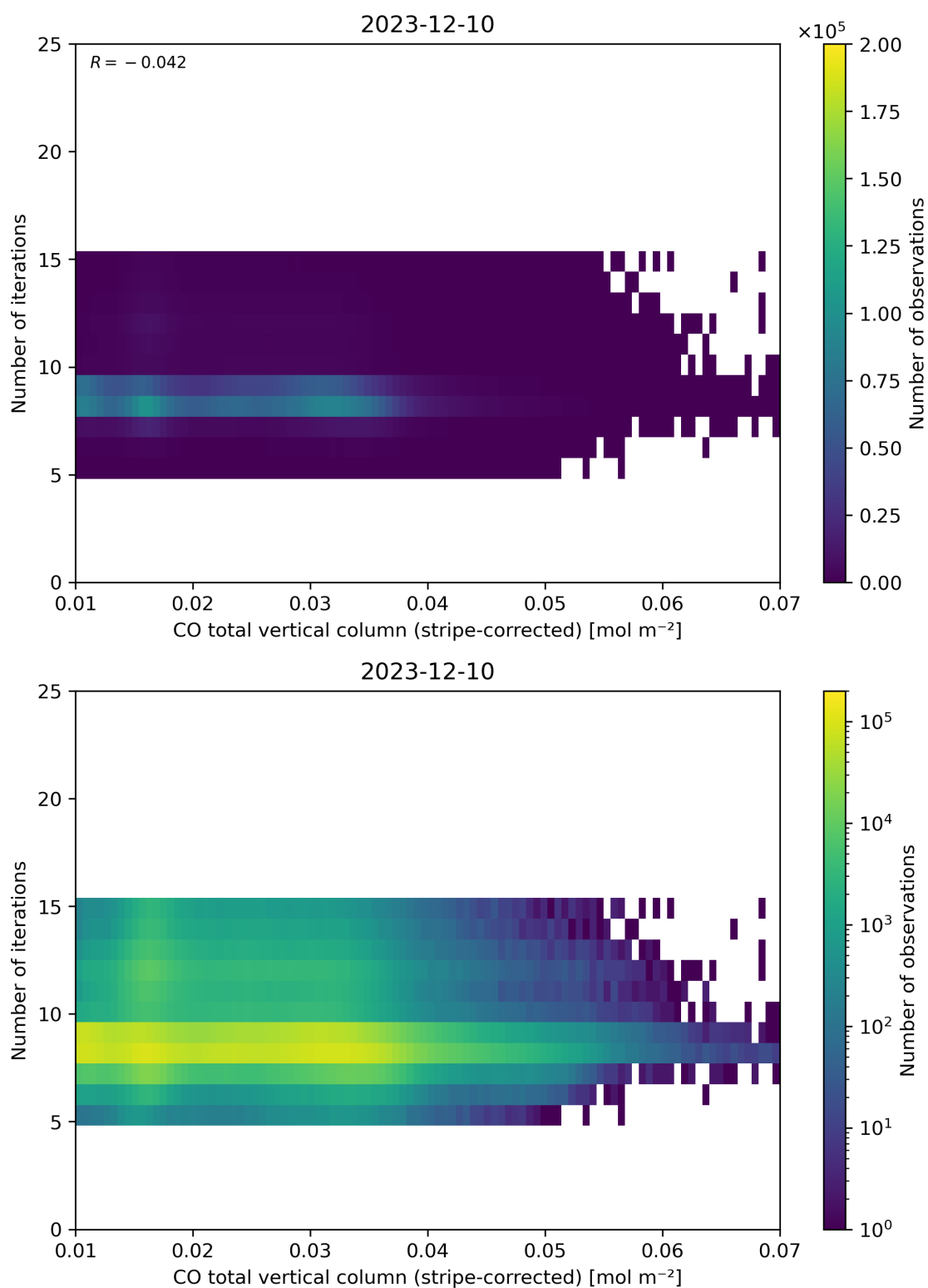
Figure 39: Scatter density plot of “CO total vertical column (stripe-corrected)” against “Number of iterations” for 2023-12-09 to 2023-12-11.
