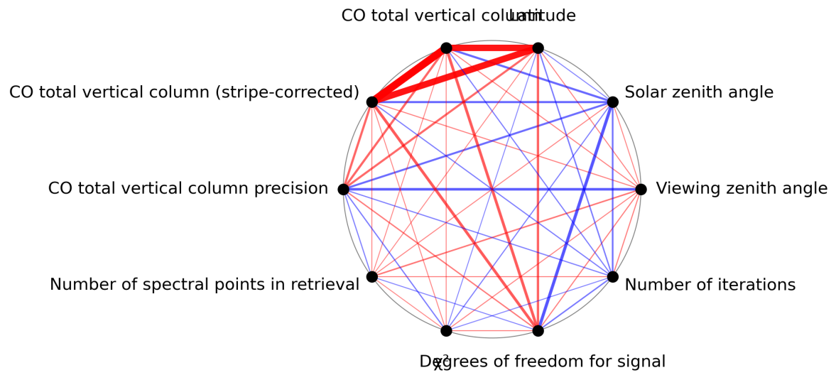
Figure 1: Map of correlation graph for 2023-12-09 to 2023-12-11.
