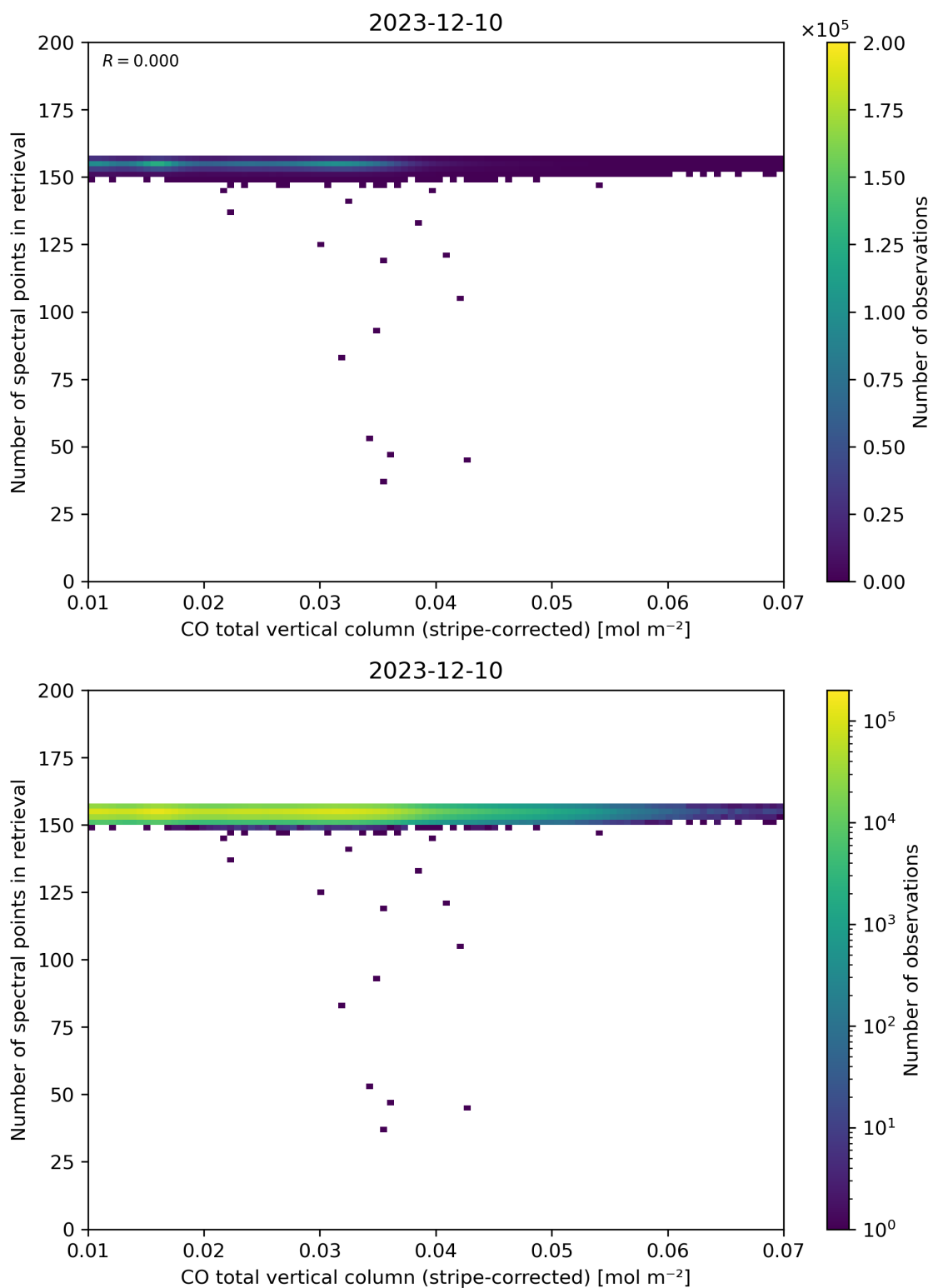
Figure 40: Scatter density plot of “CO total vertical column (stripe-corrected)” against “Number of spectral points in retrieval” for 2023-12-09 to 2023-12-11.
