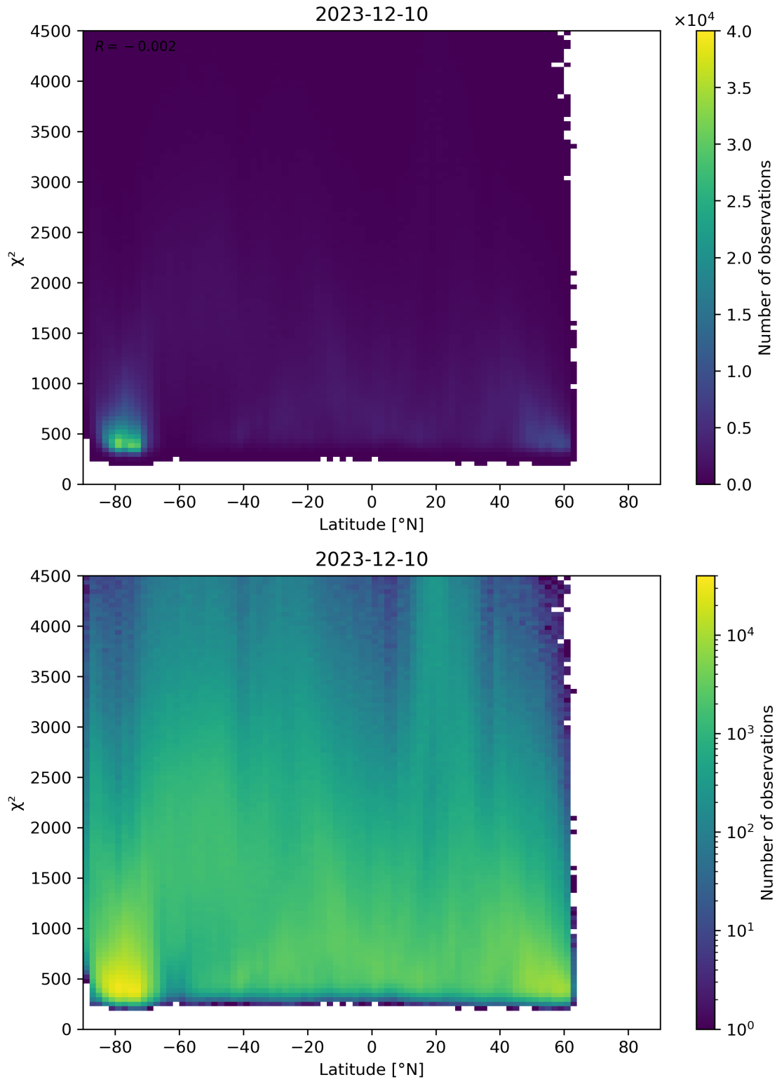
Figure 54: Scatter density plot of “Latitude” against “ \chi^2 ” for 2023-12-09 to 2023-12-11.
