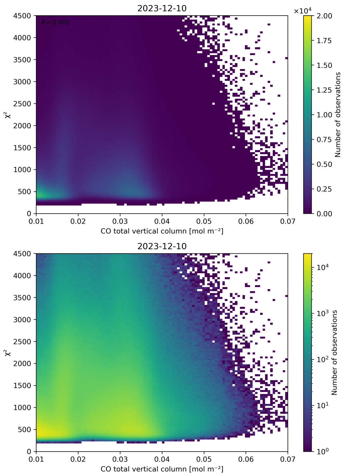
Figure 35: Scatter density plot of “CO total vertical column” against “ \chi^2 ” for 2023-12-09 to 2023-12-11.
