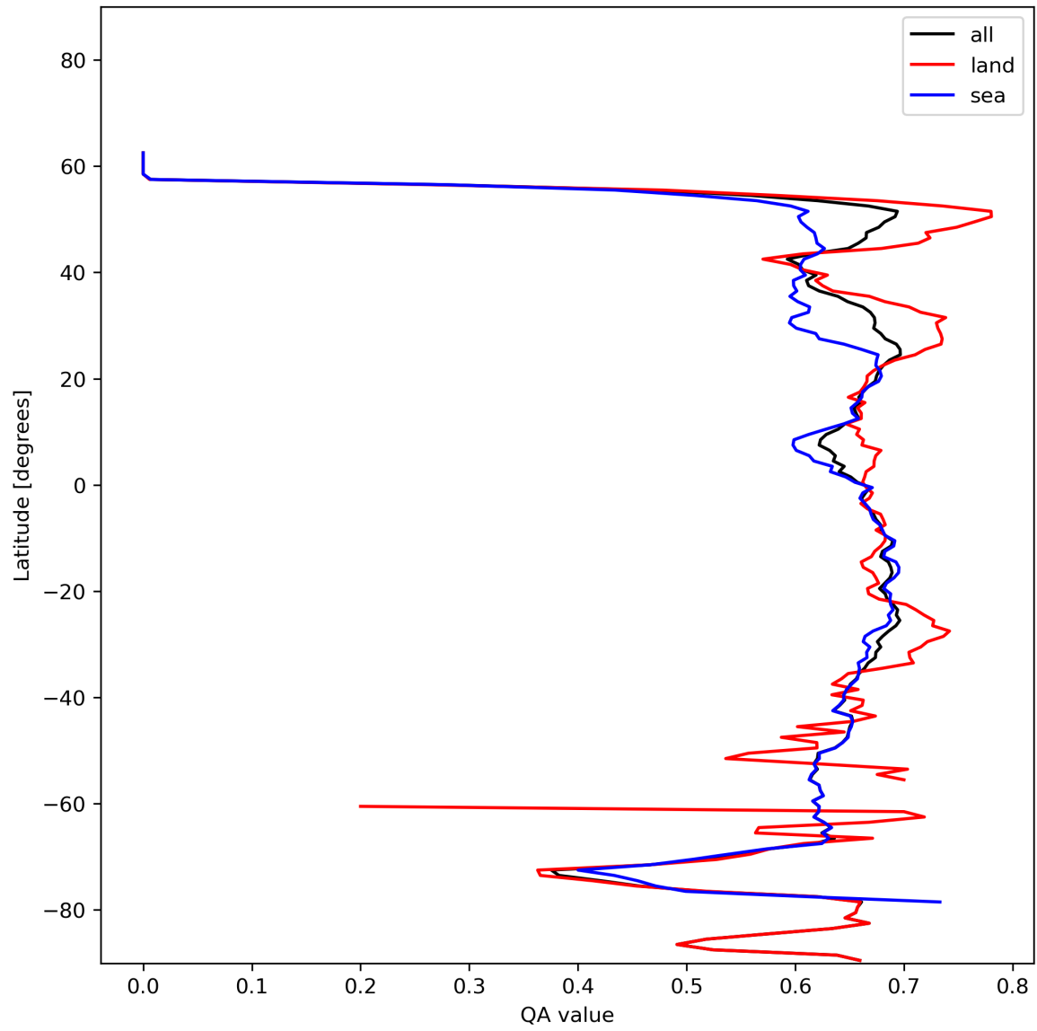
Figure 9: Zonal average of “QA value” for 2023-12-09 to 2023-12-11.
