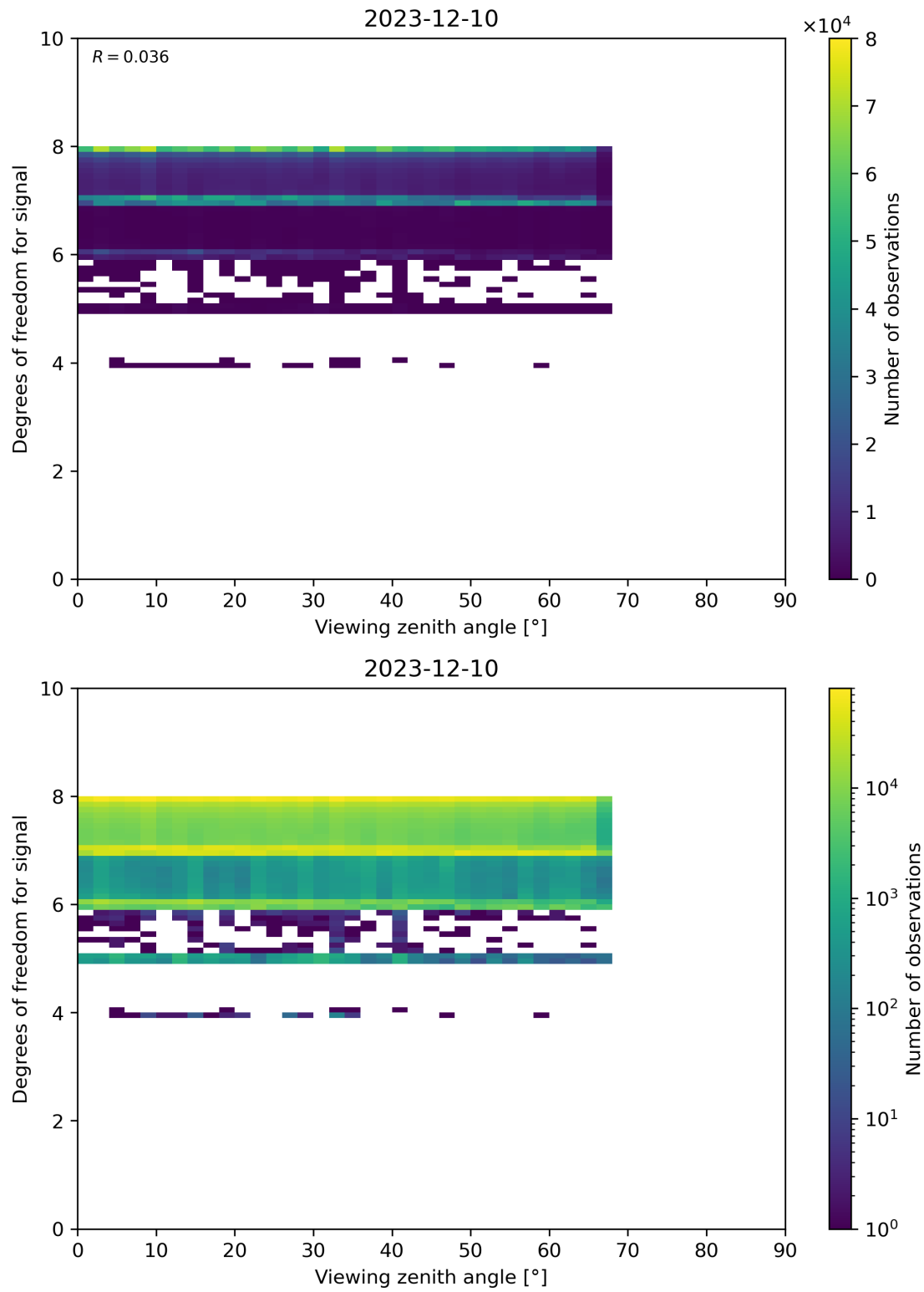
Figure 73: Scatter density plot of “Viewing zenith angle” against “Degrees of freedom for signal” for 2023-12-09 to 2023-12-11.
