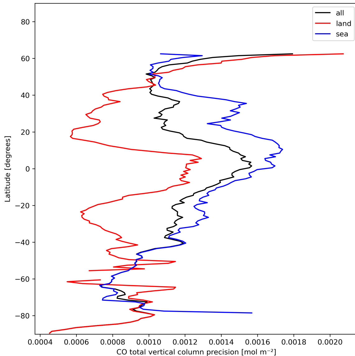
Figure 12: Zonal average of “CO total vertical column precision” for 2023-12-09 to 2023-12-11.
