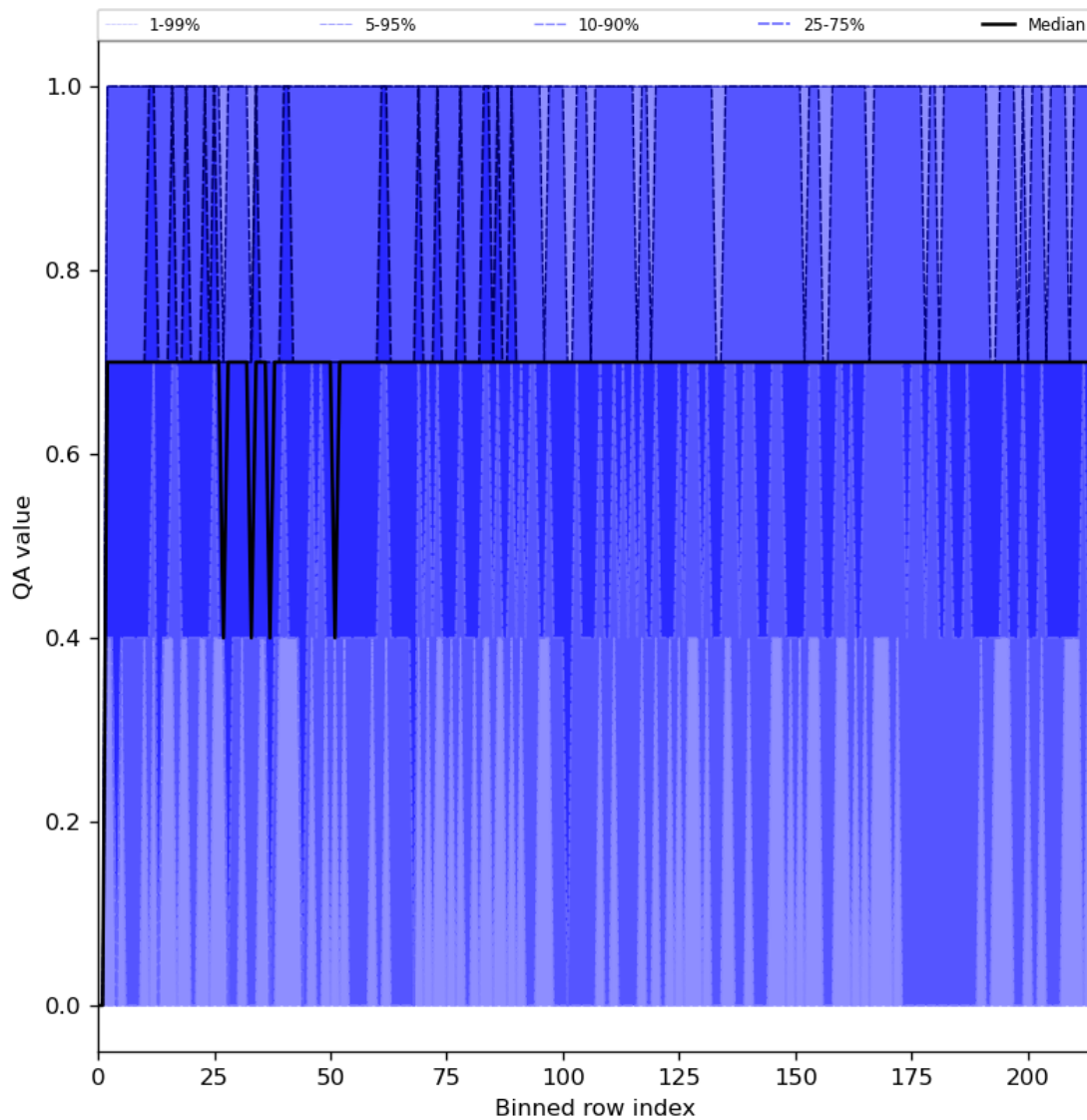
Figure 25: Along track statistics of “QA value” for 2023-12-09 to 2023-12-11
