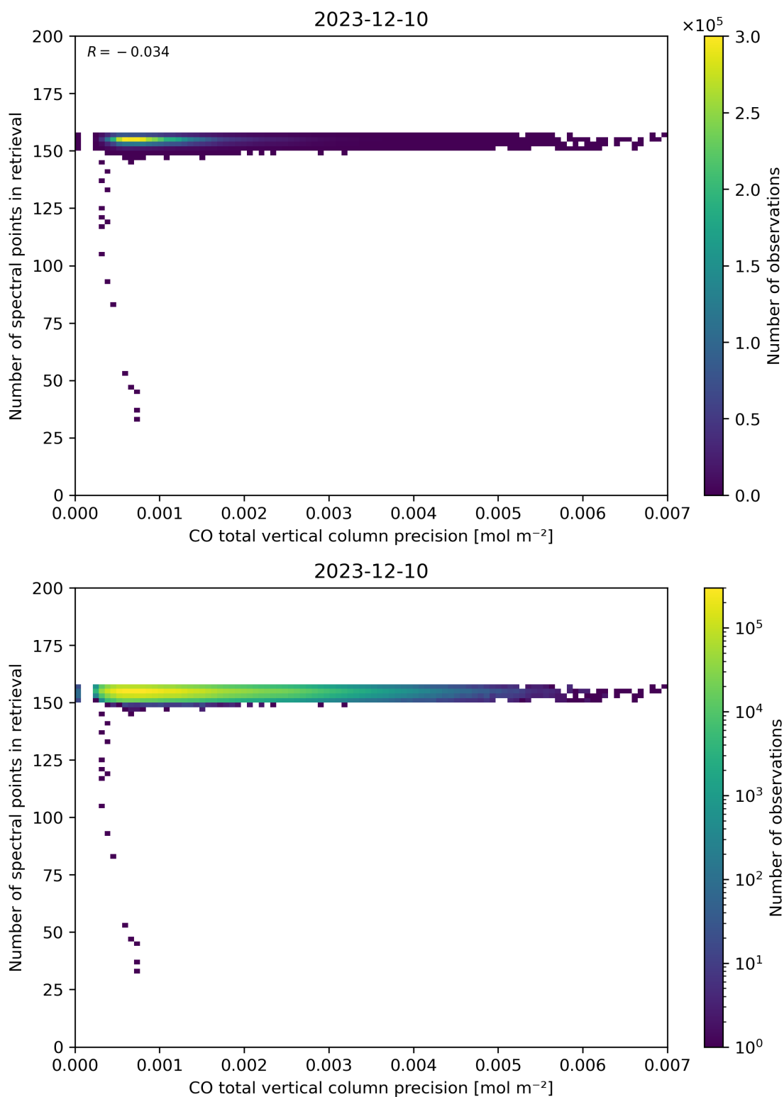
Figure 47: Scatter density plot of “CO total vertical column precision” against “Number of spectral points in retrieval” for 2023-12-09 to 2023-12-11.
