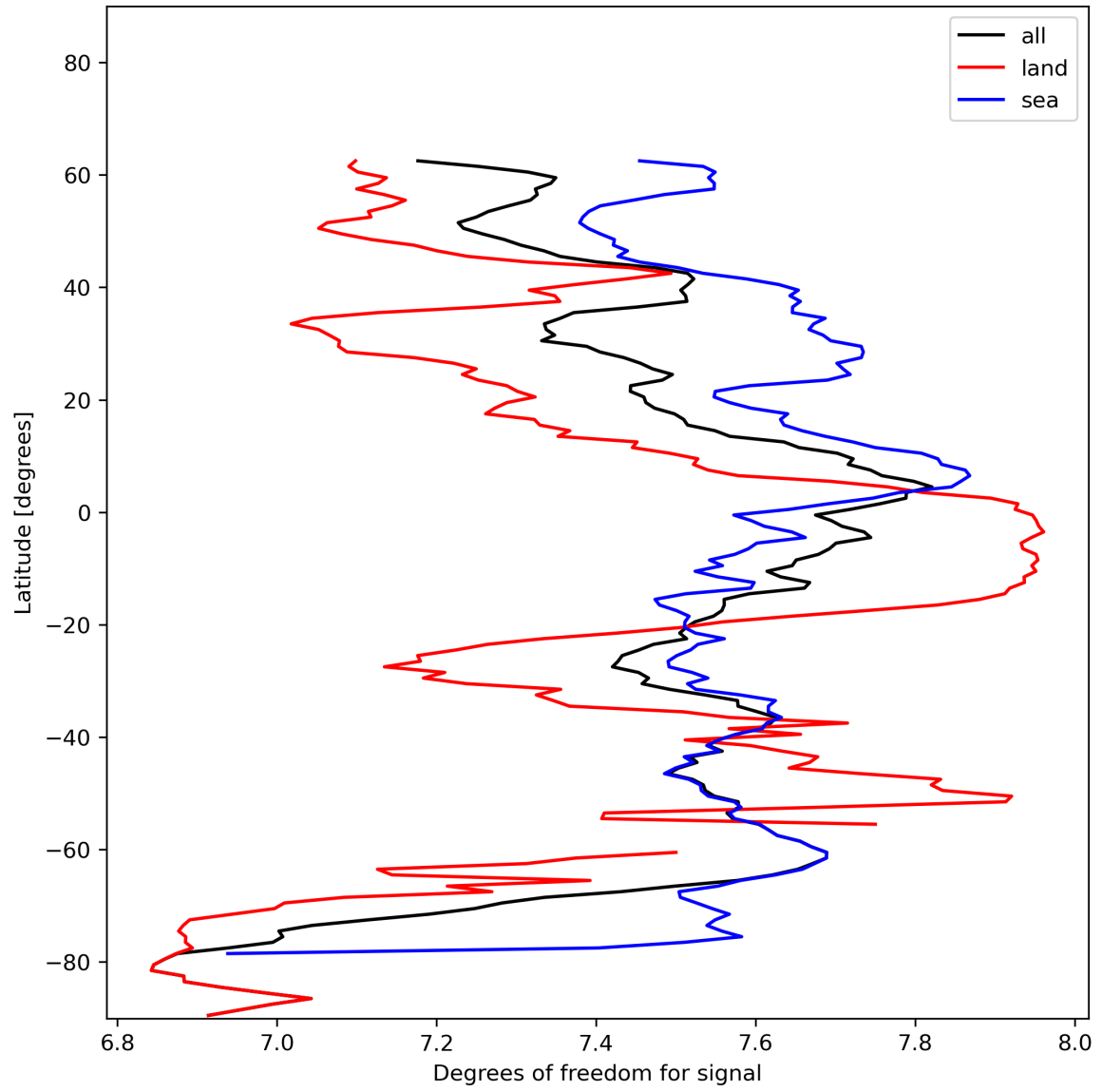
Figure 15: Zonal average of “Degrees of freedom for signal” for 2023-12-09 to 2023-12-11.
