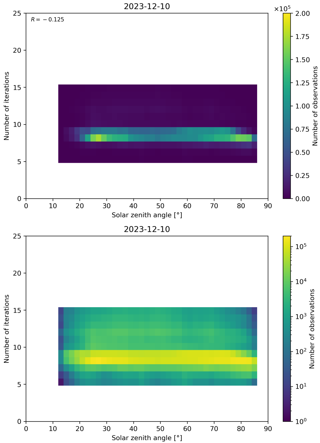
Figure 67: Scatter density plot of “Solar zenith angle” against “Number of iterations” for 2023-12-09 to 2023-12-11.
