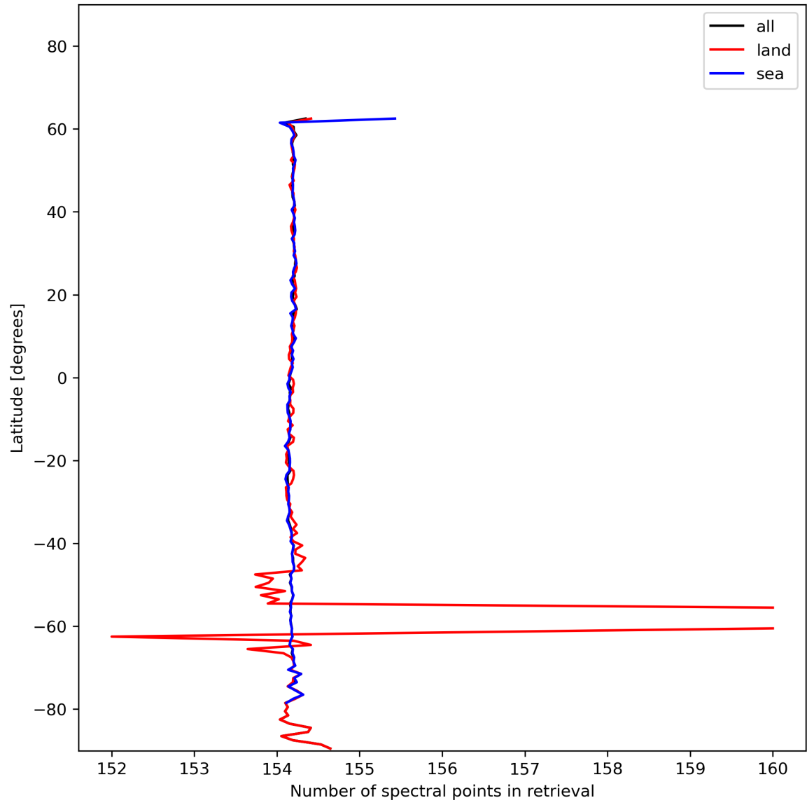
Figure 13: Zonal average of “Number of spectral points in retrieval” for 2023-12-09 to 2023-12-11.
