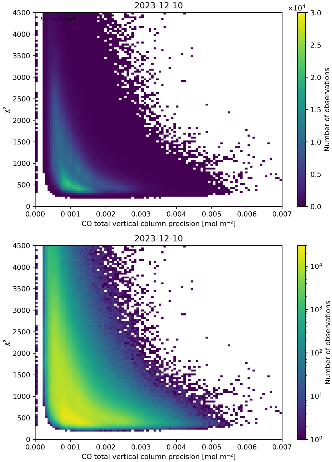
Figure 44: Scatter density plot of “CO total vertical column precision” against “ \chi^2 ” for 2023-12-09 to 2023-12-11.
