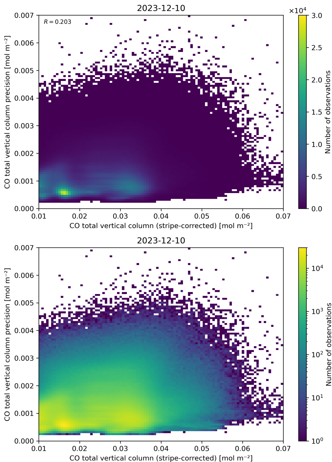
Figure 36: Scatter density plot of “CO total vertical column (stripe-corrected)” against “CO total vertical column precision” for 2023-12-09 to 2023-12-11.
