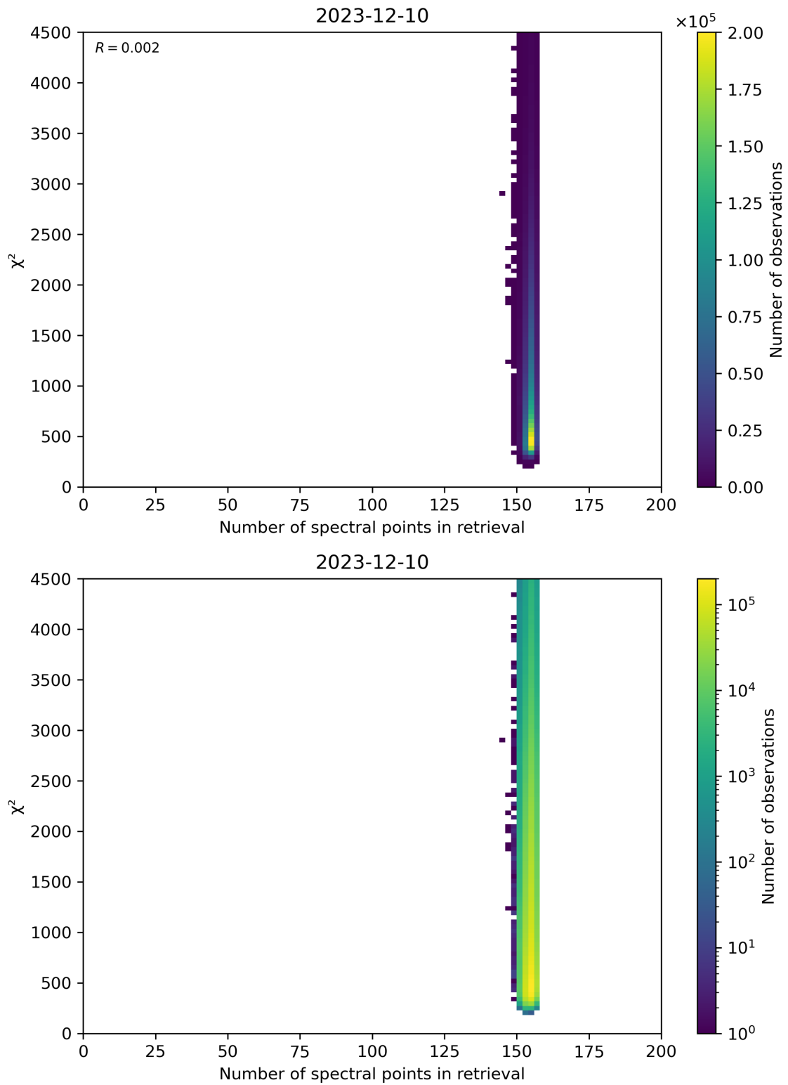
Figure 58: Scatter density plot of “Number of spectral points in retrieval” against “ \chi^2 ” for 2023-12-09 to 2023-12-11.
