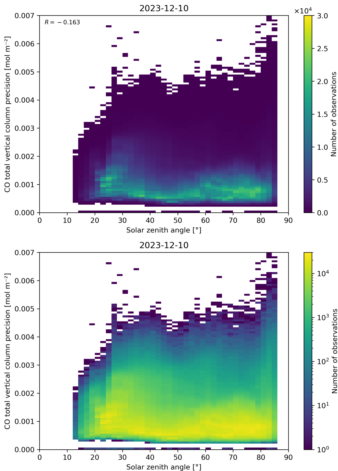
Figure 63: Scatter density plot of “Solar zenith angle” against “CO total vertical column precision” for 2023-12-09 to 2023-12-11.
