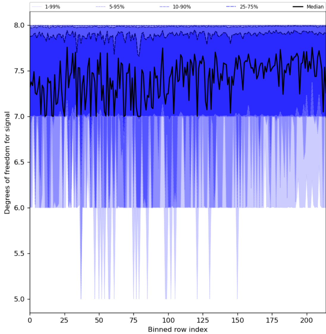
Figure 31: Along track statistics of “Degrees of freedom for signal” for 2023-12-09 to 2023-12-11
