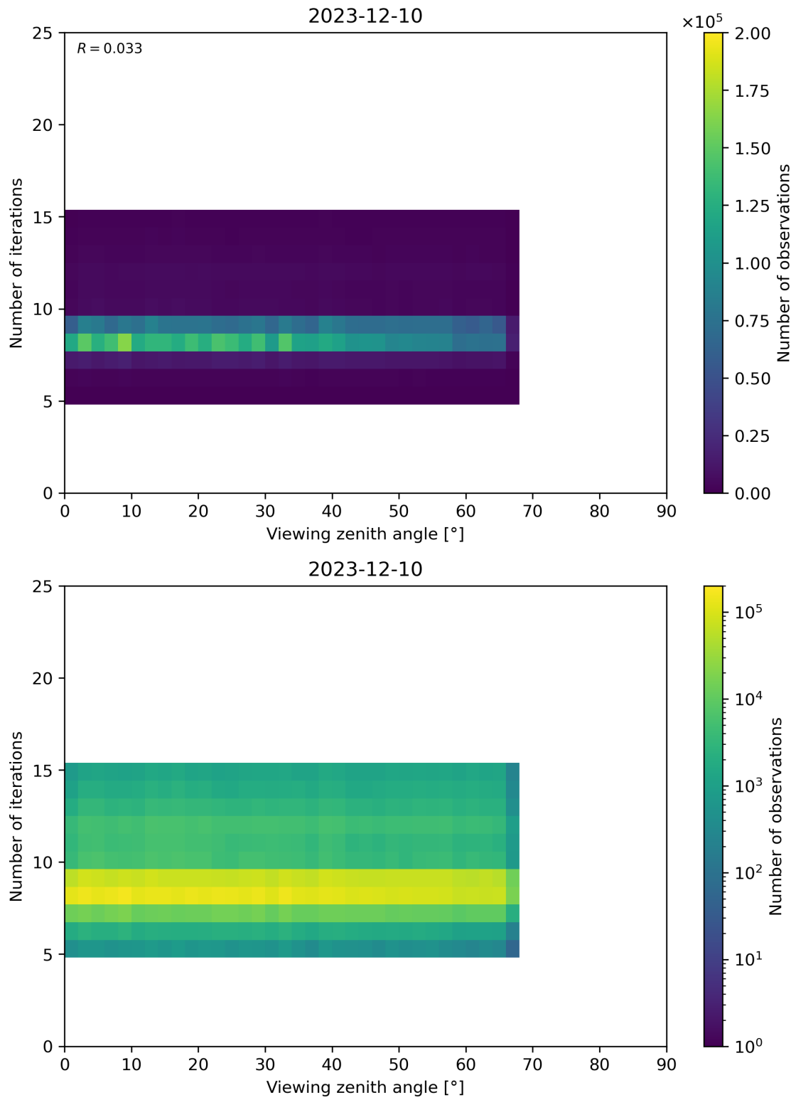
Figure 75: Scatter density plot of “Viewing zenith angle” against “Number of iterations” for 2023-12-09 to 2023-12-11.
