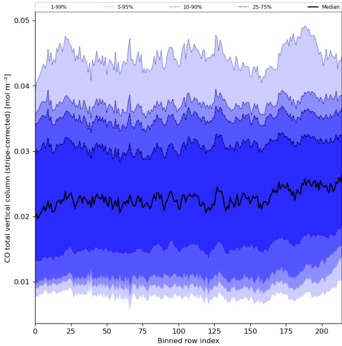
Figure 27: Along track statistics of “CO total vertical column (stripe-corrected)” for 2023-12-09 to 2023-12-11
