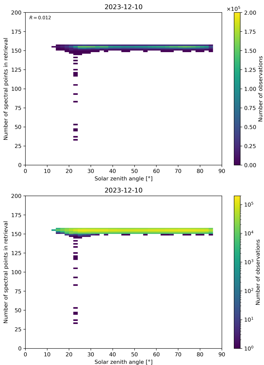
Figure 68: Scatter density plot of “Solar zenith angle” against “Number of spectral points in retrieval” for 2023-12-09 to 2023-12-11.
