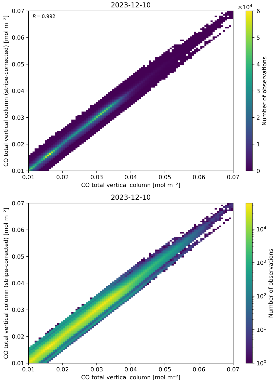
Figure 33: Scatter density plot of “CO total vertical column” against “CO total vertical column (stripe-corrected)” for 2023-12-09 to 2023-12-11.
