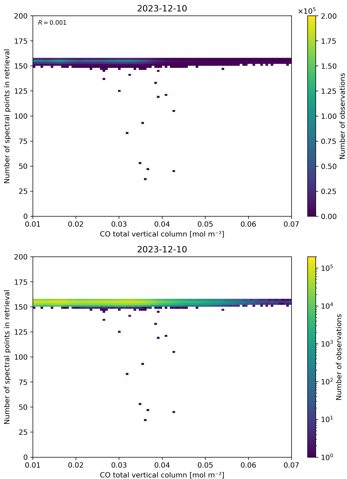
Figure 43: Scatter density plot of “CO total vertical column” against “Number of spectral points in retrieval” for 2023-12-09 to 2023-12-11.
