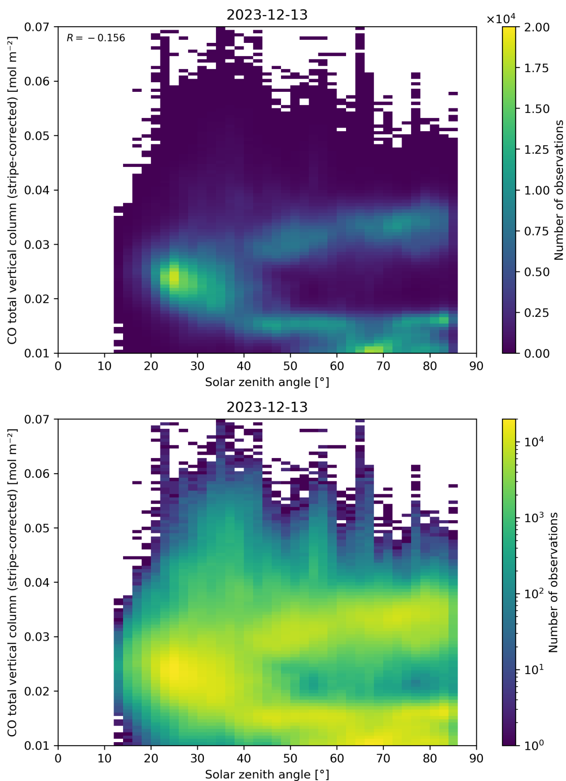
Figure 62: Scatter density plot of “Solar zenith angle” against “CO total vertical column (stripe-corrected)” for 2023-12-12 to 2023-12-14.
