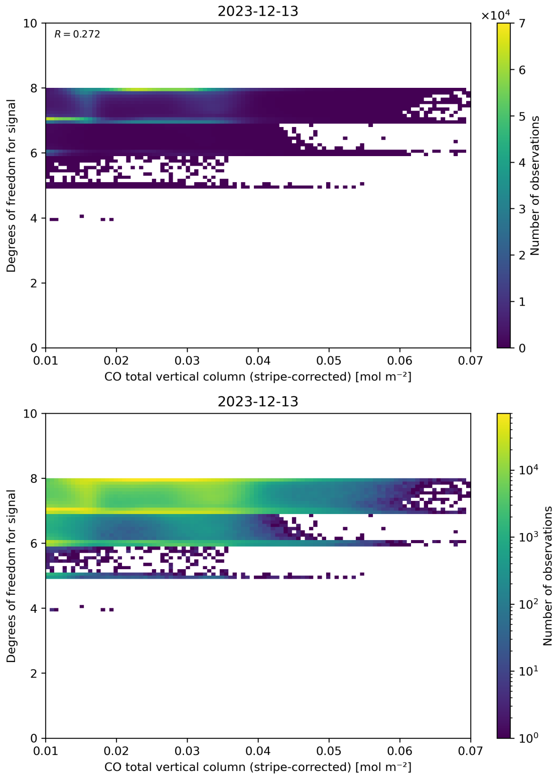
Figure 38: Scatter density plot of “CO total vertical column (stripe-corrected)” against “Degrees of freedom for signal” for 2023-12-12 to 2023-12-14.
