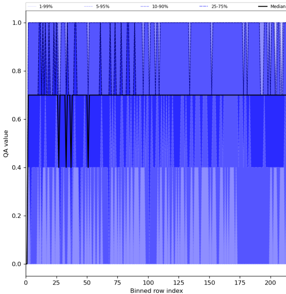
Figure 25: Along track statistics of “QA value” for 2023-12-12 to 2023-12-14
