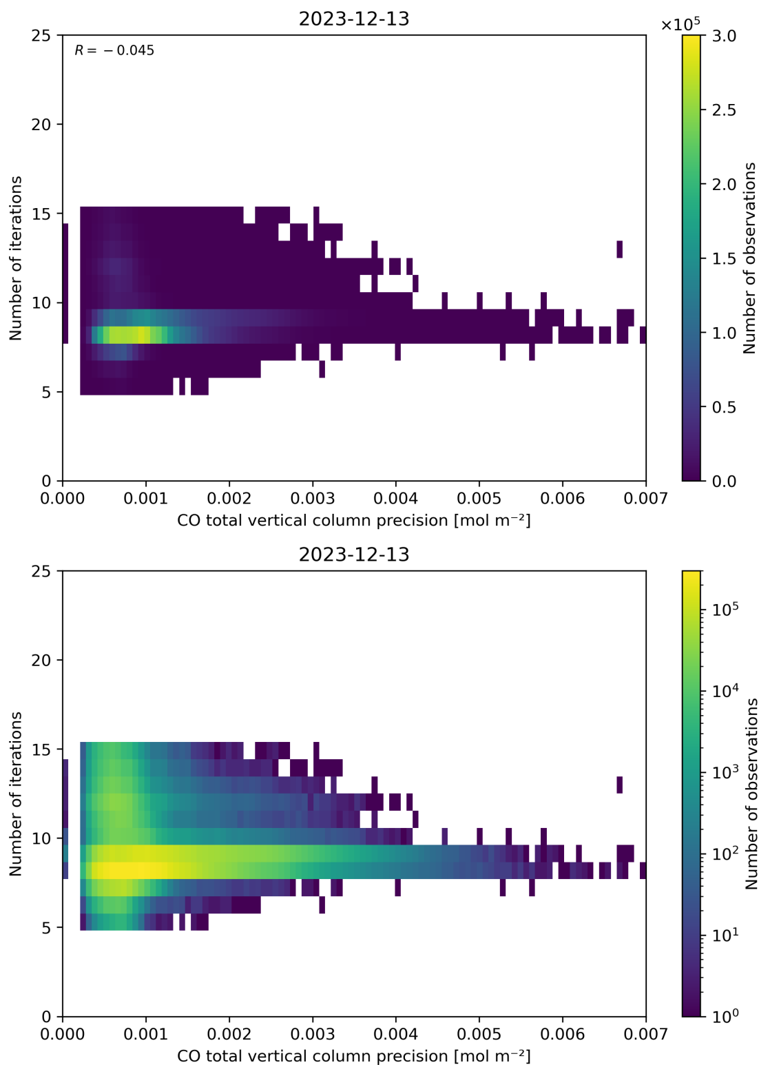
Figure 46: Scatter density plot of “CO total vertical column precision” against “Number of iterations” for 2023-12-12 to 2023-12-14.
