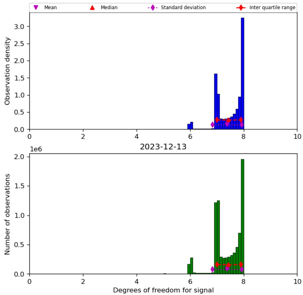
Figure 23: Histogram of “Degrees of freedom for signal” for 2023-12-12 to 2023-12-14
