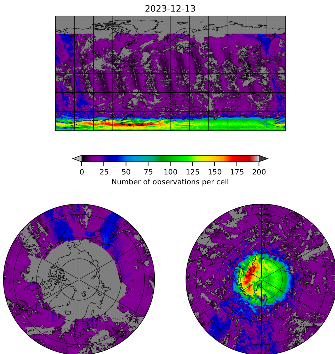
Figure 8: Map of the number of observations for 2023-12-12 to 2023-12-14
