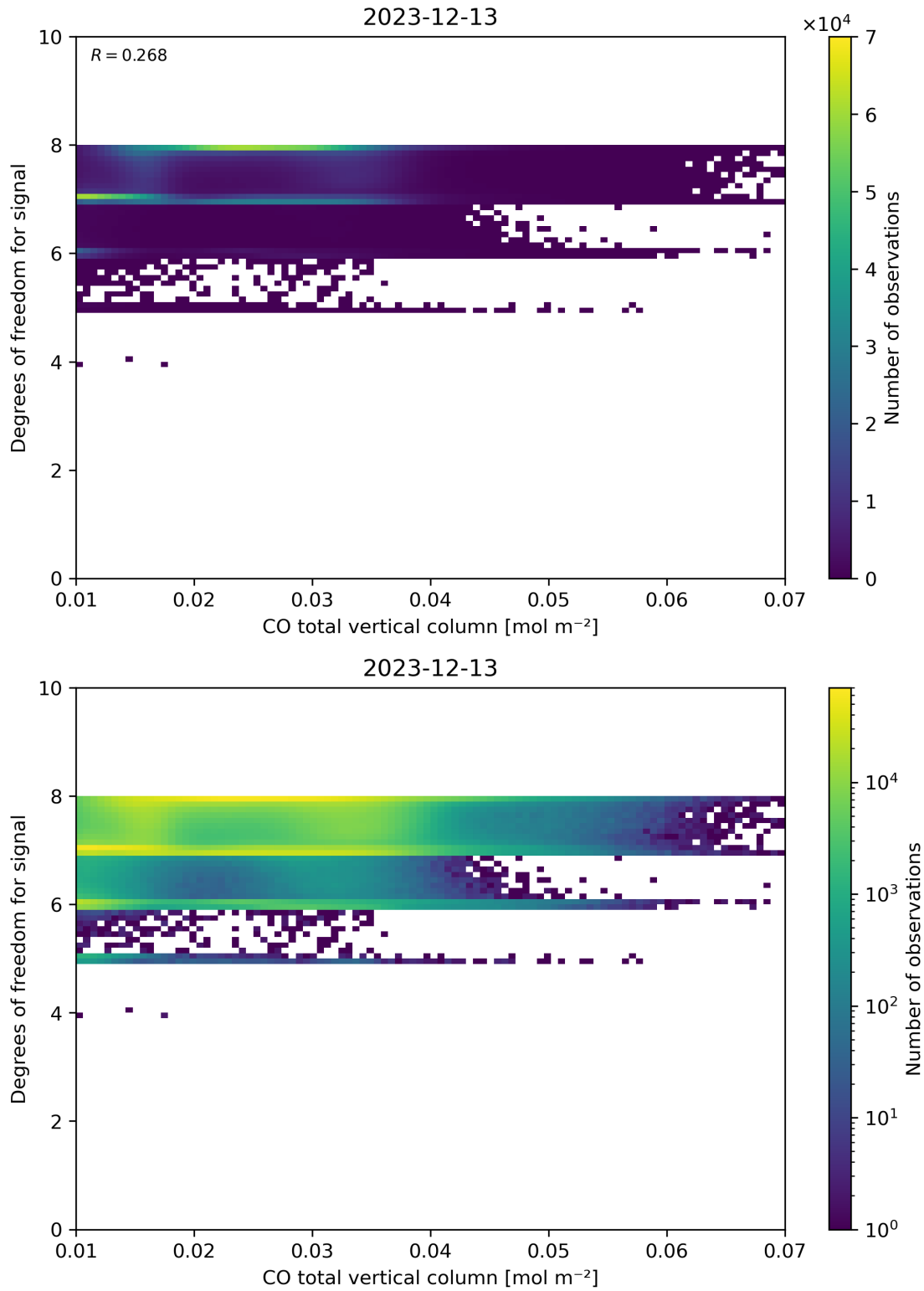
Figure 41: Scatter density plot of “CO total vertical column” against “Degrees of freedom for signal” for 2023-12-12 to 2023-12-14.
