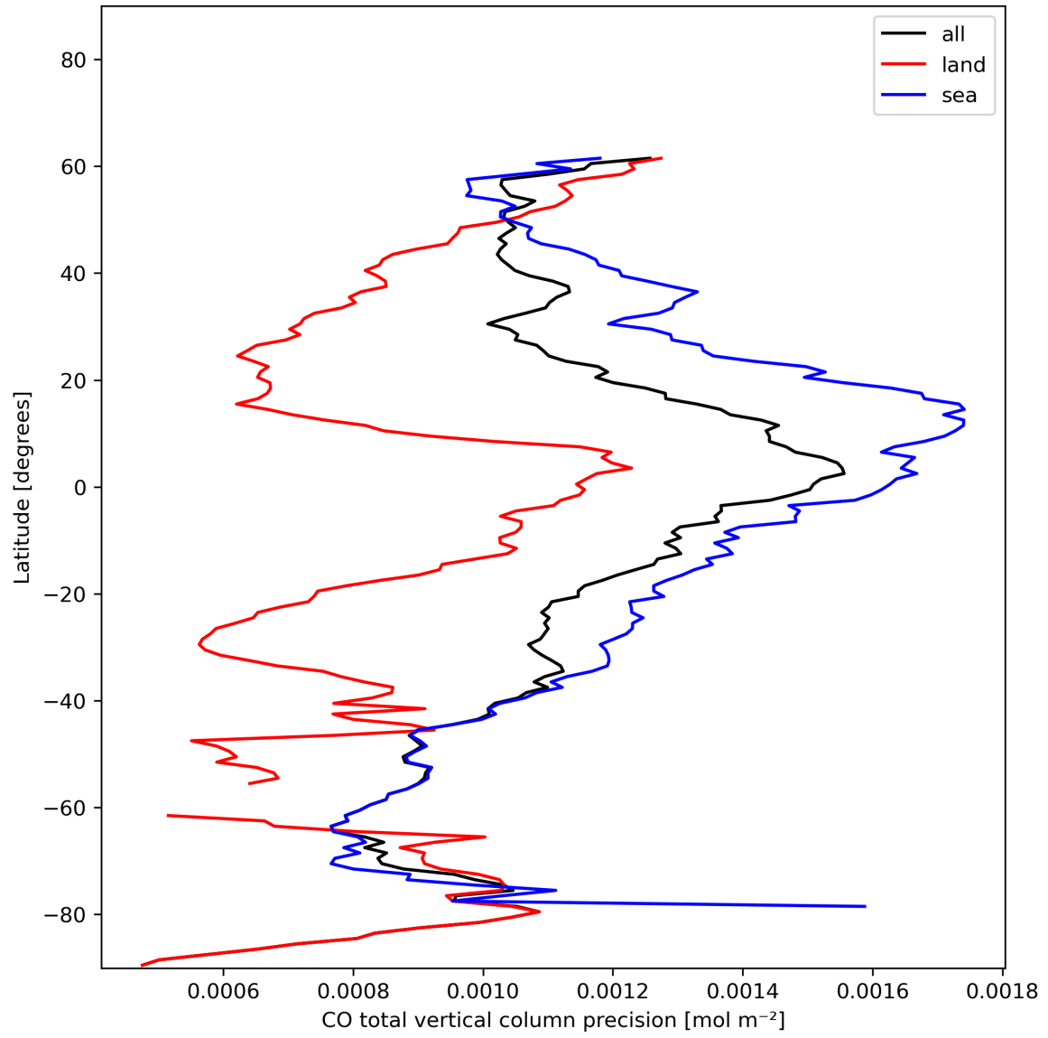
Figure 12: Zonal average of “CO total vertical column precision” for 2023-12-12 to 2023-12-14.
