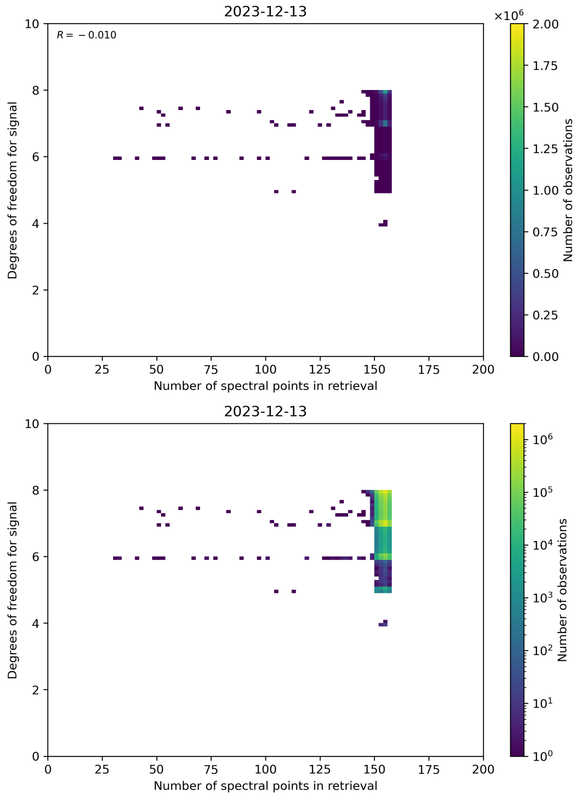
Figure 59: Scatter density plot of “Number of spectral points in retrieval” against “Degrees of freedom for signal” for 2023-12-12 to 2023-12-14.
