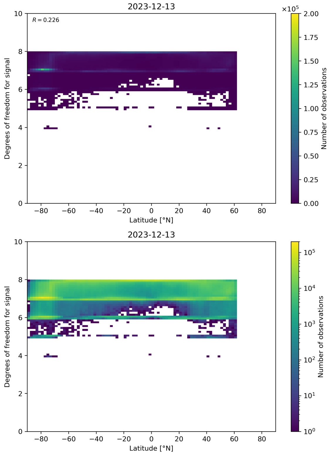
Figure 55: Scatter density plot of “Latitude” against “Degrees of freedom for signal” for 2023-12-12 to 2023-12-14.
