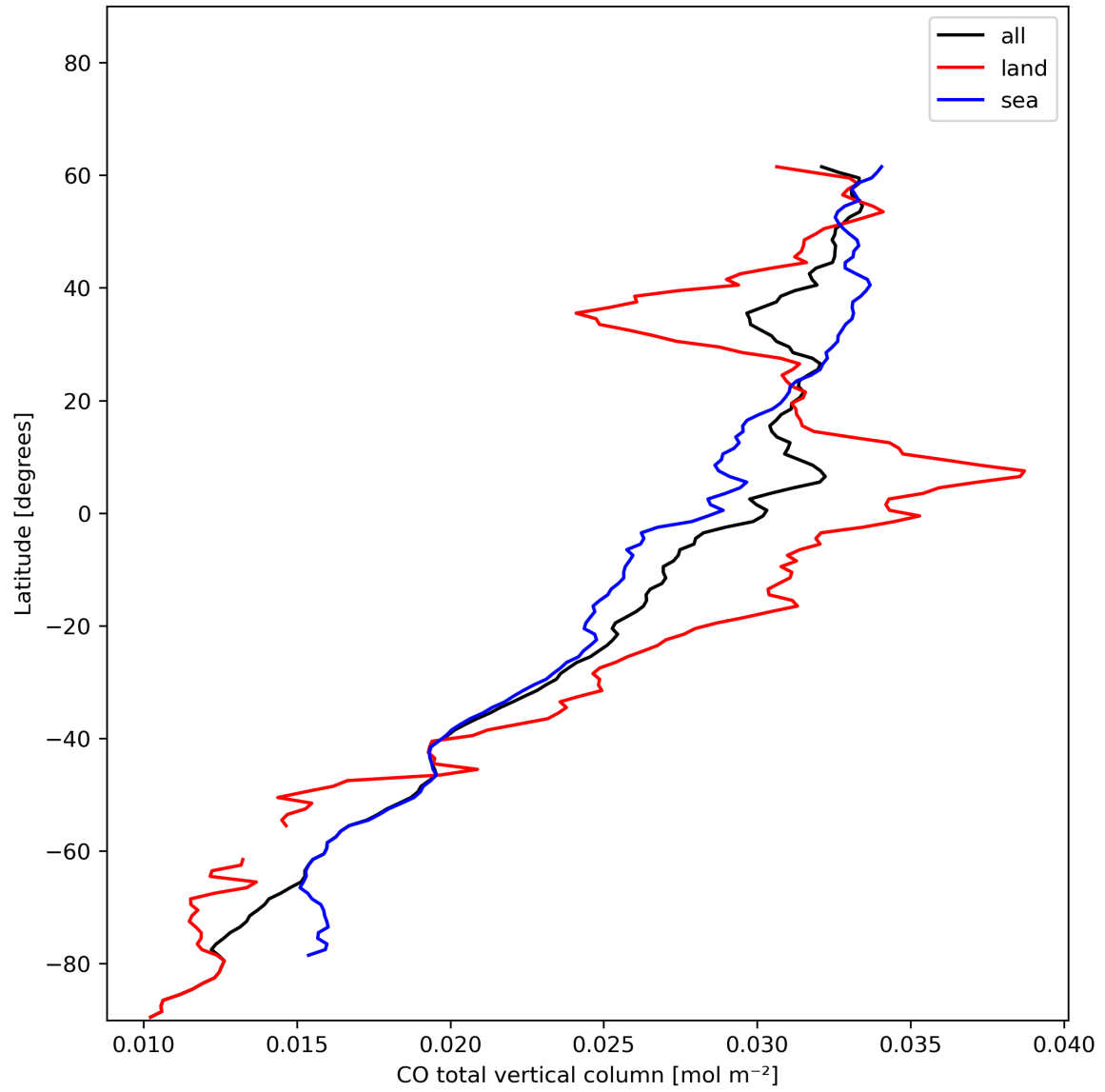
Figure 10: Zonal average of “CO total vertical column” for 2023-12-12 to 2023-12-14.
