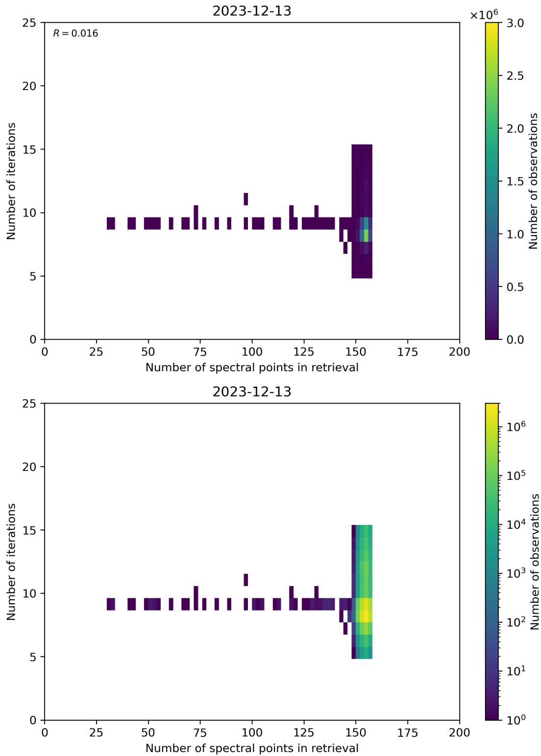
Figure 60: Scatter density plot of “Number of spectral points in retrieval” against “Number of iterations” for 2023-12-12 to 2023-12-14.
