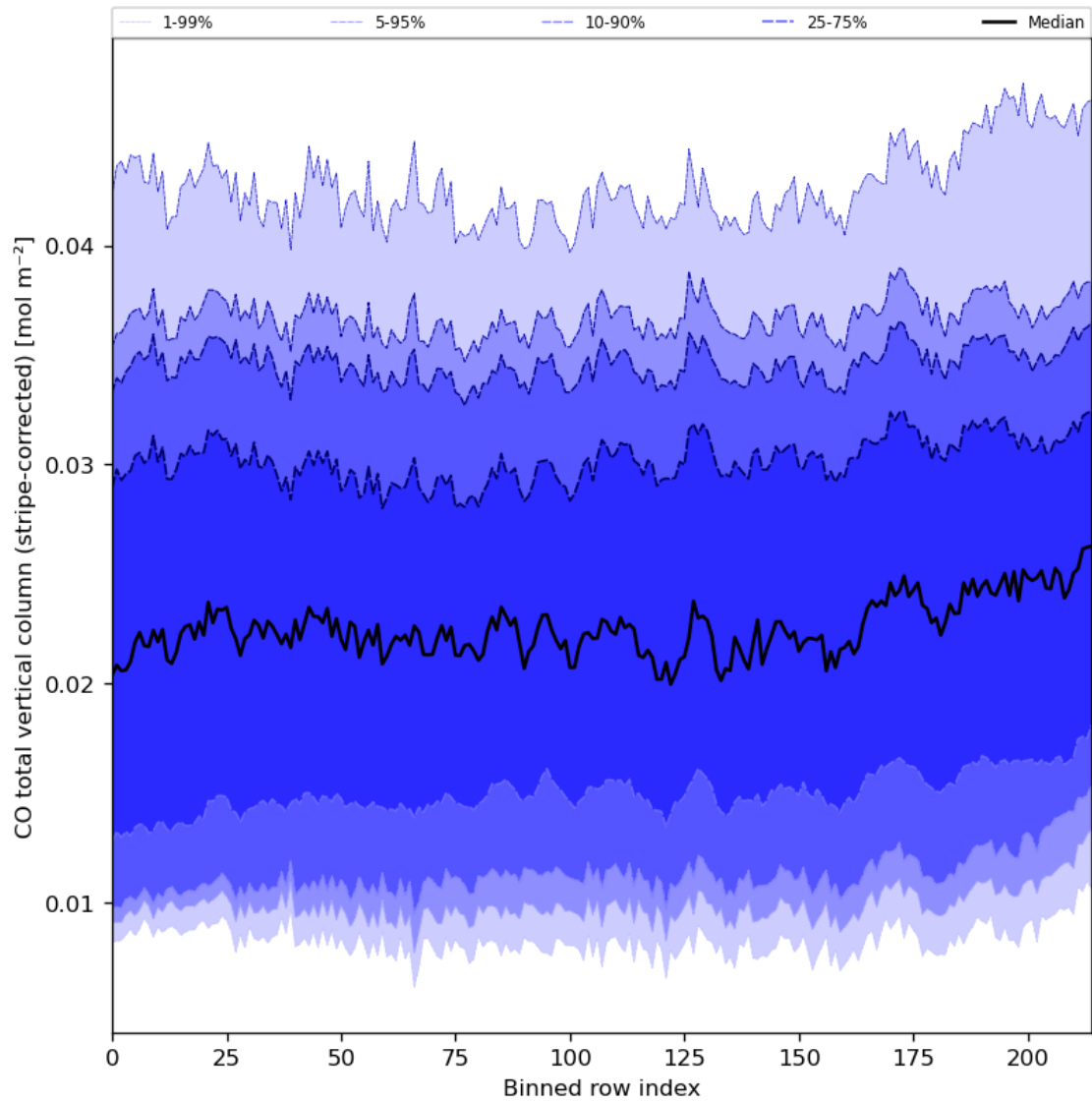
Figure 27: Along track statistics of “CO total vertical column (stripe-corrected)” for 2023-12-12 to 2023-12-14
