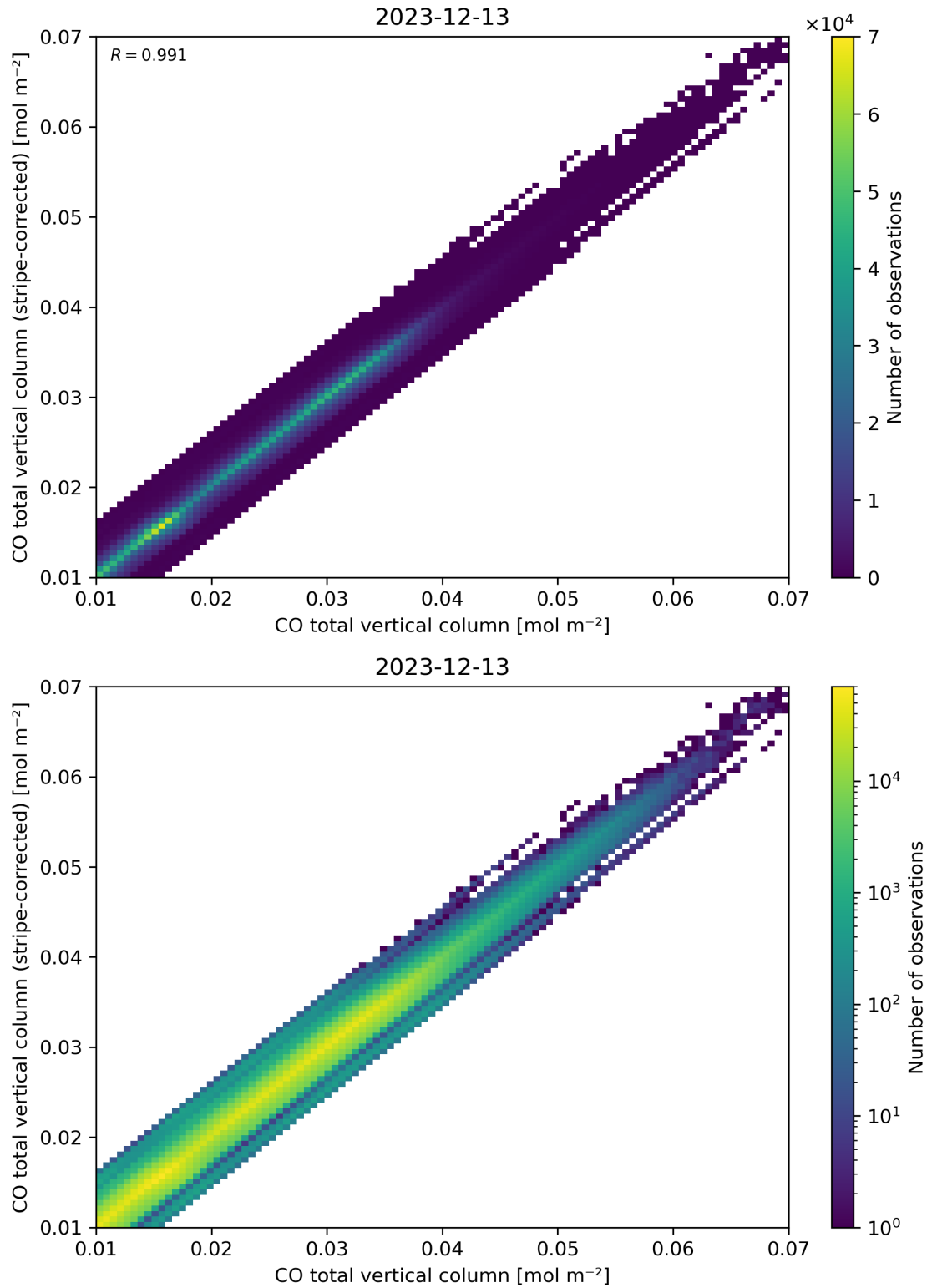
Figure 33: Scatter density plot of “CO total vertical column” against “CO total vertical column (stripe-corrected)” for 2023-12-12 to 2023-12-14.
