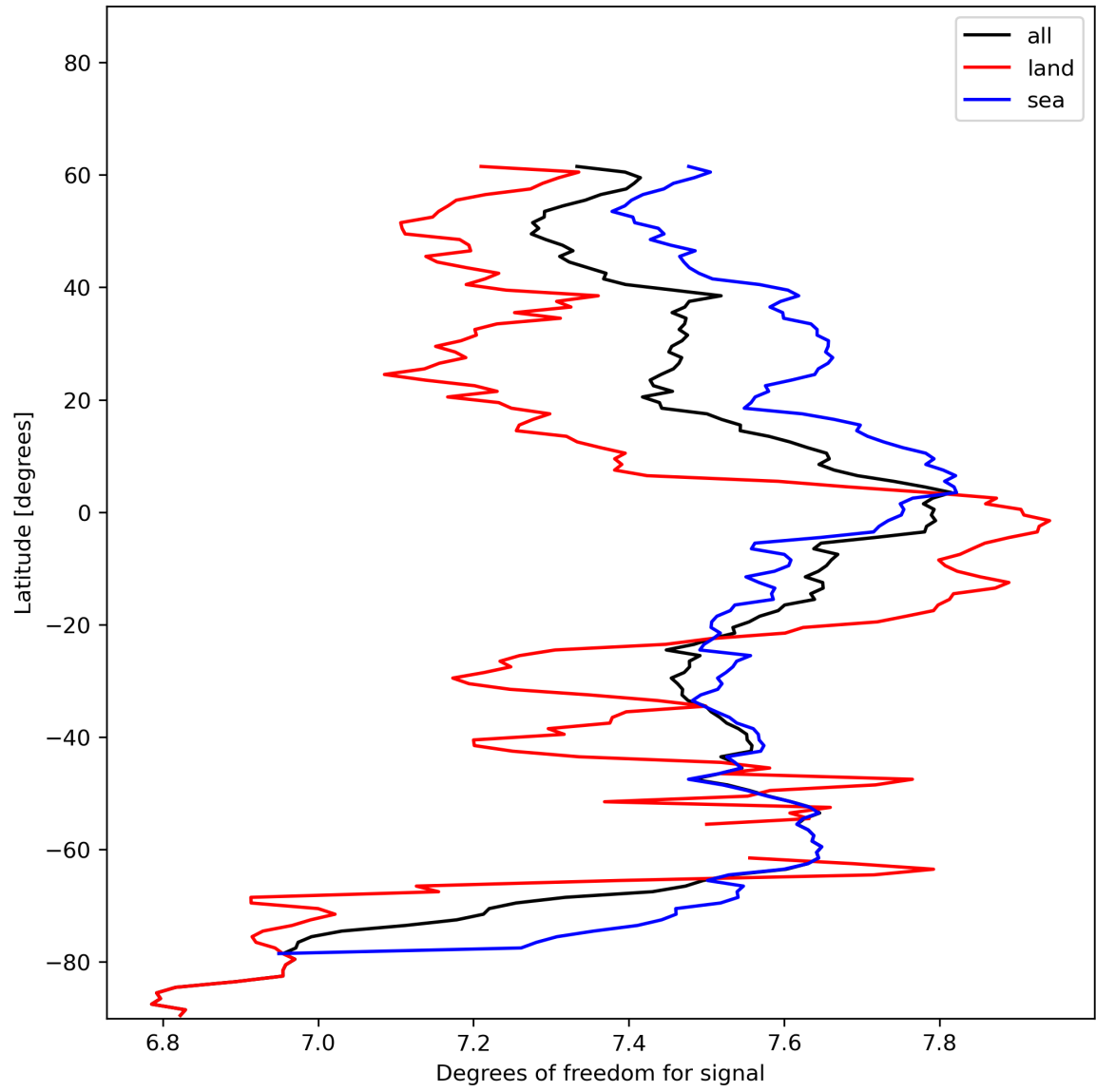
Figure 15: Zonal average of “Degrees of freedom for signal” for 2023-12-12 to 2023-12-14.
