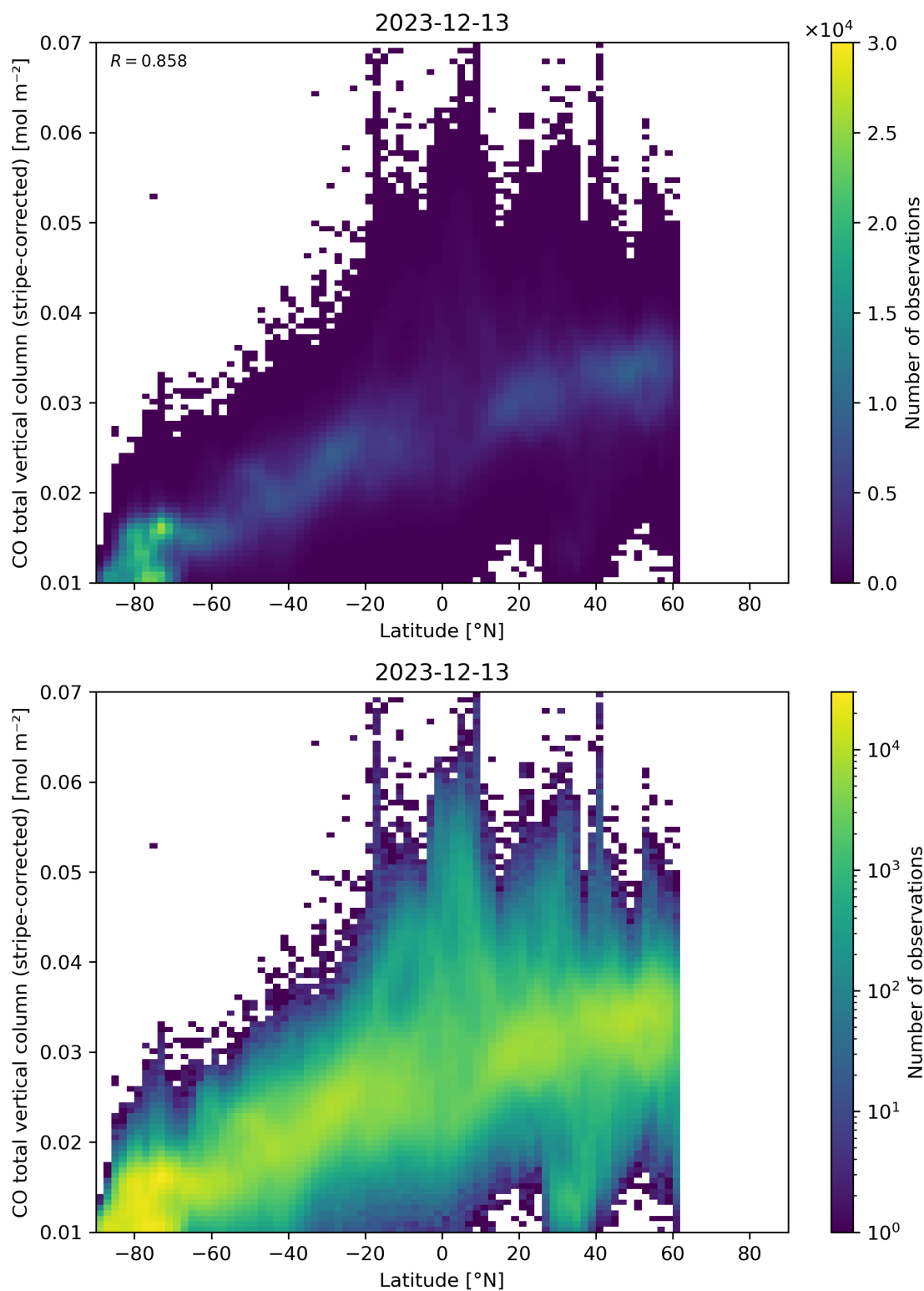
Figure 52: Scatter density plot of “Latitude” against “CO total vertical column (stripe-corrected)” for 2023-12-12 to 2023-12-14.
