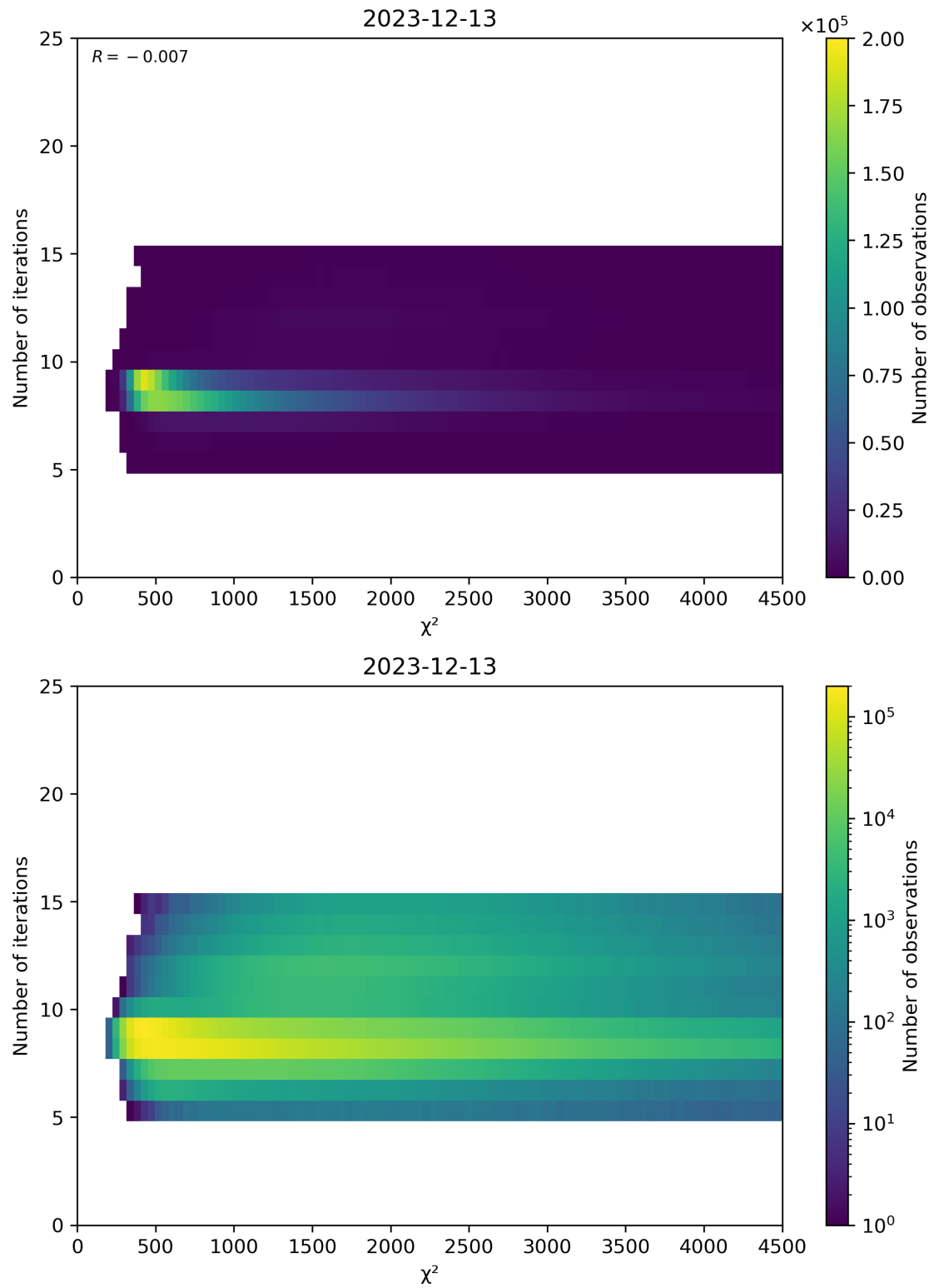
Figure 49: Scatter density plot of “ \chi^2 ” against “Number of iterations” for 2023-12-12 to 2023-12-14.
