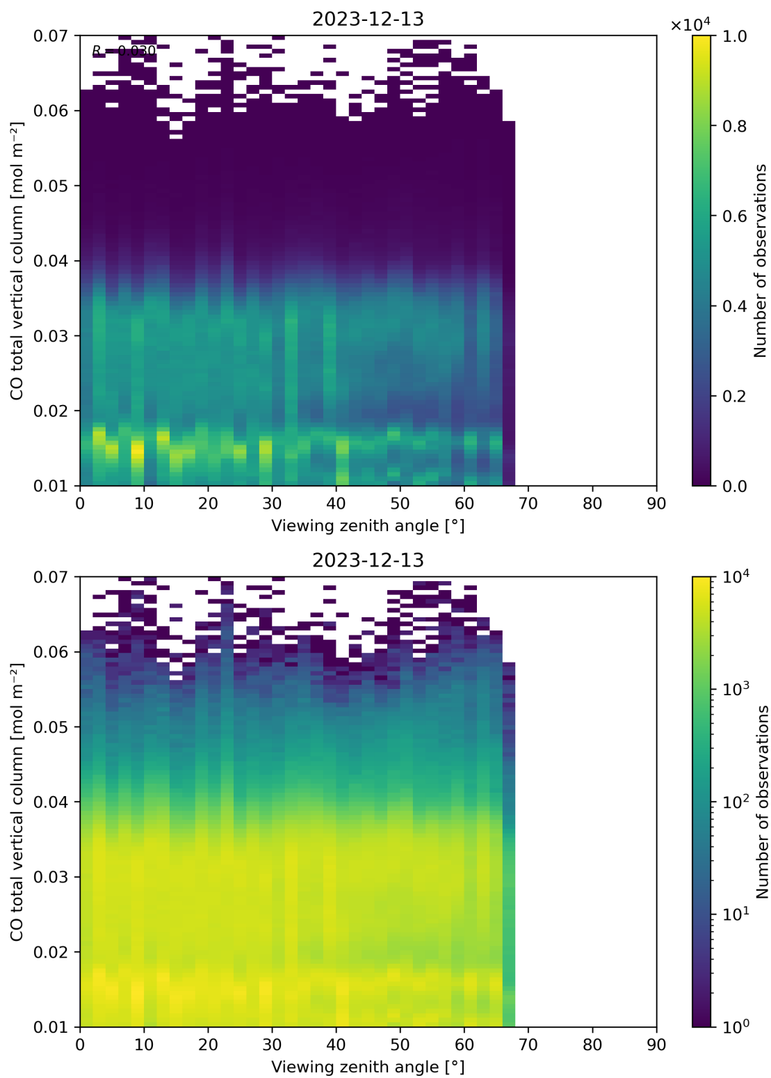
Figure 69: Scatter density plot of “Viewing zenith angle” against “CO total vertical column” for 2023-12-12 to 2023-12-14.
