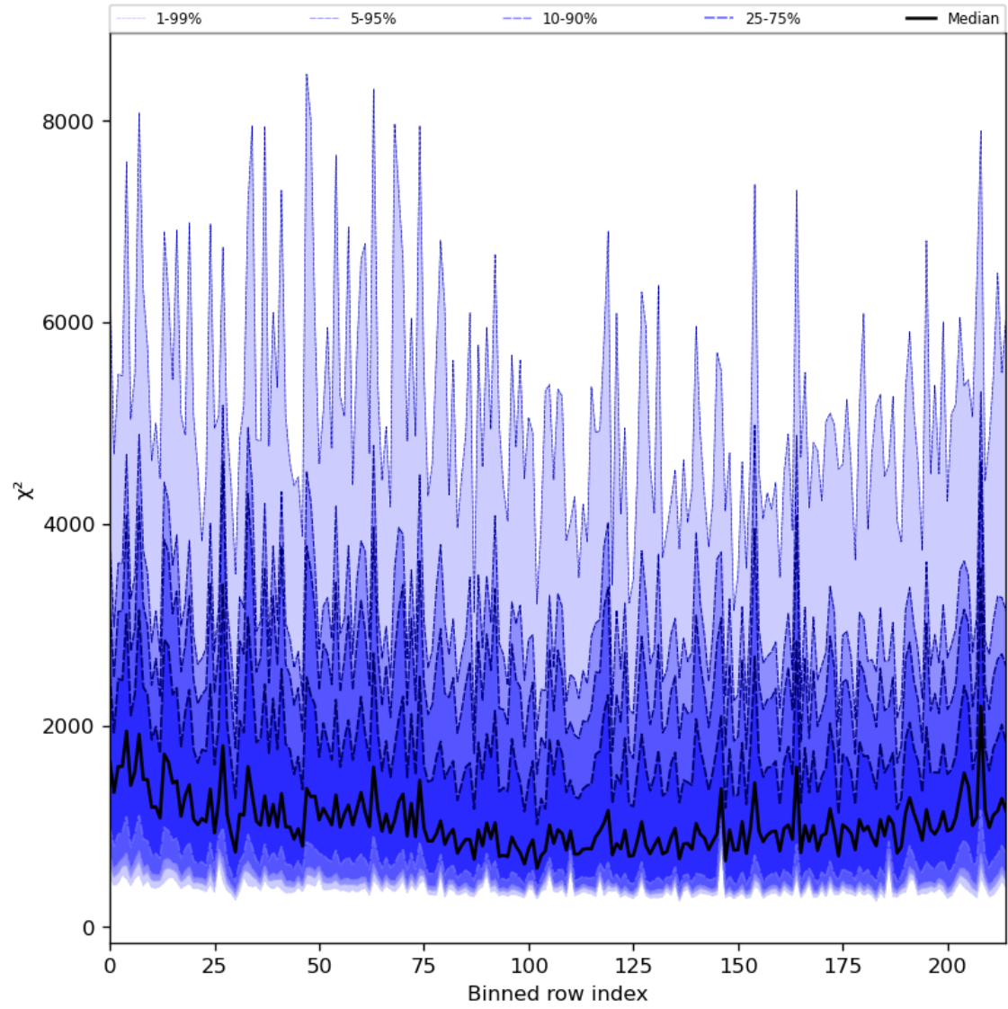
Figure 30: Along track statistics of “ \chi^2 ” for 2023-12-12 to 2023-12-14
