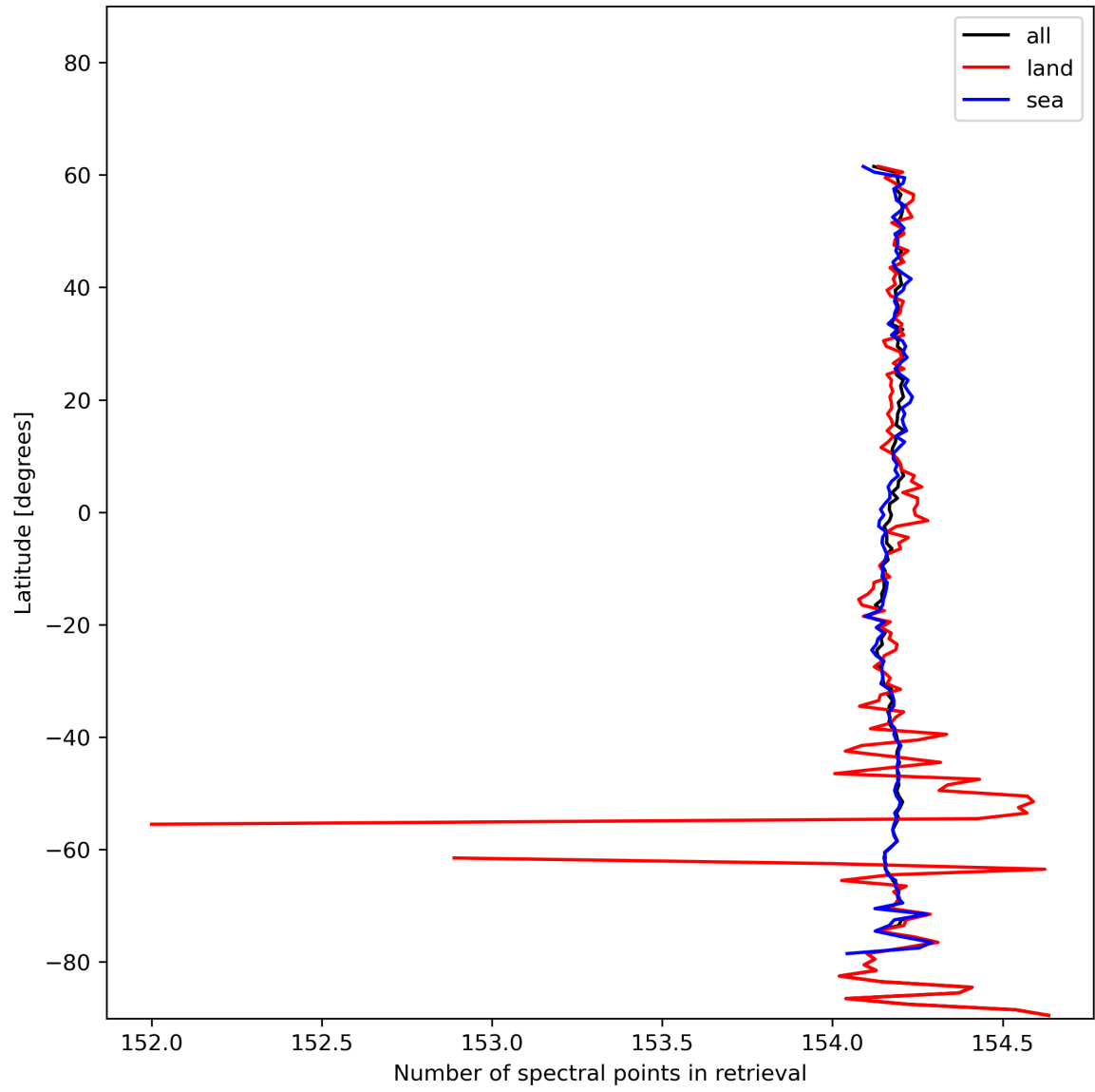
Figure 13: Zonal average of “Number of spectral points in retrieval” for 2023-12-12 to 2023-12-14.
