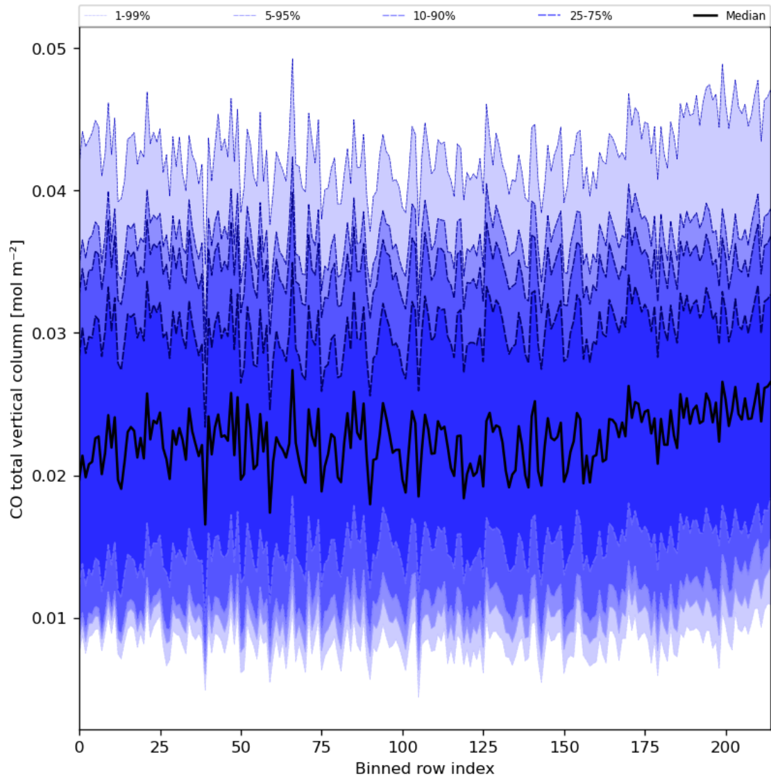
Figure 26: Along track statistics of “CO total vertical column” for 2023-12-12 to 2023-12-14
