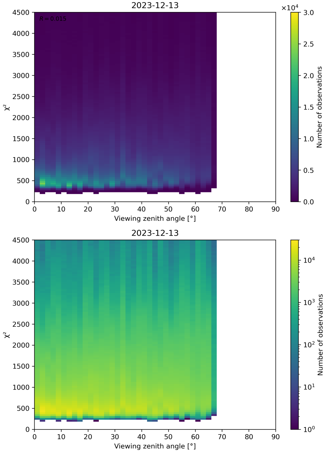
Figure 72: Scatter density plot of “Viewing zenith angle” against “ \chi^2 ” for 2023-12-12 to 2023-12-14.
