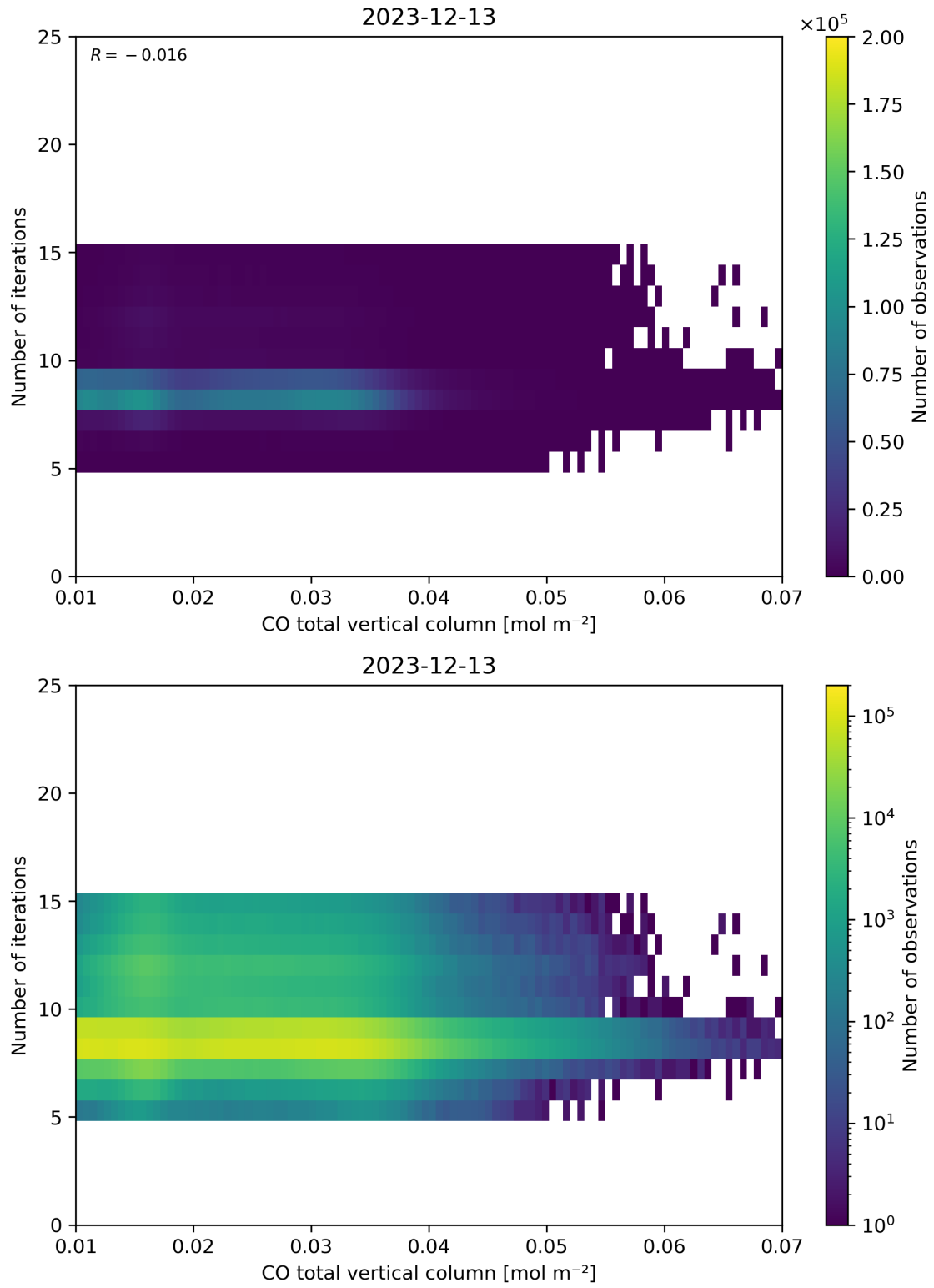
Figure 42: Scatter density plot of “CO total vertical column” against “Number of iterations” for 2023-12-12 to 2023-12-14.
