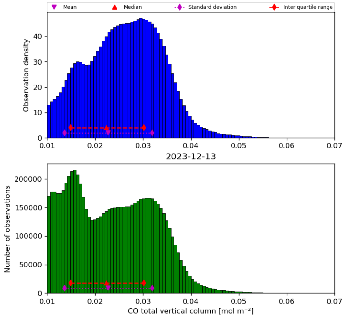
Figure 18: Histogram of “CO total vertical column” for 2023-12-12 to 2023-12-14
