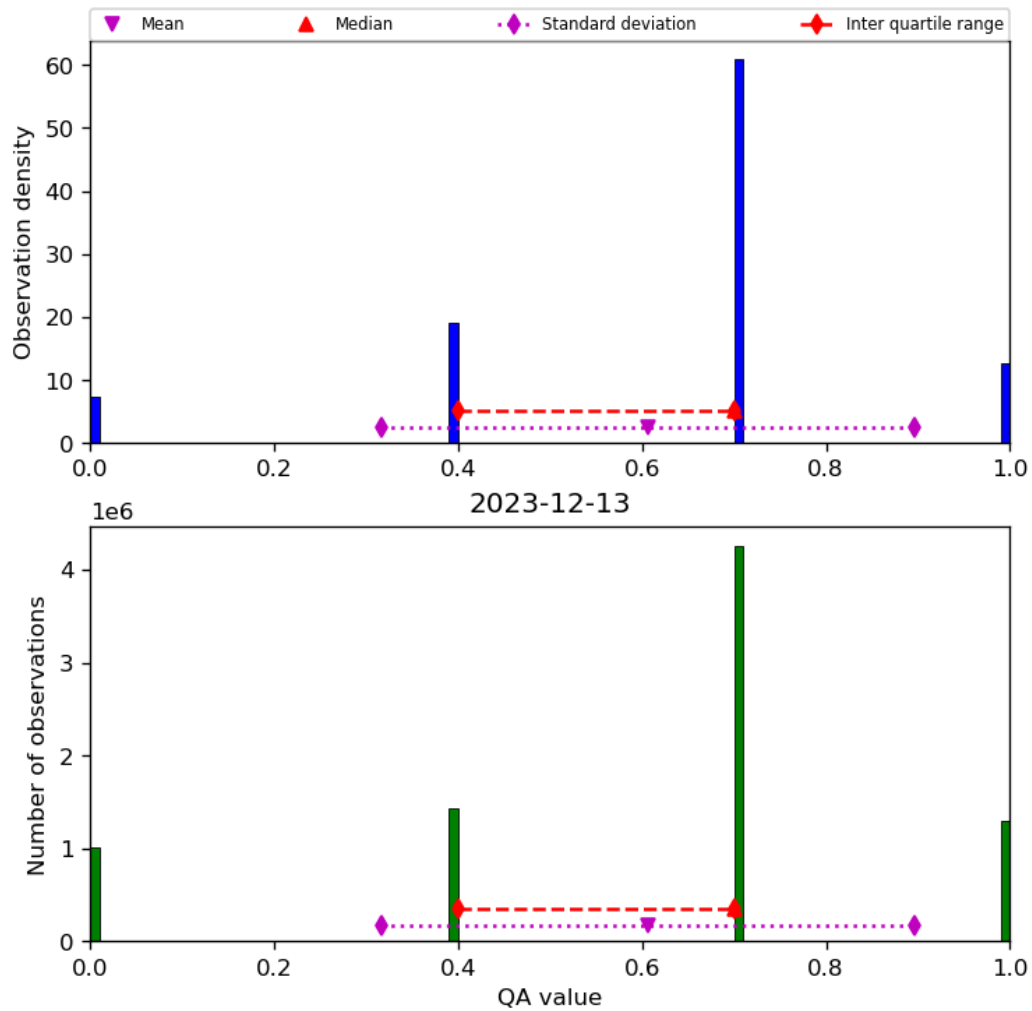
Figure 17: Histogram of “QA value” for 2023-12-12 to 2023-12-14
