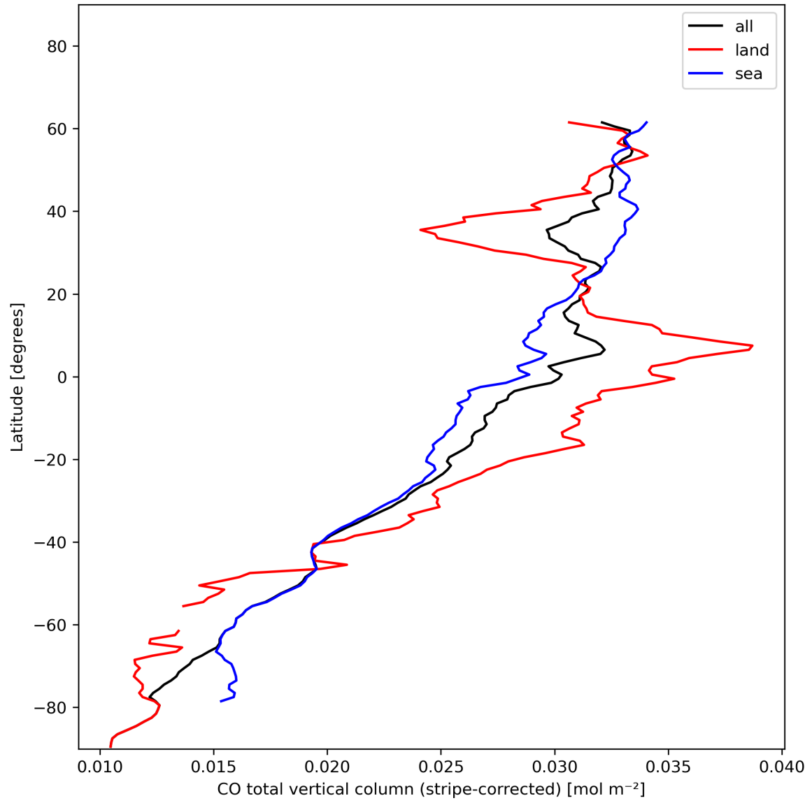
Figure 11: Zonal average of “CO total vertical column (stripe-corrected)” for 2023-12-12 to 2023-12-14.
