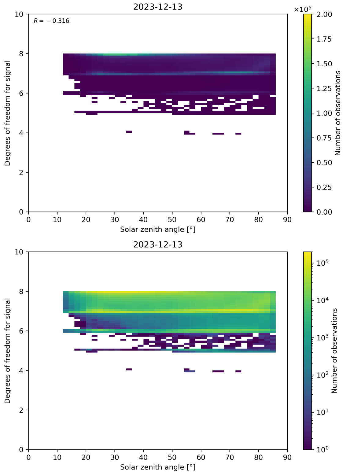
Figure 65: Scatter density plot of “Solar zenith angle” against “Degrees of freedom for signal” for 2023-12-12 to 2023-12-14.
