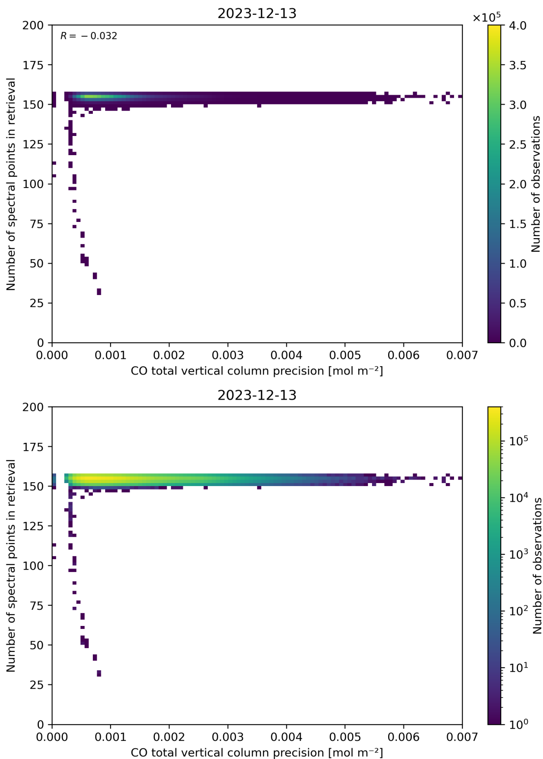
Figure 47: Scatter density plot of “CO total vertical column precision” against “Number of spectral points in retrieval” for 2023-12-12 to 2023-12-14.
