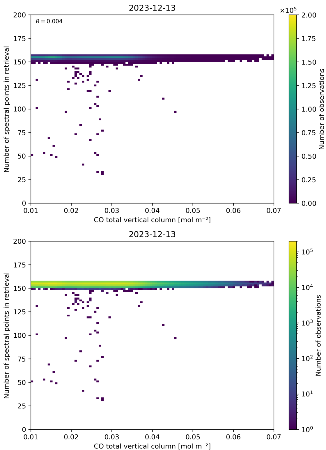
Figure 43: Scatter density plot of “CO total vertical column” against “Number of spectral points in retrieval” for 2023-12-12 to 2023-12-14.
