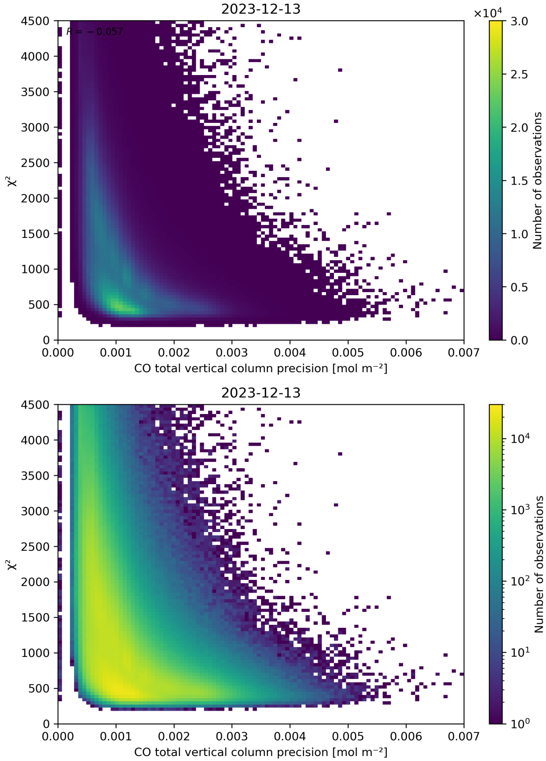
Figure 44: Scatter density plot of “CO total vertical column precision” against “ \chi^2 ” for 2023-12-12 to 2023-12-14.
