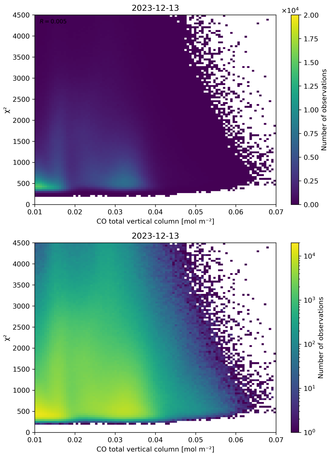
Figure 35: Scatter density plot of “CO total vertical column” against “ \chi^2 ” for 2023-12-12 to 2023-12-14.
