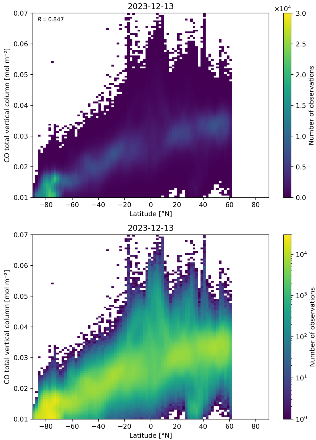
Figure 51: Scatter density plot of “Latitude” against “CO total vertical column” for 2023-12-12 to 2023-12-14.
