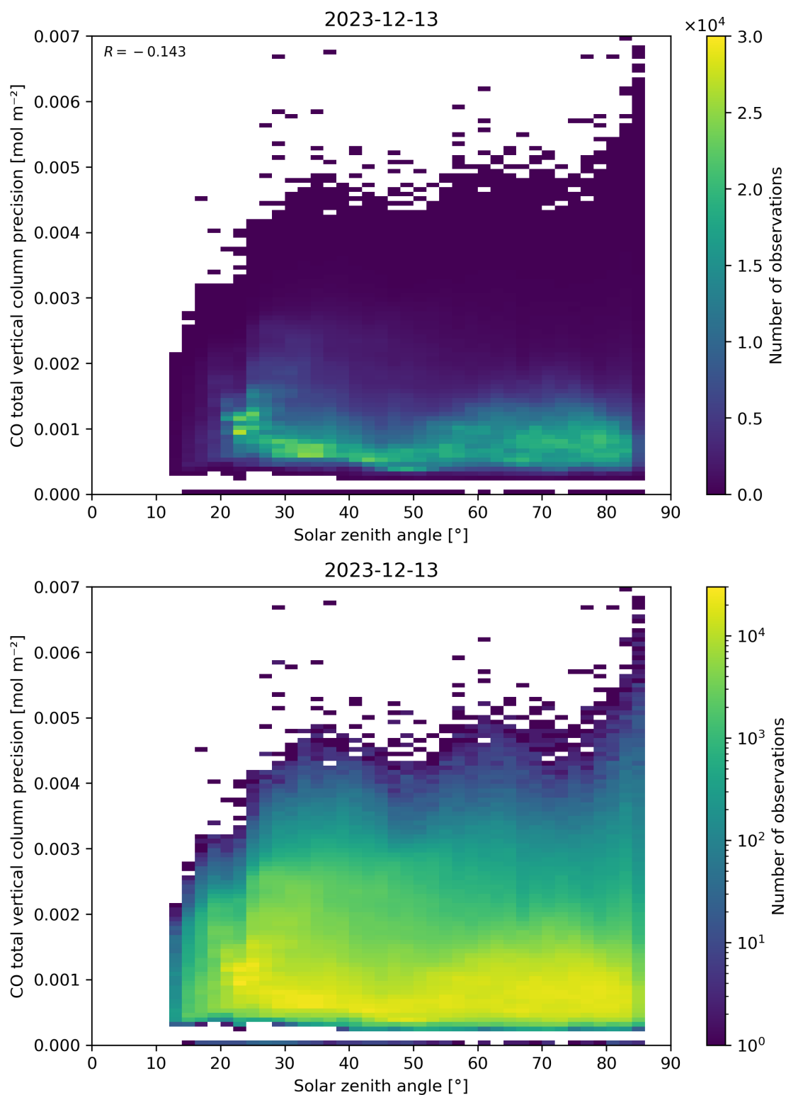
Figure 63: Scatter density plot of “Solar zenith angle” against “CO total vertical column precision” for 2023-12-12 to 2023-12-14.
