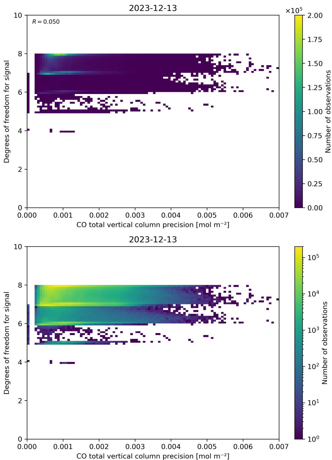
Figure 45: Scatter density plot of “CO total vertical column precision” against “Degrees of freedom for signal” for 2023-12-12 to 2023-12-14.
