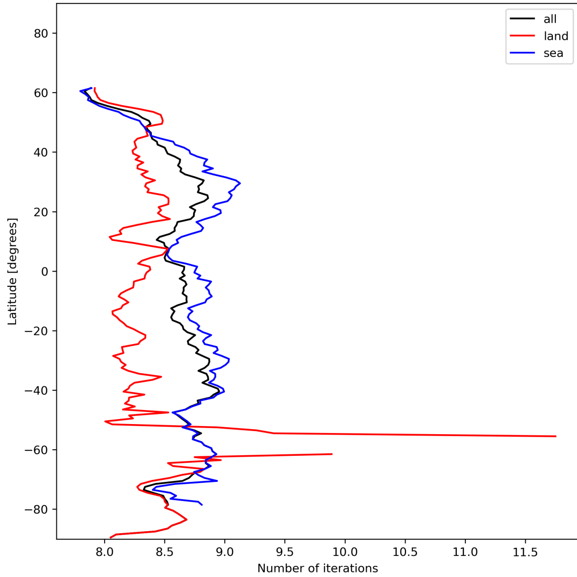
Figure 16: Zonal average of “Number of iterations” for 2023-12-12 to 2023-12-14.
