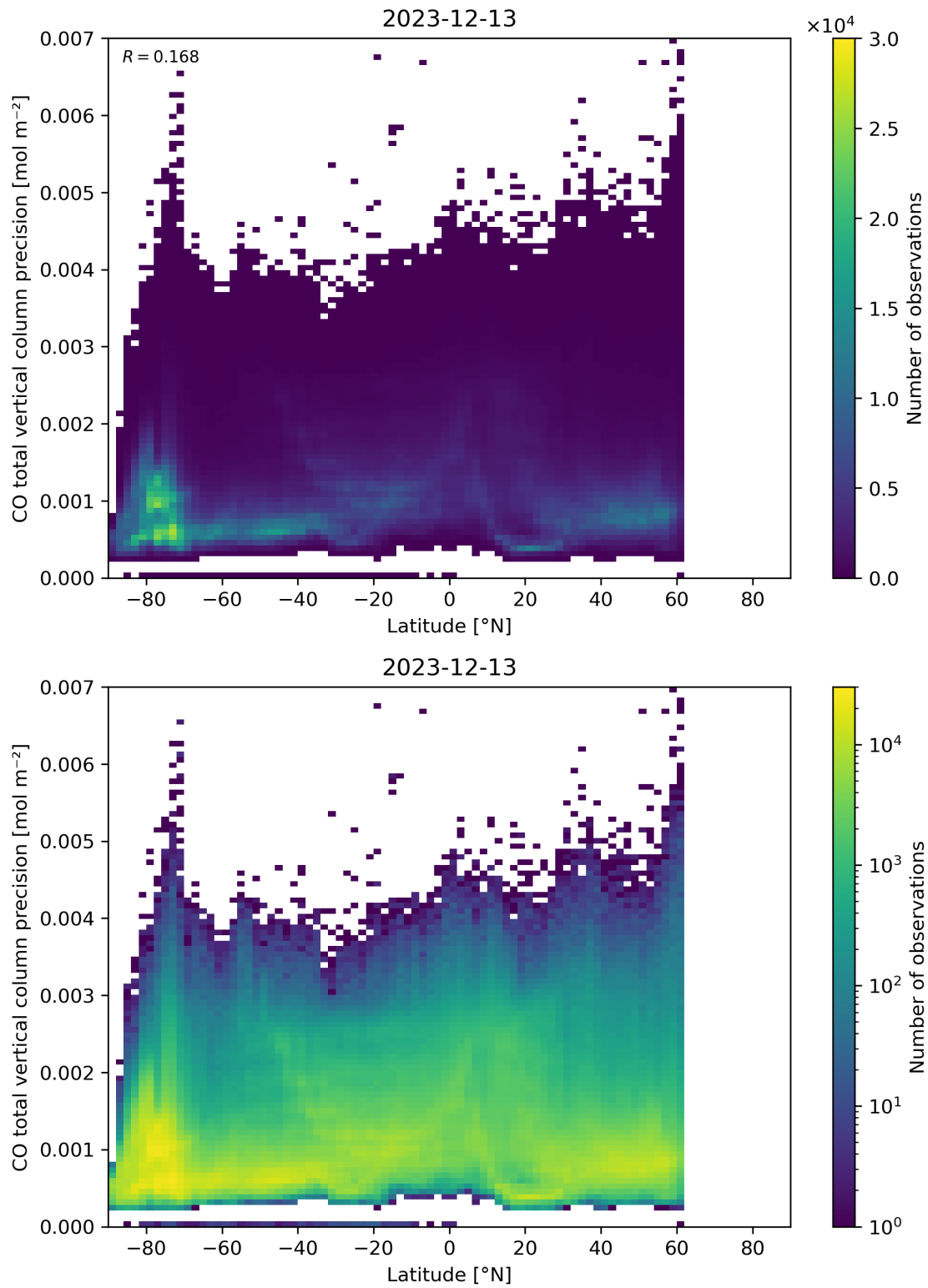
Figure 53: Scatter density plot of “Latitude” against “CO total vertical column precision” for 2023-12-12 to 2023-12-14.
