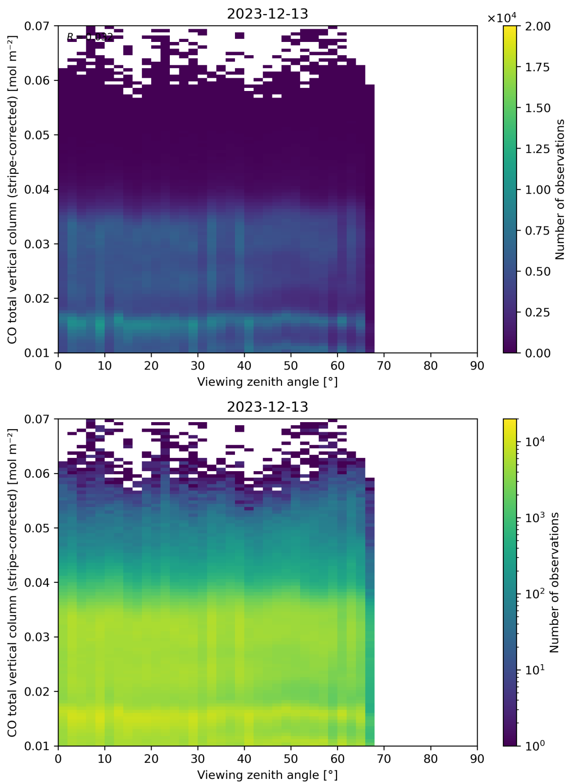
Figure 70: Scatter density plot of “Viewing zenith angle” against “CO total vertical column (stripe-corrected)” for 2023-12-12 to 2023-12-14.
