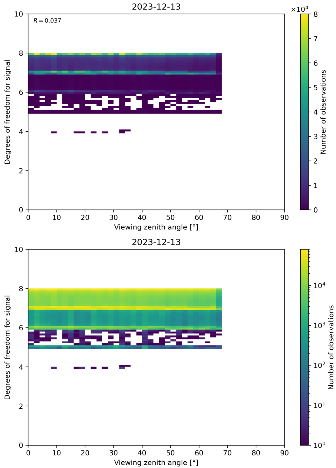
Figure 73: Scatter density plot of “Viewing zenith angle” against “Degrees of freedom for signal” for 2023-12-12 to 2023-12-14.
