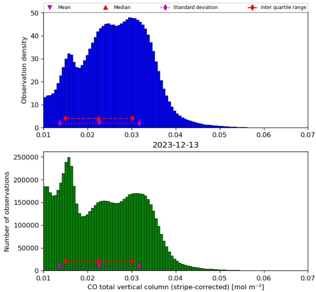
Figure 19: Histogram of “CO total vertical column (stripe-corrected)” for 2023-12-12 to 2023-12-14
