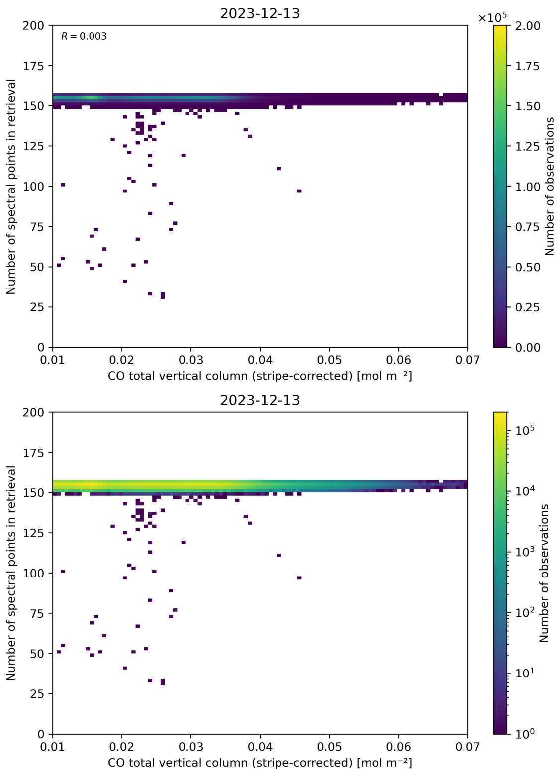
Figure 40: Scatter density plot of “CO total vertical column (stripe-corrected)” against “Number of spectral points in retrieval” for 2023-12-12 to 2023-12-14.
