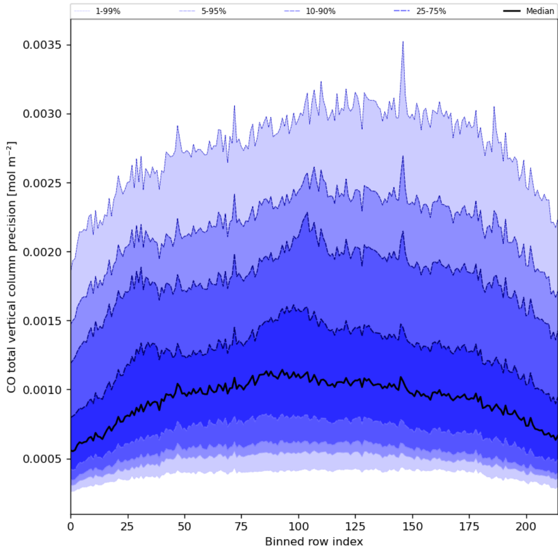
Figure 28: Along track statistics of “CO total vertical column precision” for 2023-12-12 to 2023-12-14
