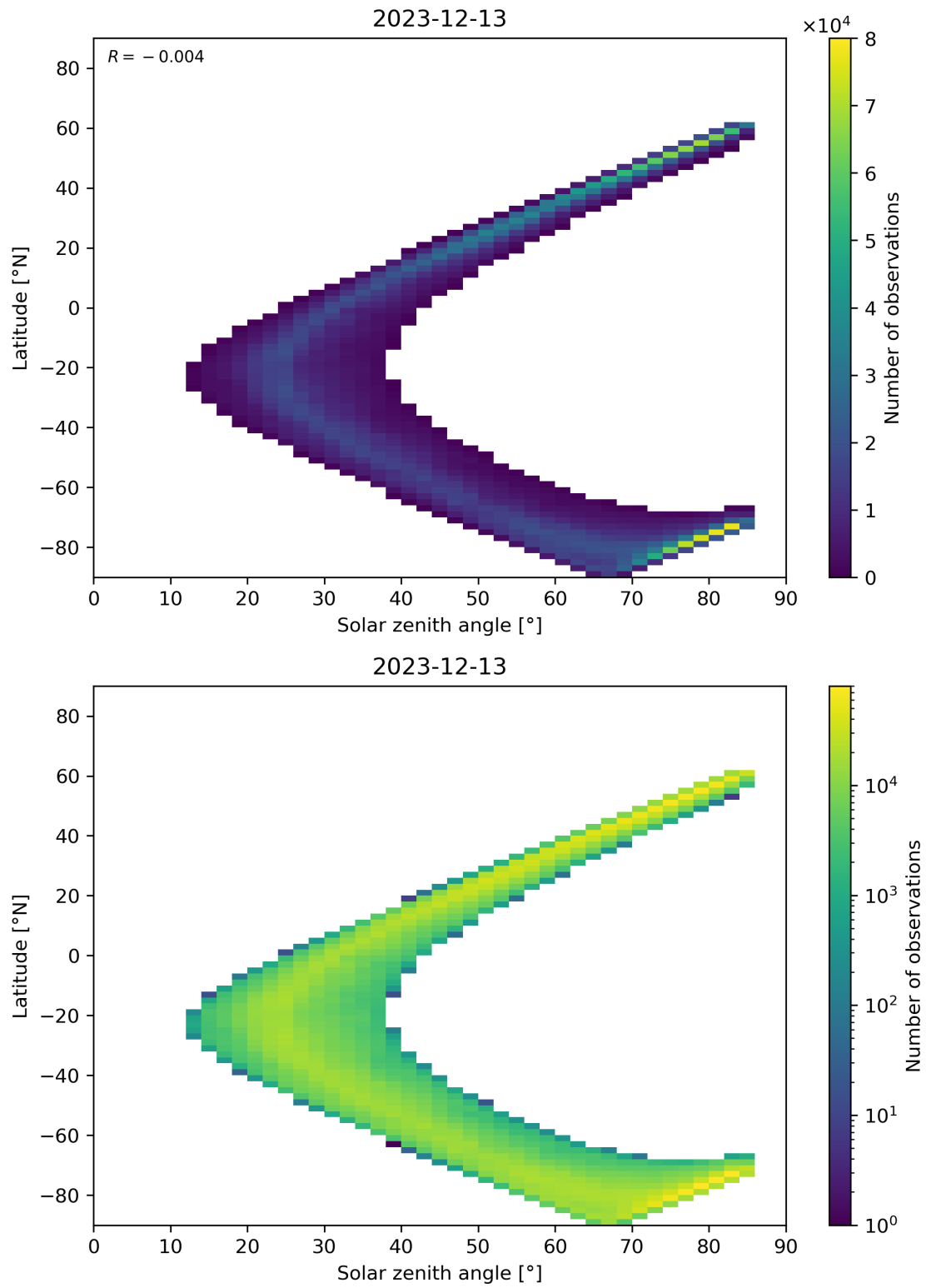
Figure 66: Scatter density plot of “Solar zenith angle” against “Latitude” for 2023-12-12 to 2023-12-14.
