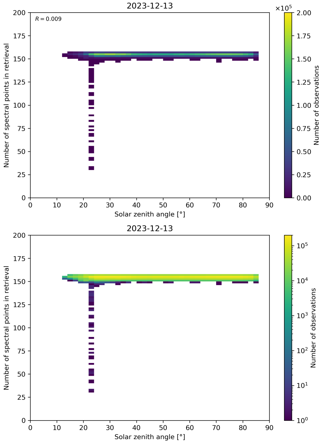
Figure 68: Scatter density plot of “Solar zenith angle” against “Number of spectral points in retrieval” for 2023-12-12 to 2023-12-14.
