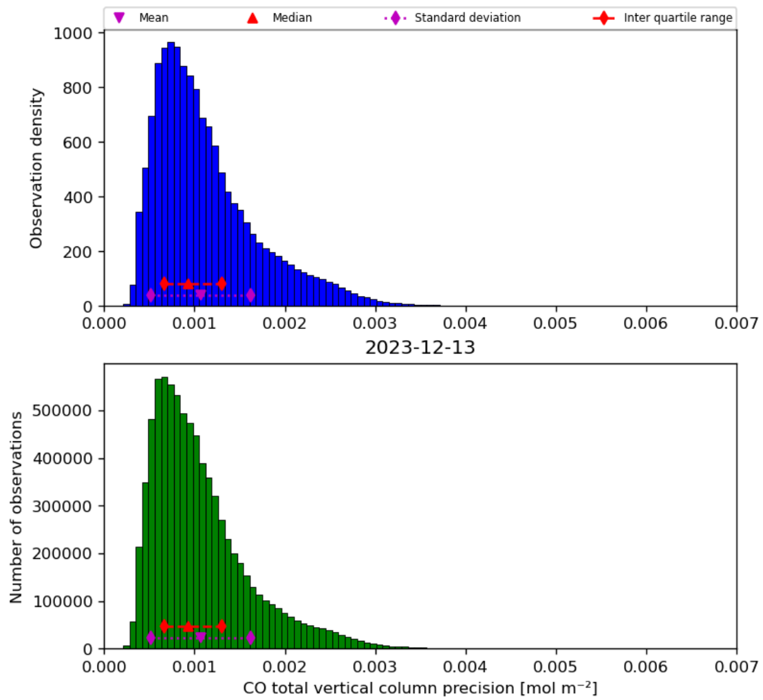
Figure 20: Histogram of “CO total vertical column precision” for 2023-12-12 to 2023-12-14
