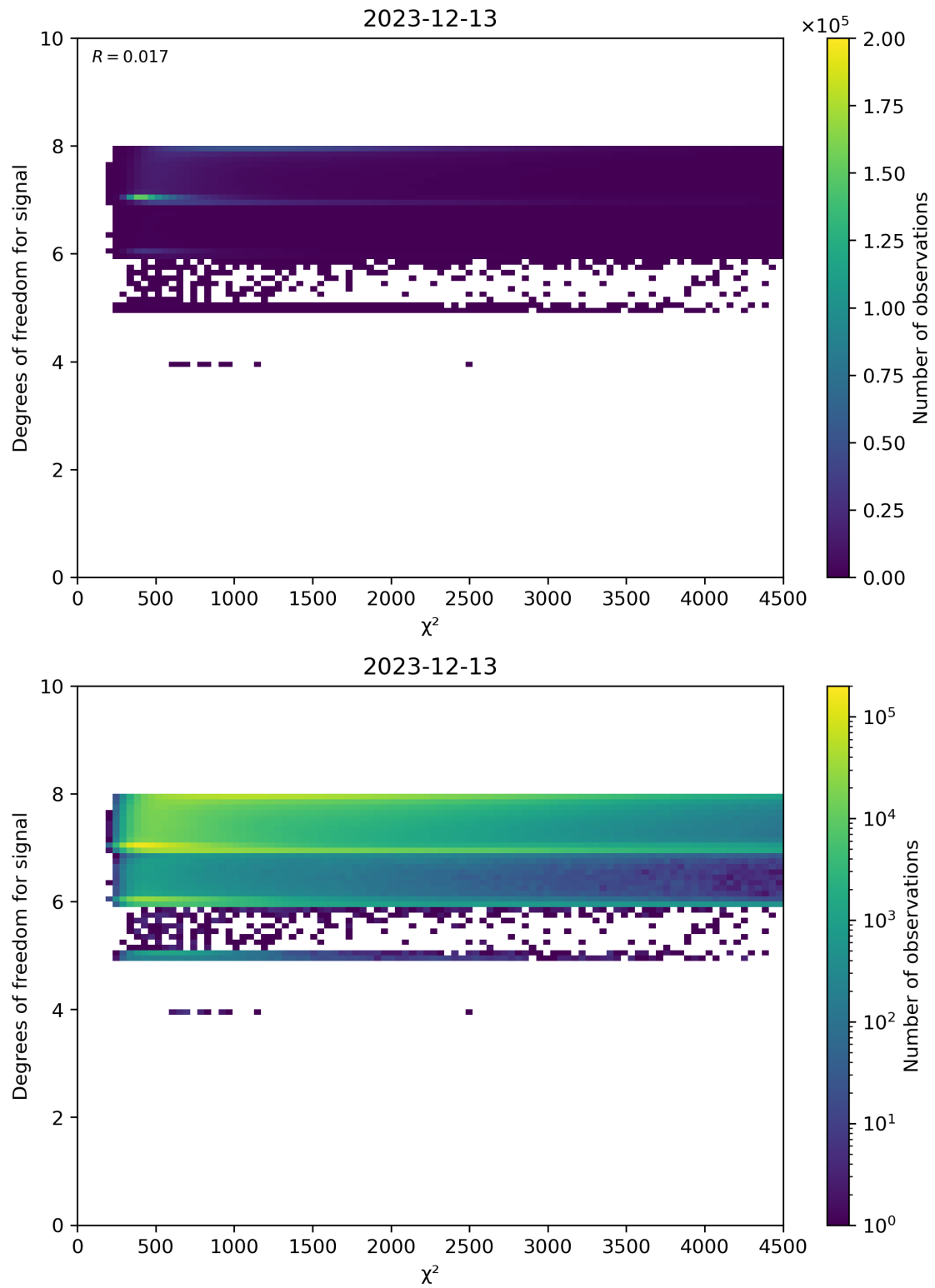
Figure 48: Scatter density plot of “ \chi^2 ” against “Degrees of freedom for signal” for 2023-12-12 to 2023-12-14.
