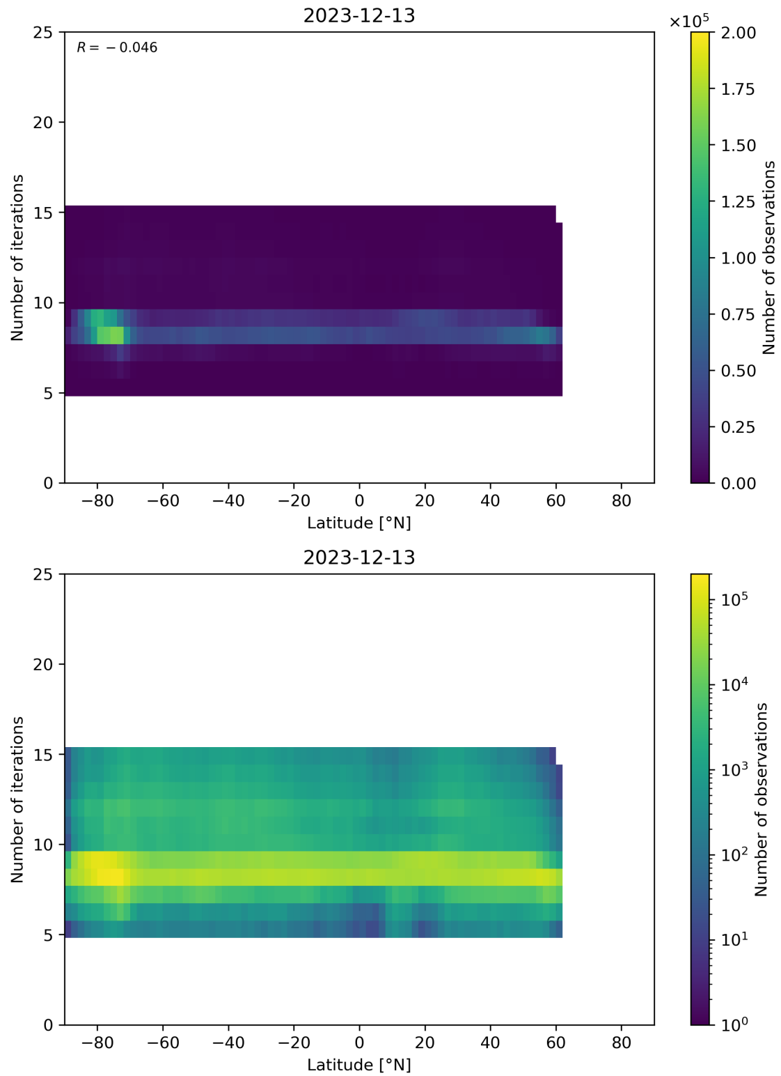
Figure 56: Scatter density plot of “Latitude” against “Number of iterations” for 2023-12-12 to 2023-12-14.
