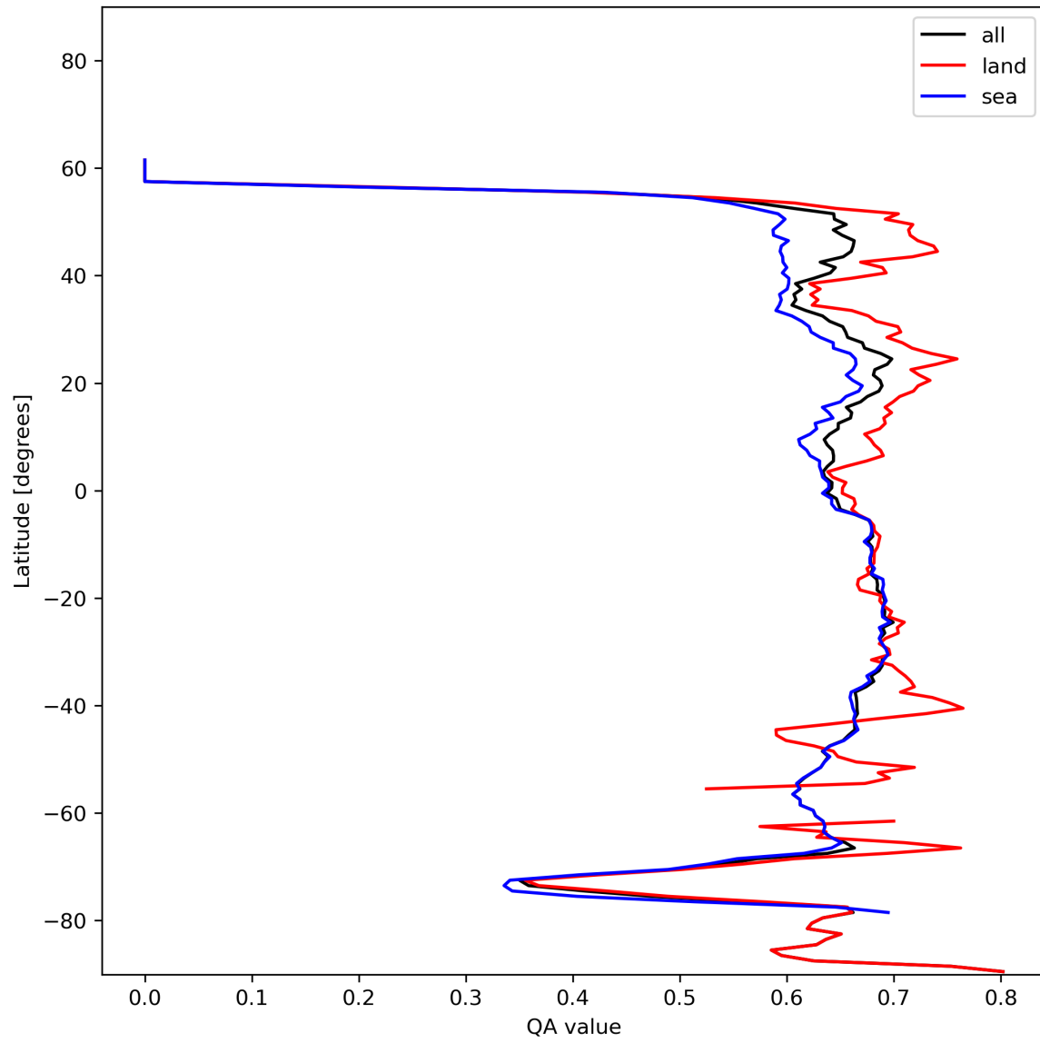
Figure 9: Zonal average of “QA value” for 2023-12-12 to 2023-12-14.
