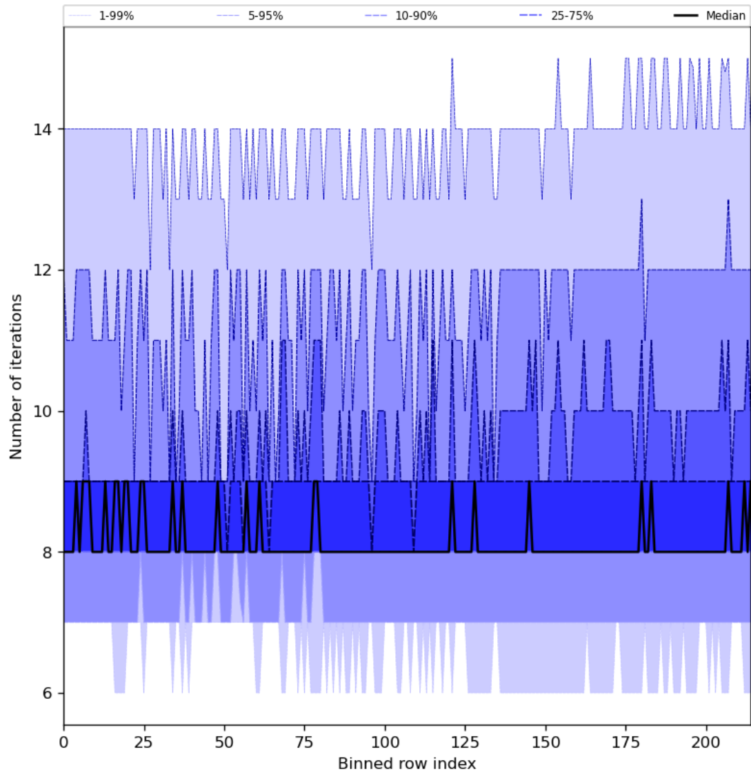
Figure 32: Along track statistics of “Number of iterations” for 2023-12-12 to 2023-12-14
