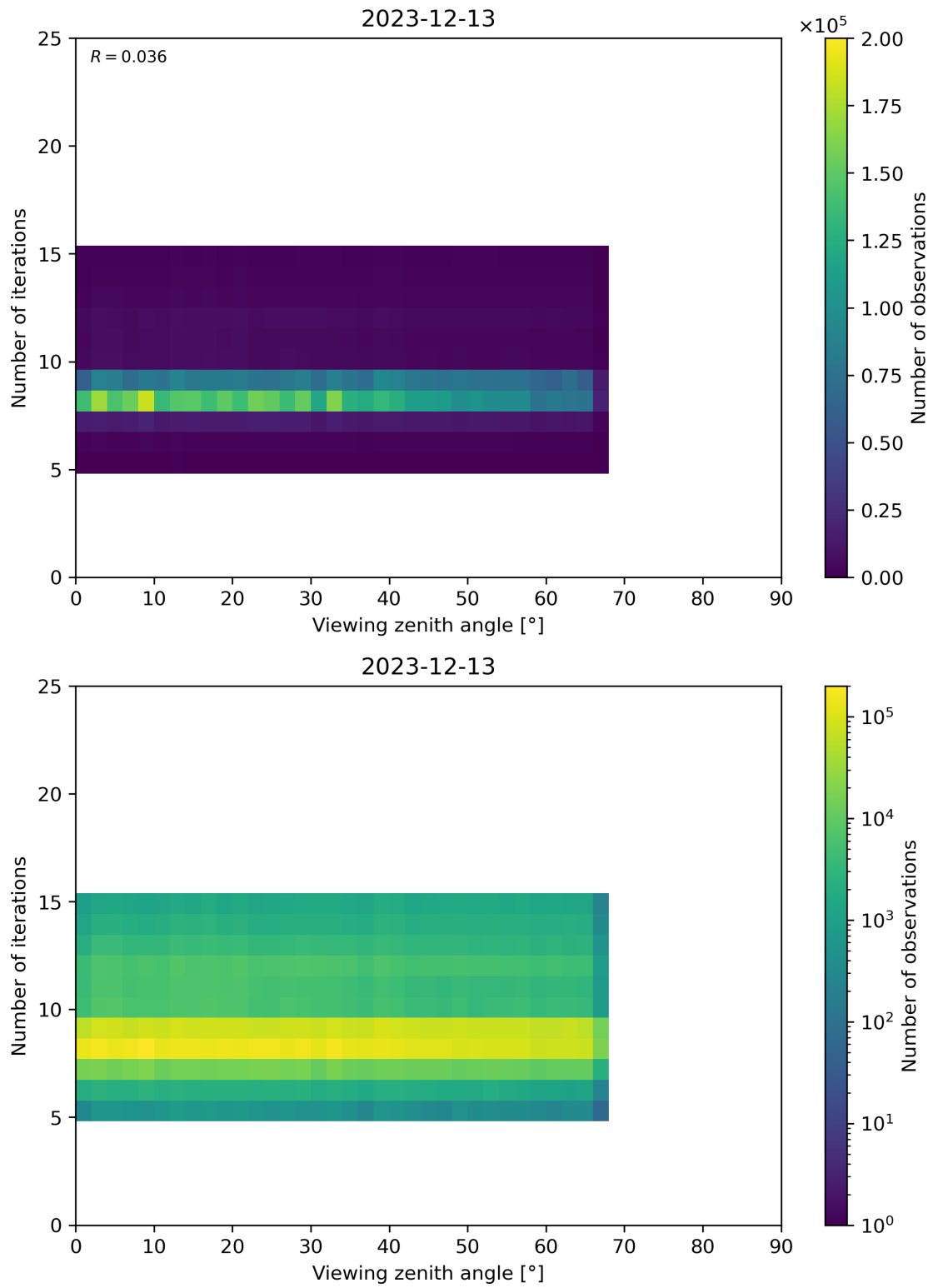
Figure 75: Scatter density plot of “Viewing zenith angle” against “Number of iterations” for 2023-12-12 to 2023-12-14.
