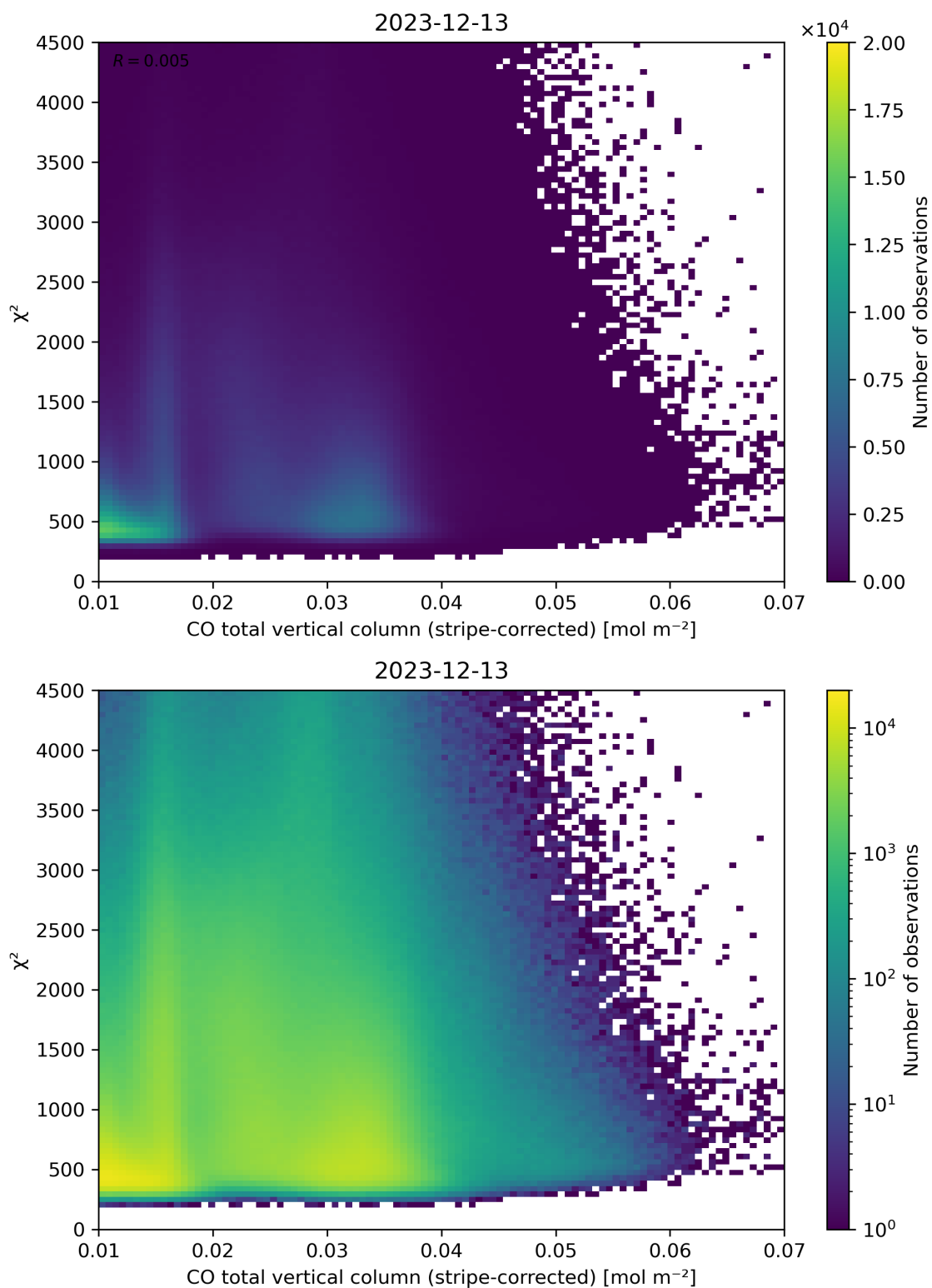
Figure 37: Scatter density plot of “CO total vertical column (stripe-corrected)” against “ \chi^2 ” for 2023-12-12 to 2023-12-14.
