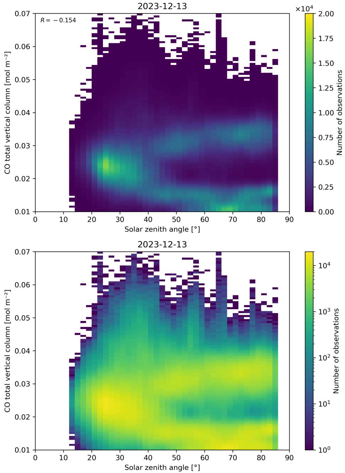
Figure 61: Scatter density plot of “Solar zenith angle” against “CO total vertical column” for 2023-12-12 to 2023-12-14.
