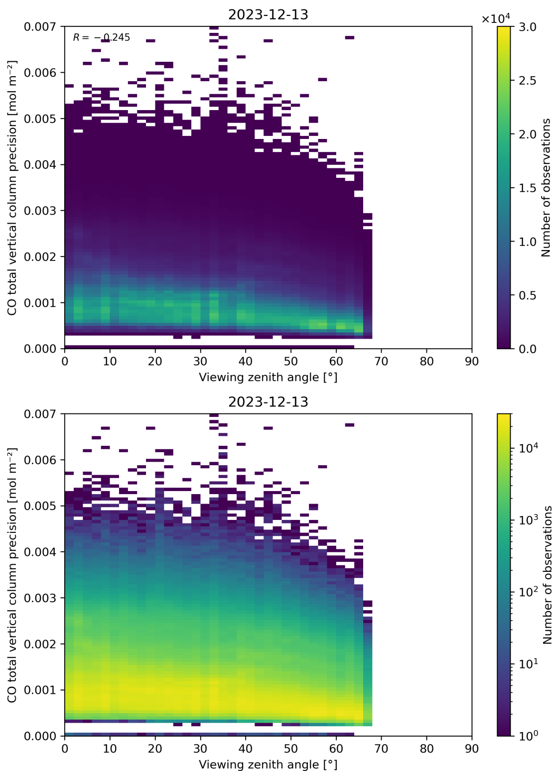
Figure 71: Scatter density plot of “Viewing zenith angle” against “CO total vertical column precision” for 2023-12-12 to 2023-12-14.
