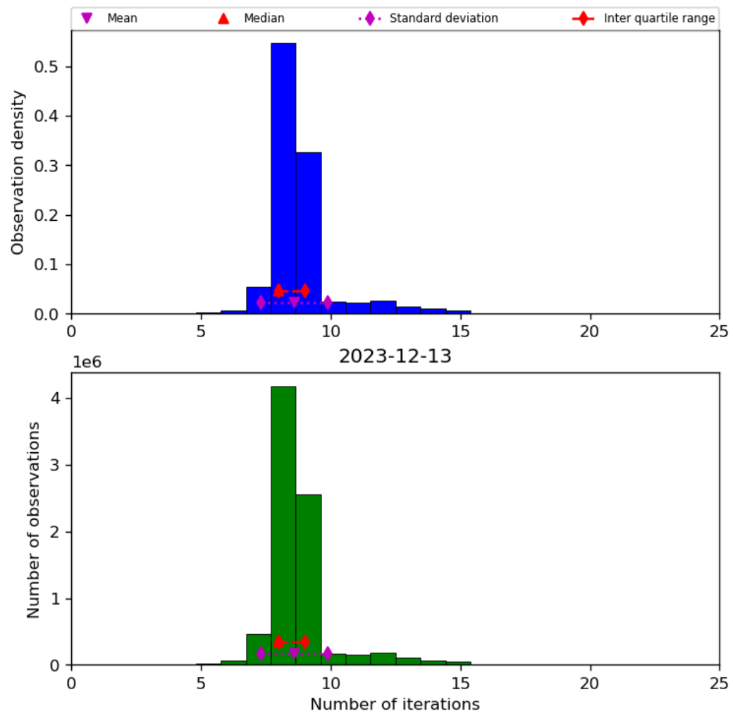
Figure 24: Histogram of “Number of iterations” for 2023-12-12 to 2023-12-14
