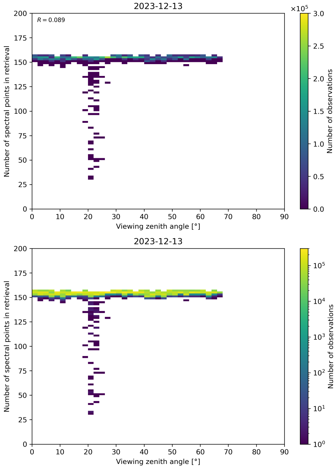
Figure 76: Scatter density plot of “Viewing zenith angle” against “Number of spectral points in retrieval” for 2023-12-12 to 2023-12-14.
