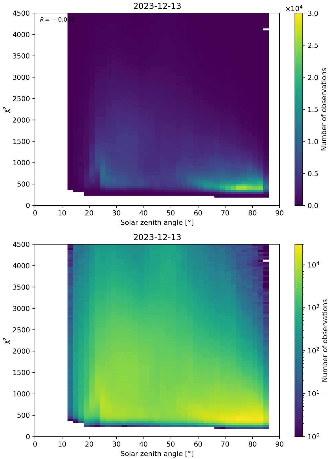
Figure 64: Scatter density plot of “Solar zenith angle” against “ \chi^2 ” for 2023-12-12 to 2023-12-14.
