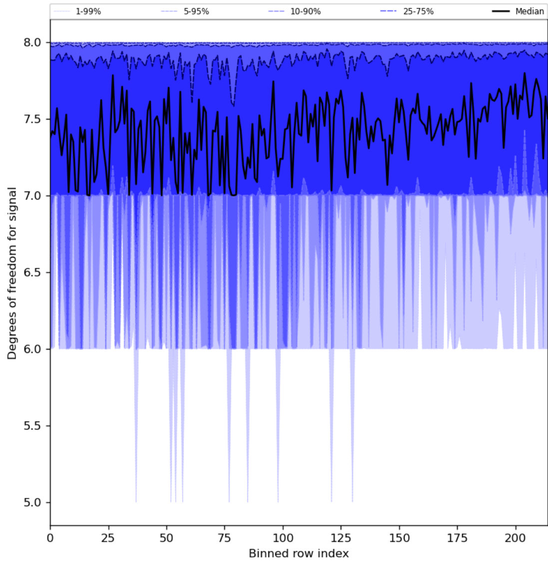
Figure 31: Along track statistics of “Degrees of freedom for signal” for 2023-12-12 to 2023-12-14
