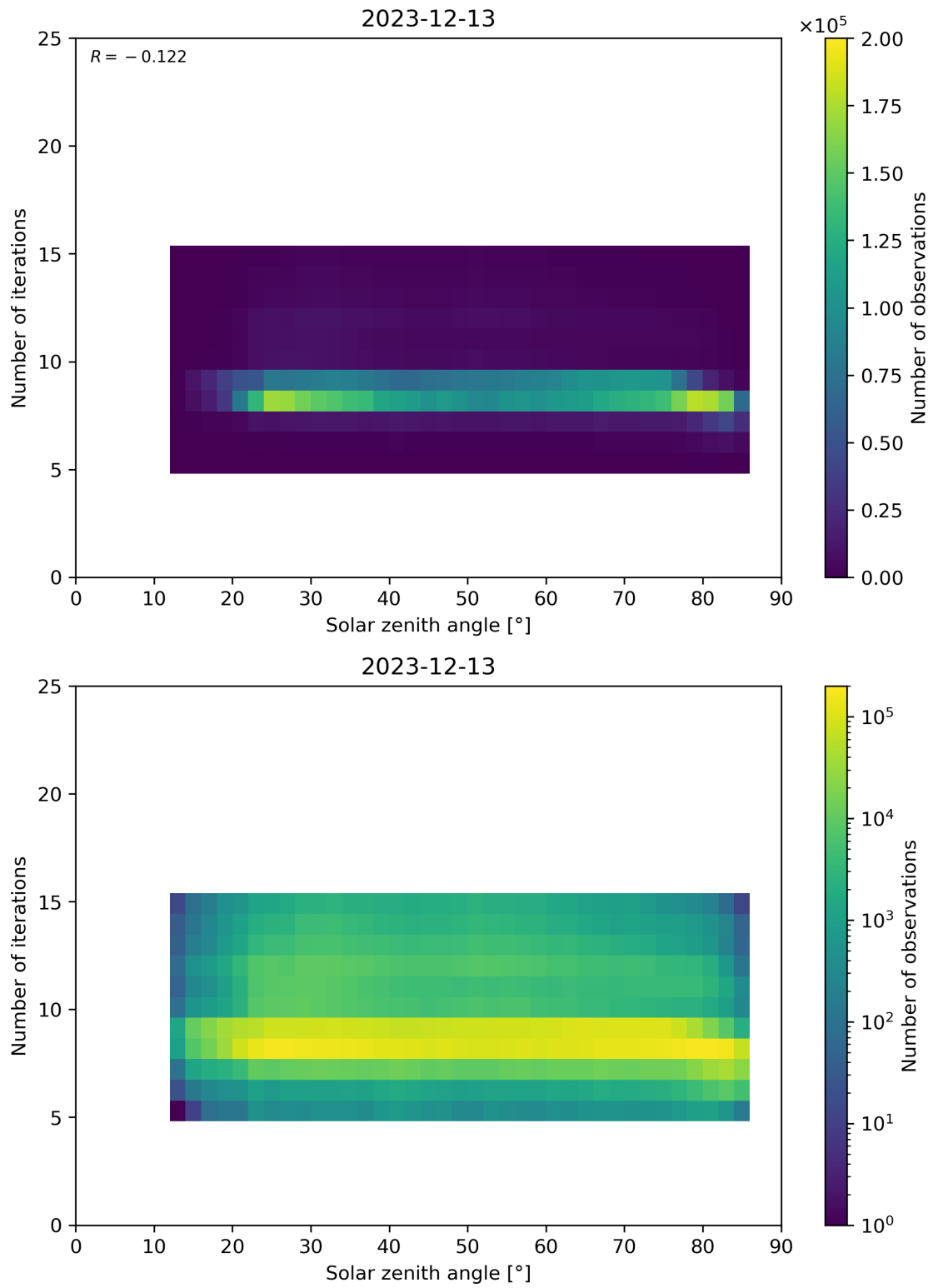
Figure 67: Scatter density plot of “Solar zenith angle” against “Number of iterations” for 2023-12-12 to 2023-12-14.
