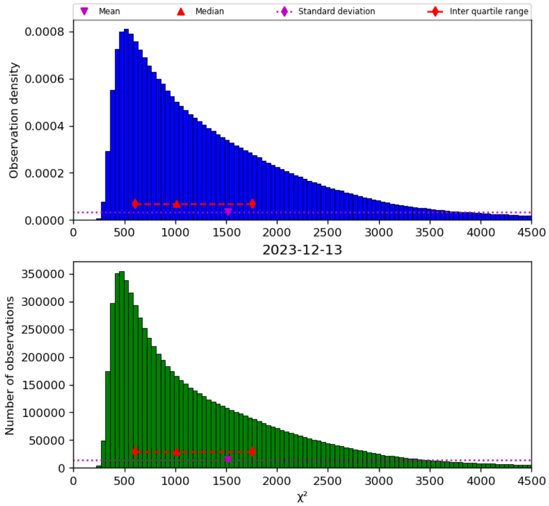
Figure 22: Histogram of “ \chi^2 ” for 2023-12-12 to 2023-12-14
