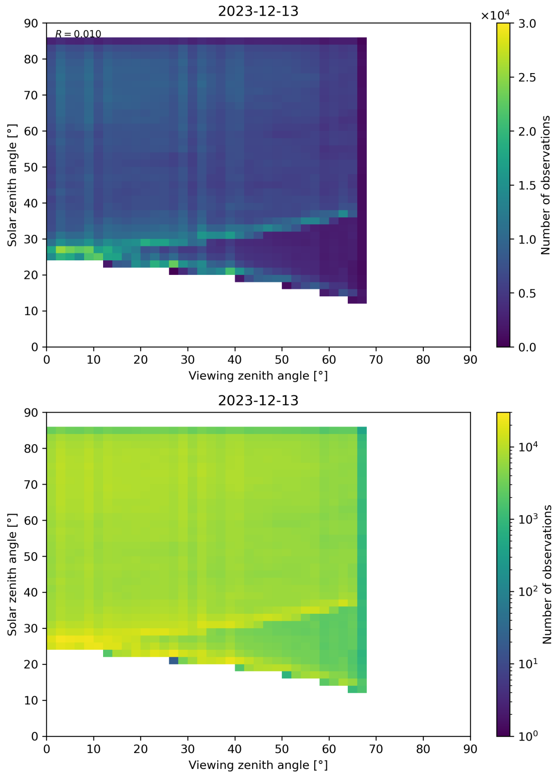
Figure 77: Scatter density plot of “Viewing zenith angle” against “Solar zenith angle” for 2023-12-12 to 2023-12-14.
