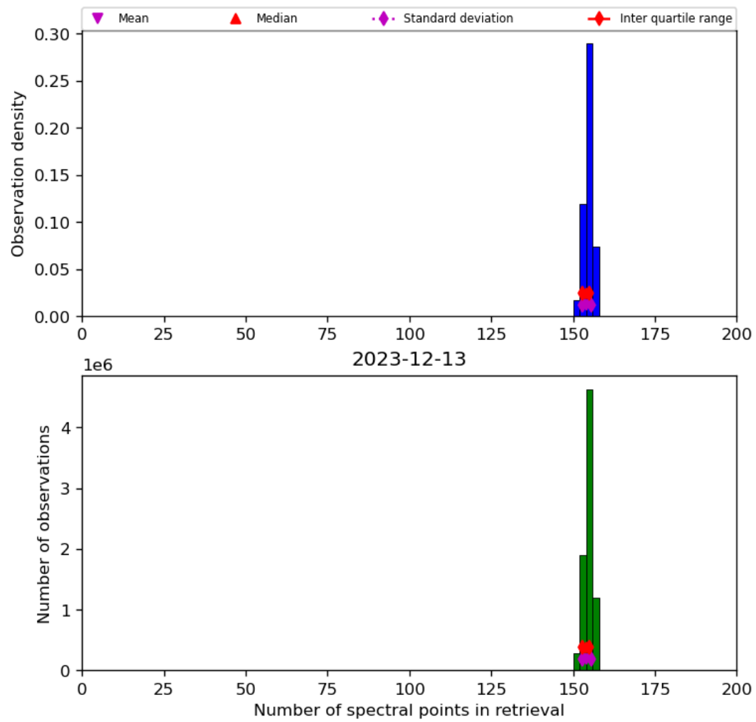
Figure 21: Histogram of “Number of spectral points in retrieval” for 2023-12-12 to 2023-12-14
