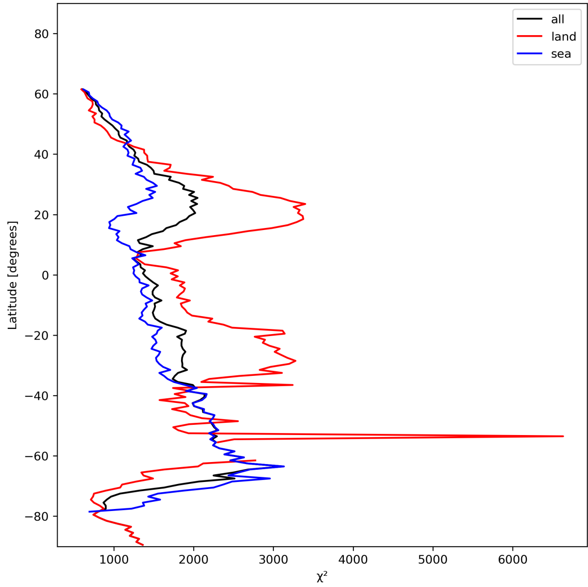
Figure 14: Zonal average of “ \chi^2 ” for 2023-12-12 to 2023-12-14.
