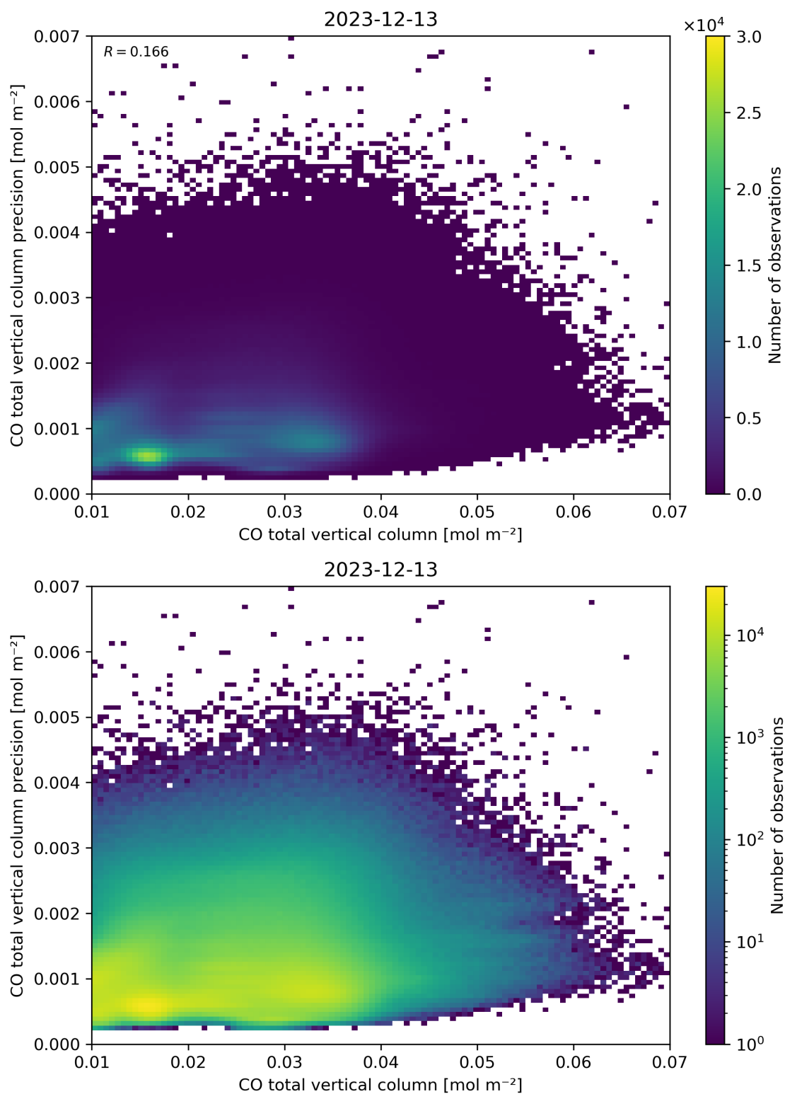
Figure 34: Scatter density plot of “CO total vertical column” against “CO total vertical column precision” for 2023-12-12 to 2023-12-14.
