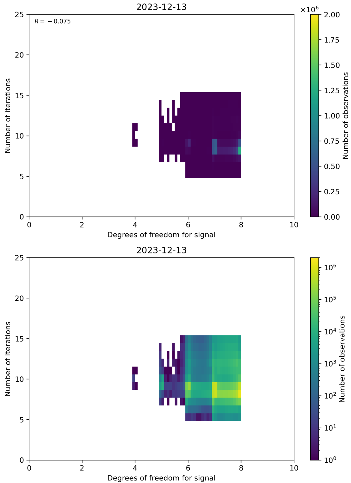
Figure 50: Scatter density plot of “Degrees of freedom for signal” against “Number of iterations” for 2023-12-12 to 2023-12-14.
