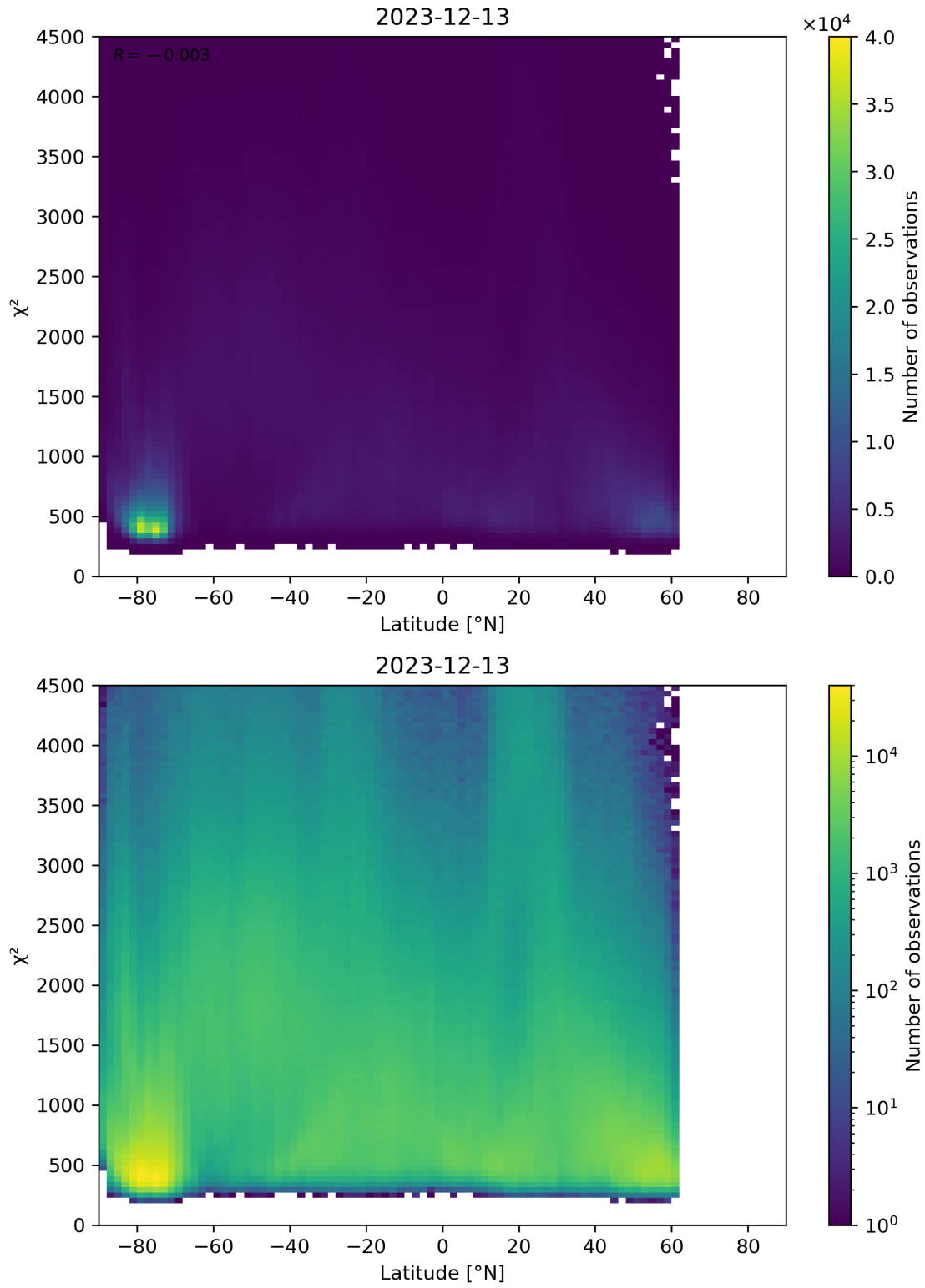
Figure 54: Scatter density plot of “Latitude” against “ \chi^2 ” for 2023-12-12 to 2023-12-14.
