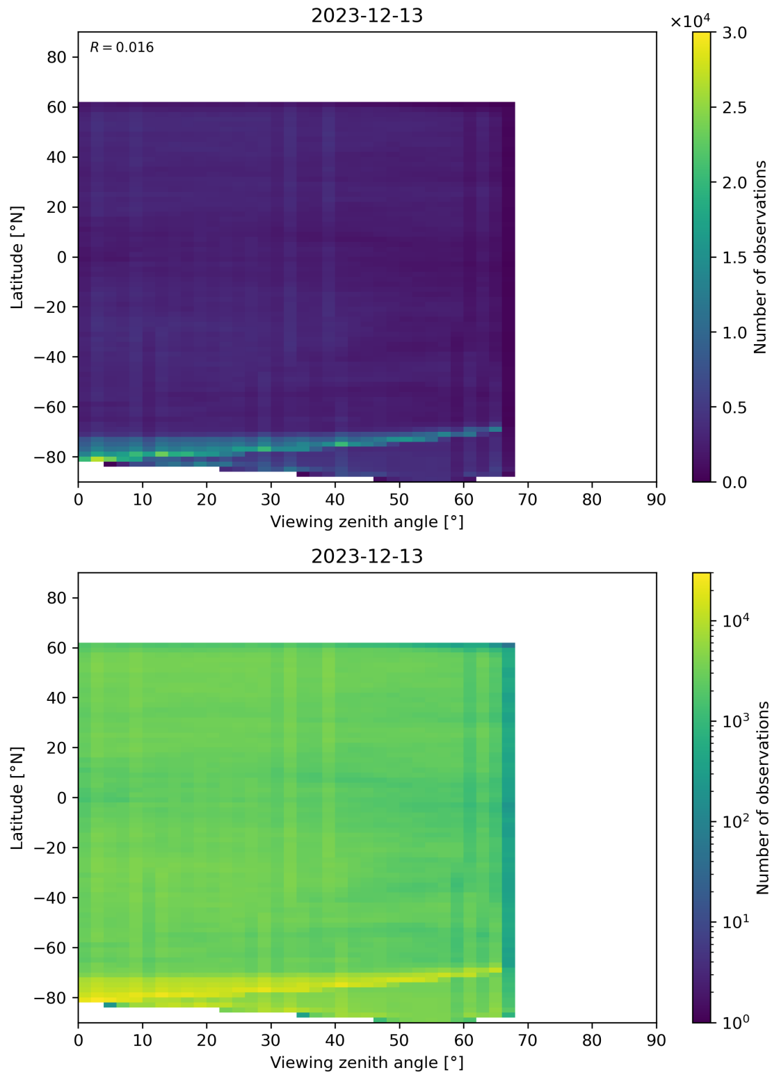
Figure 74: Scatter density plot of “Viewing zenith angle” against “Latitude” for 2023-12-12 to 2023-12-14.
