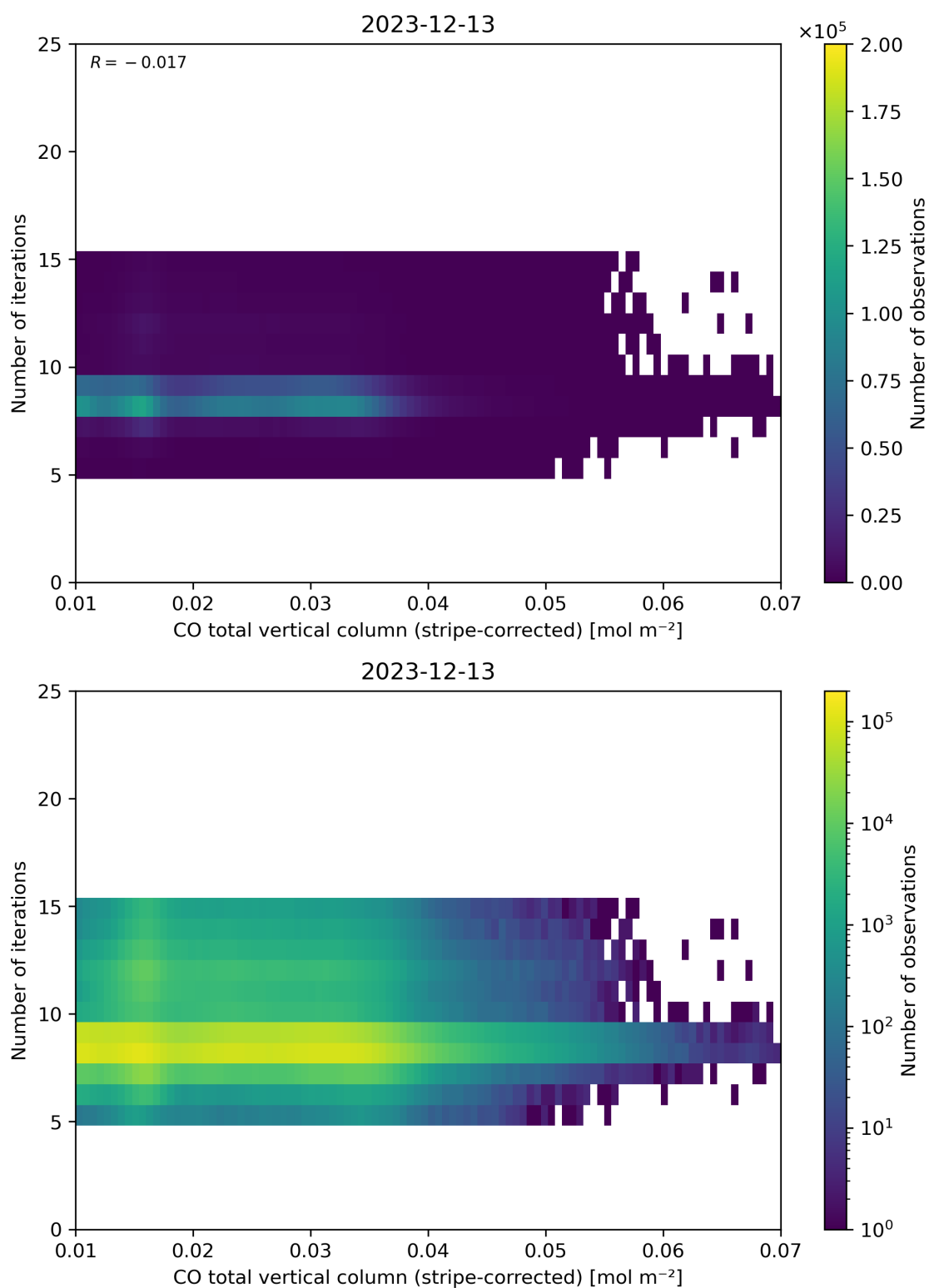
Figure 39: Scatter density plot of “CO total vertical column (stripe-corrected)” against “Number of iterations” for 2023-12-12 to 2023-12-14.
