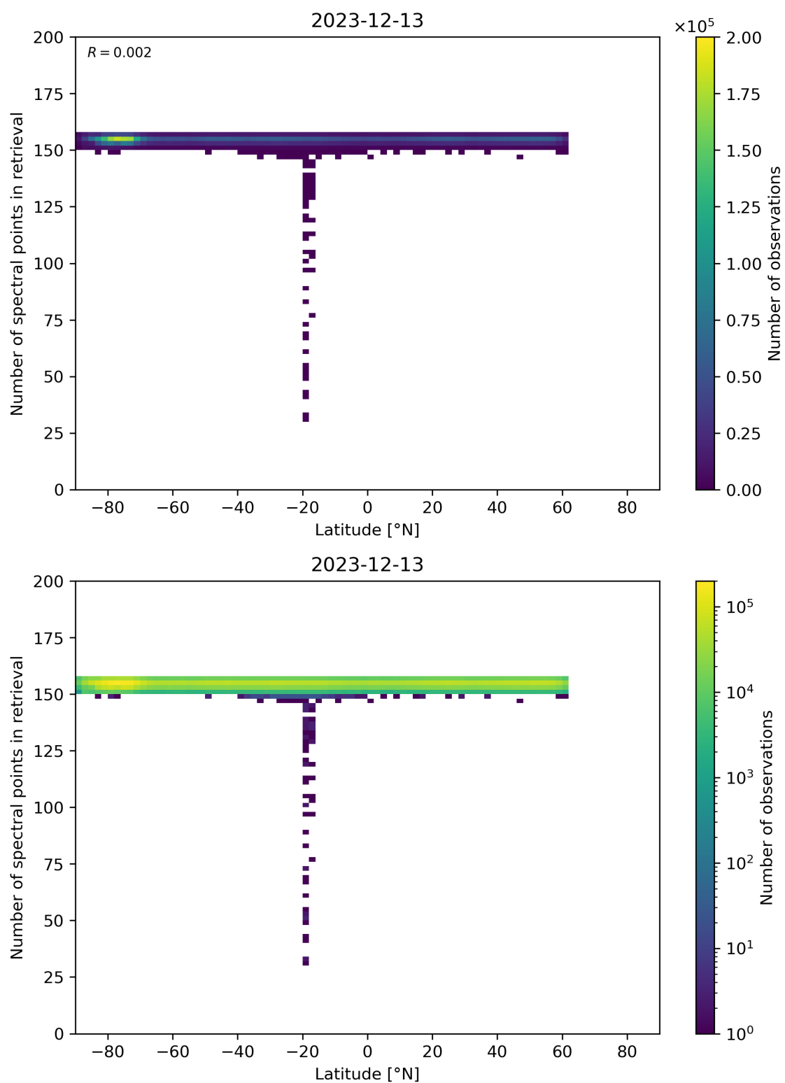
Figure 57: Scatter density plot of “Latitude” against “Number of spectral points in retrieval” for 2023-12-12 to 2023-12-14.
