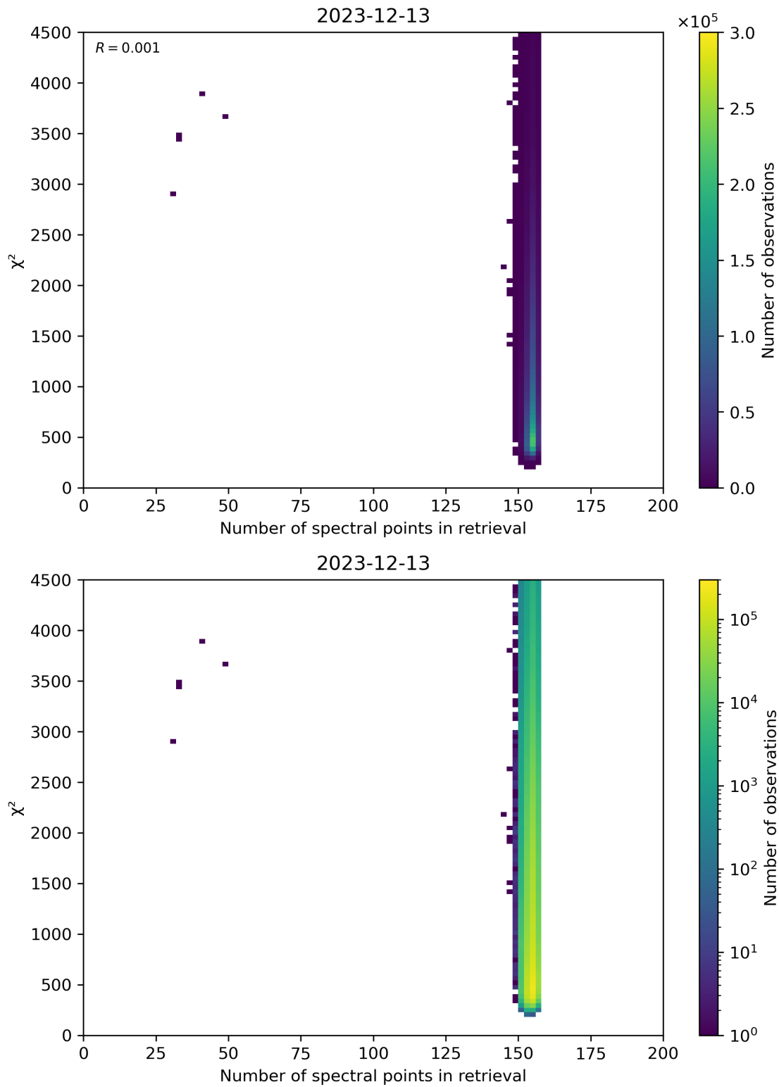
Figure 58: Scatter density plot of “Number of spectral points in retrieval” against “ \chi^2 ” for 2023-12-12 to 2023-12-14.
