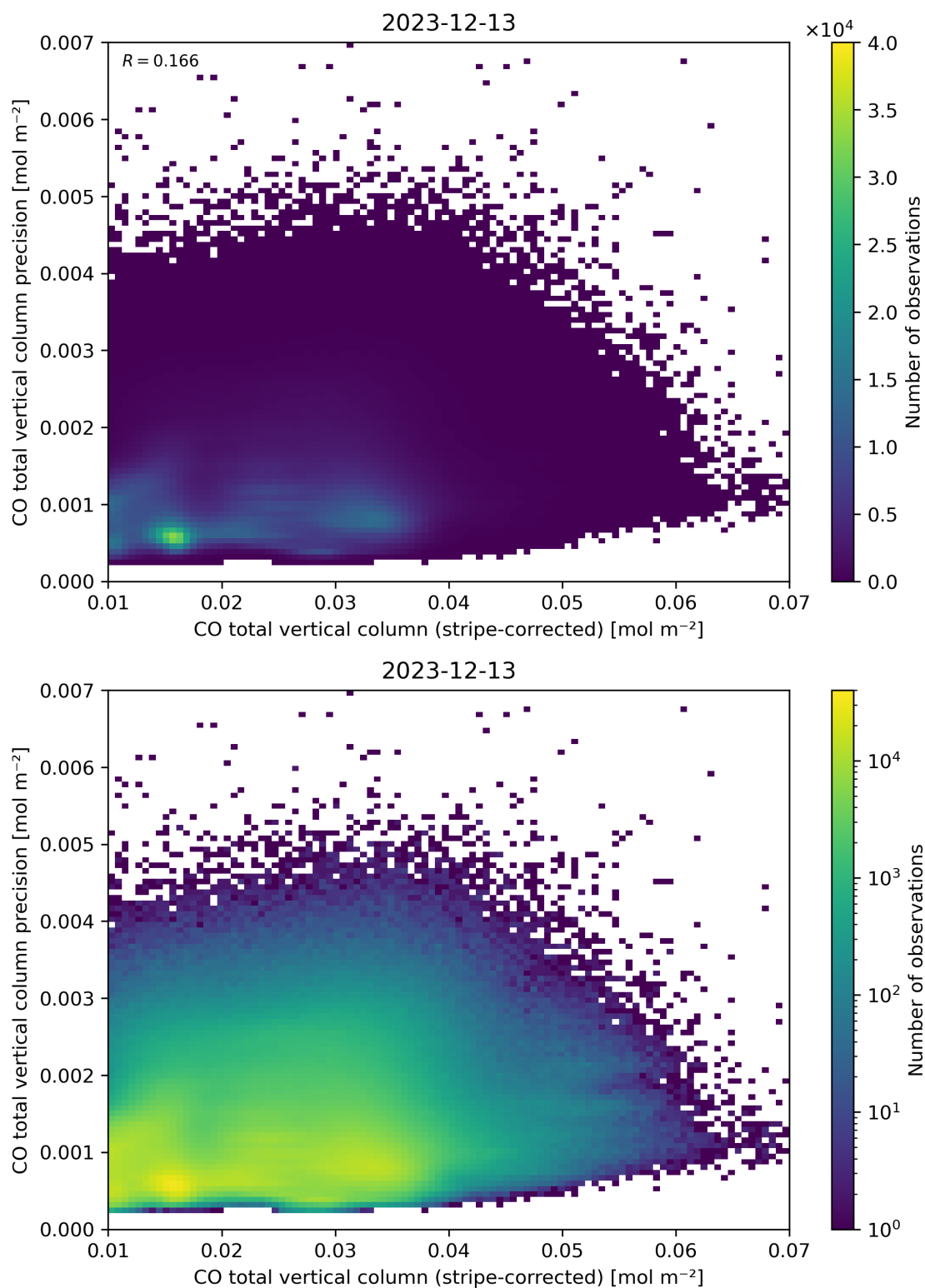
Figure 36: Scatter density plot of “CO total vertical column (stripe-corrected)” against “CO total vertical column precision” for 2023-12-12 to 2023-12-14.
