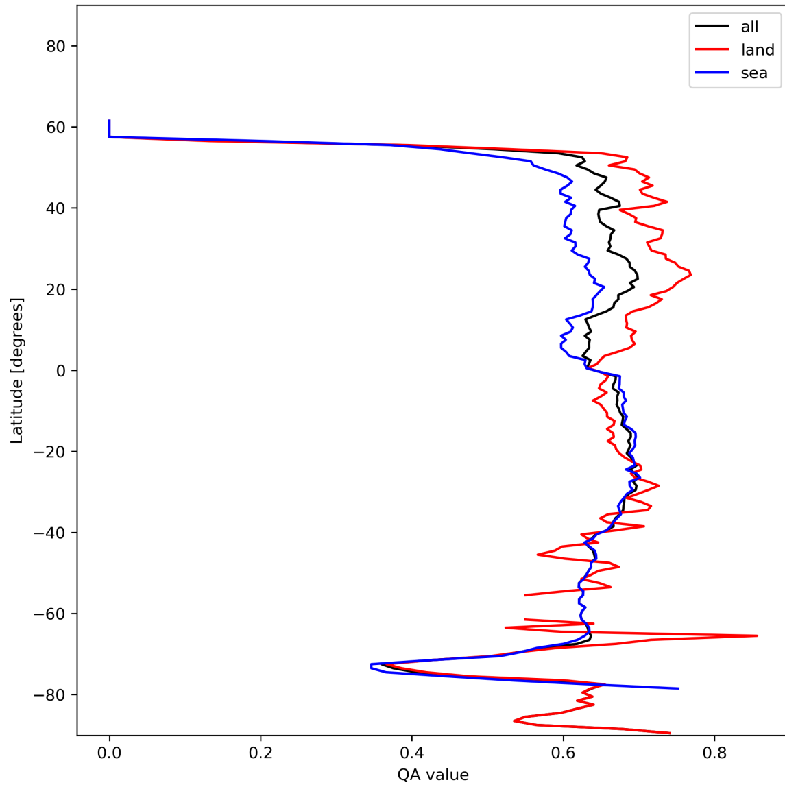
Figure 9: Zonal average of “QA value” for 2023-12-14 to 2023-12-16.
