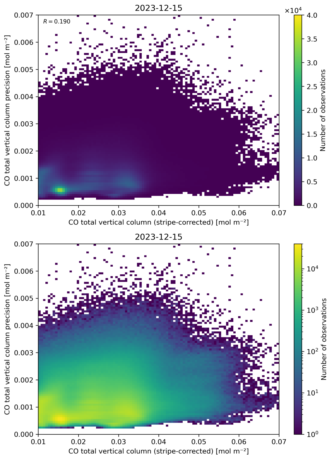
Figure 36: Scatter density plot of “CO total vertical column (stripe-corrected)” against “CO total vertical column precision” for 2023-12-14 to 2023-12-16.
