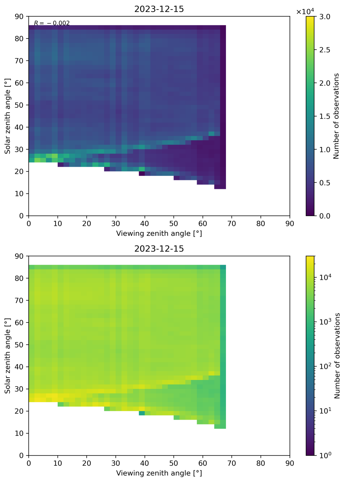
Figure 77: Scatter density plot of “Viewing zenith angle” against “Solar zenith angle” for 2023-12-14 to 2023-12-16.
