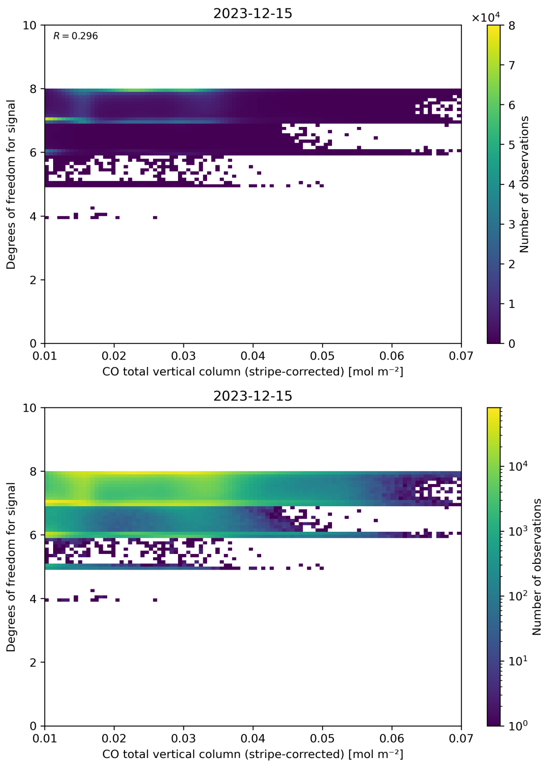
Figure 38: Scatter density plot of “CO total vertical column (stripe-corrected)” against “Degrees of freedom for signal” for 2023-12-14 to 2023-12-16.
