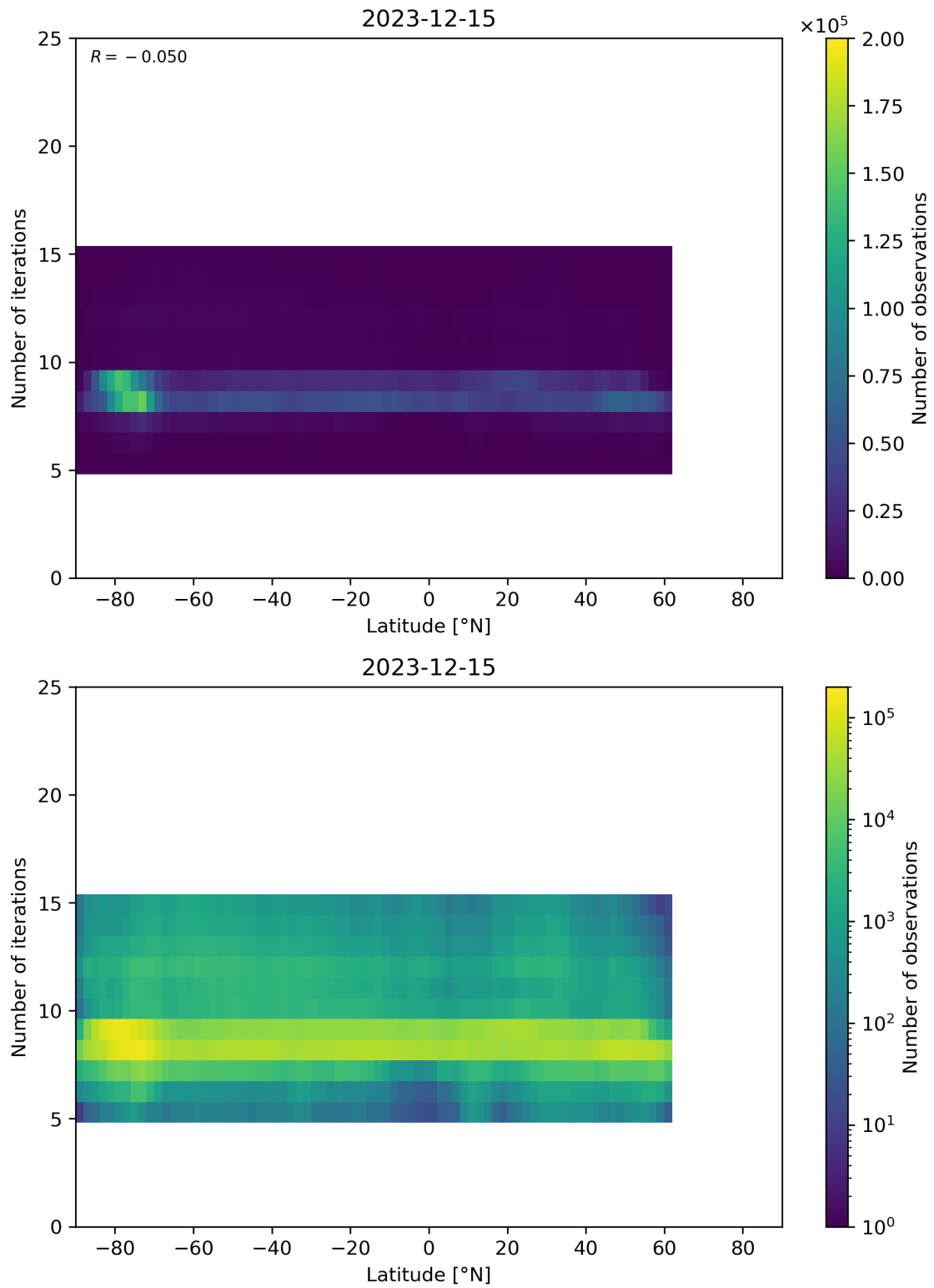
Figure 56: Scatter density plot of “Latitude” against “Number of iterations” for 2023-12-14 to 2023-12-16.
