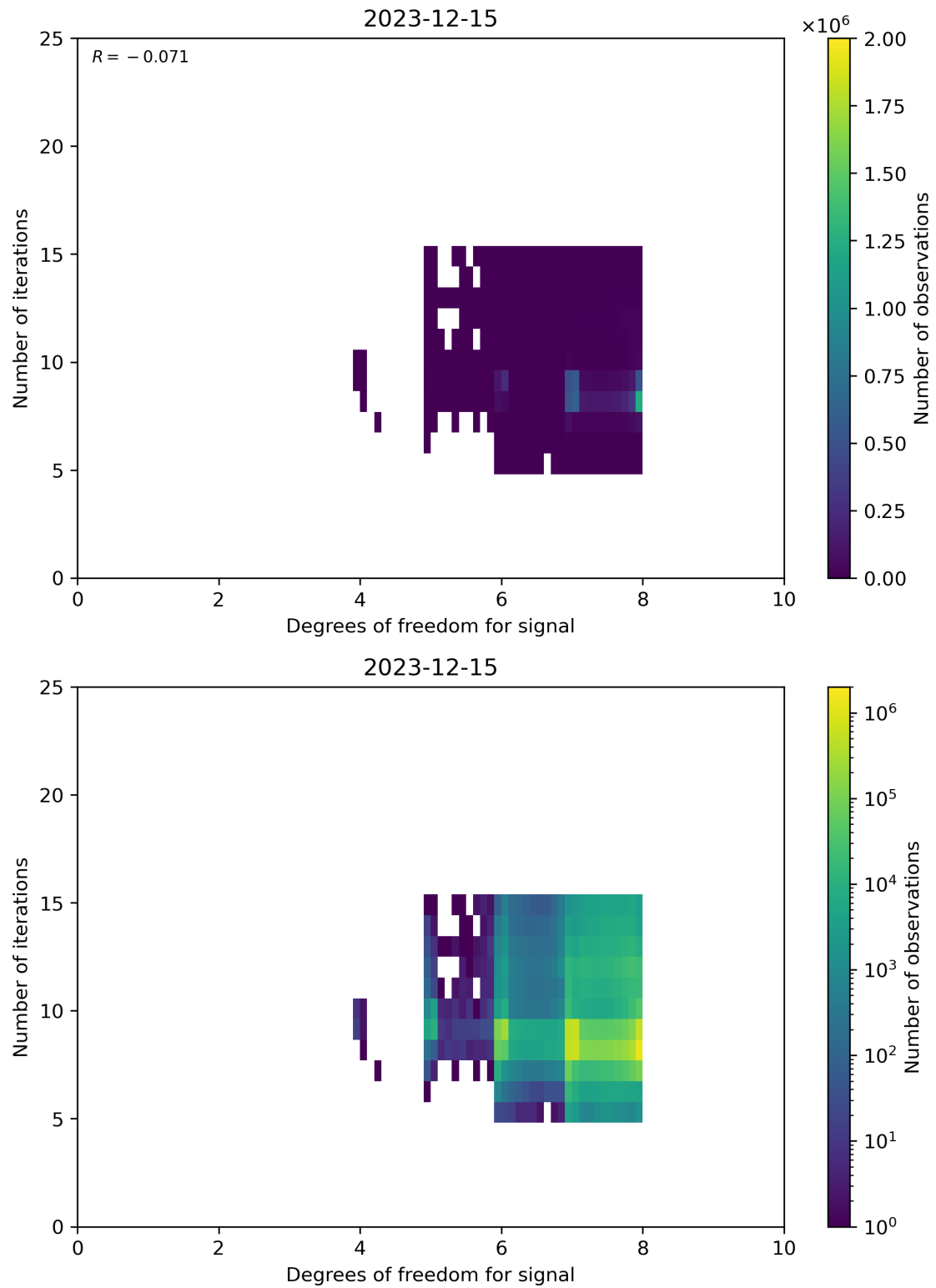
Figure 50: Scatter density plot of “Degrees of freedom for signal” against “Number of iterations” for 2023-12-14 to 2023-12-16.
