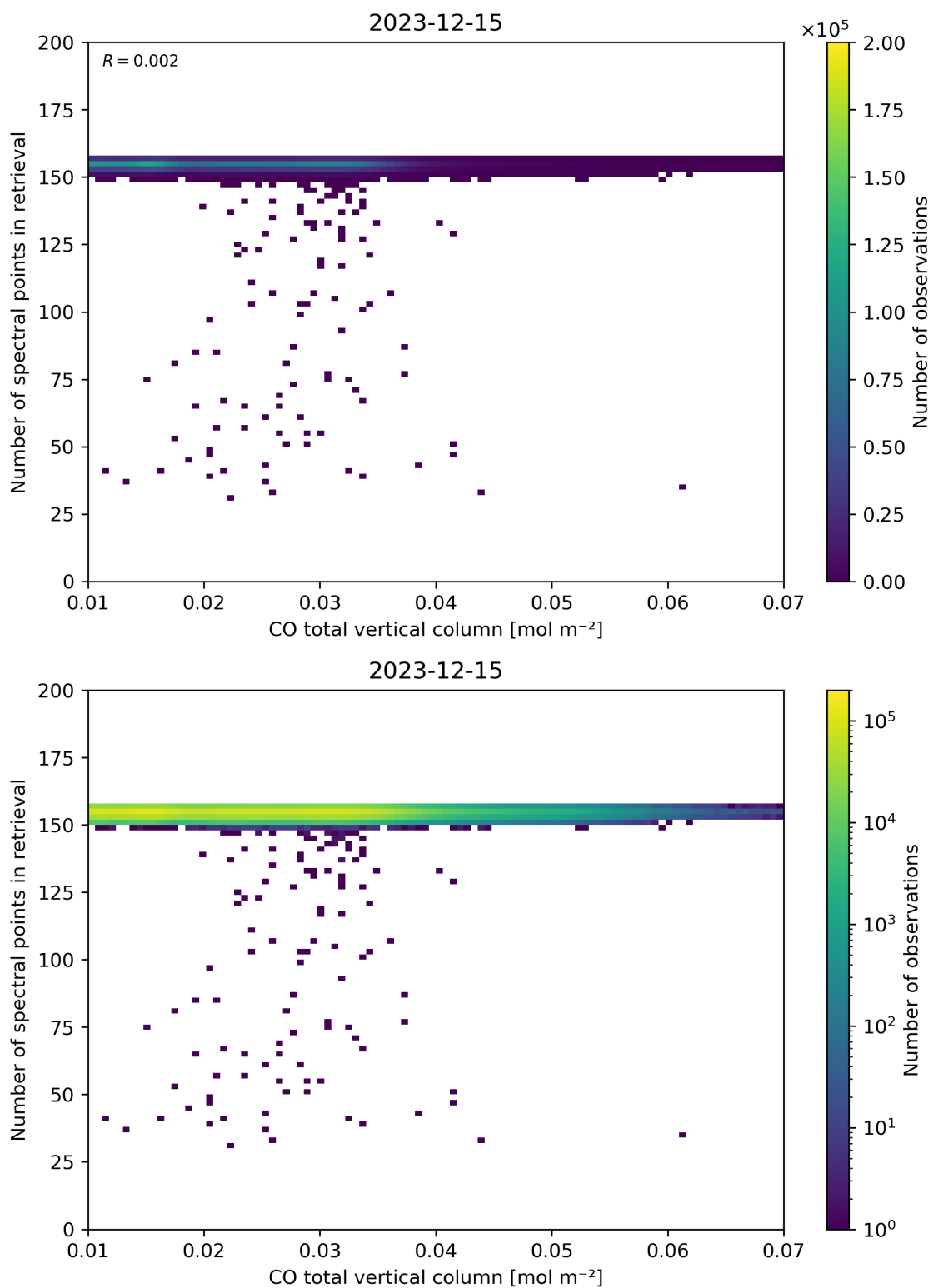
Figure 43: Scatter density plot of “CO total vertical column” against “Number of spectral points in retrieval” for 2023-12-14 to 2023-12-16.
