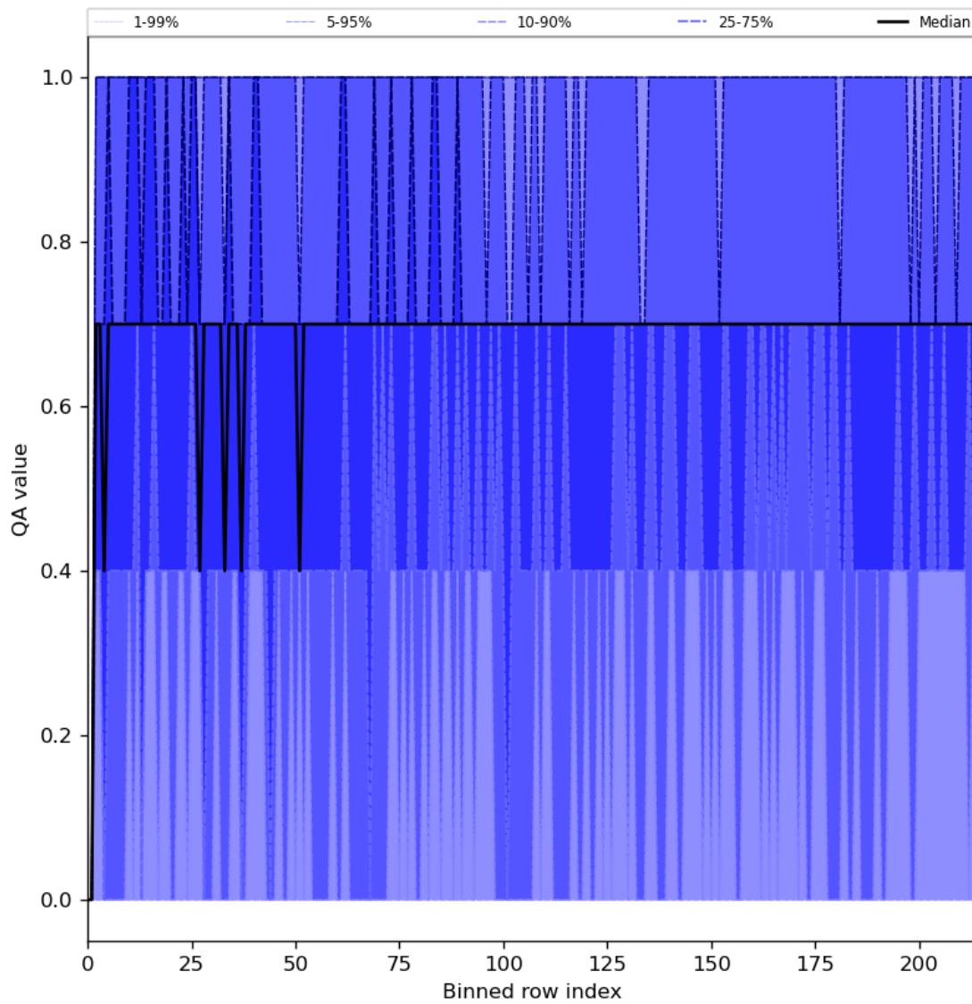
Figure 25: Along track statistics of “QA value” for 2023-12-14 to 2023-12-16
