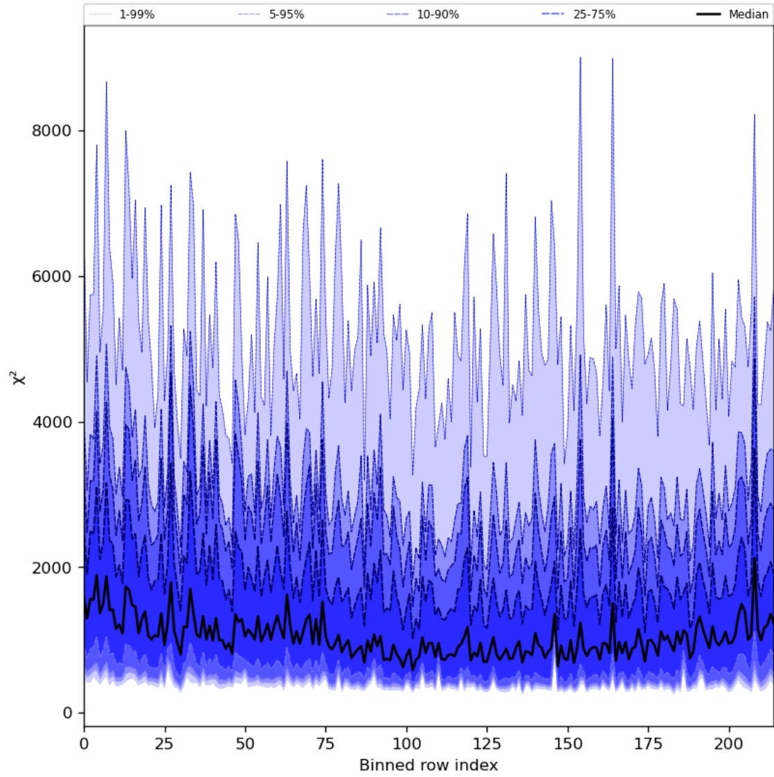
Figure 30: Along track statistics of “ \chi^2 ” for 2023-12-14 to 2023-12-16
