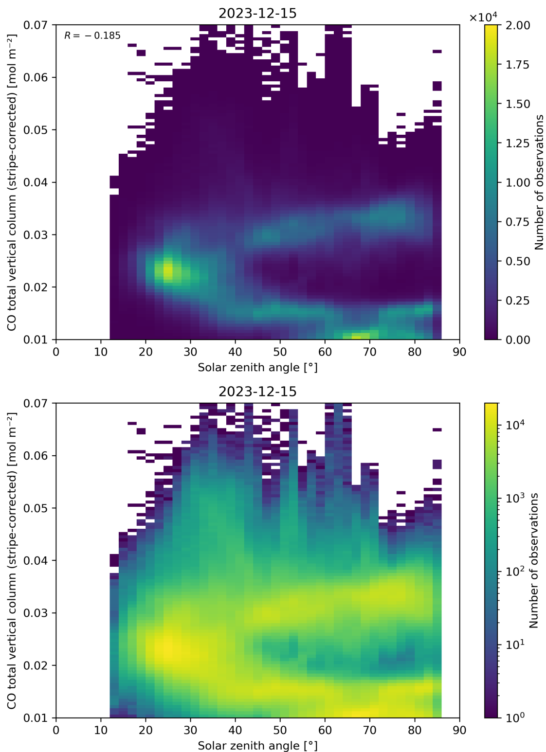
Figure 62: Scatter density plot of “Solar zenith angle” against “CO total vertical column (stripe-corrected)” for 2023-12-14 to 2023-12-16.
