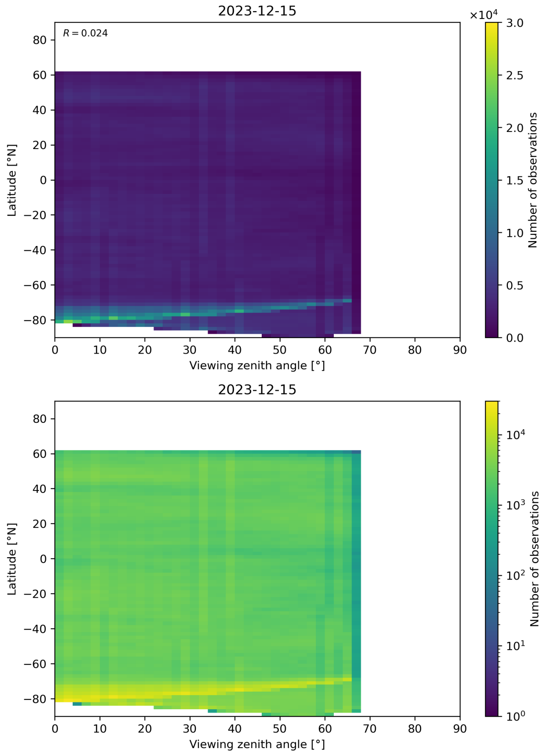
Figure 74: Scatter density plot of “Viewing zenith angle” against “Latitude” for 2023-12-14 to 2023-12-16.
