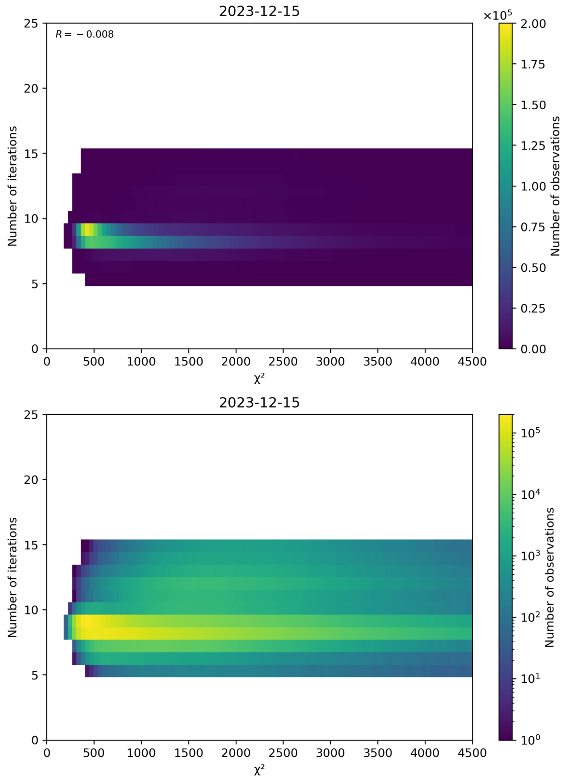
Figure 49: Scatter density plot of “ \chi^2 ” against “Number of iterations” for 2023-12-14 to 2023-12-16.
