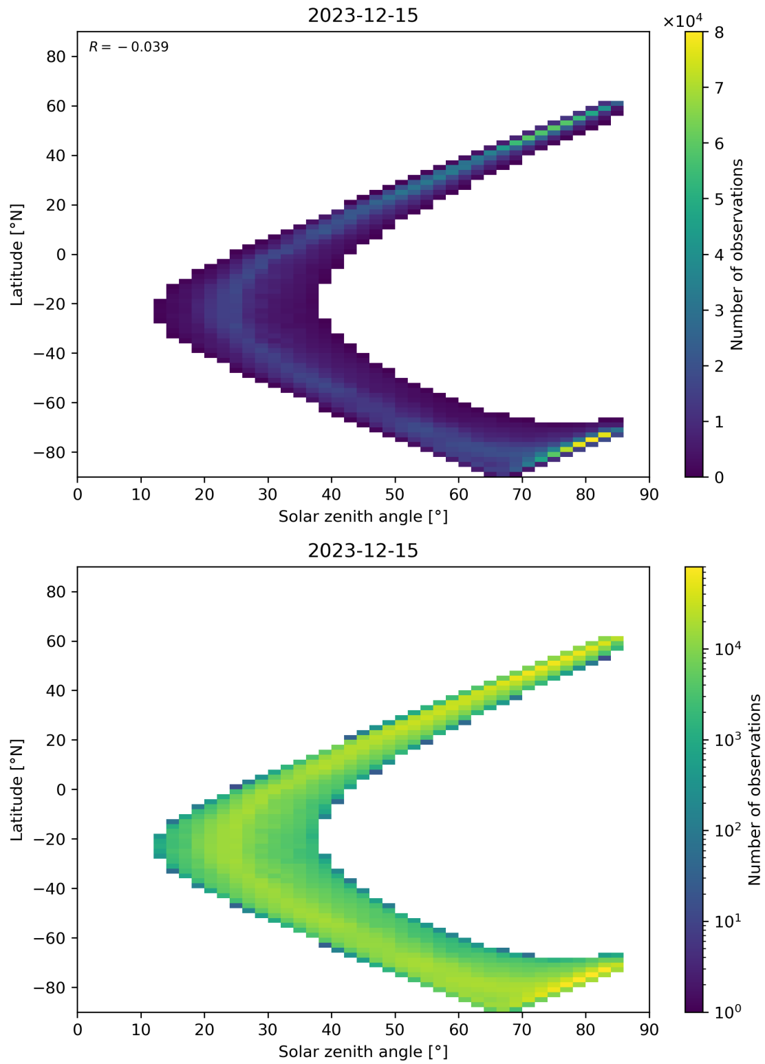
Figure 66: Scatter density plot of “Solar zenith angle” against “Latitude” for 2023-12-14 to 2023-12-16.
