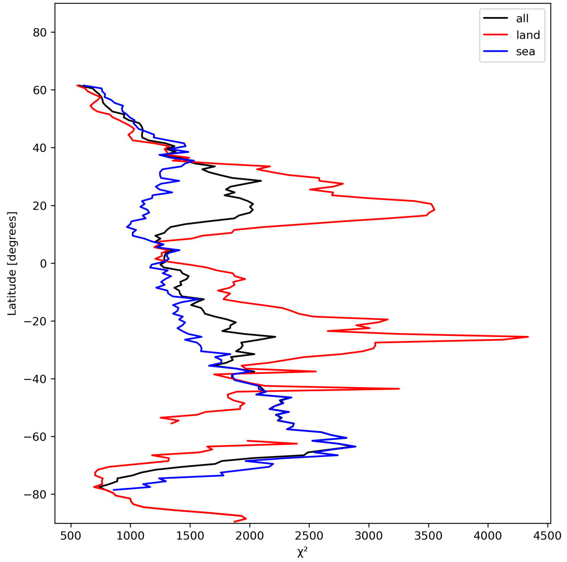
Figure 14: Zonal average of “ \chi^2 ” for 2023-12-14 to 2023-12-16.
