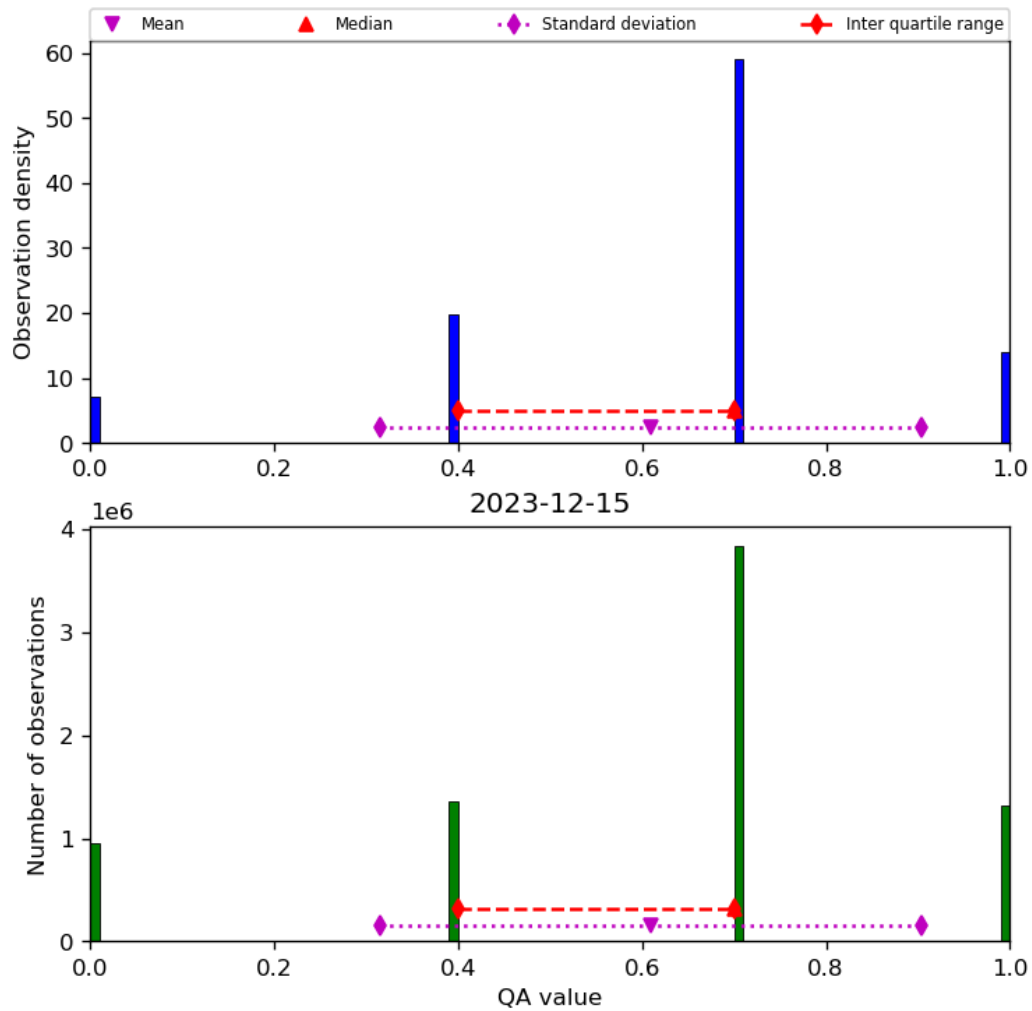
Figure 17: Histogram of “QA value” for 2023-12-14 to 2023-12-16
