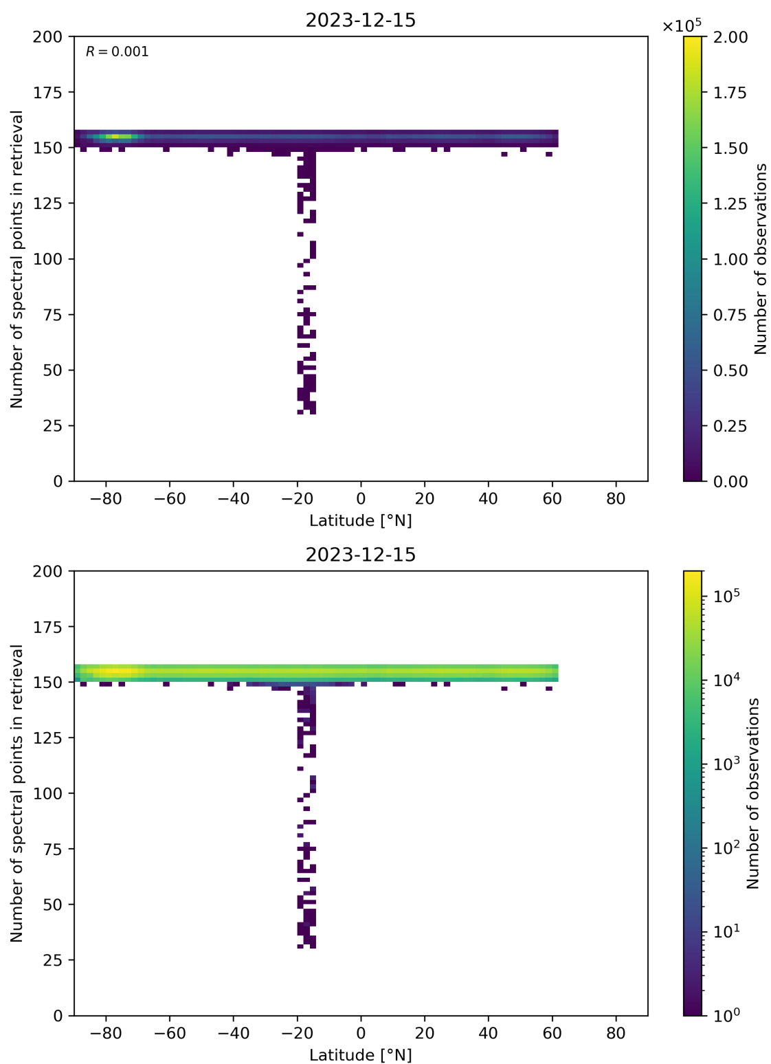
Figure 57: Scatter density plot of “Latitude” against “Number of spectral points in retrieval” for 2023-12-14 to 2023-12-16.
