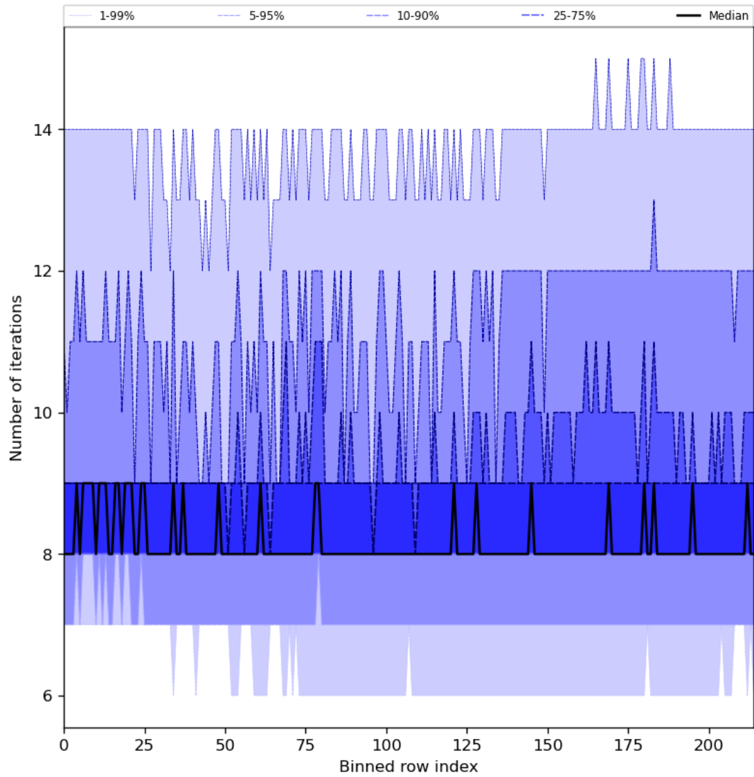
Figure 32: Along track statistics of “Number of iterations” for 2023-12-14 to 2023-12-16
