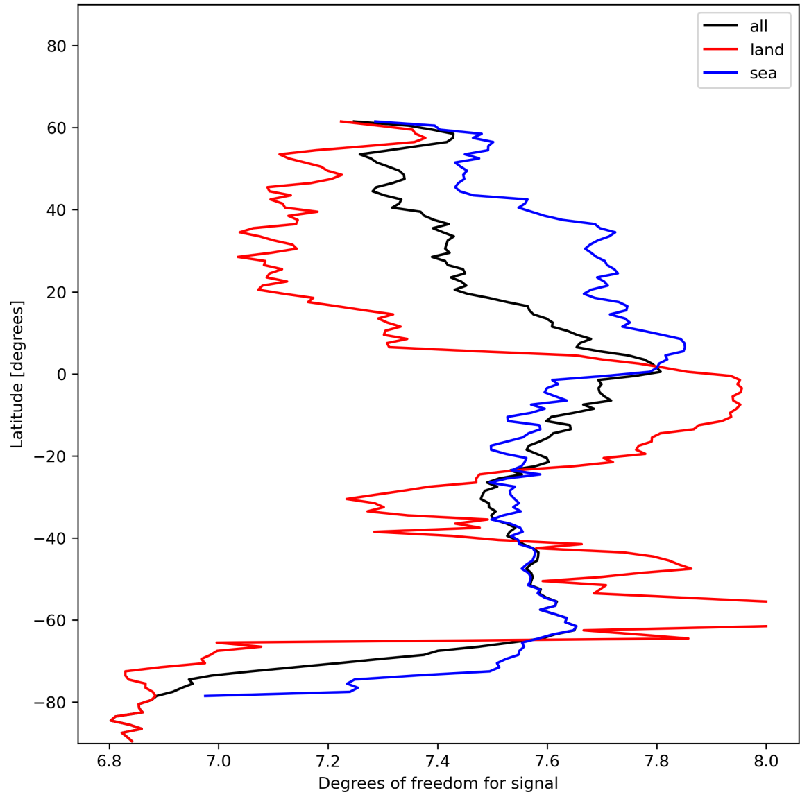
Figure 15: Zonal average of “Degrees of freedom for signal” for 2023-12-14 to 2023-12-16.
