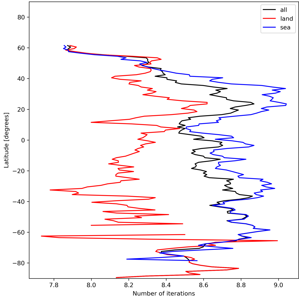
Figure 16: Zonal average of “Number of iterations” for 2023-12-14 to 2023-12-16.
