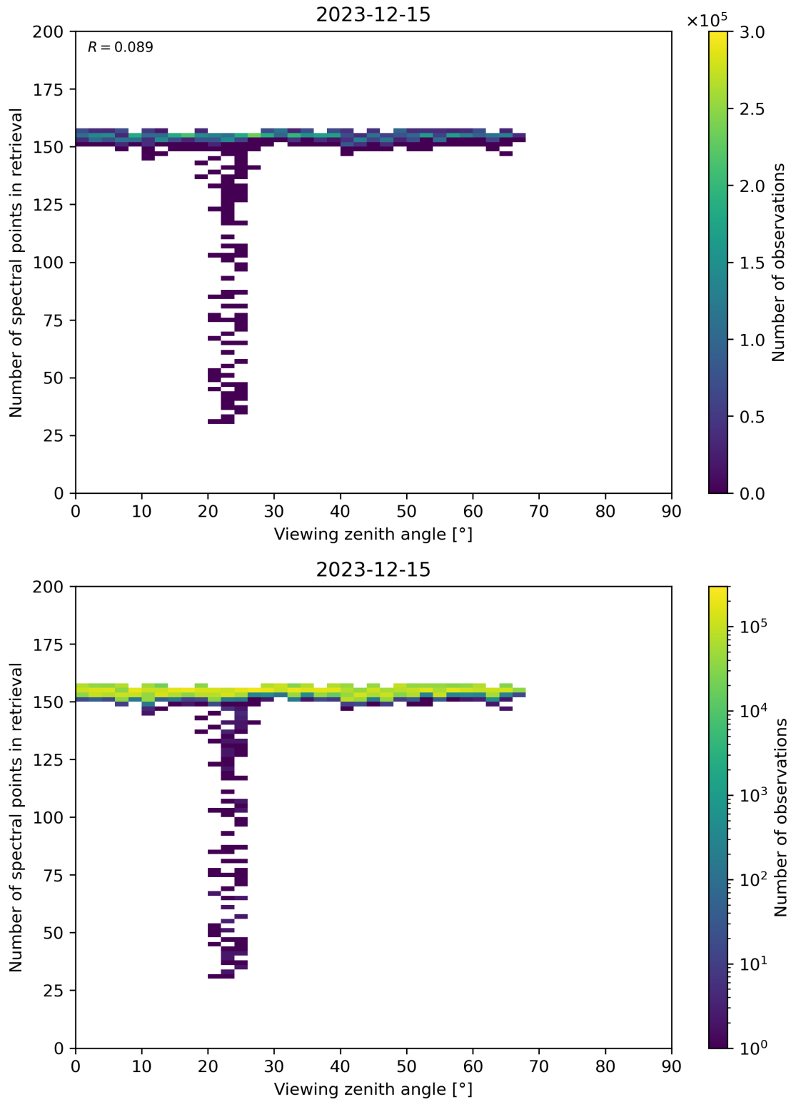
Figure 76: Scatter density plot of “Viewing zenith angle” against “Number of spectral points in retrieval” for 2023-12-14 to 2023-12-16.
