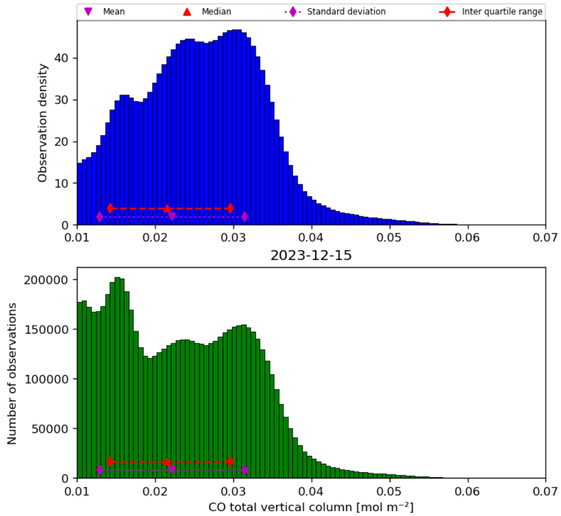
Figure 18: Histogram of “CO total vertical column” for 2023-12-14 to 2023-12-16
