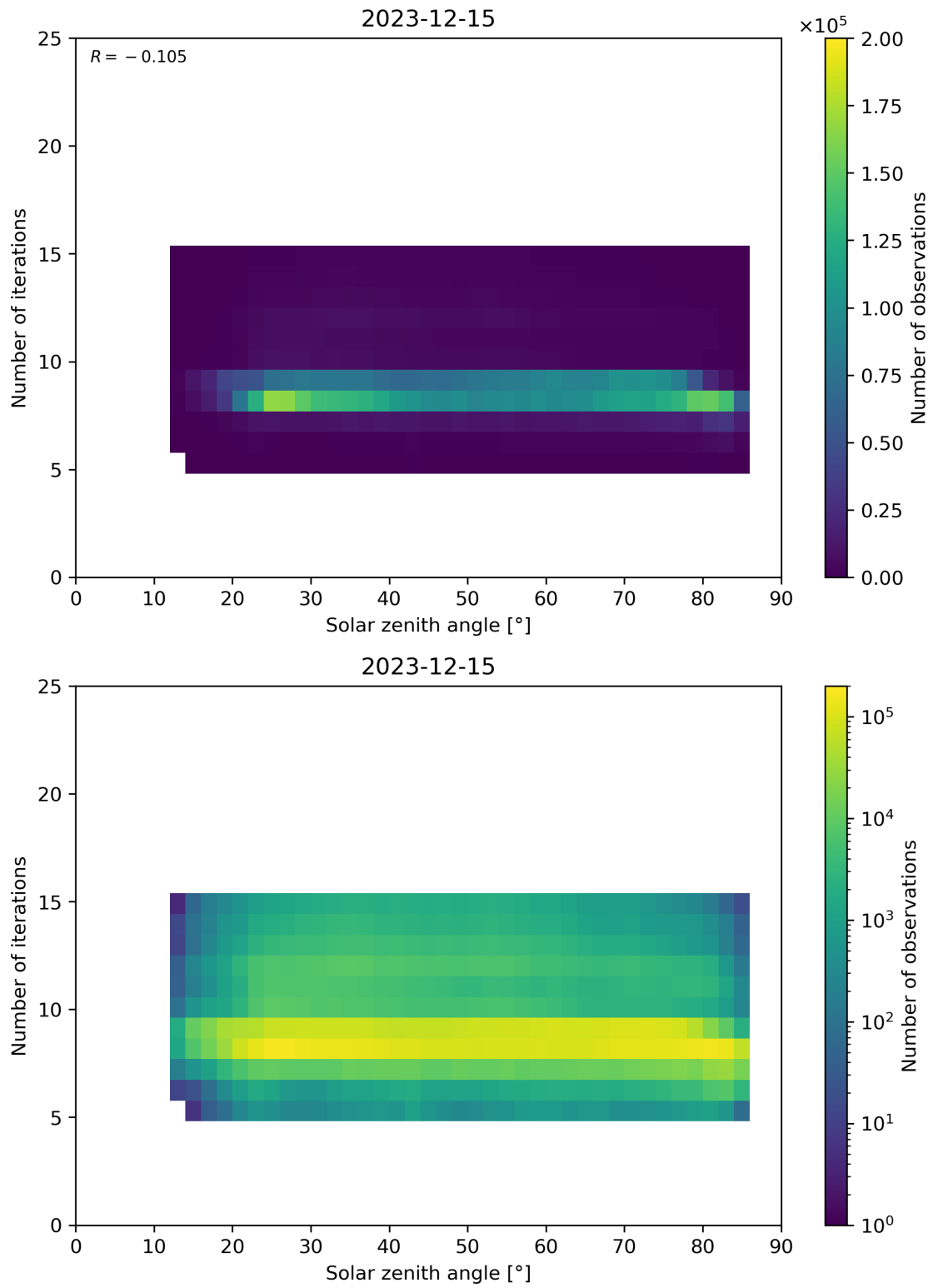
Figure 67: Scatter density plot of “Solar zenith angle” against “Number of iterations” for 2023-12-14 to 2023-12-16.
