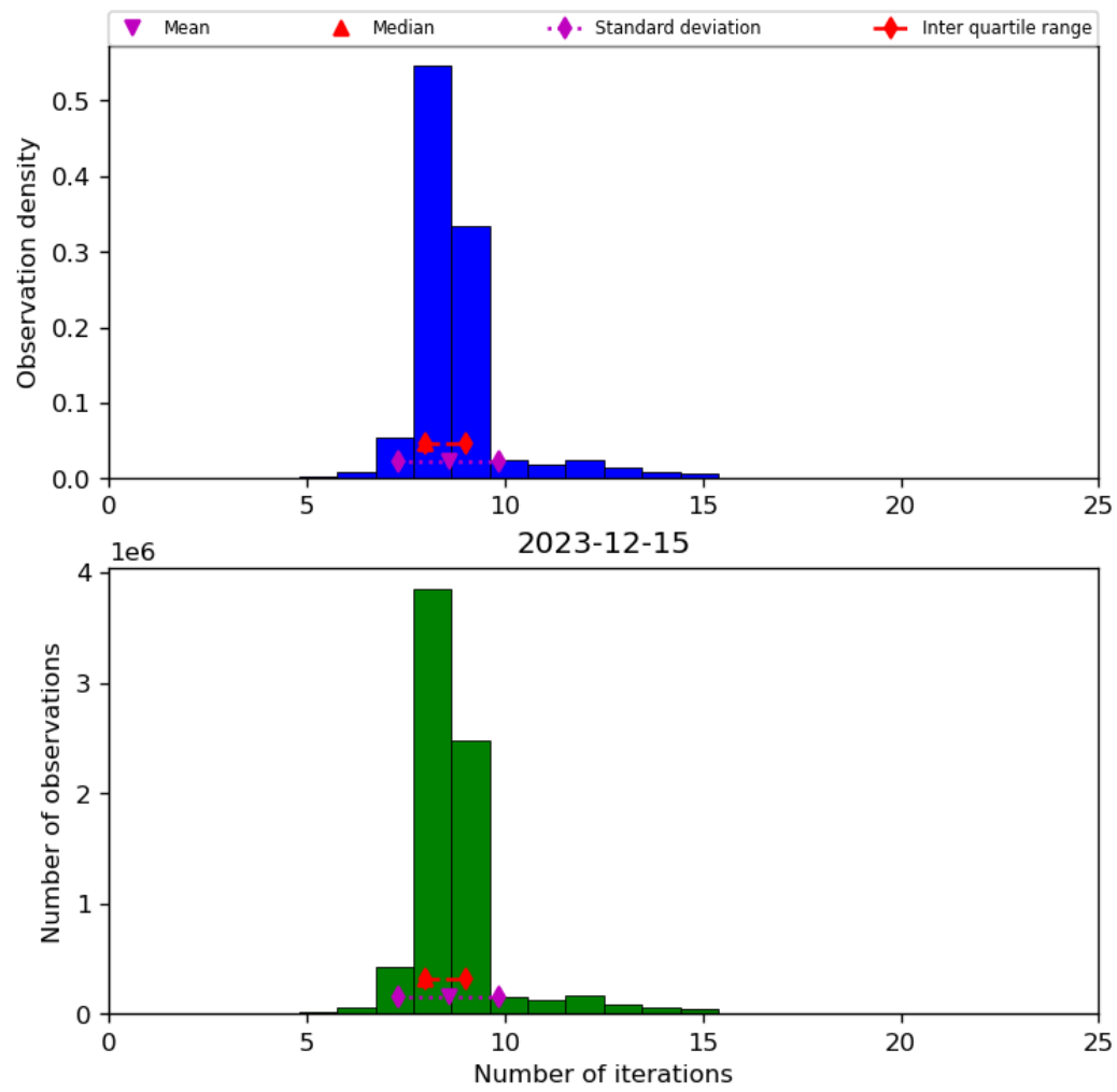
Figure 24: Histogram of “Number of iterations” for 2023-12-14 to 2023-12-16
