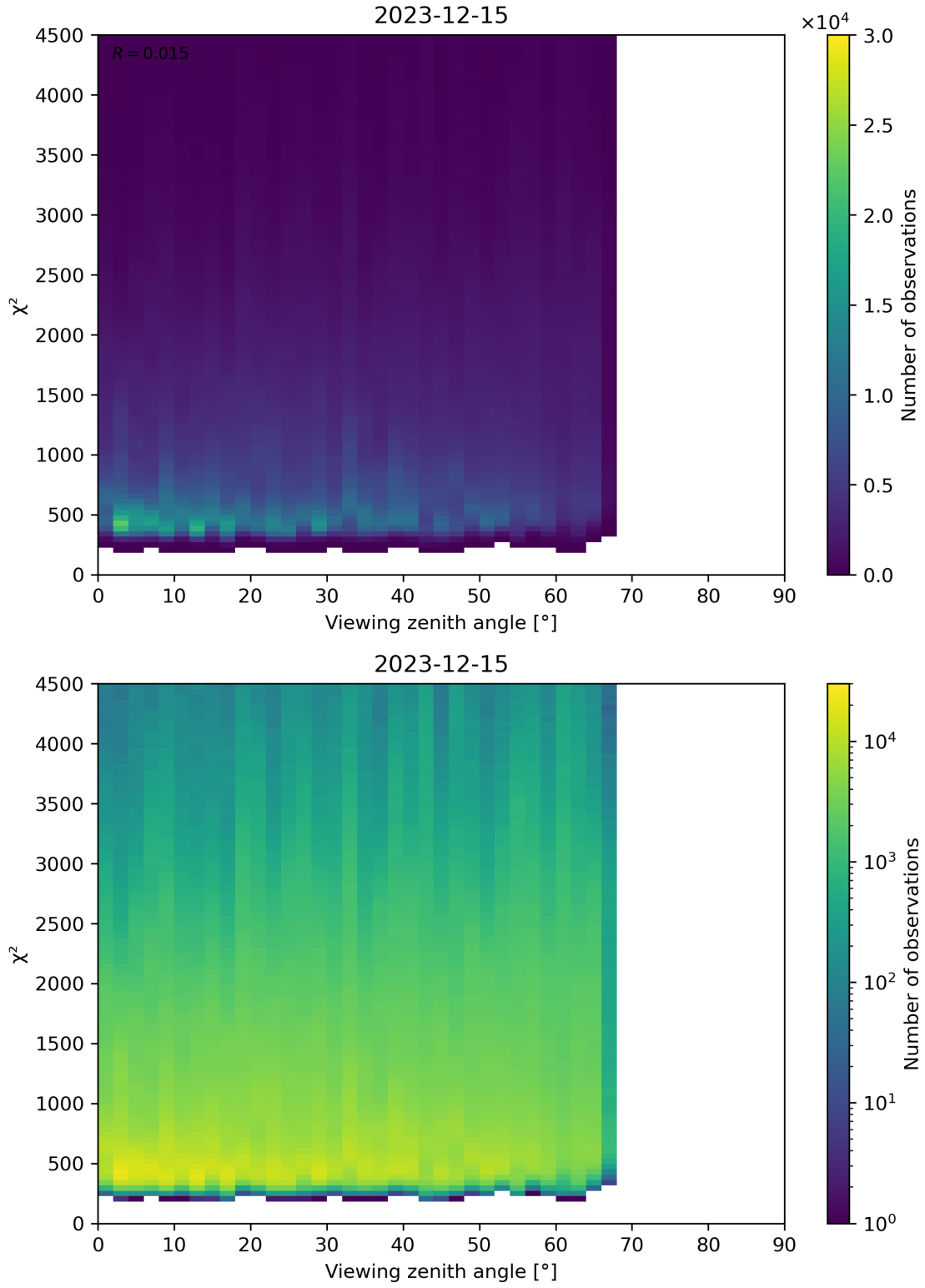
Figure 72: Scatter density plot of “Viewing zenith angle” against “ \chi^2 ” for 2023-12-14 to 2023-12-16.
