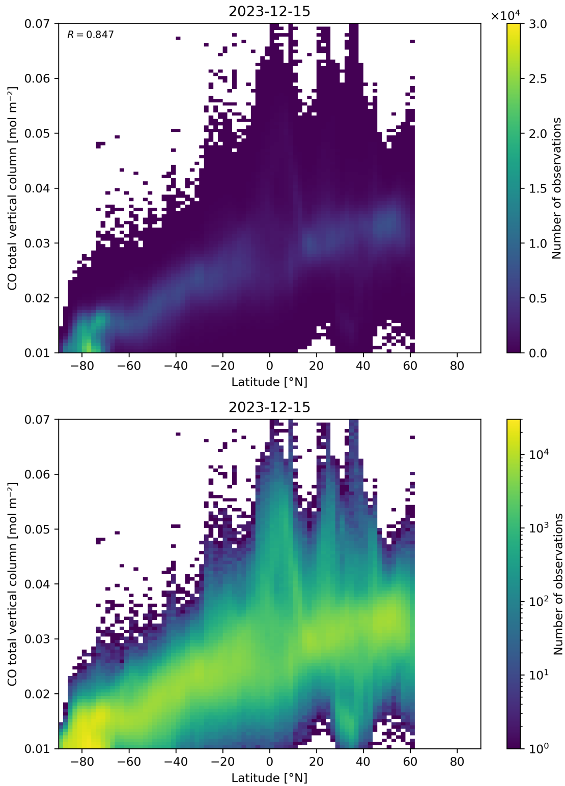
Figure 51: Scatter density plot of “Latitude” against “CO total vertical column” for 2023-12-14 to 2023-12-16.
