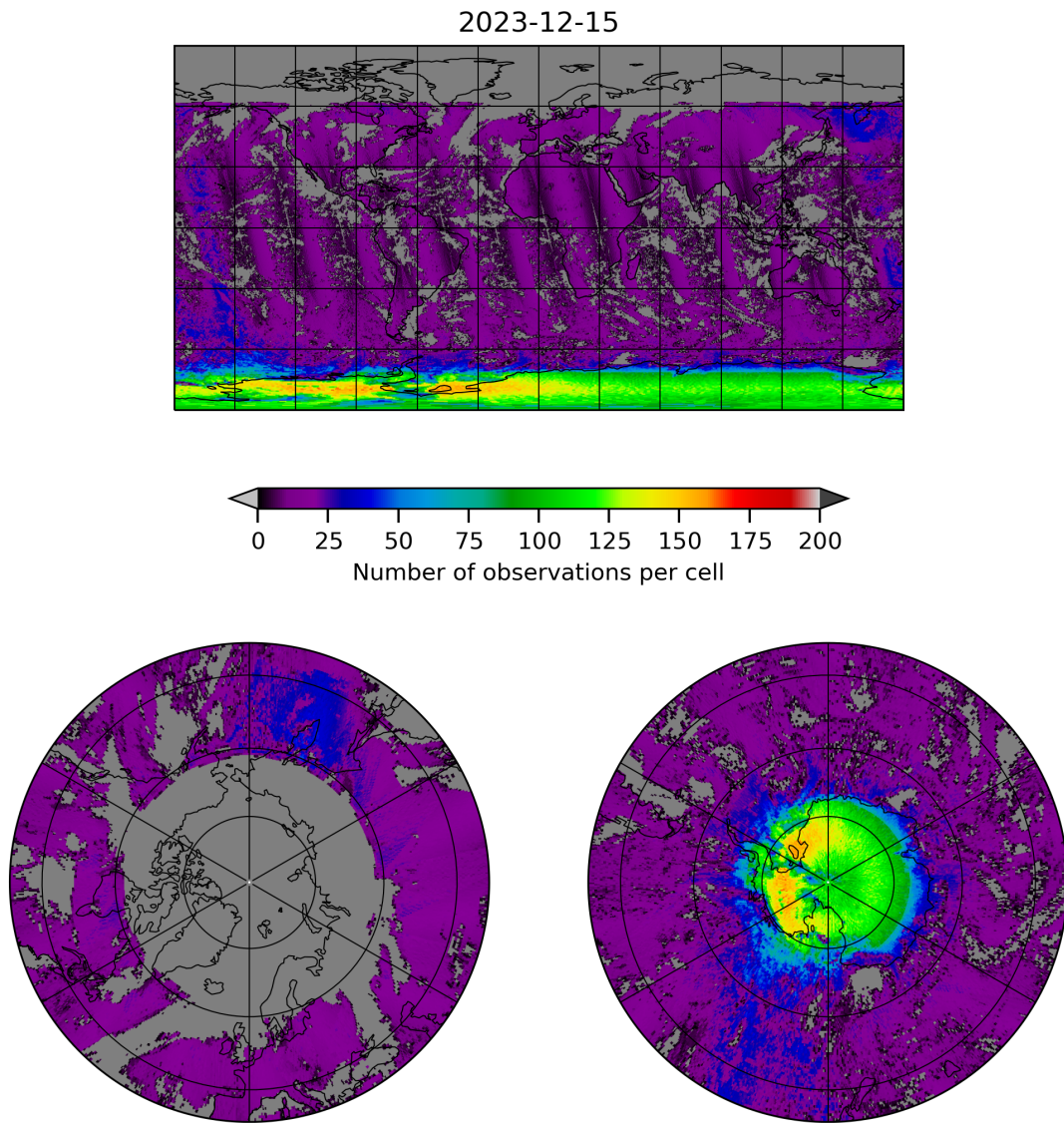
Figure 8: Map of the number of observations for 2023-12-14 to 2023-12-16
