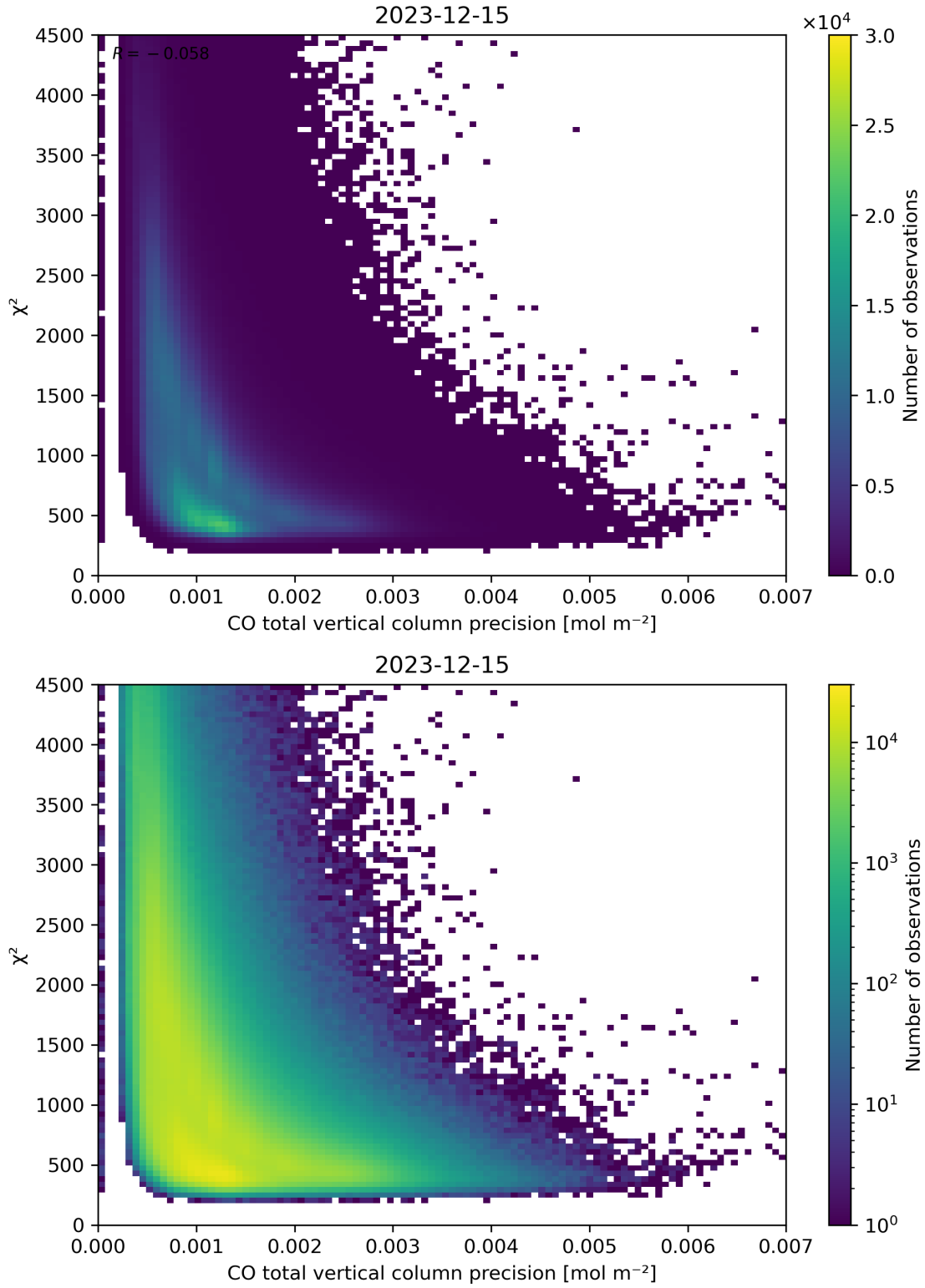
Figure 44: Scatter density plot of “CO total vertical column precision” against “ \chi^2 ” for 2023-12-14 to 2023-12-16.
