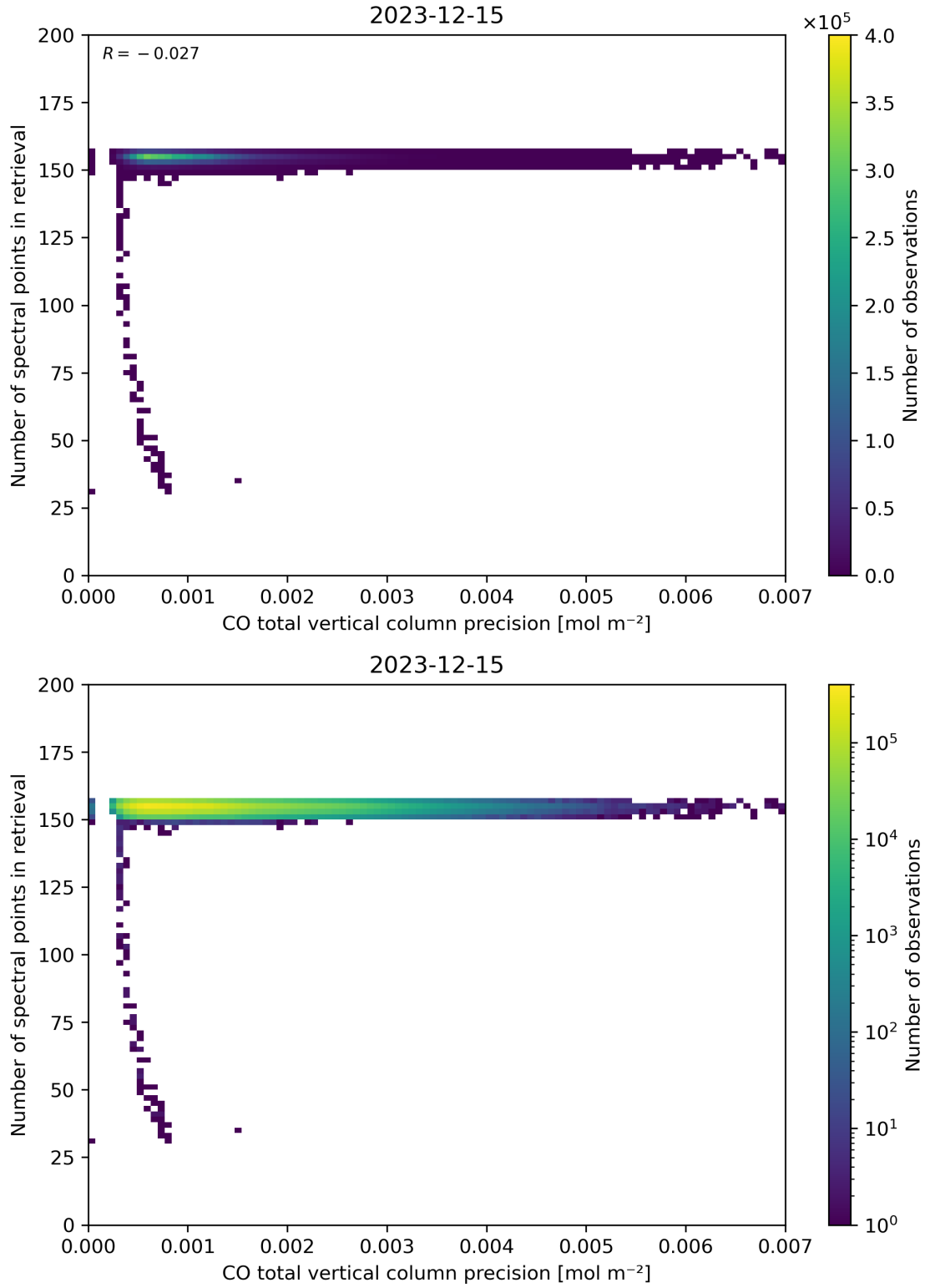
Figure 47: Scatter density plot of “CO total vertical column precision” against “Number of spectral points in retrieval” for 2023-12-14 to 2023-12-16.
