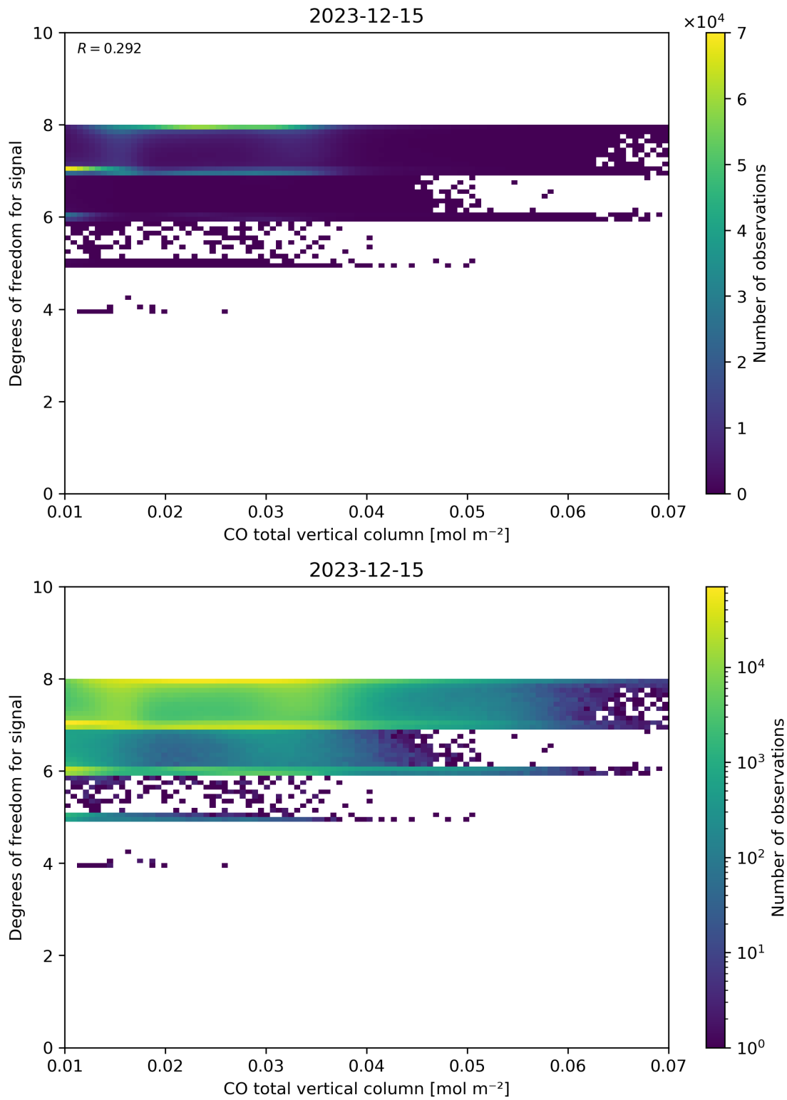
Figure 41: Scatter density plot of “CO total vertical column” against “Degrees of freedom for signal” for 2023-12-14 to 2023-12-16.
