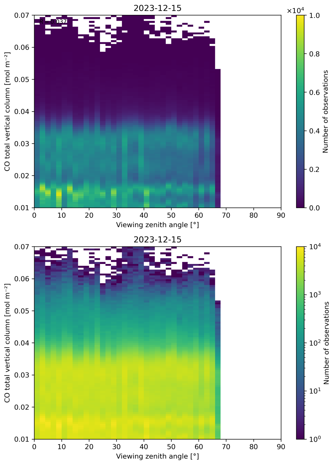
Figure 69: Scatter density plot of “Viewing zenith angle” against “CO total vertical column” for 2023-12-14 to 2023-12-16.
