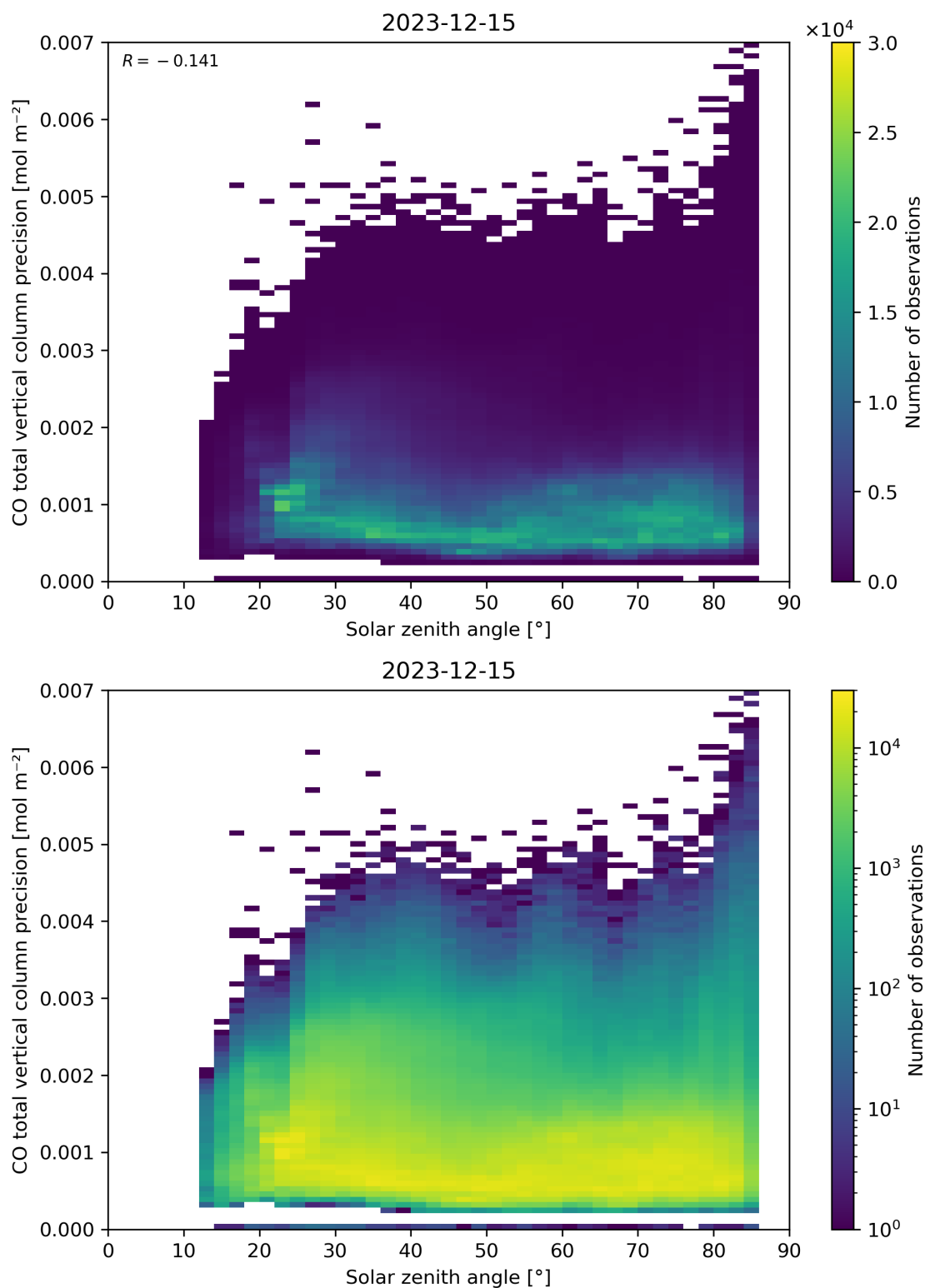
Figure 63: Scatter density plot of “Solar zenith angle” against “CO total vertical column precision” for 2023-12-14 to 2023-12-16.
