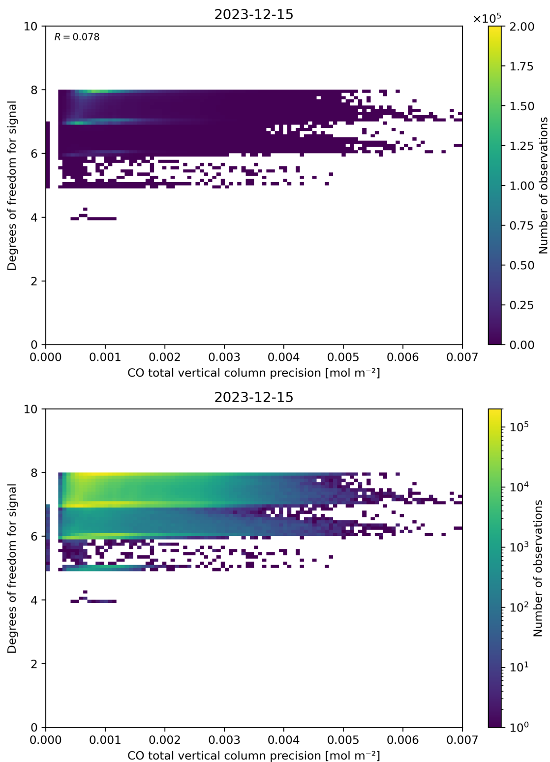
Figure 45: Scatter density plot of “CO total vertical column precision” against “Degrees of freedom for signal” for 2023-12-14 to 2023-12-16.
