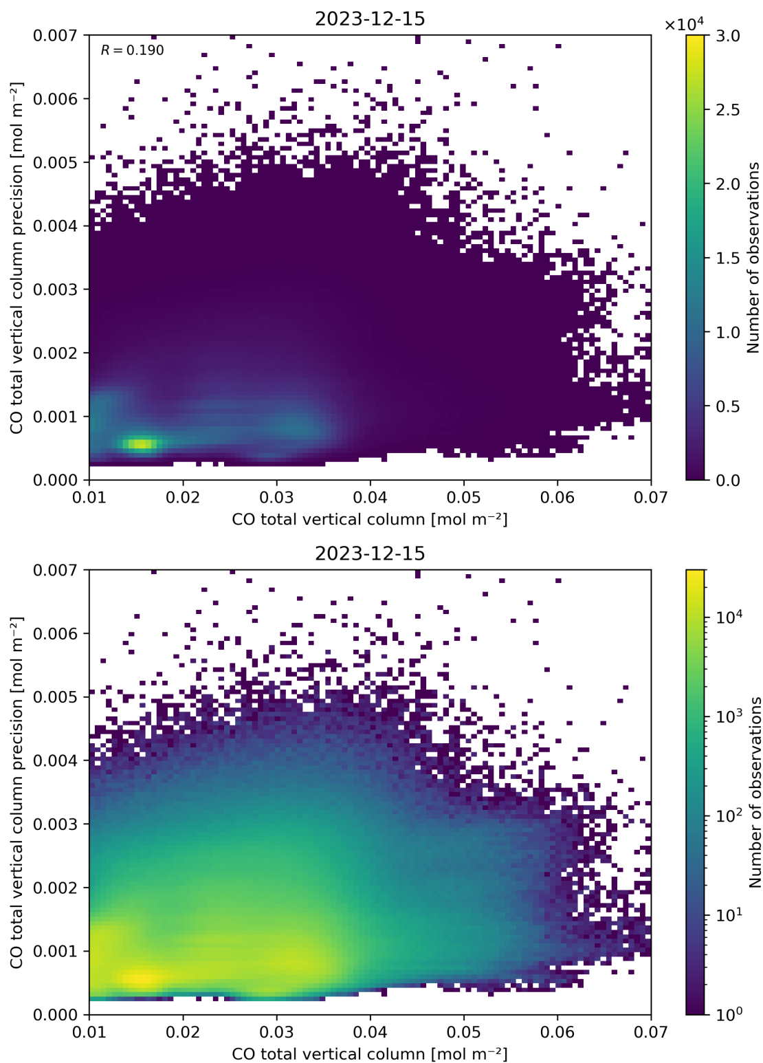
Figure 34: Scatter density plot of “CO total vertical column” against “CO total vertical column precision” for 2023-12-14 to 2023-12-16.
