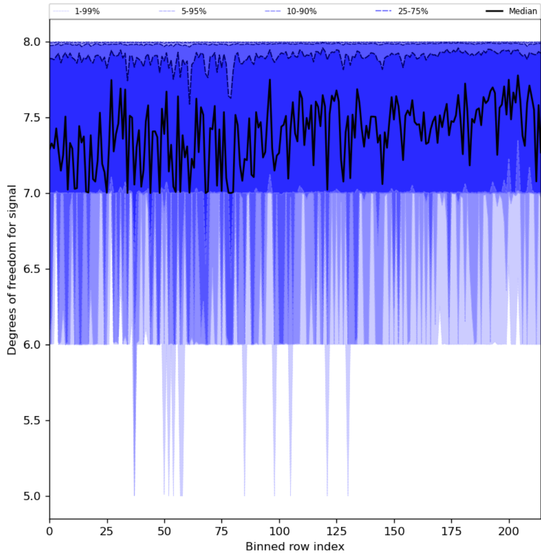
Figure 31: Along track statistics of “Degrees of freedom for signal” for 2023-12-14 to 2023-12-16
