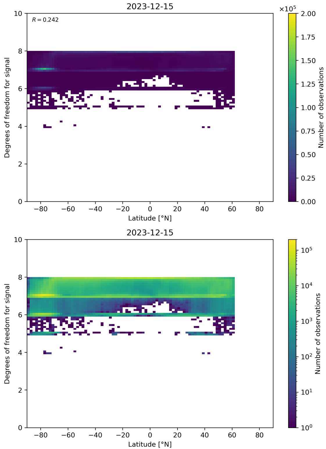
Figure 55: Scatter density plot of “Latitude” against “Degrees of freedom for signal” for 2023-12-14 to 2023-12-16.
