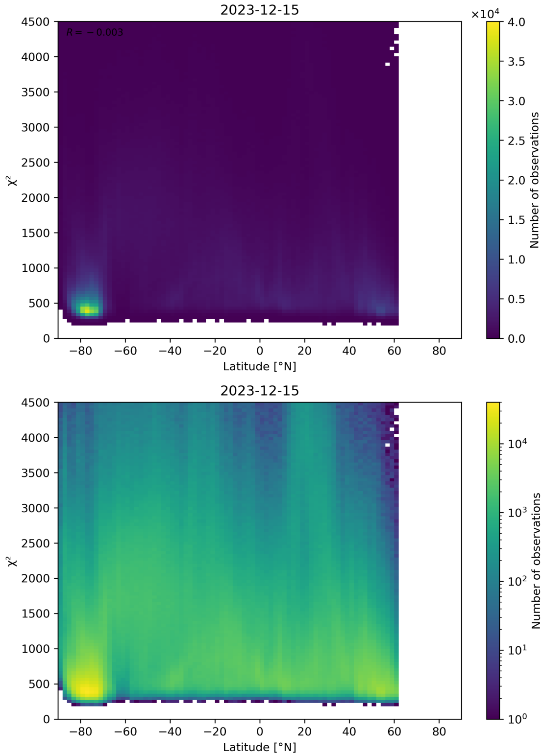
Figure 54: Scatter density plot of “Latitude” against “ \chi^2 ” for 2023-12-14 to 2023-12-16.
