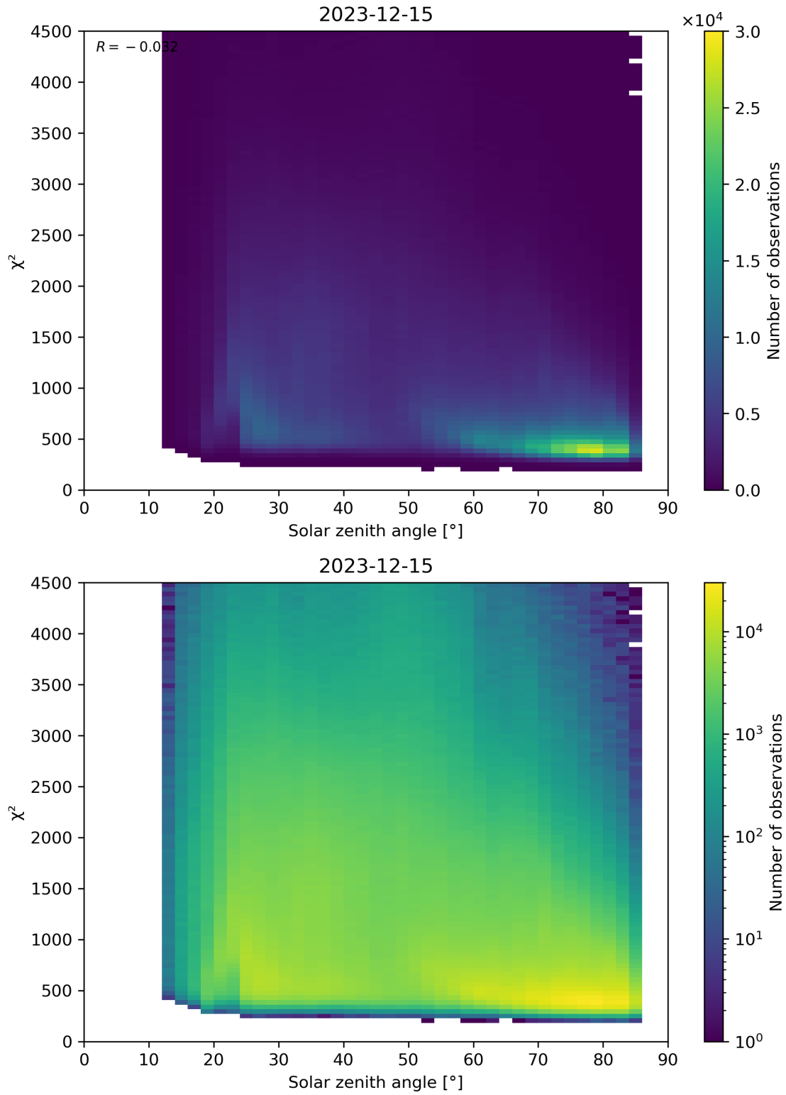
Figure 64: Scatter density plot of “Solar zenith angle” against “ \chi^2 ” for 2023-12-14 to 2023-12-16.
