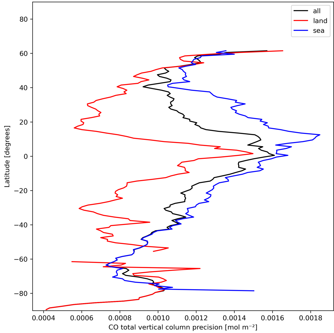
Figure 12: Zonal average of “CO total vertical column precision” for 2023-12-14 to 2023-12-16.
