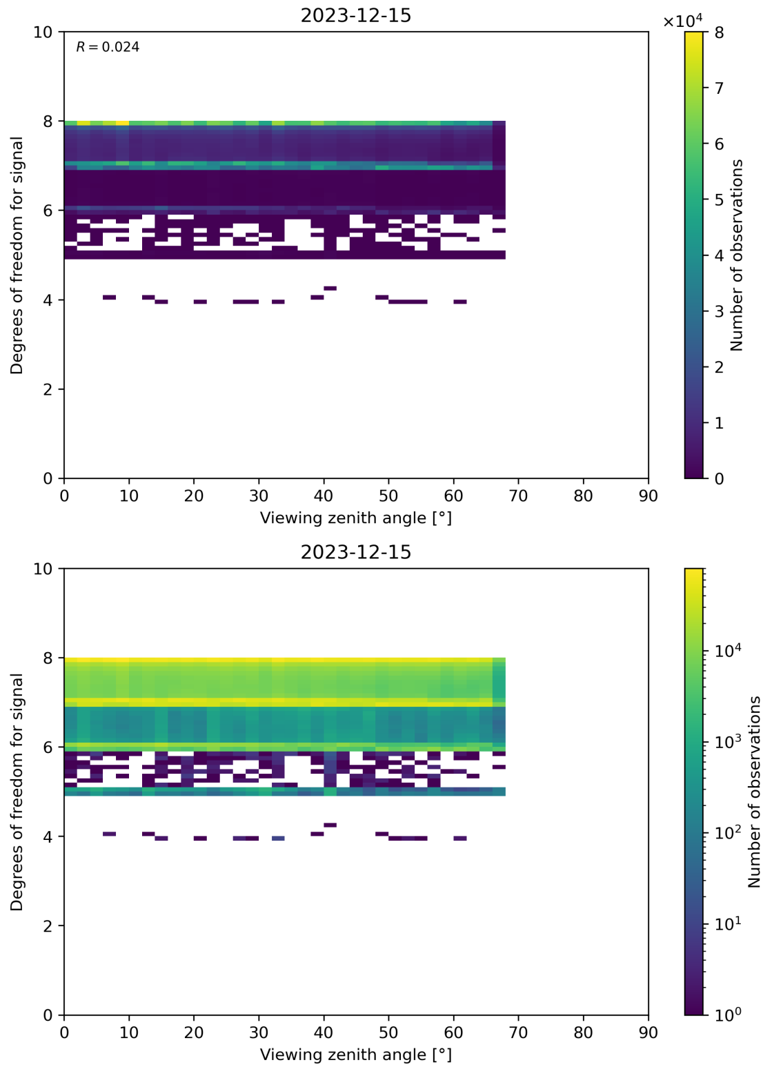
Figure 73: Scatter density plot of “Viewing zenith angle” against “Degrees of freedom for signal” for 2023-12-14 to 2023-12-16.
