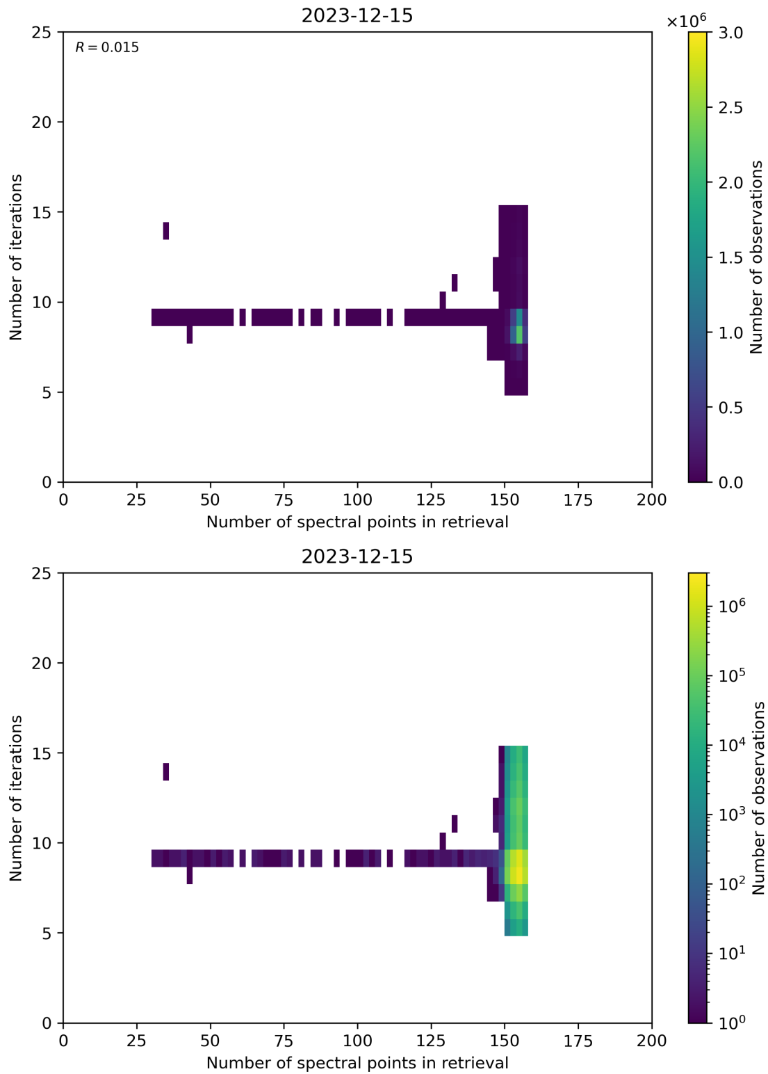
Figure 60: Scatter density plot of “Number of spectral points in retrieval” against “Number of iterations” for 2023-12-14 to 2023-12-16.
