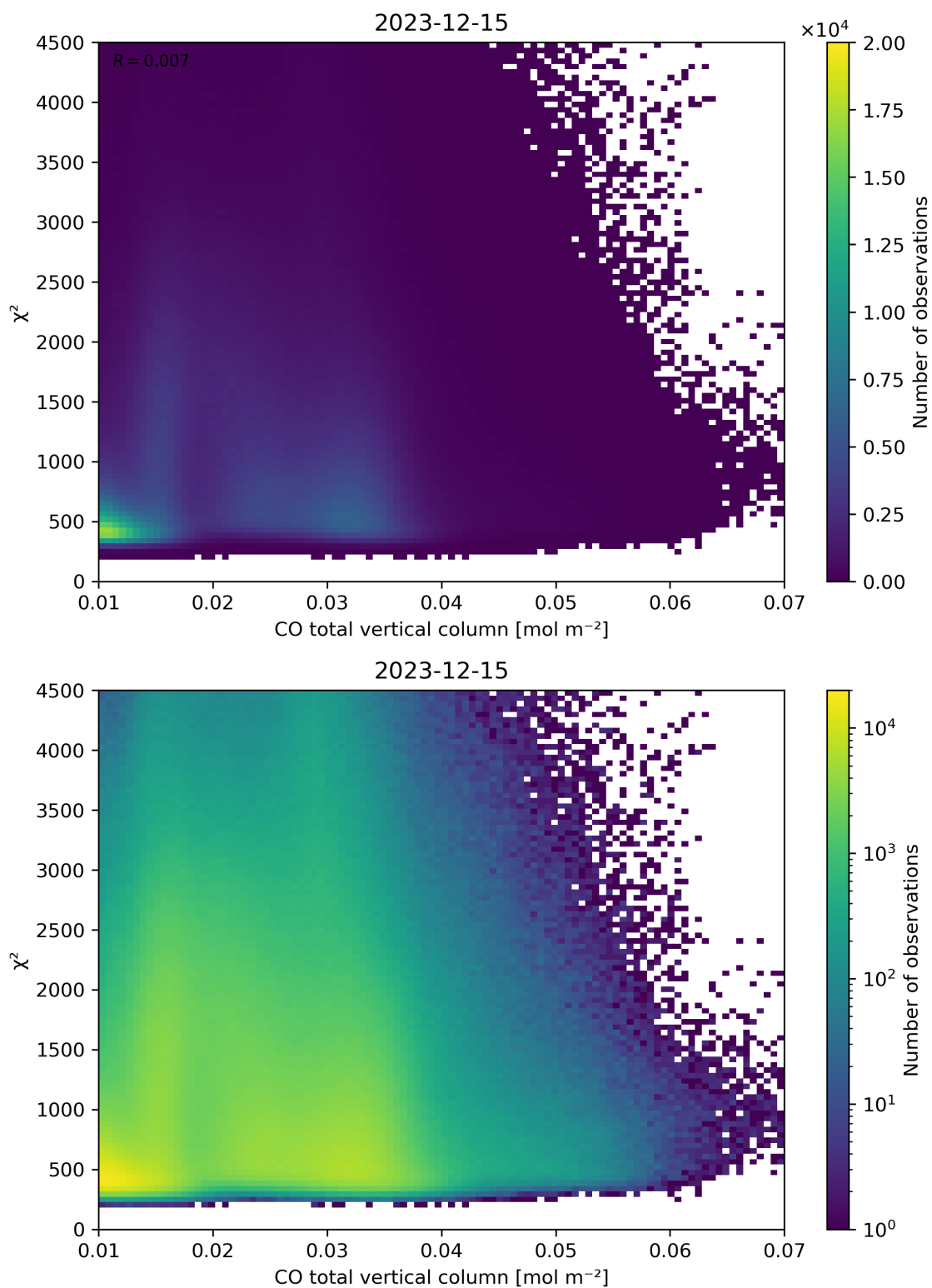
Figure 35: Scatter density plot of “CO total vertical column” against “ \chi^2 ” for 2023-12-14 to 2023-12-16.
