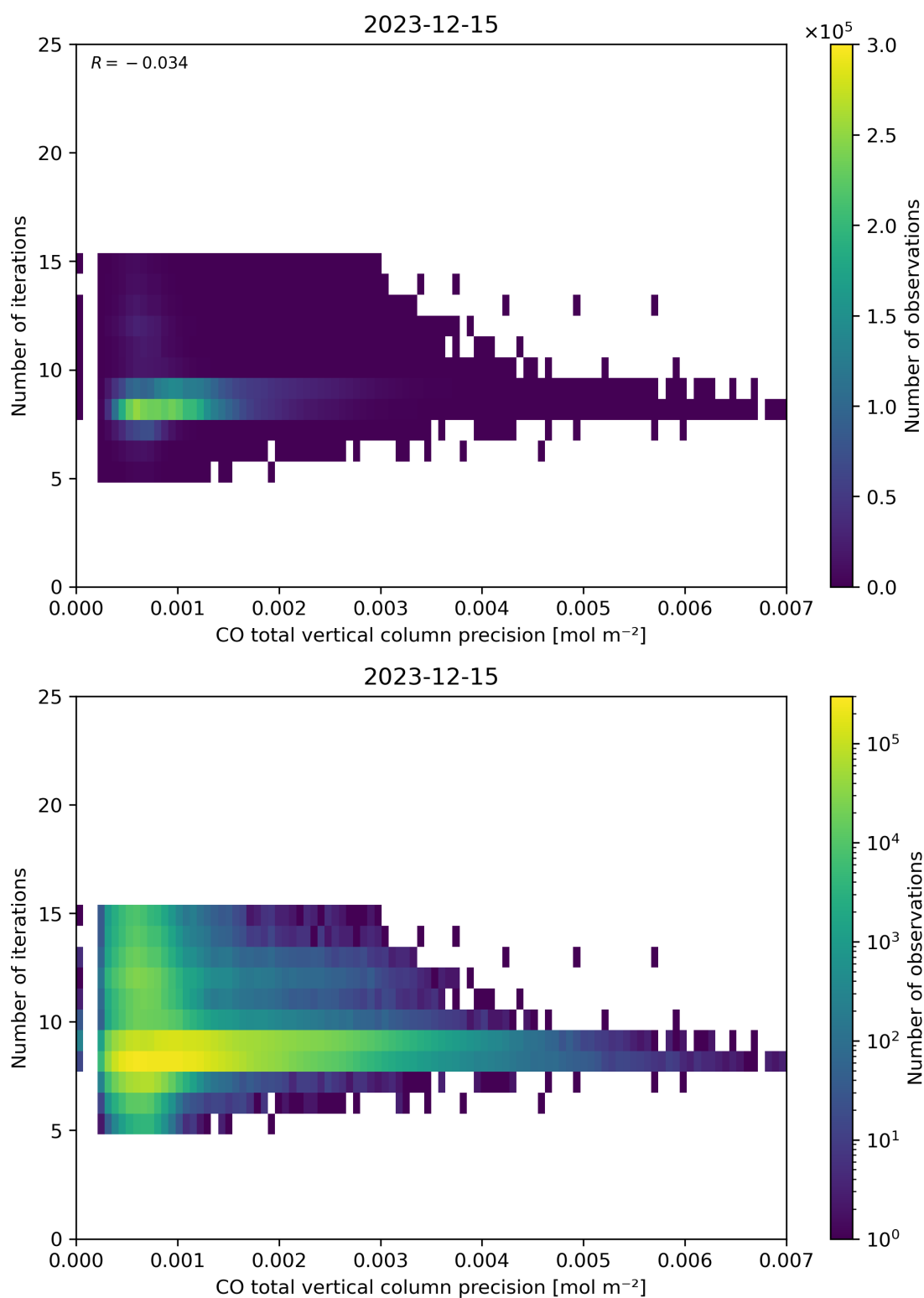
Figure 46: Scatter density plot of “CO total vertical column precision” against “Number of iterations” for 2023-12-14 to 2023-12-16.
