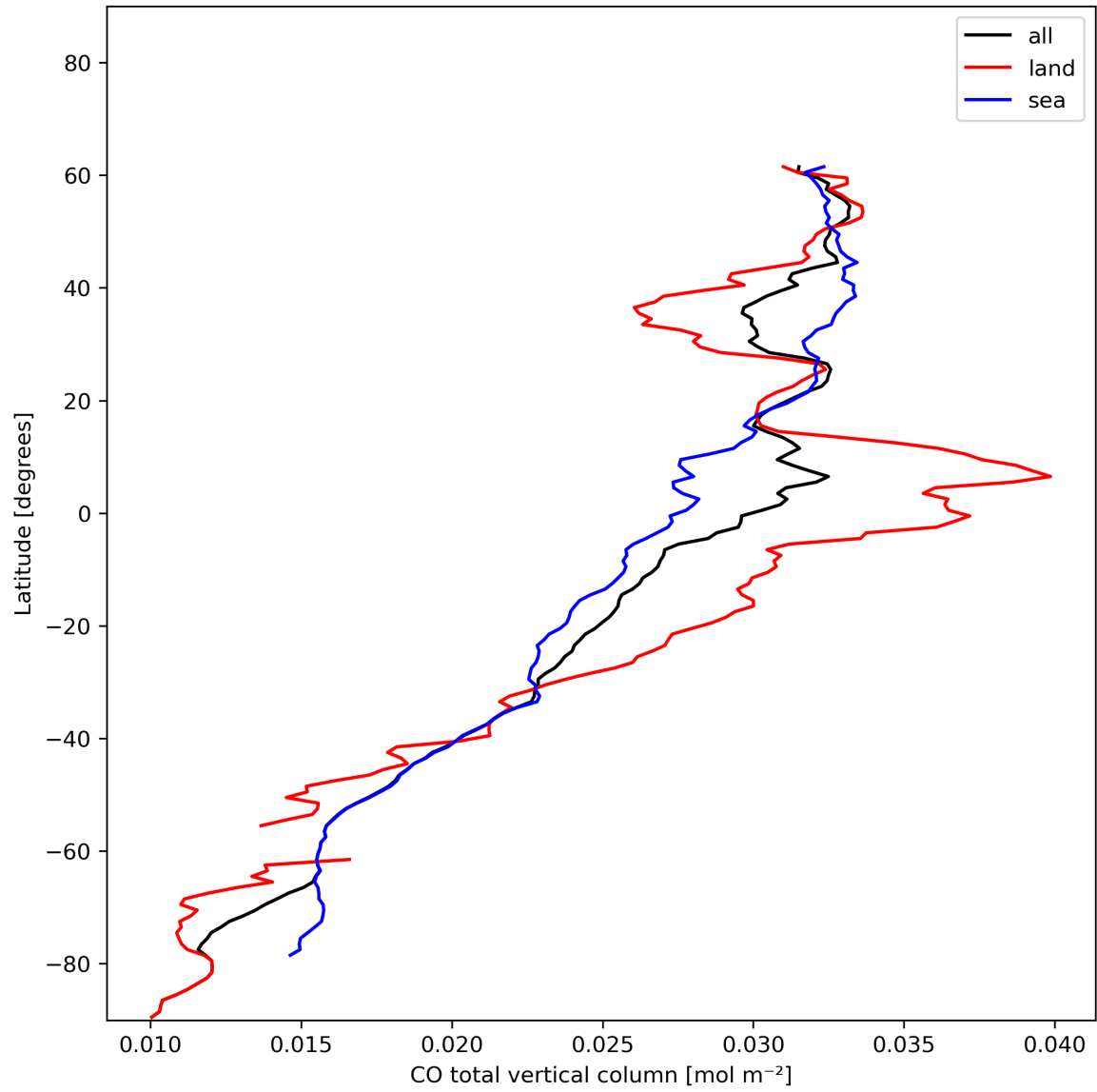
Figure 10: Zonal average of “CO total vertical column” for 2023-12-14 to 2023-12-16.
