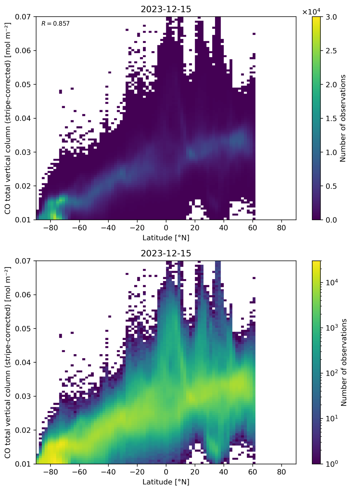
Figure 52: Scatter density plot of “Latitude” against “CO total vertical column (stripe-corrected)” for 2023-12-14 to 2023-12-16.
