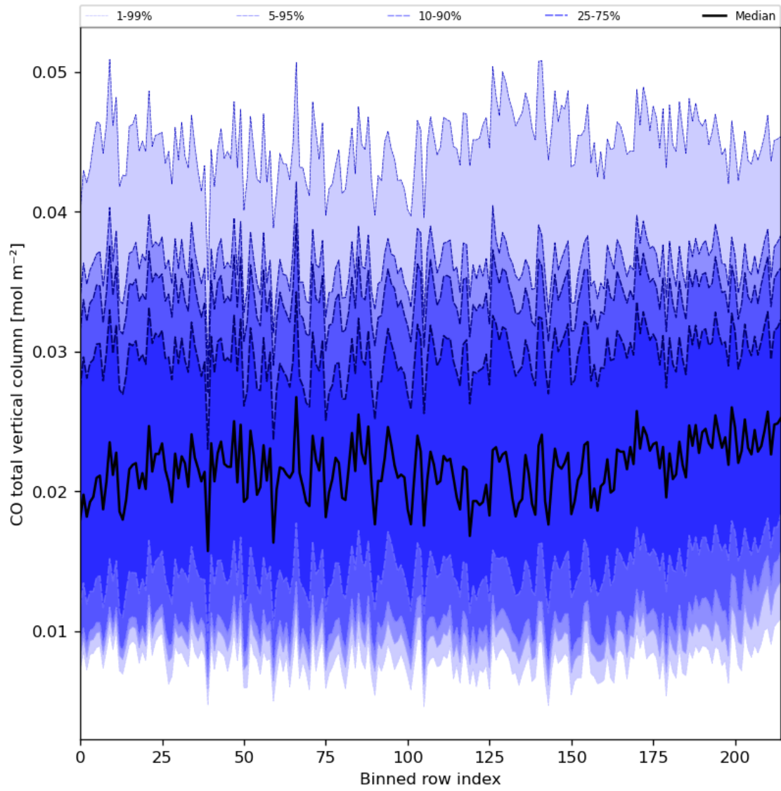
Figure 26: Along track statistics of “CO total vertical column” for 2023-12-14 to 2023-12-16
