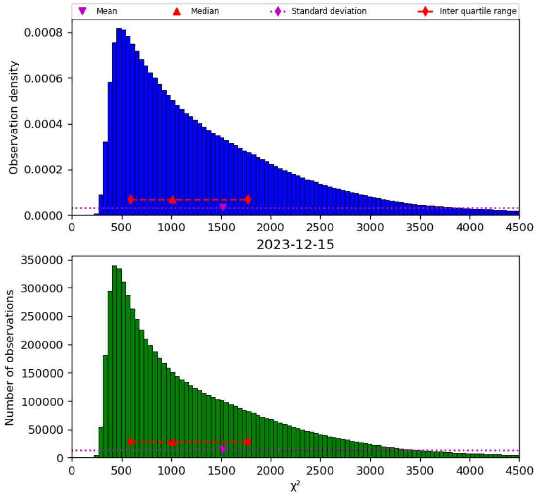
Figure 22: Histogram of “ \chi^2 ” for 2023-12-14 to 2023-12-16
