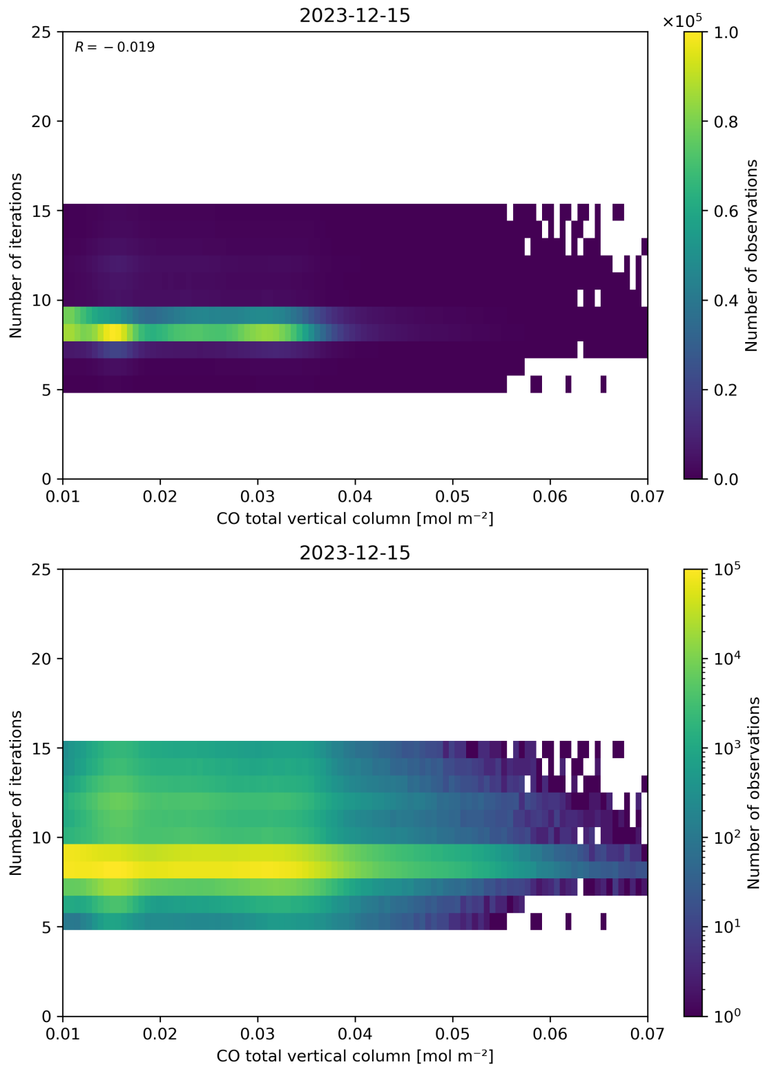
Figure 42: Scatter density plot of “CO total vertical column” against “Number of iterations” for 2023-12-14 to 2023-12-16.
