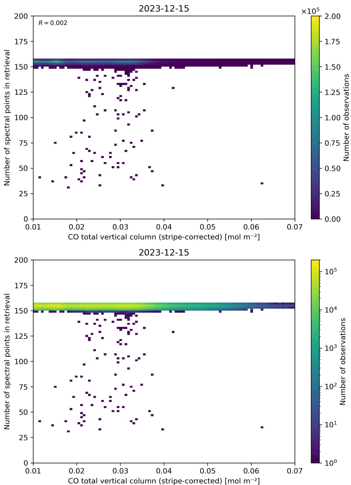
Figure 40: Scatter density plot of “CO total vertical column (stripe-corrected)” against “Number of spectral points in retrieval” for 2023-12-14 to 2023-12-16.
