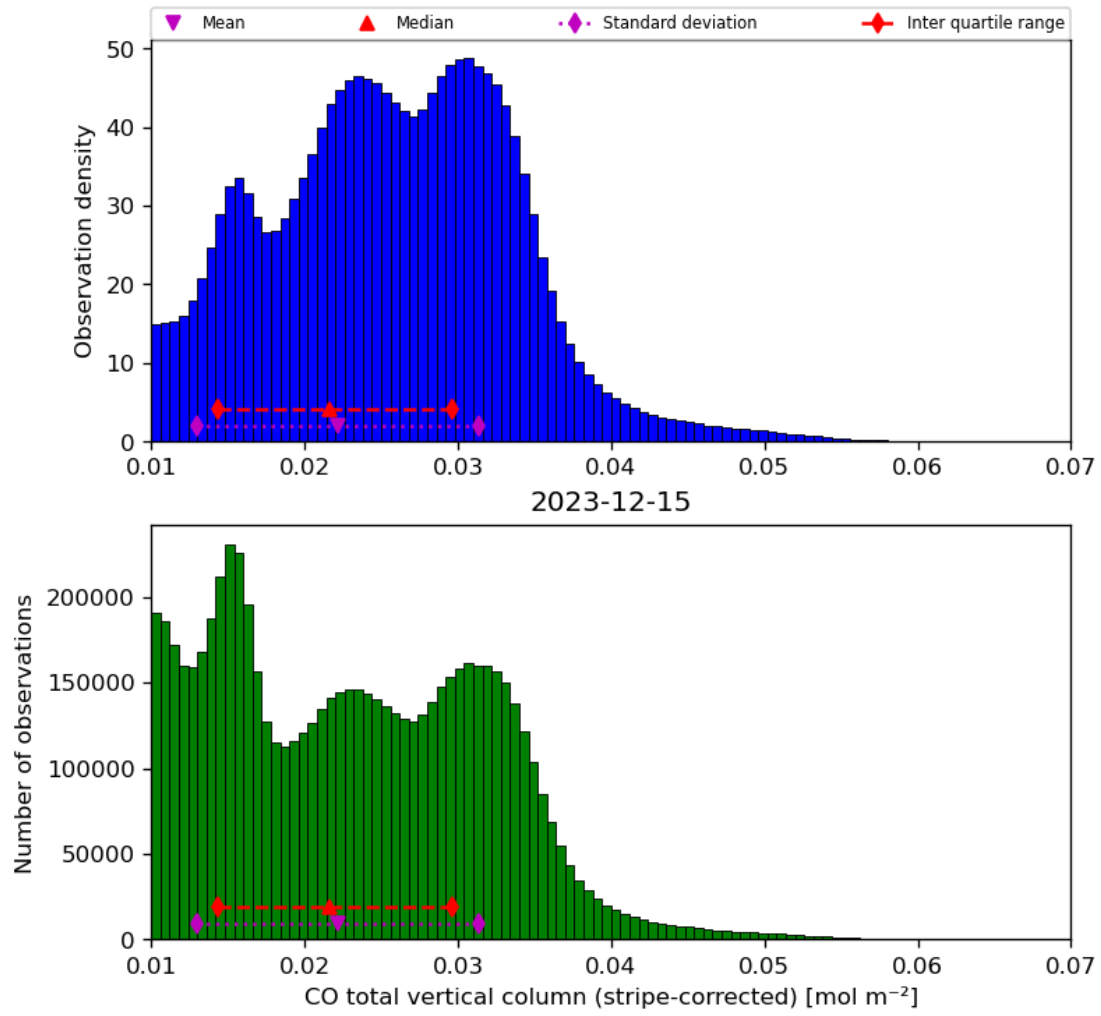
Figure 19: Histogram of “CO total vertical column (stripe-corrected)” for 2023-12-14 to 2023-12-16
