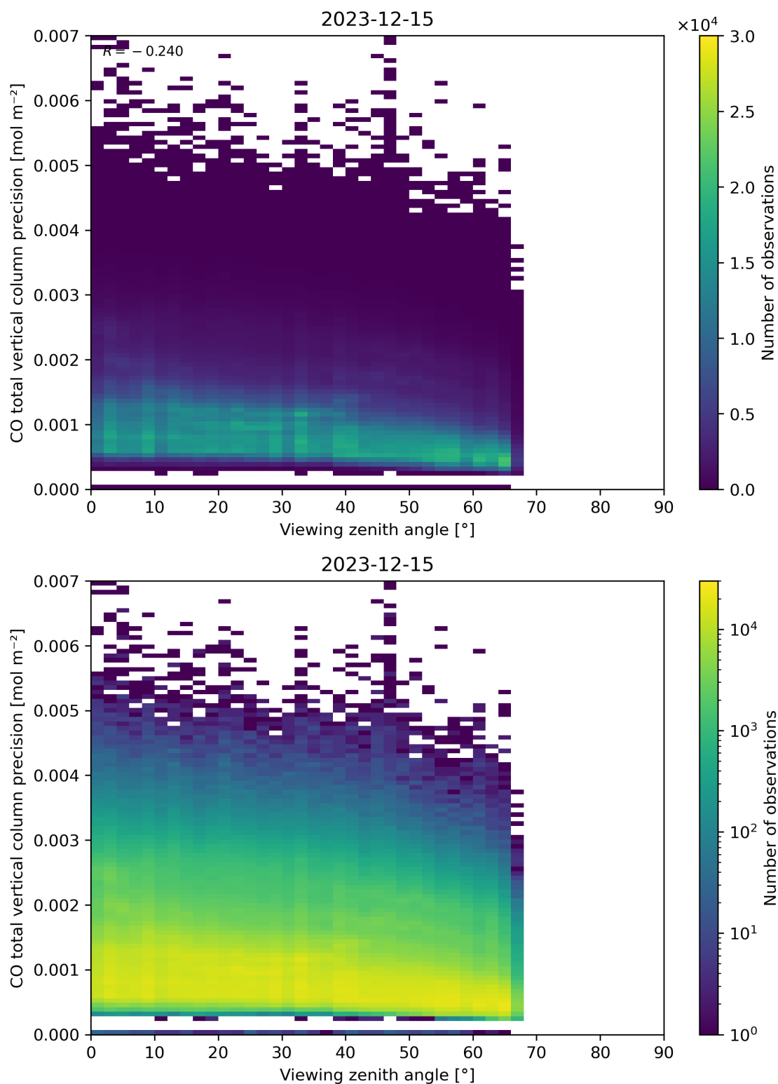
Figure 71: Scatter density plot of “Viewing zenith angle” against “CO total vertical column precision” for 2023-12-14 to 2023-12-16.
