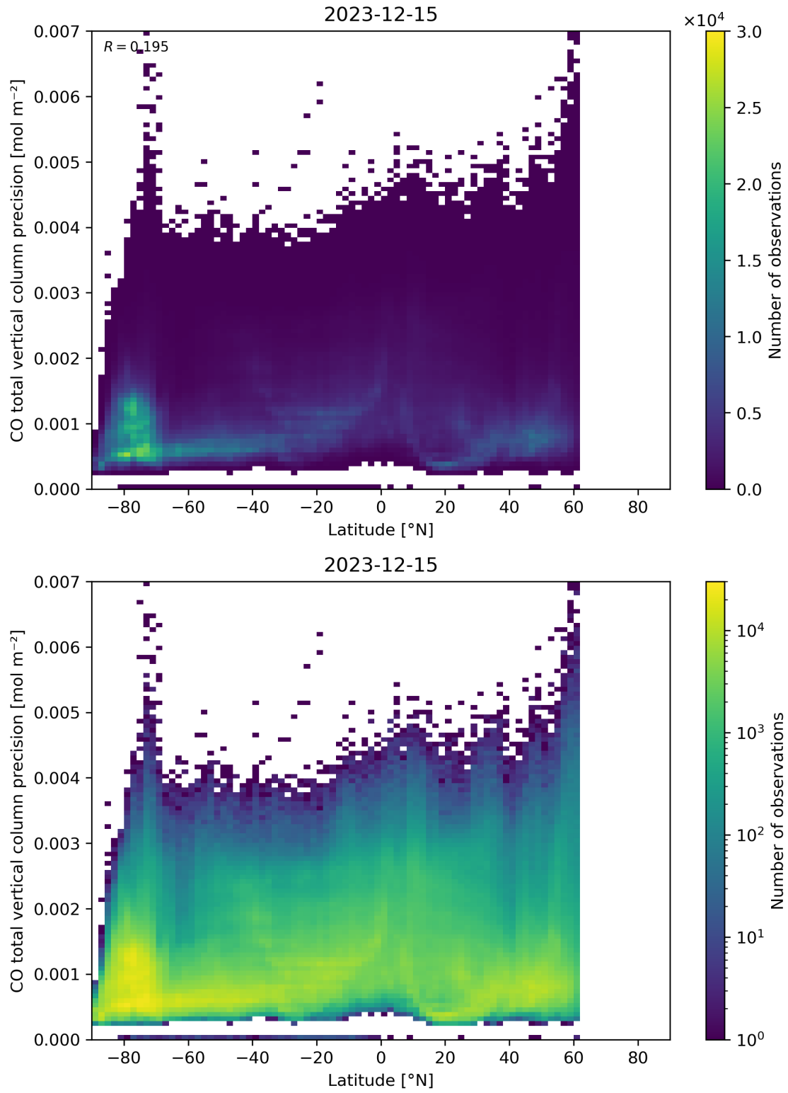
Figure 53: Scatter density plot of “Latitude” against “CO total vertical column precision” for 2023-12-14 to 2023-12-16.
