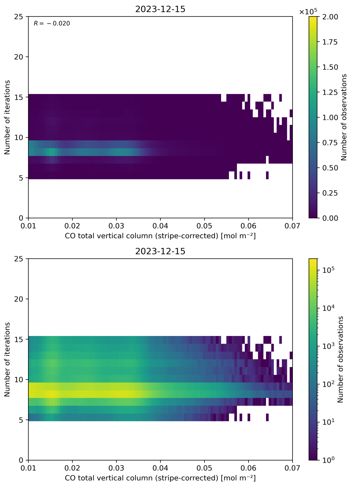
Figure 39: Scatter density plot of “CO total vertical column (stripe-corrected)” against “Number of iterations” for 2023-12-14 to 2023-12-16.
