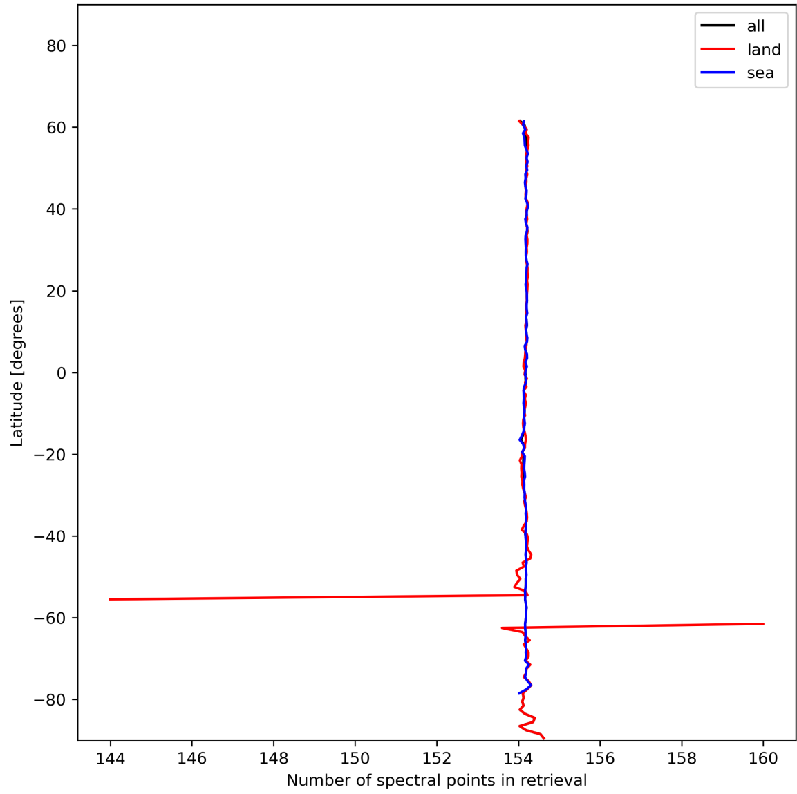
Figure 13: Zonal average of “Number of spectral points in retrieval” for 2023-12-14 to 2023-12-16.
