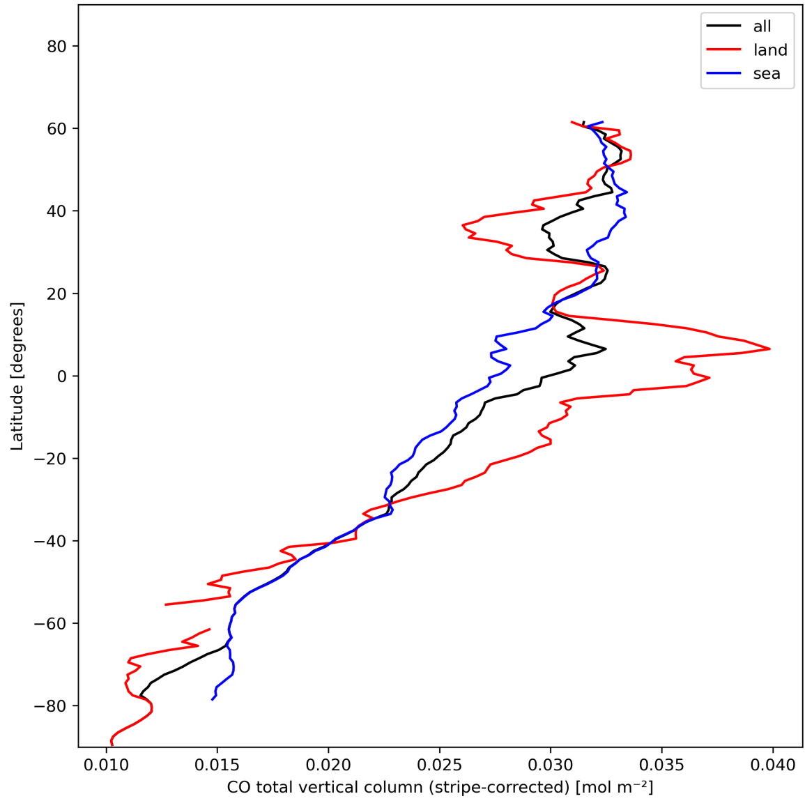
Figure 11: Zonal average of “CO total vertical column (stripe-corrected)” for 2023-12-14 to 2023-12-16.
