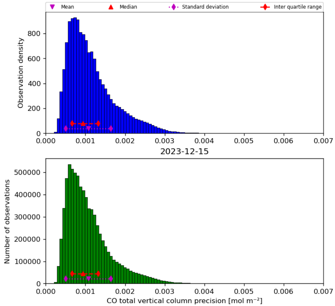
Figure 20: Histogram of “CO total vertical column precision” for 2023-12-14 to 2023-12-16
