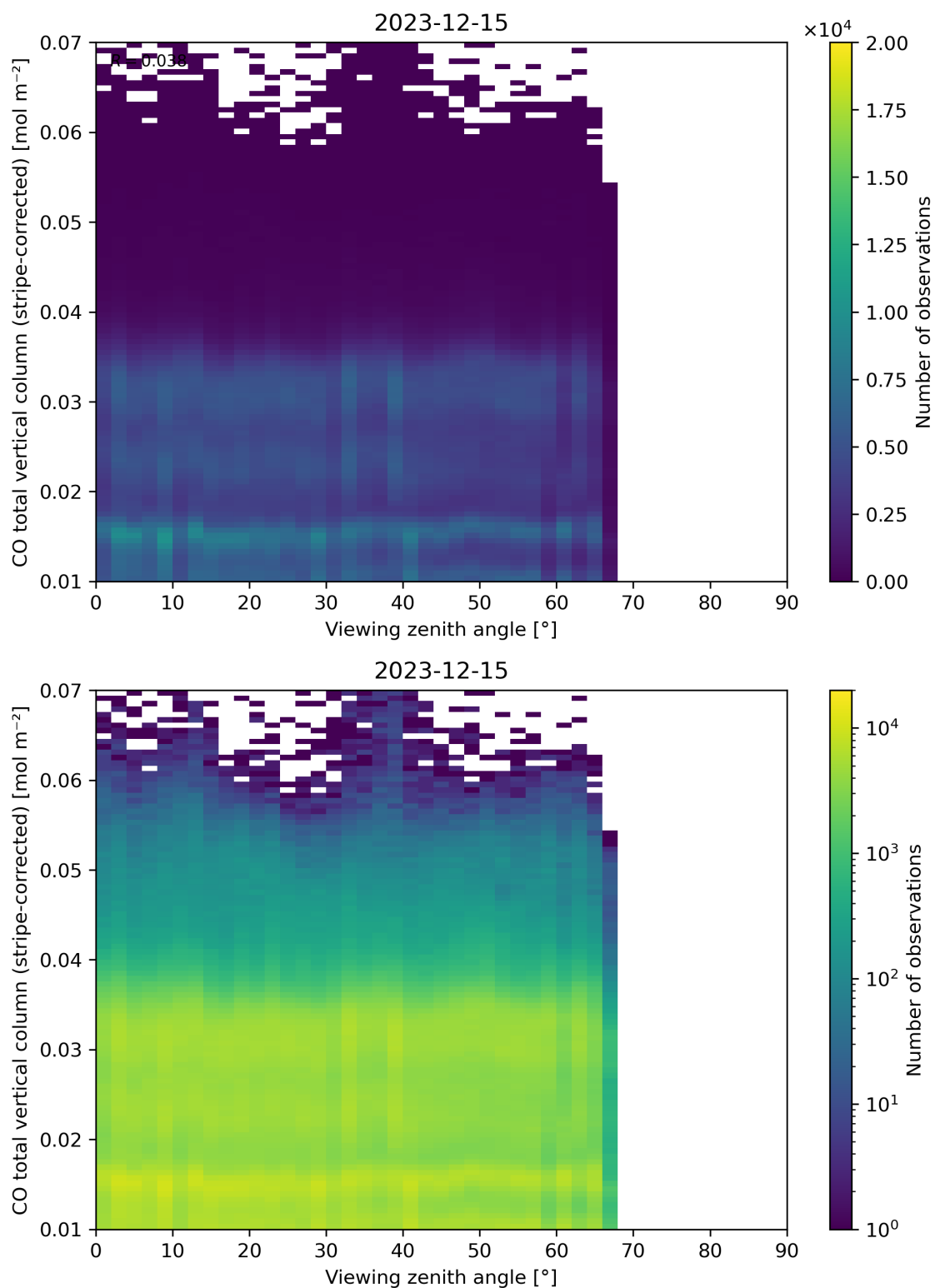
Figure 70: Scatter density plot of “Viewing zenith angle” against “CO total vertical column (stripe-corrected)” for 2023-12-14 to 2023-12-16.
