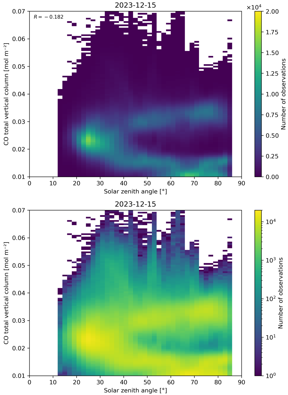
Figure 61: Scatter density plot of “Solar zenith angle” against “CO total vertical column” for 2023-12-14 to 2023-12-16.
