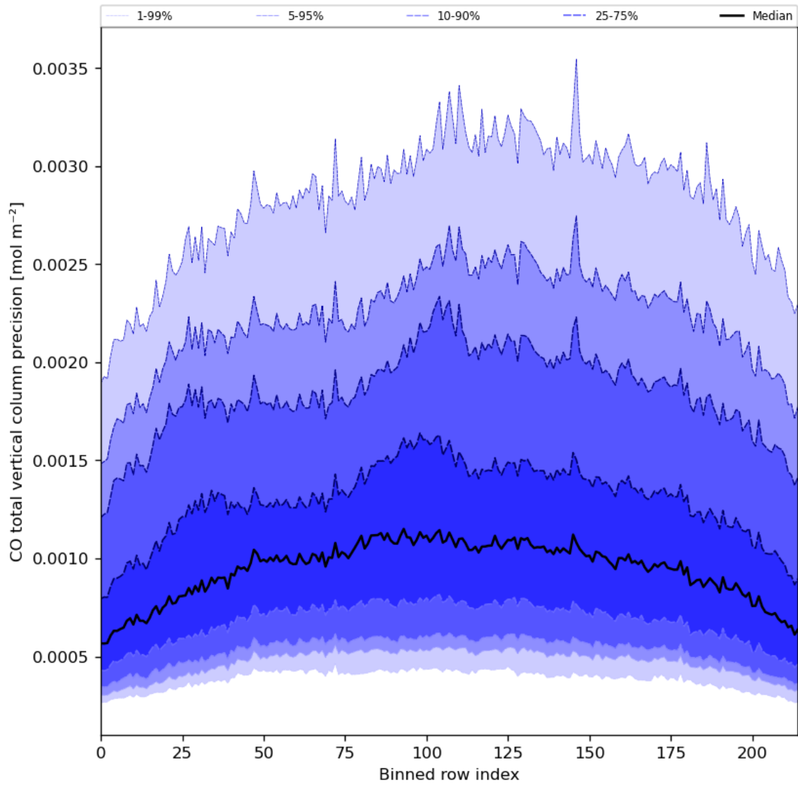
Figure 28: Along track statistics of “CO total vertical column precision” for 2023-12-14 to 2023-12-16
