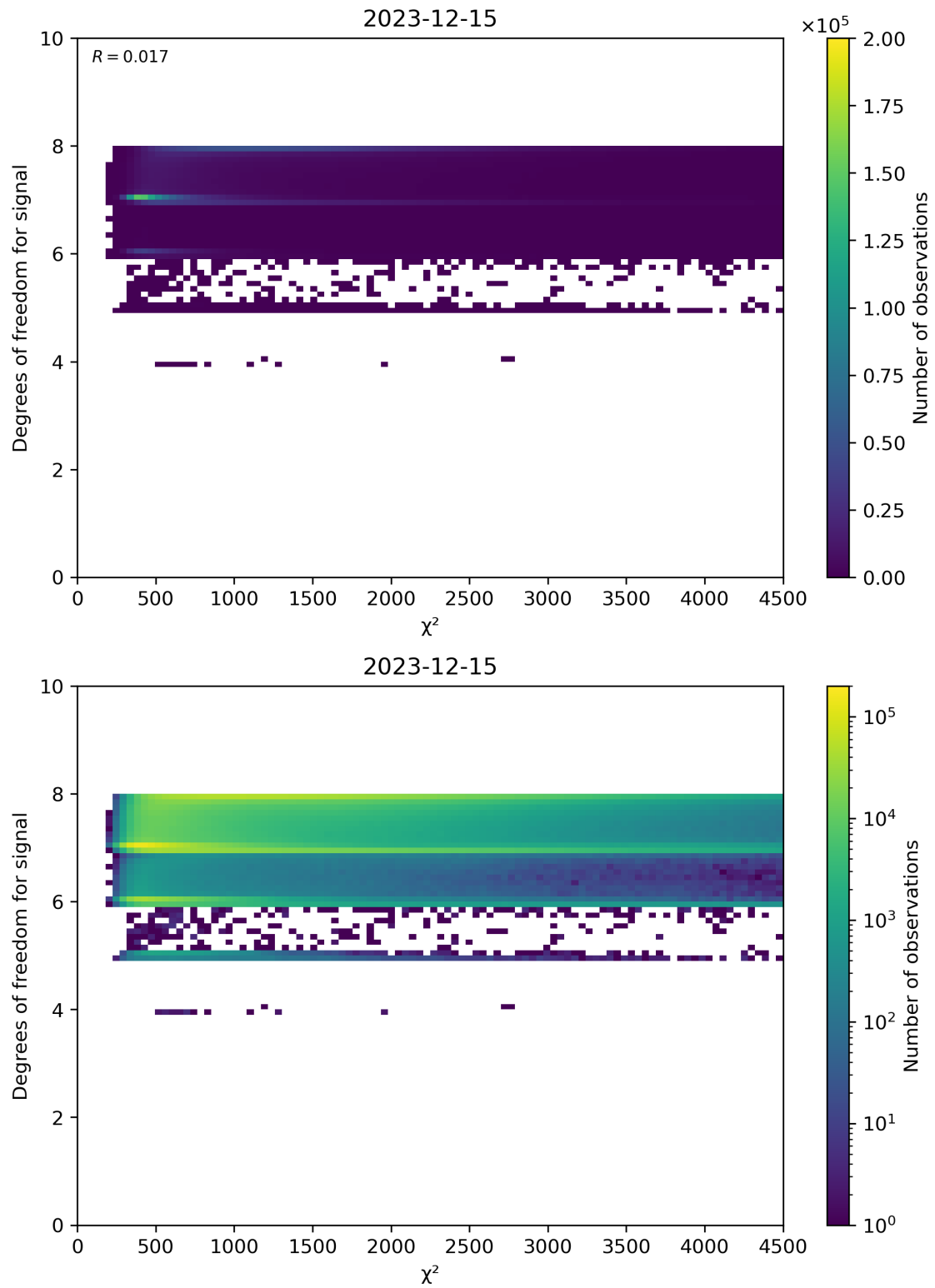
Figure 48: Scatter density plot of “ \chi^2 ” against “Degrees of freedom for signal” for 2023-12-14 to 2023-12-16.
