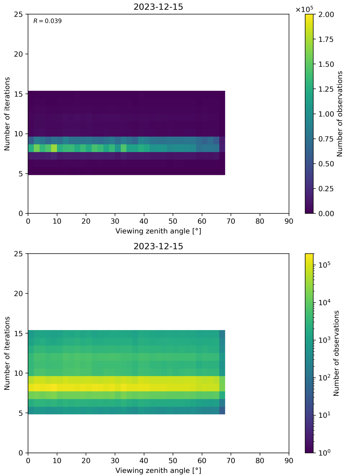
Figure 75: Scatter density plot of “Viewing zenith angle” against “Number of iterations” for 2023-12-14 to 2023-12-16.
