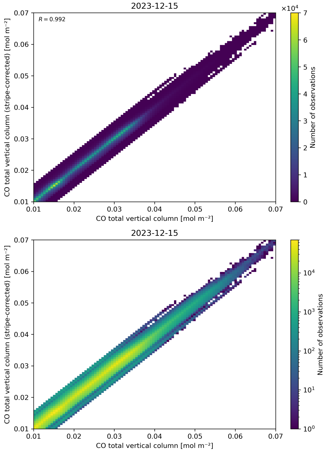
Figure 33: Scatter density plot of “CO total vertical column” against “CO total vertical column (stripe-corrected)” for 2023-12-14 to 2023-12-16.
