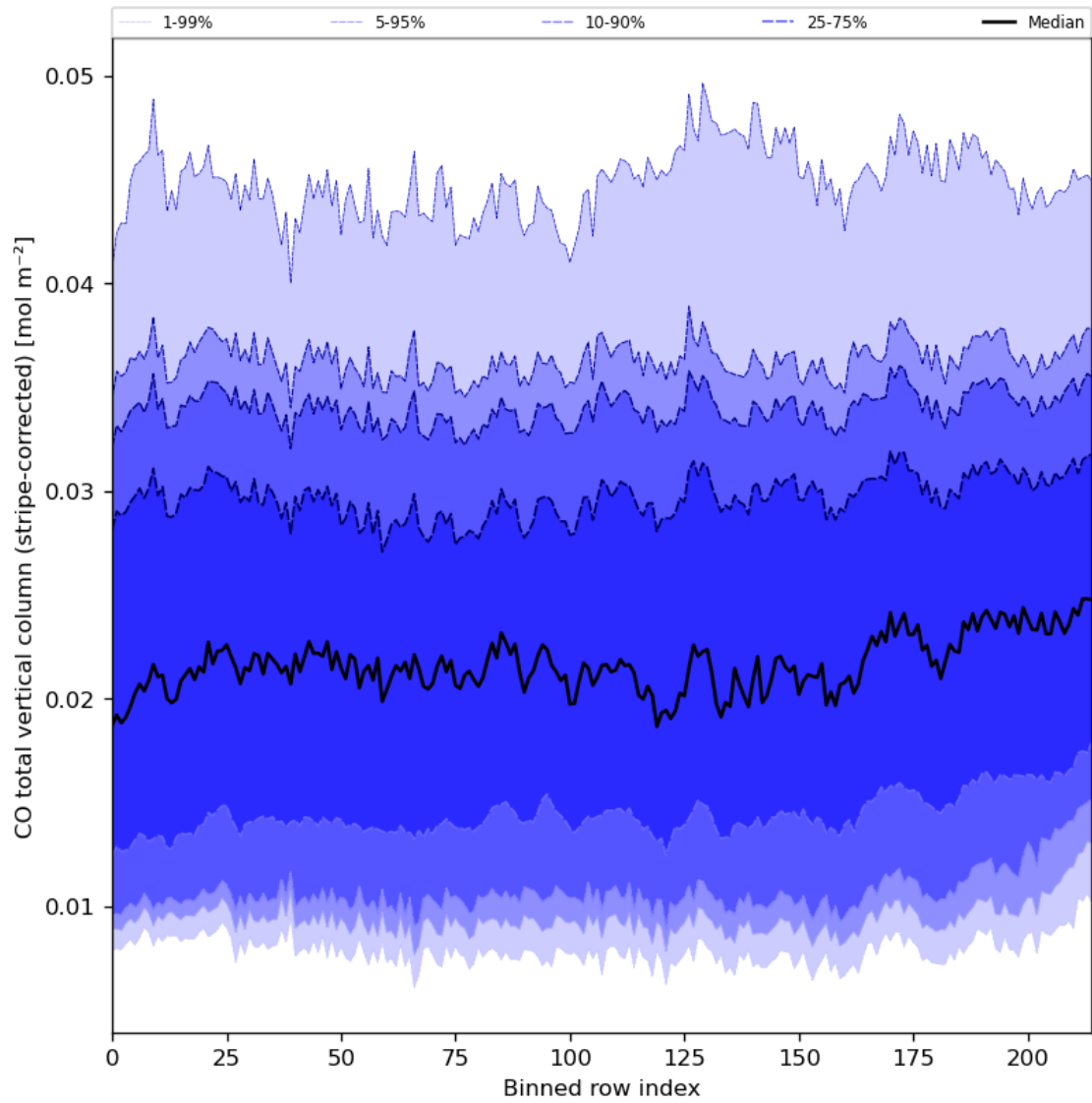
Figure 27: Along track statistics of “CO total vertical column (stripe-corrected)” for 2023-12-14 to 2023-12-16
