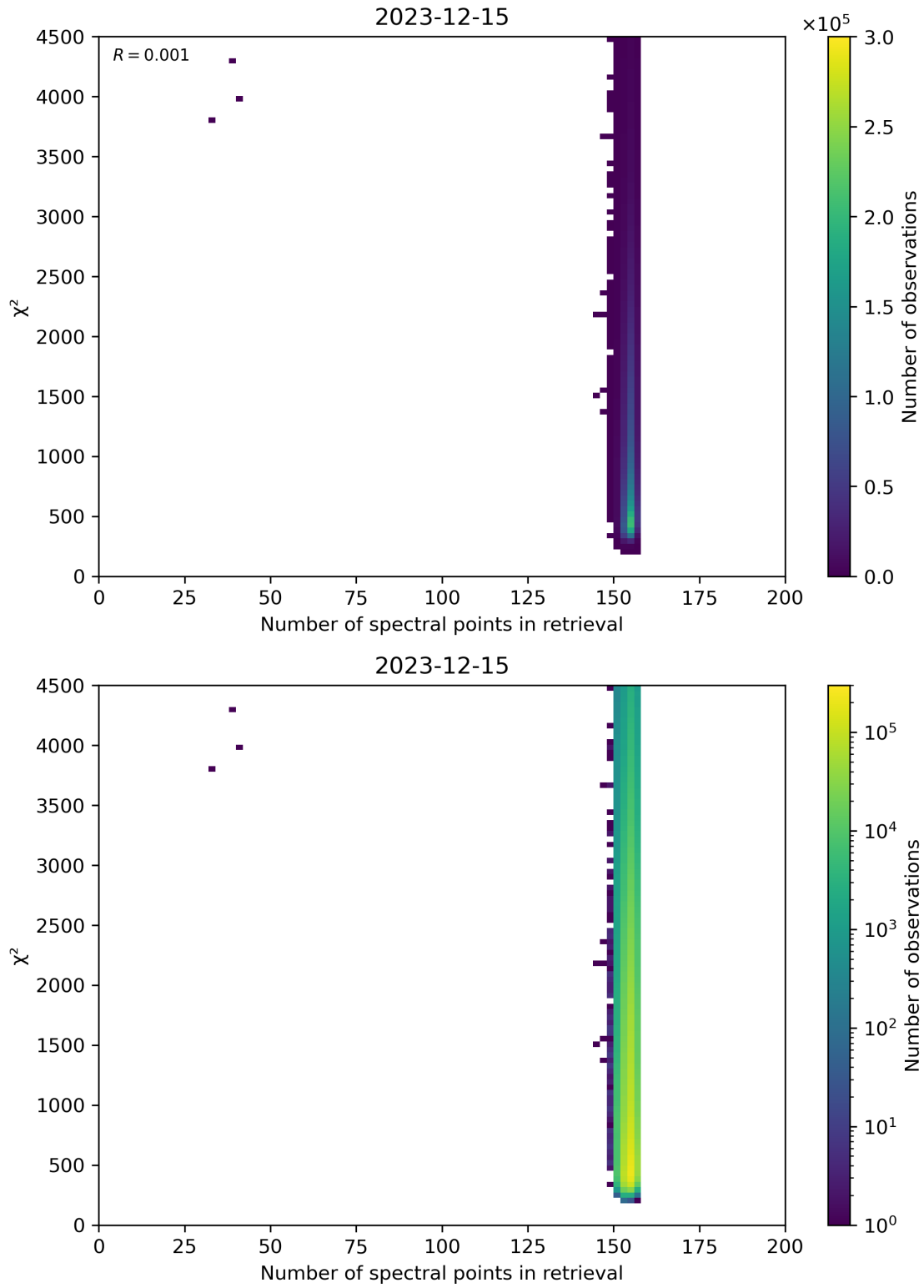
Figure 58: Scatter density plot of “Number of spectral points in retrieval” against “ \chi^2 ” for 2023-12-14 to 2023-12-16.
