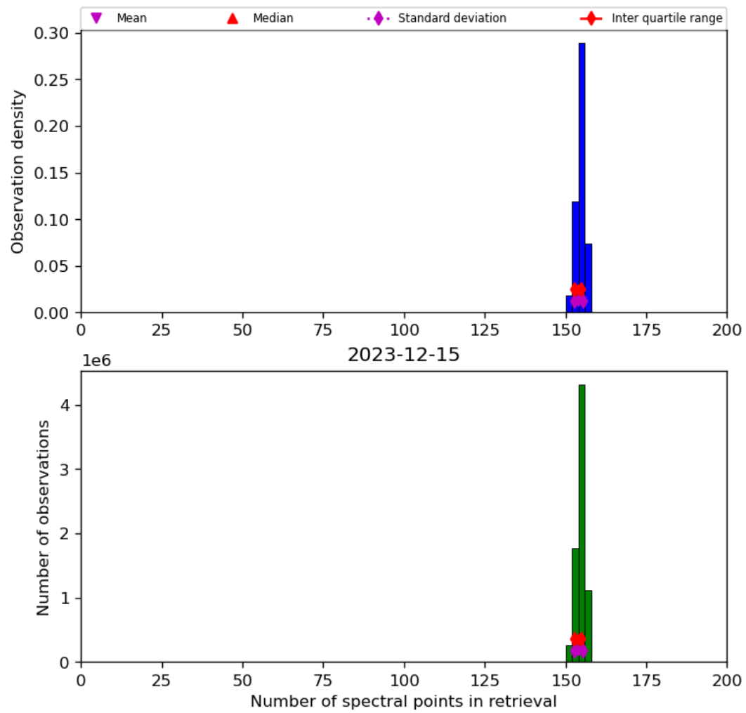
Figure 21: Histogram of “Number of spectral points in retrieval” for 2023-12-14 to 2023-12-16
