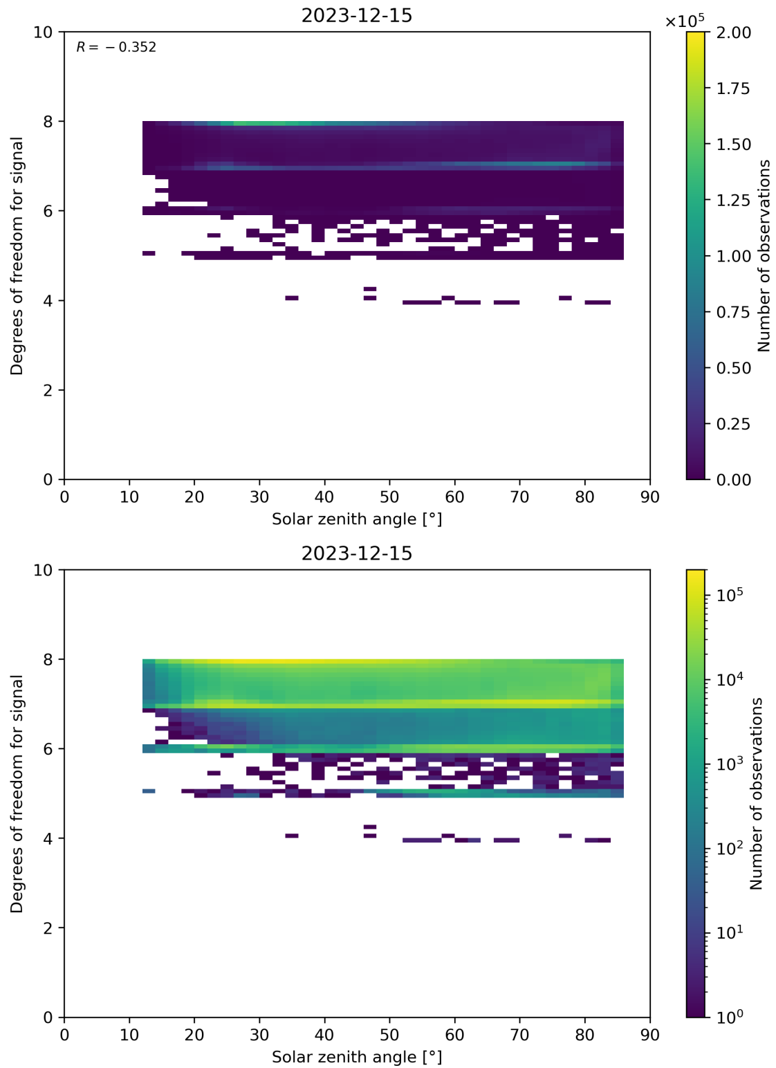
Figure 65: Scatter density plot of “Solar zenith angle” against “Degrees of freedom for signal” for 2023-12-14 to 2023-12-16.
