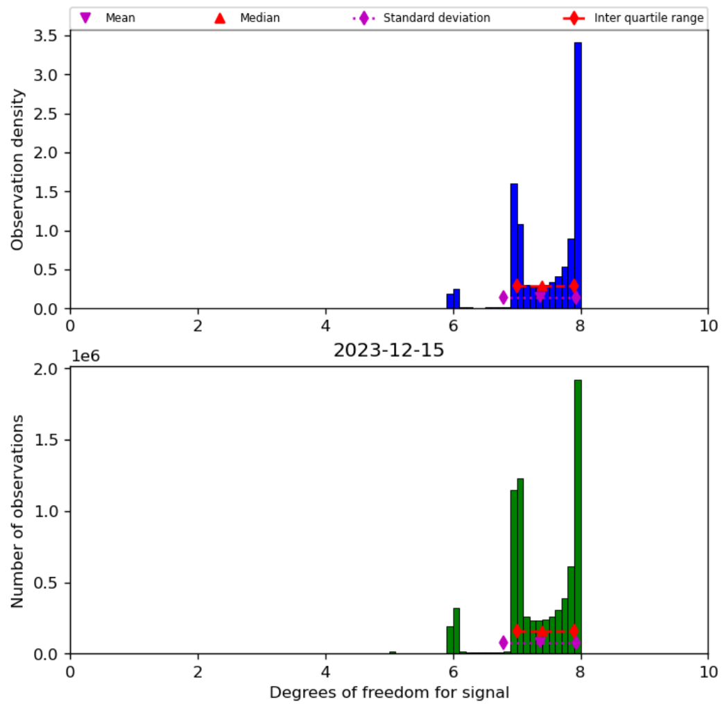
Figure 23: Histogram of “Degrees of freedom for signal” for 2023-12-14 to 2023-12-16
