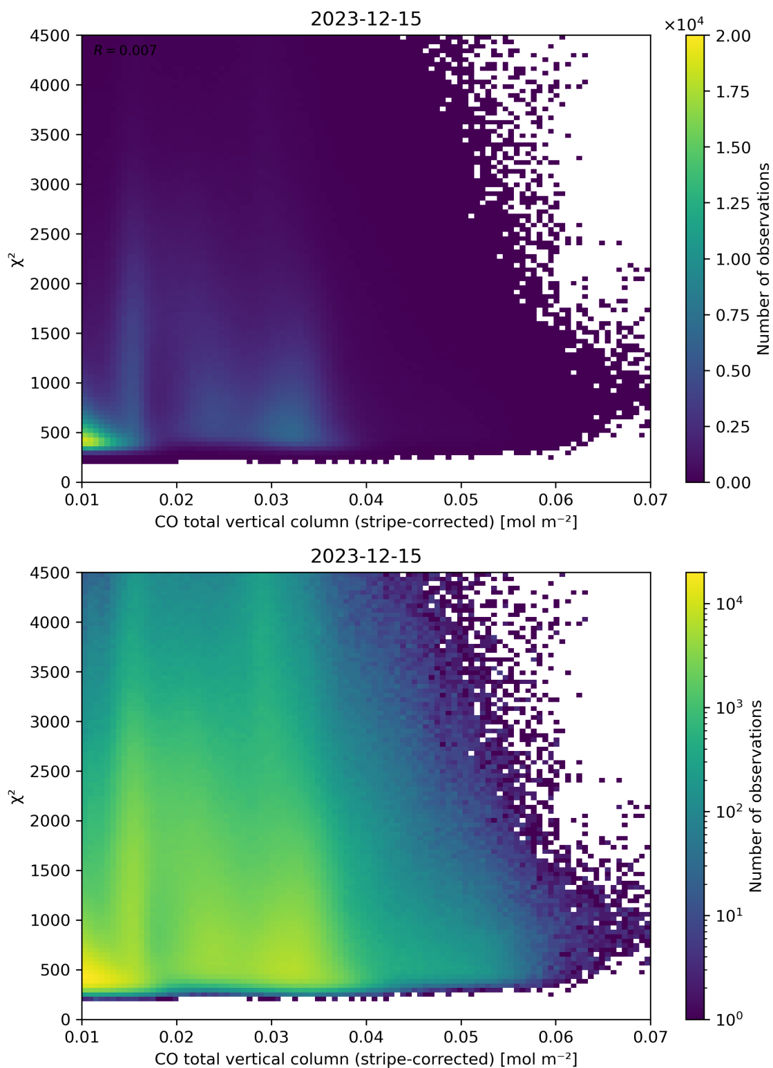
Figure 37: Scatter density plot of “CO total vertical column (stripe-corrected)” against “ \chi^2 ” for 2023-12-14 to 2023-12-16.
