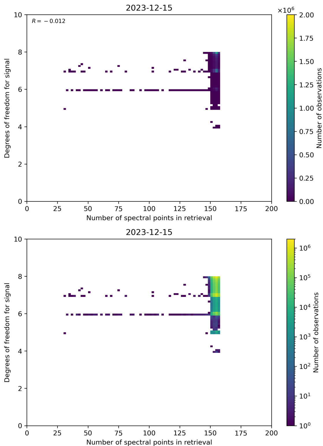
Figure 59: Scatter density plot of “Number of spectral points in retrieval” against “Degrees of freedom for signal” for 2023-12-14 to 2023-12-16.
