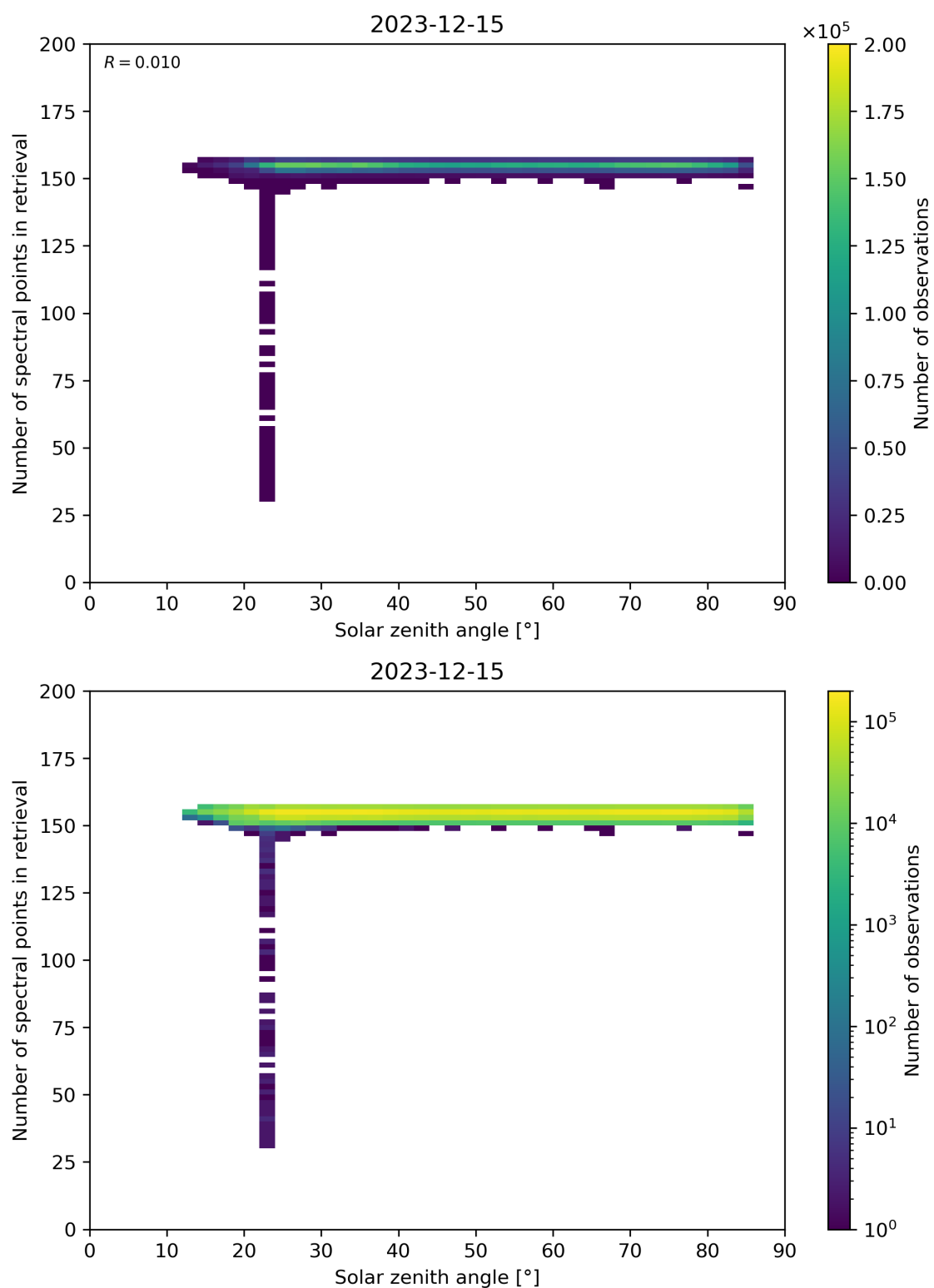
Figure 68: Scatter density plot of “Solar zenith angle” against “Number of spectral points in retrieval” for 2023-12-14 to 2023-12-16.
