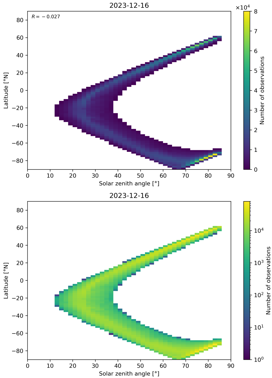
Figure 66: Scatter density plot of “Solar zenith angle” against “Latitude” for 2023-12-15 to 2023-12-17.
