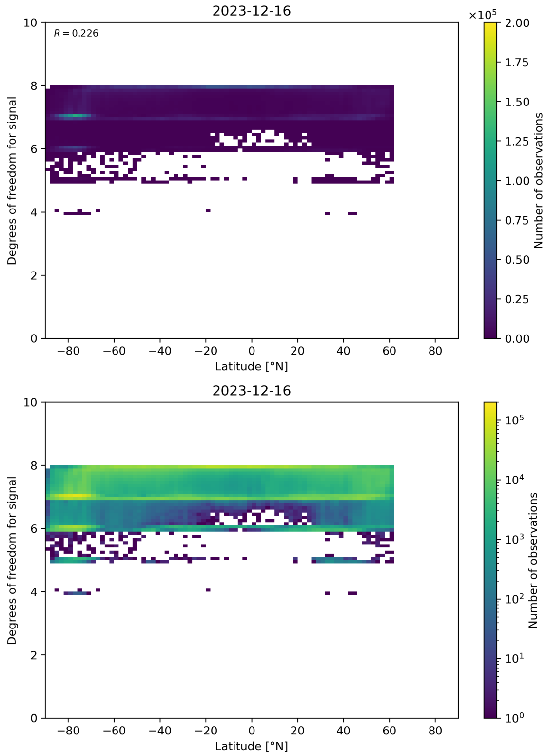
Figure 55: Scatter density plot of “Latitude” against “Degrees of freedom for signal” for 2023-12-15 to 2023-12-17.
