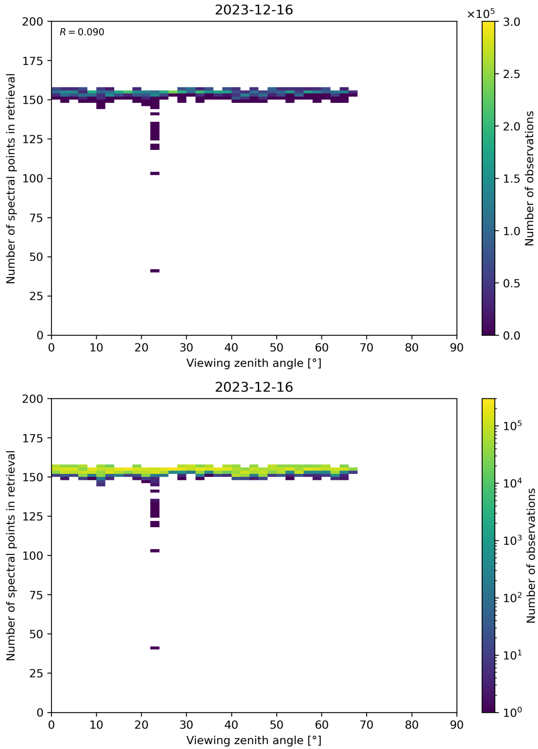
Figure 76: Scatter density plot of “Viewing zenith angle” against “Number of spectral points in retrieval” for 2023-12-15 to 2023-12-17.
