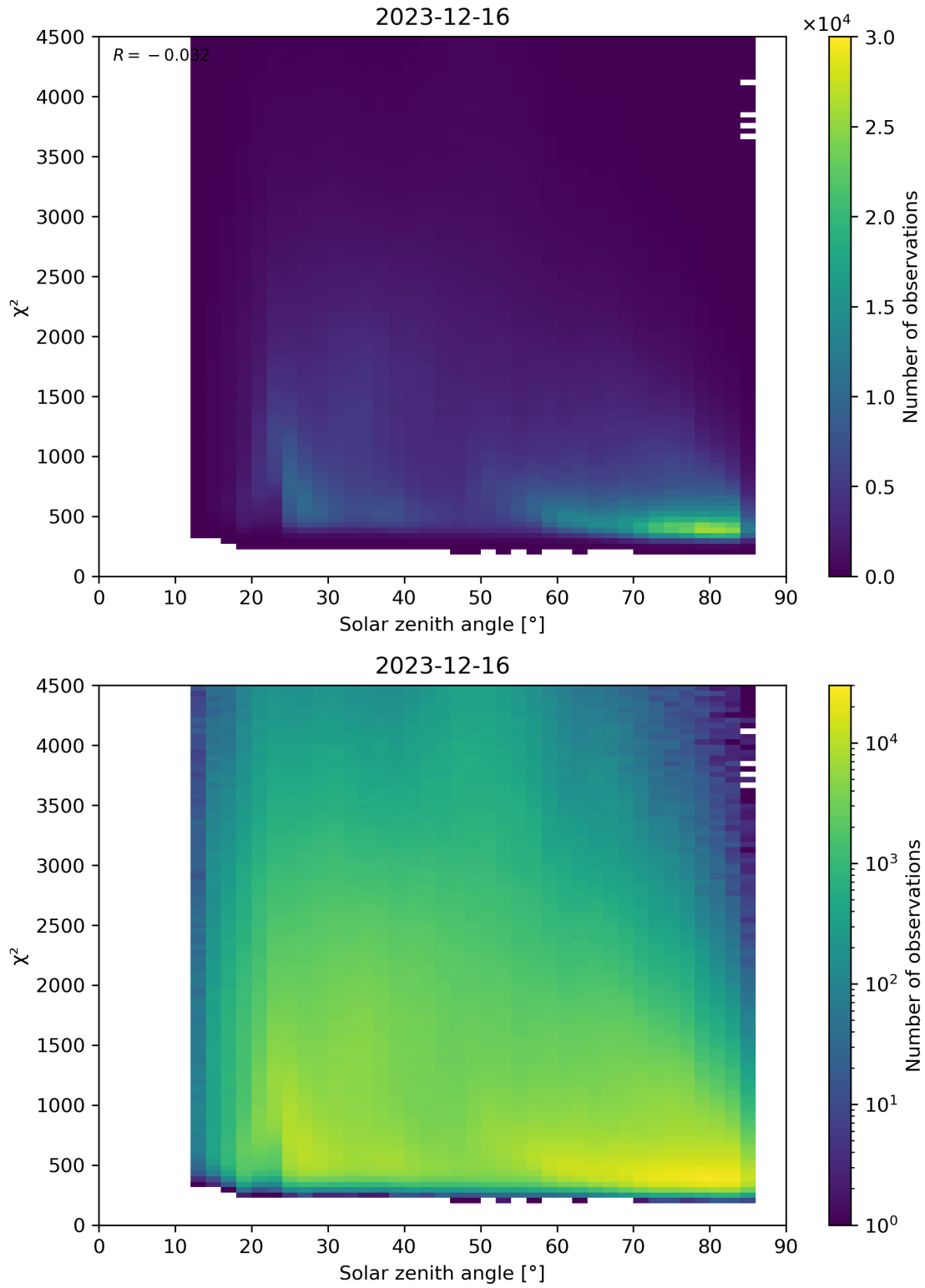
Figure 64: Scatter density plot of “Solar zenith angle” against “ \chi^2 ” for 2023-12-15 to 2023-12-17.
