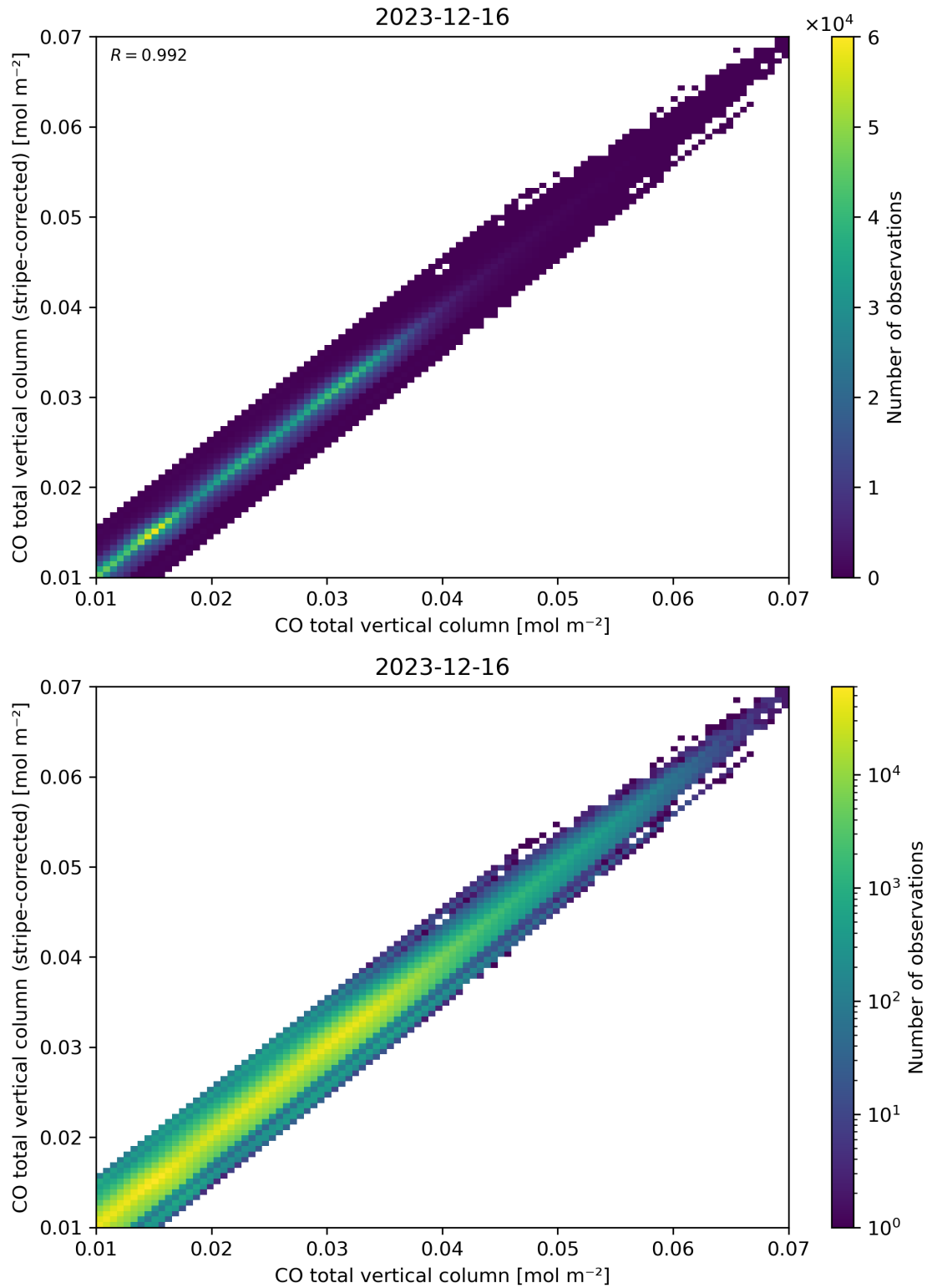
Figure 33: Scatter density plot of “CO total vertical column” against “CO total vertical column (stripe-corrected)” for 2023-12-15 to 2023-12-17.
