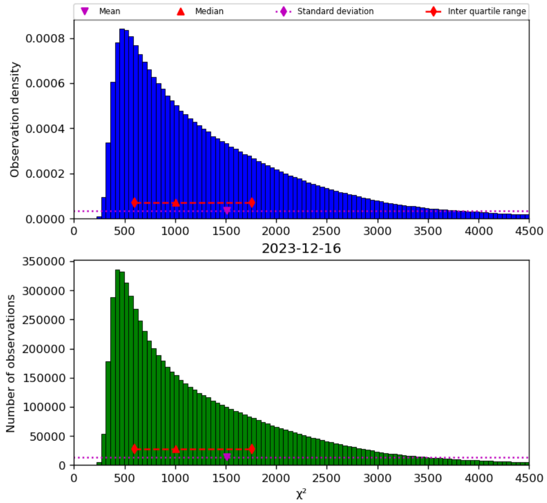
Figure 22: Histogram of “ \chi^2 ” for 2023-12-15 to 2023-12-17
