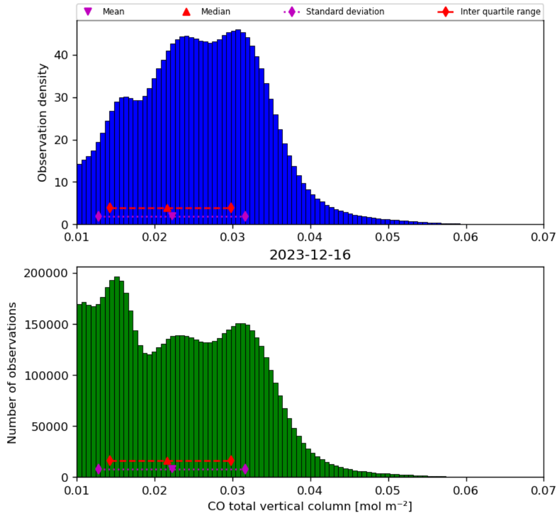
Figure 18: Histogram of “CO total vertical column” for 2023-12-15 to 2023-12-17
