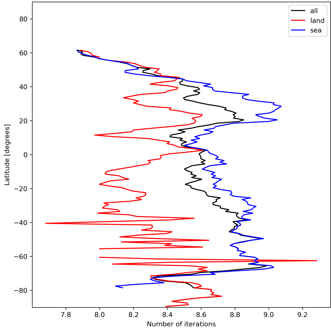
Figure 16: Zonal average of “Number of iterations” for 2023-12-15 to 2023-12-17.
