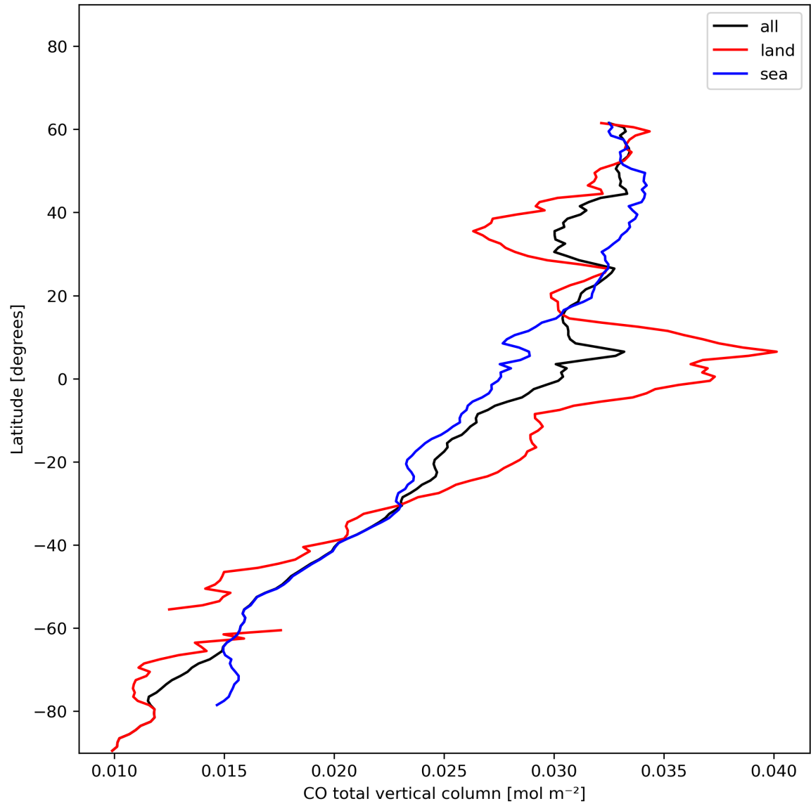
Figure 10: Zonal average of “CO total vertical column” for 2023-12-15 to 2023-12-17.
