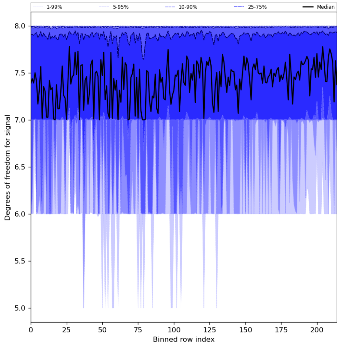
Figure 31: Along track statistics of “Degrees of freedom for signal” for 2023-12-15 to 2023-12-17
