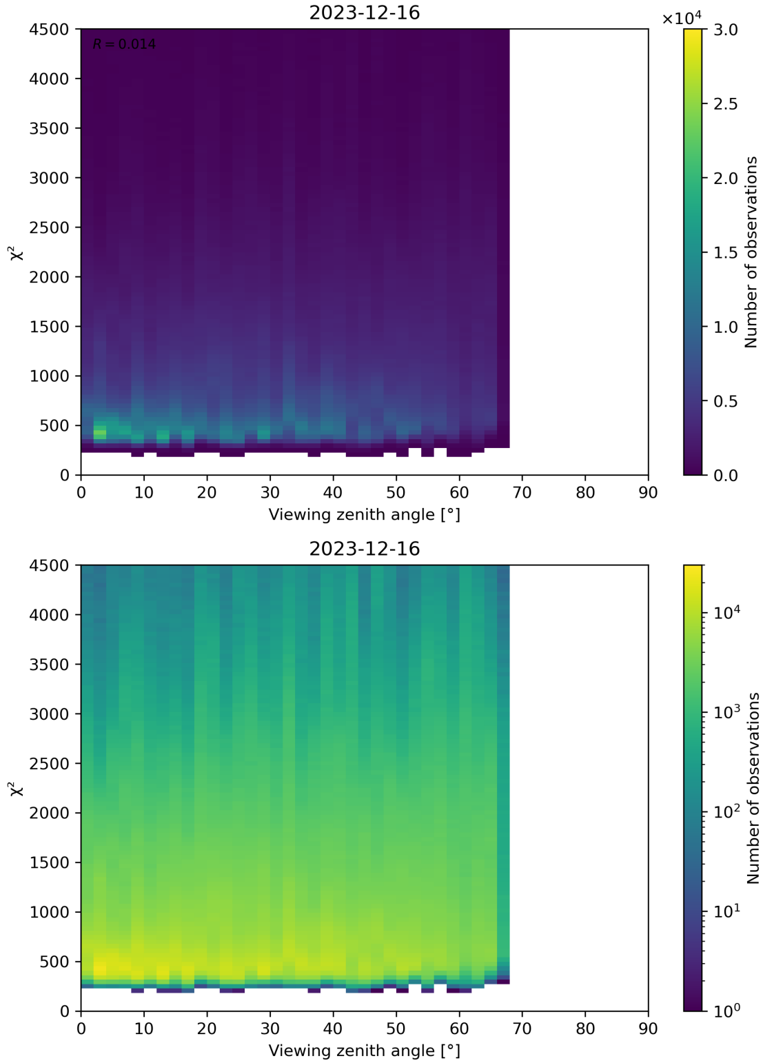
Figure 72: Scatter density plot of “Viewing zenith angle” against “ \chi^2 ” for 2023-12-15 to 2023-12-17.
