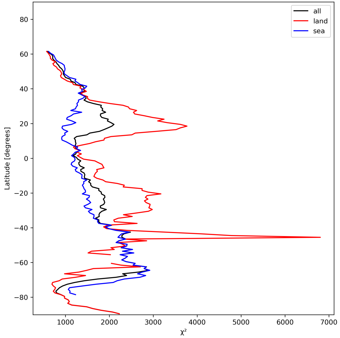
Figure 14: Zonal average of “ \chi^2 ” for 2023-12-15 to 2023-12-17.
