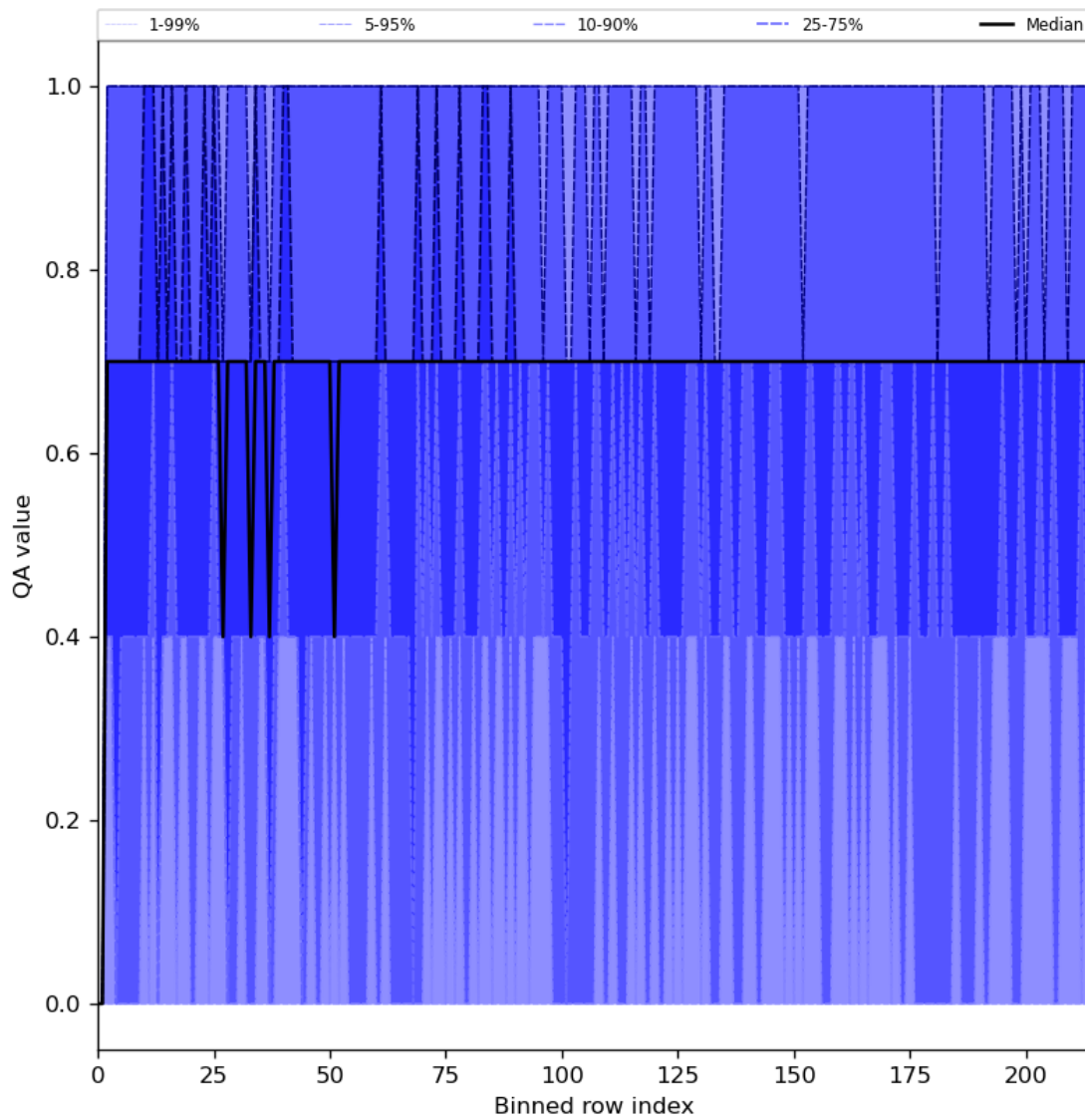
Figure 25: Along track statistics of “QA value” for 2023-12-15 to 2023-12-17
