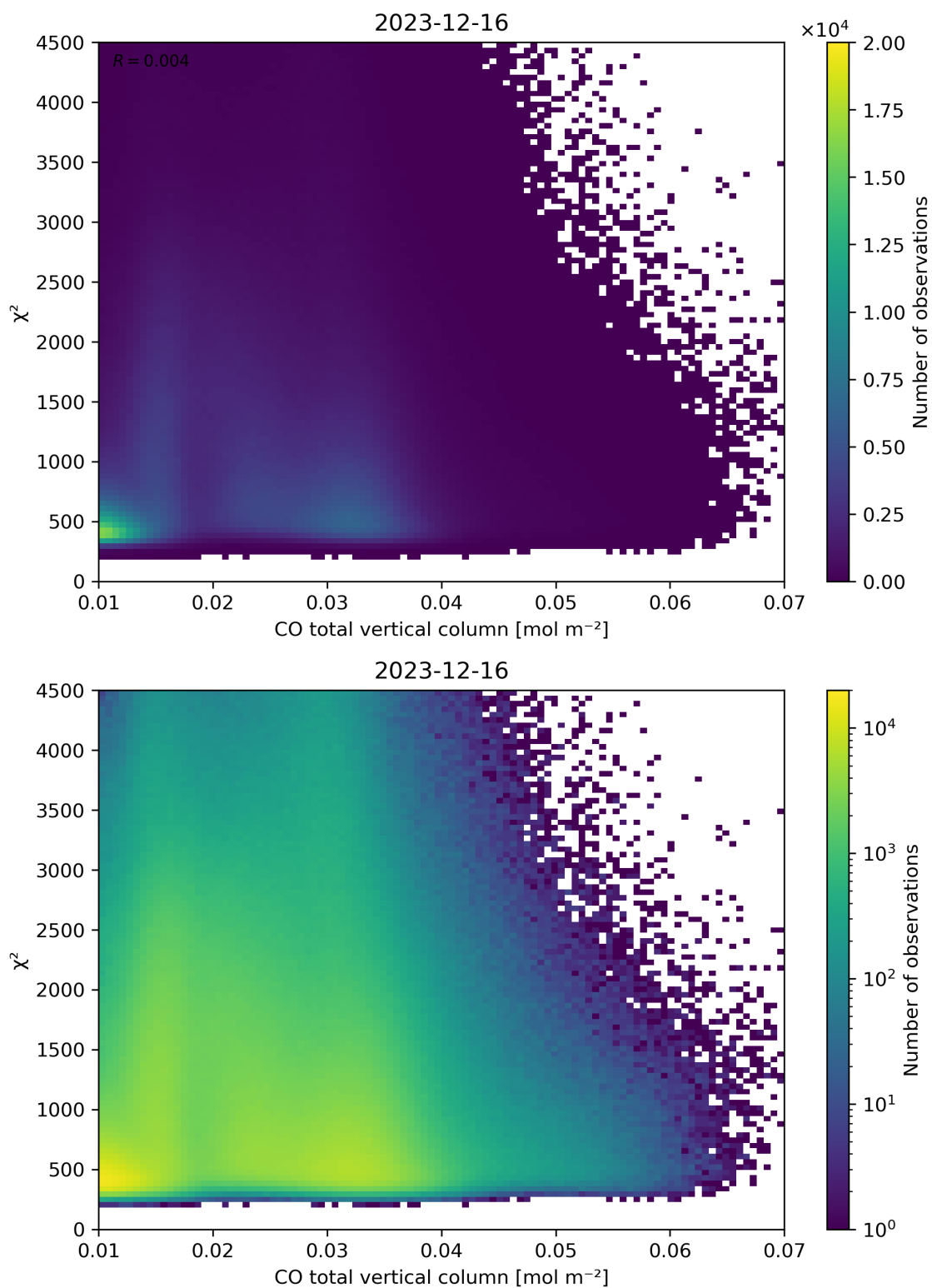
Figure 35: Scatter density plot of “CO total vertical column” against “ \chi^2 ” for 2023-12-15 to 2023-12-17.
