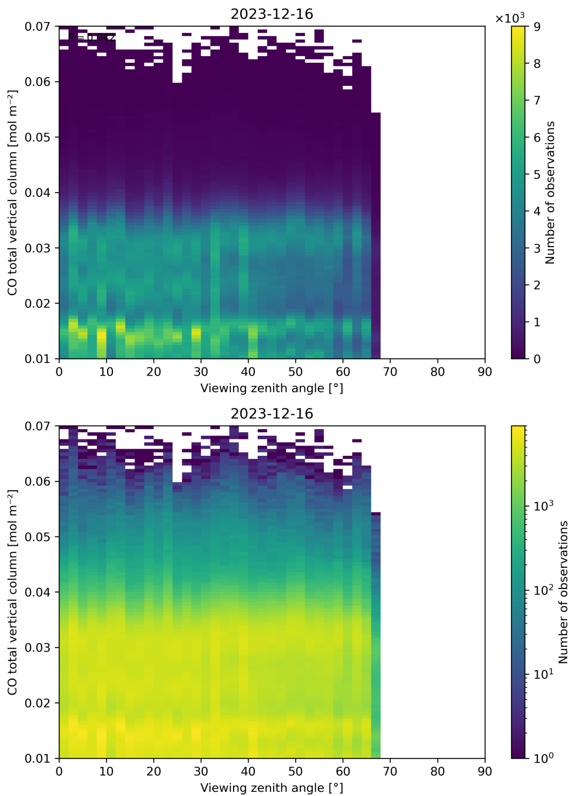
Figure 69: Scatter density plot of “Viewing zenith angle” against “CO total vertical column” for 2023-12-15 to 2023-12-17.
