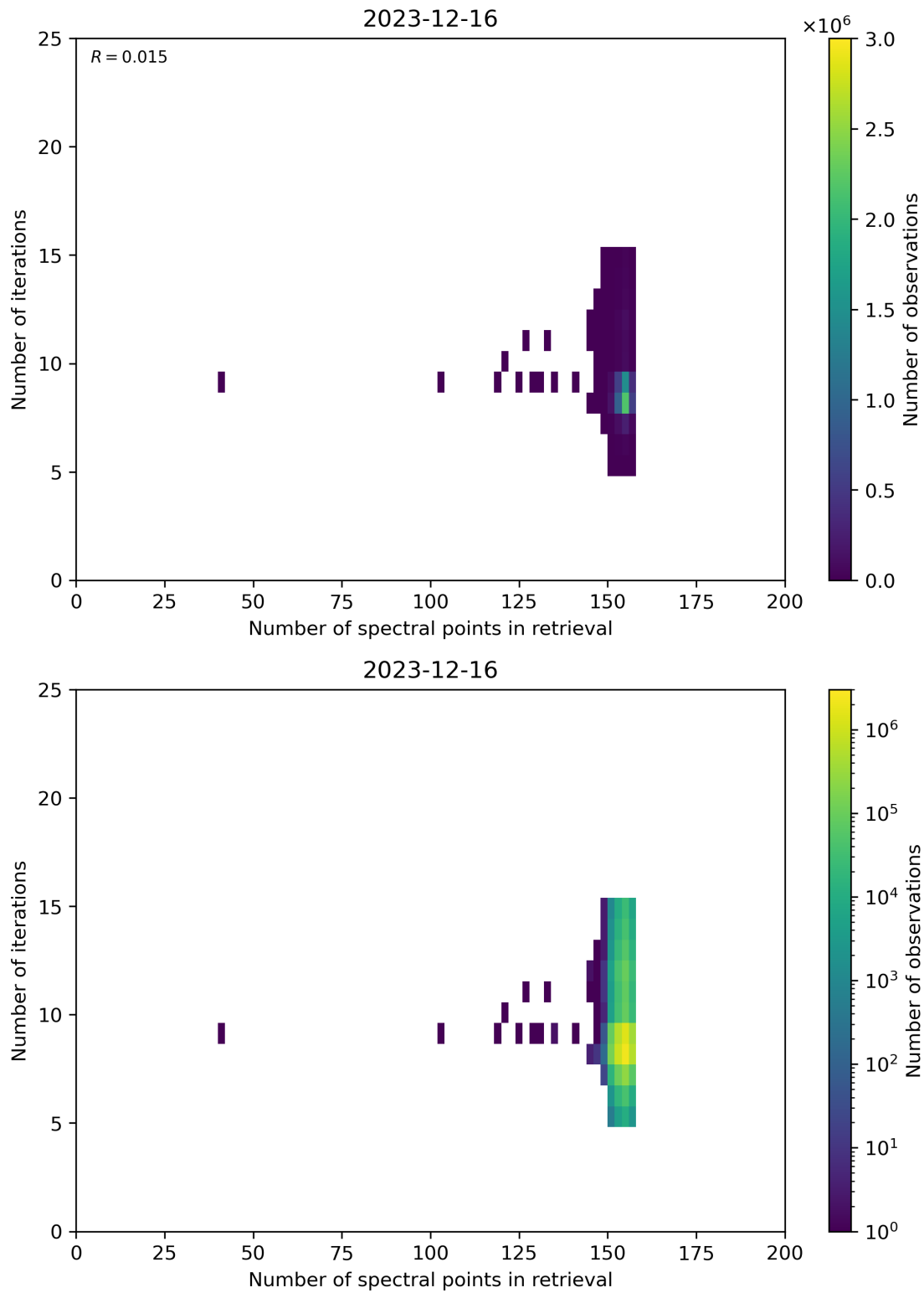
Figure 60: Scatter density plot of “Number of spectral points in retrieval” against “Number of iterations” for 2023-12-15 to 2023-12-17.
