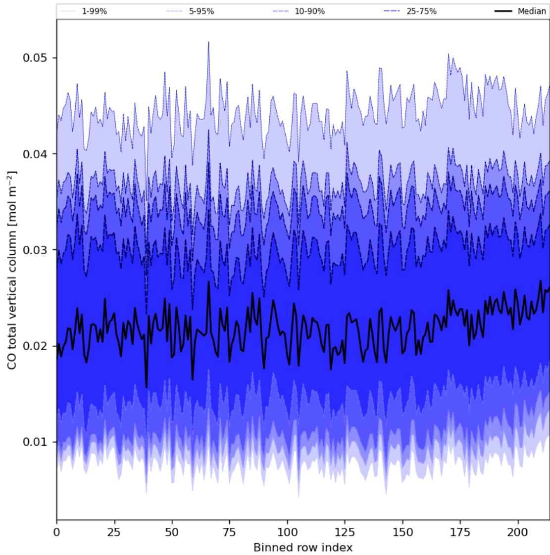
Figure 26: Along track statistics of “CO total vertical column” for 2023-12-15 to 2023-12-17
