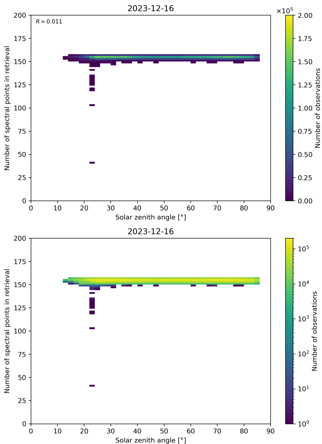
Figure 68: Scatter density plot of “Solar zenith angle” against “Number of spectral points in retrieval” for 2023-12-15 to 2023-12-17.
