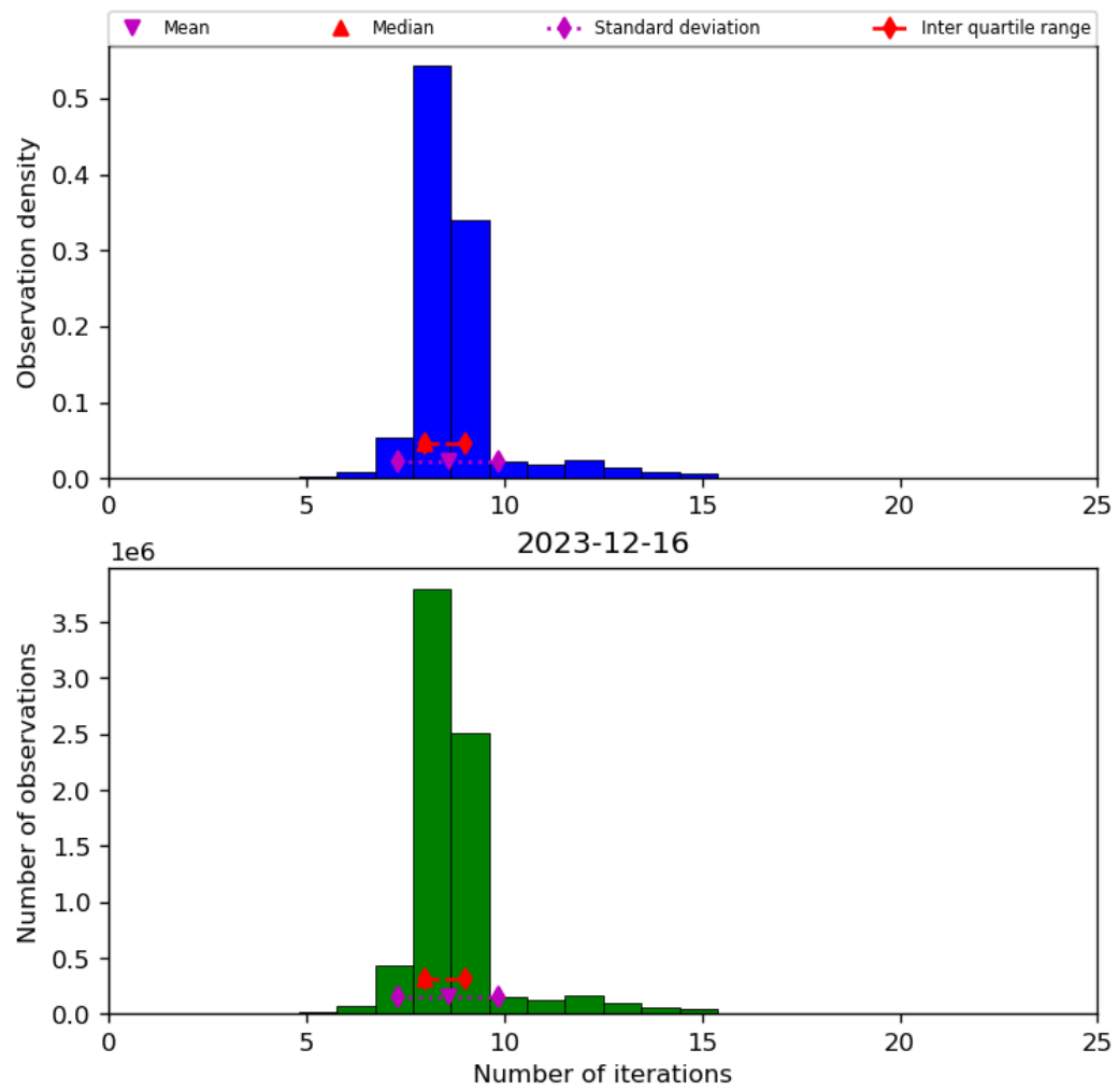
Figure 24: Histogram of “Number of iterations” for 2023-12-15 to 2023-12-17
