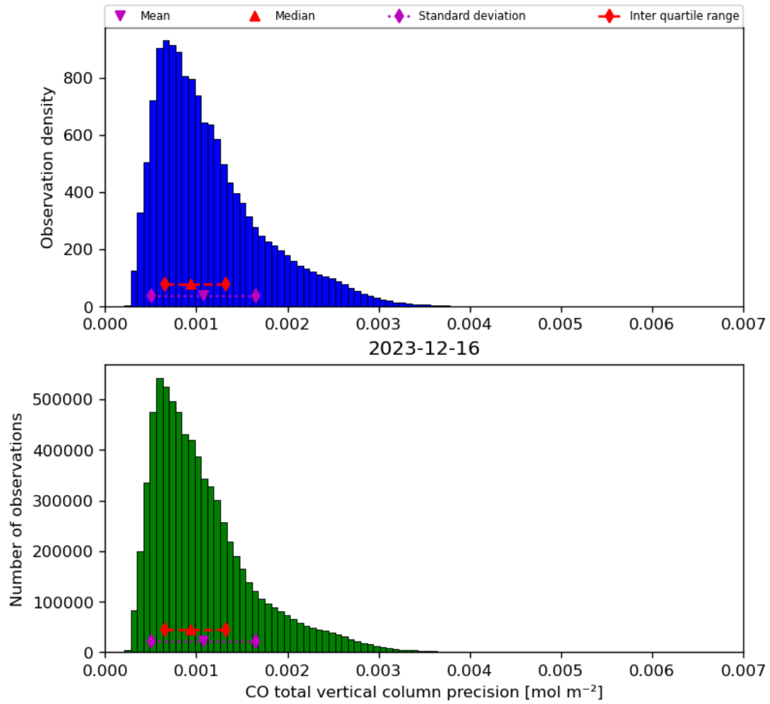
Figure 20: Histogram of “CO total vertical column precision” for 2023-12-15 to 2023-12-17
