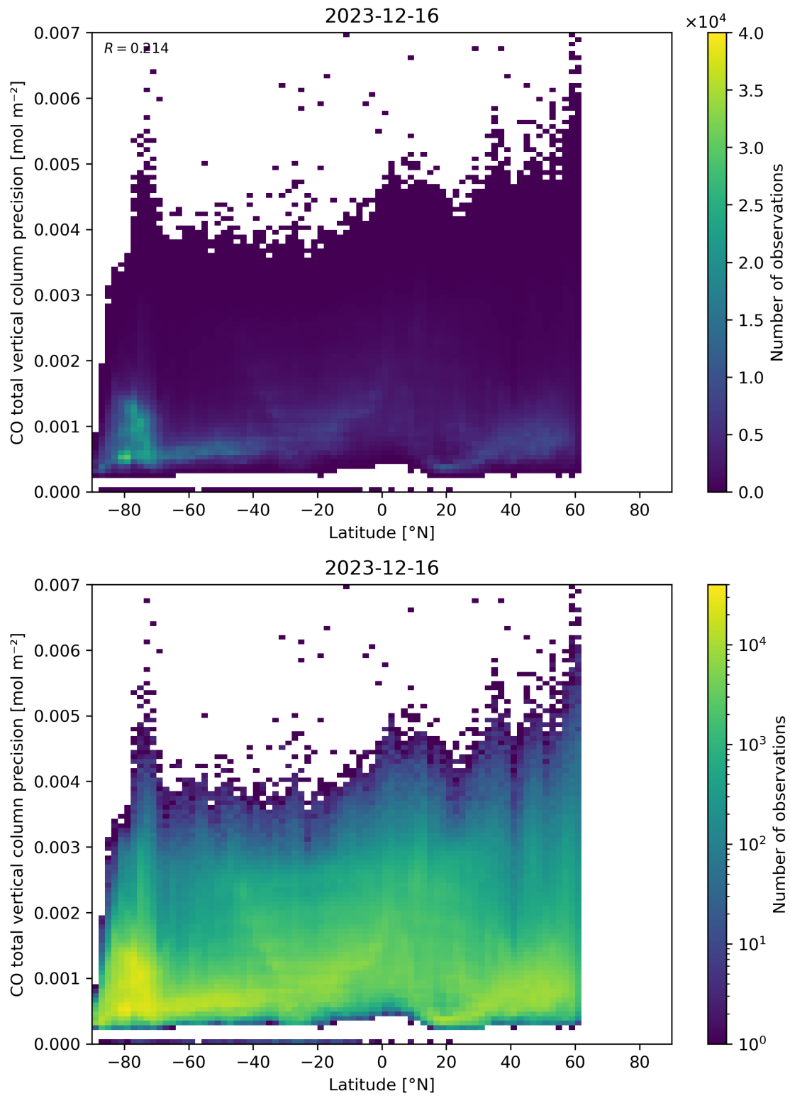
Figure 53: Scatter density plot of “Latitude” against “CO total vertical column precision” for 2023-12-15 to 2023-12-17.
