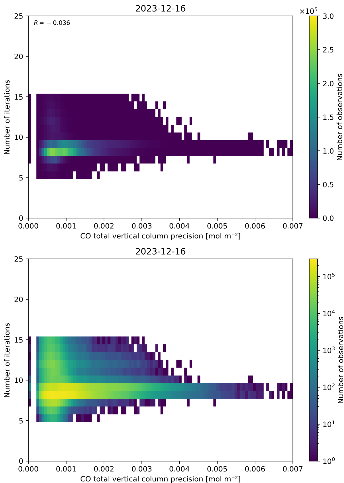
Figure 46: Scatter density plot of “CO total vertical column precision” against “Number of iterations” for 2023-12-15 to 2023-12-17.
