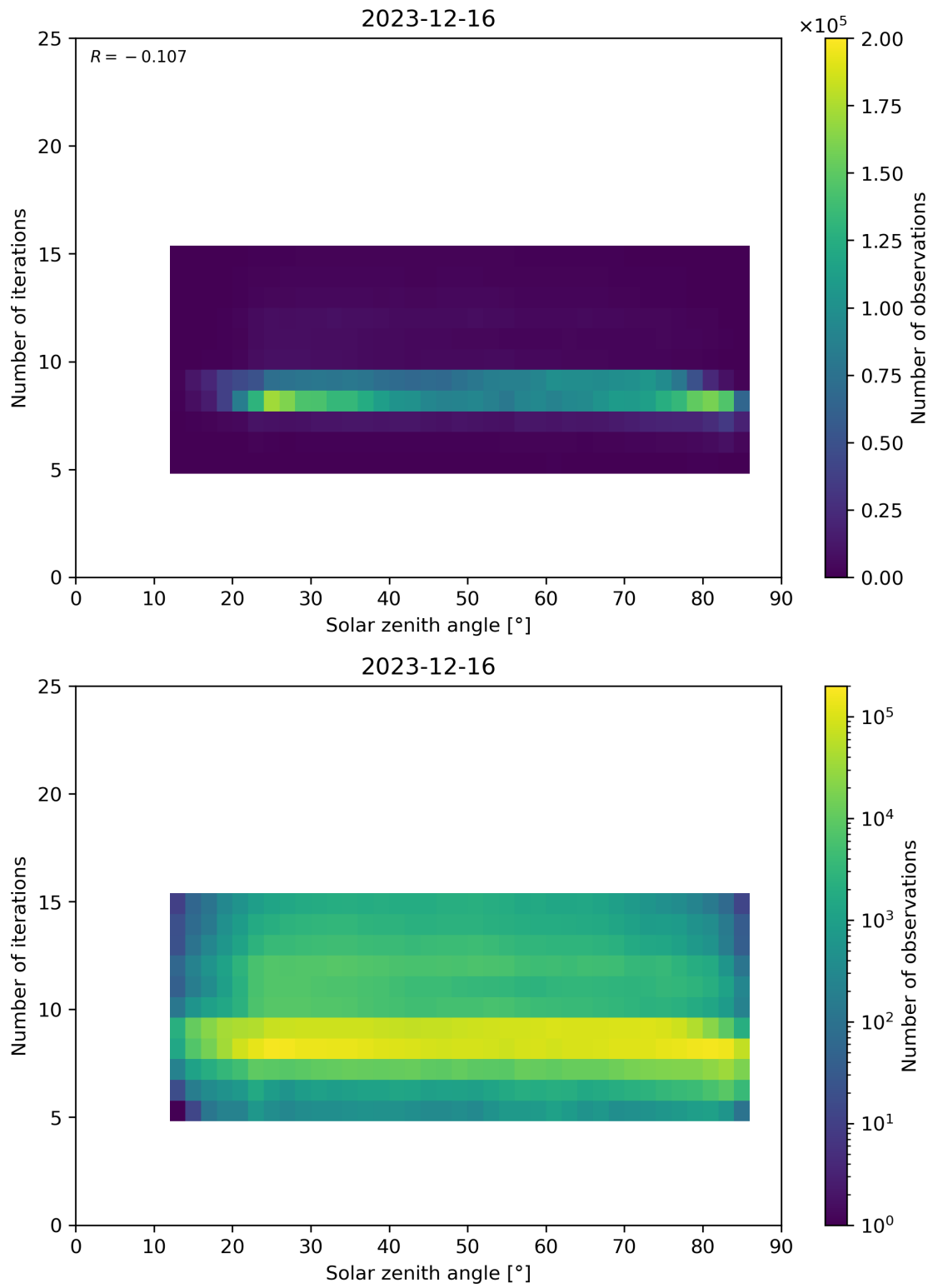
Figure 67: Scatter density plot of “Solar zenith angle” against “Number of iterations” for 2023-12-15 to 2023-12-17.
