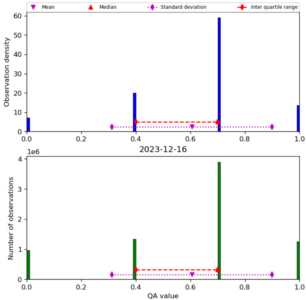
Figure 17: Histogram of “QA value” for 2023-12-15 to 2023-12-17
