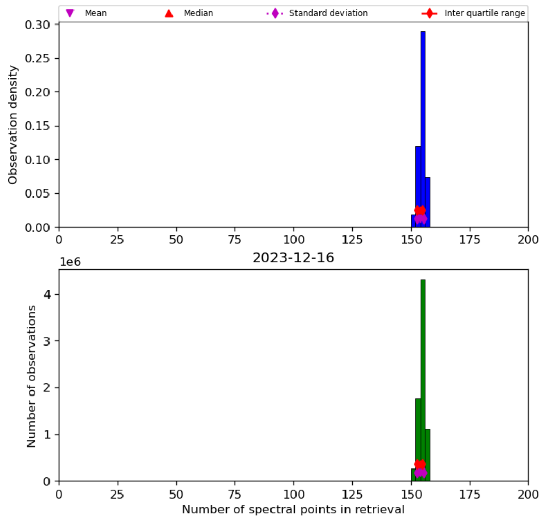
Figure 21: Histogram of “Number of spectral points in retrieval” for 2023-12-15 to 2023-12-17
