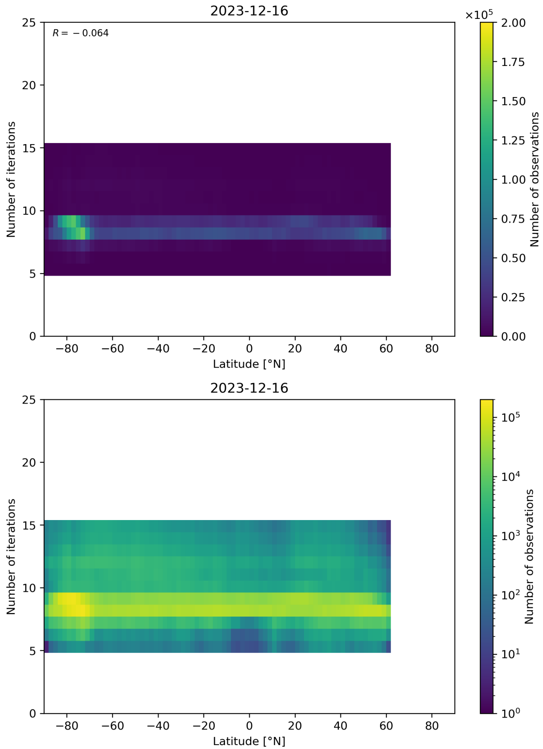
Figure 56: Scatter density plot of “Latitude” against “Number of iterations” for 2023-12-15 to 2023-12-17.
