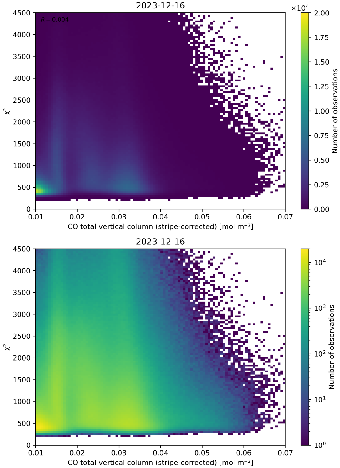
Figure 37: Scatter density plot of “CO total vertical column (stripe-corrected)” against “ \chi^2 ” for 2023-12-15 to 2023-12-17.
