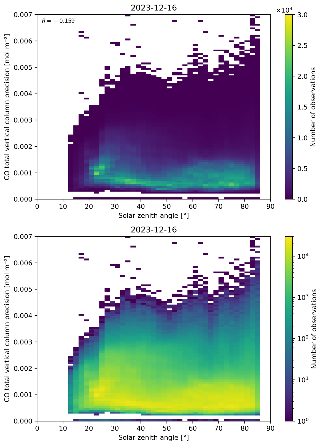
Figure 63: Scatter density plot of “Solar zenith angle” against “CO total vertical column precision” for 2023-12-15 to 2023-12-17.
