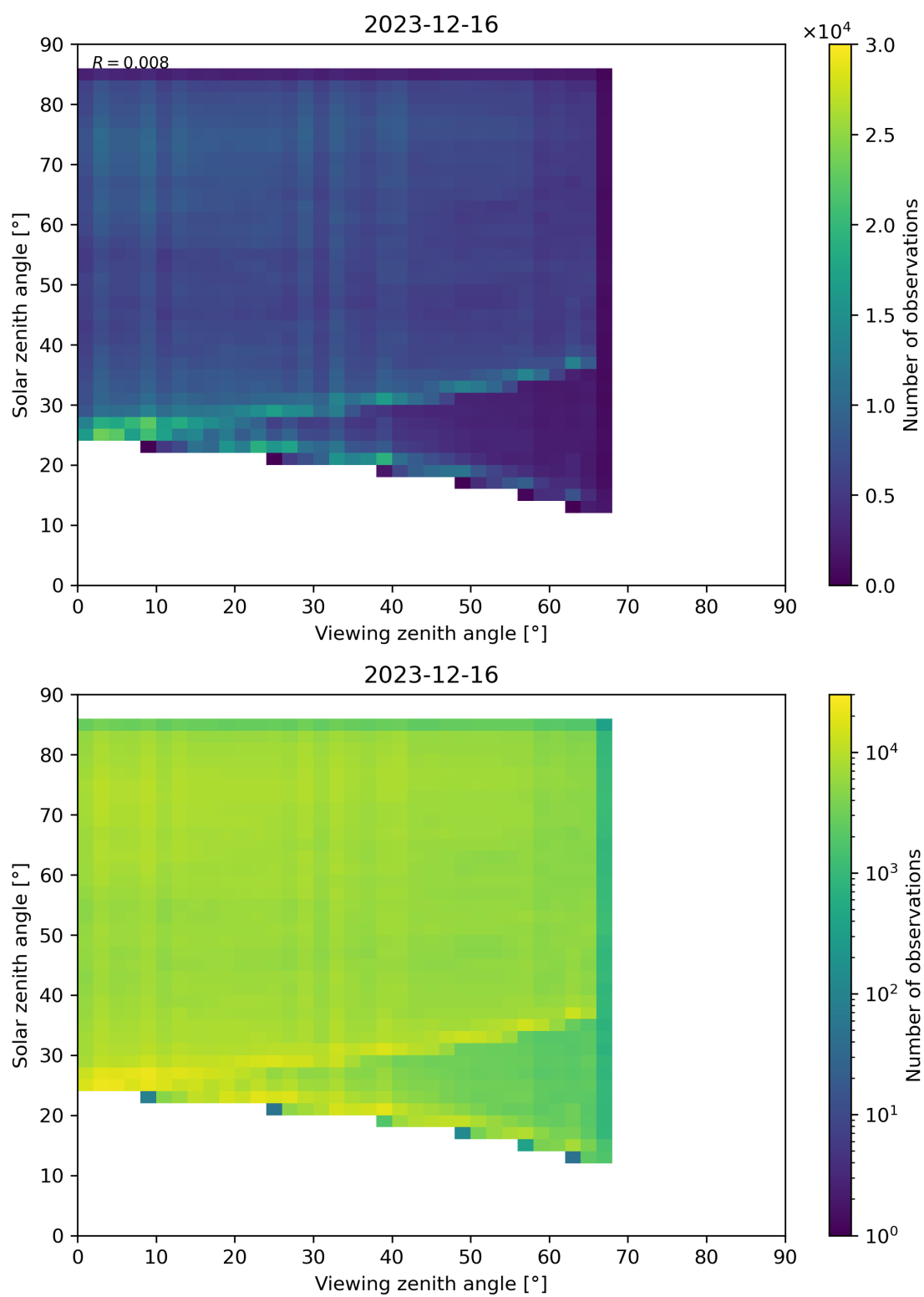
Figure 77: Scatter density plot of “Viewing zenith angle” against “Solar zenith angle” for 2023-12-15 to 2023-12-17.
