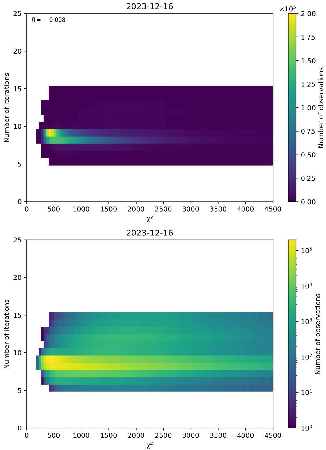
Figure 49: Scatter density plot of “ \chi^2 ” against “Number of iterations” for 2023-12-15 to 2023-12-17.
