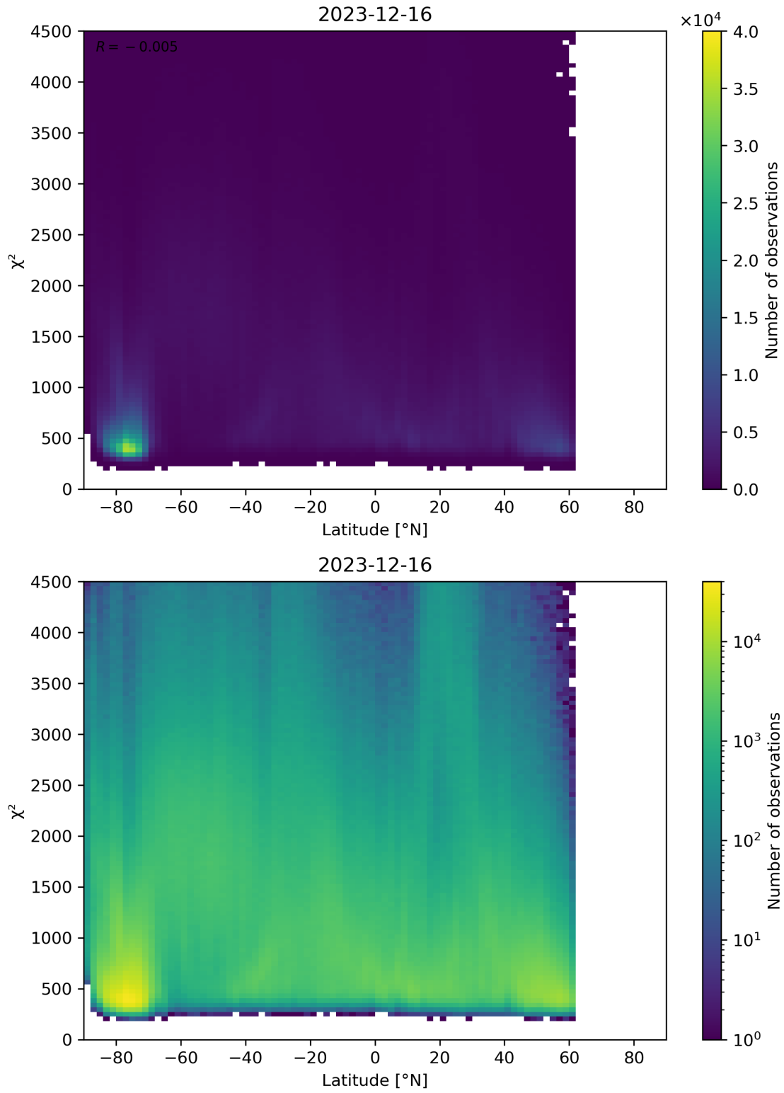
Figure 54: Scatter density plot of “Latitude” against “ \chi^2 ” for 2023-12-15 to 2023-12-17.
