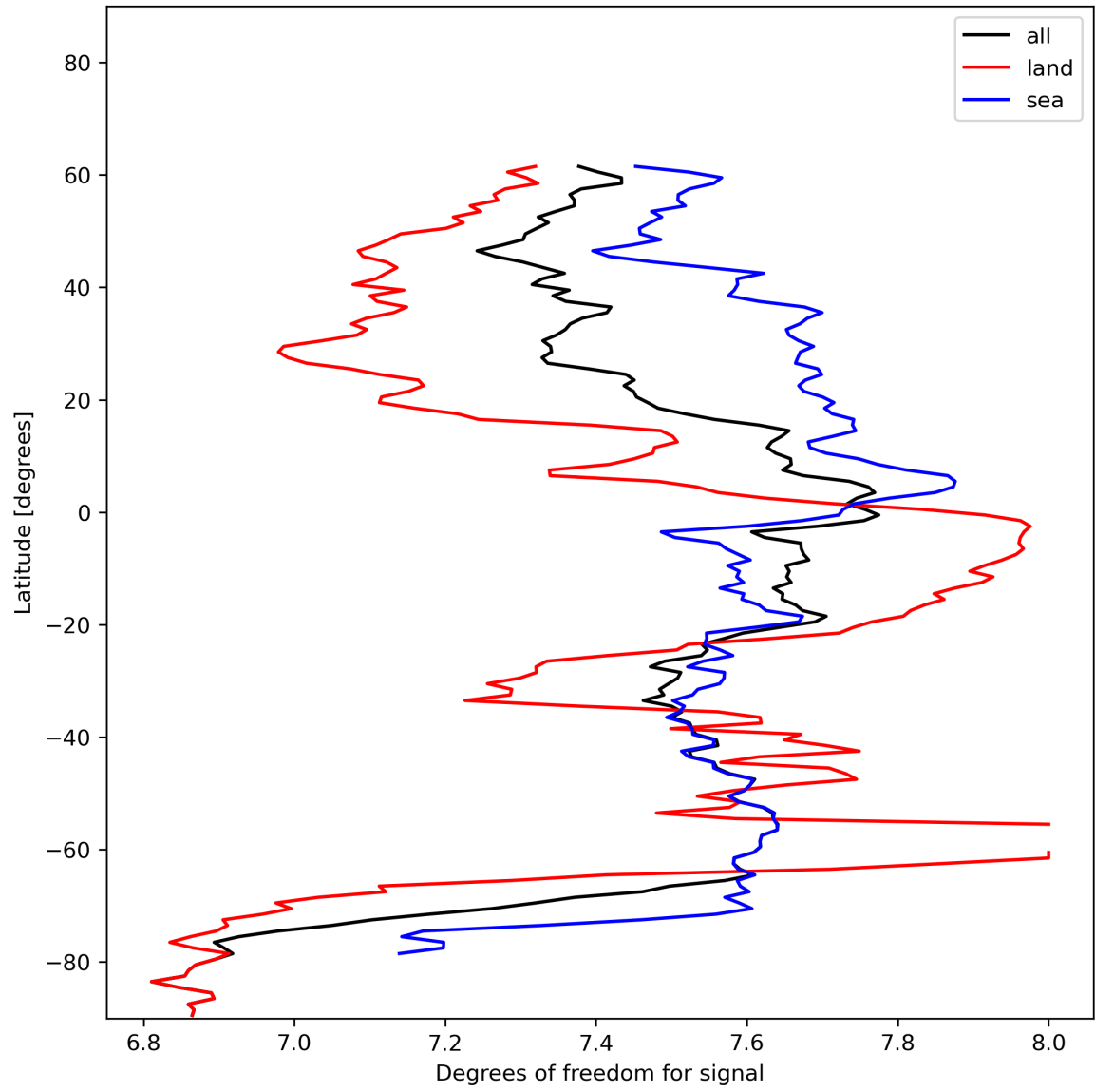
Figure 15: Zonal average of “Degrees of freedom for signal” for 2023-12-15 to 2023-12-17.
