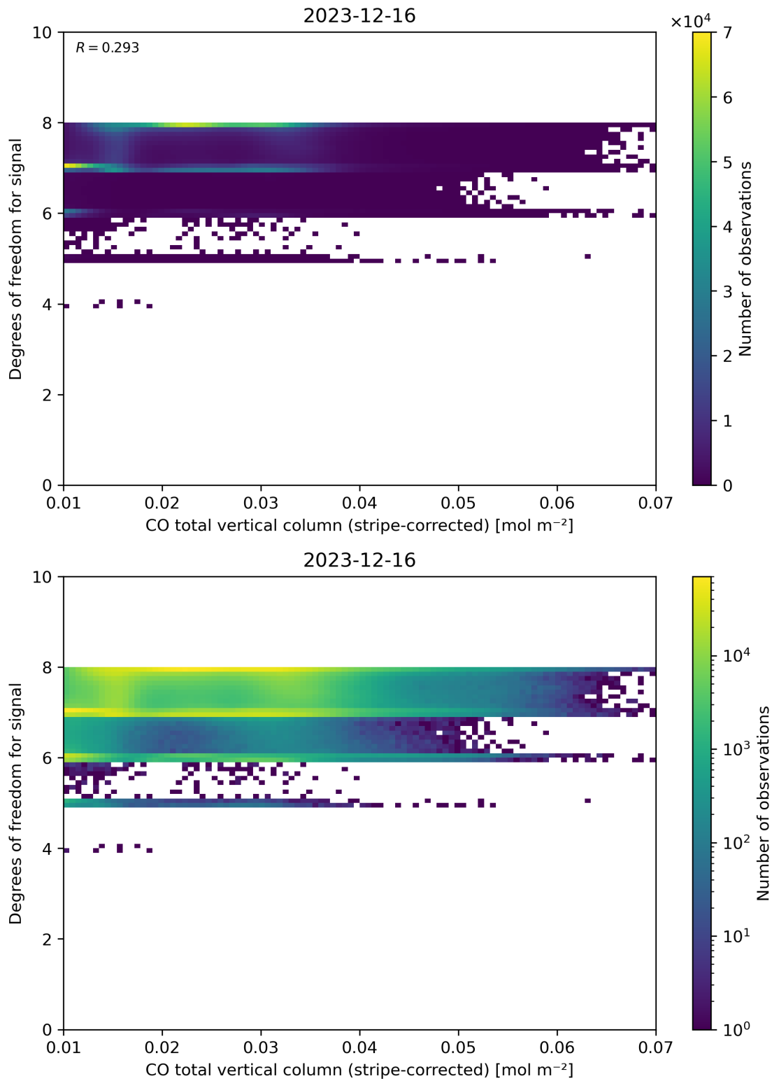
Figure 38: Scatter density plot of “CO total vertical column (stripe-corrected)” against “Degrees of freedom for signal” for 2023-12-15 to 2023-12-17.
