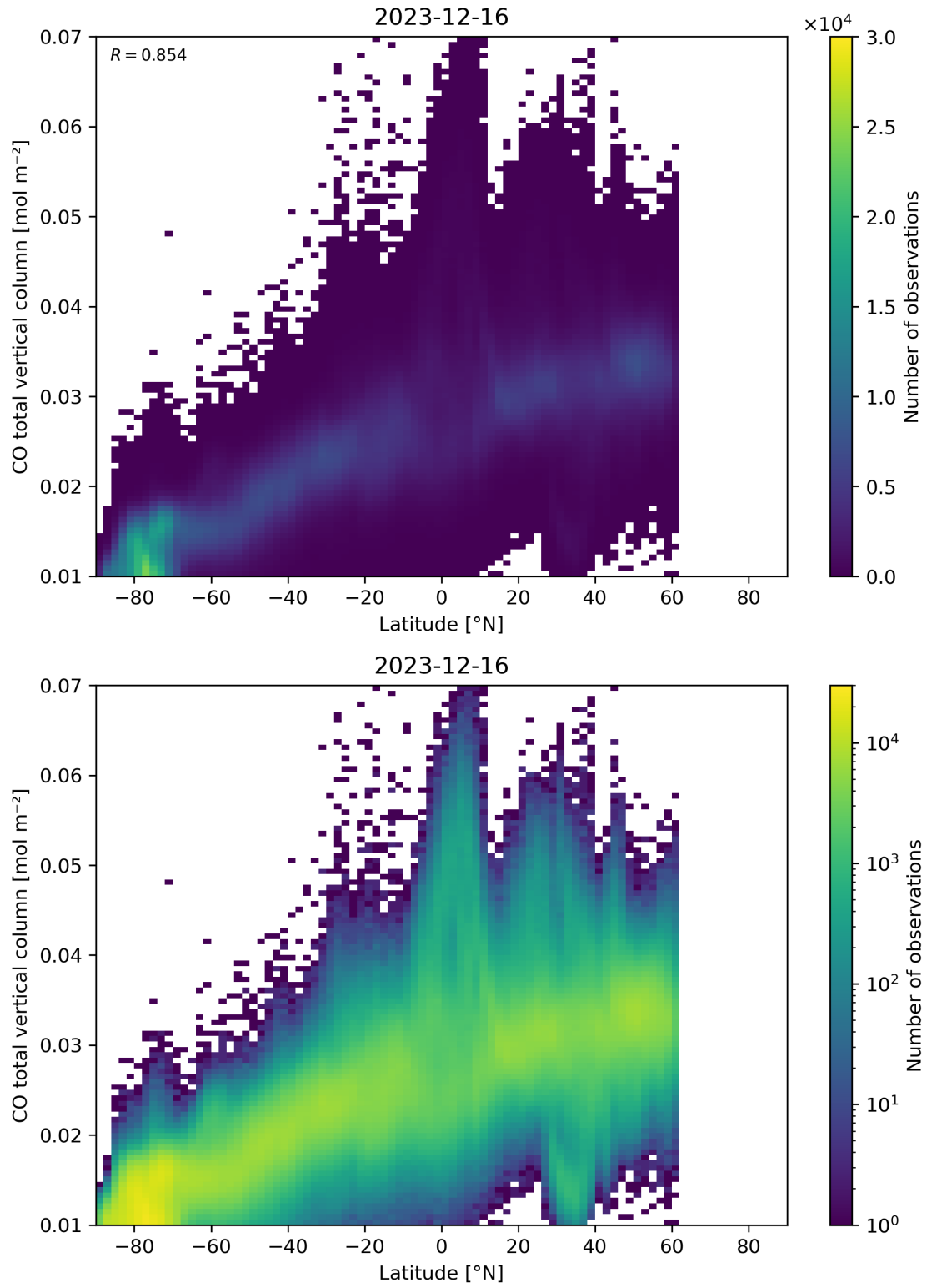
Figure 51: Scatter density plot of “Latitude” against “CO total vertical column” for 2023-12-15 to 2023-12-17.
