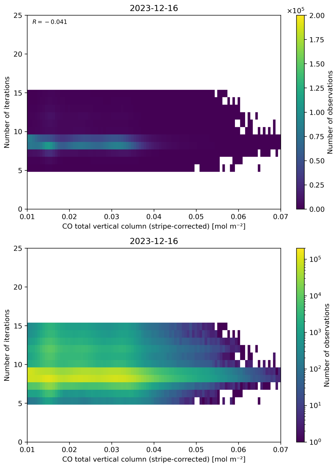
Figure 39: Scatter density plot of “CO total vertical column (stripe-corrected)” against “Number of iterations” for 2023-12-15 to 2023-12-17.
