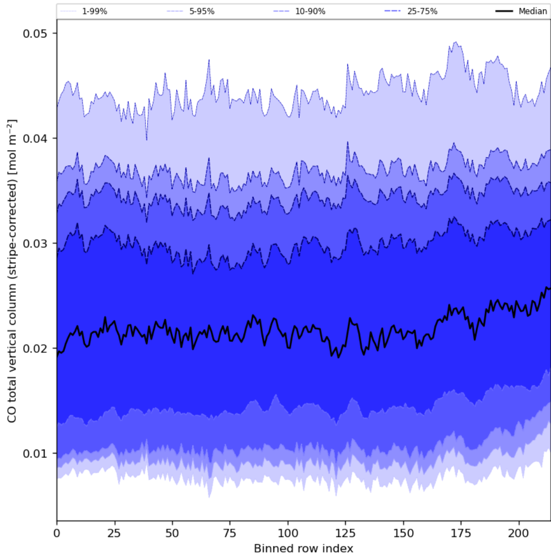
Figure 27: Along track statistics of “CO total vertical column (stripe-corrected)” for 2023-12-15 to 2023-12-17
