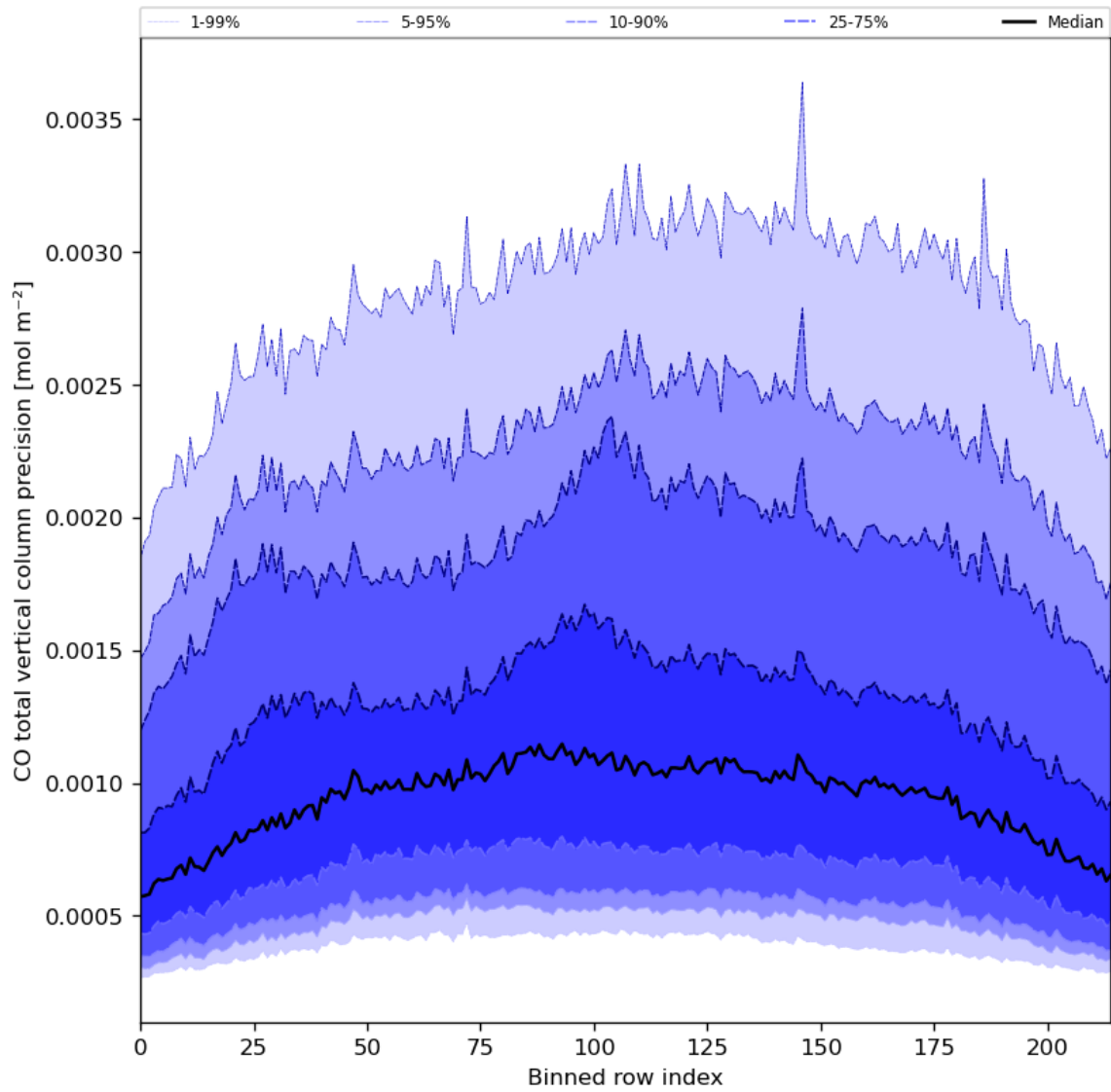
Figure 28: Along track statistics of “CO total vertical column precision” for 2023-12-15 to 2023-12-17
