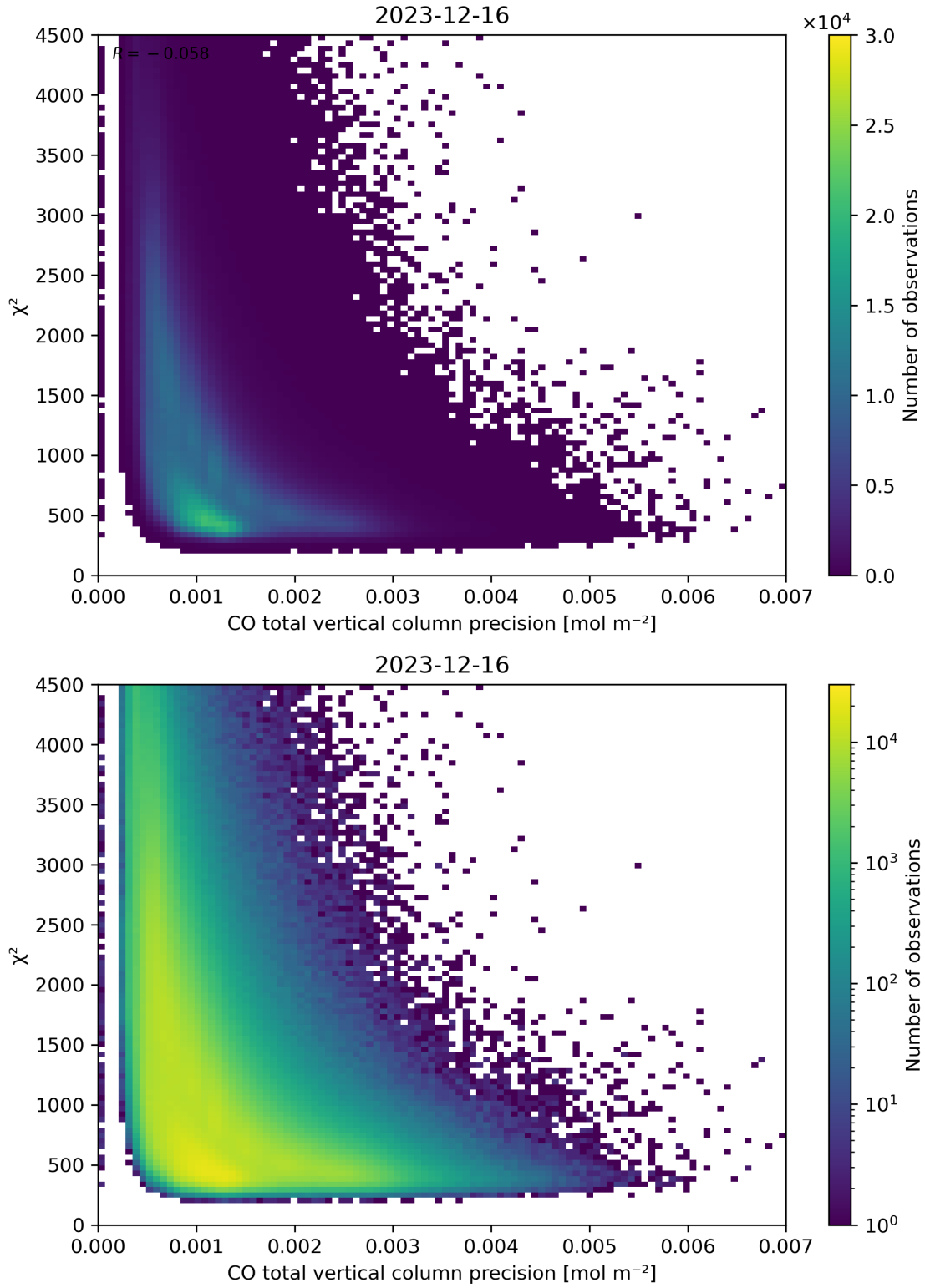
Figure 44: Scatter density plot of “CO total vertical column precision” against “ \chi^2 ” for 2023-12-15 to 2023-12-17.
