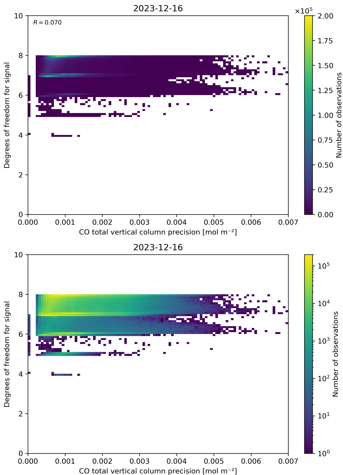
Figure 45: Scatter density plot of “CO total vertical column precision” against “Degrees of freedom for signal” for 2023-12-15 to 2023-12-17.
