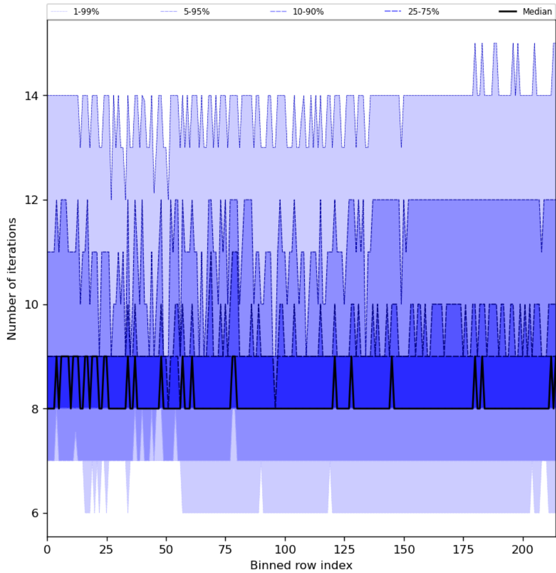
Figure 32: Along track statistics of “Number of iterations” for 2023-12-15 to 2023-12-17
