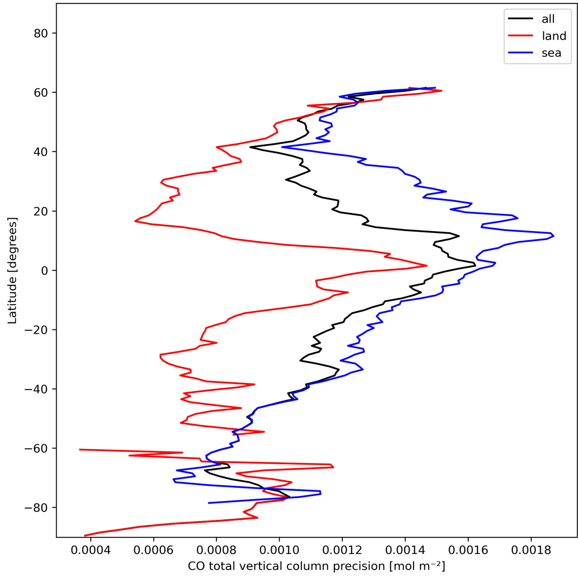
Figure 12: Zonal average of “CO total vertical column precision” for 2023-12-15 to 2023-12-17.
