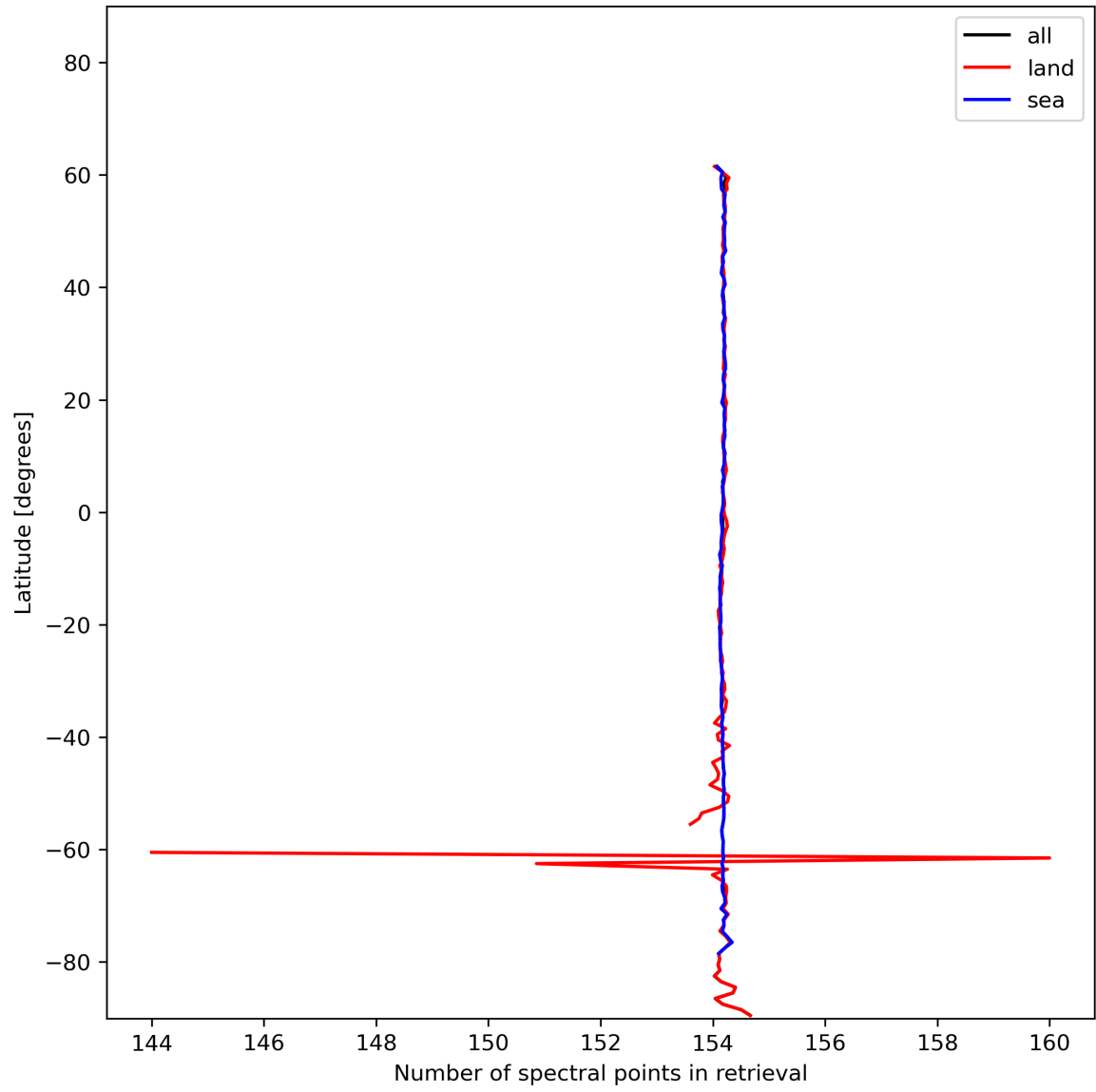
Figure 13: Zonal average of “Number of spectral points in retrieval” for 2023-12-15 to 2023-12-17.
