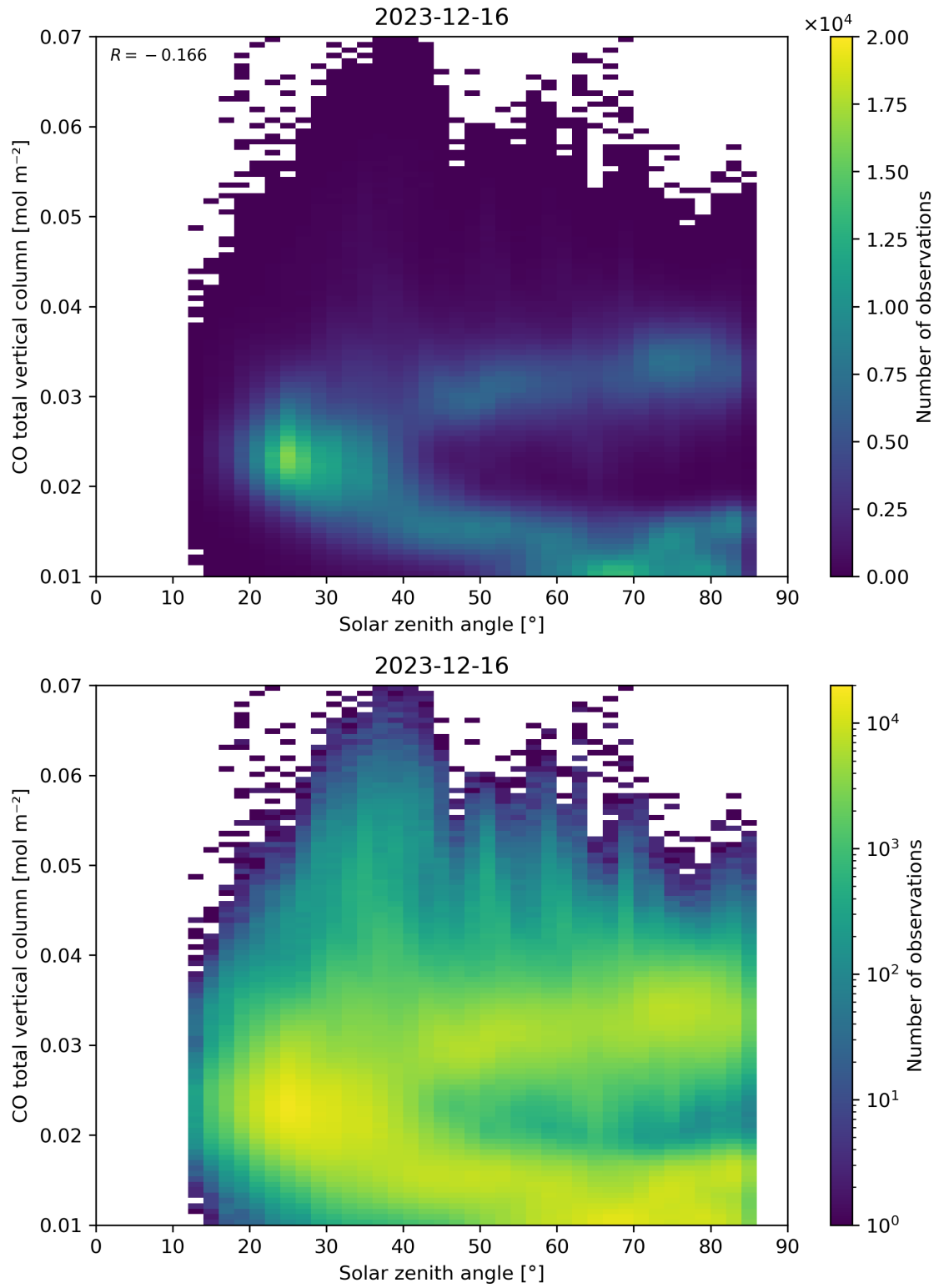
Figure 61: Scatter density plot of “Solar zenith angle” against “CO total vertical column” for 2023-12-15 to 2023-12-17.
