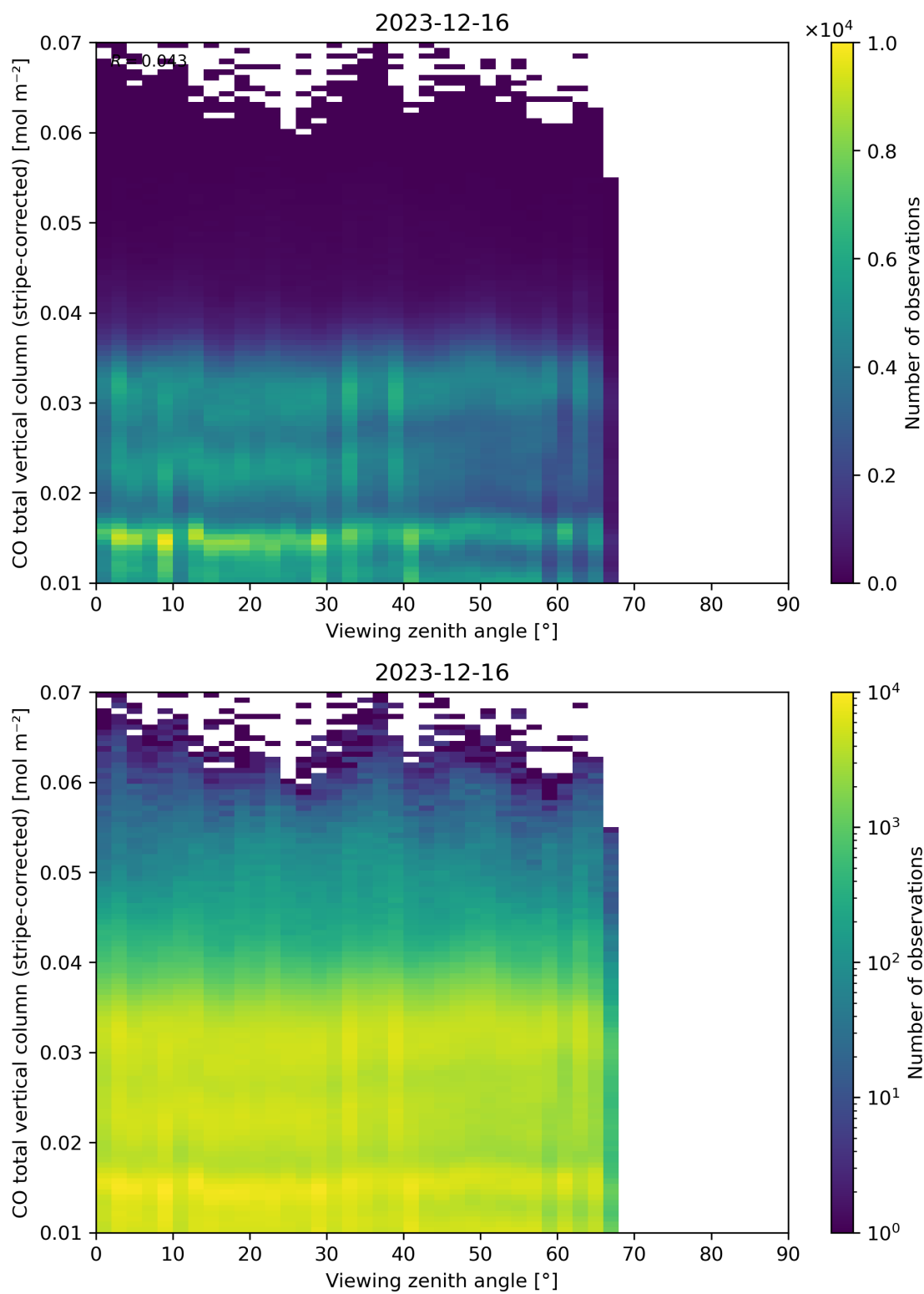
Figure 70: Scatter density plot of “Viewing zenith angle” against “CO total vertical column (stripe-corrected)” for 2023-12-15 to 2023-12-17.
