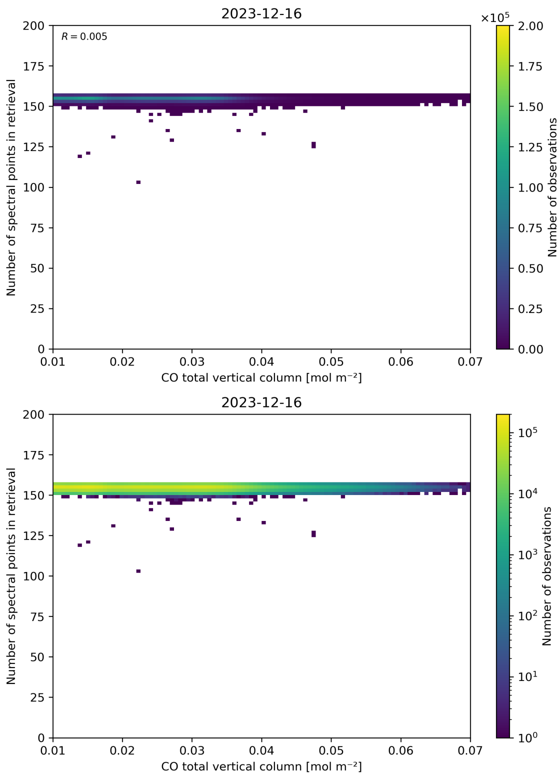
Figure 43: Scatter density plot of “CO total vertical column” against “Number of spectral points in retrieval” for 2023-12-15 to 2023-12-17.
