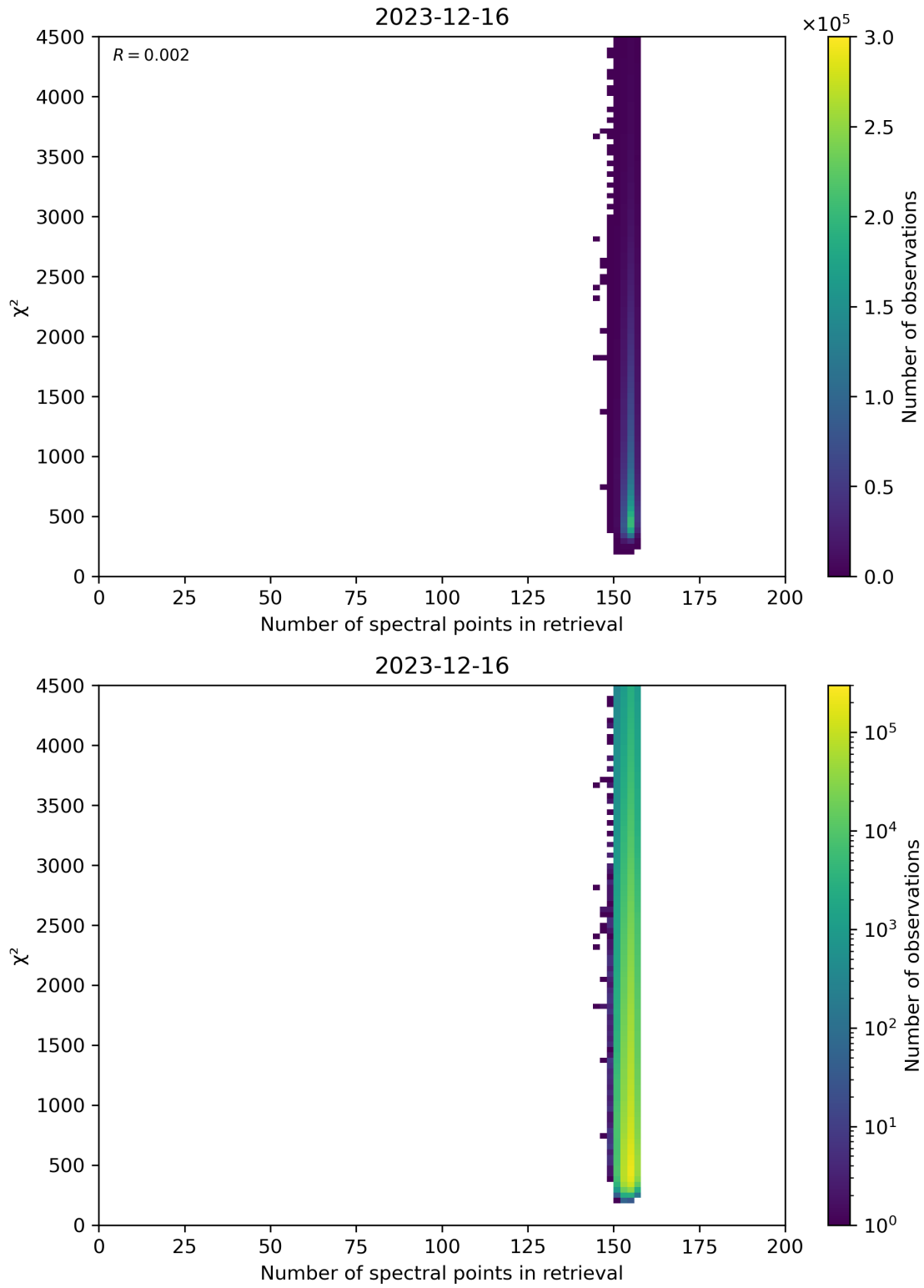
Figure 58: Scatter density plot of “Number of spectral points in retrieval” against “ \chi^2 ” for 2023-12-15 to 2023-12-17.
