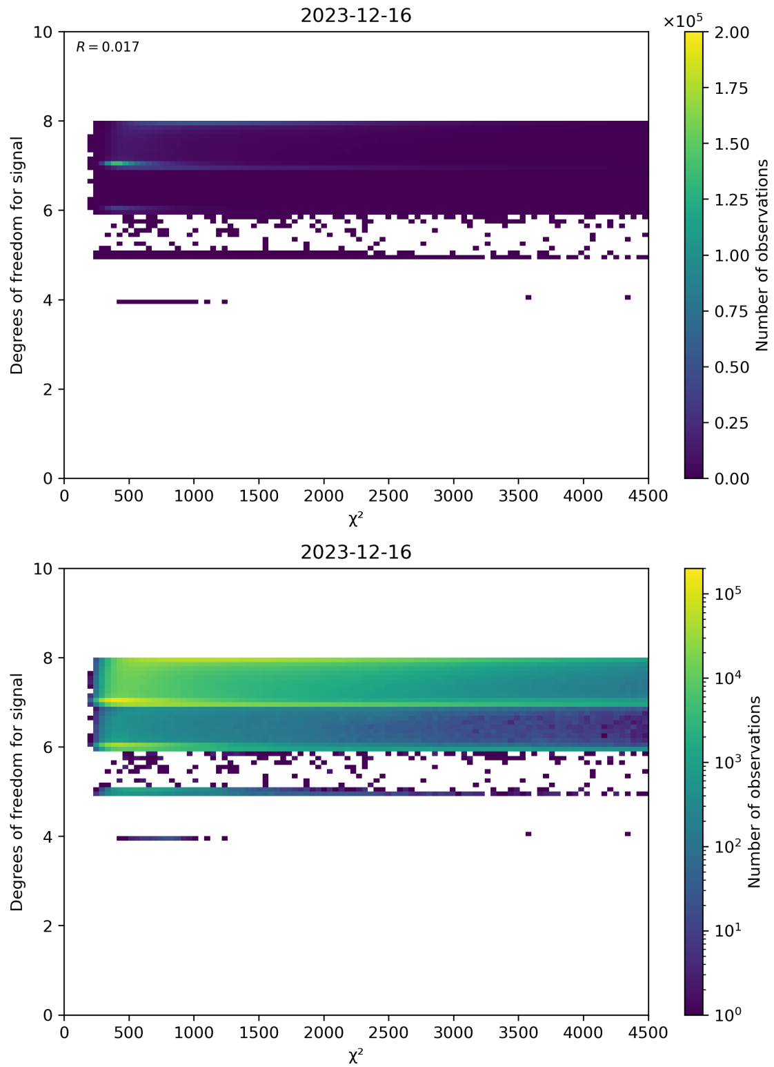
Figure 48: Scatter density plot of “ \chi^2 ” against “Degrees of freedom for signal” for 2023-12-15 to 2023-12-17.
