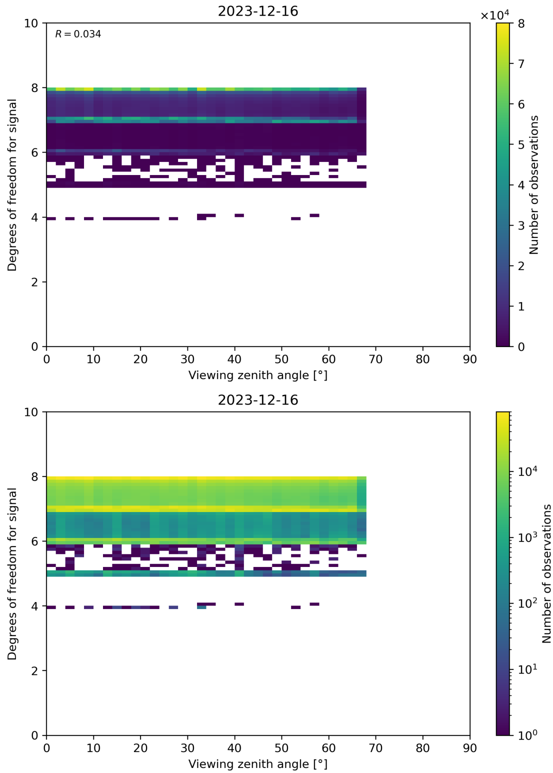
Figure 73: Scatter density plot of “Viewing zenith angle” against “Degrees of freedom for signal” for 2023-12-15 to 2023-12-17.
