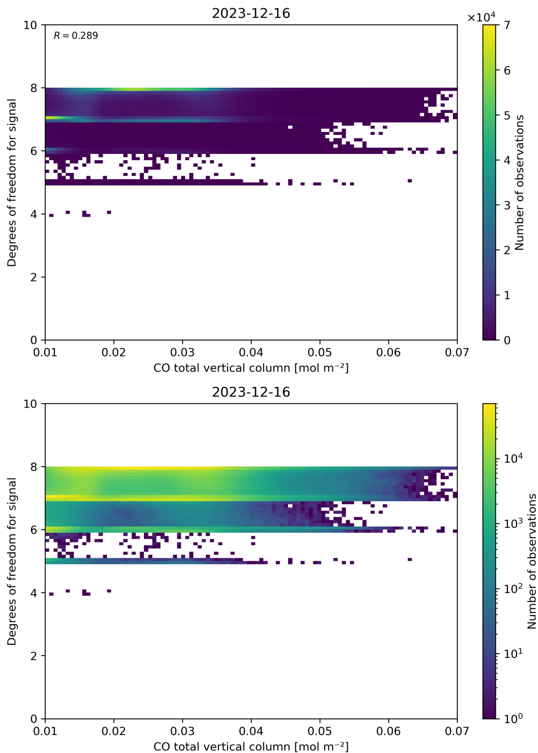
Figure 41: Scatter density plot of “CO total vertical column” against “Degrees of freedom for signal” for 2023-12-15 to 2023-12-17.
