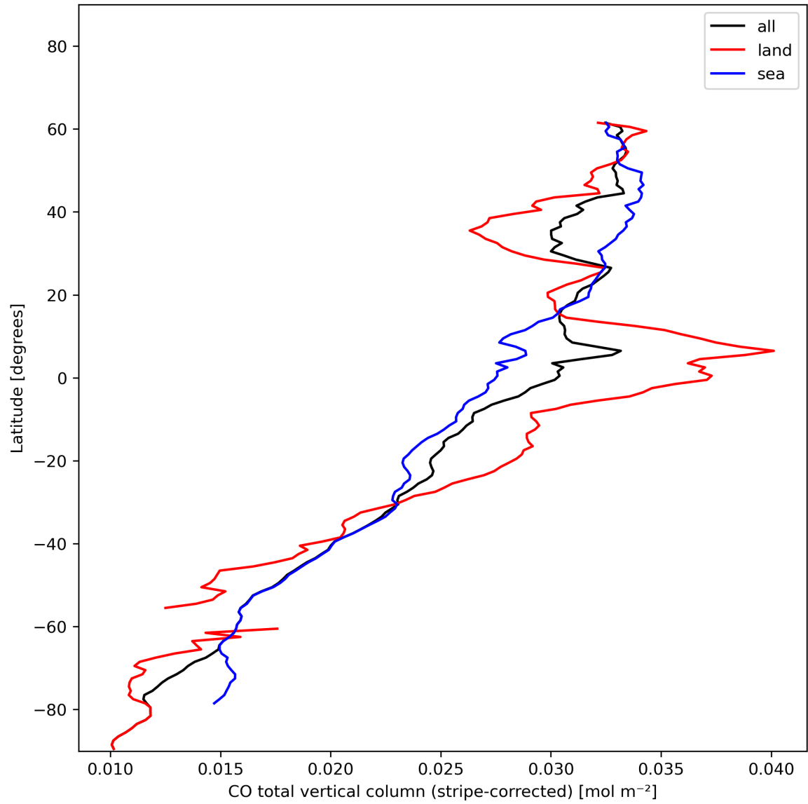
Figure 11: Zonal average of “CO total vertical column (stripe-corrected)” for 2023-12-15 to 2023-12-17.
