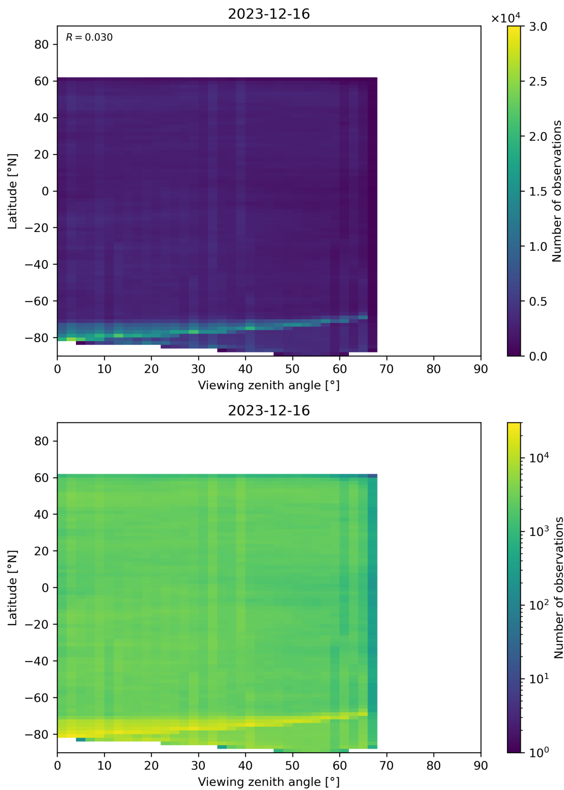
Figure 74: Scatter density plot of “Viewing zenith angle” against “Latitude” for 2023-12-15 to 2023-12-17.
