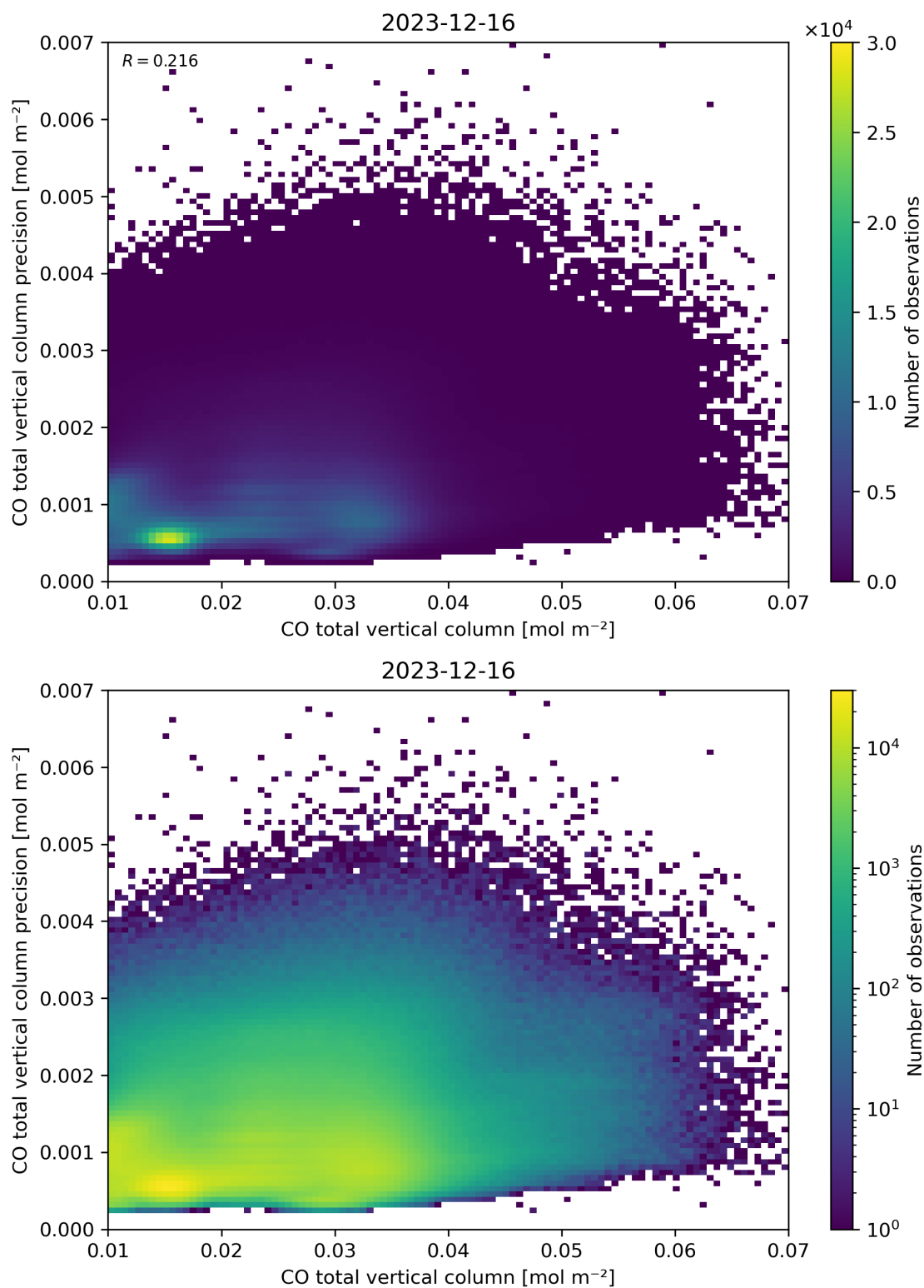
Figure 34: Scatter density plot of “CO total vertical column” against “CO total vertical column precision” for 2023-12-15 to 2023-12-17.
