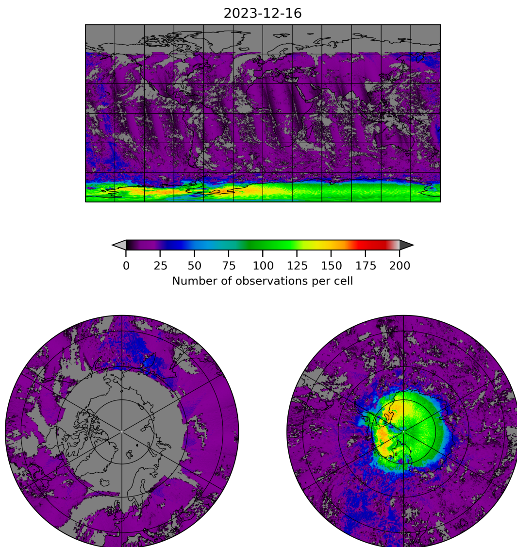
Figure 8: Map of the number of observations for 2023-12-15 to 2023-12-17
