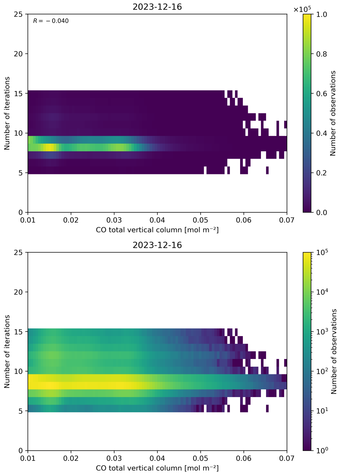
Figure 42: Scatter density plot of “CO total vertical column” against “Number of iterations” for 2023-12-15 to 2023-12-17.
