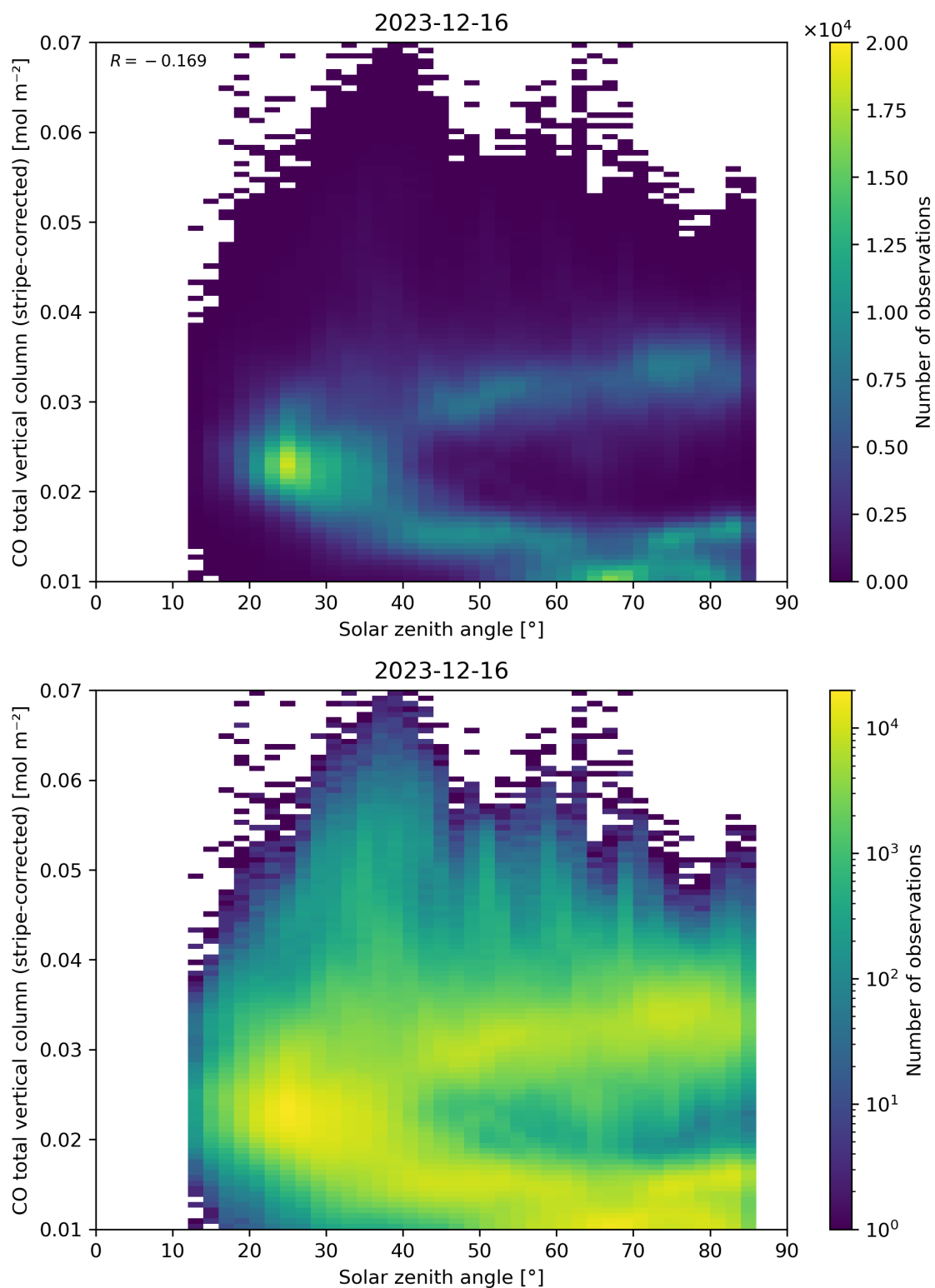
Figure 62: Scatter density plot of “Solar zenith angle” against “CO total vertical column (stripe-corrected)” for 2023-12-15 to 2023-12-17.
