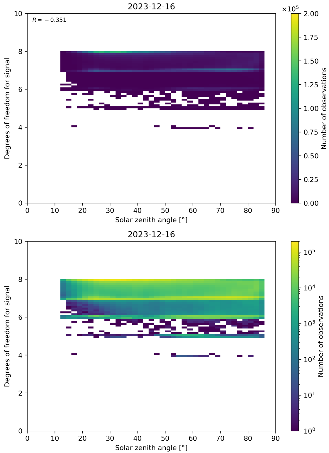
Figure 65: Scatter density plot of “Solar zenith angle” against “Degrees of freedom for signal” for 2023-12-15 to 2023-12-17.
