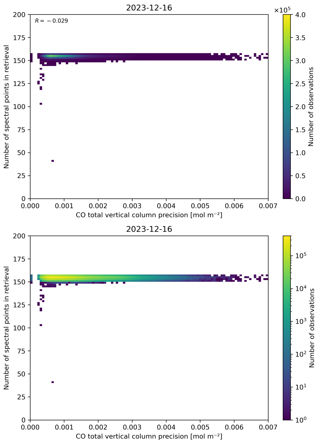
Figure 47: Scatter density plot of “CO total vertical column precision” against “Number of spectral points in retrieval” for 2023-12-15 to 2023-12-17.
