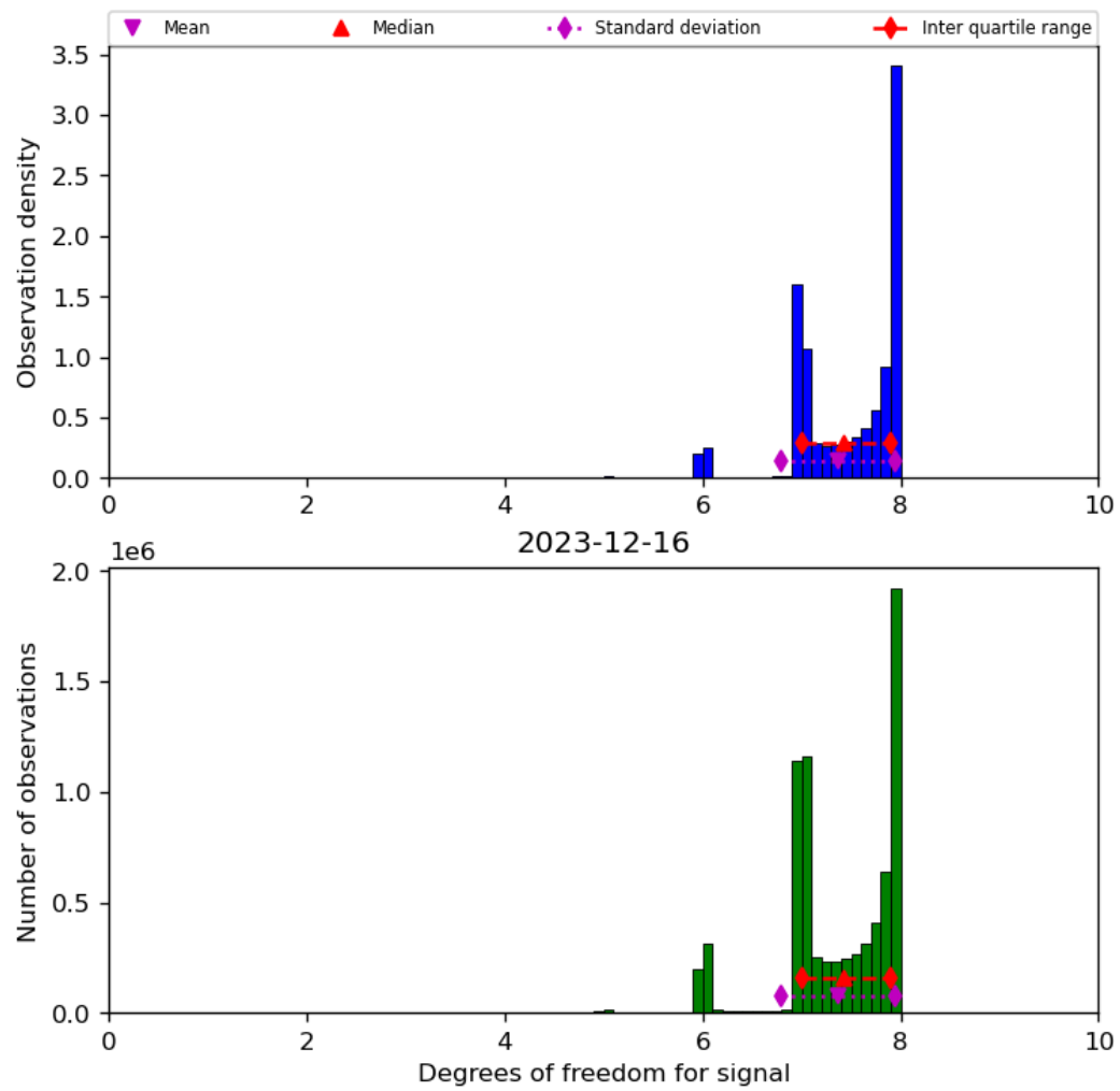
Figure 23: Histogram of “Degrees of freedom for signal” for 2023-12-15 to 2023-12-17
