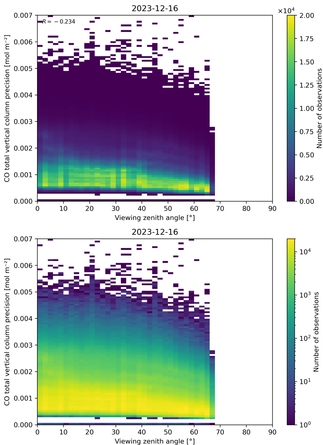
Figure 71: Scatter density plot of “Viewing zenith angle” against “CO total vertical column precision” for 2023-12-15 to 2023-12-17.
