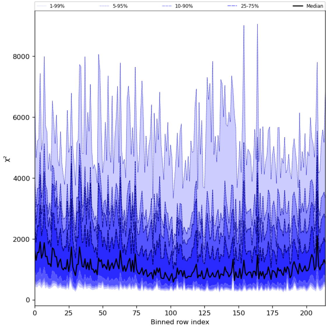
Figure 30: Along track statistics of “ \chi^2 ” for 2023-12-15 to 2023-12-17
