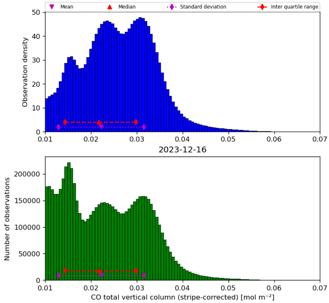
Figure 19: Histogram of “CO total vertical column (stripe-corrected)” for 2023-12-15 to 2023-12-17
