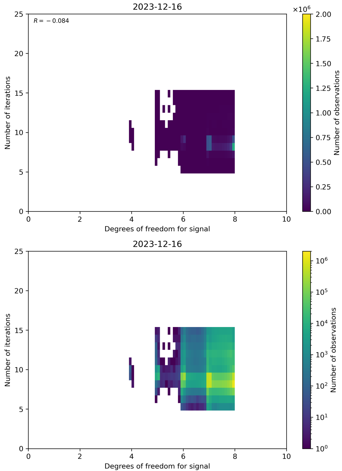
Figure 50: Scatter density plot of “Degrees of freedom for signal” against “Number of iterations” for 2023-12-15 to 2023-12-17.
