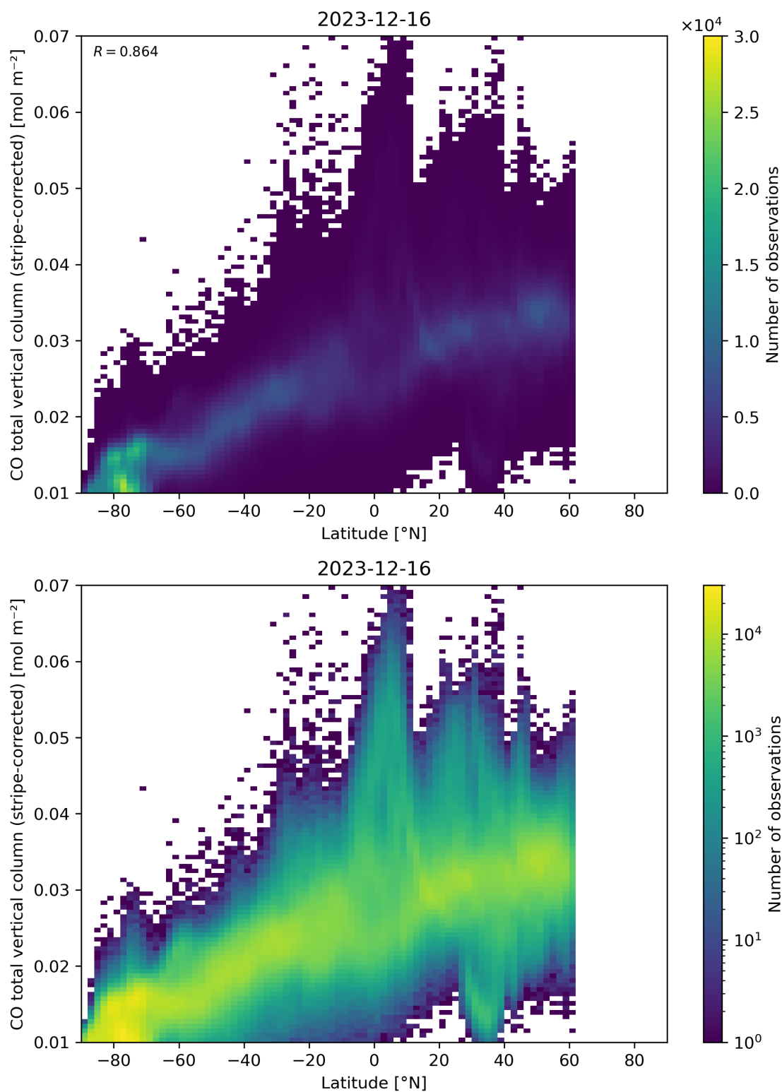
Figure 52: Scatter density plot of “Latitude” against “CO total vertical column (stripe-corrected)” for 2023-12-15 to 2023-12-17.
