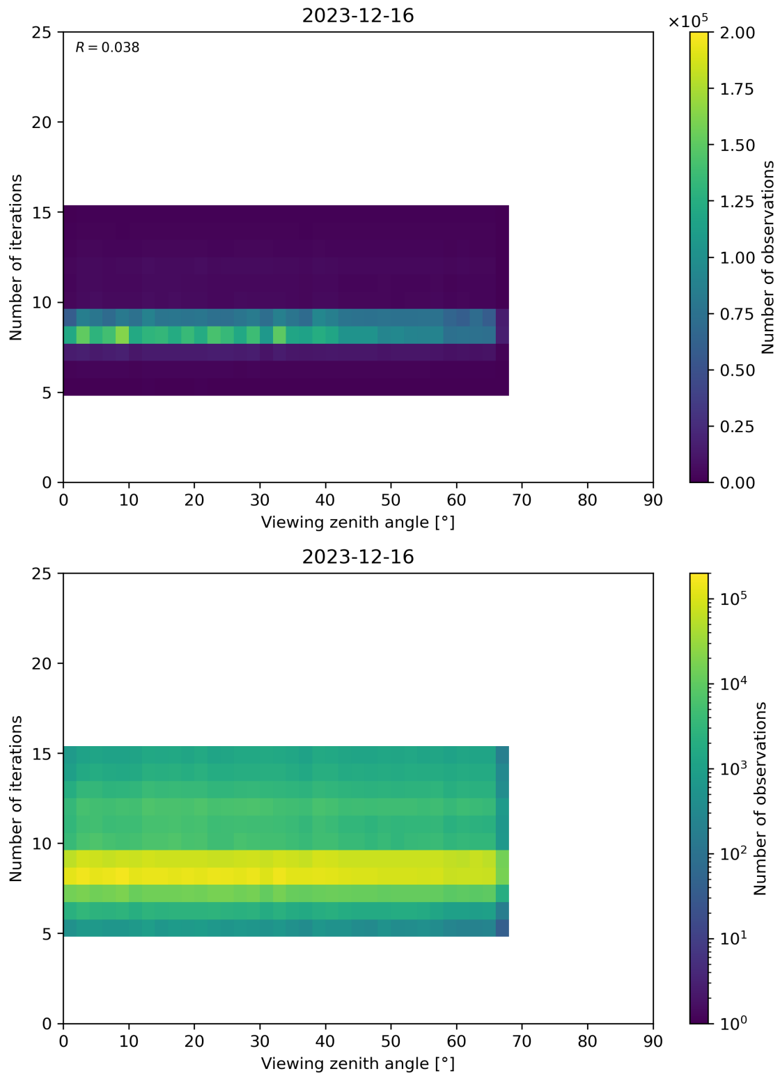
Figure 75: Scatter density plot of “Viewing zenith angle” against “Number of iterations” for 2023-12-15 to 2023-12-17.
