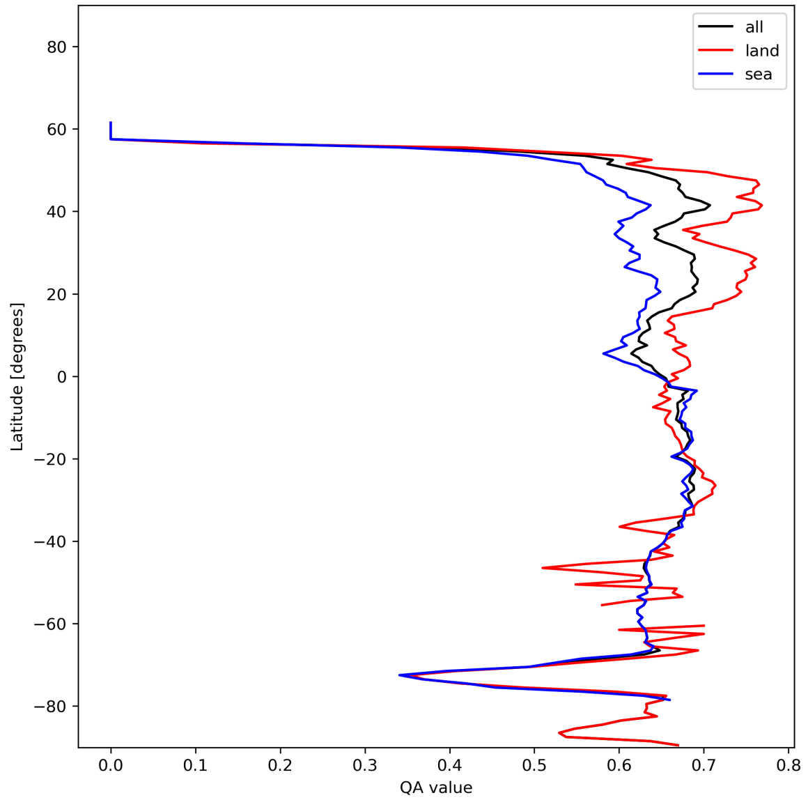
Figure 9: Zonal average of “QA value” for 2023-12-15 to 2023-12-17.
