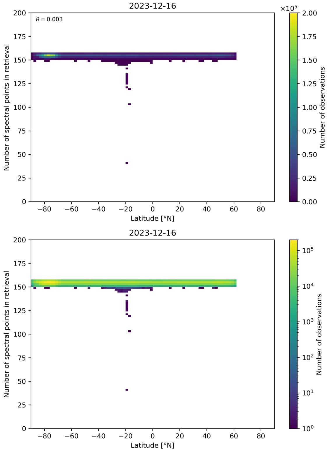
Figure 57: Scatter density plot of “Latitude” against “Number of spectral points in retrieval” for 2023-12-15 to 2023-12-17.
