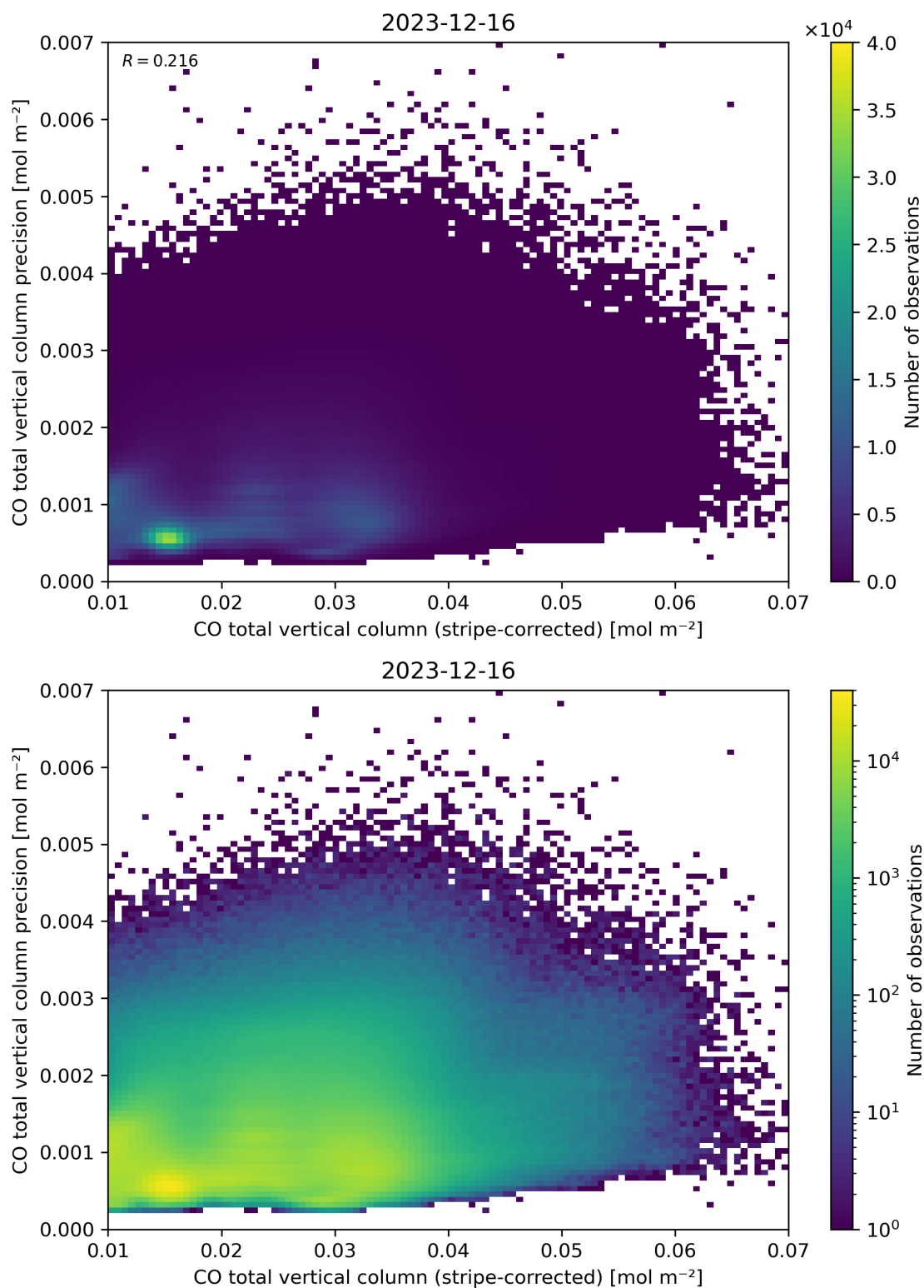
Figure 36: Scatter density plot of “CO total vertical column (stripe-corrected)” against “CO total vertical column precision” for 2023-12-15 to 2023-12-17.
