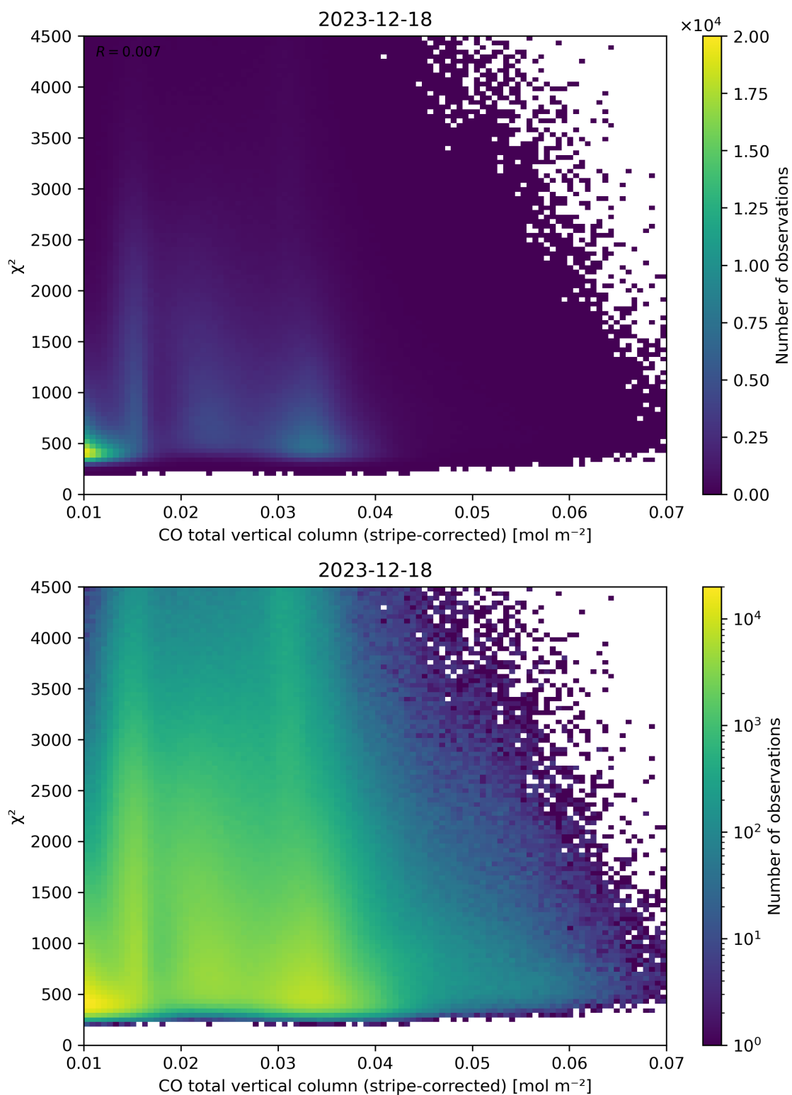
Figure 37: Scatter density plot of “CO total vertical column (stripe-corrected)” against “ \chi^2 ” for 2023-12-17 to 2023-12-19.
