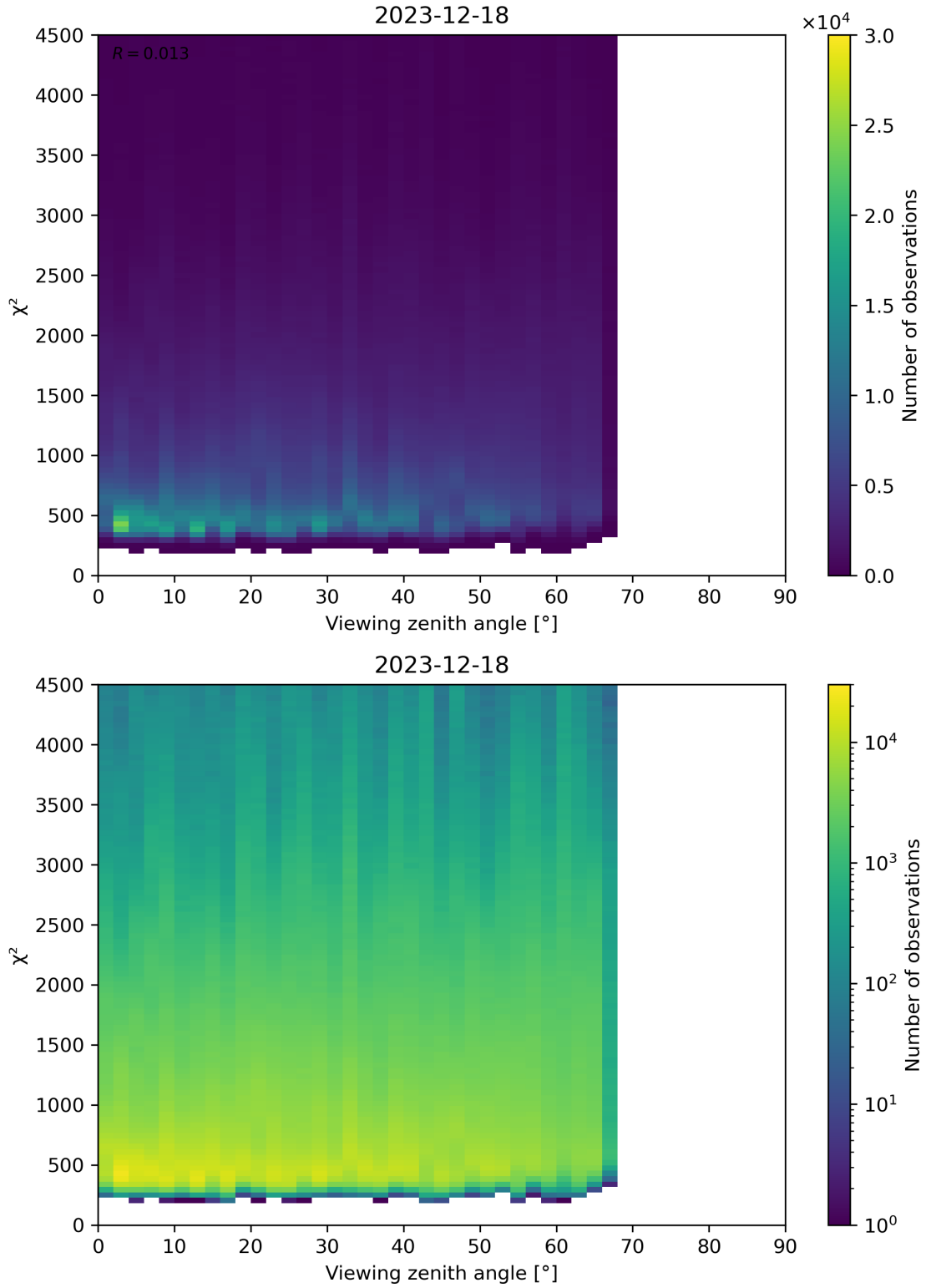
Figure 72: Scatter density plot of “Viewing zenith angle” against “ \chi^2 ” for 2023-12-17 to 2023-12-19.
