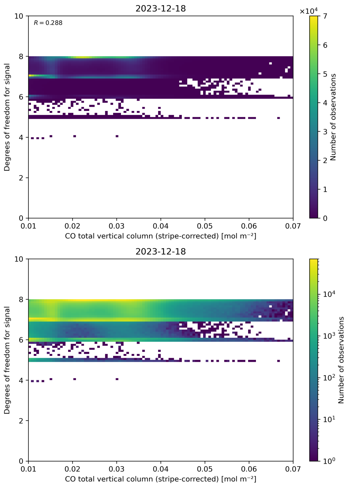
Figure 38: Scatter density plot of “CO total vertical column (stripe-corrected)” against “Degrees of freedom for signal” for 2023-12-17 to 2023-12-19.
