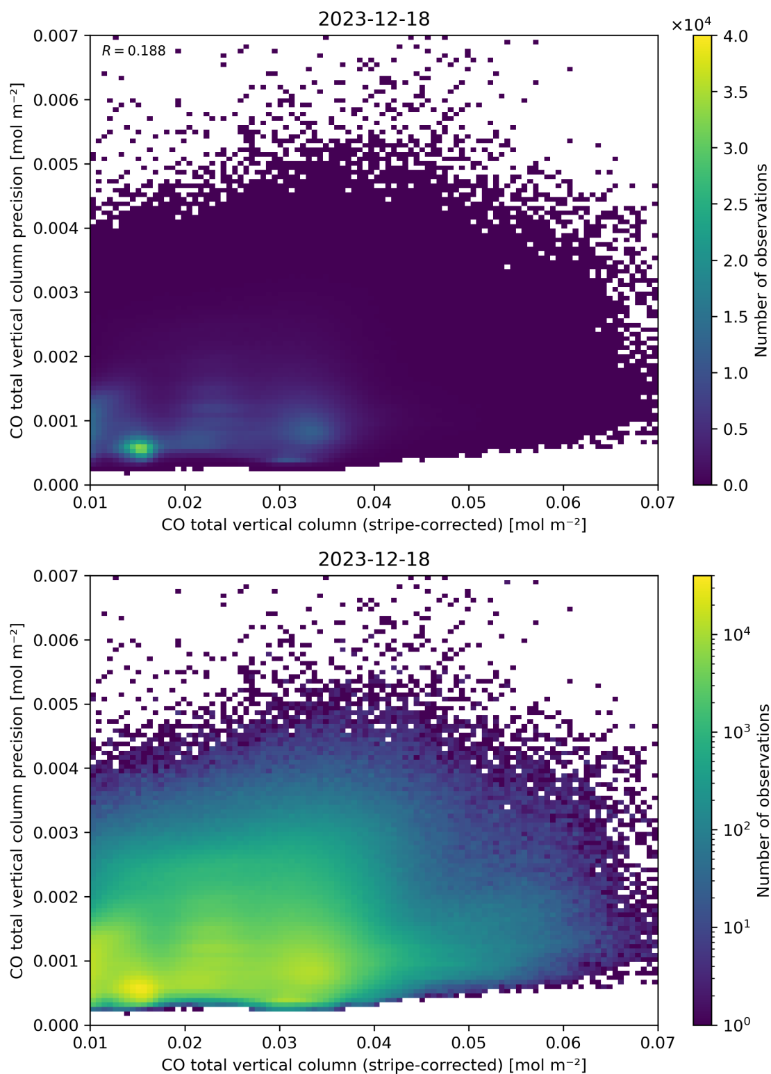
Figure 36: Scatter density plot of “CO total vertical column (stripe-corrected)” against “CO total vertical column precision” for 2023-12-17 to 2023-12-19.
