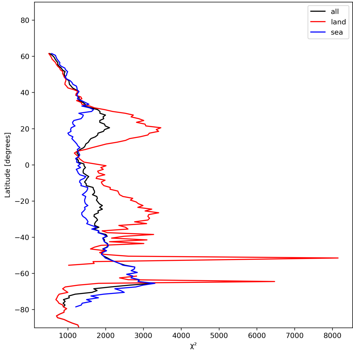
Figure 14: Zonal average of “ \chi^2 ” for 2023-12-17 to 2023-12-19.
