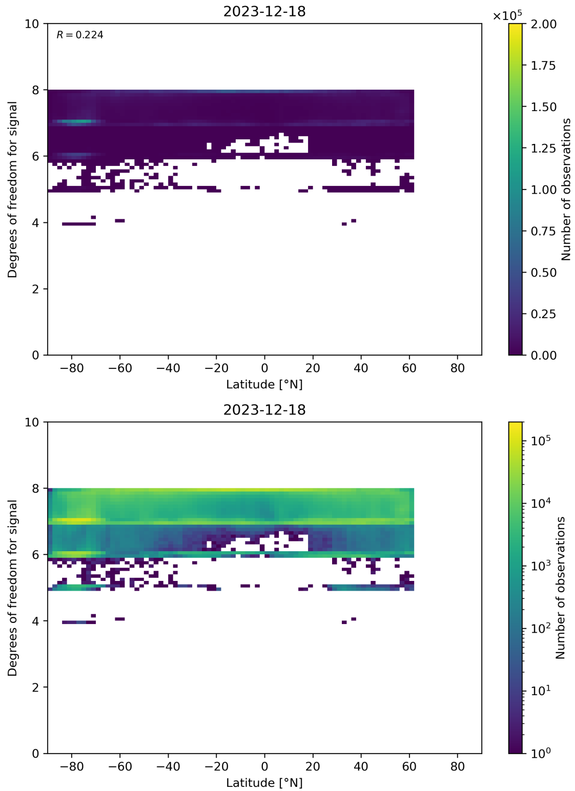
Figure 55: Scatter density plot of “Latitude” against “Degrees of freedom for signal” for 2023-12-17 to 2023-12-19.
