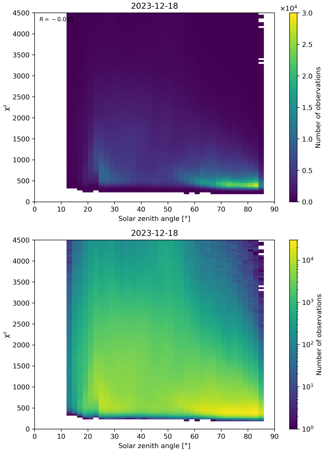
Figure 64: Scatter density plot of “Solar zenith angle” against “ \chi^2 ” for 2023-12-17 to 2023-12-19.
