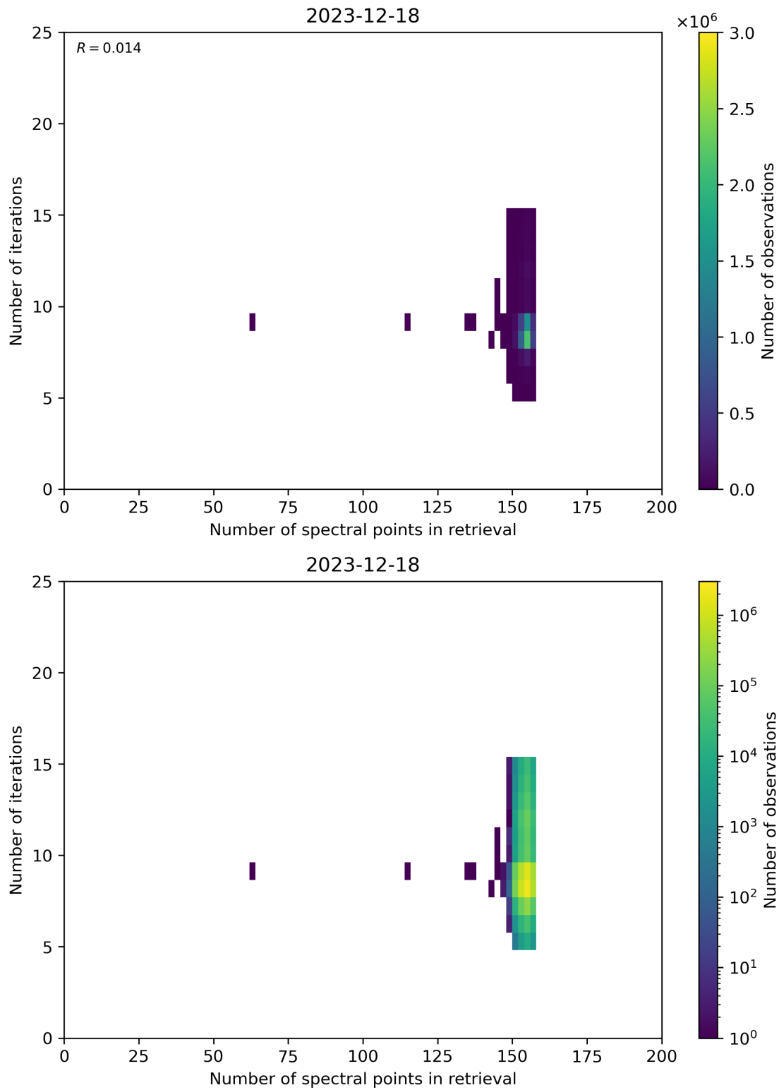
Figure 60: Scatter density plot of “Number of spectral points in retrieval” against “Number of iterations” for 2023-12-17 to 2023-12-19.
