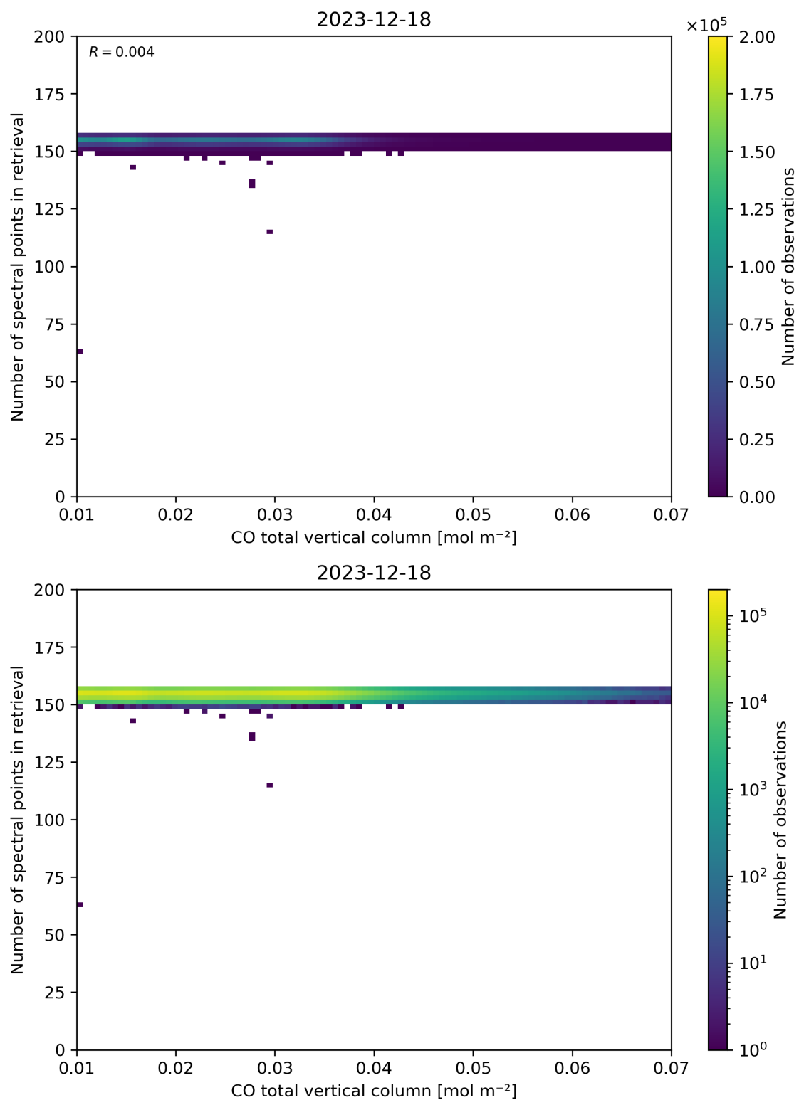
Figure 43: Scatter density plot of “CO total vertical column” against “Number of spectral points in retrieval” for 2023-12-17 to 2023-12-19.
