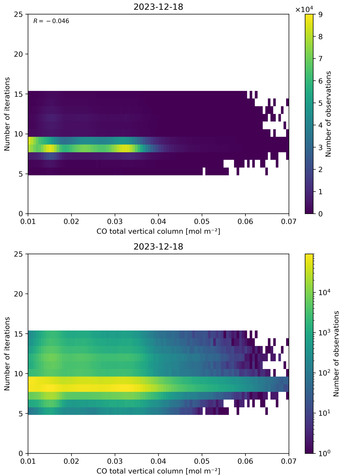
Figure 42: Scatter density plot of “CO total vertical column” against “Number of iterations” for 2023-12-17 to 2023-12-19.
