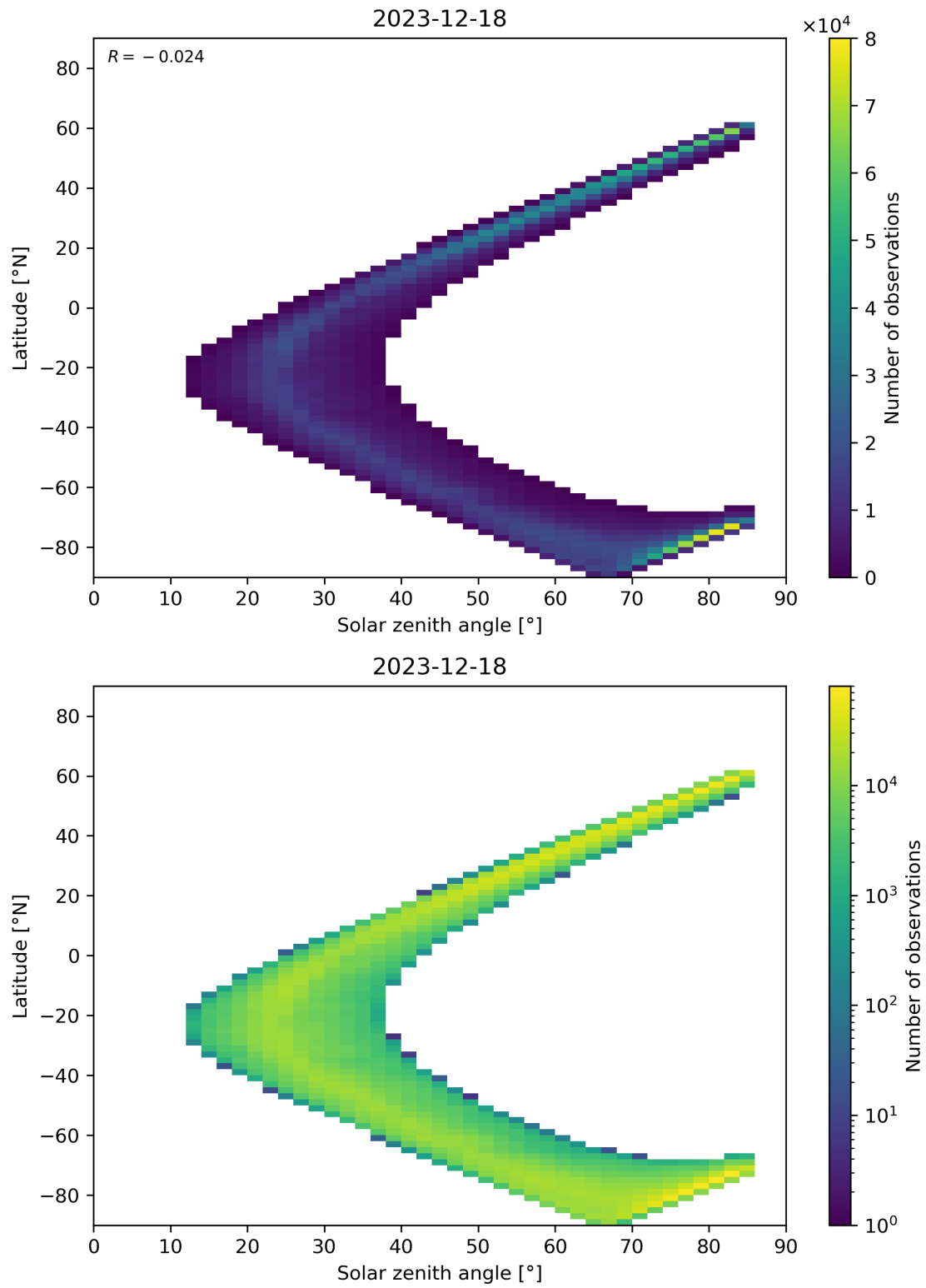
Figure 66: Scatter density plot of “Solar zenith angle” against “Latitude” for 2023-12-17 to 2023-12-19.
