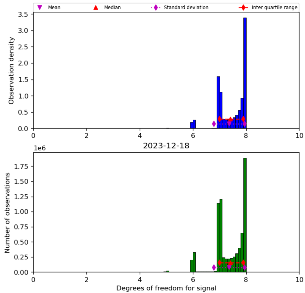
Figure 23: Histogram of “Degrees of freedom for signal” for 2023-12-17 to 2023-12-19
