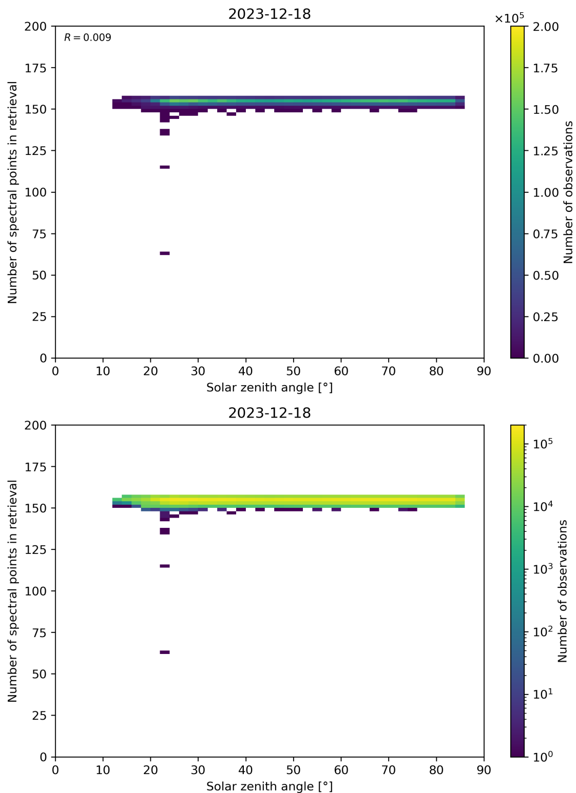
Figure 68: Scatter density plot of “Solar zenith angle” against “Number of spectral points in retrieval” for 2023-12-17 to 2023-12-19.
