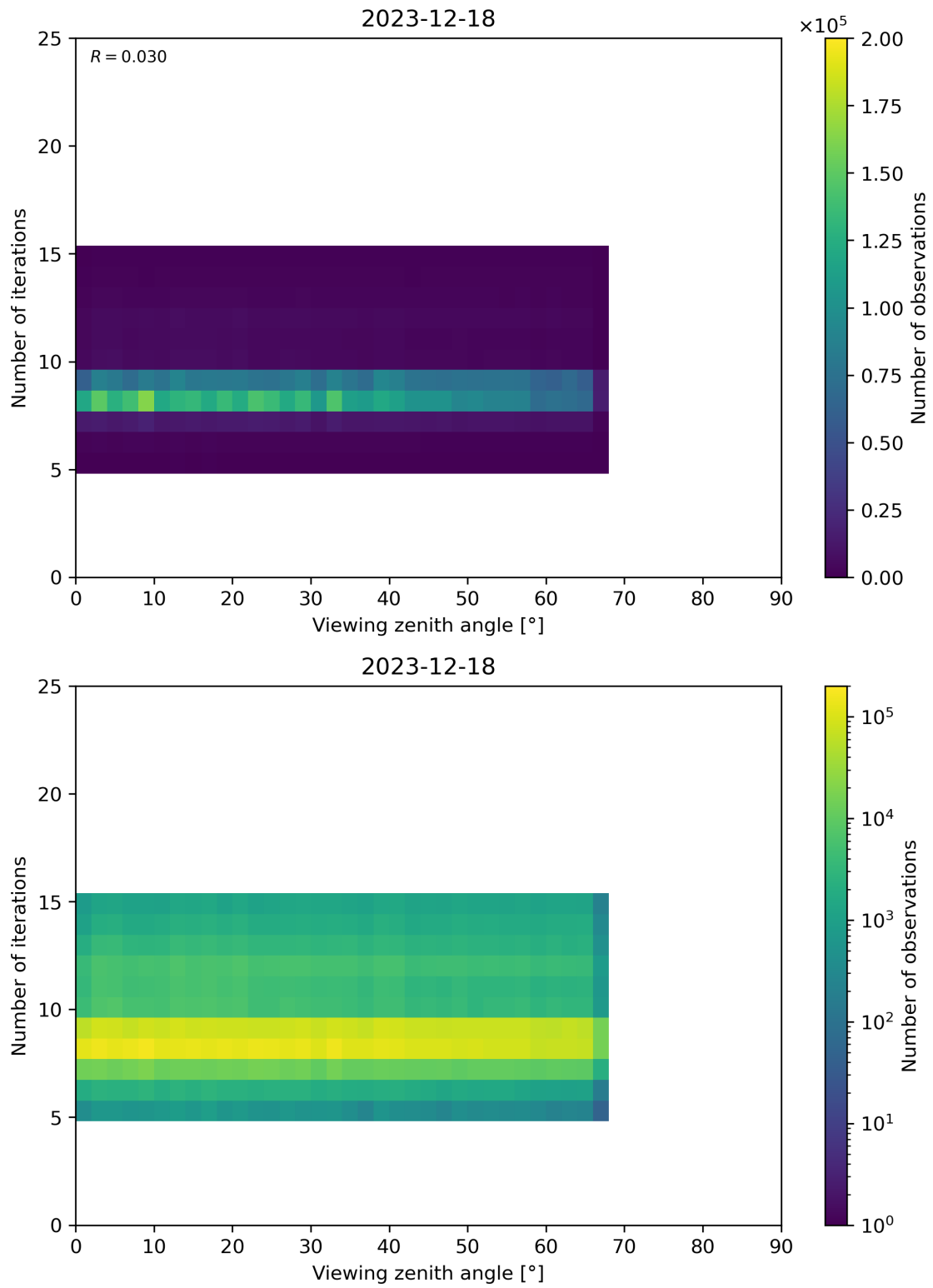
Figure 75: Scatter density plot of “Viewing zenith angle” against “Number of iterations” for 2023-12-17 to 2023-12-19.
