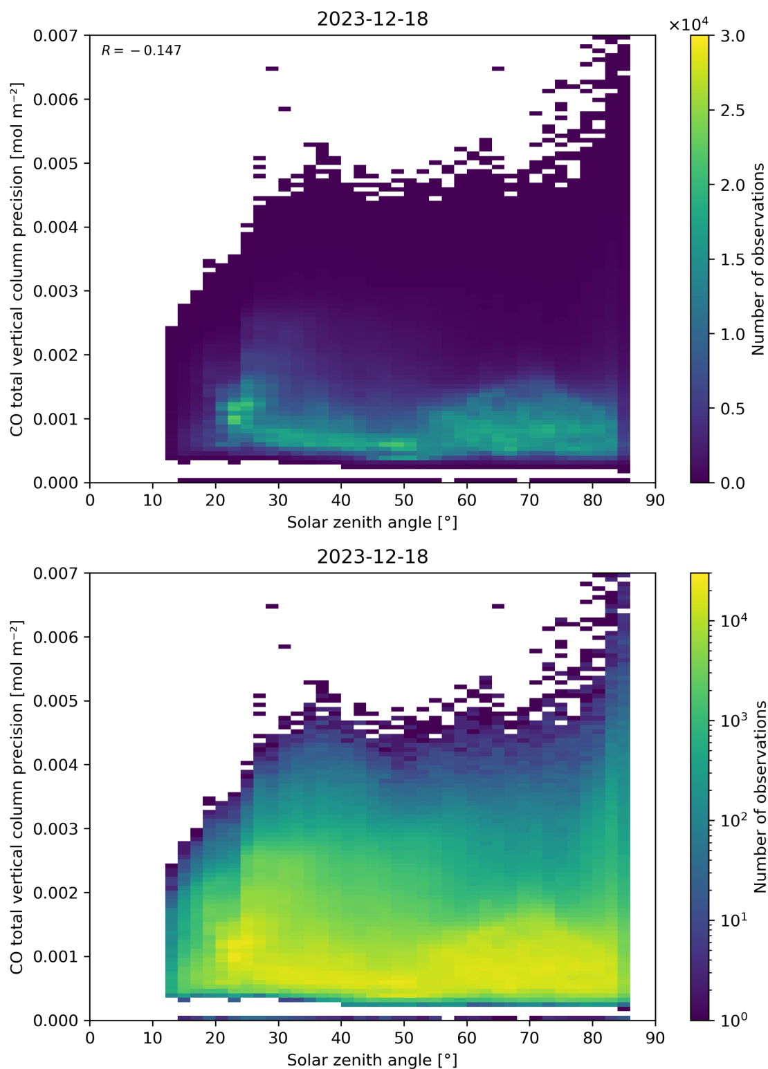
Figure 63: Scatter density plot of “Solar zenith angle” against “CO total vertical column precision” for 2023-12-17 to 2023-12-19.
