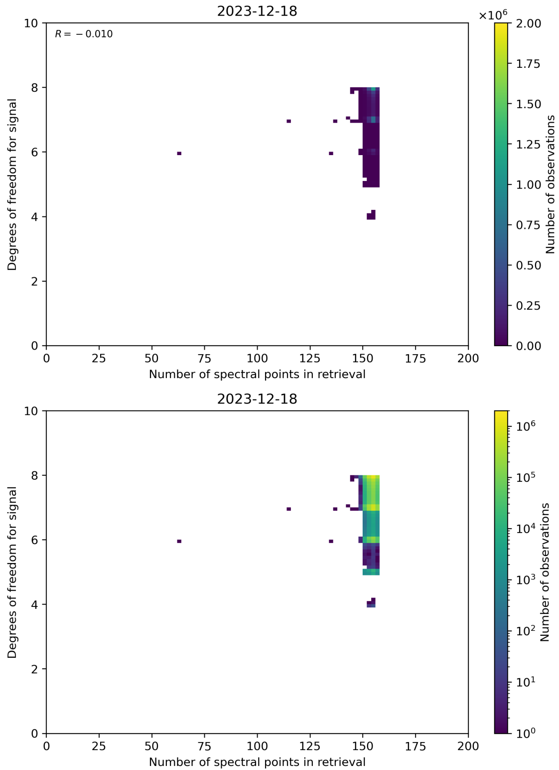
Figure 59: Scatter density plot of “Number of spectral points in retrieval” against “Degrees of freedom for signal” for 2023-12-17 to 2023-12-19.
