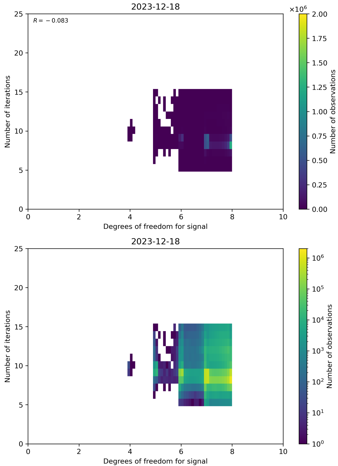
Figure 50: Scatter density plot of “Degrees of freedom for signal” against “Number of iterations” for 2023-12-17 to 2023-12-19.
