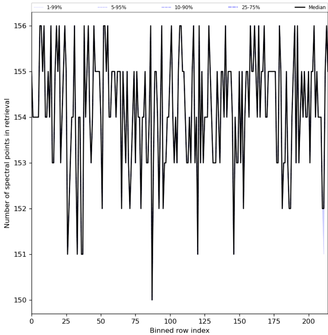
Figure 29: Along track statistics of “Number of spectral points in retrieval” for 2023-12-17 to 2023-12-19
