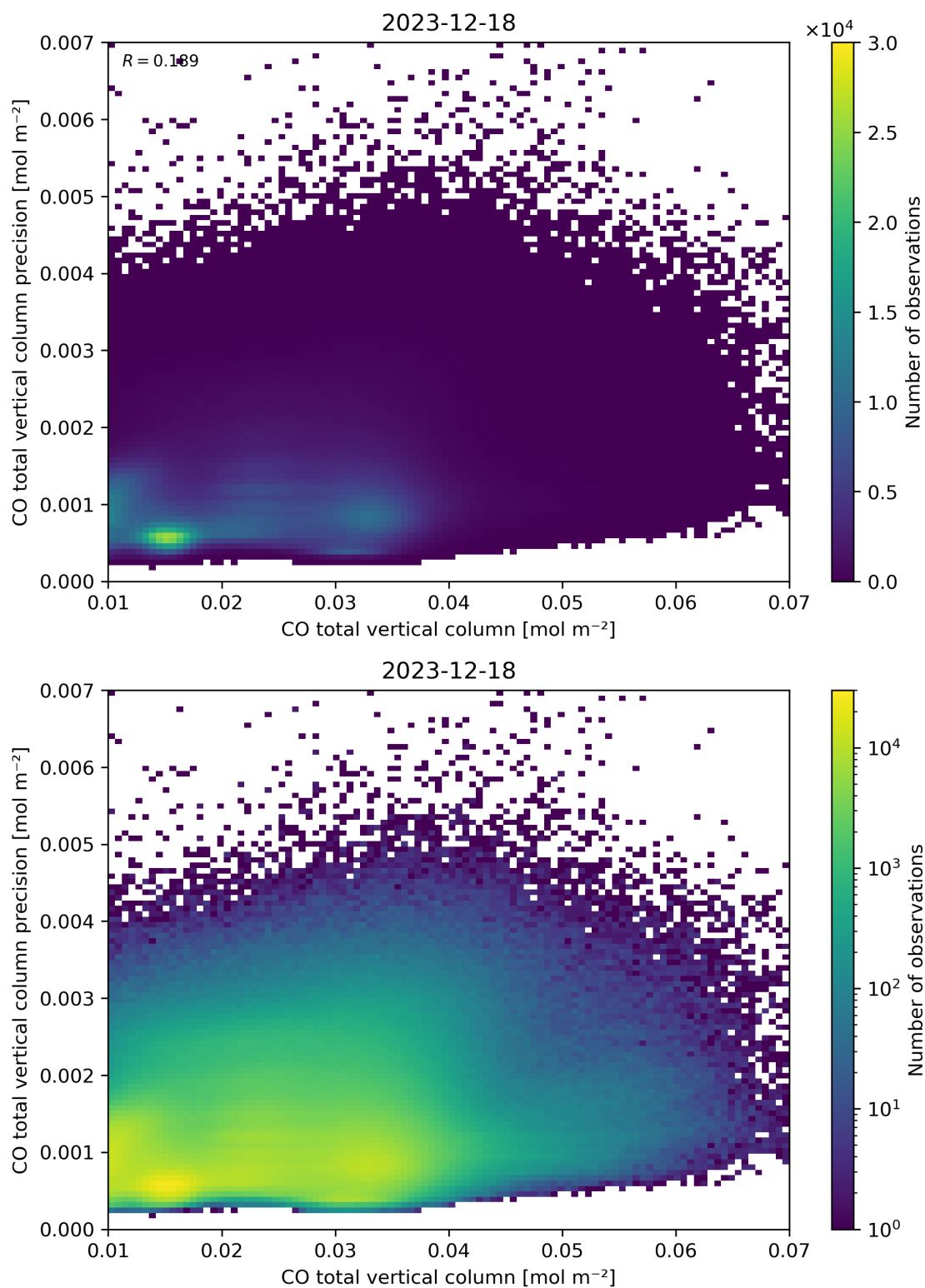
Figure 34: Scatter density plot of “CO total vertical column” against “CO total vertical column precision” for 2023-12-17 to 2023-12-19.
