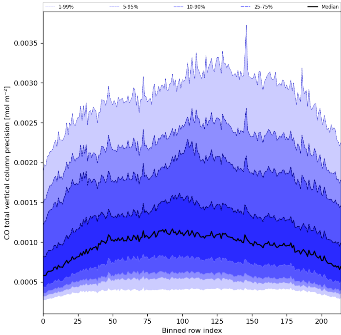
Figure 28: Along track statistics of “CO total vertical column precision” for 2023-12-17 to 2023-12-19
