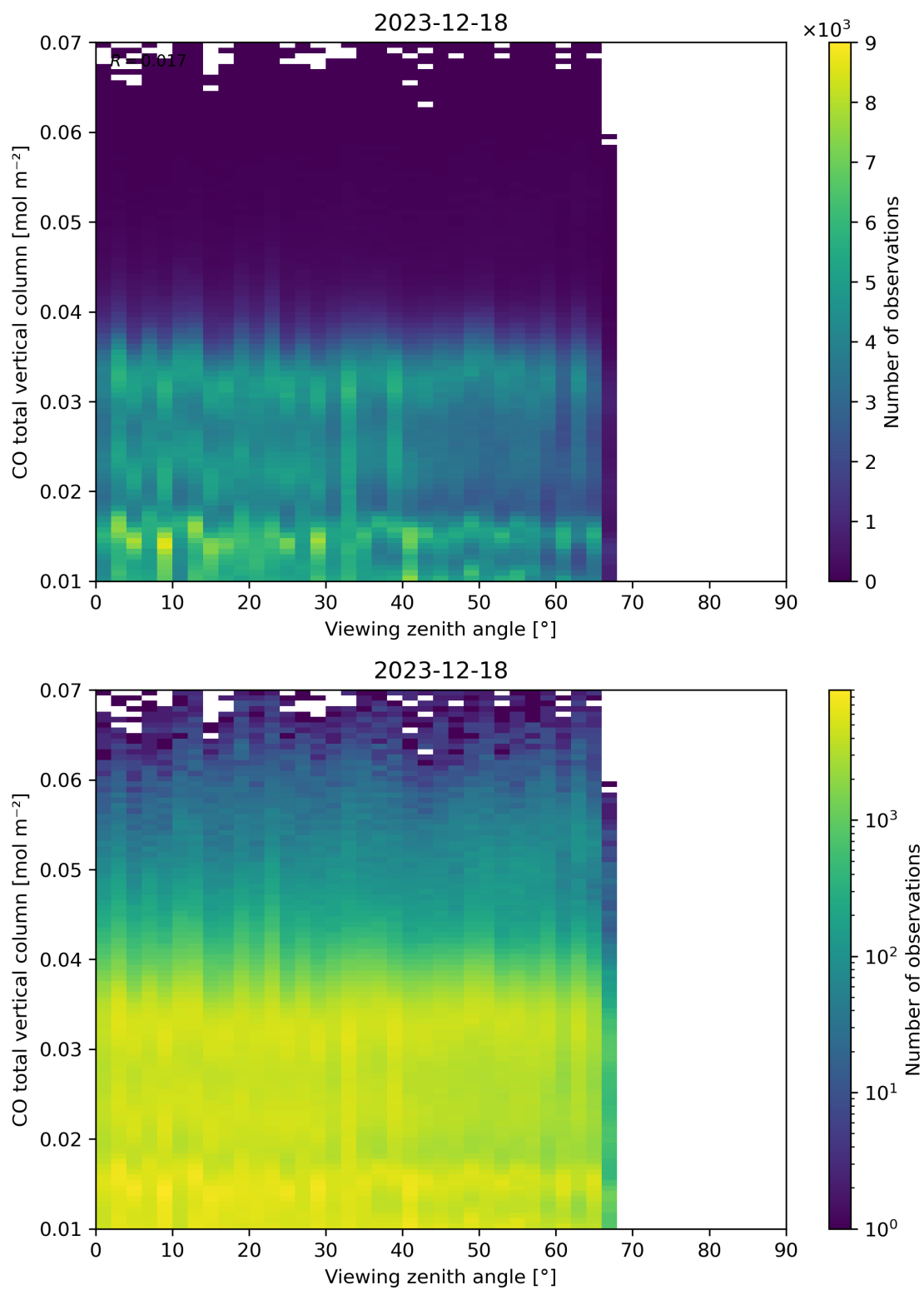
Figure 69: Scatter density plot of “Viewing zenith angle” against “CO total vertical column” for 2023-12-17 to 2023-12-19.
