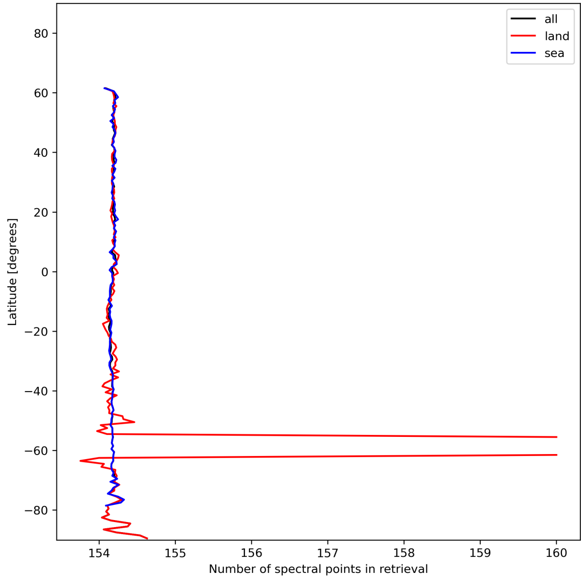
Figure 13: Zonal average of “Number of spectral points in retrieval” for 2023-12-17 to 2023-12-19.
