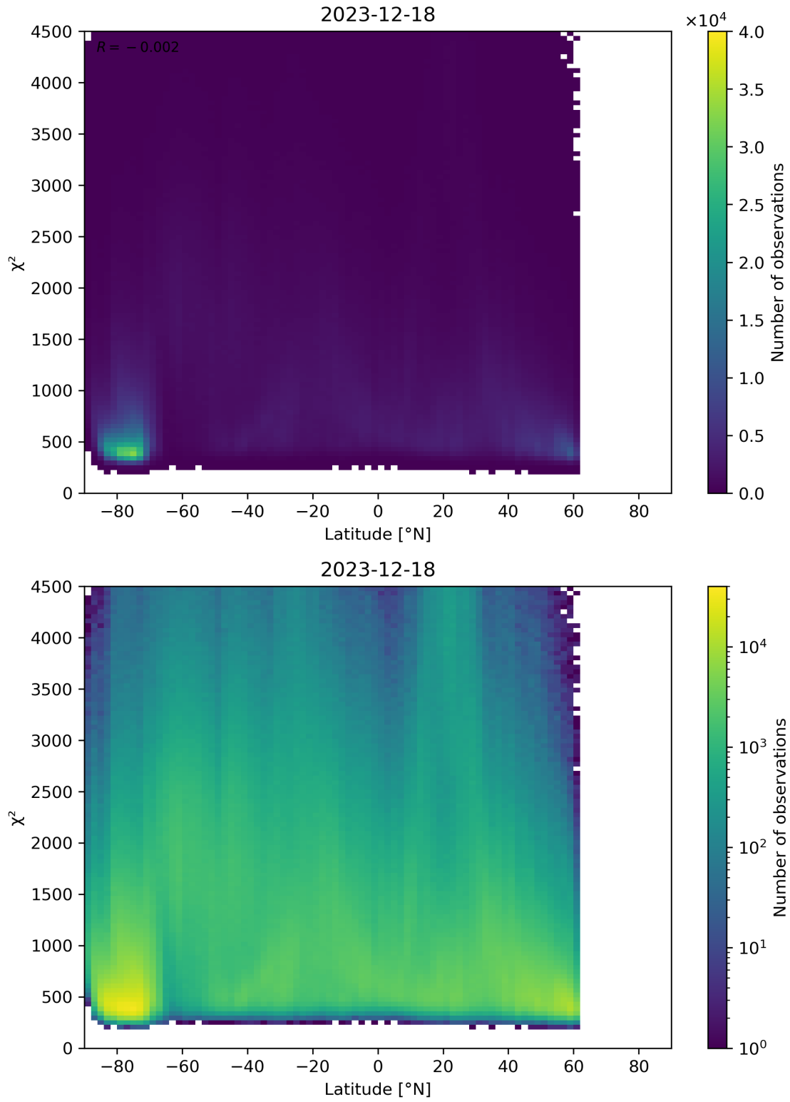
Figure 54: Scatter density plot of “Latitude” against “ \chi^2 ” for 2023-12-17 to 2023-12-19.
