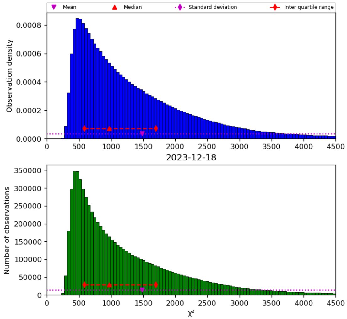
Figure 22: Histogram of “ \chi^2 ” for 2023-12-17 to 2023-12-19
