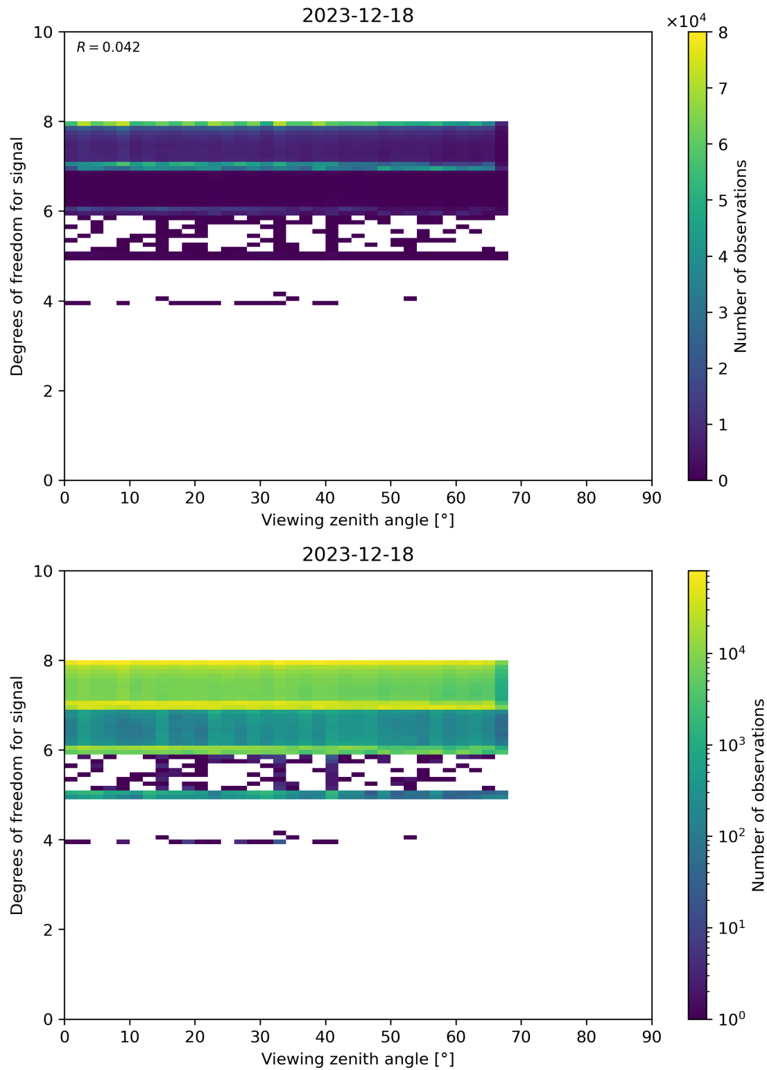
Figure 73: Scatter density plot of “Viewing zenith angle” against “Degrees of freedom for signal” for 2023-12-17 to 2023-12-19.
