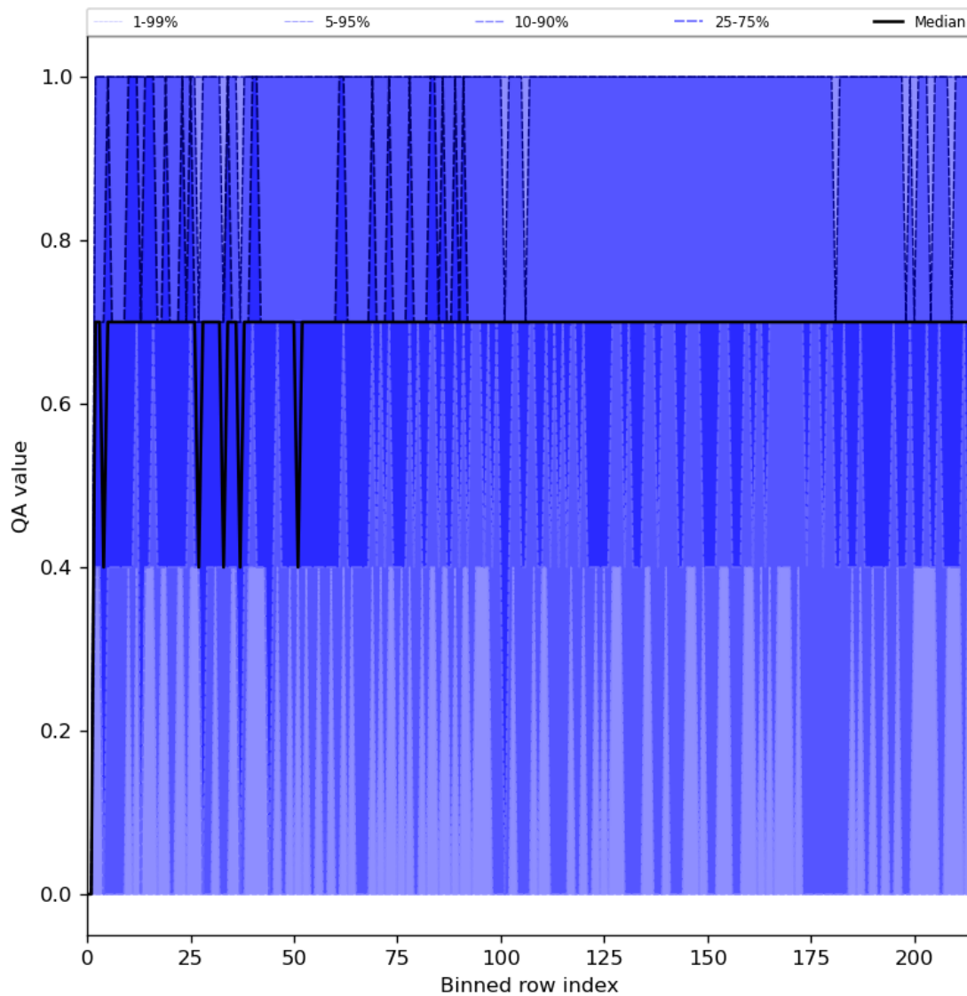
Figure 25: Along track statistics of “QA value” for 2023-12-17 to 2023-12-19
