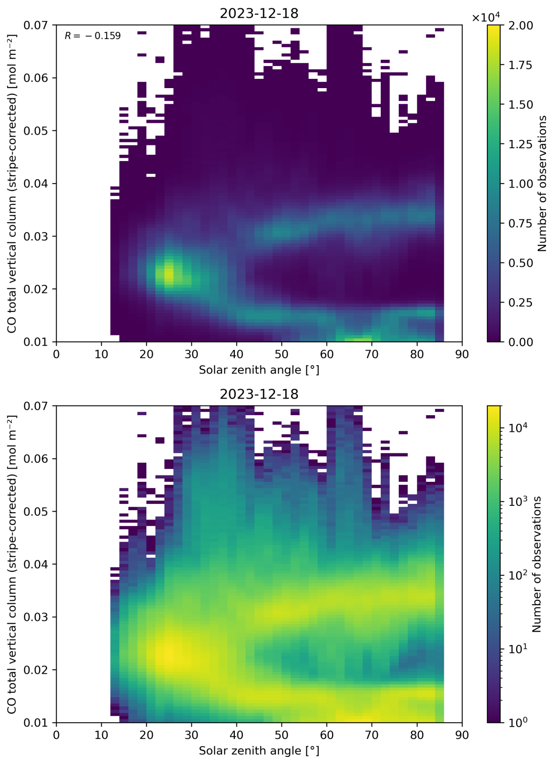
Figure 62: Scatter density plot of “Solar zenith angle” against “CO total vertical column (stripe-corrected)” for 2023-12-17 to 2023-12-19.
