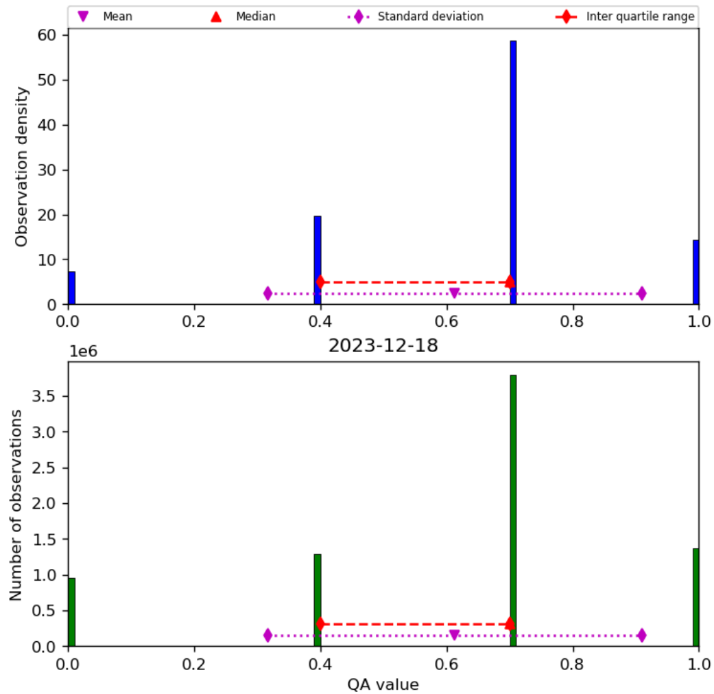
Figure 17: Histogram of “QA value” for 2023-12-17 to 2023-12-19
