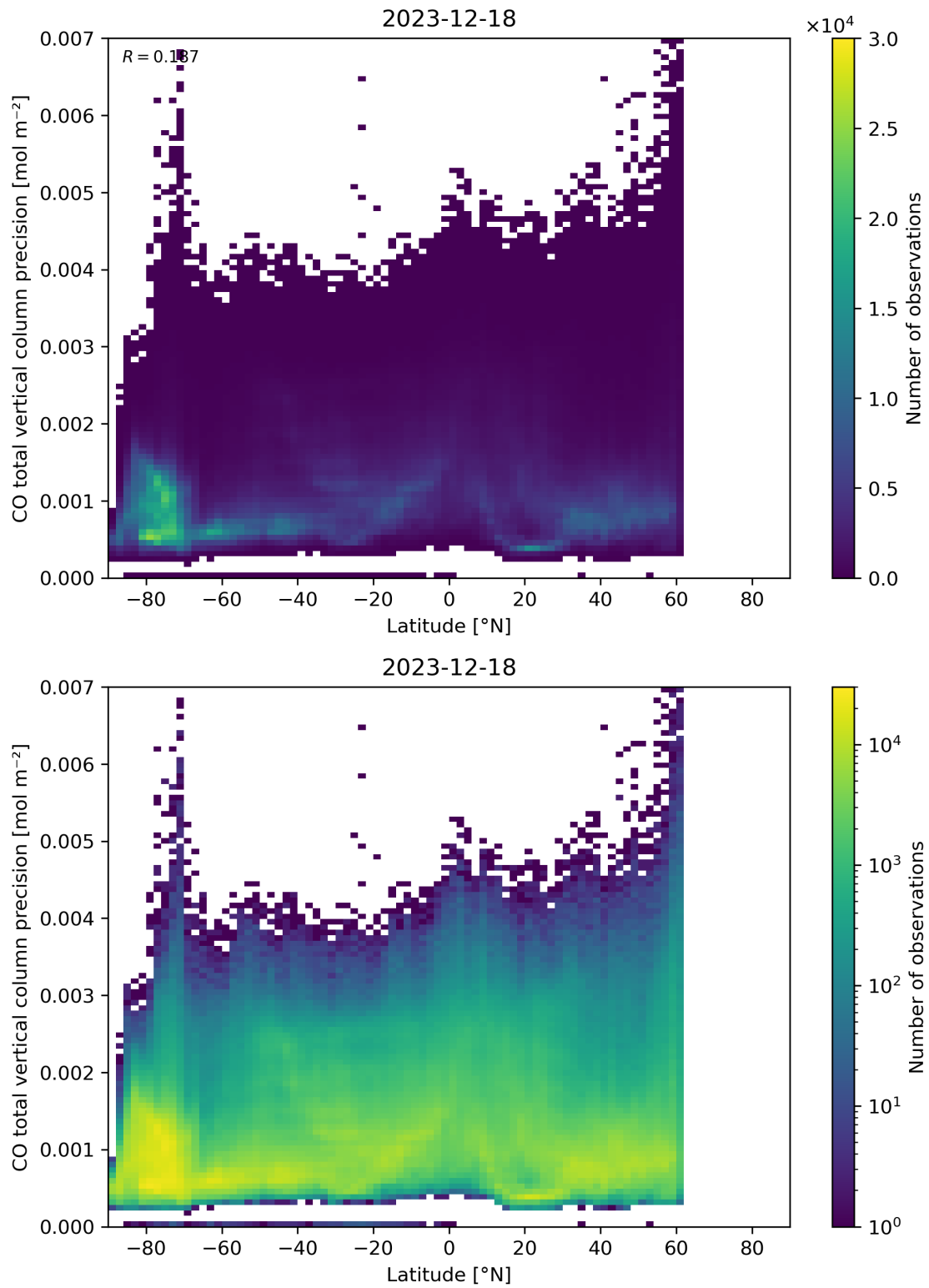
Figure 53: Scatter density plot of “Latitude” against “CO total vertical column precision” for 2023-12-17 to 2023-12-19.
