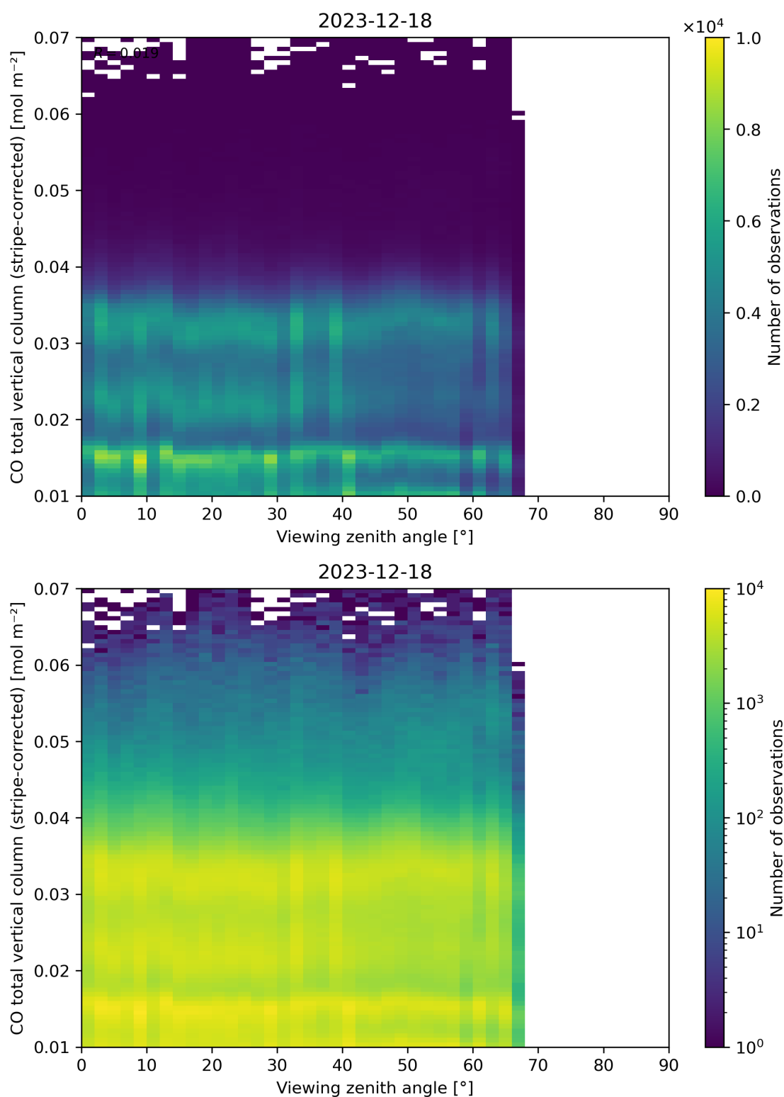
Figure 70: Scatter density plot of “Viewing zenith angle” against “CO total vertical column (stripe-corrected)” for 2023-12-17 to 2023-12-19.
