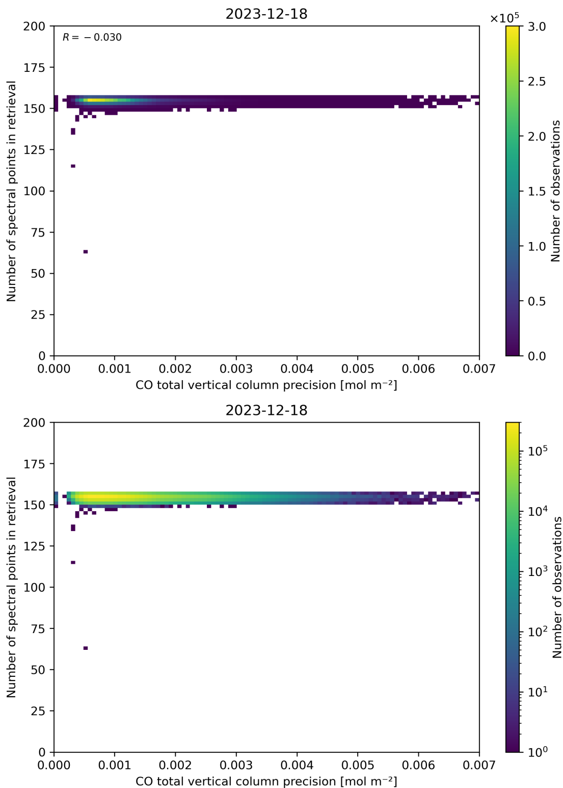
Figure 47: Scatter density plot of “CO total vertical column precision” against “Number of spectral points in retrieval” for 2023-12-17 to 2023-12-19.
