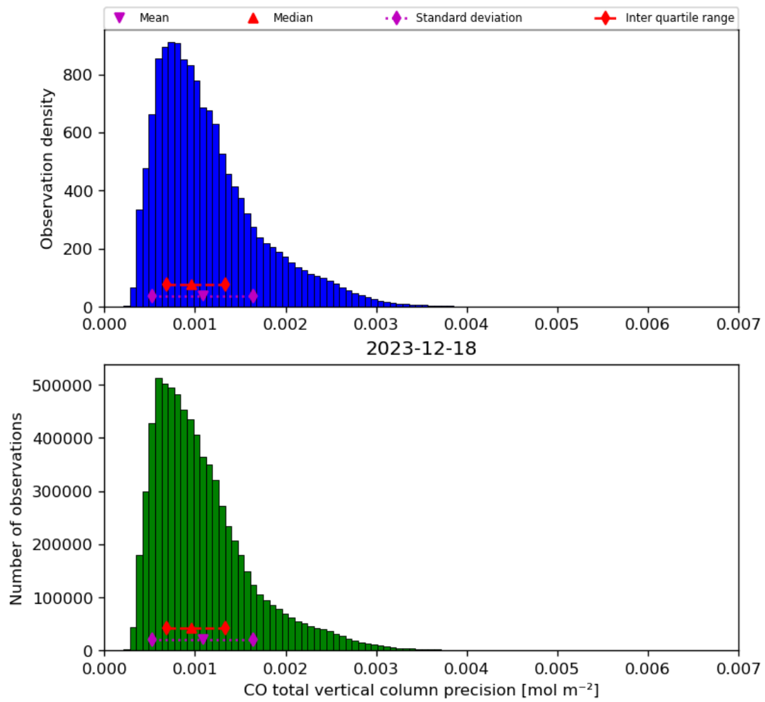
Figure 20: Histogram of “CO total vertical column precision” for 2023-12-17 to 2023-12-19
