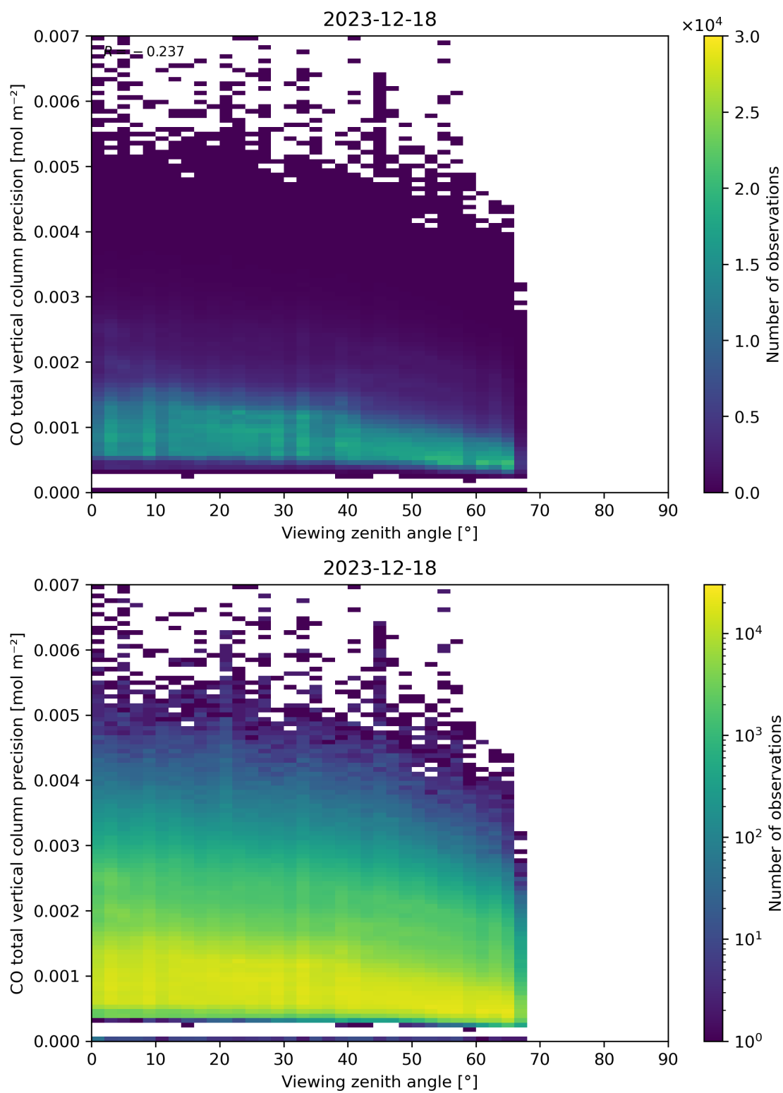
Figure 71: Scatter density plot of “Viewing zenith angle” against “CO total vertical column precision” for 2023-12-17 to 2023-12-19.
