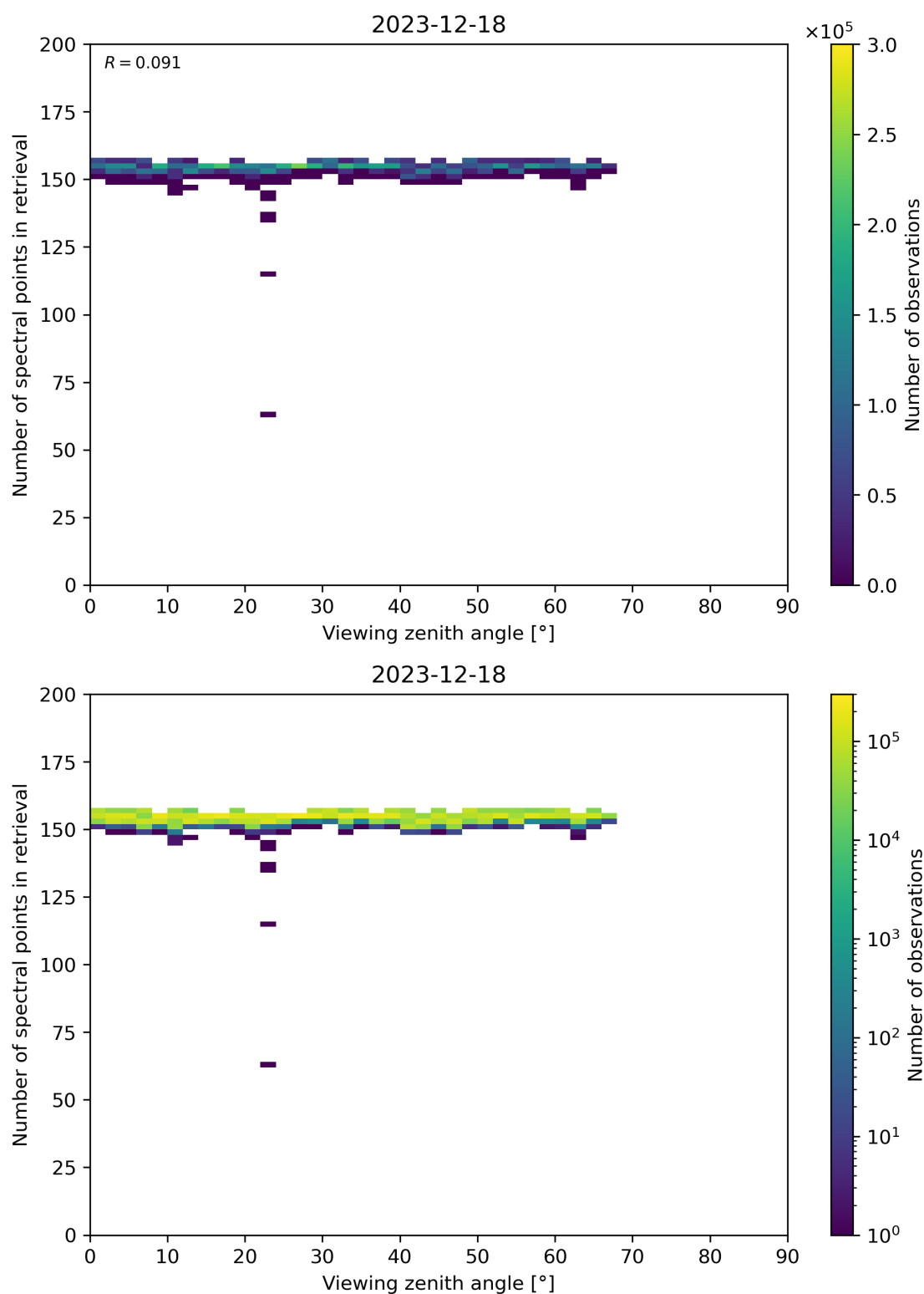
Figure 76: Scatter density plot of “Viewing zenith angle” against “Number of spectral points in retrieval” for 2023-12-17 to 2023-12-19.
