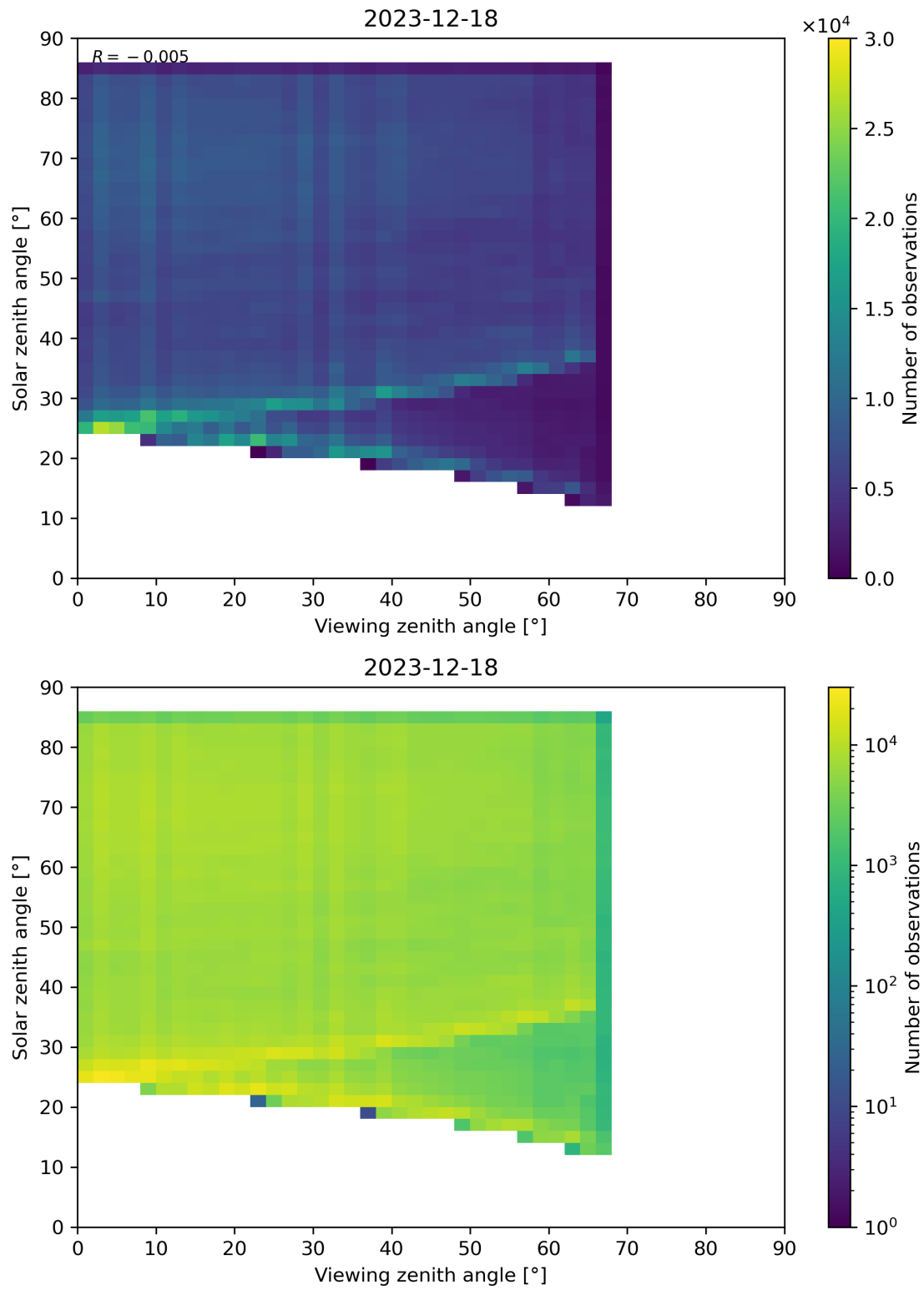
Figure 77: Scatter density plot of “Viewing zenith angle” against “Solar zenith angle” for 2023-12-17 to 2023-12-19.
