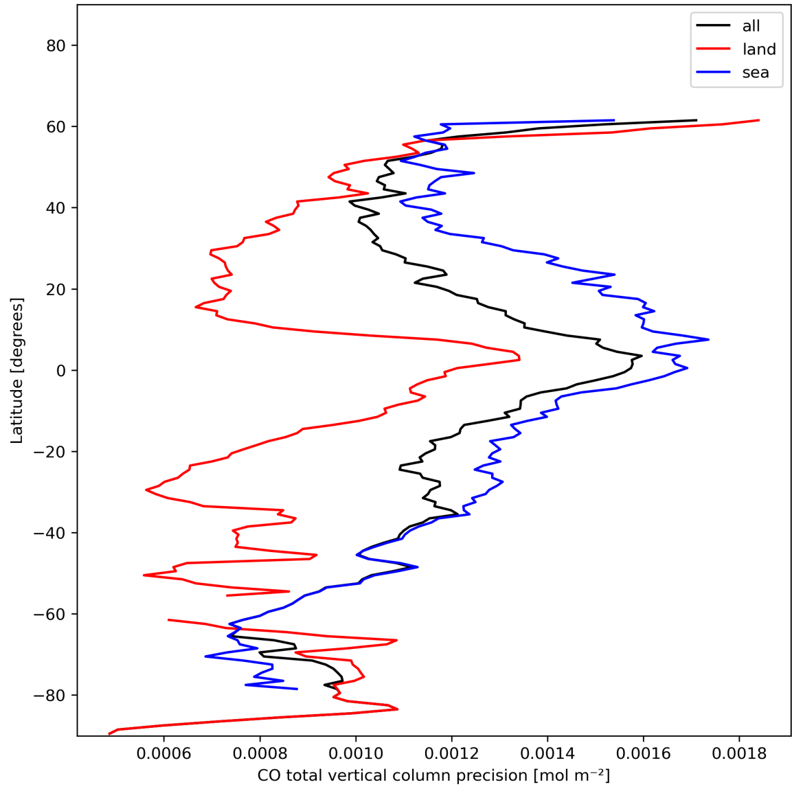
Figure 12: Zonal average of “CO total vertical column precision” for 2023-12-17 to 2023-12-19.
