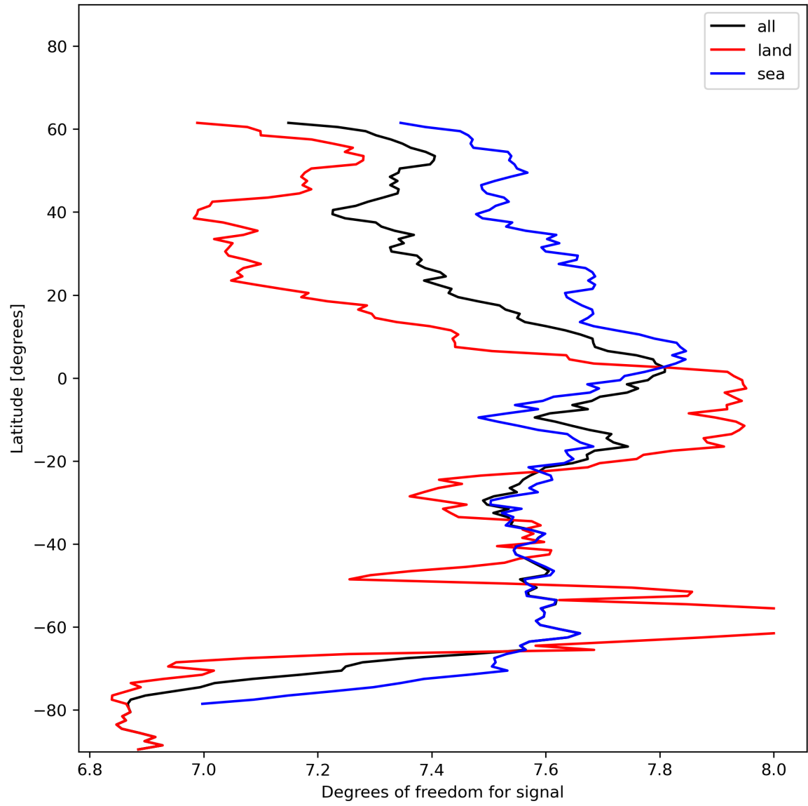
Figure 15: Zonal average of “Degrees of freedom for signal” for 2023-12-17 to 2023-12-19.
