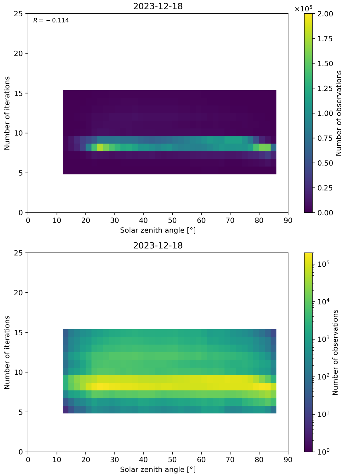
Figure 67: Scatter density plot of “Solar zenith angle” against “Number of iterations” for 2023-12-17 to 2023-12-19.
