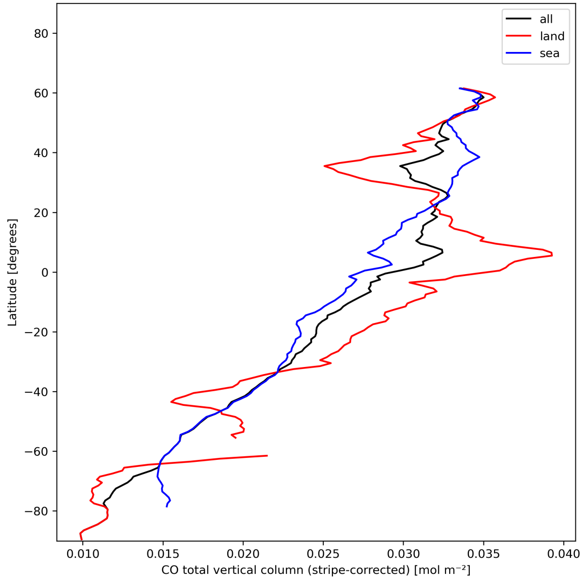
Figure 11: Zonal average of “CO total vertical column (stripe-corrected)” for 2023-12-17 to 2023-12-19.
