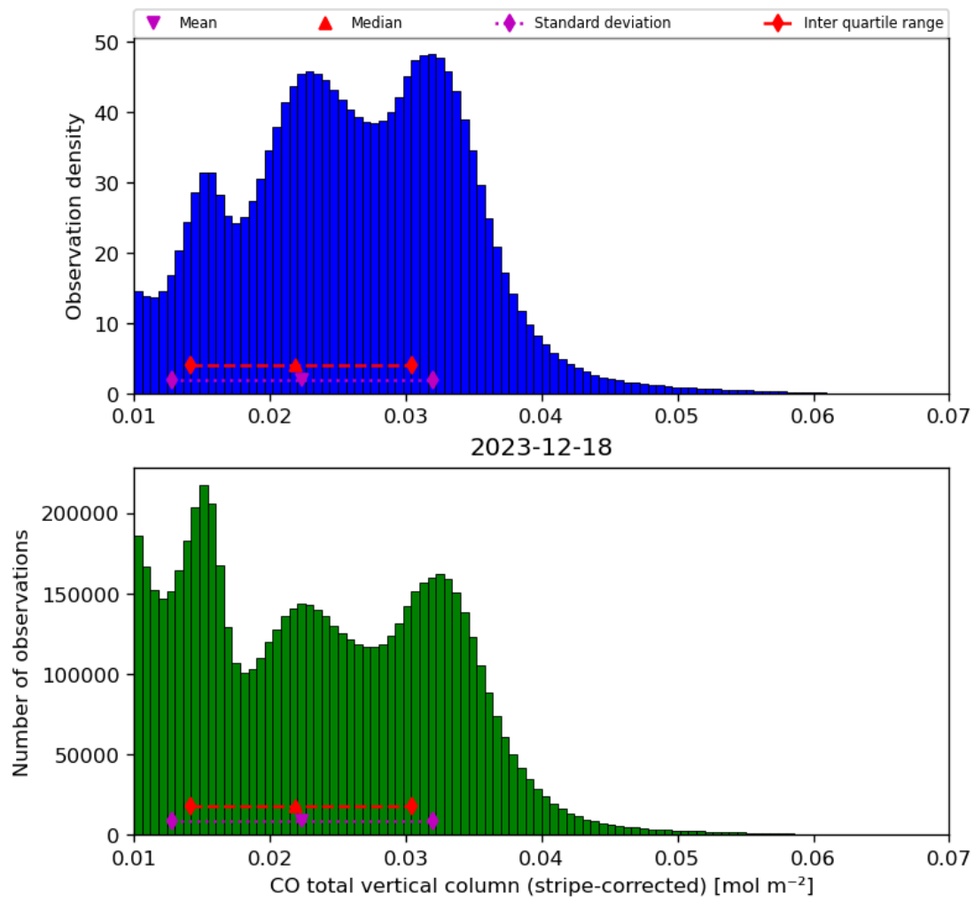
Figure 19: Histogram of “CO total vertical column (stripe-corrected)” for 2023-12-17 to 2023-12-19
