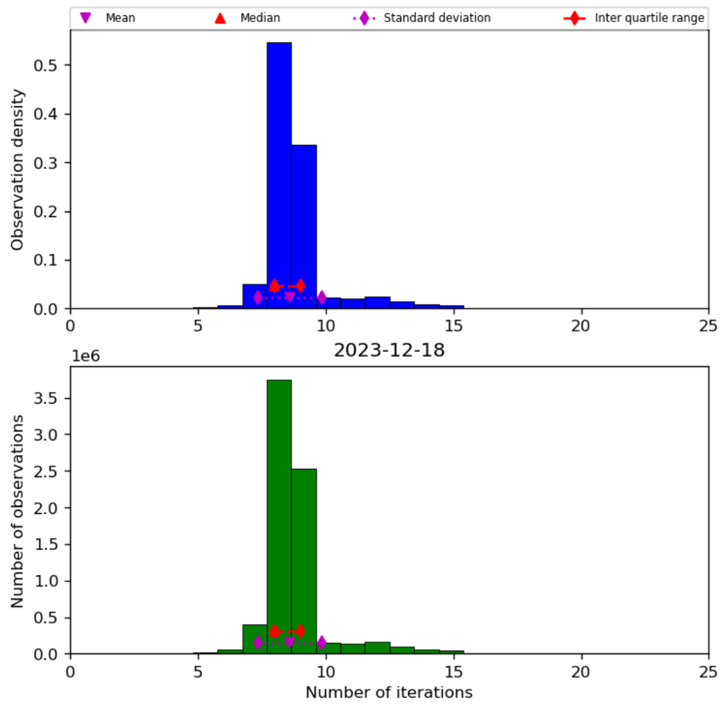
Figure 24: Histogram of “Number of iterations” for 2023-12-17 to 2023-12-19
