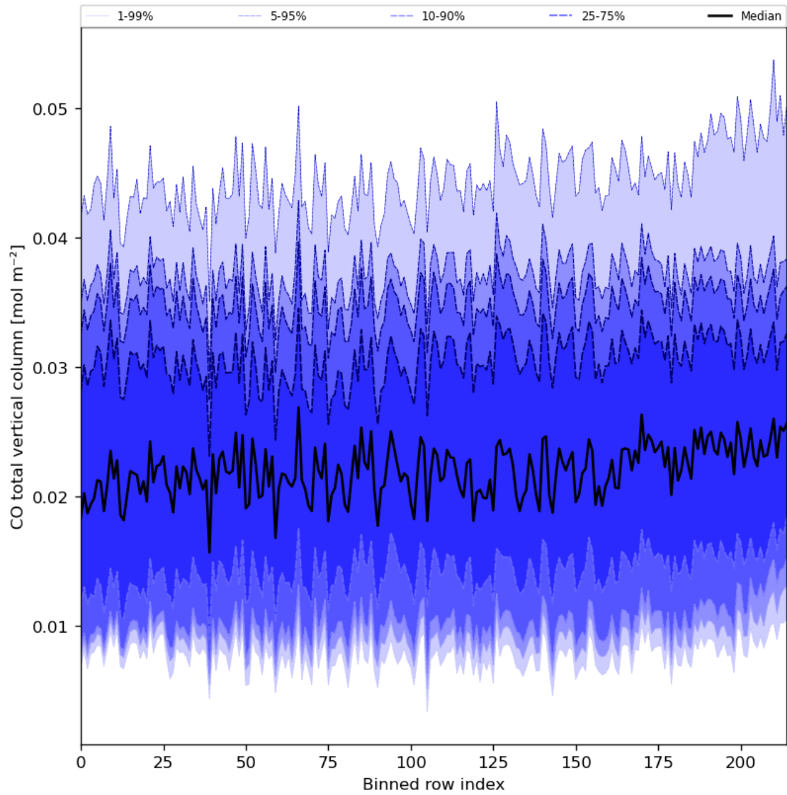
Figure 26: Along track statistics of “CO total vertical column” for 2023-12-17 to 2023-12-19
