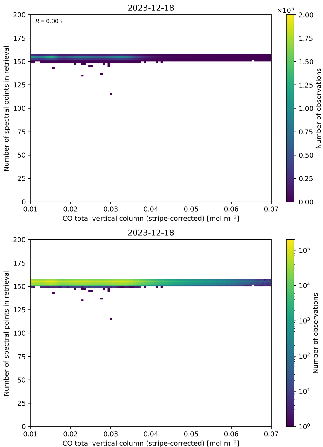
Figure 40: Scatter density plot of “CO total vertical column (stripe-corrected)” against “Number of spectral points in retrieval” for 2023-12-17 to 2023-12-19.
