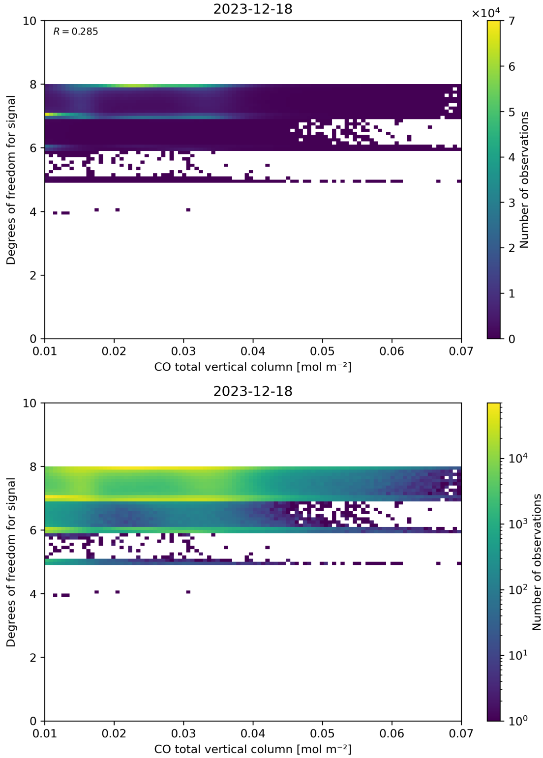
Figure 41: Scatter density plot of “CO total vertical column” against “Degrees of freedom for signal” for 2023-12-17 to 2023-12-19.
