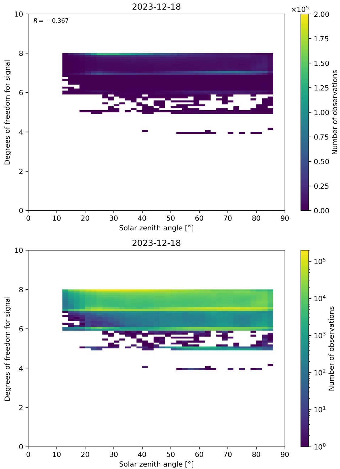
Figure 65: Scatter density plot of “Solar zenith angle” against “Degrees of freedom for signal” for 2023-12-17 to 2023-12-19.
