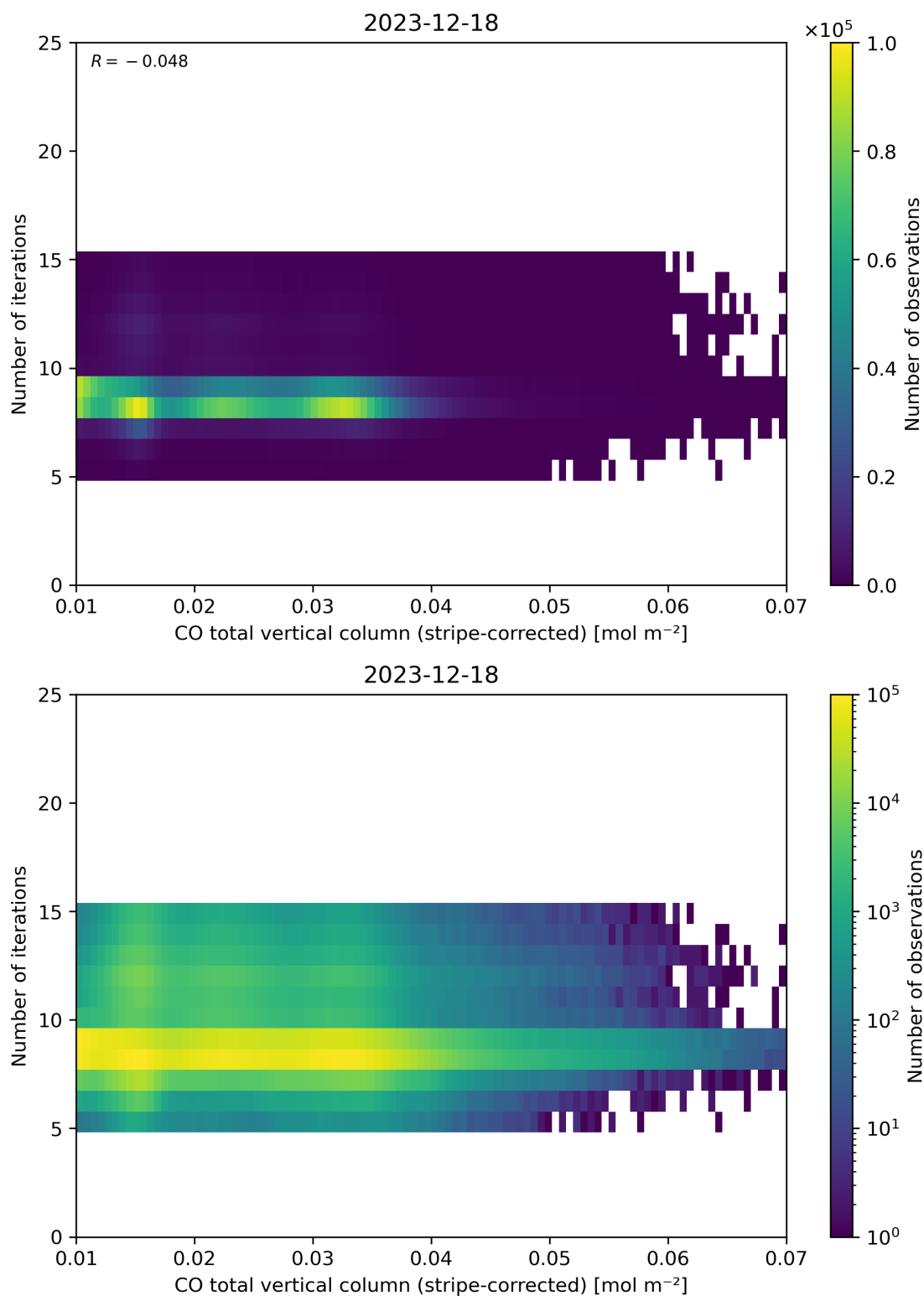
Figure 39: Scatter density plot of “CO total vertical column (stripe-corrected)” against “Number of iterations” for 2023-12-17 to 2023-12-19.
