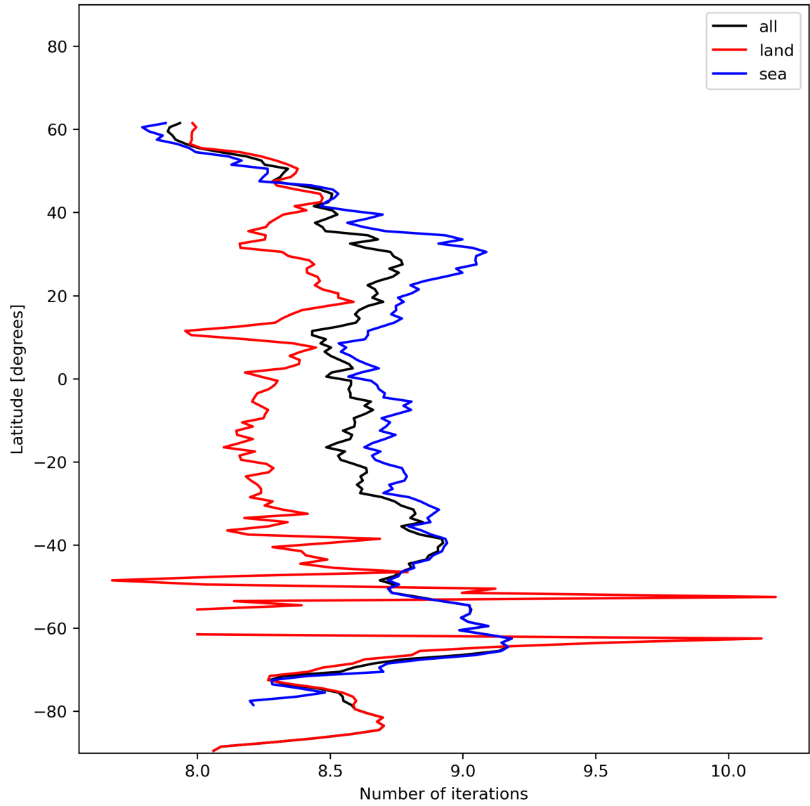
Figure 16: Zonal average of “Number of iterations” for 2023-12-17 to 2023-12-19.
