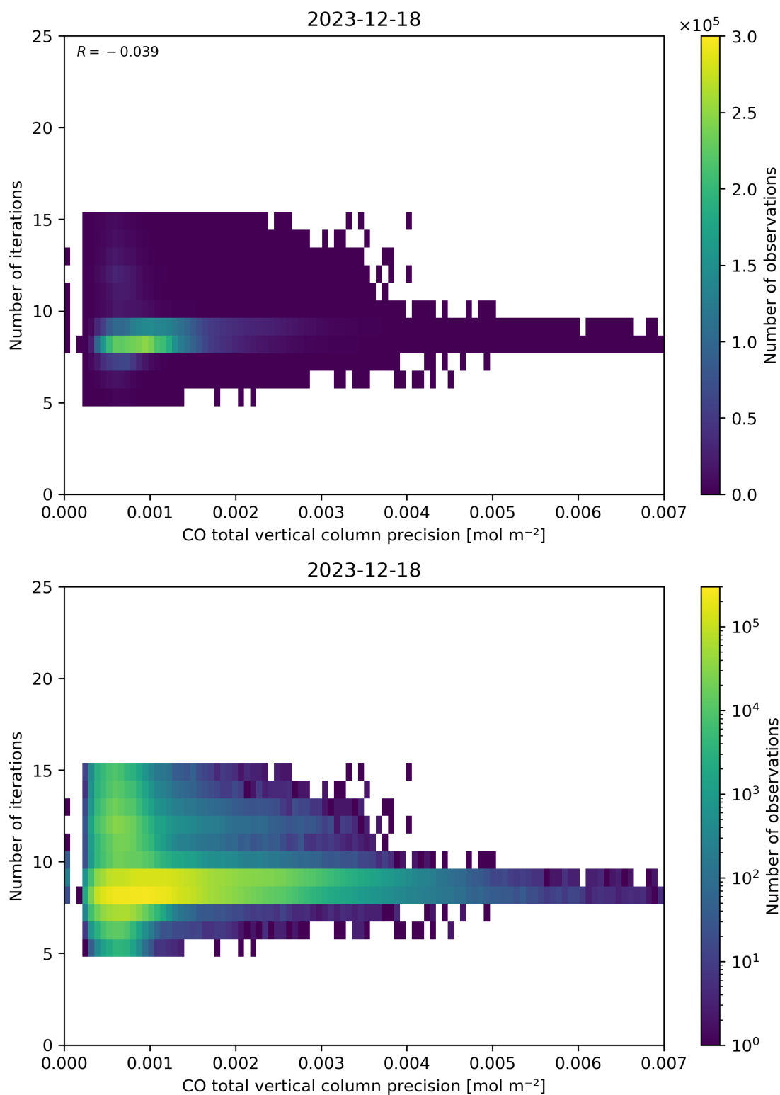
Figure 46: Scatter density plot of “CO total vertical column precision” against “Number of iterations” for 2023-12-17 to 2023-12-19.
