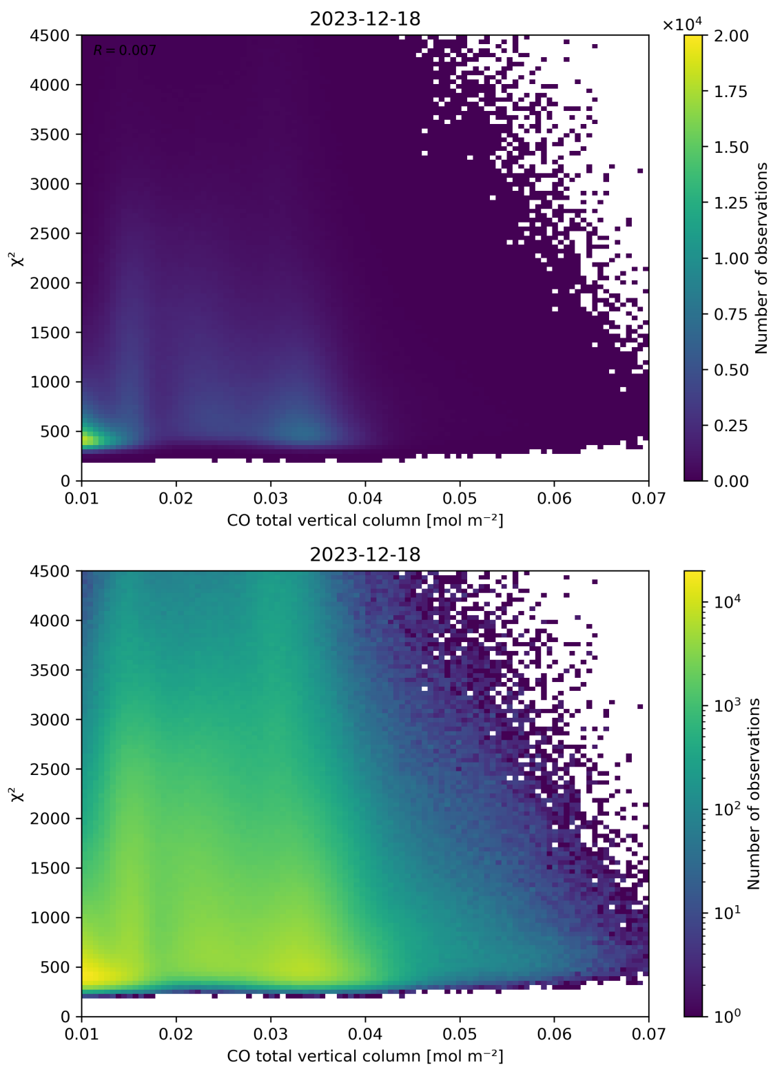
Figure 35: Scatter density plot of “CO total vertical column” against “ \chi^2 ” for 2023-12-17 to 2023-12-19.
