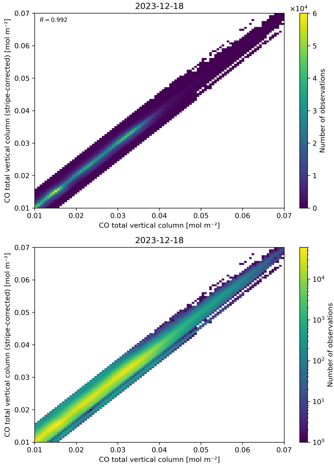
Figure 33: Scatter density plot of “CO total vertical column” against “CO total vertical column (stripe-corrected)” for 2023-12-17 to 2023-12-19.
