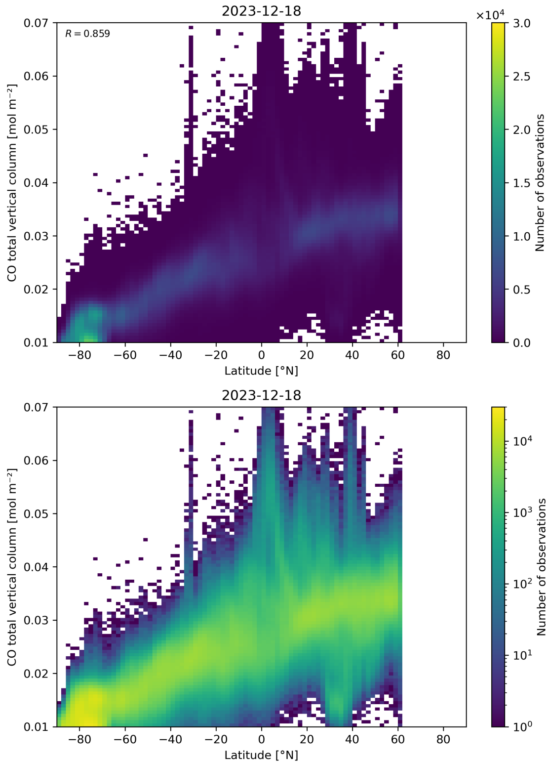
Figure 51: Scatter density plot of “Latitude” against “CO total vertical column” for 2023-12-17 to 2023-12-19.
