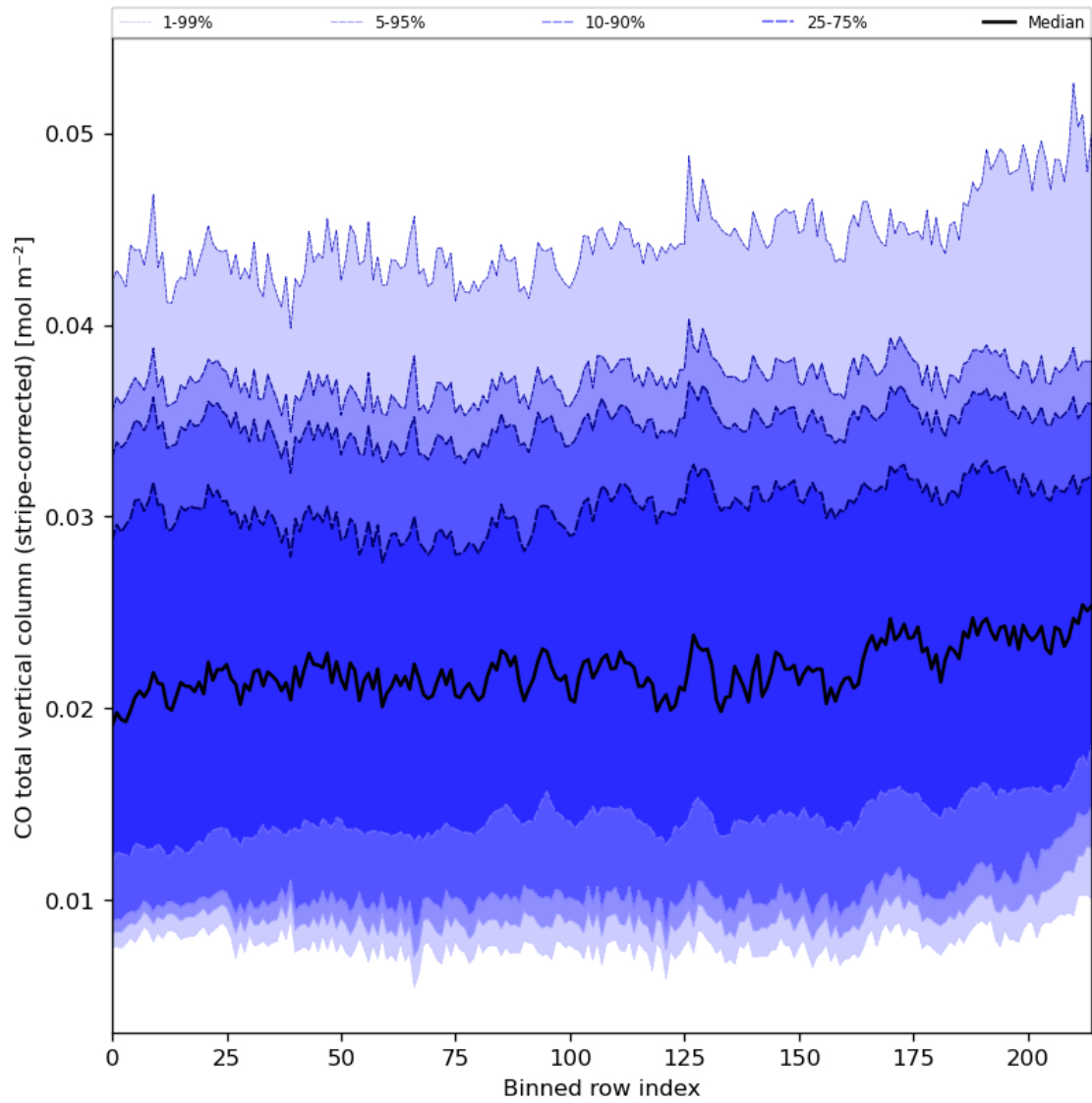
Figure 27: Along track statistics of “CO total vertical column (stripe-corrected)” for 2023-12-17 to 2023-12-19
