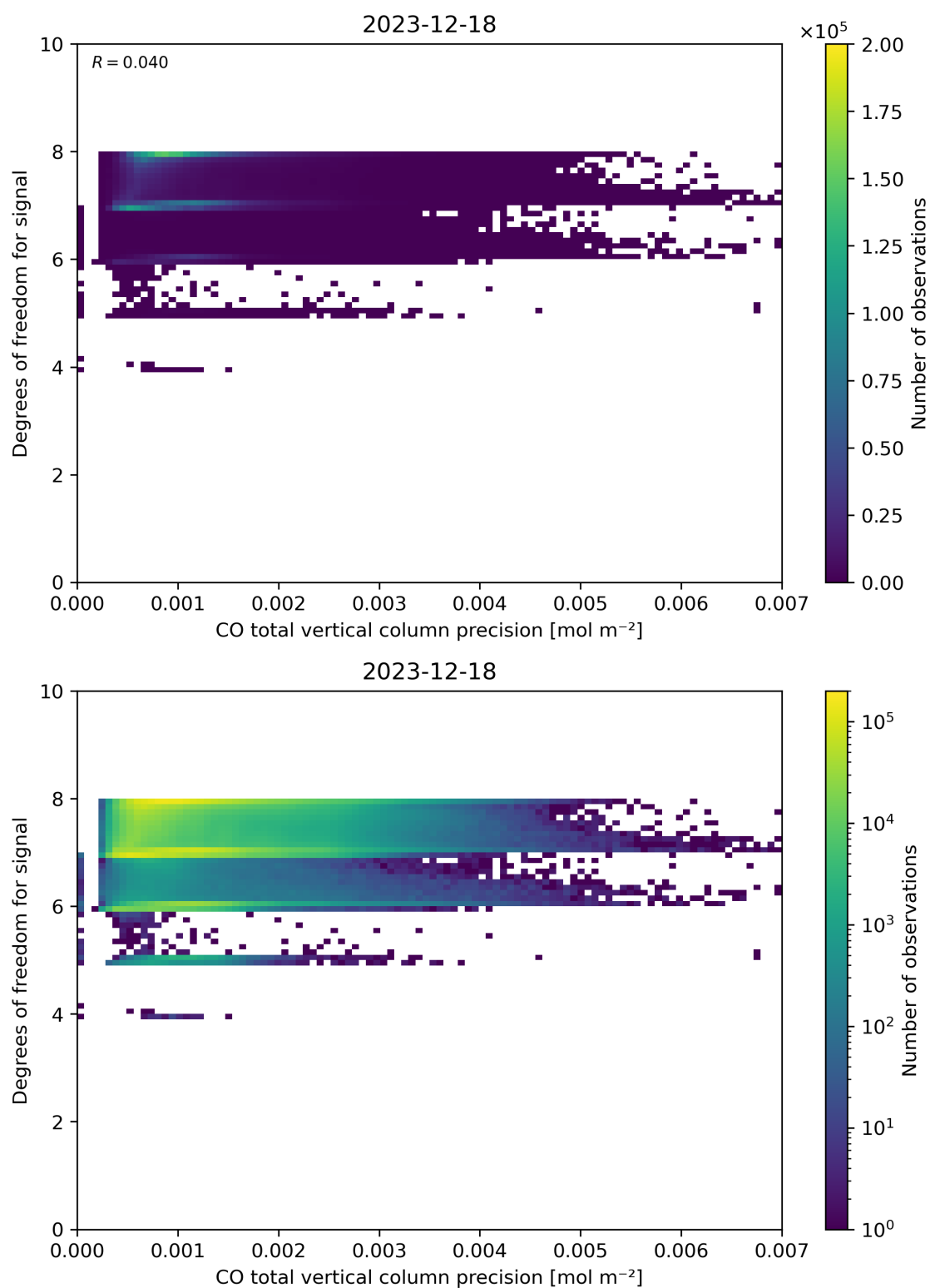
Figure 45: Scatter density plot of “CO total vertical column precision” against “Degrees of freedom for signal” for 2023-12-17 to 2023-12-19.
