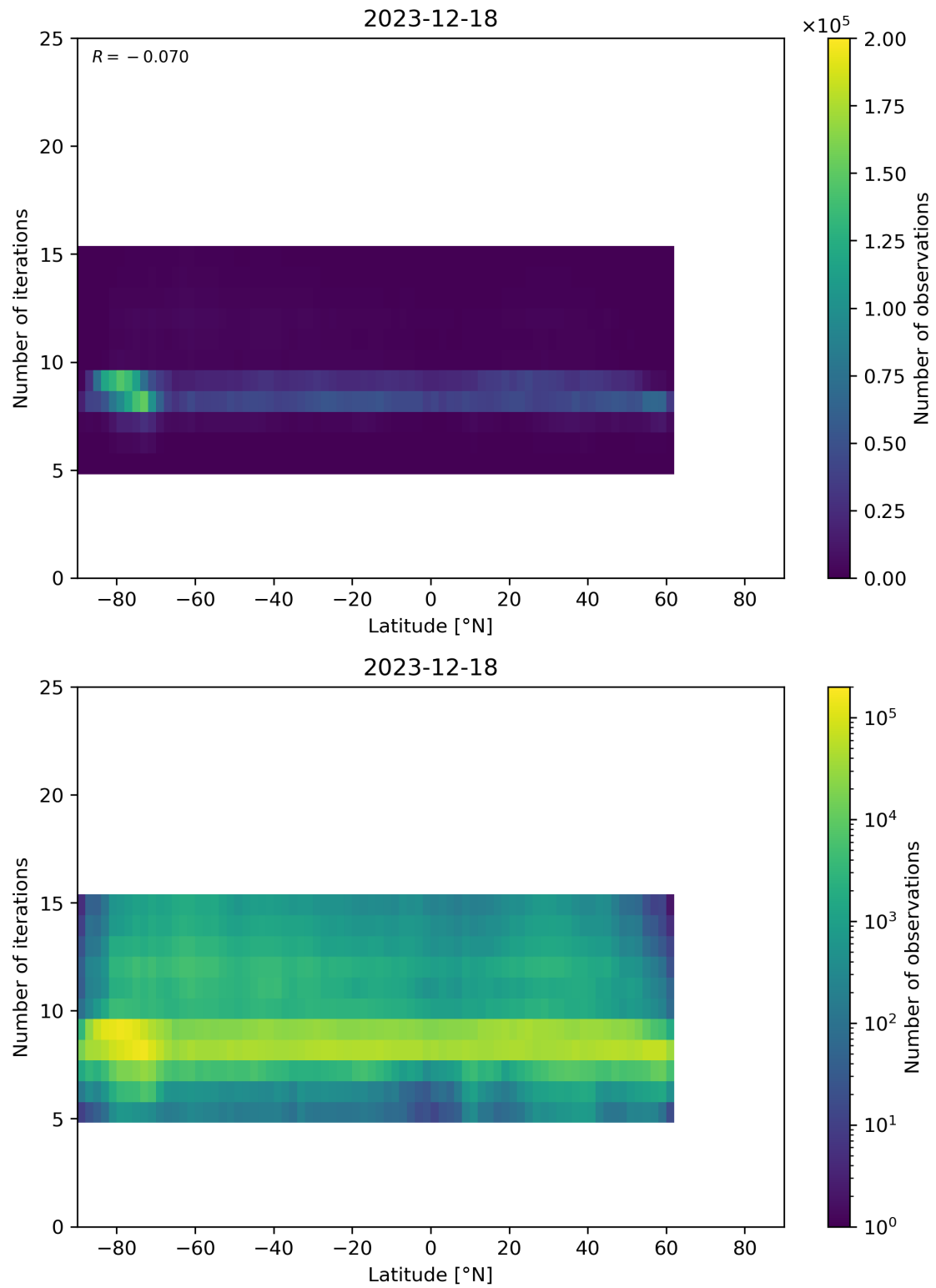
Figure 56: Scatter density plot of “Latitude” against “Number of iterations” for 2023-12-17 to 2023-12-19.
