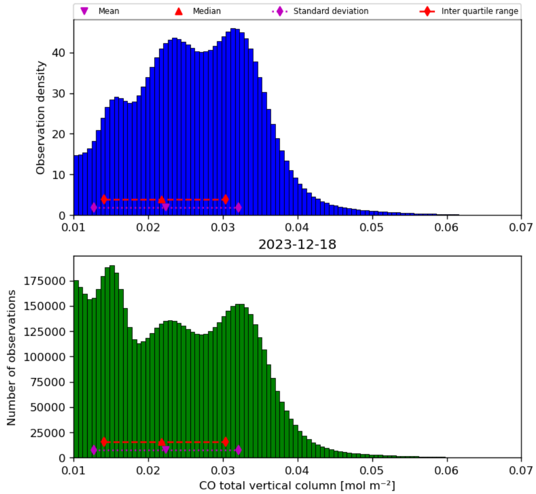
Figure 18: Histogram of “CO total vertical column” for 2023-12-17 to 2023-12-19
