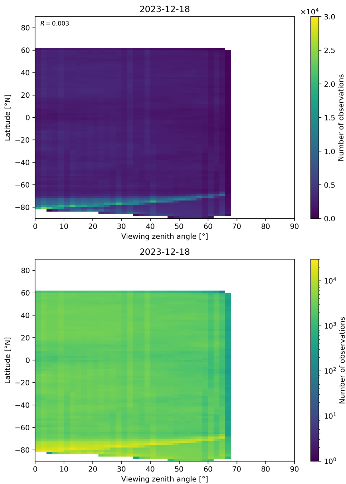
Figure 74: Scatter density plot of “Viewing zenith angle” against “Latitude” for 2023-12-17 to 2023-12-19.
