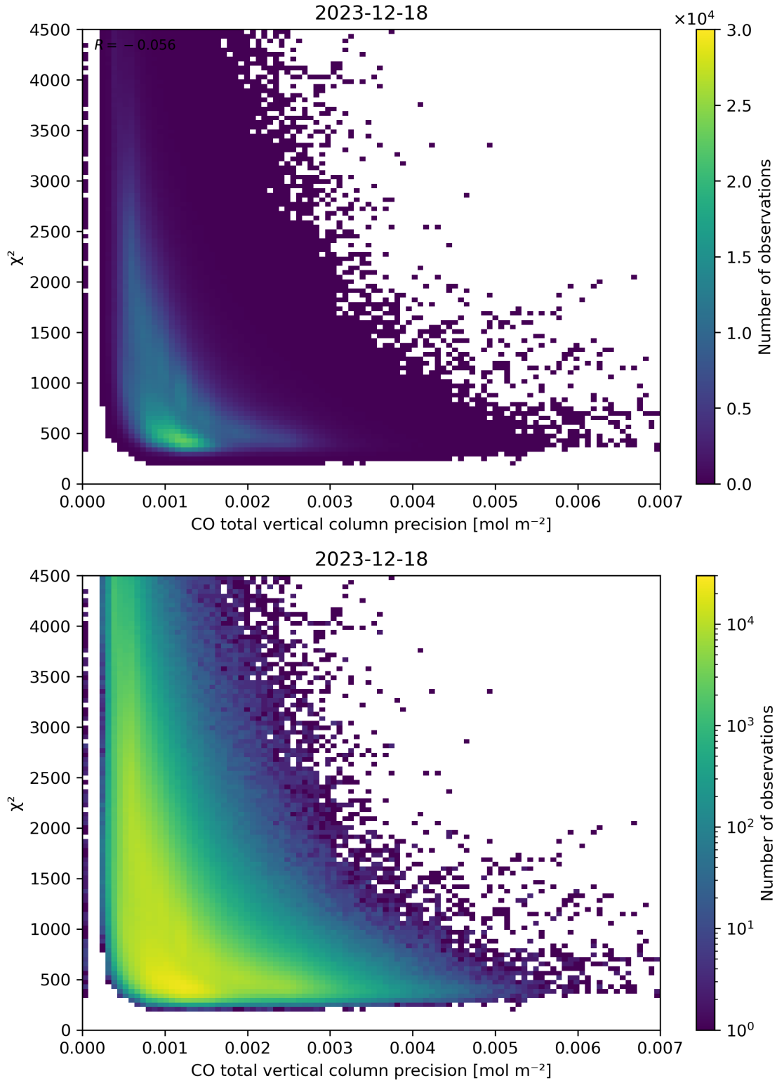
Figure 44: Scatter density plot of “CO total vertical column precision” against “ \chi^2 ” for 2023-12-17 to 2023-12-19.
