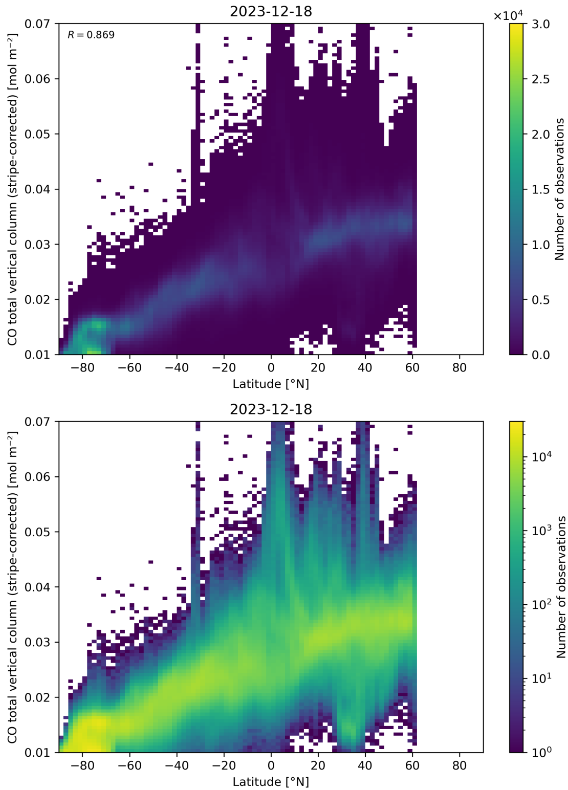
Figure 52: Scatter density plot of “Latitude” against “CO total vertical column (stripe-corrected)” for 2023-12-17 to 2023-12-19.
