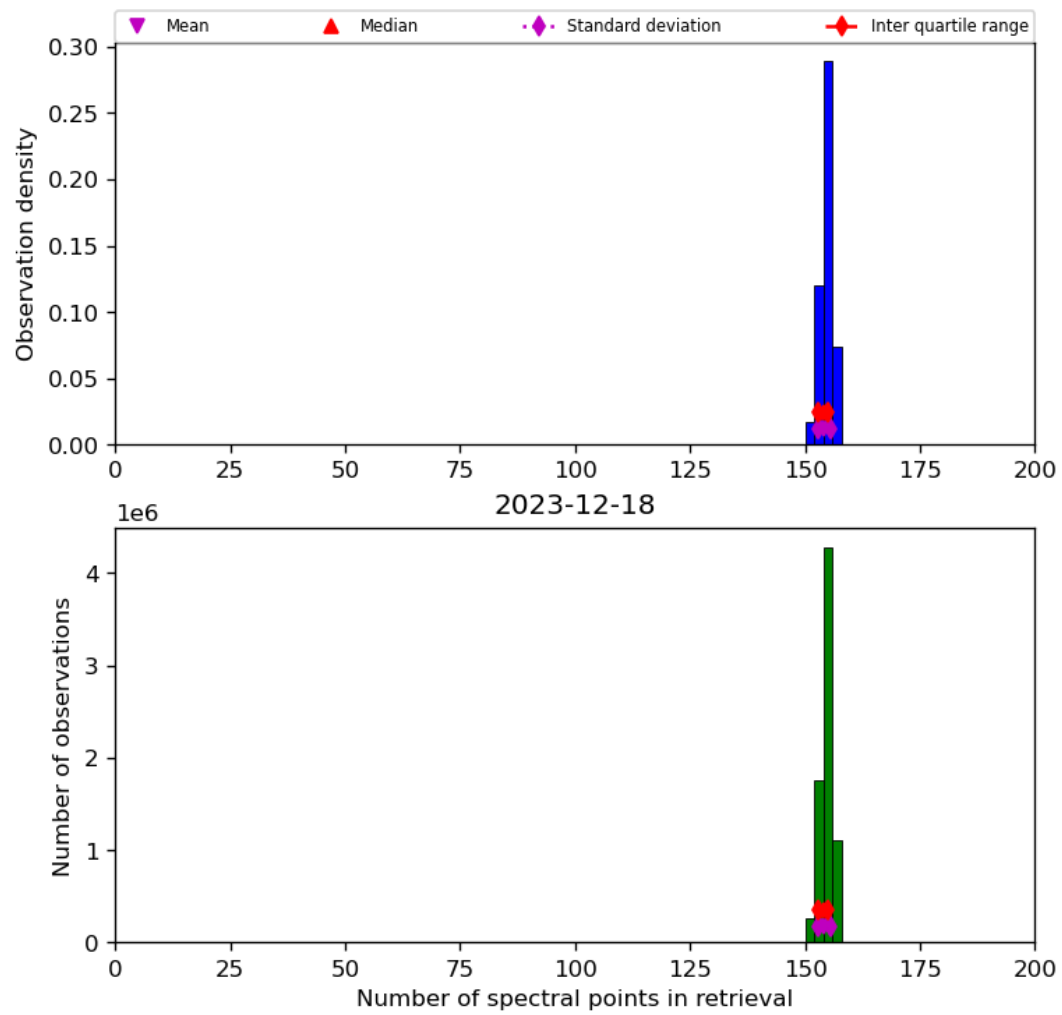
Figure 21: Histogram of “Number of spectral points in retrieval” for 2023-12-17 to 2023-12-19
