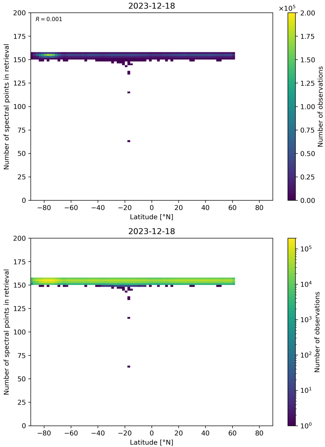
Figure 57: Scatter density plot of “Latitude” against “Number of spectral points in retrieval” for 2023-12-17 to 2023-12-19.
