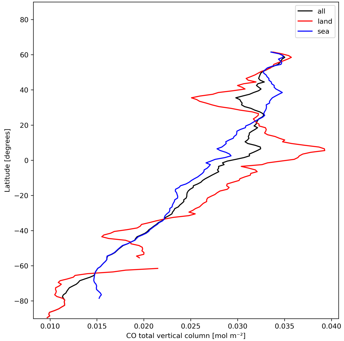
Figure 10: Zonal average of “CO total vertical column” for 2023-12-17 to 2023-12-19.
