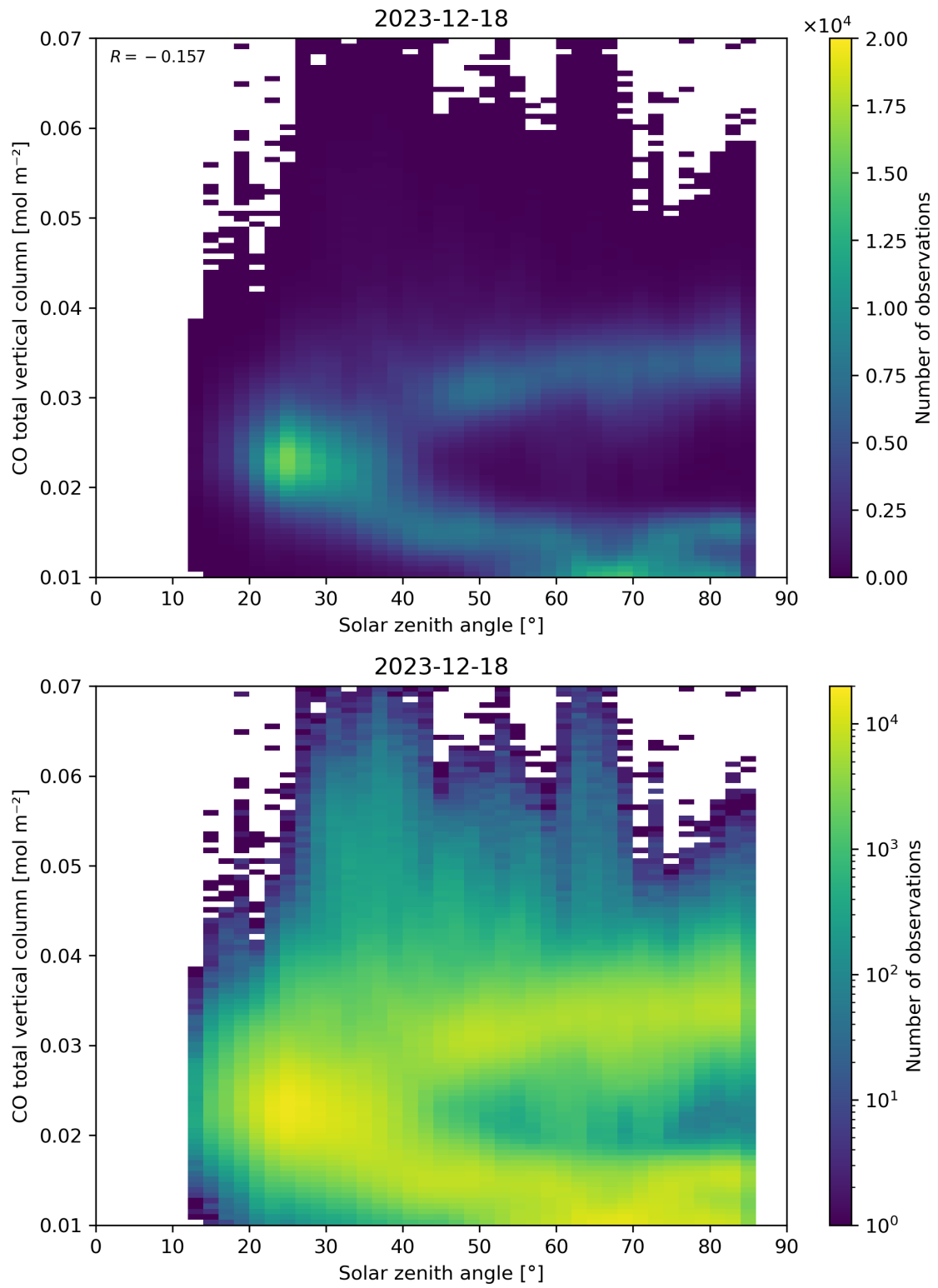
Figure 61: Scatter density plot of “Solar zenith angle” against “CO total vertical column” for 2023-12-17 to 2023-12-19.
