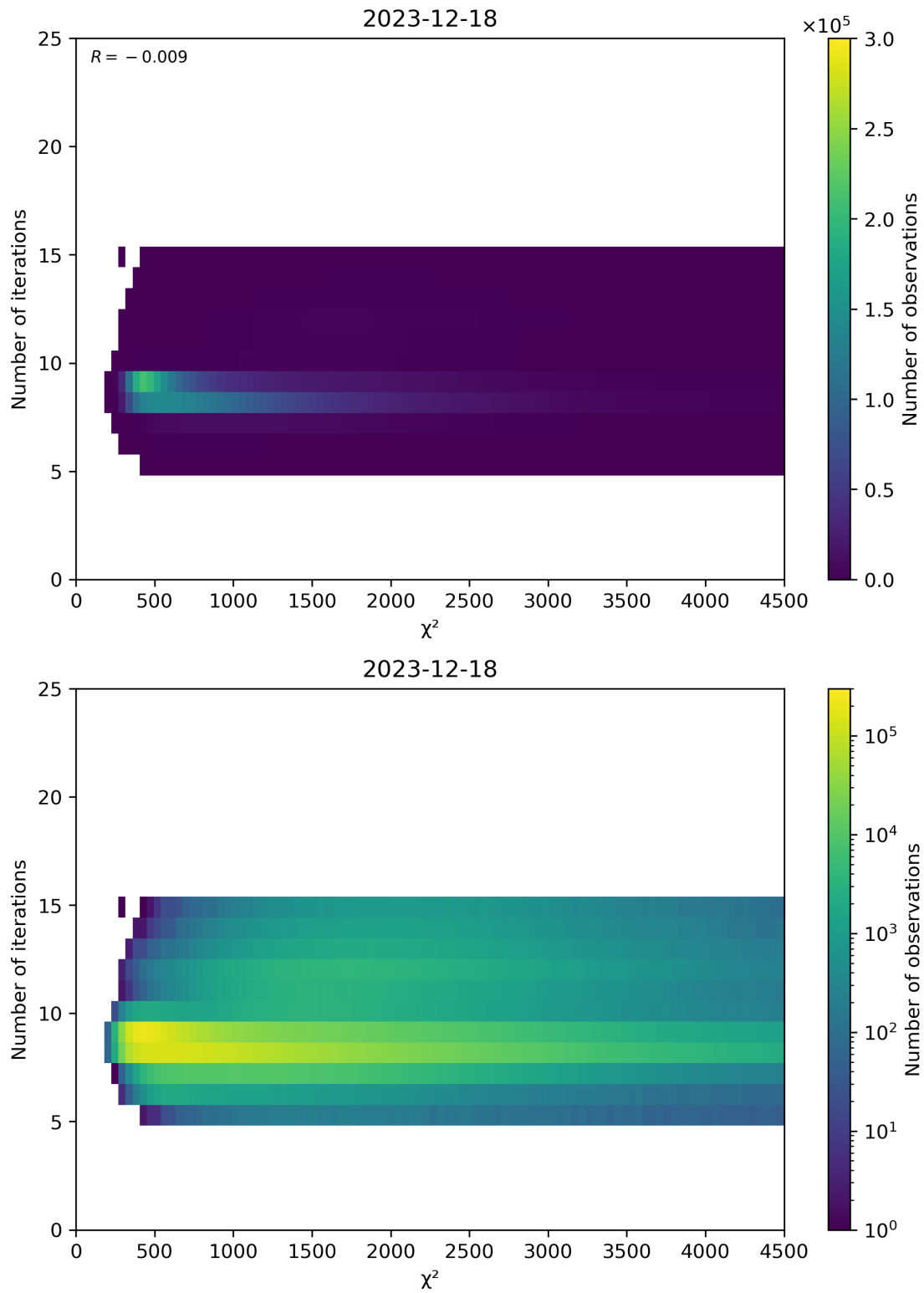
Figure 49: Scatter density plot of “ \chi^2 ” against “Number of iterations” for 2023-12-17 to 2023-12-19.
