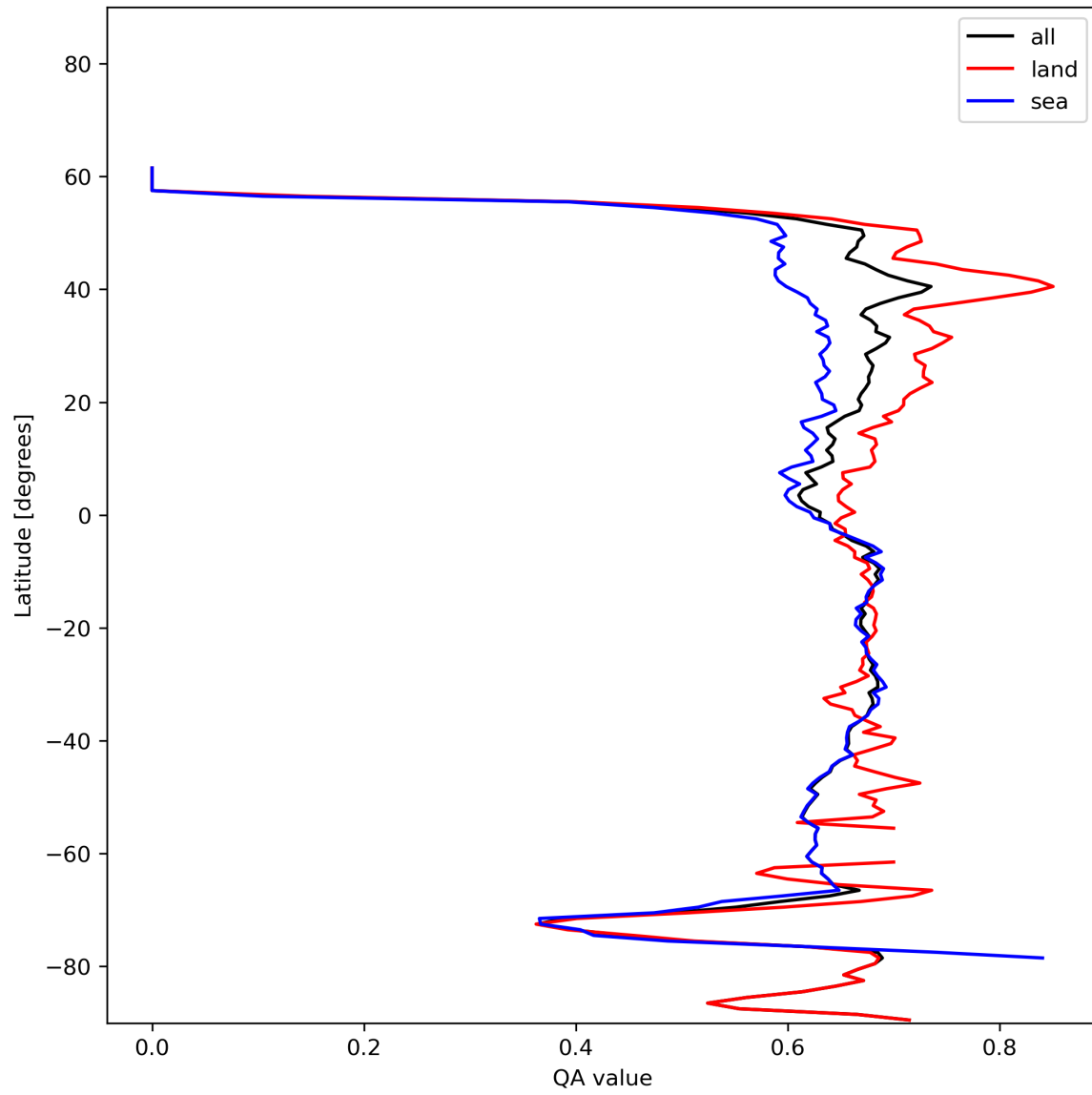
Figure 9: Zonal average of “QA value” for 2023-12-17 to 2023-12-19.
