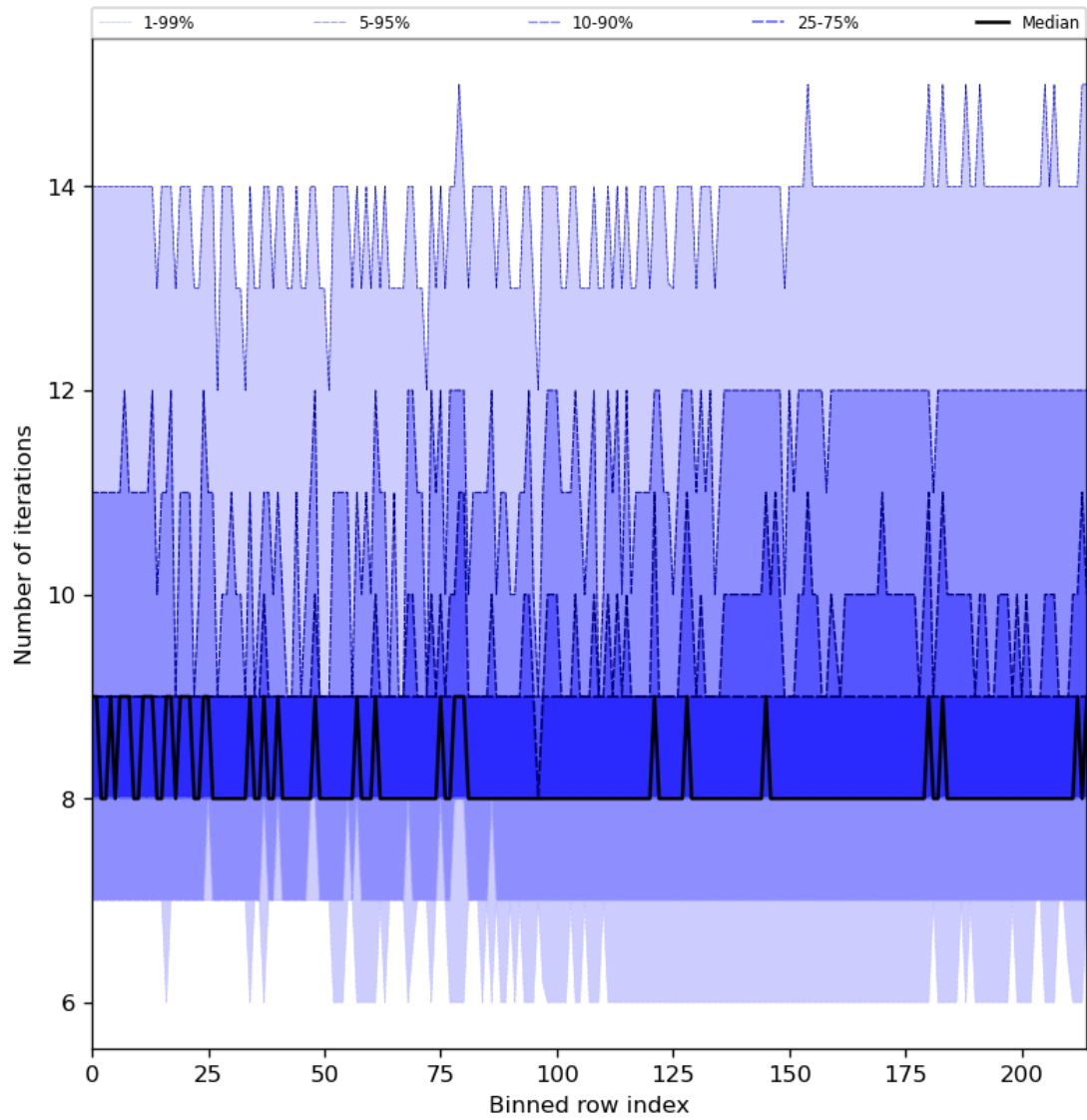
Figure 32: Along track statistics of “Number of iterations” for 2023-12-17 to 2023-12-19
