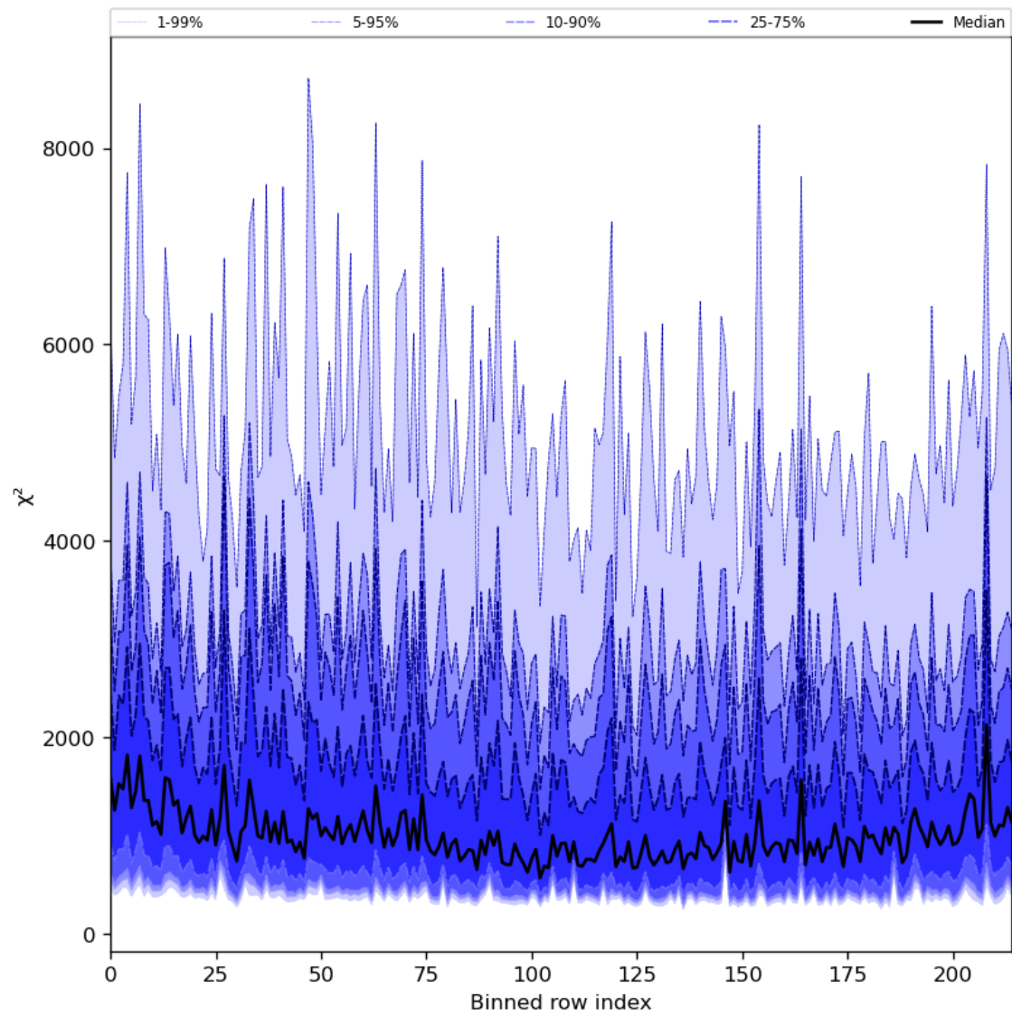
Figure 30: Along track statistics of “ \chi^2 ” for 2023-12-17 to 2023-12-19
