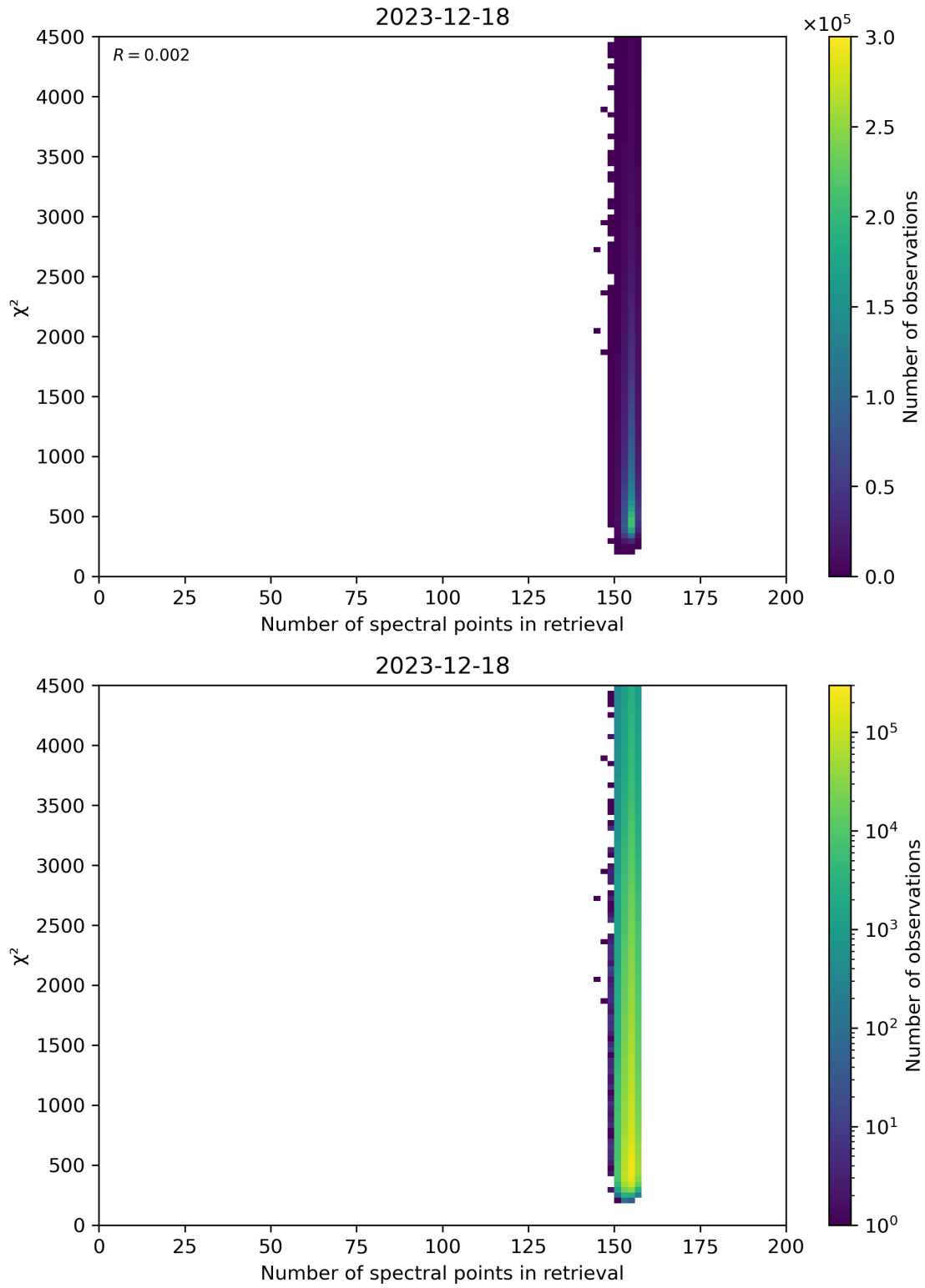
Figure 58: Scatter density plot of “Number of spectral points in retrieval” against “ \chi^2 ” for 2023-12-17 to 2023-12-19.
