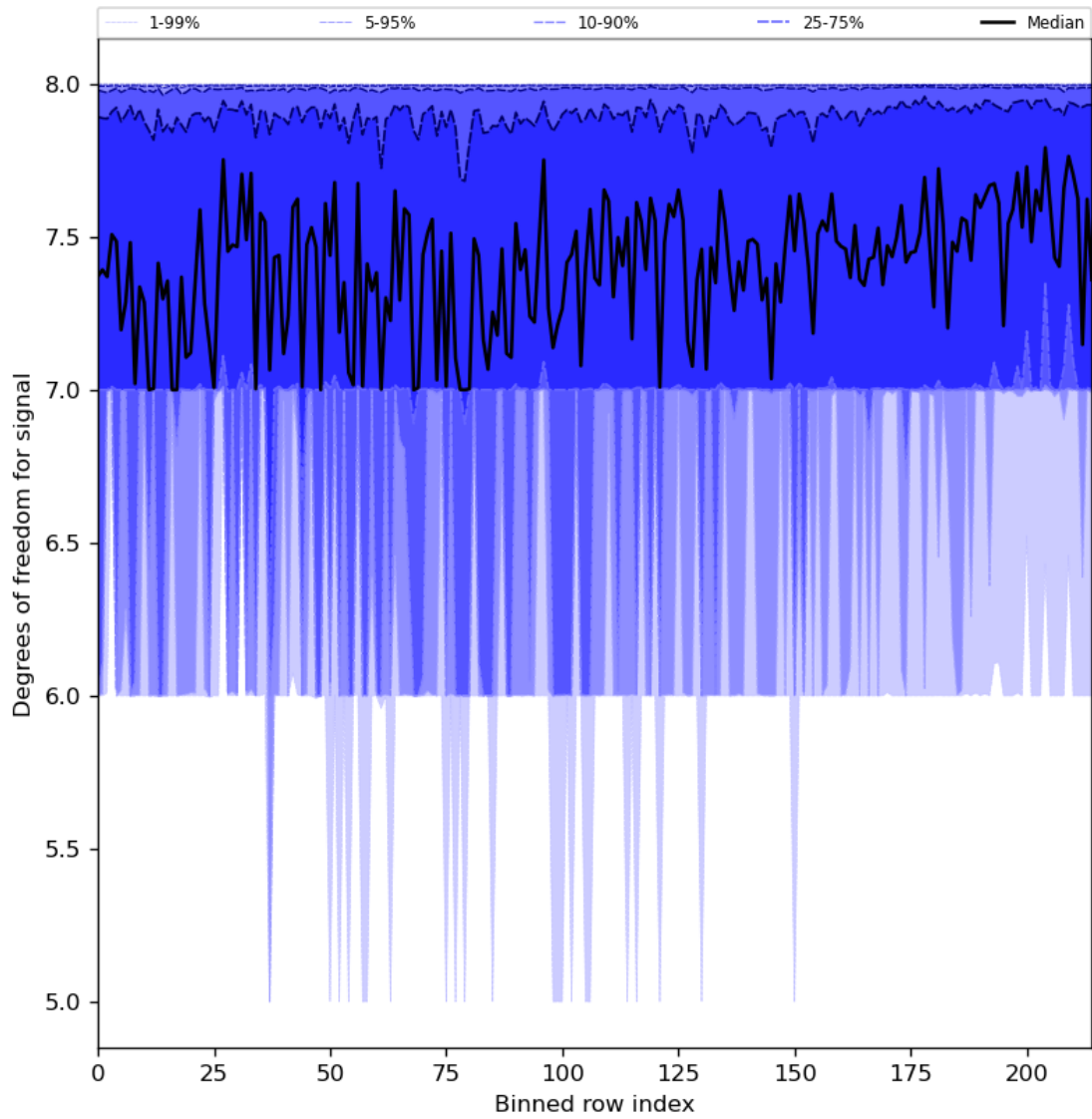
Figure 31: Along track statistics of “Degrees of freedom for signal” for 2023-12-17 to 2023-12-19
