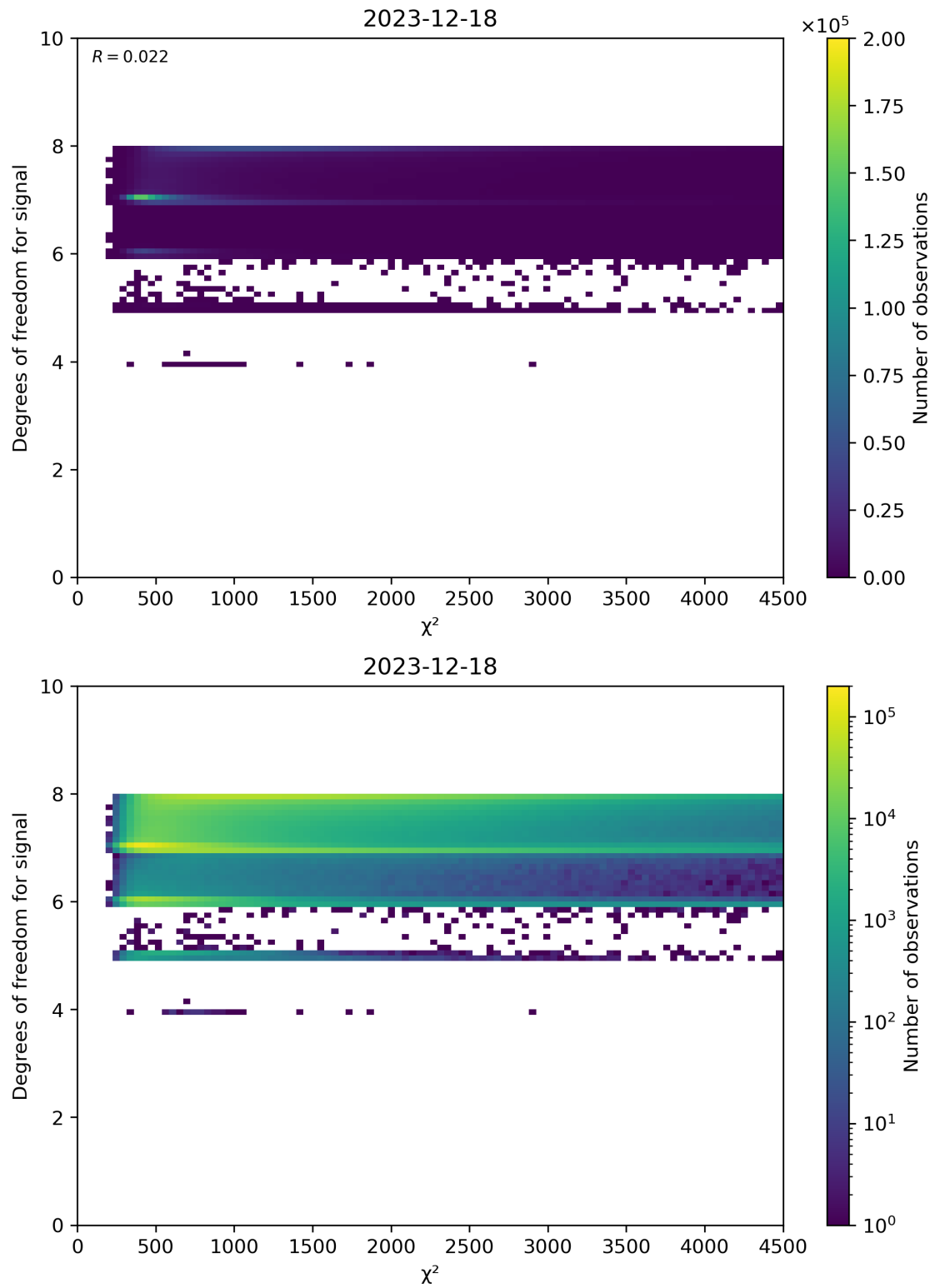
Figure 48: Scatter density plot of “ \chi^2 ” against “Degrees of freedom for signal” for 2023-12-17 to 2023-12-19.
