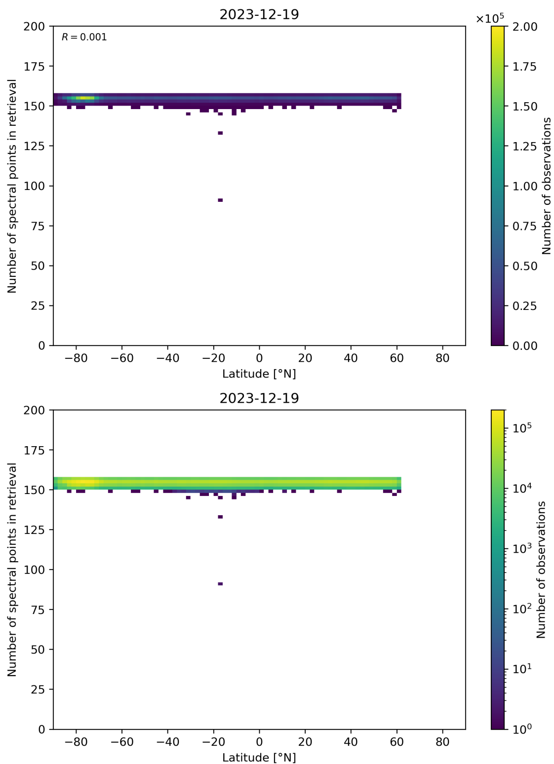
Figure 57: Scatter density plot of “Latitude” against “Number of spectral points in retrieval” for 2023-12-18 to 2023-12-20.
