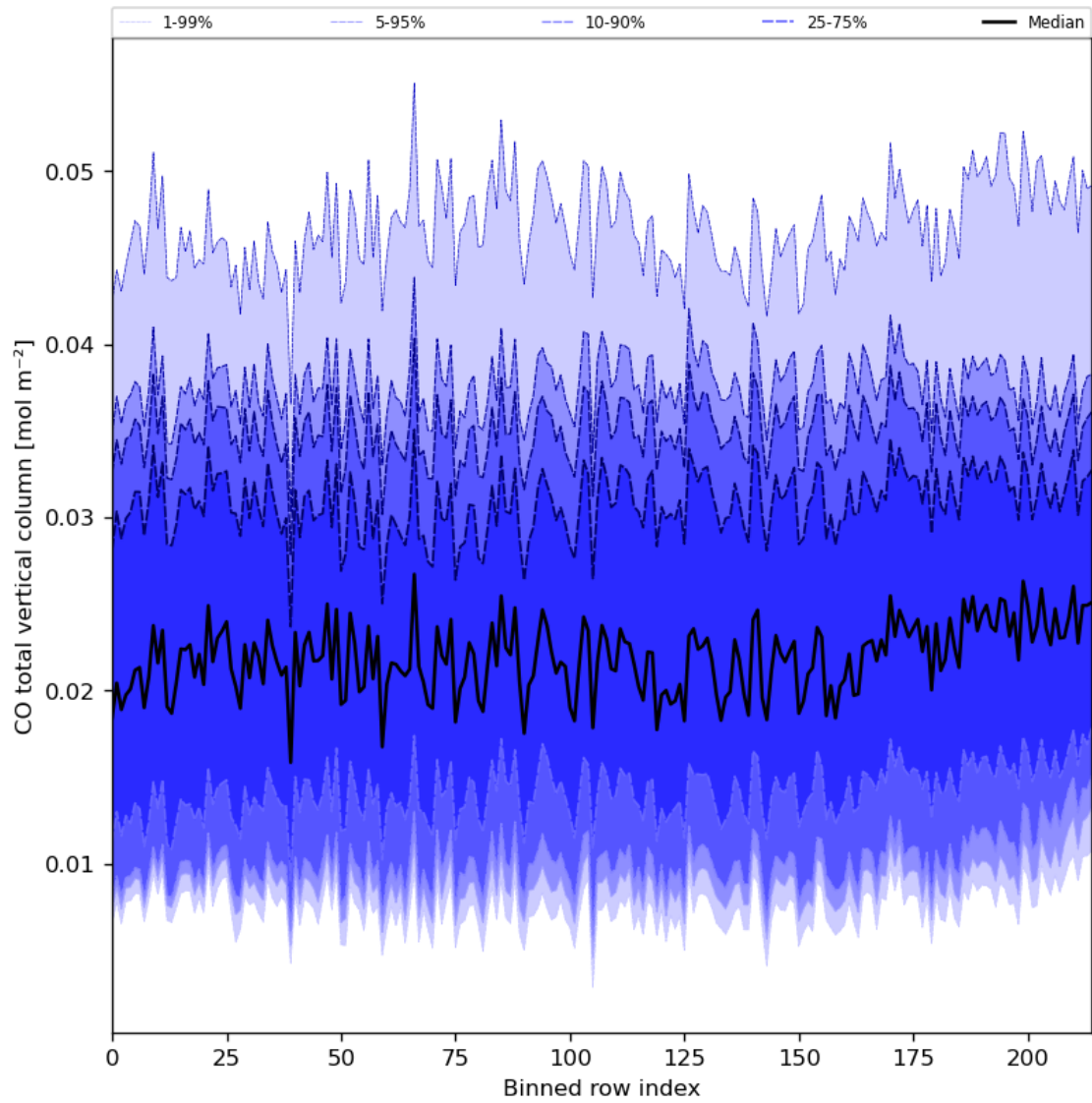
Figure 26: Along track statistics of “CO total vertical column” for 2023-12-18 to 2023-12-20
