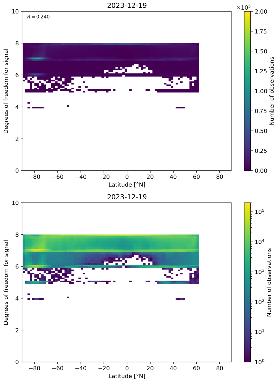
Figure 55: Scatter density plot of “Latitude” against “Degrees of freedom for signal” for 2023-12-18 to 2023-12-20.
