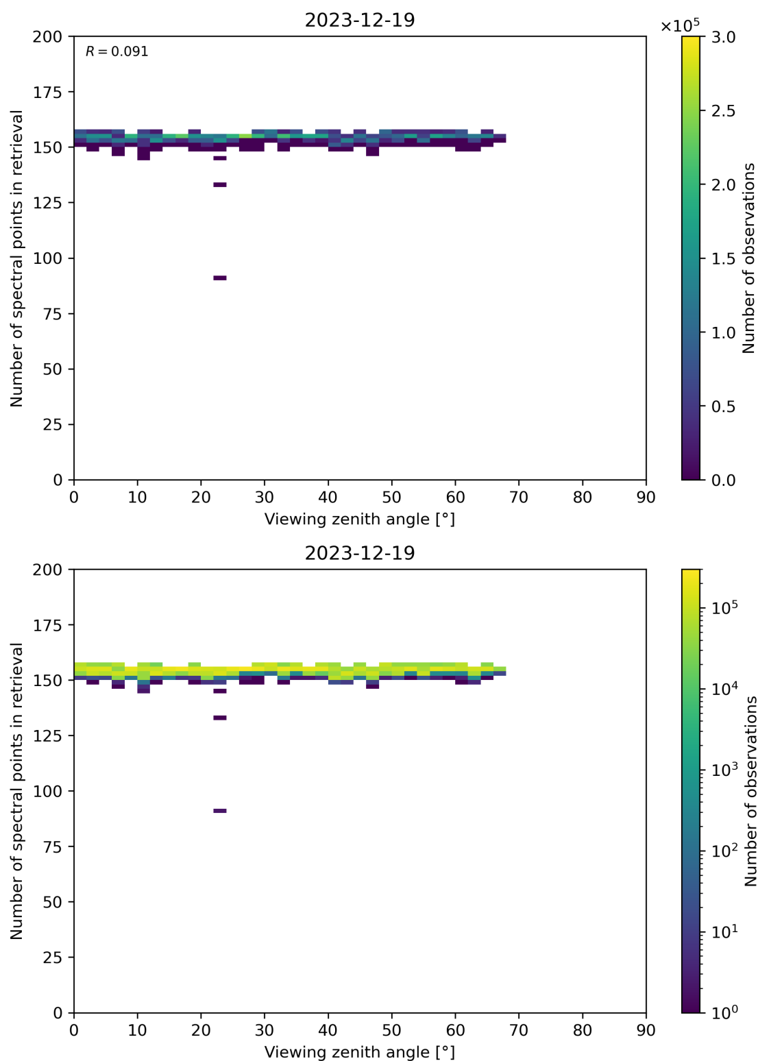
Figure 76: Scatter density plot of “Viewing zenith angle” against “Number of spectral points in retrieval” for 2023-12-18 to 2023-12-20.
