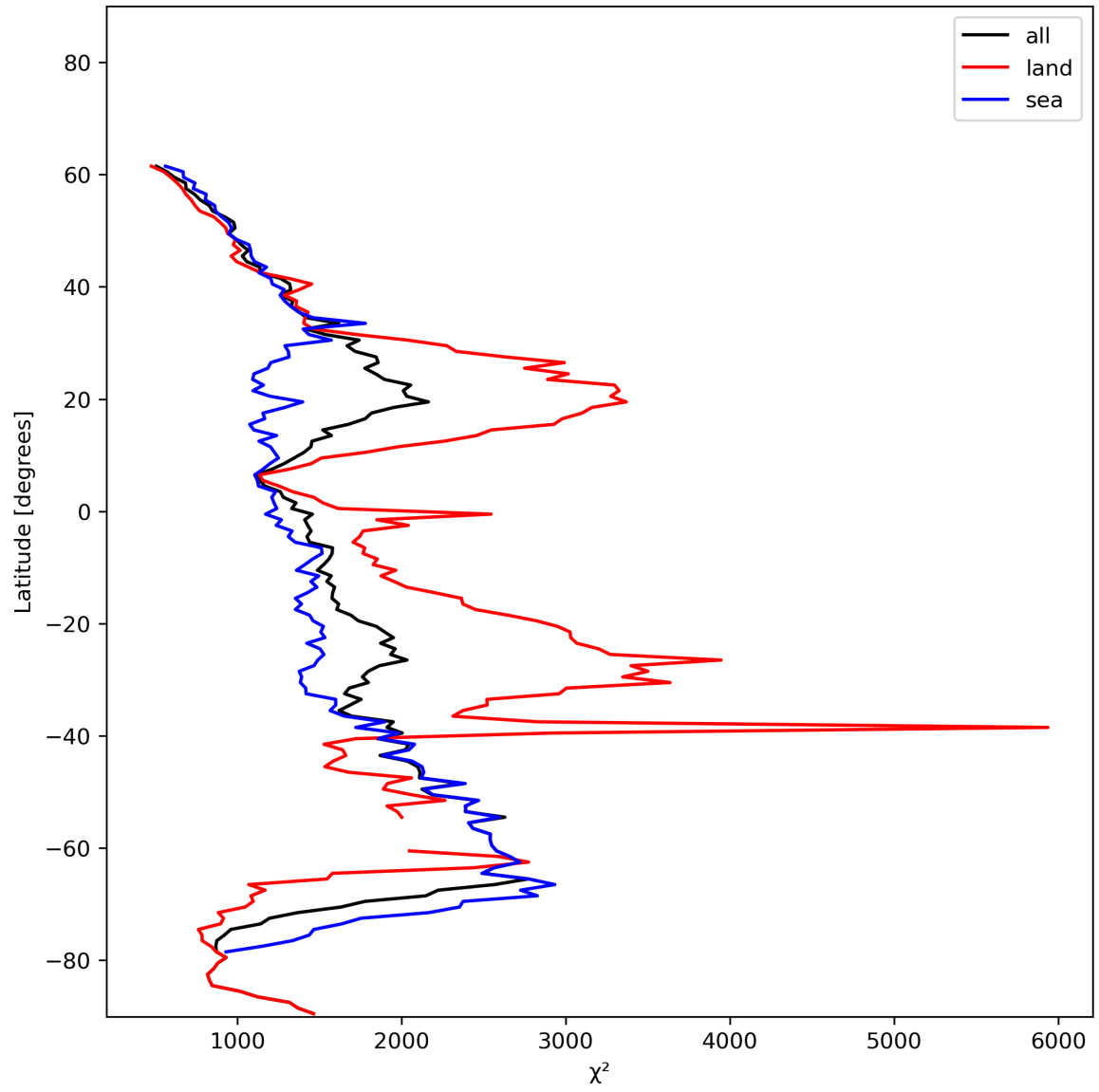
Figure 14: Zonal average of “ \chi^2 ” for 2023-12-18 to 2023-12-20.
