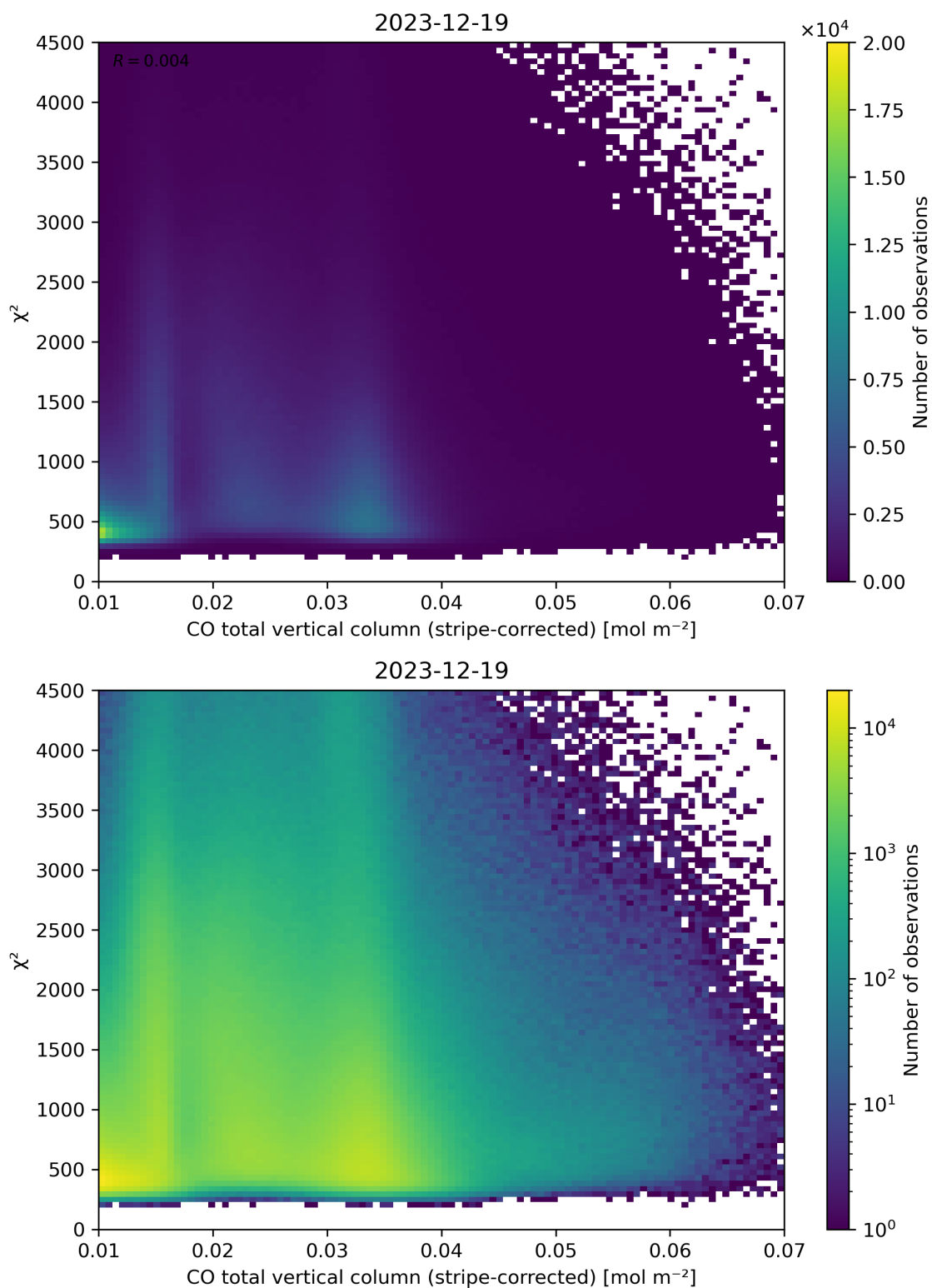
Figure 37: Scatter density plot of “CO total vertical column (stripe-corrected)” against “ \chi^2 ” for 2023-12-18 to 2023-12-20.
