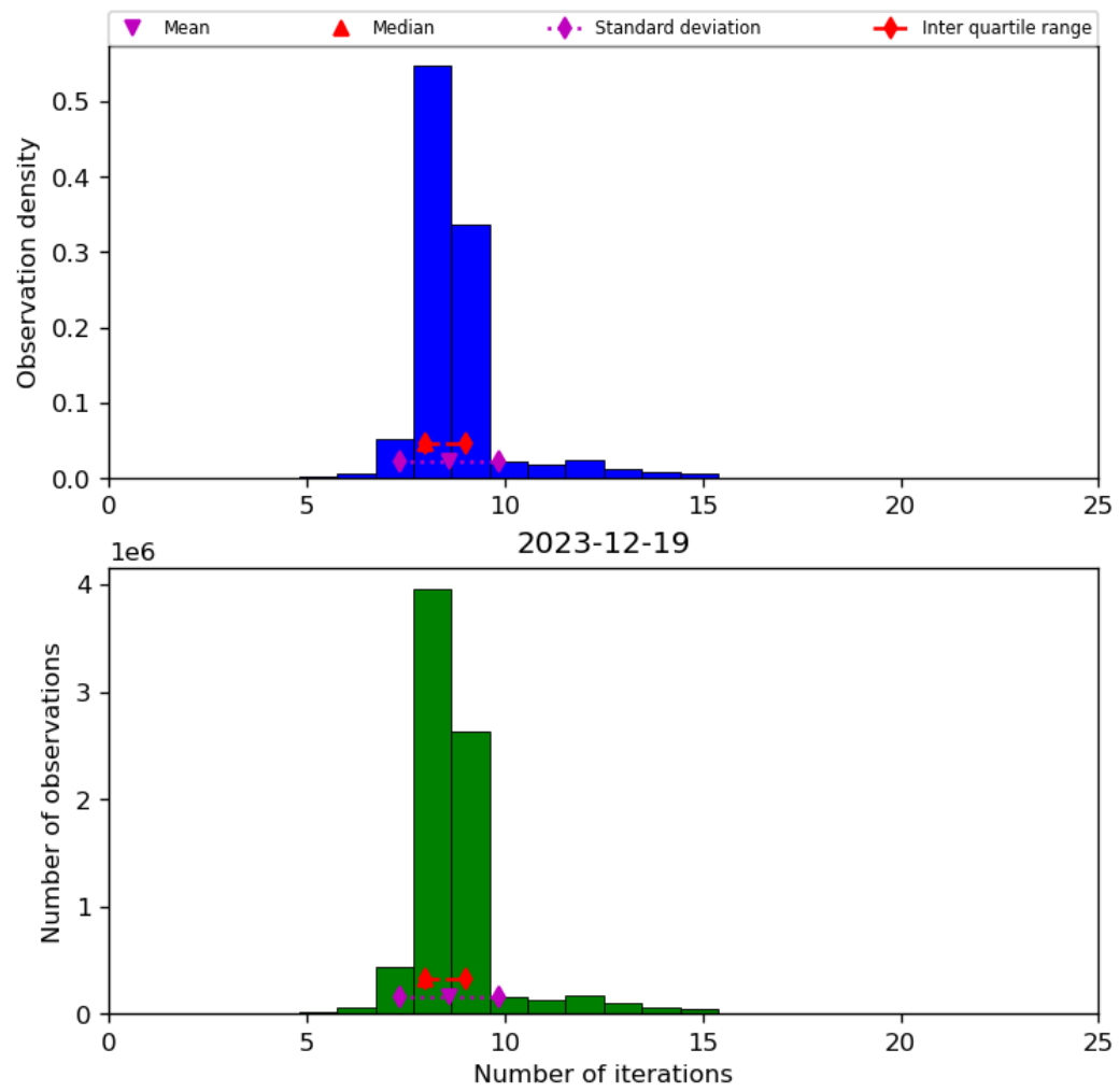
Figure 24: Histogram of “Number of iterations” for 2023-12-18 to 2023-12-20
