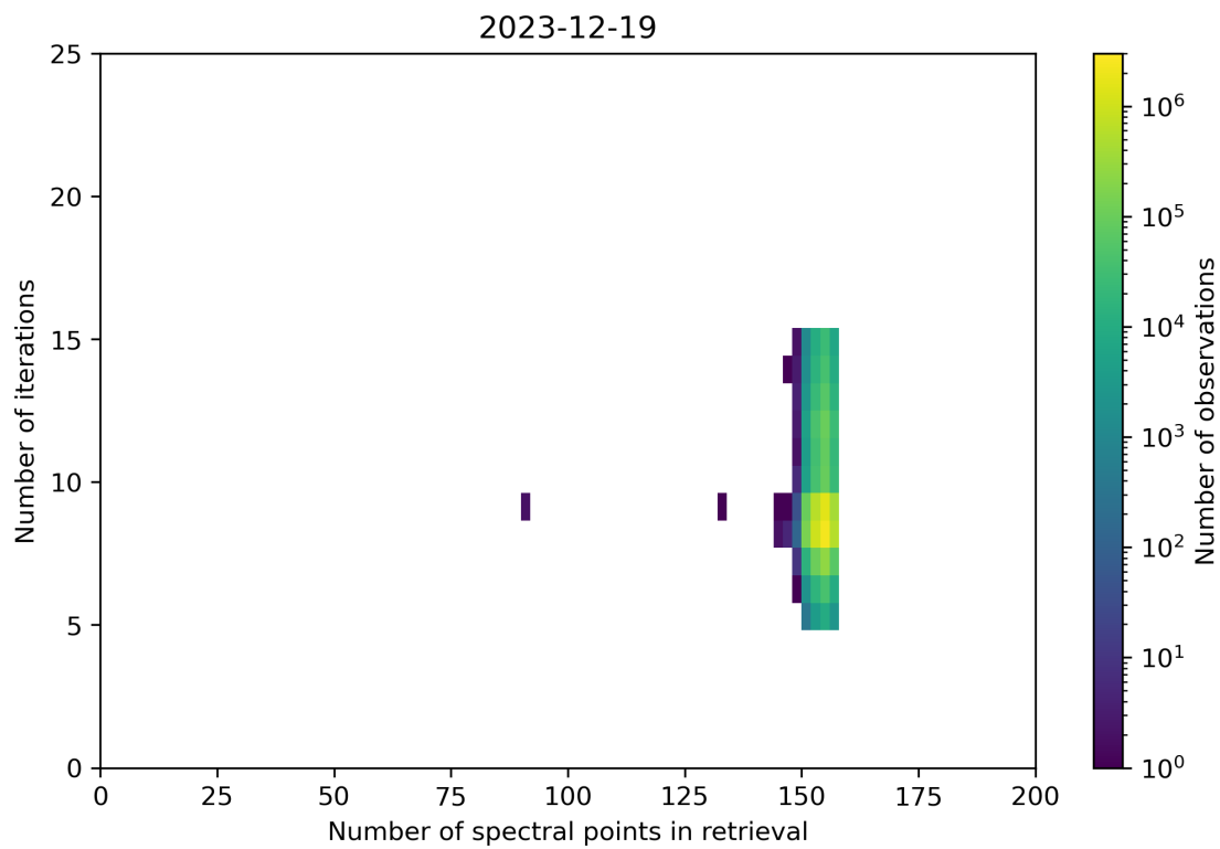
Figure 60: Scatter density plot of “Number of spectral points in retrieval” against “Number of iterations” for 2023-12-18 to 2023-12-20.
