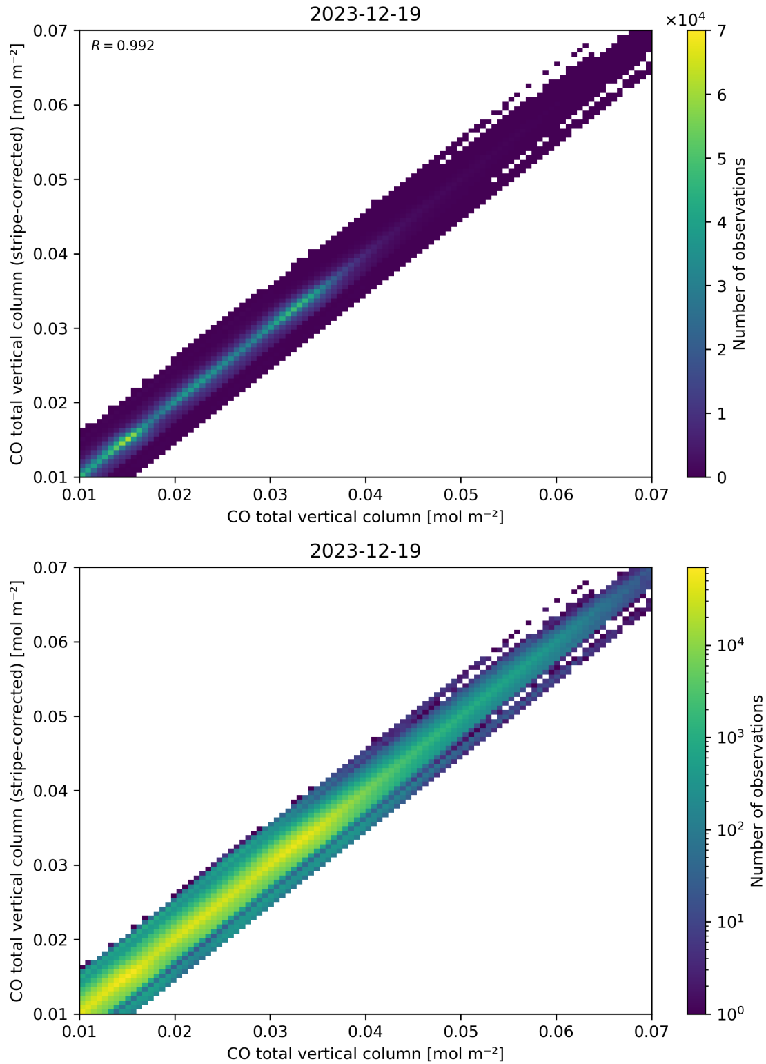
Figure 33: Scatter density plot of “CO total vertical column” against “CO total vertical column (stripe-corrected)” for 2023-12-18 to 2023-12-20.
