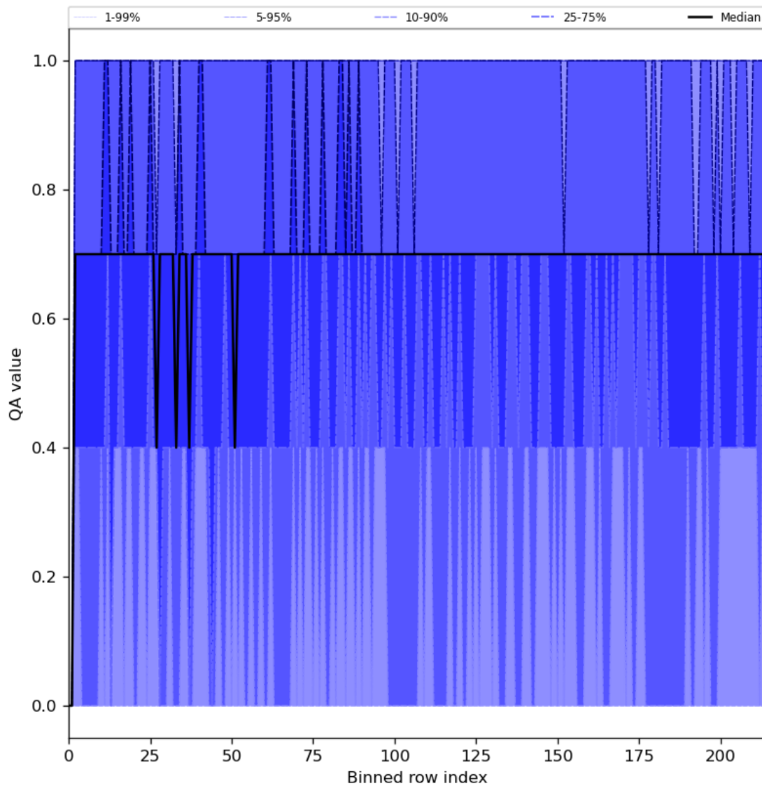
Figure 25: Along track statistics of “QA value” for 2023-12-18 to 2023-12-20
