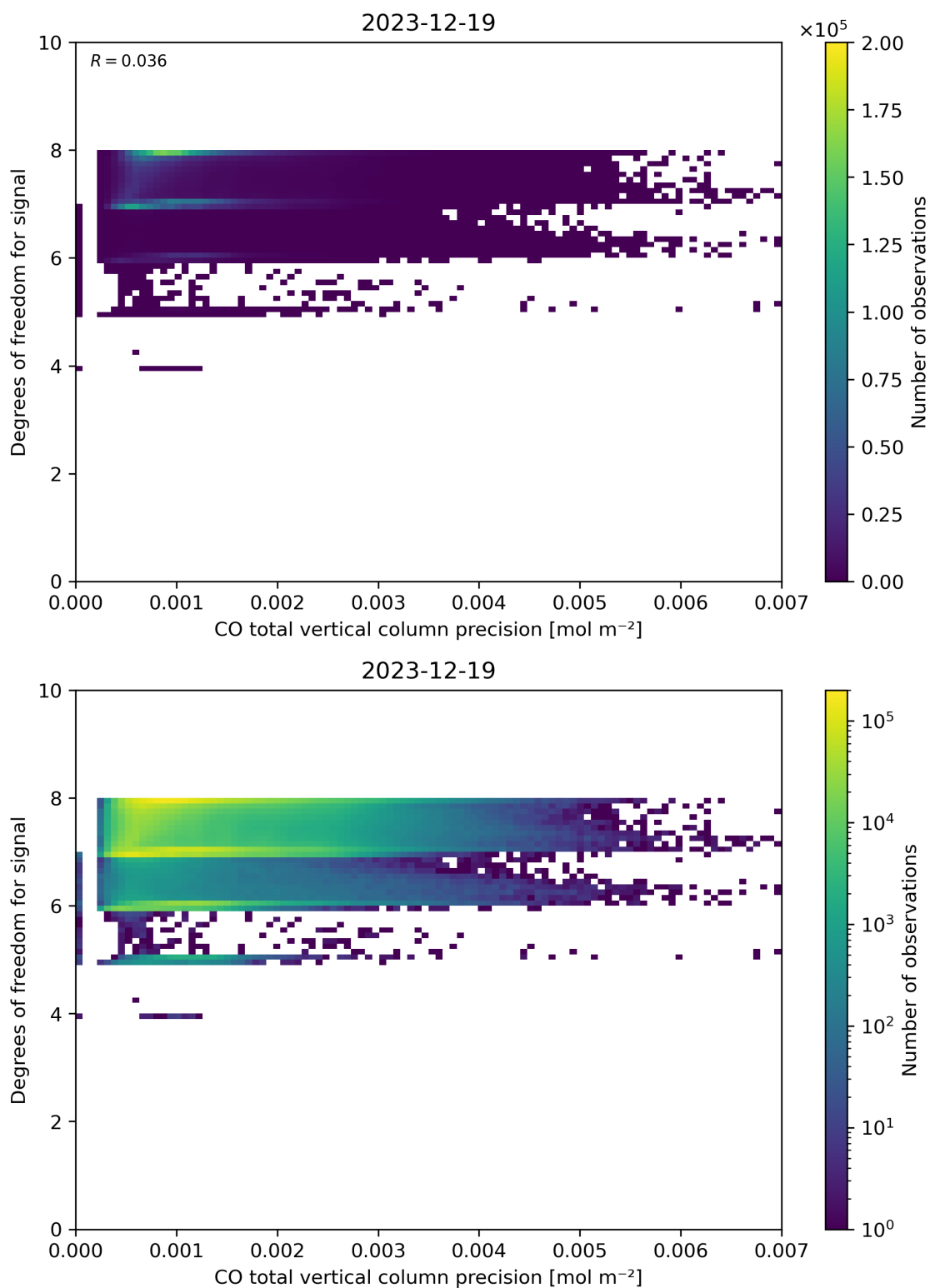
Figure 45: Scatter density plot of “CO total vertical column precision” against “Degrees of freedom for signal” for 2023-12-18 to 2023-12-20.
