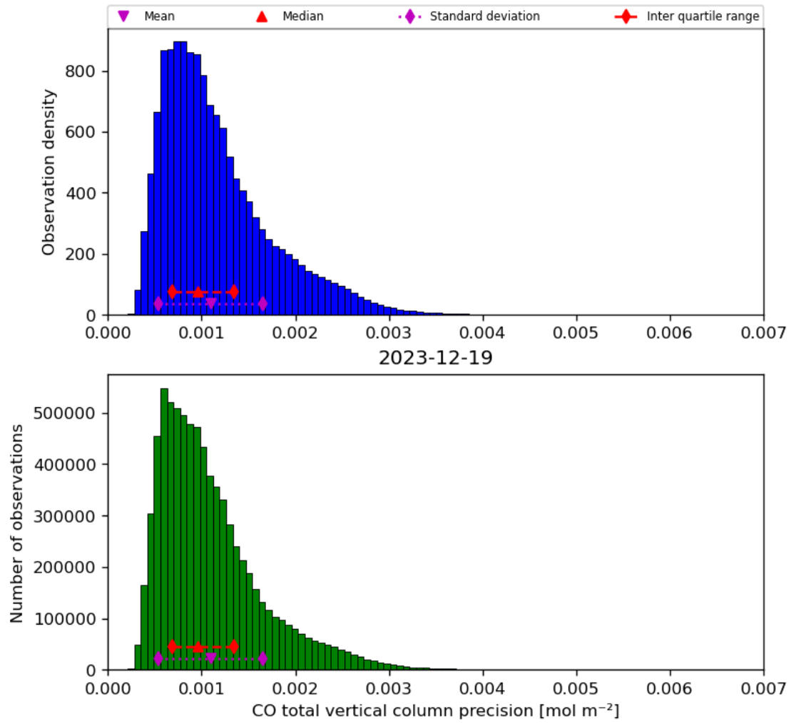
Figure 20: Histogram of “CO total vertical column precision” for 2023-12-18 to 2023-12-20
