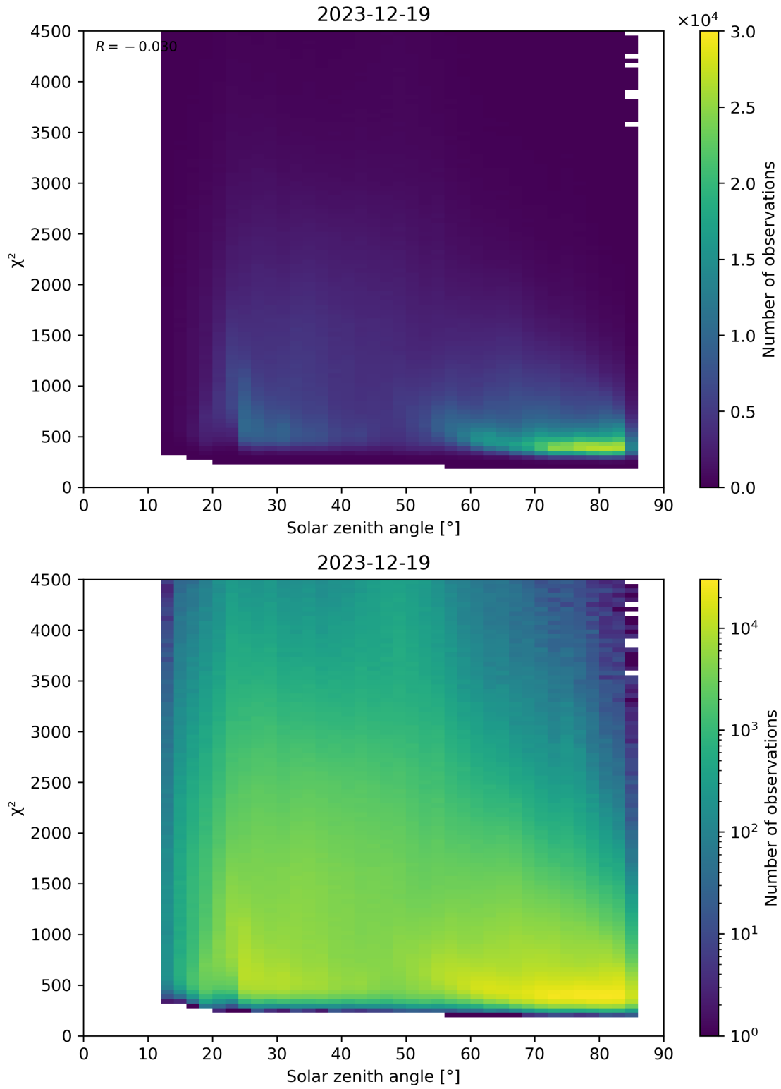
Figure 64: Scatter density plot of “Solar zenith angle” against “ \chi^2 ” for 2023-12-18 to 2023-12-20.
