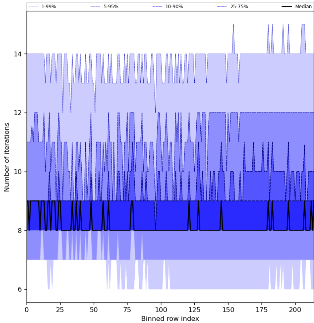
Figure 32: Along track statistics of “Number of iterations” for 2023-12-18 to 2023-12-20
