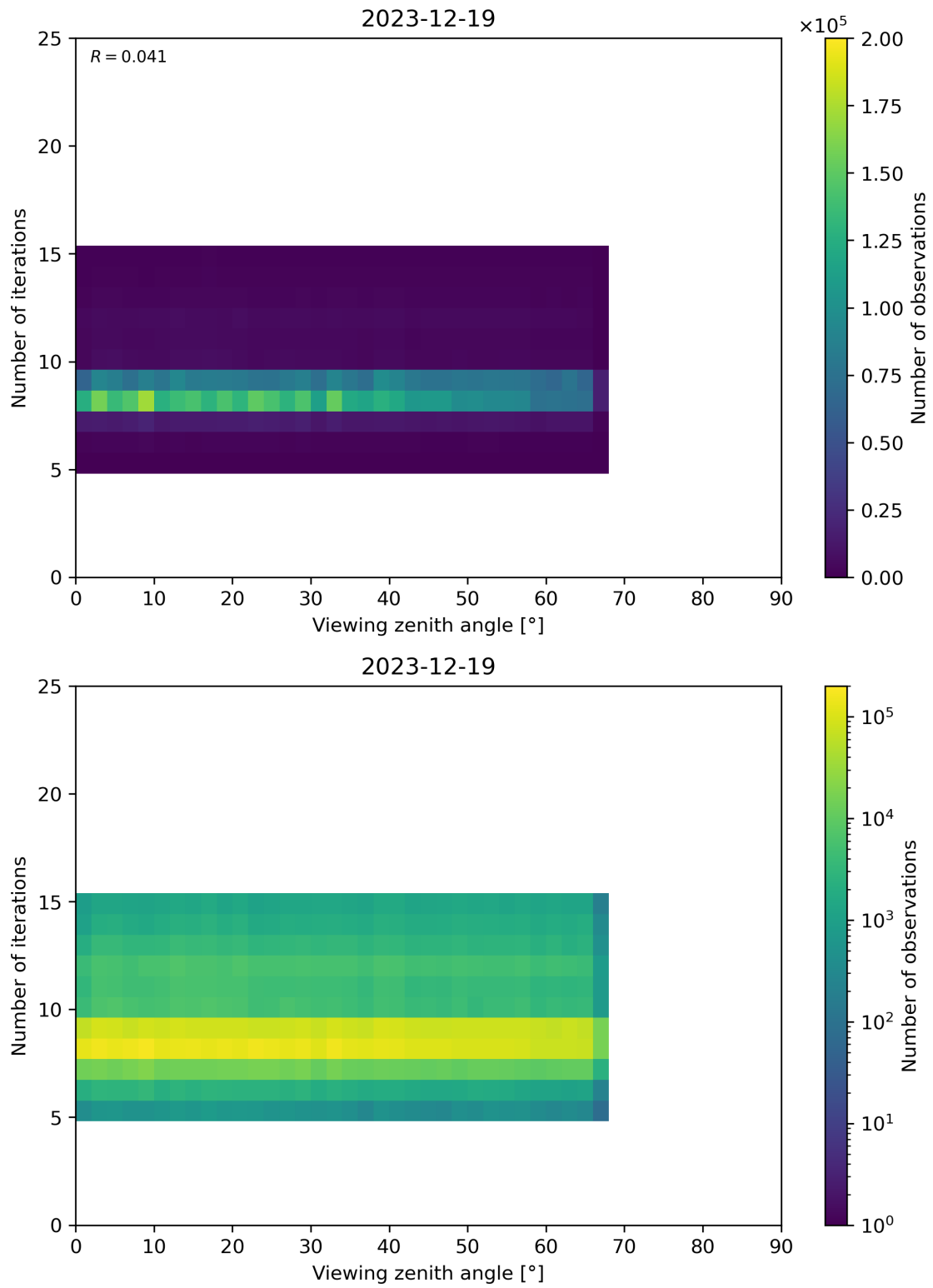
Figure 75: Scatter density plot of “Viewing zenith angle” against “Number of iterations” for 2023-12-18 to 2023-12-20.
