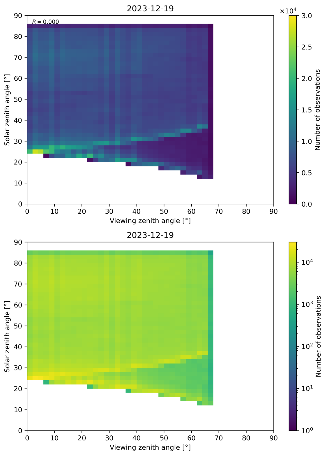
Figure 77: Scatter density plot of “Viewing zenith angle” against “Solar zenith angle” for 2023-12-18 to 2023-12-20.
