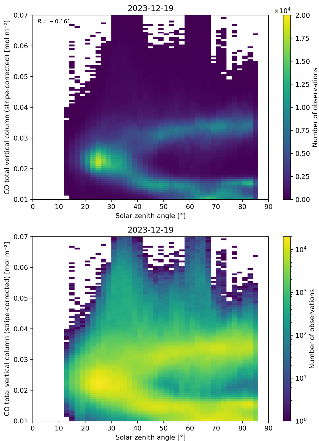
Figure 62: Scatter density plot of “Solar zenith angle” against “CO total vertical column (stripe-corrected)” for 2023-12-18 to 2023-12-20.
