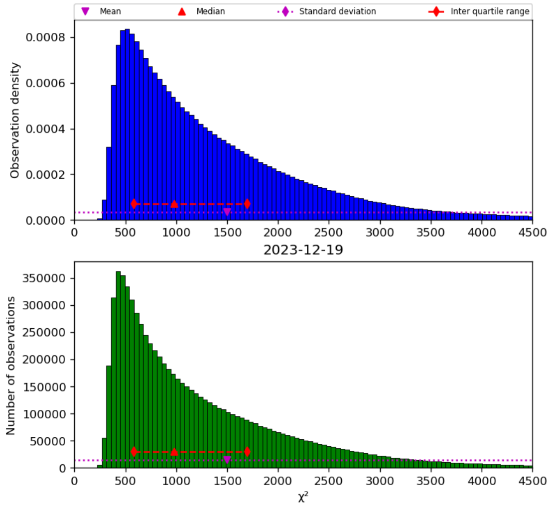
Figure 22: Histogram of “ \chi^2 ” for 2023-12-18 to 2023-12-20
