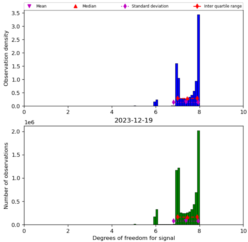
Figure 23: Histogram of “Degrees of freedom for signal” for 2023-12-18 to 2023-12-20
