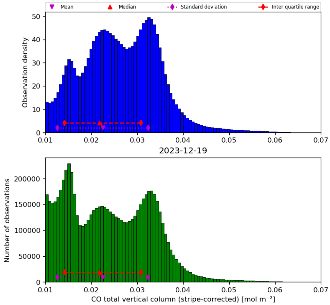
Figure 19: Histogram of “CO total vertical column (stripe-corrected)” for 2023-12-18 to 2023-12-20
