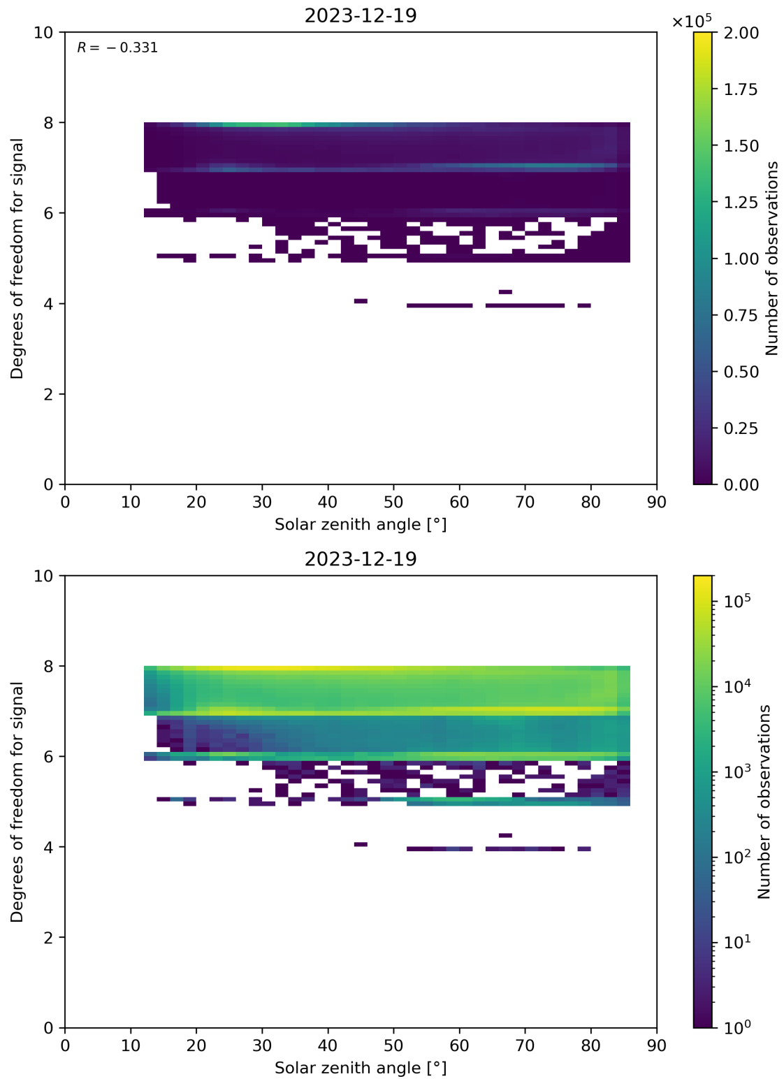
Figure 65: Scatter density plot of “Solar zenith angle” against “Degrees of freedom for signal” for 2023-12-18 to 2023-12-20.
