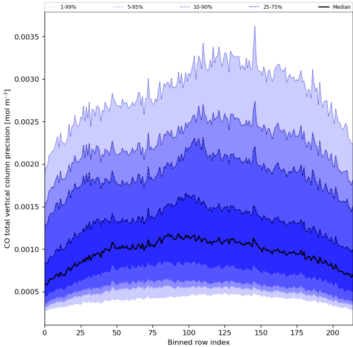
Figure 28: Along track statistics of “CO total vertical column precision” for 2023-12-18 to 2023-12-20
