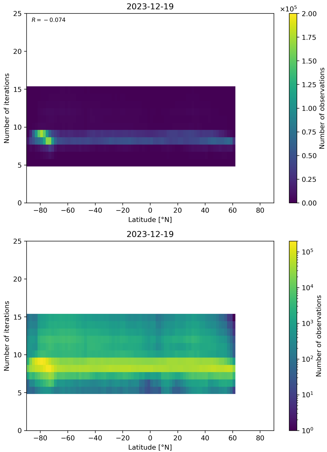
Figure 56: Scatter density plot of “Latitude” against “Number of iterations” for 2023-12-18 to 2023-12-20.
