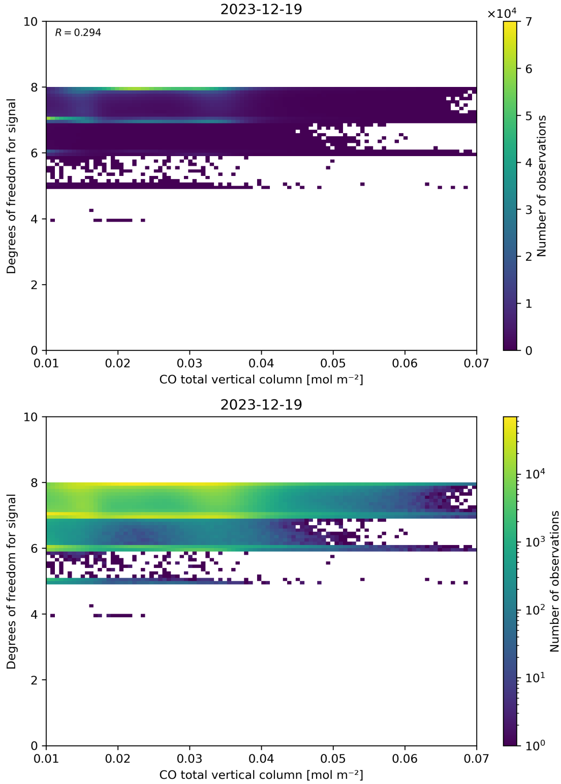
Figure 41: Scatter density plot of “CO total vertical column” against “Degrees of freedom for signal” for 2023-12-18 to 2023-12-20.
