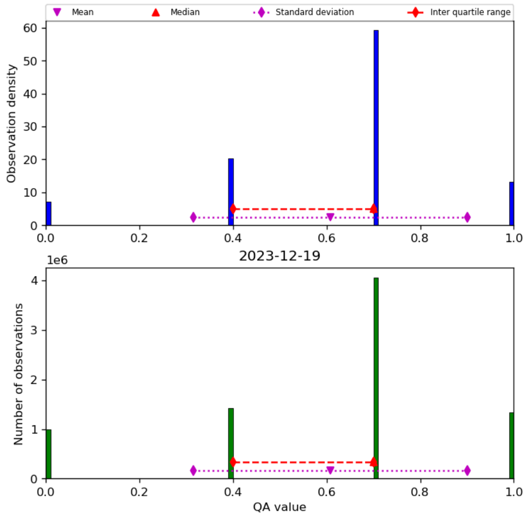
Figure 17: Histogram of “QA value” for 2023-12-18 to 2023-12-20
