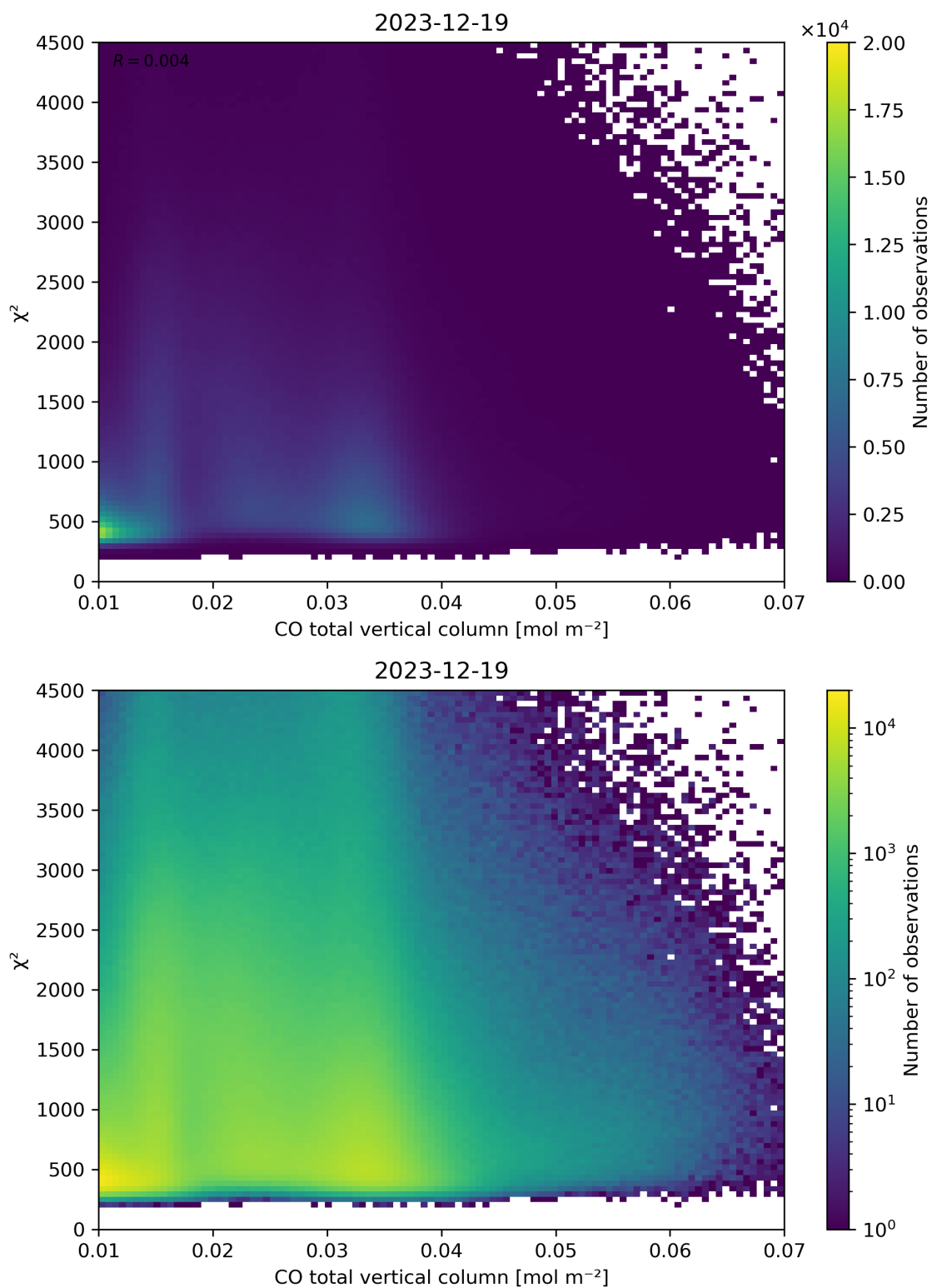
Figure 35: Scatter density plot of “CO total vertical column” against “ \chi^2 ” for 2023-12-18 to 2023-12-20.
