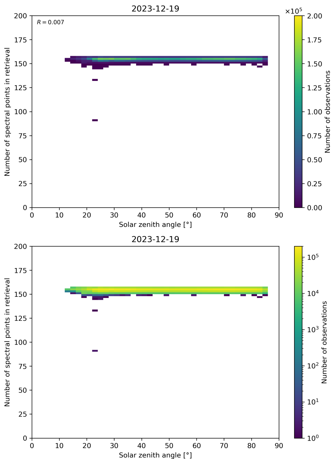
Figure 68: Scatter density plot of “Solar zenith angle” against “Number of spectral points in retrieval” for 2023-12-18 to 2023-12-20.
