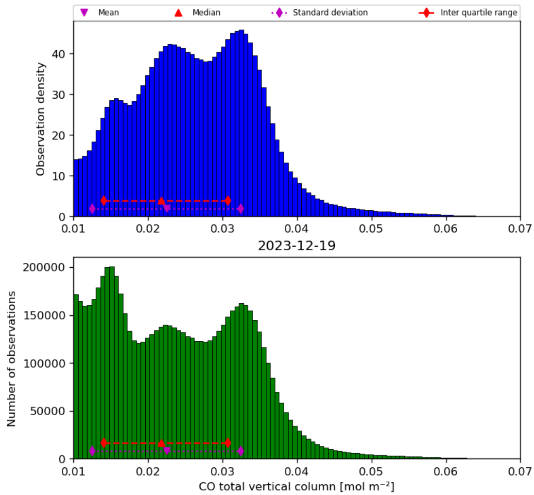
Figure 18: Histogram of “CO total vertical column” for 2023-12-18 to 2023-12-20
