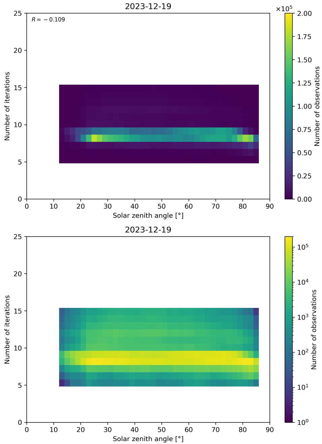
Figure 67: Scatter density plot of “Solar zenith angle” against “Number of iterations” for 2023-12-18 to 2023-12-20.
