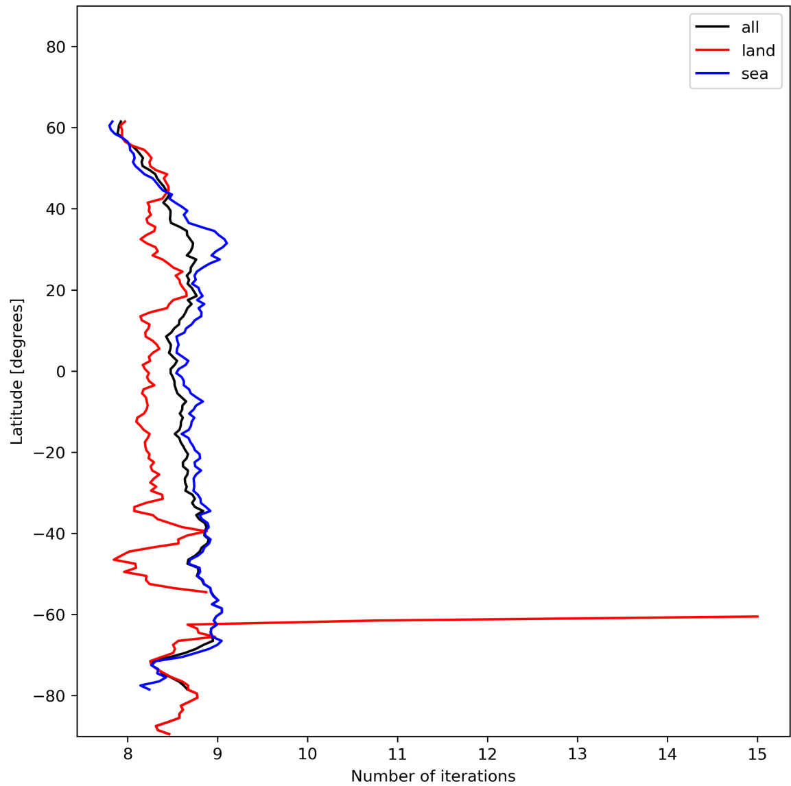
Figure 16: Zonal average of “Number of iterations” for 2023-12-18 to 2023-12-20.
