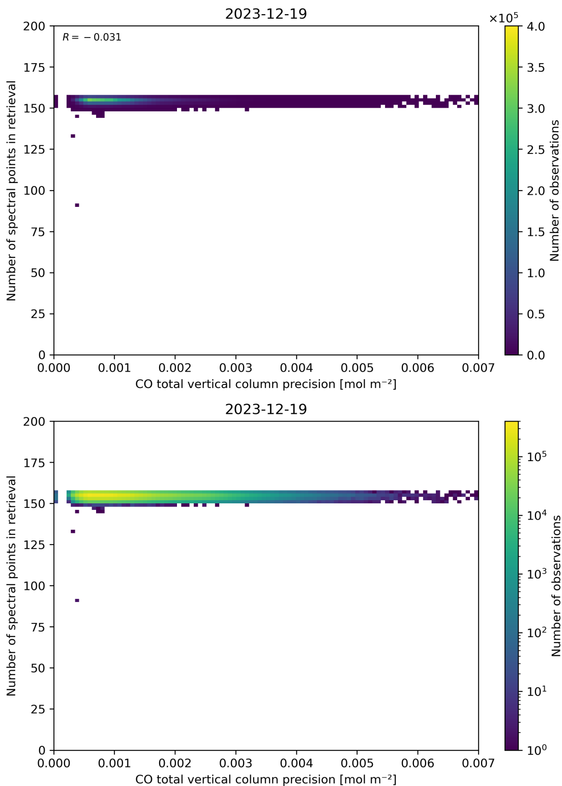
Figure 47: Scatter density plot of “CO total vertical column precision” against “Number of spectral points in retrieval” for 2023-12-18 to 2023-12-20.
