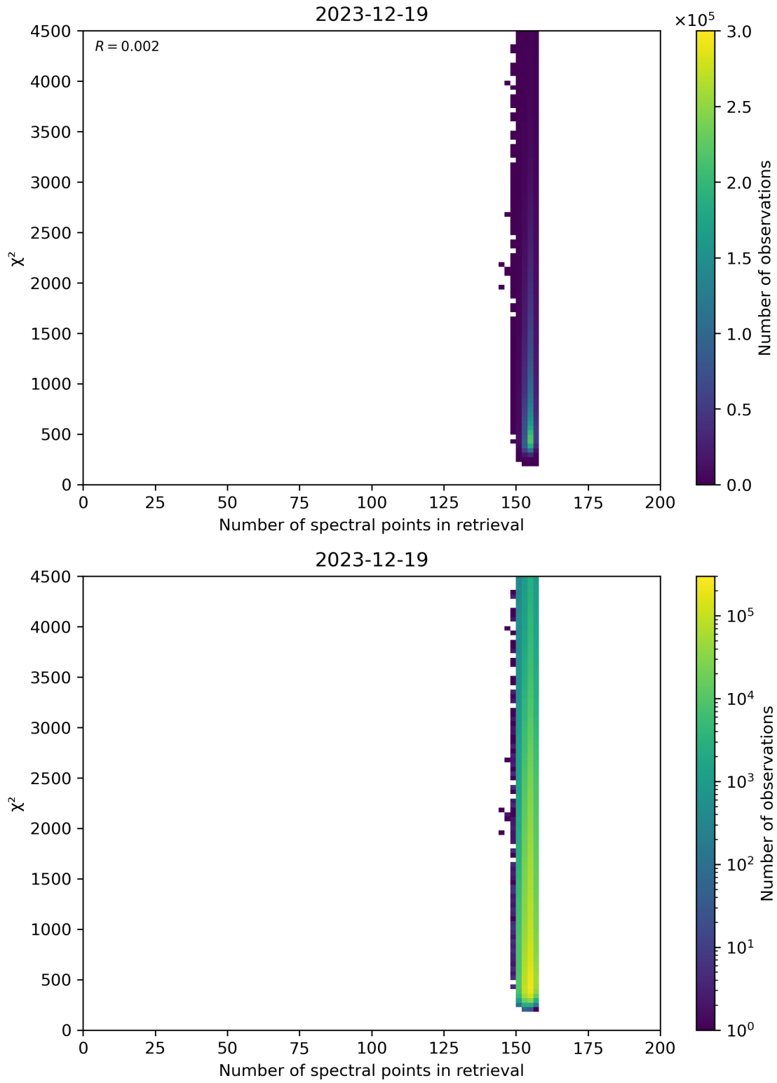
Figure 58: Scatter density plot of “Number of spectral points in retrieval” against “ \chi^2 ” for 2023-12-18 to 2023-12-20.
