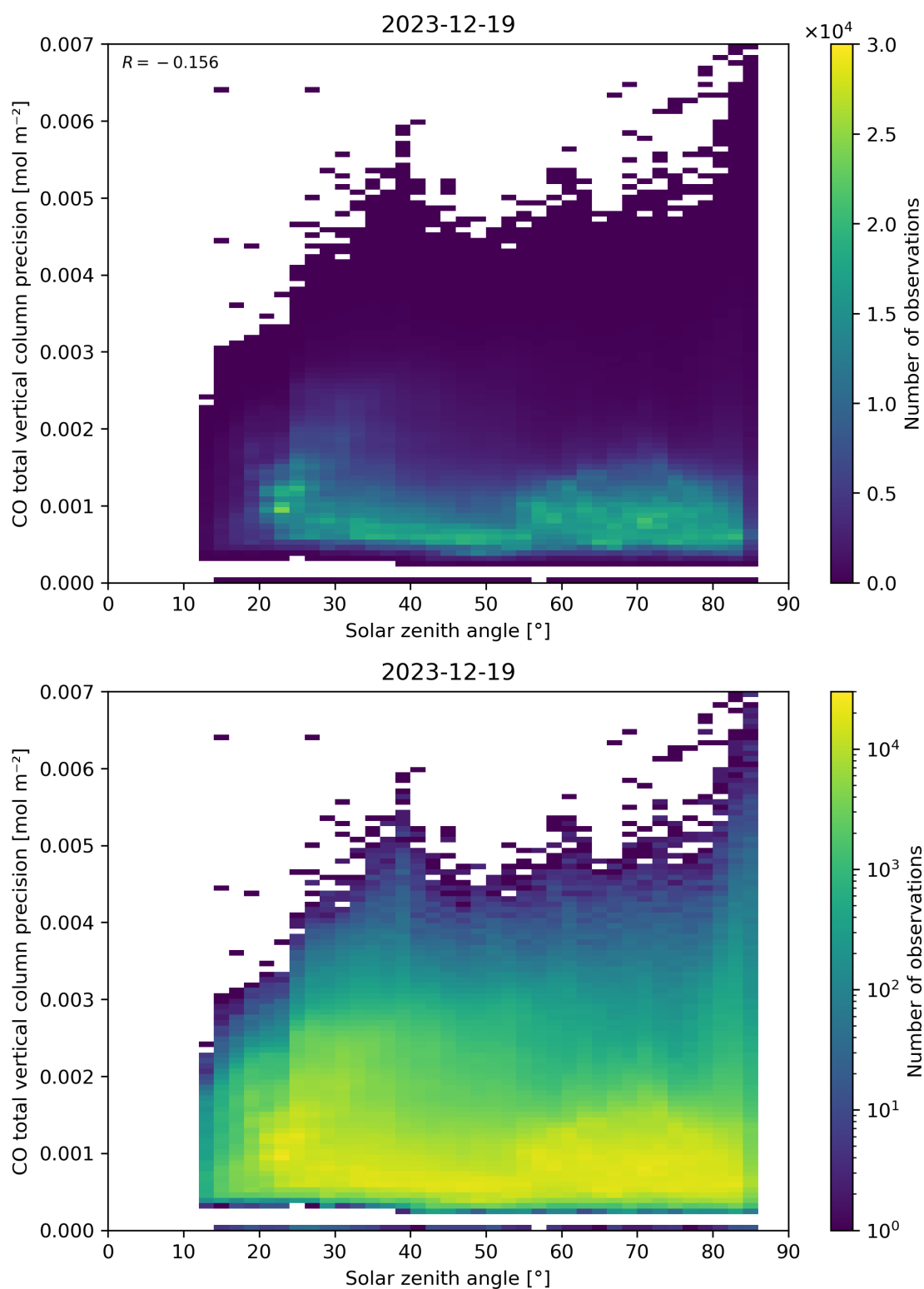
Figure 63: Scatter density plot of “Solar zenith angle” against “CO total vertical column precision” for 2023-12-18 to 2023-12-20.
