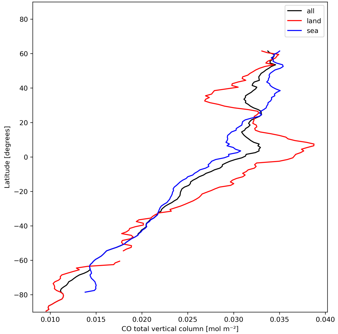
Figure 10: Zonal average of “CO total vertical column” for 2023-12-18 to 2023-12-20.
