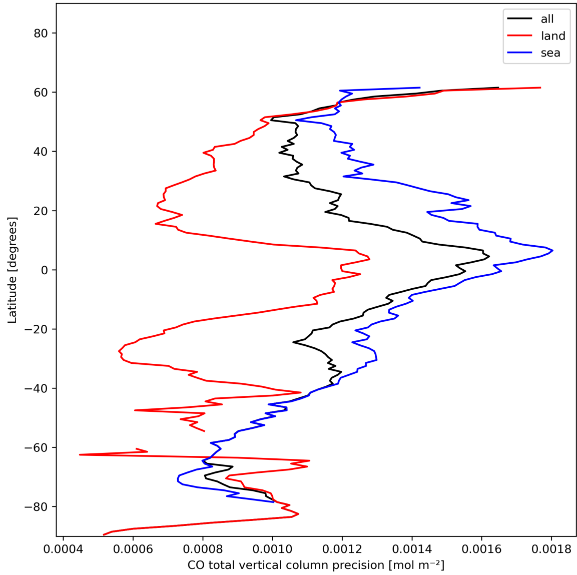
Figure 12: Zonal average of “CO total vertical column precision” for 2023-12-18 to 2023-12-20.
