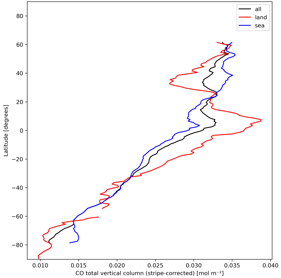
Figure 11: Zonal average of “CO total vertical column (stripe-corrected)” for 2023-12-18 to 2023-12-20.
