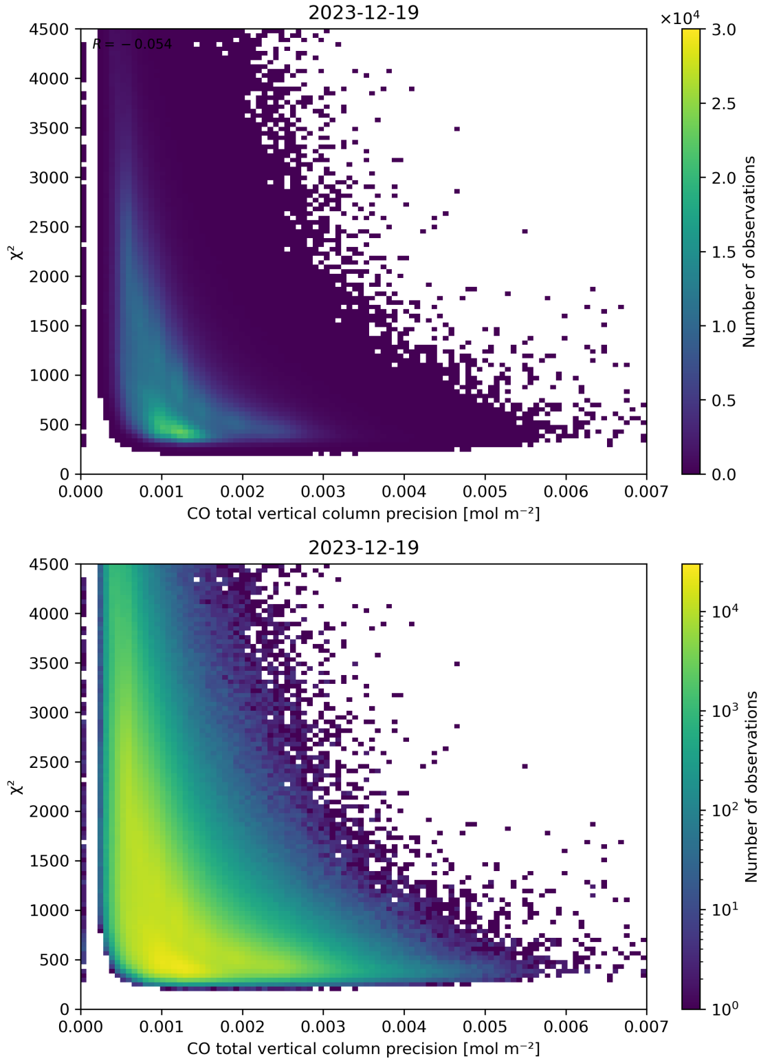
Figure 44: Scatter density plot of “CO total vertical column precision” against “ \chi^2 ” for 2023-12-18 to 2023-12-20.
