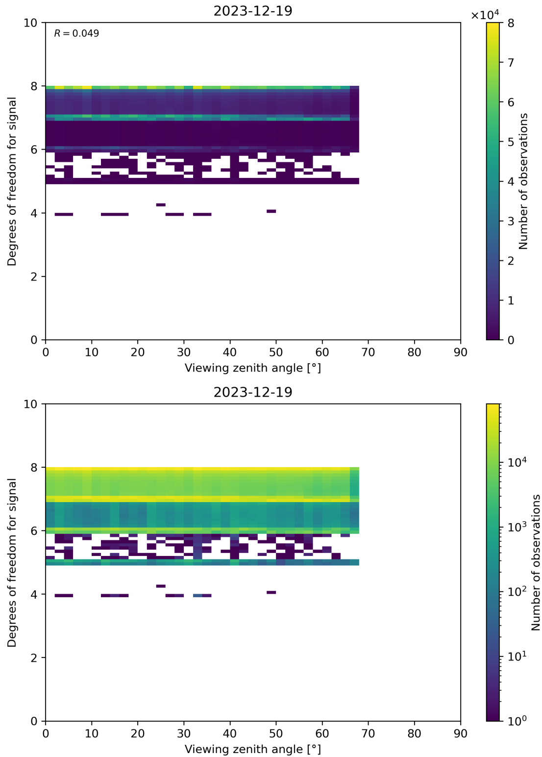
Figure 73: Scatter density plot of “Viewing zenith angle” against “Degrees of freedom for signal” for 2023-12-18 to 2023-12-20.
