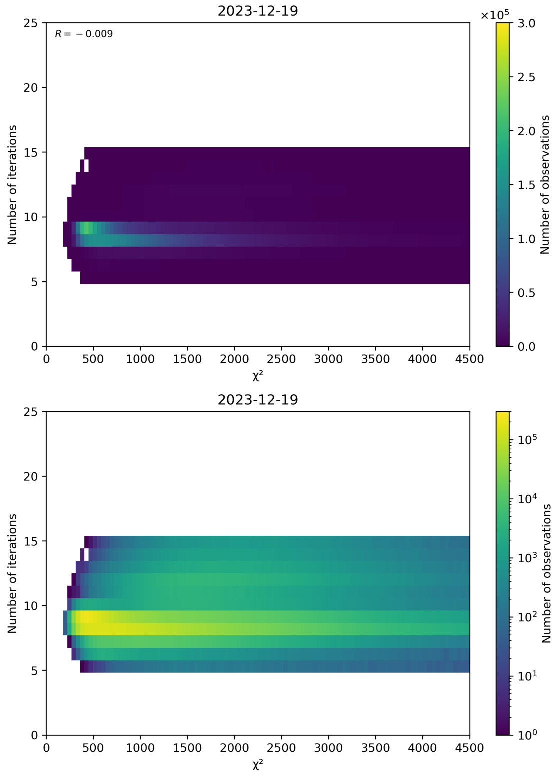
Figure 49: Scatter density plot of “ \chi^2 ” against “Number of iterations” for 2023-12-18 to 2023-12-20.
