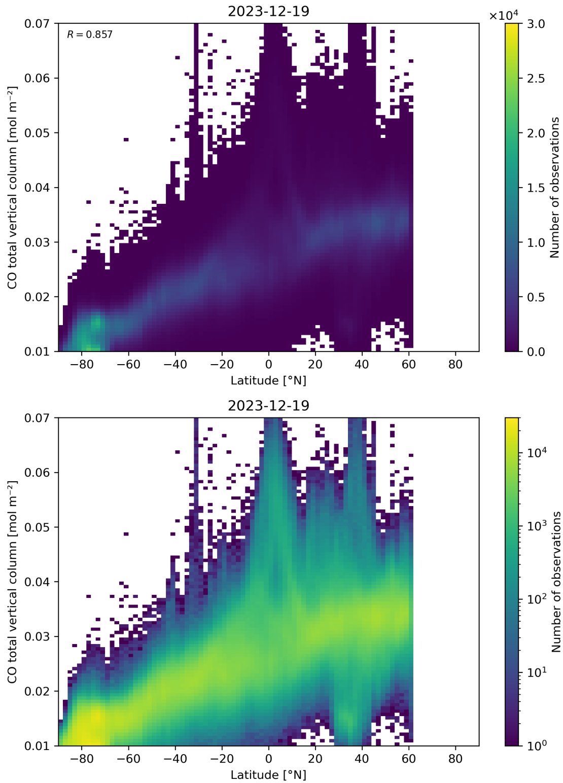
Figure 51: Scatter density plot of “Latitude” against “CO total vertical column” for 2023-12-18 to 2023-12-20.
