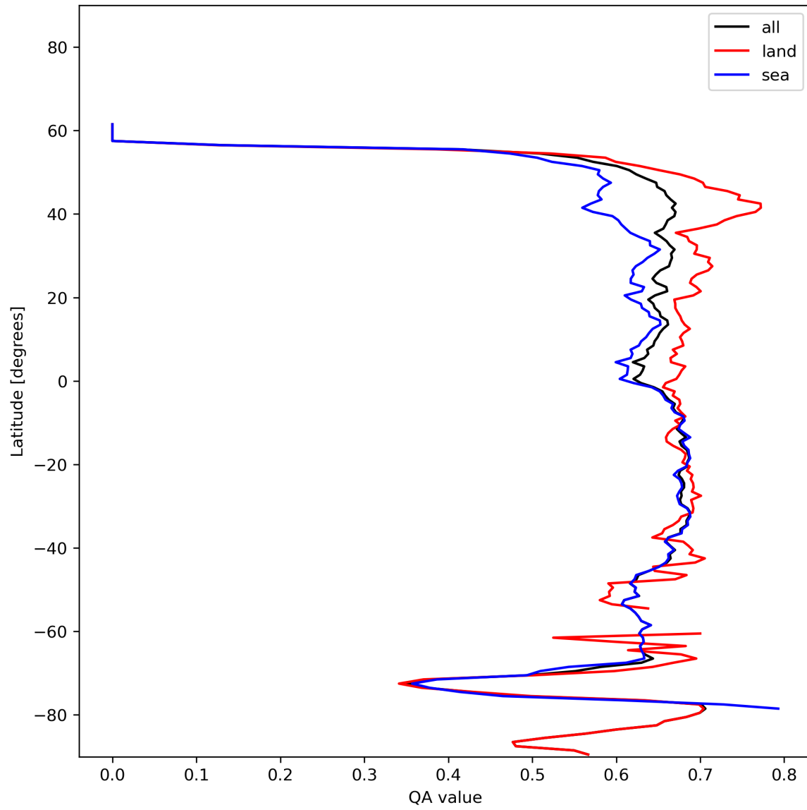
Figure 9: Zonal average of “QA value” for 2023-12-18 to 2023-12-20.
