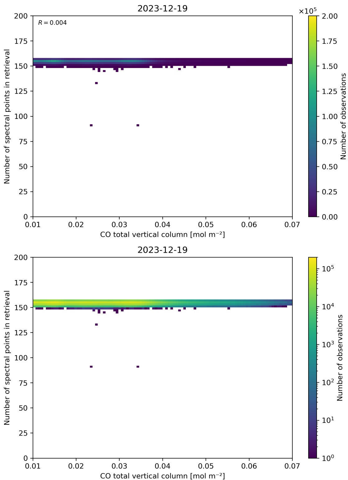
Figure 43: Scatter density plot of “CO total vertical column” against “Number of spectral points in retrieval” for 2023-12-18 to 2023-12-20.
