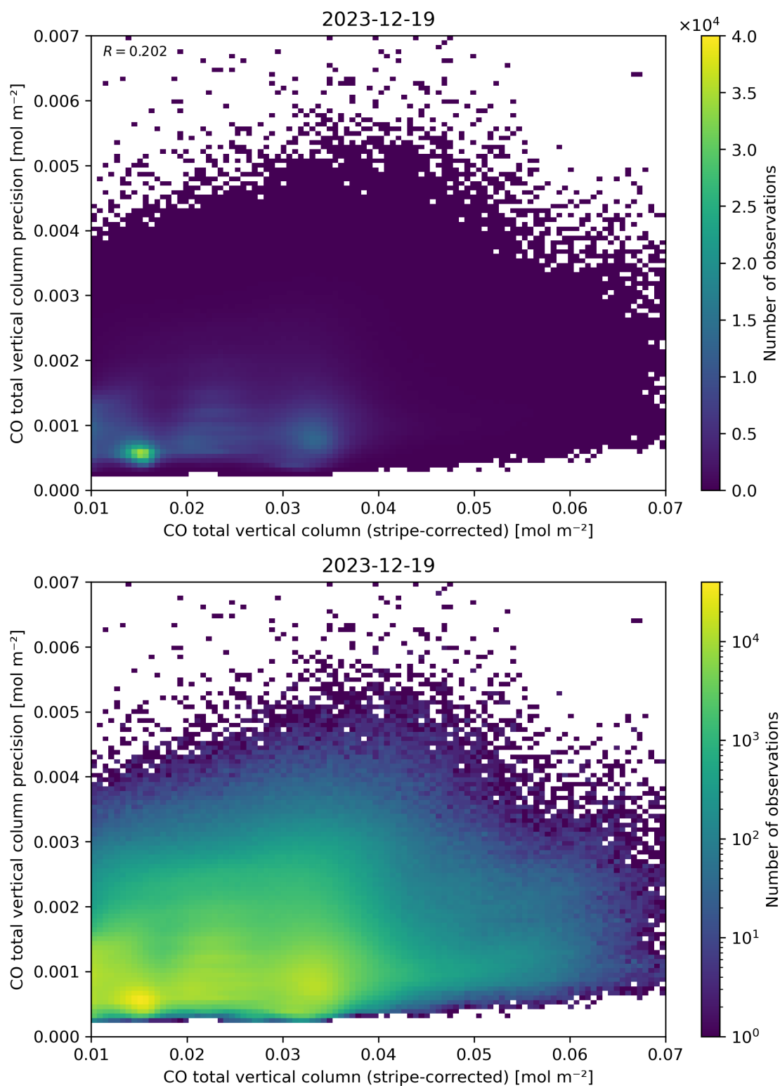
Figure 36: Scatter density plot of “CO total vertical column (stripe-corrected)” against “CO total vertical column precision” for 2023-12-18 to 2023-12-20.
