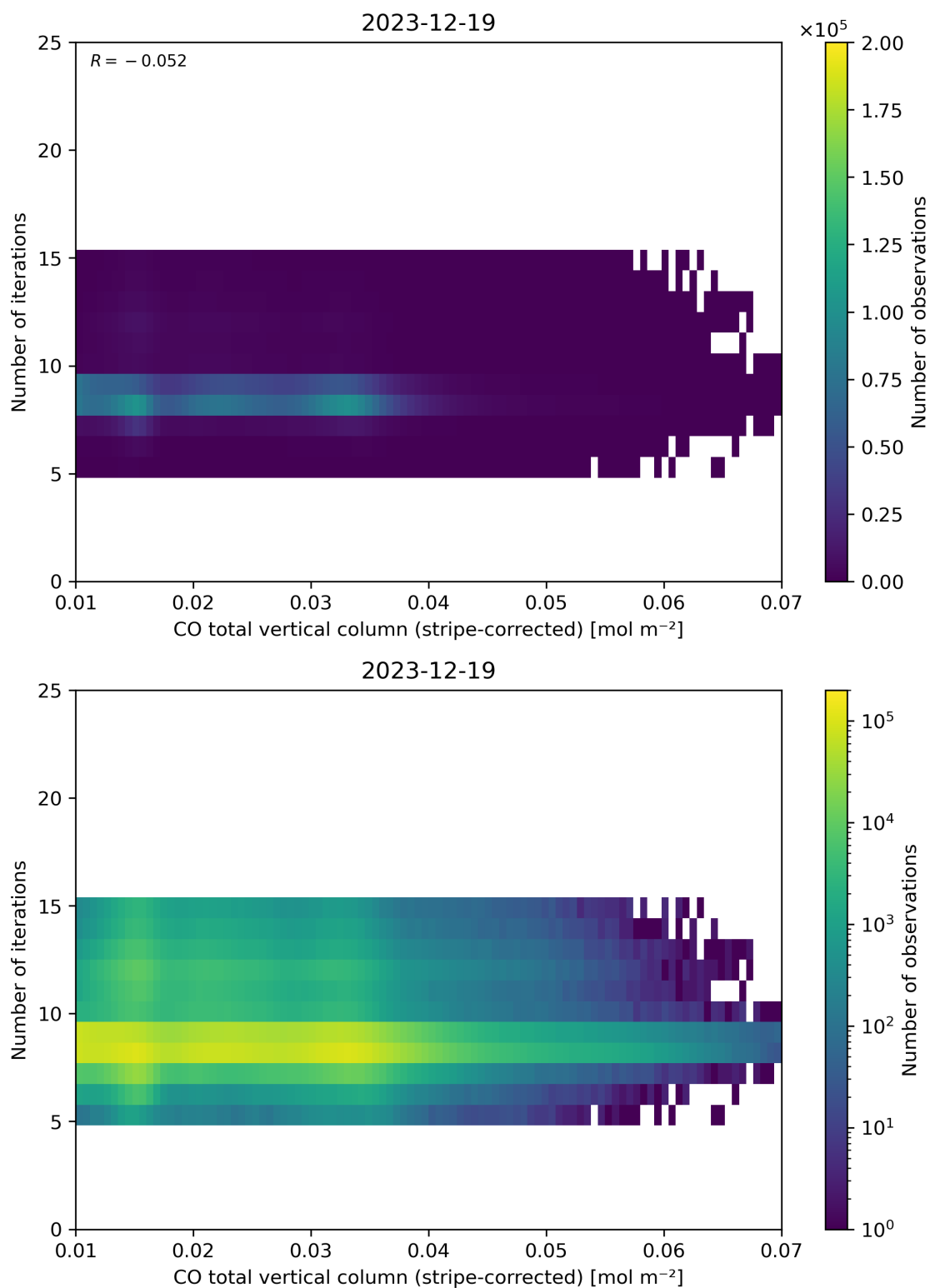
Figure 39: Scatter density plot of “CO total vertical column (stripe-corrected)” against “Number of iterations” for 2023-12-18 to 2023-12-20.
