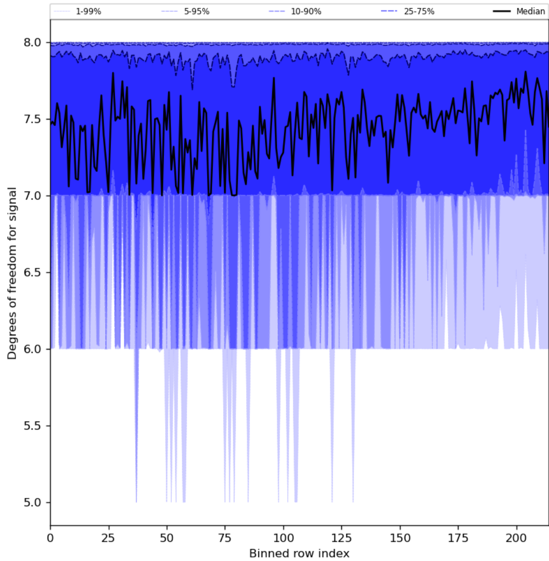
Figure 31: Along track statistics of “Degrees of freedom for signal” for 2023-12-18 to 2023-12-20
