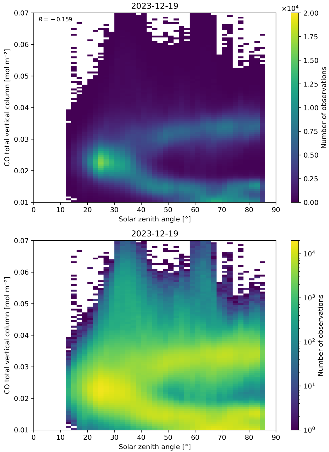
Figure 61: Scatter density plot of “Solar zenith angle” against “CO total vertical column” for 2023-12-18 to 2023-12-20.
