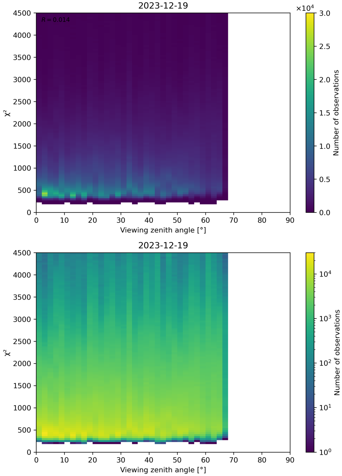
Figure 72: Scatter density plot of “Viewing zenith angle” against “ \chi^2 ” for 2023-12-18 to 2023-12-20.
