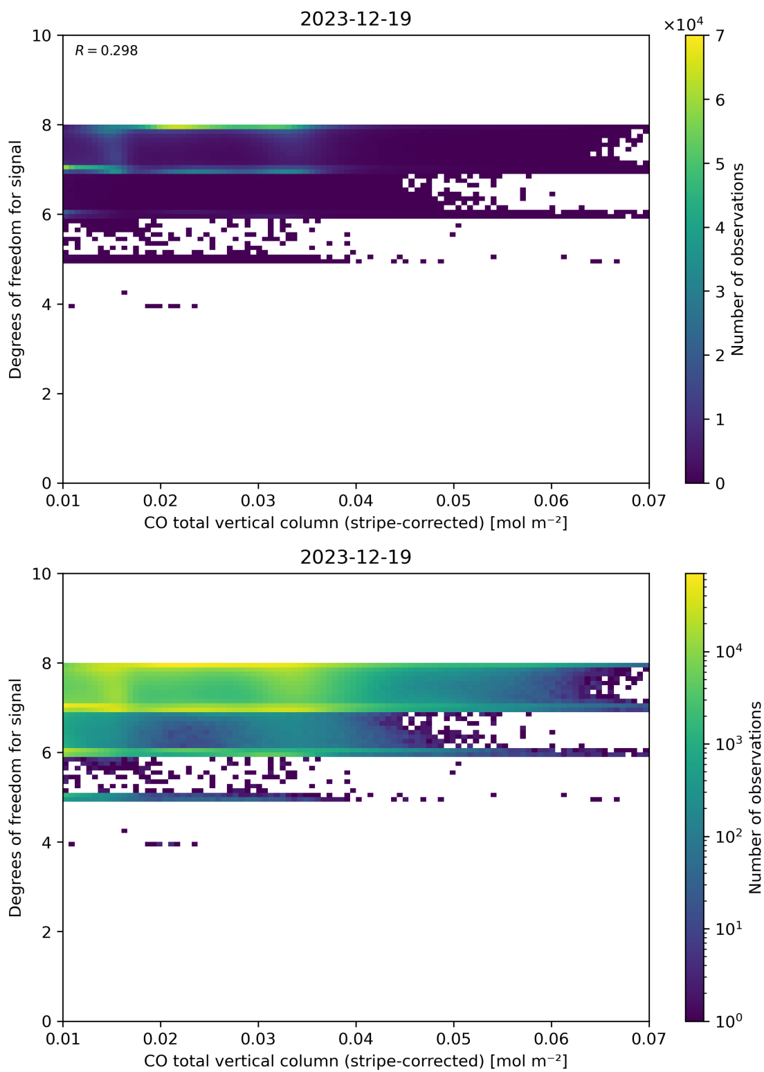
Figure 38: Scatter density plot of “CO total vertical column (stripe-corrected)” against “Degrees of freedom for signal” for 2023-12-18 to 2023-12-20.
