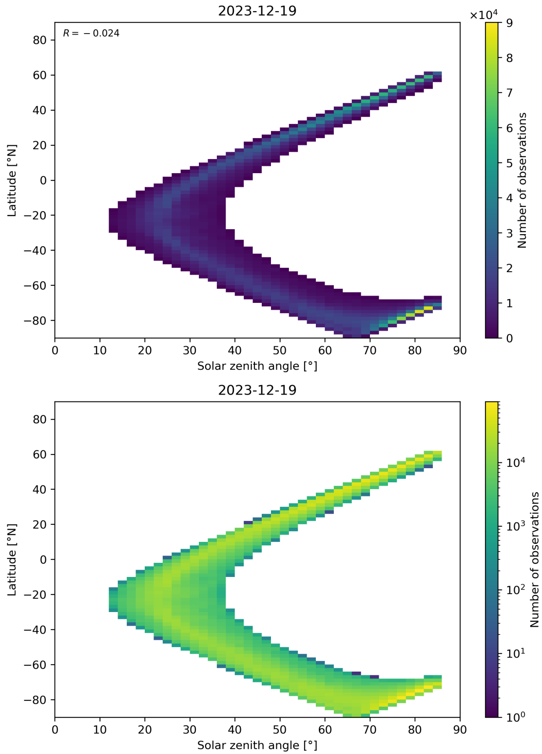
Figure 66: Scatter density plot of “Solar zenith angle” against “Latitude” for 2023-12-18 to 2023-12-20.
