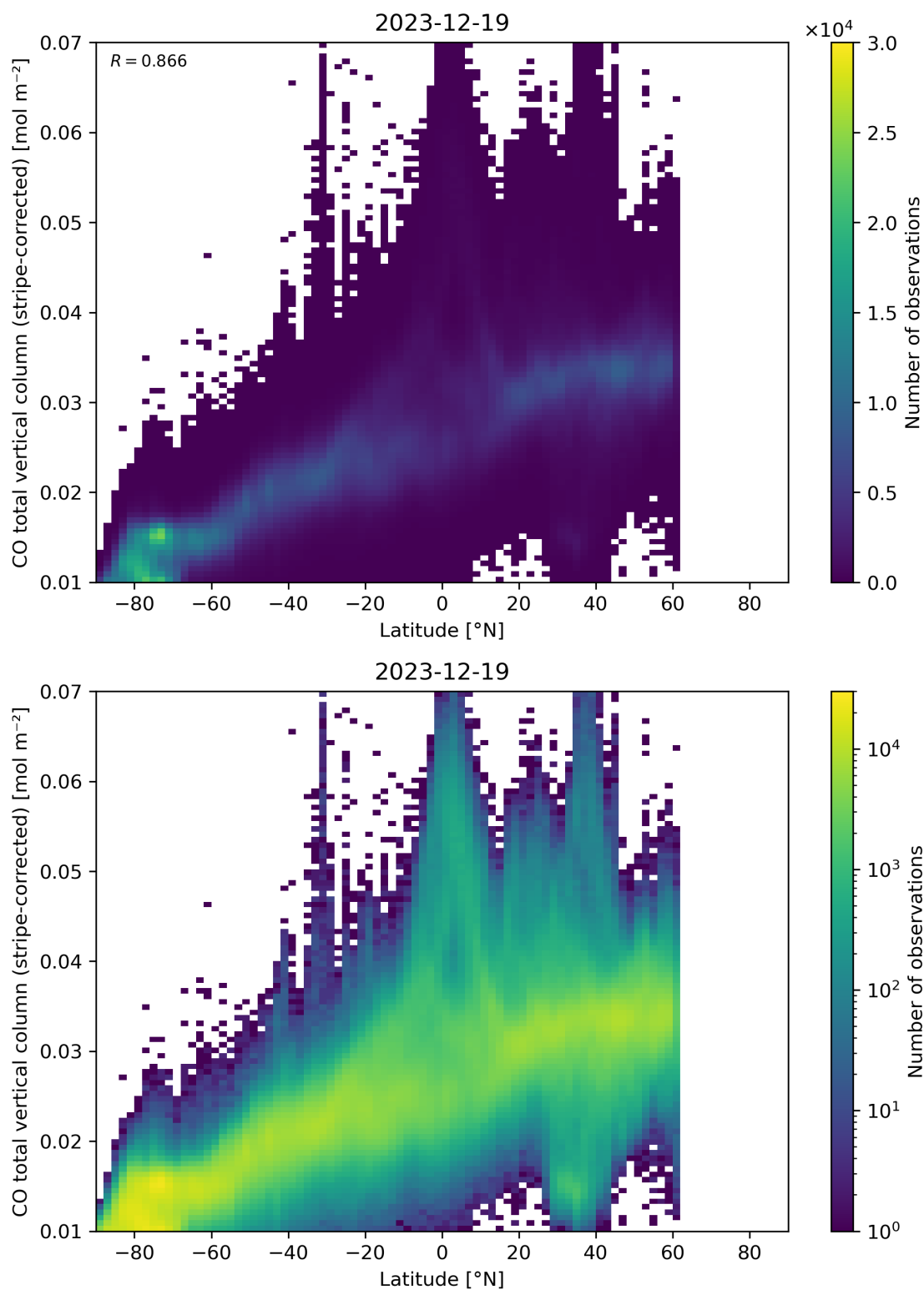
Figure 52: Scatter density plot of “Latitude” against “CO total vertical column (stripe-corrected)” for 2023-12-18 to 2023-12-20.
