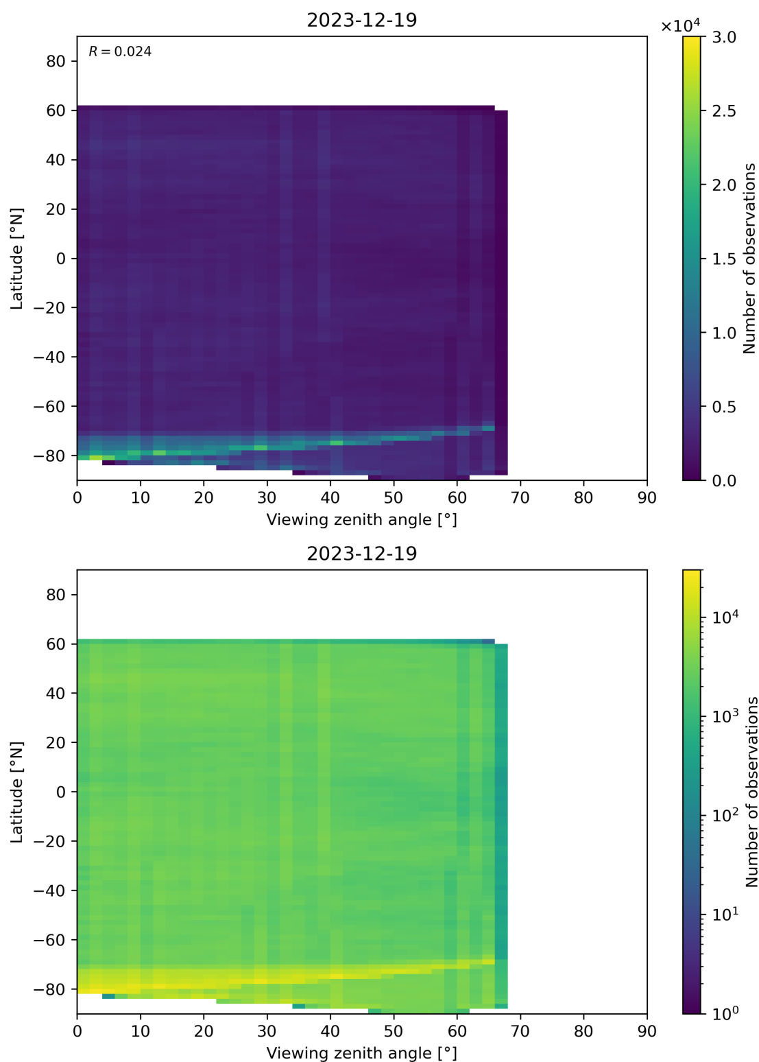
Figure 74: Scatter density plot of “Viewing zenith angle” against “Latitude” for 2023-12-18 to 2023-12-20.
