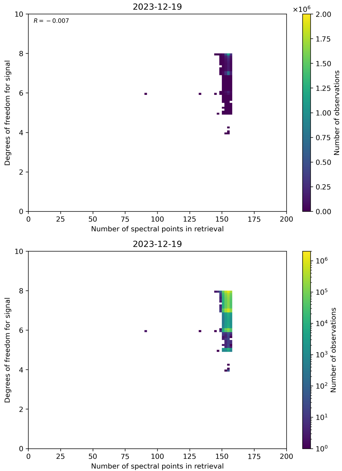
Figure 59: Scatter density plot of “Number of spectral points in retrieval” against “Degrees of freedom for signal” for 2023-12-18 to 2023-12-20.
