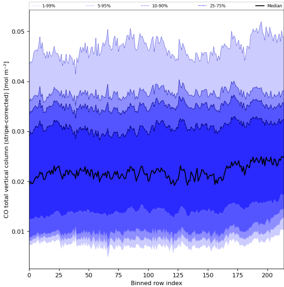
Figure 27: Along track statistics of “CO total vertical column (stripe-corrected)” for 2023-12-18 to 2023-12-20
