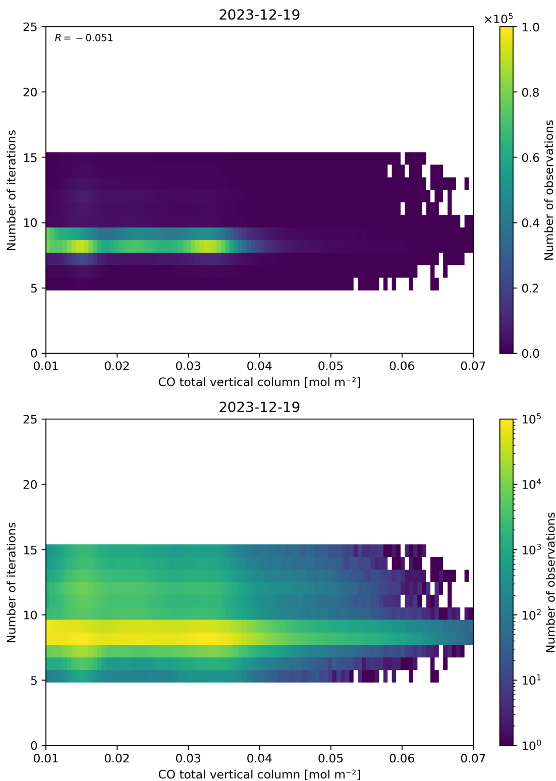
Figure 42: Scatter density plot of “CO total vertical column” against “Number of iterations” for 2023-12-18 to 2023-12-20.
