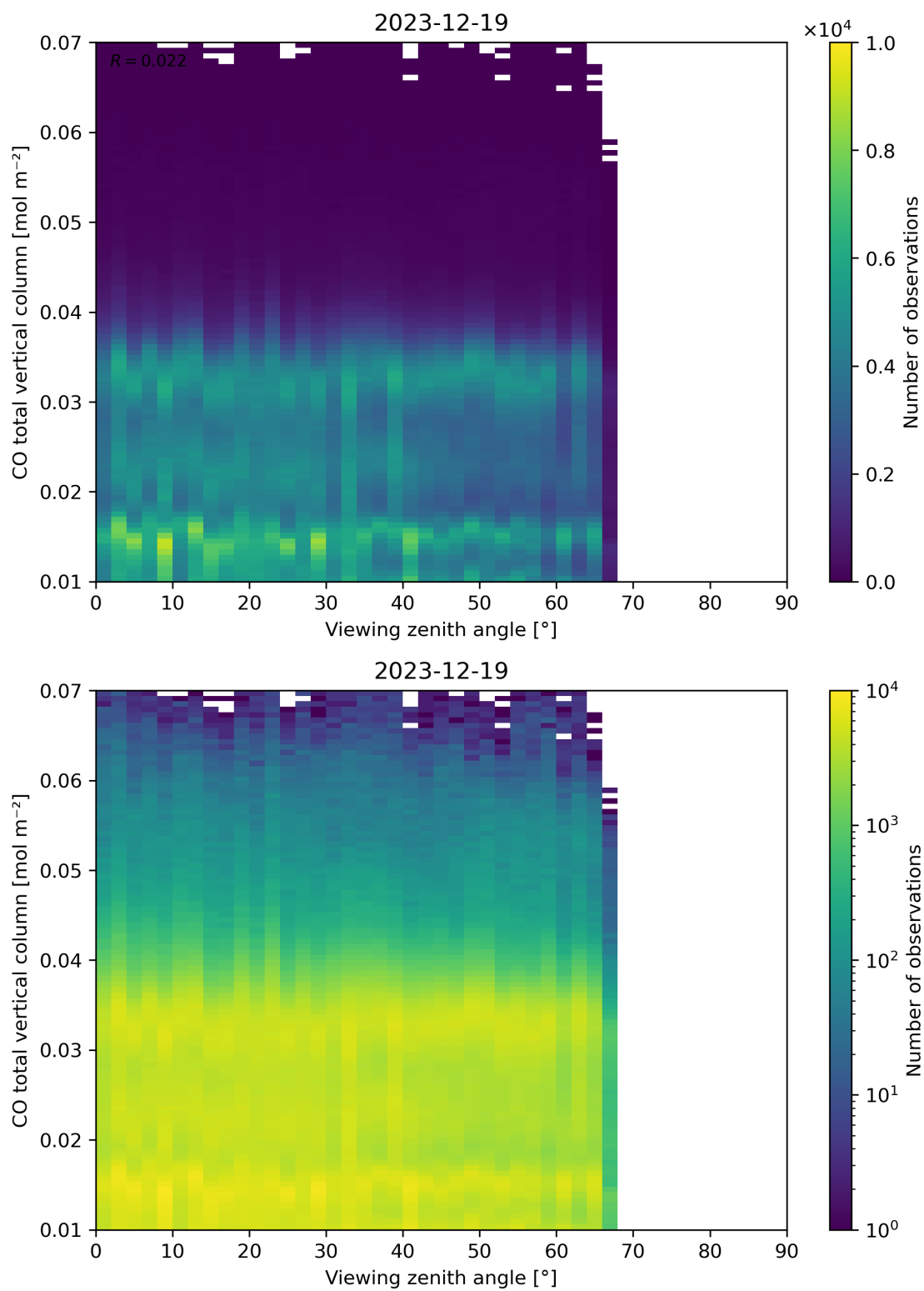
Figure 69: Scatter density plot of “Viewing zenith angle” against “CO total vertical column” for 2023-12-18 to 2023-12-20.
