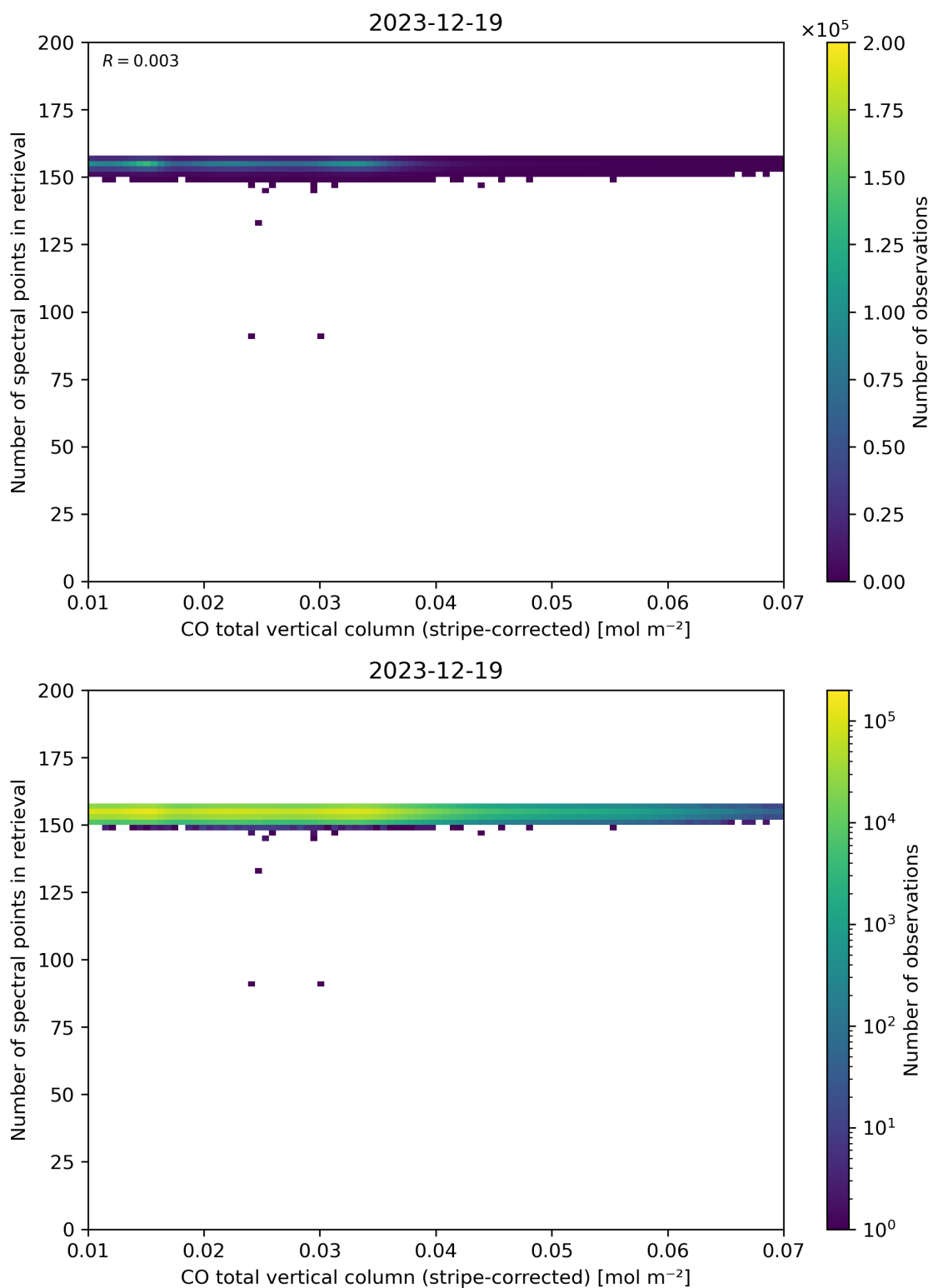
Figure 40: Scatter density plot of “CO total vertical column (stripe-corrected)” against “Number of spectral points in retrieval” for 2023-12-18 to 2023-12-20.
