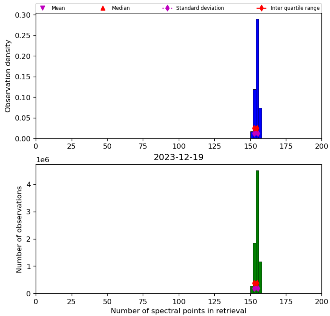
Figure 21: Histogram of “Number of spectral points in retrieval” for 2023-12-18 to 2023-12-20
