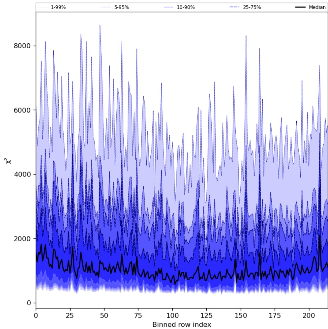
Figure 30: Along track statistics of “ \chi^2 ” for 2023-12-18 to 2023-12-20
