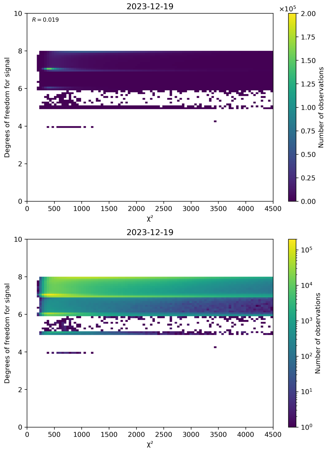
Figure 48: Scatter density plot of “ \chi^2 ” against “Degrees of freedom for signal” for 2023-12-18 to 2023-12-20.
