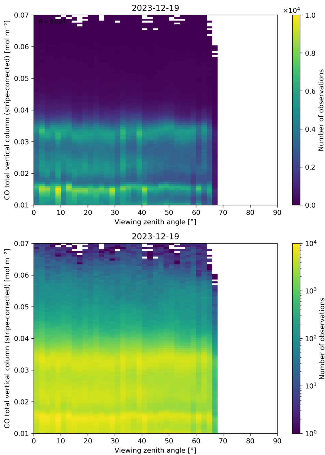
Figure 70: Scatter density plot of “Viewing zenith angle” against “CO total vertical column (stripe-corrected)” for 2023-12-18 to 2023-12-20.
