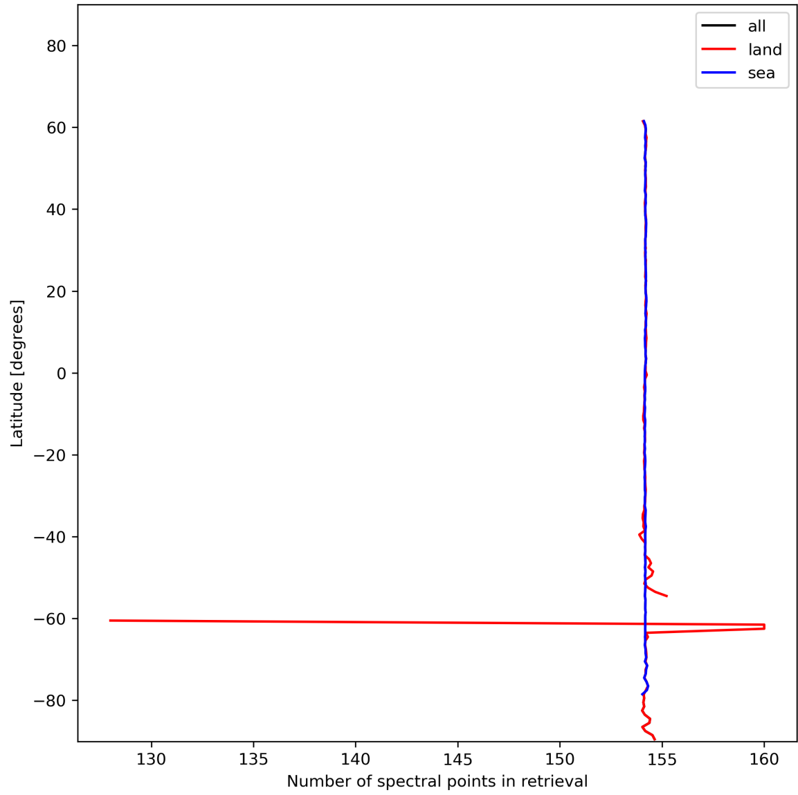
Figure 13: Zonal average of “Number of spectral points in retrieval” for 2023-12-18 to 2023-12-20.
