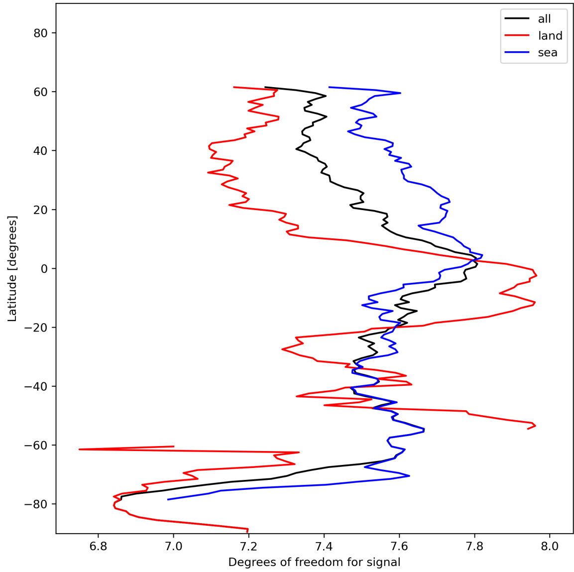
Figure 15: Zonal average of “Degrees of freedom for signal” for 2023-12-18 to 2023-12-20.
