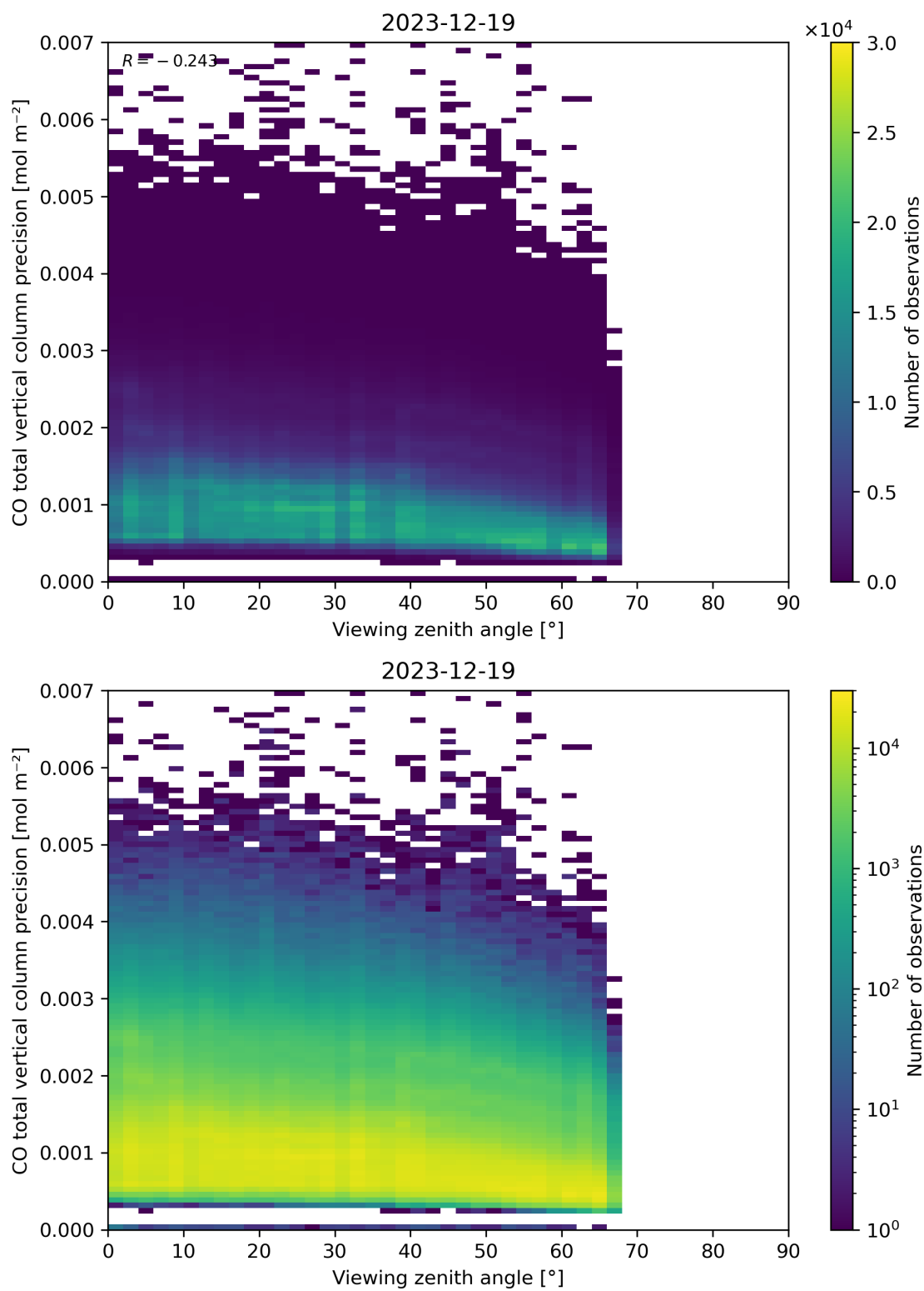
Figure 71: Scatter density plot of “Viewing zenith angle” against “CO total vertical column precision” for 2023-12-18 to 2023-12-20.
