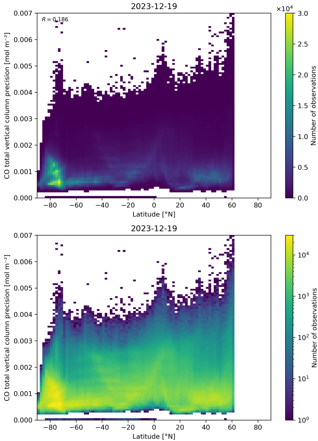
Figure 53: Scatter density plot of “Latitude” against “CO total vertical column precision” for 2023-12-18 to 2023-12-20.
