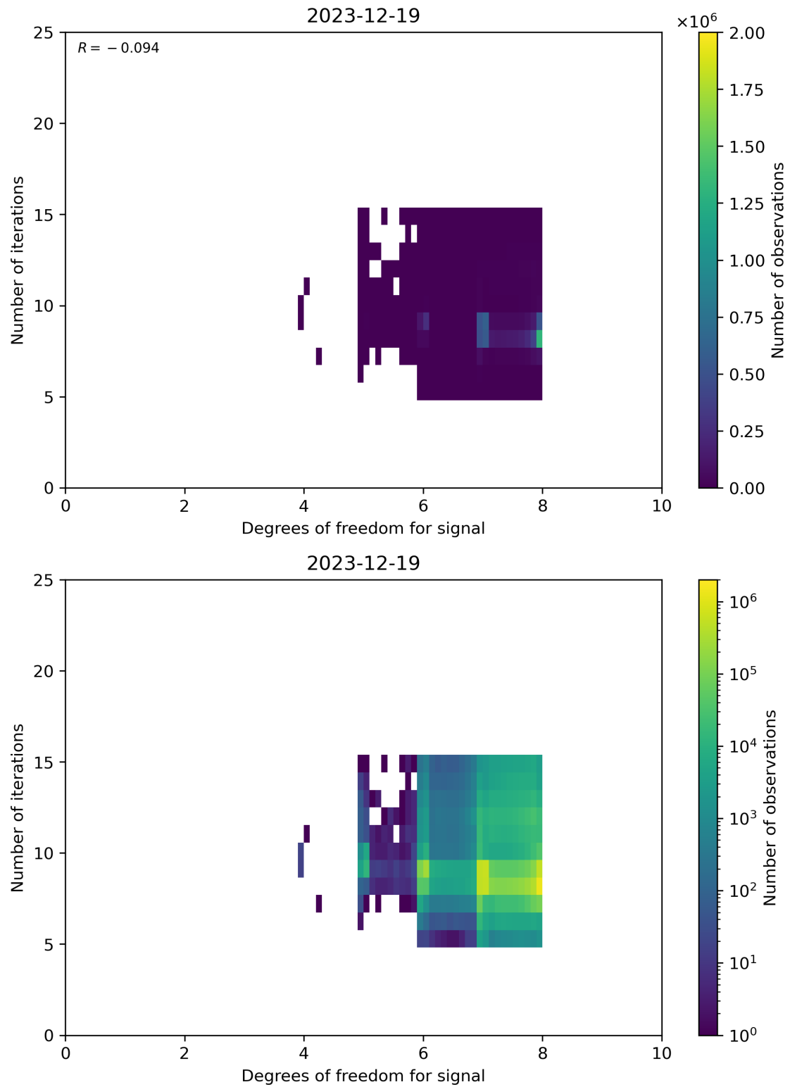
Figure 50: Scatter density plot of “Degrees of freedom for signal” against “Number of iterations” for 2023-12-18 to 2023-12-20.
