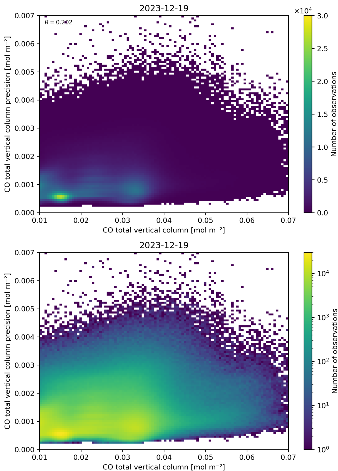
Figure 34: Scatter density plot of “CO total vertical column” against “CO total vertical column precision” for 2023-12-18 to 2023-12-20.
