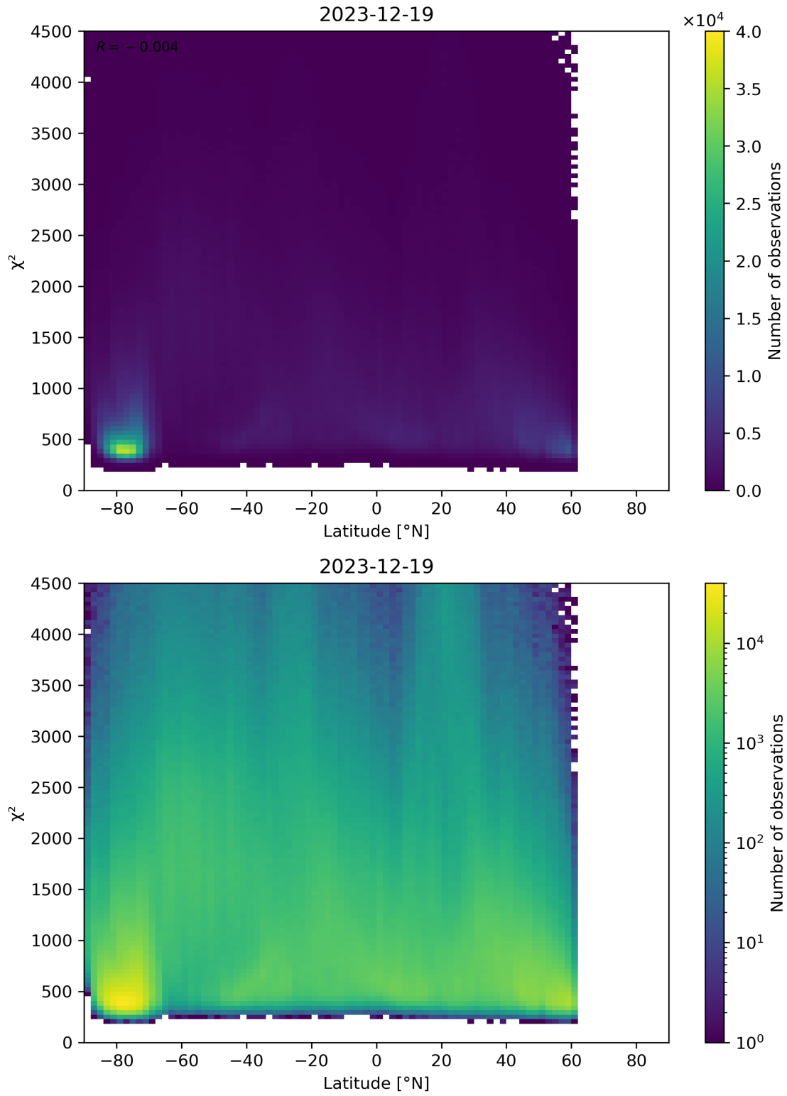
Figure 54: Scatter density plot of “Latitude” against “ \chi^2 ” for 2023-12-18 to 2023-12-20.
