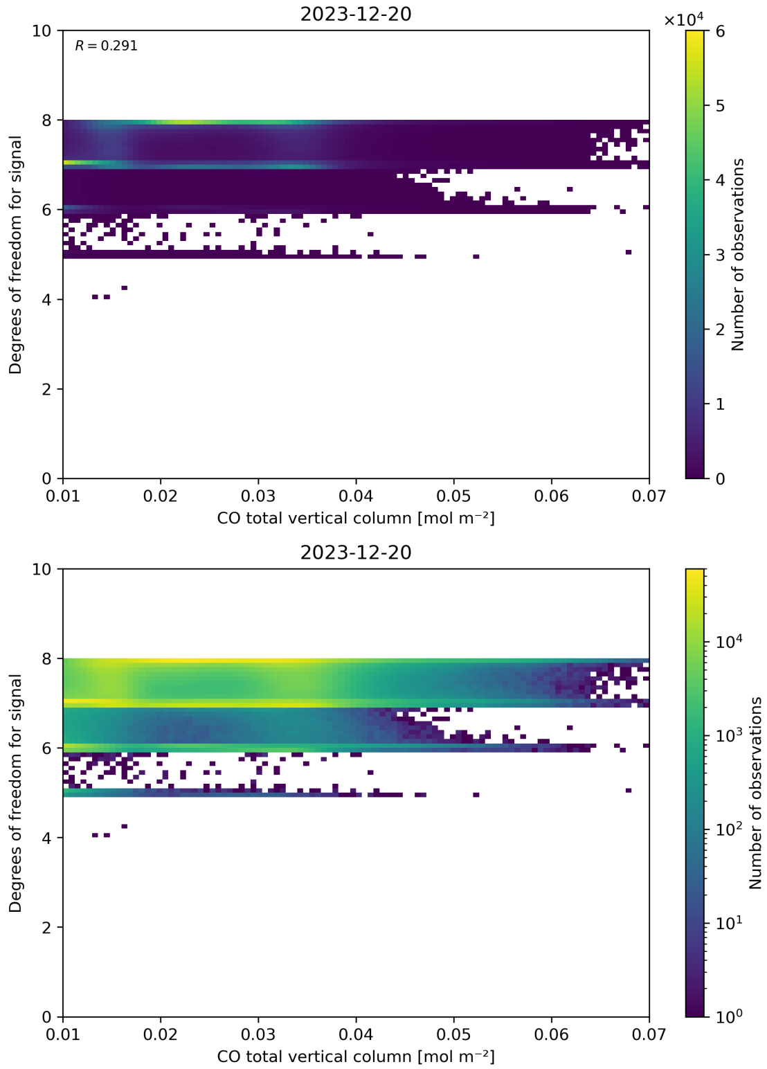
Figure 41: Scatter density plot of “CO total vertical column” against “Degrees of freedom for signal” for 2023-12-20 to 2023-12-21.
