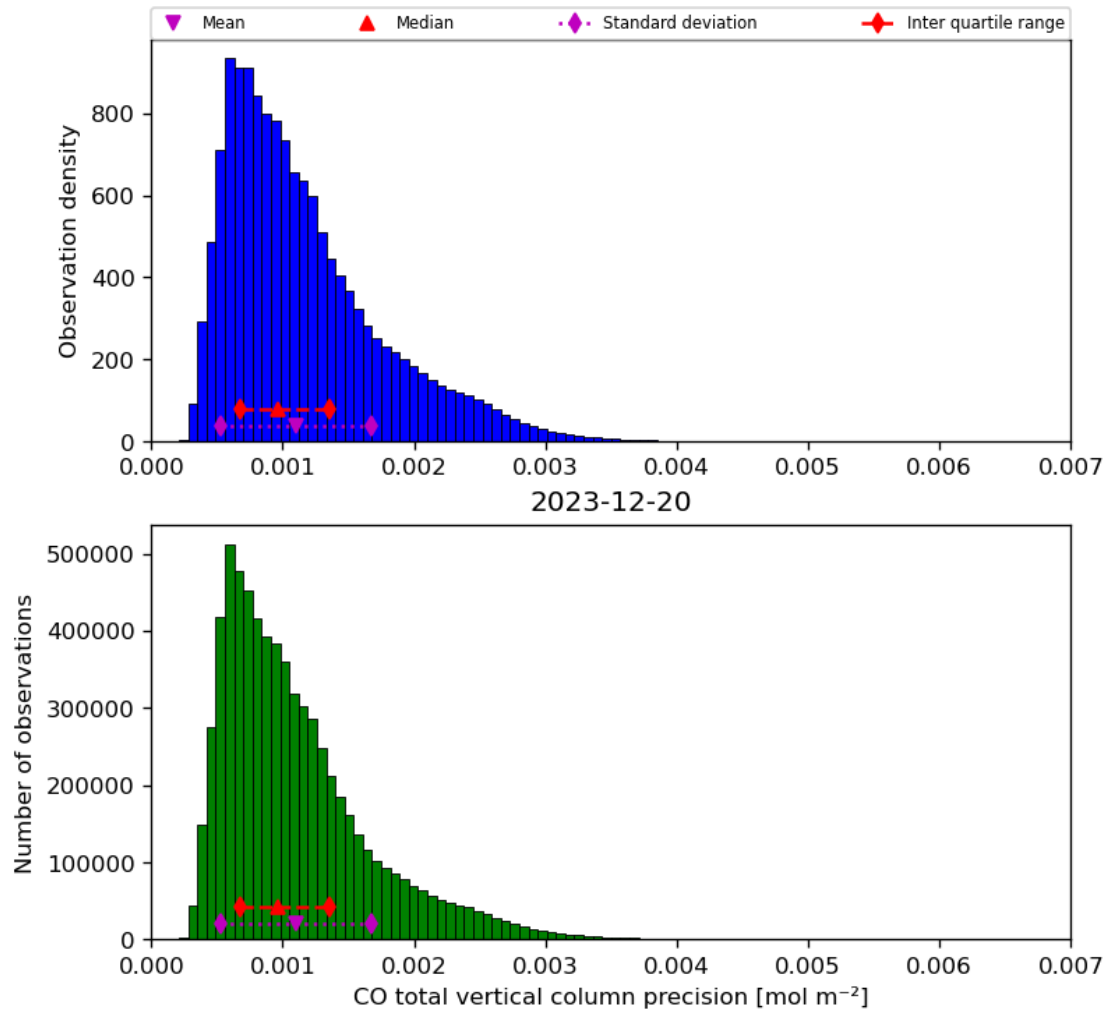
Figure 20: Histogram of “CO total vertical column precision” for 2023-12-20 to 2023-12-21
