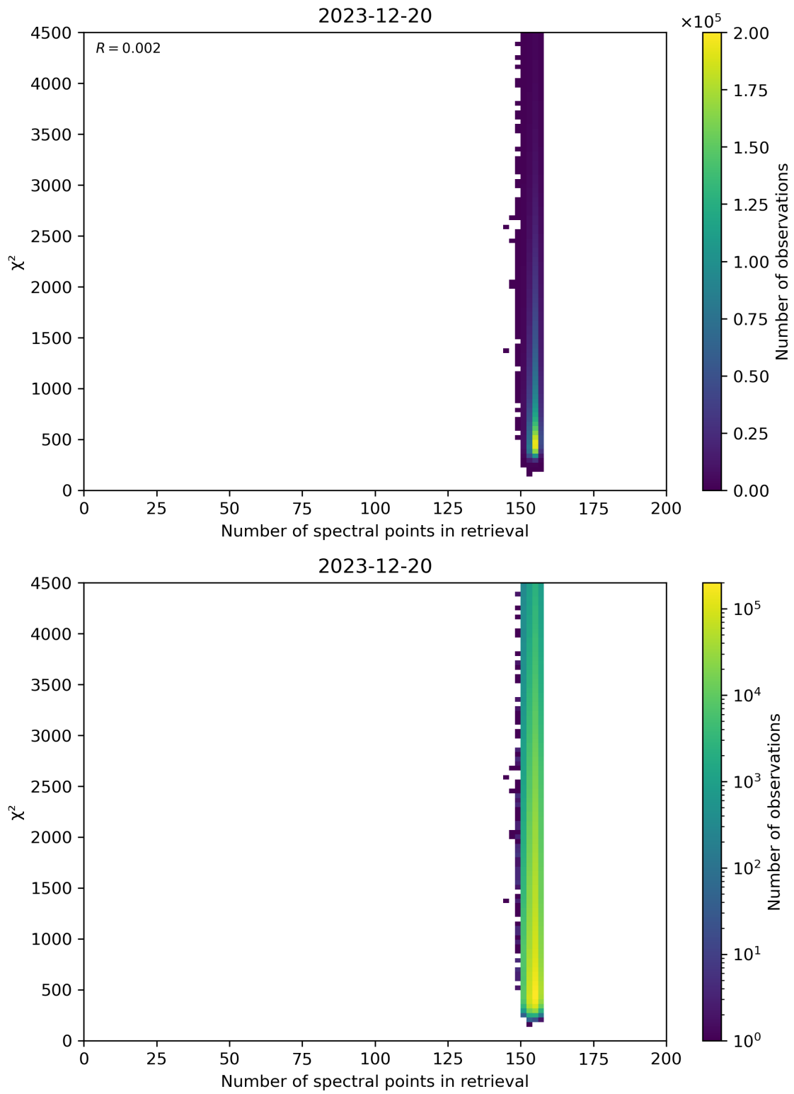
Figure 58: Scatter density plot of “Number of spectral points in retrieval” against “ \chi^2 ” for 2023-12-20 to 2023-12-21.
