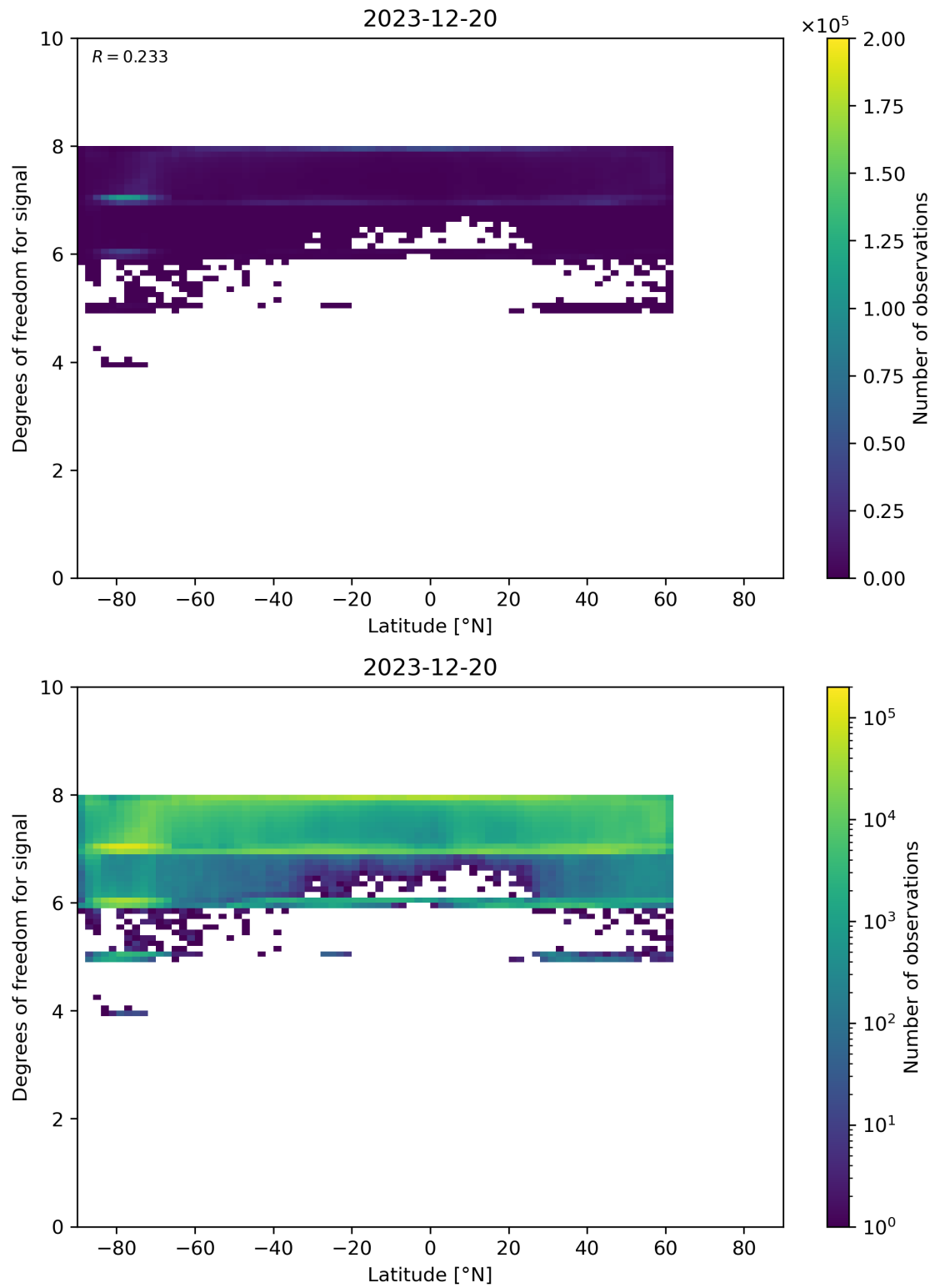
Figure 55: Scatter density plot of “Latitude” against “Degrees of freedom for signal” for 2023-12-20 to 2023-12-21.
