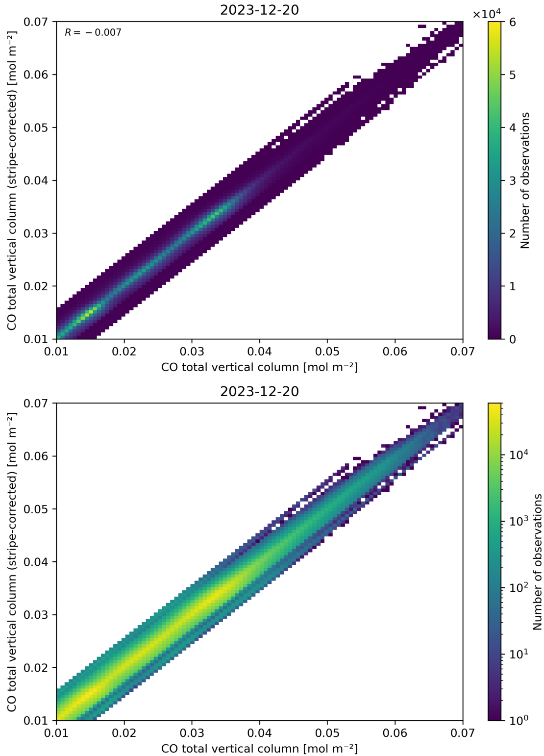
Figure 33: Scatter density plot of “CO total vertical column” against “CO total vertical column (stripe-corrected)” for 2023-12-20 to 2023-12-21.
