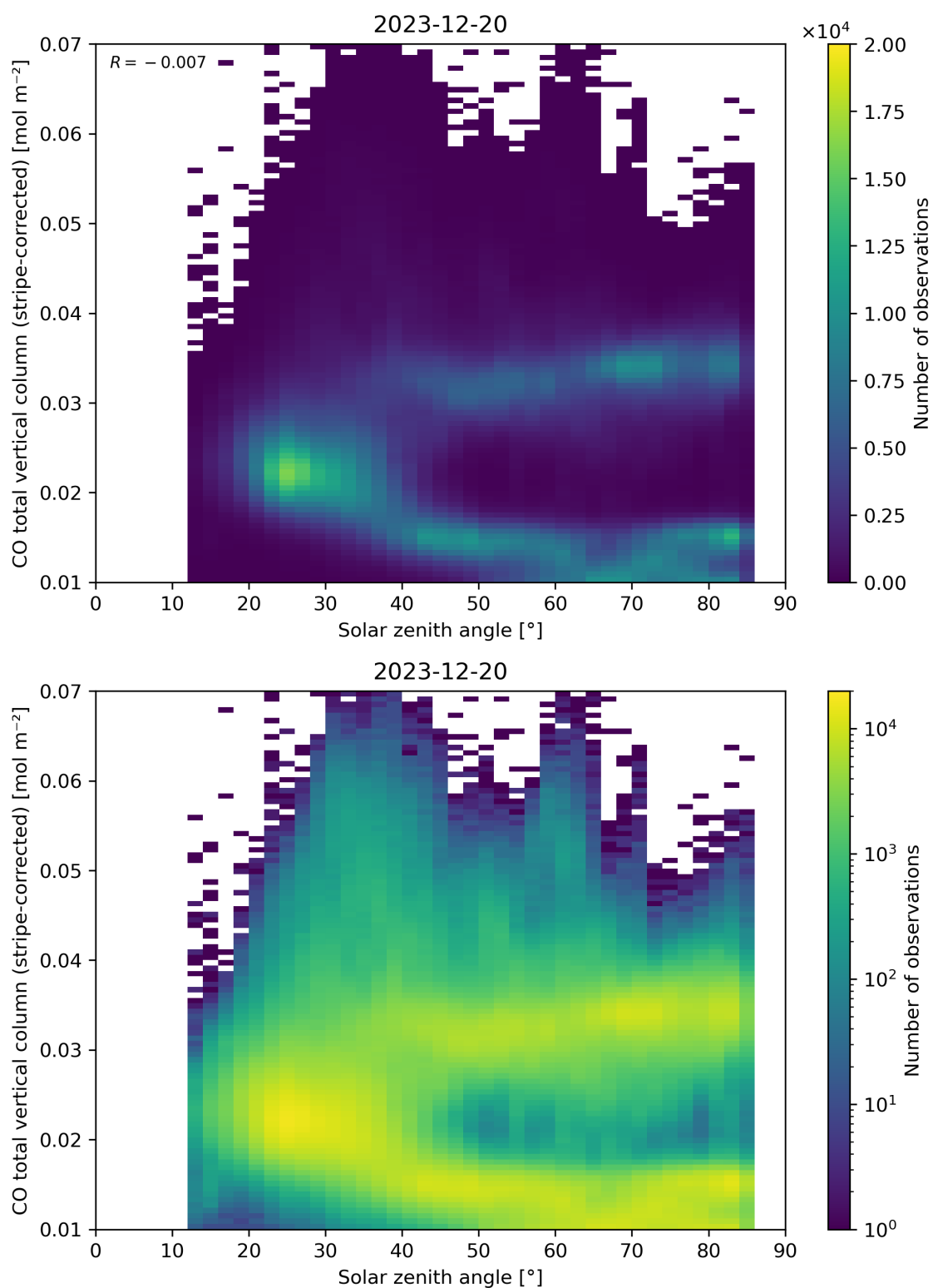
Figure 62: Scatter density plot of “Solar zenith angle” against “CO total vertical column (stripe-corrected)” for 2023-12-20 to 2023-12-21.
