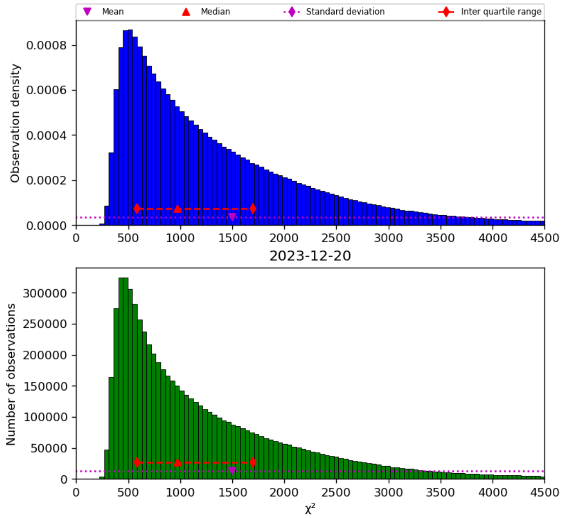
Figure 22: Histogram of “ \chi^2 ” for 2023-12-20 to 2023-12-21
