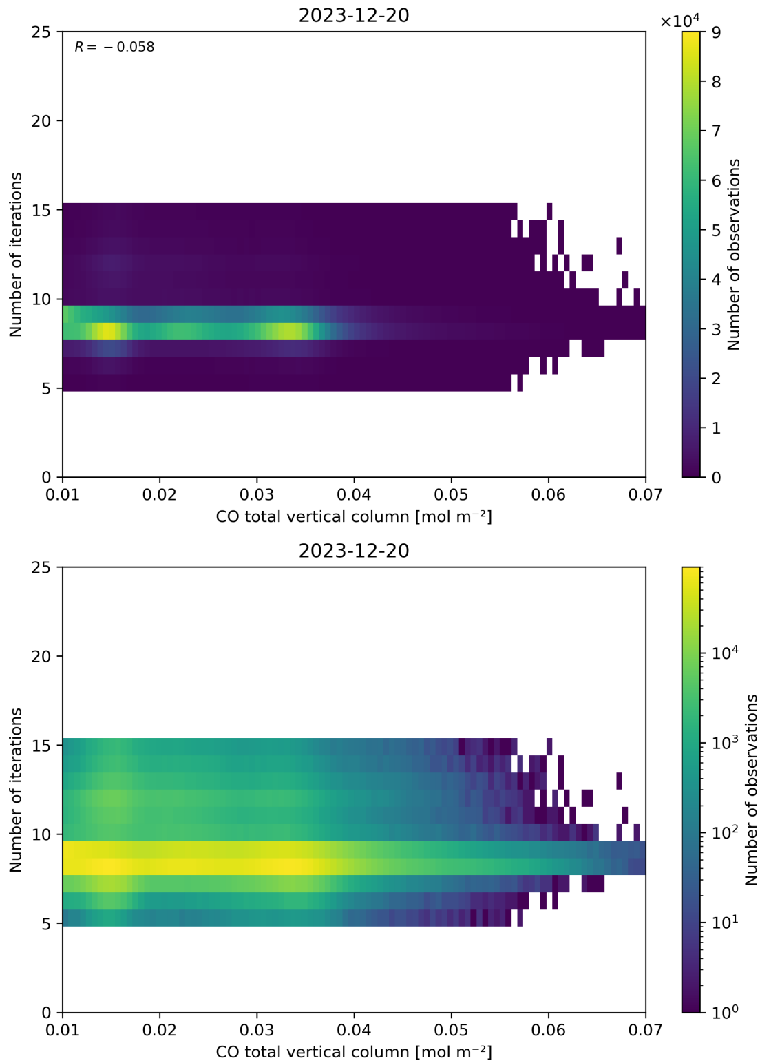
Figure 42: Scatter density plot of “CO total vertical column” against “Number of iterations” for 2023-12-20 to 2023-12-21.
