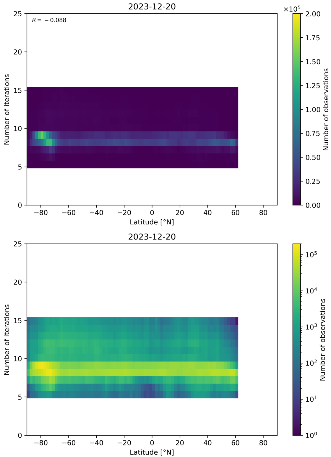
Figure 56: Scatter density plot of “Latitude” against “Number of iterations” for 2023-12-20 to 2023-12-21.
