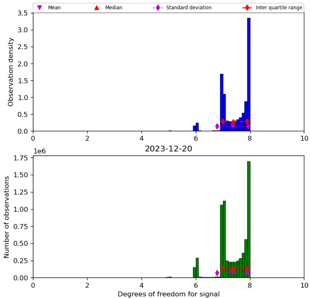
Figure 23: Histogram of “Degrees of freedom for signal” for 2023-12-20 to 2023-12-21
