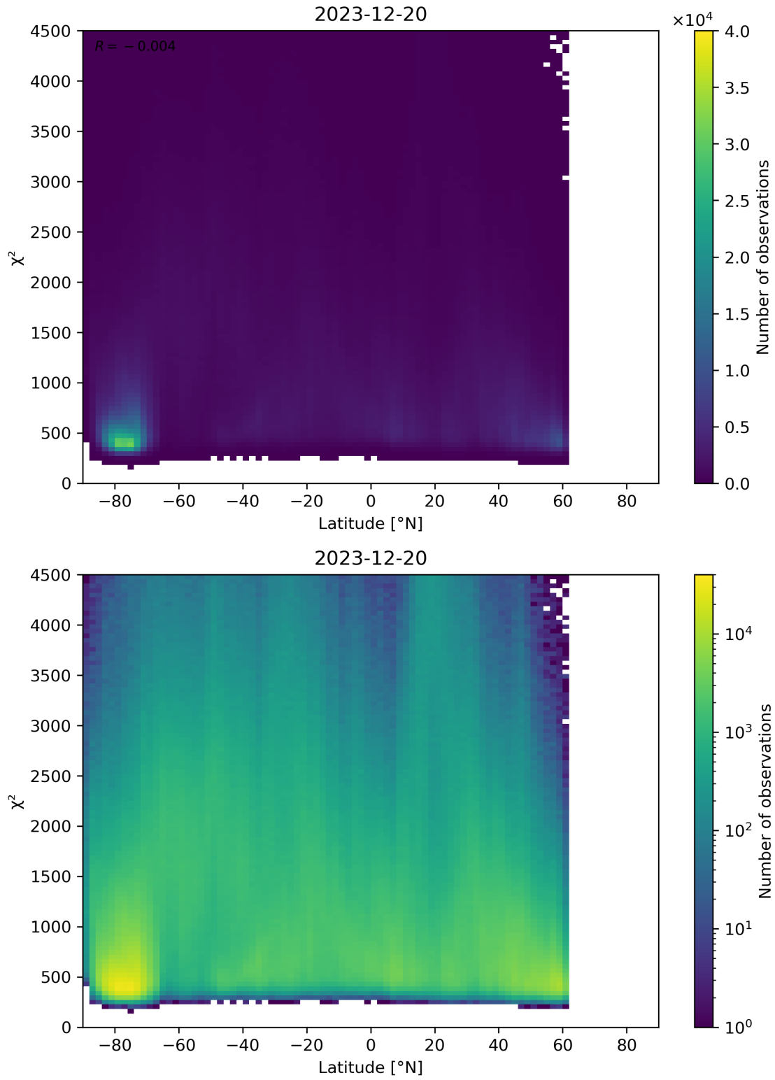
Figure 54: Scatter density plot of “Latitude” against “ \chi^2 ” for 2023-12-20 to 2023-12-21.
