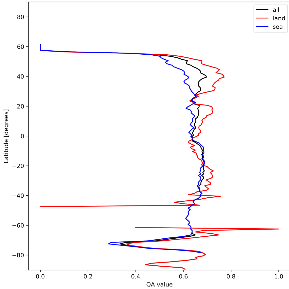
Figure 9: Zonal average of “QA value” for 2023-12-20 to 2023-12-21.
