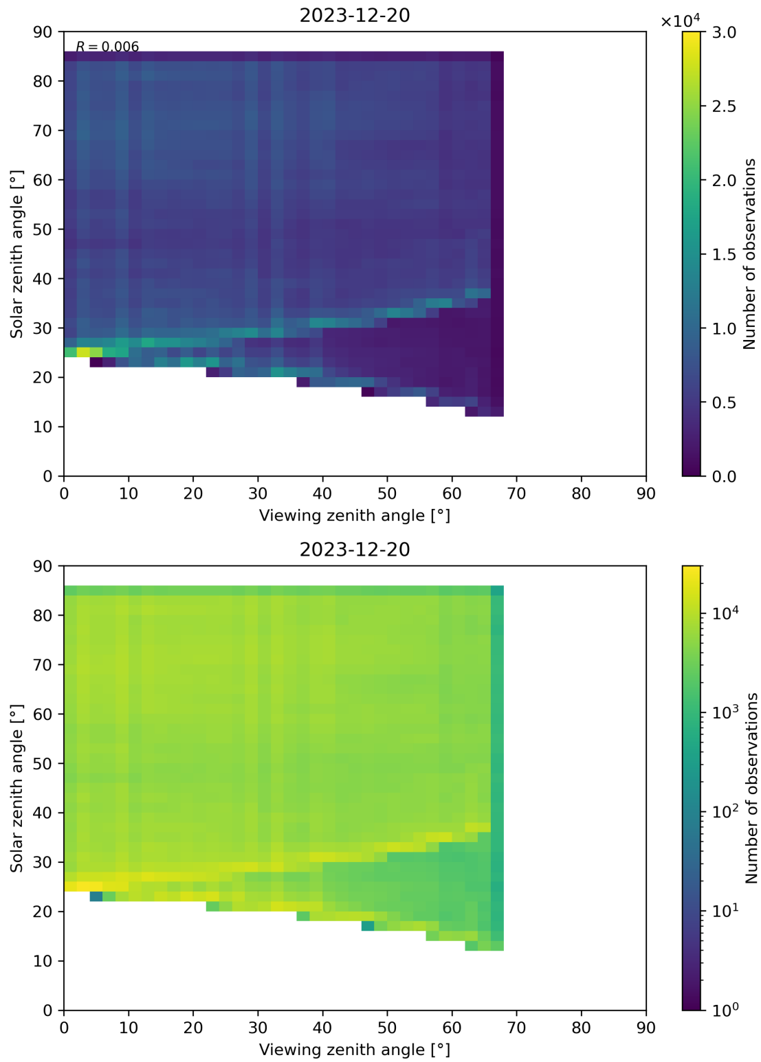
Figure 77: Scatter density plot of “Viewing zenith angle” against “Solar zenith angle” for 2023-12-20 to 2023-12-21.
