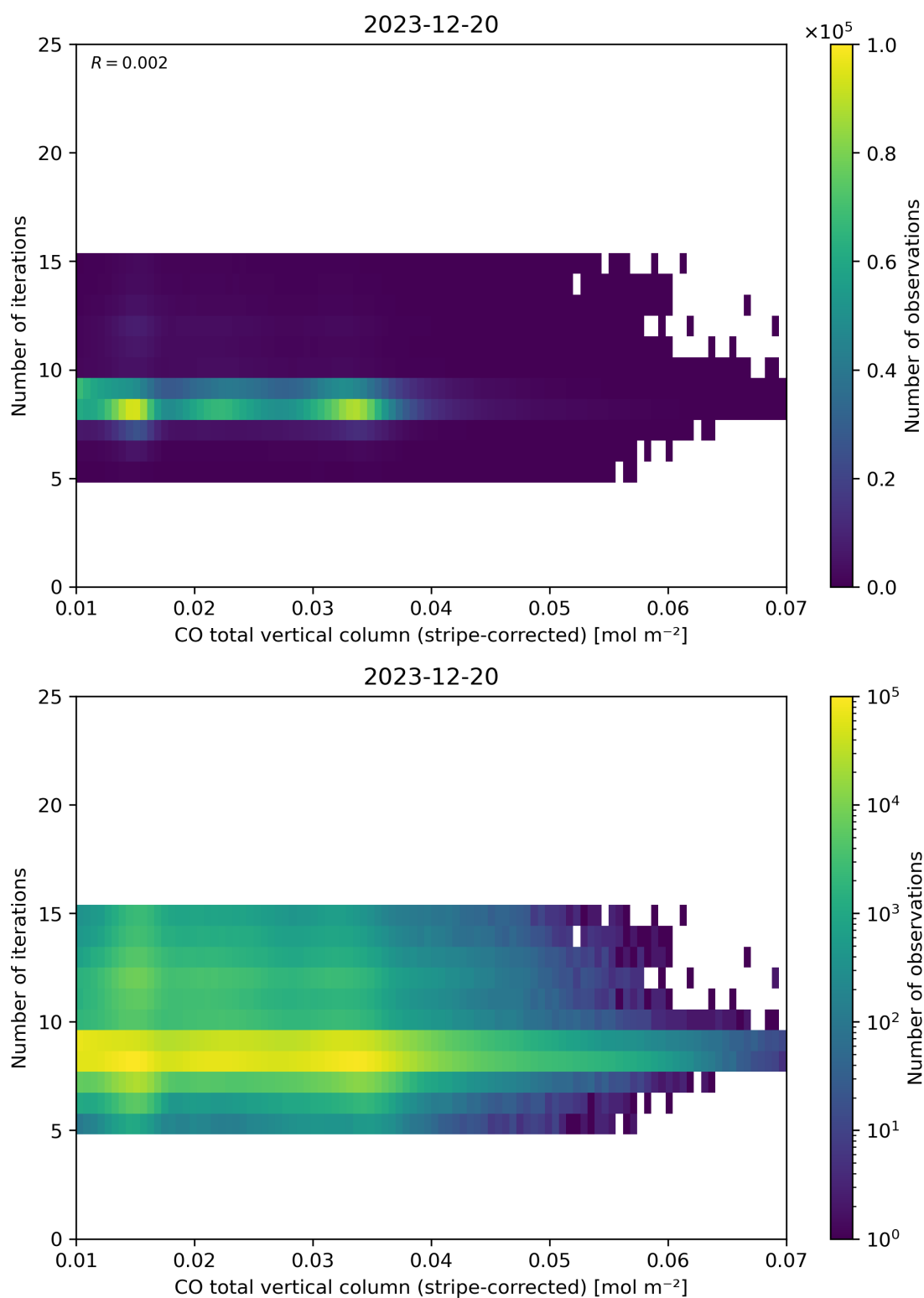
Figure 39: Scatter density plot of “CO total vertical column (stripe-corrected)” against “Number of iterations” for 2023-12-20 to 2023-12-21.
