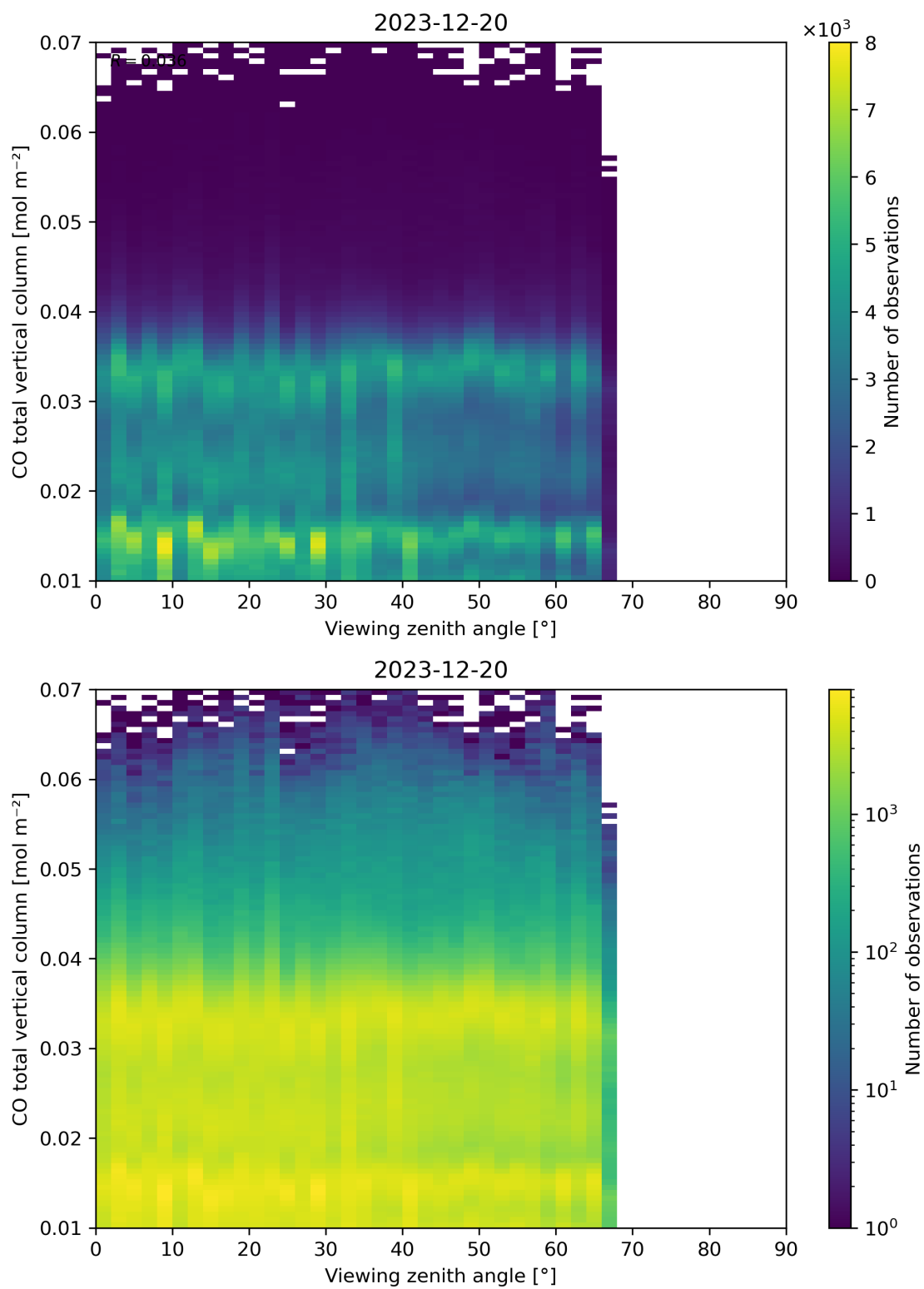
Figure 69: Scatter density plot of “Viewing zenith angle” against “CO total vertical column” for 2023-12-20 to 2023-12-21.
