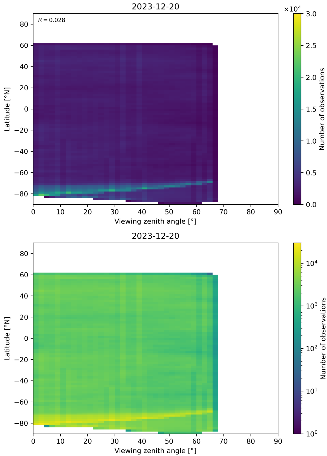
Figure 74: Scatter density plot of “Viewing zenith angle” against “Latitude” for 2023-12-20 to 2023-12-21.
