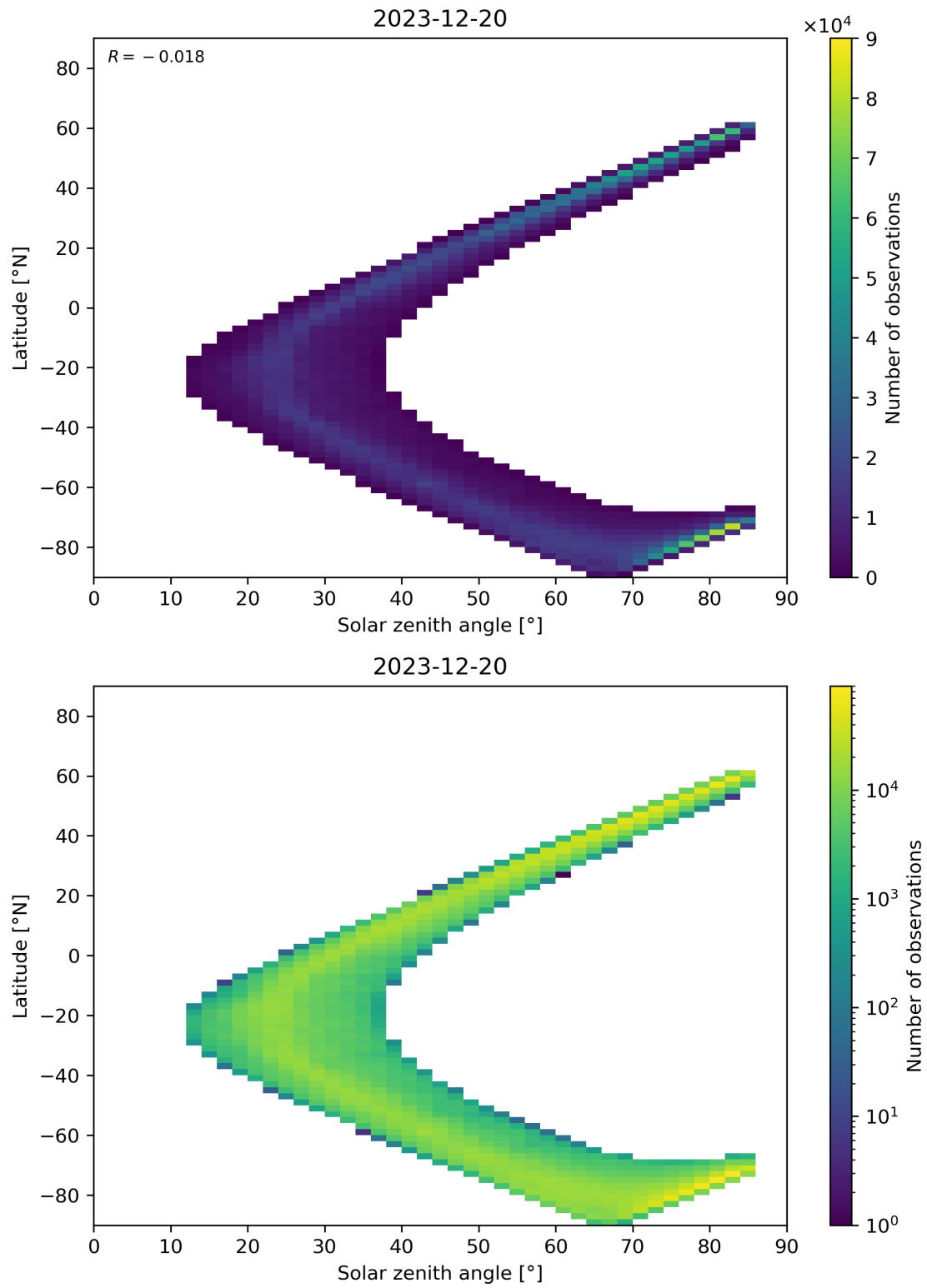
Figure 66: Scatter density plot of “Solar zenith angle” against “Latitude” for 2023-12-20 to 2023-12-21.
