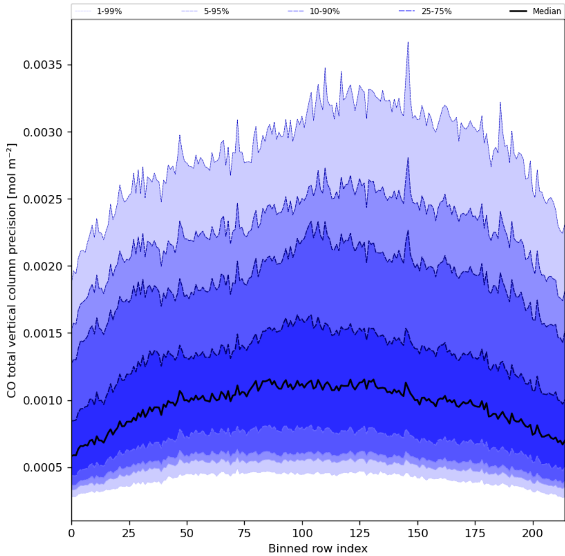
Figure 28: Along track statistics of “CO total vertical column precision” for 2023-12-20 to 2023-12-21
