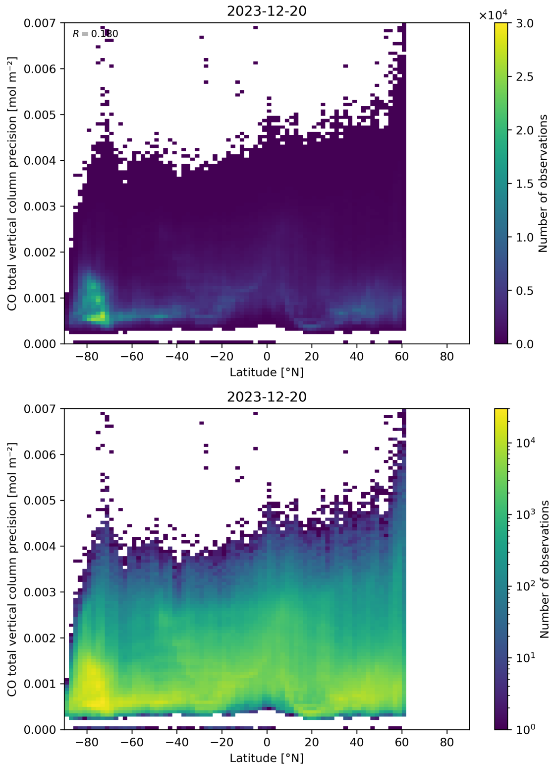
Figure 53: Scatter density plot of “Latitude” against “CO total vertical column precision” for 2023-12-20 to 2023-12-21.
