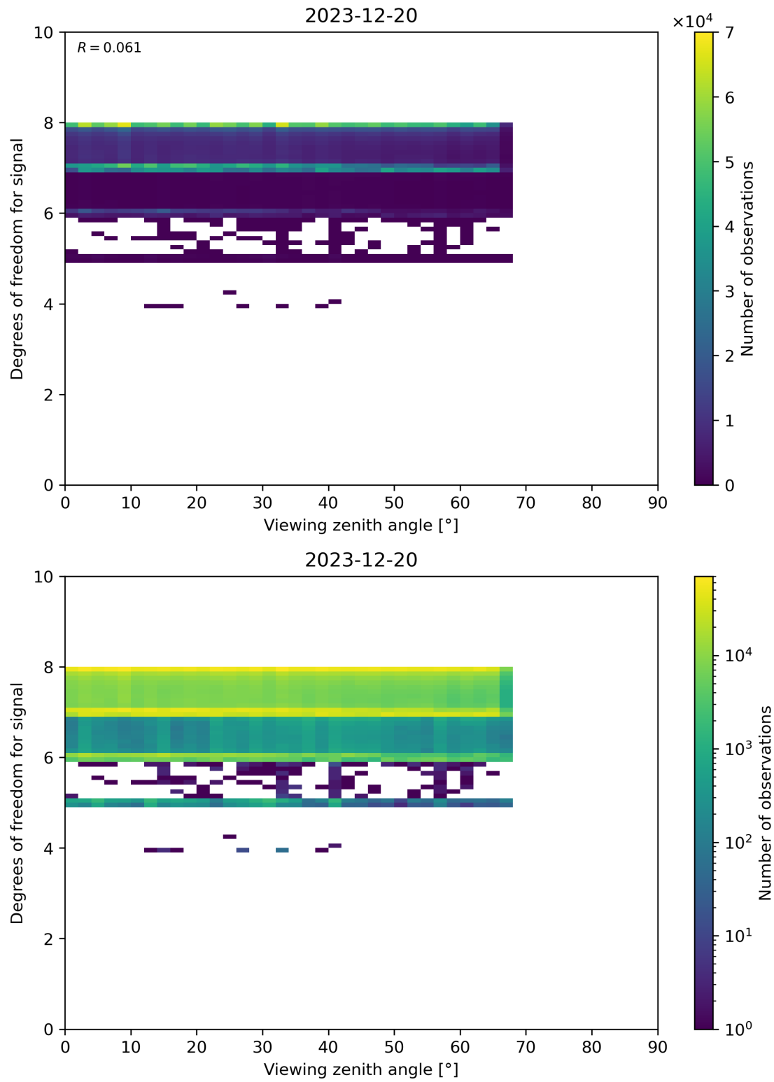
Figure 73: Scatter density plot of “Viewing zenith angle” against “Degrees of freedom for signal” for 2023-12-20 to 2023-12-21.
