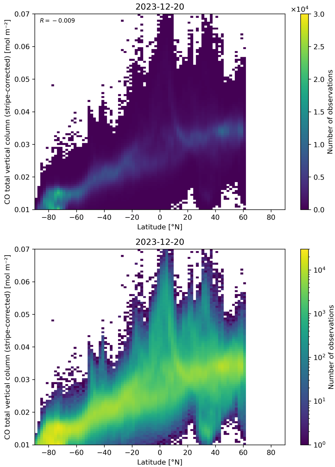
Figure 52: Scatter density plot of “Latitude” against “CO total vertical column (stripe-corrected)” for 2023-12-20 to 2023-12-21.
