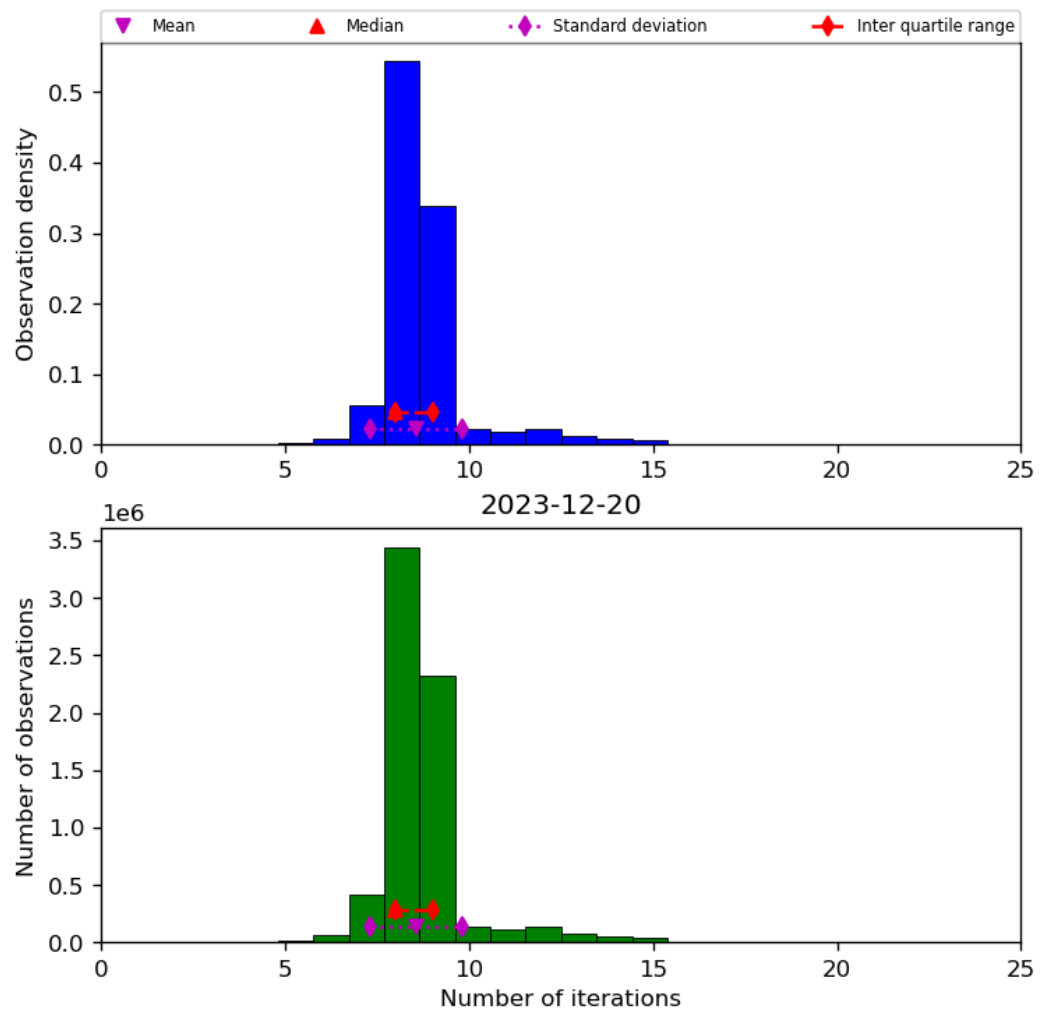
Figure 24: Histogram of “Number of iterations” for 2023-12-20 to 2023-12-21
