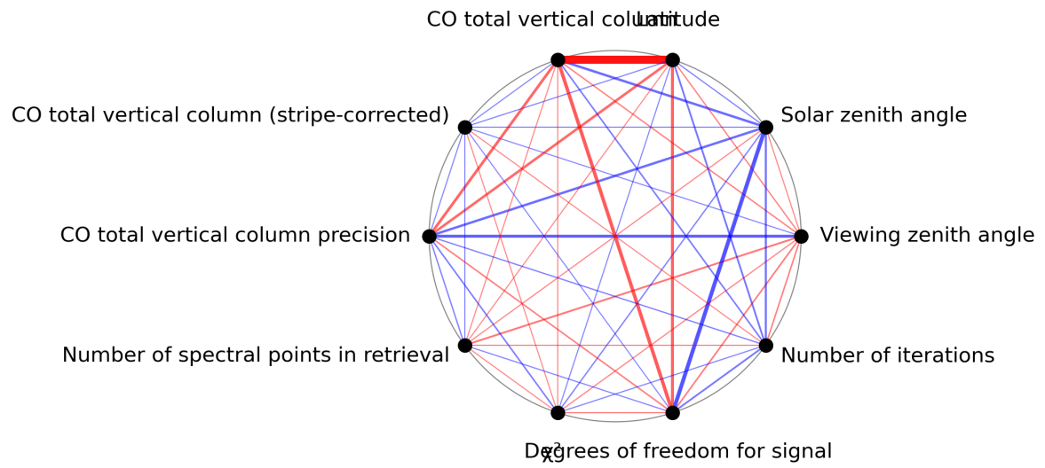
Figure 1: Map of correlation graph for 2023-12-20 to 2023-12-21.
