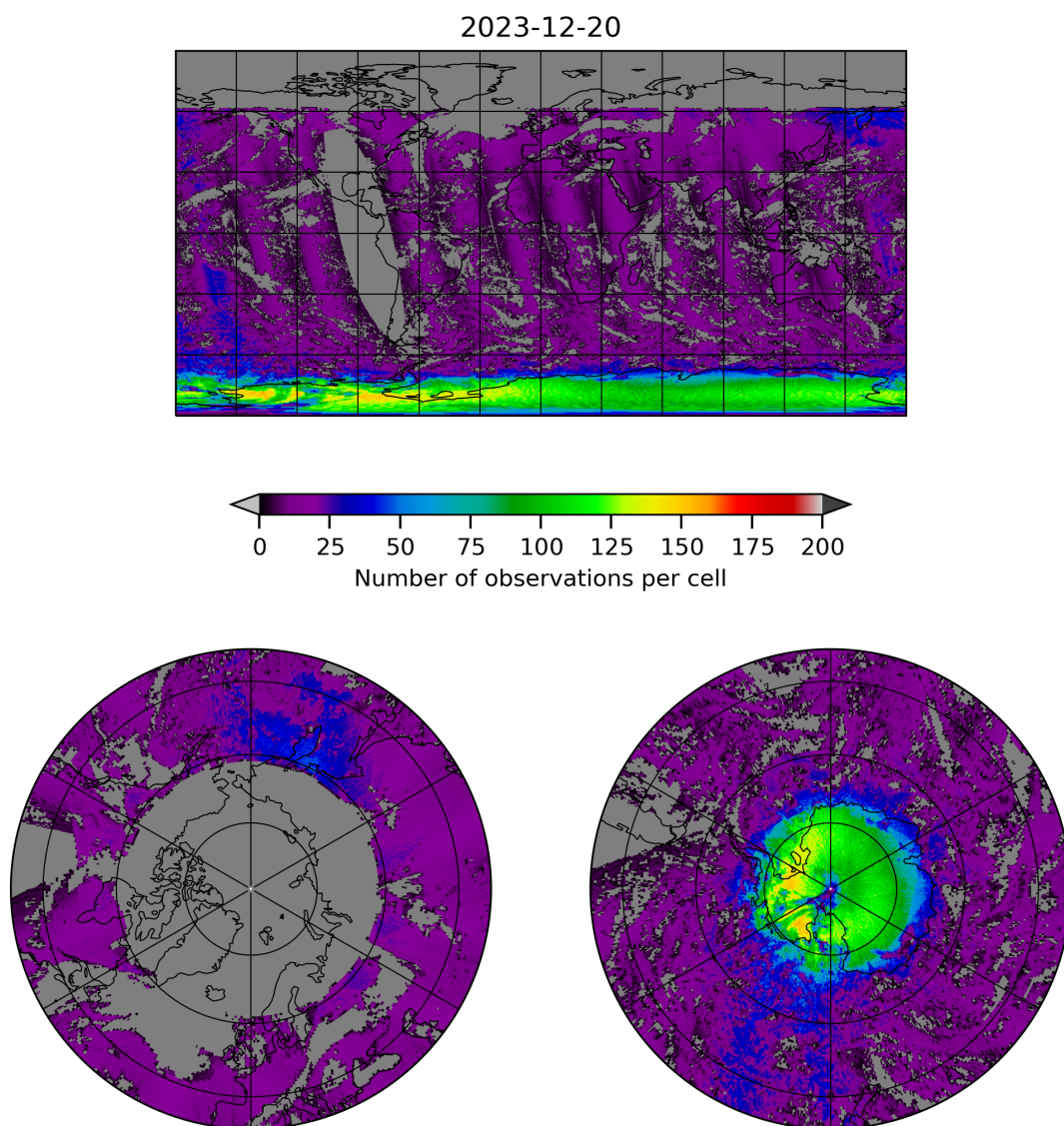
Figure 8: Map of the number of observations for 2023-12-20 to 2023-12-21
