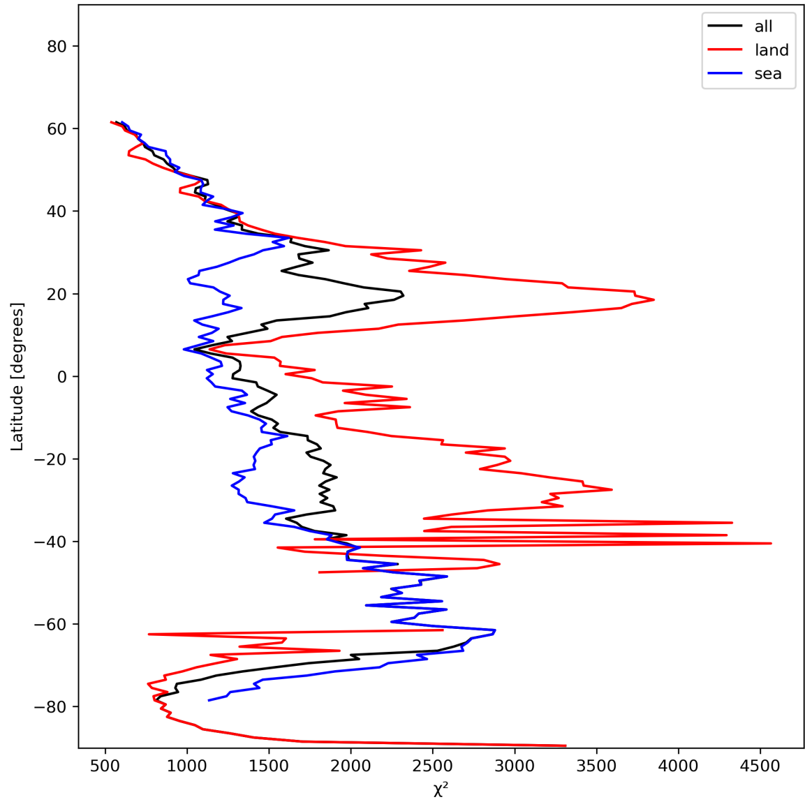
Figure 14: Zonal average of “ \chi^2 ” for 2023-12-20 to 2023-12-21.
