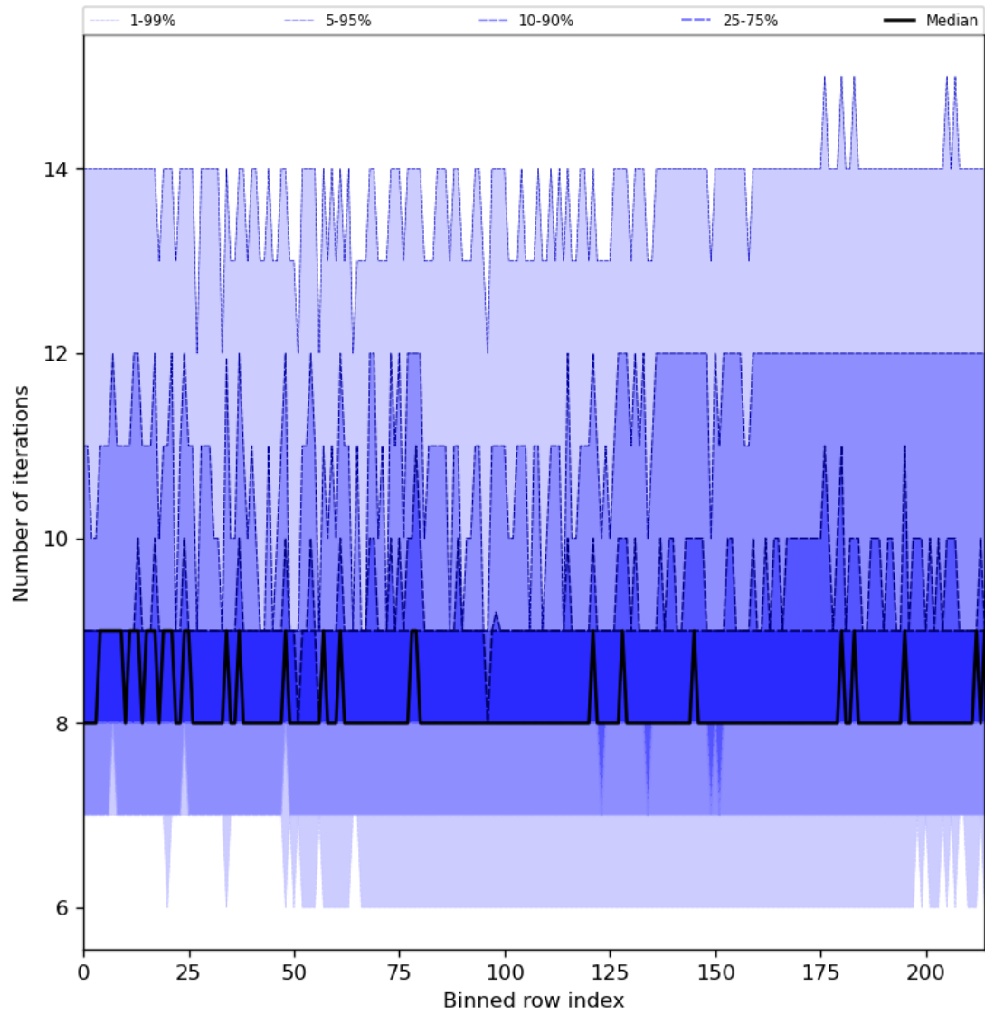
Figure 32: Along track statistics of “Number of iterations” for 2023-12-20 to 2023-12-21
