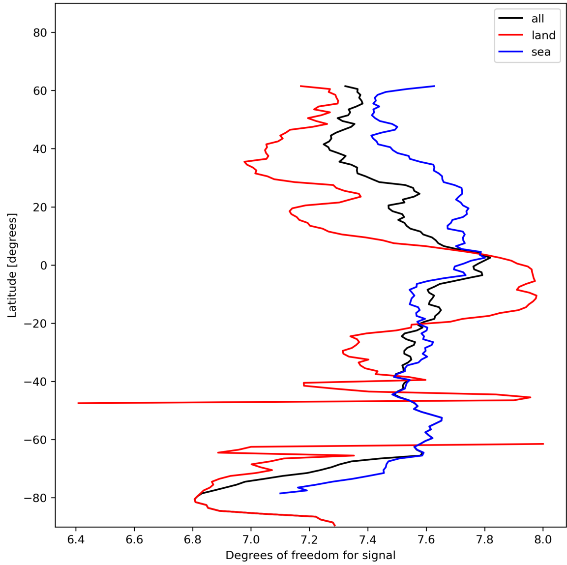
Figure 15: Zonal average of “Degrees of freedom for signal” for 2023-12-20 to 2023-12-21.
