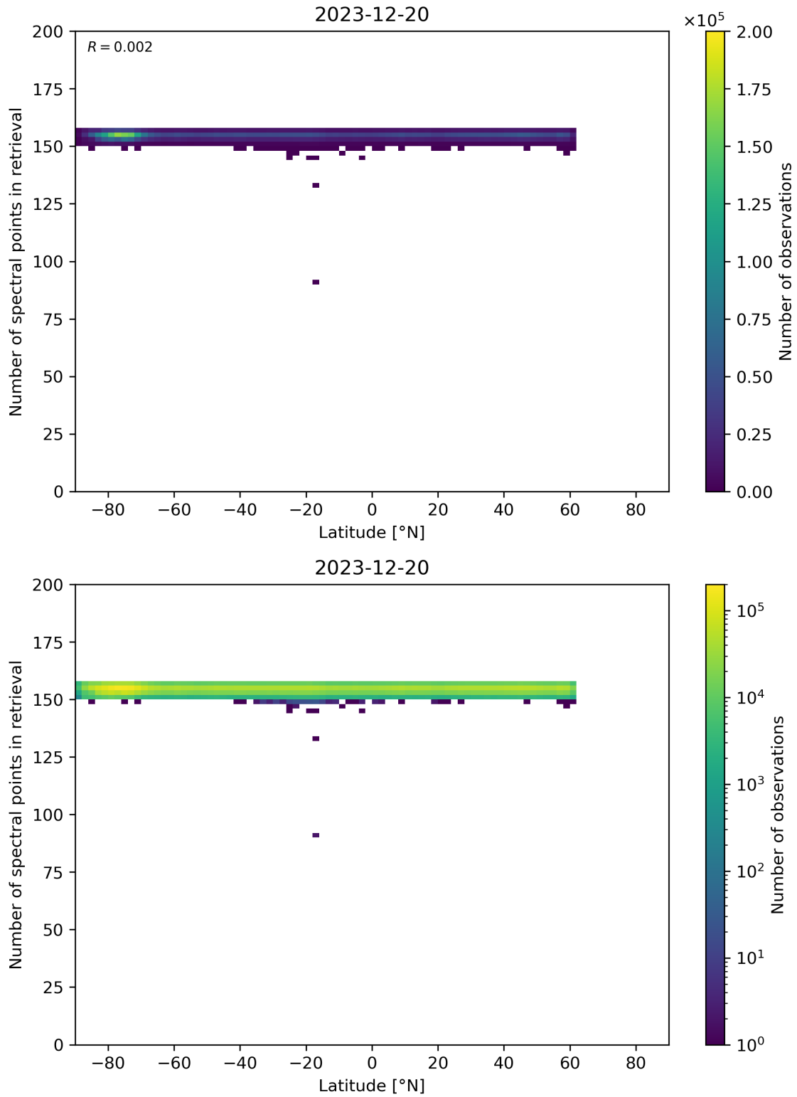
Figure 57: Scatter density plot of “Latitude” against “Number of spectral points in retrieval” for 2023-12-20 to 2023-12-21.
