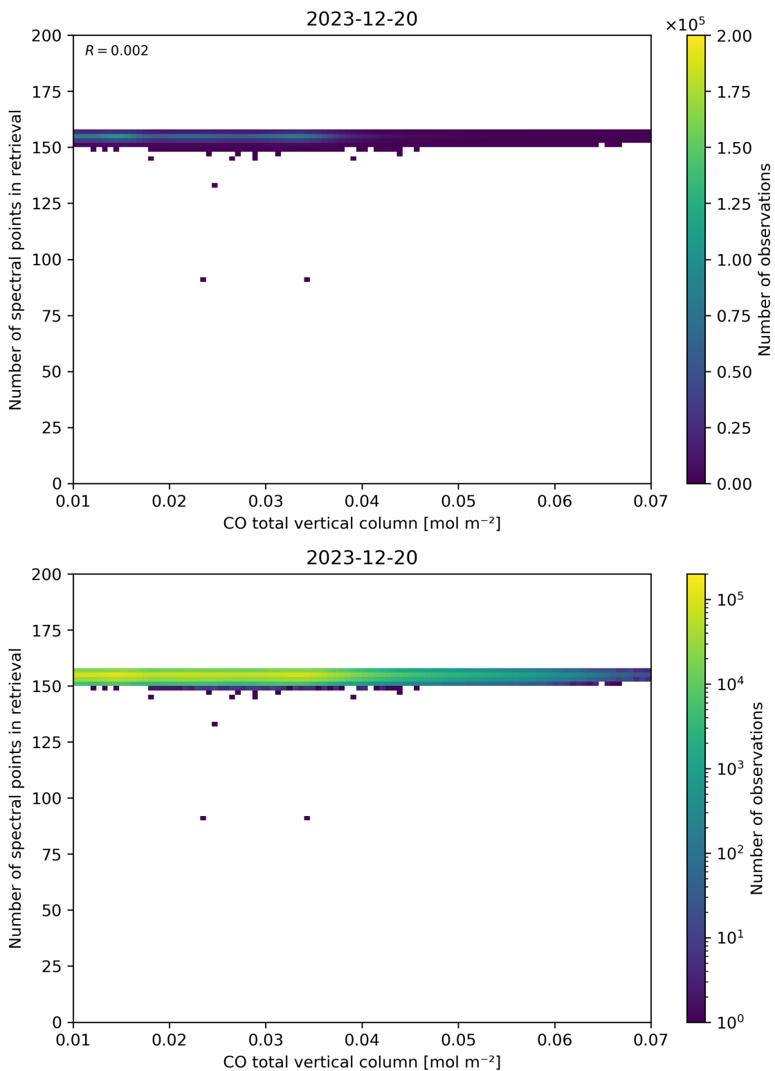
Figure 43: Scatter density plot of “CO total vertical column” against “Number of spectral points in retrieval” for 2023-12-20 to 2023-12-21.
