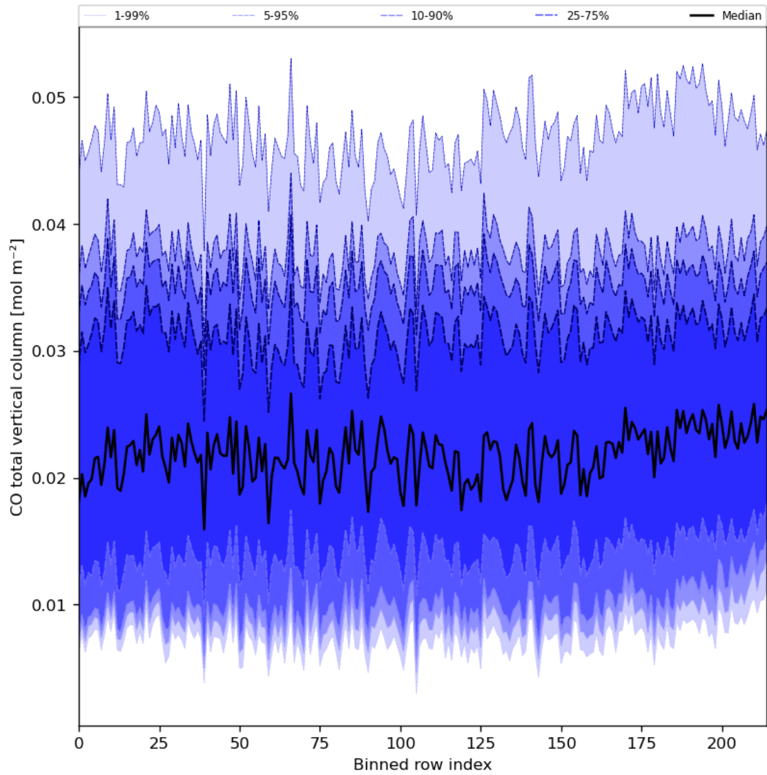
Figure 26: Along track statistics of “CO total vertical column” for 2023-12-20 to 2023-12-21
