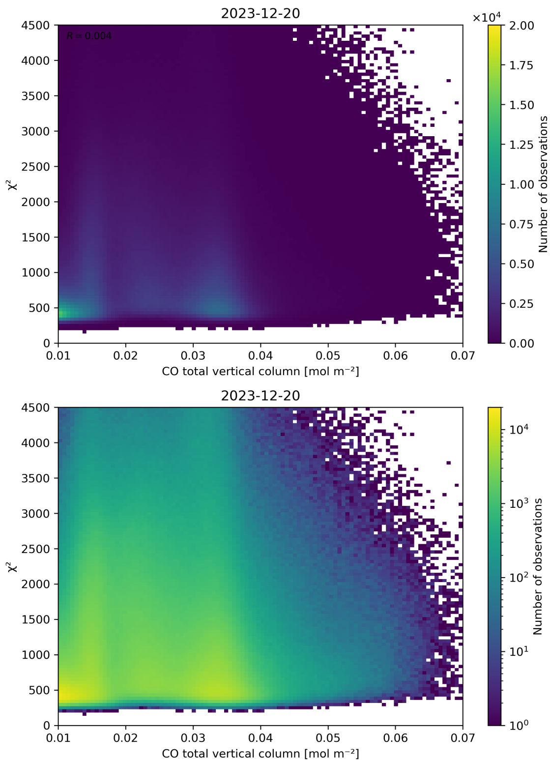
Figure 35: Scatter density plot of “CO total vertical column” against “ \chi^2 ” for 2023-12-20 to 2023-12-21.
