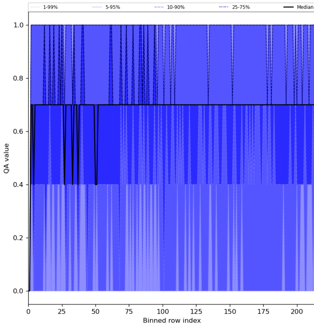
Figure 25: Along track statistics of “QA value” for 2023-12-20 to 2023-12-21
