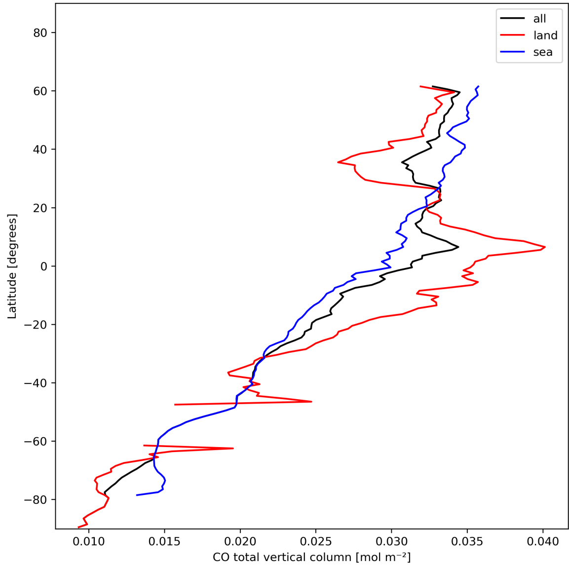
Figure 10: Zonal average of “CO total vertical column” for 2023-12-20 to 2023-12-21.
