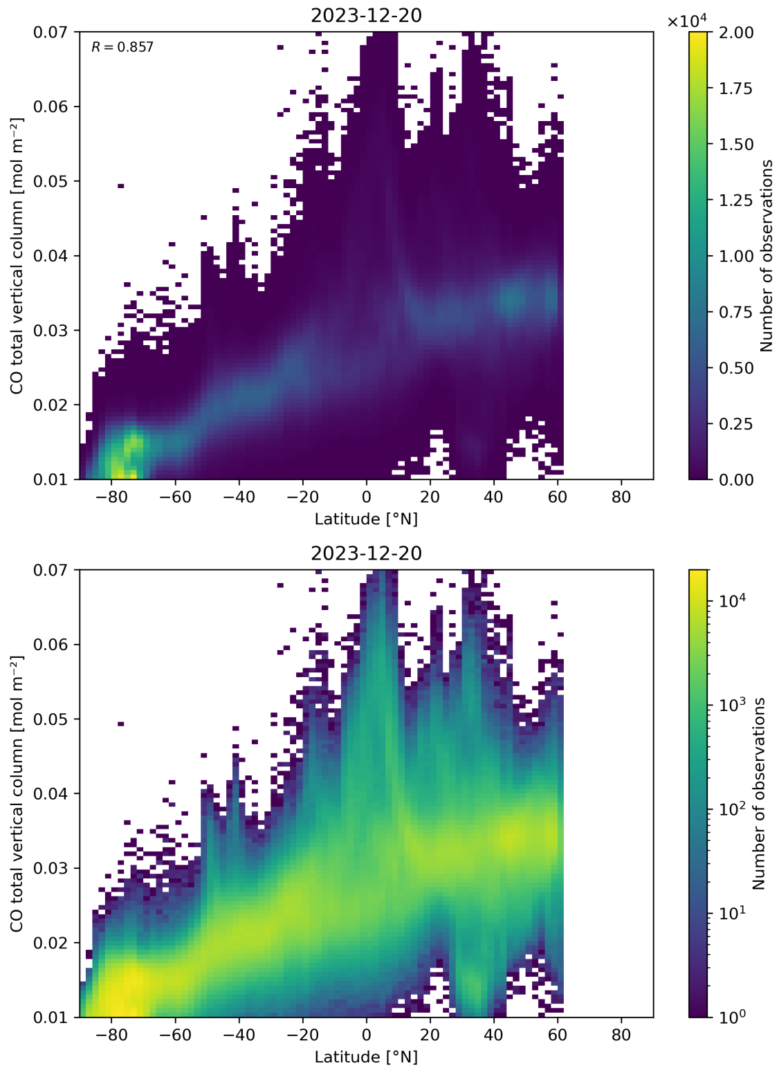
Figure 51: Scatter density plot of “Latitude” against “CO total vertical column” for 2023-12-20 to 2023-12-21.
