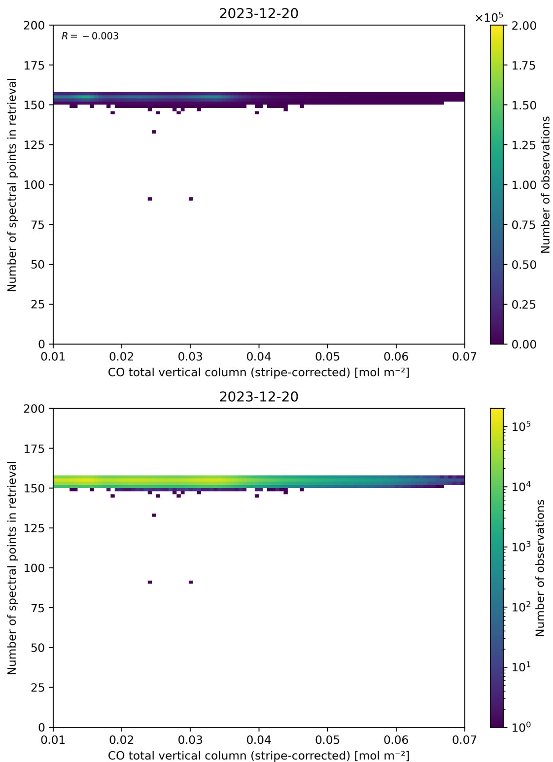
Figure 40: Scatter density plot of “CO total vertical column (stripe-corrected)” against “Number of spectral points in retrieval” for 2023-12-20 to 2023-12-21.
