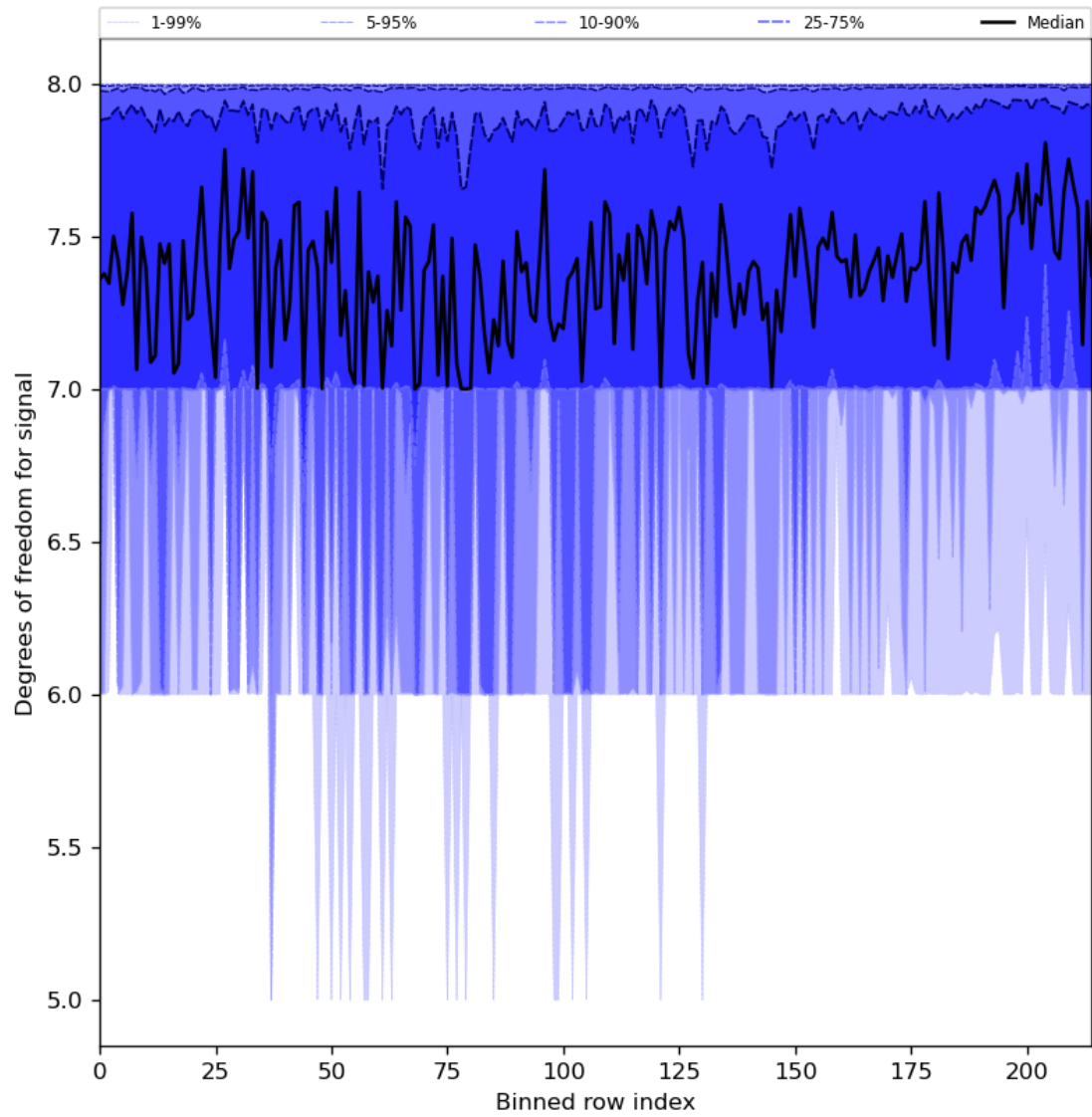
Figure 31: Along track statistics of “Degrees of freedom for signal” for 2023-12-20 to 2023-12-21
