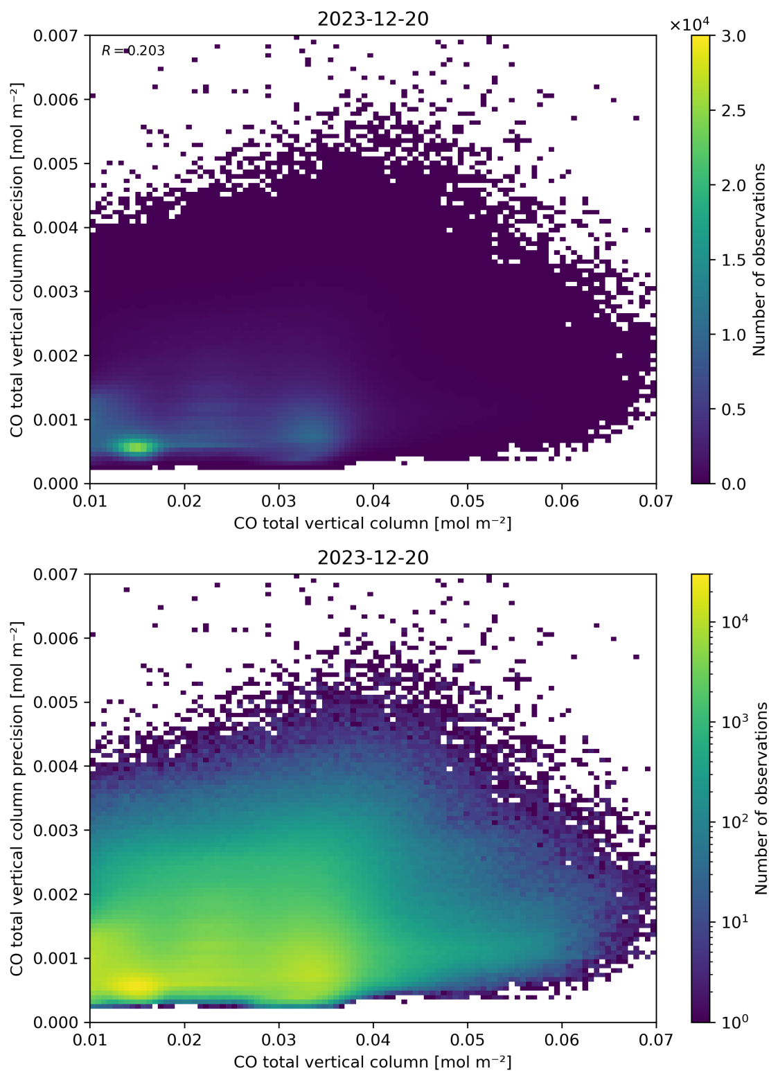
Figure 34: Scatter density plot of “CO total vertical column” against “CO total vertical column precision” for 2023-12-20 to 2023-12-21.
