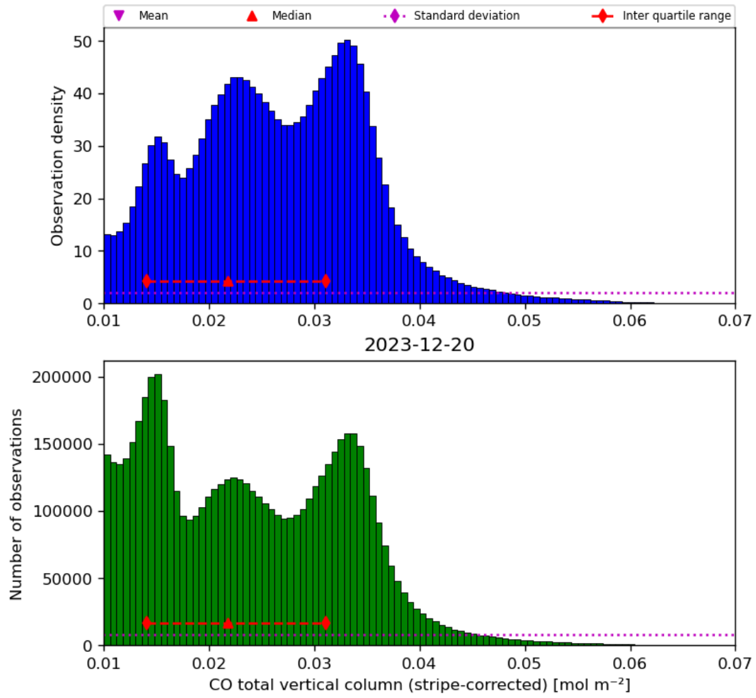
Figure 19: Histogram of “CO total vertical column (stripe-corrected)” for 2023-12-20 to 2023-12-21
