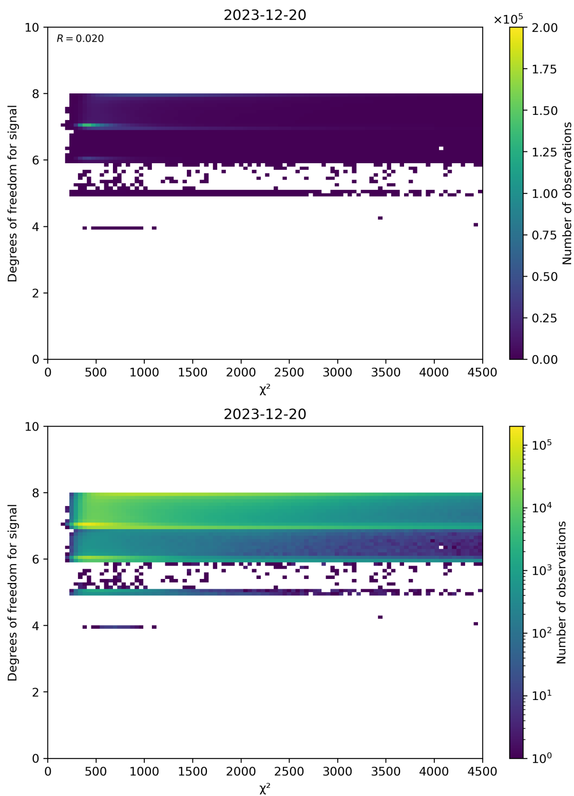
Figure 48: Scatter density plot of “ \chi^2 ” against “Degrees of freedom for signal” for 2023-12-20 to 2023-12-21.
