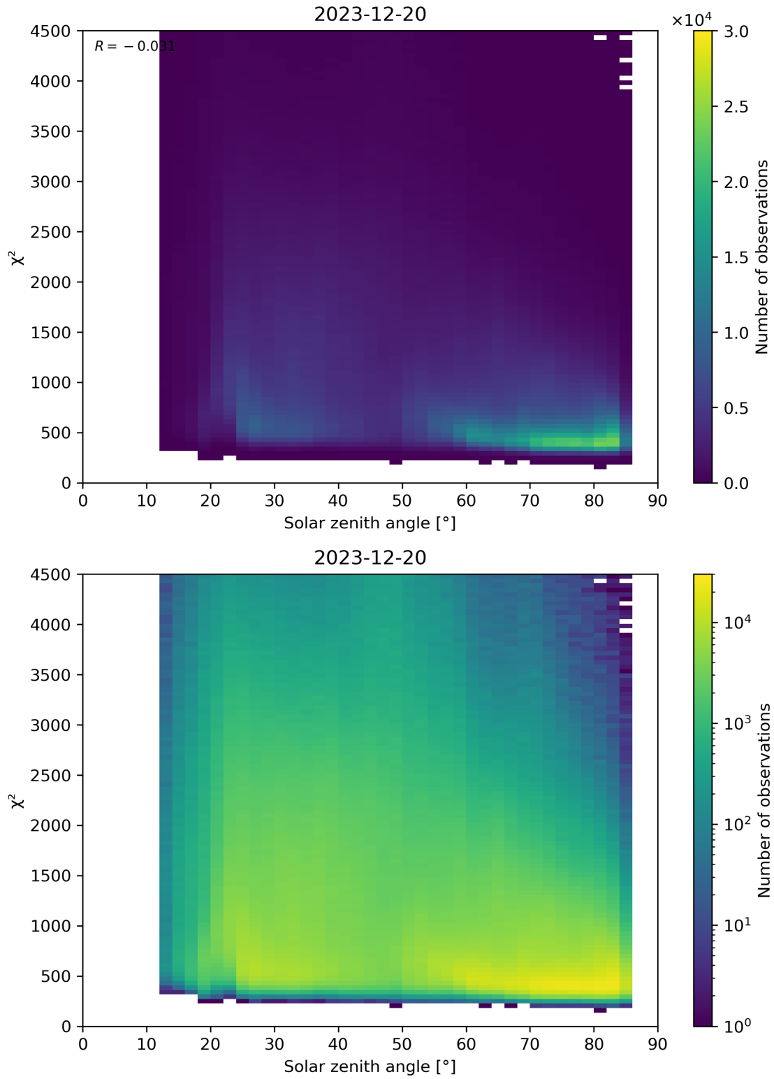
Figure 64: Scatter density plot of “Solar zenith angle” against “ \chi^2 ” for 2023-12-20 to 2023-12-21.
