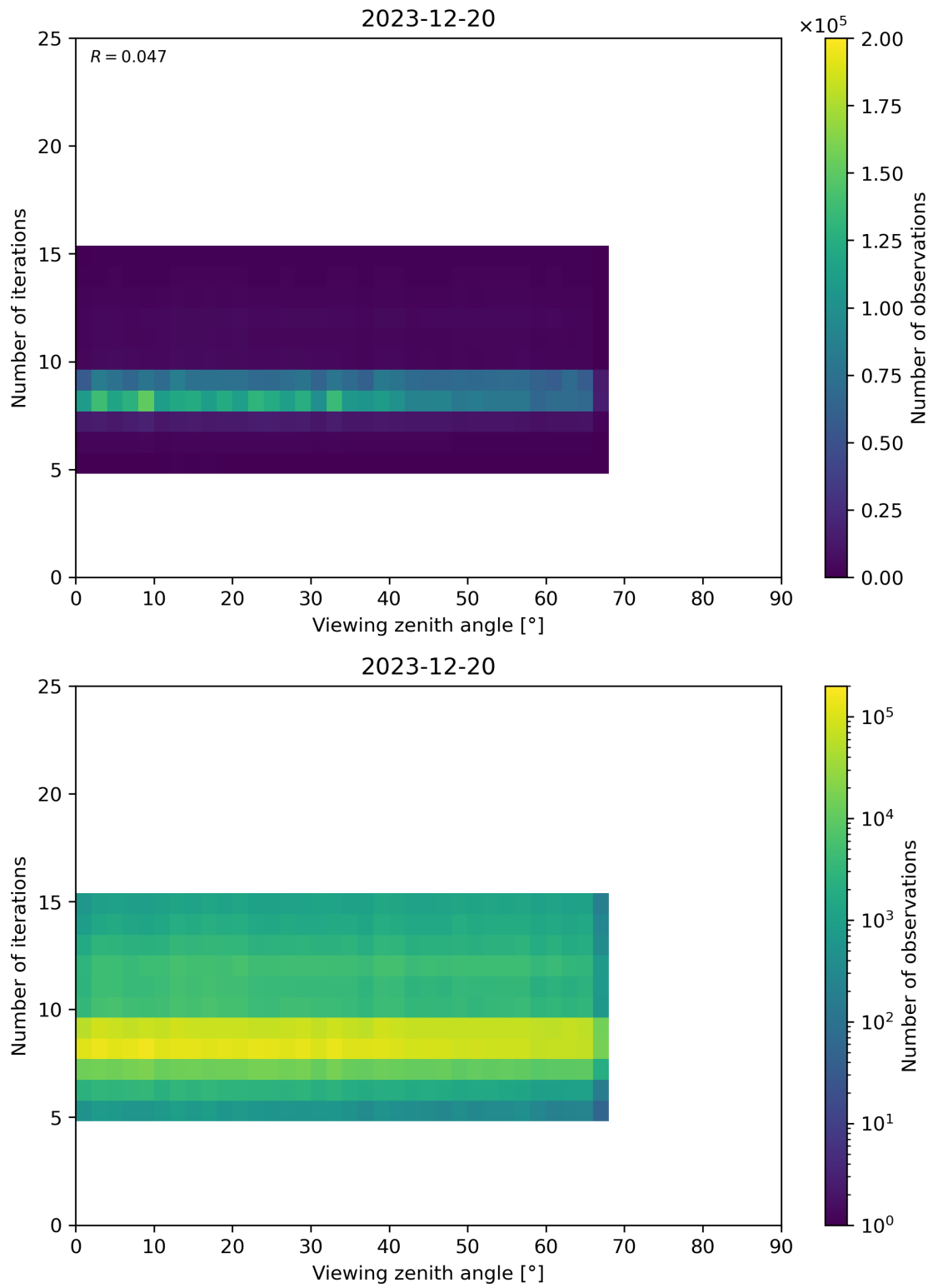
Figure 75: Scatter density plot of “Viewing zenith angle” against “Number of iterations” for 2023-12-20 to 2023-12-21.
