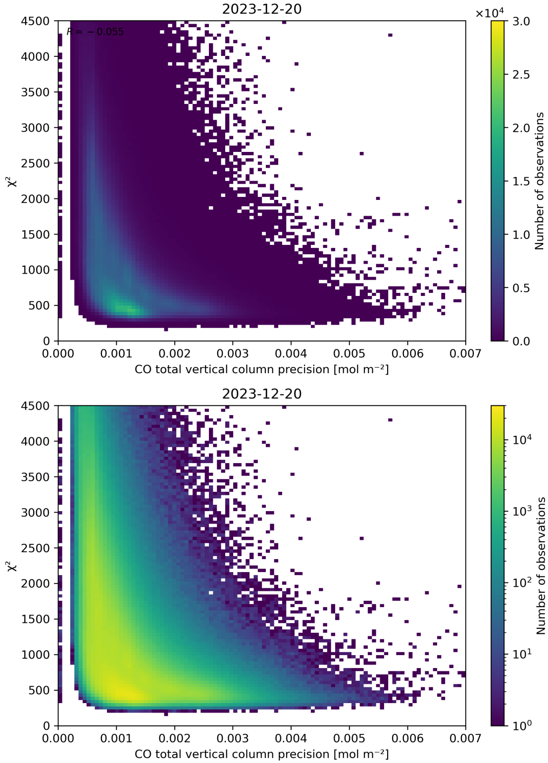
Figure 44: Scatter density plot of “CO total vertical column precision” against “ \chi^2 ” for 2023-12-20 to 2023-12-21.
