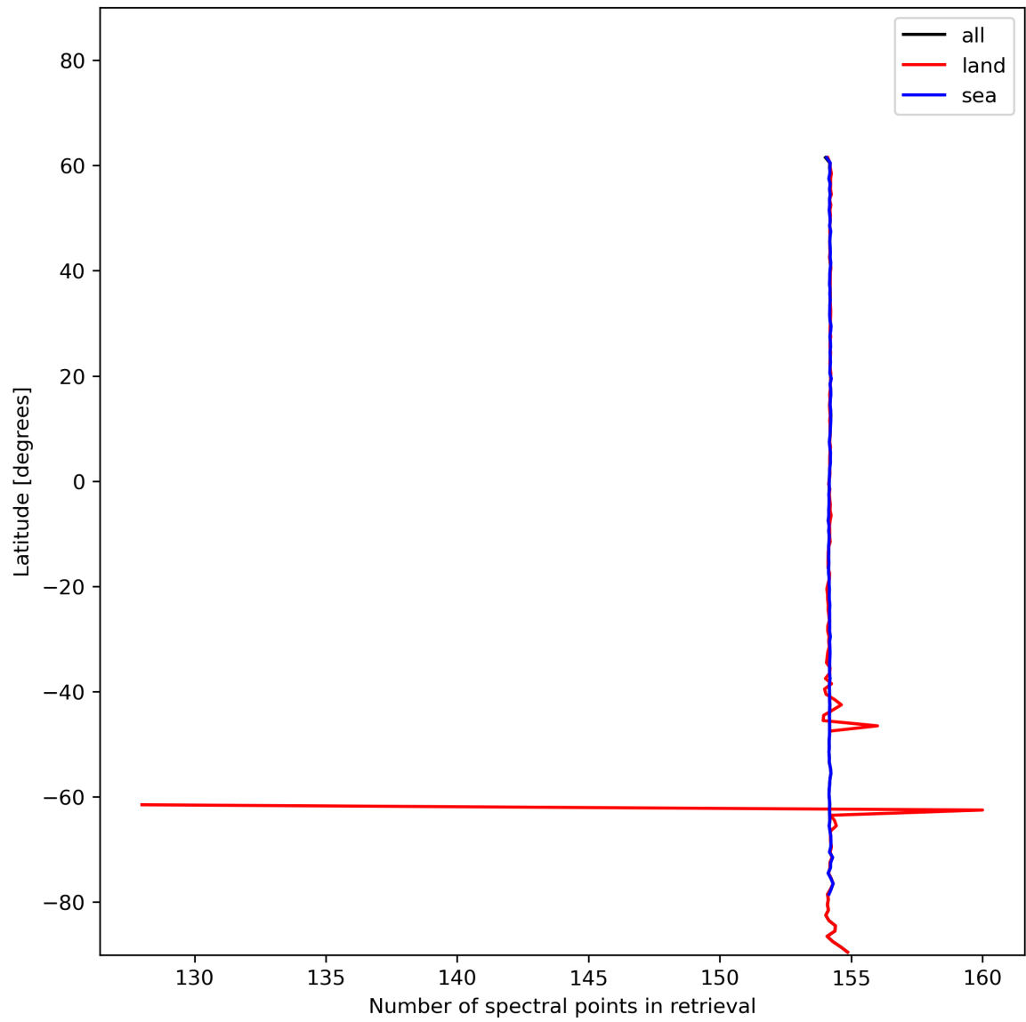
Figure 13: Zonal average of “Number of spectral points in retrieval” for 2023-12-20 to 2023-12-21.
