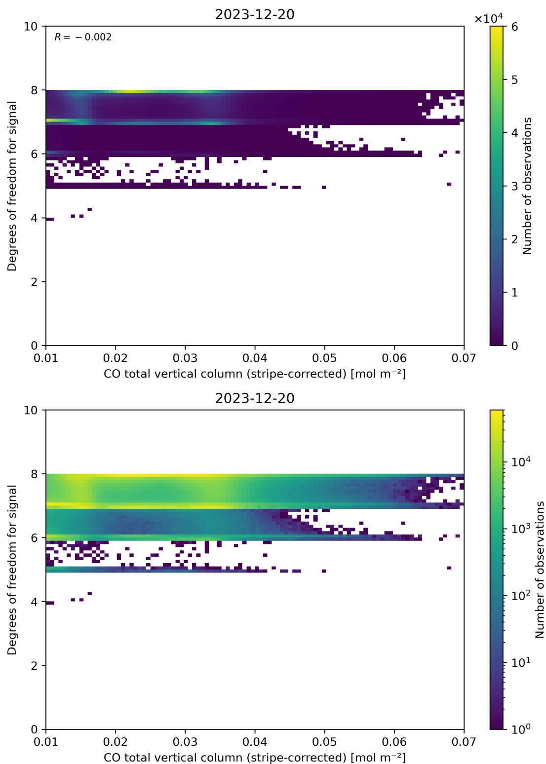
Figure 38: Scatter density plot of “CO total vertical column (stripe-corrected)” against “Degrees of freedom for signal” for 2023-12-20 to 2023-12-21.
