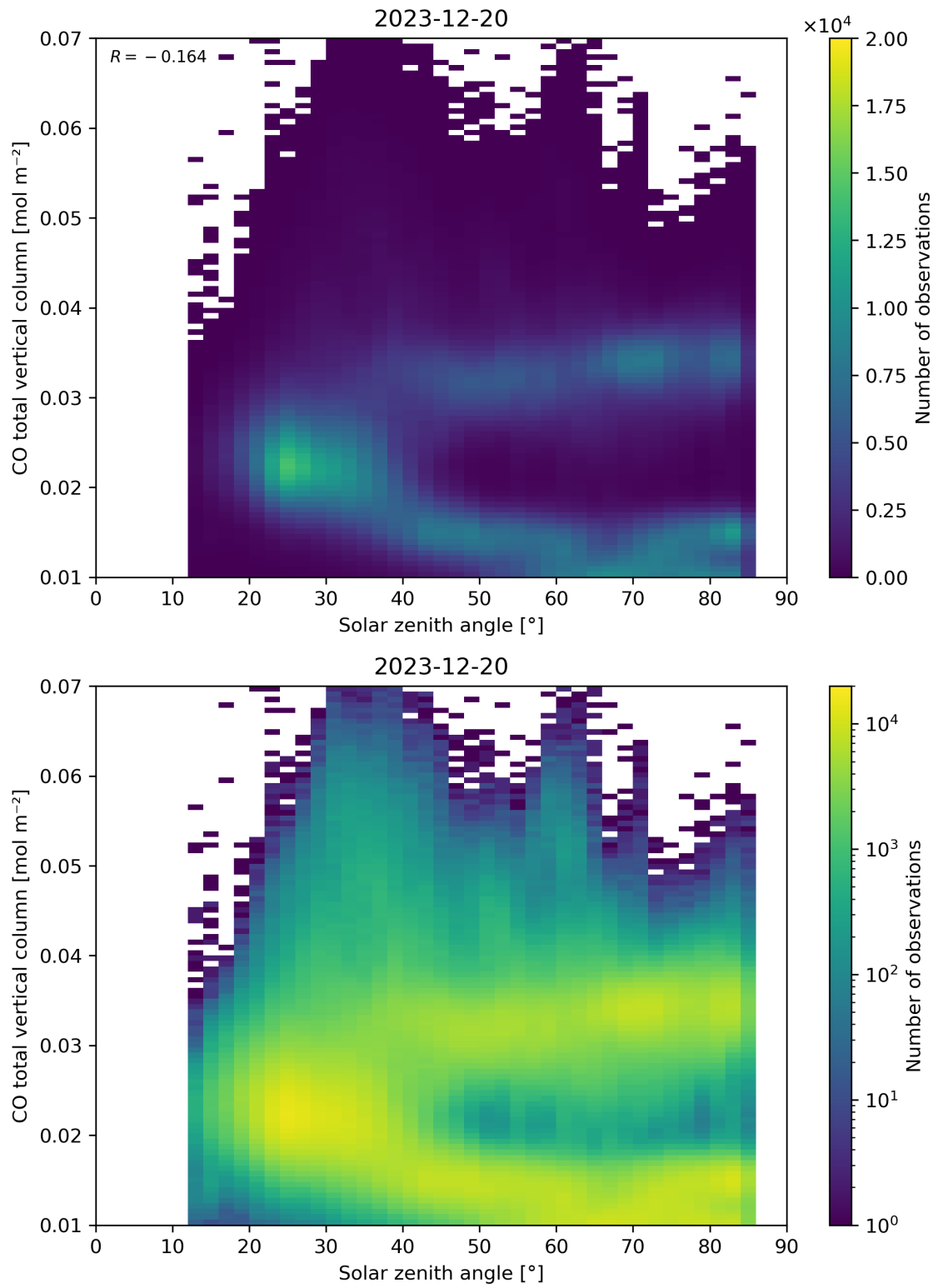
Figure 61: Scatter density plot of “Solar zenith angle” against “CO total vertical column” for 2023-12-20 to 2023-12-21.
