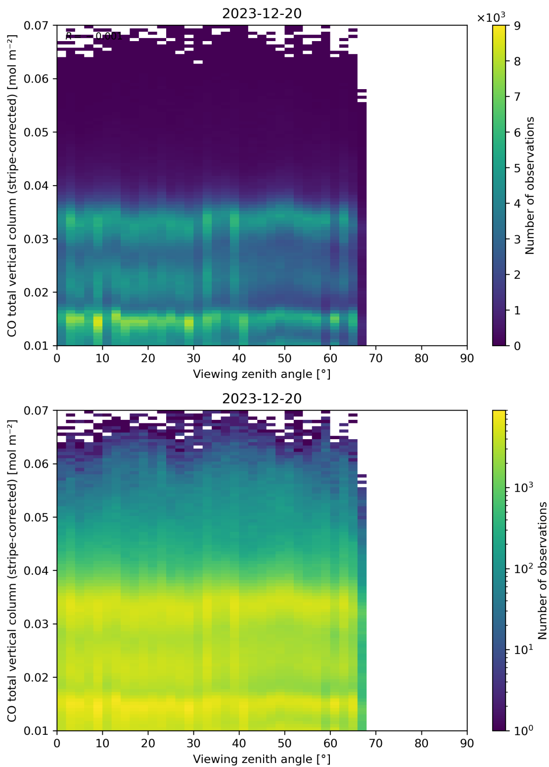
Figure 70: Scatter density plot of “Viewing zenith angle” against “CO total vertical column (stripe-corrected)” for 2023-12-20 to 2023-12-21.
