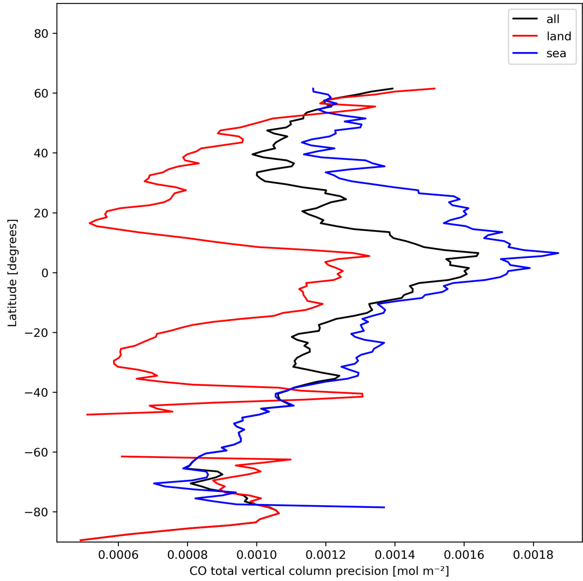
Figure 12: Zonal average of “CO total vertical column precision” for 2023-12-20 to 2023-12-21.
