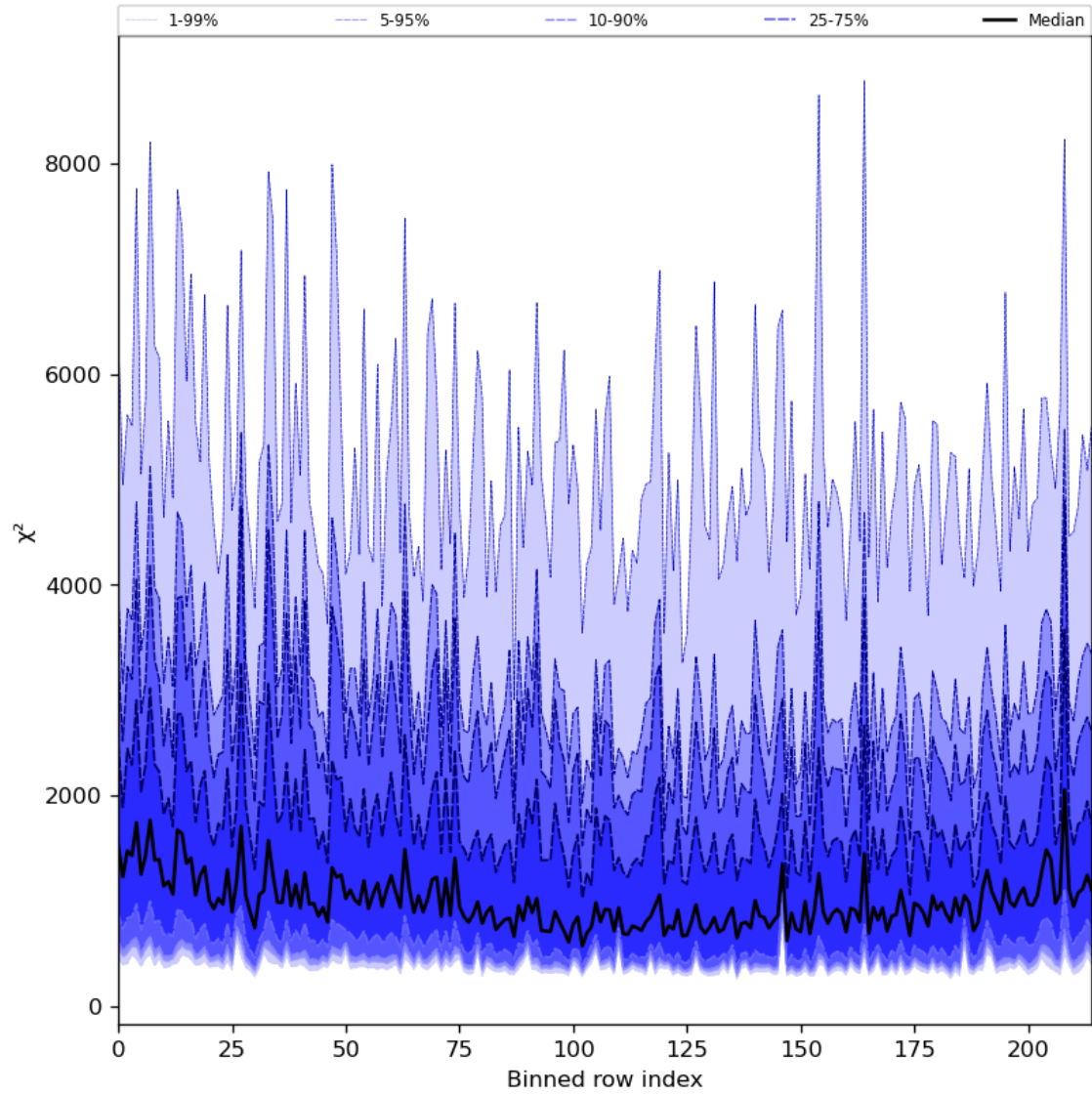
Figure 30: Along track statistics of “ \chi^2 ” for 2023-12-20 to 2023-12-21
