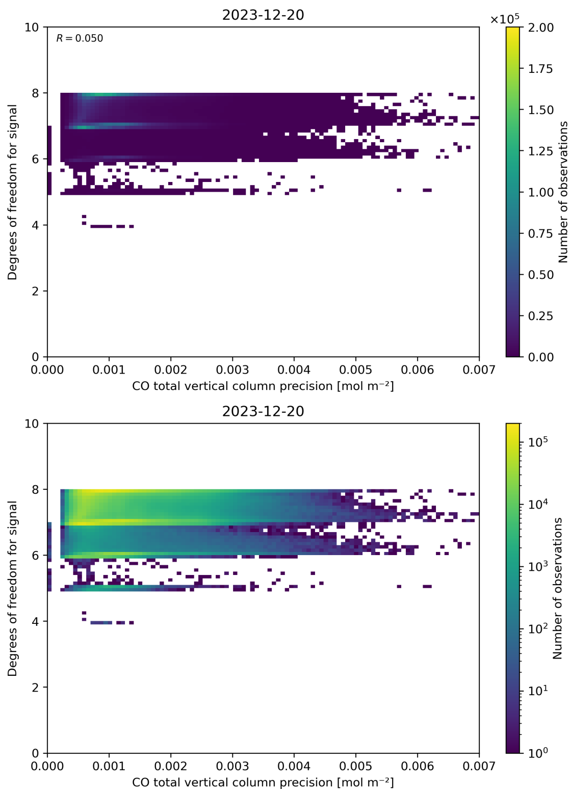
Figure 45: Scatter density plot of “CO total vertical column precision” against “Degrees of freedom for signal” for 2023-12-20 to 2023-12-21.
