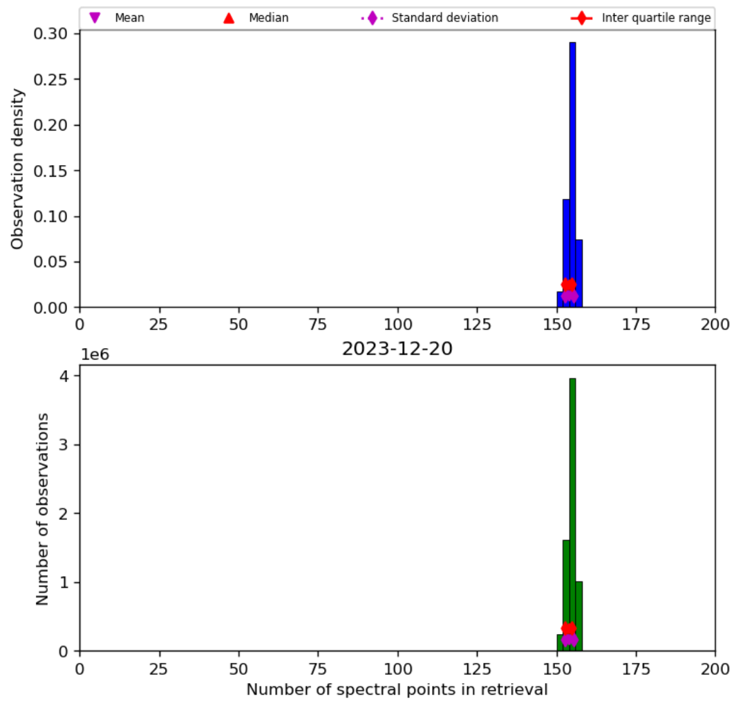
Figure 21: Histogram of “Number of spectral points in retrieval” for 2023-12-20 to 2023-12-21
