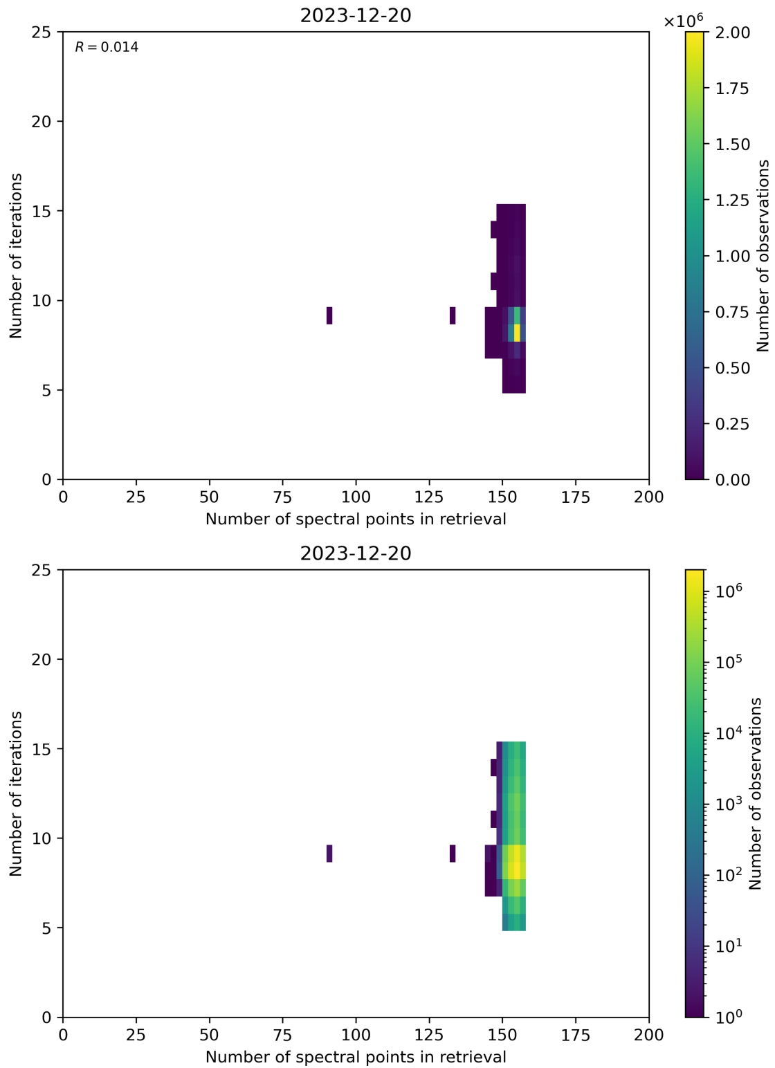
Figure 60: Scatter density plot of “Number of spectral points in retrieval” against “Number of iterations” for 2023-12-20 to 2023-12-21.
