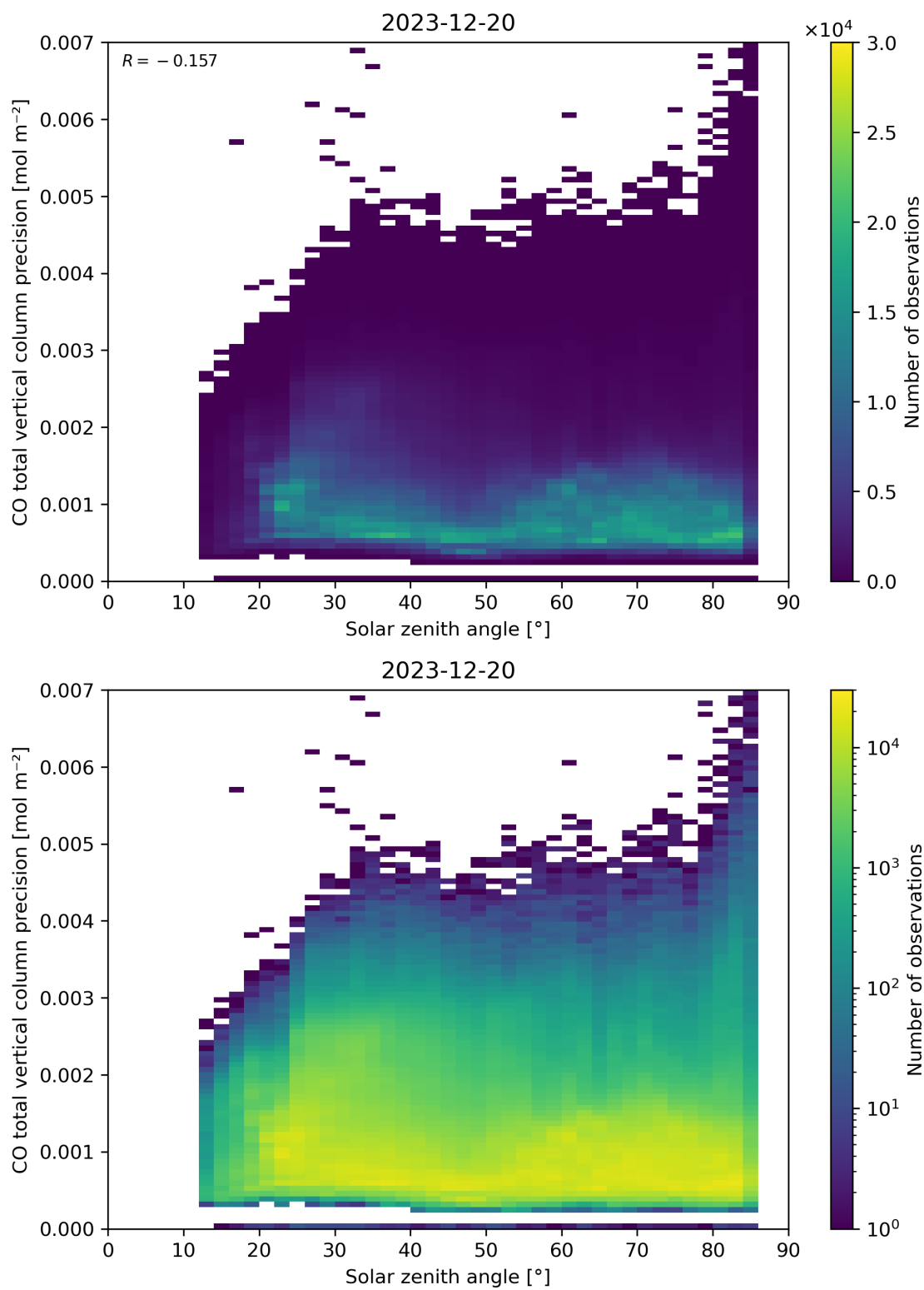
Figure 63: Scatter density plot of “Solar zenith angle” against “CO total vertical column precision” for 2023-12-20 to 2023-12-21.
