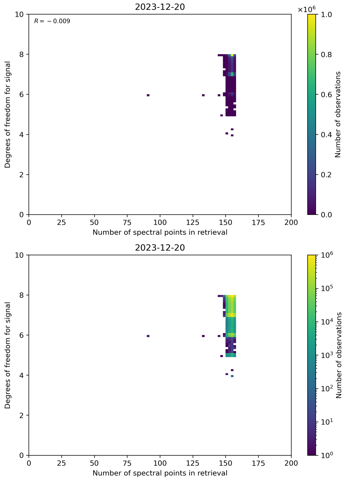
Figure 59: Scatter density plot of “Number of spectral points in retrieval” against “Degrees of freedom for signal” for 2023-12-20 to 2023-12-21.
