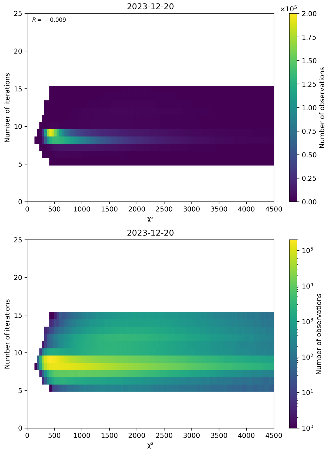
Figure 49: Scatter density plot of “ \chi^2 ” against “Number of iterations” for 2023-12-20 to 2023-12-21.
