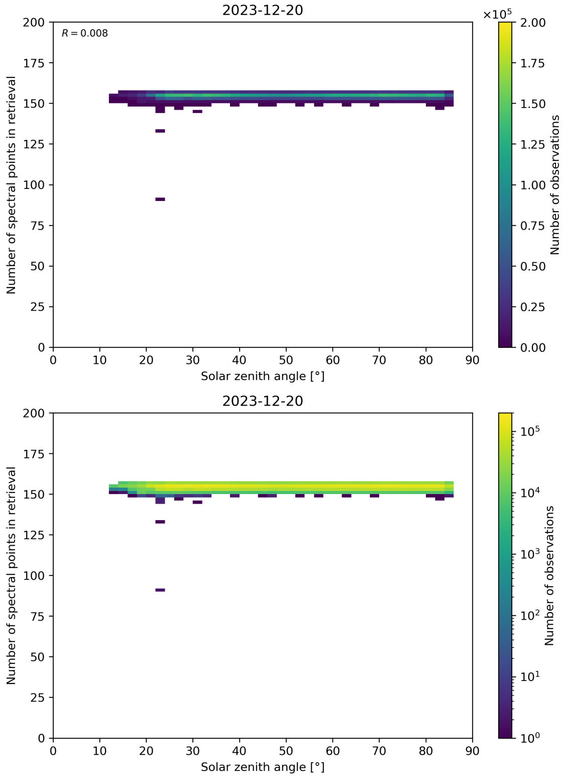
Figure 68: Scatter density plot of “Solar zenith angle” against “Number of spectral points in retrieval” for 2023-12-20 to 2023-12-21.
