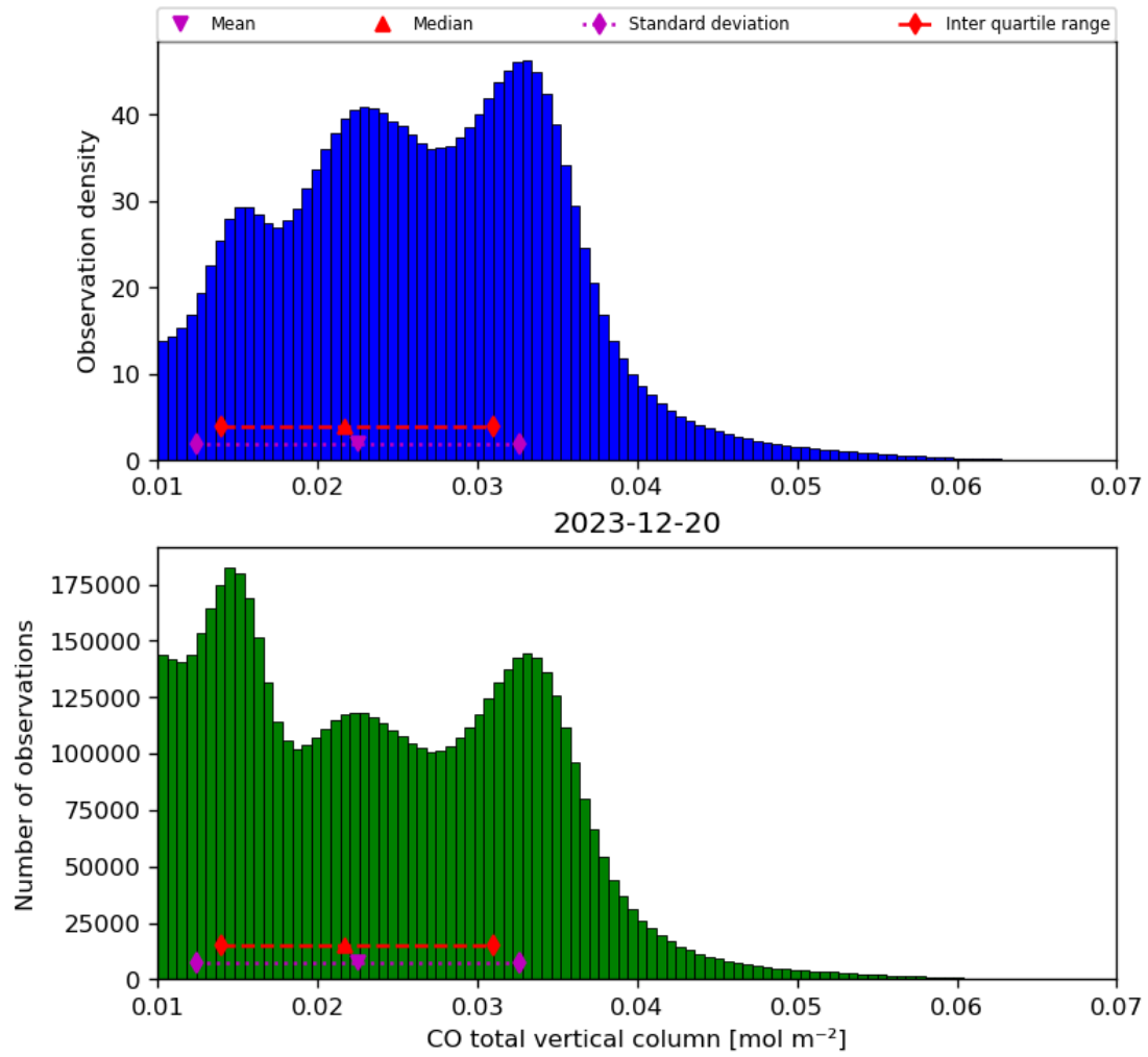
Figure 18: Histogram of “CO total vertical column” for 2023-12-20 to 2023-12-21
