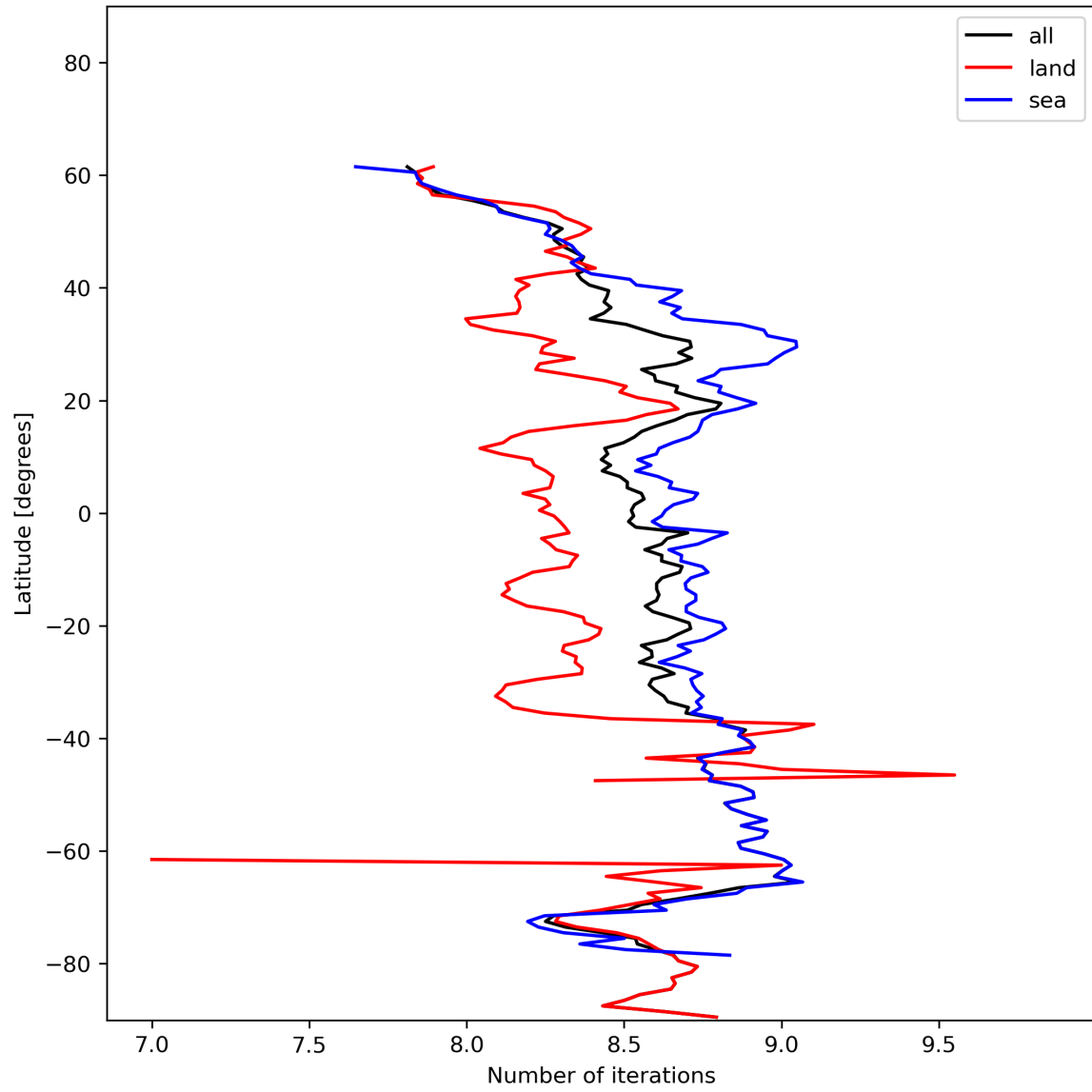
Figure 16: Zonal average of “Number of iterations” for 2023-12-20 to 2023-12-21.
