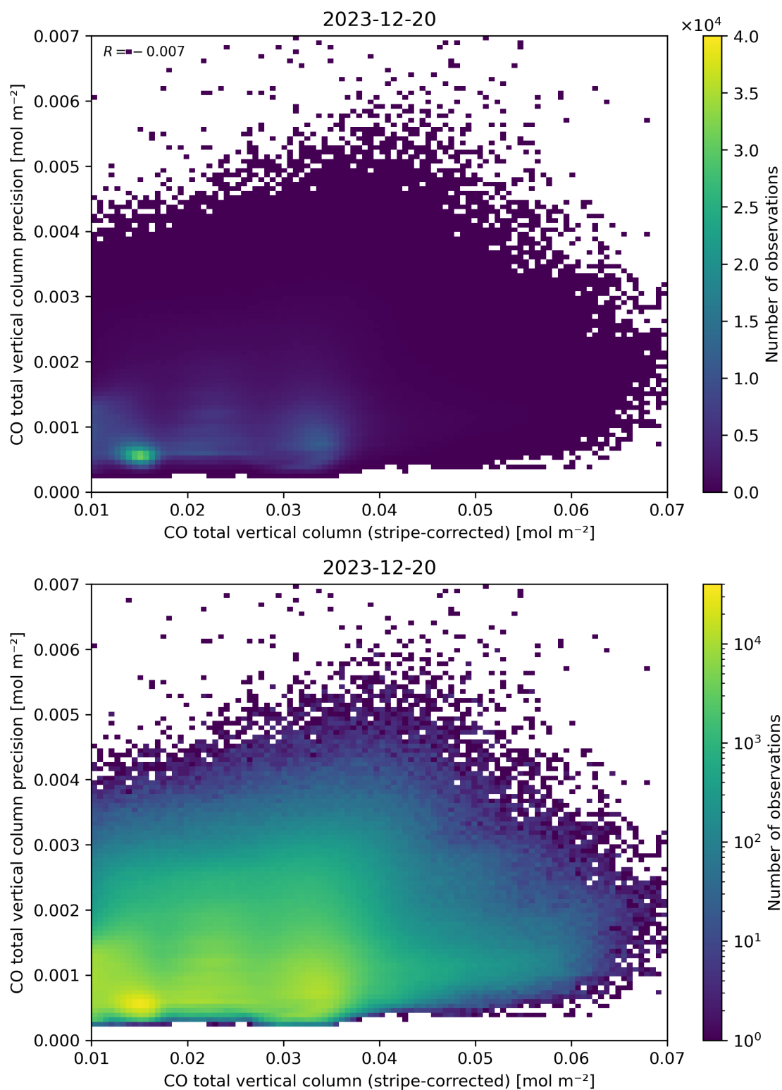
Figure 36: Scatter density plot of “CO total vertical column (stripe-corrected)” against “CO total vertical column precision” for 2023-12-20 to 2023-12-21.
