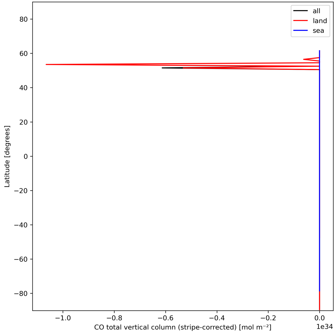
Figure 11: Zonal average of “CO total vertical column (stripe-corrected)” for 2023-12-20 to 2023-12-21.
