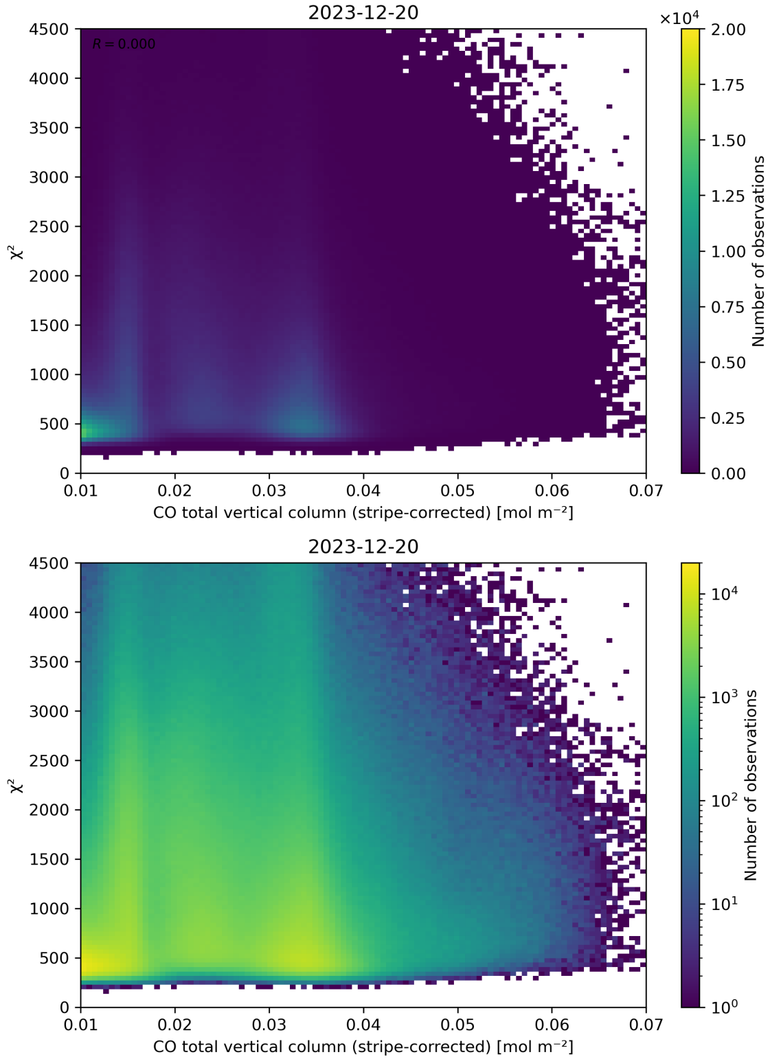
Figure 37: Scatter density plot of “CO total vertical column (stripe-corrected)” against “ \chi^2 ” for 2023-12-20 to 2023-12-21.
