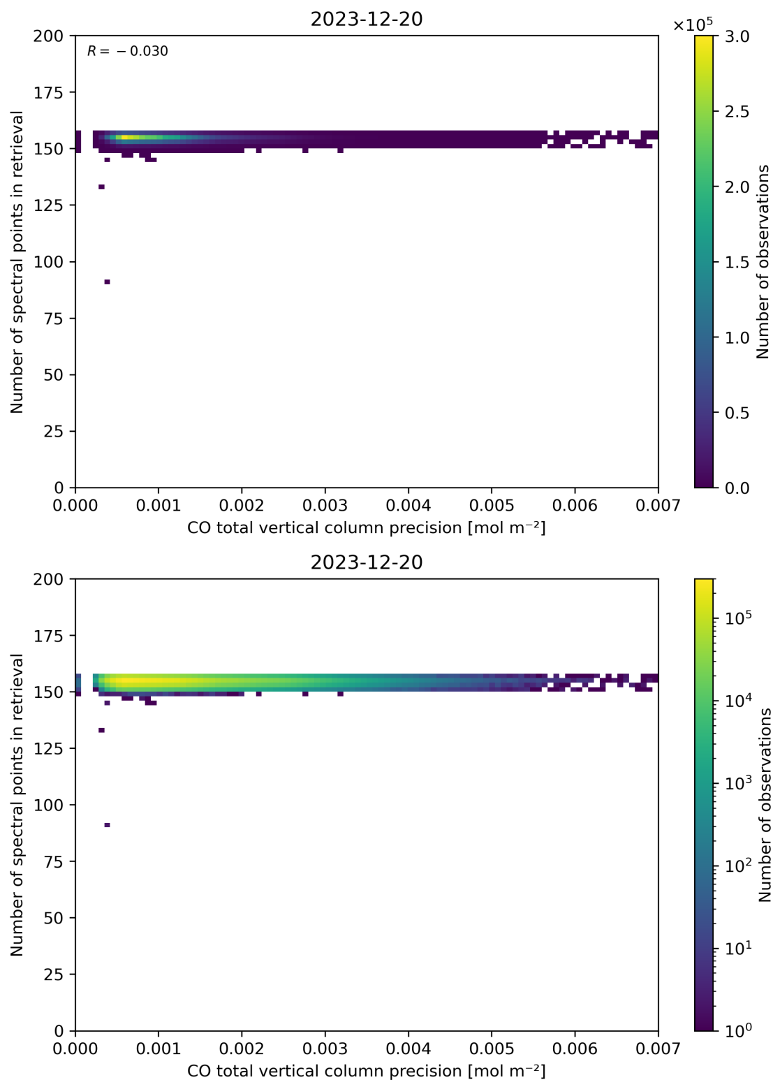
Figure 47: Scatter density plot of “CO total vertical column precision” against “Number of spectral points in retrieval” for 2023-12-20 to 2023-12-21.
