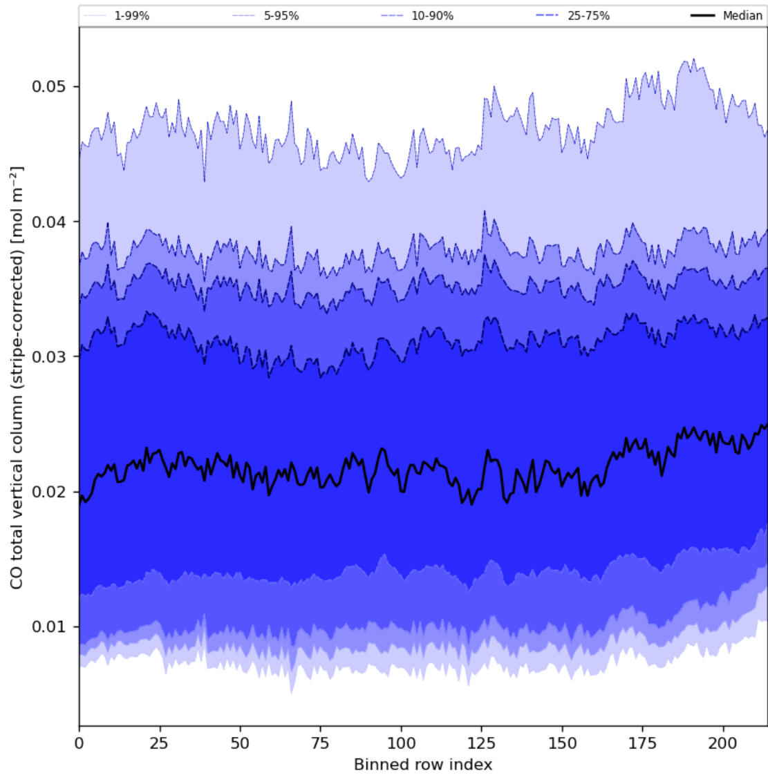
Figure 27: Along track statistics of “CO total vertical column (stripe-corrected)” for 2023-12-20 to 2023-12-21
