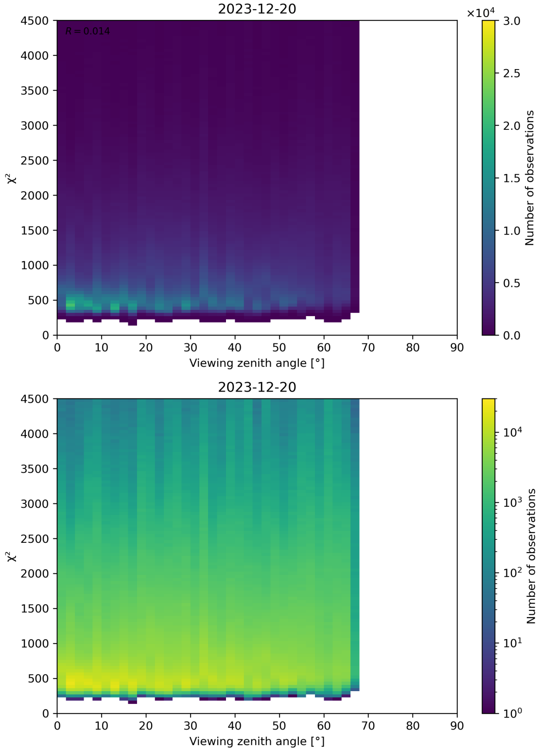
Figure 72: Scatter density plot of “Viewing zenith angle” against “ \chi^2 ” for 2023-12-20 to 2023-12-21.
