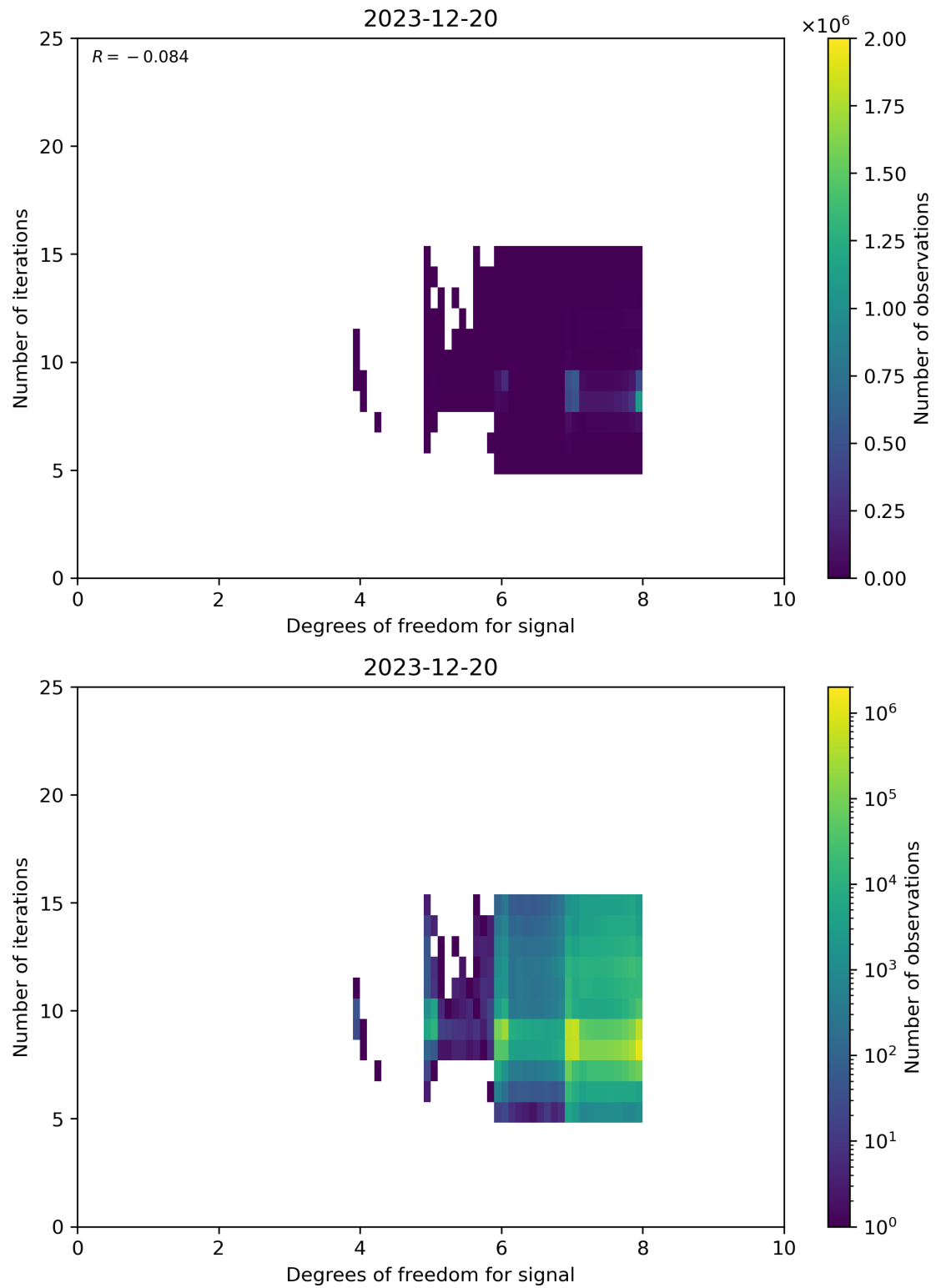
Figure 50: Scatter density plot of “Degrees of freedom for signal” against “Number of iterations” for 2023-12-20 to 2023-12-21.
