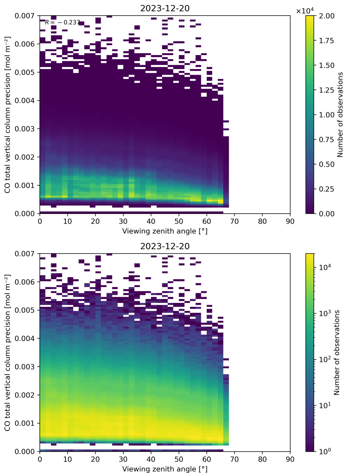
Figure 71: Scatter density plot of “Viewing zenith angle” against “CO total vertical column precision” for 2023-12-20 to 2023-12-21.
