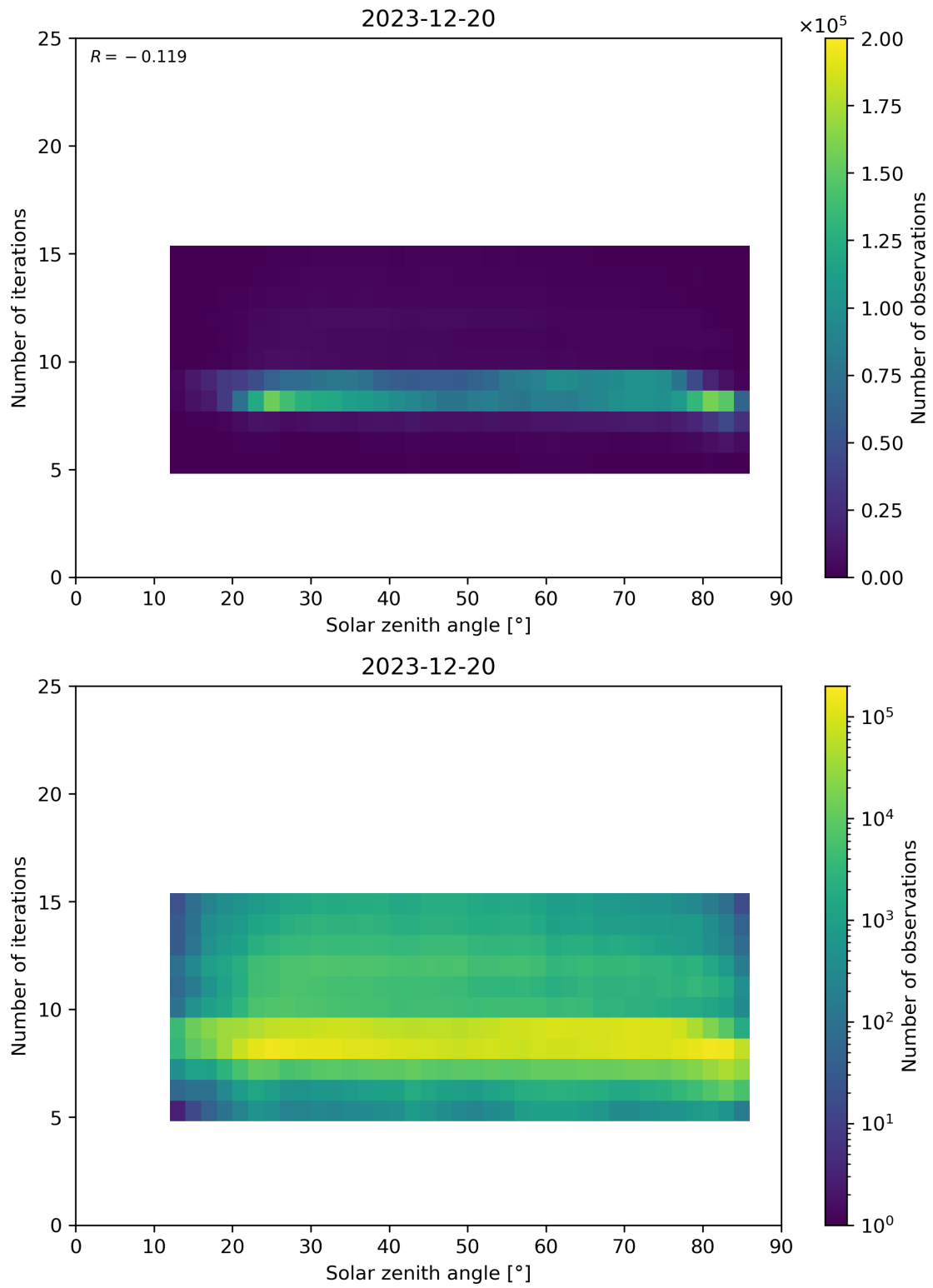
Figure 67: Scatter density plot of “Solar zenith angle” against “Number of iterations” for 2023-12-20 to 2023-12-21.
