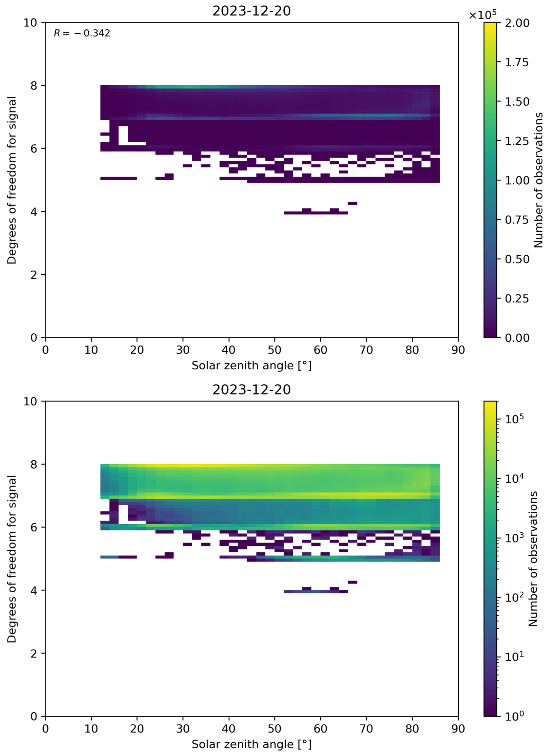
Figure 65: Scatter density plot of “Solar zenith angle” against “Degrees of freedom for signal” for 2023-12-20 to 2023-12-21.
