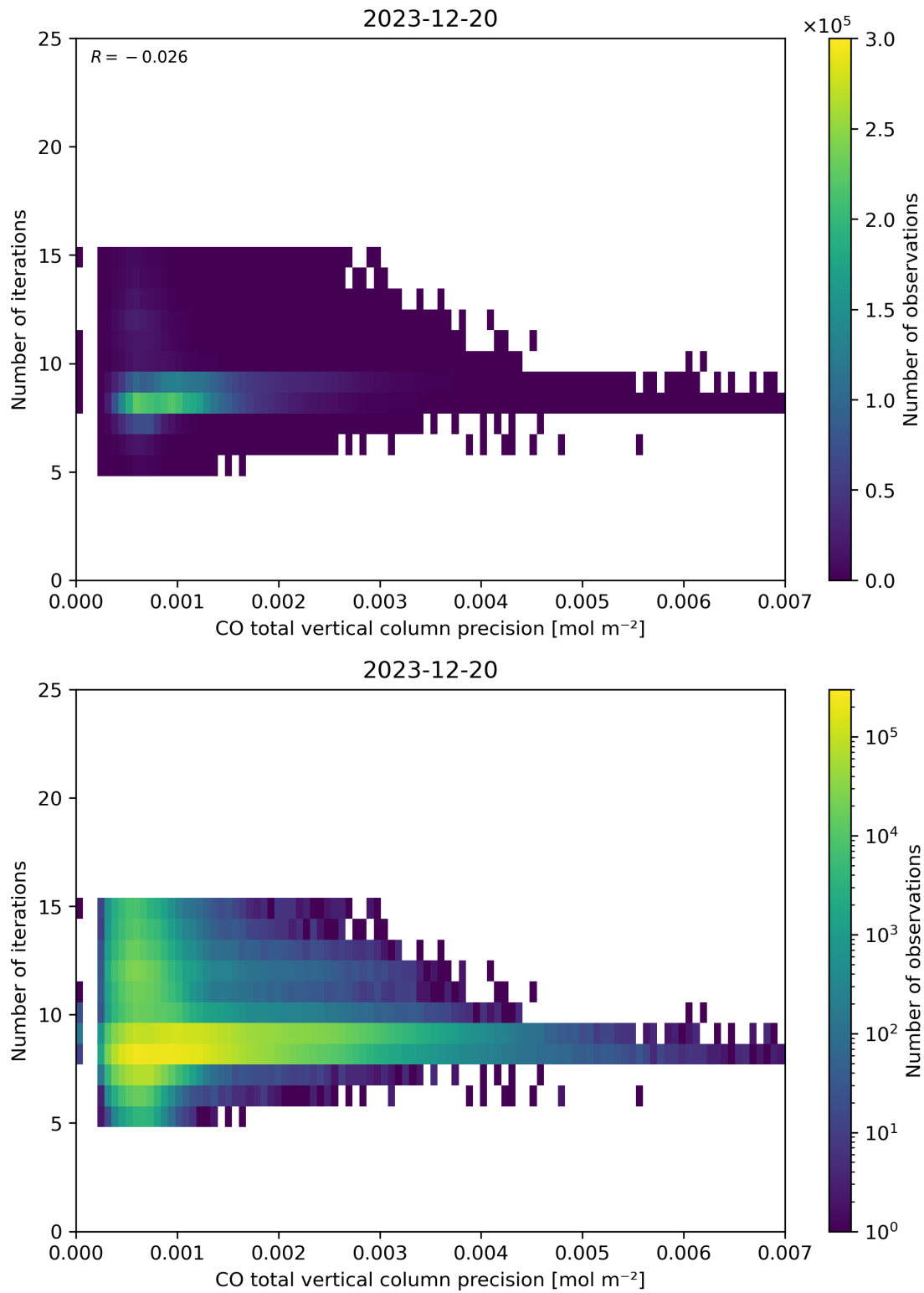
Figure 46: Scatter density plot of “CO total vertical column precision” against “Number of iterations” for 2023-12-20 to 2023-12-21.
