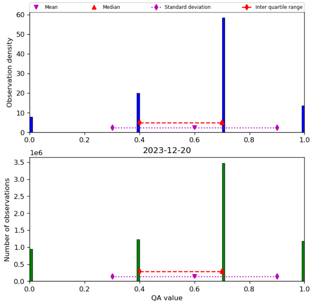
Figure 17: Histogram of “QA value” for 2023-12-20 to 2023-12-21
