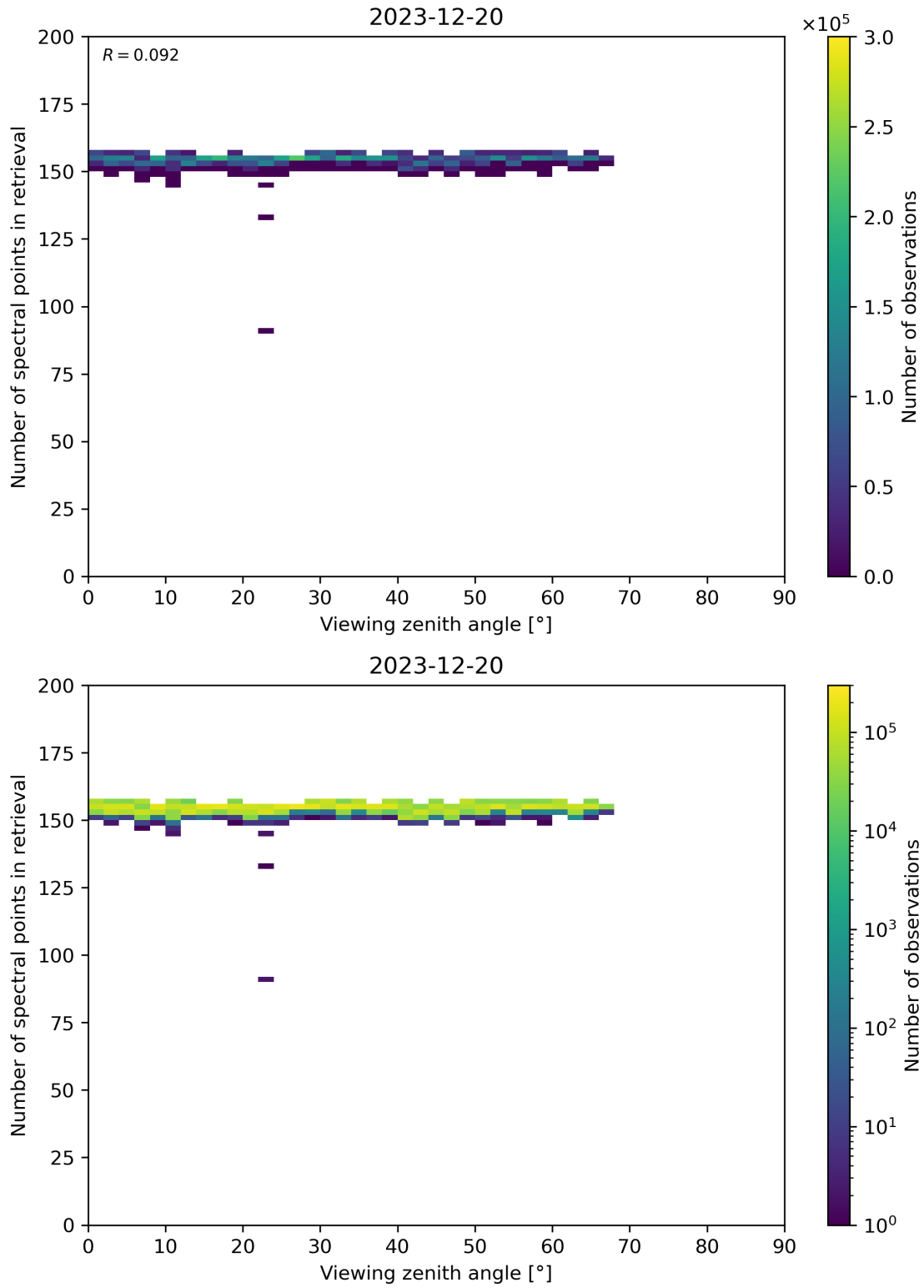
Figure 76: Scatter density plot of “Viewing zenith angle” against “Number of spectral points in retrieval” for 2023-12-20 to 2023-12-21.
