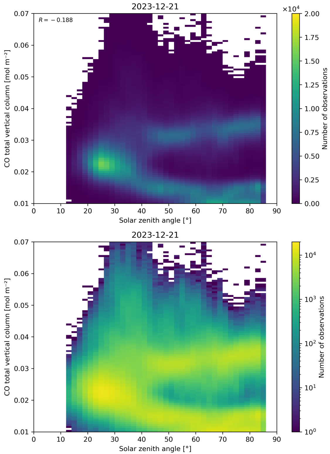
Figure 61: Scatter density plot of “Solar zenith angle” against “CO total vertical column” for 2023-12-20 to 2023-12-22.
