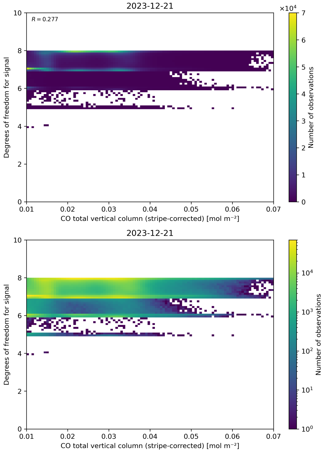
Figure 38: Scatter density plot of “CO total vertical column (stripe-corrected)” against “Degrees of freedom for signal” for 2023-12-20 to 2023-12-22.
