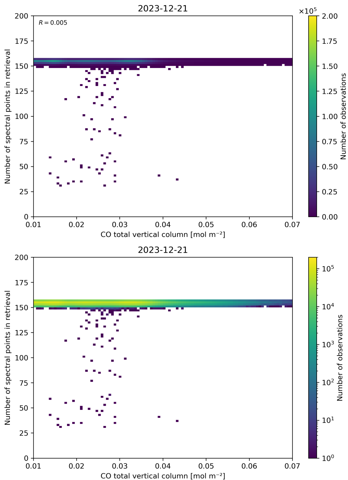
Figure 43: Scatter density plot of “CO total vertical column” against “Number of spectral points in retrieval” for 2023-12-20 to 2023-12-22.
