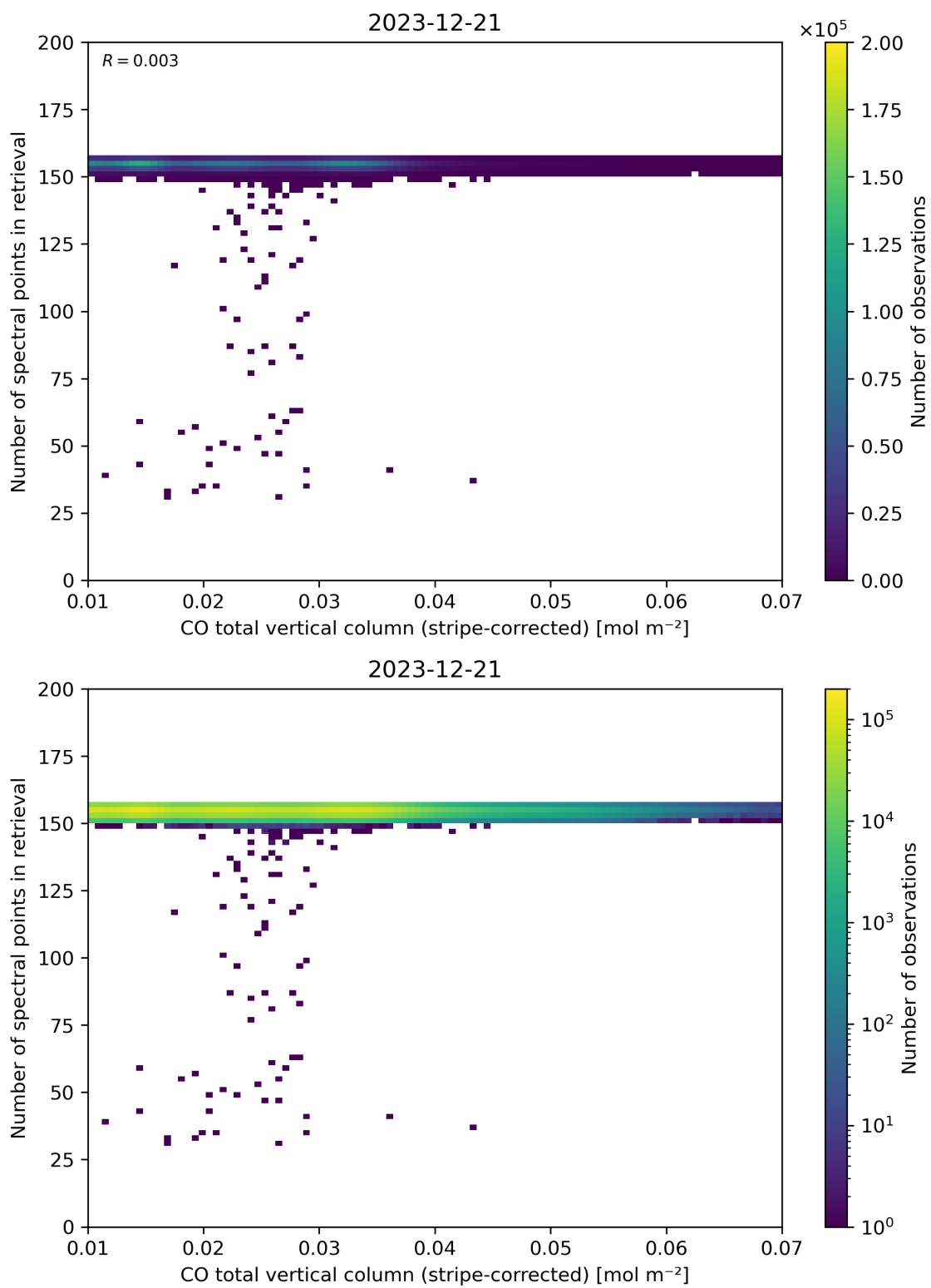
Figure 40: Scatter density plot of “CO total vertical column (stripe-corrected)” against “Number of spectral points in retrieval” for 2023-12-20 to 2023-12-22.
