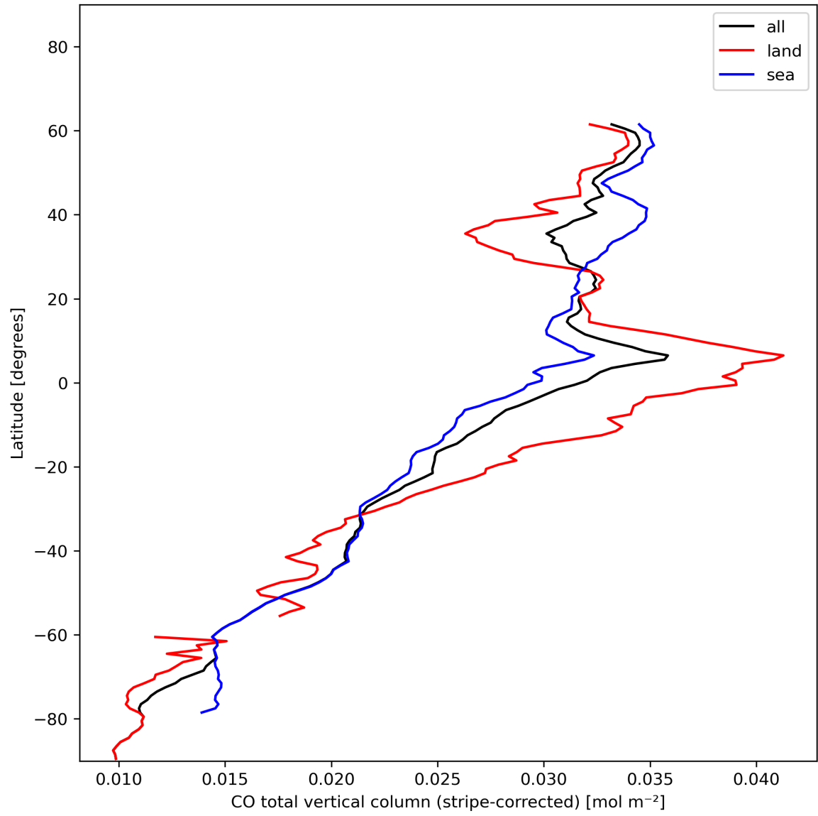
Figure 11: Zonal average of “CO total vertical column (stripe-corrected)” for 2023-12-20 to 2023-12-22.
