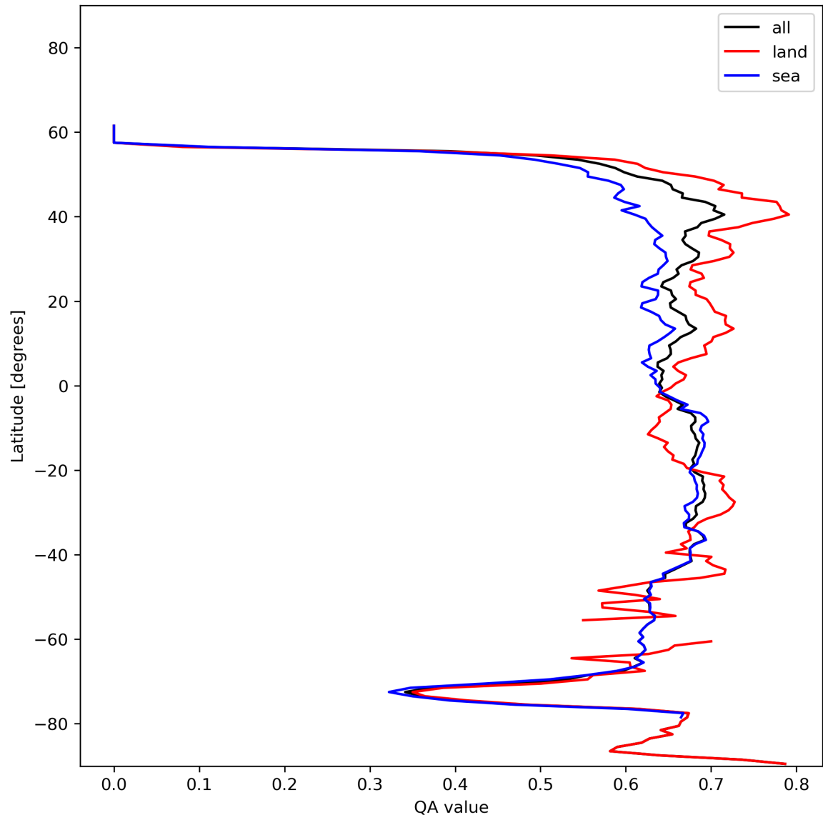
Figure 9: Zonal average of “QA value” for 2023-12-20 to 2023-12-22.
