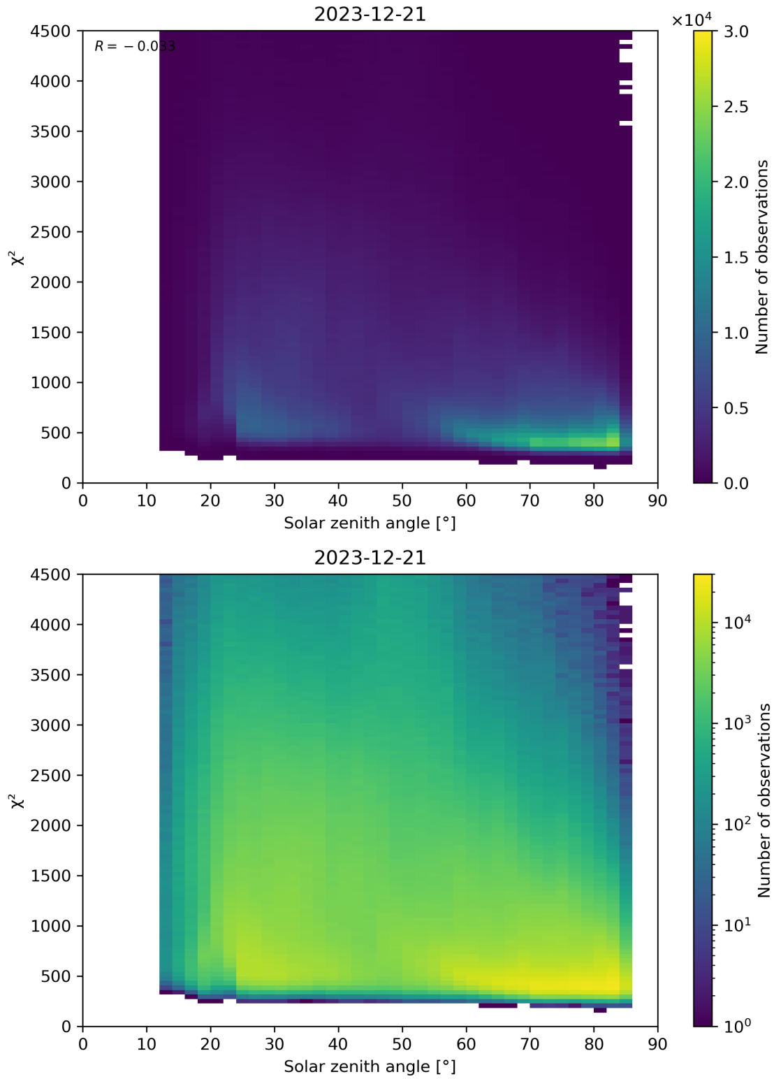
Figure 64: Scatter density plot of “Solar zenith angle” against “ \chi^2 ” for 2023-12-20 to 2023-12-22.
