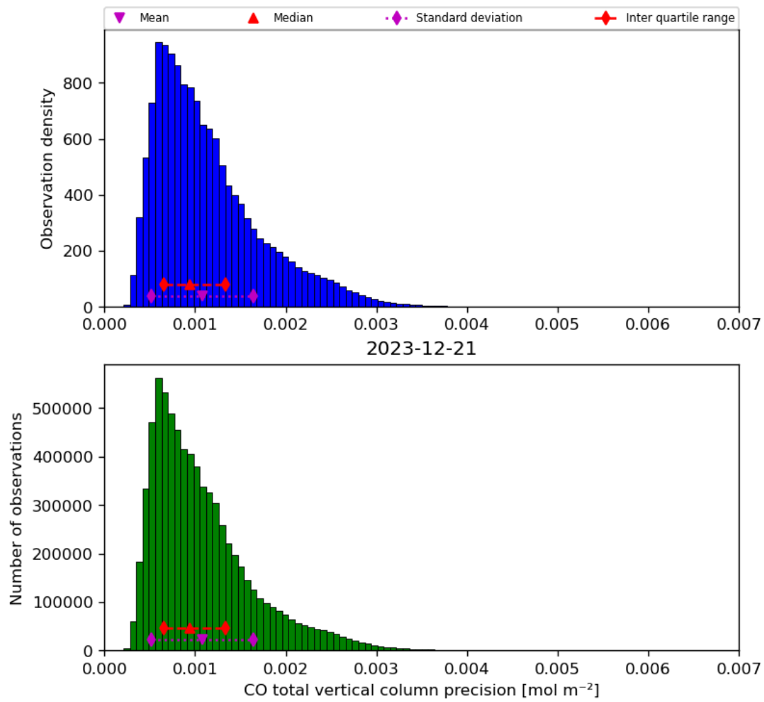
Figure 20: Histogram of “CO total vertical column precision” for 2023-12-20 to 2023-12-22
