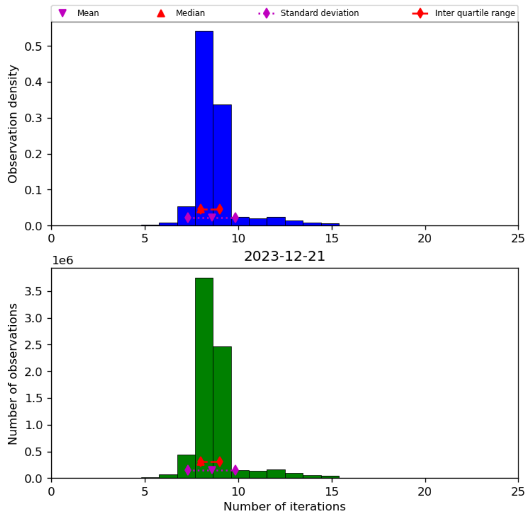
Figure 24: Histogram of “Number of iterations” for 2023-12-20 to 2023-12-22
