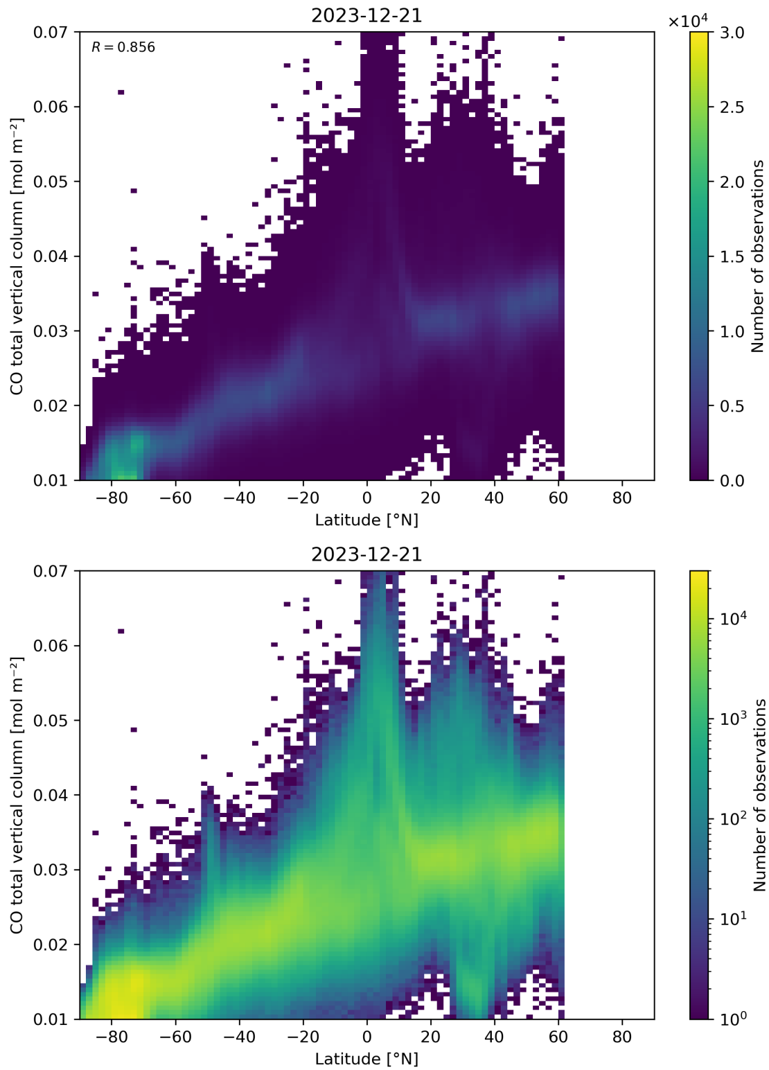
Figure 51: Scatter density plot of “Latitude” against “CO total vertical column” for 2023-12-20 to 2023-12-22.
