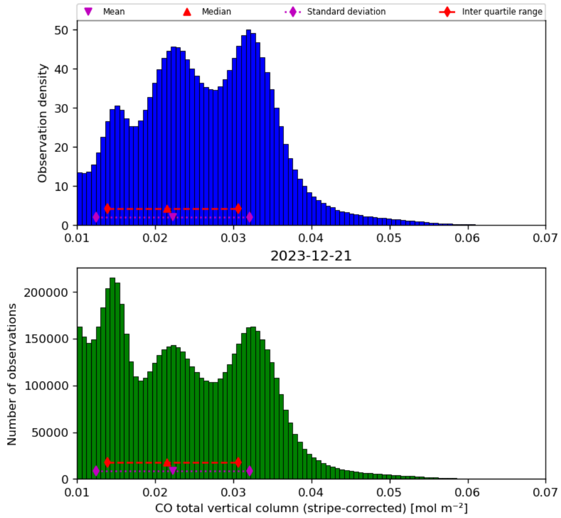
Figure 19: Histogram of “CO total vertical column (stripe-corrected)” for 2023-12-20 to 2023-12-22
