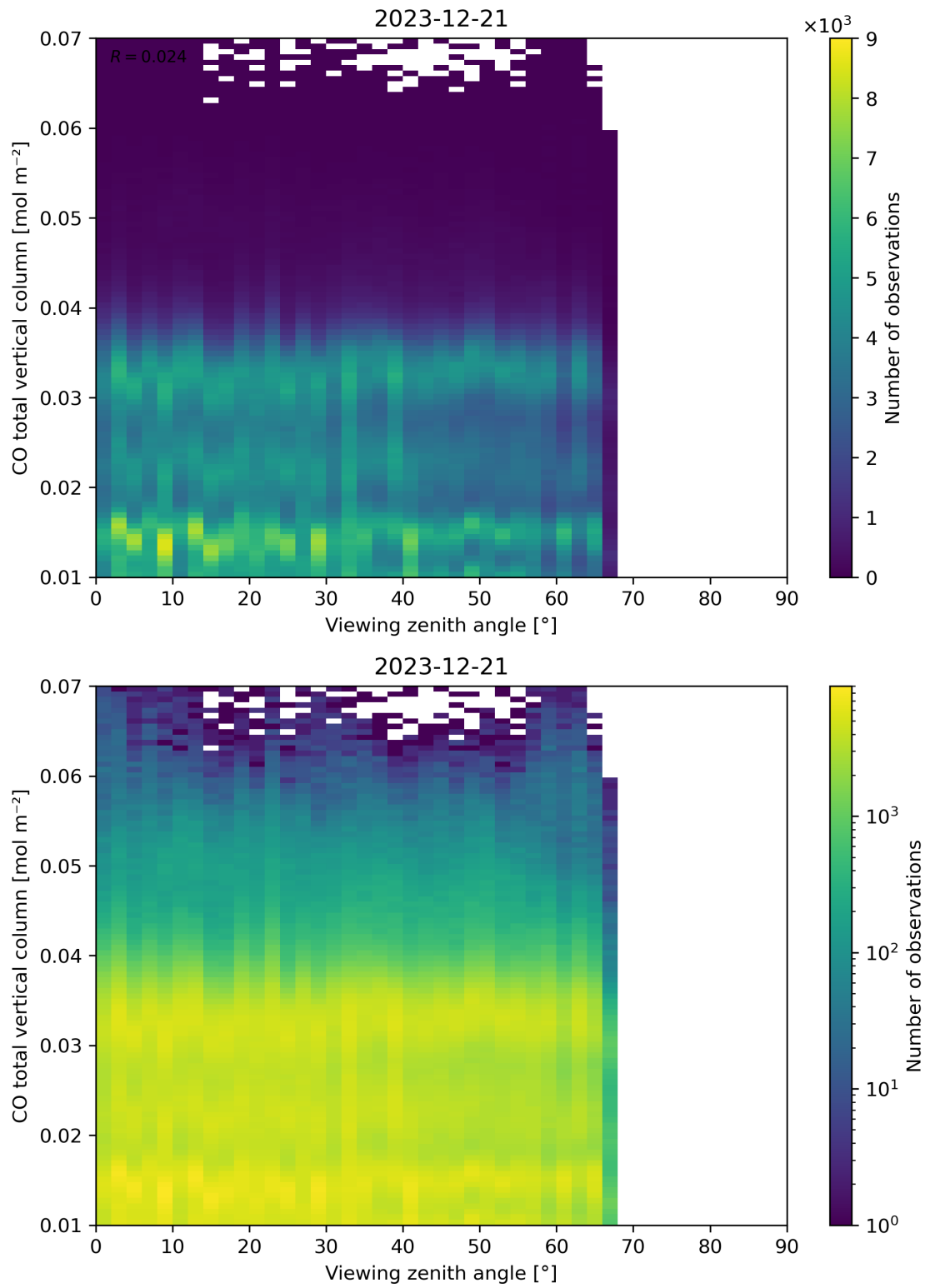
Figure 69: Scatter density plot of “Viewing zenith angle” against “CO total vertical column” for 2023-12-20 to 2023-12-22.
