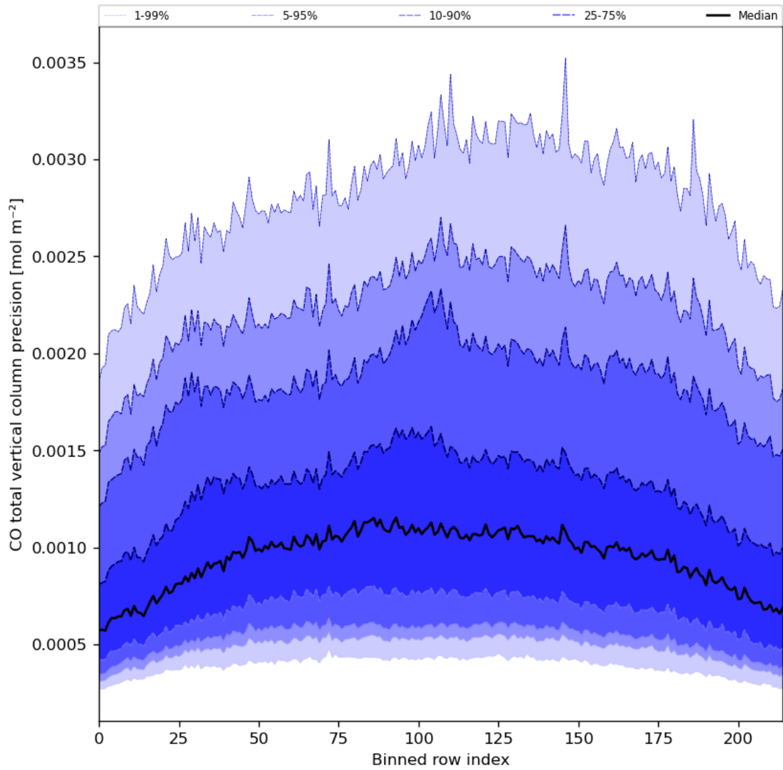
Figure 28: Along track statistics of “CO total vertical column precision” for 2023-12-20 to 2023-12-22
