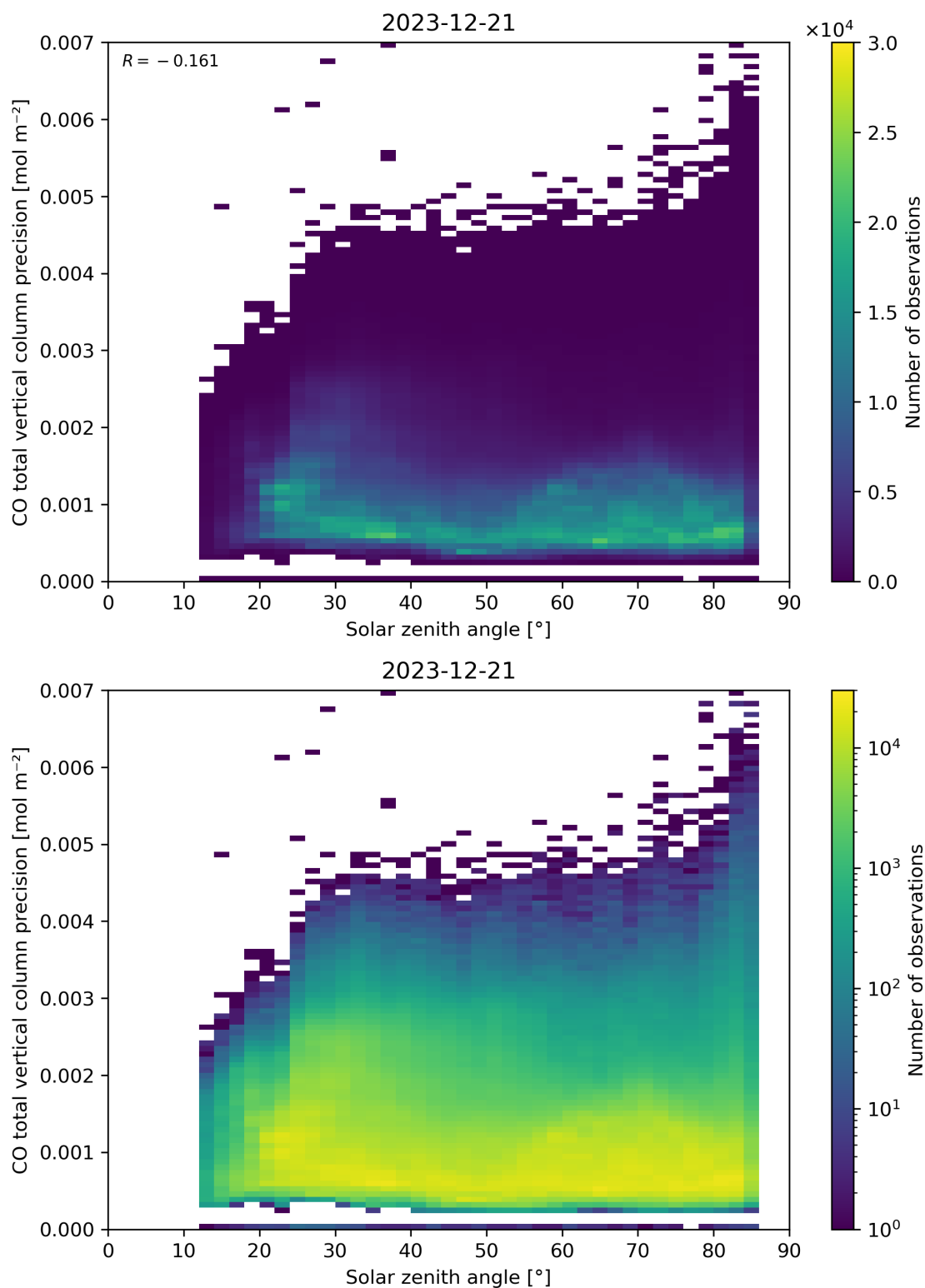
Figure 63: Scatter density plot of “Solar zenith angle” against “CO total vertical column precision” for 2023-12-20 to 2023-12-22.
