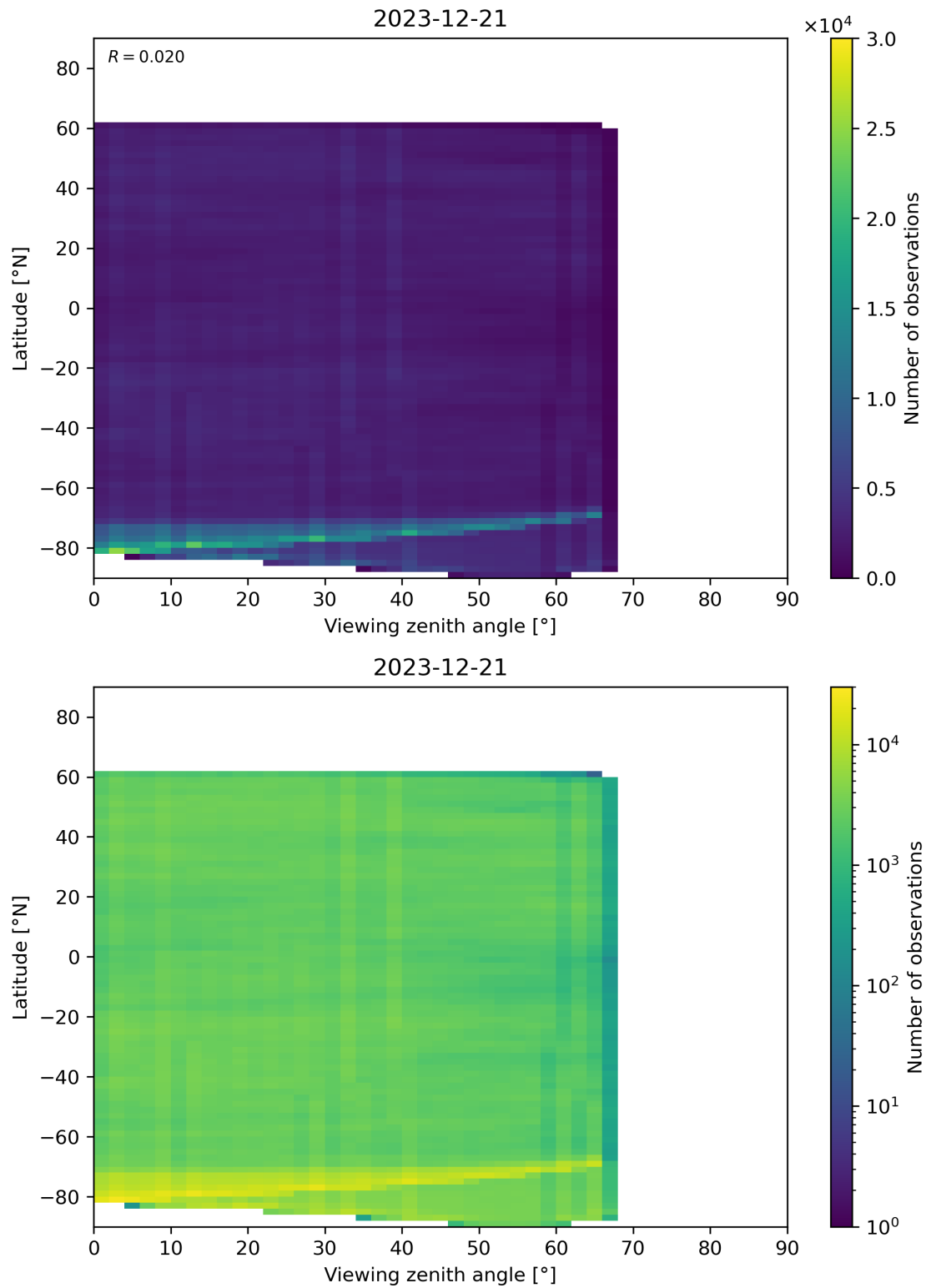
Figure 74: Scatter density plot of “Viewing zenith angle” against “Latitude” for 2023-12-20 to 2023-12-22.
