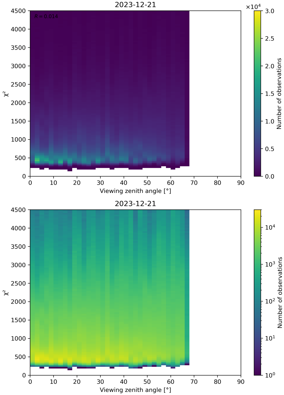
Figure 72: Scatter density plot of “Viewing zenith angle” against “ \chi^2 ” for 2023-12-20 to 2023-12-22.
