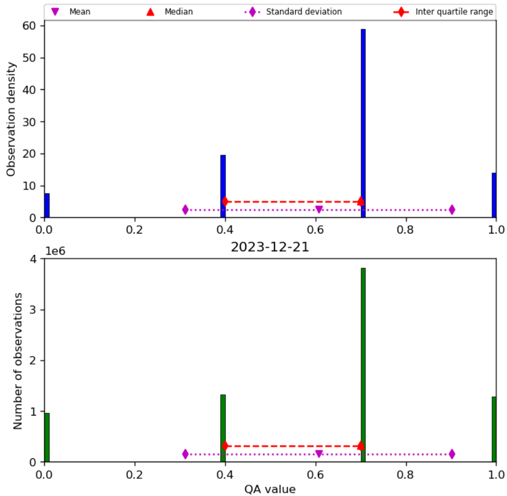
Figure 17: Histogram of “QA value” for 2023-12-20 to 2023-12-22
