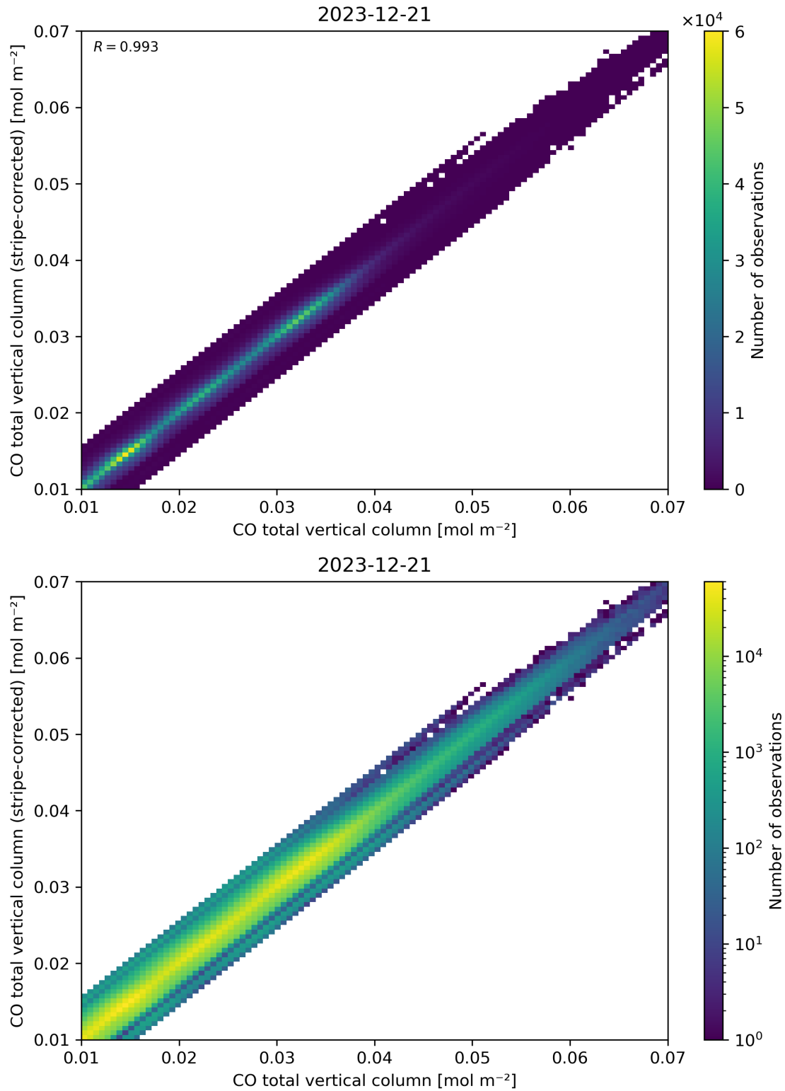
Figure 33: Scatter density plot of “CO total vertical column” against “CO total vertical column (stripe-corrected)” for 2023-12-20 to 2023-12-22.
