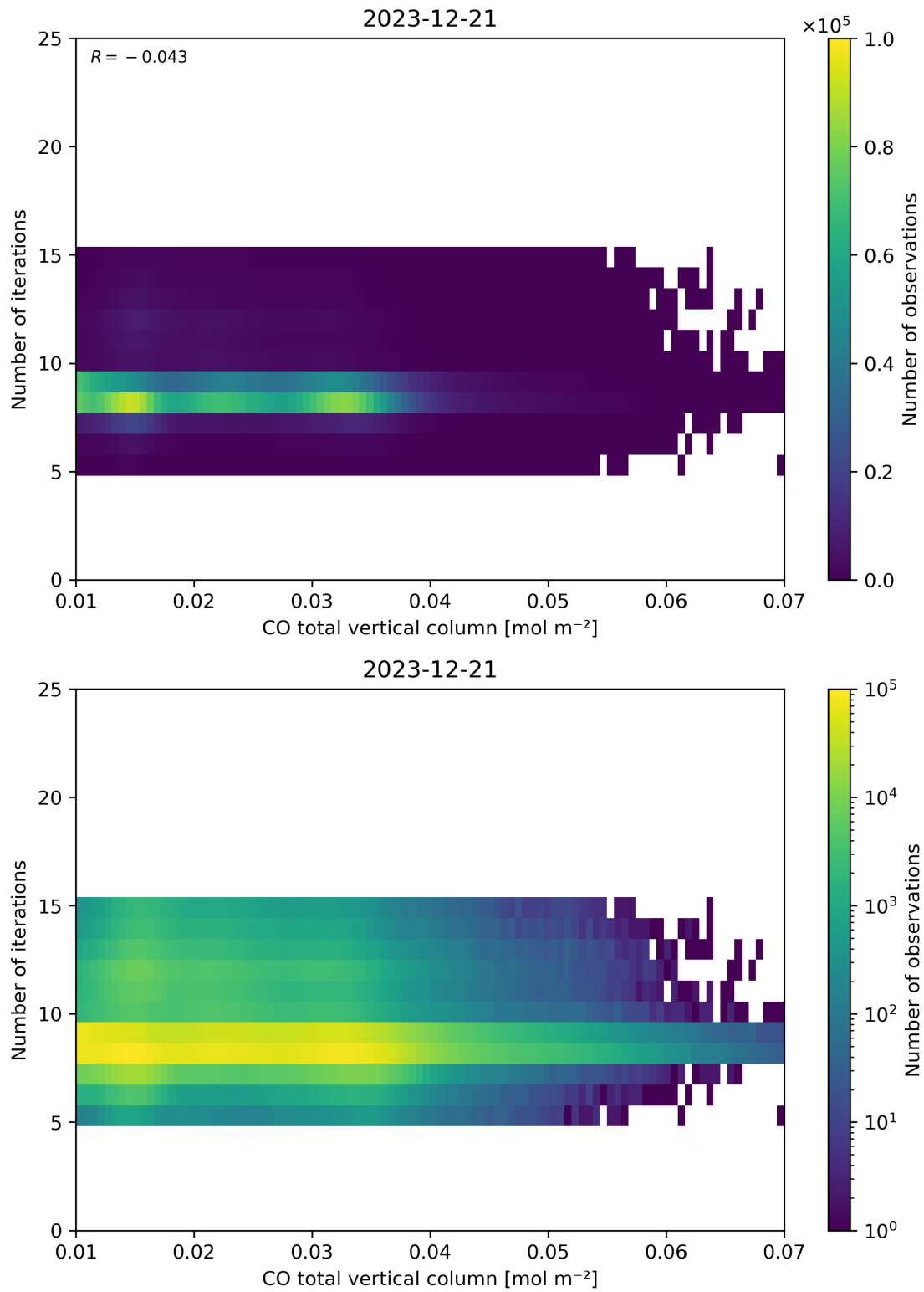
Figure 42: Scatter density plot of “CO total vertical column” against “Number of iterations” for 2023-12-20 to 2023-12-22.
