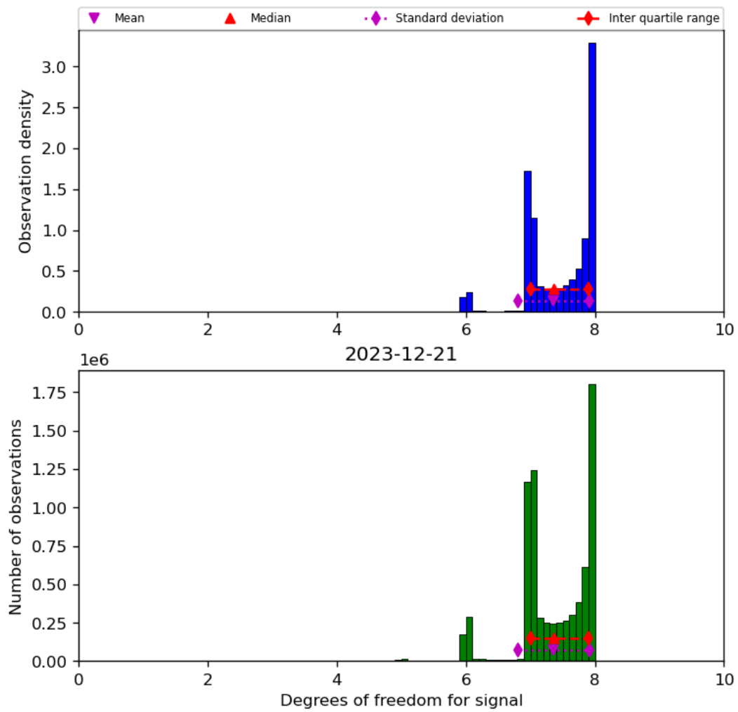
Figure 23: Histogram of “Degrees of freedom for signal” for 2023-12-20 to 2023-12-22
