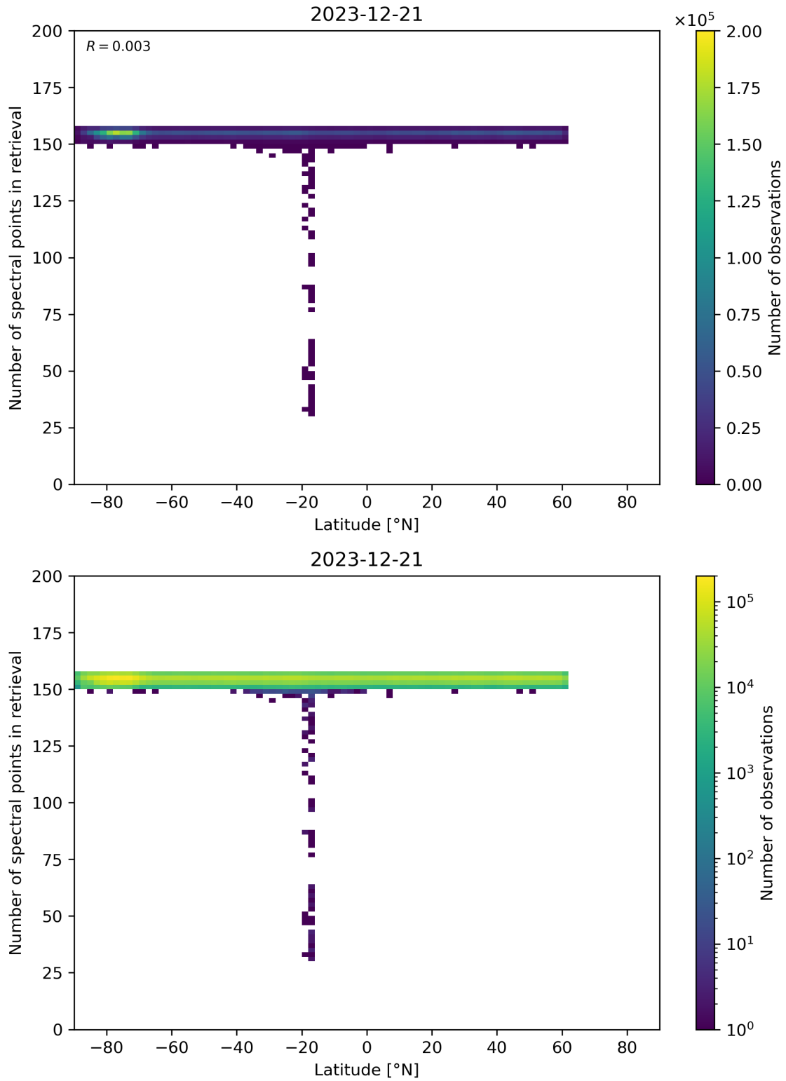
Figure 57: Scatter density plot of “Latitude” against “Number of spectral points in retrieval” for 2023-12-20 to 2023-12-22.
