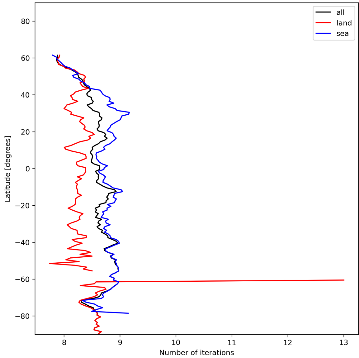
Figure 16: Zonal average of “Number of iterations” for 2023-12-20 to 2023-12-22.
