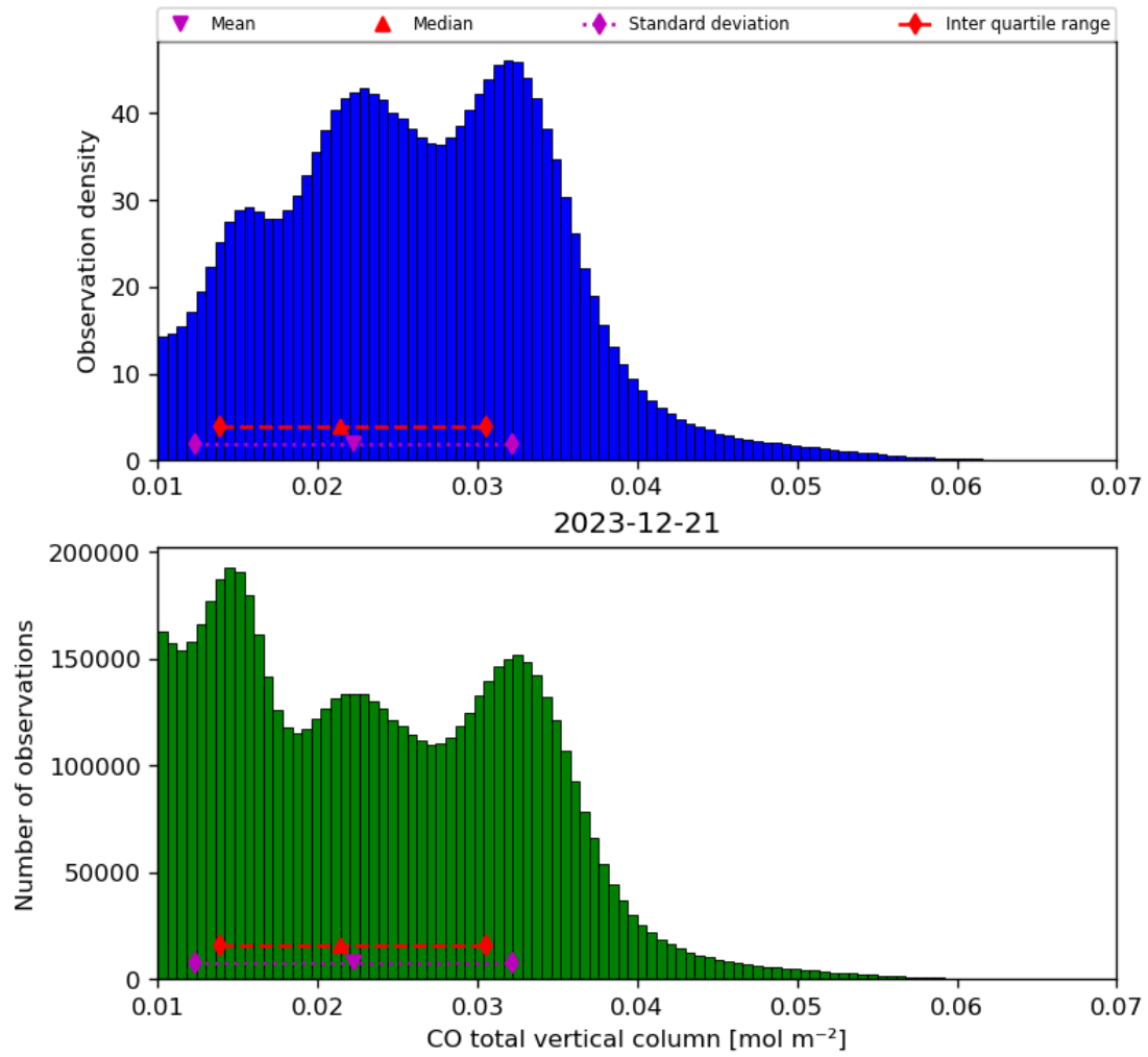
Figure 18: Histogram of “CO total vertical column” for 2023-12-20 to 2023-12-22
