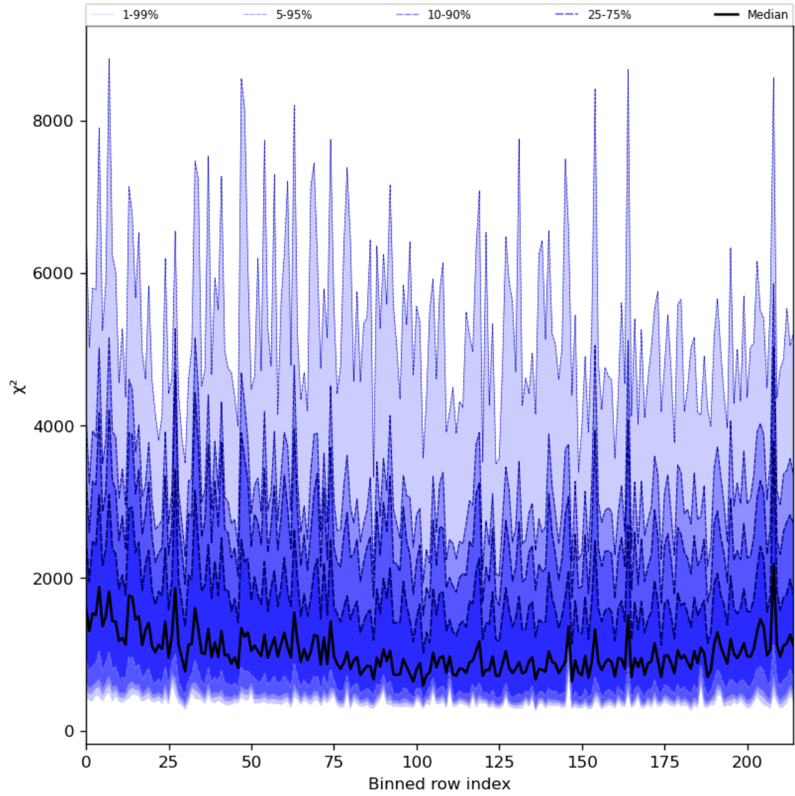
Figure 30: Along track statistics of “ \chi^2 ” for 2023-12-20 to 2023-12-22
