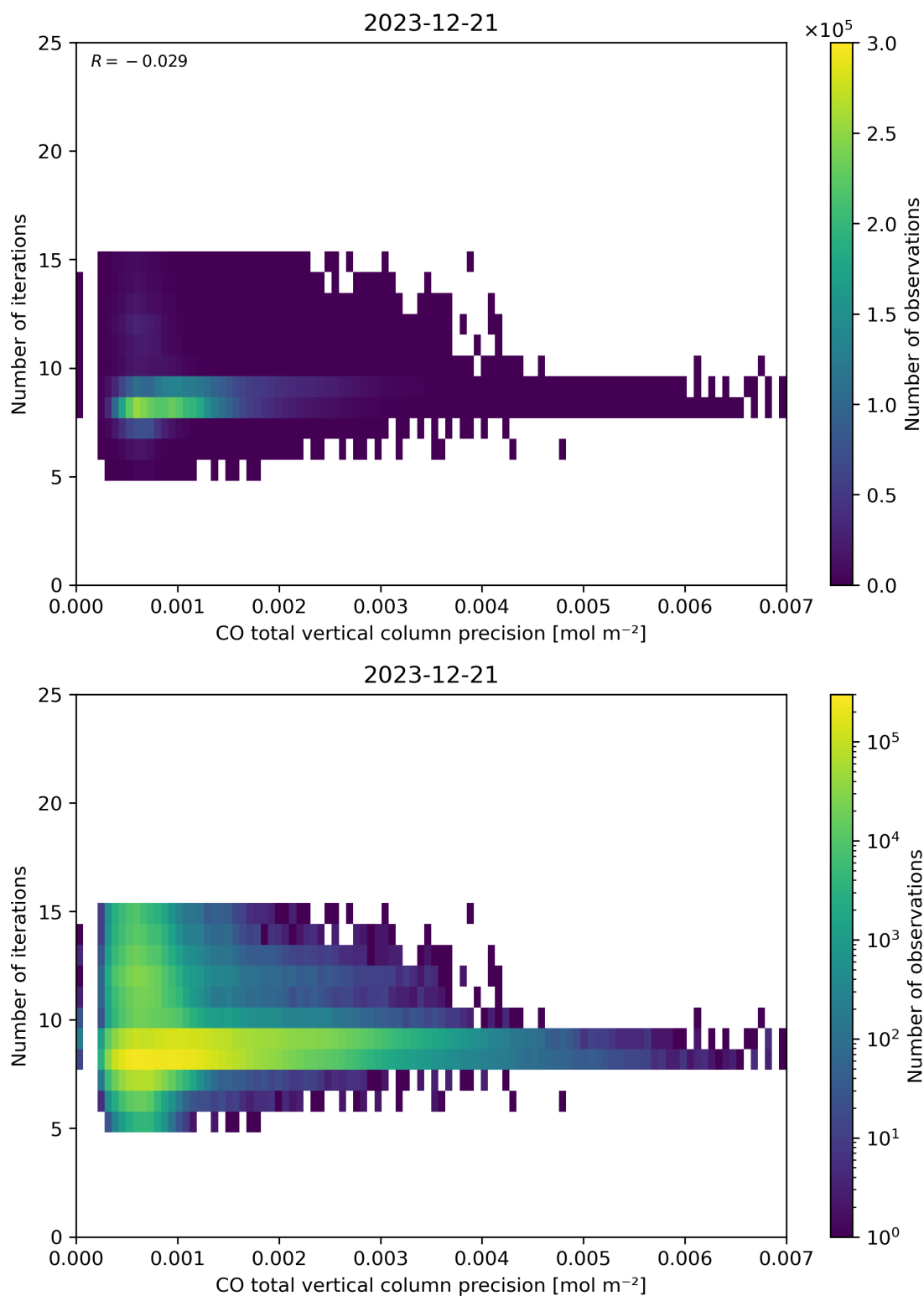
Figure 46: Scatter density plot of “CO total vertical column precision” against “Number of iterations” for 2023-12-20 to 2023-12-22.
