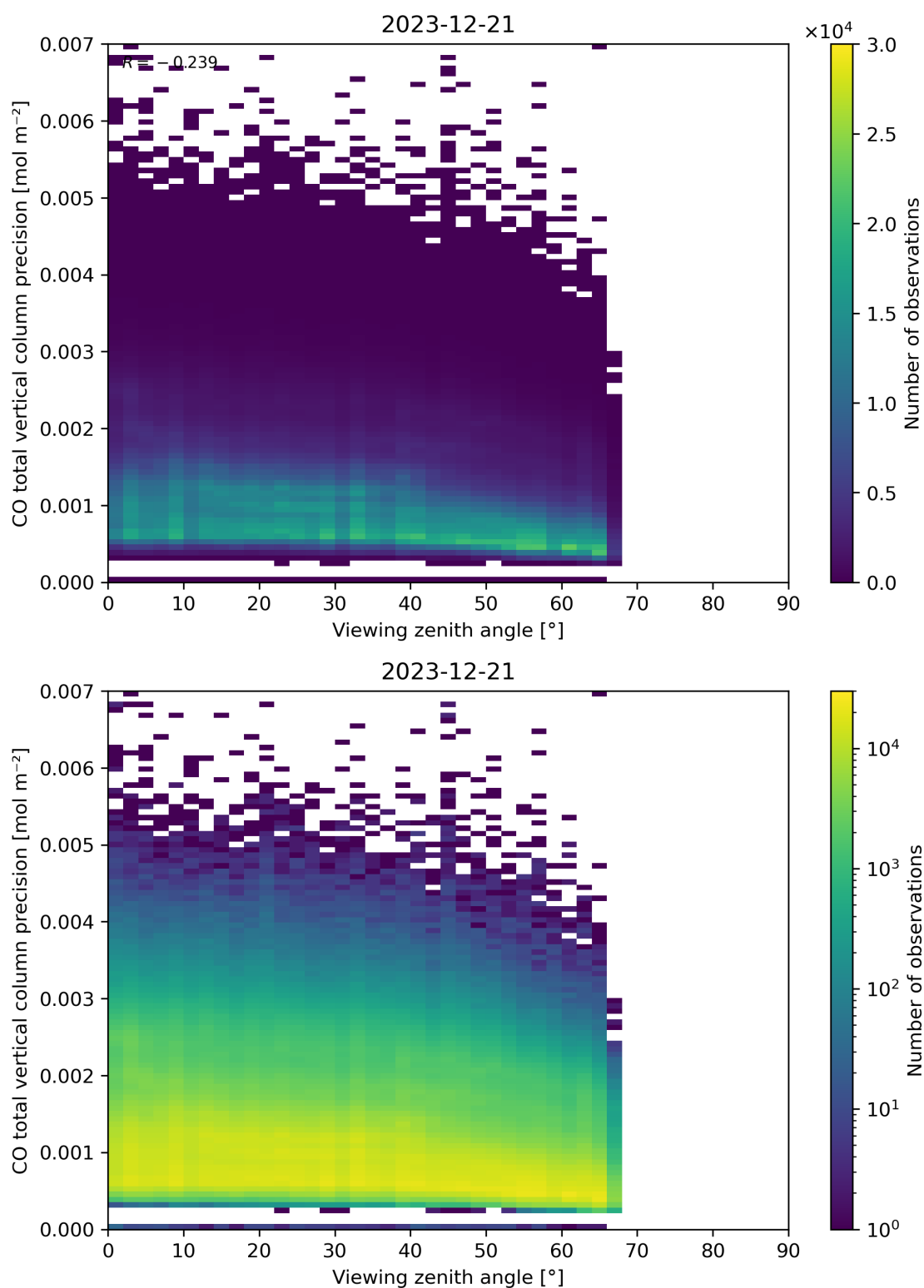
Figure 71: Scatter density plot of “Viewing zenith angle” against “CO total vertical column precision” for 2023-12-20 to 2023-12-22.
