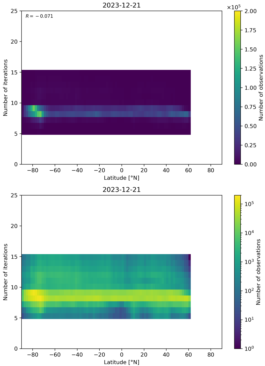
Figure 56: Scatter density plot of “Latitude” against “Number of iterations” for 2023-12-20 to 2023-12-22.
