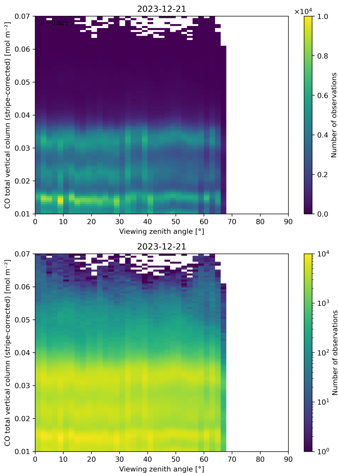
Figure 70: Scatter density plot of “Viewing zenith angle” against “CO total vertical column (stripe-corrected)” for 2023-12-20 to 2023-12-22.
