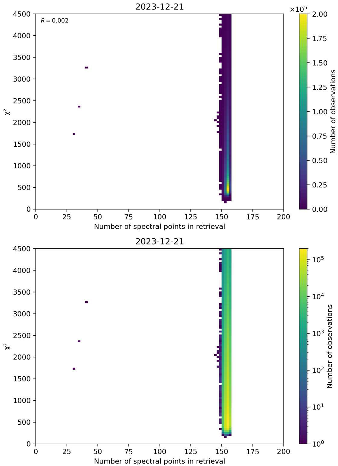
Figure 58: Scatter density plot of “Number of spectral points in retrieval” against “ \chi^2 ” for 2023-12-20 to 2023-12-22.
