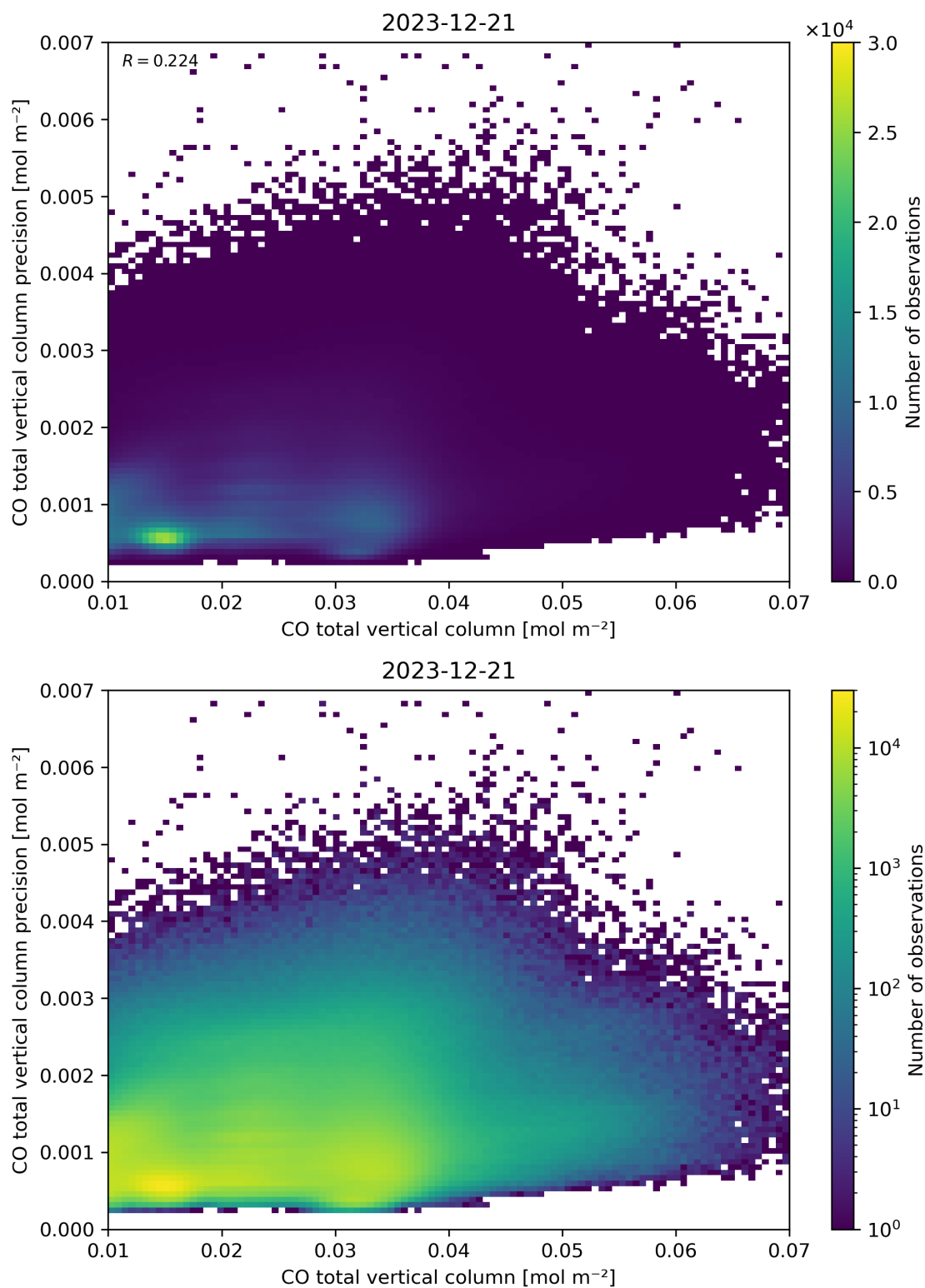
Figure 34: Scatter density plot of “CO total vertical column” against “CO total vertical column precision” for 2023-12-20 to 2023-12-22.
