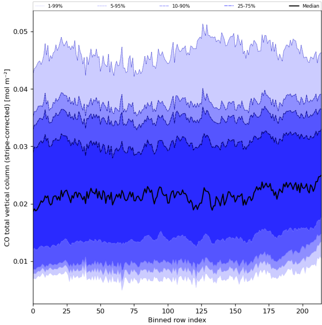
Figure 27: Along track statistics of “CO total vertical column (stripe-corrected)” for 2023-12-20 to 2023-12-22
