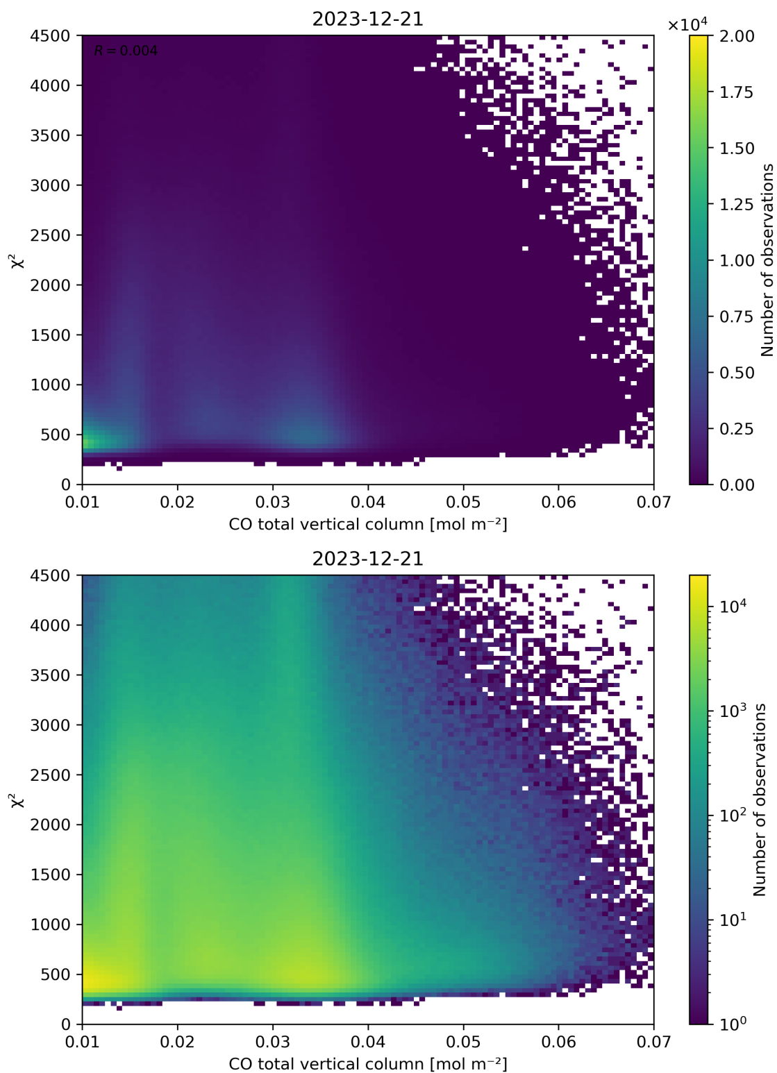
Figure 35: Scatter density plot of “CO total vertical column” against “ \chi^2 ” for 2023-12-20 to 2023-12-22.
