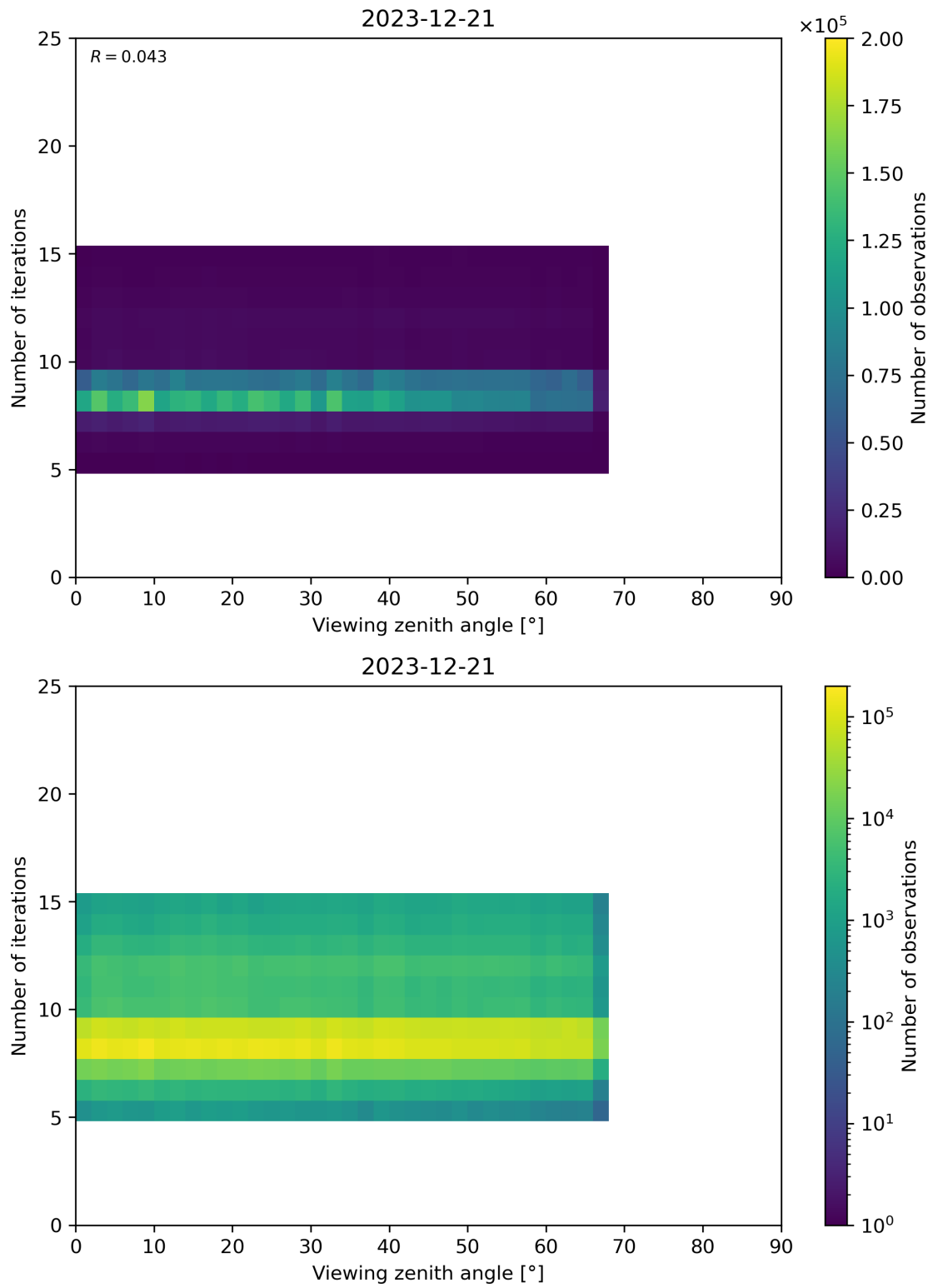
Figure 75: Scatter density plot of “Viewing zenith angle” against “Number of iterations” for 2023-12-20 to 2023-12-22.
