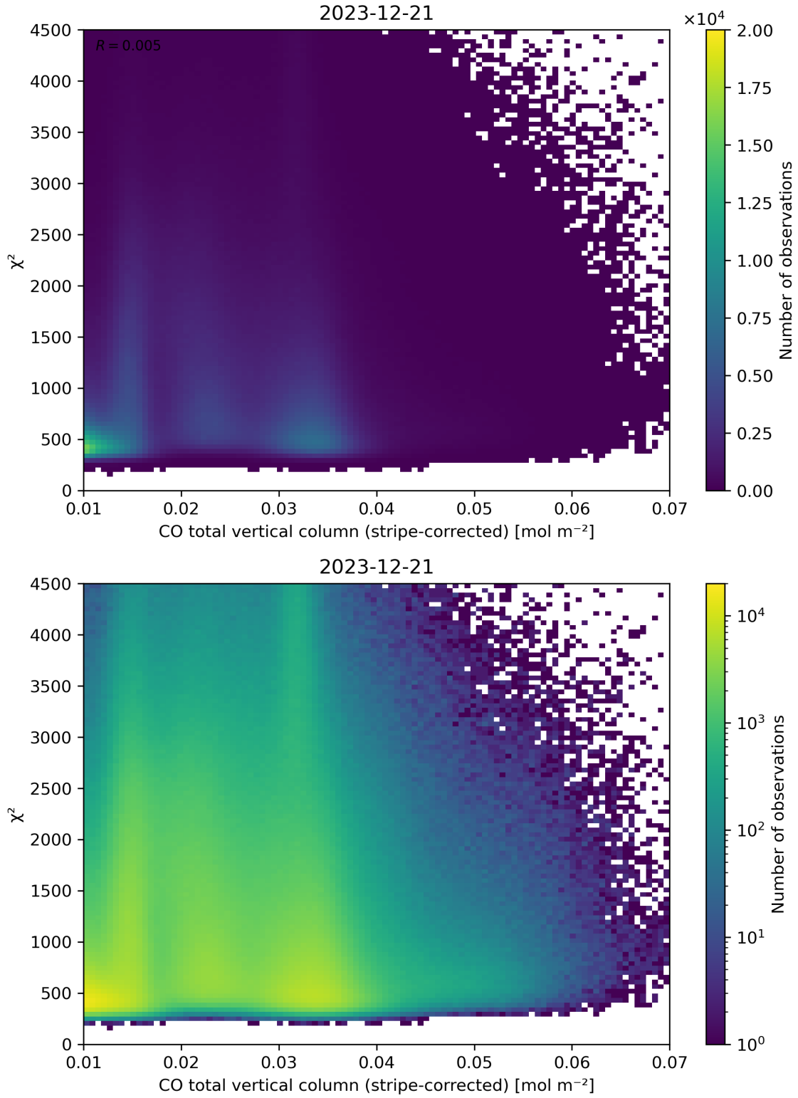
Figure 37: Scatter density plot of “CO total vertical column (stripe-corrected)” against “ \chi^2 ” for 2023-12-20 to 2023-12-22.
