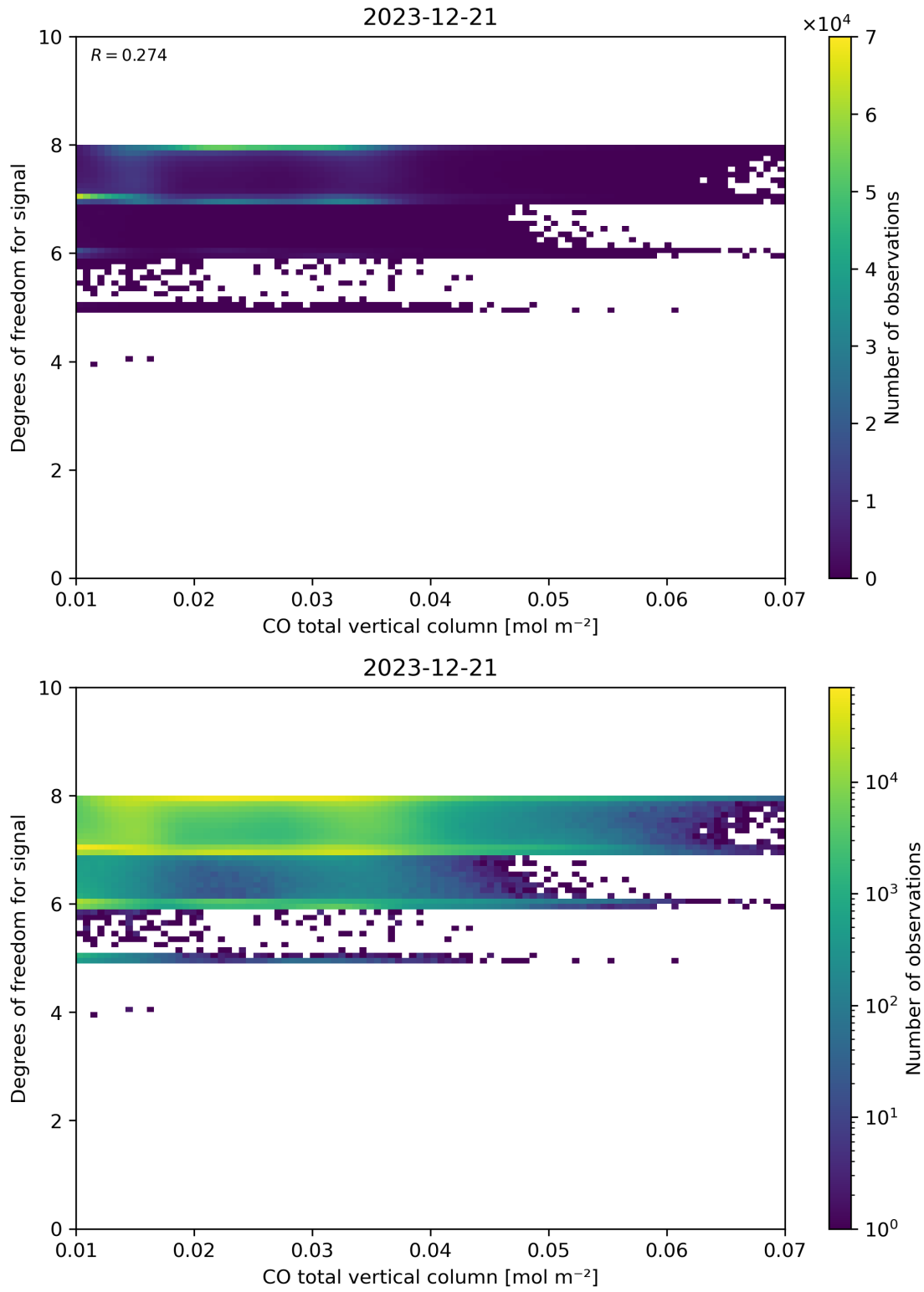
Figure 41: Scatter density plot of “CO total vertical column” against “Degrees of freedom for signal” for 2023-12-20 to 2023-12-22.
