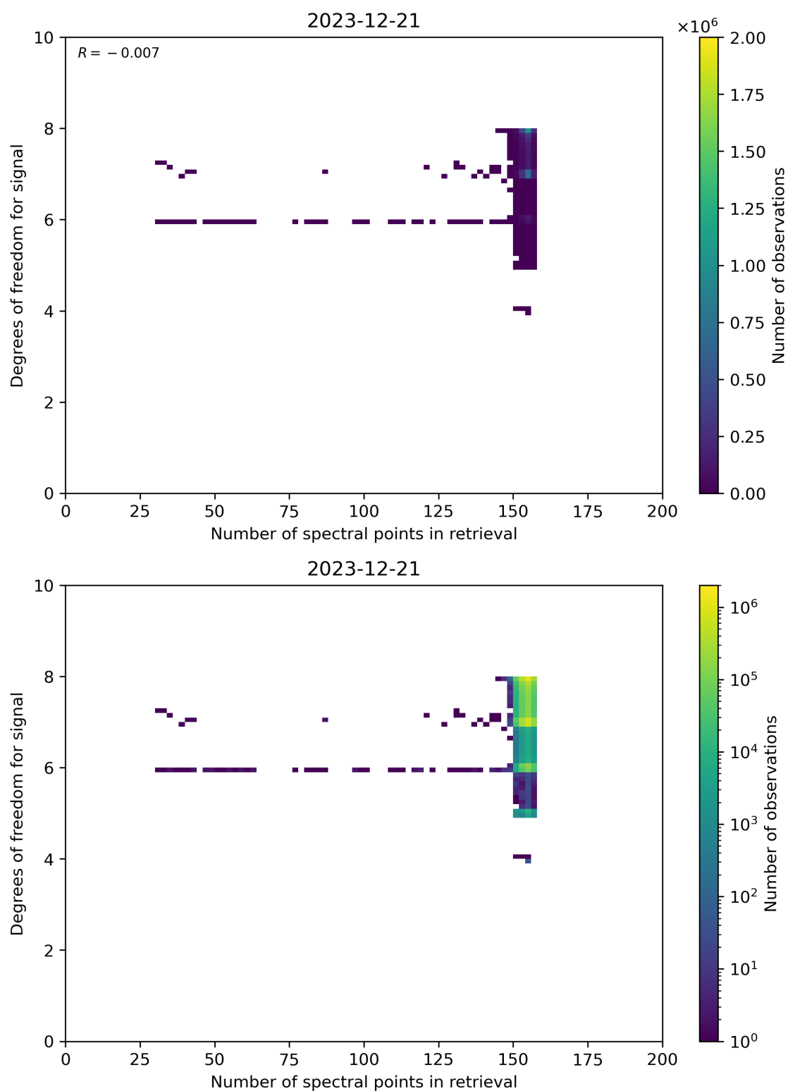
Figure 59: Scatter density plot of “Number of spectral points in retrieval” against “Degrees of freedom for signal” for 2023-12-20 to 2023-12-22.
