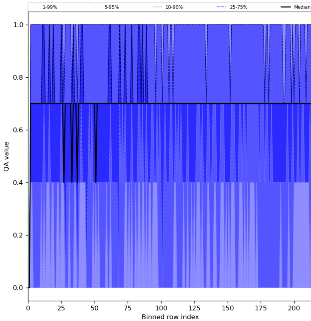
Figure 25: Along track statistics of “QA value” for 2023-12-20 to 2023-12-22
