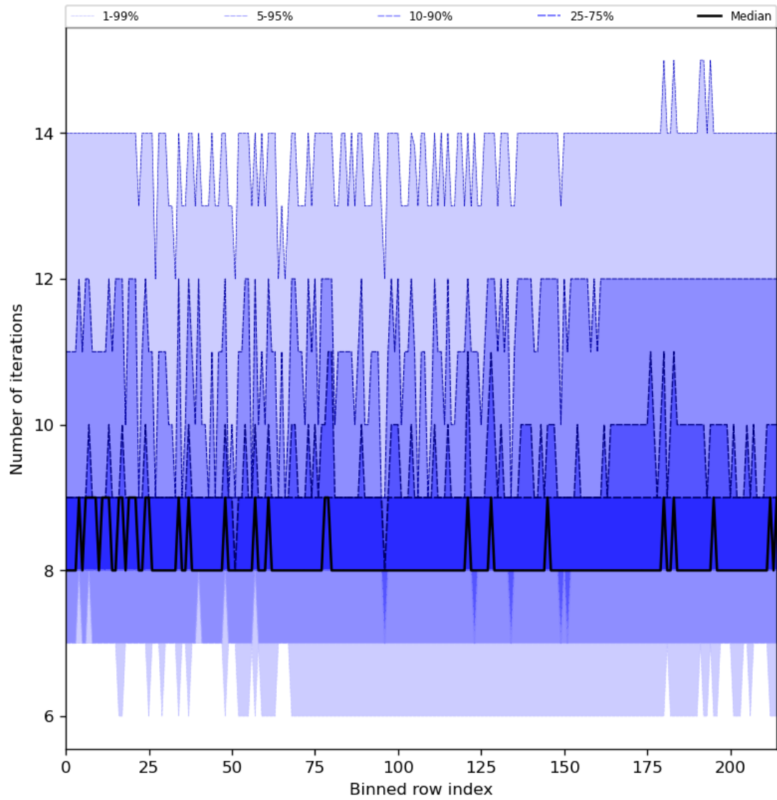
Figure 32: Along track statistics of “Number of iterations” for 2023-12-20 to 2023-12-22
