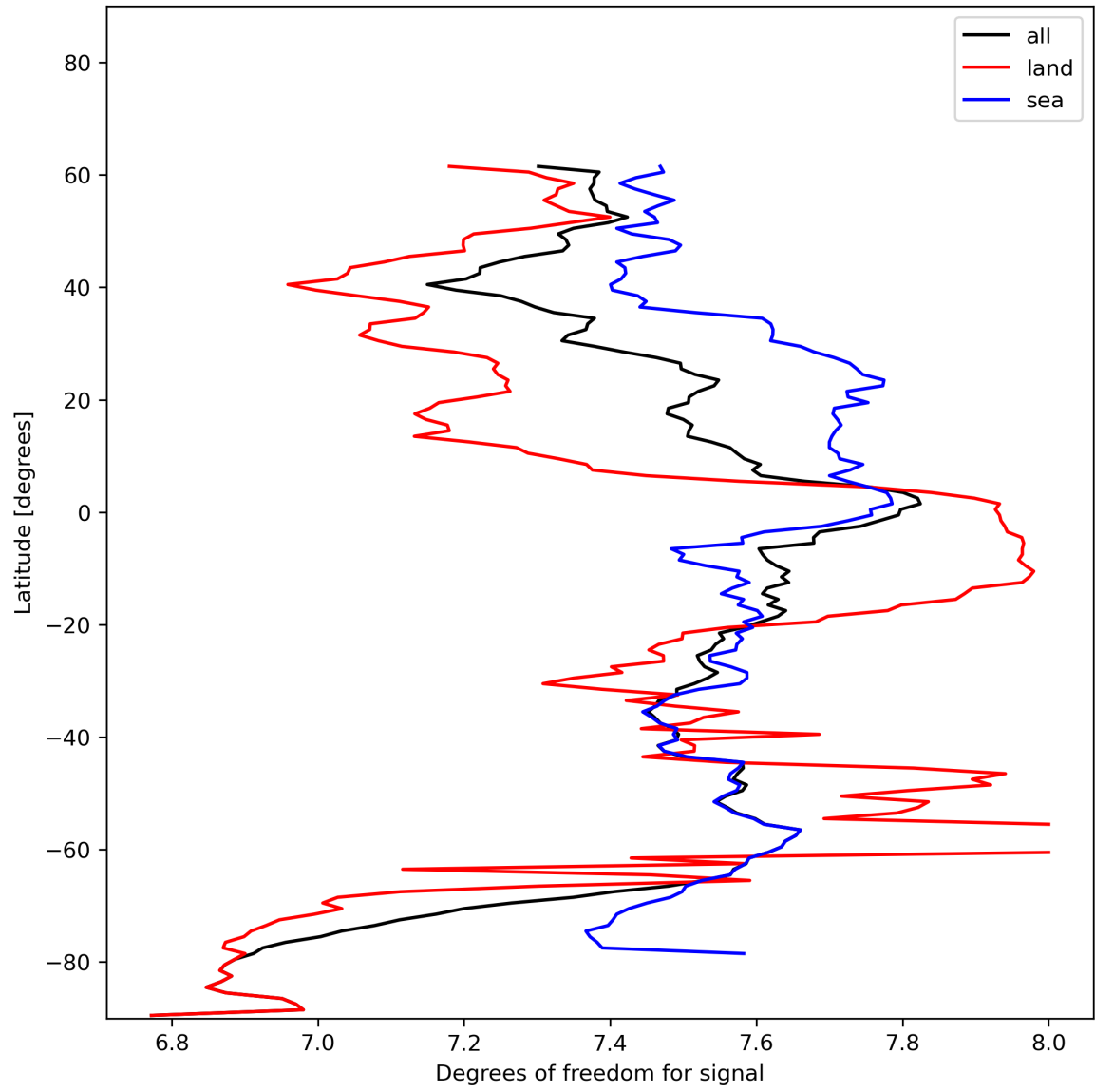
Figure 15: Zonal average of “Degrees of freedom for signal” for 2023-12-20 to 2023-12-22.
