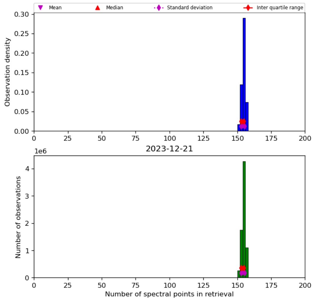
Figure 21: Histogram of “Number of spectral points in retrieval” for 2023-12-20 to 2023-12-22
