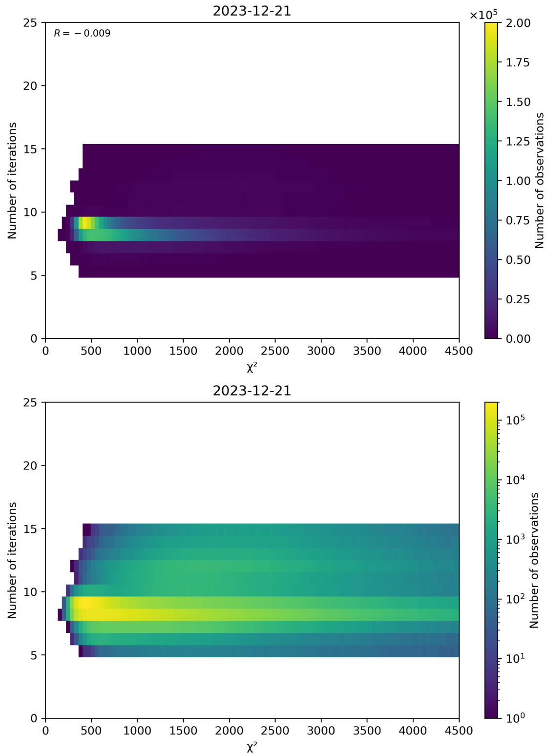
Figure 49: Scatter density plot of “ \chi^2 ” against “Number of iterations” for 2023-12-20 to 2023-12-22.
