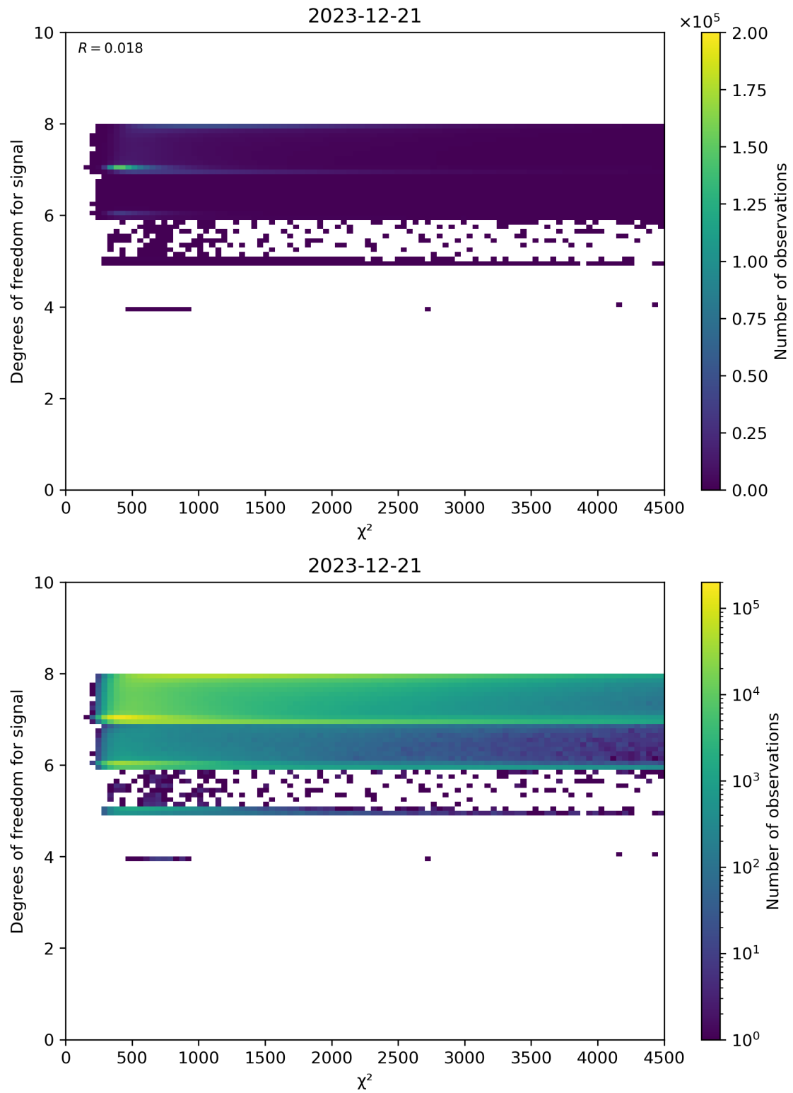
Figure 48: Scatter density plot of “ \chi^2 ” against “Degrees of freedom for signal” for 2023-12-20 to 2023-12-22.
