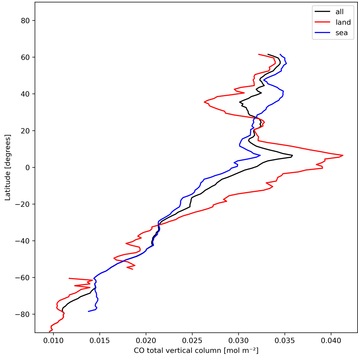
Figure 10: Zonal average of “CO total vertical column” for 2023-12-20 to 2023-12-22.
