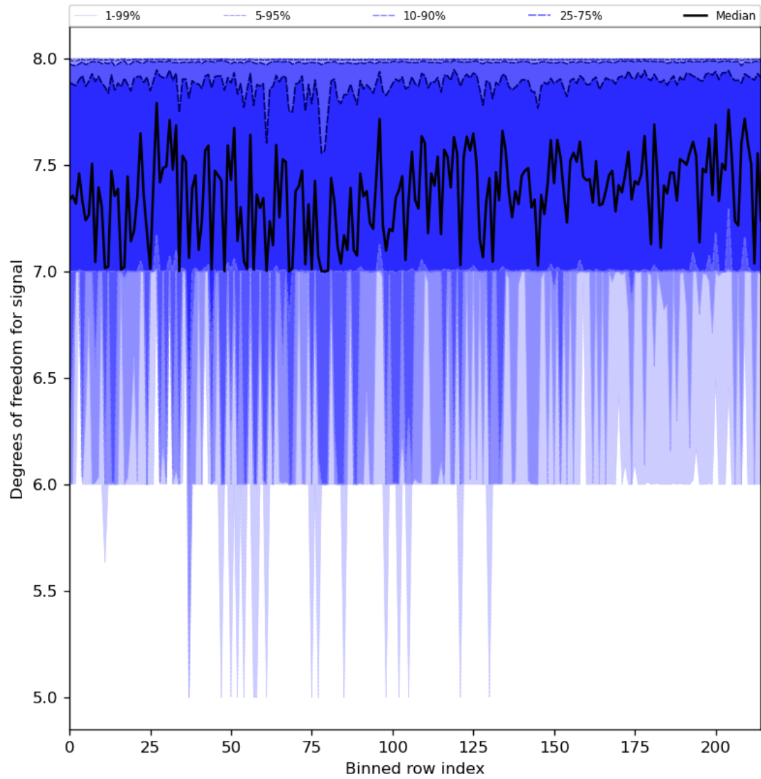
Figure 31: Along track statistics of “Degrees of freedom for signal” for 2023-12-20 to 2023-12-22
