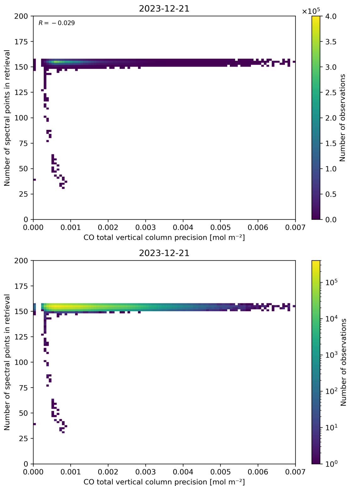
Figure 47: Scatter density plot of “CO total vertical column precision” against “Number of spectral points in retrieval” for 2023-12-20 to 2023-12-22.
