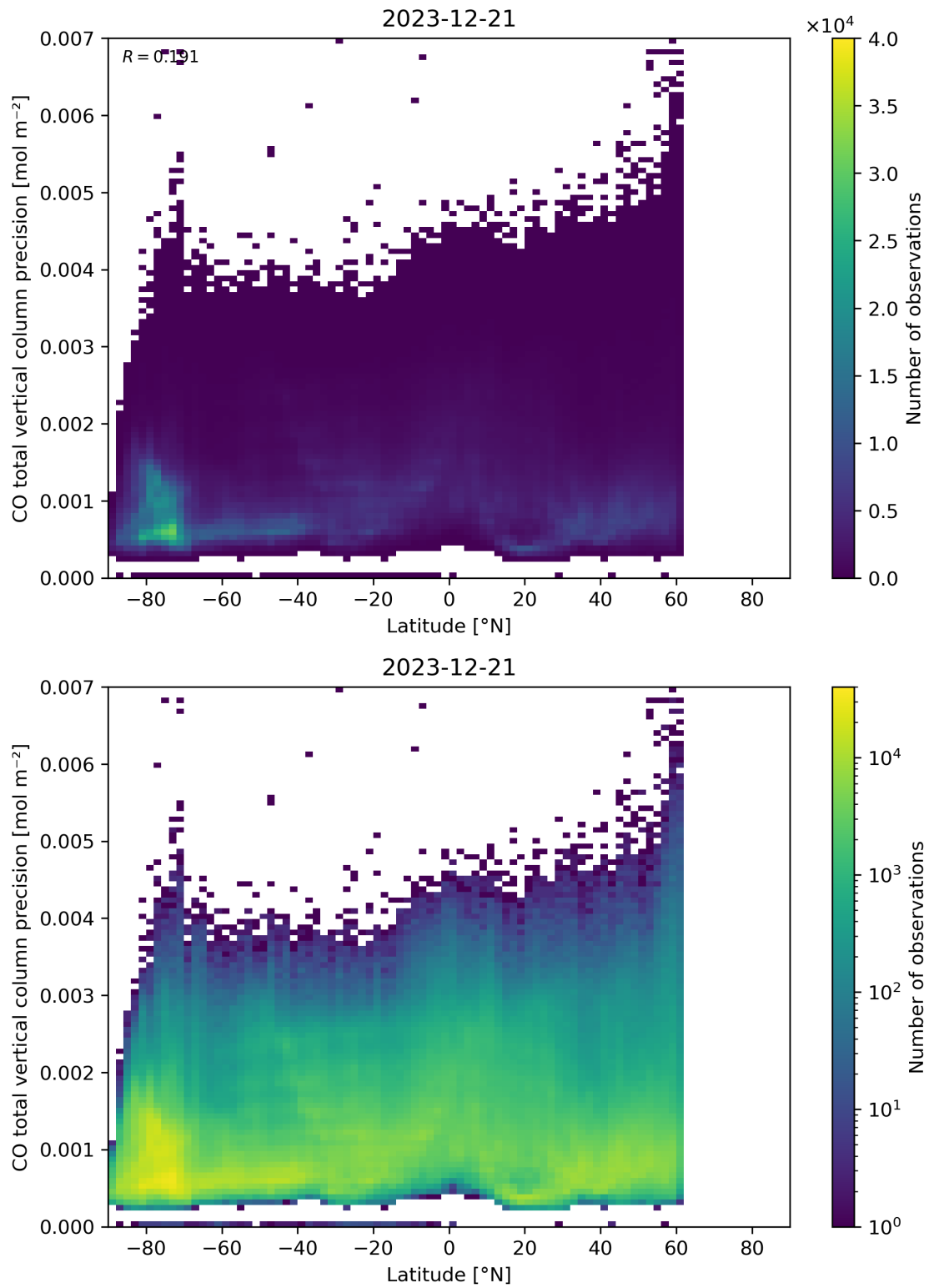
Figure 53: Scatter density plot of “Latitude” against “CO total vertical column precision” for 2023-12-20 to 2023-12-22.
