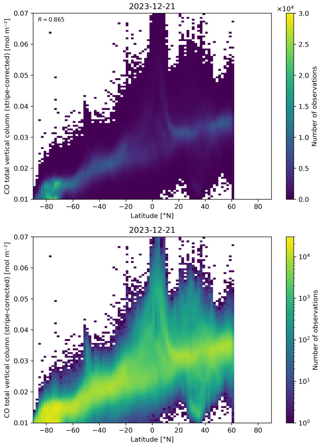
Figure 52: Scatter density plot of “Latitude” against “CO total vertical column (stripe-corrected)” for 2023-12-20 to 2023-12-22.
