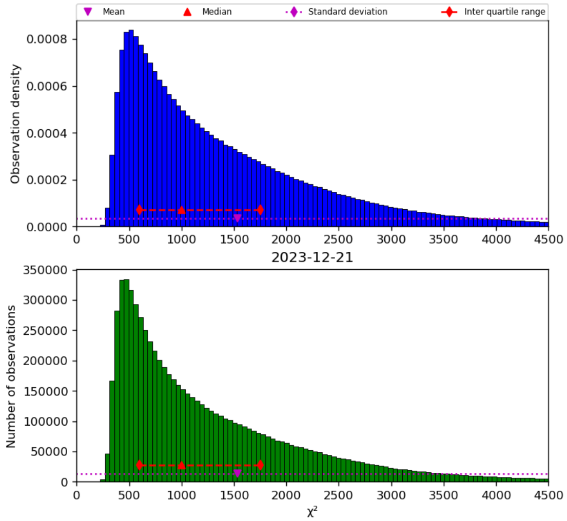
Figure 22: Histogram of “ \chi^2 ” for 2023-12-20 to 2023-12-22
