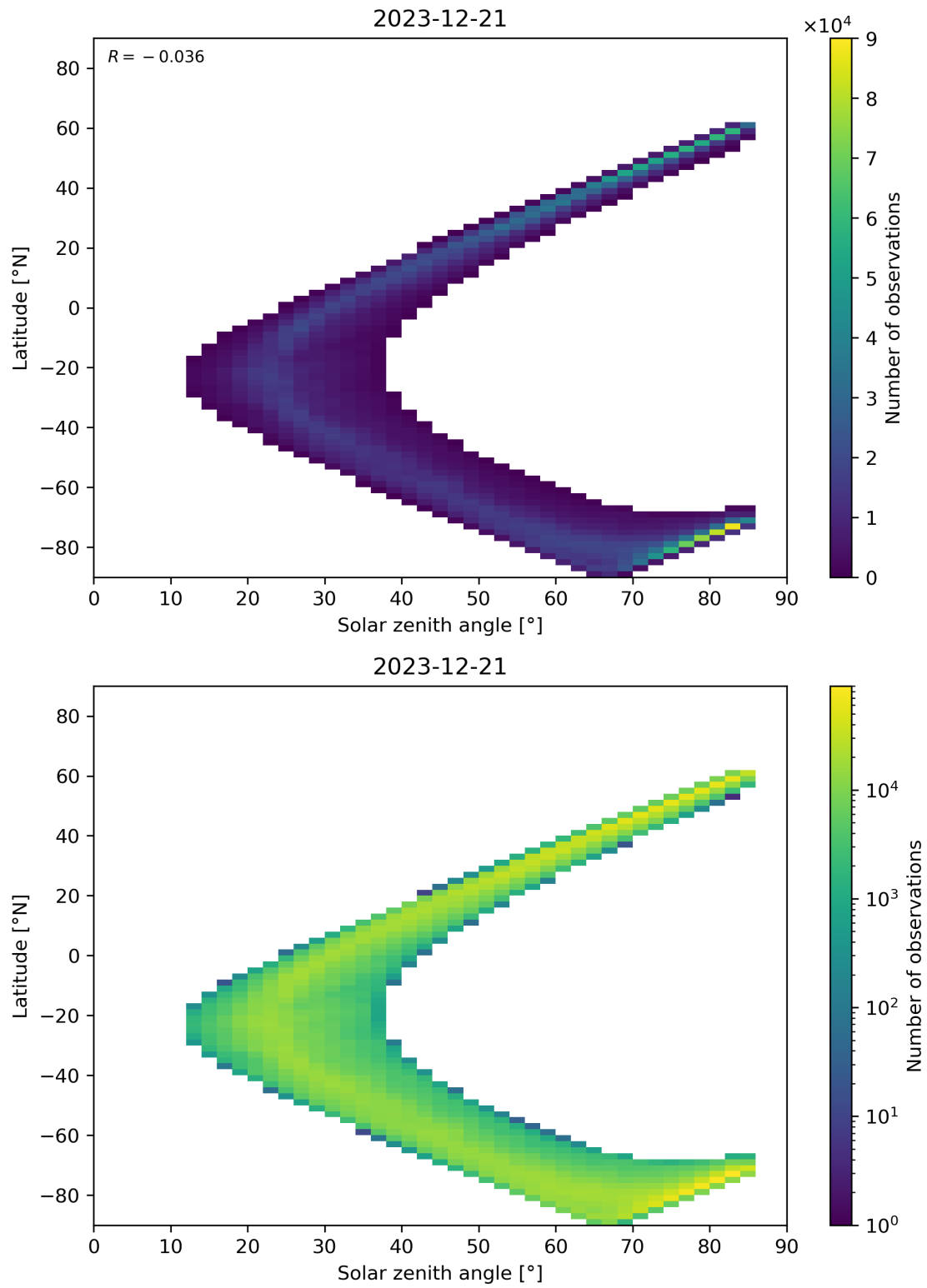
Figure 66: Scatter density plot of “Solar zenith angle” against “Latitude” for 2023-12-20 to 2023-12-22.
