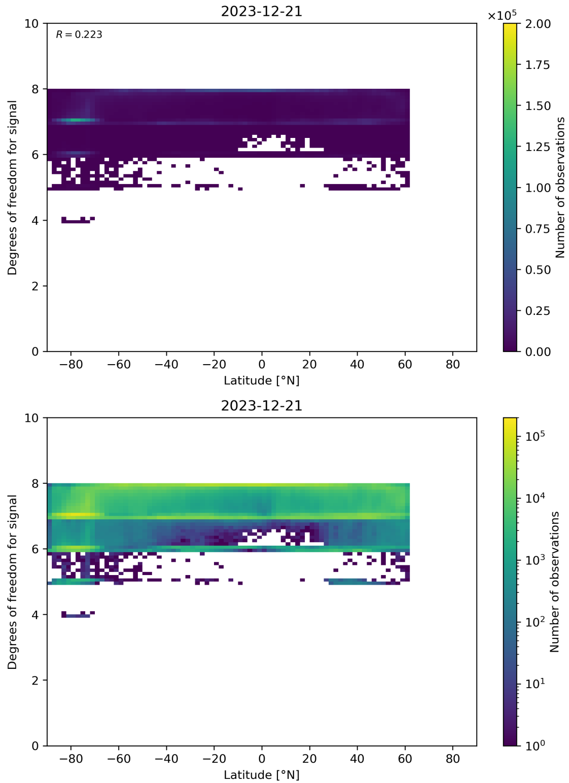
Figure 55: Scatter density plot of “Latitude” against “Degrees of freedom for signal” for 2023-12-20 to 2023-12-22.
