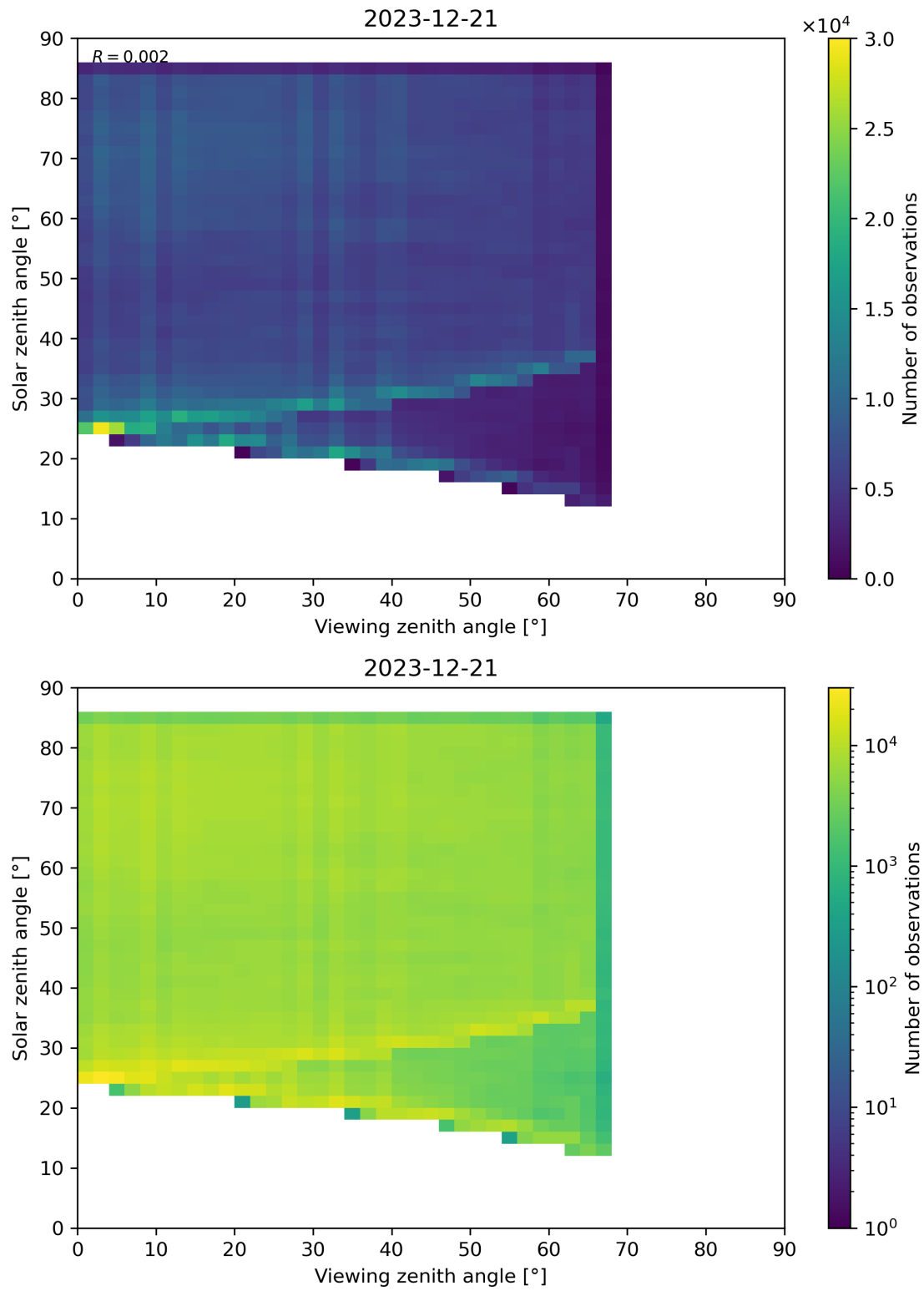
Figure 77: Scatter density plot of “Viewing zenith angle” against “Solar zenith angle” for 2023-12-20 to 2023-12-22.
