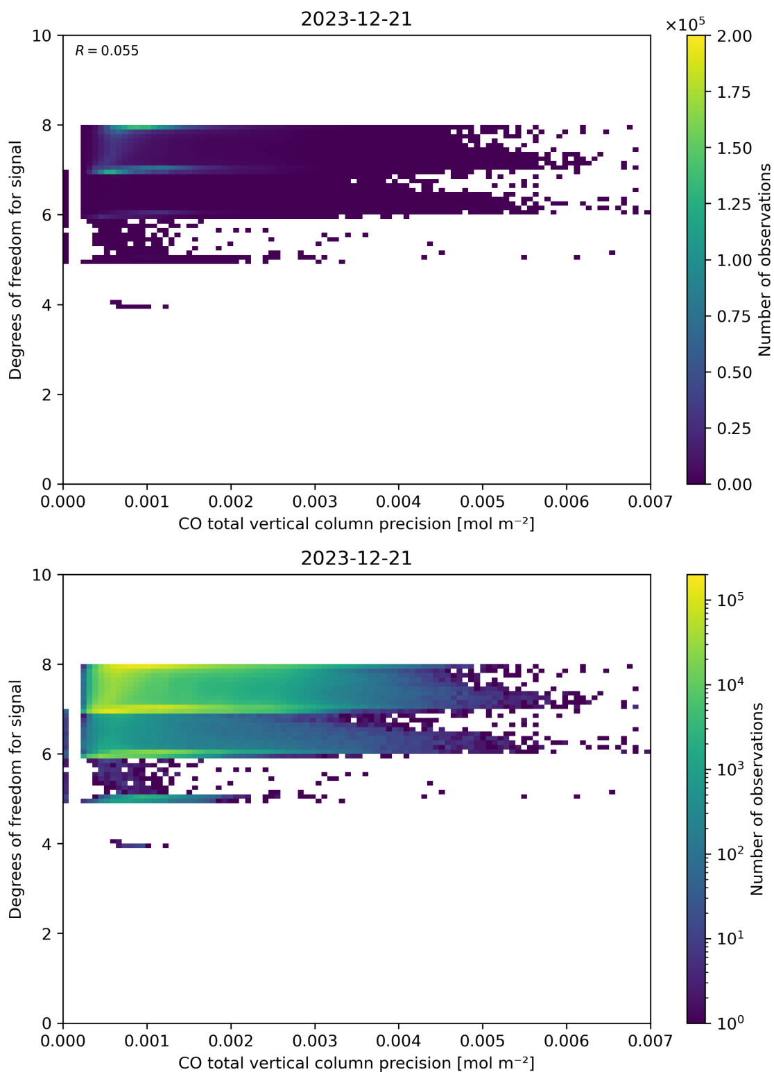
Figure 45: Scatter density plot of “CO total vertical column precision” against “Degrees of freedom for signal” for 2023-12-20 to 2023-12-22.
