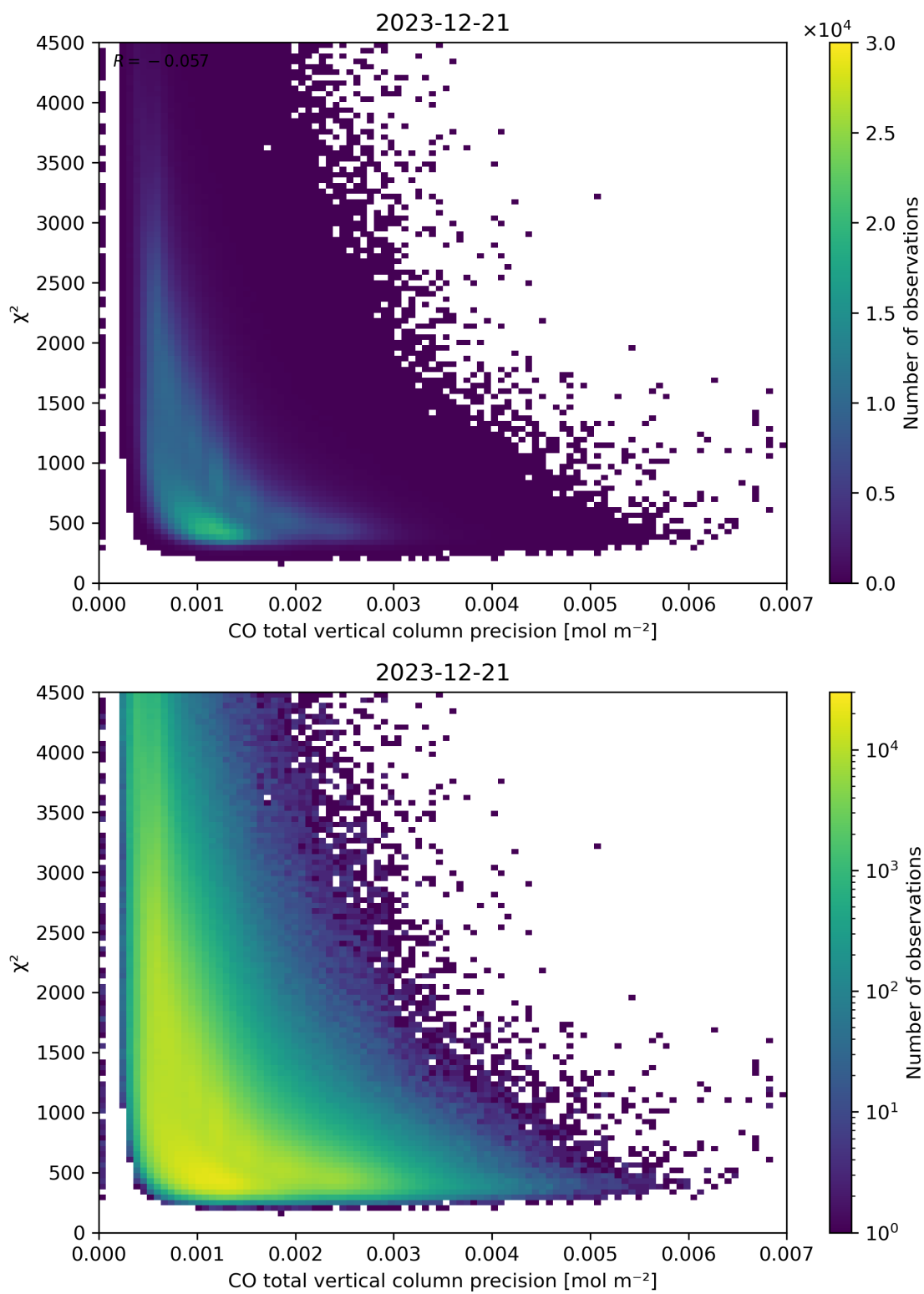
Figure 44: Scatter density plot of “CO total vertical column precision” against “ \chi^2 ” for 2023-12-20 to 2023-12-22.
