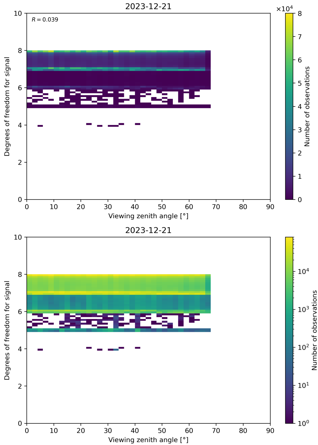
Figure 73: Scatter density plot of “Viewing zenith angle” against “Degrees of freedom for signal” for 2023-12-20 to 2023-12-22.
