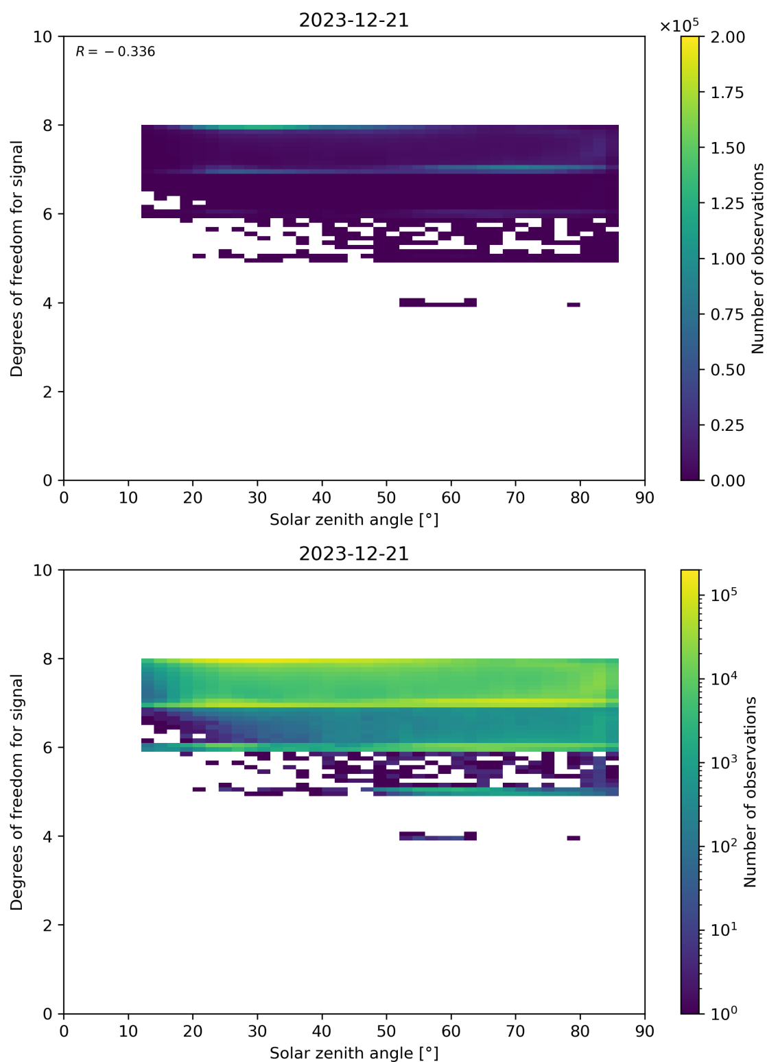
Figure 65: Scatter density plot of “Solar zenith angle” against “Degrees of freedom for signal” for 2023-12-20 to 2023-12-22.
