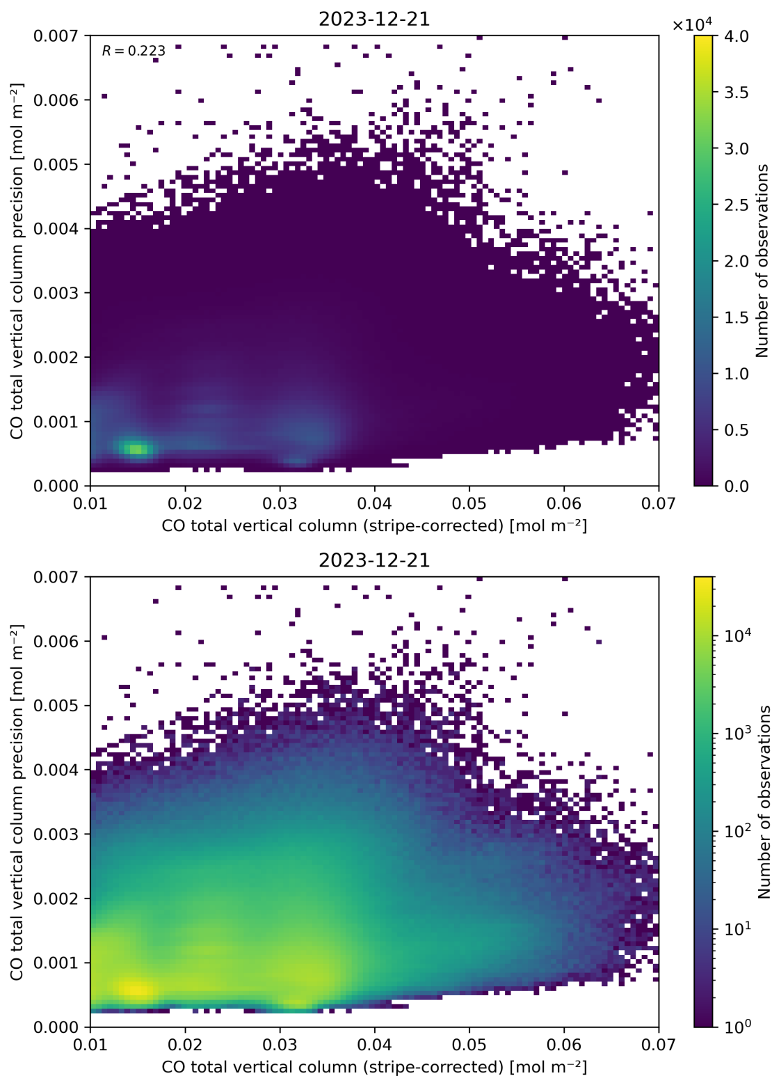
Figure 36: Scatter density plot of “CO total vertical column (stripe-corrected)” against “CO total vertical column precision” for 2023-12-20 to 2023-12-22.
