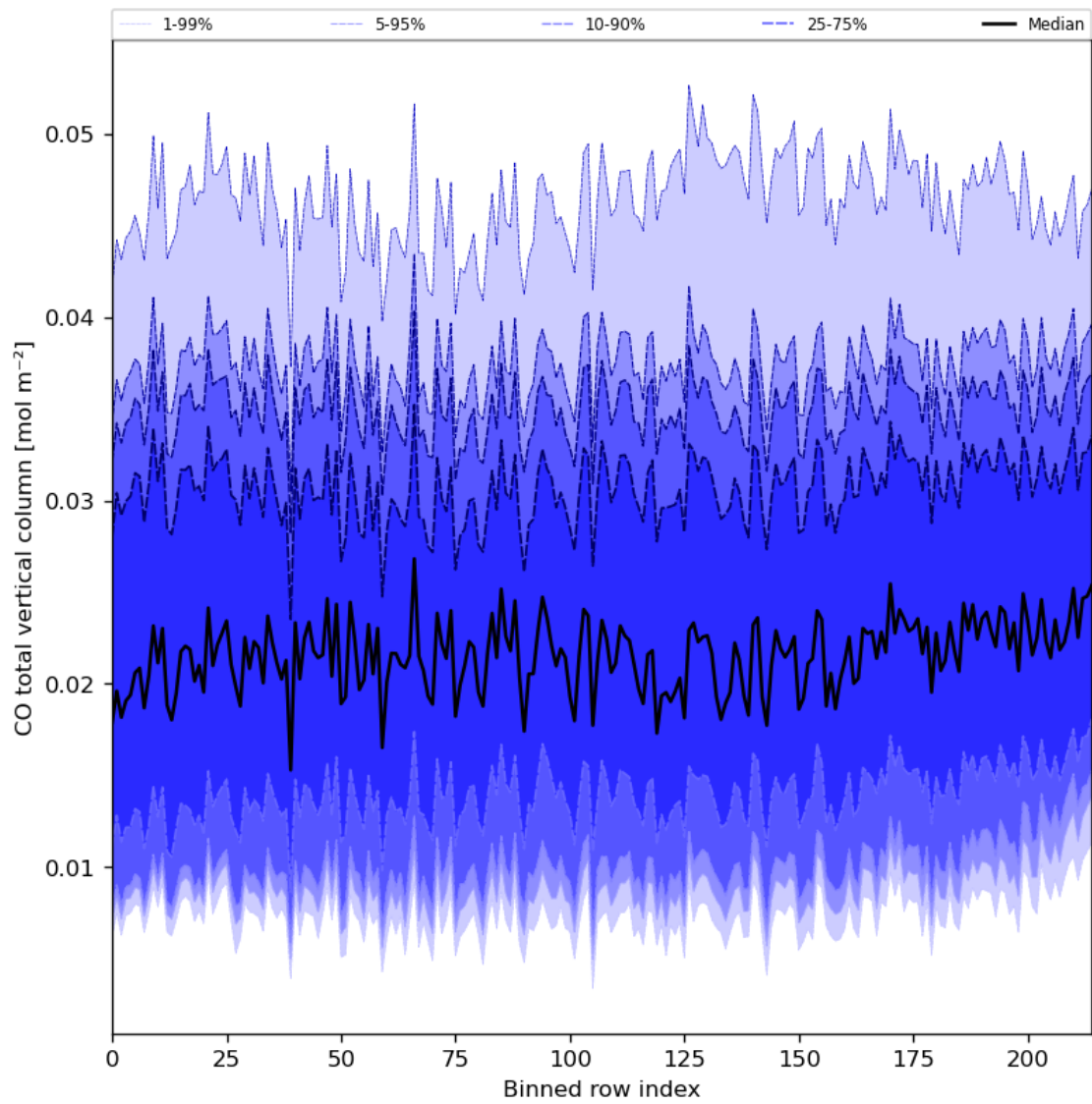
Figure 26: Along track statistics of “CO total vertical column” for 2023-12-20 to 2023-12-22
