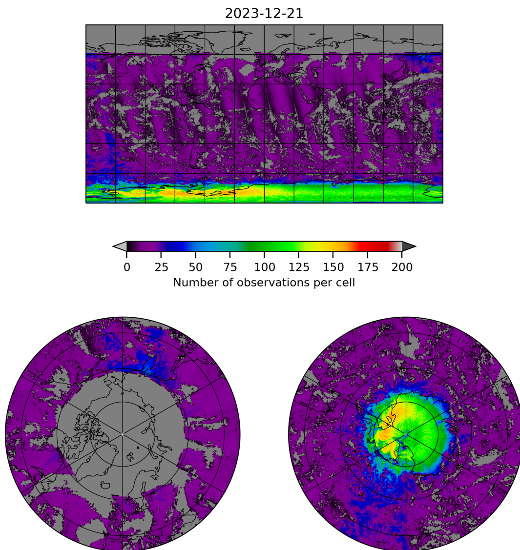
Figure 8: Map of the number of observations for 2023-12-20 to 2023-12-22
