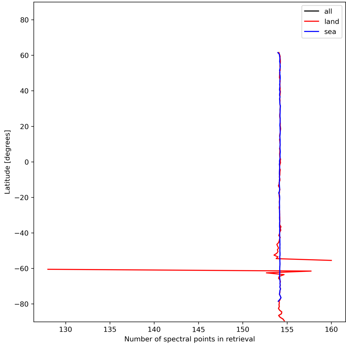
Figure 13: Zonal average of “Number of spectral points in retrieval” for 2023-12-20 to 2023-12-22.
