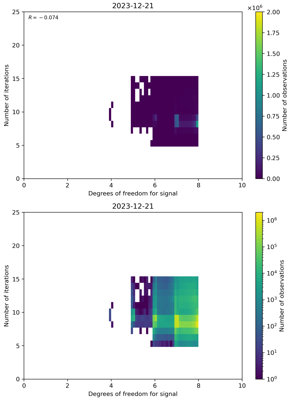
Figure 50: Scatter density plot of “Degrees of freedom for signal” against “Number of iterations” for 2023-12-20 to 2023-12-22.
