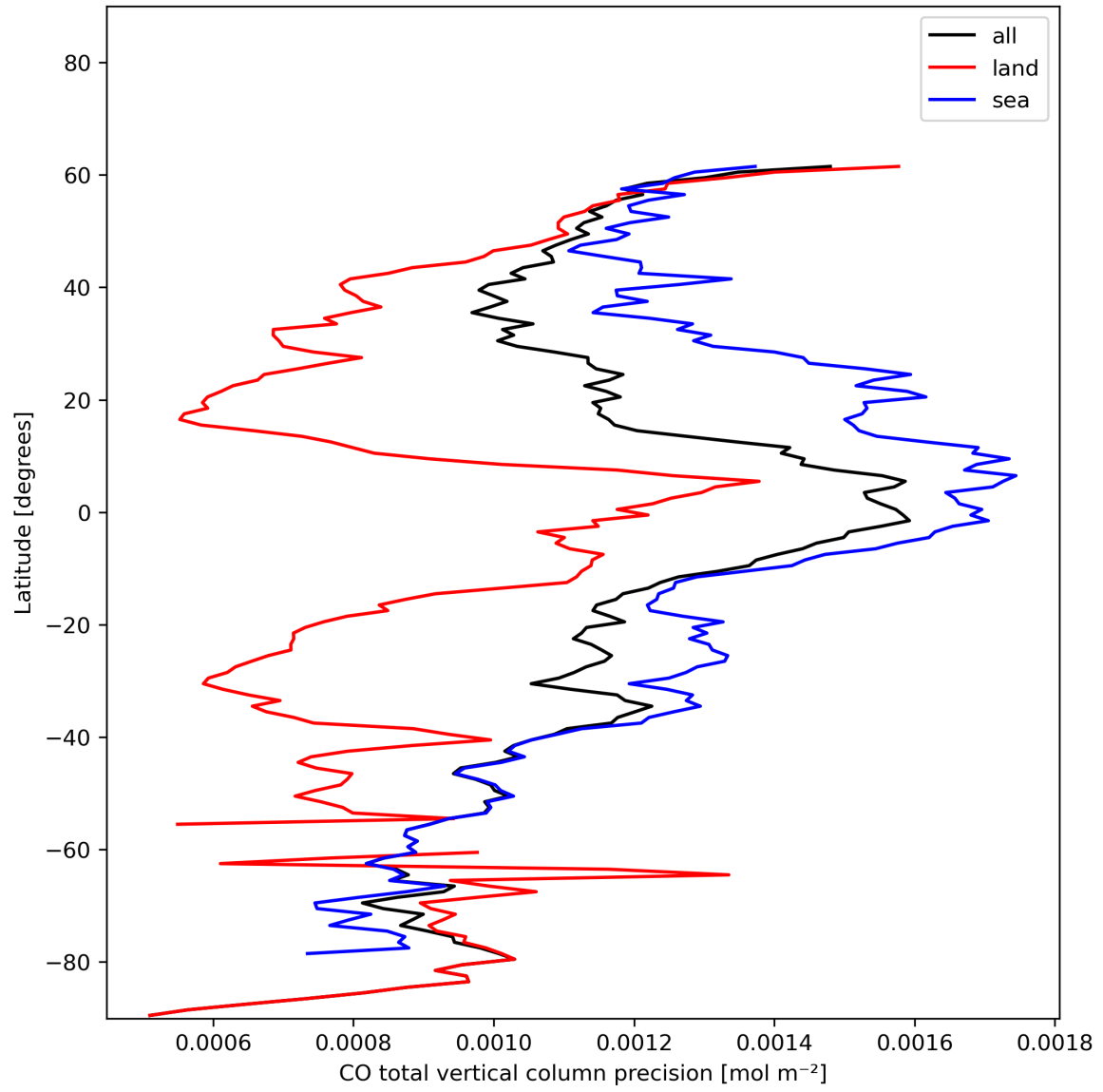
Figure 12: Zonal average of “CO total vertical column precision” for 2023-12-20 to 2023-12-22.
