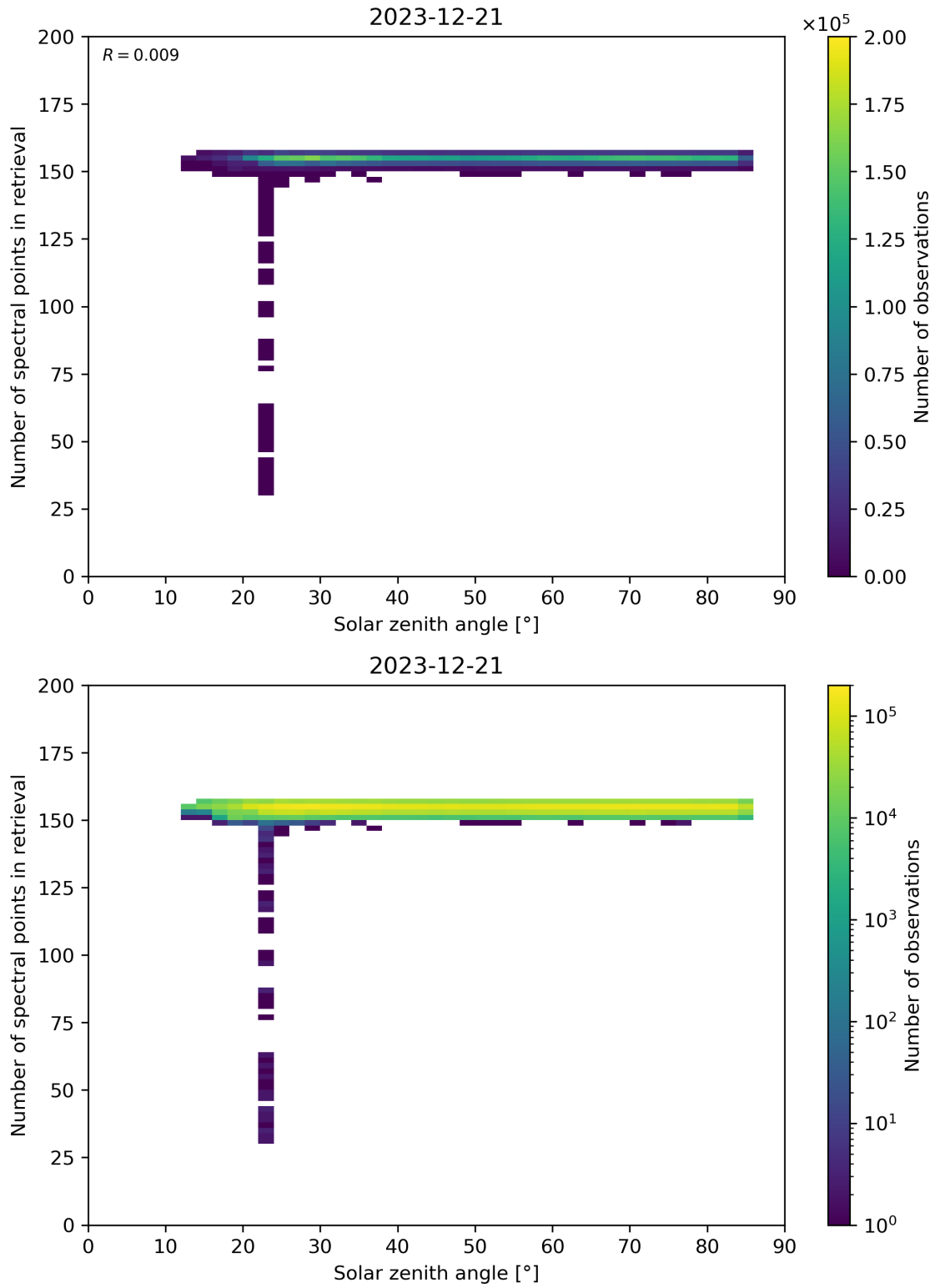
Figure 68: Scatter density plot of “Solar zenith angle” against “Number of spectral points in retrieval” for 2023-12-20 to 2023-12-22.
