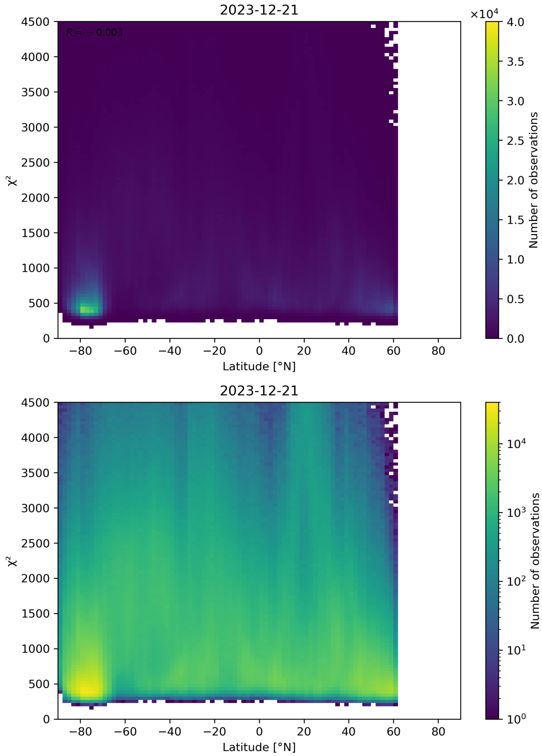
Figure 54: Scatter density plot of “Latitude” against “ \chi^2 ” for 2023-12-20 to 2023-12-22.
