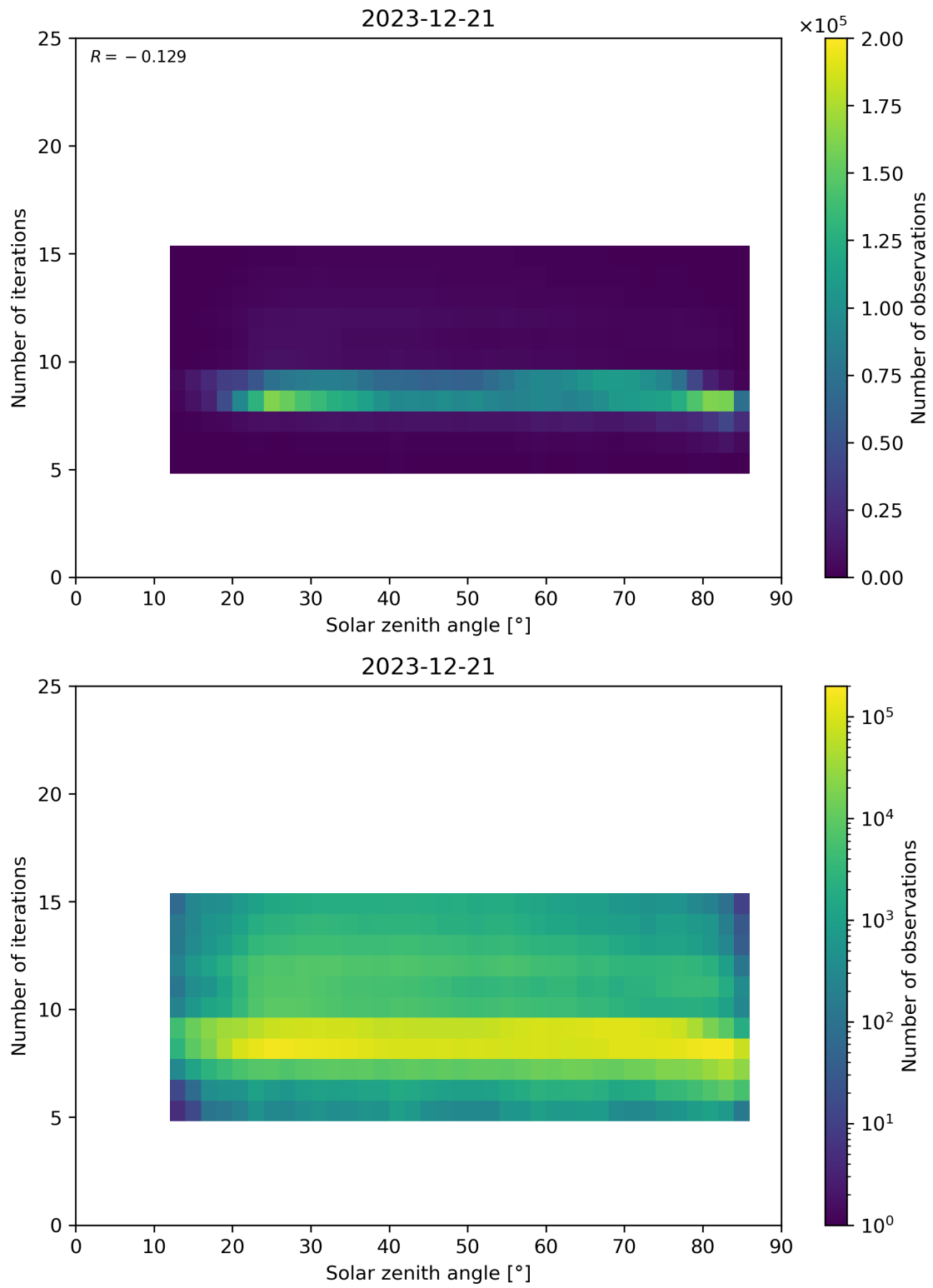
Figure 67: Scatter density plot of “Solar zenith angle” against “Number of iterations” for 2023-12-20 to 2023-12-22.
