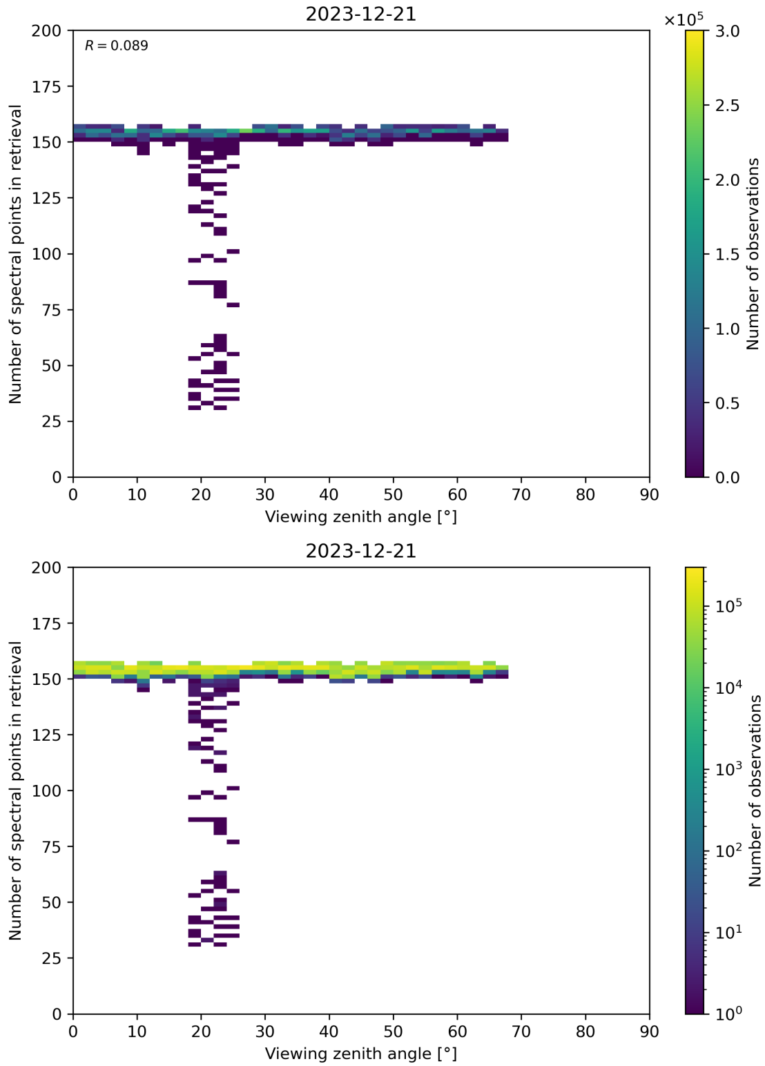
Figure 76: Scatter density plot of “Viewing zenith angle” against “Number of spectral points in retrieval” for 2023-12-20 to 2023-12-22.
