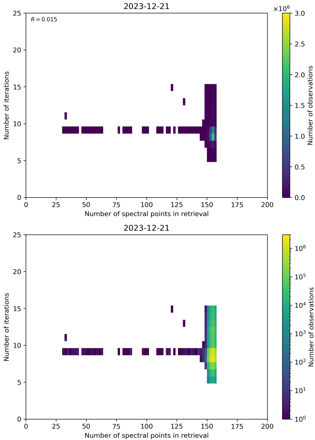
Figure 60: Scatter density plot of “Number of spectral points in retrieval” against “Number of iterations” for 2023-12-20 to 2023-12-22.
