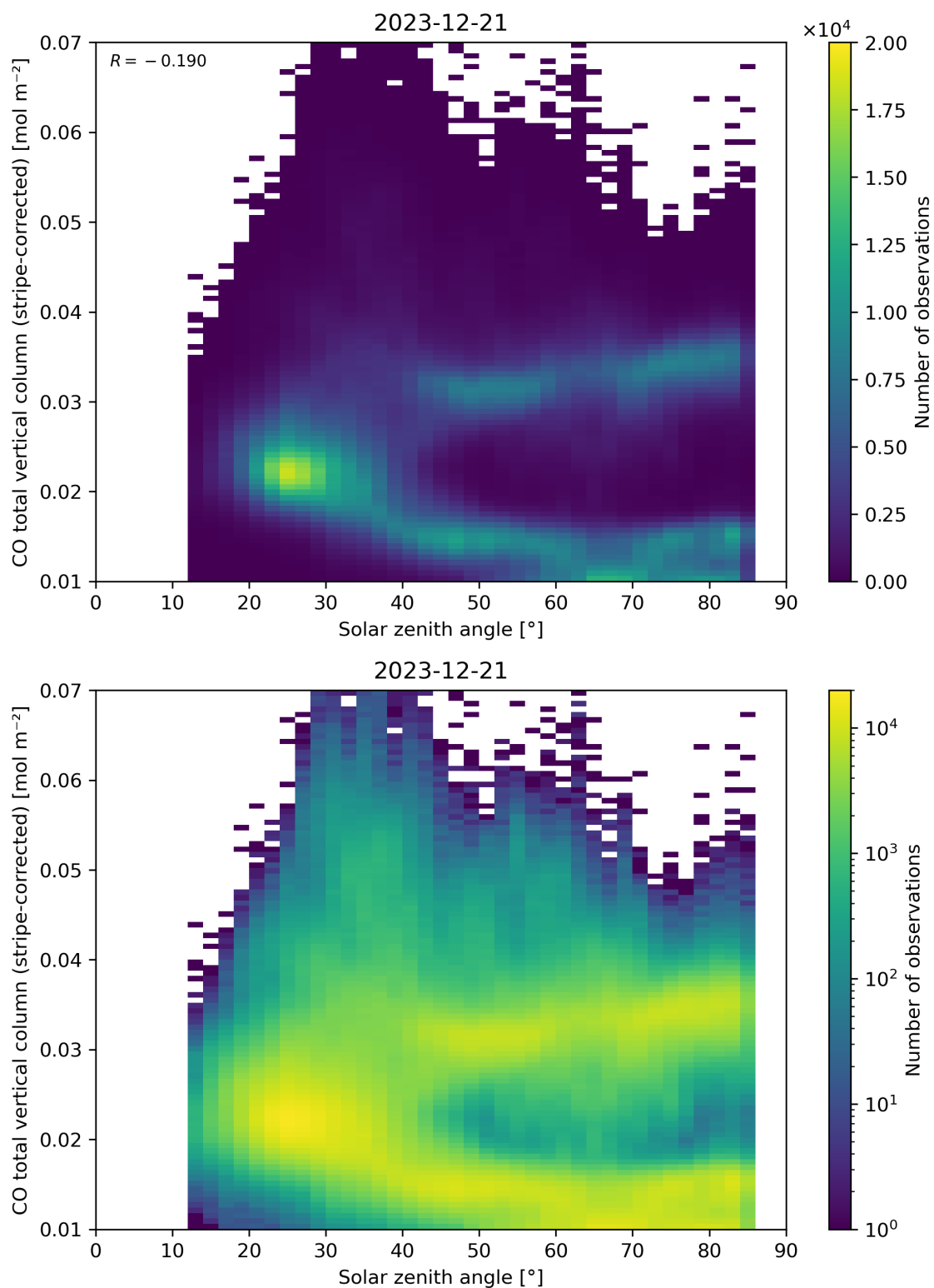
Figure 62: Scatter density plot of “Solar zenith angle” against “CO total vertical column (stripe-corrected)” for 2023-12-20 to 2023-12-22.
