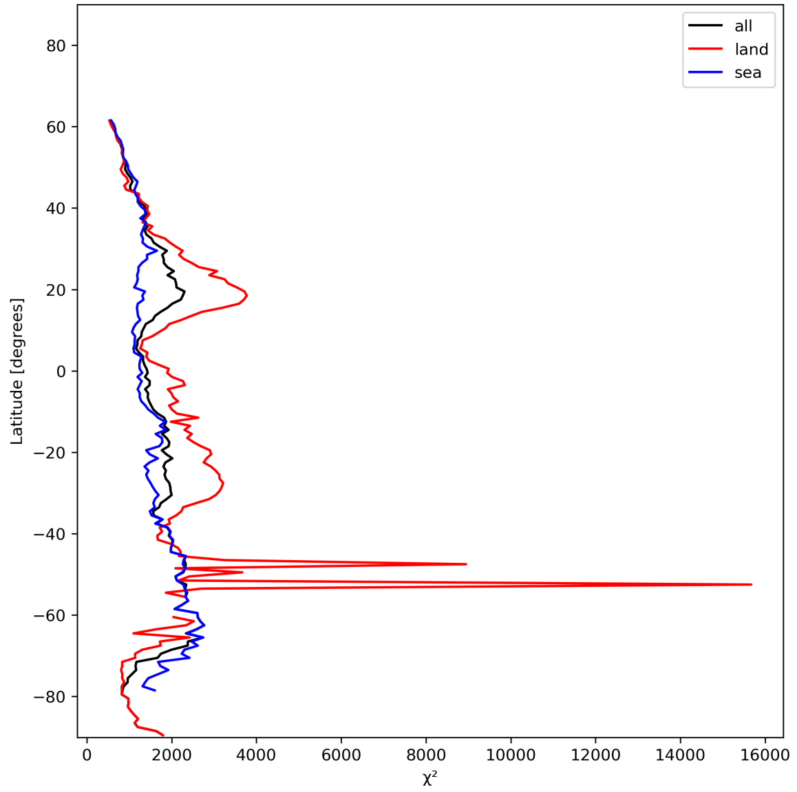
Figure 14: Zonal average of “ \chi^2 ” for 2023-12-20 to 2023-12-22.
