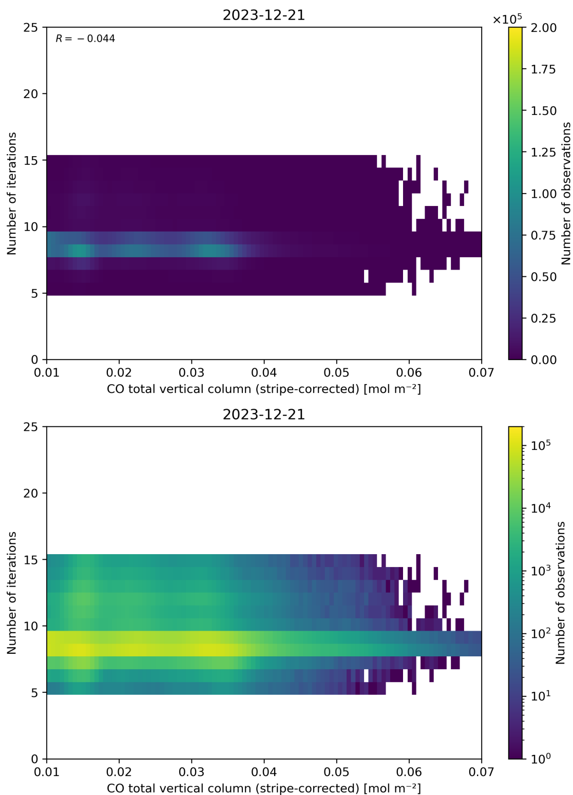
Figure 39: Scatter density plot of “CO total vertical column (stripe-corrected)” against “Number of iterations” for 2023-12-20 to 2023-12-22.
