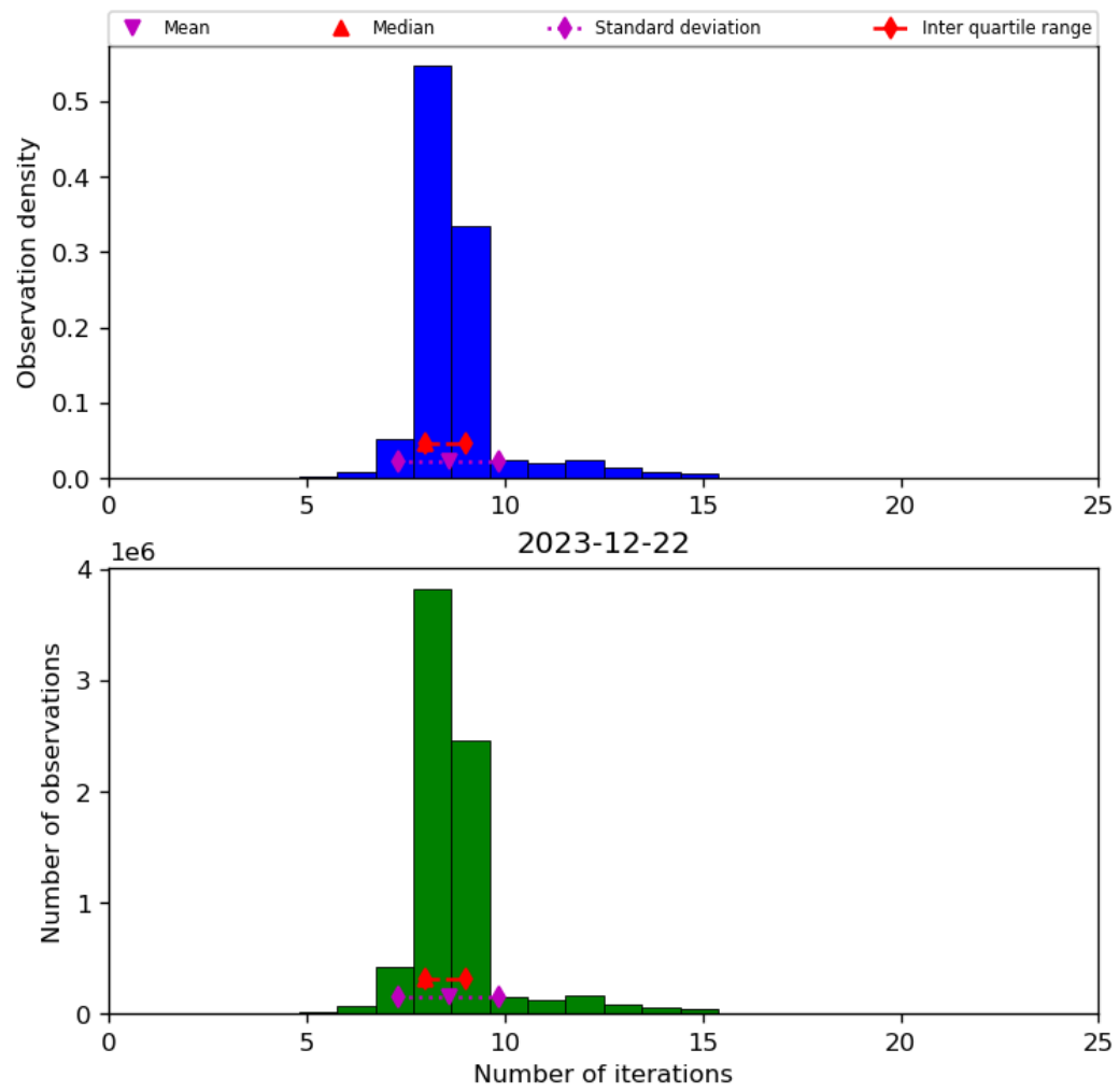
Figure 24: Histogram of “Number of iterations” for 2023-12-21 to 2023-12-23
