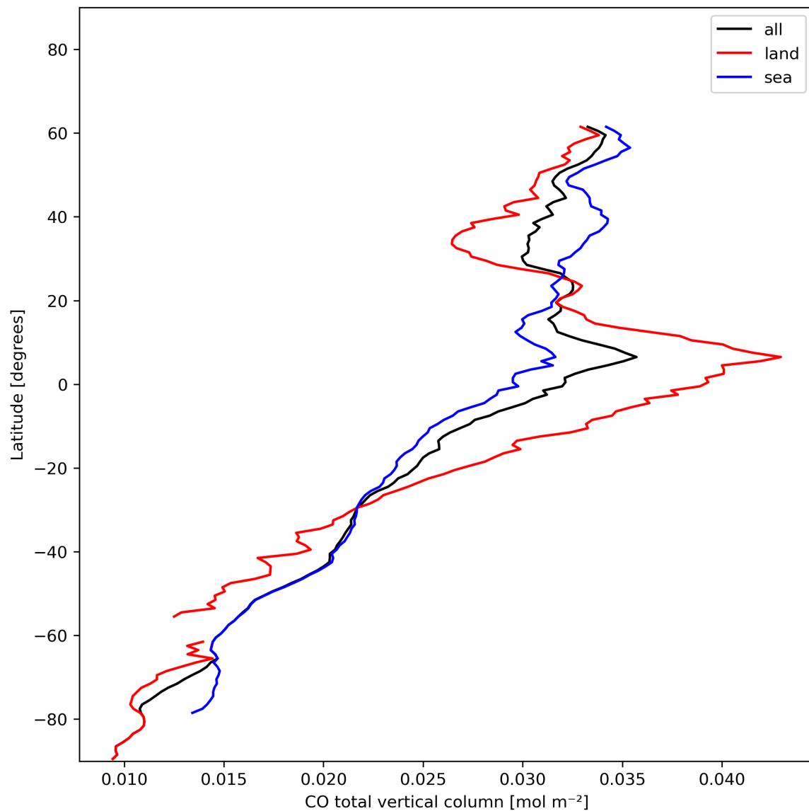
Figure 10: Zonal average of “CO total vertical column” for 2023-12-21 to 2023-12-23.
