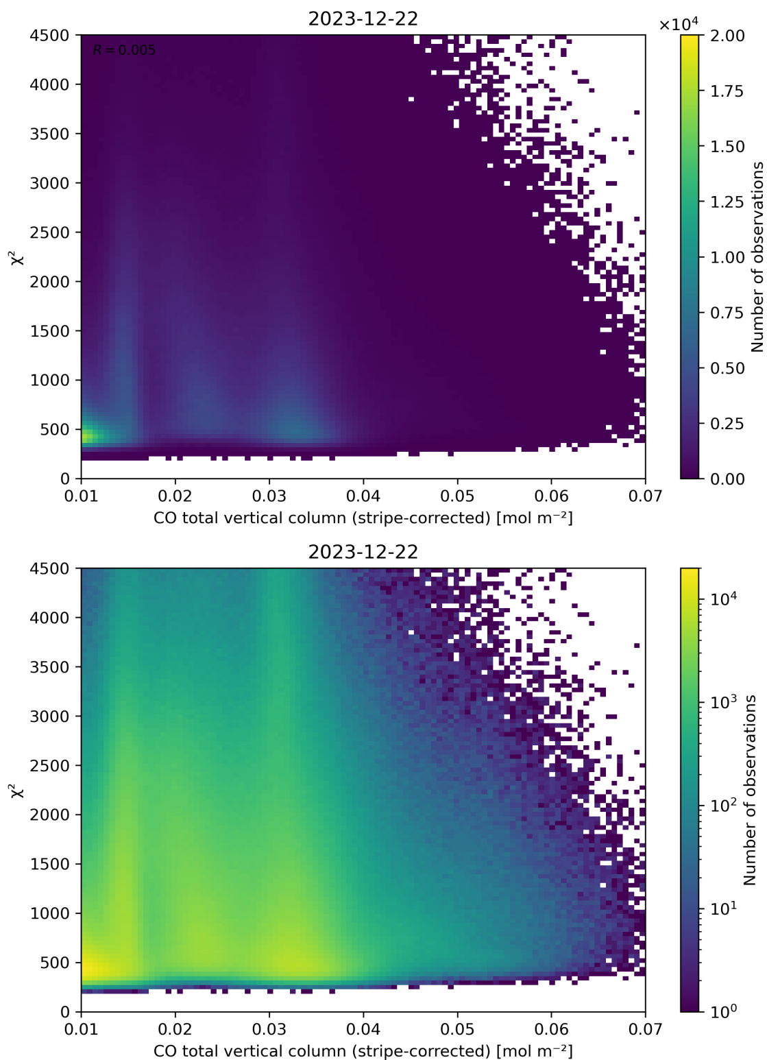
Figure 37: Scatter density plot of “CO total vertical column (stripe-corrected)” against “ \chi^2 ” for 2023-12-21 to 2023-12-23.
