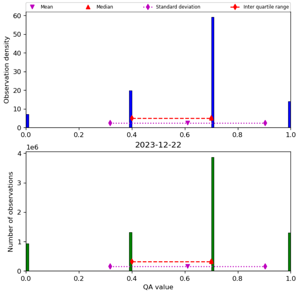
Figure 17: Histogram of “QA value” for 2023-12-21 to 2023-12-23
