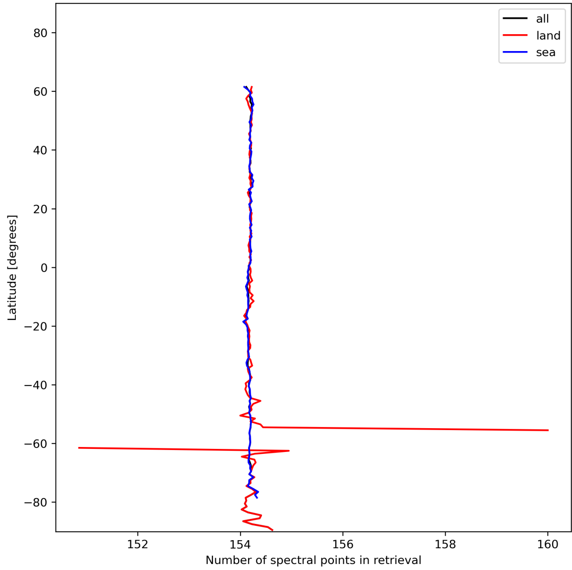
Figure 13: Zonal average of “Number of spectral points in retrieval” for 2023-12-21 to 2023-12-23.
