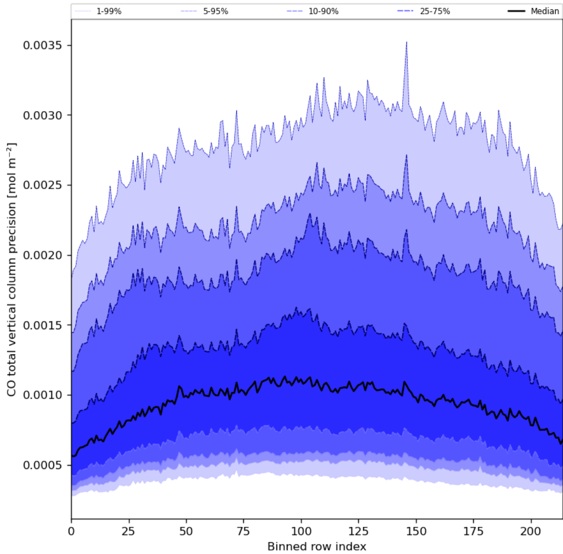
Figure 28: Along track statistics of “CO total vertical column precision” for 2023-12-21 to 2023-12-23
