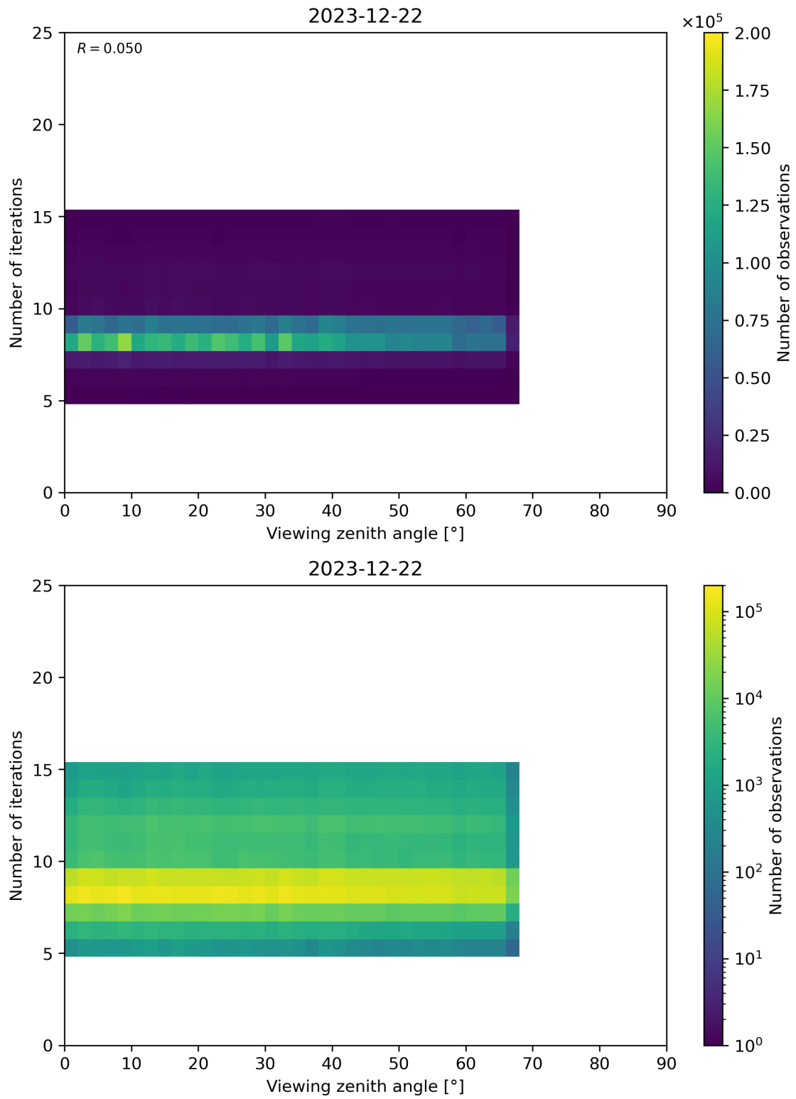
Figure 75: Scatter density plot of “Viewing zenith angle” against “Number of iterations” for 2023-12-21 to 2023-12-23.
