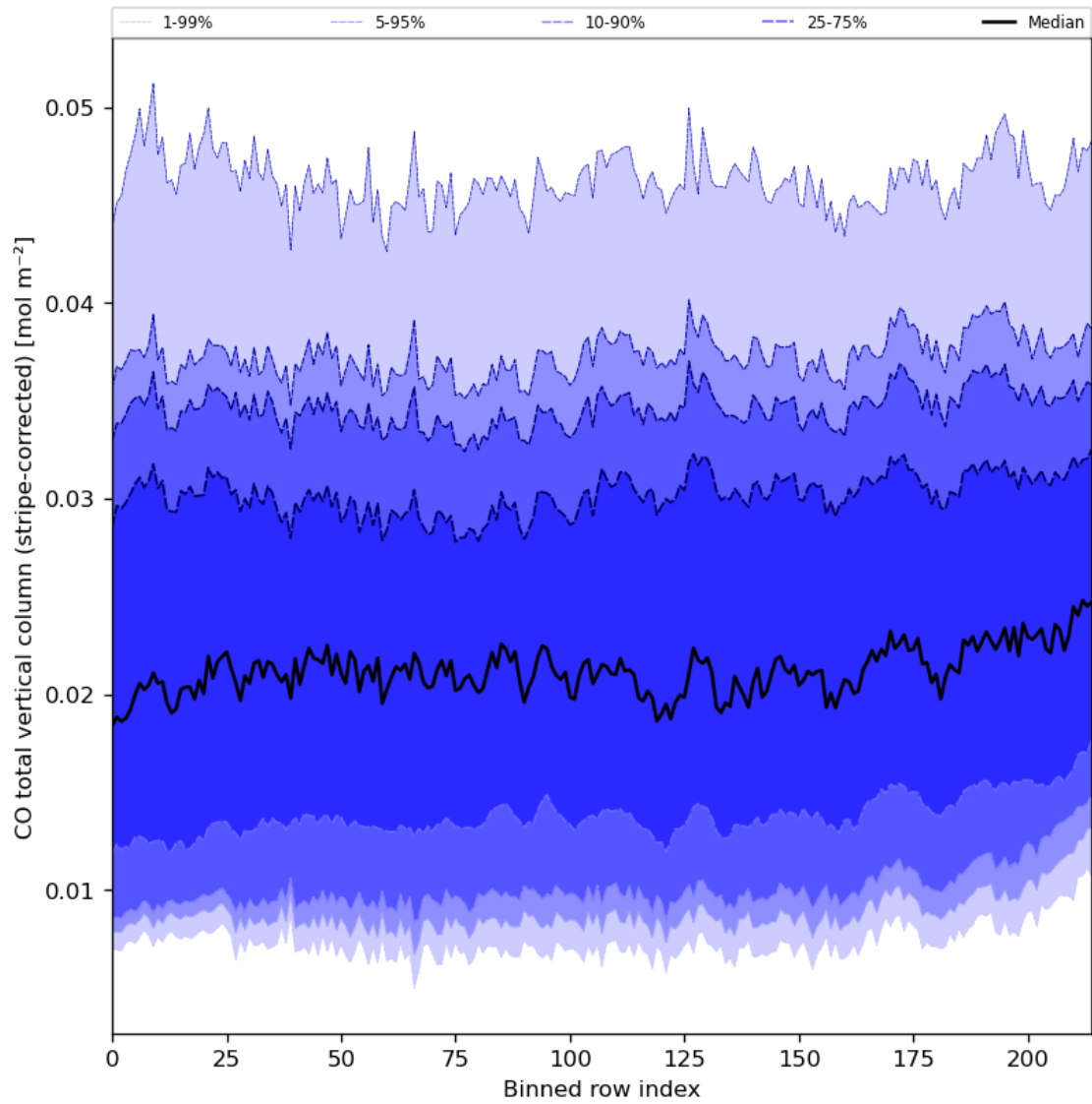
Figure 27: Along track statistics of “CO total vertical column (stripe-corrected)” for 2023-12-21 to 2023-12-23
