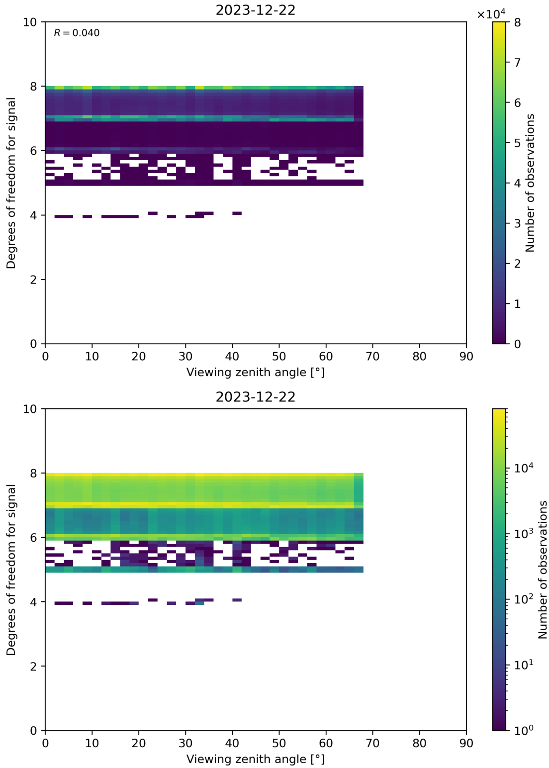
Figure 73: Scatter density plot of “Viewing zenith angle” against “Degrees of freedom for signal” for 2023-12-21 to 2023-12-23.
