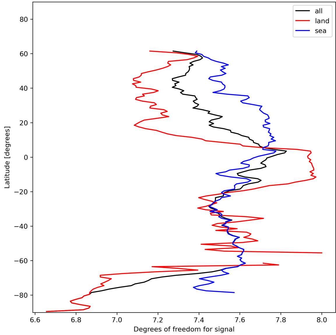
Figure 15: Zonal average of “Degrees of freedom for signal” for 2023-12-21 to 2023-12-23.
