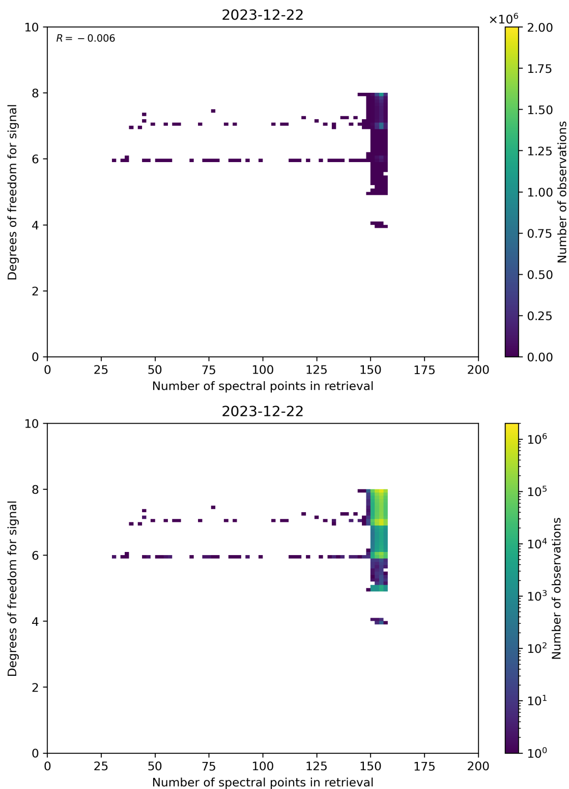
Figure 59: Scatter density plot of “Number of spectral points in retrieval” against “Degrees of freedom for signal” for 2023-12-21 to 2023-12-23.
