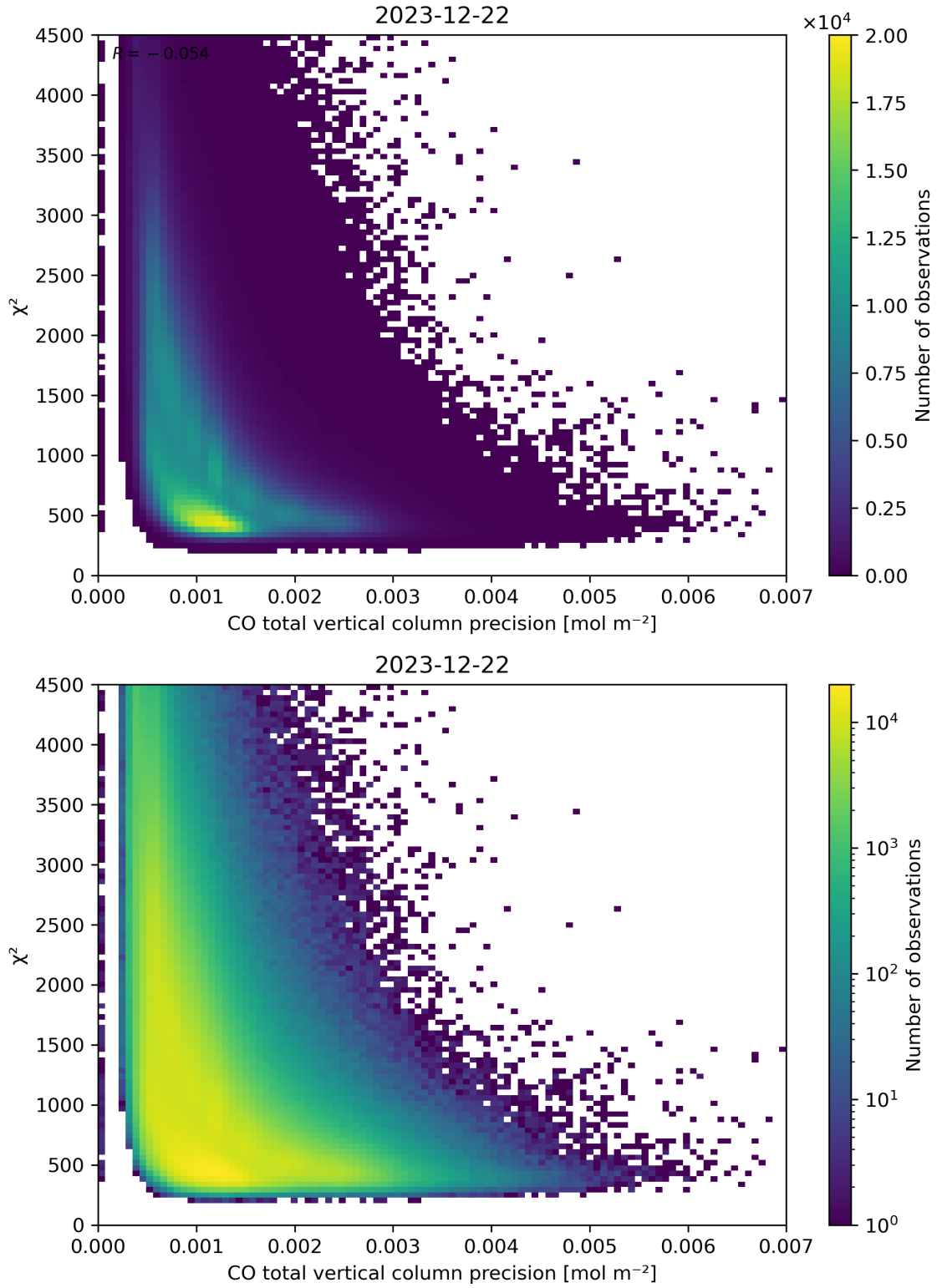
Figure 44: Scatter density plot of “CO total vertical column precision” against “ \chi^2 ” for 2023-12-21 to 2023-12-23.
