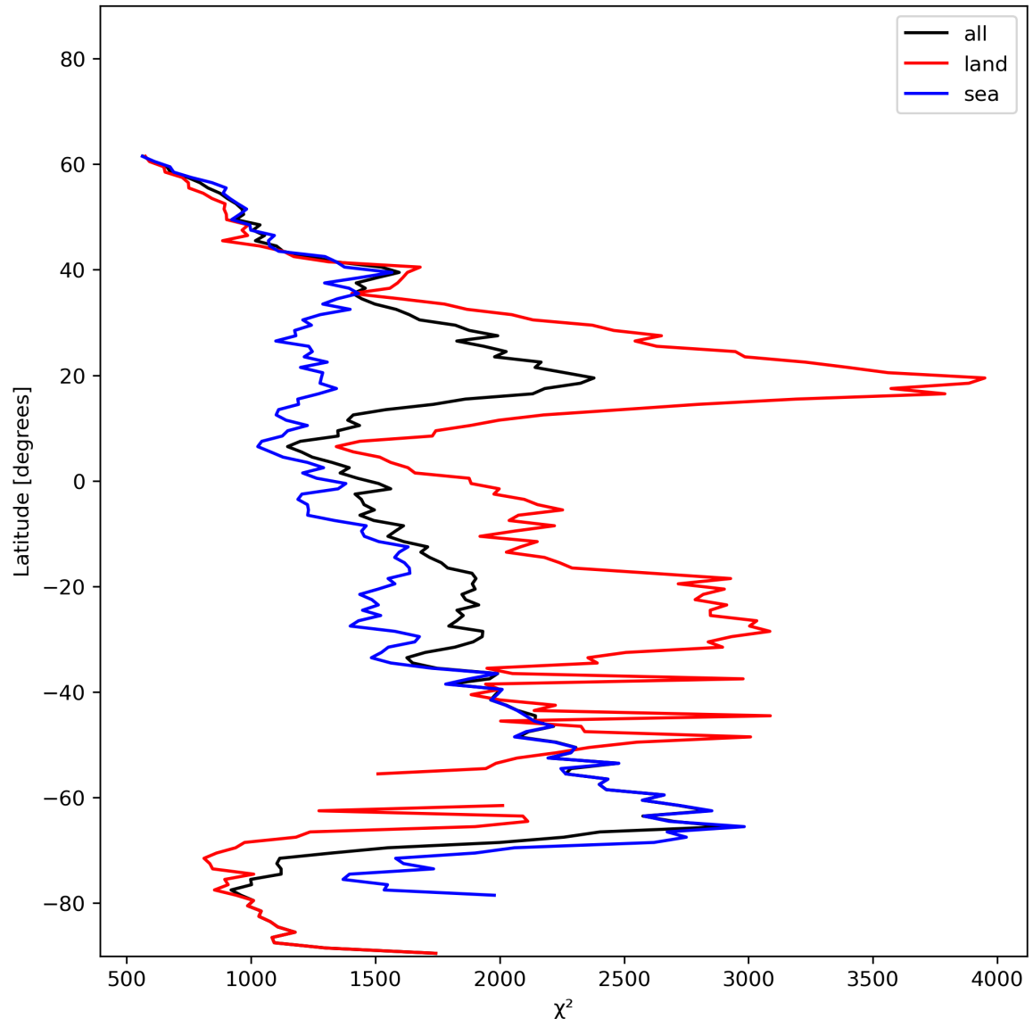
Figure 14: Zonal average of “ \chi^2 ” for 2023-12-21 to 2023-12-23.
