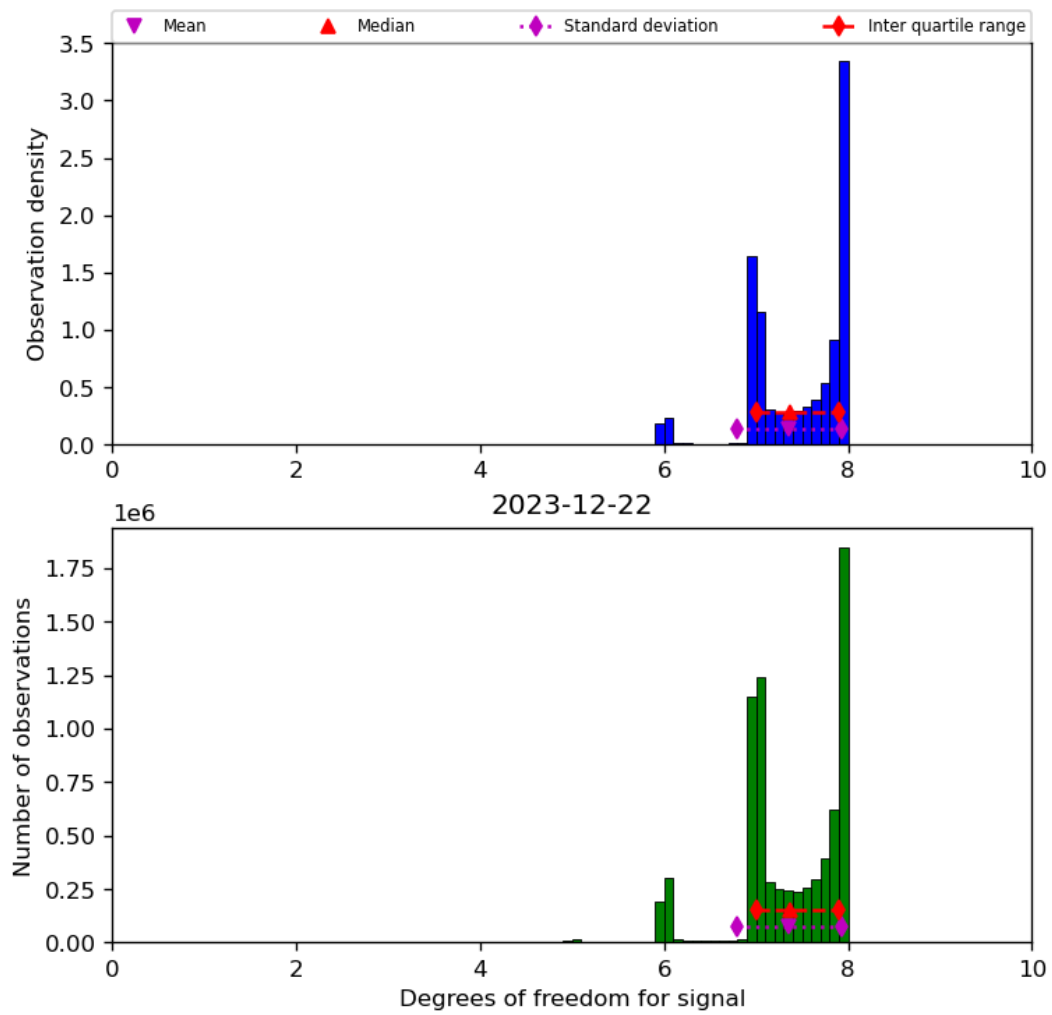
Figure 23: Histogram of “Degrees of freedom for signal” for 2023-12-21 to 2023-12-23
