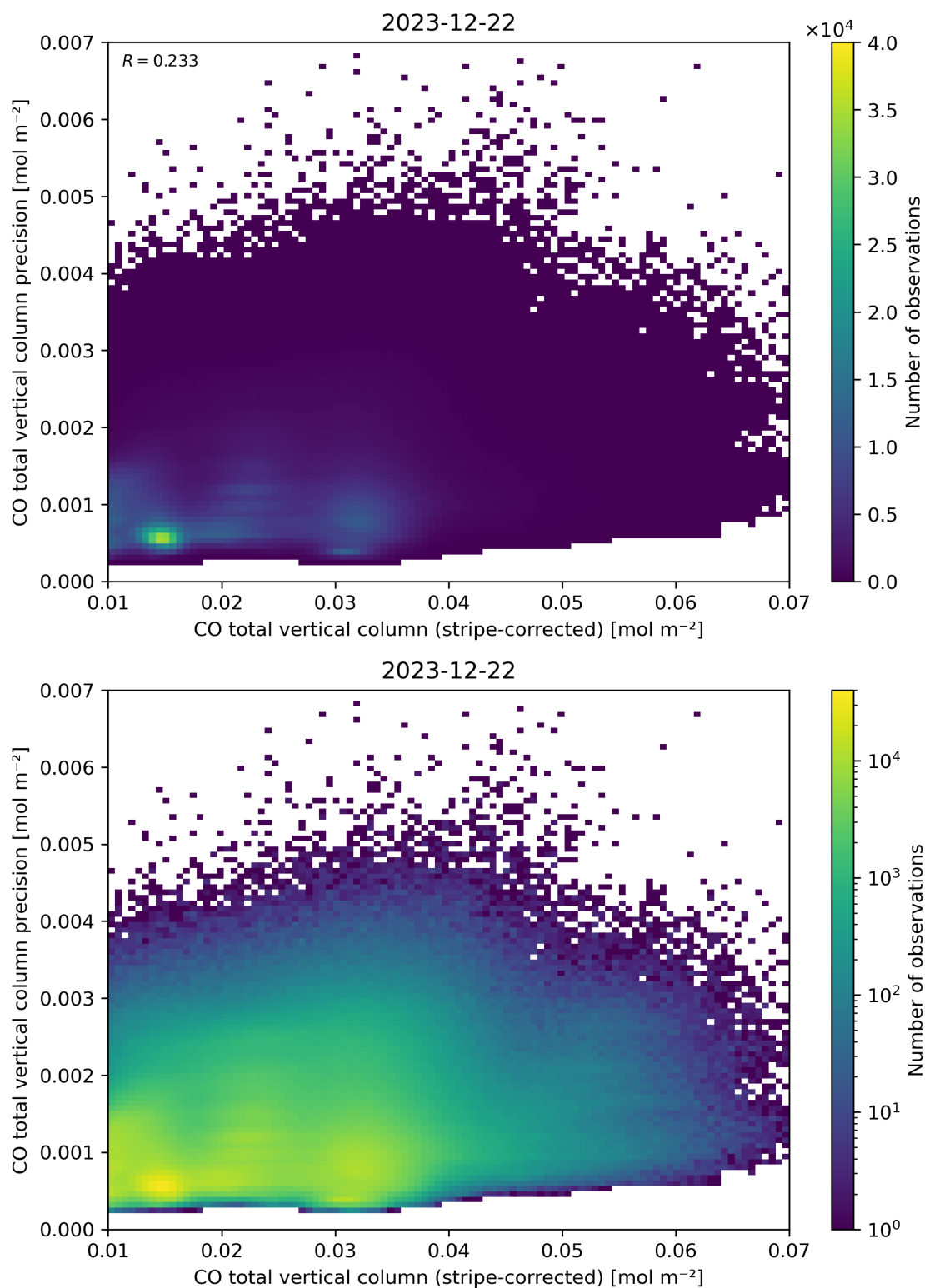
Figure 36: Scatter density plot of “CO total vertical column (stripe-corrected)” against “CO total vertical column precision” for 2023-12-21 to 2023-12-23.
