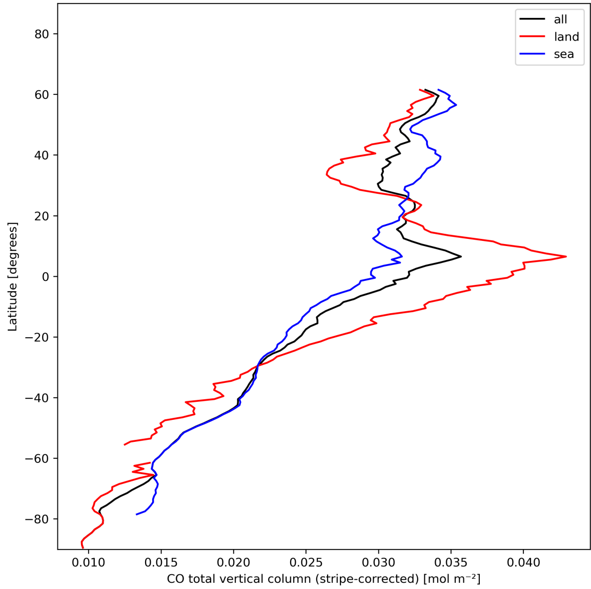
Figure 11: Zonal average of “CO total vertical column (stripe-corrected)” for 2023-12-21 to 2023-12-23.
