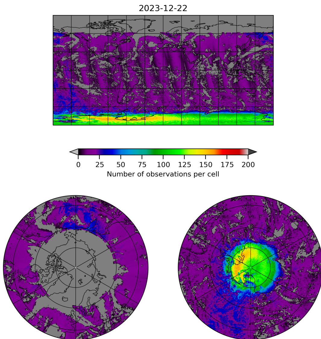
Figure 8: Map of the number of observations for 2023-12-21 to 2023-12-23
