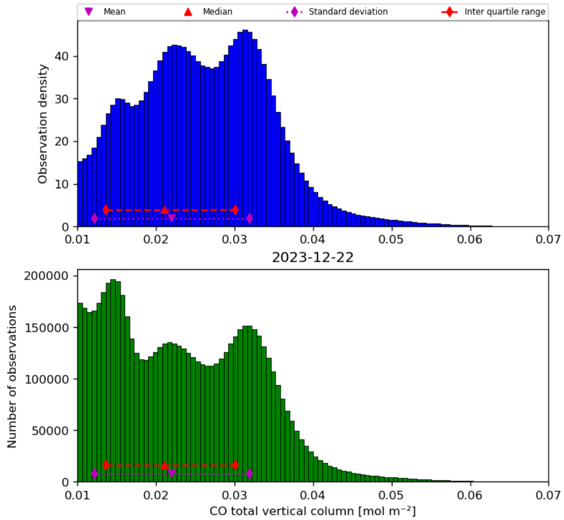
Figure 18: Histogram of “CO total vertical column” for 2023-12-21 to 2023-12-23
