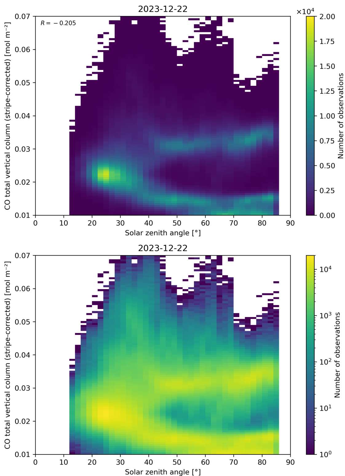
Figure 62: Scatter density plot of “Solar zenith angle” against “CO total vertical column (stripe-corrected)” for 2023-12-21 to 2023-12-23.
