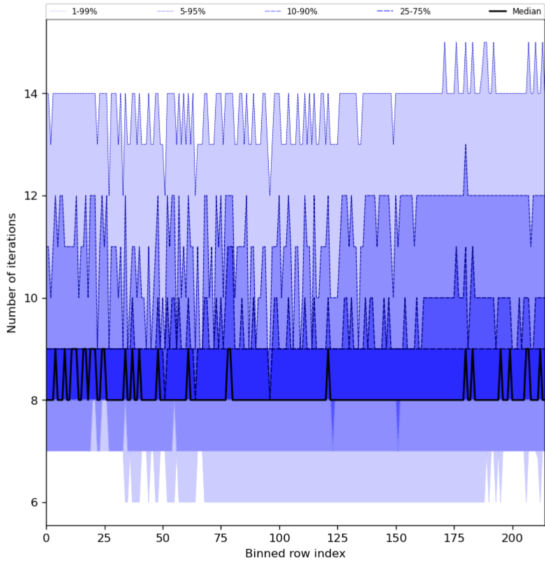
Figure 32: Along track statistics of “Number of iterations” for 2023-12-21 to 2023-12-23
