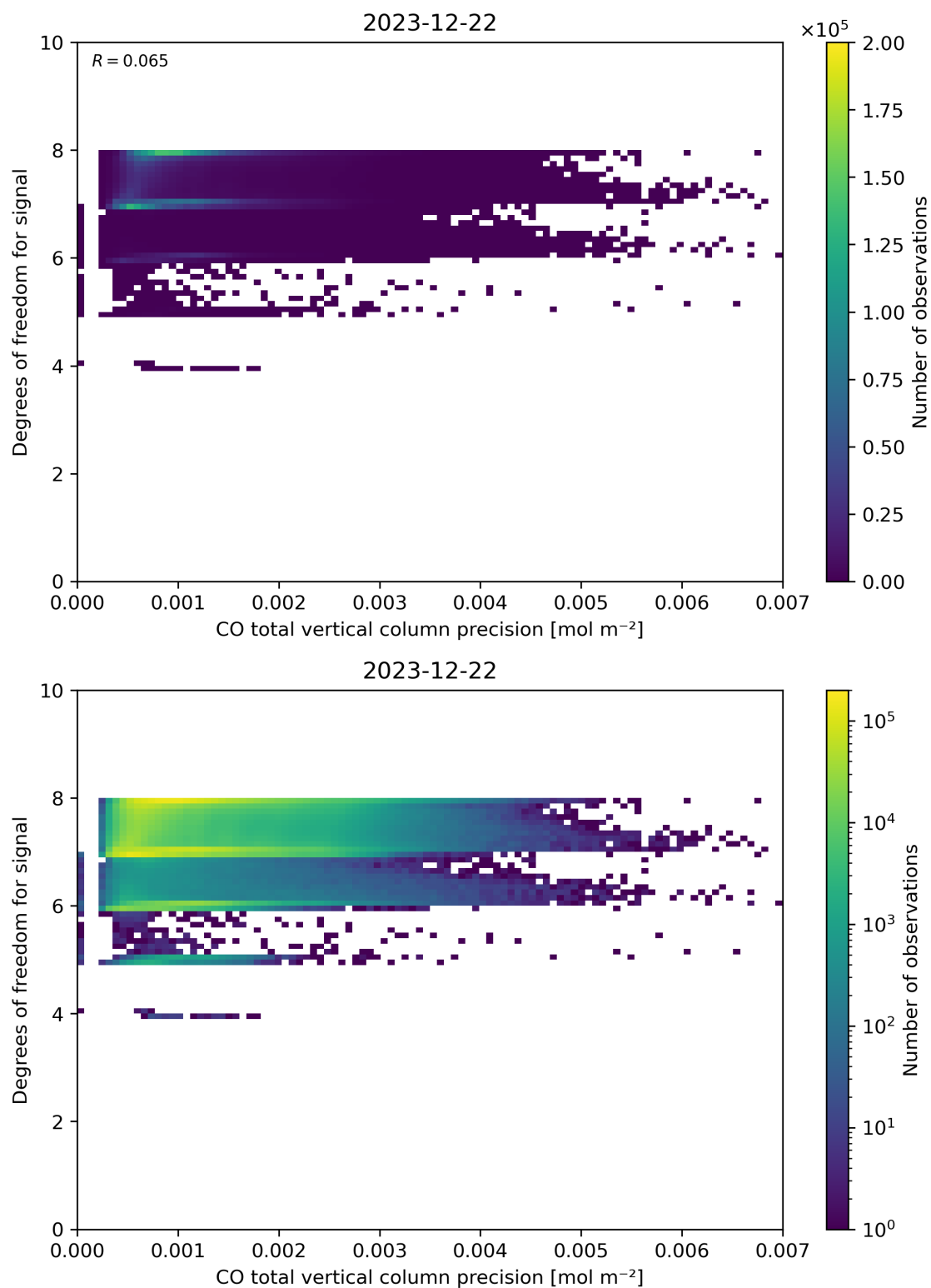
Figure 45: Scatter density plot of “CO total vertical column precision” against “Degrees of freedom for signal” for 2023-12-21 to 2023-12-23.
