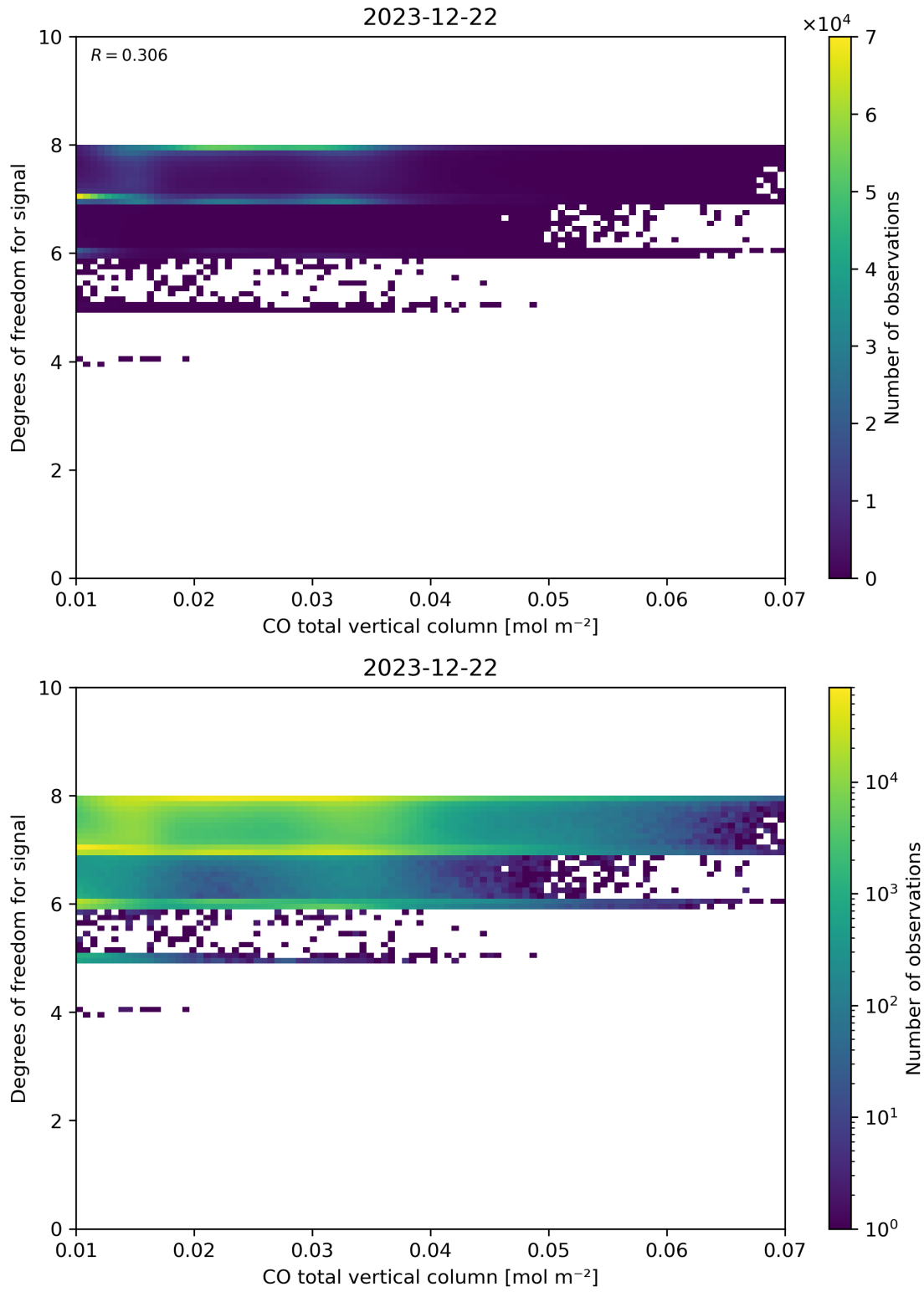
Figure 41: Scatter density plot of “CO total vertical column” against “Degrees of freedom for signal” for 2023-12-21 to 2023-12-23.
