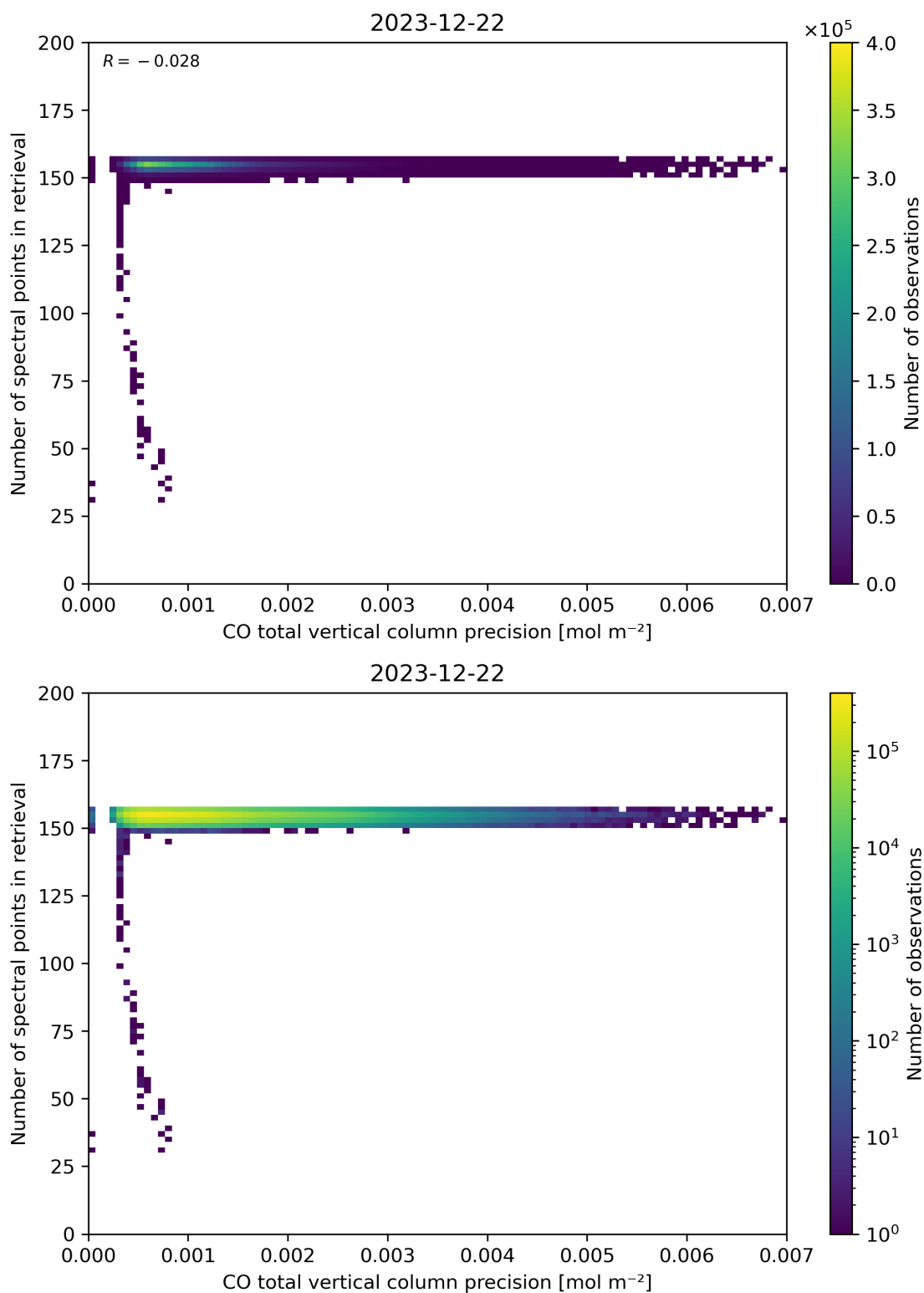
Figure 47: Scatter density plot of “CO total vertical column precision” against “Number of spectral points in retrieval” for 2023-12-21 to 2023-12-23.
