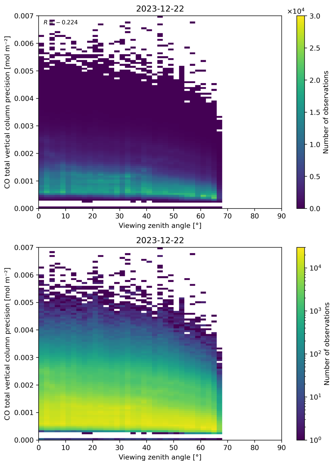
Figure 71: Scatter density plot of “Viewing zenith angle” against “CO total vertical column precision” for 2023-12-21 to 2023-12-23.
