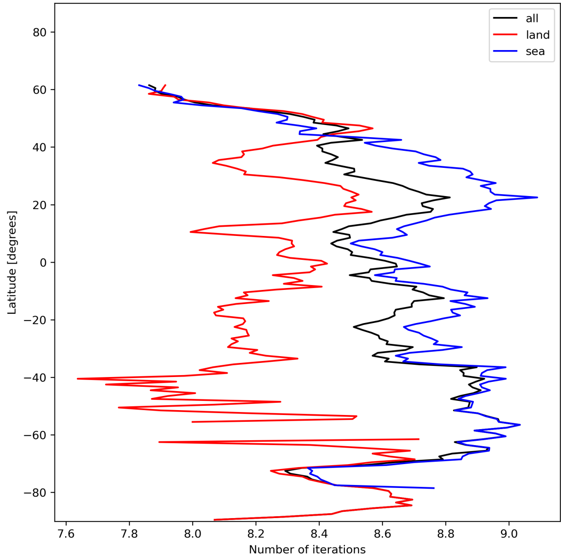
Figure 16: Zonal average of “Number of iterations” for 2023-12-21 to 2023-12-23.
