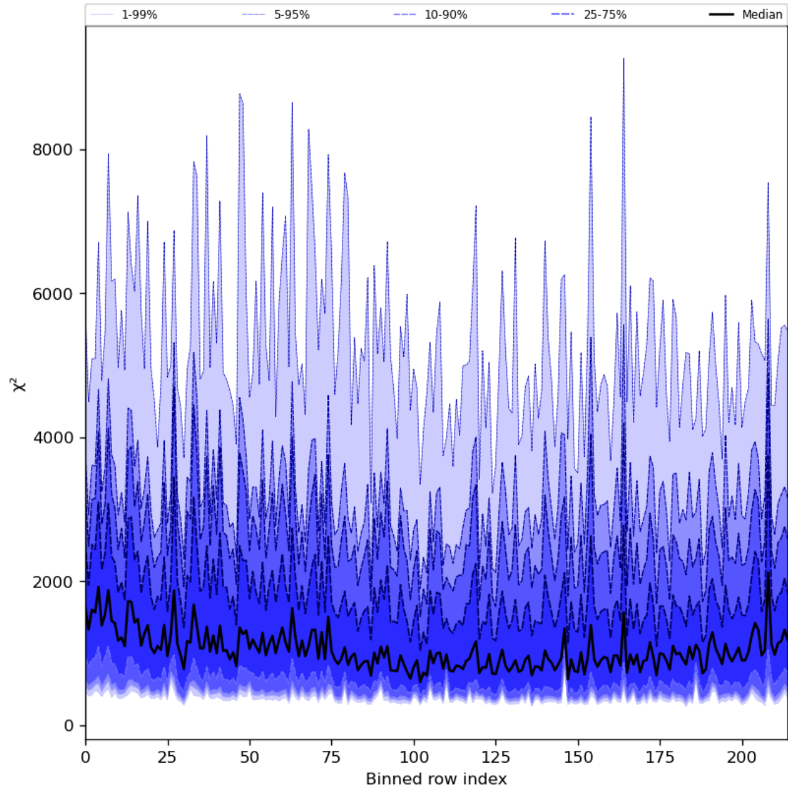
Figure 30: Along track statistics of “ \chi^2 ” for 2023-12-21 to 2023-12-23
