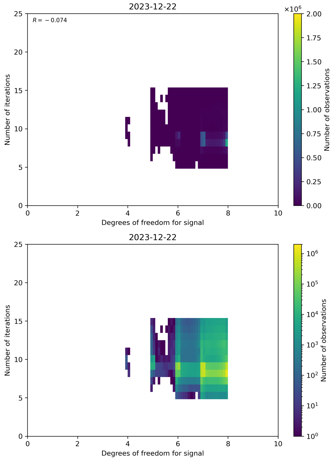
Figure 50: Scatter density plot of “Degrees of freedom for signal” against “Number of iterations” for 2023-12-21 to 2023-12-23.
