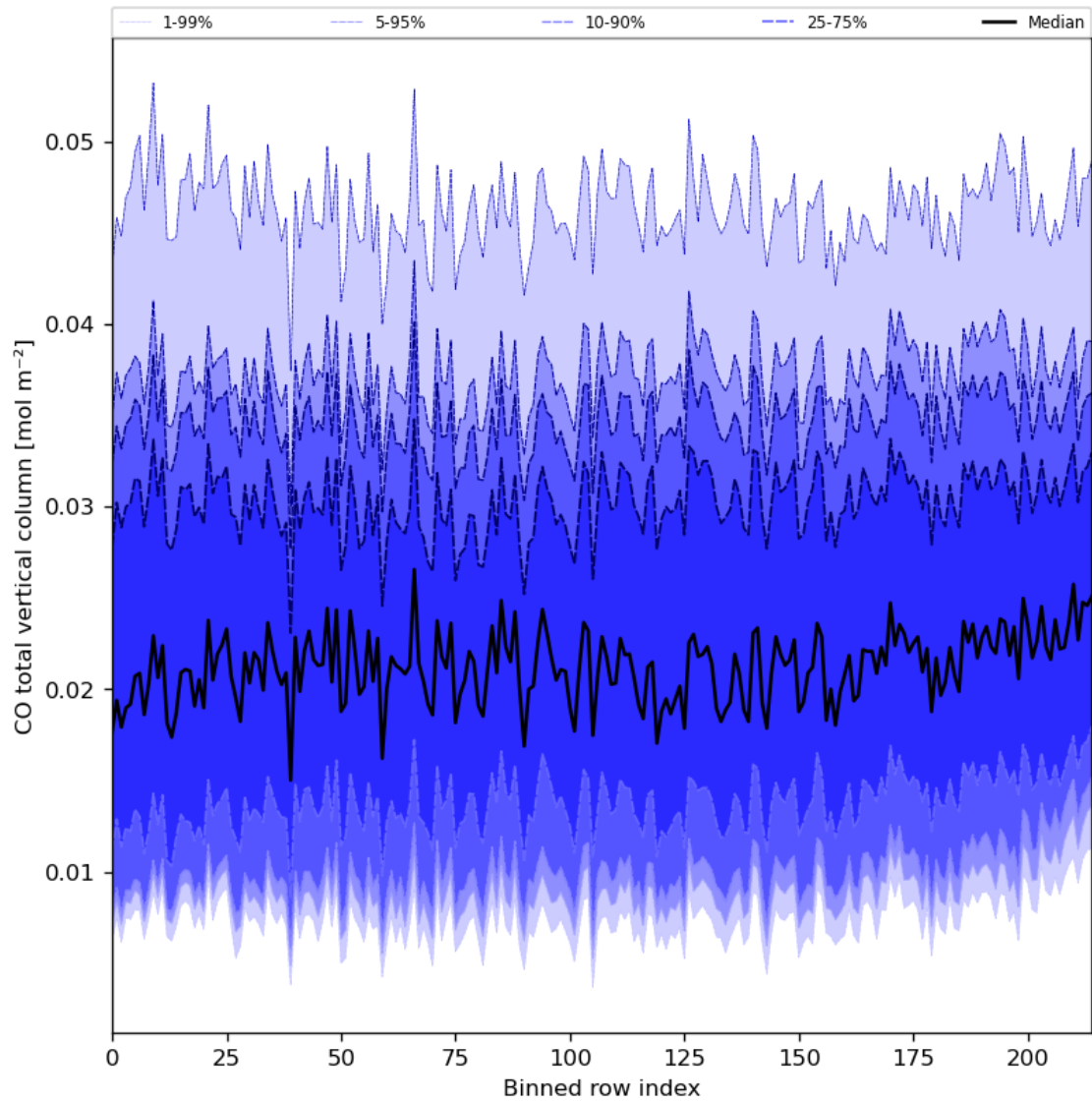
Figure 26: Along track statistics of “CO total vertical column” for 2023-12-21 to 2023-12-23
