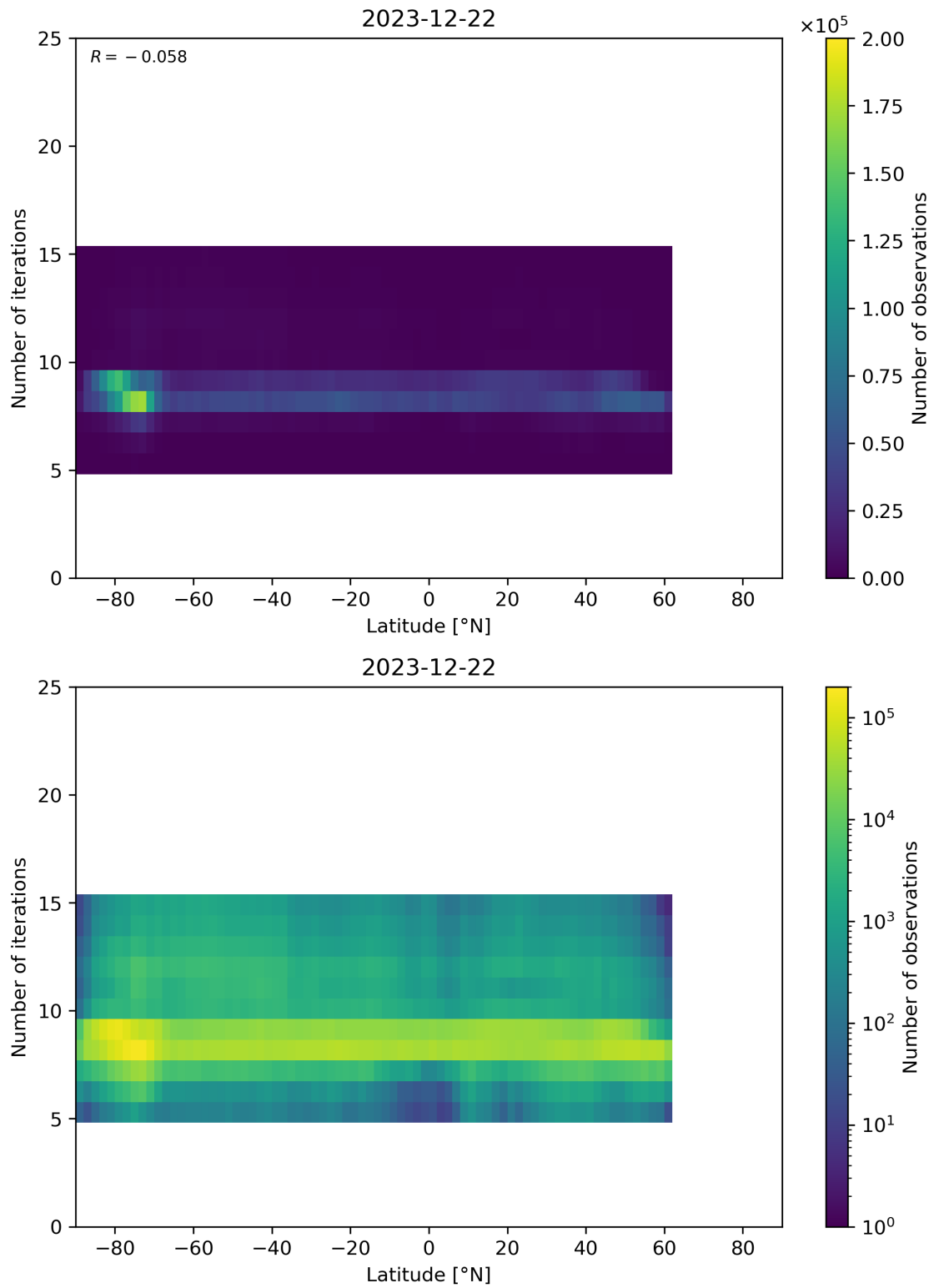
Figure 56: Scatter density plot of “Latitude” against “Number of iterations” for 2023-12-21 to 2023-12-23.
