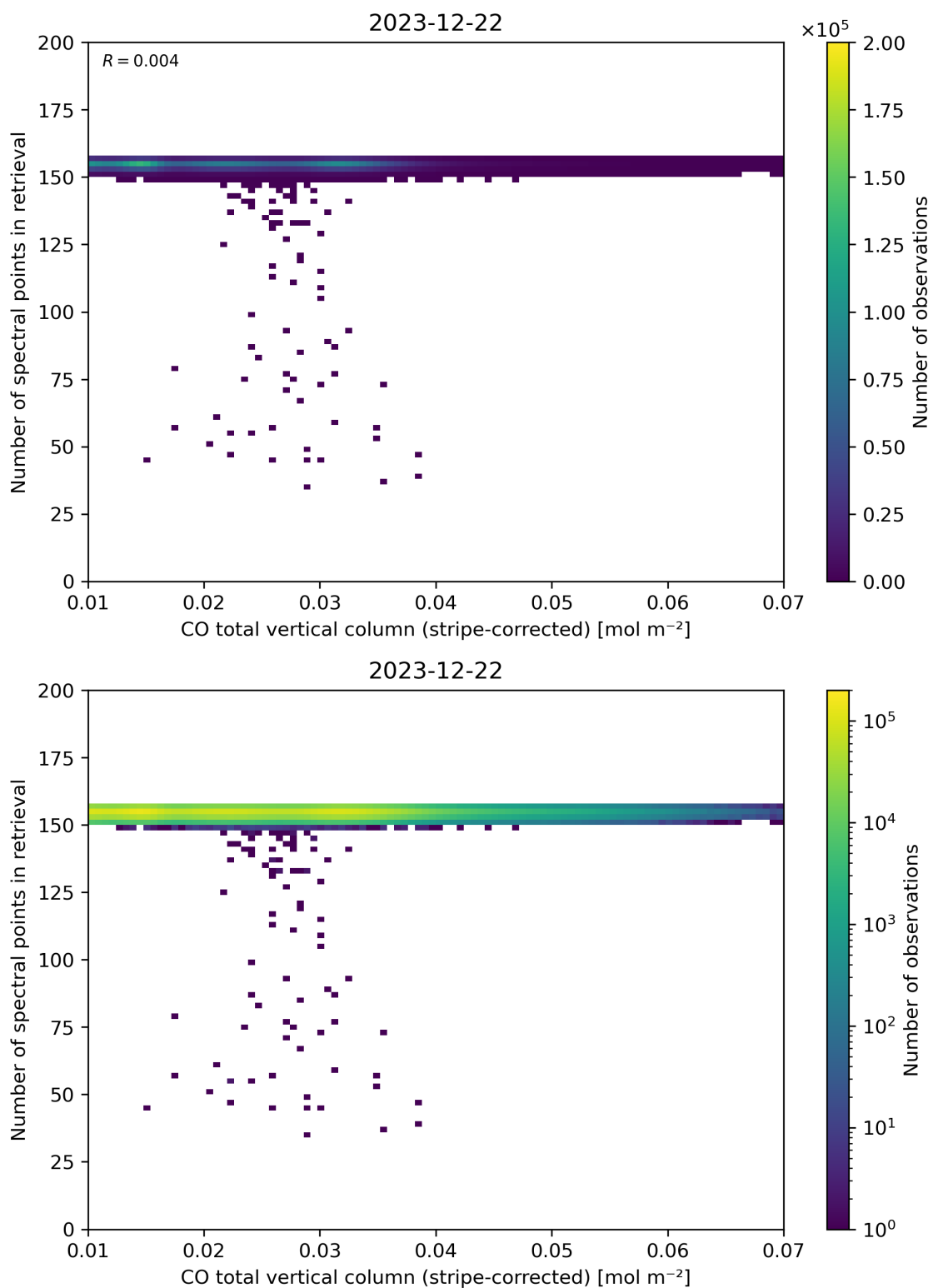
Figure 40: Scatter density plot of “CO total vertical column (stripe-corrected)” against “Number of spectral points in retrieval” for 2023-12-21 to 2023-12-23.
