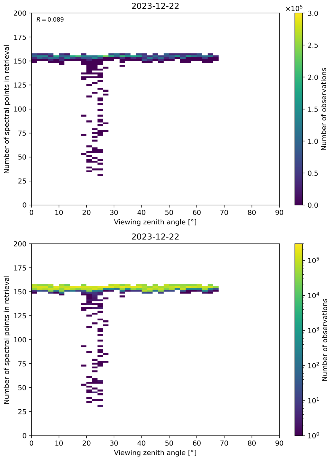
Figure 76: Scatter density plot of “Viewing zenith angle” against “Number of spectral points in retrieval” for 2023-12-21 to 2023-12-23.
