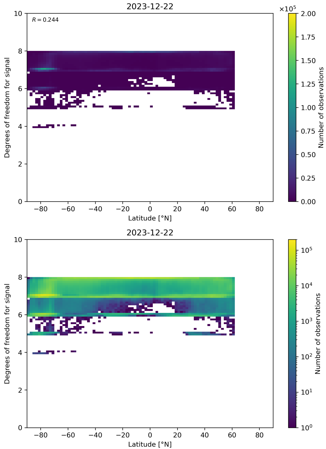
Figure 55: Scatter density plot of “Latitude” against “Degrees of freedom for signal” for 2023-12-21 to 2023-12-23.
