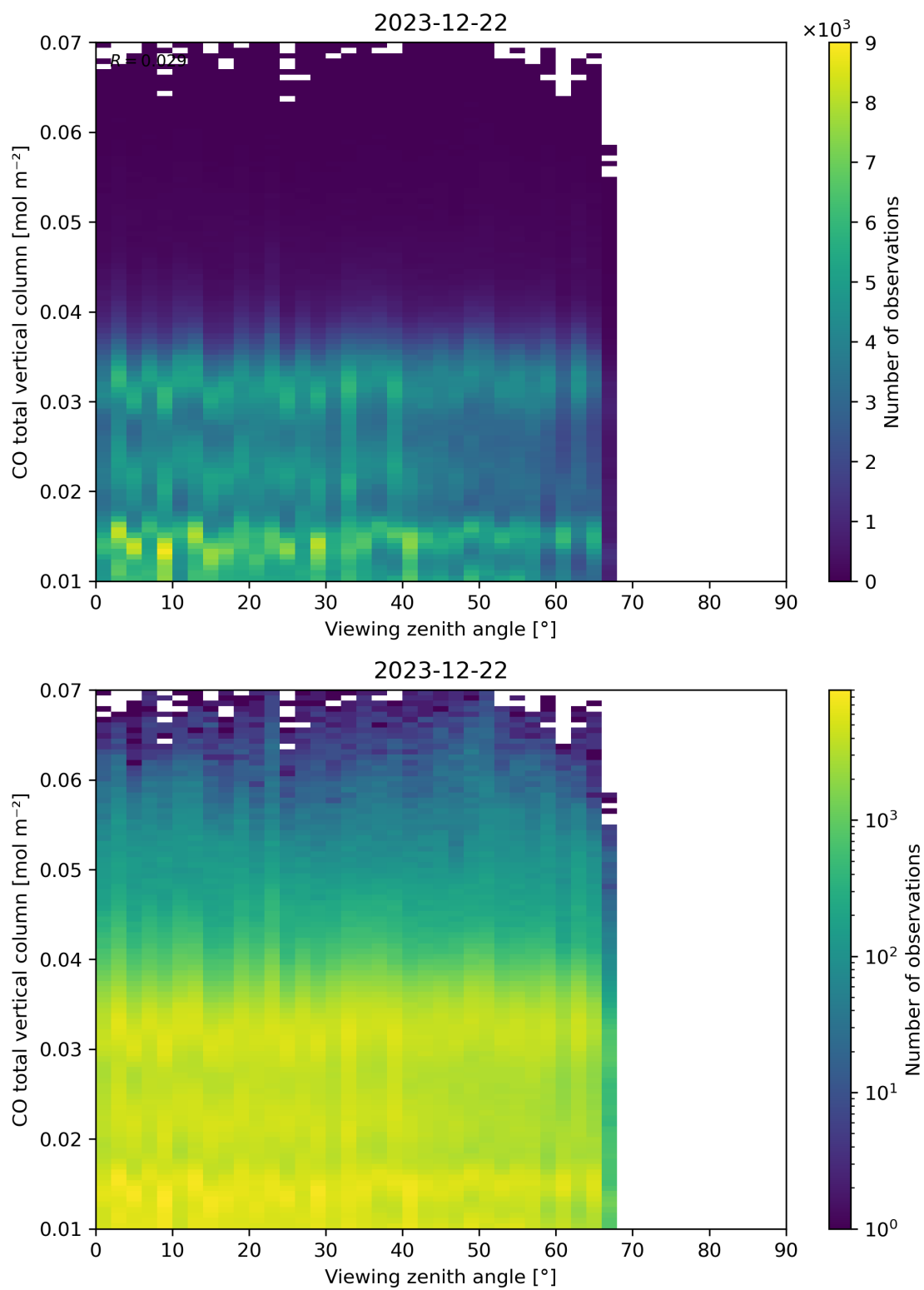
Figure 69: Scatter density plot of “Viewing zenith angle” against “CO total vertical column” for 2023-12-21 to 2023-12-23.
