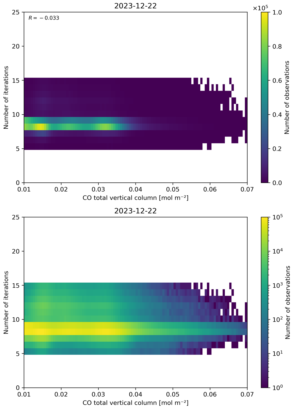
Figure 42: Scatter density plot of “CO total vertical column” against “Number of iterations” for 2023-12-21 to 2023-12-23.
