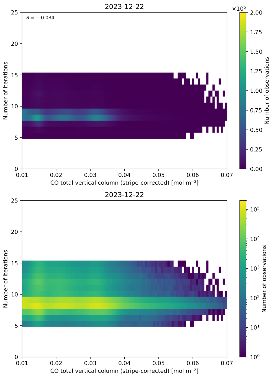
Figure 39: Scatter density plot of “CO total vertical column (stripe-corrected)” against “Number of iterations” for 2023-12-21 to 2023-12-23.
