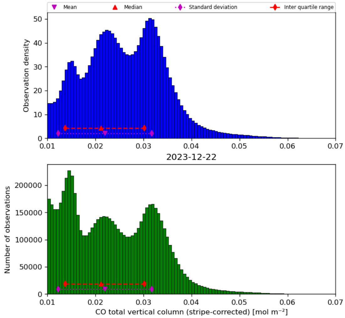
Figure 19: Histogram of “CO total vertical column (stripe-corrected)” for 2023-12-21 to 2023-12-23
