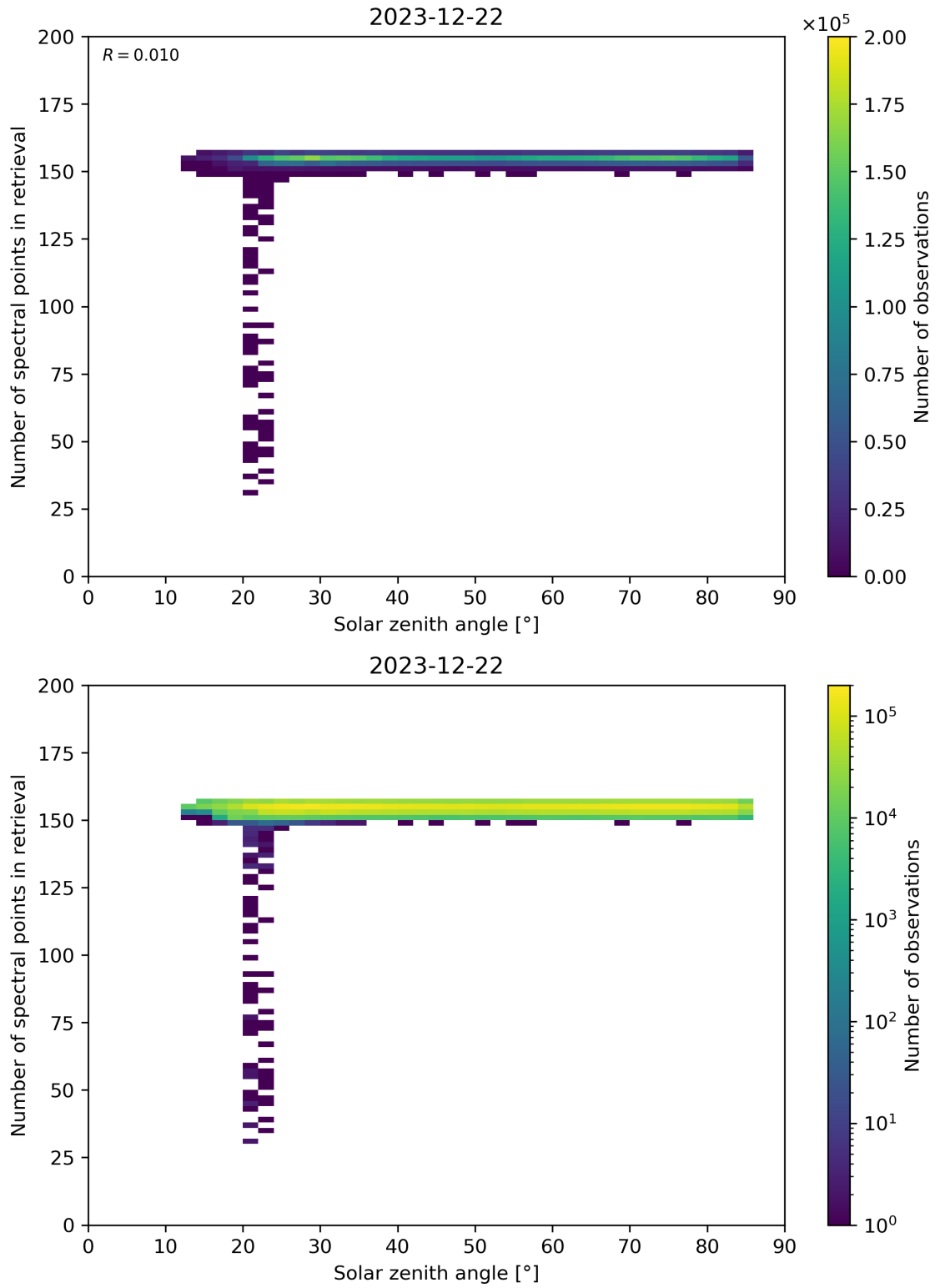
Figure 68: Scatter density plot of “Solar zenith angle” against “Number of spectral points in retrieval” for 2023-12-21 to 2023-12-23.
