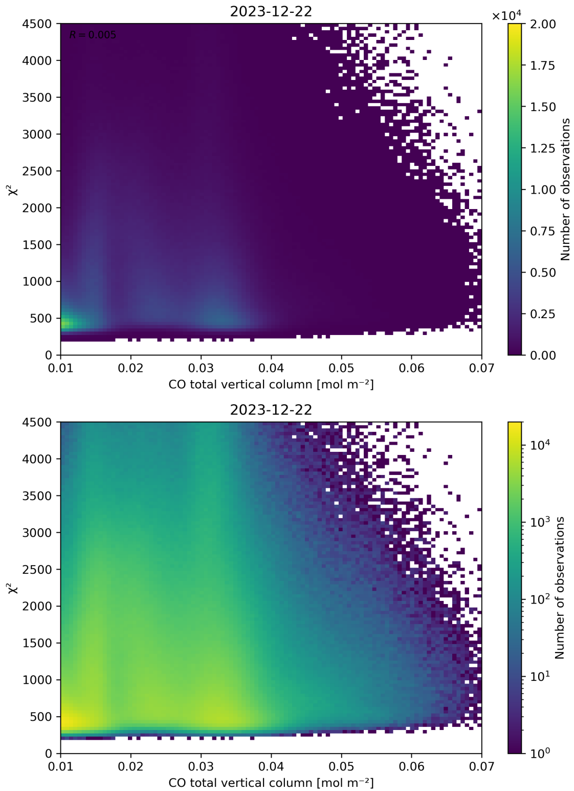
Figure 35: Scatter density plot of “CO total vertical column” against “ \chi^2 ” for 2023-12-21 to 2023-12-23.
