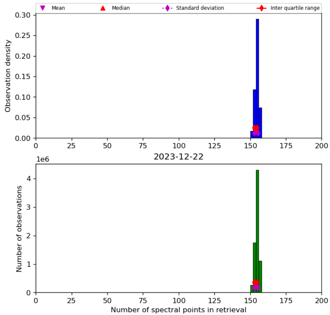
Figure 21: Histogram of “Number of spectral points in retrieval” for 2023-12-21 to 2023-12-23
