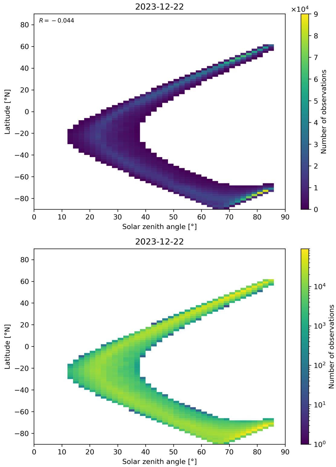
Figure 66: Scatter density plot of “Solar zenith angle” against “Latitude” for 2023-12-21 to 2023-12-23.
