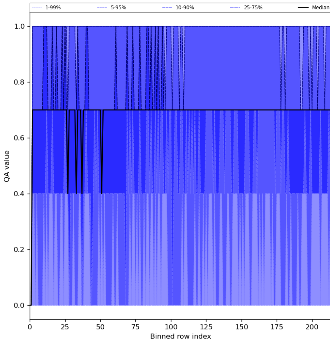
Figure 25: Along track statistics of “QA value” for 2023-12-21 to 2023-12-23
