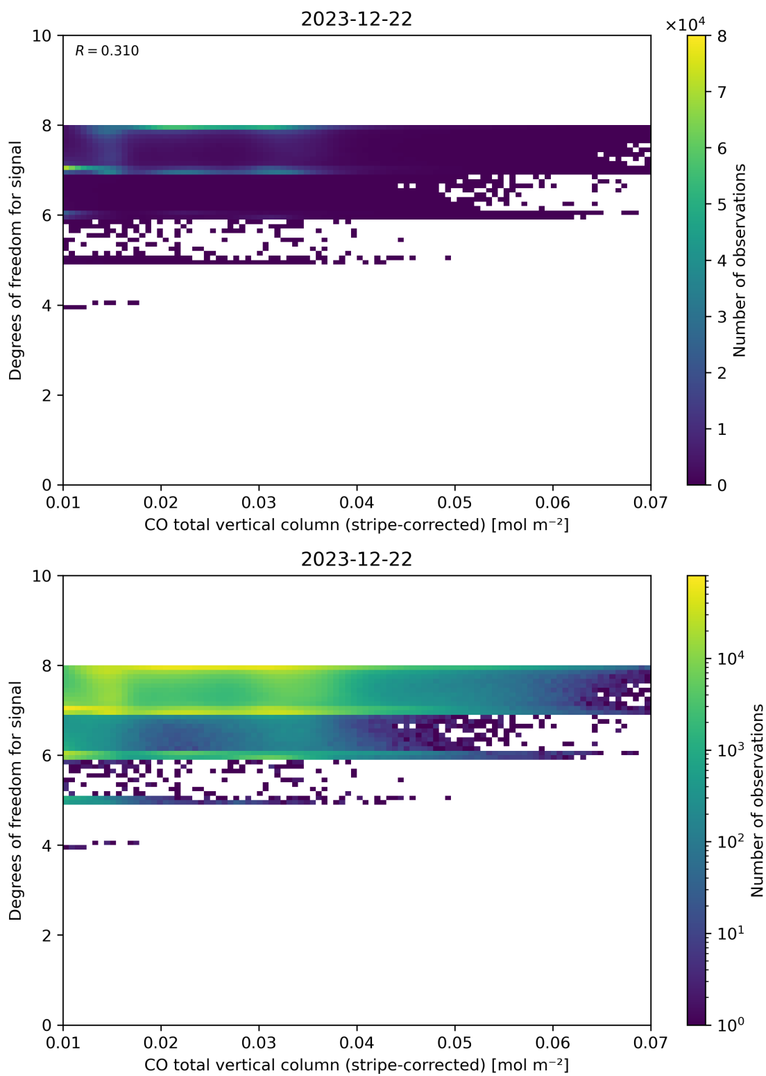
Figure 38: Scatter density plot of “CO total vertical column (stripe-corrected)” against “Degrees of freedom for signal” for 2023-12-21 to 2023-12-23.
