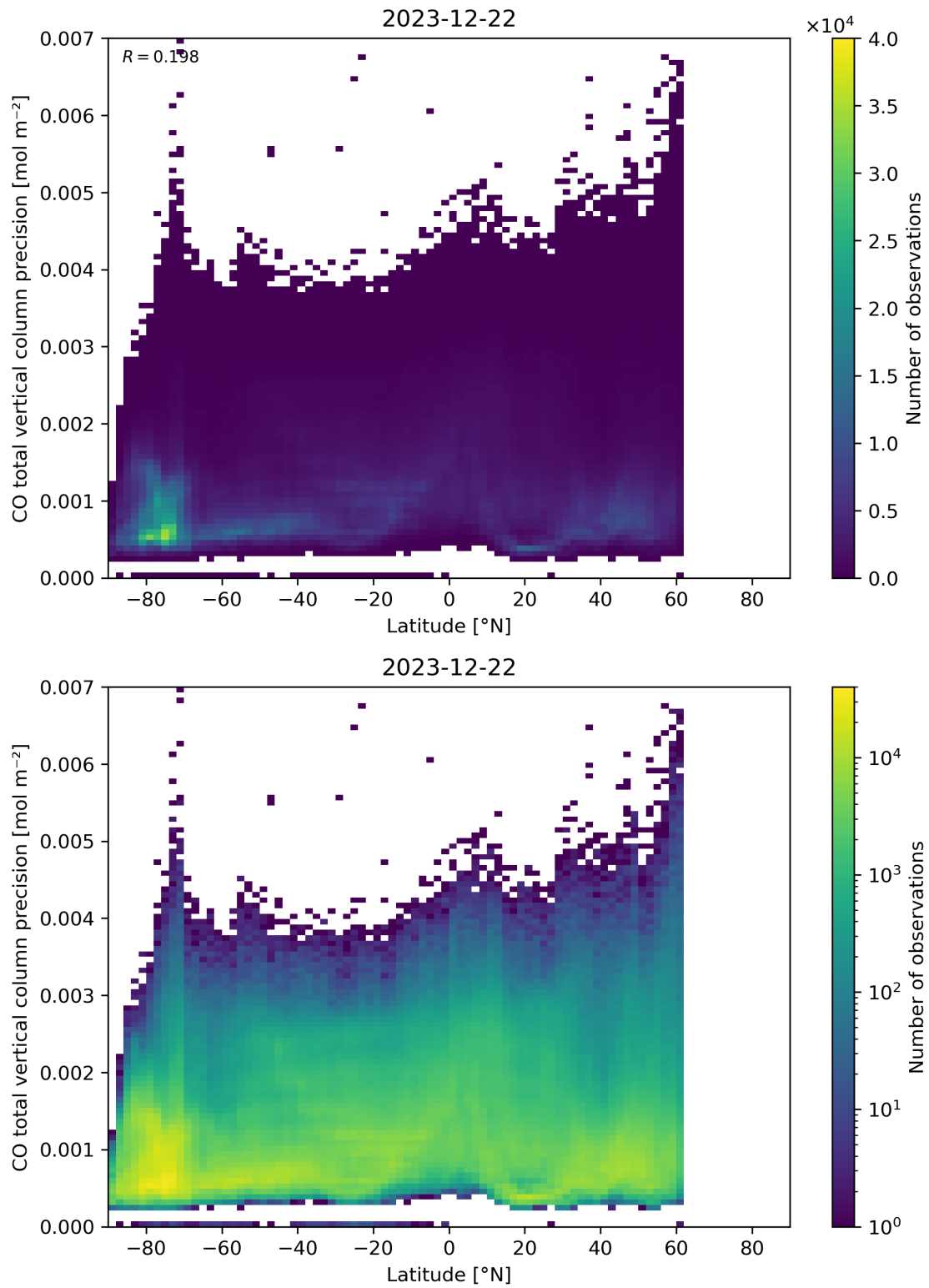
Figure 53: Scatter density plot of “Latitude” against “CO total vertical column precision” for 2023-12-21 to 2023-12-23.
