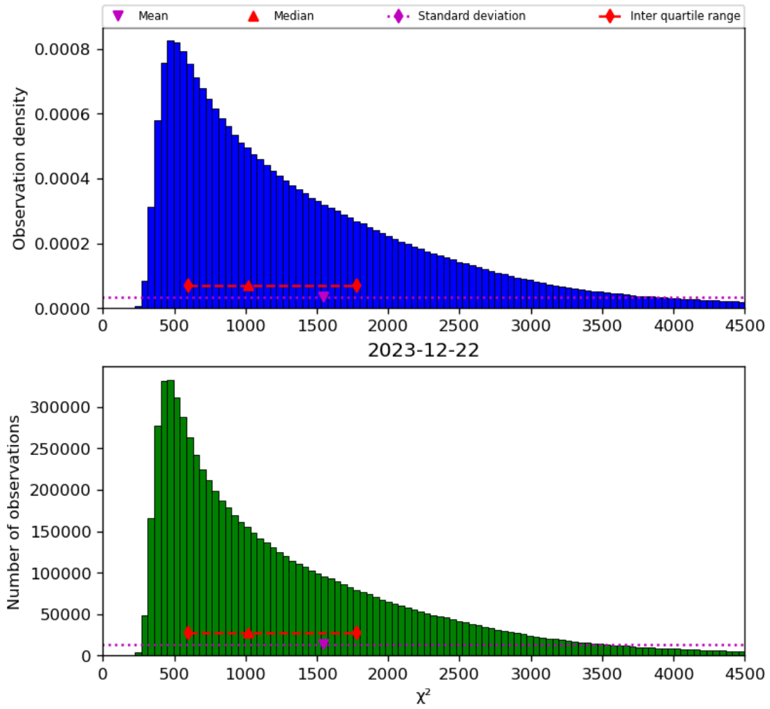
Figure 22: Histogram of “ \chi^2 ” for 2023-12-21 to 2023-12-23
