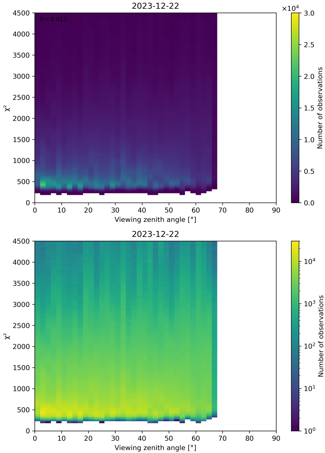
Figure 72: Scatter density plot of “Viewing zenith angle” against “ \chi^2 ” for 2023-12-21 to 2023-12-23.
