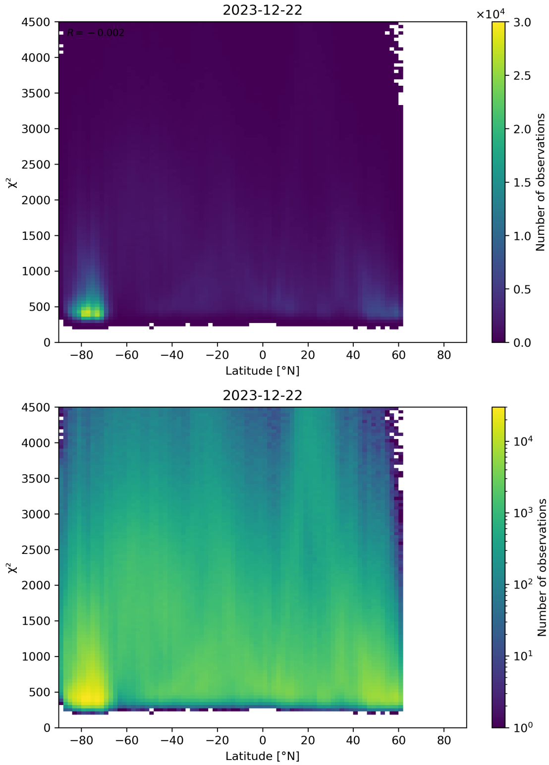
Figure 54: Scatter density plot of “Latitude” against “ \chi^2 ” for 2023-12-21 to 2023-12-23.
