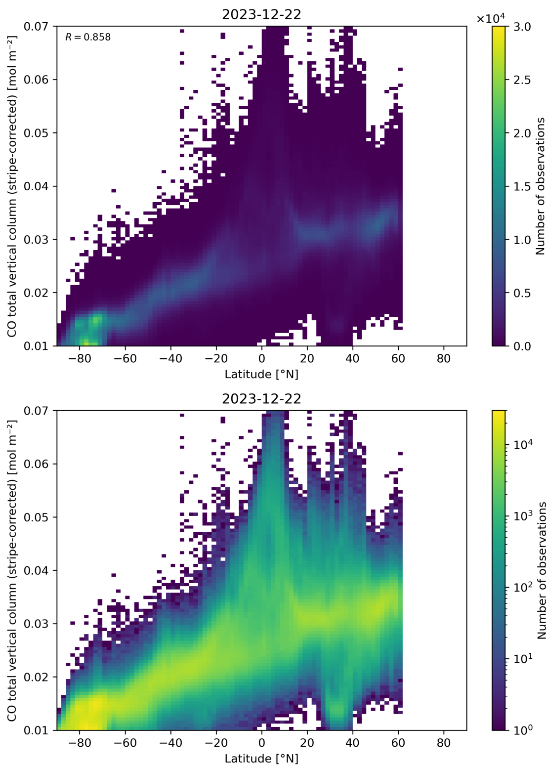
Figure 52: Scatter density plot of “Latitude” against “CO total vertical column (stripe-corrected)” for 2023-12-21 to 2023-12-23.
