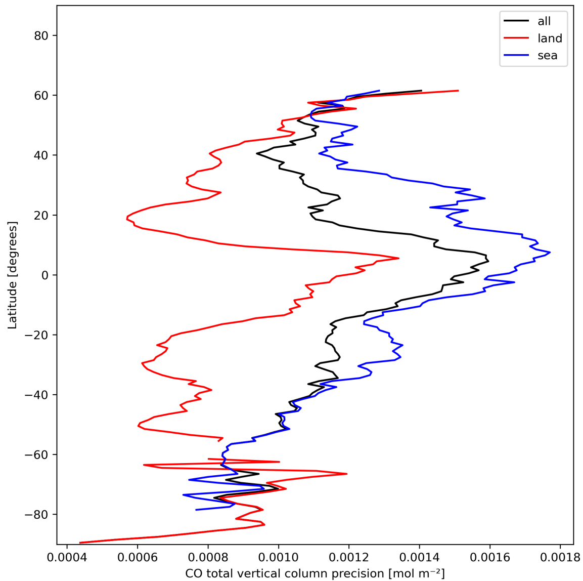
Figure 12: Zonal average of “CO total vertical column precision” for 2023-12-21 to 2023-12-23.
