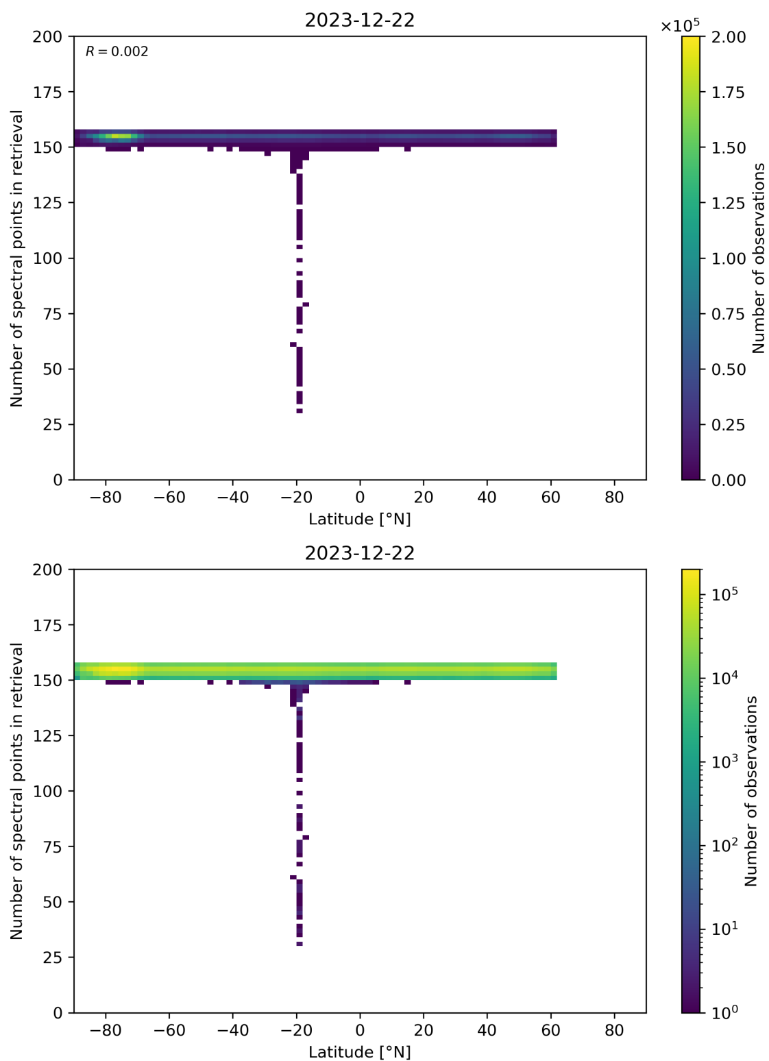
Figure 57: Scatter density plot of “Latitude” against “Number of spectral points in retrieval” for 2023-12-21 to 2023-12-23.
