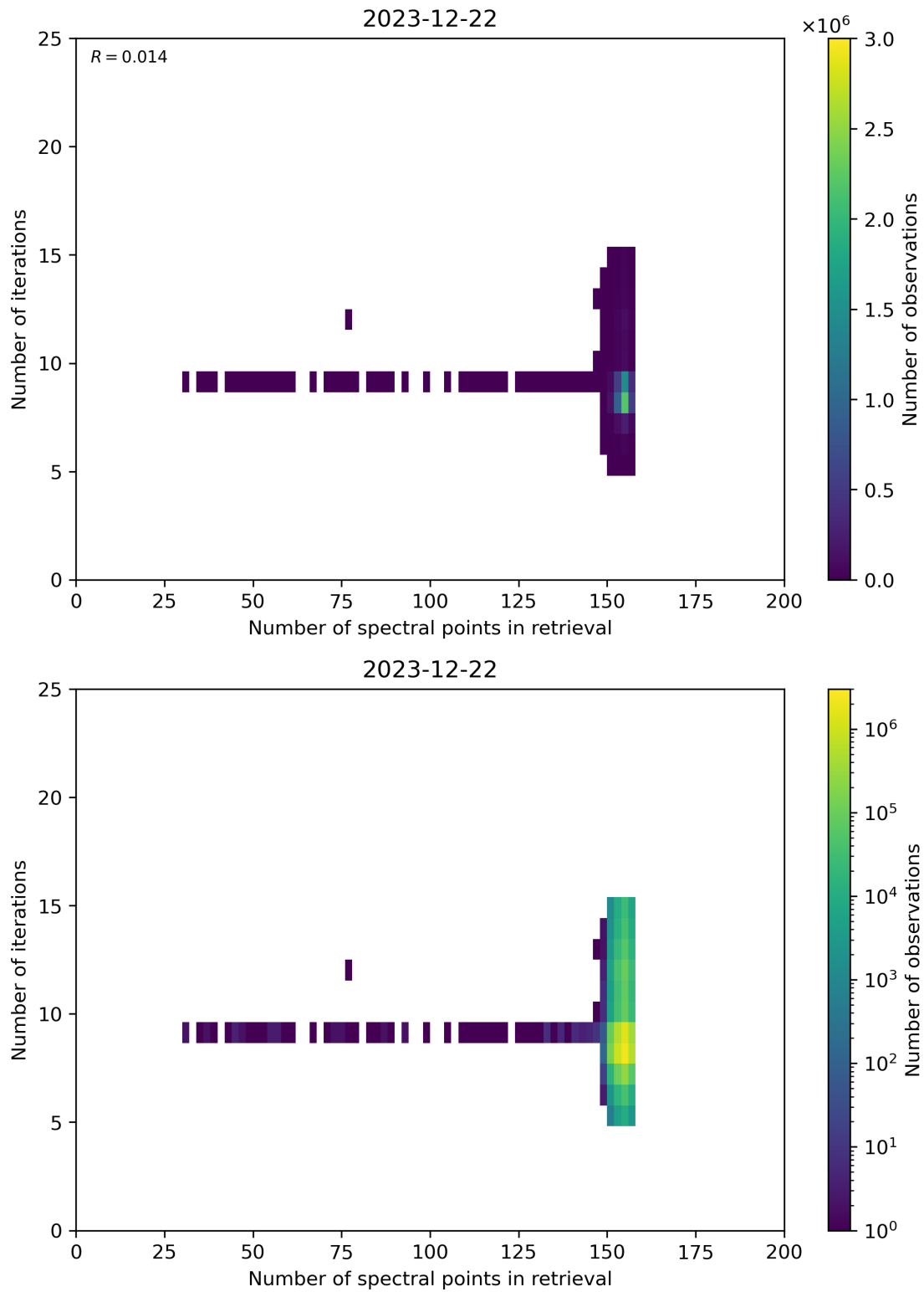
Figure 60: Scatter density plot of “Number of spectral points in retrieval” against “Number of iterations” for 2023-12-21 to 2023-12-23.
