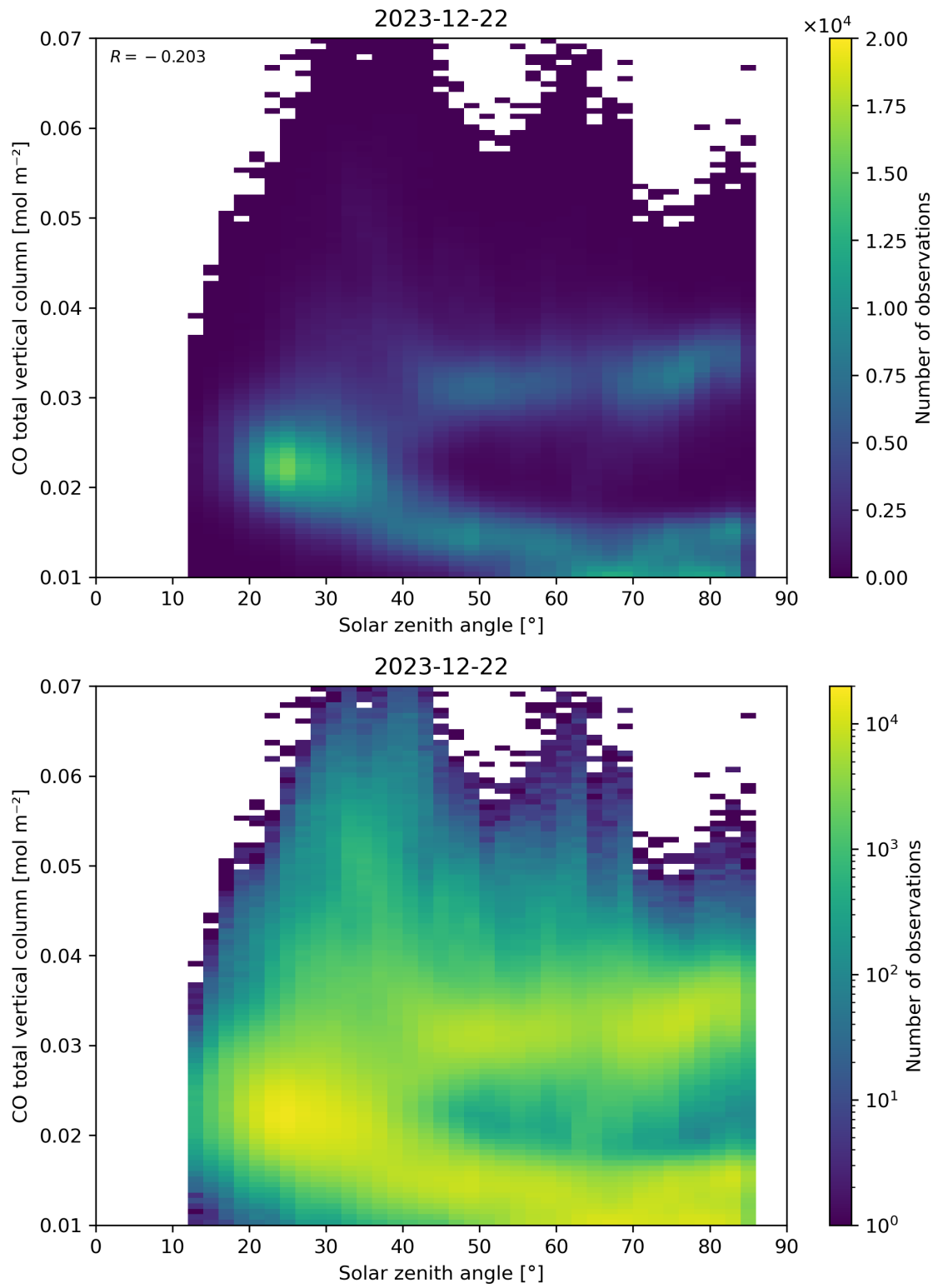
Figure 61: Scatter density plot of “Solar zenith angle” against “CO total vertical column” for 2023-12-21 to 2023-12-23.
