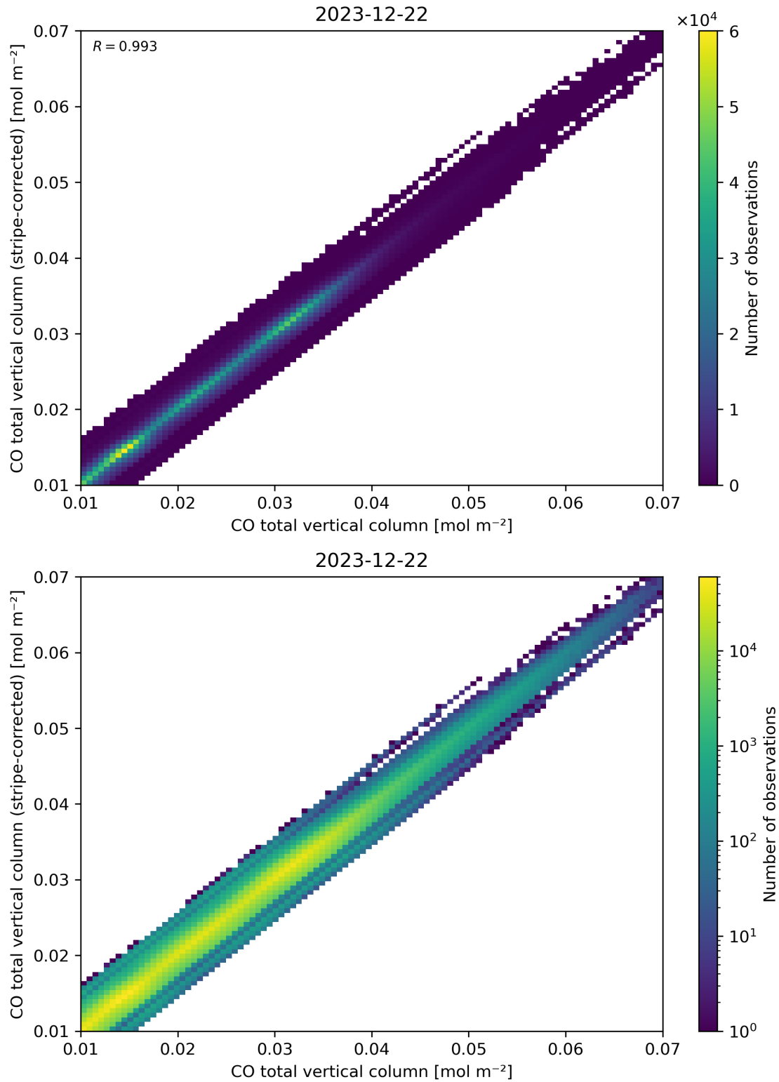
Figure 33: Scatter density plot of “CO total vertical column” against “CO total vertical column (stripe-corrected)” for 2023-12-21 to 2023-12-23.
