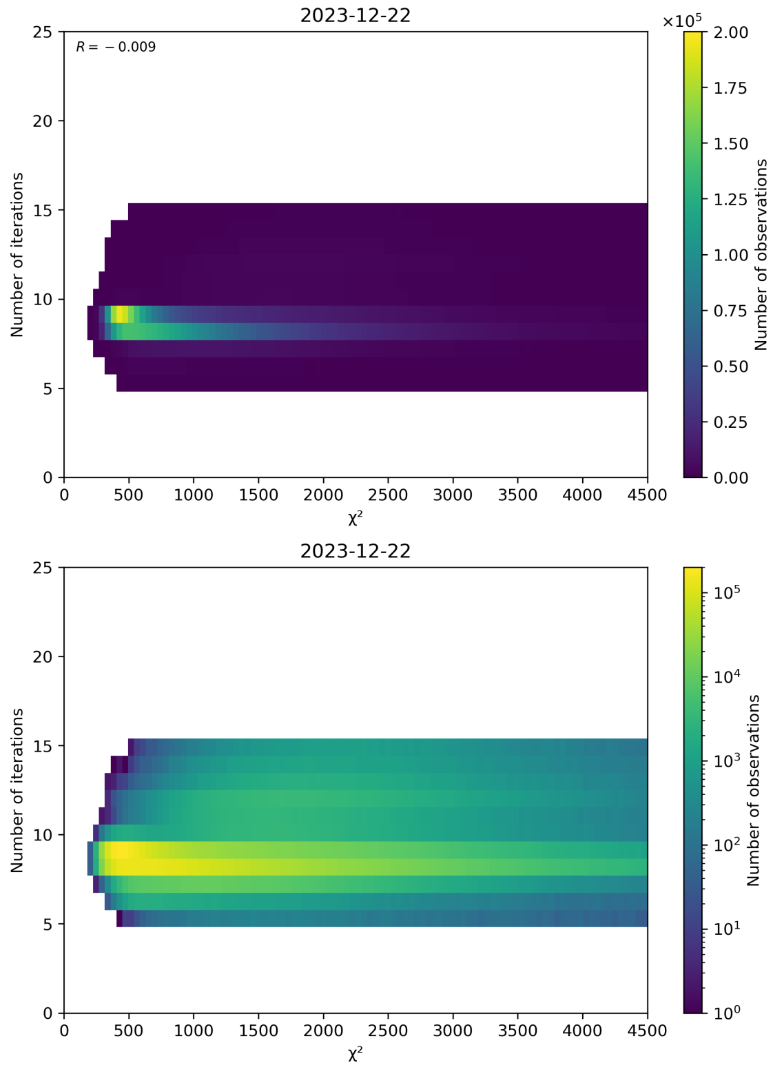
Figure 49: Scatter density plot of “ \chi^2 ” against “Number of iterations” for 2023-12-21 to 2023-12-23.
