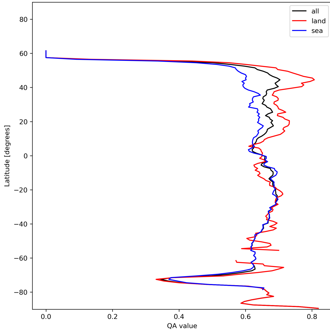
Figure 9: Zonal average of “QA value” for 2023-12-21 to 2023-12-23.
