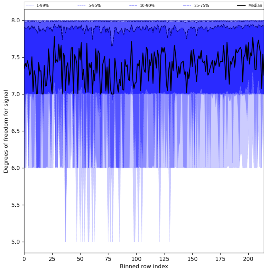
Figure 31: Along track statistics of “Degrees of freedom for signal” for 2023-12-21 to 2023-12-23
