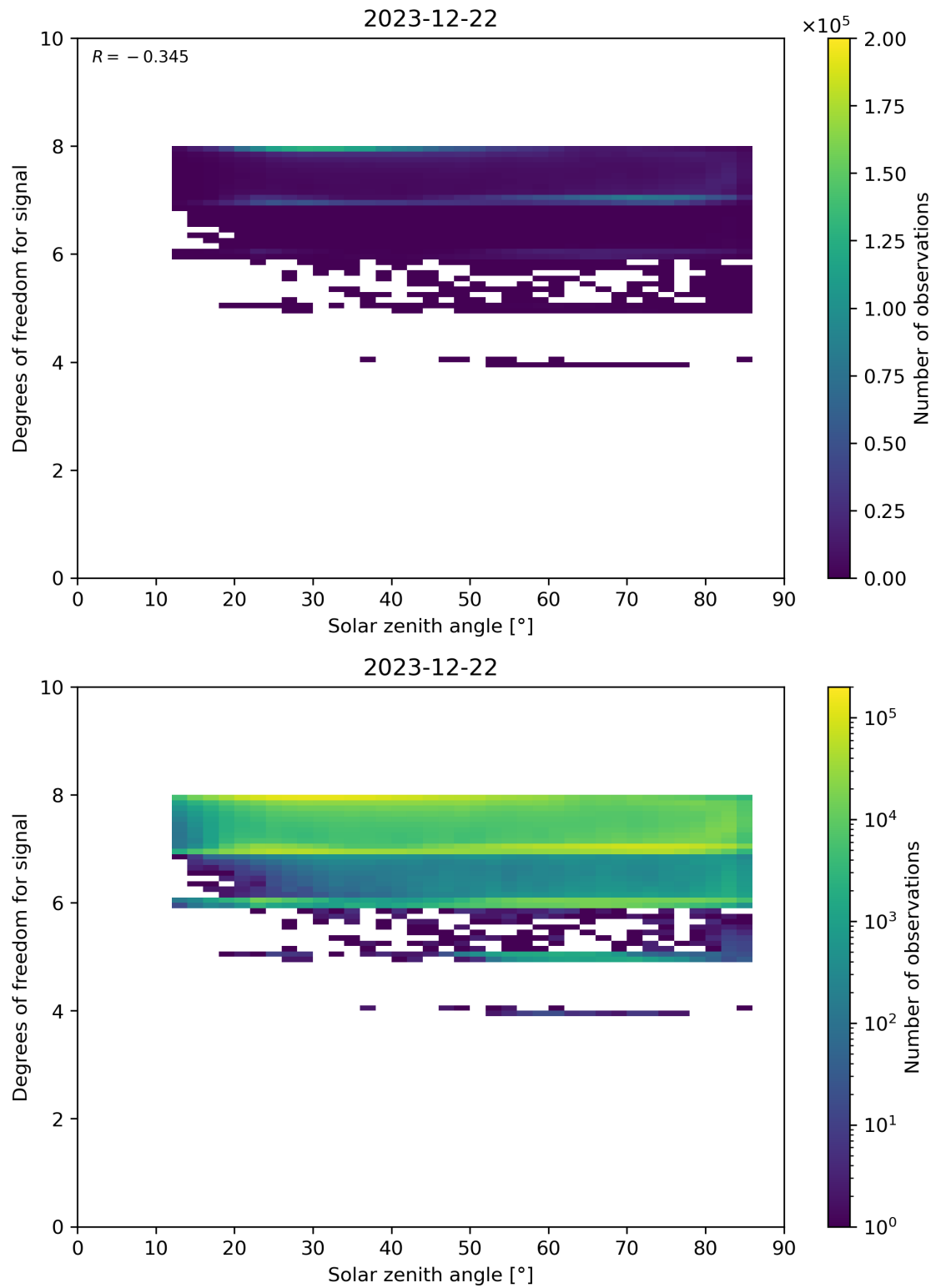
Figure 65: Scatter density plot of “Solar zenith angle” against “Degrees of freedom for signal” for 2023-12-21 to 2023-12-23.
