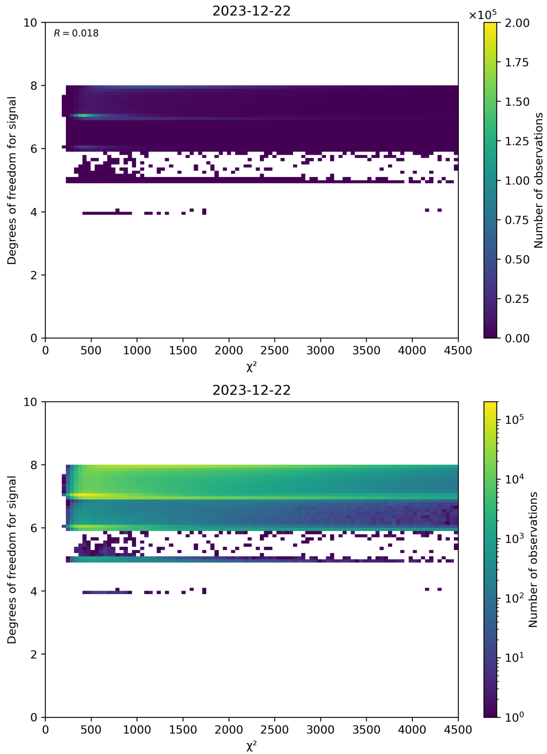
Figure 48: Scatter density plot of “ \chi^2 ” against “Degrees of freedom for signal” for 2023-12-21 to 2023-12-23.
