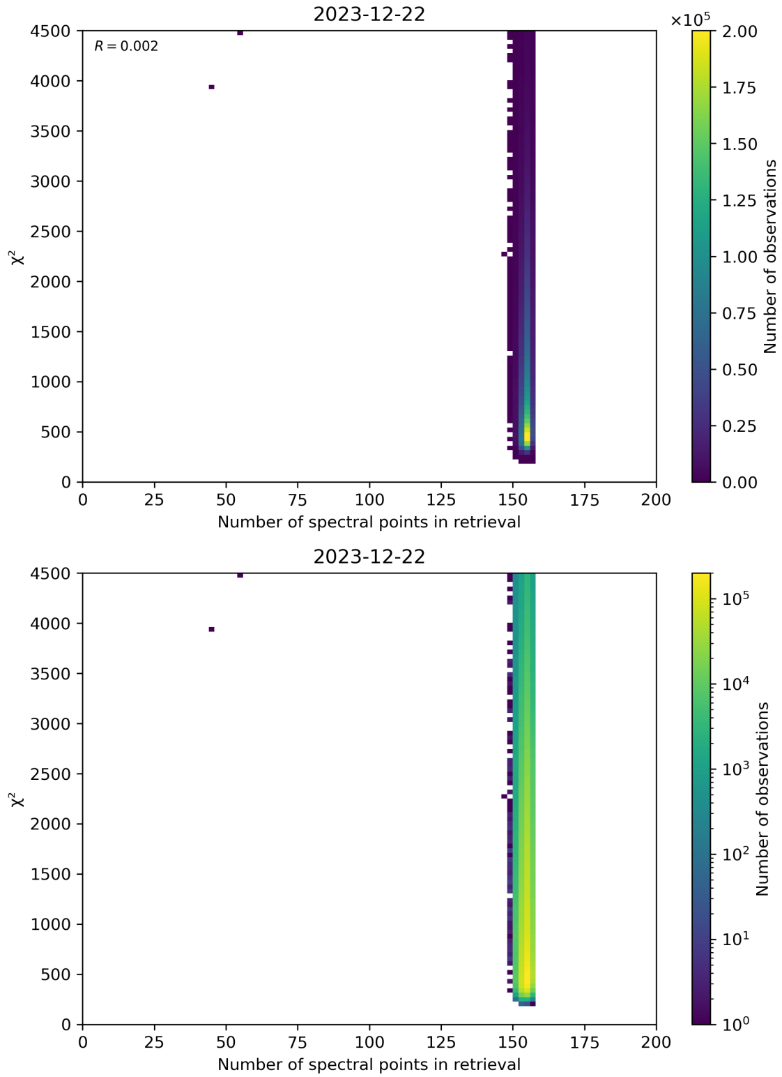
Figure 58: Scatter density plot of “Number of spectral points in retrieval” against “ \chi^2 ” for 2023-12-21 to 2023-12-23.
