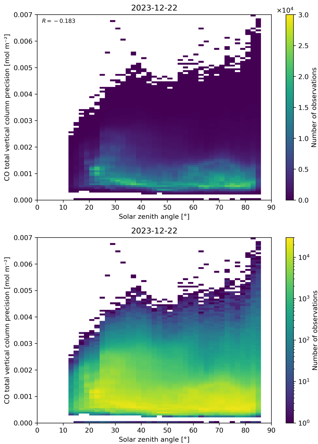
Figure 63: Scatter density plot of “Solar zenith angle” against “CO total vertical column precision” for 2023-12-21 to 2023-12-23.
