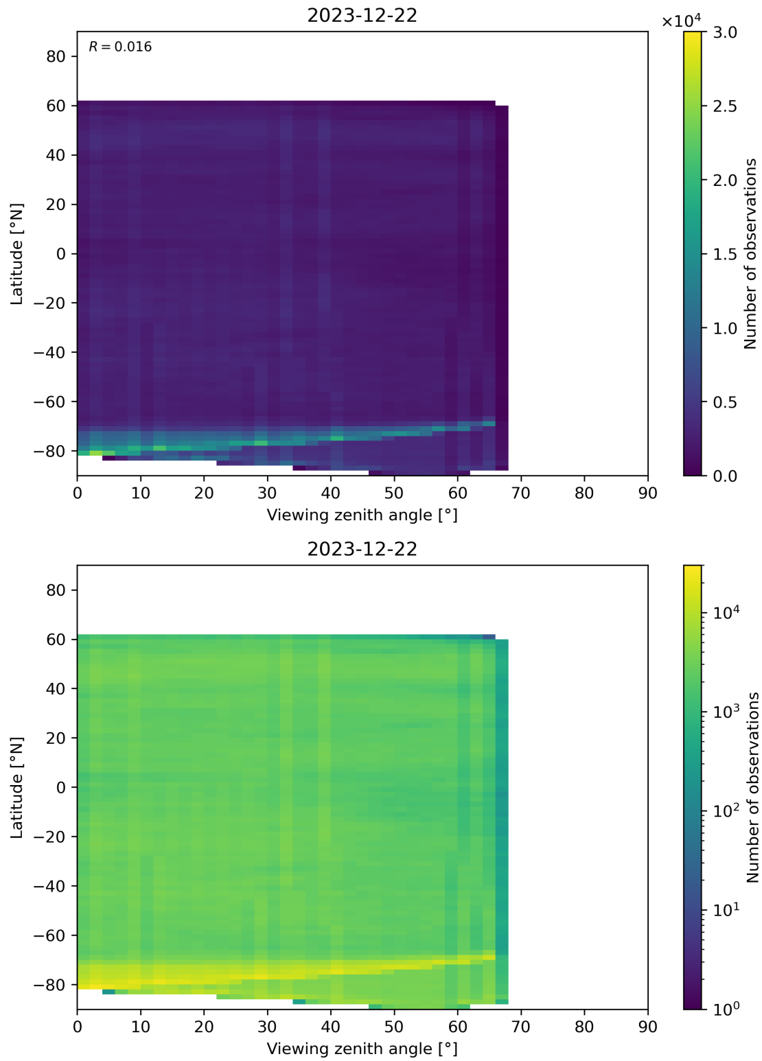
Figure 74: Scatter density plot of “Viewing zenith angle” against “Latitude” for 2023-12-21 to 2023-12-23.
