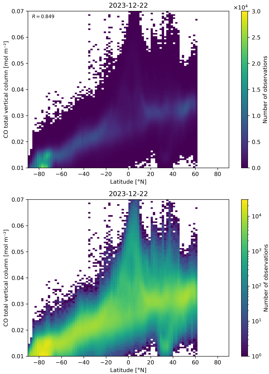
Figure 51: Scatter density plot of “Latitude” against “CO total vertical column” for 2023-12-21 to 2023-12-23.
