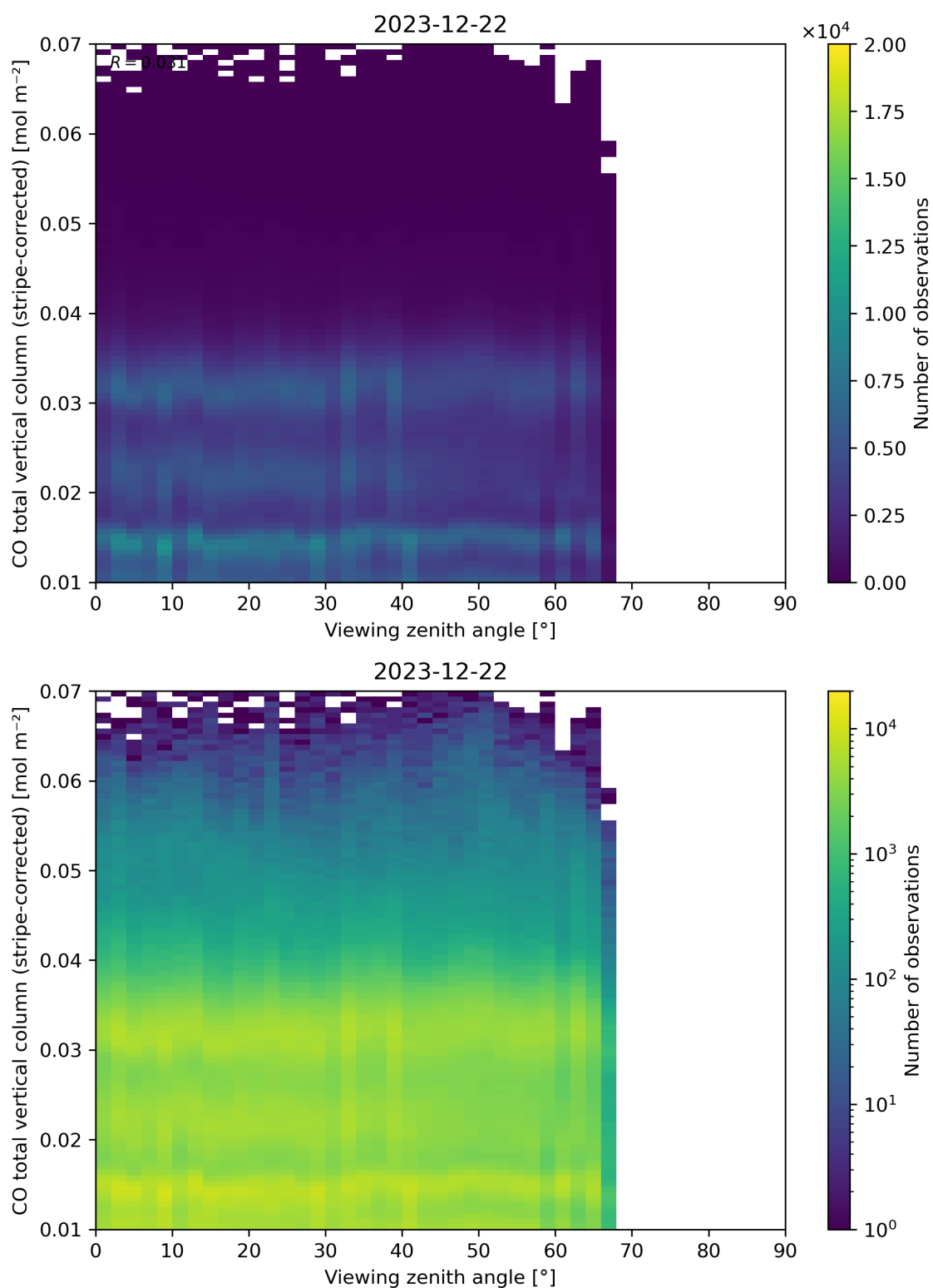
Figure 70: Scatter density plot of “Viewing zenith angle” against “CO total vertical column (stripe-corrected)” for 2023-12-21 to 2023-12-23.
