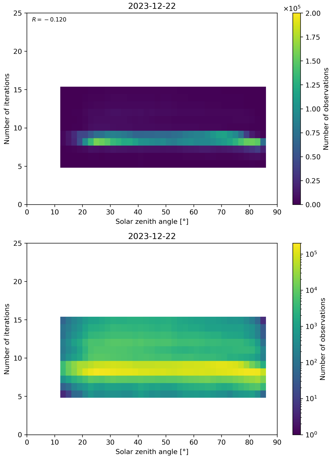
Figure 67: Scatter density plot of “Solar zenith angle” against “Number of iterations” for 2023-12-21 to 2023-12-23.
