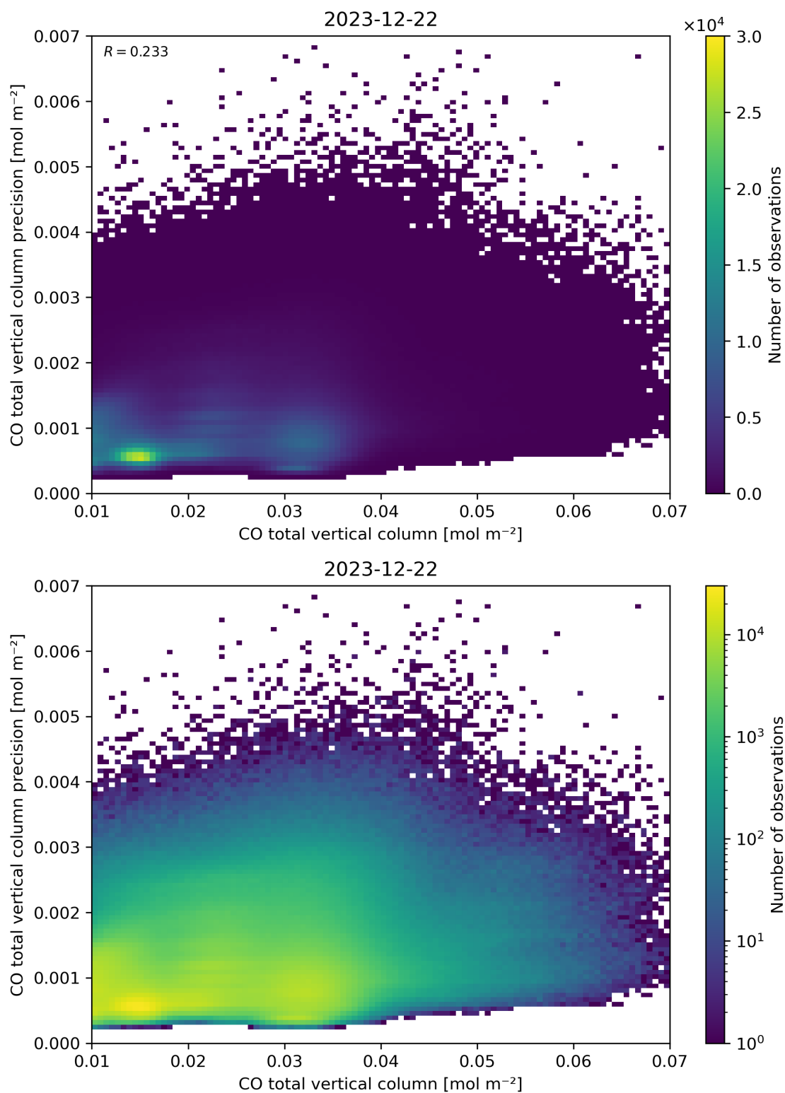
Figure 34: Scatter density plot of “CO total vertical column” against “CO total vertical column precision” for 2023-12-21 to 2023-12-23.
