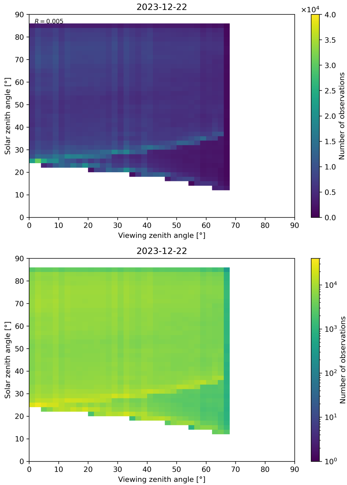
Figure 77: Scatter density plot of “Viewing zenith angle” against “Solar zenith angle” for 2023-12-21 to 2023-12-23.
