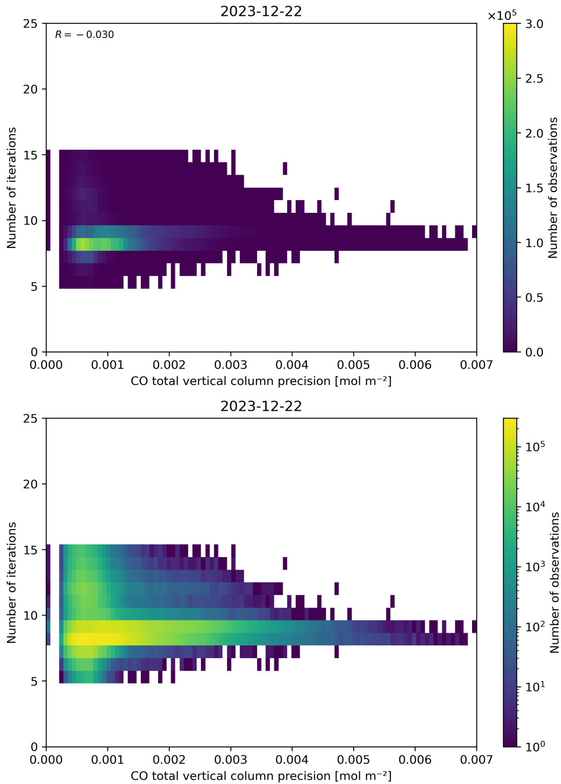
Figure 46: Scatter density plot of “CO total vertical column precision” against “Number of iterations” for 2023-12-21 to 2023-12-23.
