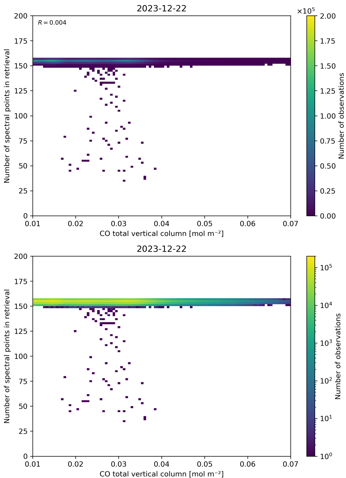
Figure 43: Scatter density plot of “CO total vertical column” against “Number of spectral points in retrieval” for 2023-12-21 to 2023-12-23.
