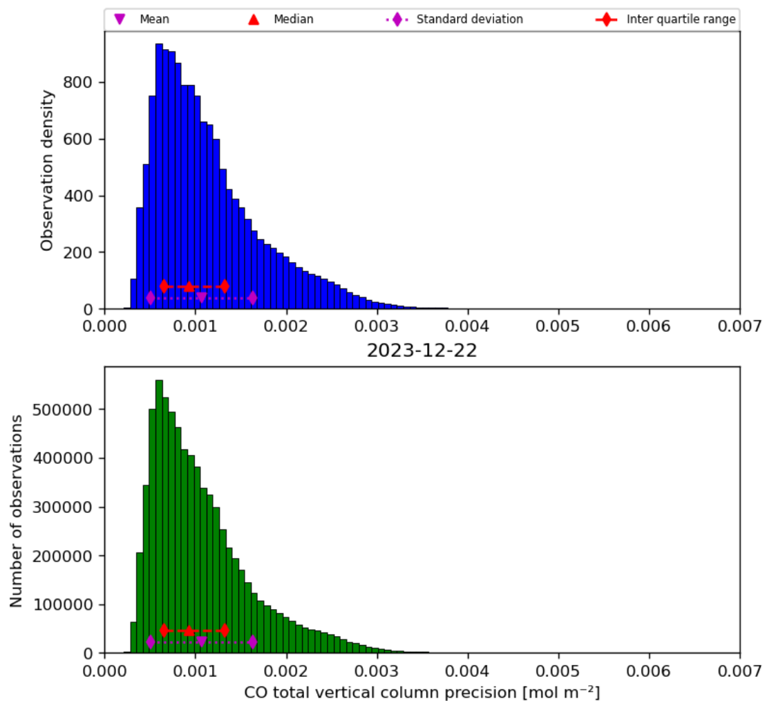
Figure 20: Histogram of “CO total vertical column precision” for 2023-12-21 to 2023-12-23
