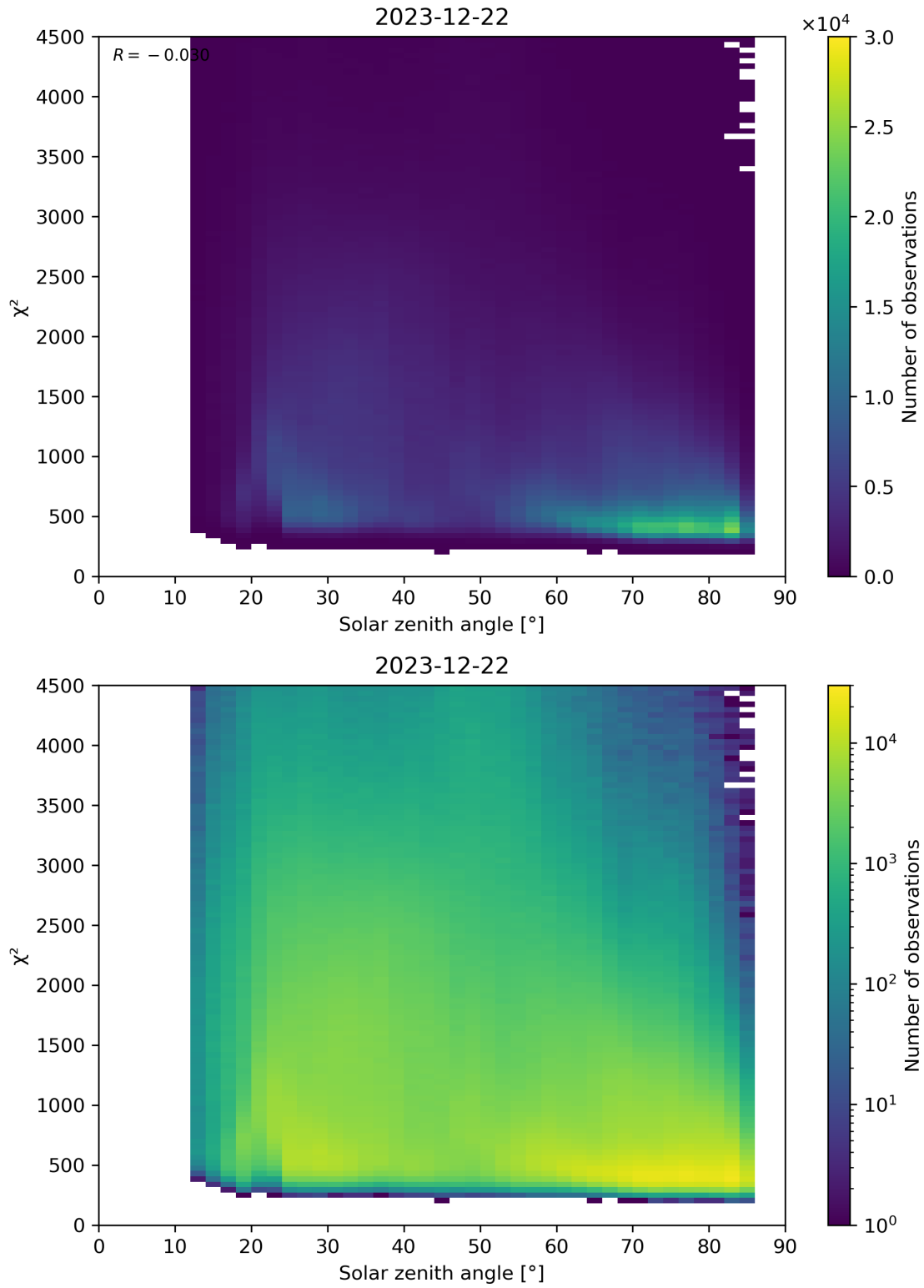
Figure 64: Scatter density plot of “Solar zenith angle” against “ \chi^2 ” for 2023-12-21 to 2023-12-23.
