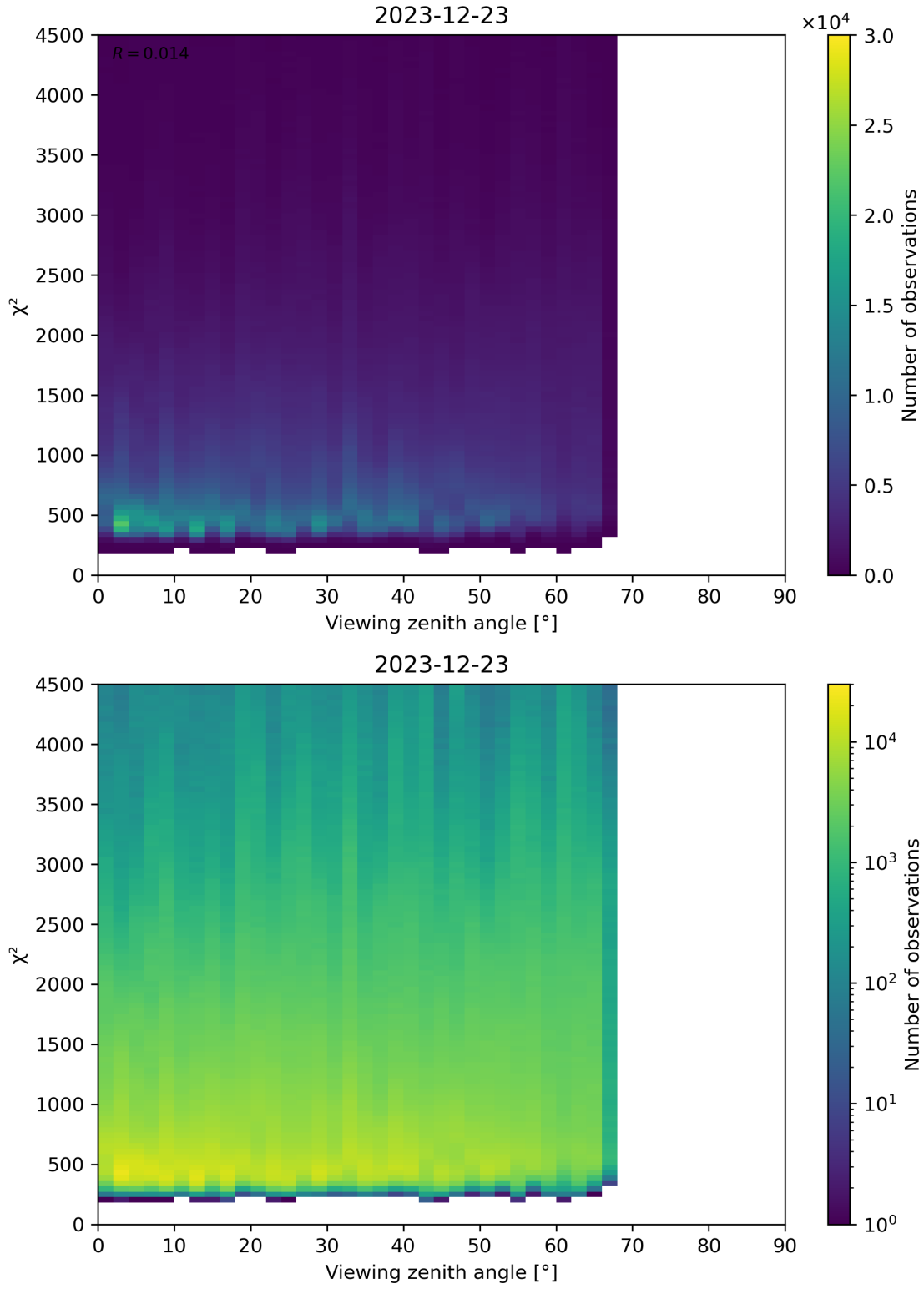
Figure 72: Scatter density plot of “Viewing zenith angle” against “ \chi^2 ” for 2023-12-22 to 2023-12-24.
