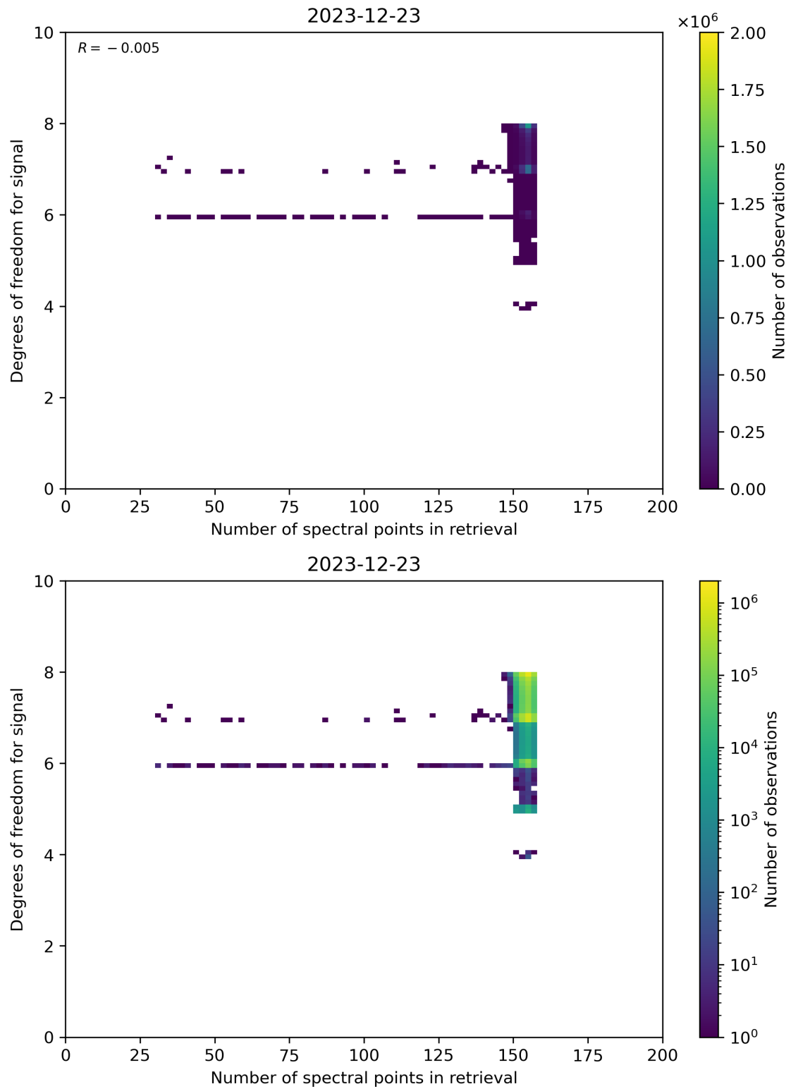
Figure 59: Scatter density plot of “Number of spectral points in retrieval” against “Degrees of freedom for signal” for 2023-12-22 to 2023-12-24.
