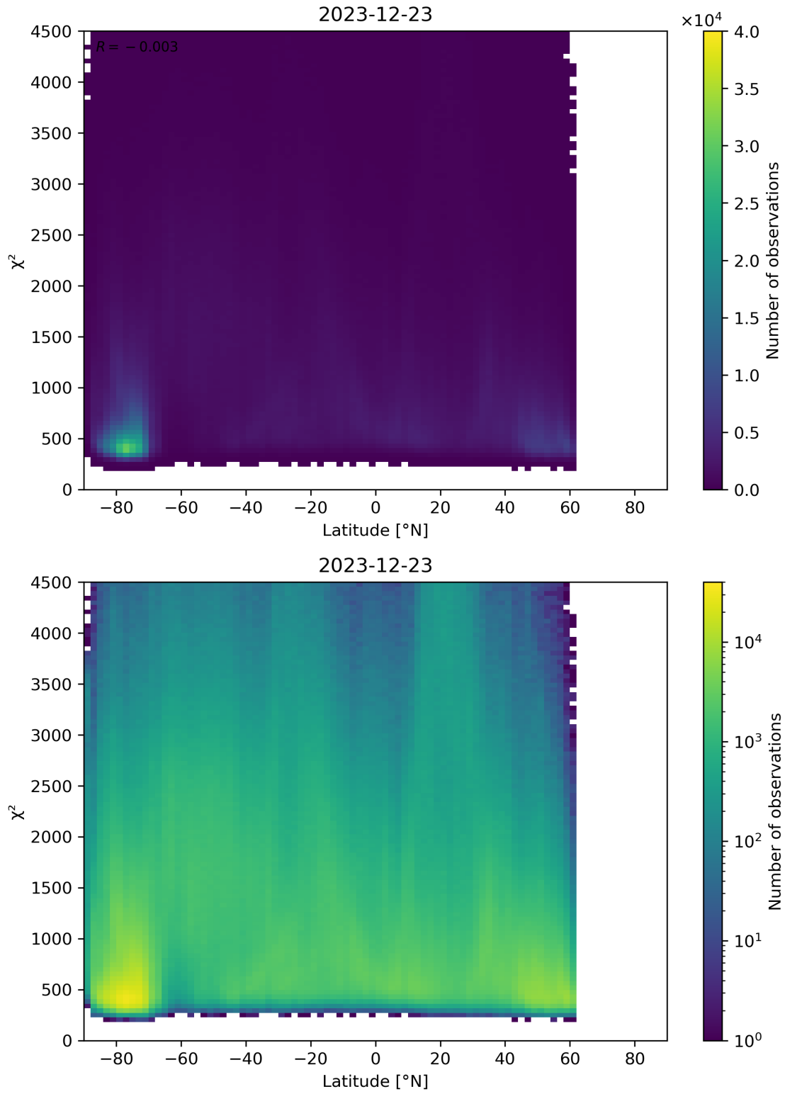
Figure 54: Scatter density plot of “Latitude” against “ \chi^2 ” for 2023-12-22 to 2023-12-24.
