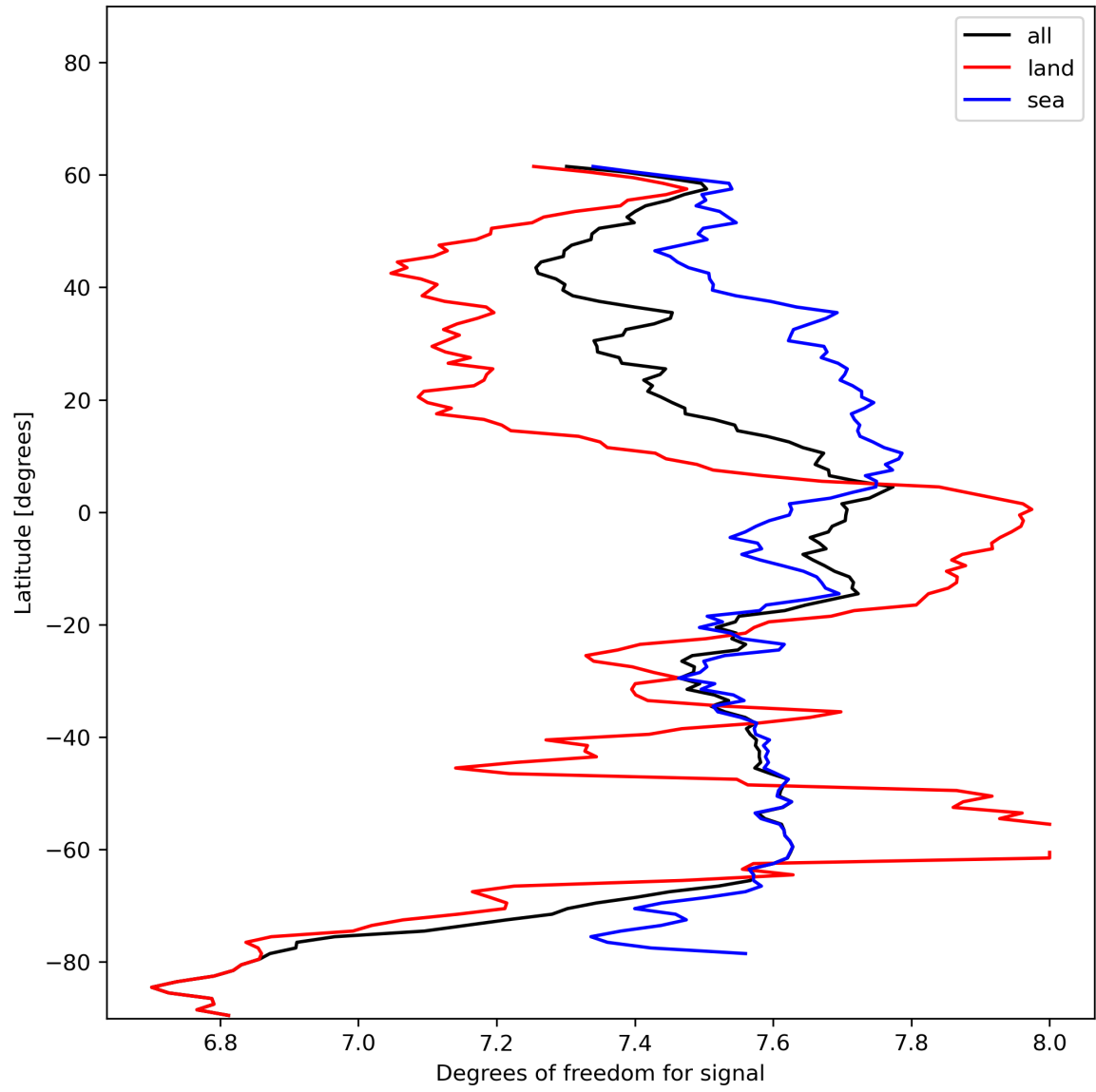
Figure 15: Zonal average of “Degrees of freedom for signal” for 2023-12-22 to 2023-12-24.
