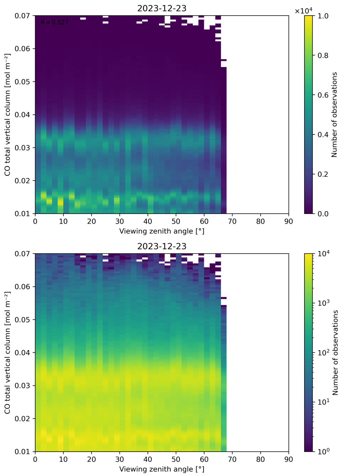
Figure 69: Scatter density plot of “Viewing zenith angle” against “CO total vertical column” for 2023-12-22 to 2023-12-24.
