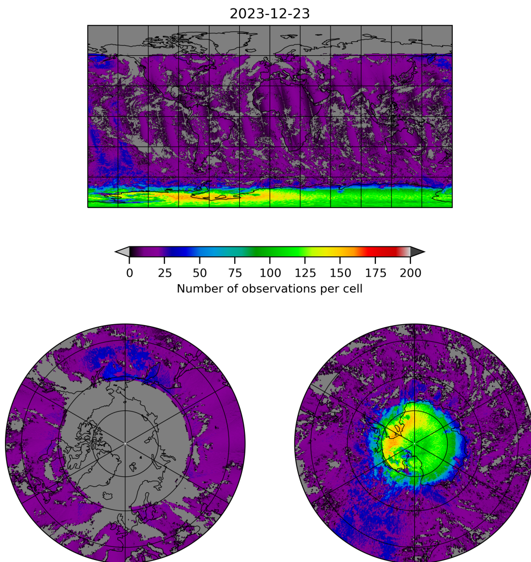
Figure 8: Map of the number of observations for 2023-12-22 to 2023-12-24
