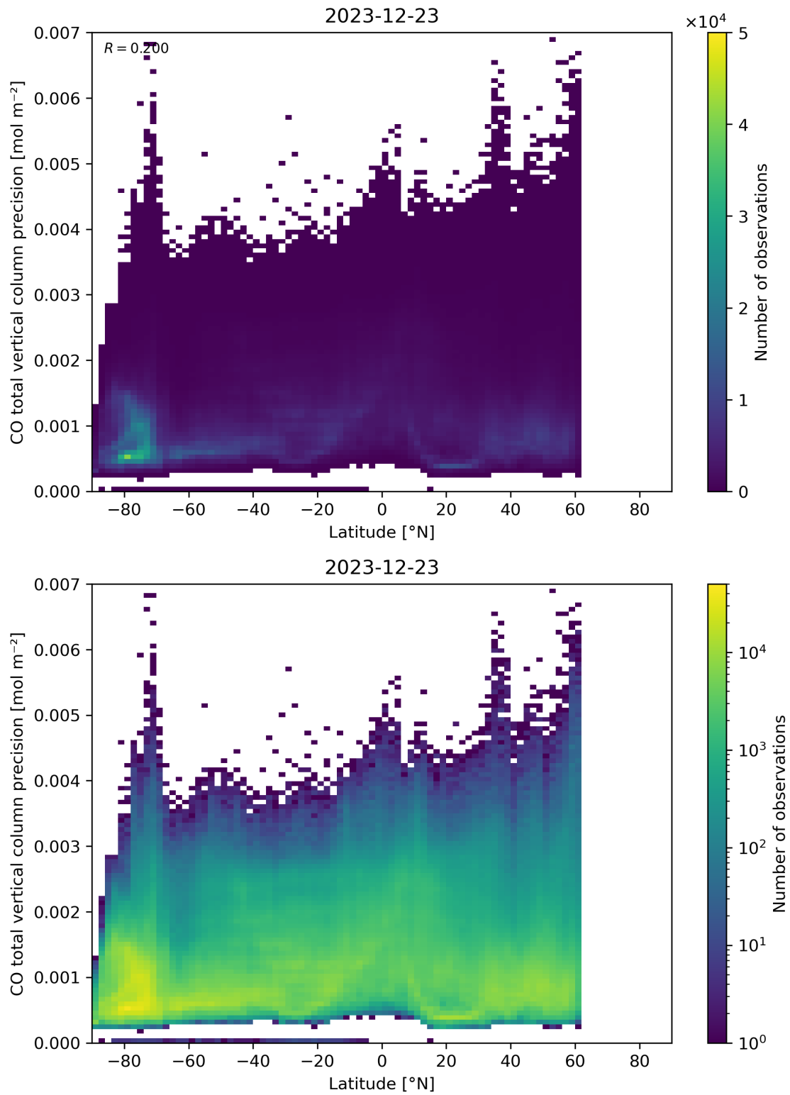
Figure 53: Scatter density plot of “Latitude” against “CO total vertical column precision” for 2023-12-22 to 2023-12-24.
