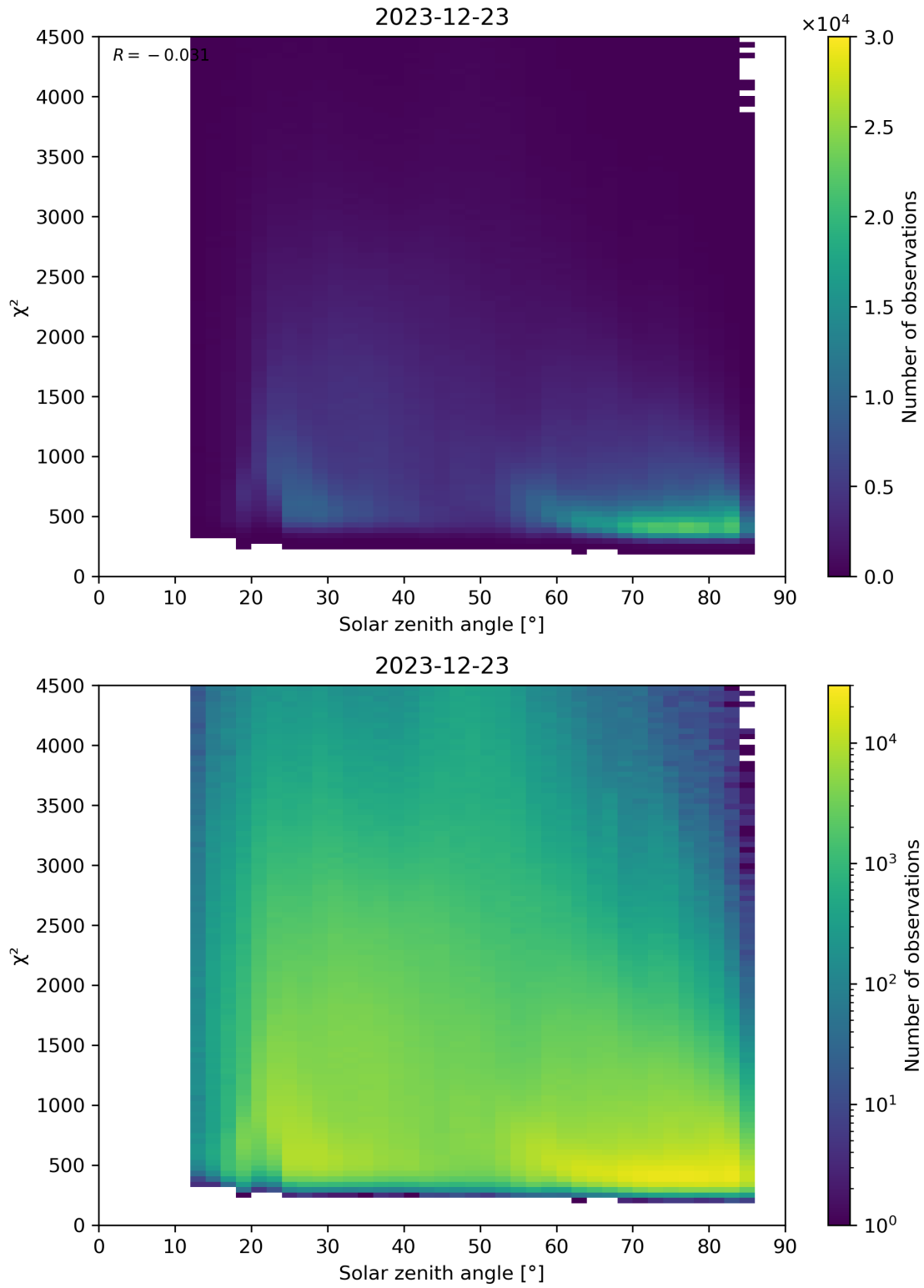
Figure 64: Scatter density plot of “Solar zenith angle” against “ \chi^2 ” for 2023-12-22 to 2023-12-24.
