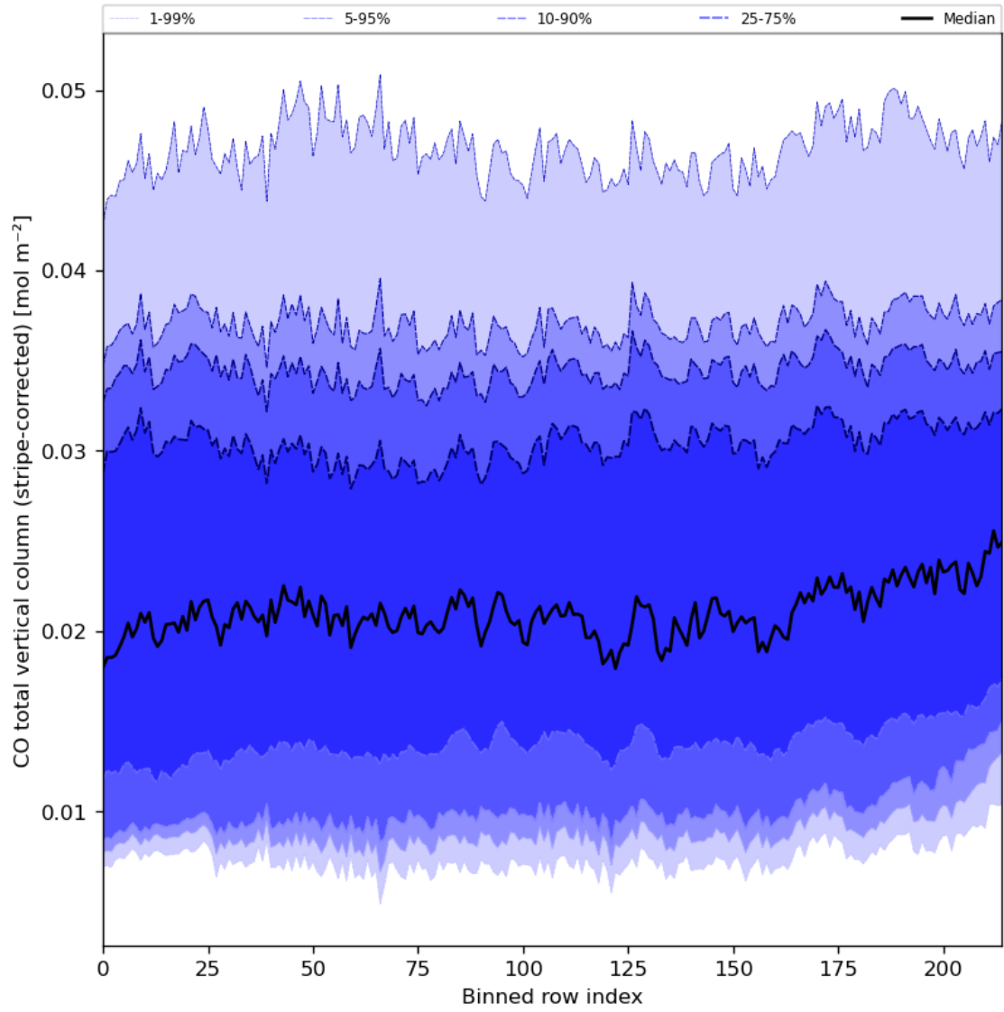
Figure 27: Along track statistics of “CO total vertical column (stripe-corrected)” for 2023-12-22 to 2023-12-24
