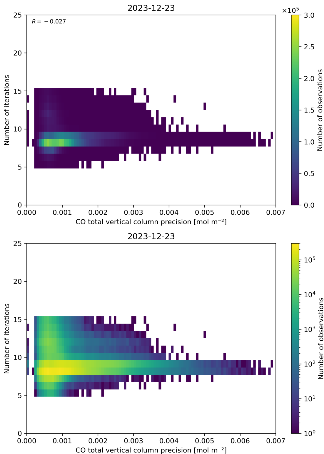
Figure 46: Scatter density plot of “CO total vertical column precision” against “Number of iterations” for 2023-12-22 to 2023-12-24.
