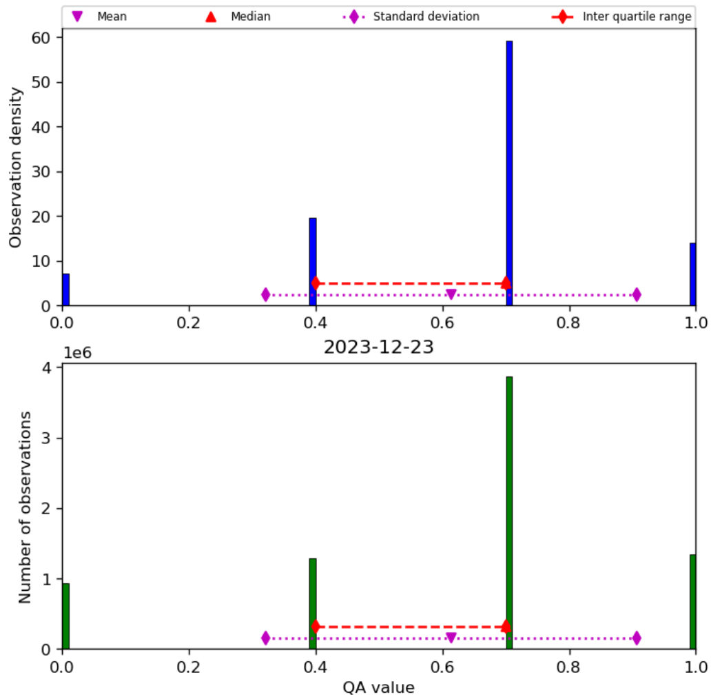
Figure 17: Histogram of “QA value” for 2023-12-22 to 2023-12-24
