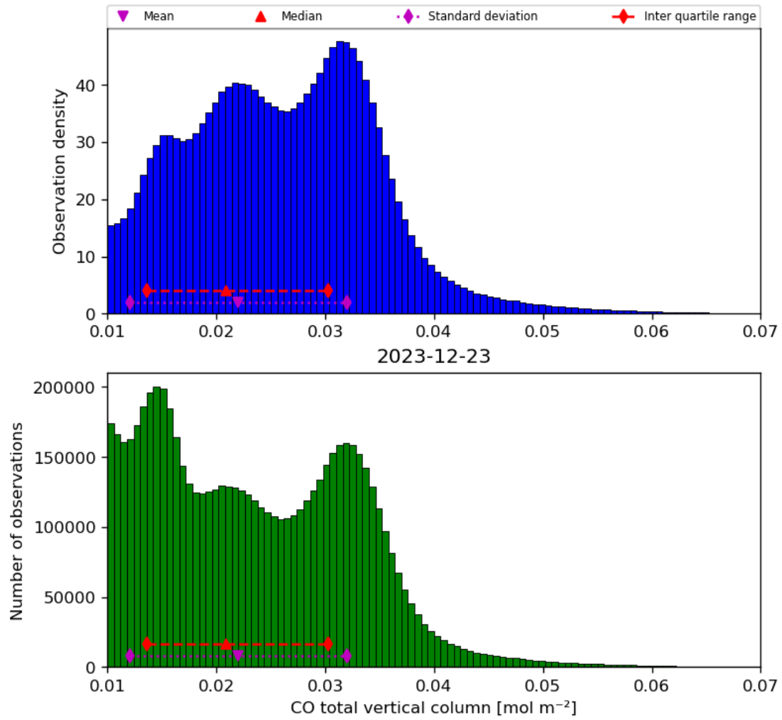
Figure 18: Histogram of “CO total vertical column” for 2023-12-22 to 2023-12-24
