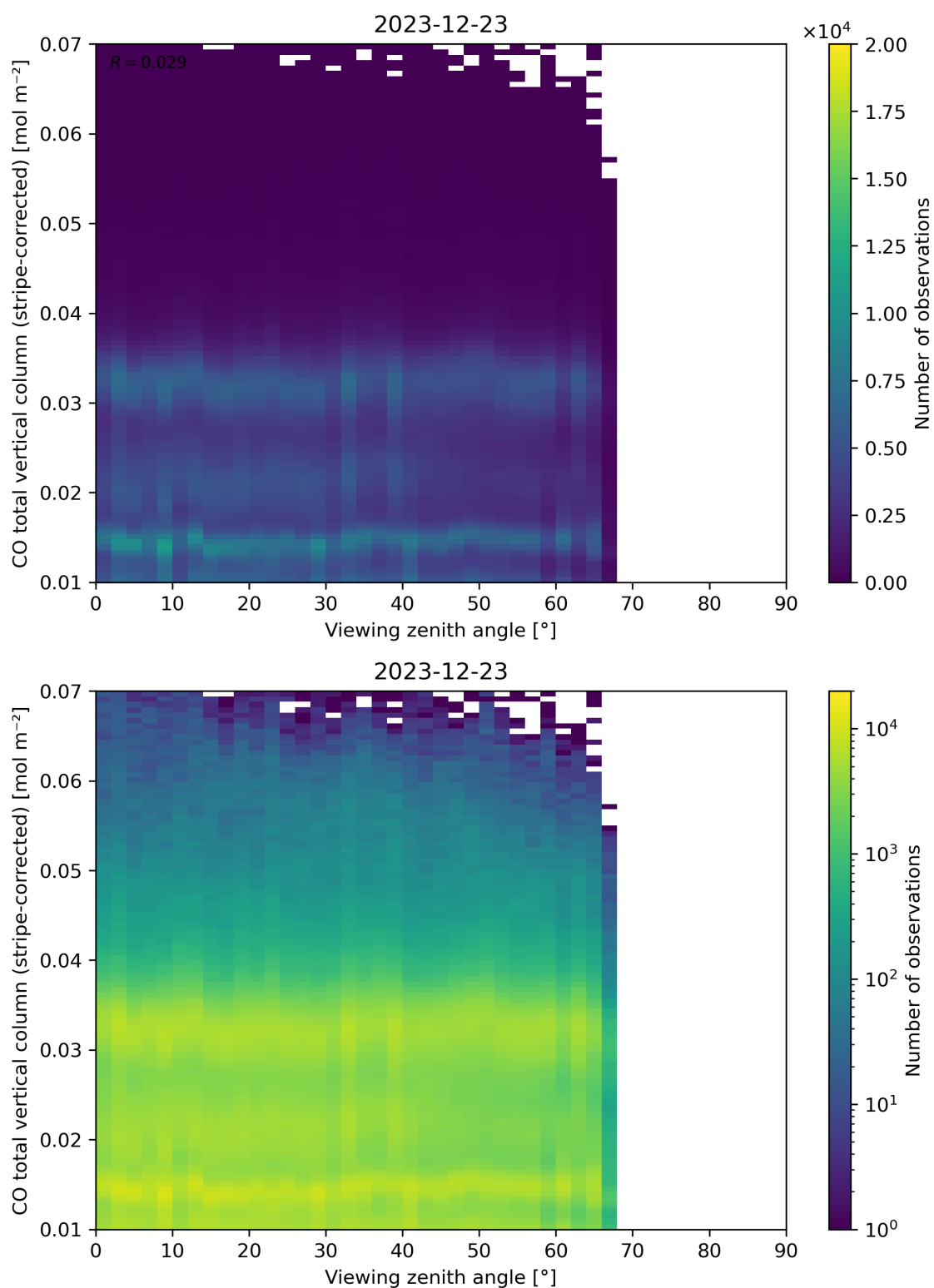
Figure 70: Scatter density plot of “Viewing zenith angle” against “CO total vertical column (stripe-corrected)” for 2023-12-22 to 2023-12-24.
