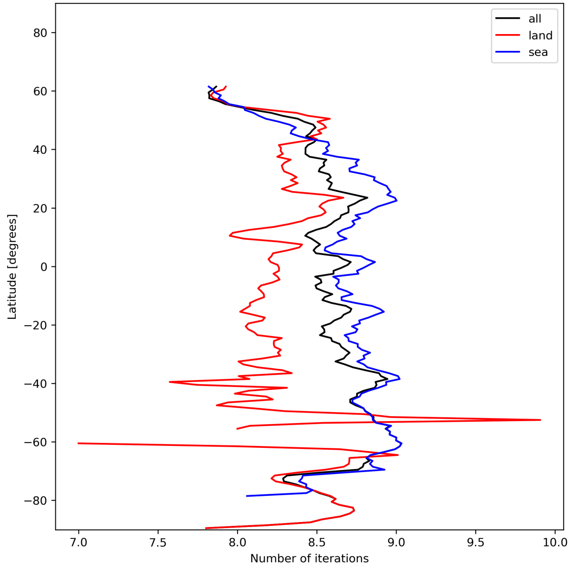
Figure 16: Zonal average of “Number of iterations” for 2023-12-22 to 2023-12-24.
