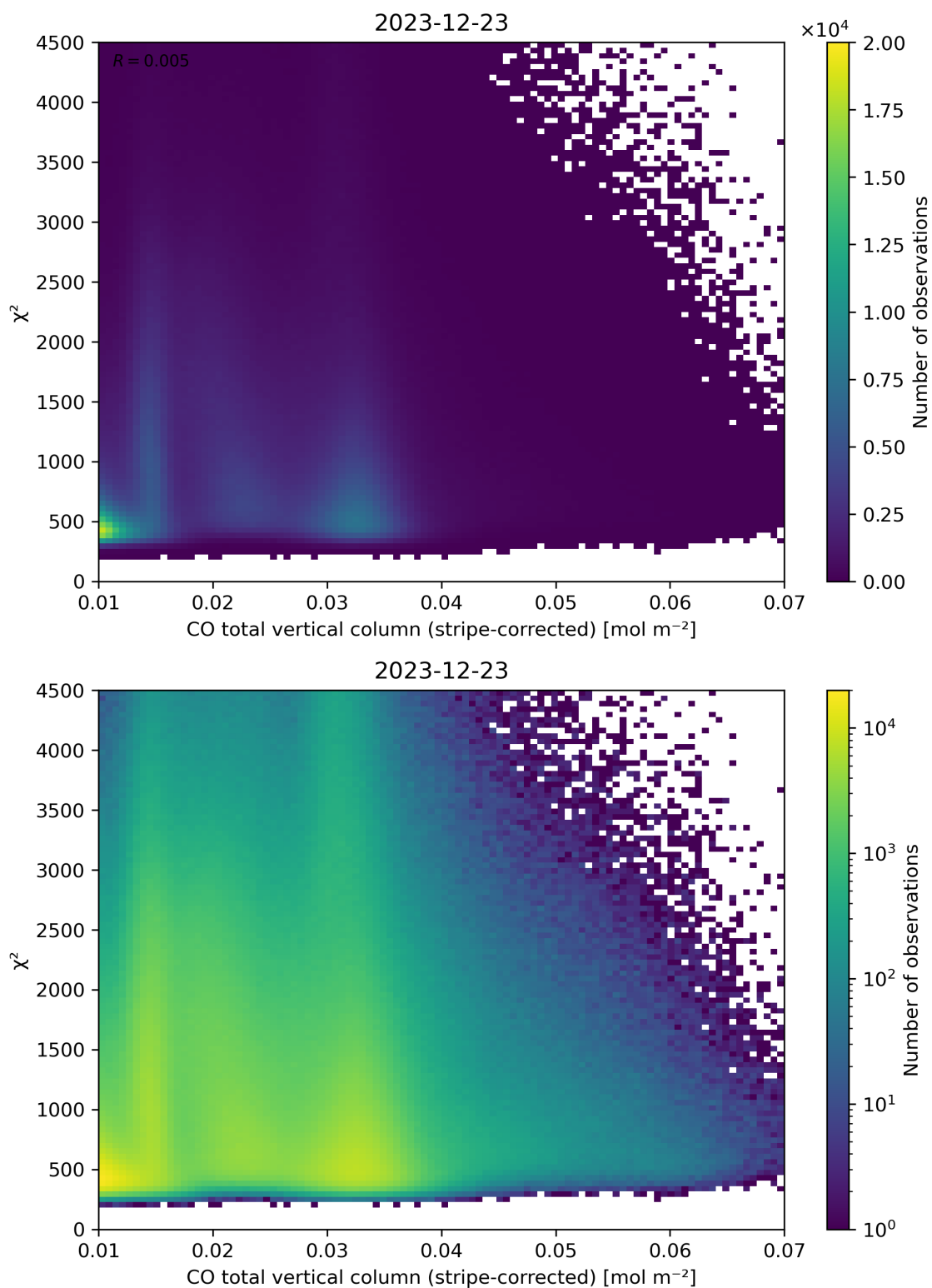
Figure 37: Scatter density plot of “CO total vertical column (stripe-corrected)” against “ \chi^2 ” for 2023-12-22 to 2023-12-24.
