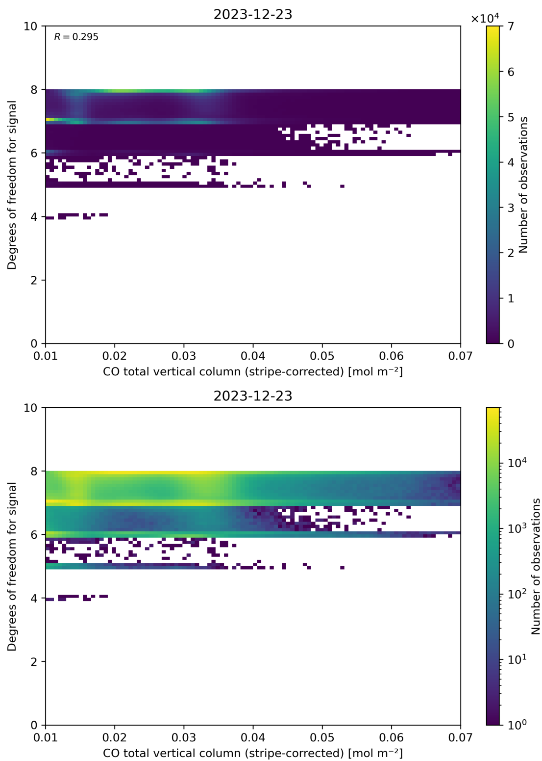
Figure 38: Scatter density plot of “CO total vertical column (stripe-corrected)” against “Degrees of freedom for signal” for 2023-12-22 to 2023-12-24.
