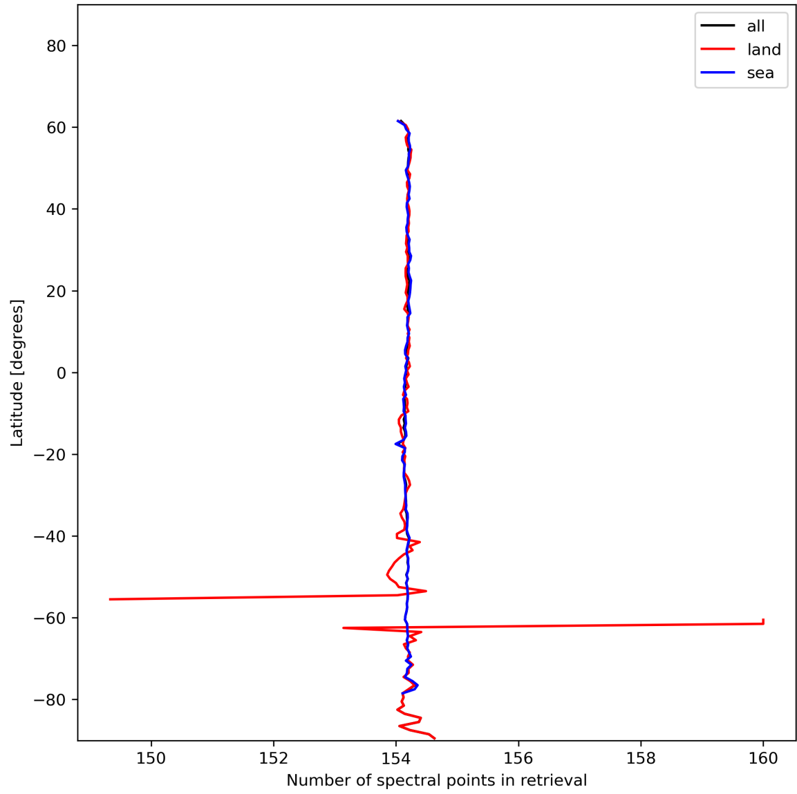
Figure 13: Zonal average of “Number of spectral points in retrieval” for 2023-12-22 to 2023-12-24.
