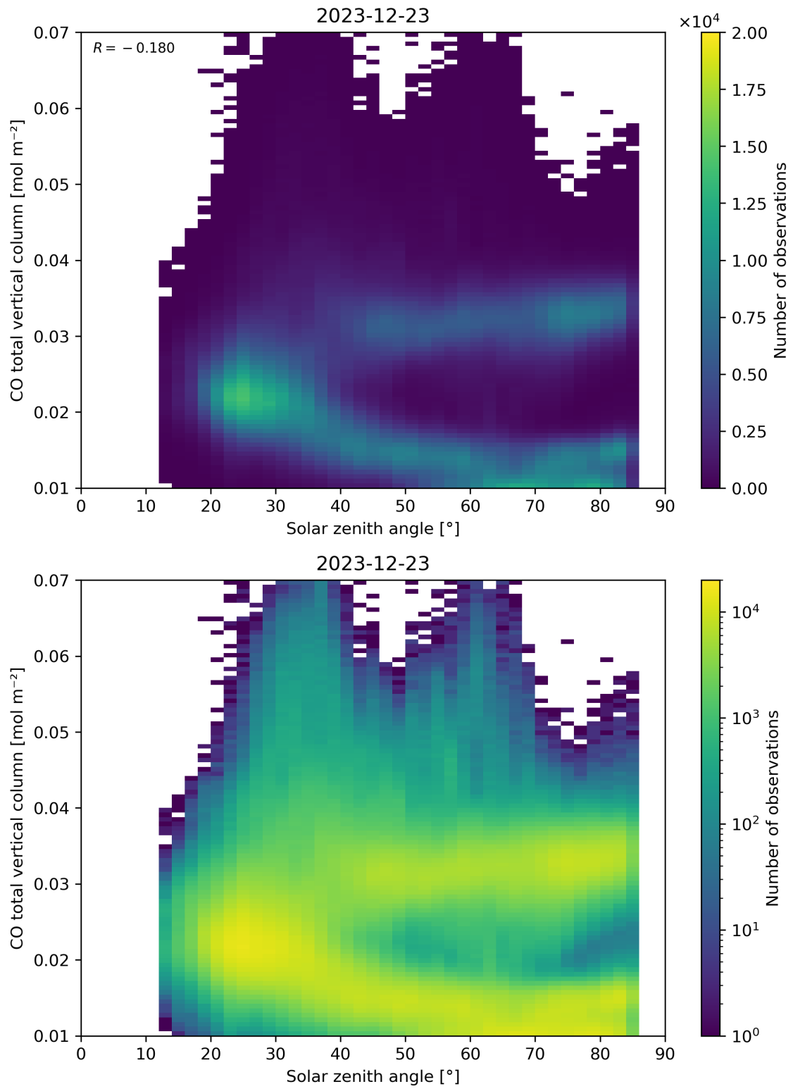
Figure 61: Scatter density plot of “Solar zenith angle” against “CO total vertical column” for 2023-12-22 to 2023-12-24.
