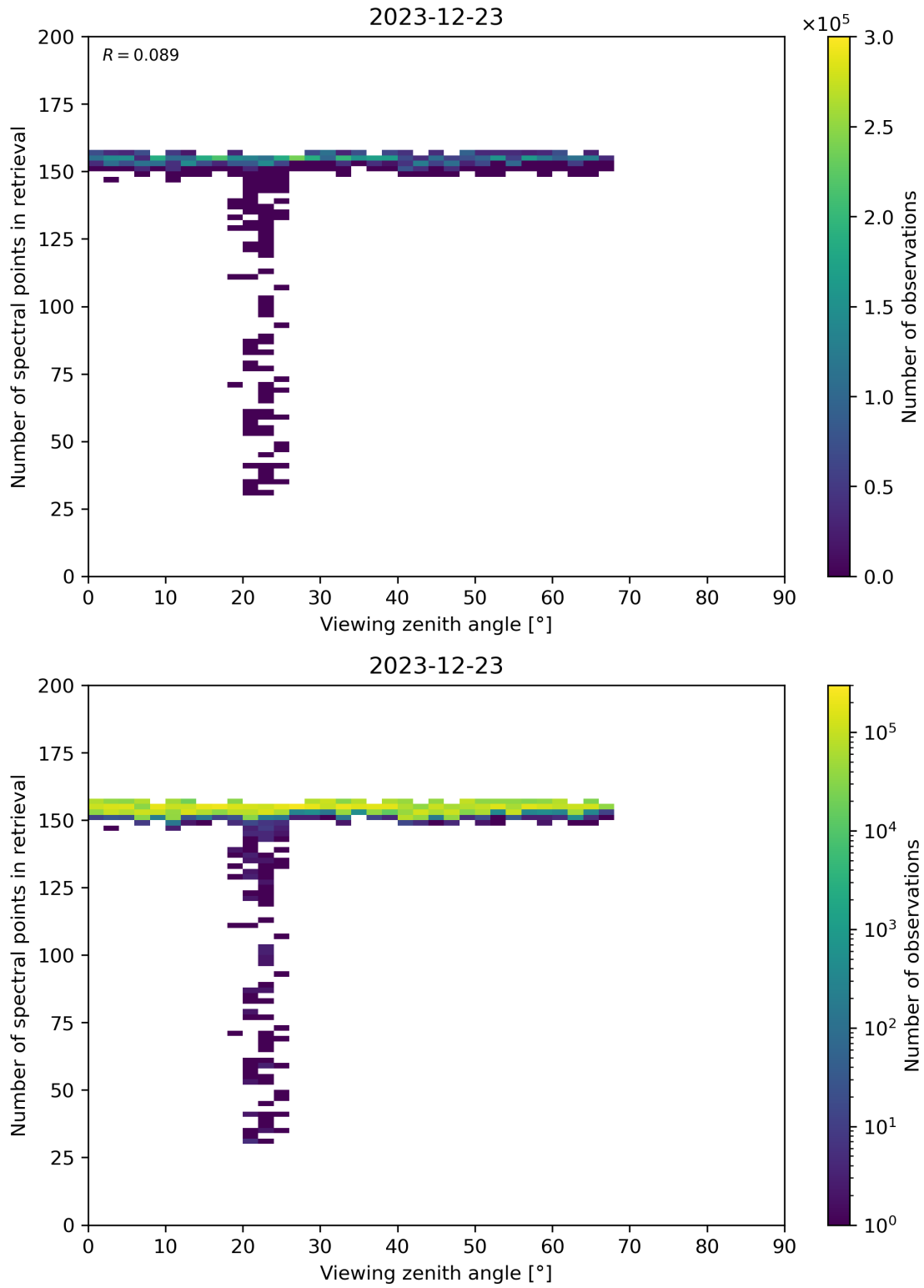
Figure 76: Scatter density plot of “Viewing zenith angle” against “Number of spectral points in retrieval” for 2023-12-22 to 2023-12-24.
