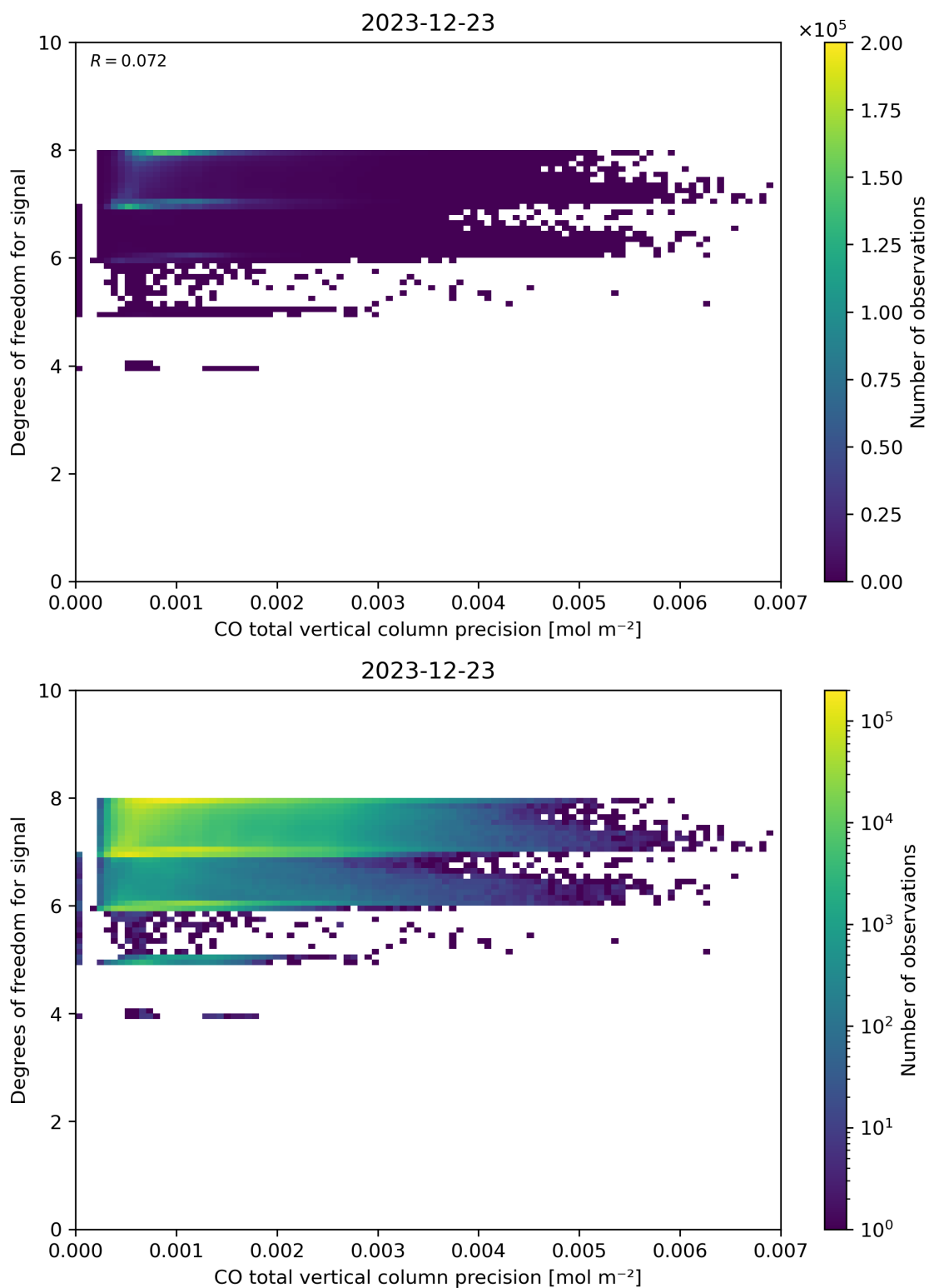
Figure 45: Scatter density plot of “CO total vertical column precision” against “Degrees of freedom for signal” for 2023-12-22 to 2023-12-24.
