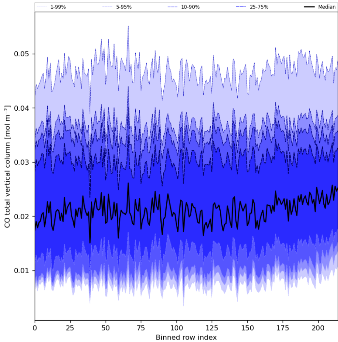
Figure 26: Along track statistics of “CO total vertical column” for 2023-12-22 to 2023-12-24
