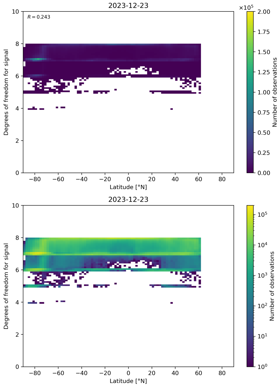
Figure 55: Scatter density plot of “Latitude” against “Degrees of freedom for signal” for 2023-12-22 to 2023-12-24.
