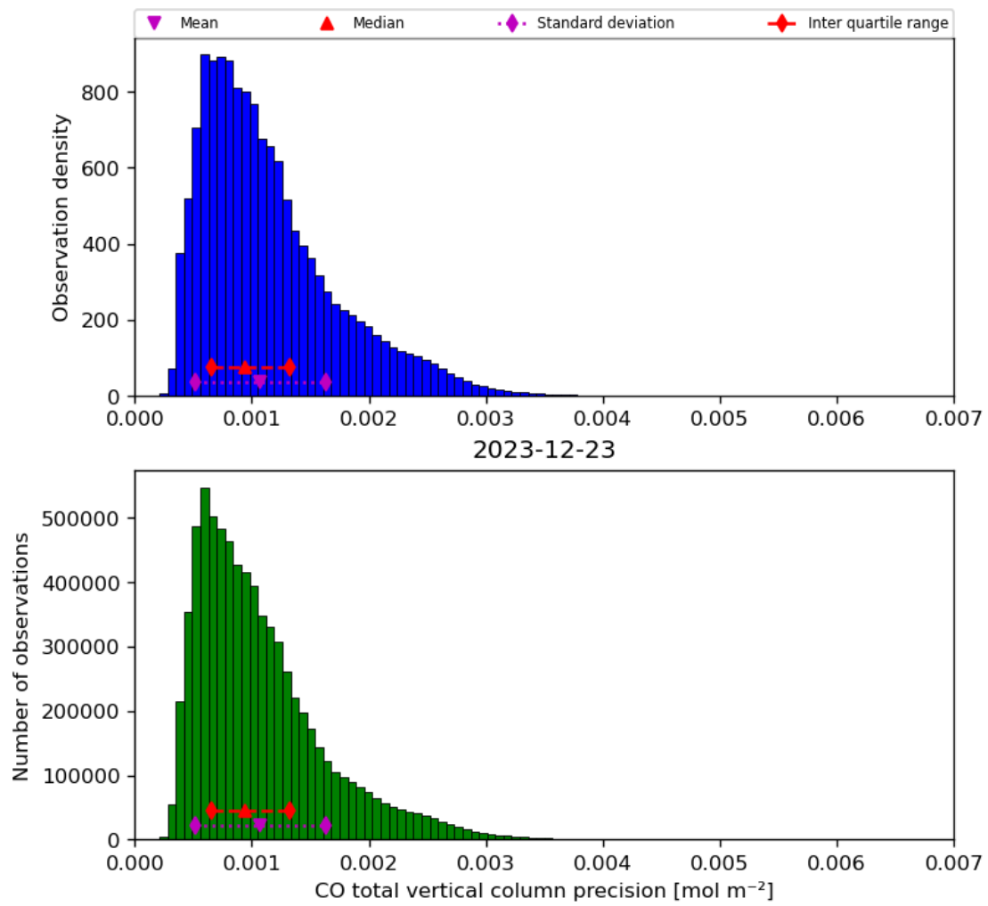
Figure 20: Histogram of “CO total vertical column precision” for 2023-12-22 to 2023-12-24
