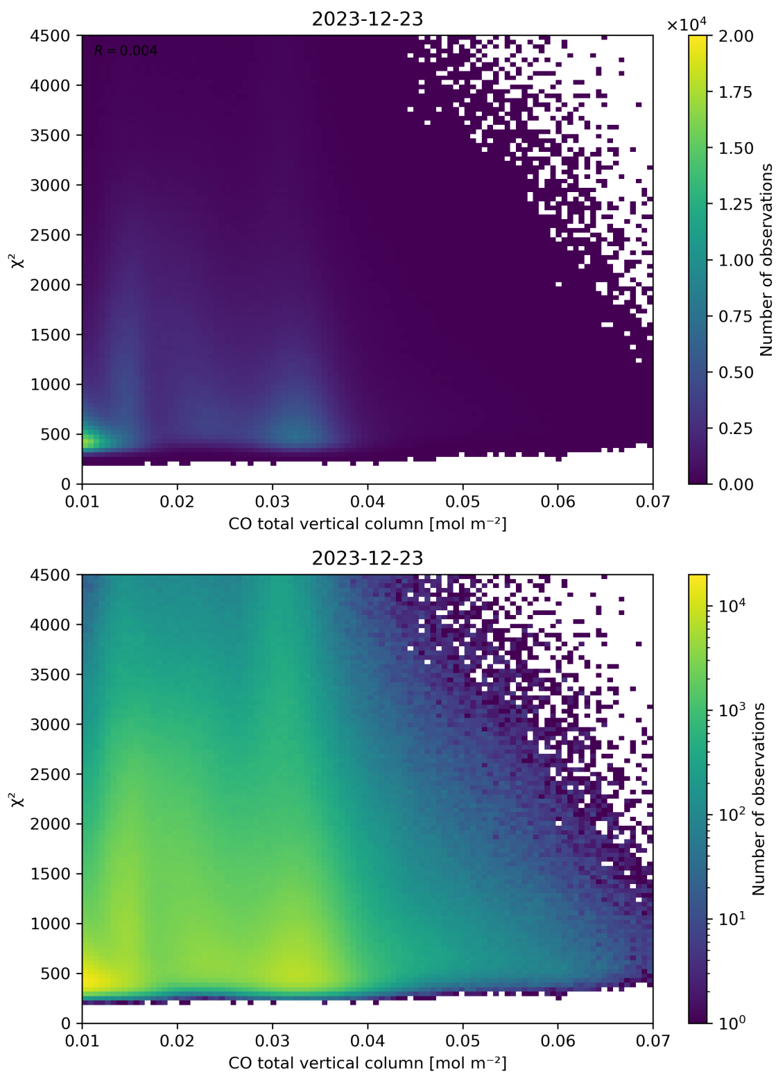
Figure 35: Scatter density plot of “CO total vertical column” against “ \chi^2 ” for 2023-12-22 to 2023-12-24.
