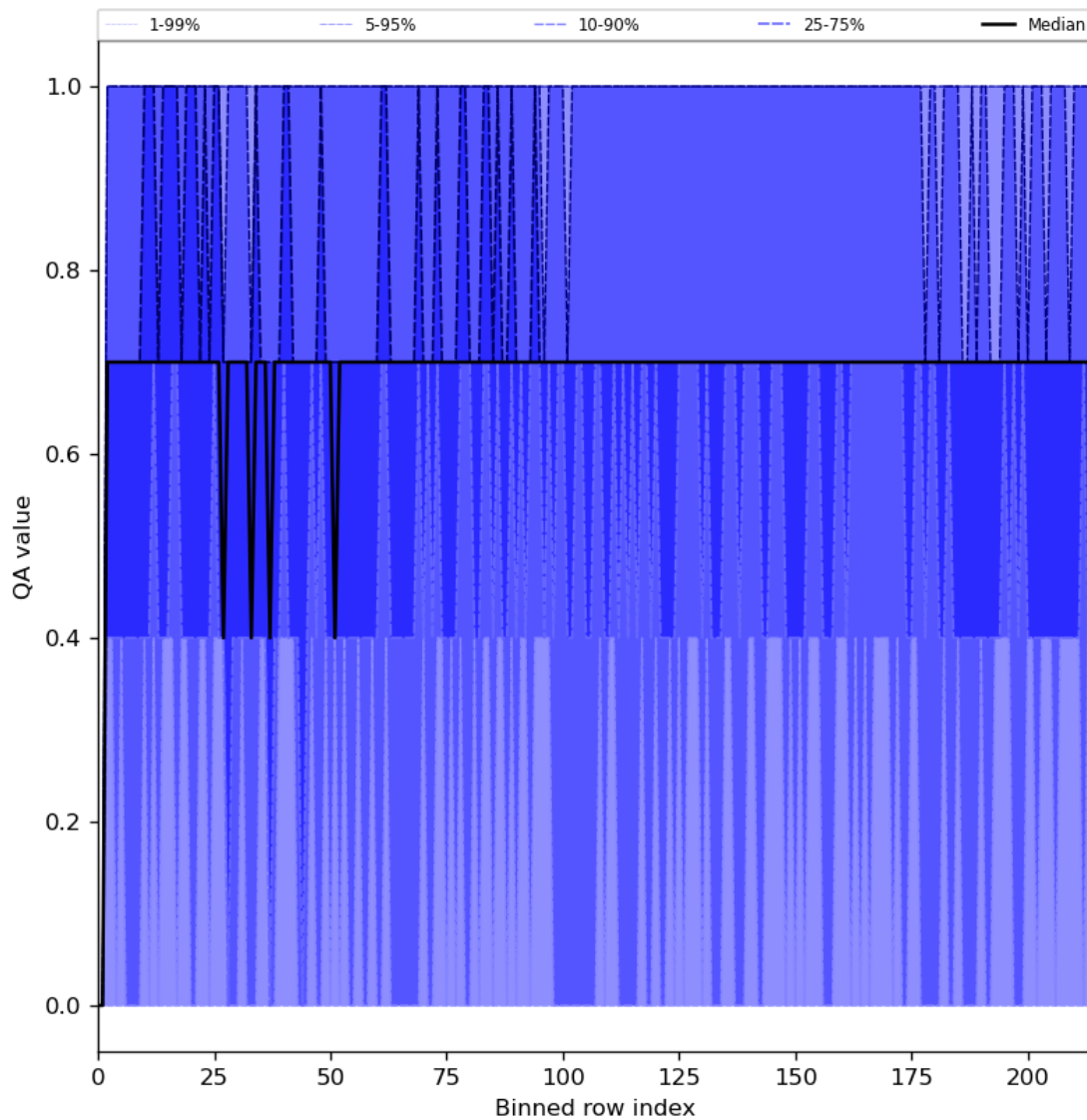
Figure 25: Along track statistics of “QA value” for 2023-12-22 to 2023-12-24
