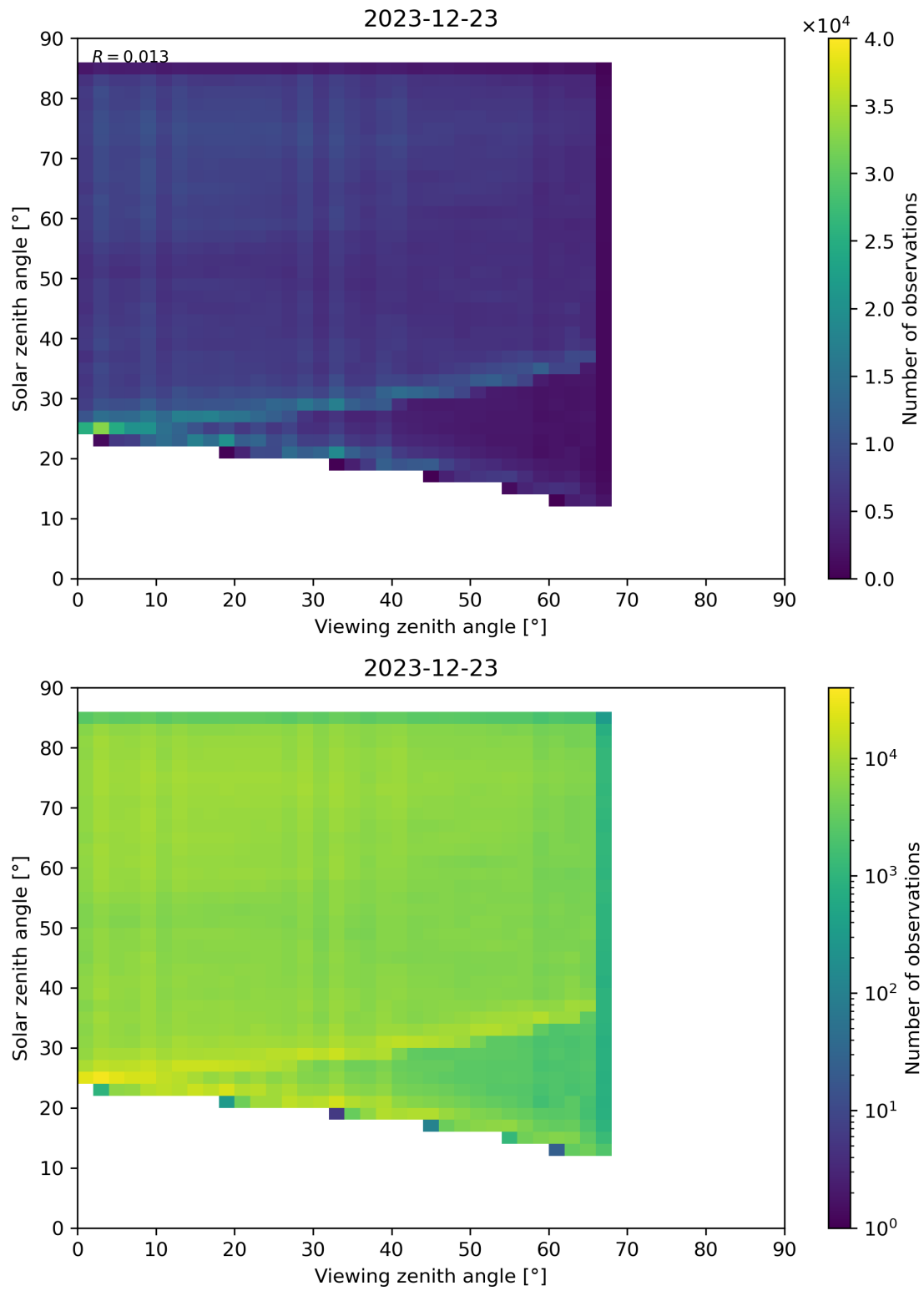
Figure 77: Scatter density plot of “Viewing zenith angle” against “Solar zenith angle” for 2023-12-22 to 2023-12-24.
