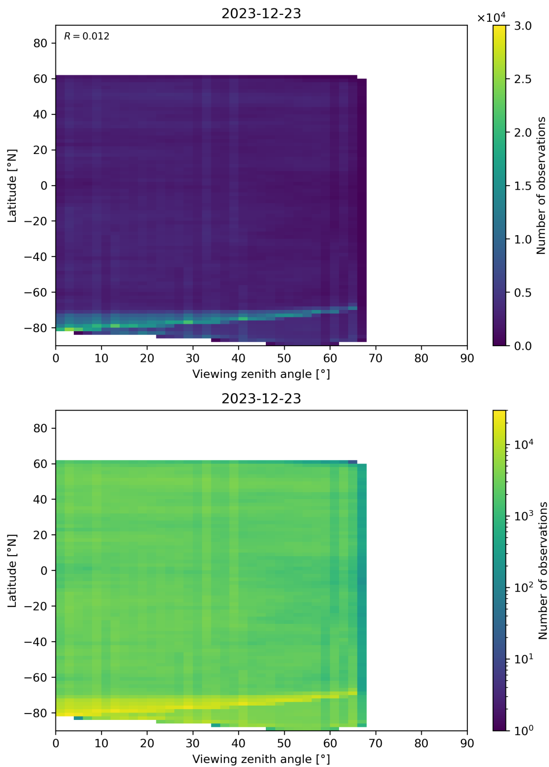
Figure 74: Scatter density plot of “Viewing zenith angle” against “Latitude” for 2023-12-22 to 2023-12-24.
