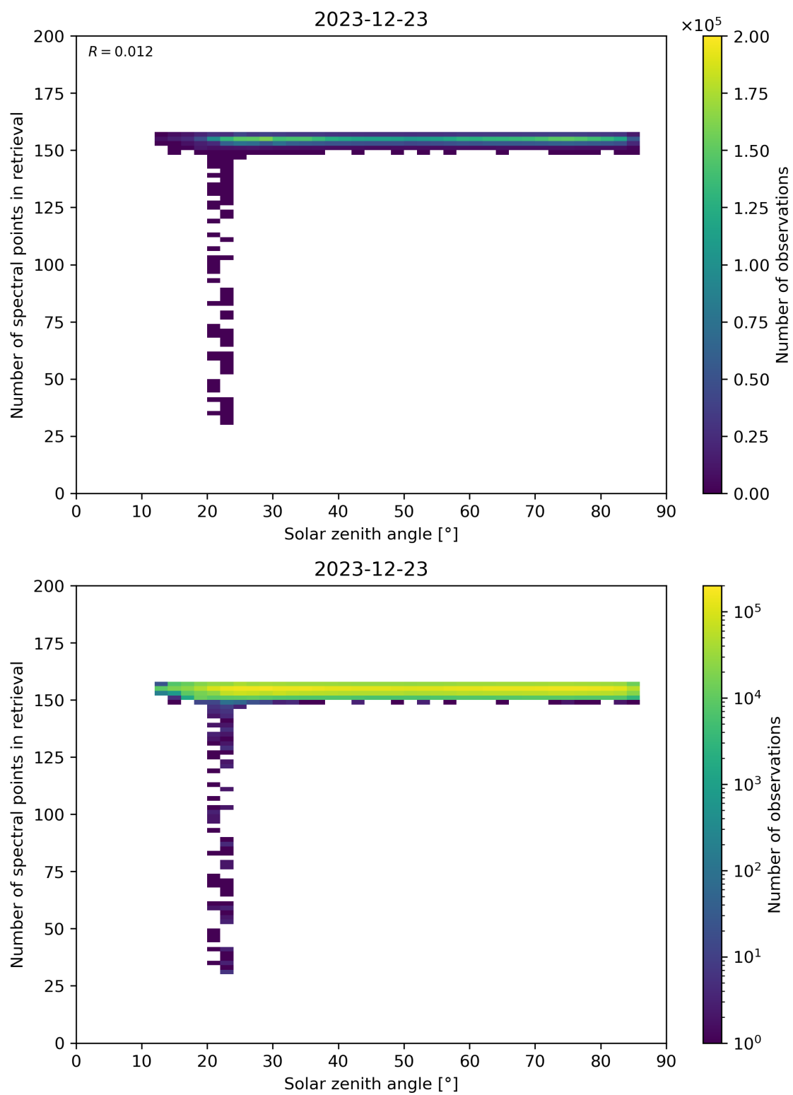
Figure 68: Scatter density plot of “Solar zenith angle” against “Number of spectral points in retrieval” for 2023-12-22 to 2023-12-24.
