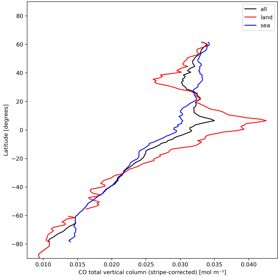
Figure 11: Zonal average of “CO total vertical column (stripe-corrected)” for 2023-12-22 to 2023-12-24.
