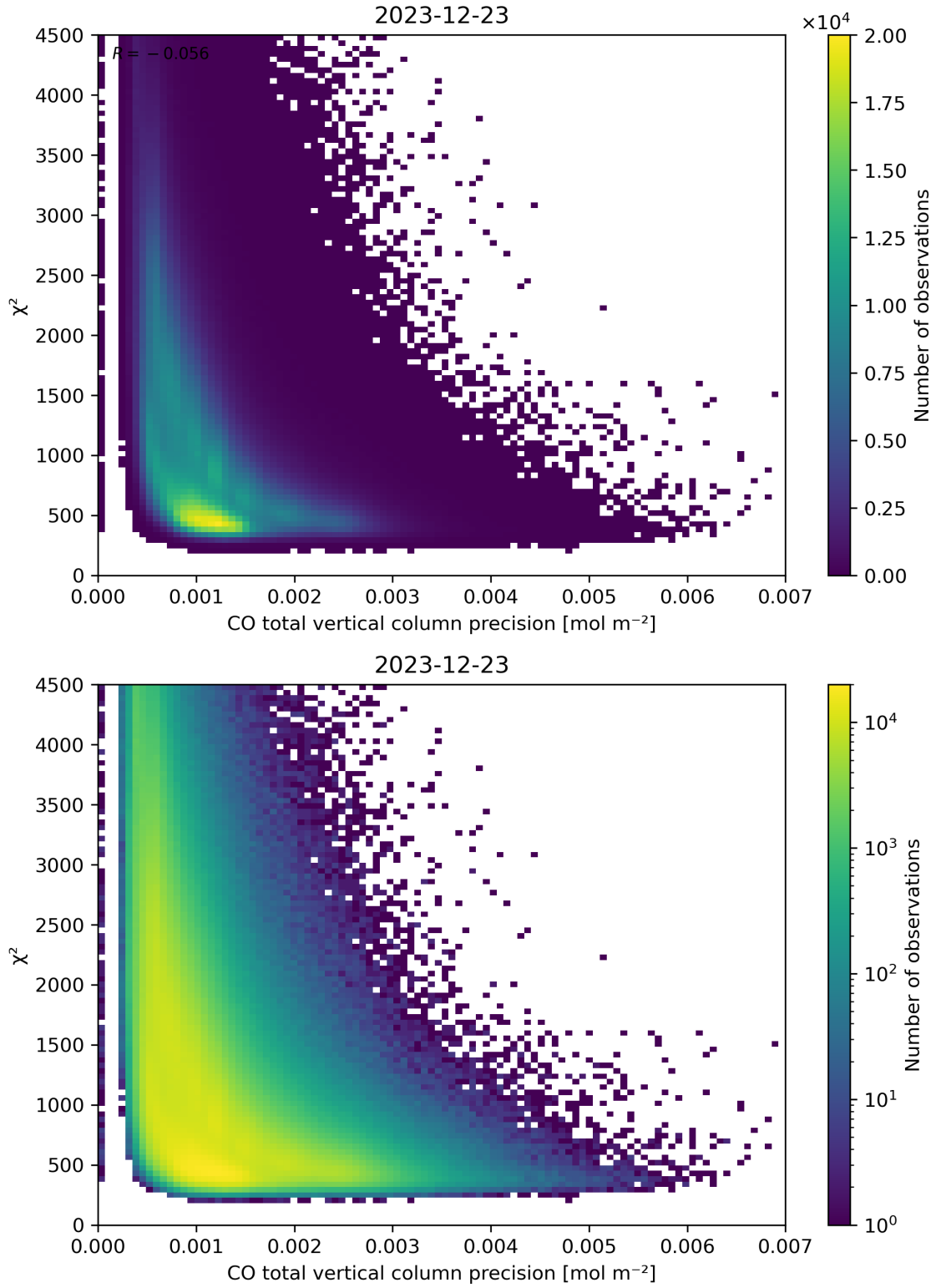
Figure 44: Scatter density plot of “CO total vertical column precision” against “ \chi^2 ” for 2023-12-22 to 2023-12-24.
