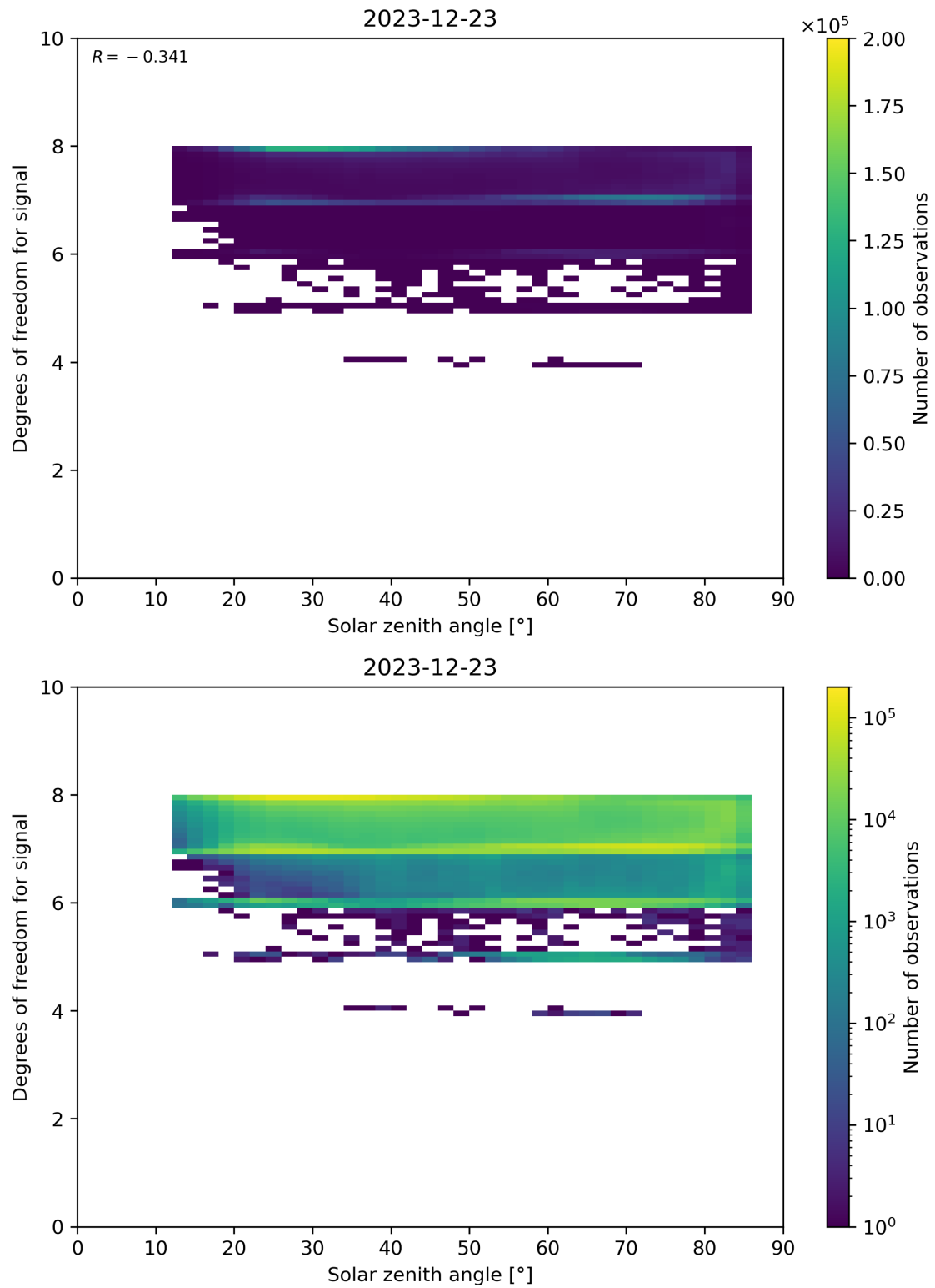
Figure 65: Scatter density plot of “Solar zenith angle” against “Degrees of freedom for signal” for 2023-12-22 to 2023-12-24.
