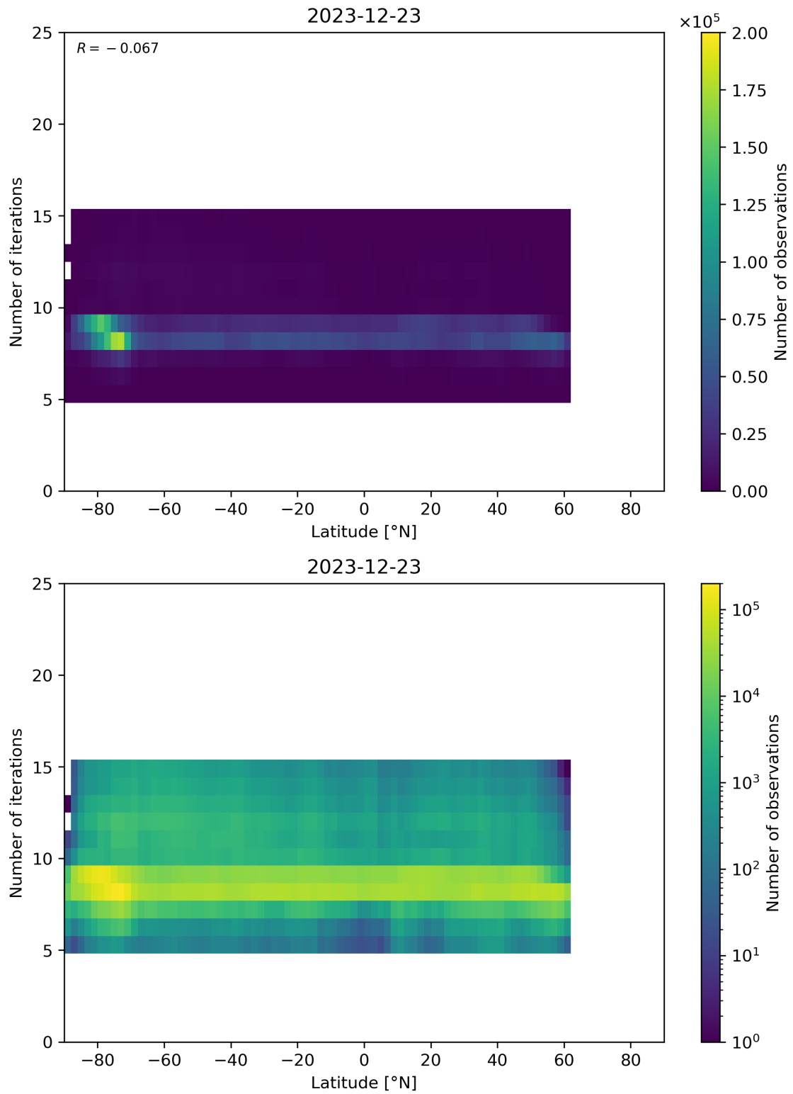
Figure 56: Scatter density plot of “Latitude” against “Number of iterations” for 2023-12-22 to 2023-12-24.
