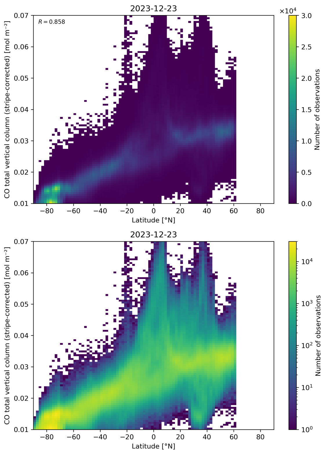
Figure 52: Scatter density plot of “Latitude” against “CO total vertical column (stripe-corrected)” for 2023-12-22 to 2023-12-24.
