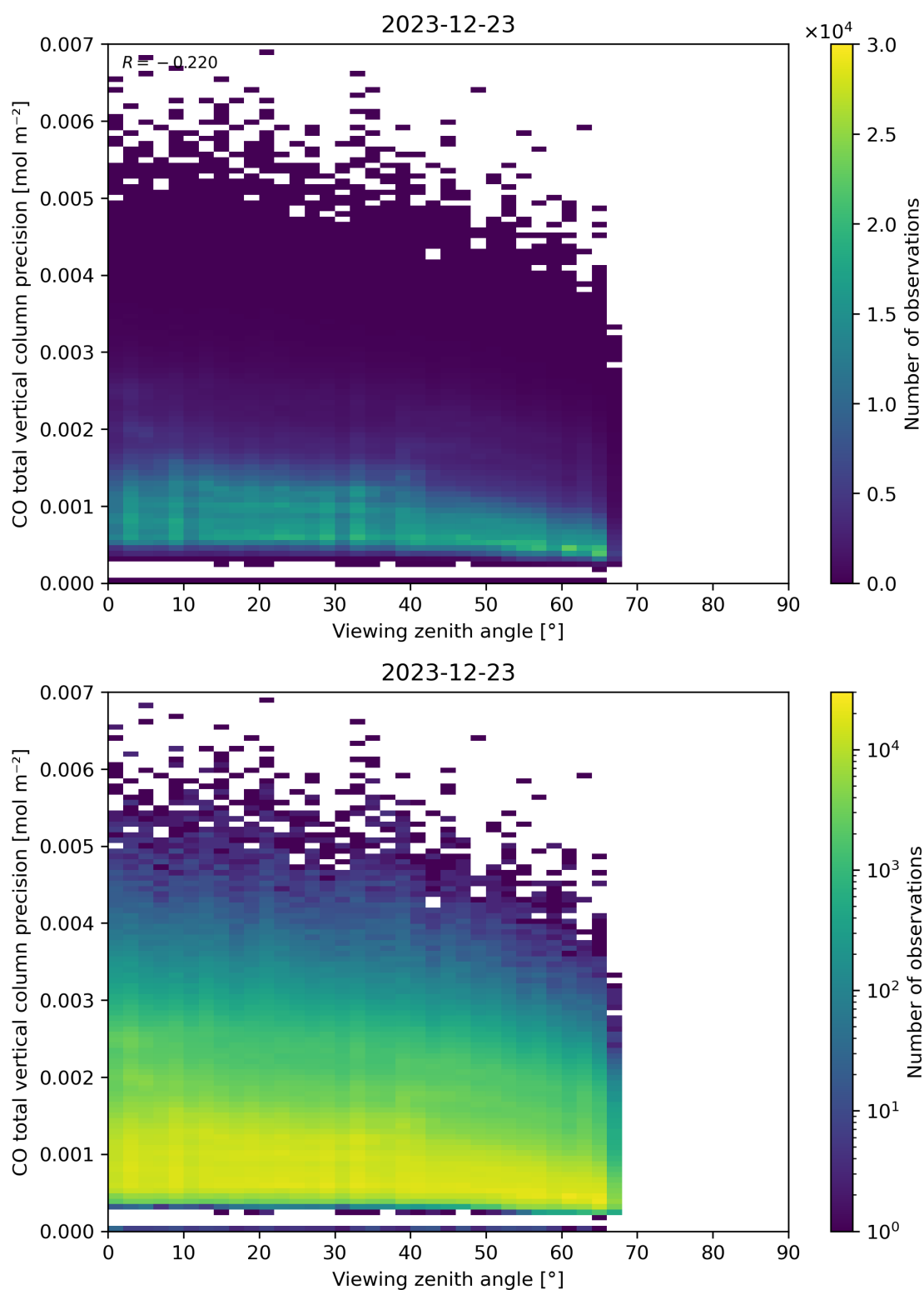
Figure 71: Scatter density plot of “Viewing zenith angle” against “CO total vertical column precision” for 2023-12-22 to 2023-12-24.
