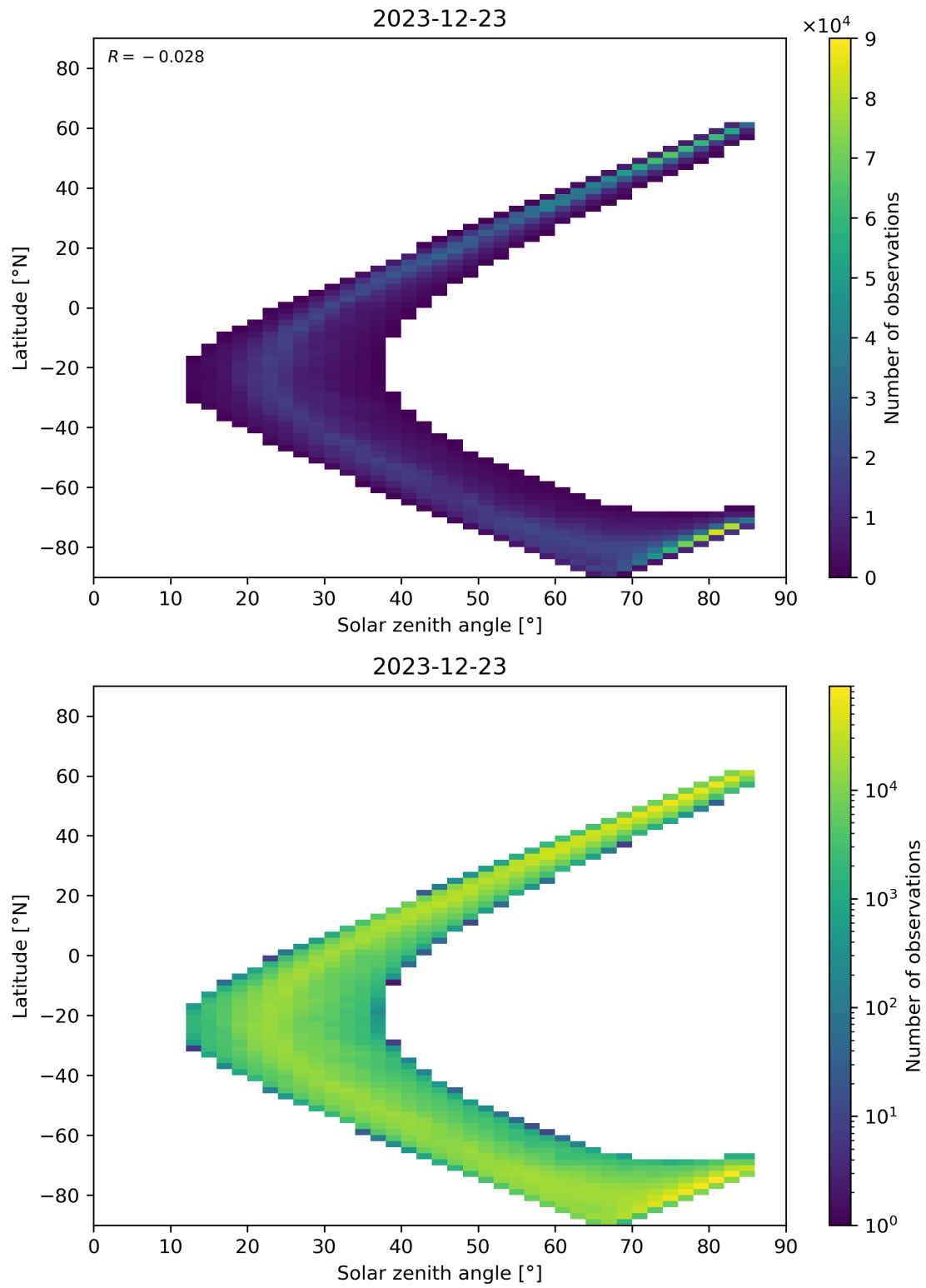
Figure 66: Scatter density plot of “Solar zenith angle” against “Latitude” for 2023-12-22 to 2023-12-24.
