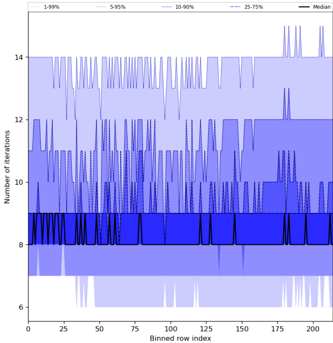
Figure 32: Along track statistics of “Number of iterations” for 2023-12-22 to 2023-12-24
