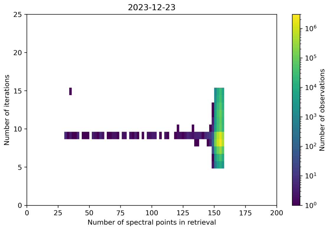
Figure 60: Scatter density plot of “Number of spectral points in retrieval” against “Number of iterations” for 2023-12-22 to 2023-12-24.
