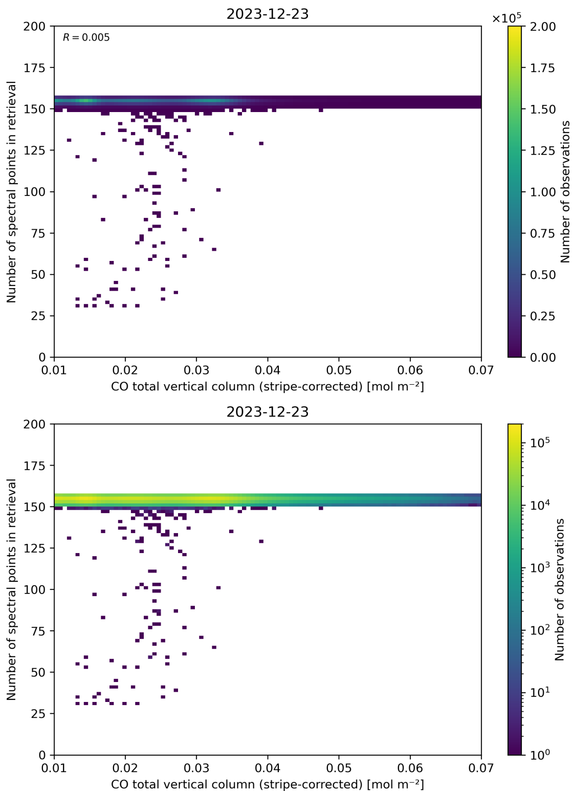
Figure 40: Scatter density plot of “CO total vertical column (stripe-corrected)” against “Number of spectral points in retrieval” for 2023-12-22 to 2023-12-24.
