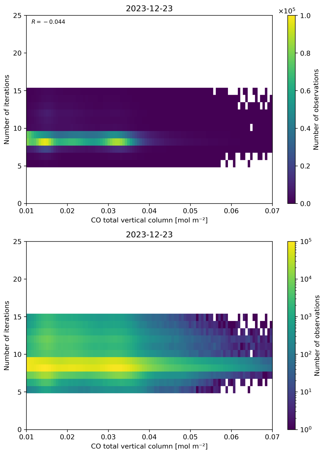
Figure 42: Scatter density plot of “CO total vertical column” against “Number of iterations” for 2023-12-22 to 2023-12-24.
