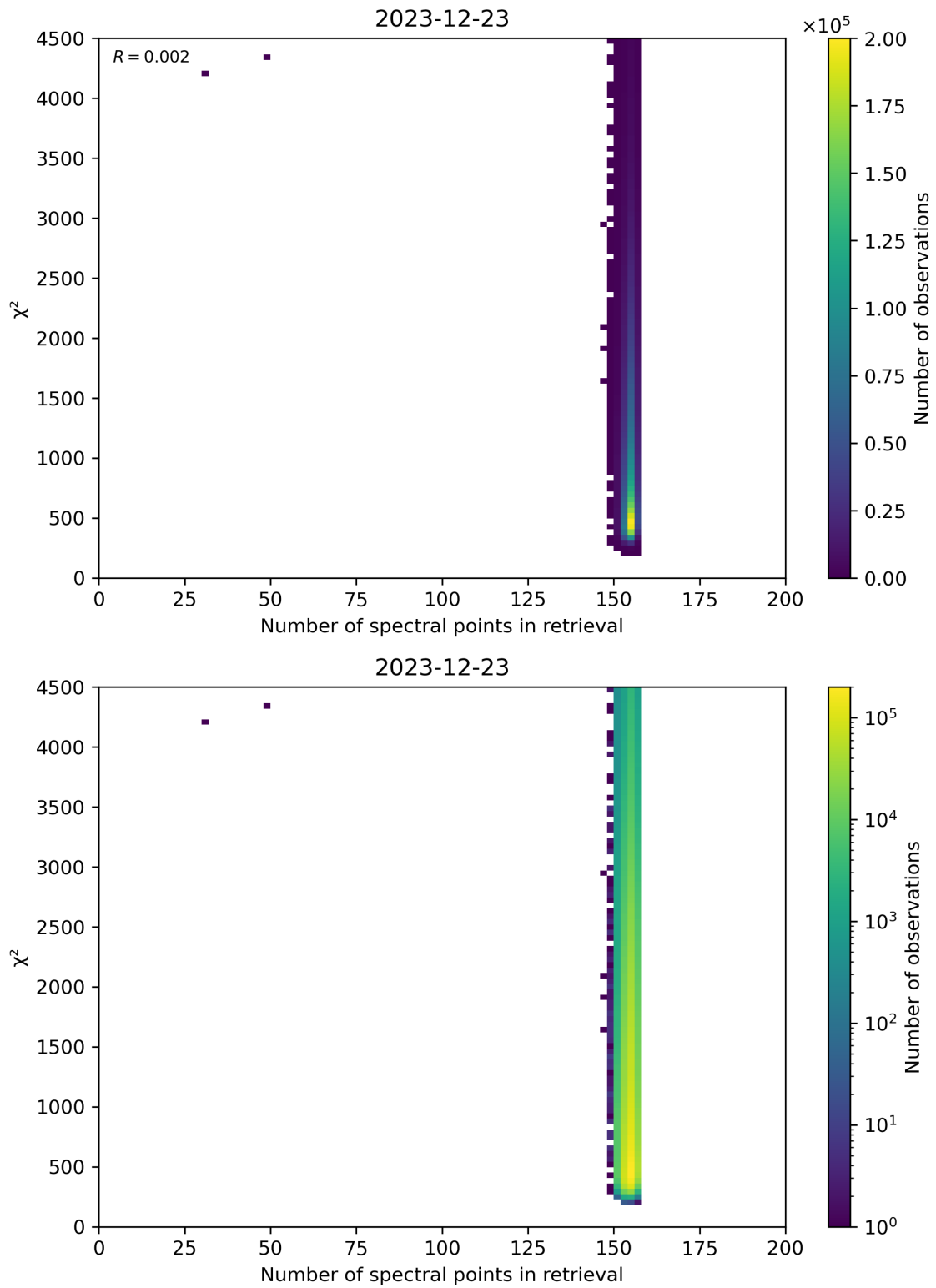
Figure 58: Scatter density plot of “Number of spectral points in retrieval” against “ \chi^2 ” for 2023-12-22 to 2023-12-24.
