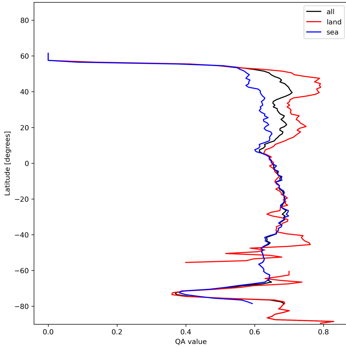
Figure 9: Zonal average of “QA value” for 2023-12-22 to 2023-12-24.
