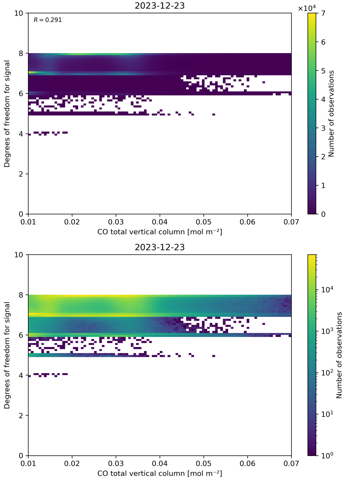
Figure 41: Scatter density plot of “CO total vertical column” against “Degrees of freedom for signal” for 2023-12-22 to 2023-12-24.
