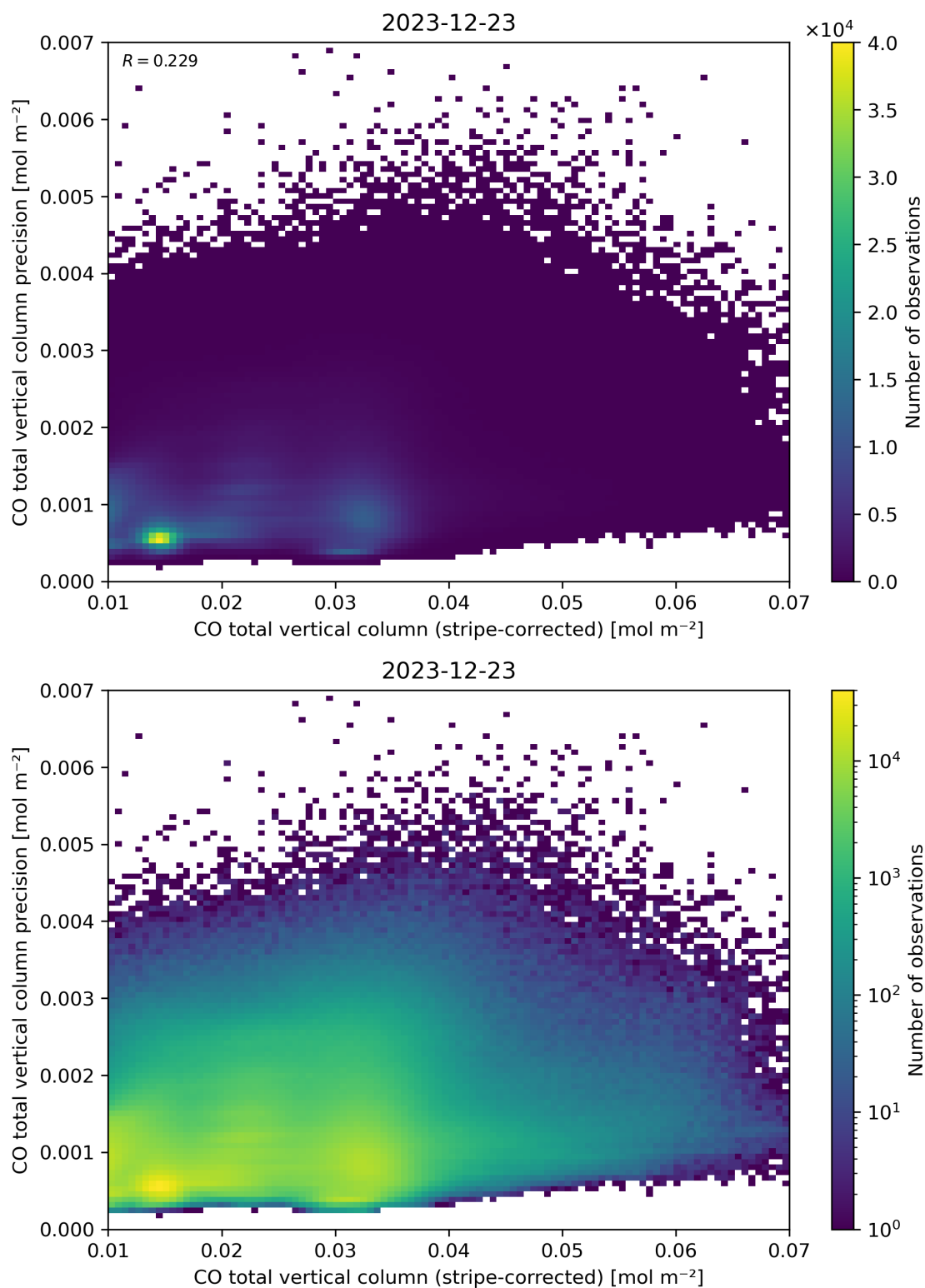
Figure 36: Scatter density plot of “CO total vertical column (stripe-corrected)” against “CO total vertical column precision” for 2023-12-22 to 2023-12-24.
