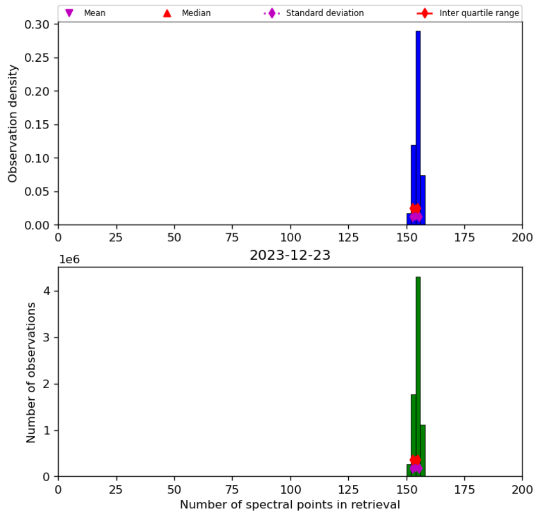
Figure 21: Histogram of “Number of spectral points in retrieval” for 2023-12-22 to 2023-12-24
