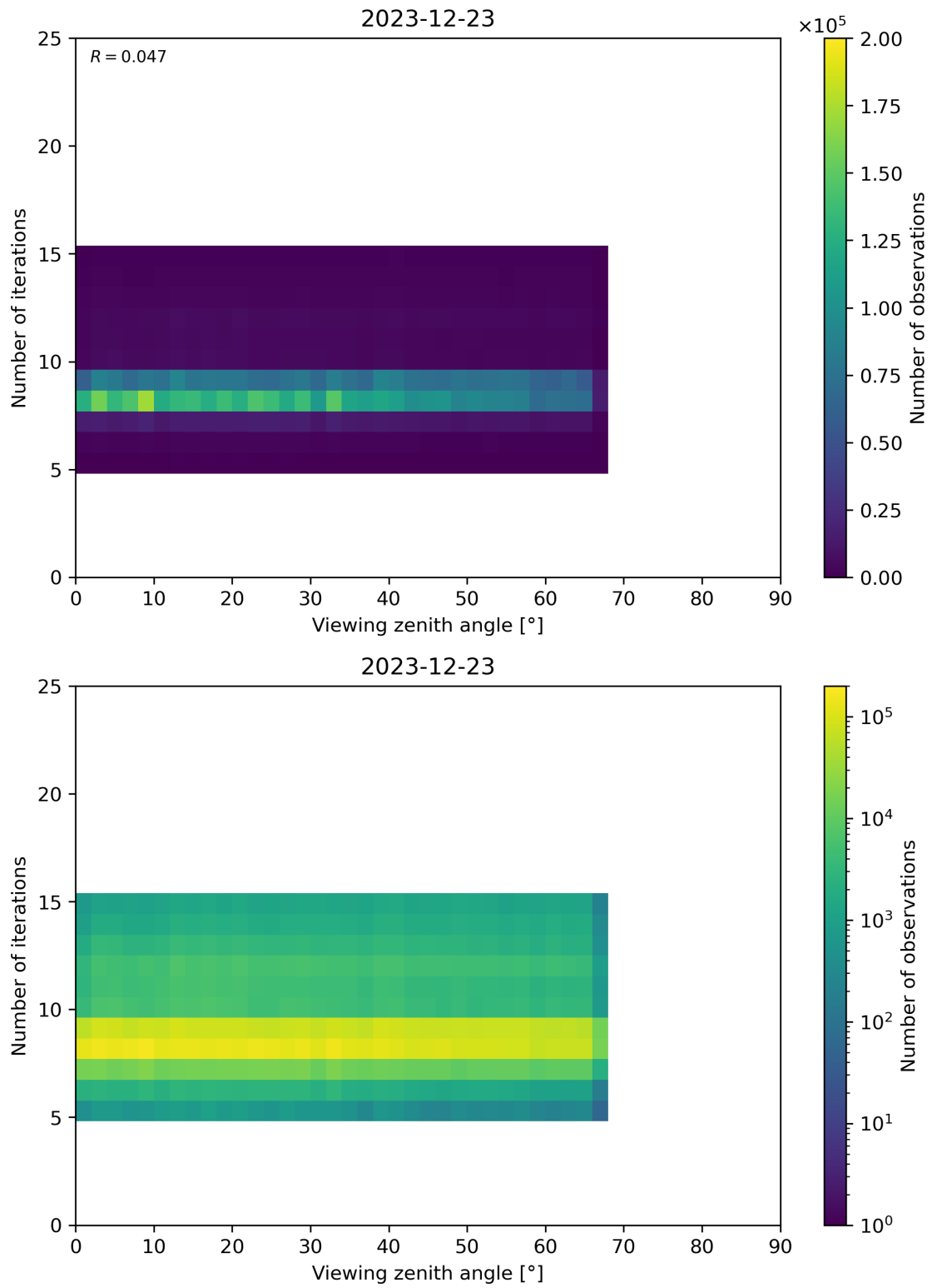
Figure 75: Scatter density plot of “Viewing zenith angle” against “Number of iterations” for 2023-12-22 to 2023-12-24.
