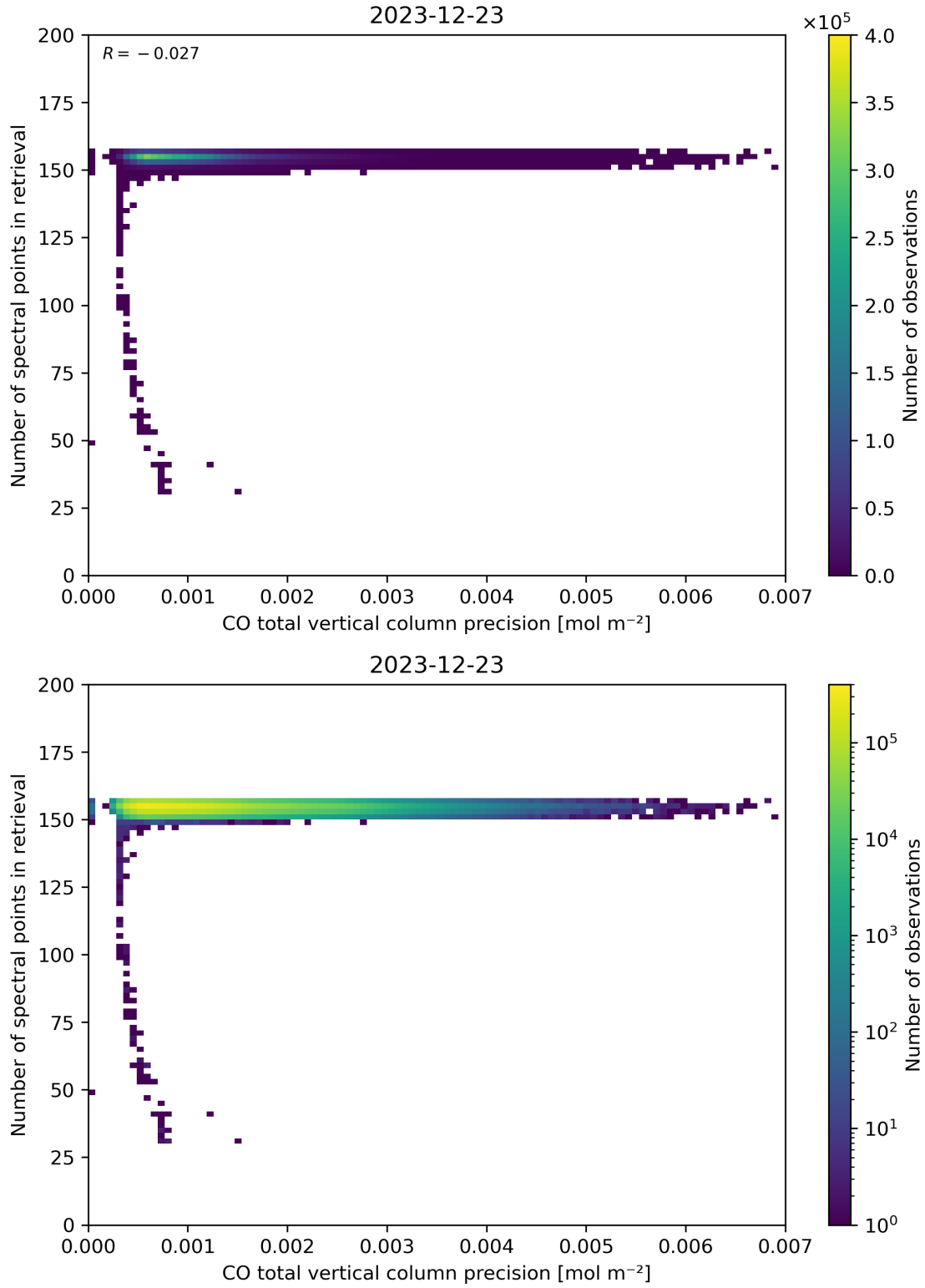
Figure 47: Scatter density plot of “CO total vertical column precision” against “Number of spectral points in retrieval” for 2023-12-22 to 2023-12-24.
