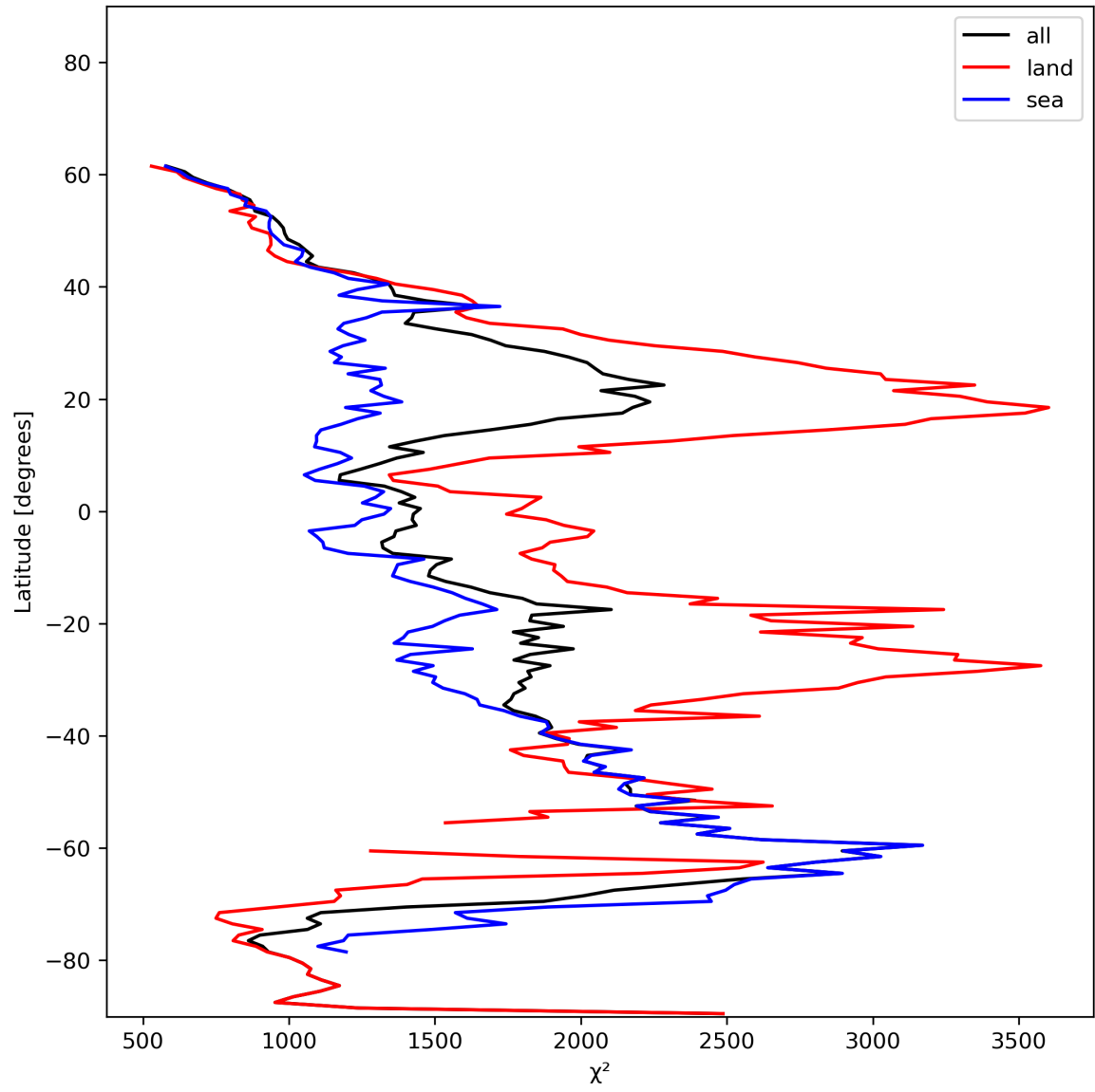
Figure 14: Zonal average of “ \chi^2 ” for 2023-12-22 to 2023-12-24.
