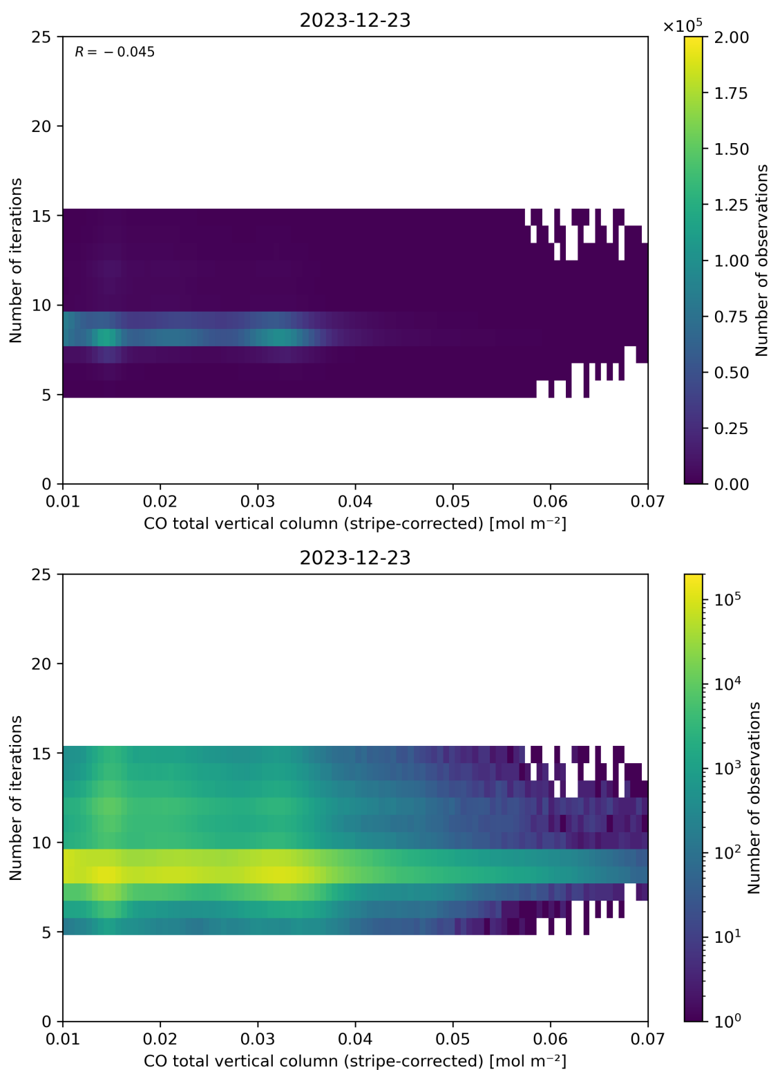
Figure 39: Scatter density plot of “CO total vertical column (stripe-corrected)” against “Number of iterations” for 2023-12-22 to 2023-12-24.
