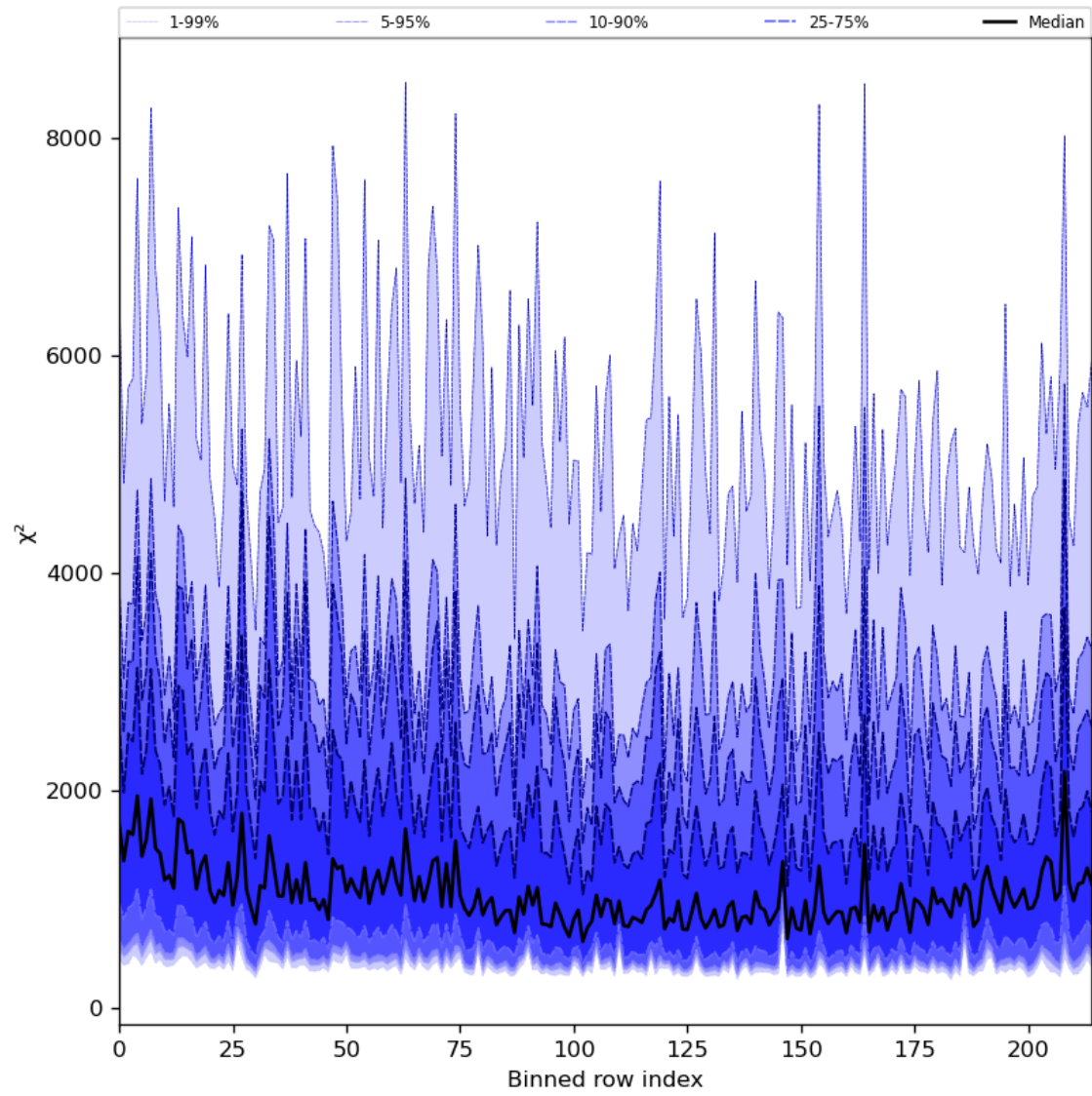
Figure 30: Along track statistics of “ \chi^2 ” for 2023-12-22 to 2023-12-24
