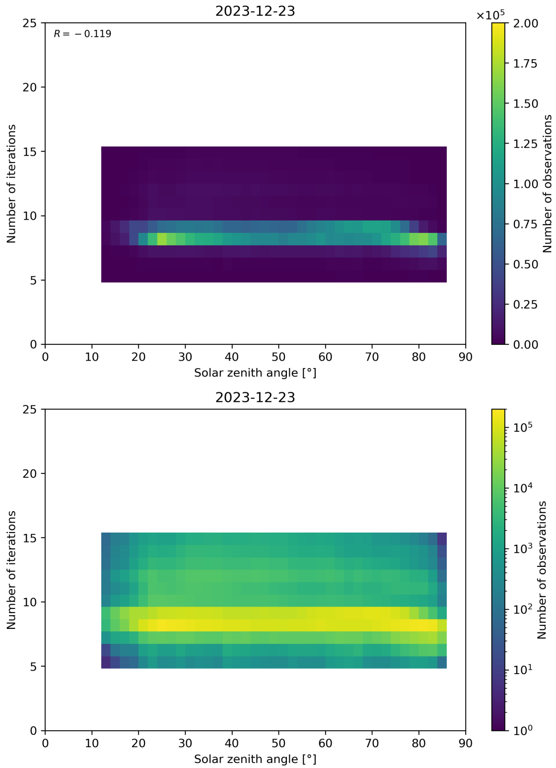
Figure 67: Scatter density plot of “Solar zenith angle” against “Number of iterations” for 2023-12-22 to 2023-12-24.
