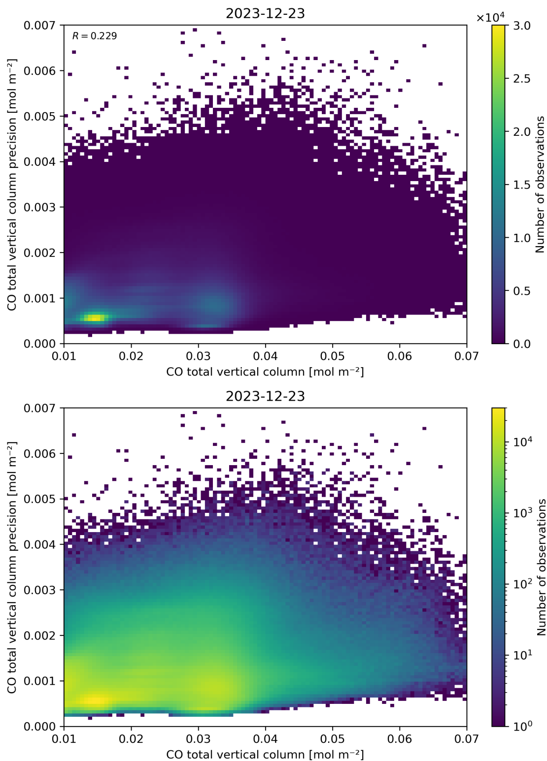
Figure 34: Scatter density plot of “CO total vertical column” against “CO total vertical column precision” for 2023-12-22 to 2023-12-24.
