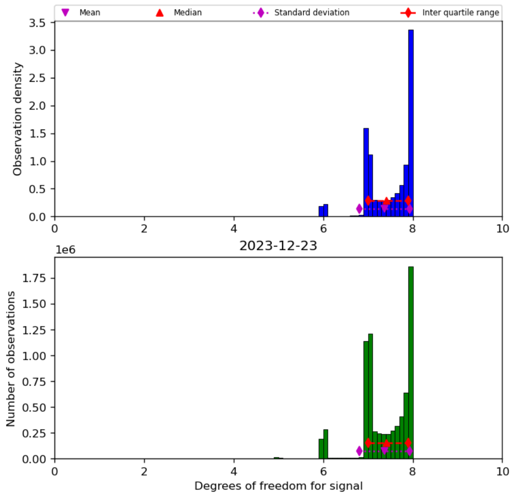
Figure 23: Histogram of “Degrees of freedom for signal” for 2023-12-22 to 2023-12-24
