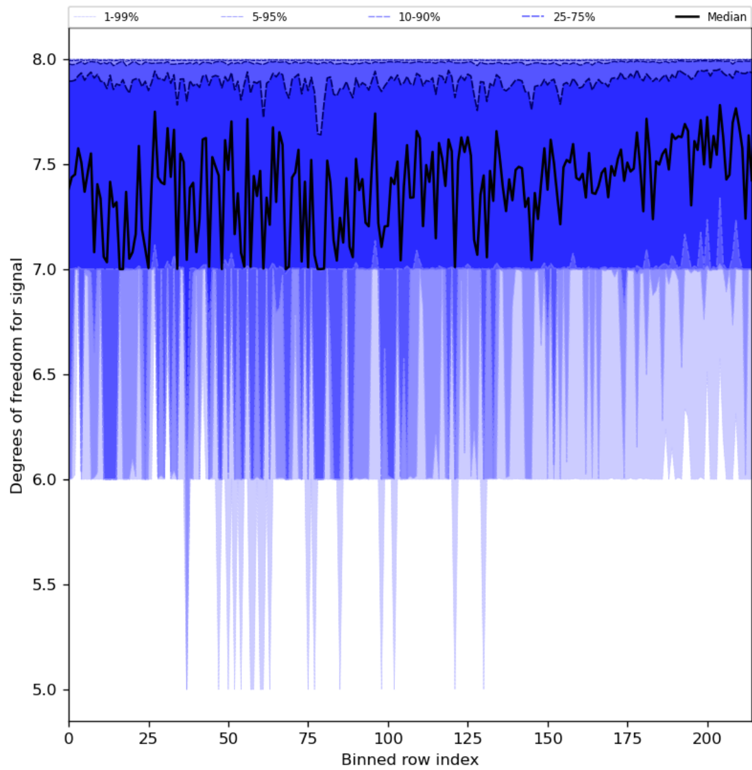
Figure 31: Along track statistics of “Degrees of freedom for signal” for 2023-12-22 to 2023-12-24
