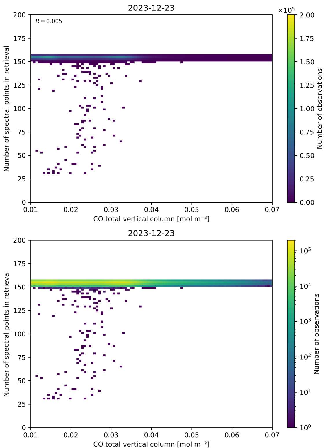
Figure 43: Scatter density plot of “CO total vertical column” against “Number of spectral points in retrieval” for 2023-12-22 to 2023-12-24.
