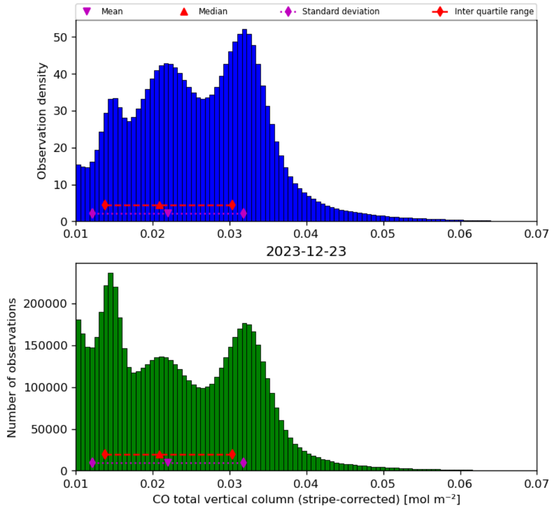
Figure 19: Histogram of “CO total vertical column (stripe-corrected)” for 2023-12-22 to 2023-12-24
