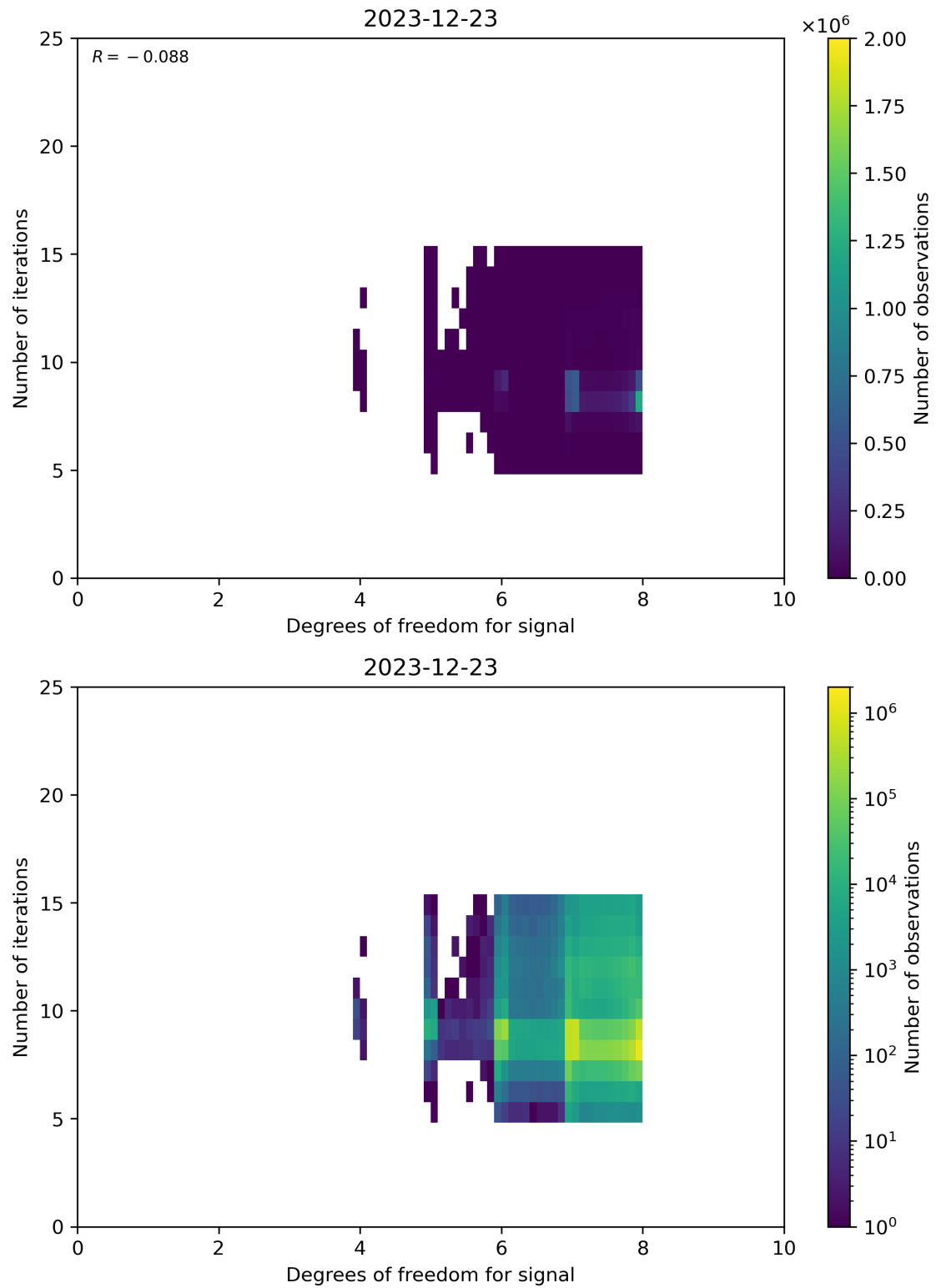
Figure 50: Scatter density plot of “Degrees of freedom for signal” against “Number of iterations” for 2023-12-22 to 2023-12-24.
