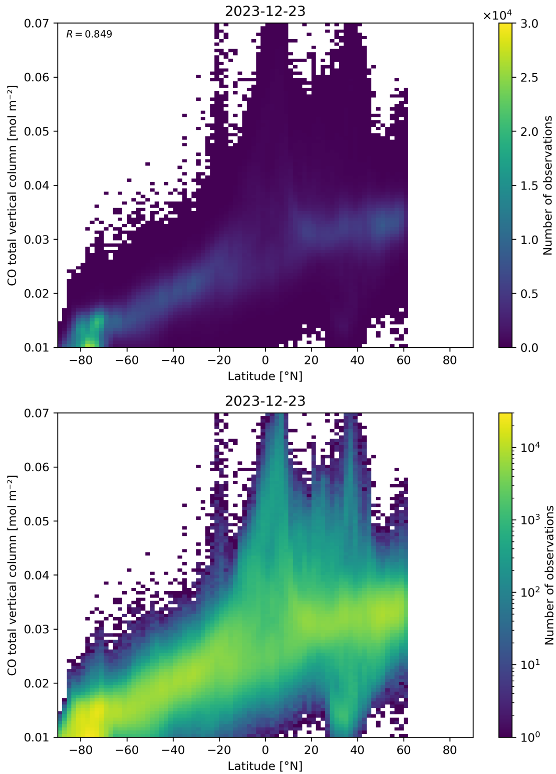
Figure 51: Scatter density plot of “Latitude” against “CO total vertical column” for 2023-12-22 to 2023-12-24.
