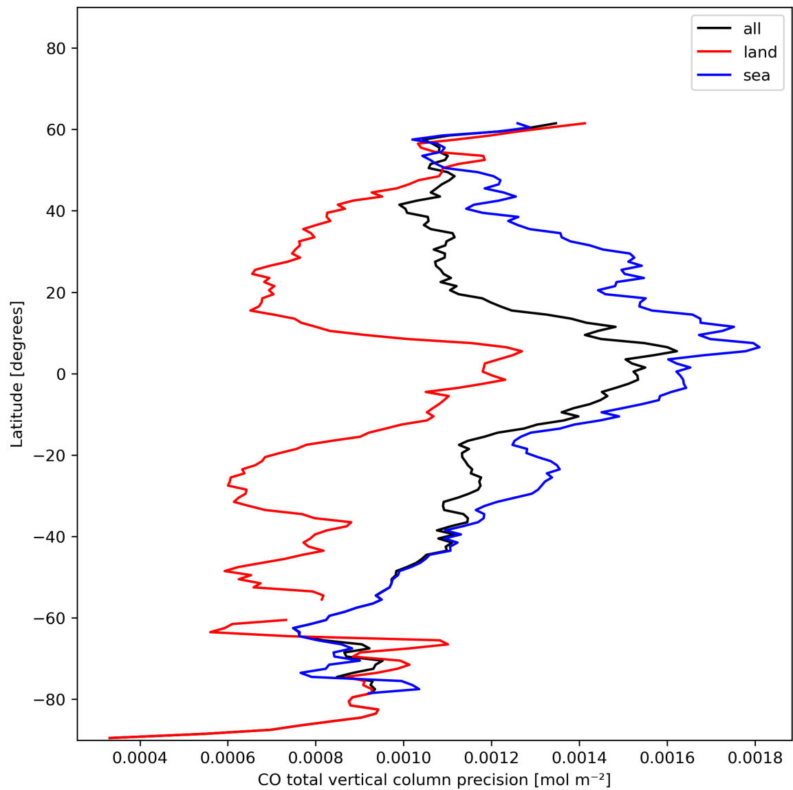
Figure 12: Zonal average of “CO total vertical column precision” for 2023-12-22 to 2023-12-24.
