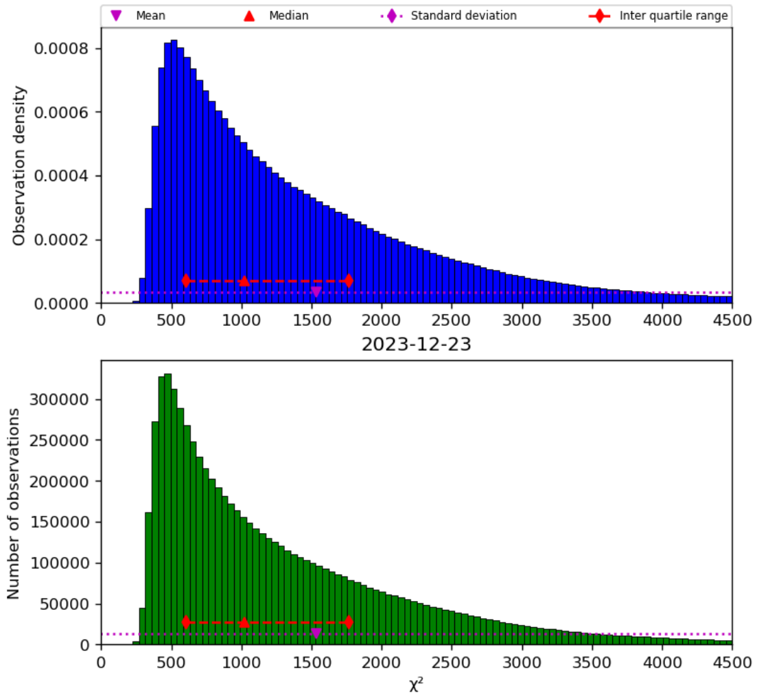
Figure 22: Histogram of “ \chi^2 ” for 2023-12-22 to 2023-12-24
