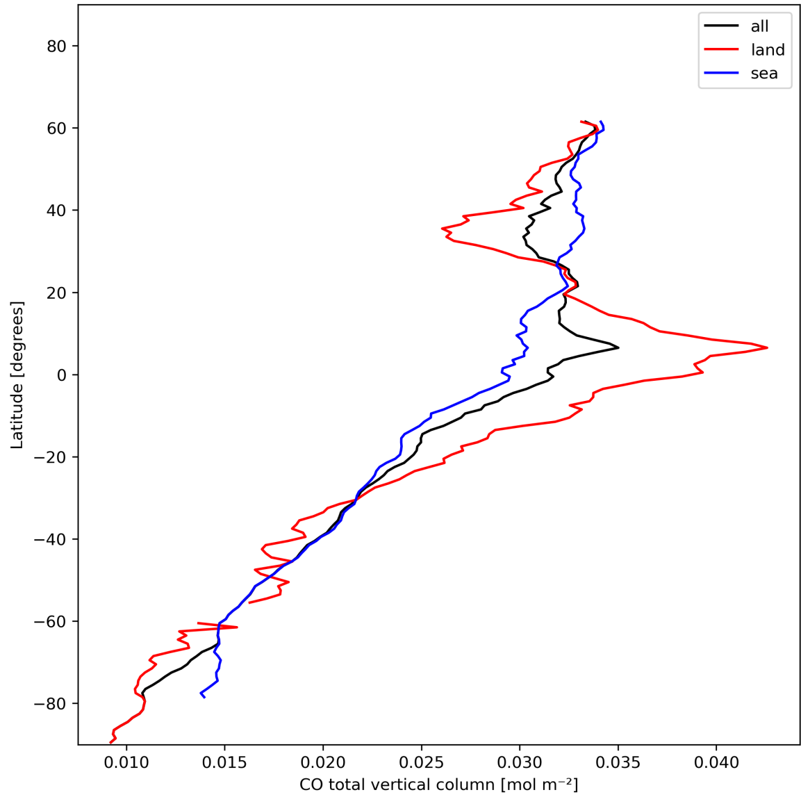
Figure 10: Zonal average of “CO total vertical column” for 2023-12-22 to 2023-12-24.
