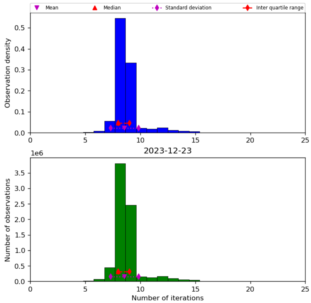
Figure 24: Histogram of “Number of iterations” for 2023-12-22 to 2023-12-24
