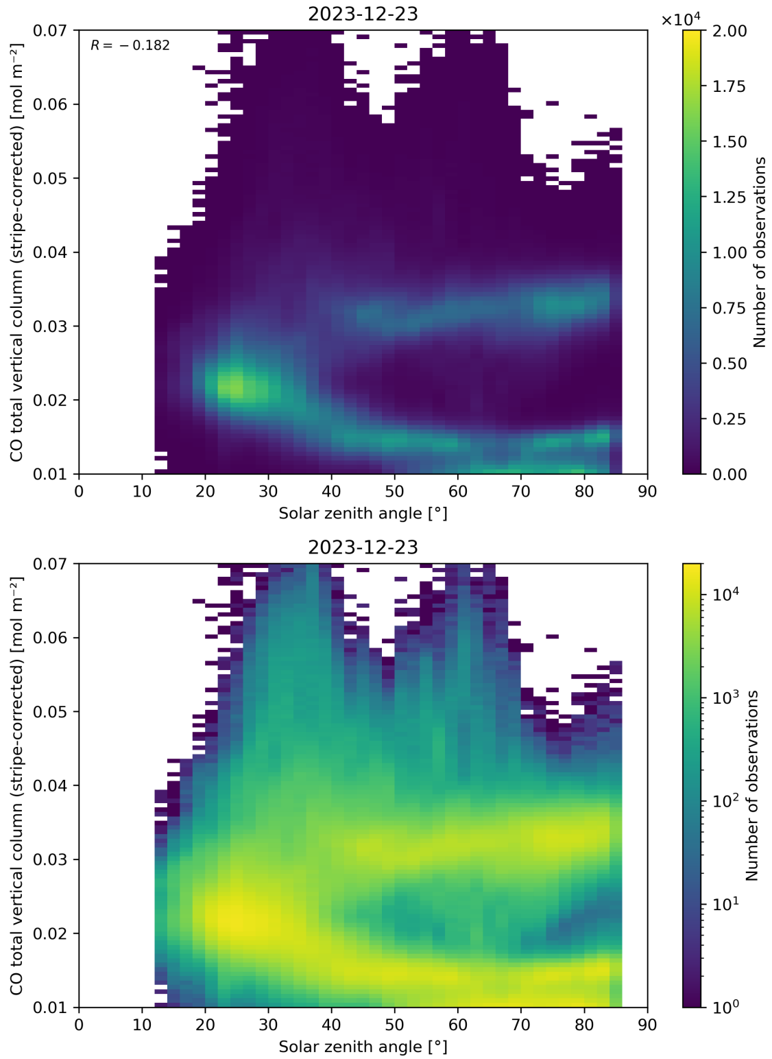
Figure 62: Scatter density plot of “Solar zenith angle” against “CO total vertical column (stripe-corrected)” for 2023-12-22 to 2023-12-24.
