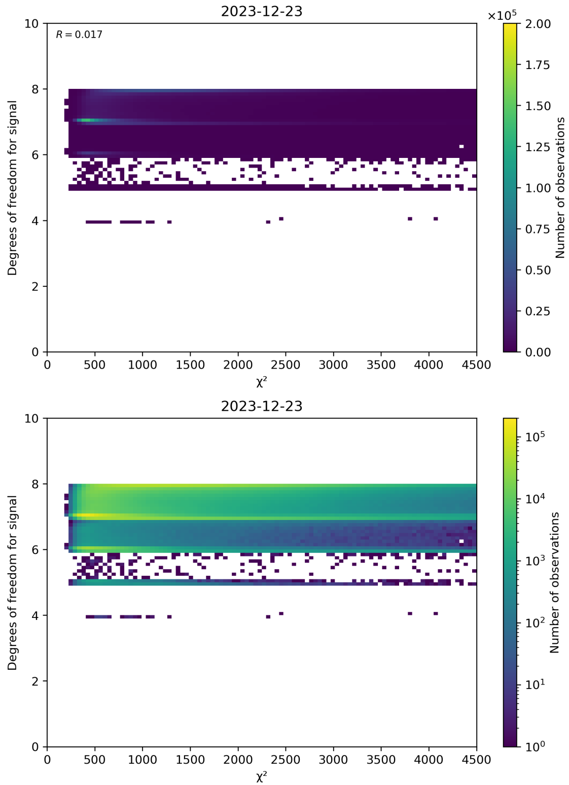
Figure 48: Scatter density plot of “ \chi^2 ” against “Degrees of freedom for signal” for 2023-12-22 to 2023-12-24.
