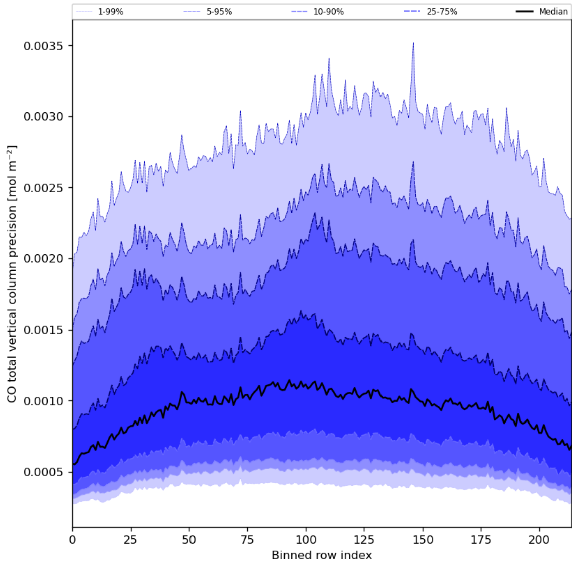
Figure 28: Along track statistics of “CO total vertical column precision” for 2023-12-22 to 2023-12-24
