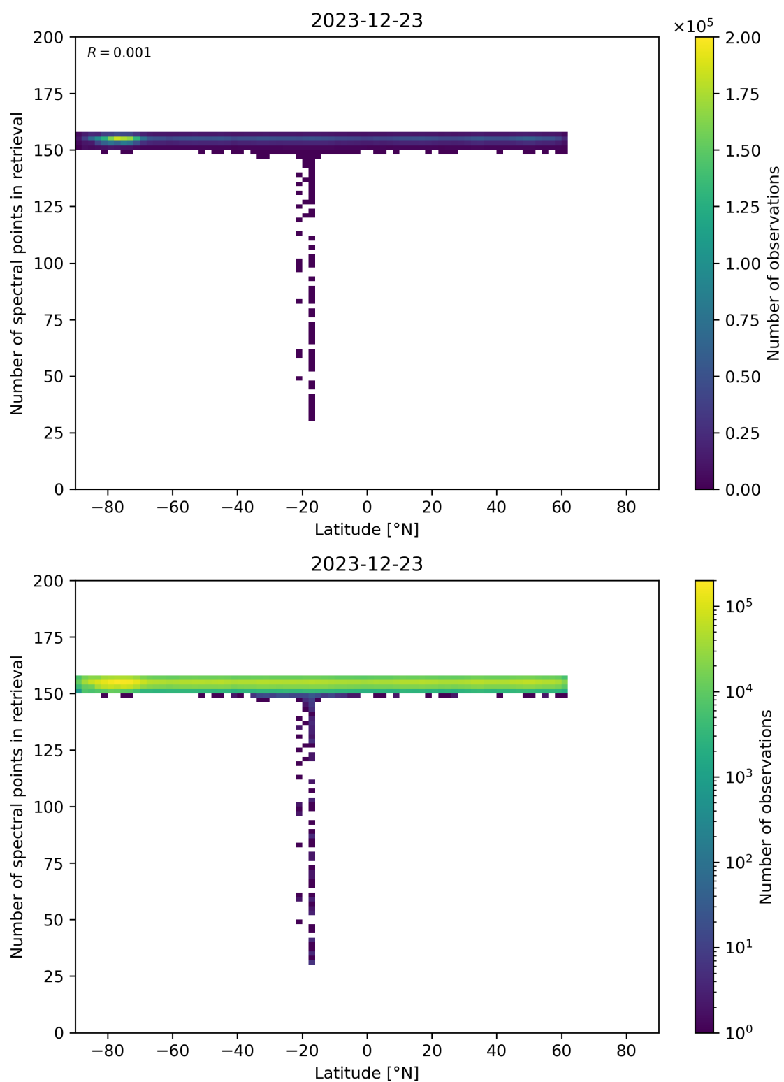
Figure 57: Scatter density plot of “Latitude” against “Number of spectral points in retrieval” for 2023-12-22 to 2023-12-24.
