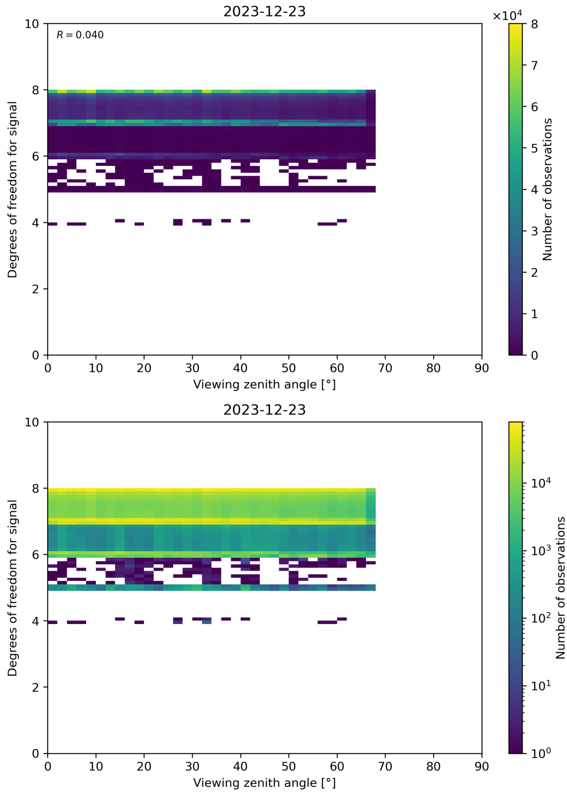
Figure 73: Scatter density plot of “Viewing zenith angle” against “Degrees of freedom for signal” for 2023-12-22 to 2023-12-24.
