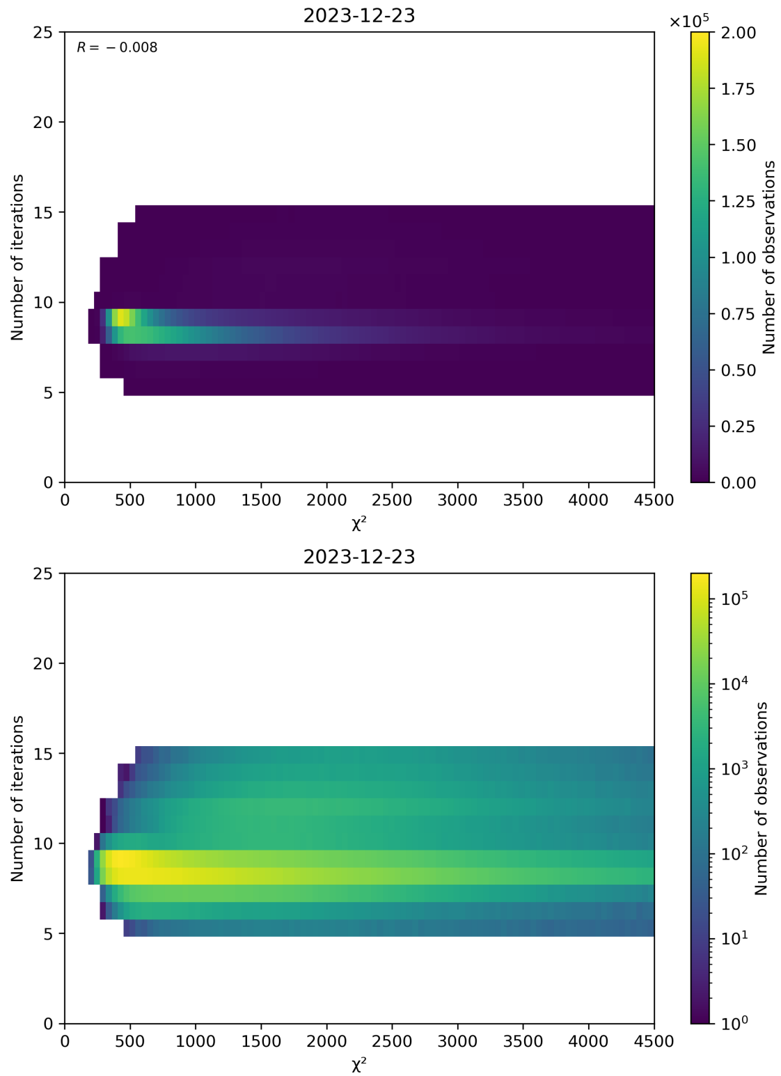
Figure 49: Scatter density plot of “ \chi^2 ” against “Number of iterations” for 2023-12-22 to 2023-12-24.
