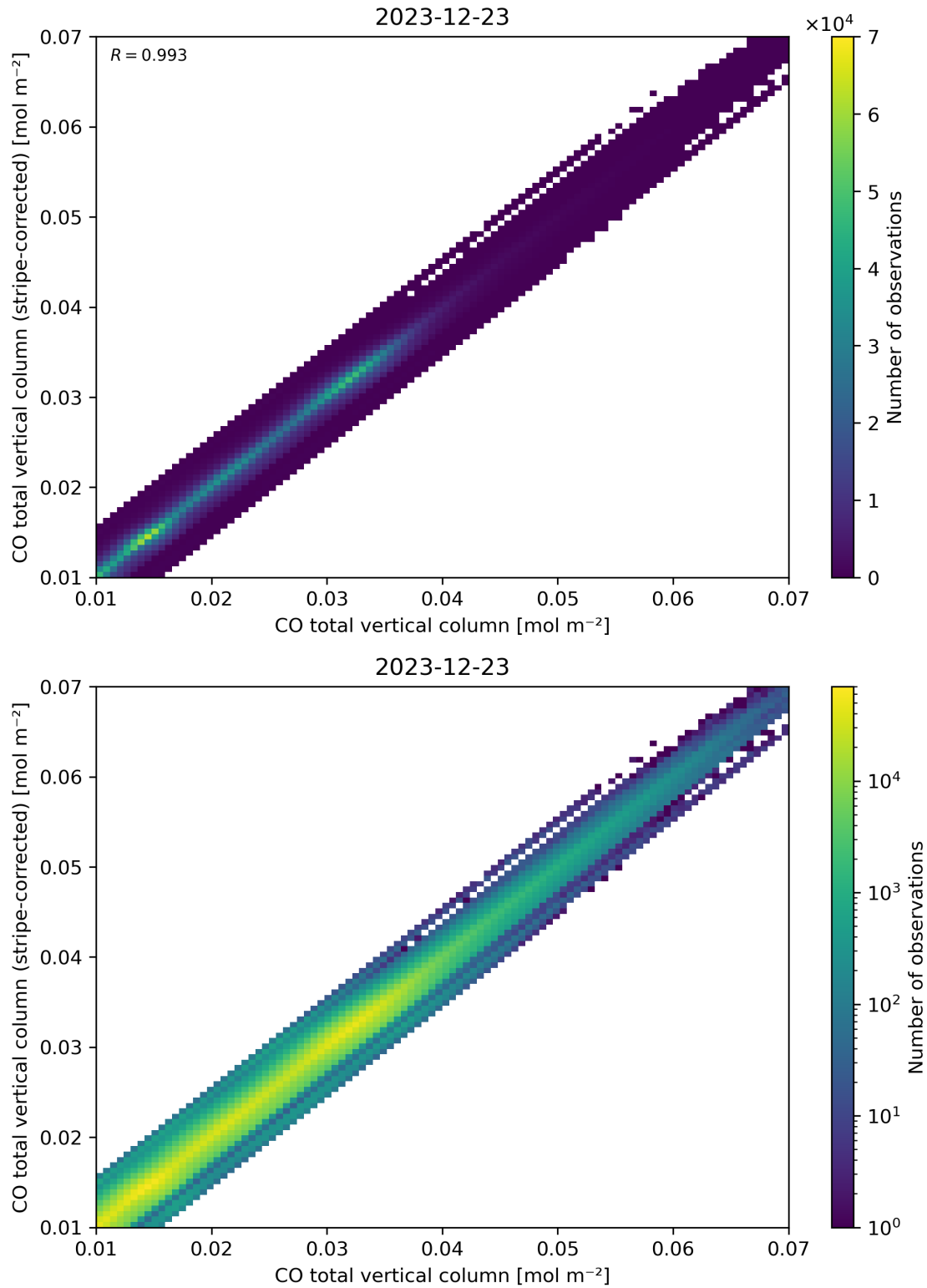
Figure 33: Scatter density plot of “CO total vertical column” against “CO total vertical column (stripe-corrected)” for 2023-12-22 to 2023-12-24.
