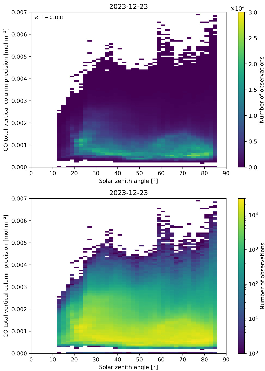
Figure 63: Scatter density plot of “Solar zenith angle” against “CO total vertical column precision” for 2023-12-22 to 2023-12-24.
