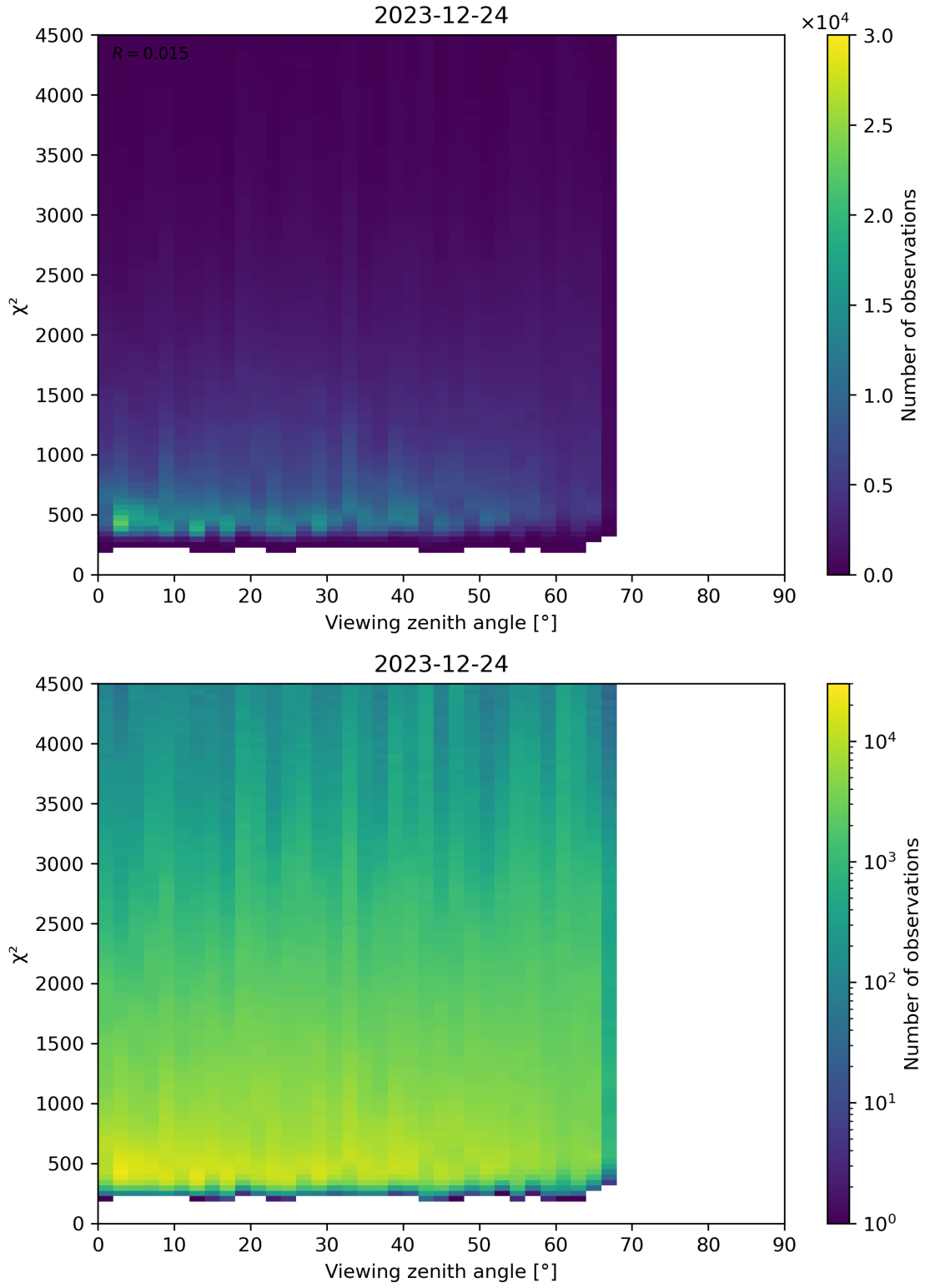
Figure 72: Scatter density plot of “Viewing zenith angle” against “ \chi^2 ” for 2023-12-23 to 2023-12-25.
