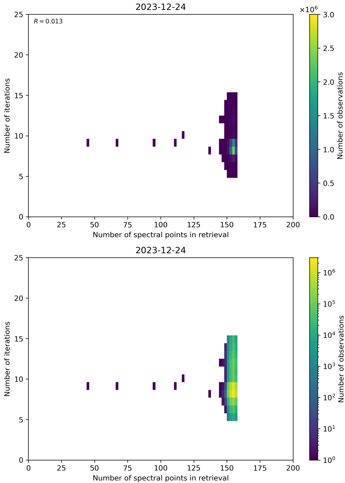
Figure 60: Scatter density plot of “Number of spectral points in retrieval” against “Number of iterations” for 2023-12-23 to 2023-12-25.
