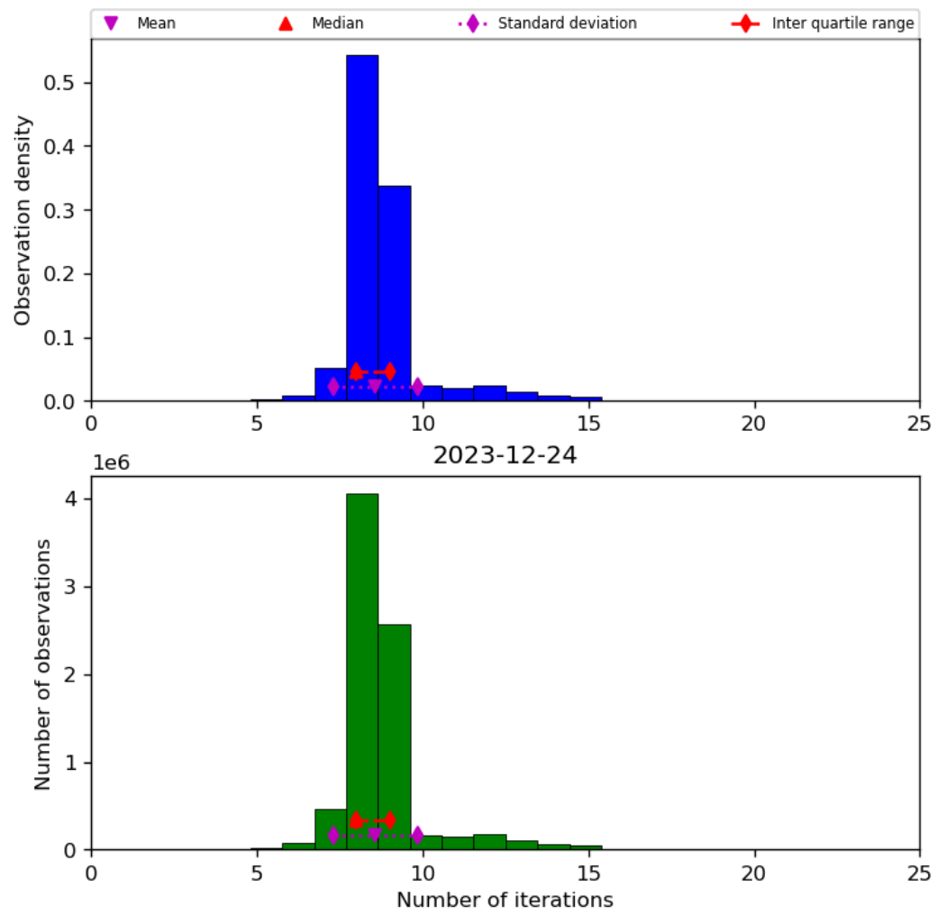
Figure 24: Histogram of “Number of iterations” for 2023-12-23 to 2023-12-25
