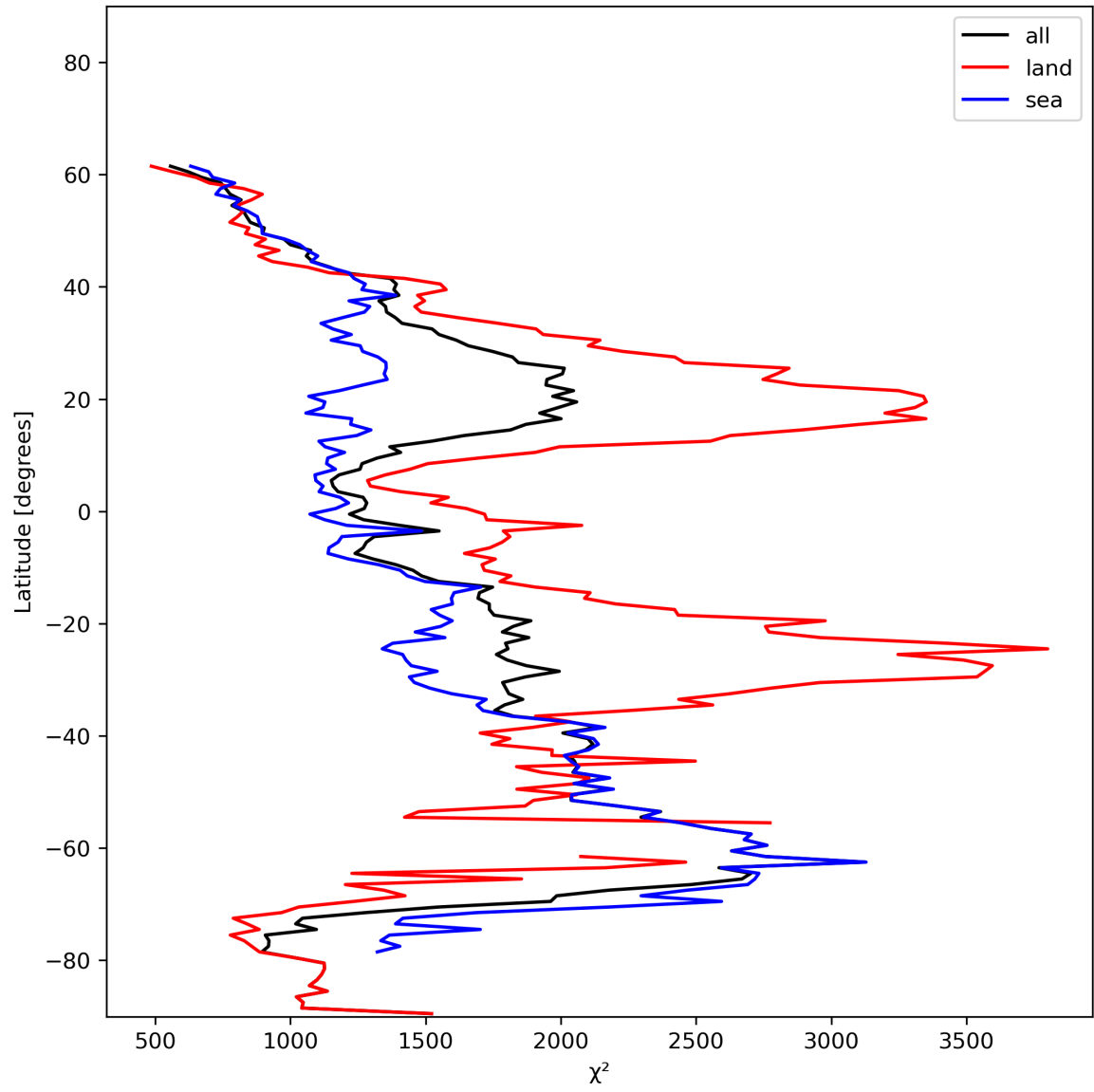
Figure 14: Zonal average of “ \chi^2 ” for 2023-12-23 to 2023-12-25.
