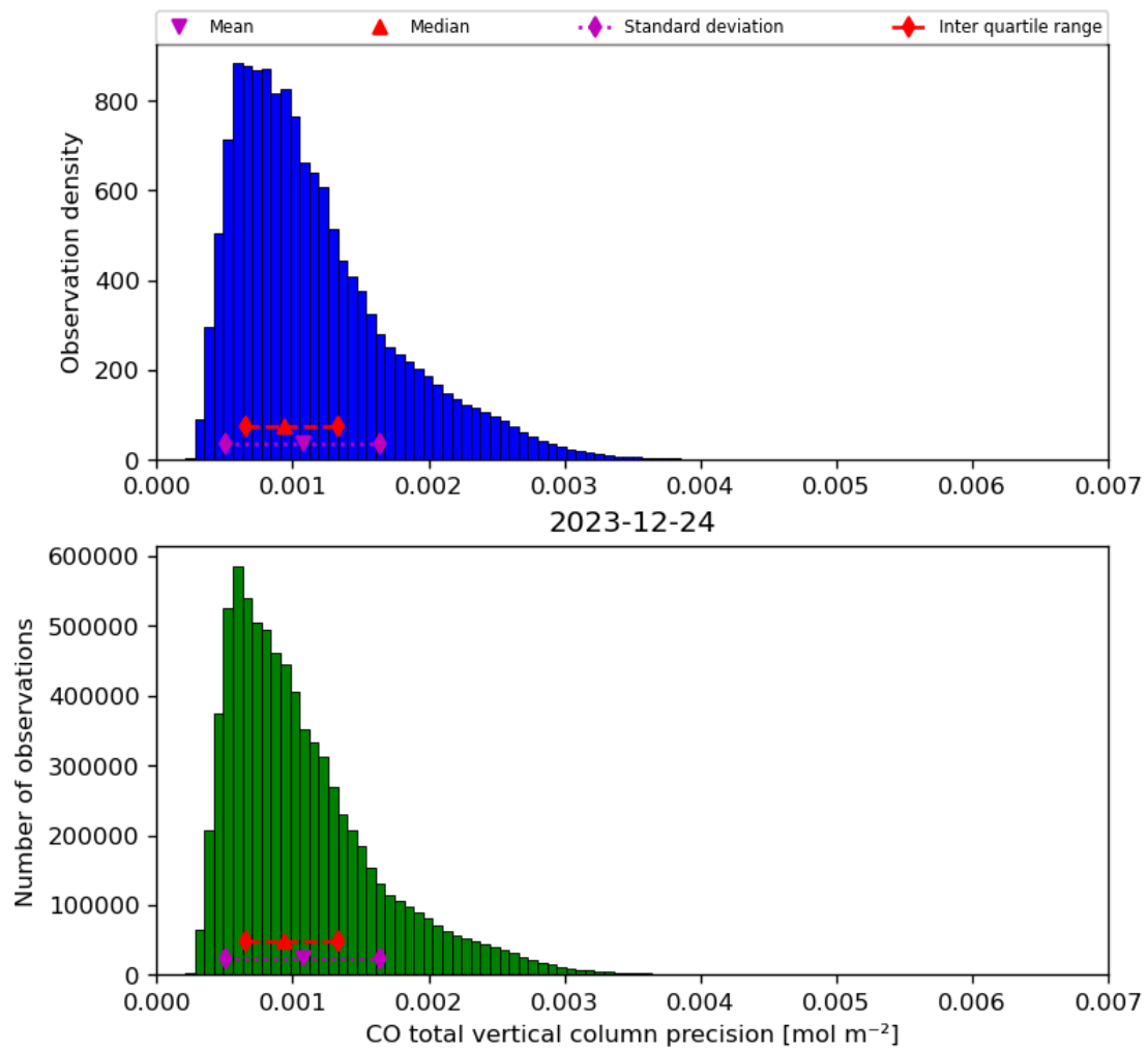
Figure 20: Histogram of “CO total vertical column precision” for 2023-12-23 to 2023-12-25
