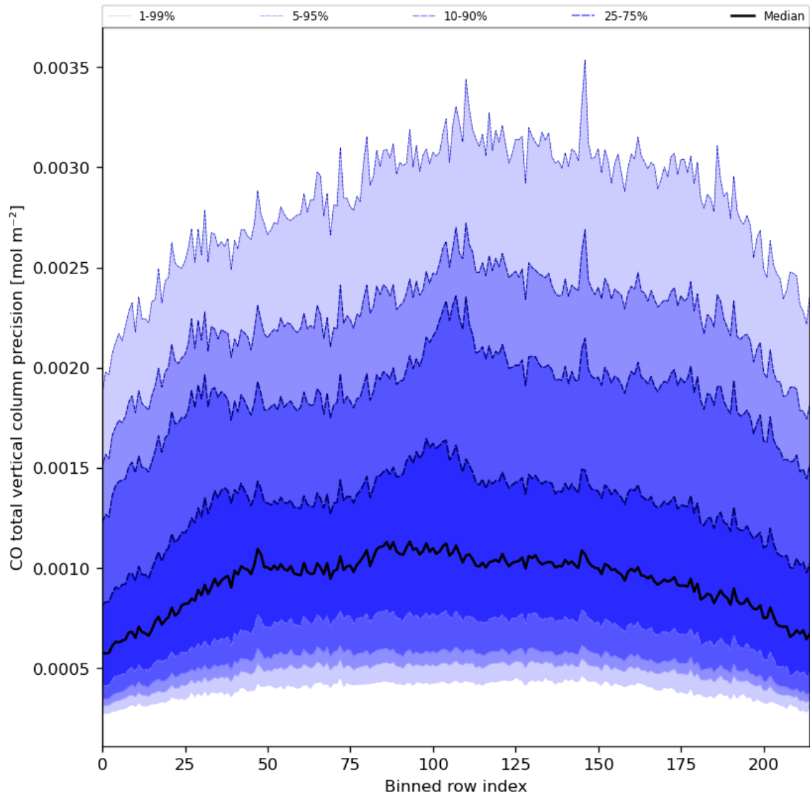
Figure 28: Along track statistics of “CO total vertical column precision” for 2023-12-23 to 2023-12-25
