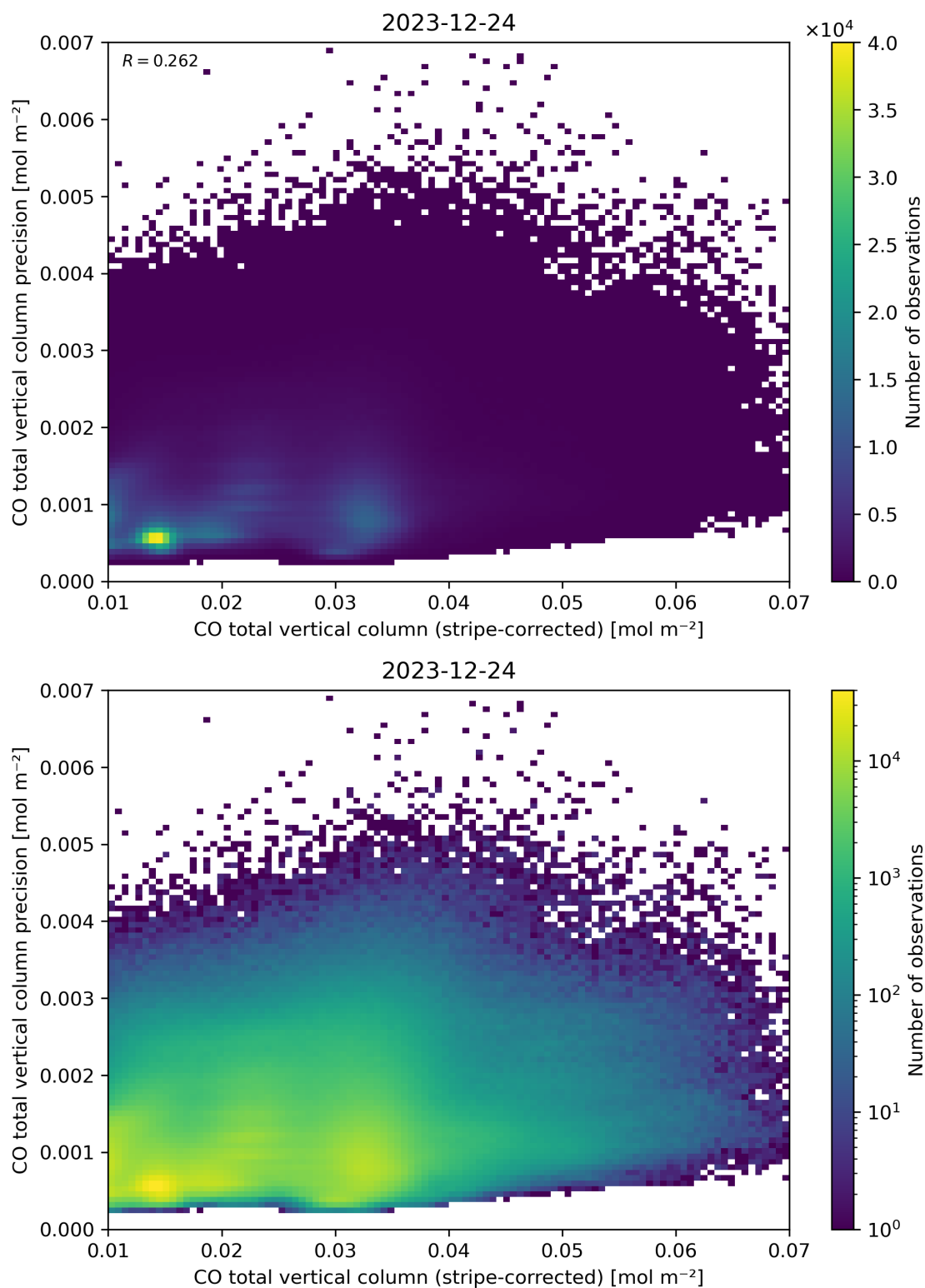
Figure 36: Scatter density plot of “CO total vertical column (stripe-corrected)” against “CO total vertical column precision” for 2023-12-23 to 2023-12-25.
