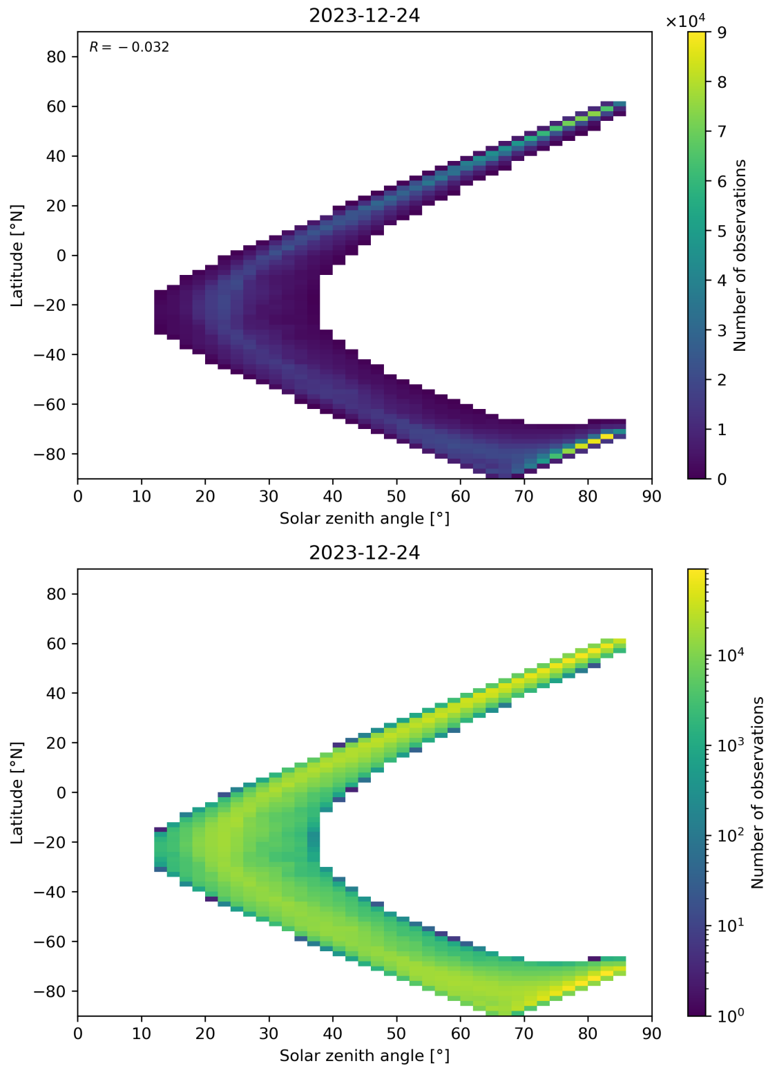
Figure 66: Scatter density plot of “Solar zenith angle” against “Latitude” for 2023-12-23 to 2023-12-25.
