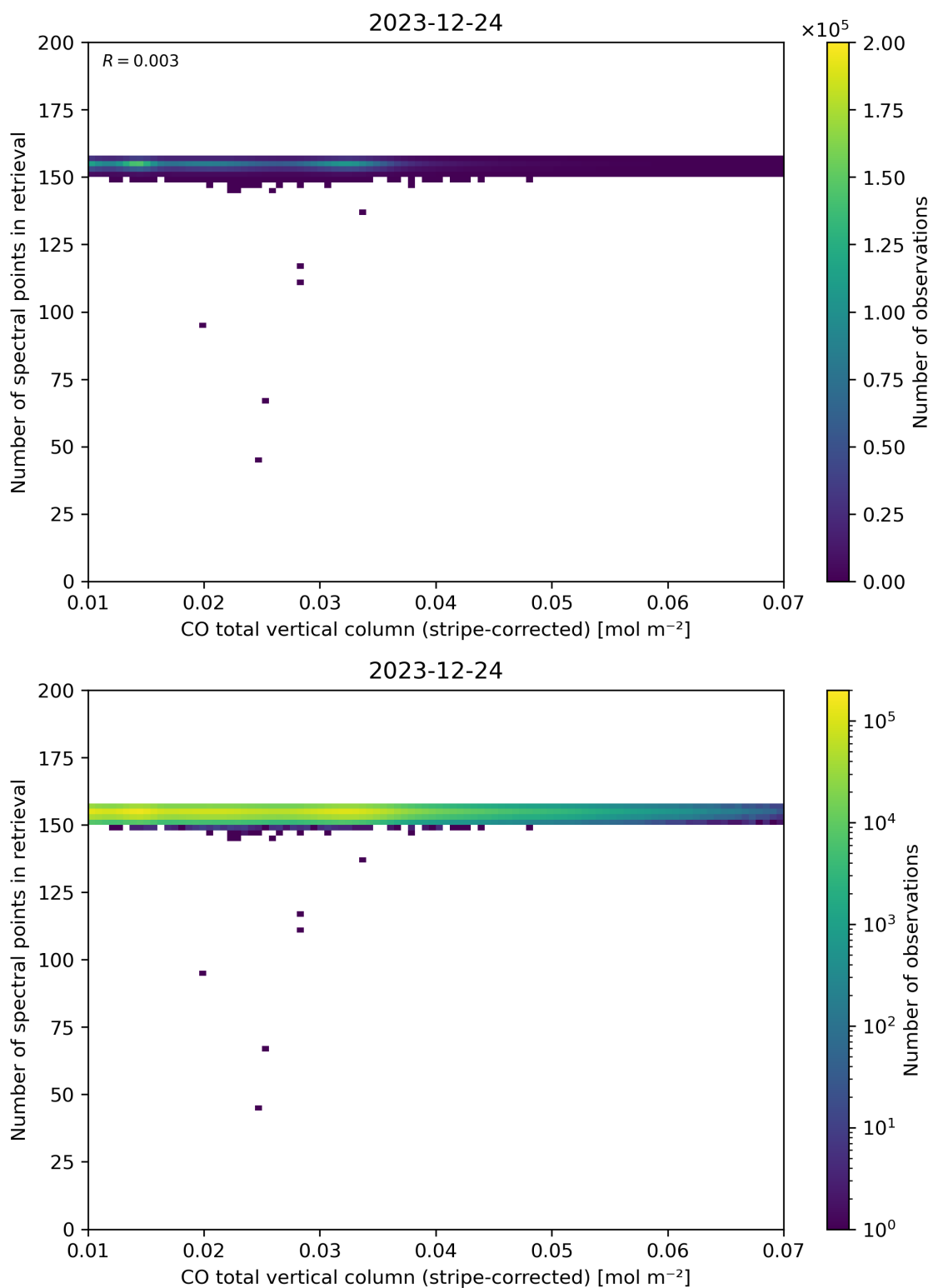
Figure 40: Scatter density plot of “CO total vertical column (stripe-corrected)” against “Number of spectral points in retrieval” for 2023-12-23 to 2023-12-25.
