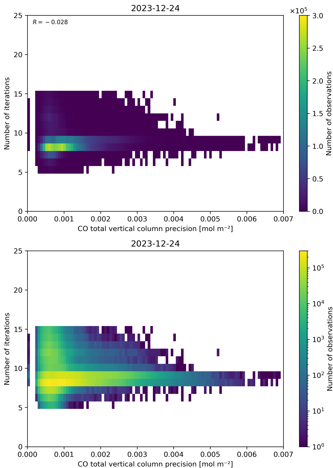
Figure 46: Scatter density plot of “CO total vertical column precision” against “Number of iterations” for 2023-12-23 to 2023-12-25.
