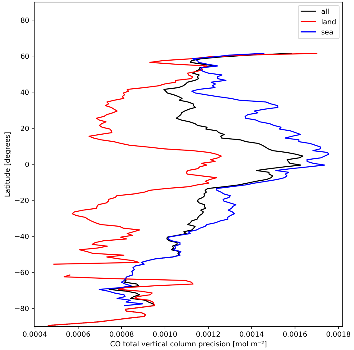
Figure 12: Zonal average of “CO total vertical column precision” for 2023-12-23 to 2023-12-25.
