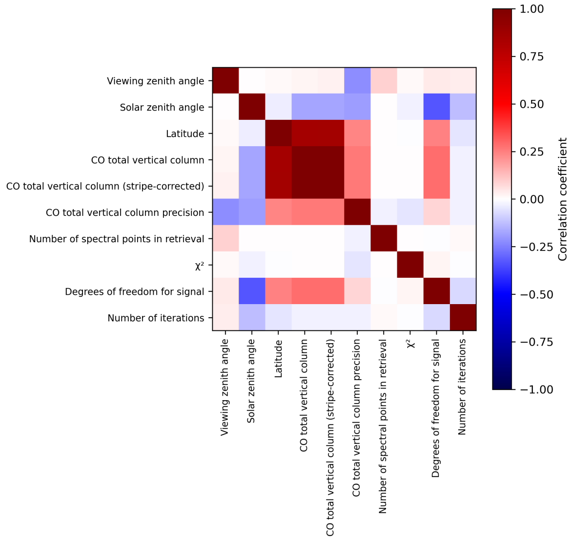
Figure 2: Map of correlation matrix for 2023-12-23 to 2023-12-25.
