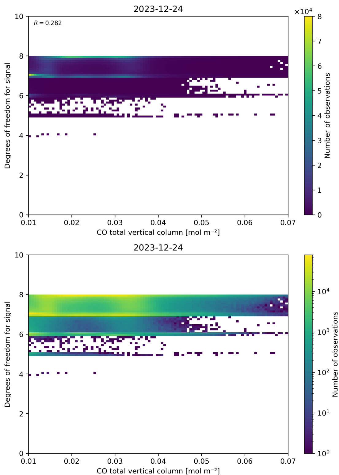
Figure 41: Scatter density plot of “CO total vertical column” against “Degrees of freedom for signal” for 2023-12-23 to 2023-12-25.
