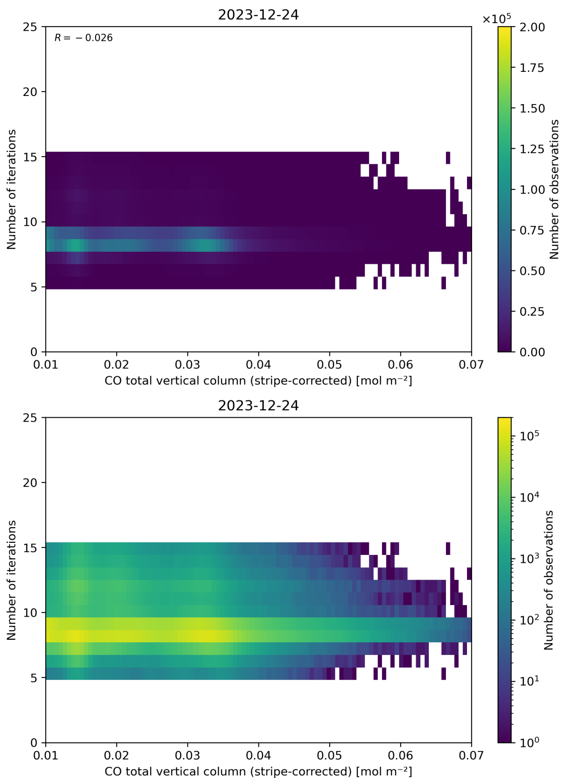
Figure 39: Scatter density plot of “CO total vertical column (stripe-corrected)” against “Number of iterations” for 2023-12-23 to 2023-12-25.
