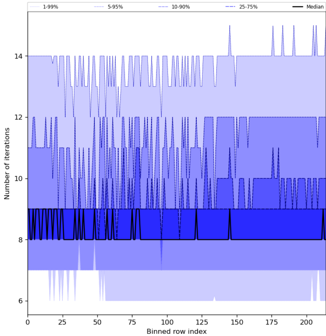
Figure 32: Along track statistics of “Number of iterations” for 2023-12-23 to 2023-12-25
