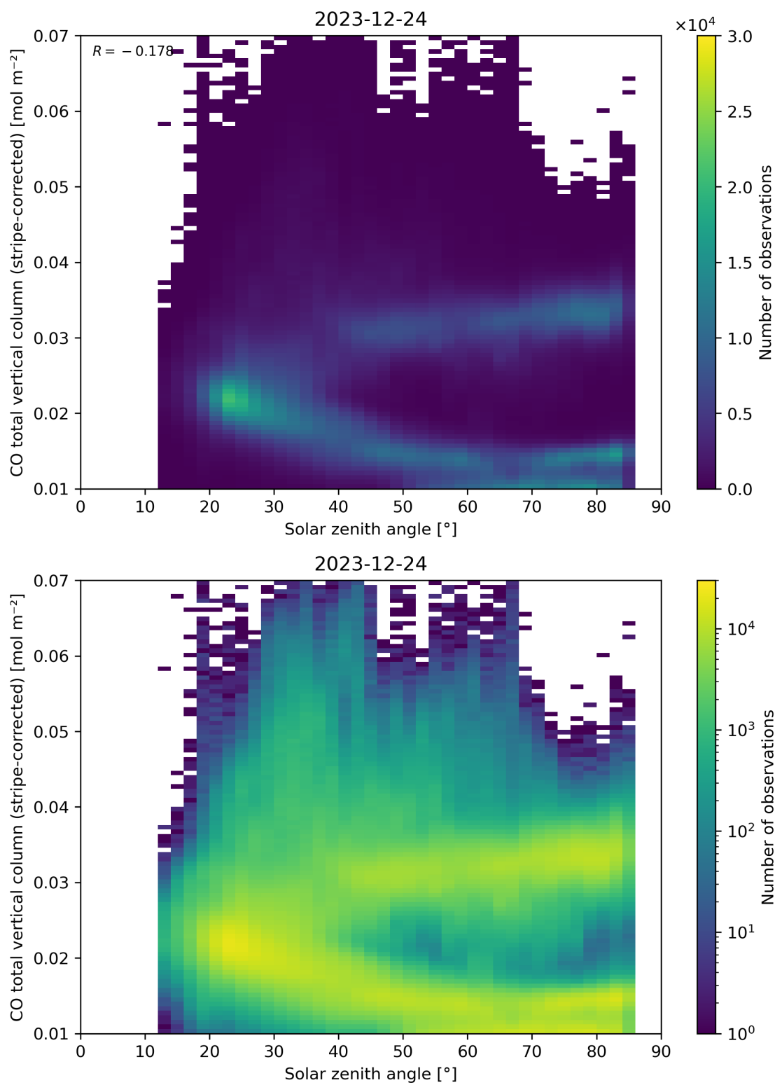
Figure 62: Scatter density plot of “Solar zenith angle” against “CO total vertical column (stripe-corrected)” for 2023-12-23 to 2023-12-25.
