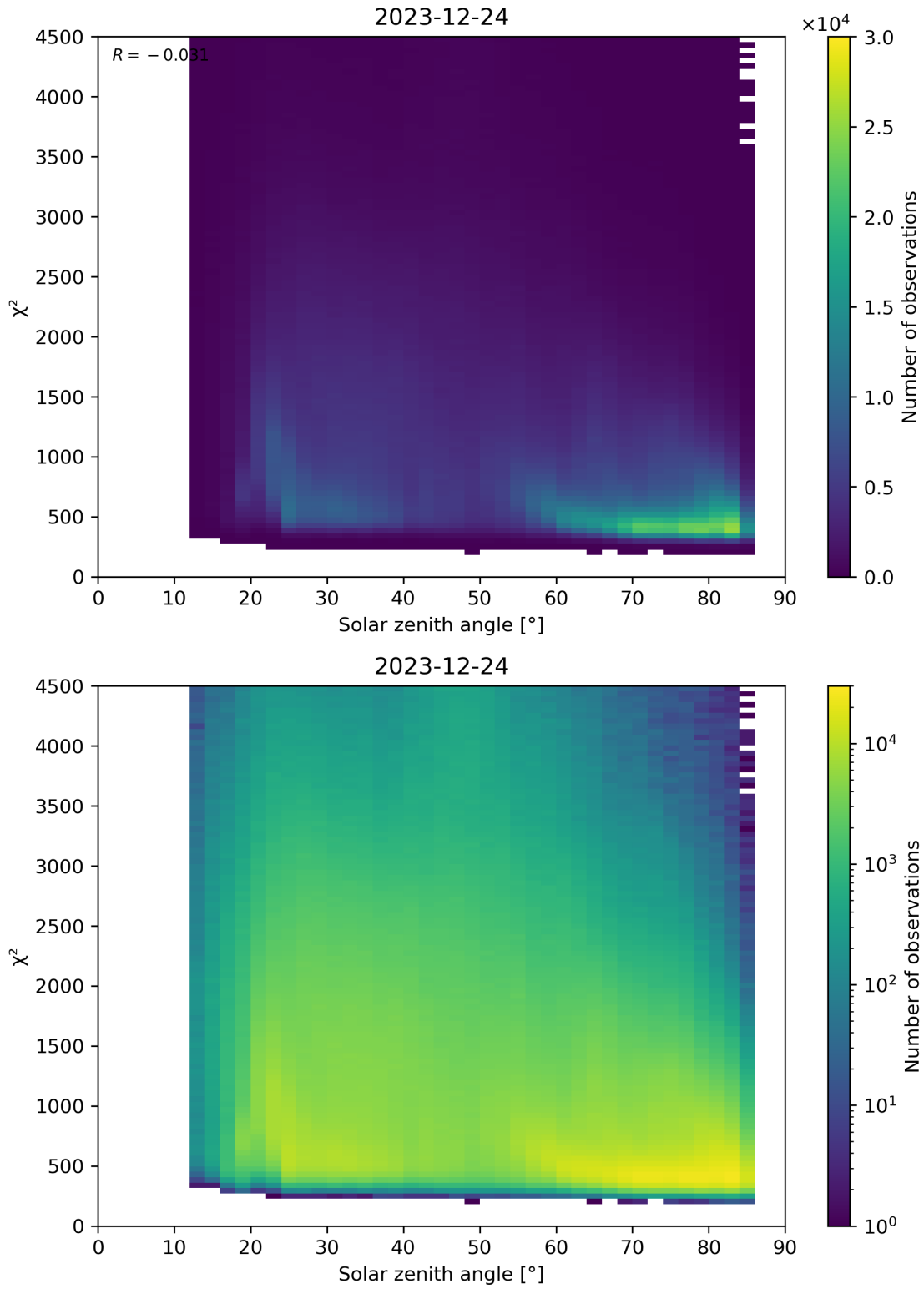
Figure 64: Scatter density plot of “Solar zenith angle” against “ \chi^2 ” for 2023-12-23 to 2023-12-25.
