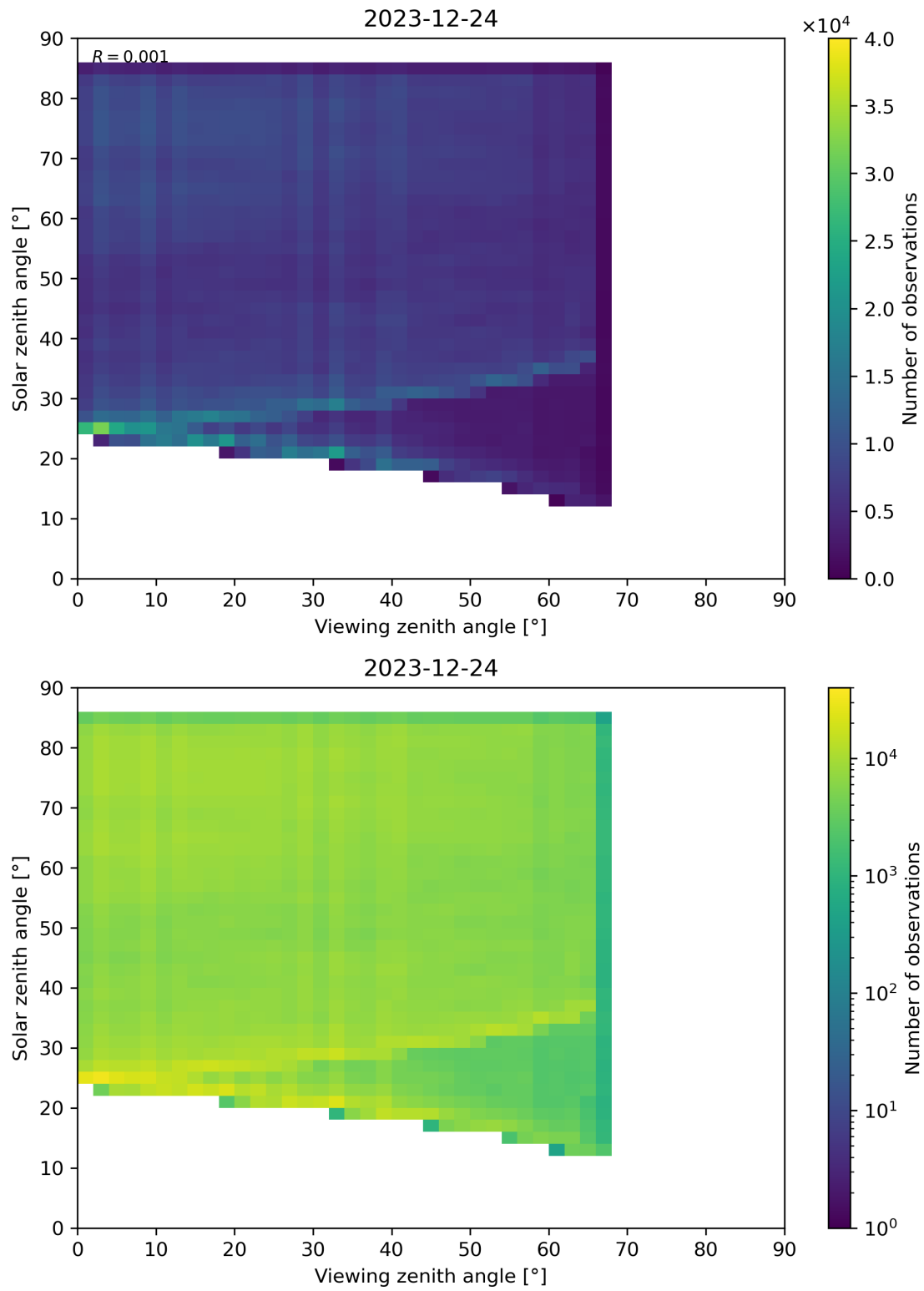
Figure 77: Scatter density plot of “Viewing zenith angle” against “Solar zenith angle” for 2023-12-23 to 2023-12-25.
