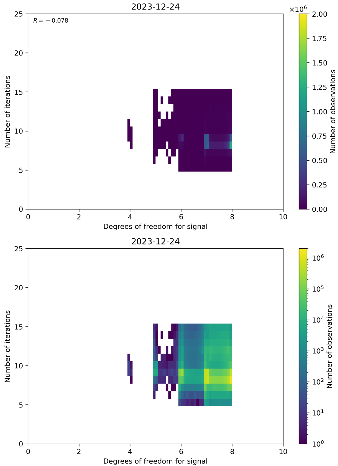
Figure 50: Scatter density plot of “Degrees of freedom for signal” against “Number of iterations” for 2023-12-23 to 2023-12-25.
