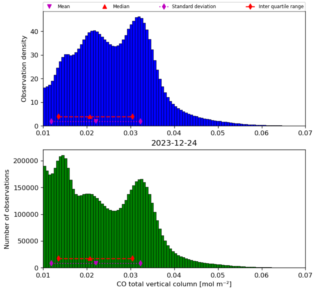
Figure 18: Histogram of “CO total vertical column” for 2023-12-23 to 2023-12-25
