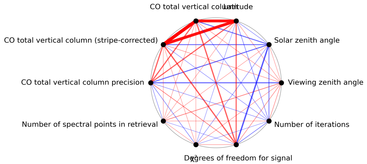
Figure 1: Map of correlation graph for 2023-12-23 to 2023-12-25.
