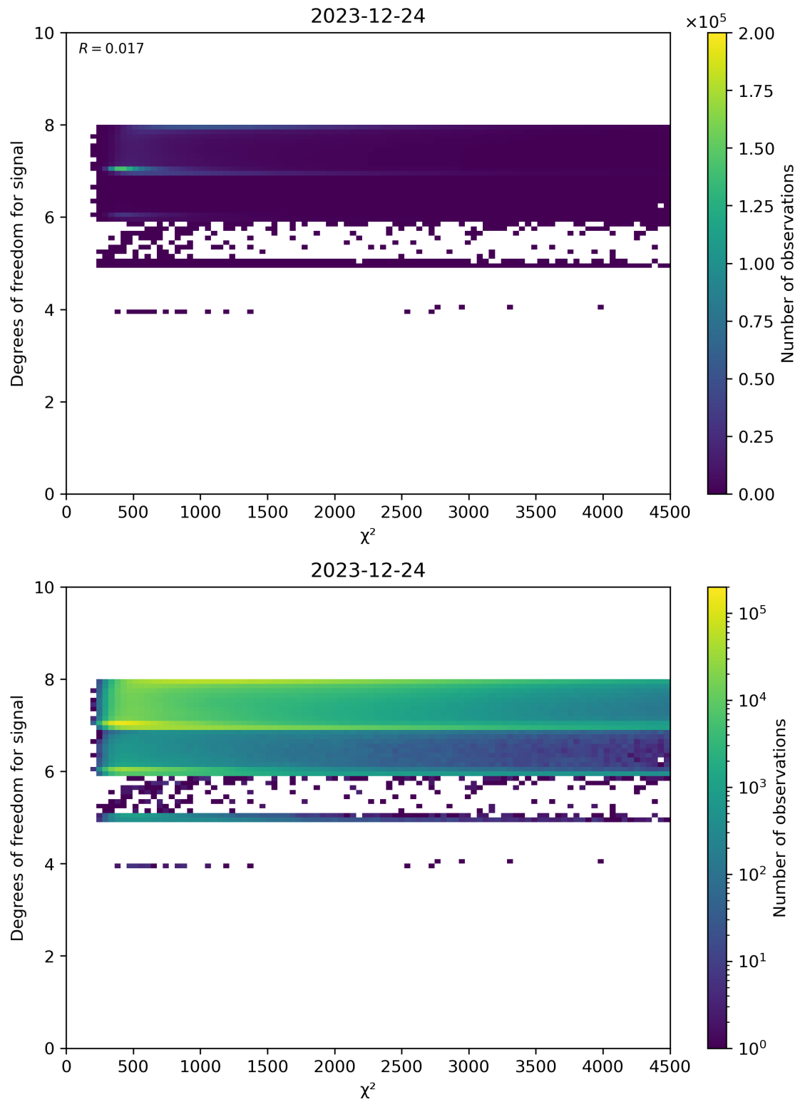
Figure 48: Scatter density plot of “ \chi^2 ” against “Degrees of freedom for signal” for 2023-12-23 to 2023-12-25.
