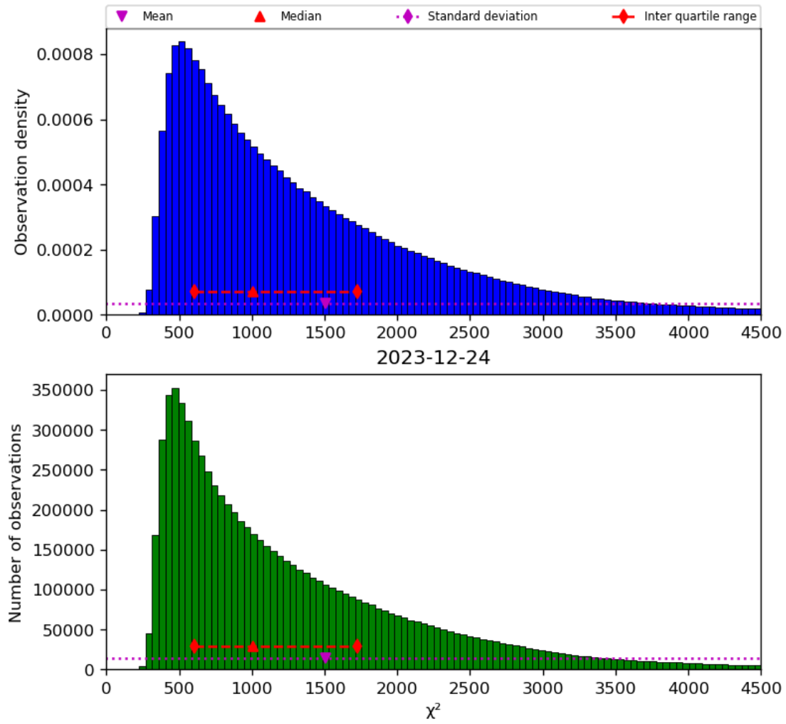
Figure 22: Histogram of “ \chi^2 ” for 2023-12-23 to 2023-12-25
