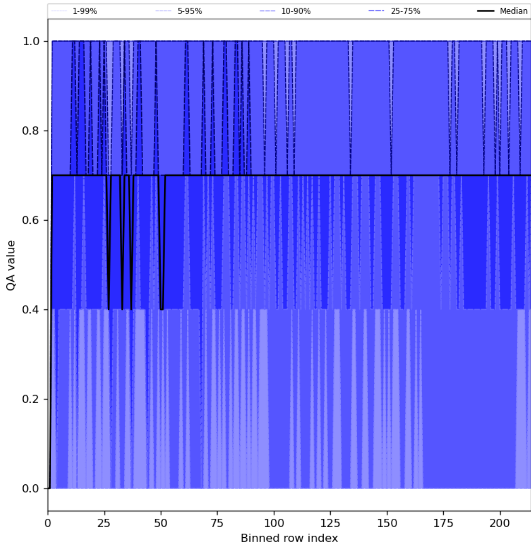
Figure 25: Along track statistics of “QA value” for 2023-12-23 to 2023-12-25
