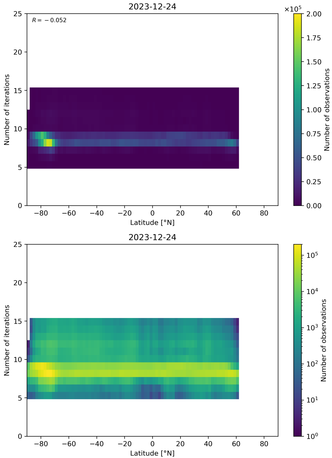
Figure 56: Scatter density plot of “Latitude” against “Number of iterations” for 2023-12-23 to 2023-12-25.
