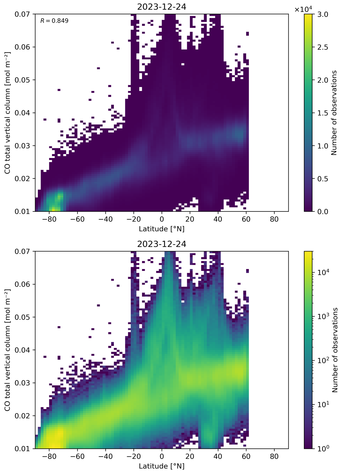
Figure 51: Scatter density plot of “Latitude” against “CO total vertical column” for 2023-12-23 to 2023-12-25.
