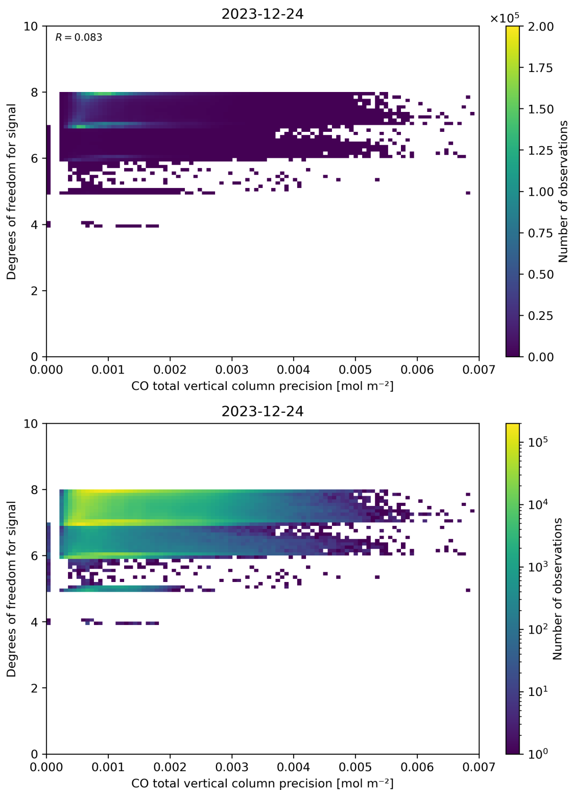
Figure 45: Scatter density plot of “CO total vertical column precision” against “Degrees of freedom for signal” for 2023-12-23 to 2023-12-25.
