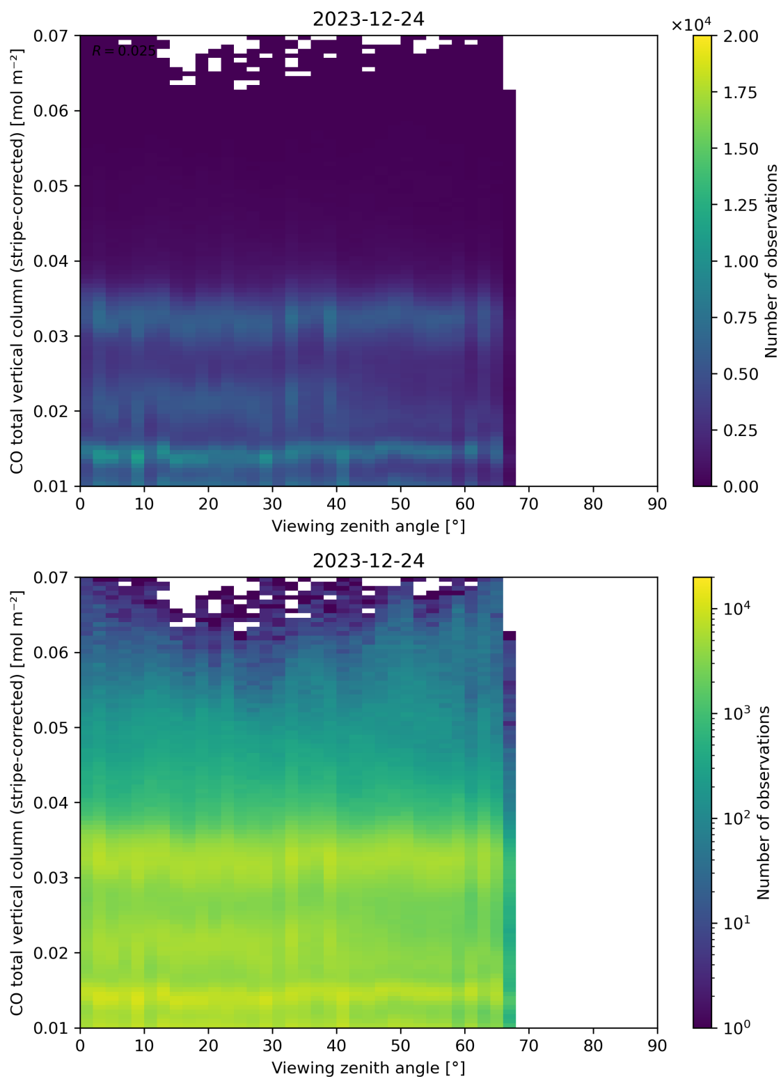
Figure 70: Scatter density plot of “Viewing zenith angle” against “CO total vertical column (stripe-corrected)” for 2023-12-23 to 2023-12-25.
