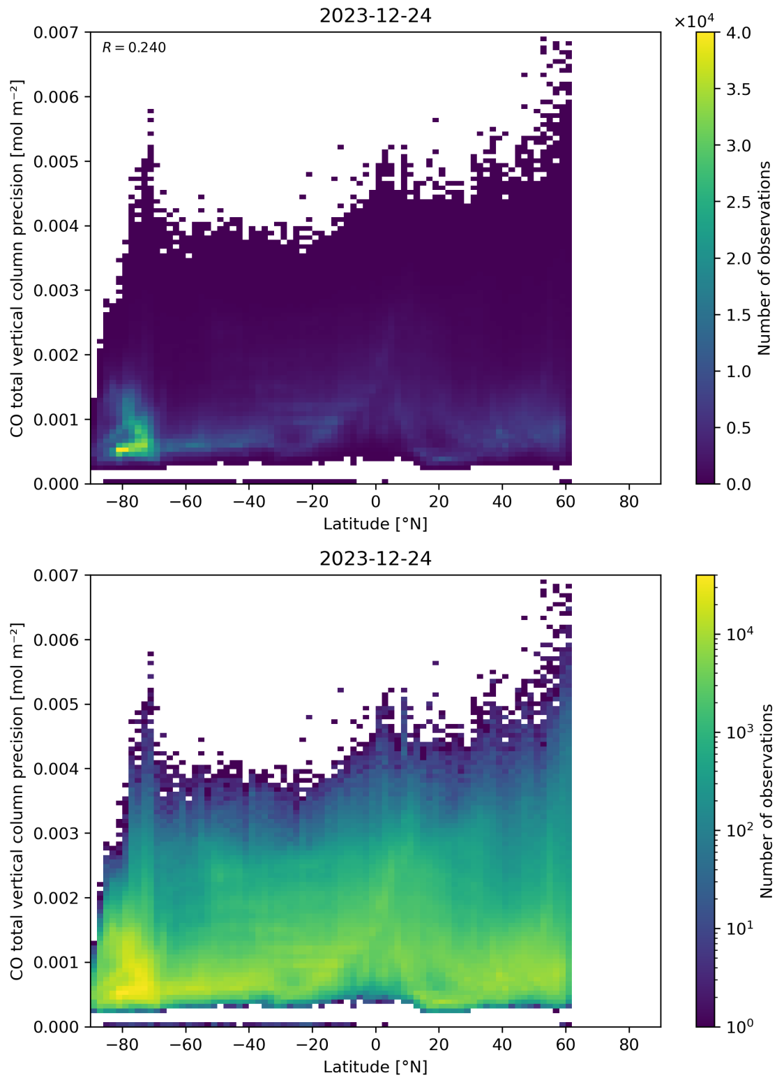
Figure 53: Scatter density plot of “Latitude” against “CO total vertical column precision” for 2023-12-23 to 2023-12-25.
