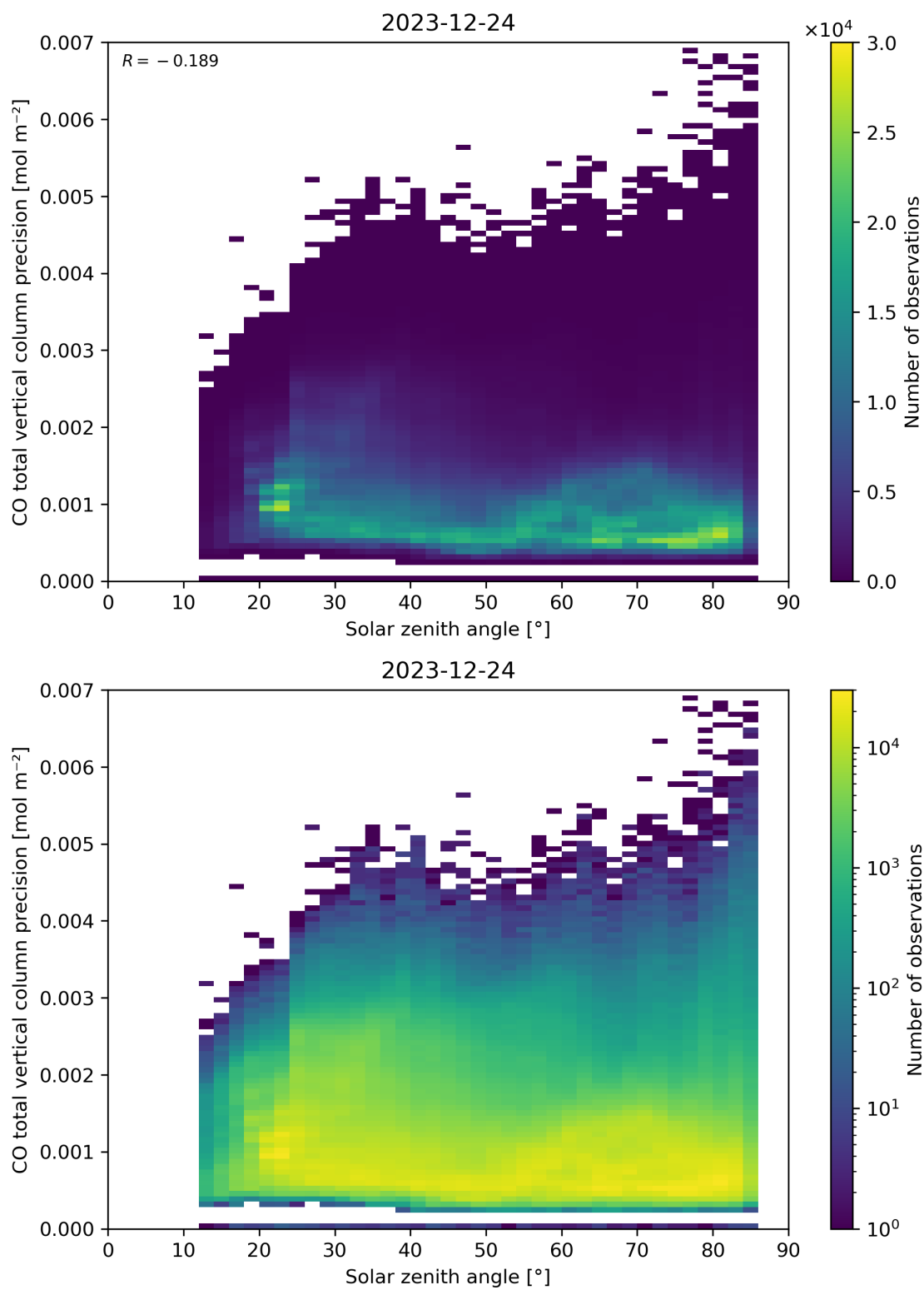
Figure 63: Scatter density plot of “Solar zenith angle” against “CO total vertical column precision” for 2023-12-23 to 2023-12-25.
