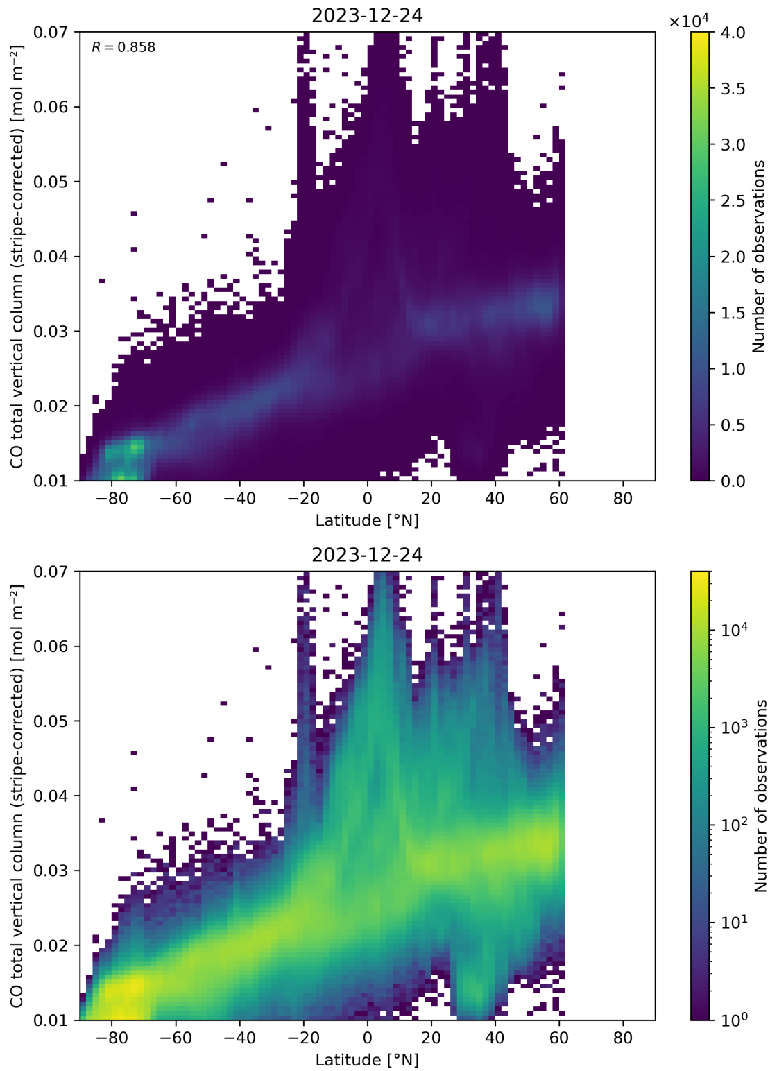
Figure 52: Scatter density plot of “Latitude” against “CO total vertical column (stripe-corrected)” for 2023-12-23 to 2023-12-25.
