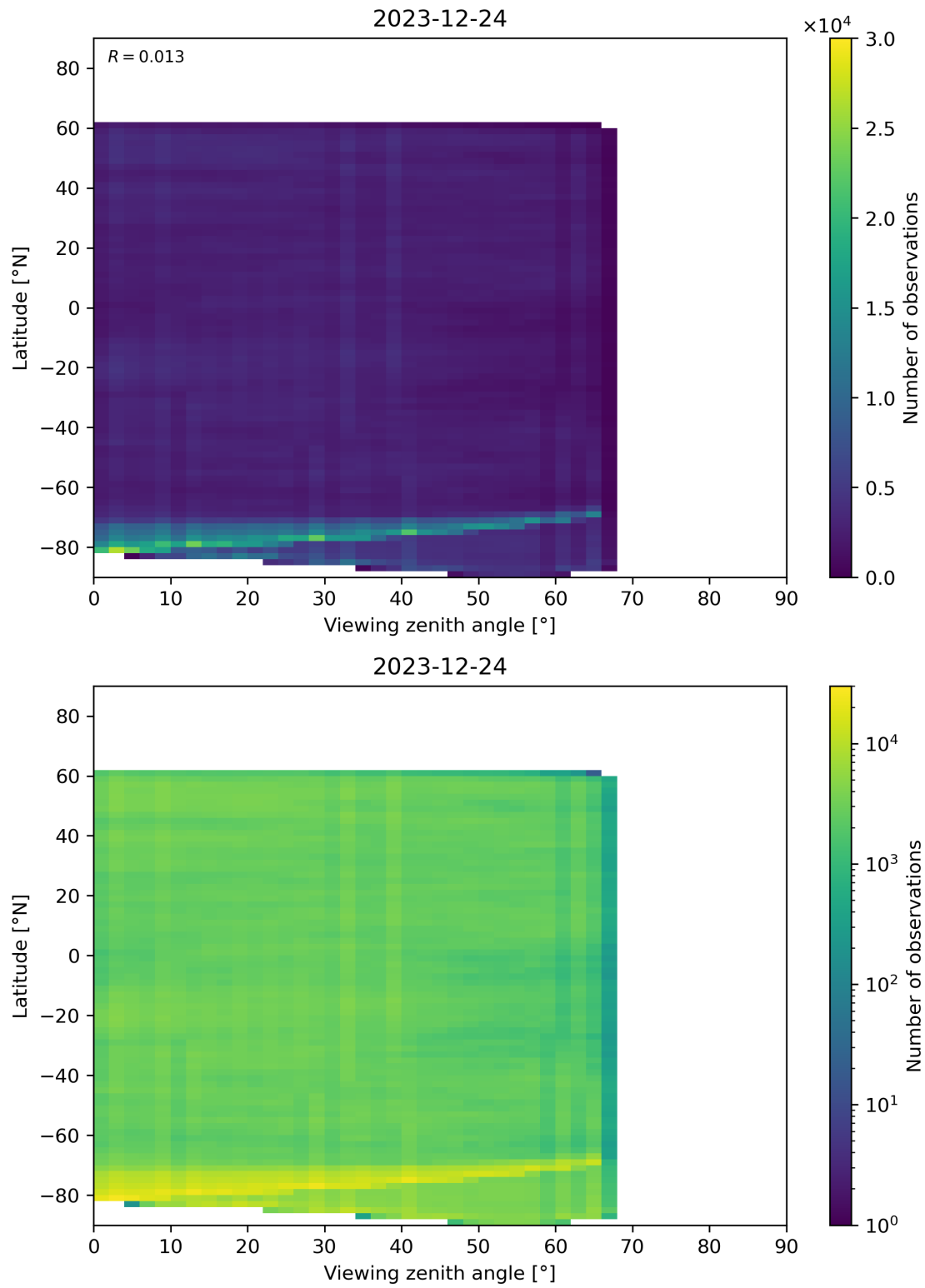
Figure 74: Scatter density plot of “Viewing zenith angle” against “Latitude” for 2023-12-23 to 2023-12-25.
