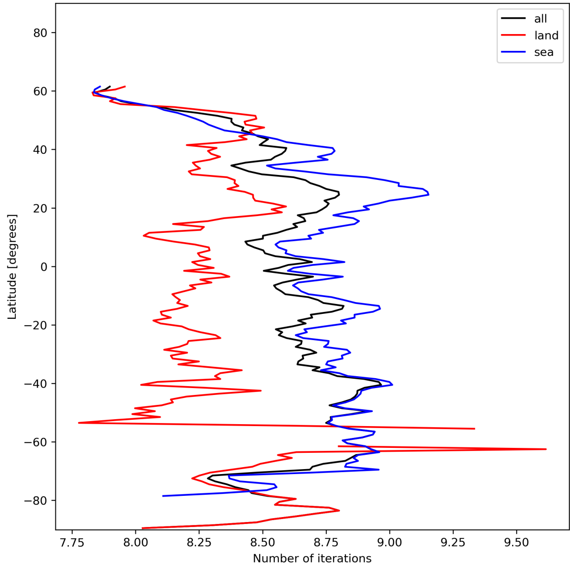
Figure 16: Zonal average of “Number of iterations” for 2023-12-23 to 2023-12-25.
