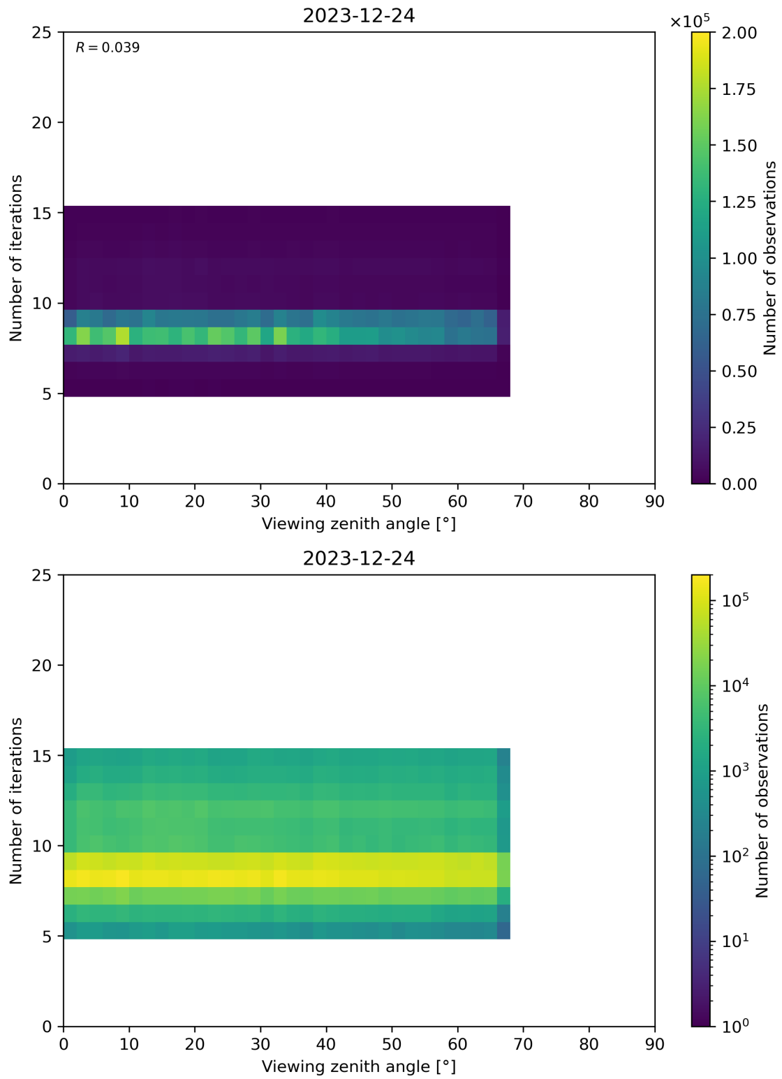
Figure 75: Scatter density plot of “Viewing zenith angle” against “Number of iterations” for 2023-12-23 to 2023-12-25.
