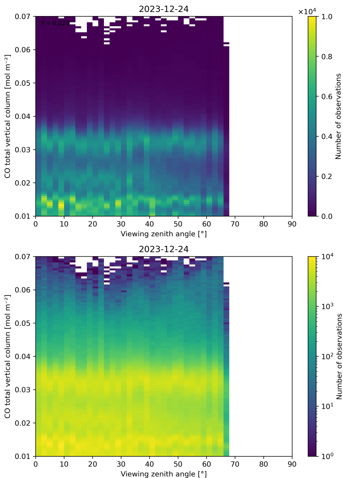
Figure 69: Scatter density plot of “Viewing zenith angle” against “CO total vertical column” for 2023-12-23 to 2023-12-25.
