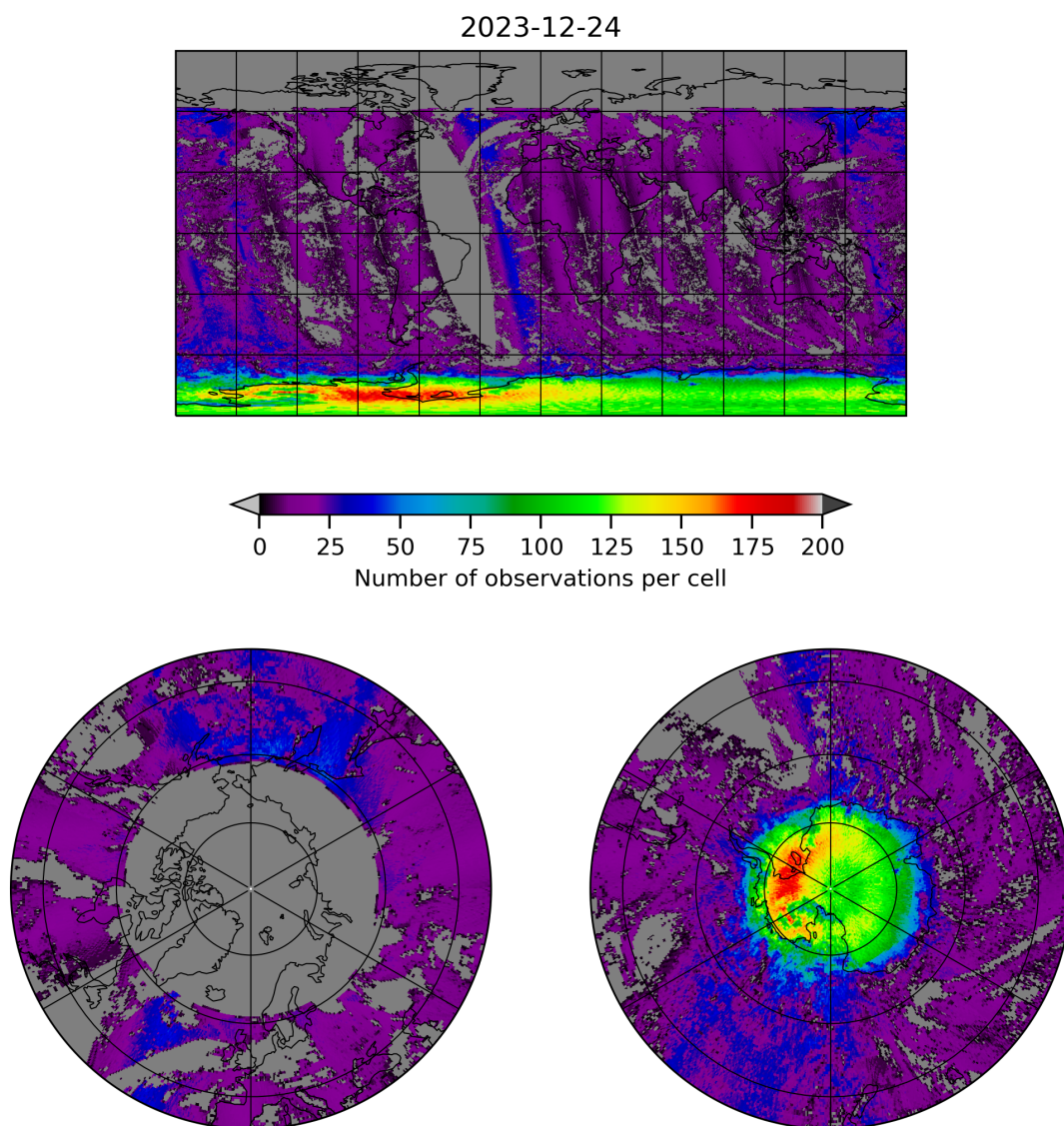
Figure 8: Map of the number of observations for 2023-12-23 to 2023-12-25
