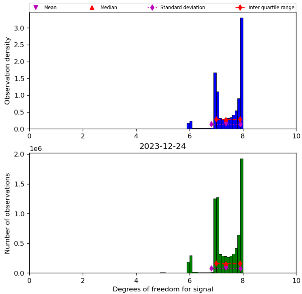
Figure 23: Histogram of “Degrees of freedom for signal” for 2023-12-23 to 2023-12-25
