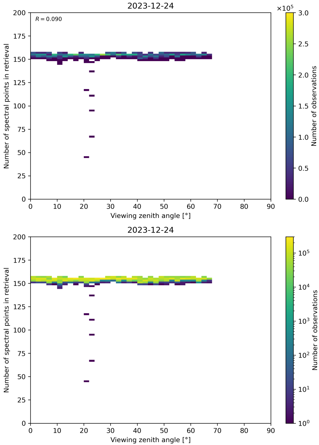
Figure 76: Scatter density plot of “Viewing zenith angle” against “Number of spectral points in retrieval” for 2023-12-23 to 2023-12-25.
