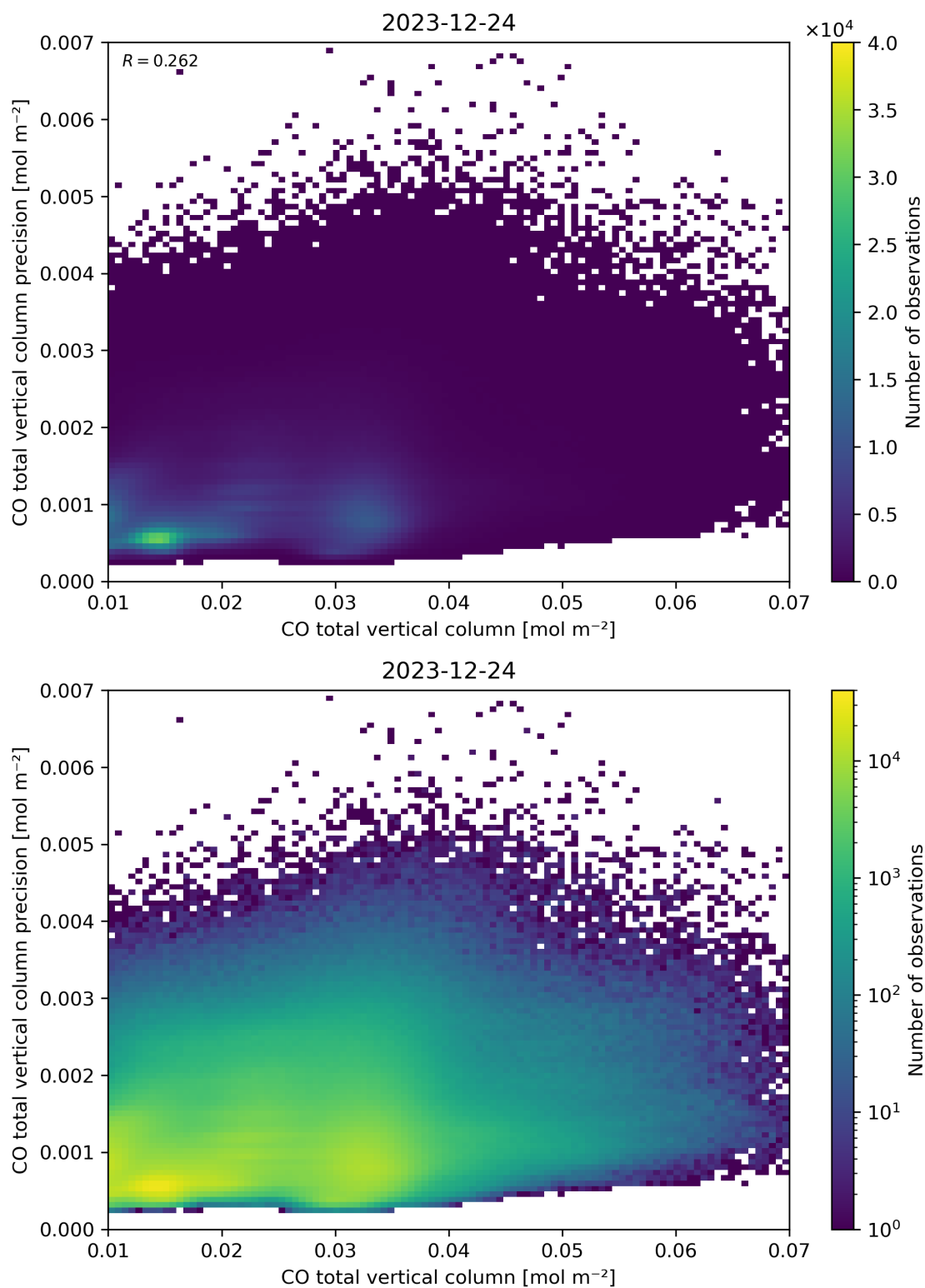
Figure 34: Scatter density plot of “CO total vertical column” against “CO total vertical column precision” for 2023-12-23 to 2023-12-25.
