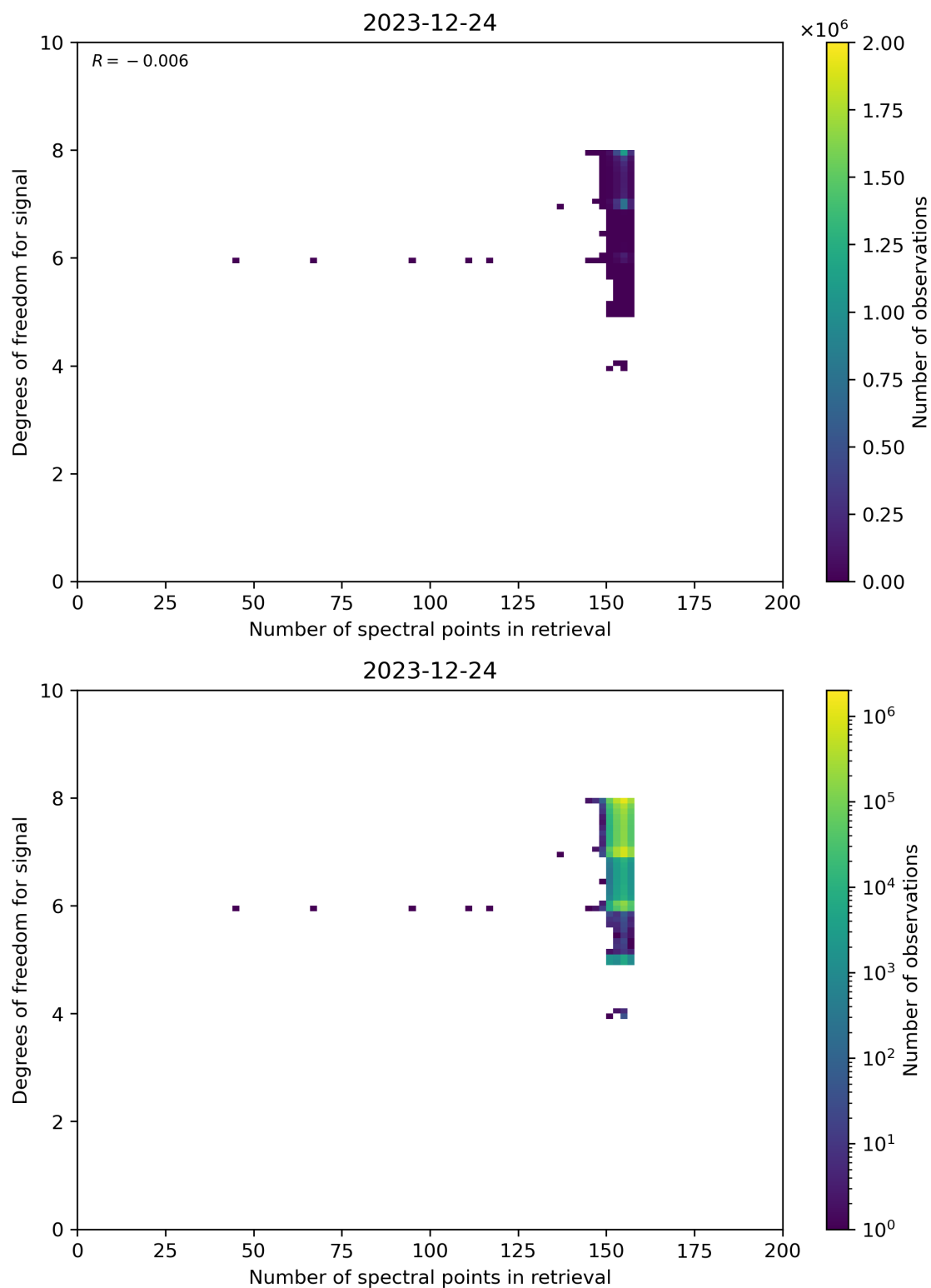
Figure 59: Scatter density plot of “Number of spectral points in retrieval” against “Degrees of freedom for signal” for 2023-12-23 to 2023-12-25.
