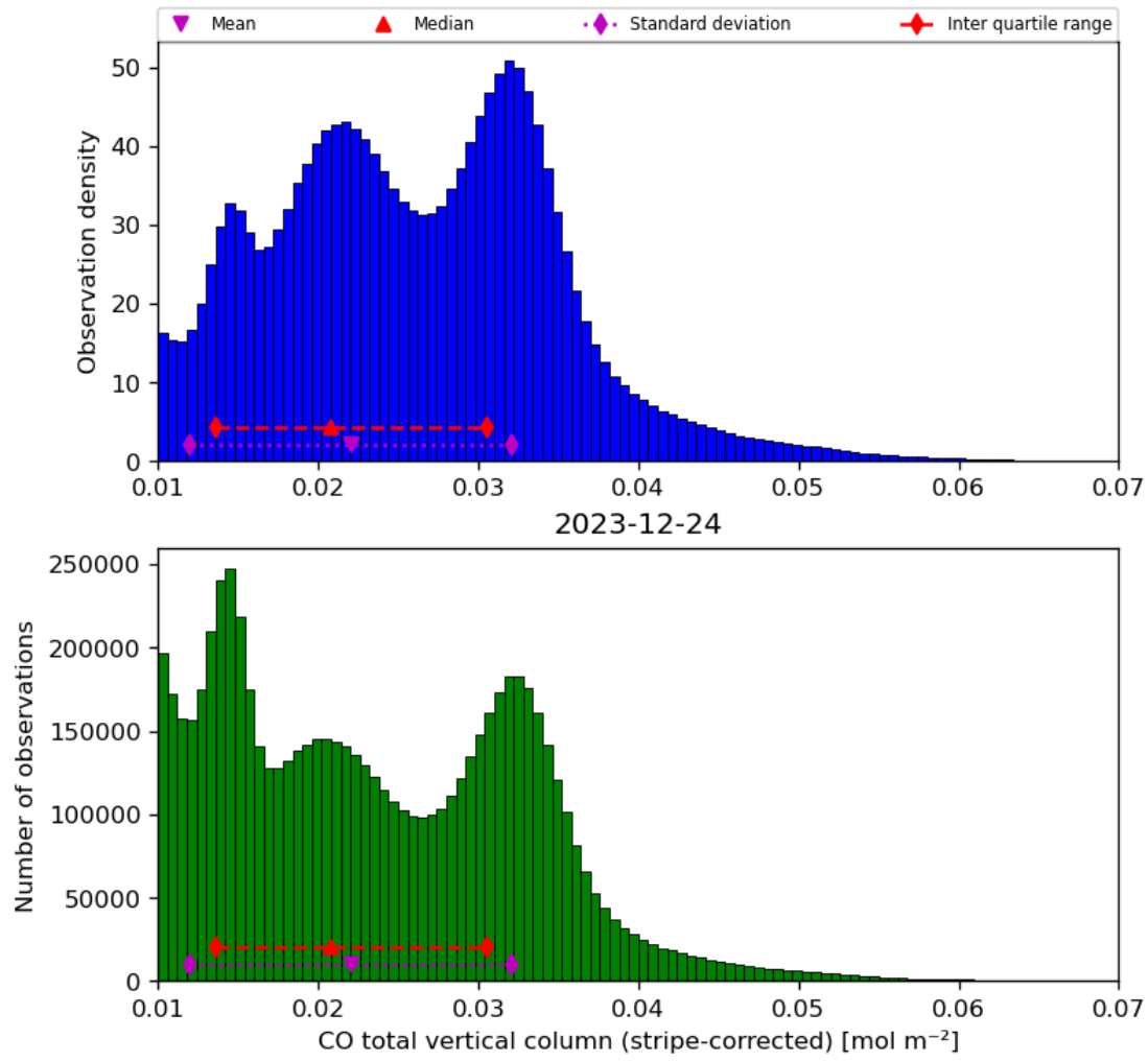
Figure 19: Histogram of “CO total vertical column (stripe-corrected)” for 2023-12-23 to 2023-12-25
