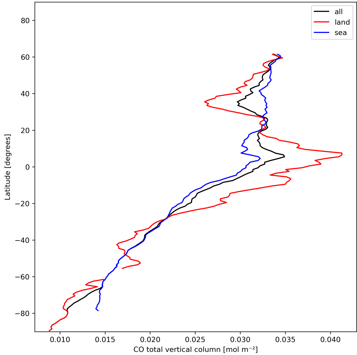
Figure 10: Zonal average of “CO total vertical column” for 2023-12-23 to 2023-12-25.
