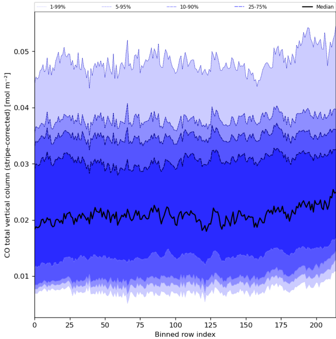
Figure 27: Along track statistics of “CO total vertical column (stripe-corrected)” for 2023-12-23 to 2023-12-25
