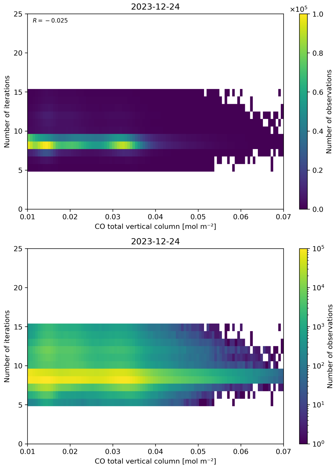
Figure 42: Scatter density plot of “CO total vertical column” against “Number of iterations” for 2023-12-23 to 2023-12-25.
