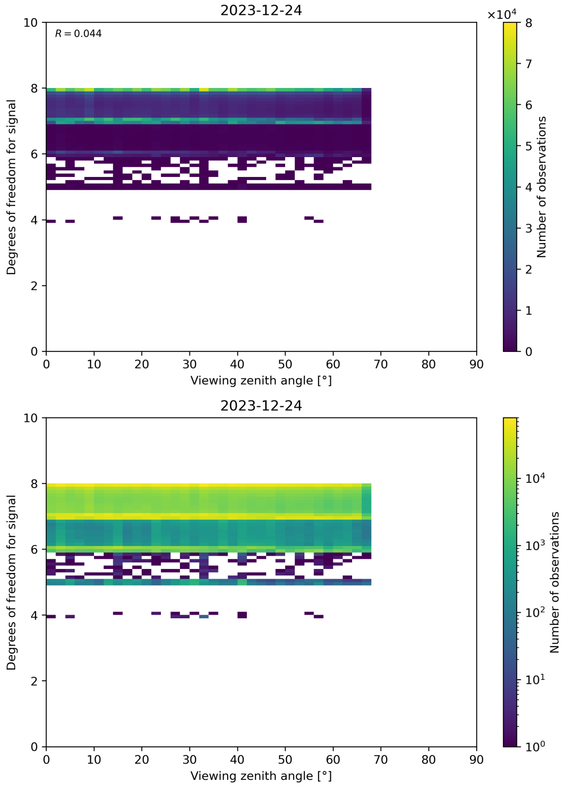
Figure 73: Scatter density plot of “Viewing zenith angle” against “Degrees of freedom for signal” for 2023-12-23 to 2023-12-25.
