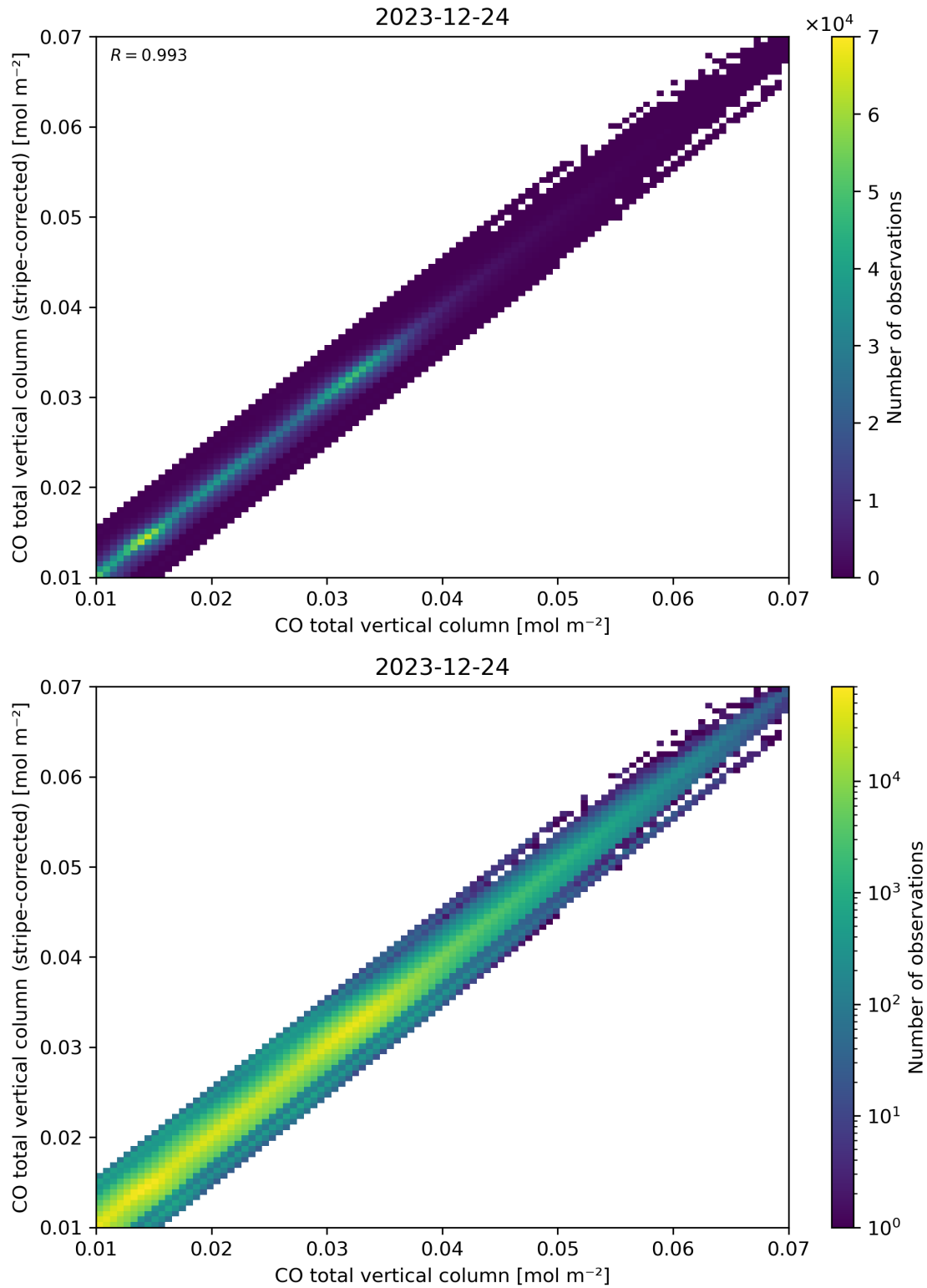
Figure 33: Scatter density plot of “CO total vertical column” against “CO total vertical column (stripe-corrected)” for 2023-12-23 to 2023-12-25.
