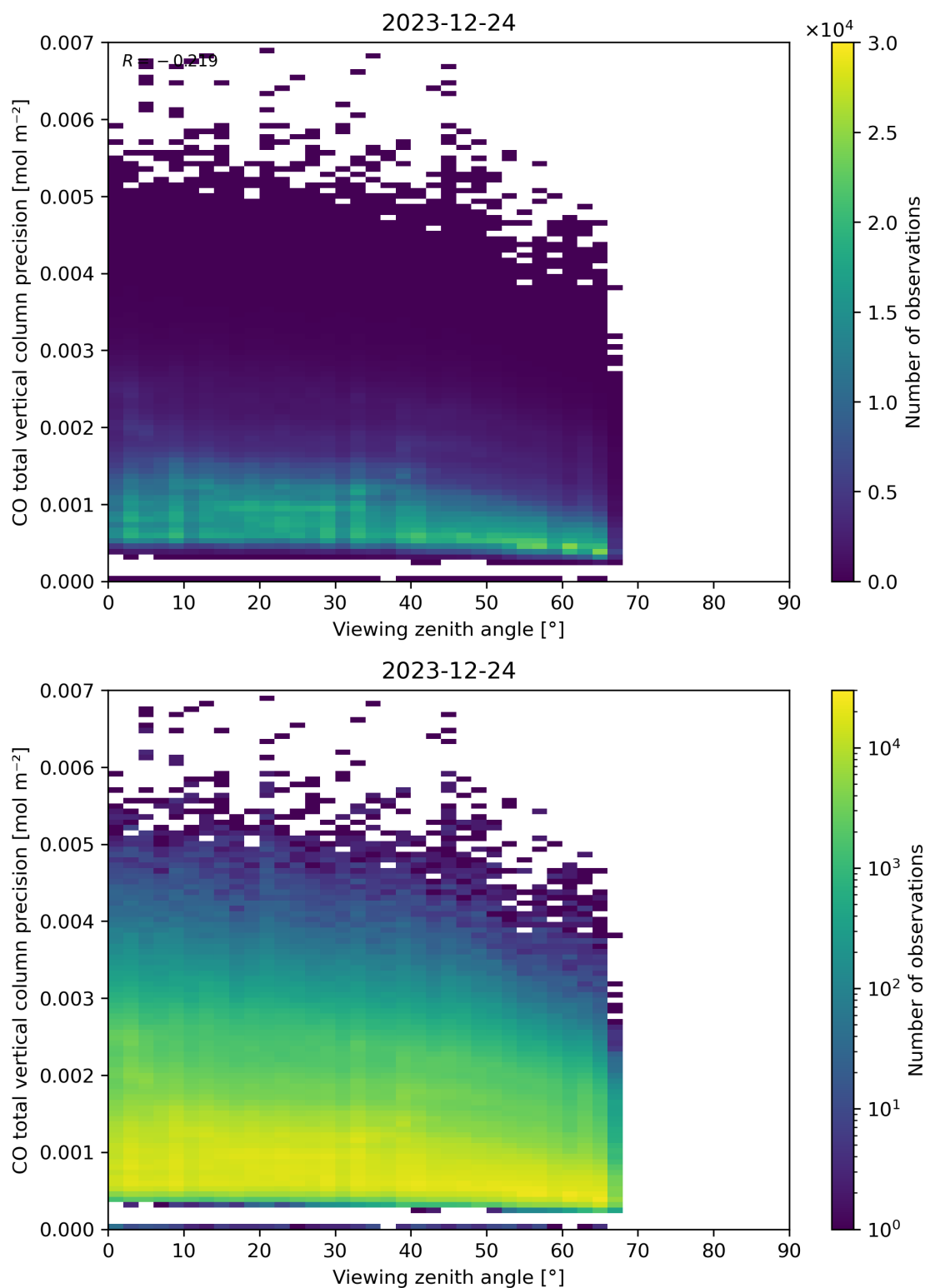
Figure 71: Scatter density plot of “Viewing zenith angle” against “CO total vertical column precision” for 2023-12-23 to 2023-12-25.
