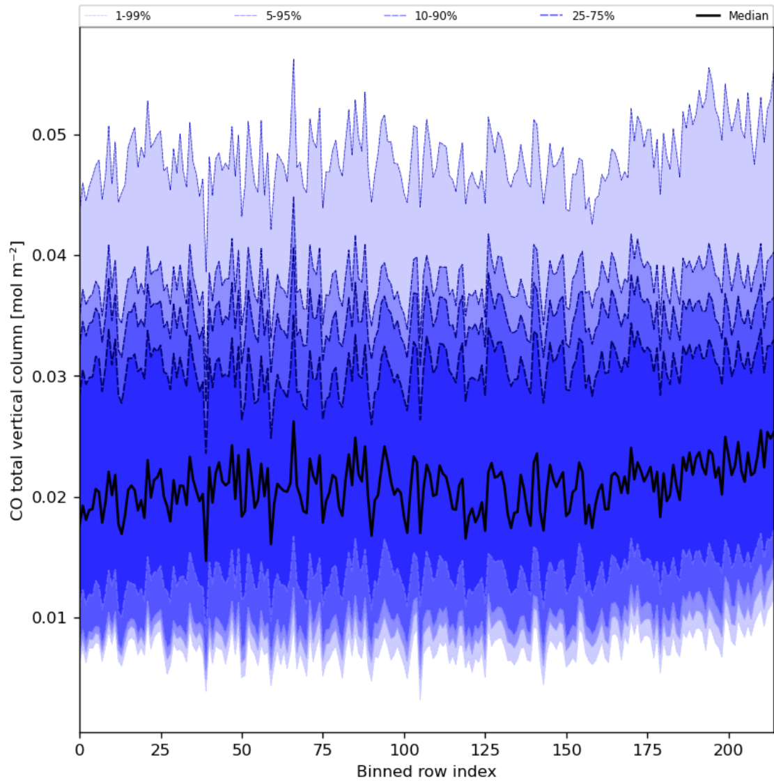
Figure 26: Along track statistics of “CO total vertical column” for 2023-12-23 to 2023-12-25
