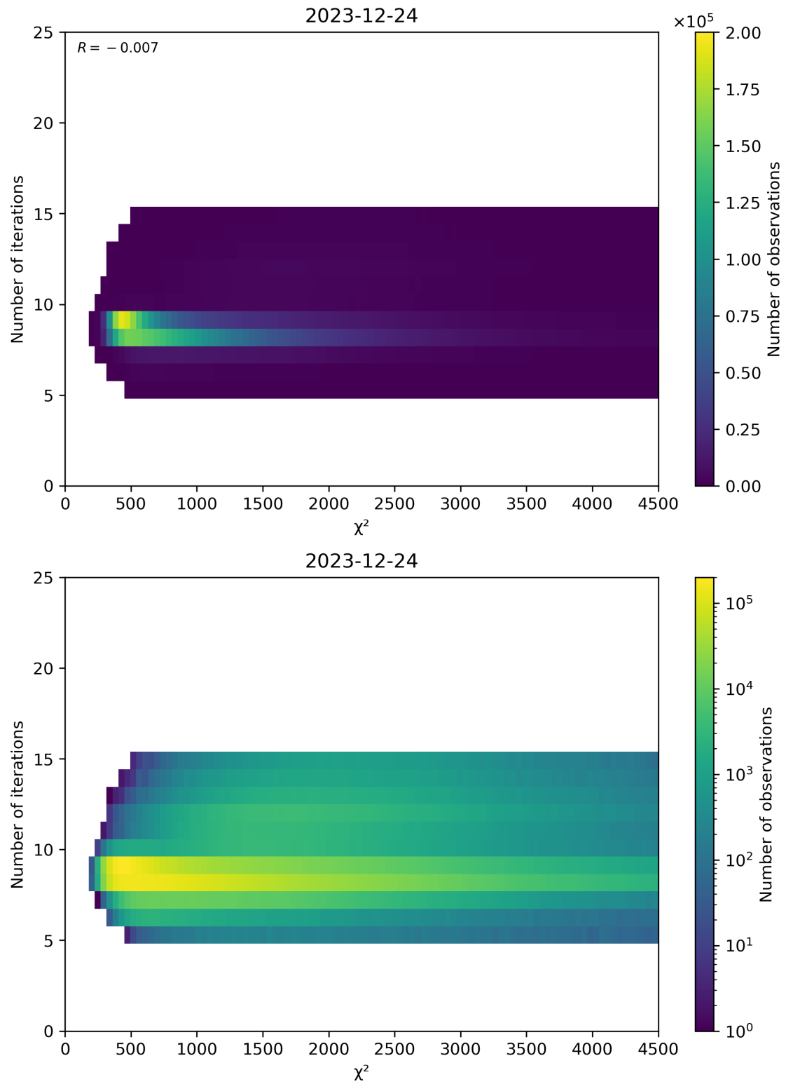
Figure 49: Scatter density plot of “ \chi^2 ” against “Number of iterations” for 2023-12-23 to 2023-12-25.
