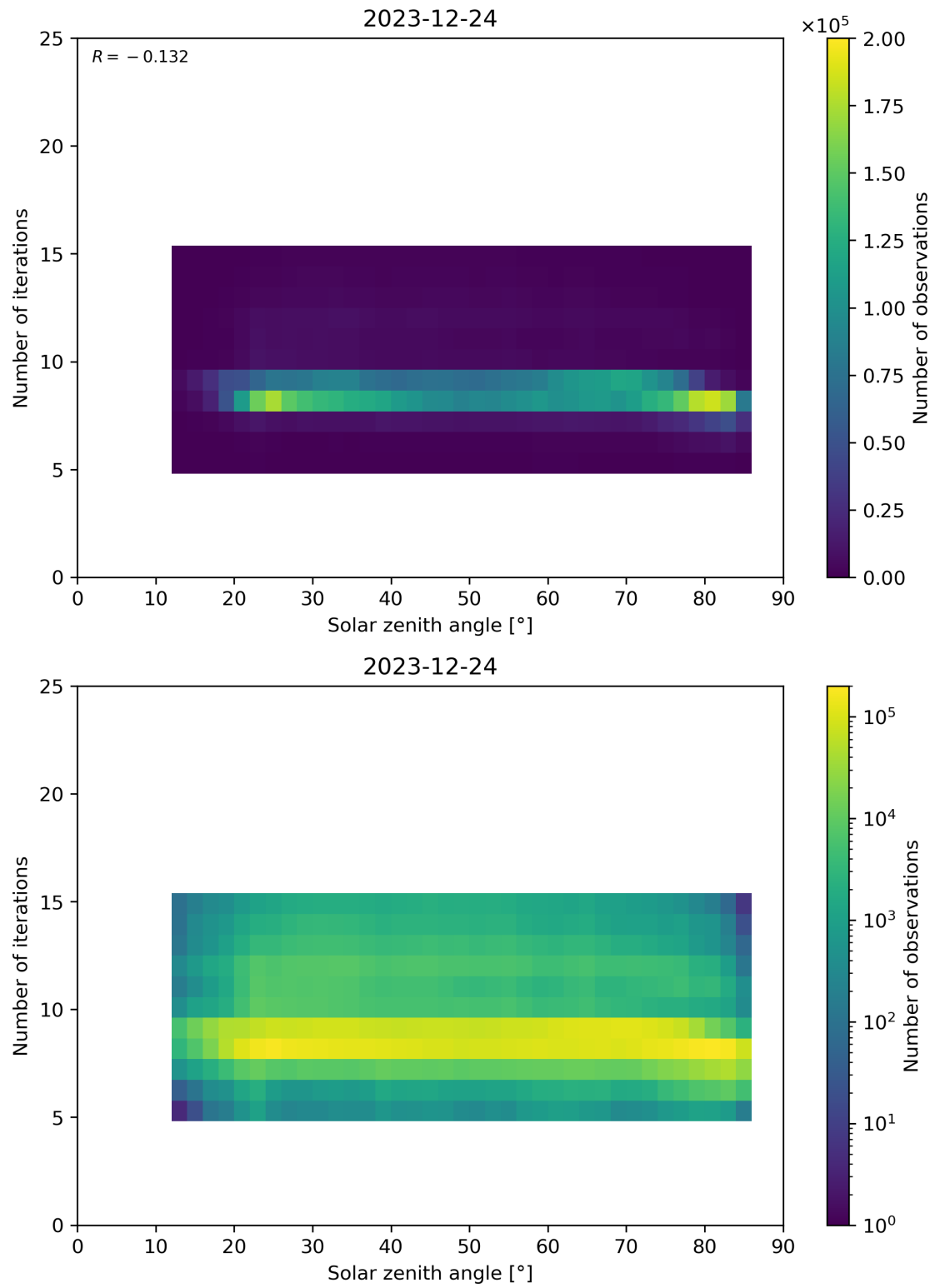
Figure 67: Scatter density plot of “Solar zenith angle” against “Number of iterations” for 2023-12-23 to 2023-12-25.
