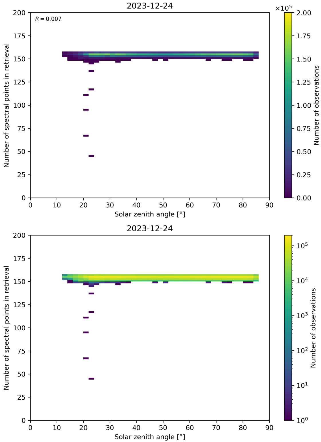
Figure 68: Scatter density plot of “Solar zenith angle” against “Number of spectral points in retrieval” for 2023-12-23 to 2023-12-25.
