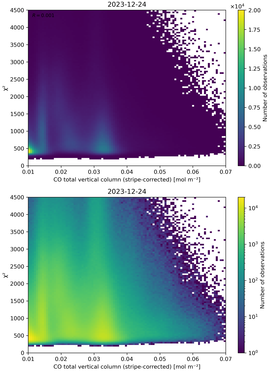
Figure 37: Scatter density plot of “CO total vertical column (stripe-corrected)” against “ \chi^2 ” for 2023-12-23 to 2023-12-25.
