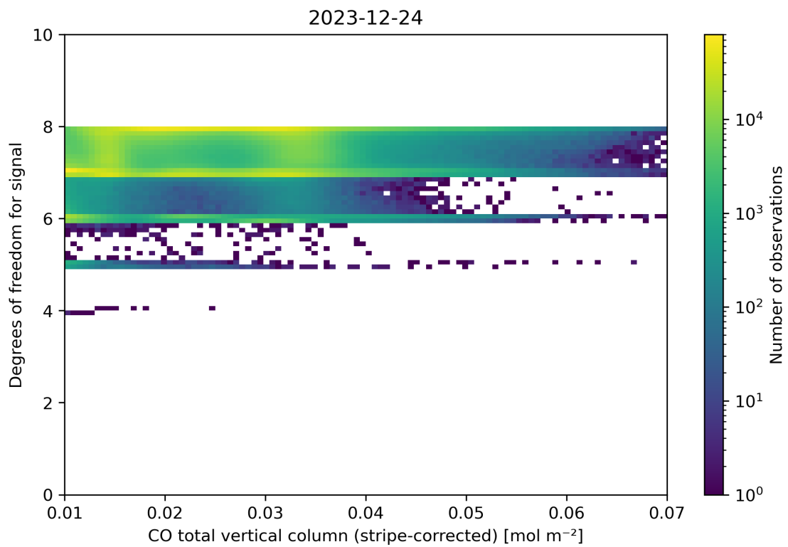
Figure 38: Scatter density plot of “CO total vertical column (stripe-corrected)” against “Degrees of freedom for signal” for 2023-12-23 to 2023-12-25.
