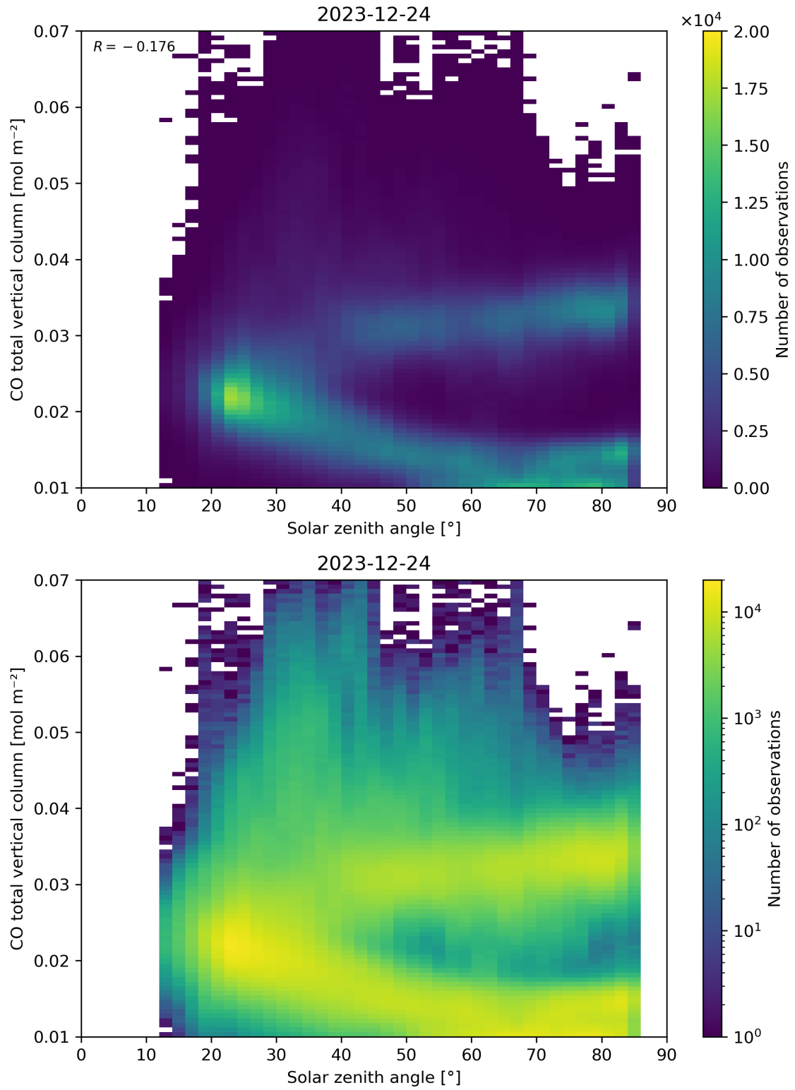
Figure 61: Scatter density plot of “Solar zenith angle” against “CO total vertical column” for 2023-12-23 to 2023-12-25.
