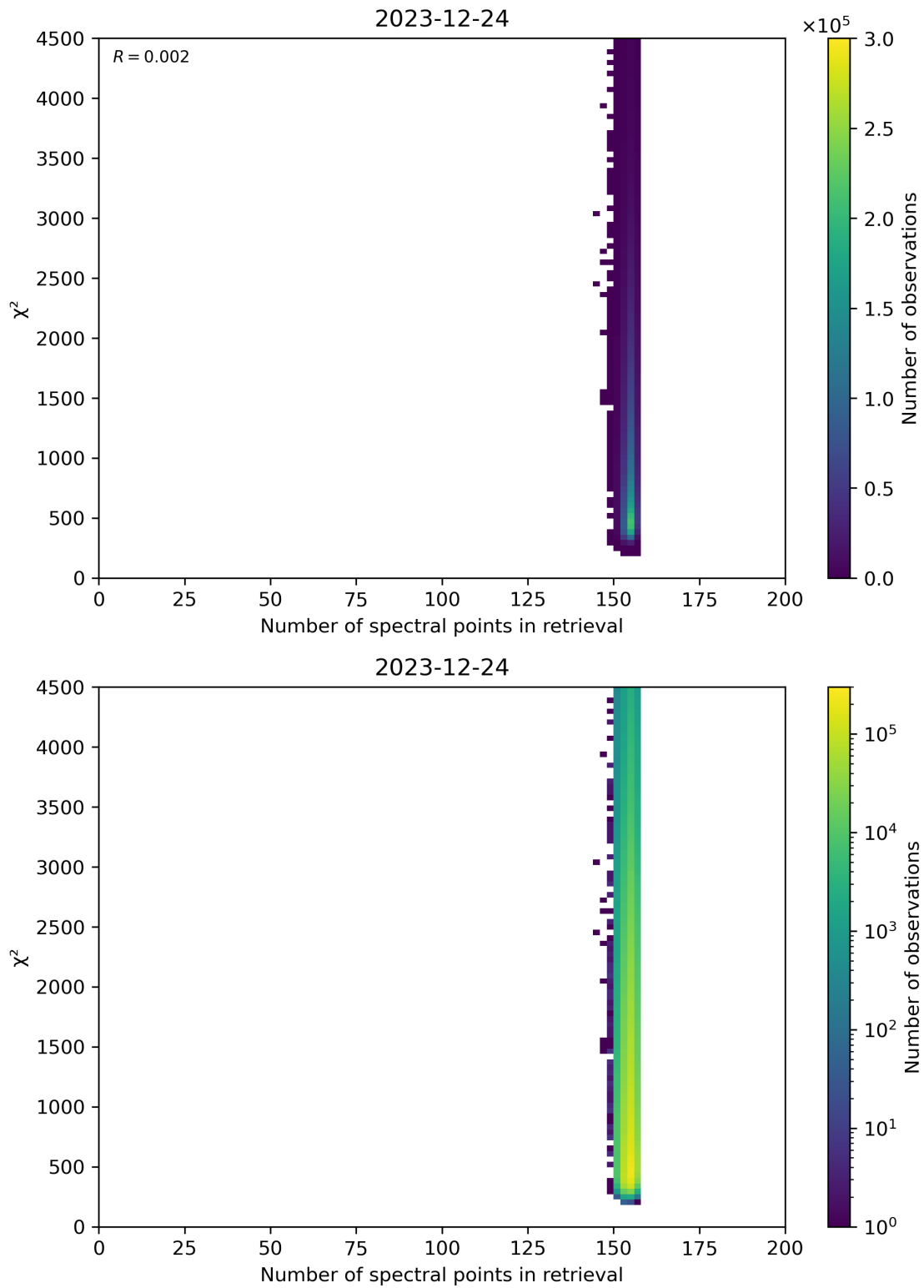
Figure 58: Scatter density plot of “Number of spectral points in retrieval” against “ \chi^2 ” for 2023-12-23 to 2023-12-25.
