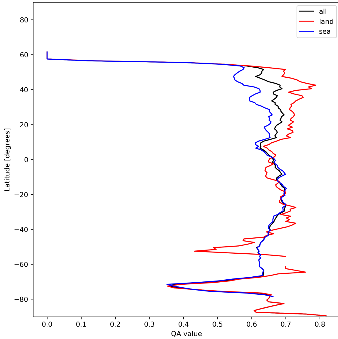
Figure 9: Zonal average of “QA value” for 2023-12-23 to 2023-12-25.
