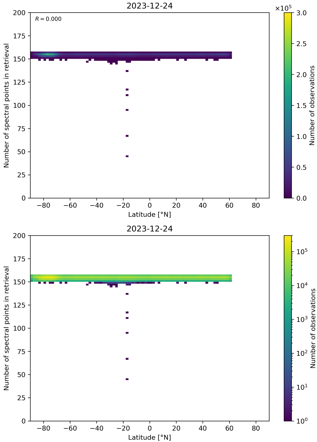
Figure 57: Scatter density plot of “Latitude” against “Number of spectral points in retrieval” for 2023-12-23 to 2023-12-25.
