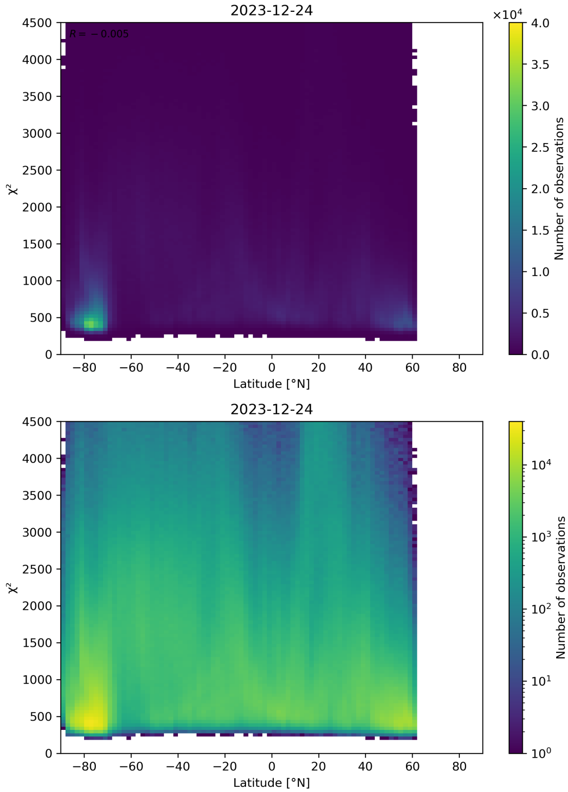
Figure 54: Scatter density plot of “Latitude” against “ \chi^2 ” for 2023-12-23 to 2023-12-25.
