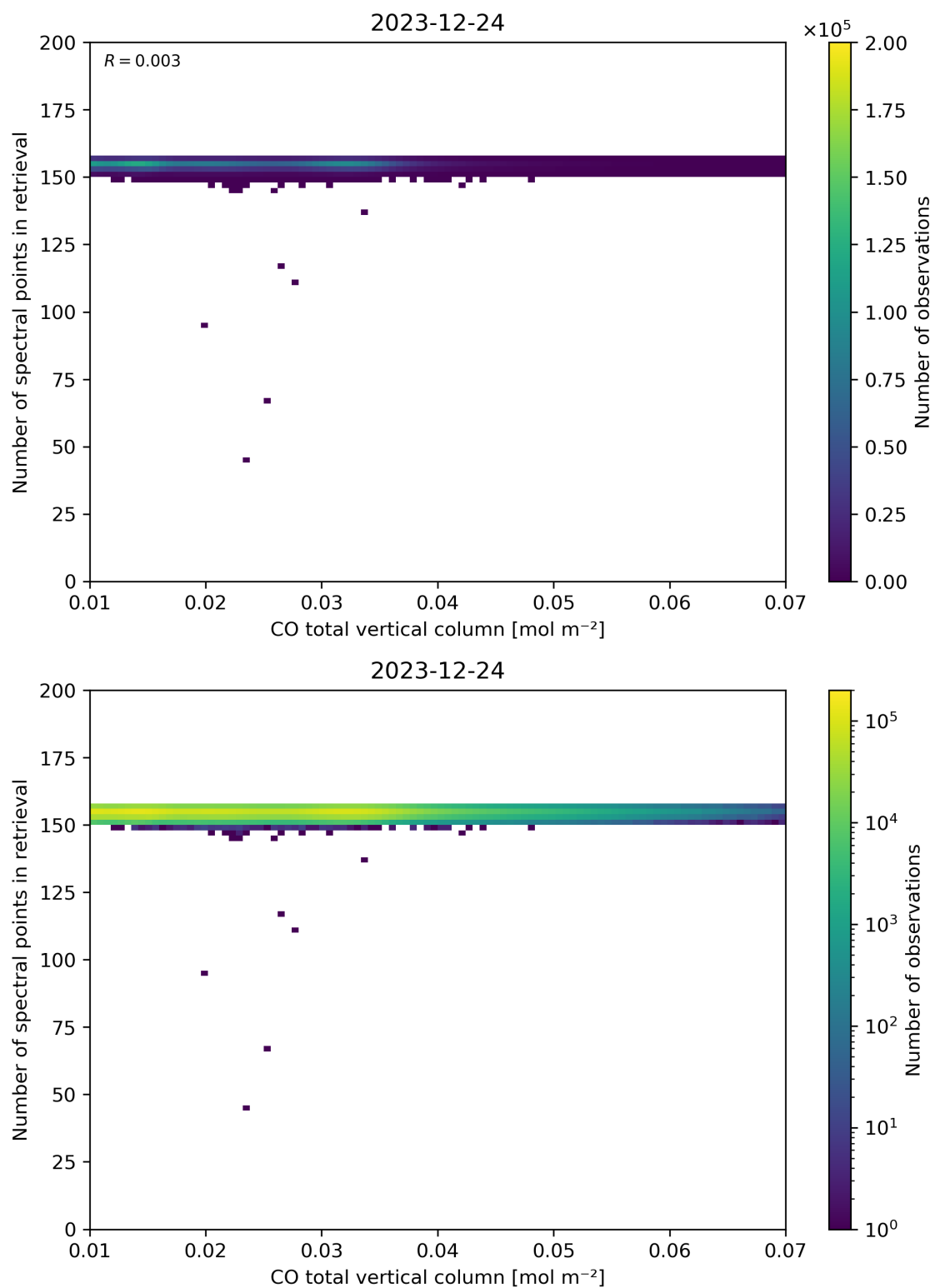
Figure 43: Scatter density plot of “CO total vertical column” against “Number of spectral points in retrieval” for 2023-12-23 to 2023-12-25.
