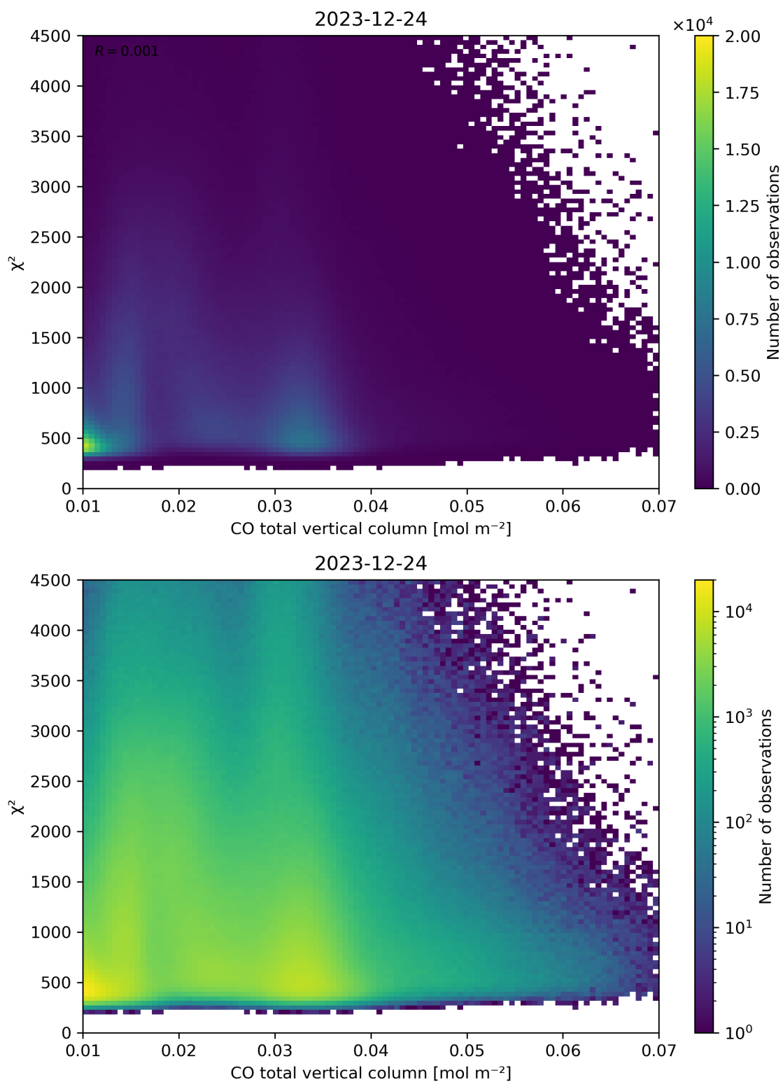
Figure 35: Scatter density plot of “CO total vertical column” against “ \chi^2 ” for 2023-12-23 to 2023-12-25.
