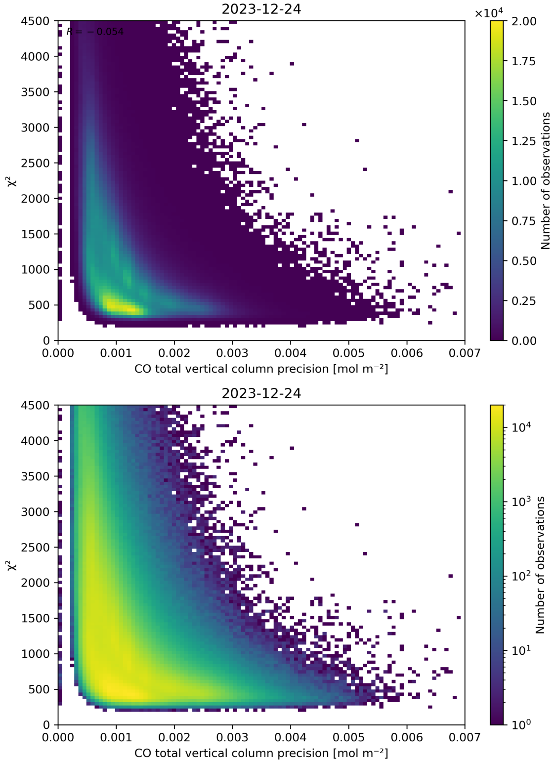
Figure 44: Scatter density plot of “CO total vertical column precision” against “ \chi^2 ” for 2023-12-23 to 2023-12-25.
