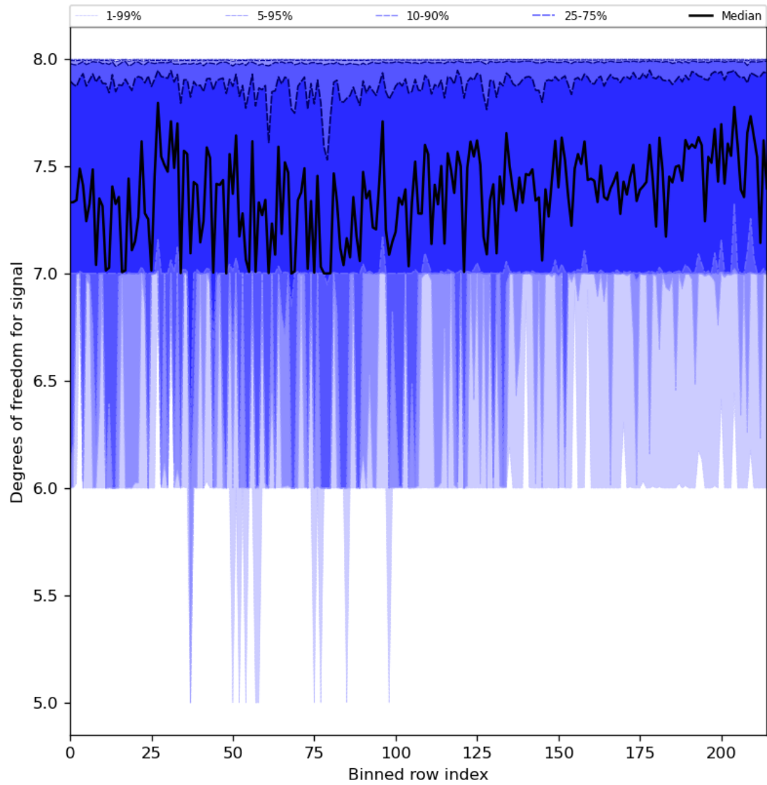
Figure 31: Along track statistics of “Degrees of freedom for signal” for 2023-12-23 to 2023-12-25
