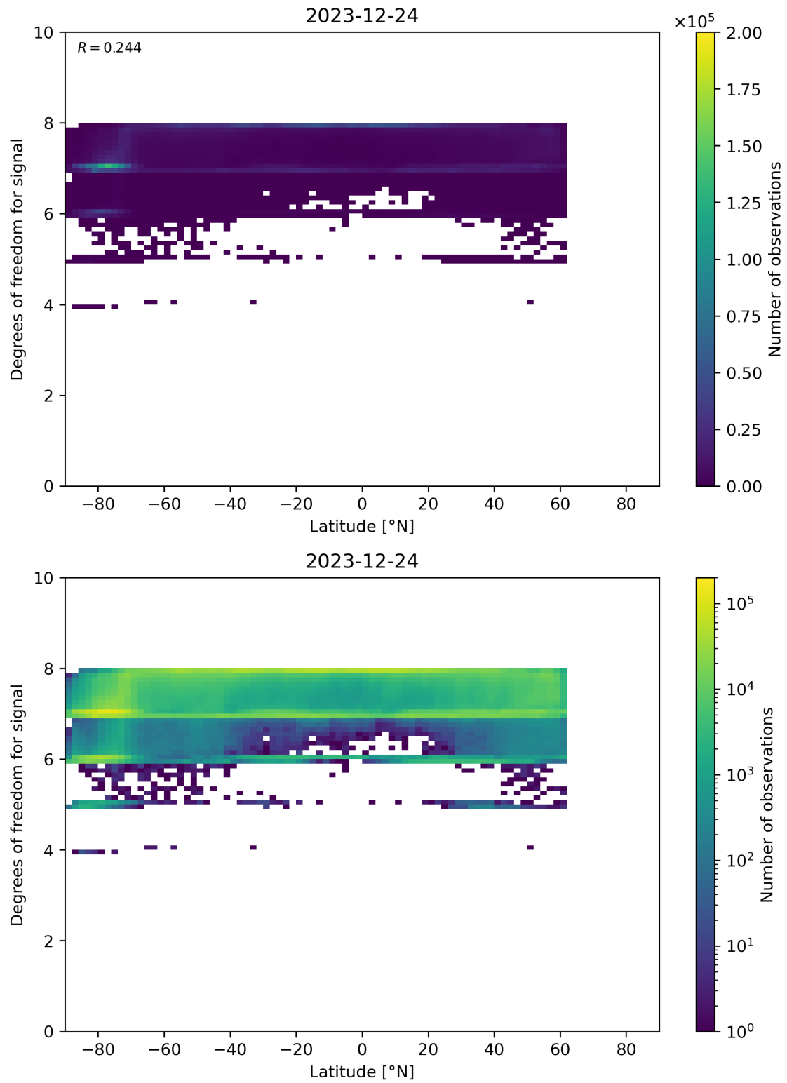
Figure 55: Scatter density plot of “Latitude” against “Degrees of freedom for signal” for 2023-12-23 to 2023-12-25.
