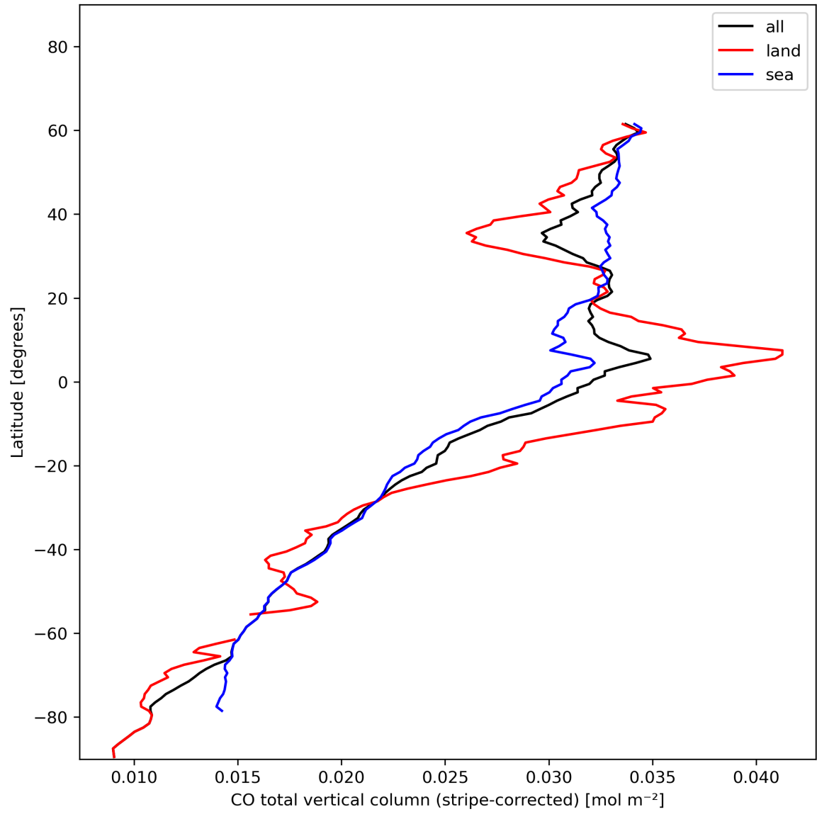
Figure 11: Zonal average of “CO total vertical column (stripe-corrected)” for 2023-12-23 to 2023-12-25.
