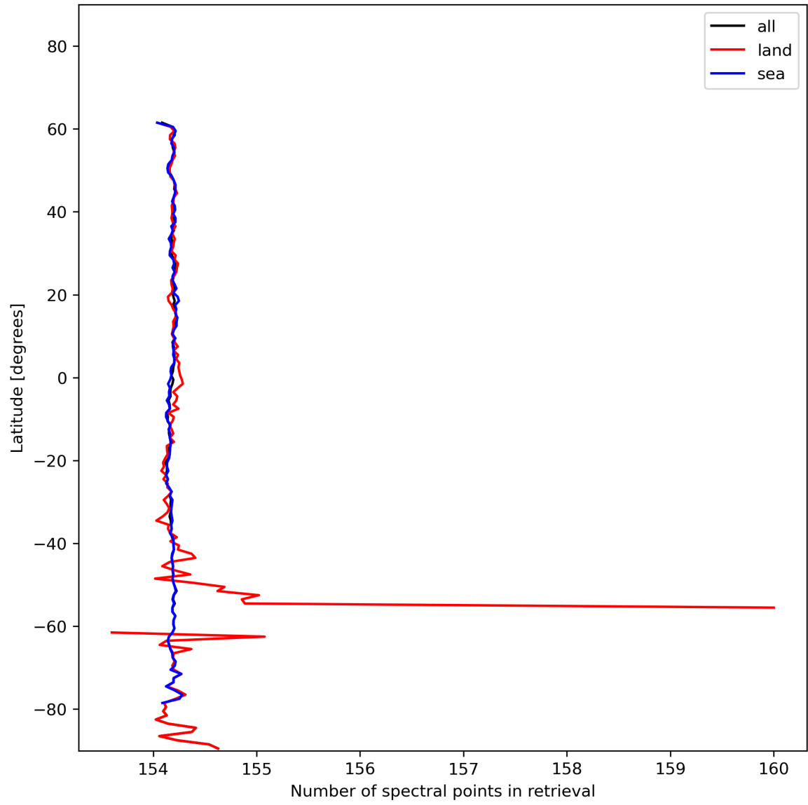
Figure 13: Zonal average of “Number of spectral points in retrieval” for 2023-12-23 to 2023-12-25.
