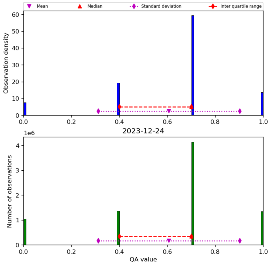
Figure 17: Histogram of “QA value” for 2023-12-23 to 2023-12-25
