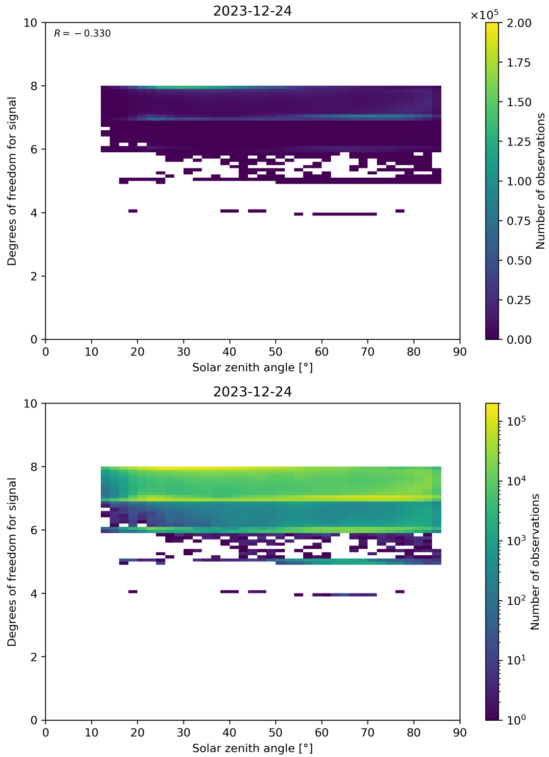
Figure 65: Scatter density plot of “Solar zenith angle” against “Degrees of freedom for signal” for 2023-12-23 to 2023-12-25.
