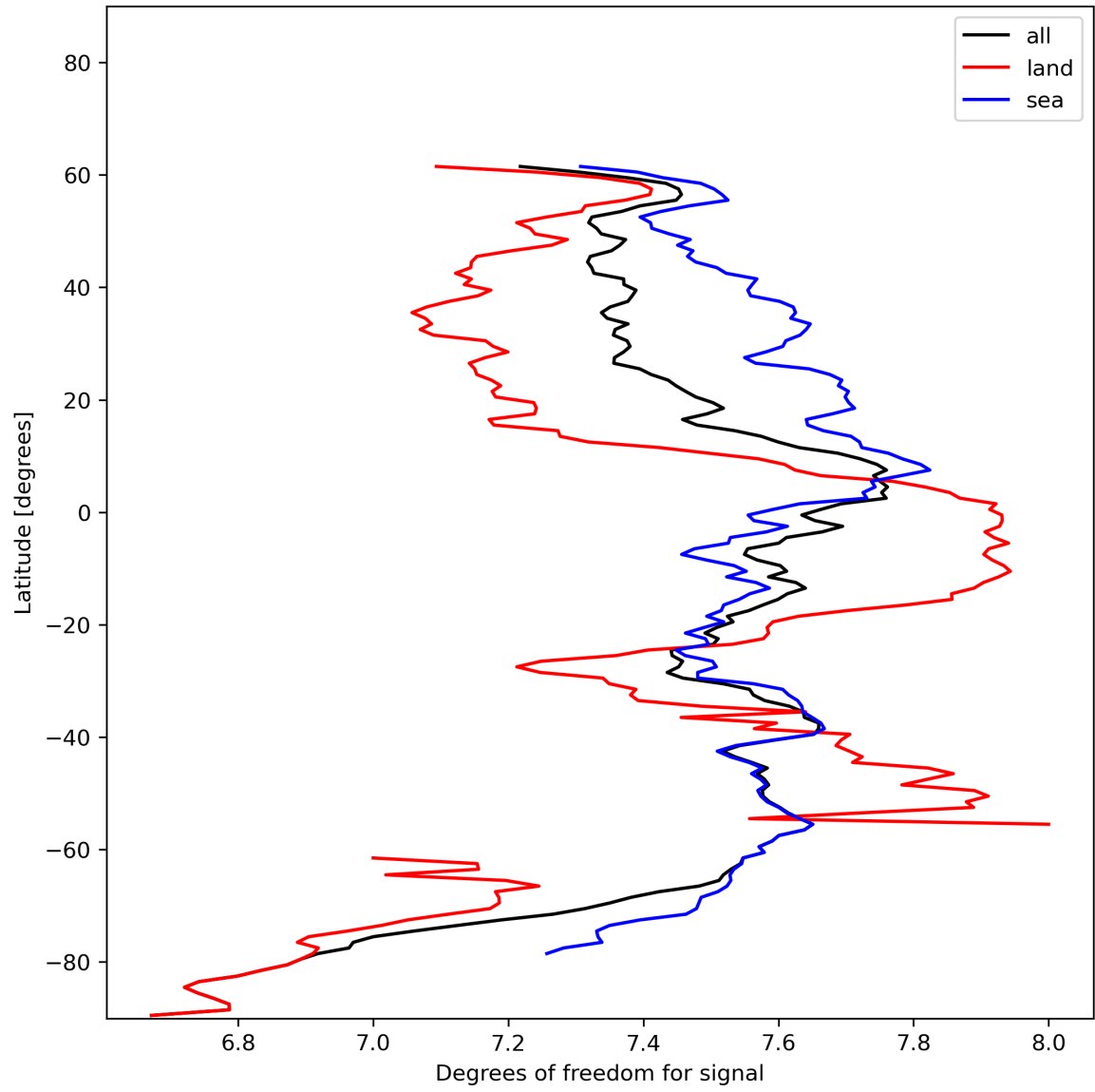
Figure 15: Zonal average of “Degrees of freedom for signal” for 2023-12-23 to 2023-12-25.
