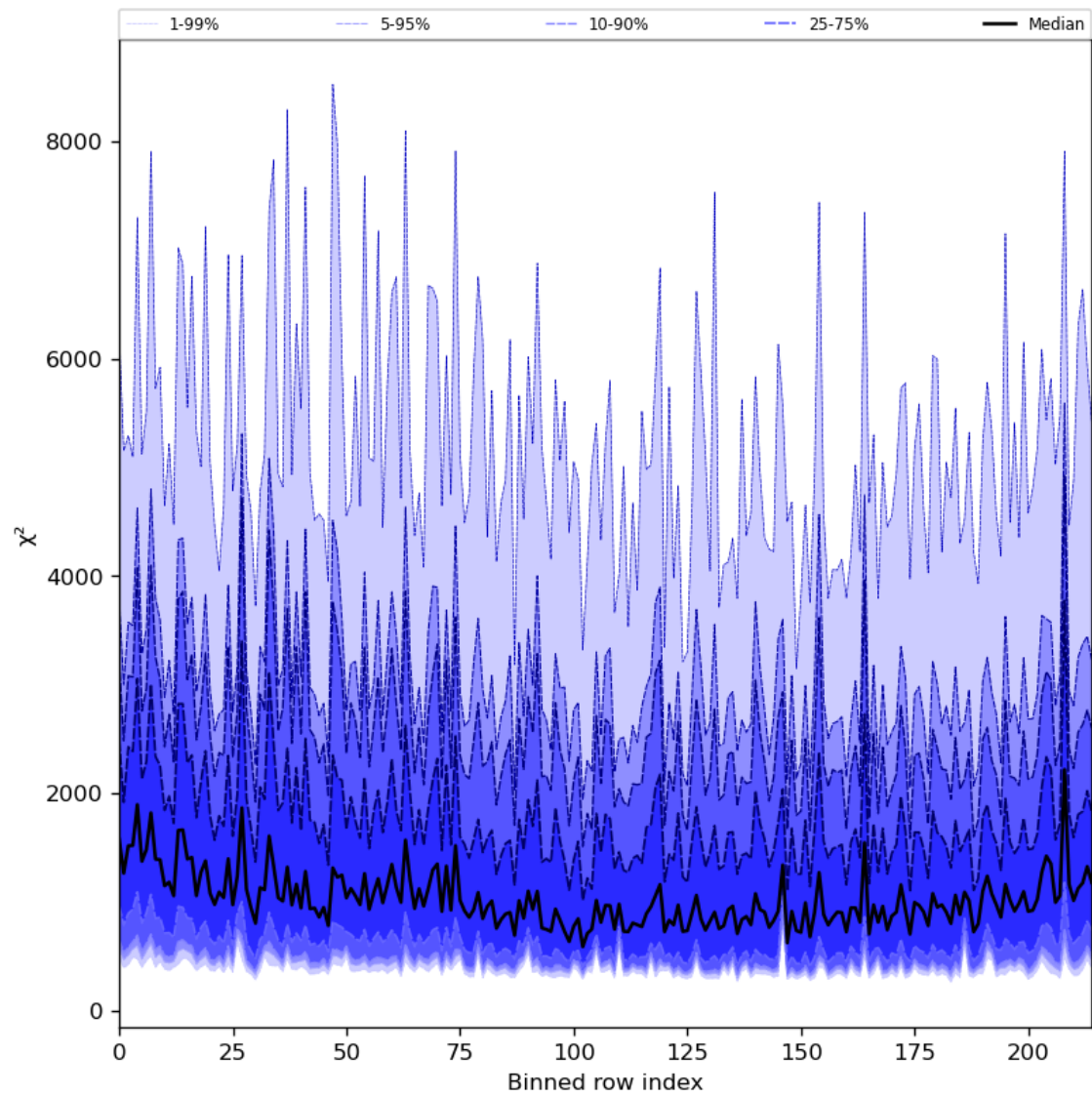
Figure 30: Along track statistics of “ \chi^2 ” for 2023-12-23 to 2023-12-25
