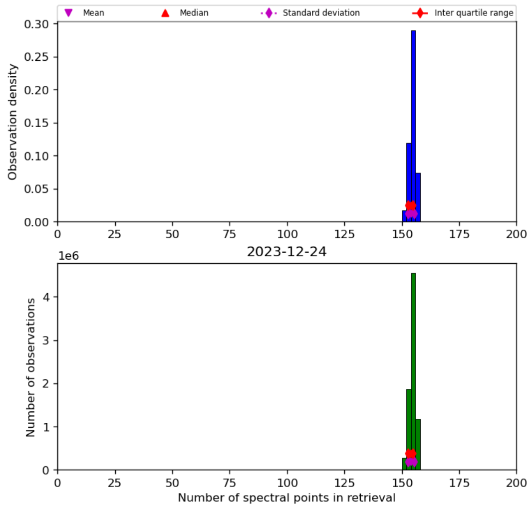
Figure 21: Histogram of “Number of spectral points in retrieval” for 2023-12-23 to 2023-12-25
