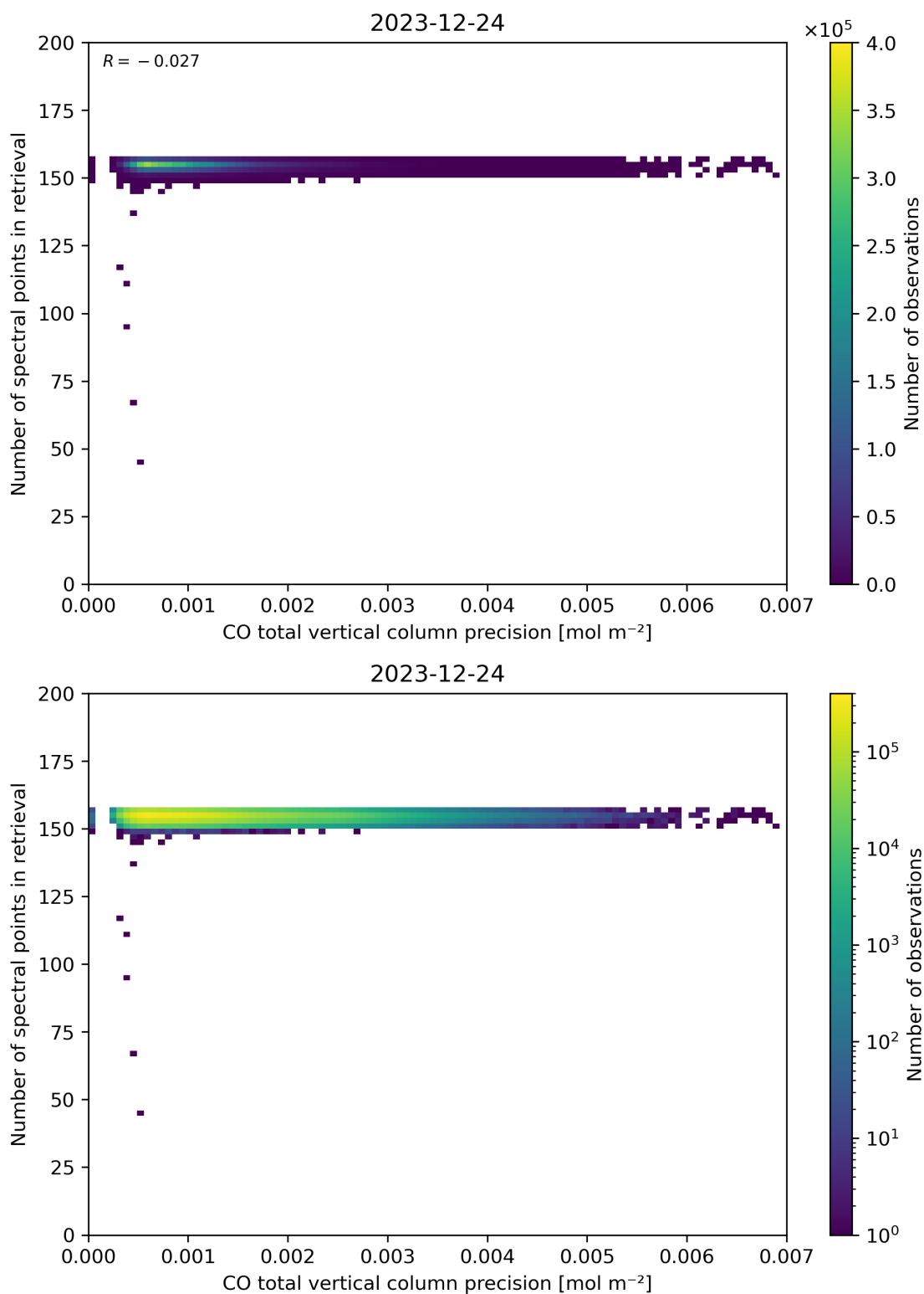
Figure 47: Scatter density plot of “CO total vertical column precision” against “Number of spectral points in retrieval” for 2023-12-23 to 2023-12-25.
