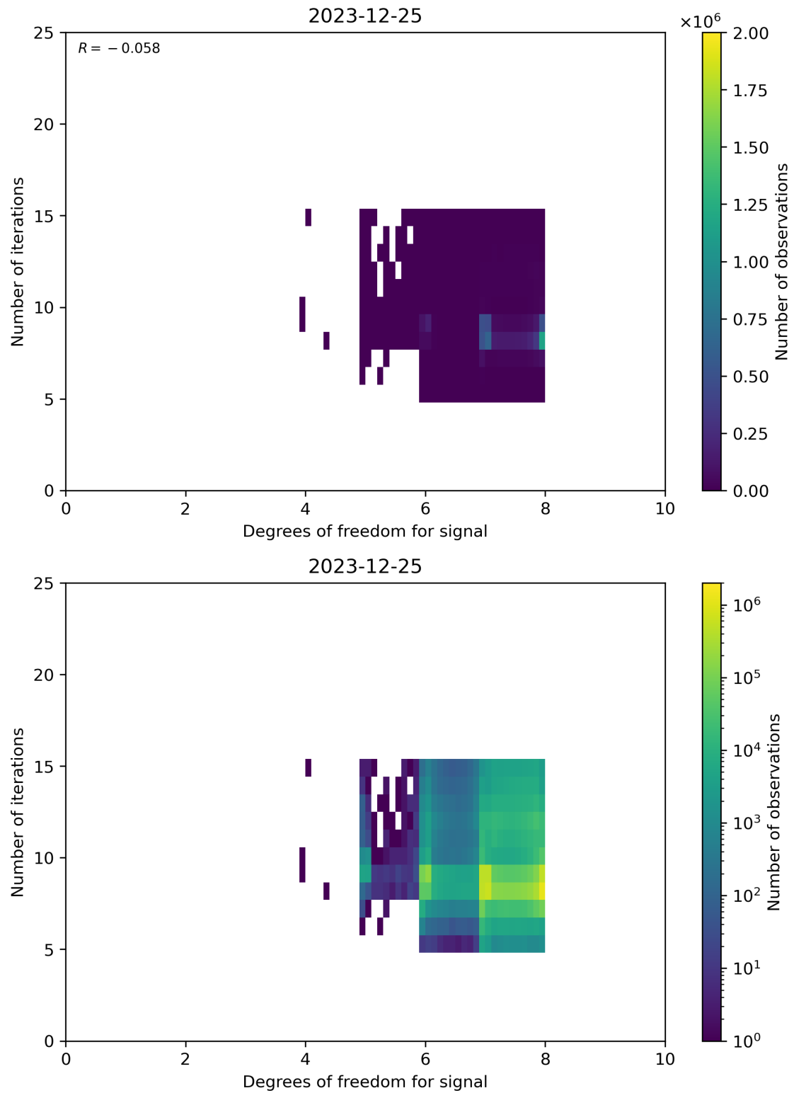
Figure 50: Scatter density plot of “Degrees of freedom for signal” against “Number of iterations” for 2023-12-25 to 2023-12-26.
