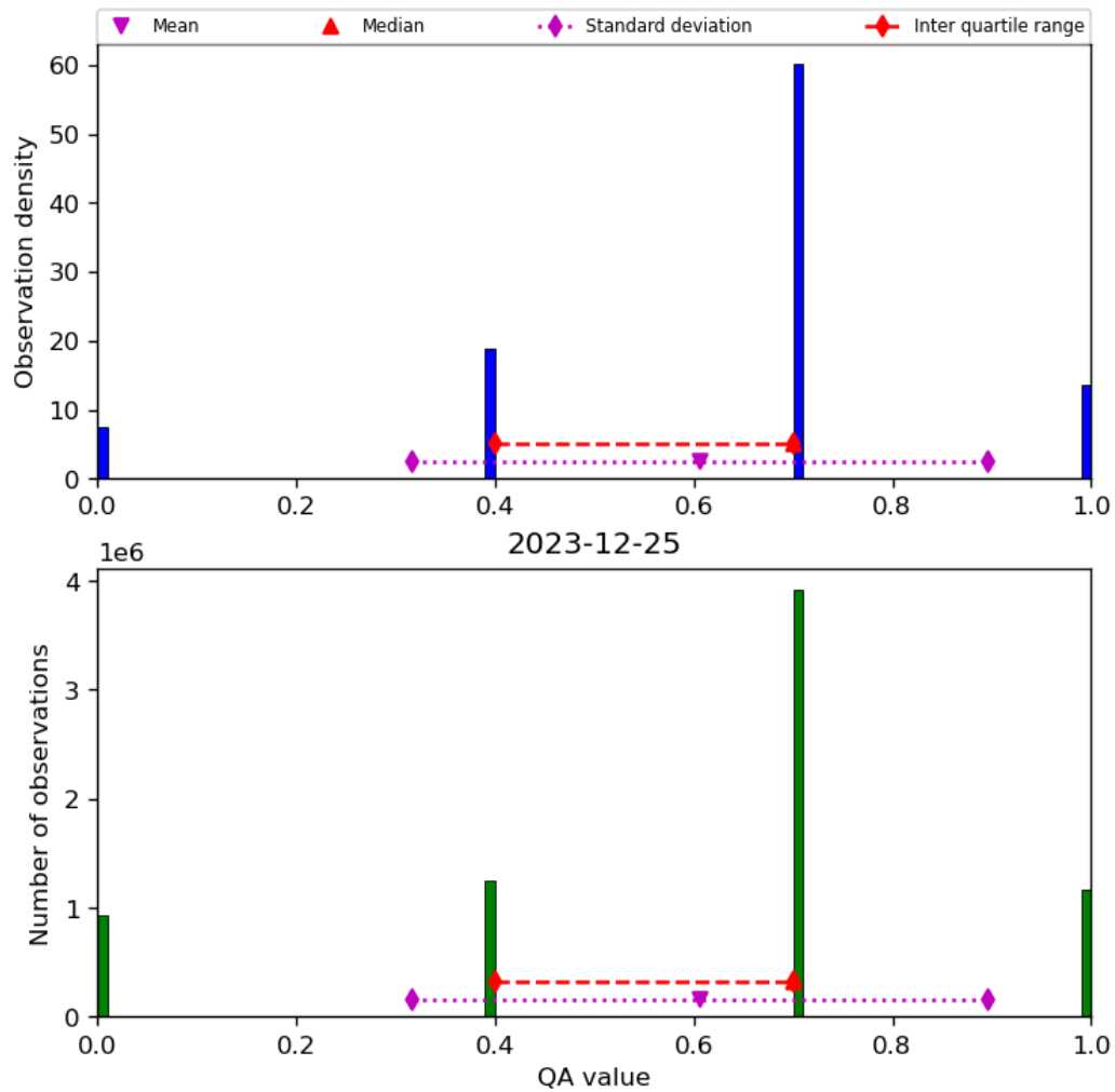
Figure 17: Histogram of “QA value” for 2023-12-25 to 2023-12-26
