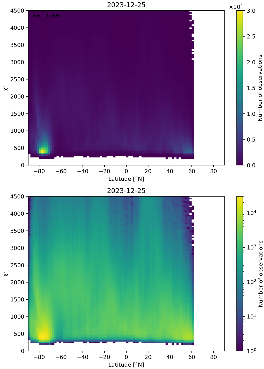
Figure 54: Scatter density plot of “Latitude” against “ \chi^2 ” for 2023-12-25 to 2023-12-26.
