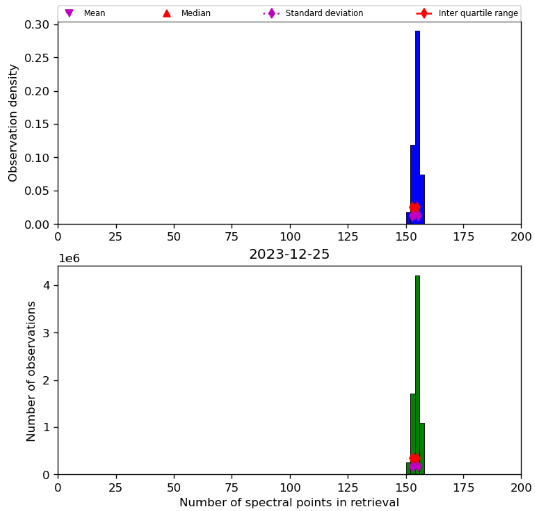
Figure 21: Histogram of “Number of spectral points in retrieval” for 2023-12-25 to 2023-12-26
