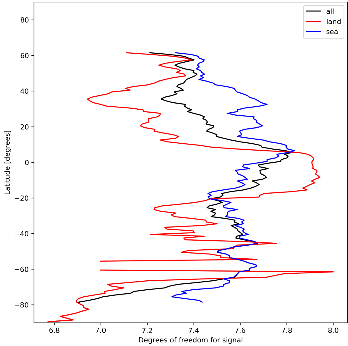
Figure 15: Zonal average of “Degrees of freedom for signal” for 2023-12-25 to 2023-12-26.
