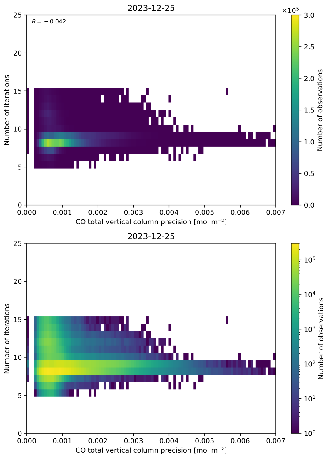
Figure 46: Scatter density plot of “CO total vertical column precision” against “Number of iterations” for 2023-12-25 to 2023-12-26.
