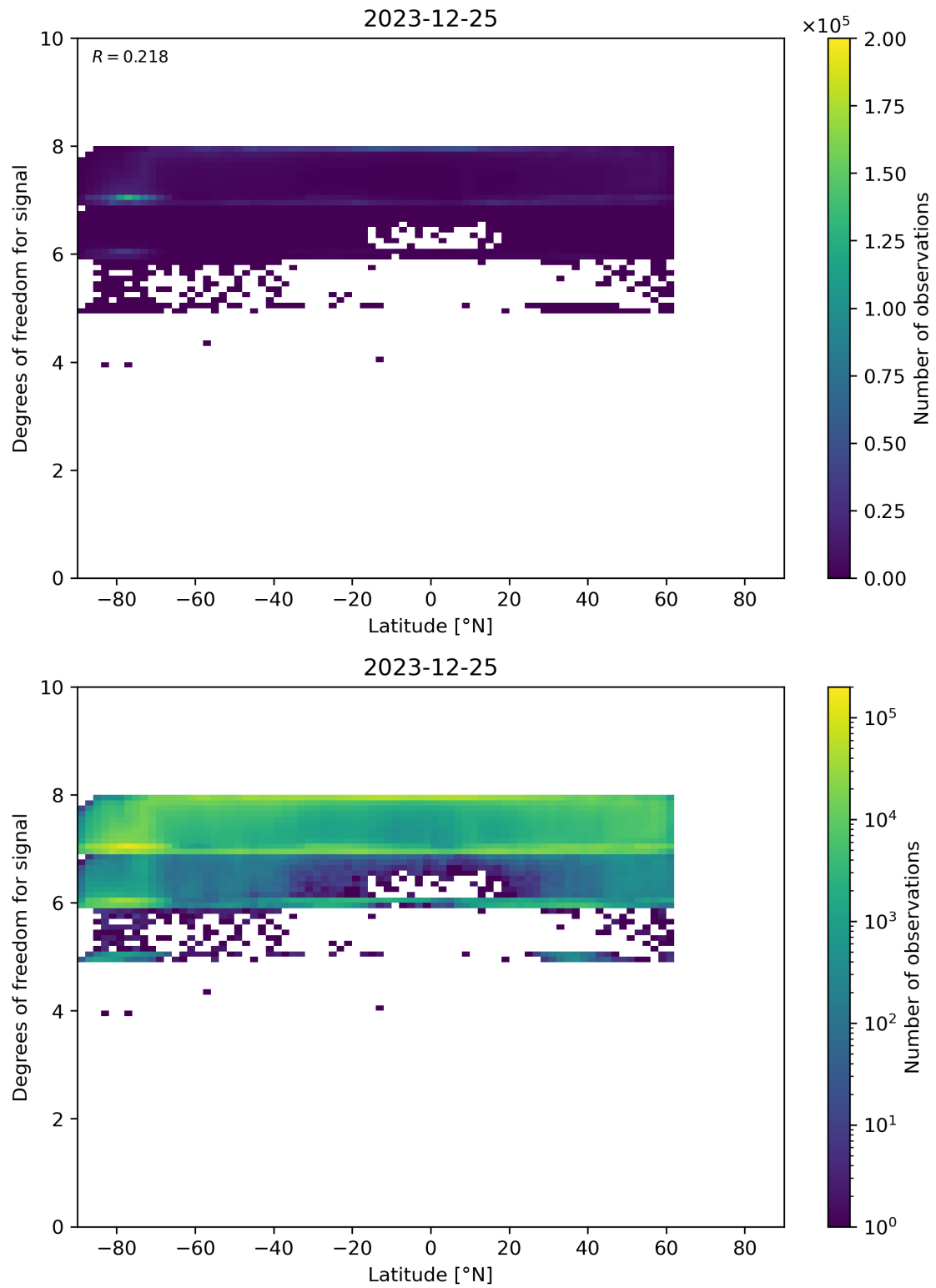
Figure 55: Scatter density plot of “Latitude” against “Degrees of freedom for signal” for 2023-12-25 to 2023-12-26.
