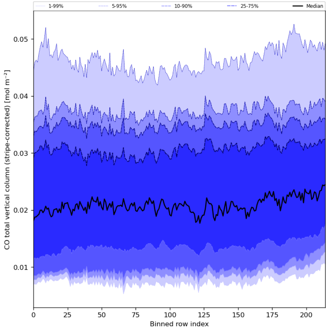
Figure 27: Along track statistics of “CO total vertical column (stripe-corrected)” for 2023-12-25 to 2023-12-26
