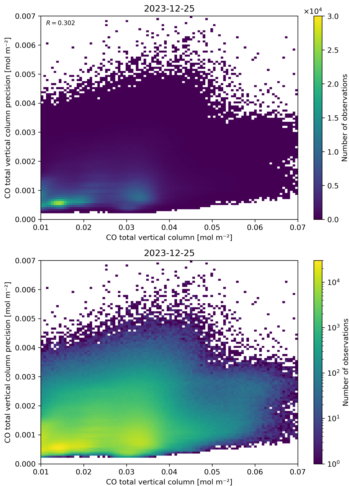
Figure 34: Scatter density plot of “CO total vertical column” against “CO total vertical column precision” for 2023-12-25 to 2023-12-26.
