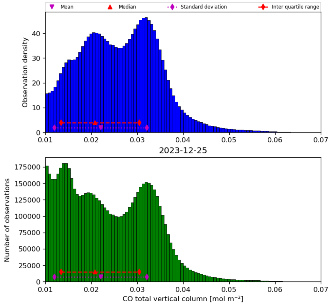
Figure 18: Histogram of “CO total vertical column” for 2023-12-25 to 2023-12-26
