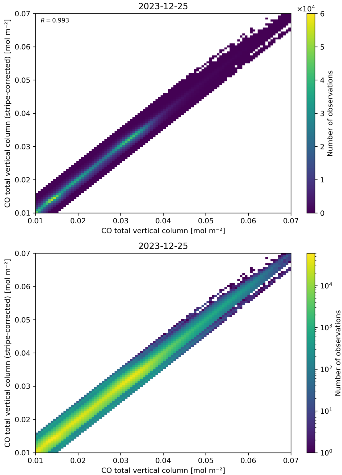
Figure 33: Scatter density plot of “CO total vertical column” against “CO total vertical column (stripe-corrected)” for 2023-12-25 to 2023-12-26.
