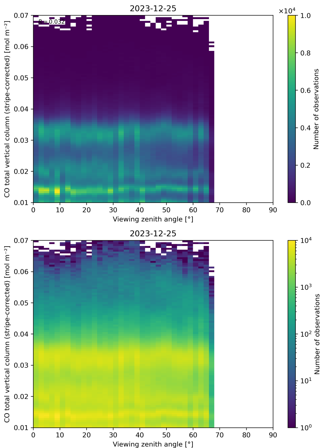
Figure 70: Scatter density plot of “Viewing zenith angle” against “CO total vertical column (stripe-corrected)” for 2023-12-25 to 2023-12-26.
