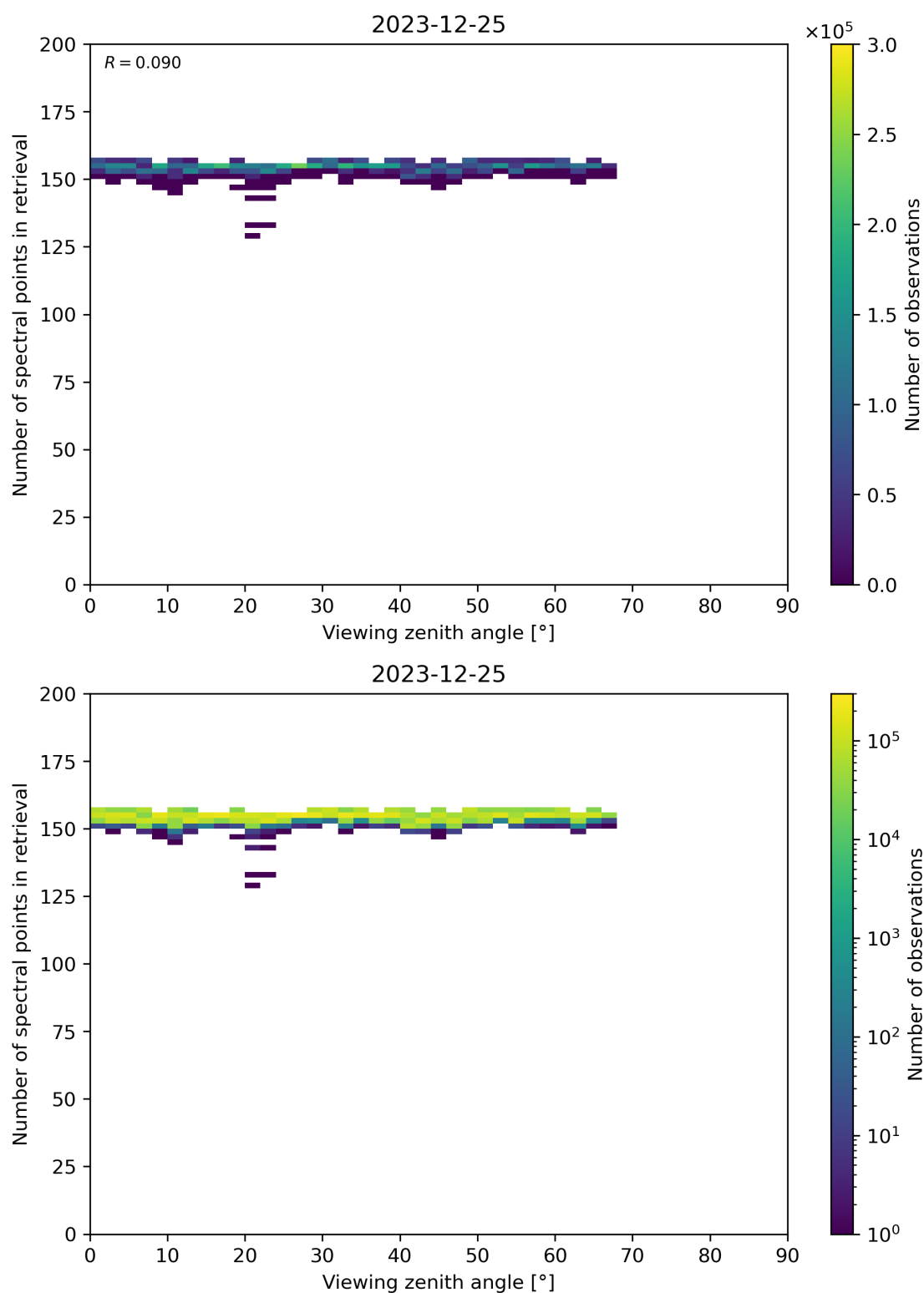
Figure 76: Scatter density plot of “Viewing zenith angle” against “Number of spectral points in retrieval” for 2023-12-25 to 2023-12-26.
