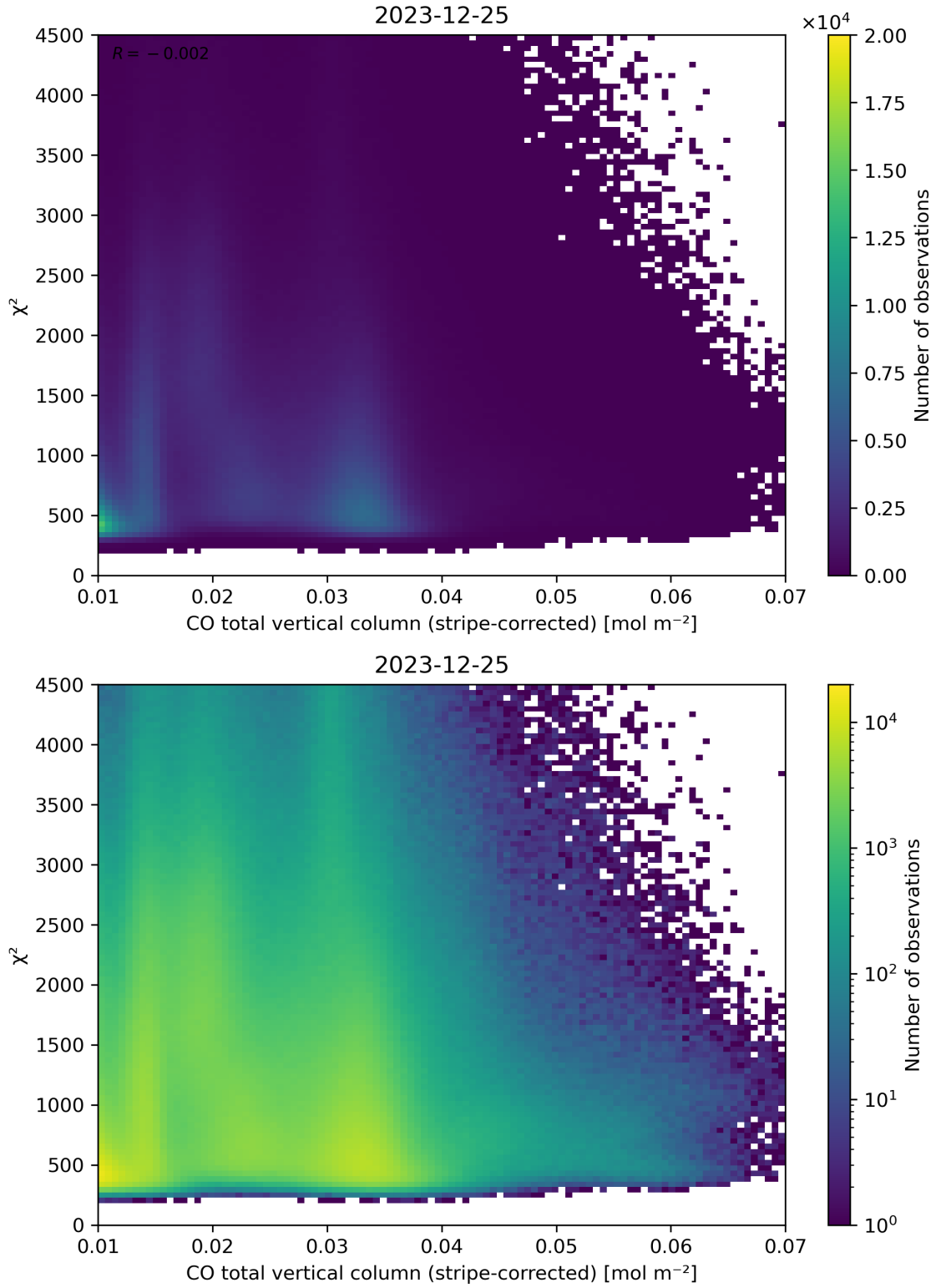
Figure 37: Scatter density plot of “CO total vertical column (stripe-corrected)” against “ \chi^2 ” for 2023-12-25 to 2023-12-26.
