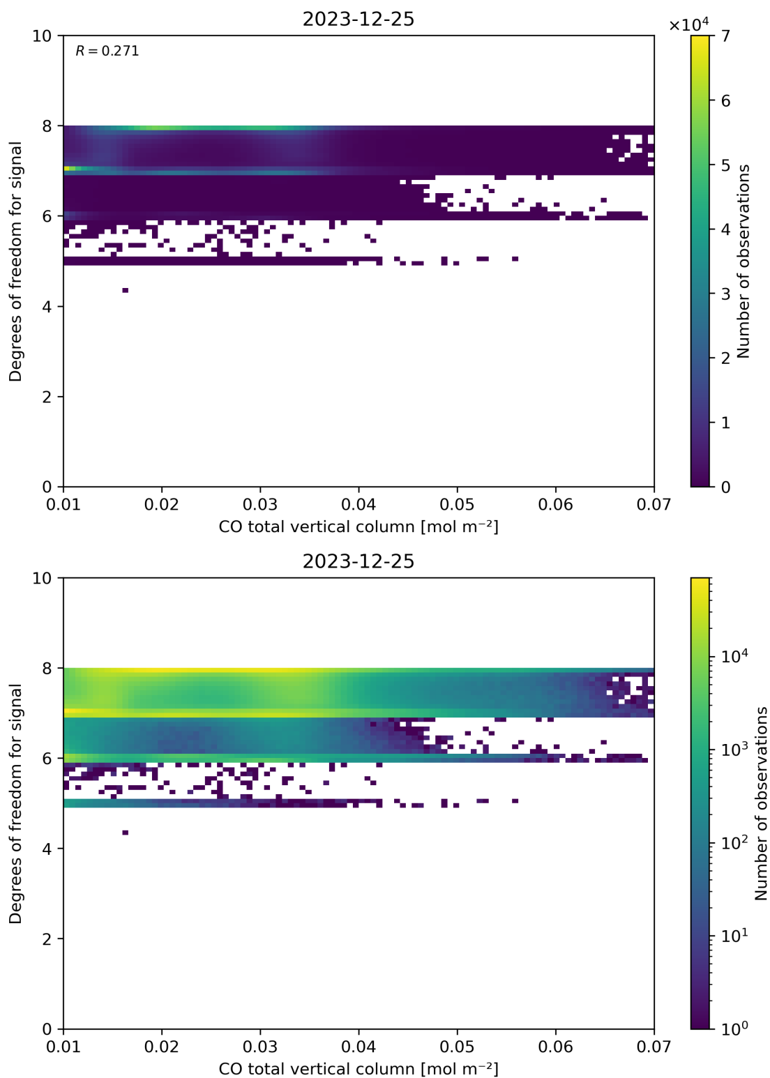
Figure 41: Scatter density plot of “CO total vertical column” against “Degrees of freedom for signal” for 2023-12-25 to 2023-12-26.
