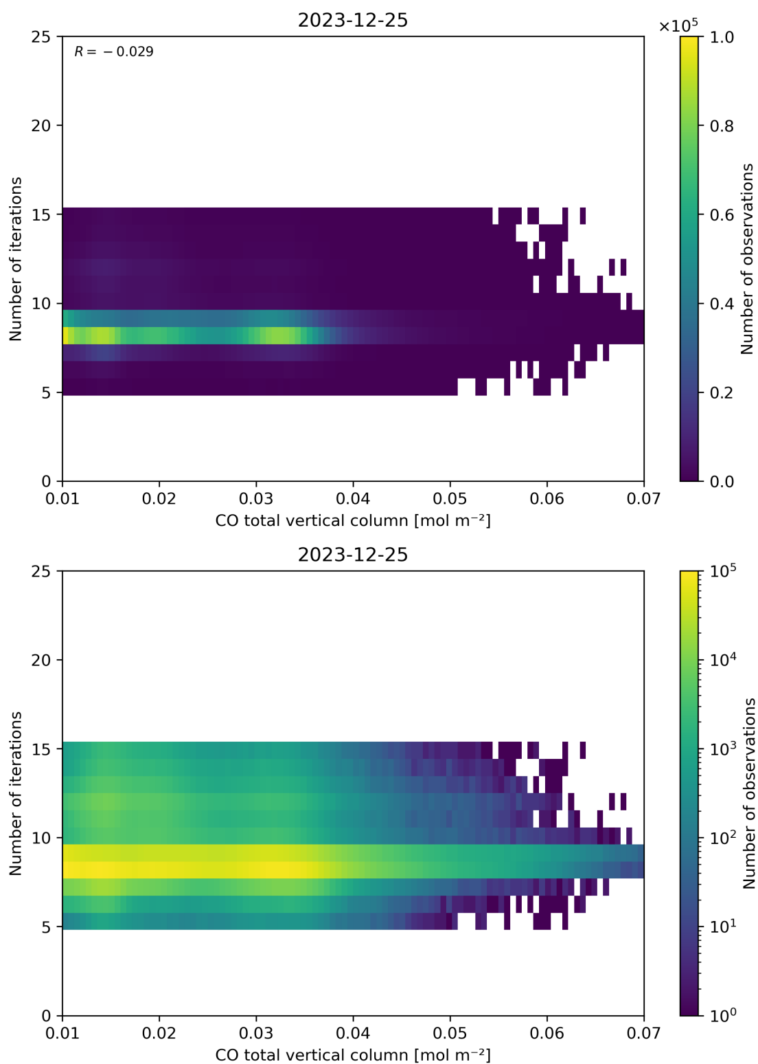
Figure 42: Scatter density plot of “CO total vertical column” against “Number of iterations” for 2023-12-25 to 2023-12-26.
