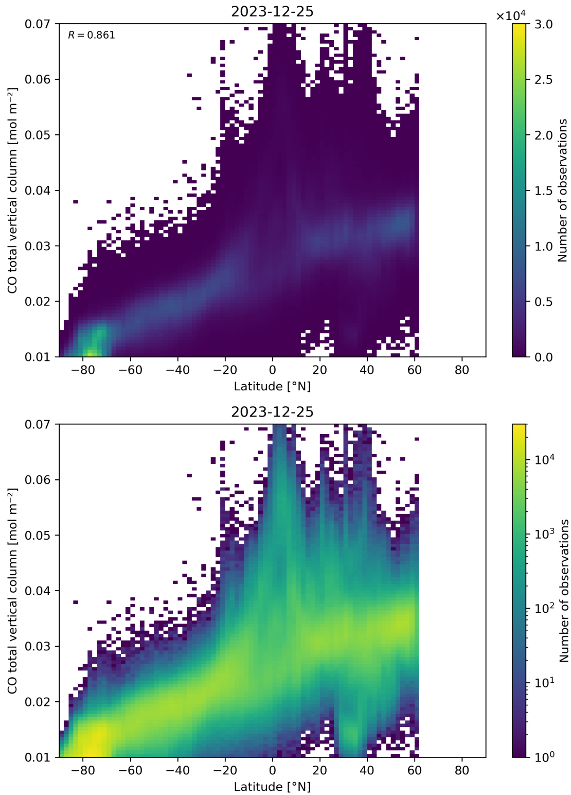
Figure 51: Scatter density plot of “Latitude” against “CO total vertical column” for 2023-12-25 to 2023-12-26.
