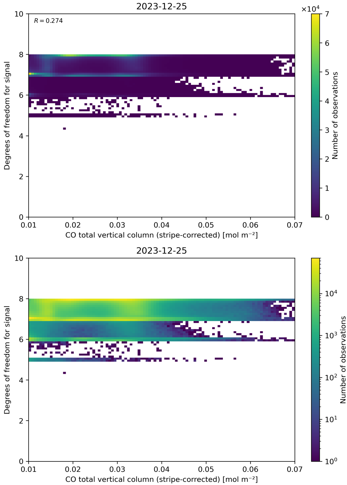
Figure 38: Scatter density plot of “CO total vertical column (stripe-corrected)” against “Degrees of freedom for signal” for 2023-12-25 to 2023-12-26.
