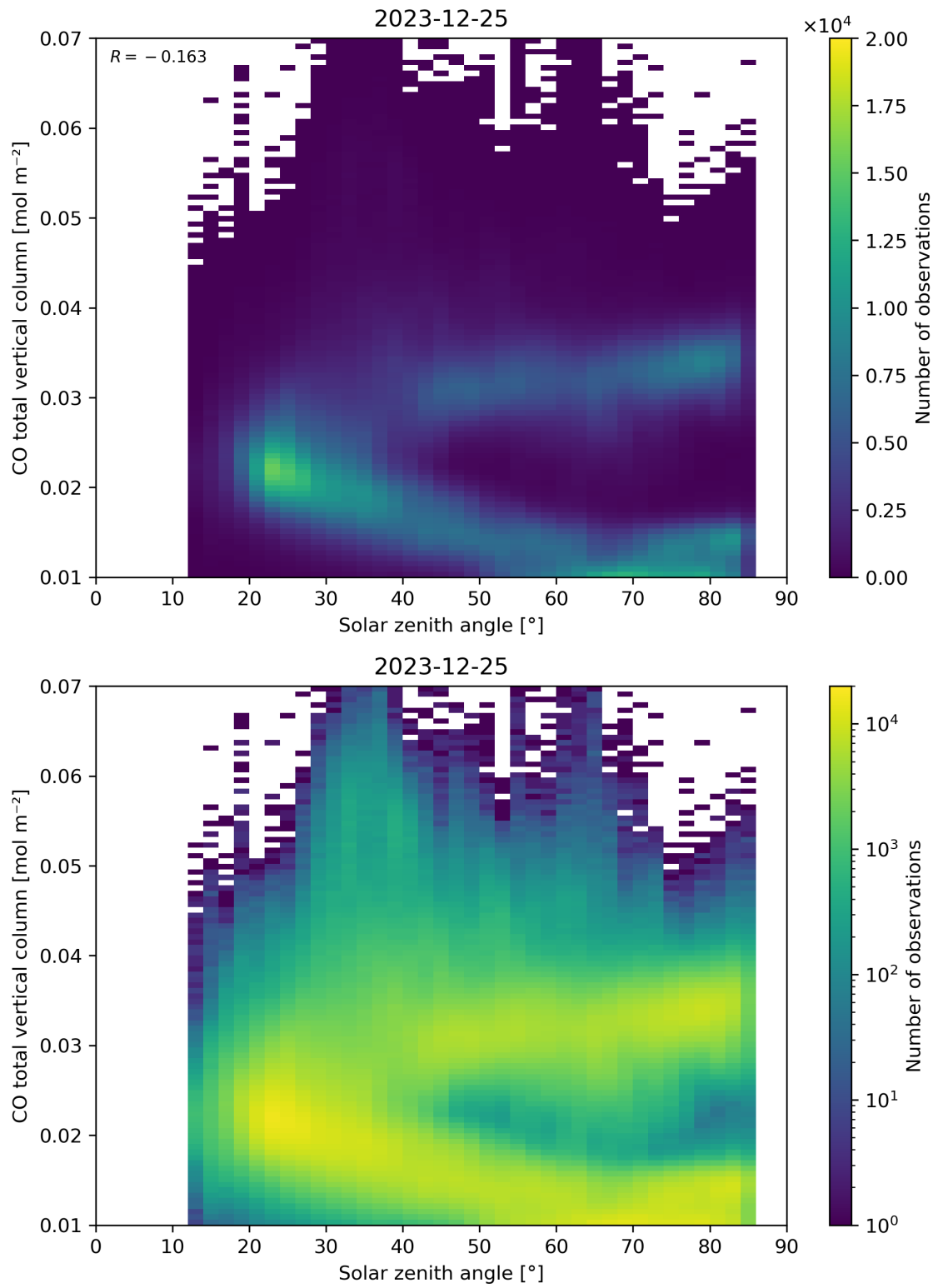
Figure 61: Scatter density plot of “Solar zenith angle” against “CO total vertical column” for 2023-12-25 to 2023-12-26.
