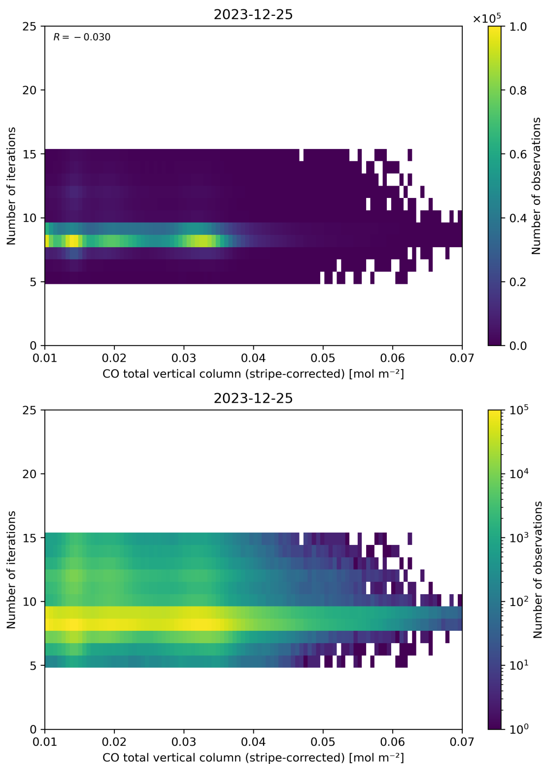
Figure 39: Scatter density plot of “CO total vertical column (stripe-corrected)” against “Number of iterations” for 2023-12-25 to 2023-12-26.
