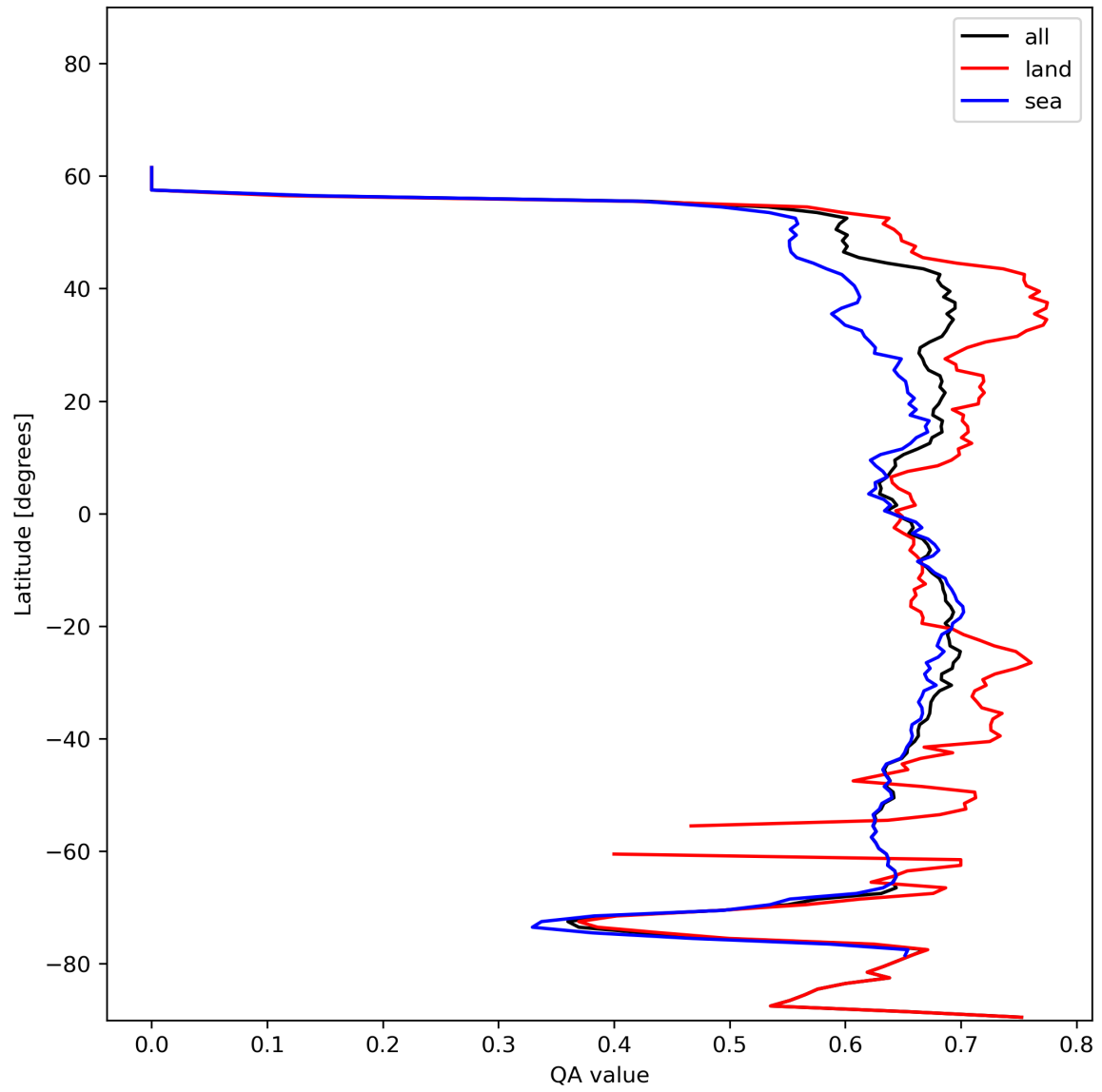
Figure 9: Zonal average of “QA value” for 2023-12-25 to 2023-12-26.
