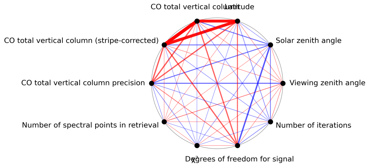
Figure 1: Map of correlation graph for 2023-12-25 to 2023-12-26.
