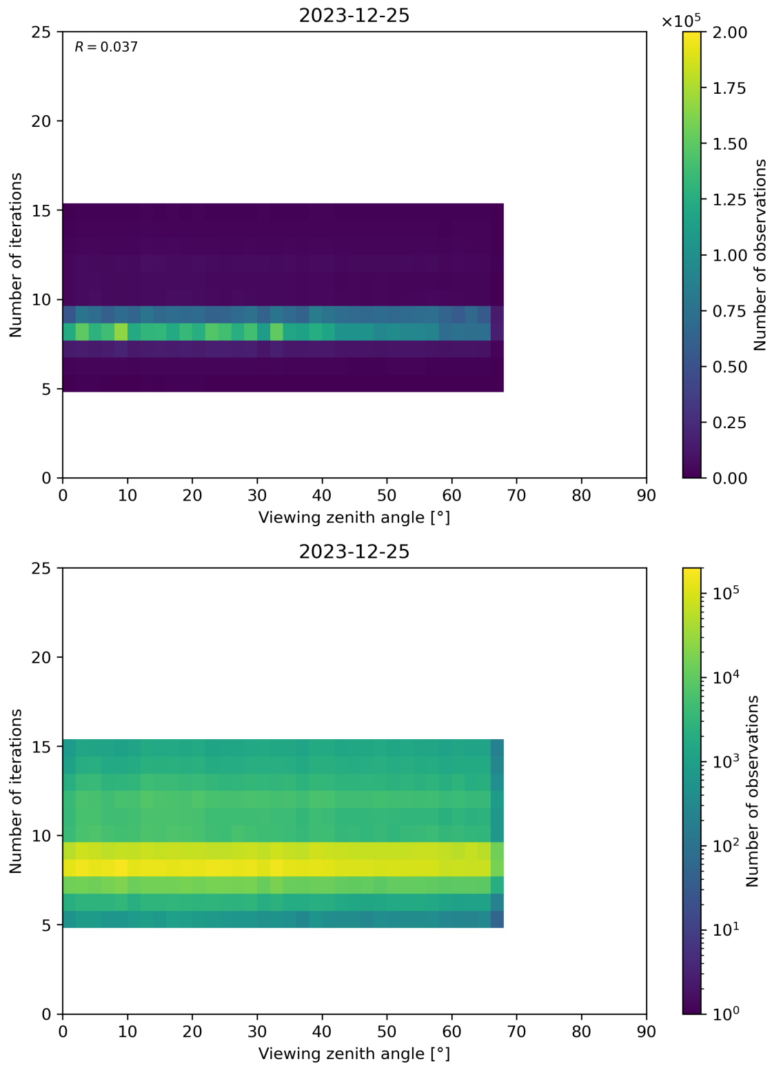
Figure 75: Scatter density plot of “Viewing zenith angle” against “Number of iterations” for 2023-12-25 to 2023-12-26.
