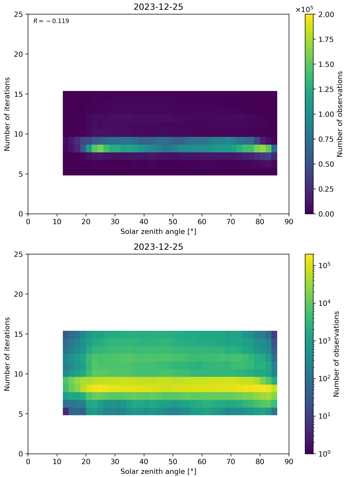
Figure 67: Scatter density plot of “Solar zenith angle” against “Number of iterations” for 2023-12-25 to 2023-12-26.
