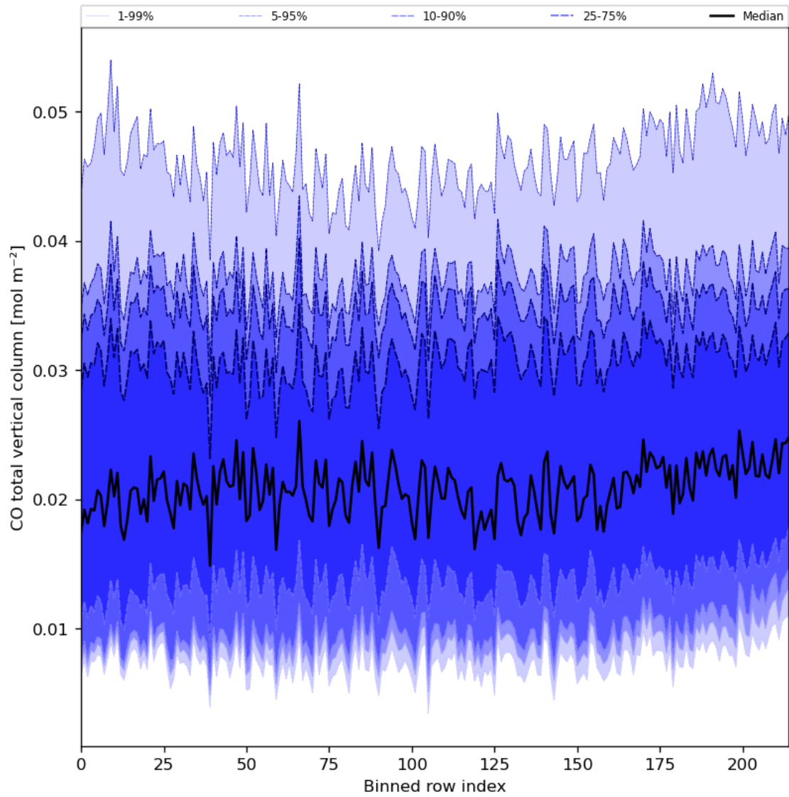
Figure 26: Along track statistics of “CO total vertical column” for 2023-12-25 to 2023-12-26
