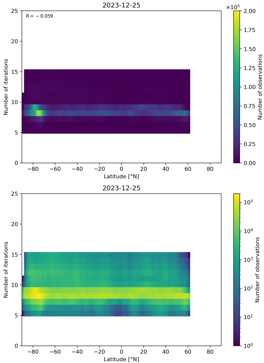
Figure 56: Scatter density plot of “Latitude” against “Number of iterations” for 2023-12-25 to 2023-12-26.
