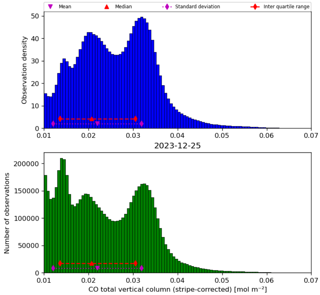
Figure 19: Histogram of “CO total vertical column (stripe-corrected)” for 2023-12-25 to 2023-12-26
