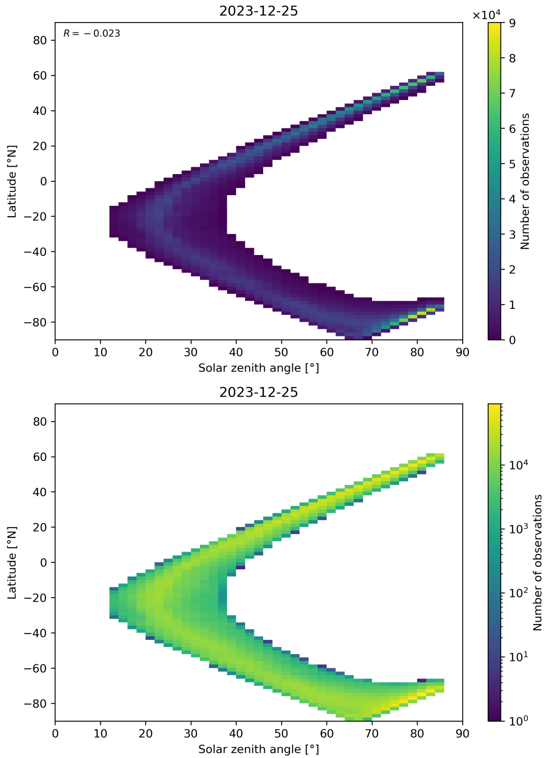
Figure 66: Scatter density plot of “Solar zenith angle” against “Latitude” for 2023-12-25 to 2023-12-26.
