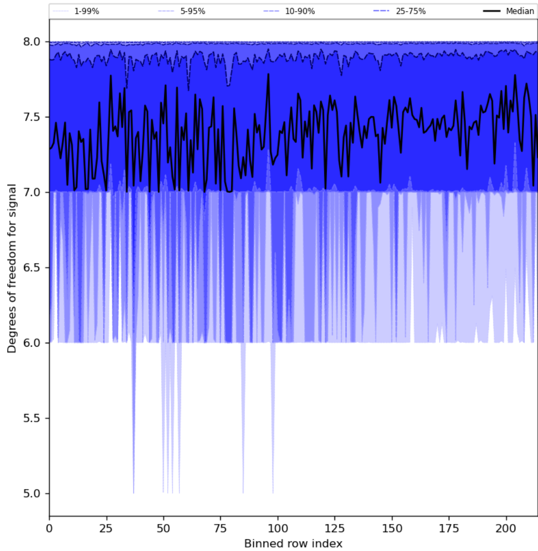
Figure 31: Along track statistics of “Degrees of freedom for signal” for 2023-12-25 to 2023-12-26
