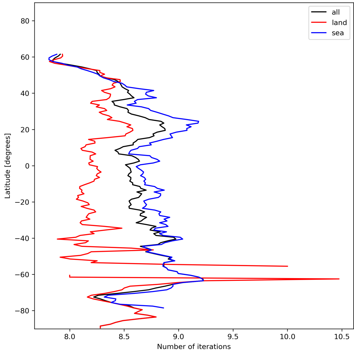
Figure 16: Zonal average of “Number of iterations” for 2023-12-25 to 2023-12-26.
