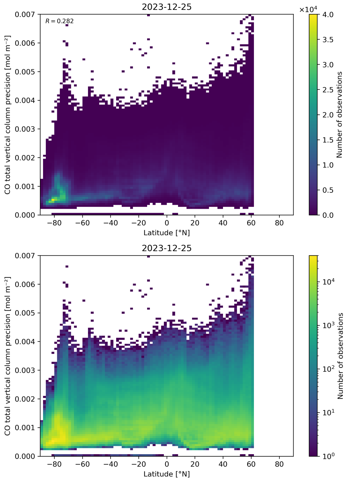
Figure 53: Scatter density plot of “Latitude” against “CO total vertical column precision” for 2023-12-25 to 2023-12-26.
