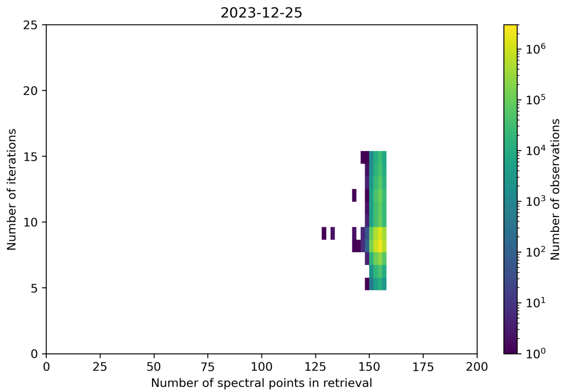
Figure 60: Scatter density plot of “Number of spectral points in retrieval” against “Number of iterations” for 2023-12-25 to 2023-12-26.
