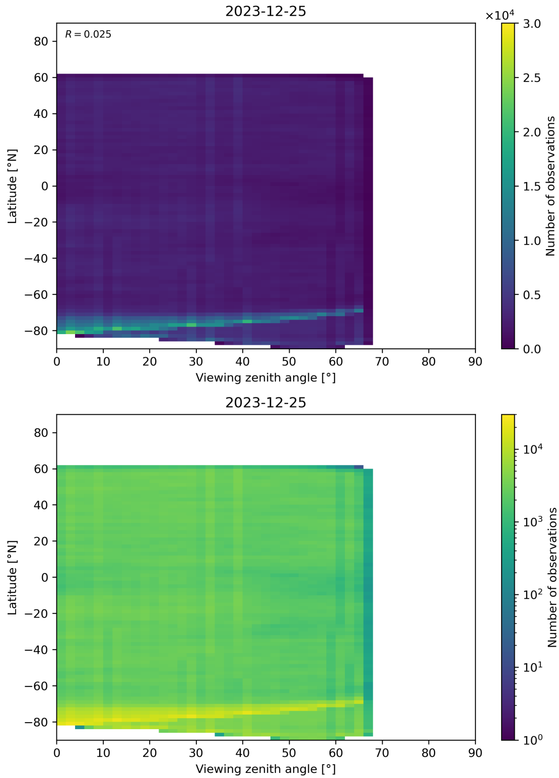
Figure 74: Scatter density plot of “Viewing zenith angle” against “Latitude” for 2023-12-25 to 2023-12-26.
