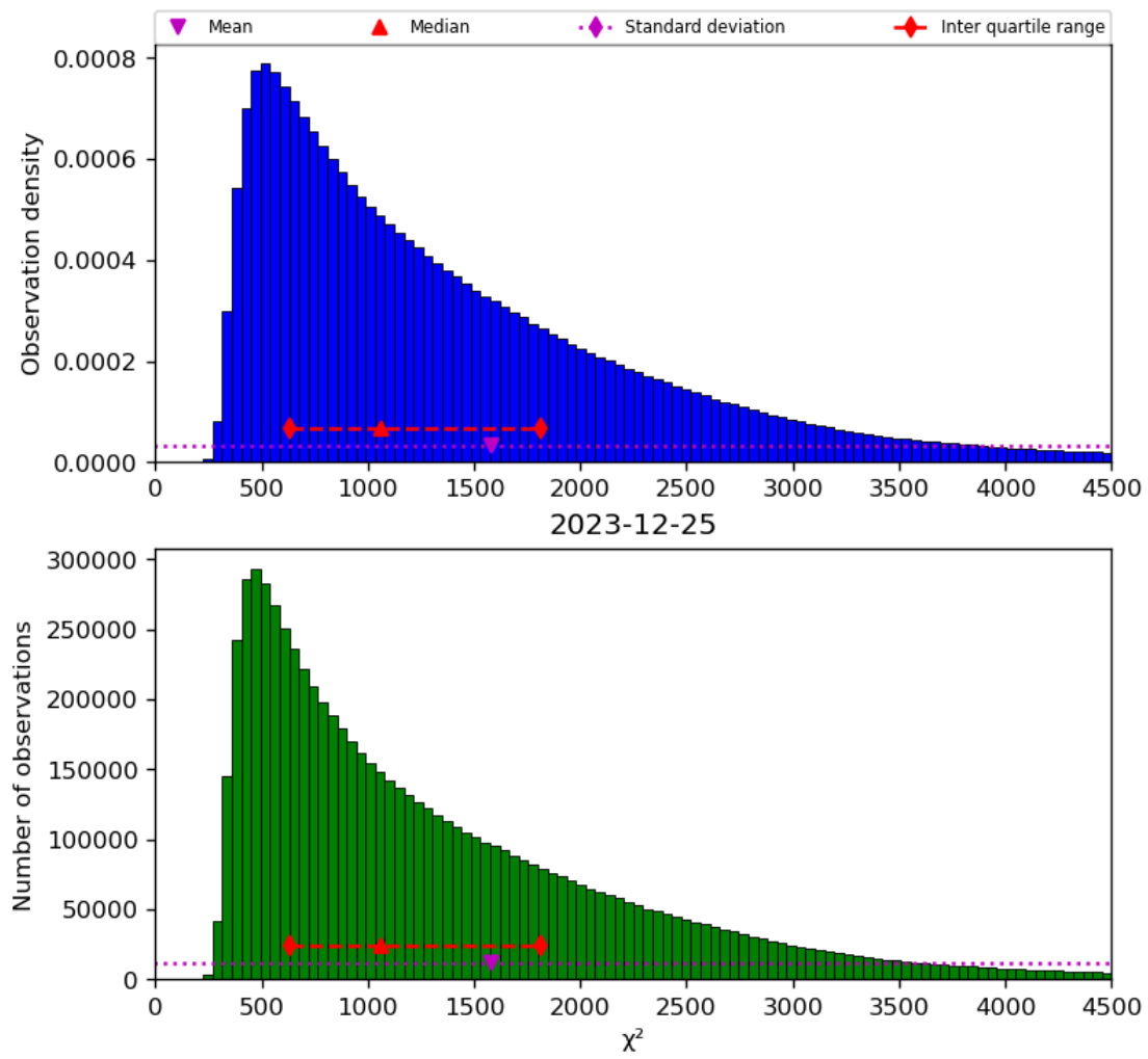
Figure 22: Histogram of “ \chi^2 ” for 2023-12-25 to 2023-12-26
