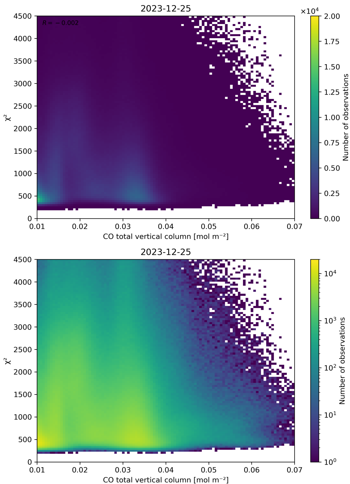
Figure 35: Scatter density plot of “CO total vertical column” against “ \chi^2 ” for 2023-12-25 to 2023-12-26.
