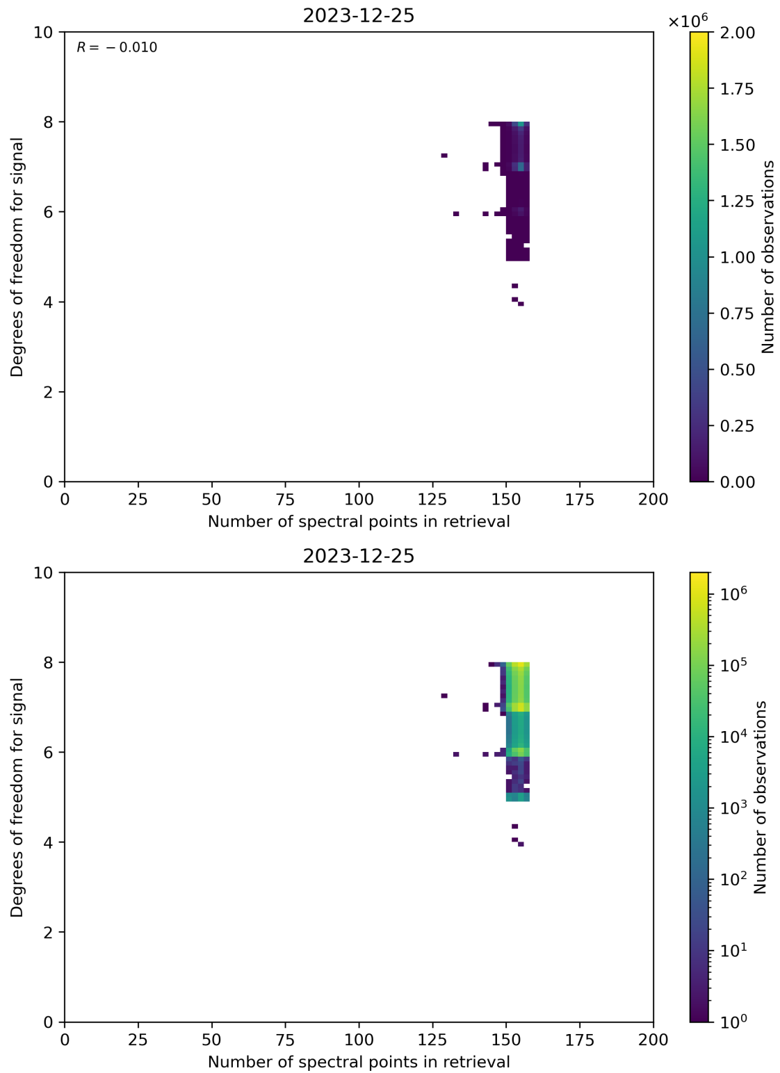
Figure 59: Scatter density plot of “Number of spectral points in retrieval” against “Degrees of freedom for signal” for 2023-12-25 to 2023-12-26.
