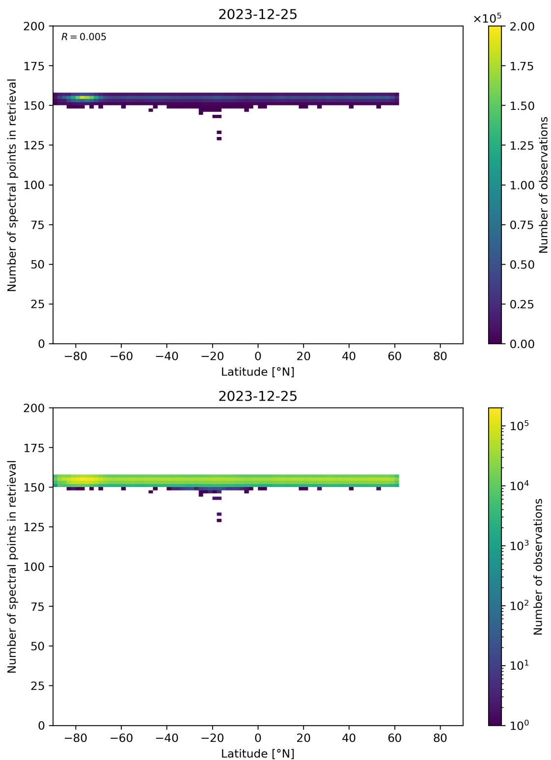
Figure 57: Scatter density plot of “Latitude” against “Number of spectral points in retrieval” for 2023-12-25 to 2023-12-26.
