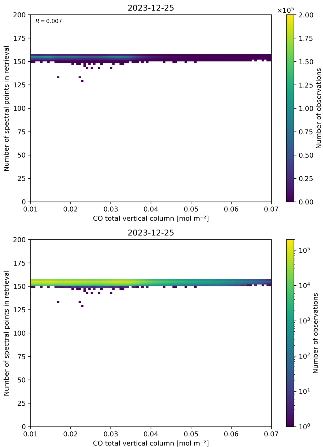
Figure 43: Scatter density plot of “CO total vertical column” against “Number of spectral points in retrieval” for 2023-12-25 to 2023-12-26.
