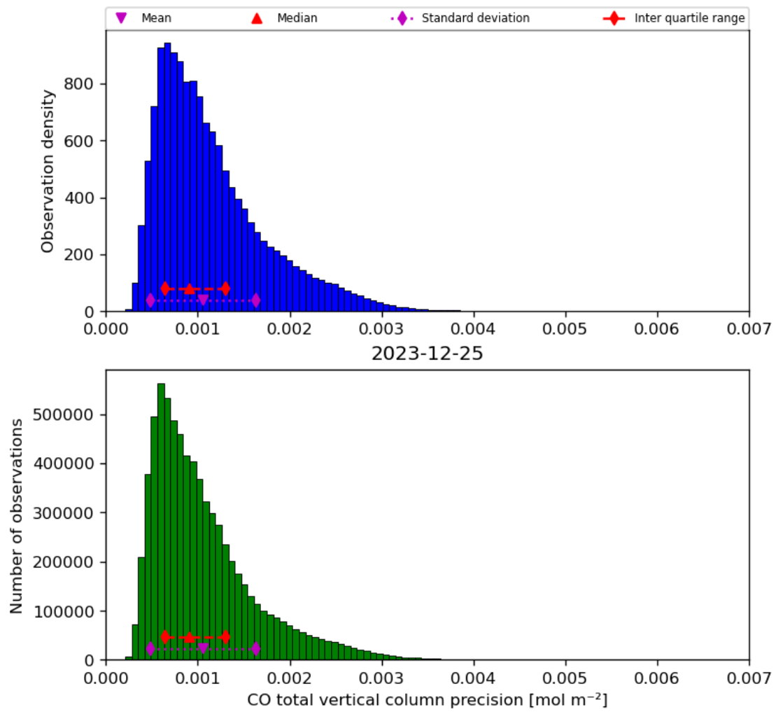
Figure 20: Histogram of “CO total vertical column precision” for 2023-12-25 to 2023-12-26
