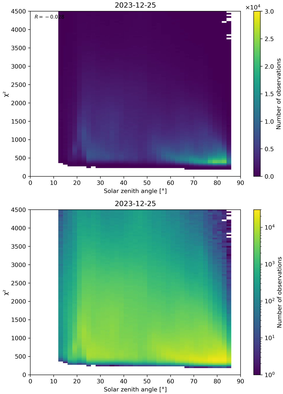
Figure 64: Scatter density plot of “Solar zenith angle” against “ \chi^2 ” for 2023-12-25 to 2023-12-26.
