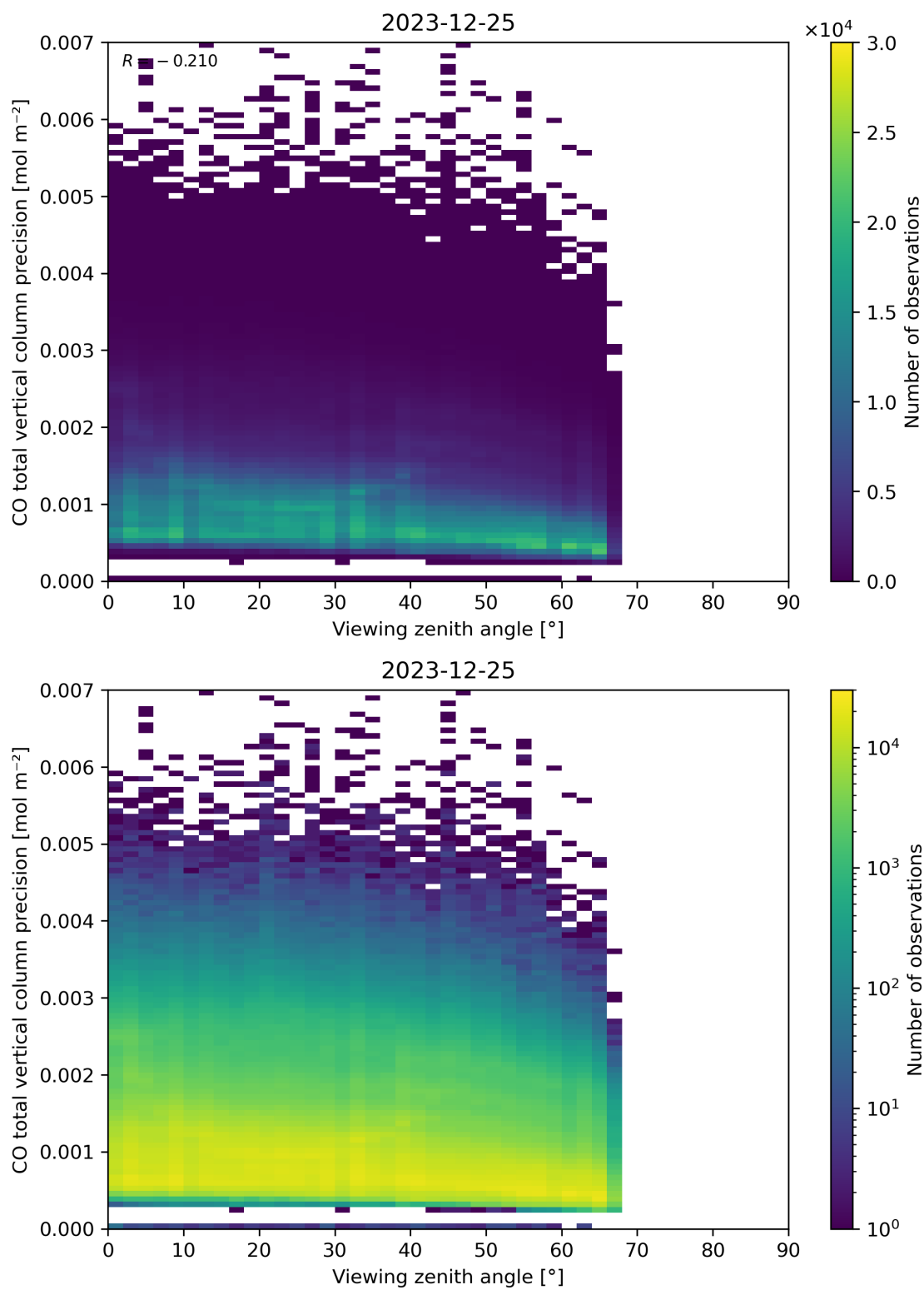
Figure 71: Scatter density plot of “Viewing zenith angle” against “CO total vertical column precision” for 2023-12-25 to 2023-12-26.
