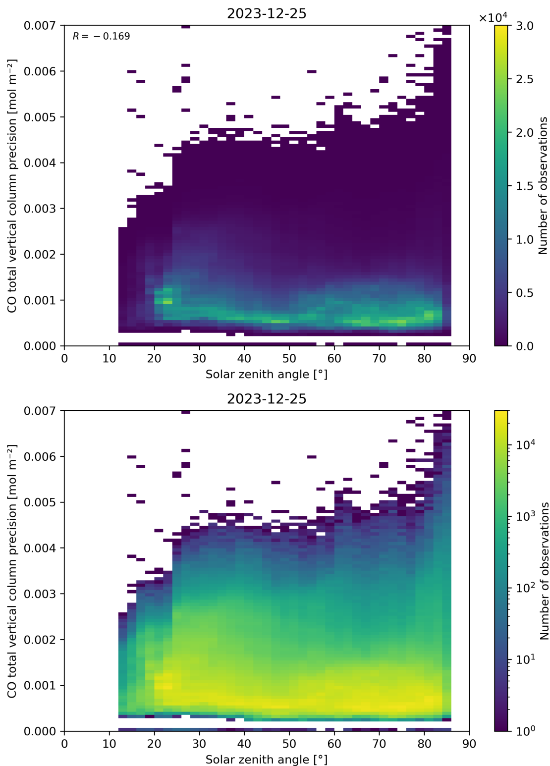
Figure 63: Scatter density plot of “Solar zenith angle” against “CO total vertical column precision” for 2023-12-25 to 2023-12-26.
