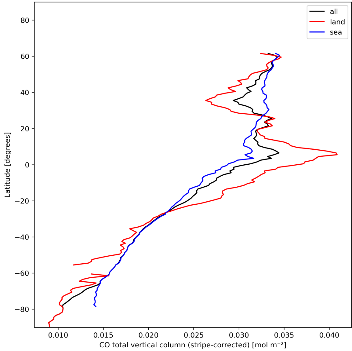
Figure 11: Zonal average of “CO total vertical column (stripe-corrected)” for 2023-12-25 to 2023-12-26.
