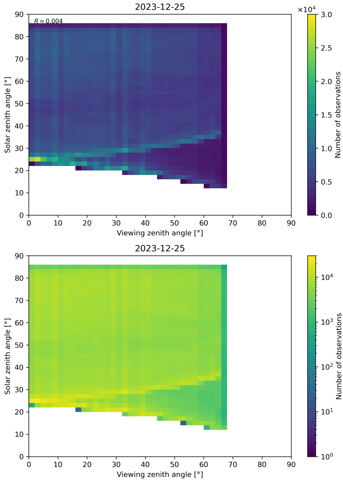
Figure 77: Scatter density plot of “Viewing zenith angle” against “Solar zenith angle” for 2023-12-25 to 2023-12-26.
