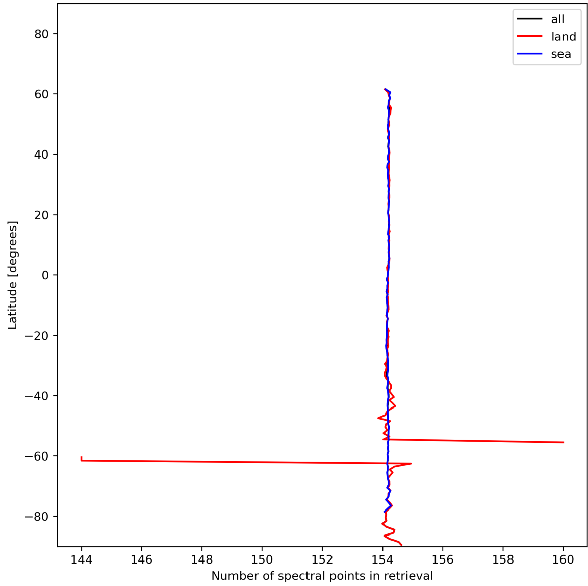
Figure 13: Zonal average of “Number of spectral points in retrieval” for 2023-12-25 to 2023-12-26.
