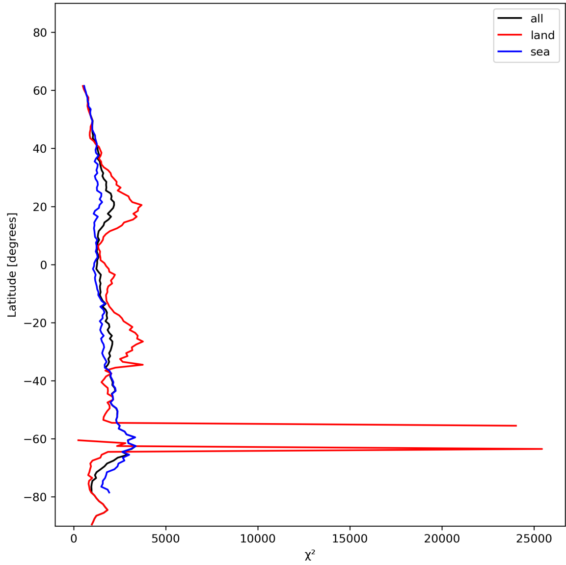
Figure 14: Zonal average of “ \chi^2 ” for 2023-12-25 to 2023-12-26.
