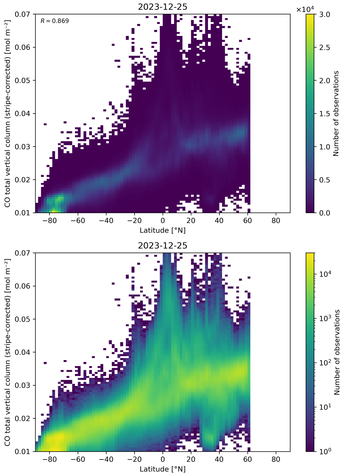
Figure 52: Scatter density plot of “Latitude” against “CO total vertical column (stripe-corrected)” for 2023-12-25 to 2023-12-26.
