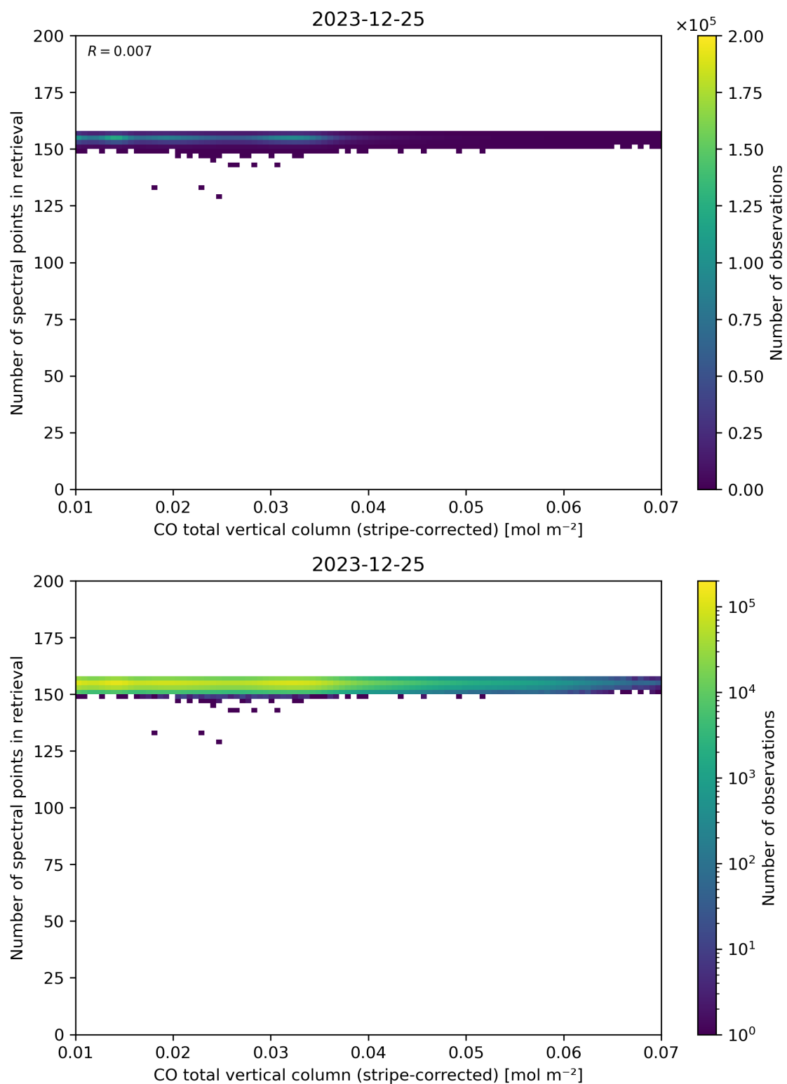
Figure 40: Scatter density plot of “CO total vertical column (stripe-corrected)” against “Number of spectral points in retrieval” for 2023-12-25 to 2023-12-26.
