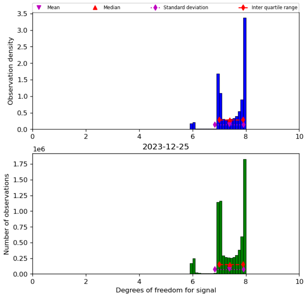
Figure 23: Histogram of “Degrees of freedom for signal” for 2023-12-25 to 2023-12-26
