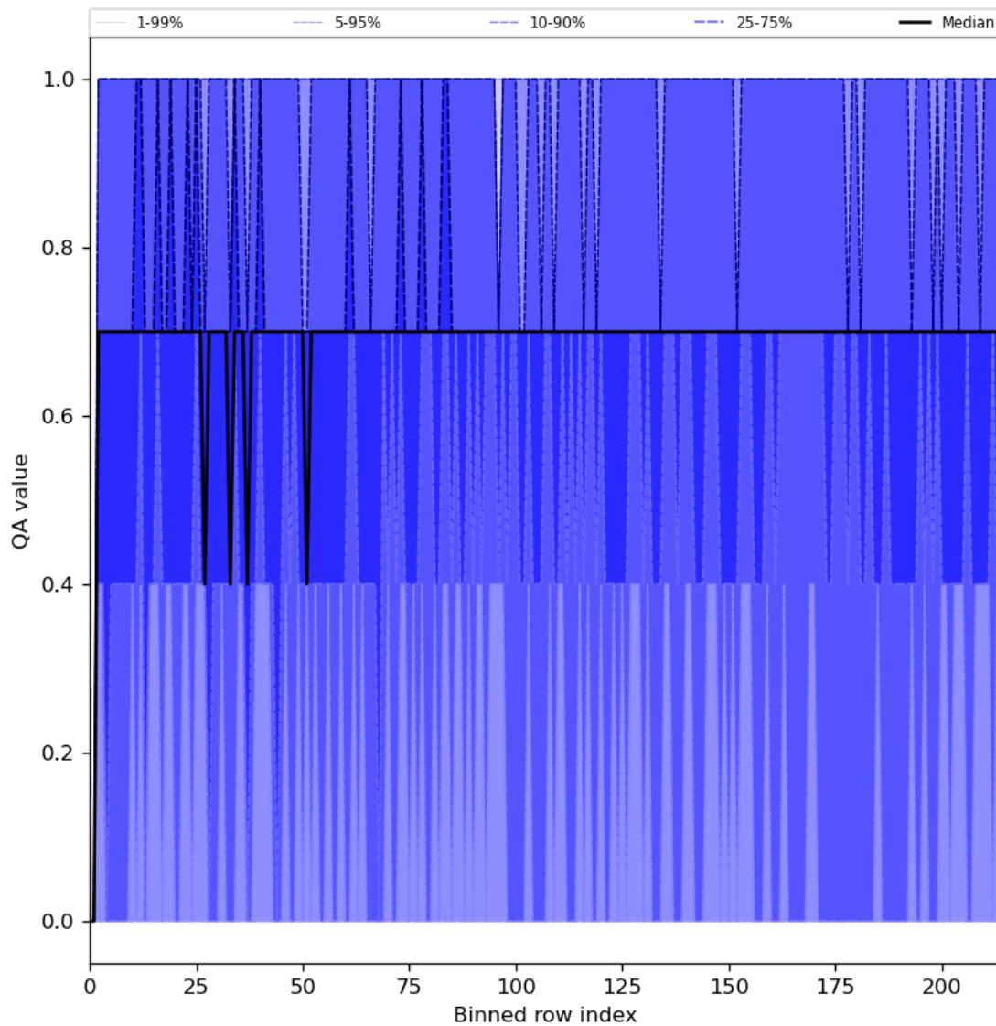
Figure 25: Along track statistics of “QA value” for 2023-12-25 to 2023-12-26
