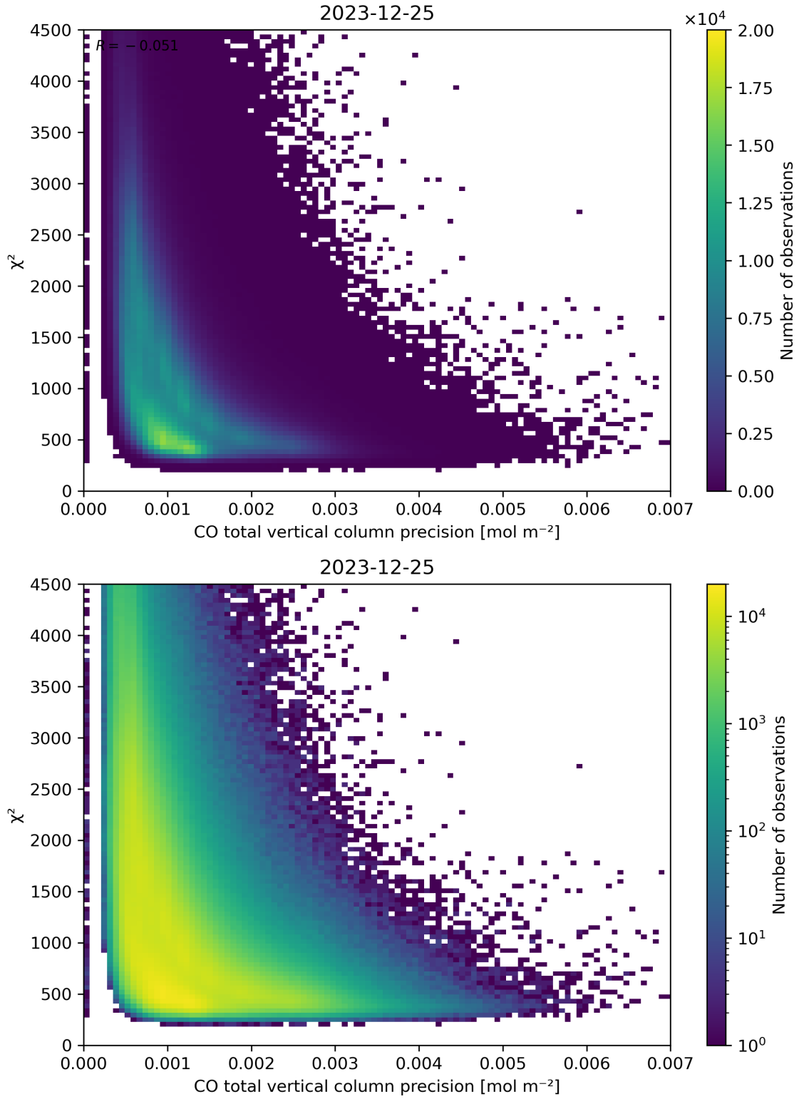
Figure 44: Scatter density plot of “CO total vertical column precision” against “ \chi^2 ” for 2023-12-25 to 2023-12-26.
