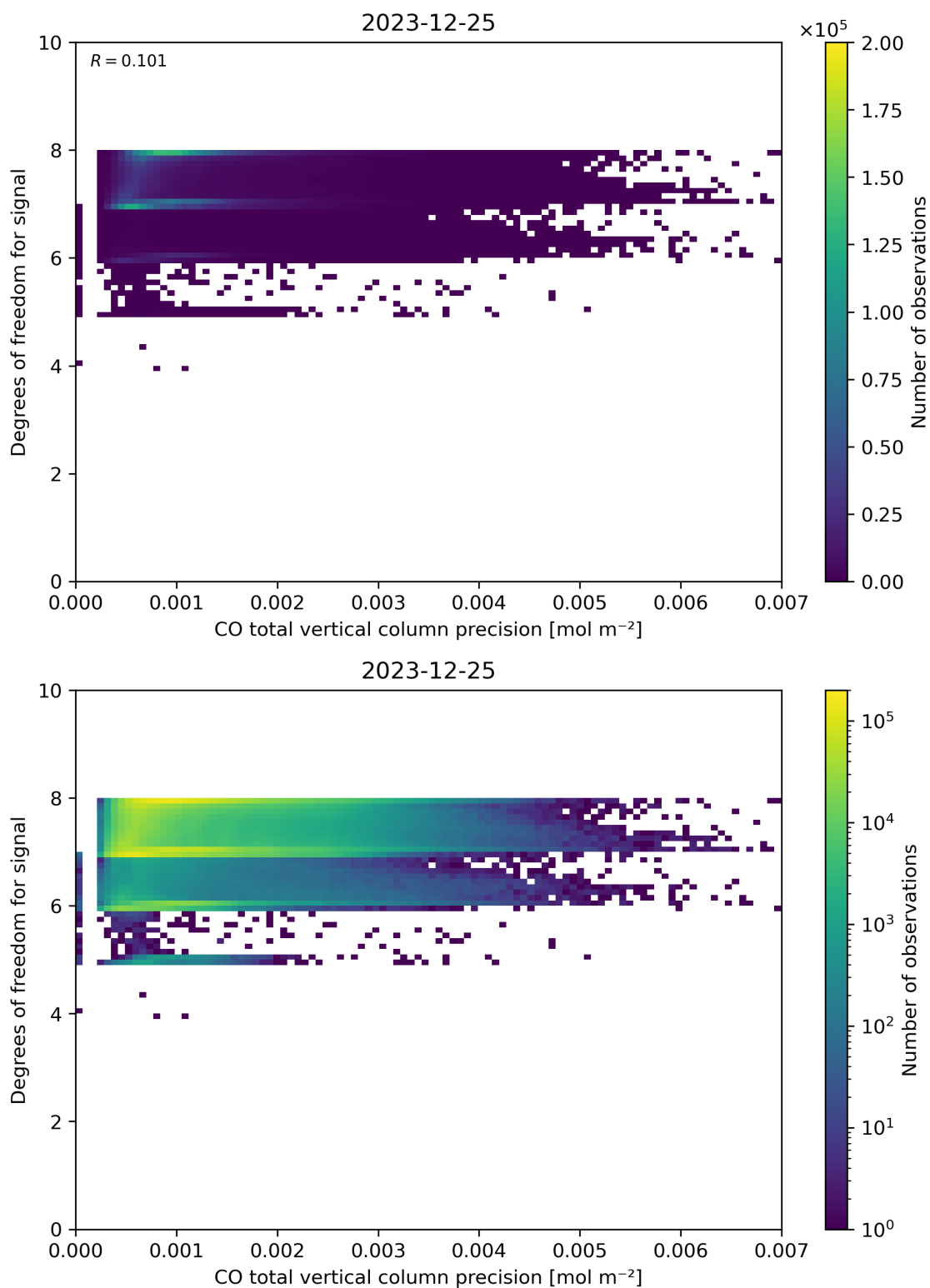
Figure 45: Scatter density plot of “CO total vertical column precision” against “Degrees of freedom for signal” for 2023-12-25 to 2023-12-26.
