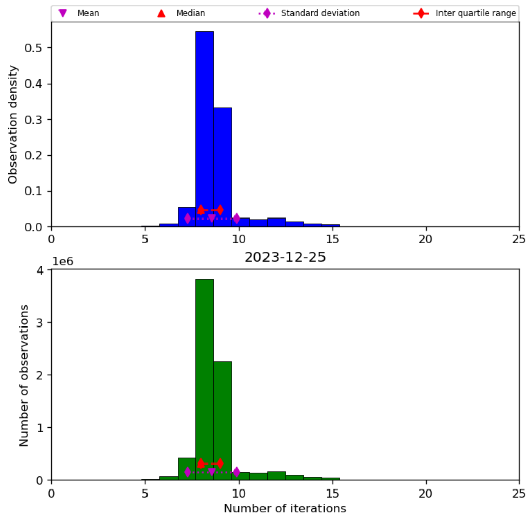
Figure 24: Histogram of “Number of iterations” for 2023-12-25 to 2023-12-26
