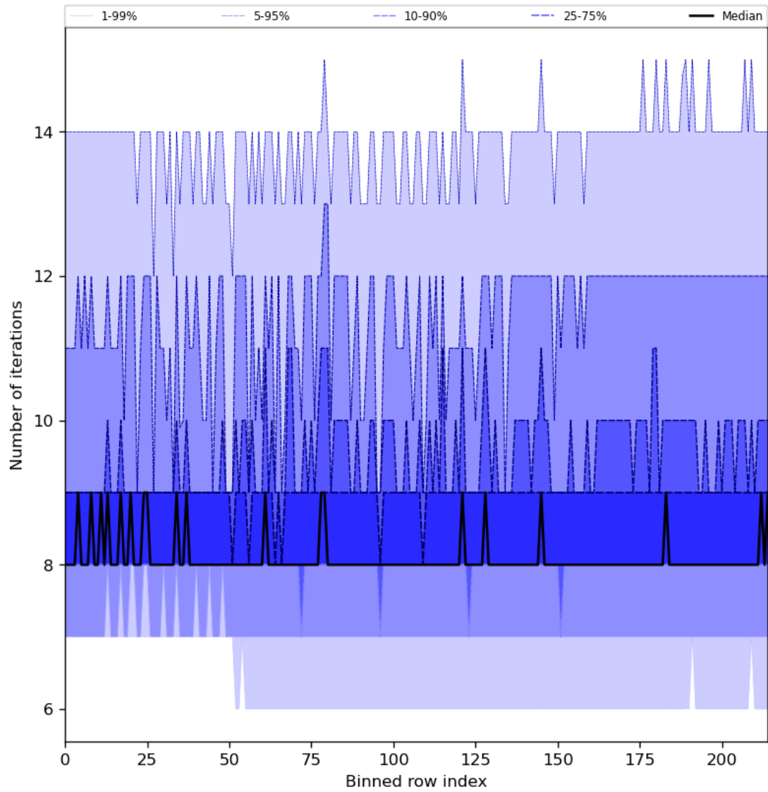
Figure 32: Along track statistics of “Number of iterations” for 2023-12-25 to 2023-12-26
