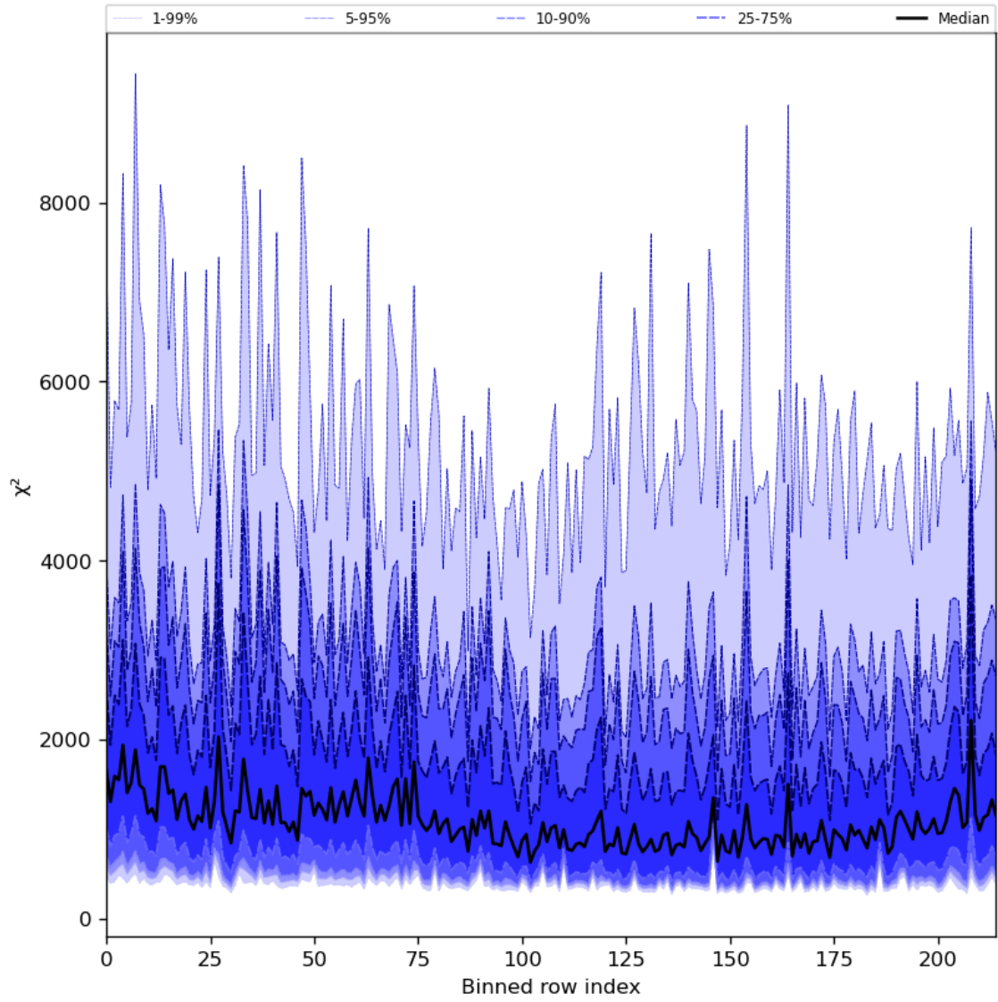
Figure 30: Along track statistics of “ \chi^2 ” for 2023-12-25 to 2023-12-26
