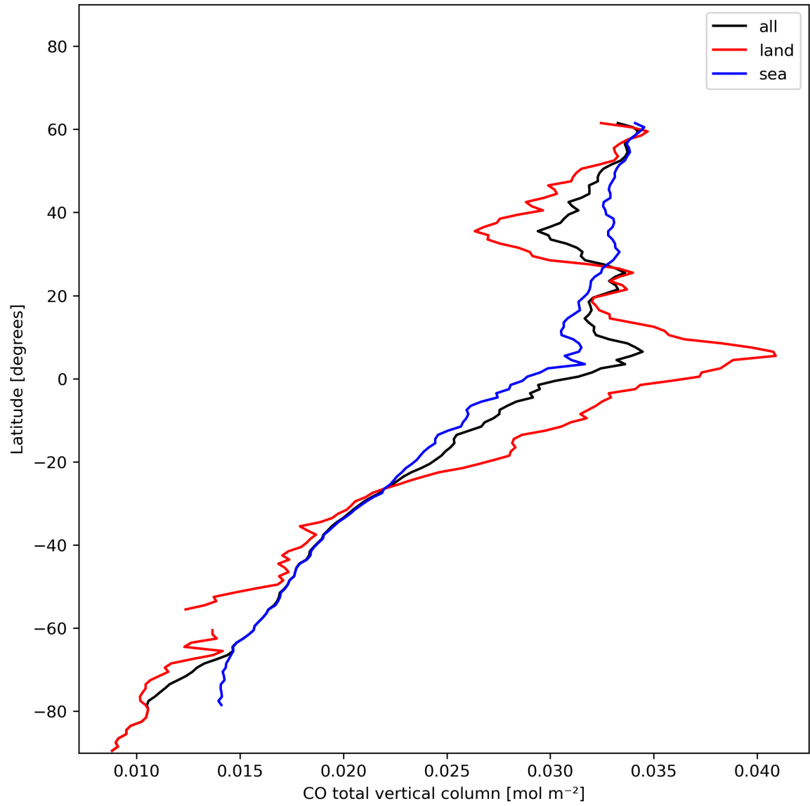
Figure 10: Zonal average of “CO total vertical column” for 2023-12-25 to 2023-12-26.
