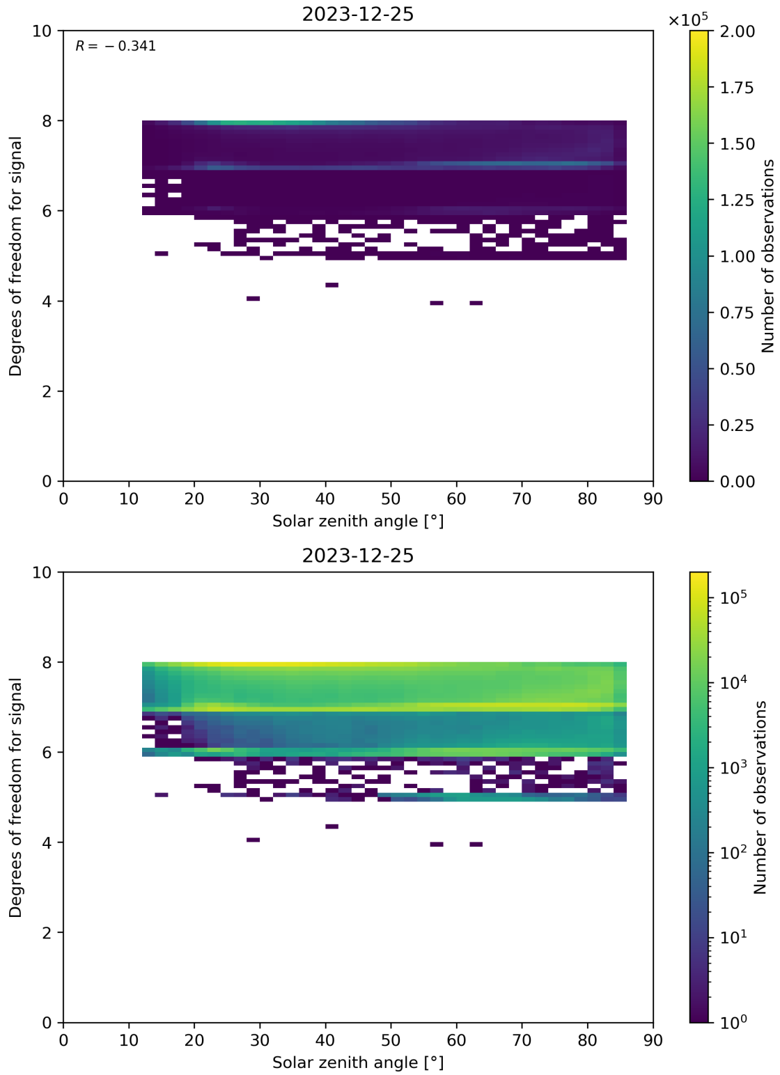
Figure 65: Scatter density plot of “Solar zenith angle” against “Degrees of freedom for signal” for 2023-12-25 to 2023-12-26.
