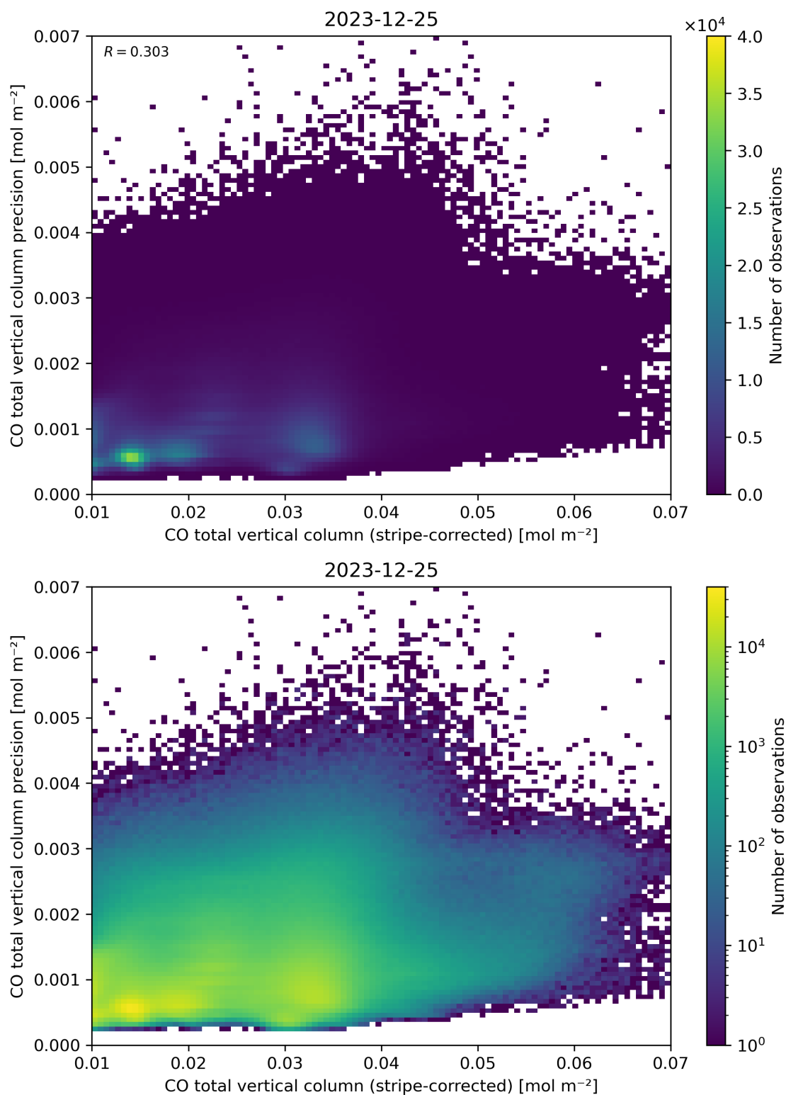
Figure 36: Scatter density plot of “CO total vertical column (stripe-corrected)” against “CO total vertical column precision” for 2023-12-25 to 2023-12-26.
