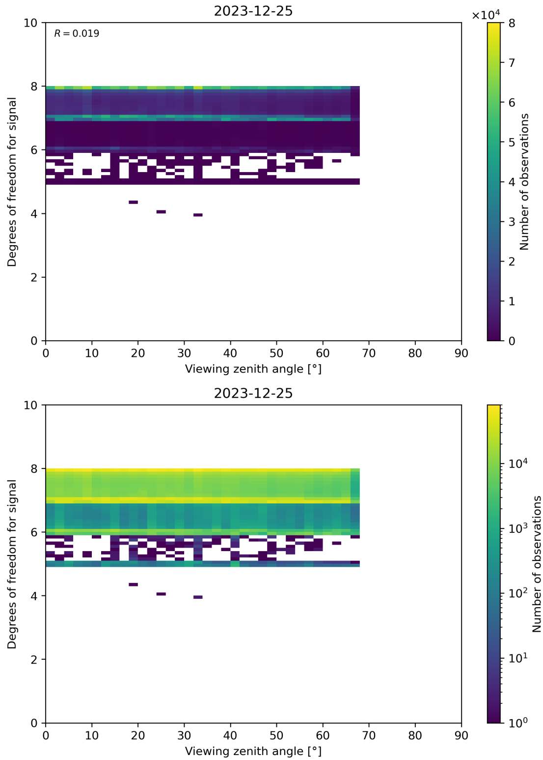
Figure 73: Scatter density plot of “Viewing zenith angle” against “Degrees of freedom for signal” for 2023-12-25 to 2023-12-26.
