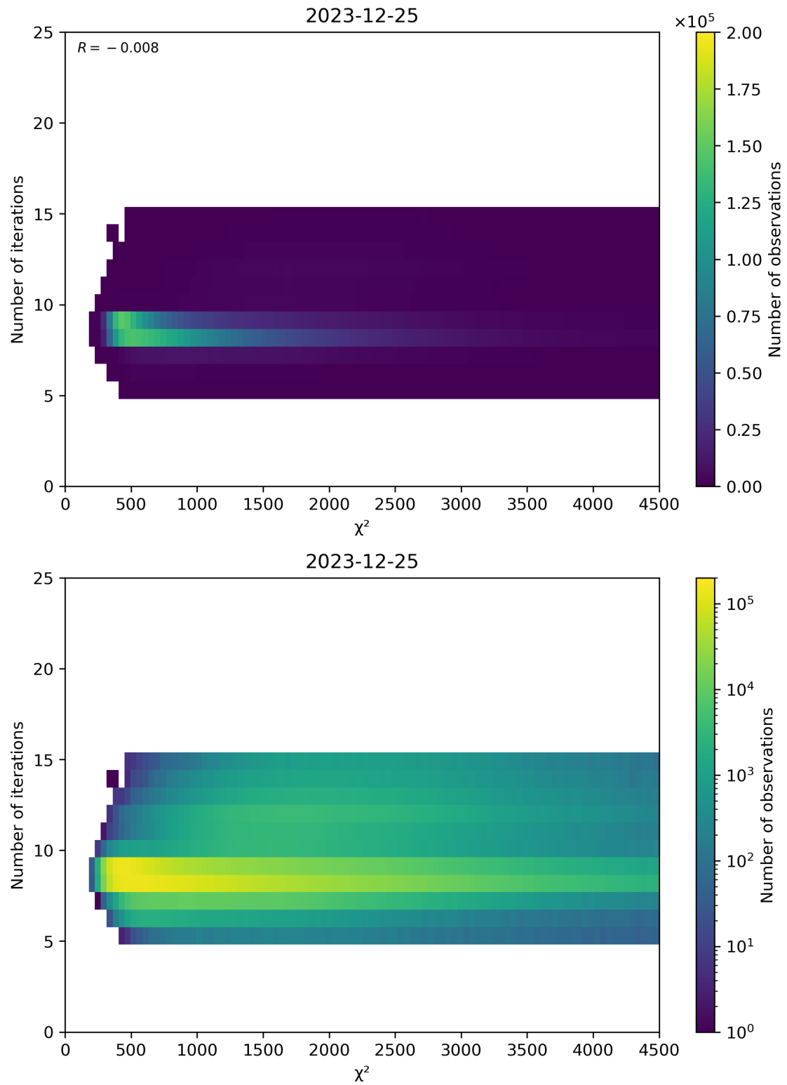
Figure 49: Scatter density plot of “ \chi^2 ” against “Number of iterations” for 2023-12-25 to 2023-12-26.
