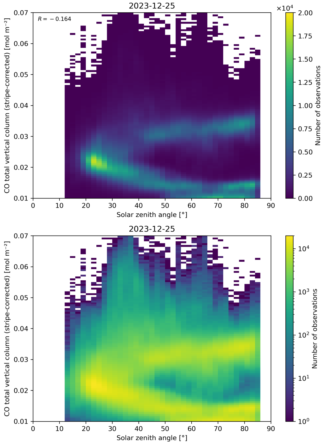
Figure 62: Scatter density plot of “Solar zenith angle” against “CO total vertical column (stripe-corrected)” for 2023-12-25 to 2023-12-26.
