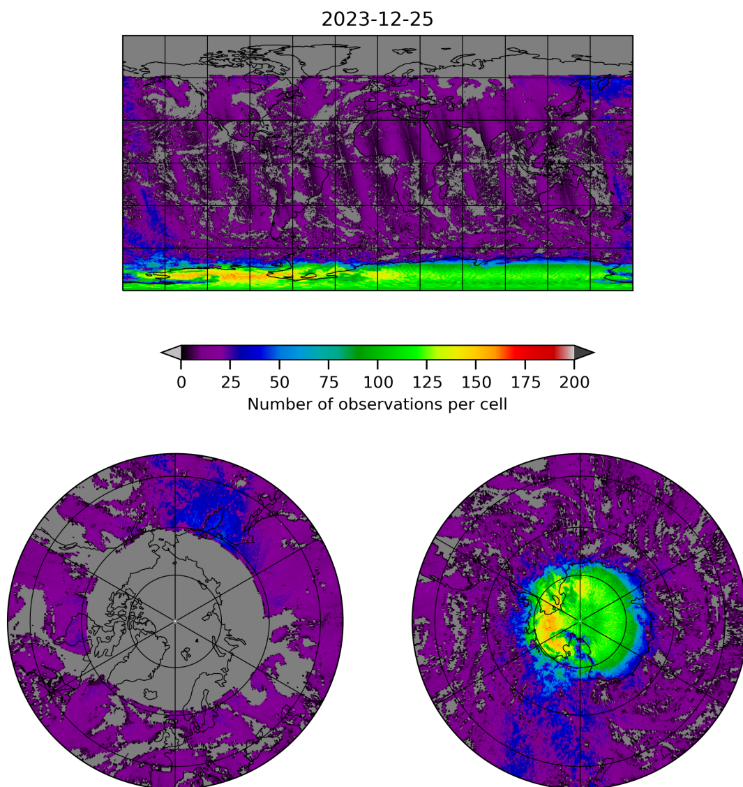
Figure 8: Map of the number of observations for 2023-12-25 to 2023-12-26
