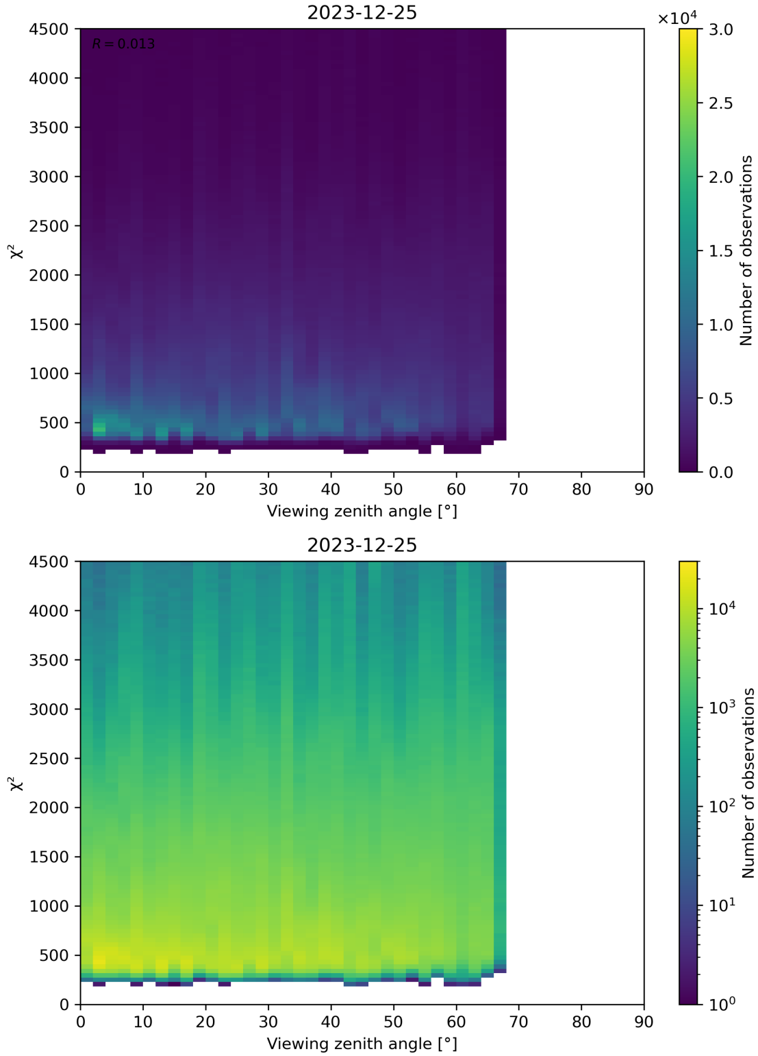
Figure 72: Scatter density plot of “Viewing zenith angle” against “ \chi^2 ” for 2023-12-25 to 2023-12-26.
