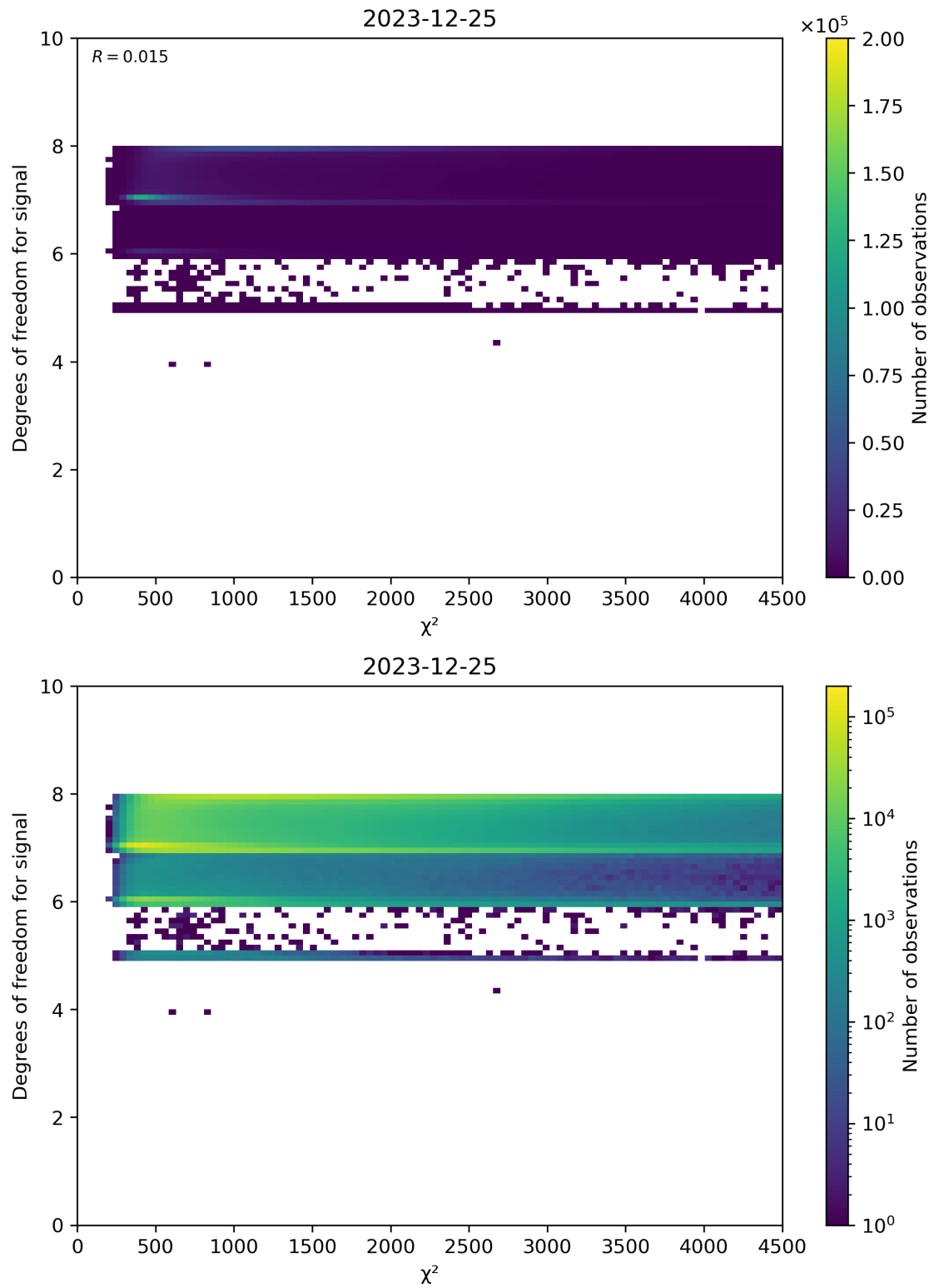
Figure 48: Scatter density plot of “ \chi^2 ” against “Degrees of freedom for signal” for 2023-12-25 to 2023-12-26.
