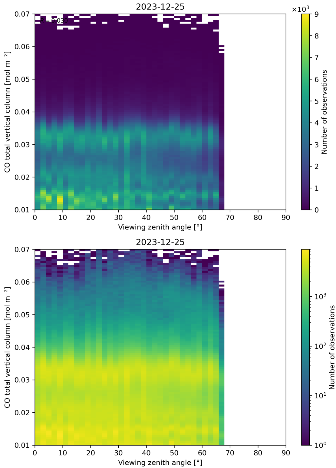
Figure 69: Scatter density plot of “Viewing zenith angle” against “CO total vertical column” for 2023-12-25 to 2023-12-26.
