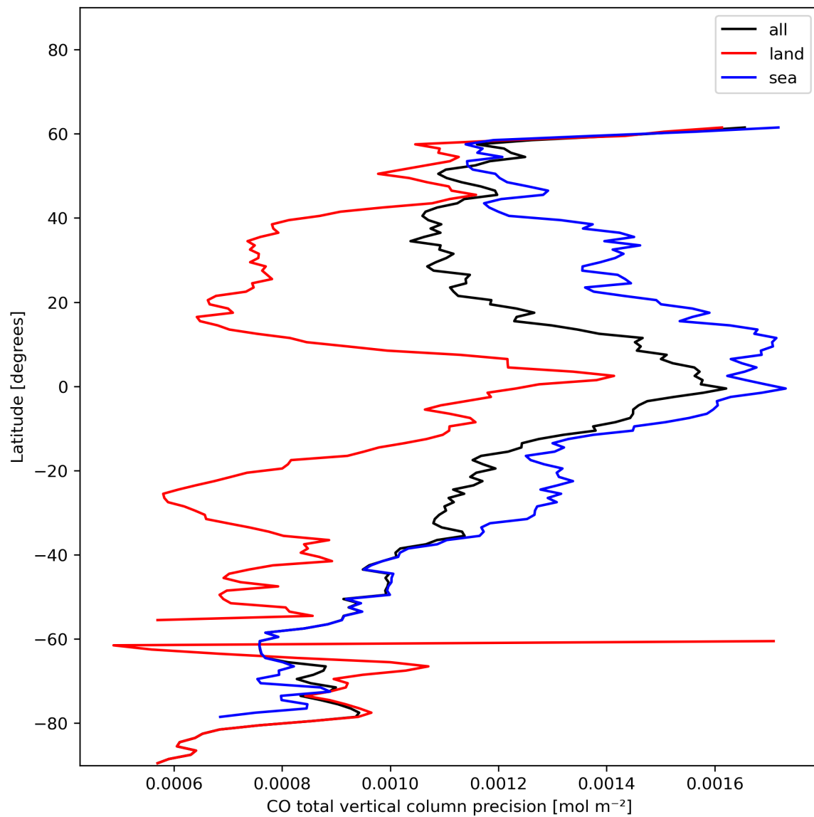
Figure 12: Zonal average of “CO total vertical column precision” for 2023-12-25 to 2023-12-26.
