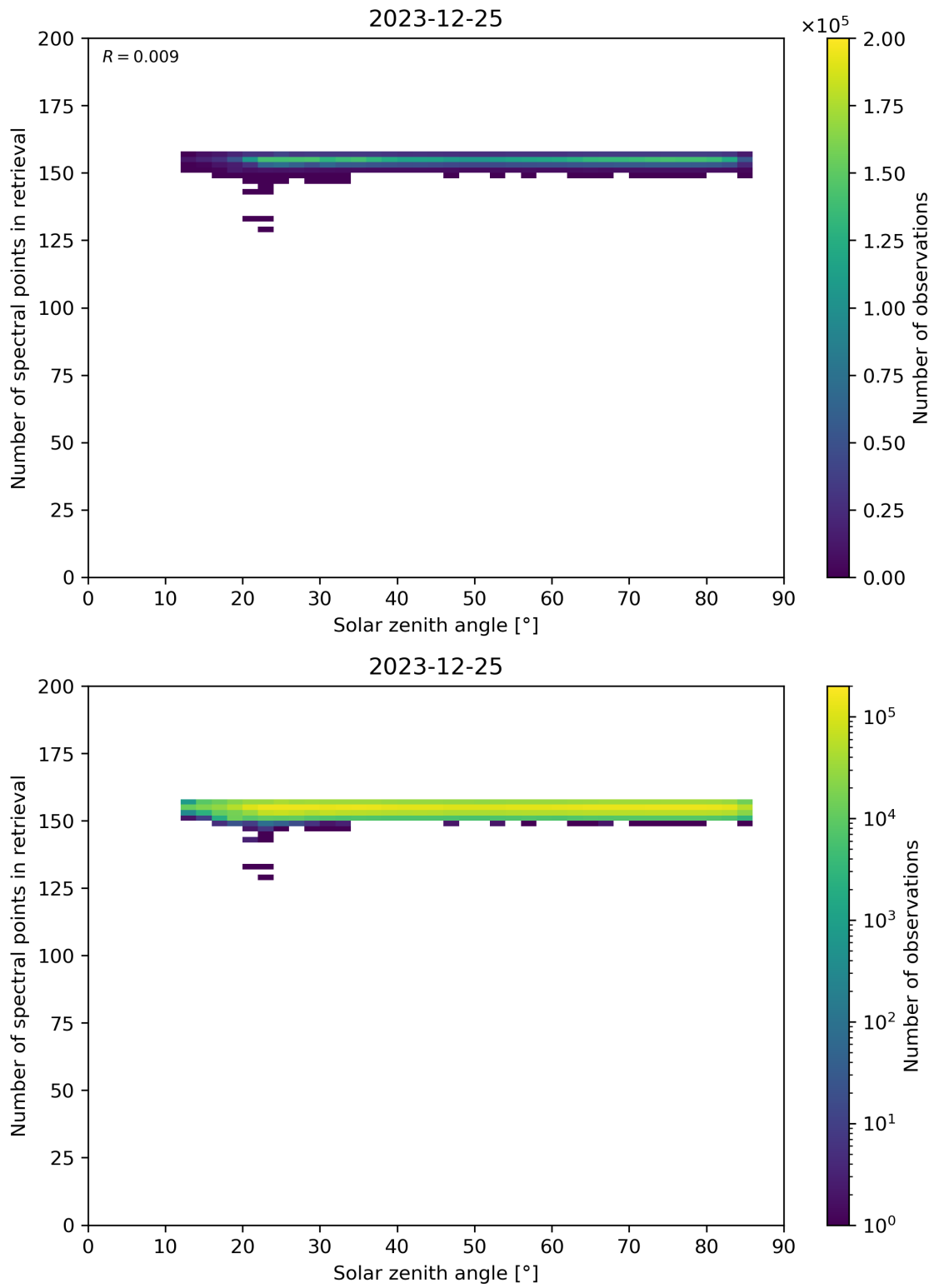
Figure 68: Scatter density plot of “Solar zenith angle” against “Number of spectral points in retrieval” for 2023-12-25 to 2023-12-26.
