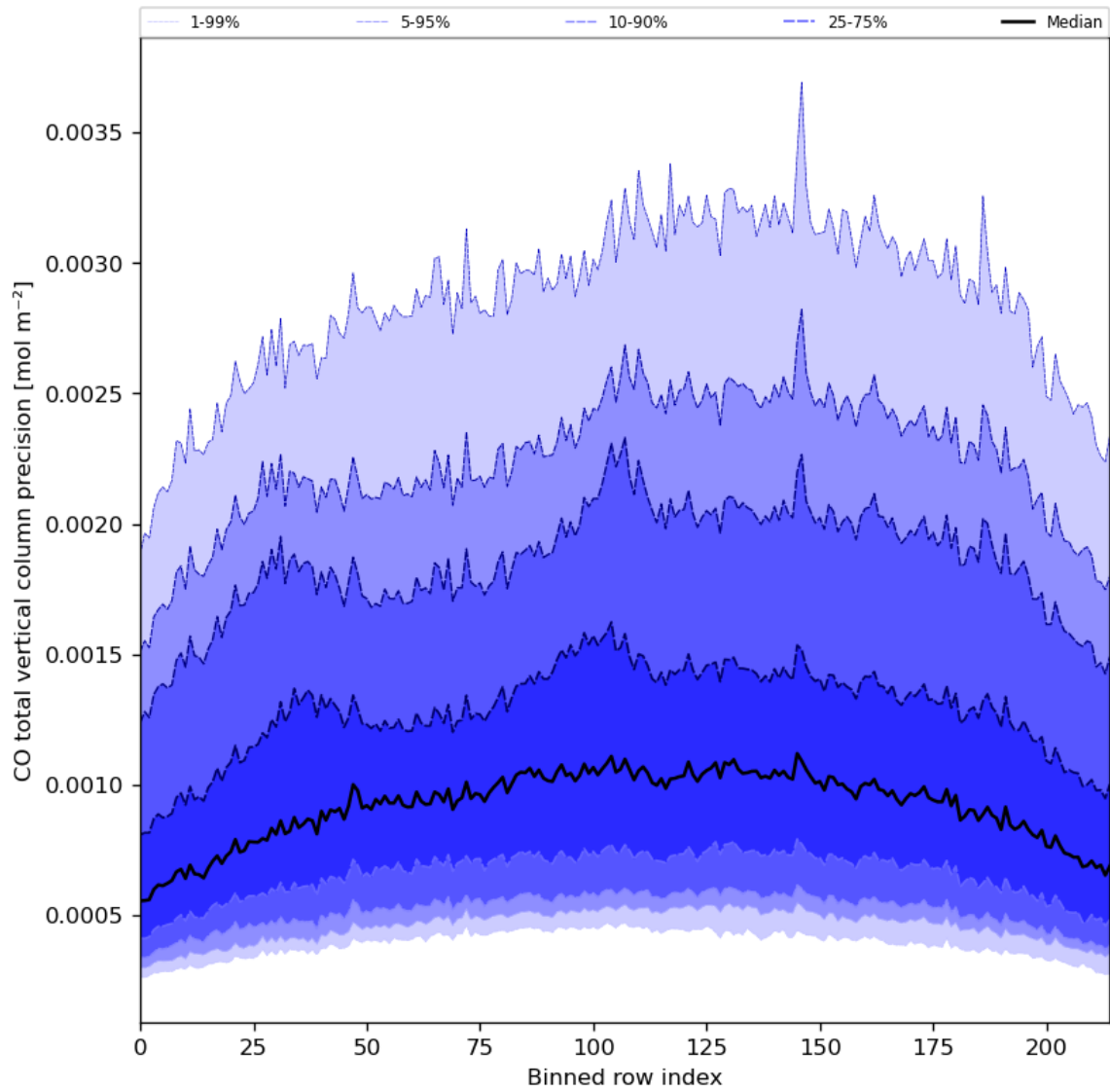
Figure 28: Along track statistics of “CO total vertical column precision” for 2023-12-25 to 2023-12-26
