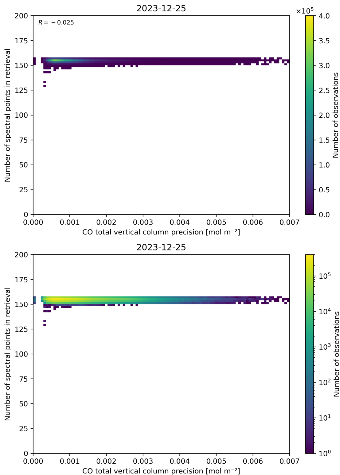
Figure 47: Scatter density plot of “CO total vertical column precision” against “Number of spectral points in retrieval” for 2023-12-25 to 2023-12-26.
