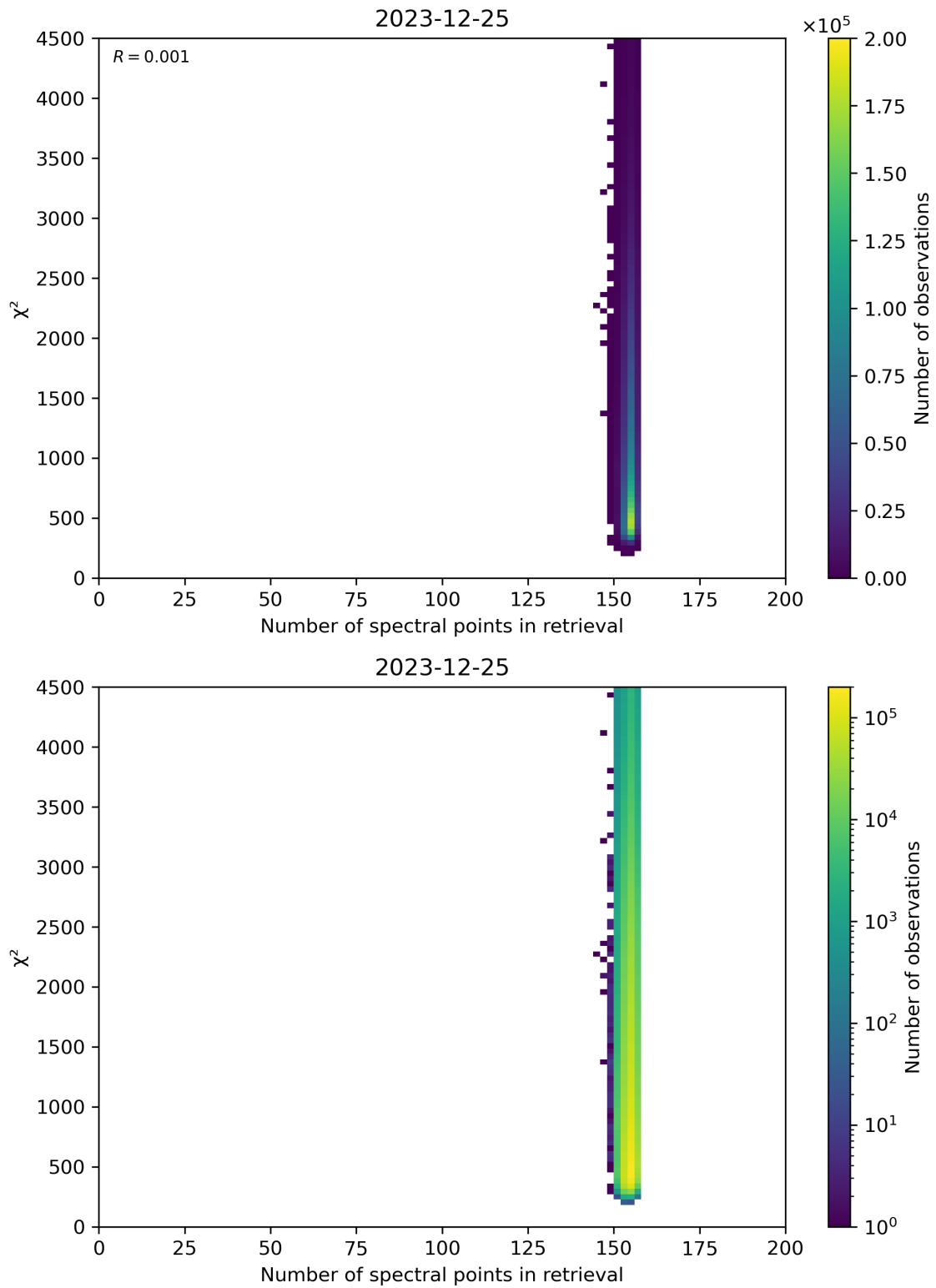
Figure 58: Scatter density plot of “Number of spectral points in retrieval” against “ \chi^2 ” for 2023-12-25 to 2023-12-26.
