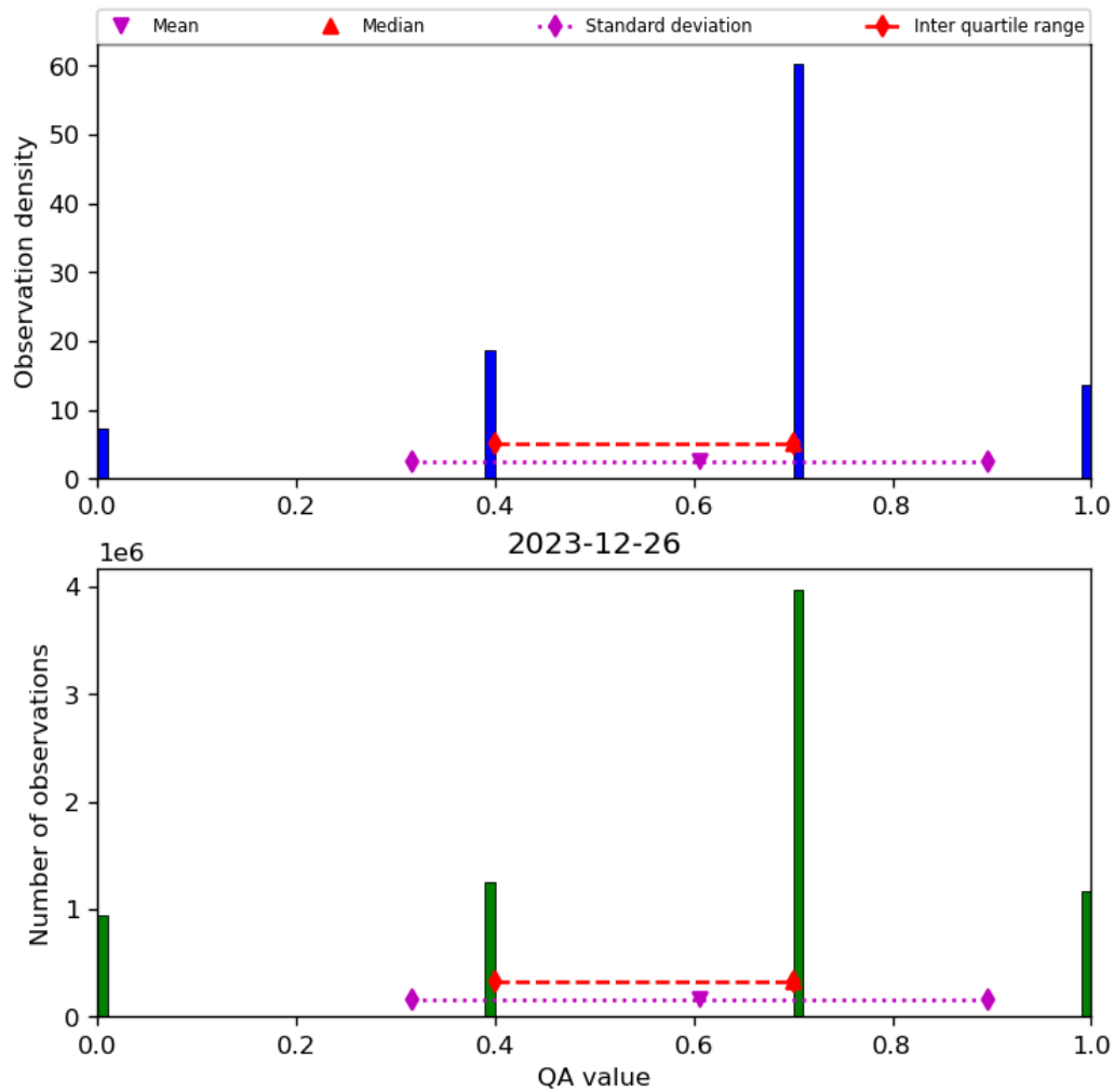
Figure 17: Histogram of “QA value” for 2023-12-25 to 2023-12-27
