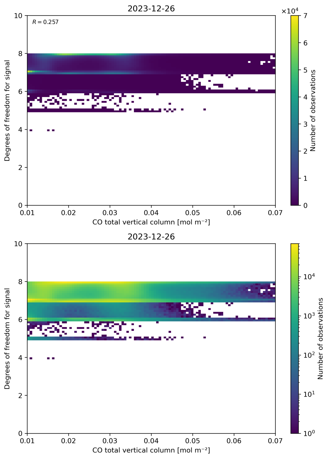
Figure 41: Scatter density plot of “CO total vertical column” against “Degrees of freedom for signal” for 2023-12-25 to 2023-12-27.
