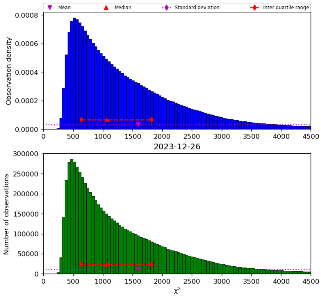
Figure 22: Histogram of “ \chi^2 ” for 2023-12-25 to 2023-12-27
