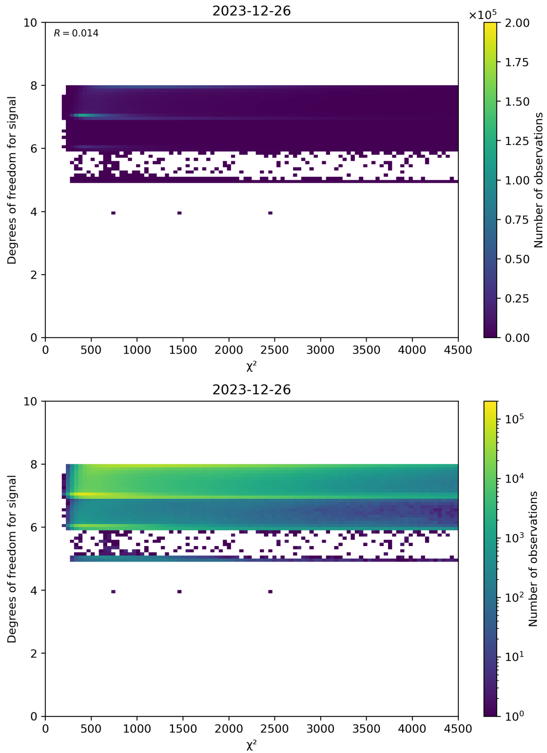
Figure 48: Scatter density plot of “ \chi^2 ” against “Degrees of freedom for signal” for 2023-12-25 to 2023-12-27.
