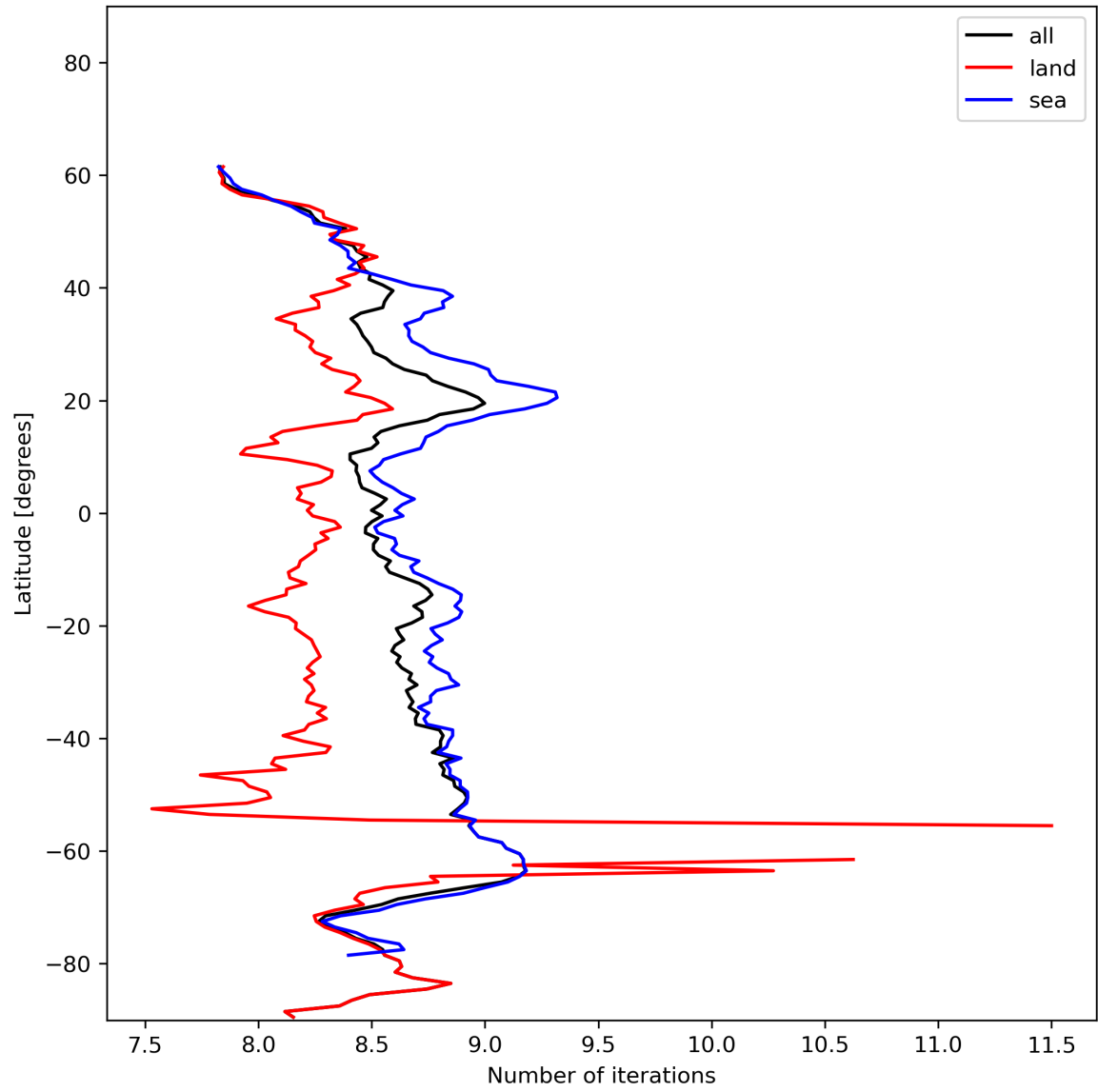
Figure 16: Zonal average of “Number of iterations” for 2023-12-25 to 2023-12-27.
