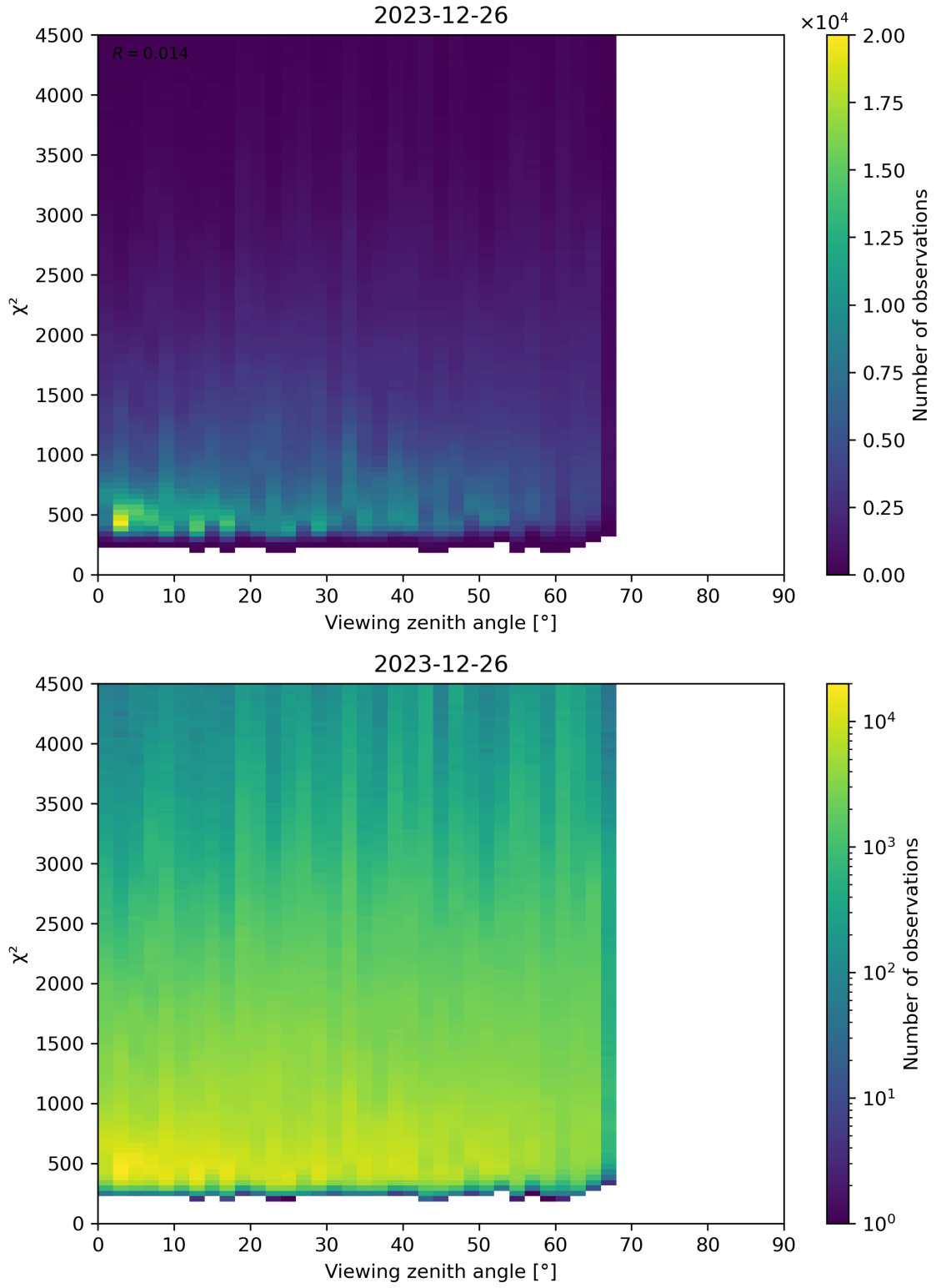
Figure 72: Scatter density plot of “Viewing zenith angle” against “ \chi^2 ” for 2023-12-25 to 2023-12-27.
