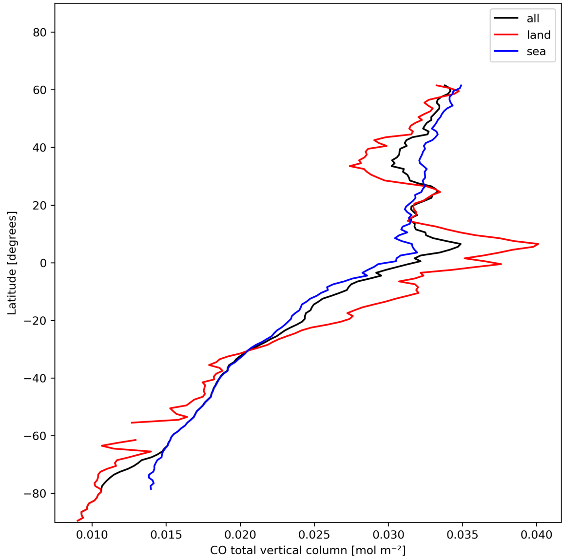
Figure 10: Zonal average of “CO total vertical column” for 2023-12-25 to 2023-12-27.
