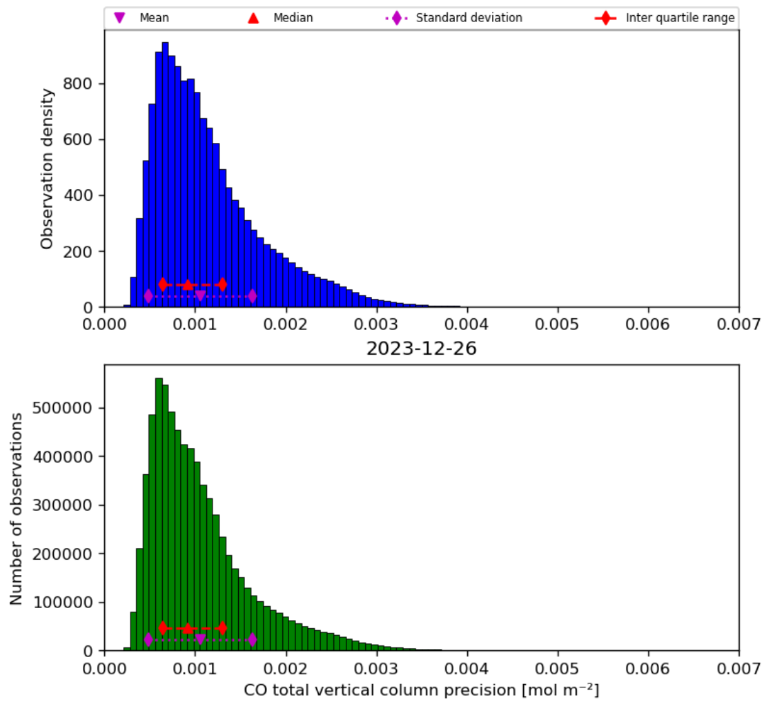
Figure 20: Histogram of “CO total vertical column precision” for 2023-12-25 to 2023-12-27
