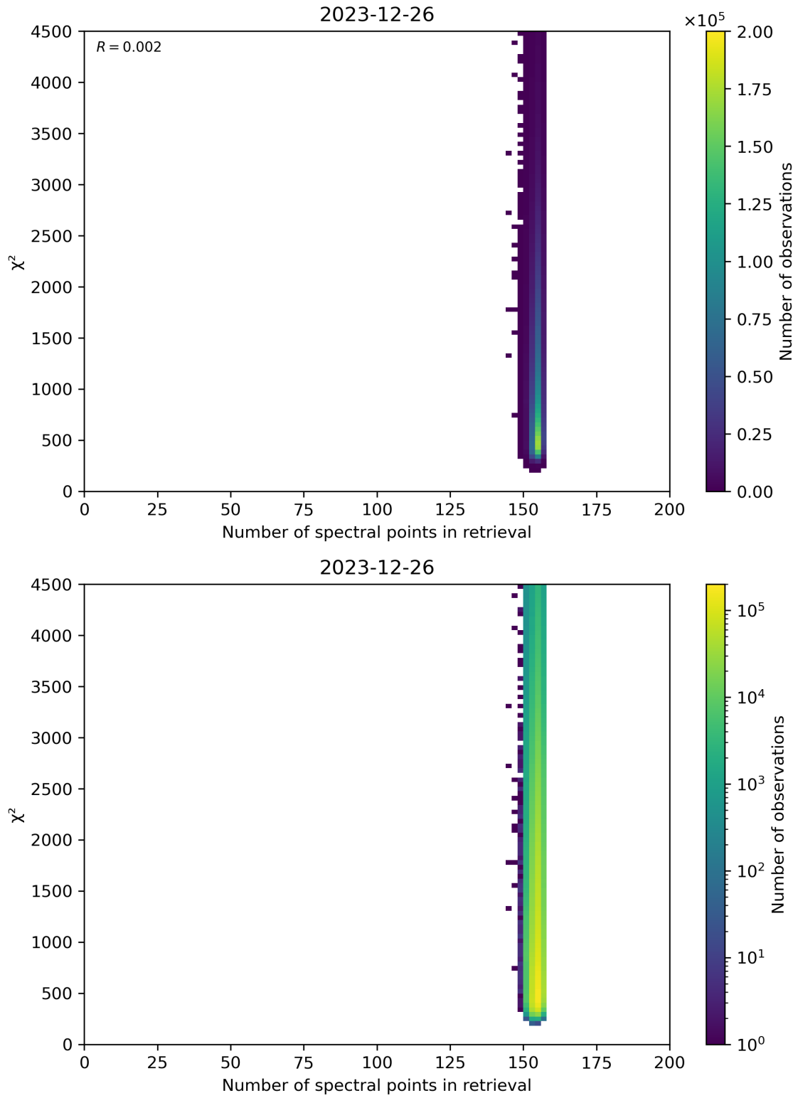
Figure 58: Scatter density plot of “Number of spectral points in retrieval” against “ \chi^2 ” for 2023-12-25 to 2023-12-27.
