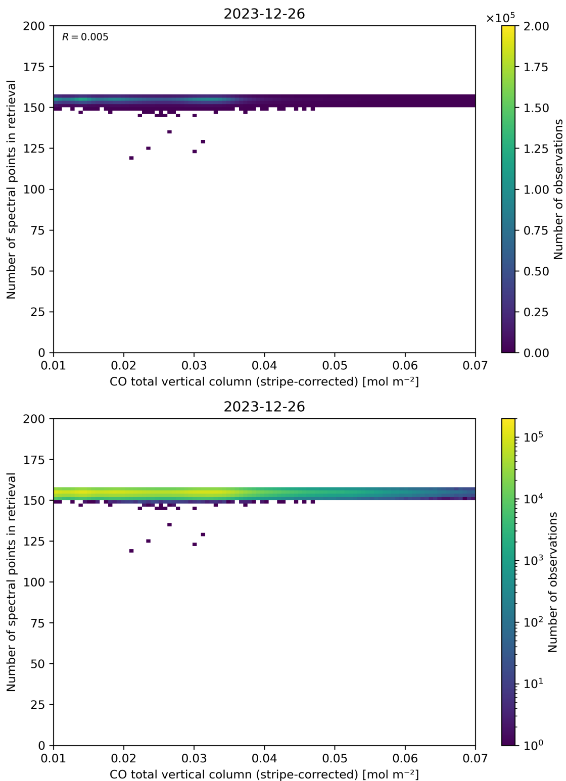
Figure 40: Scatter density plot of “CO total vertical column (stripe-corrected)” against “Number of spectral points in retrieval” for 2023-12-25 to 2023-12-27.
