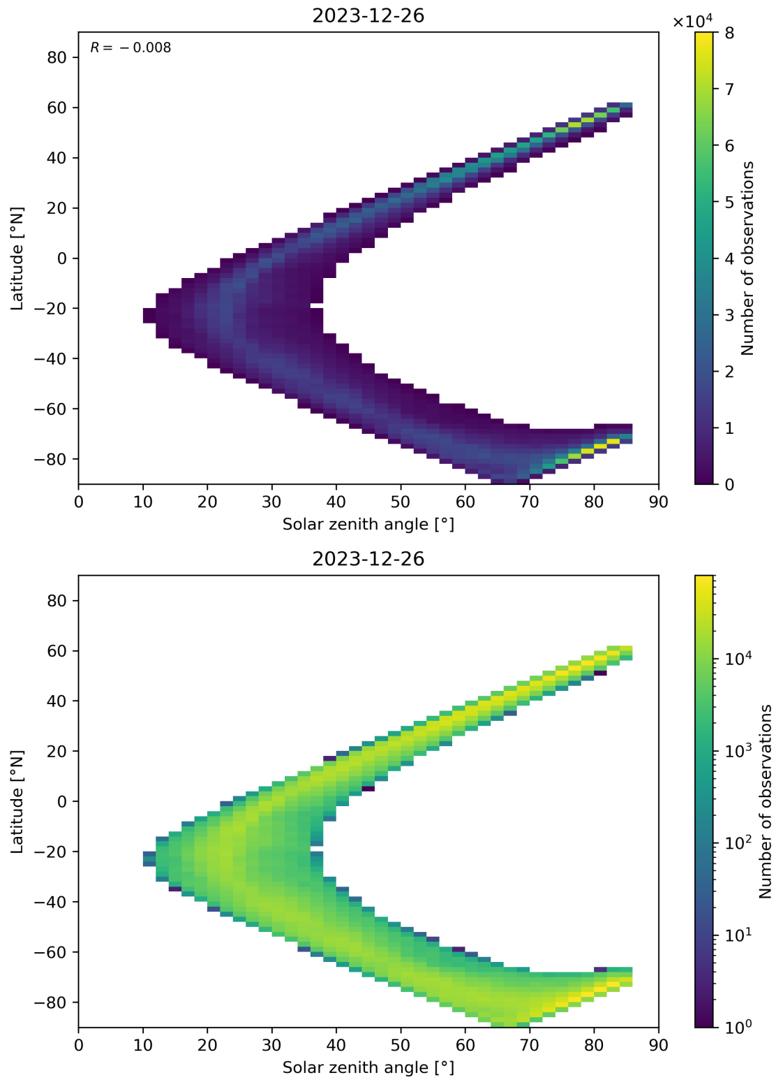
Figure 66: Scatter density plot of “Solar zenith angle” against “Latitude” for 2023-12-25 to 2023-12-27.
