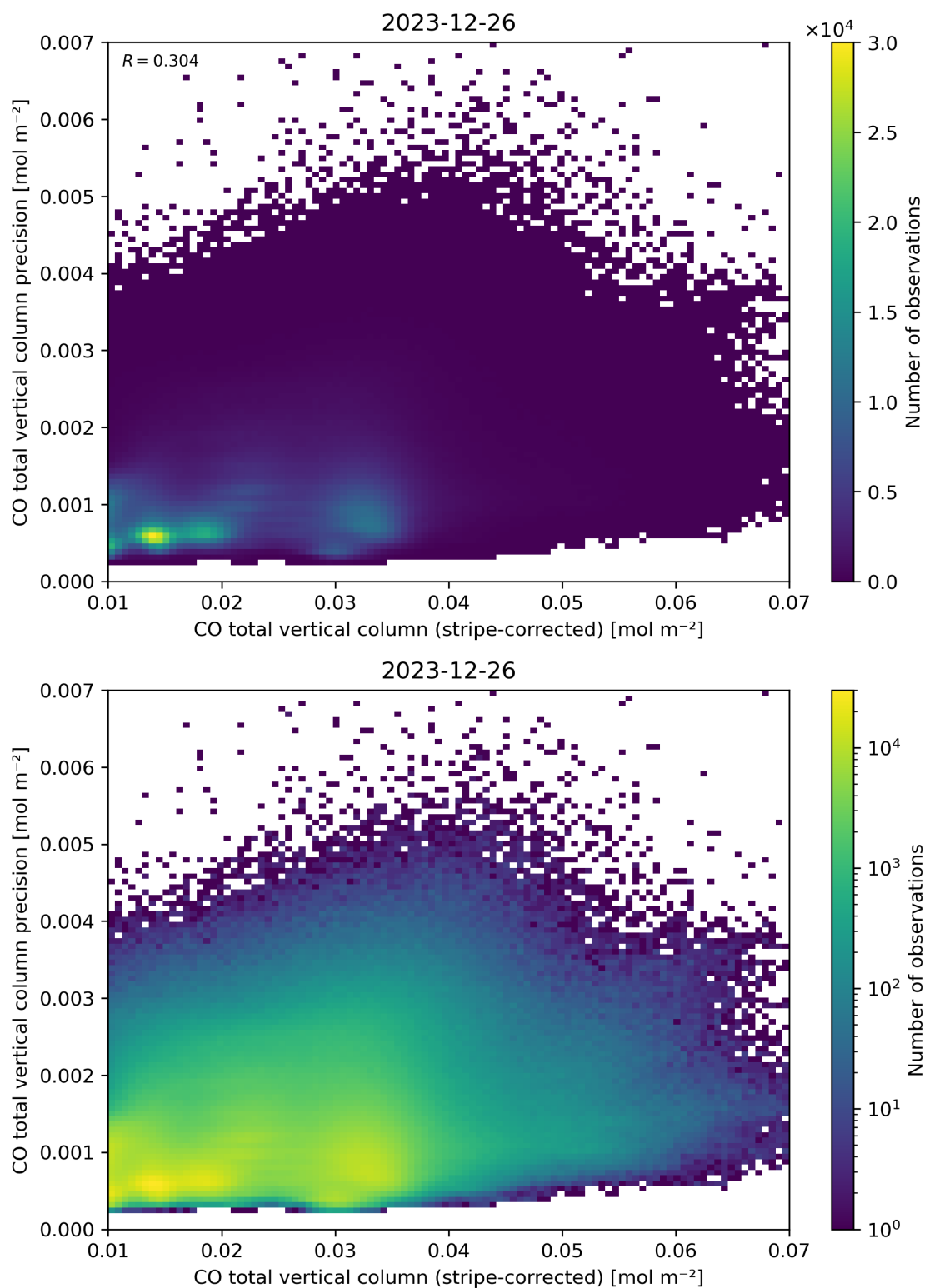
Figure 36: Scatter density plot of “CO total vertical column (stripe-corrected)” against “CO total vertical column precision” for 2023-12-25 to 2023-12-27.
