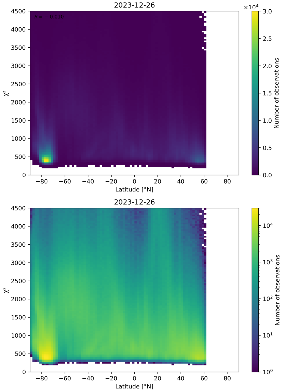
Figure 54: Scatter density plot of “Latitude” against “ \chi^2 ” for 2023-12-25 to 2023-12-27.
