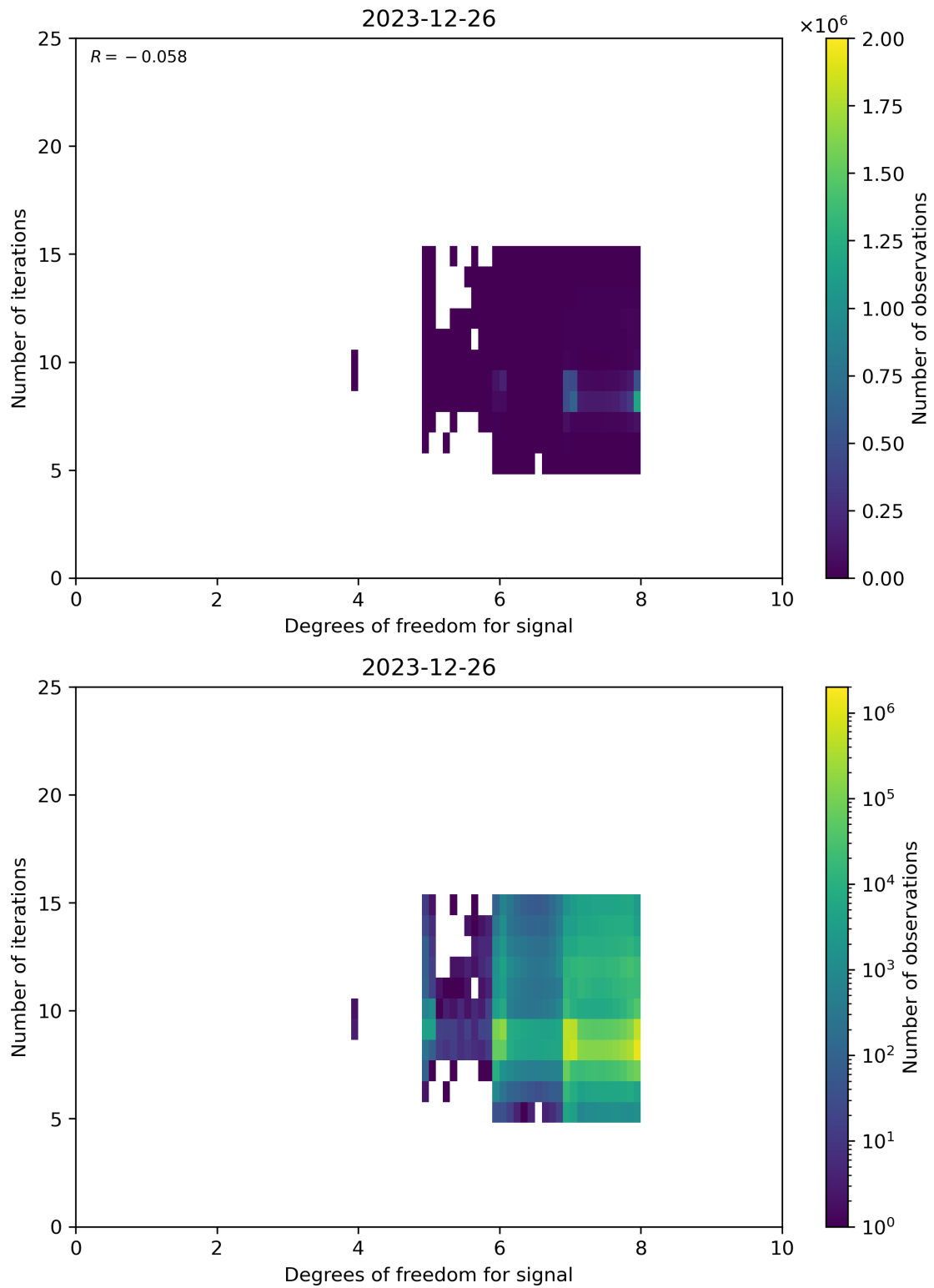
Figure 50: Scatter density plot of “Degrees of freedom for signal” against “Number of iterations” for 2023-12-25 to 2023-12-27.
