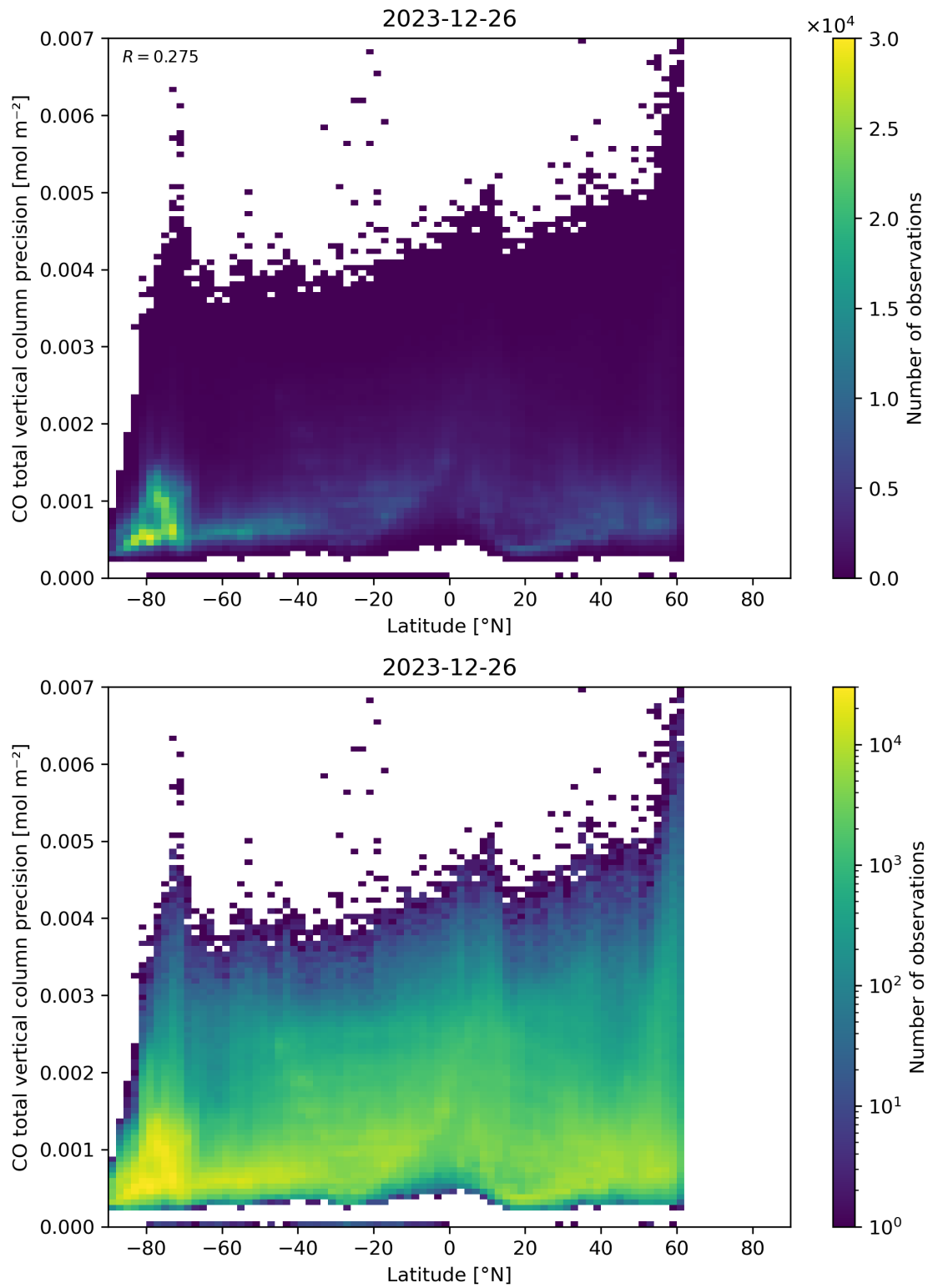
Figure 53: Scatter density plot of “Latitude” against “CO total vertical column precision” for 2023-12-25 to 2023-12-27.
