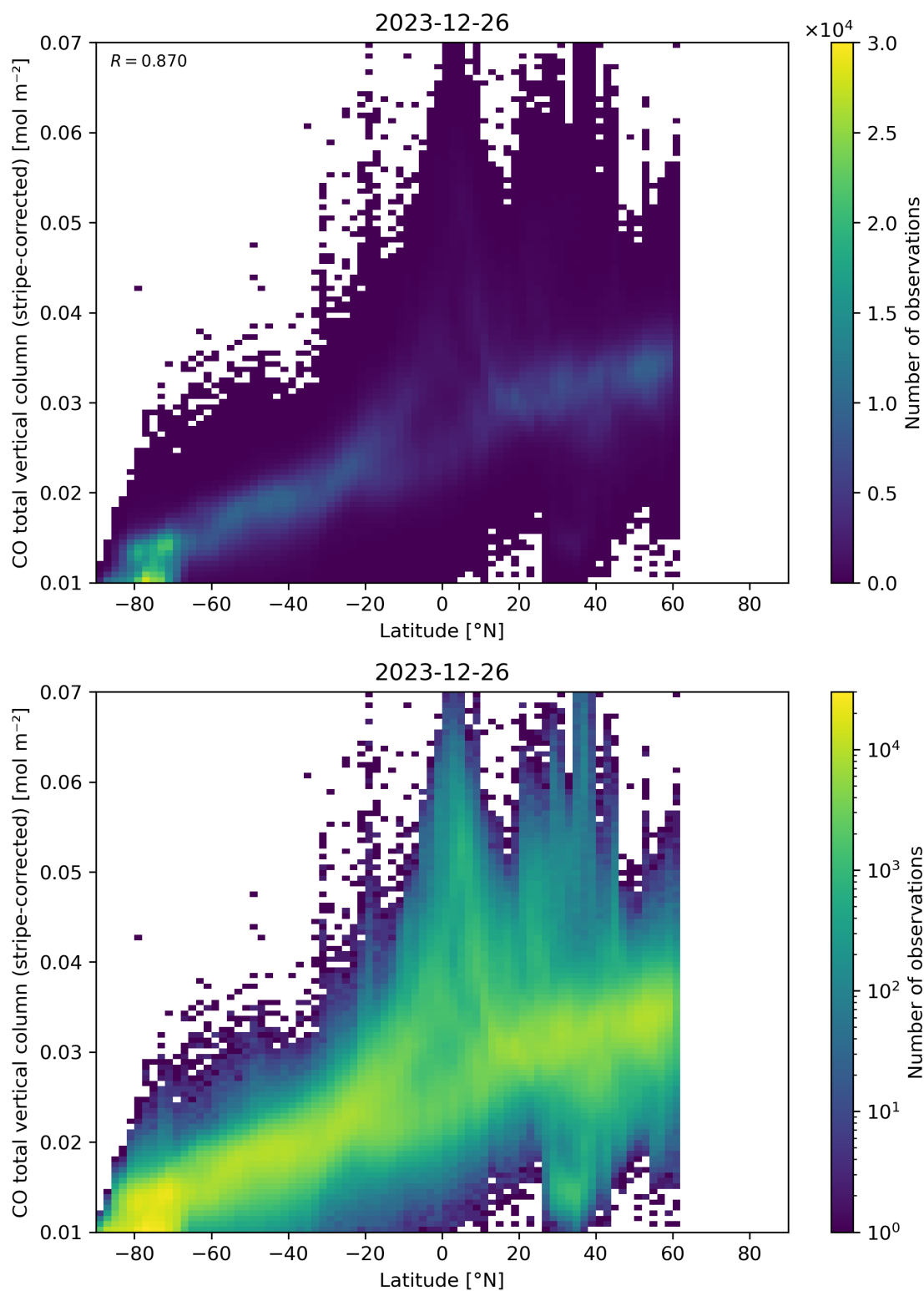
Figure 52: Scatter density plot of “Latitude” against “CO total vertical column (stripe-corrected)” for 2023-12-25 to 2023-12-27.
