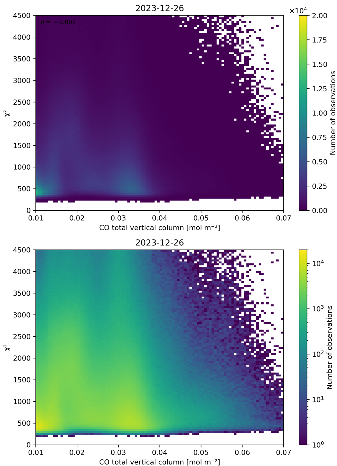
Figure 35: Scatter density plot of “CO total vertical column” against “ \chi^2 ” for 2023-12-25 to 2023-12-27.
