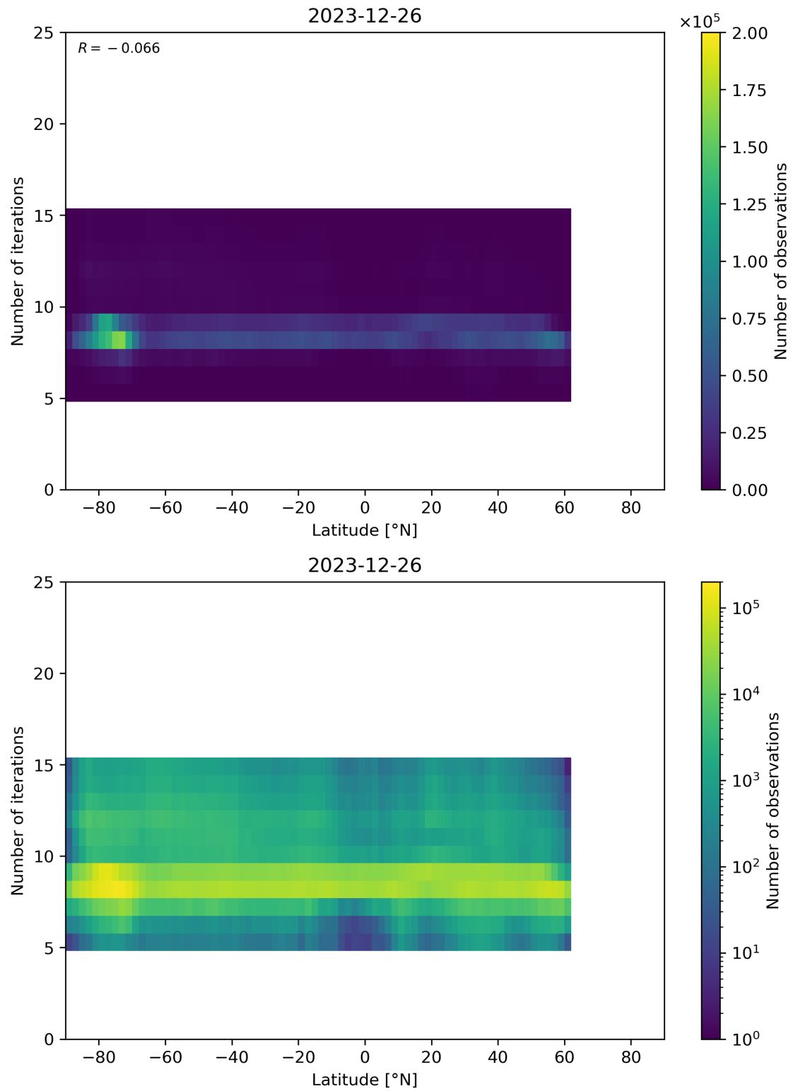
Figure 56: Scatter density plot of “Latitude” against “Number of iterations” for 2023-12-25 to 2023-12-27.
