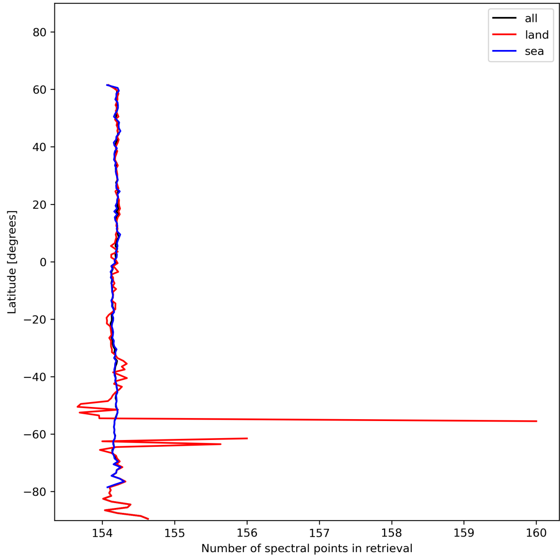
Figure 13: Zonal average of “Number of spectral points in retrieval” for 2023-12-25 to 2023-12-27.
