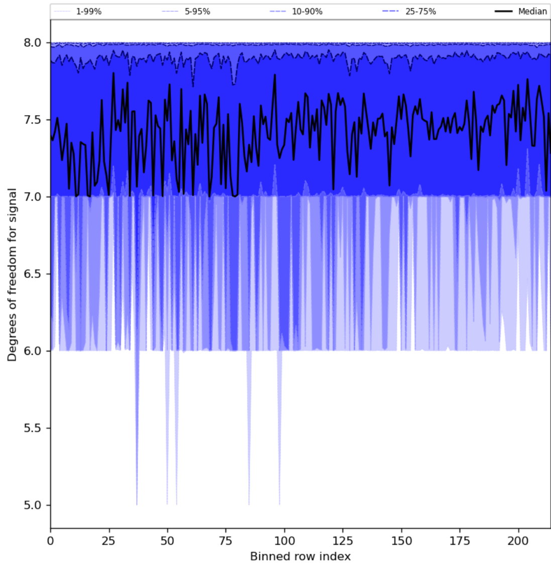
Figure 31: Along track statistics of “Degrees of freedom for signal” for 2023-12-25 to 2023-12-27
