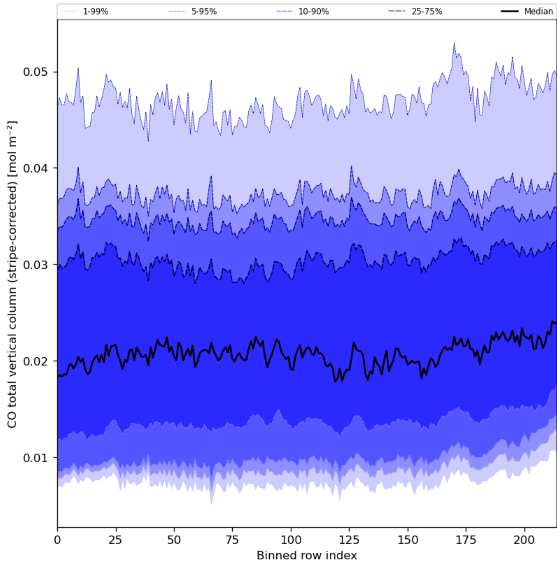
Figure 27: Along track statistics of “CO total vertical column (stripe-corrected)” for 2023-12-25 to 2023-12-27
