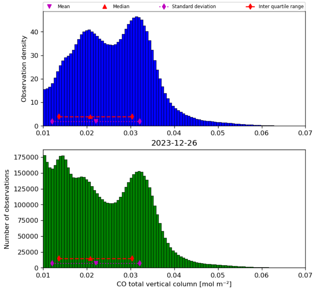
Figure 18: Histogram of “CO total vertical column” for 2023-12-25 to 2023-12-27
