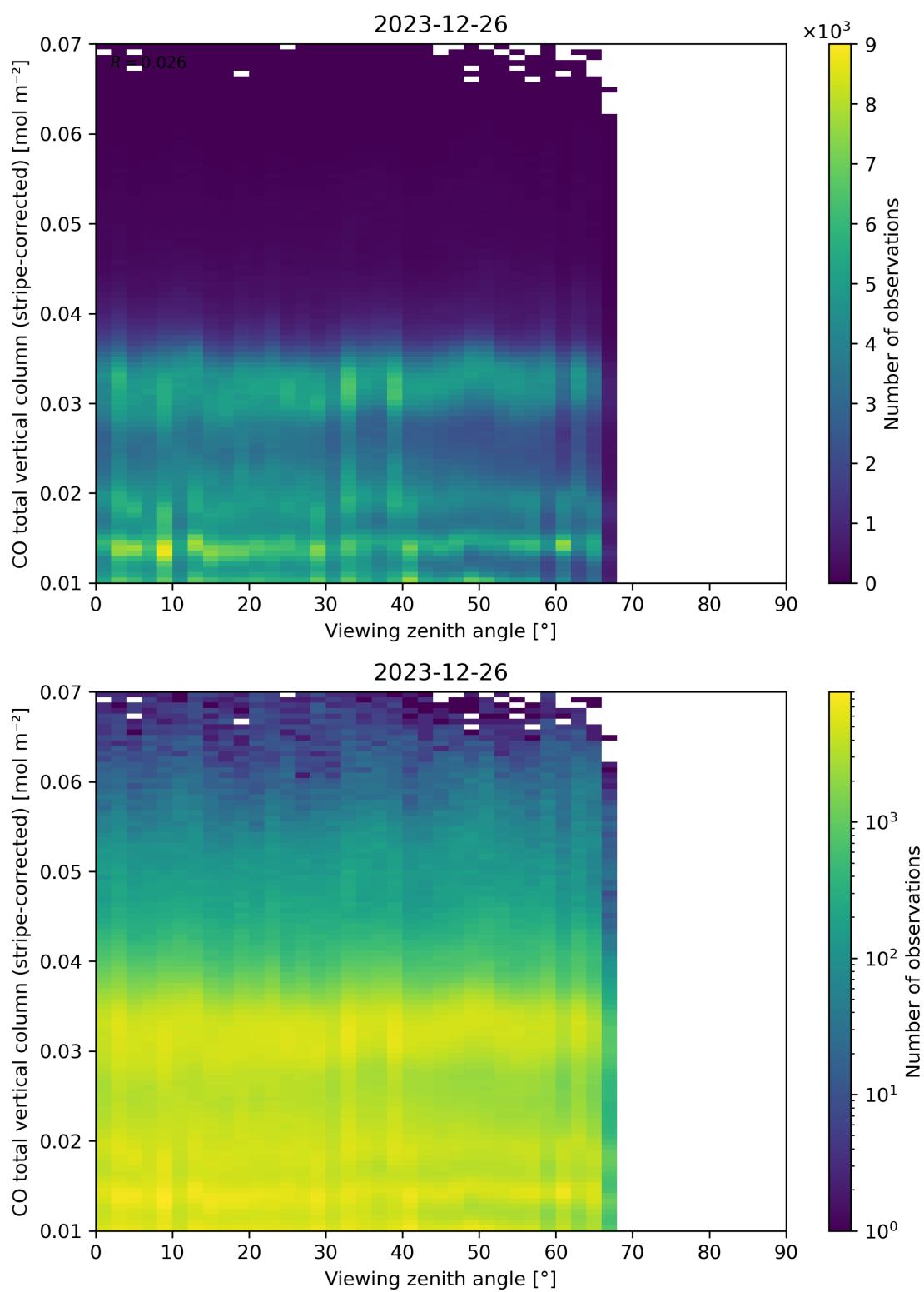
Figure 70: Scatter density plot of “Viewing zenith angle” against “CO total vertical column (stripe-corrected)” for 2023-12-25 to 2023-12-27.
