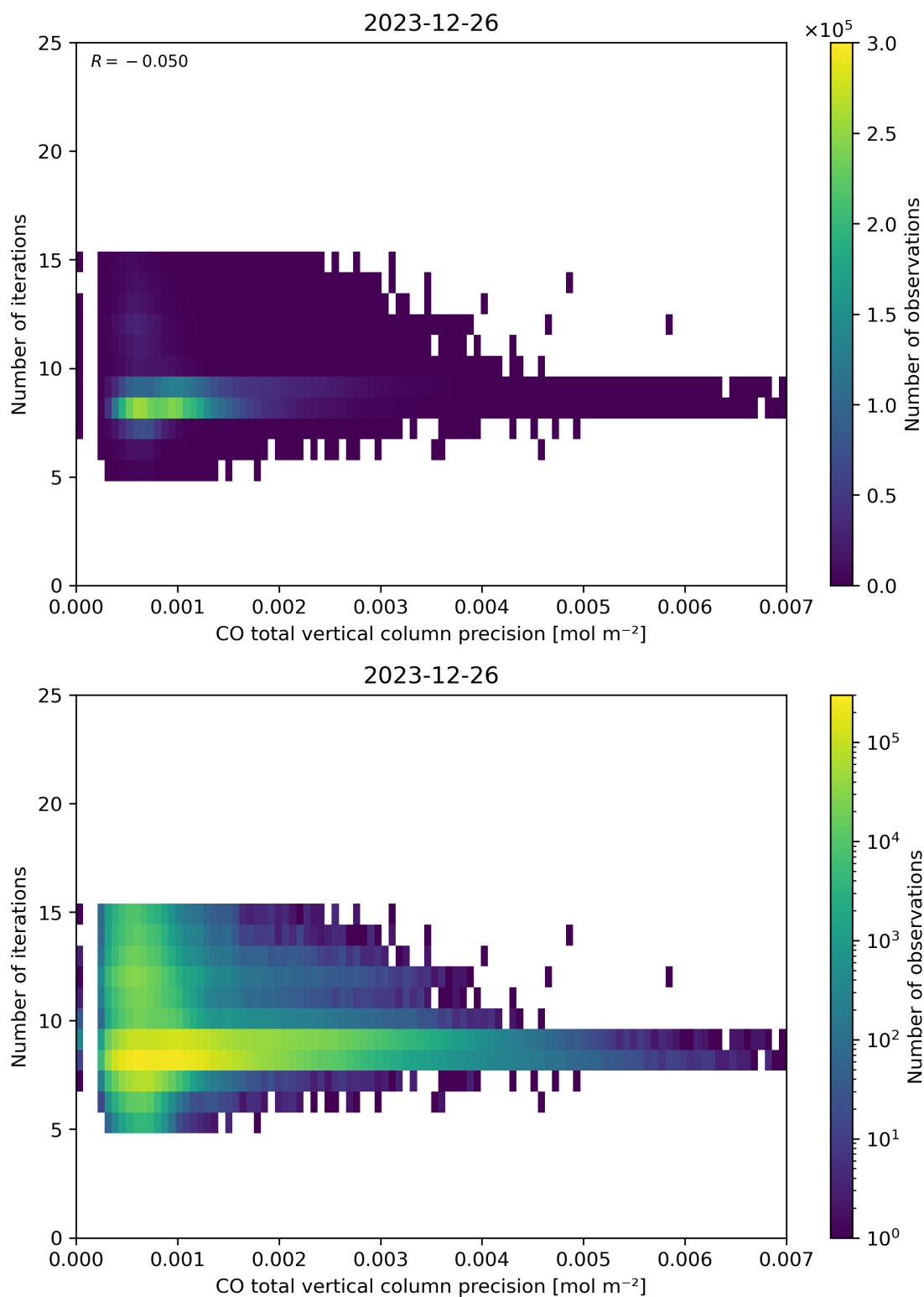
Figure 46: Scatter density plot of “CO total vertical column precision” against “Number of iterations” for 2023-12-25 to 2023-12-27.
