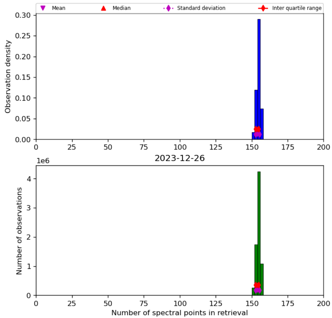
Figure 21: Histogram of “Number of spectral points in retrieval” for 2023-12-25 to 2023-12-27
