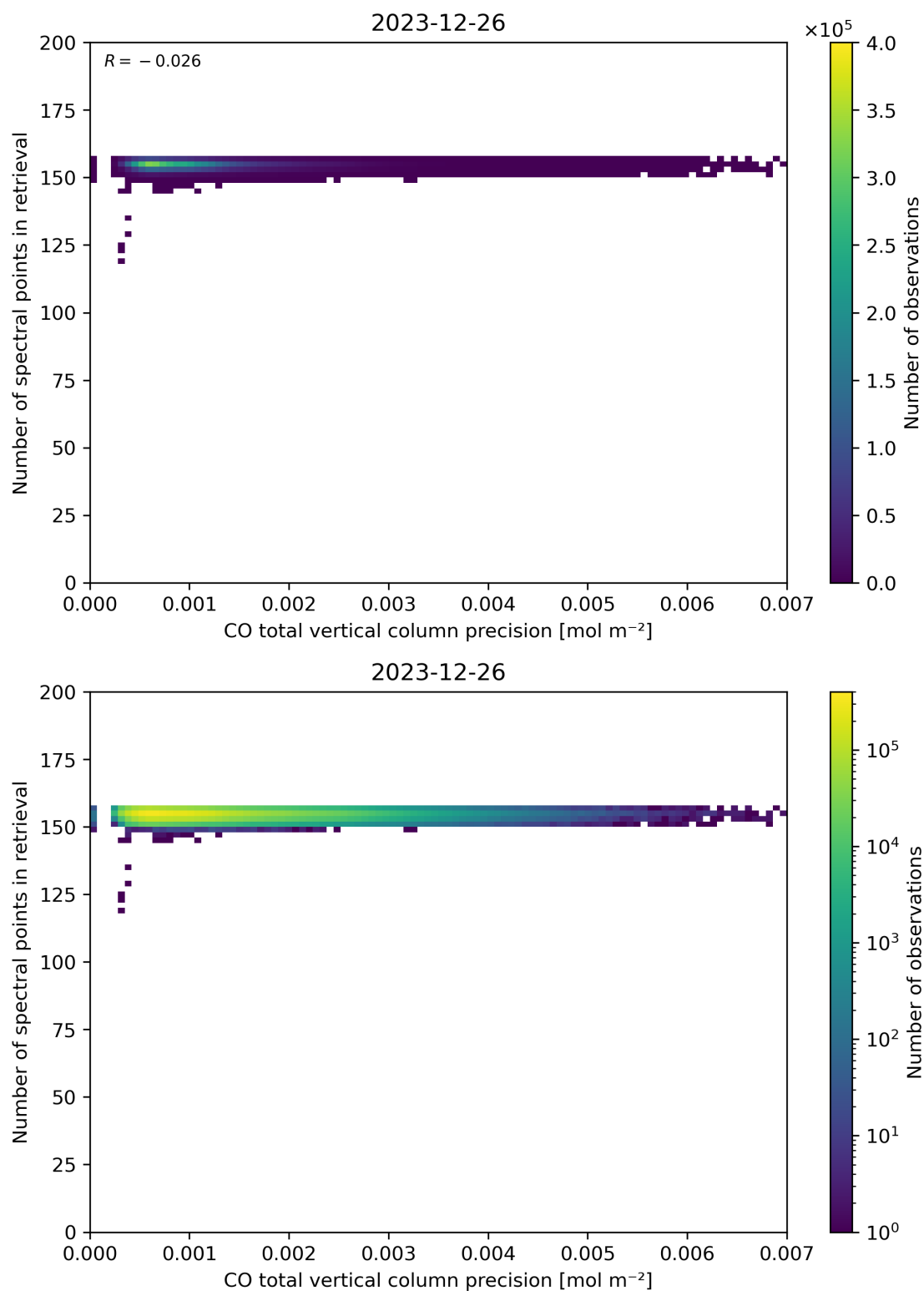
Figure 47: Scatter density plot of “CO total vertical column precision” against “Number of spectral points in retrieval” for 2023-12-25 to 2023-12-27.
