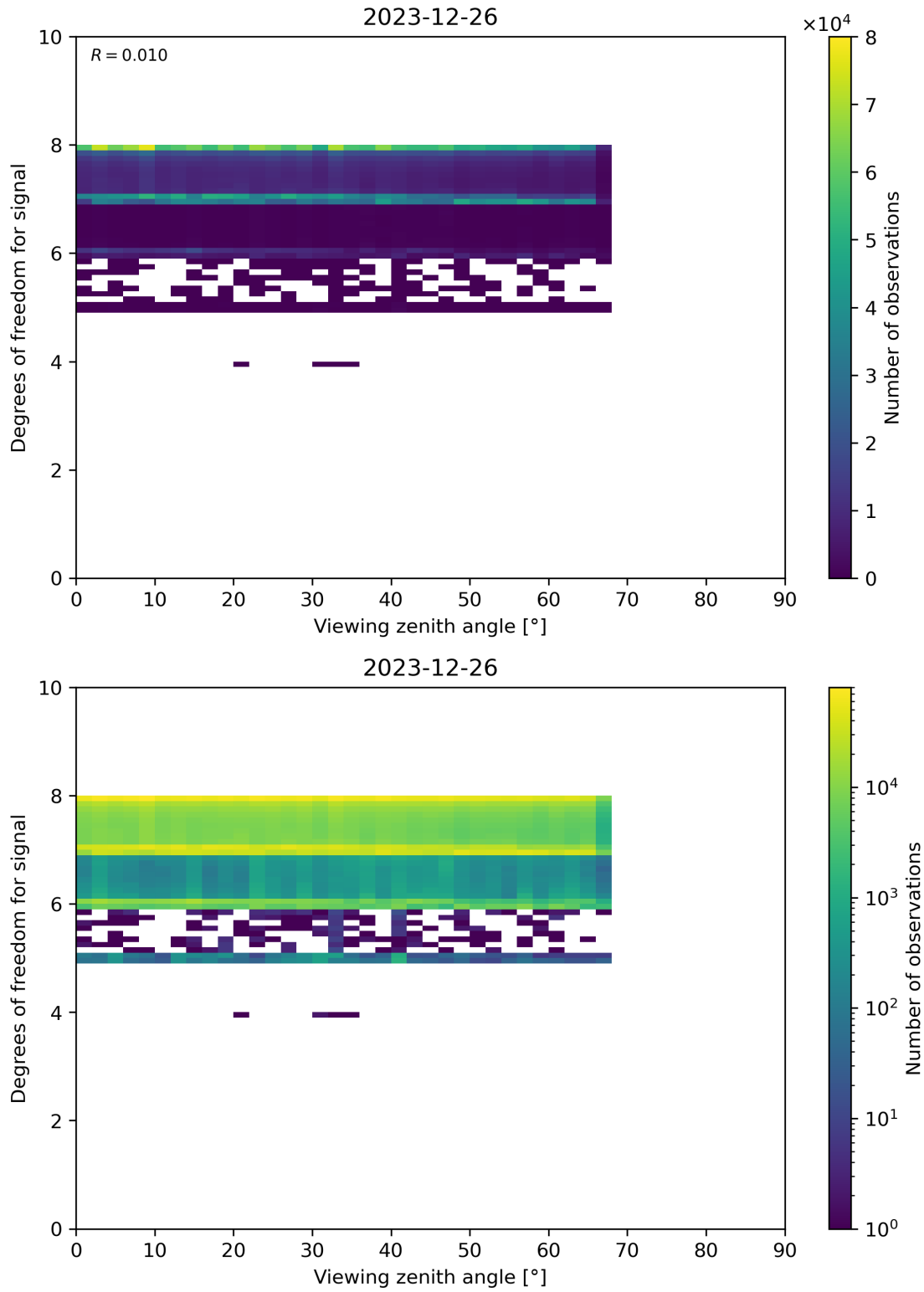
Figure 73: Scatter density plot of “Viewing zenith angle” against “Degrees of freedom for signal” for 2023-12-25 to 2023-12-27.
