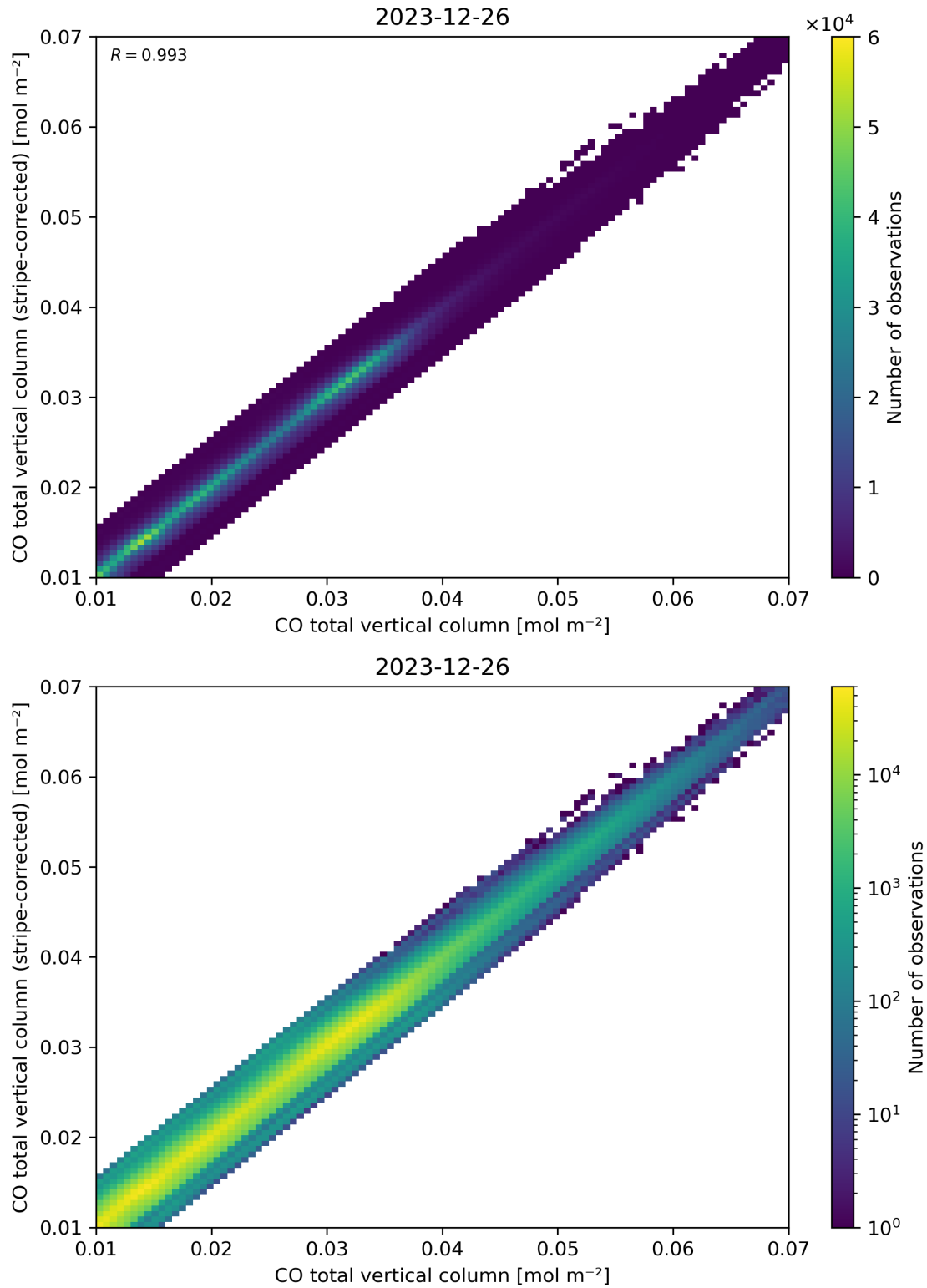
Figure 33: Scatter density plot of “CO total vertical column” against “CO total vertical column (stripe-corrected)” for 2023-12-25 to 2023-12-27.
