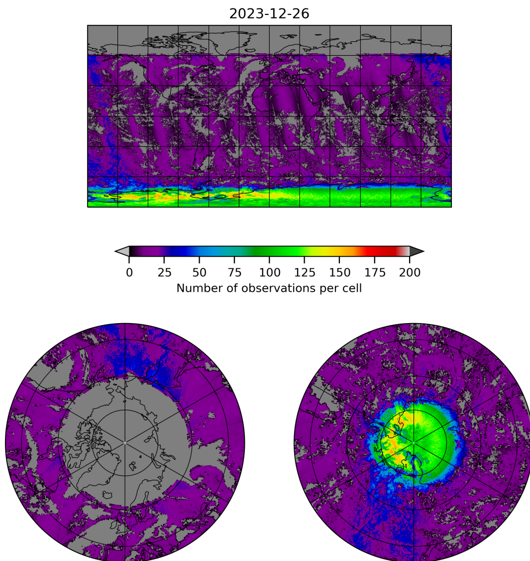
Figure 8: Map of the number of observations for 2023-12-25 to 2023-12-27
