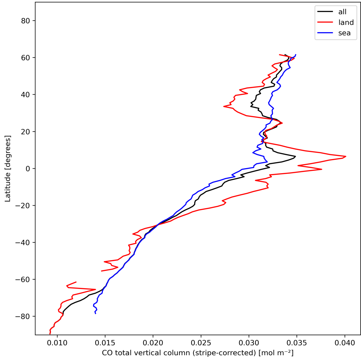
Figure 11: Zonal average of “CO total vertical column (stripe-corrected)” for 2023-12-25 to 2023-12-27.
