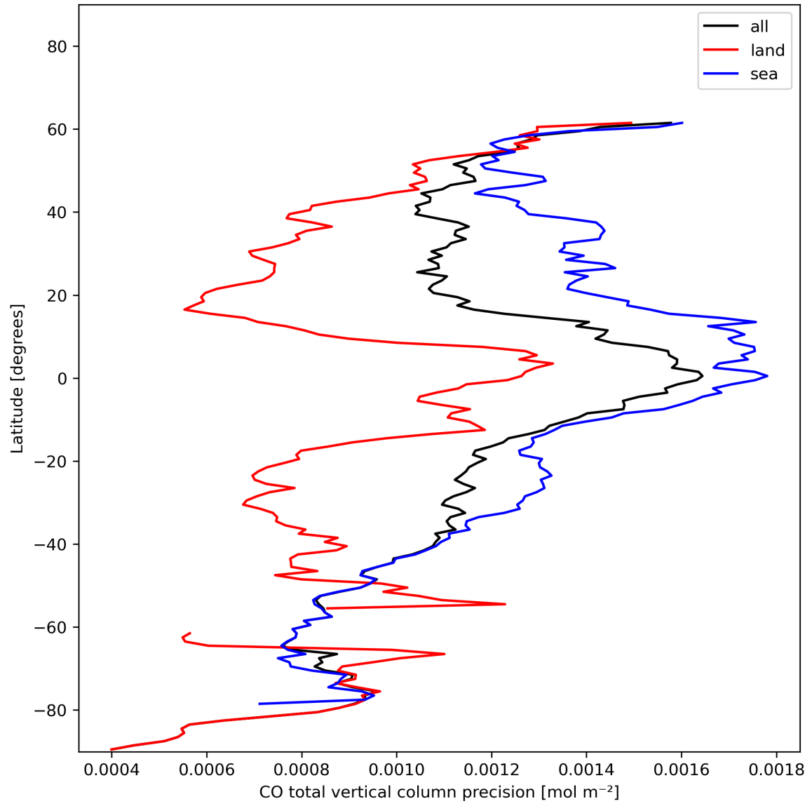
Figure 12: Zonal average of “CO total vertical column precision” for 2023-12-25 to 2023-12-27.
