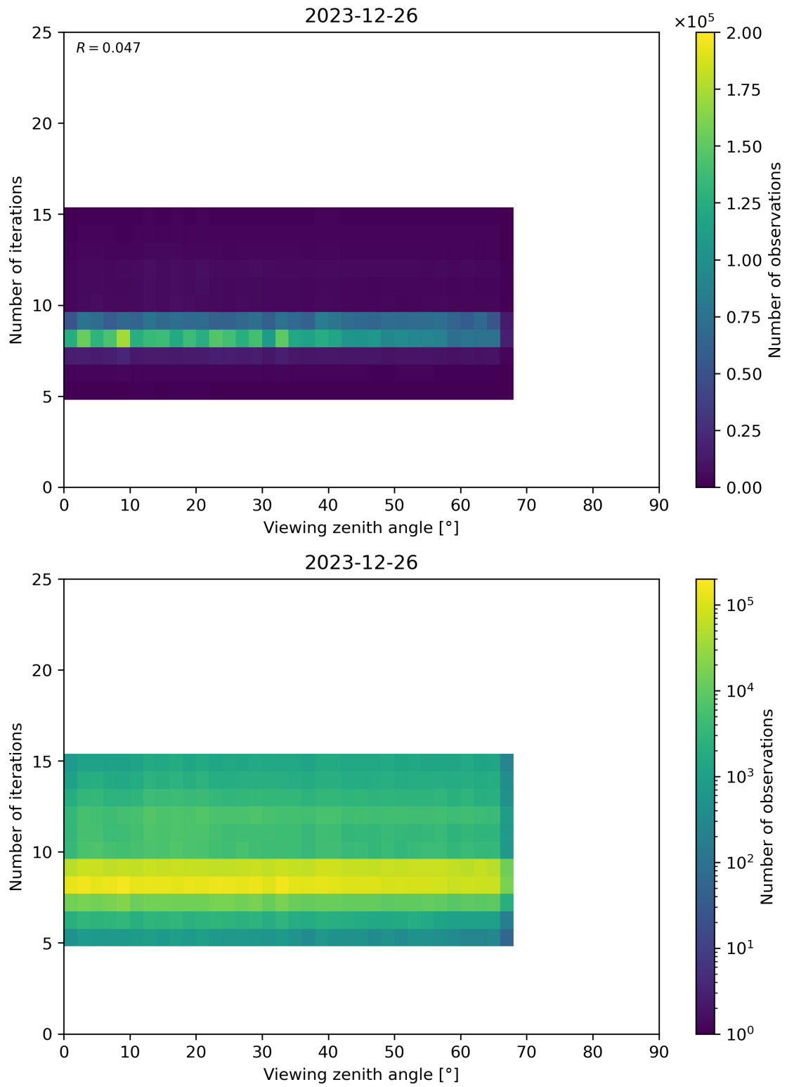
Figure 75: Scatter density plot of “Viewing zenith angle” against “Number of iterations” for 2023-12-25 to 2023-12-27.
