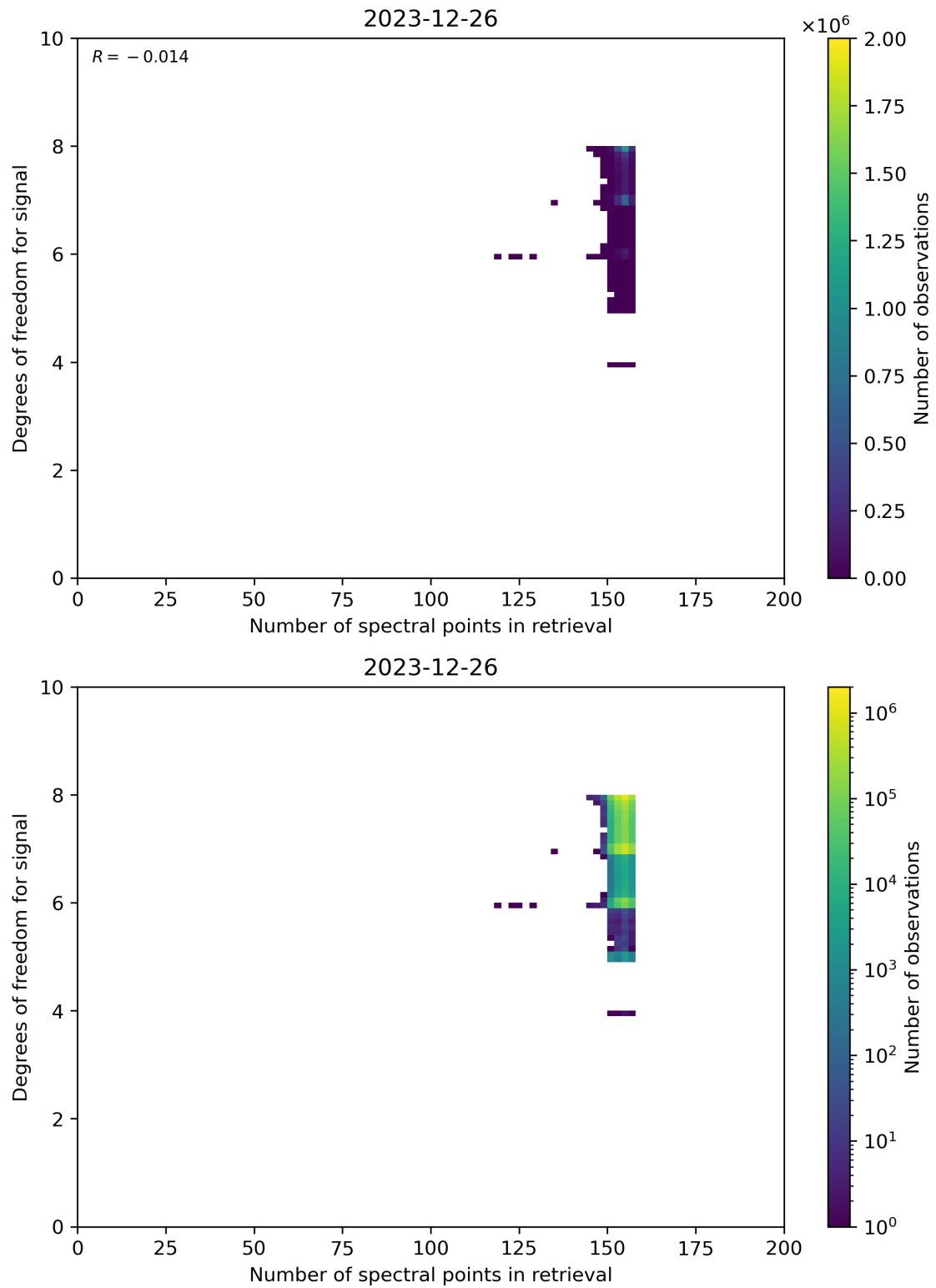
Figure 59: Scatter density plot of “Number of spectral points in retrieval” against “Degrees of freedom for signal” for 2023-12-25 to 2023-12-27.
