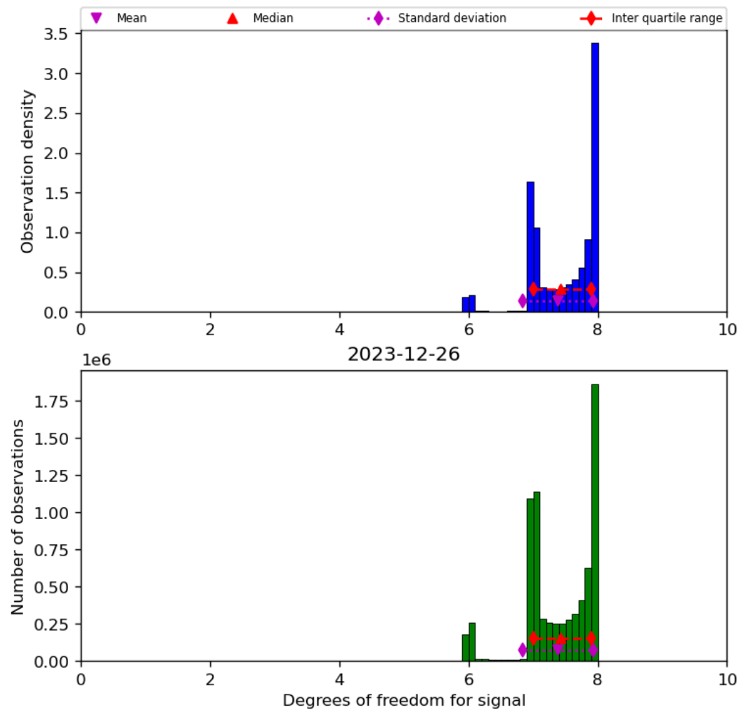
Figure 23: Histogram of “Degrees of freedom for signal” for 2023-12-25 to 2023-12-27
