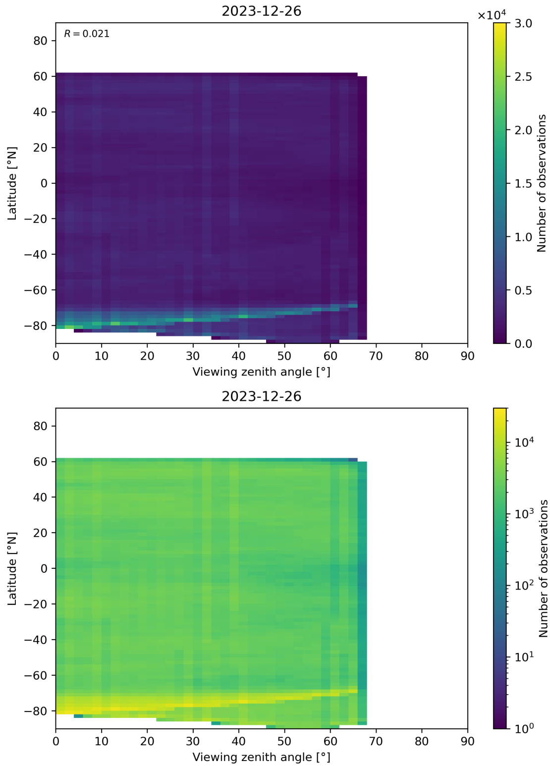
Figure 74: Scatter density plot of “Viewing zenith angle” against “Latitude” for 2023-12-25 to 2023-12-27.
