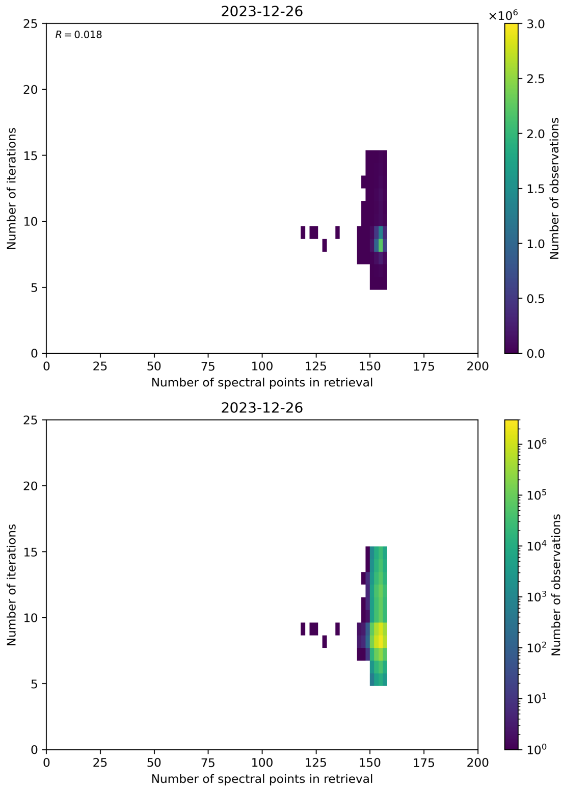
Figure 60: Scatter density plot of “Number of spectral points in retrieval” against “Number of iterations” for 2023-12-25 to 2023-12-27.
