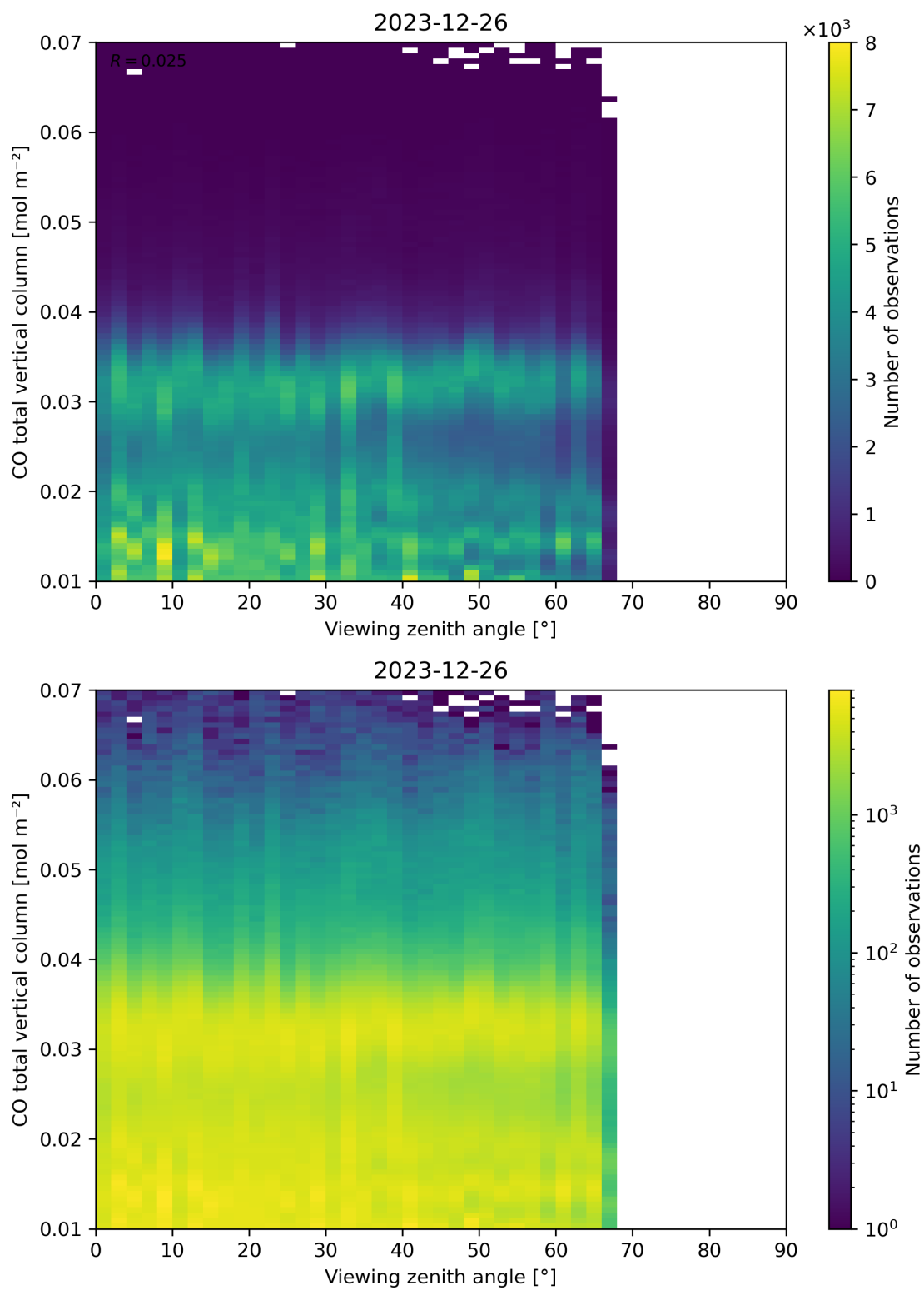
Figure 69: Scatter density plot of “Viewing zenith angle” against “CO total vertical column” for 2023-12-25 to 2023-12-27.
