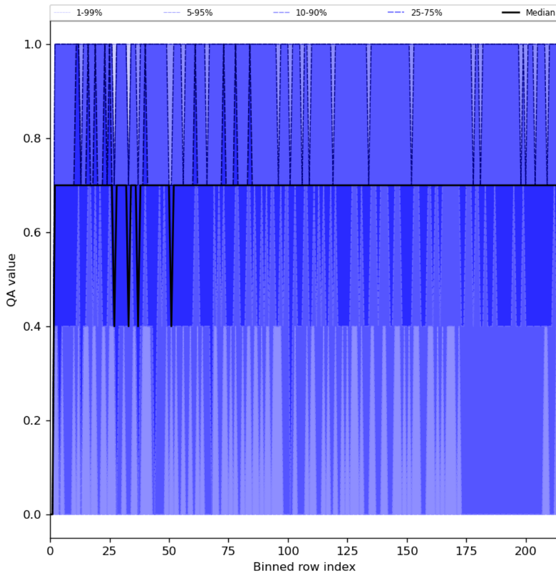
Figure 25: Along track statistics of “QA value” for 2023-12-25 to 2023-12-27
