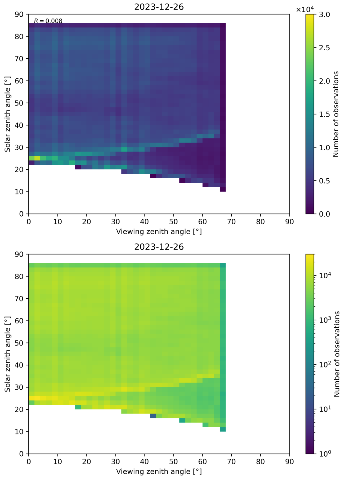
Figure 77: Scatter density plot of “Viewing zenith angle” against “Solar zenith angle” for 2023-12-25 to 2023-12-27.
