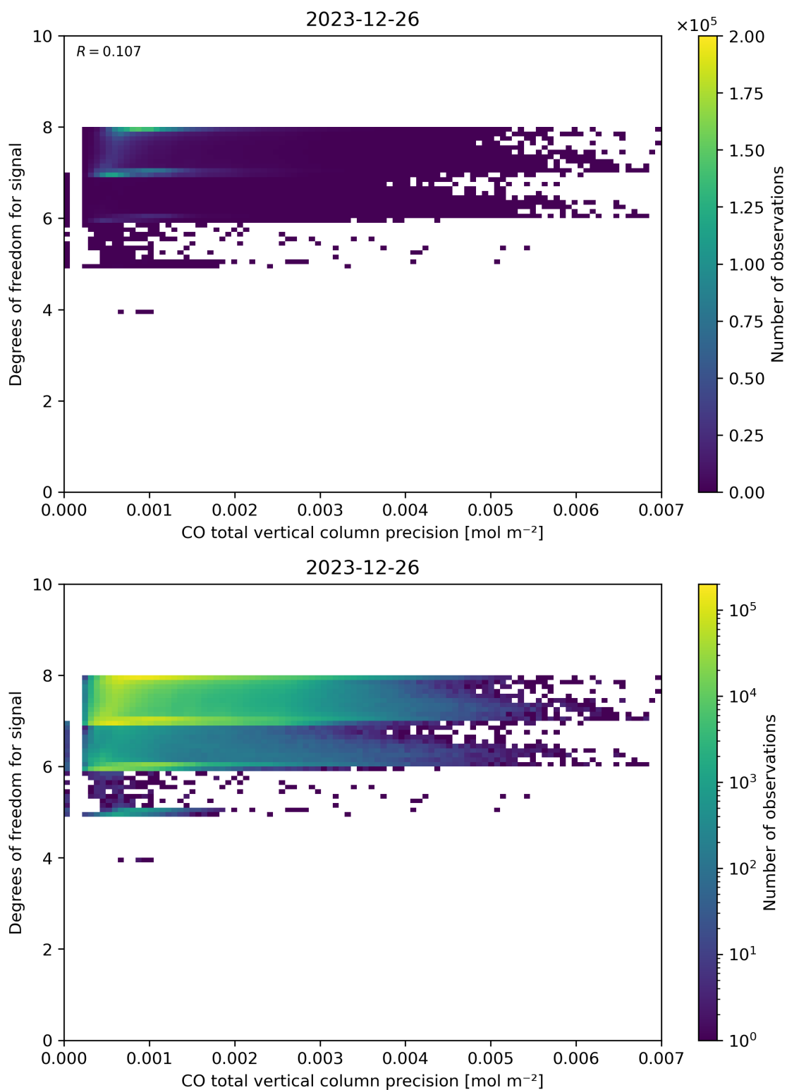
Figure 45: Scatter density plot of “CO total vertical column precision” against “Degrees of freedom for signal” for 2023-12-25 to 2023-12-27.
