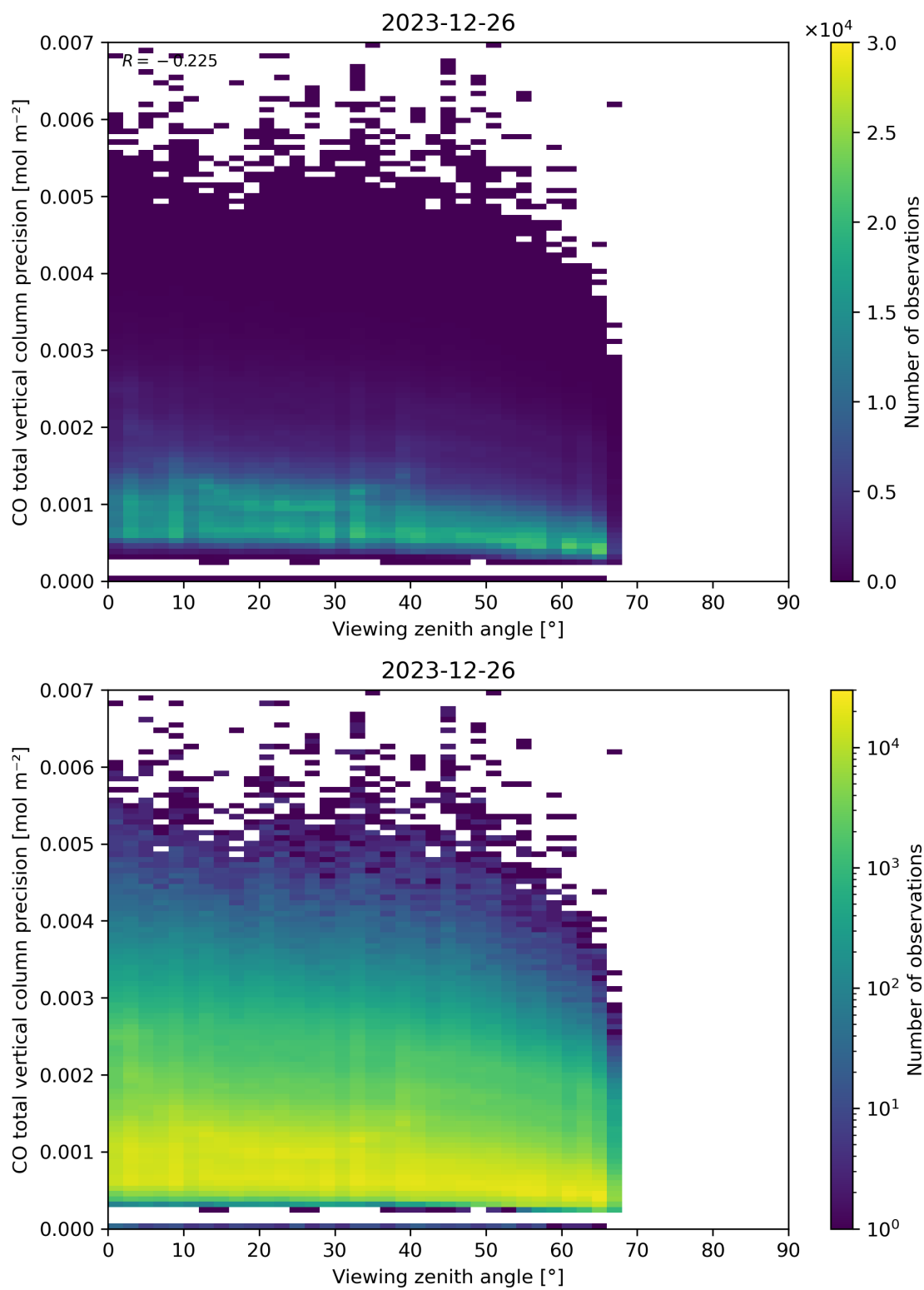
Figure 71: Scatter density plot of “Viewing zenith angle” against “CO total vertical column precision” for 2023-12-25 to 2023-12-27.
