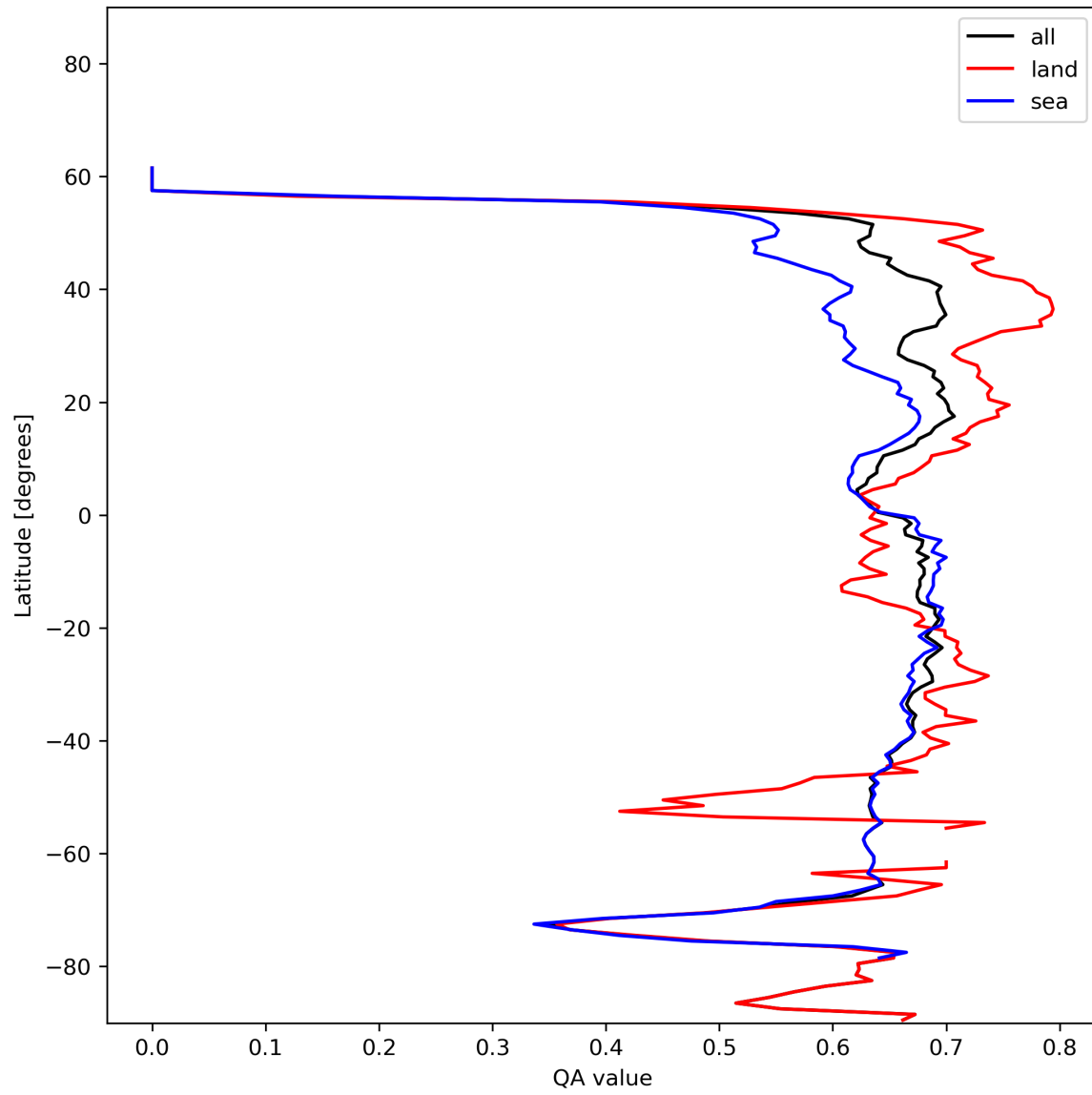
Figure 9: Zonal average of “QA value” for 2023-12-25 to 2023-12-27.
