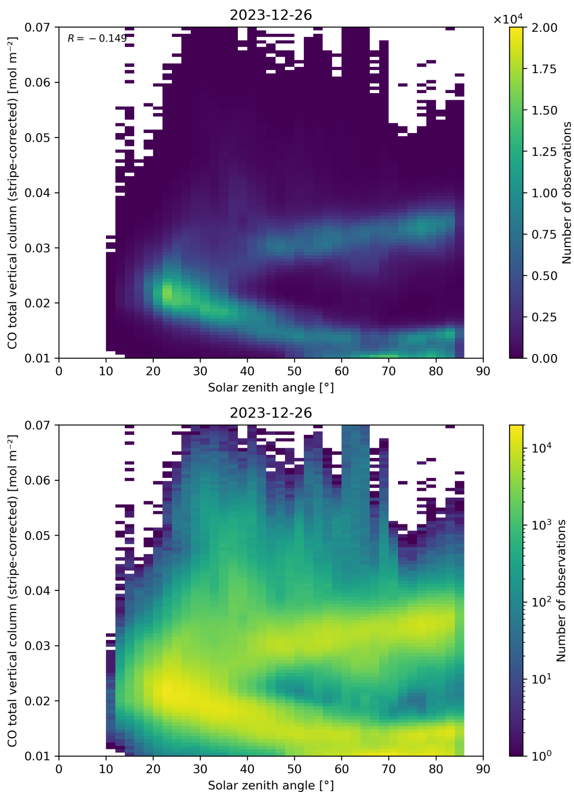
Figure 62: Scatter density plot of “Solar zenith angle” against “CO total vertical column (stripe-corrected)” for 2023-12-25 to 2023-12-27.
