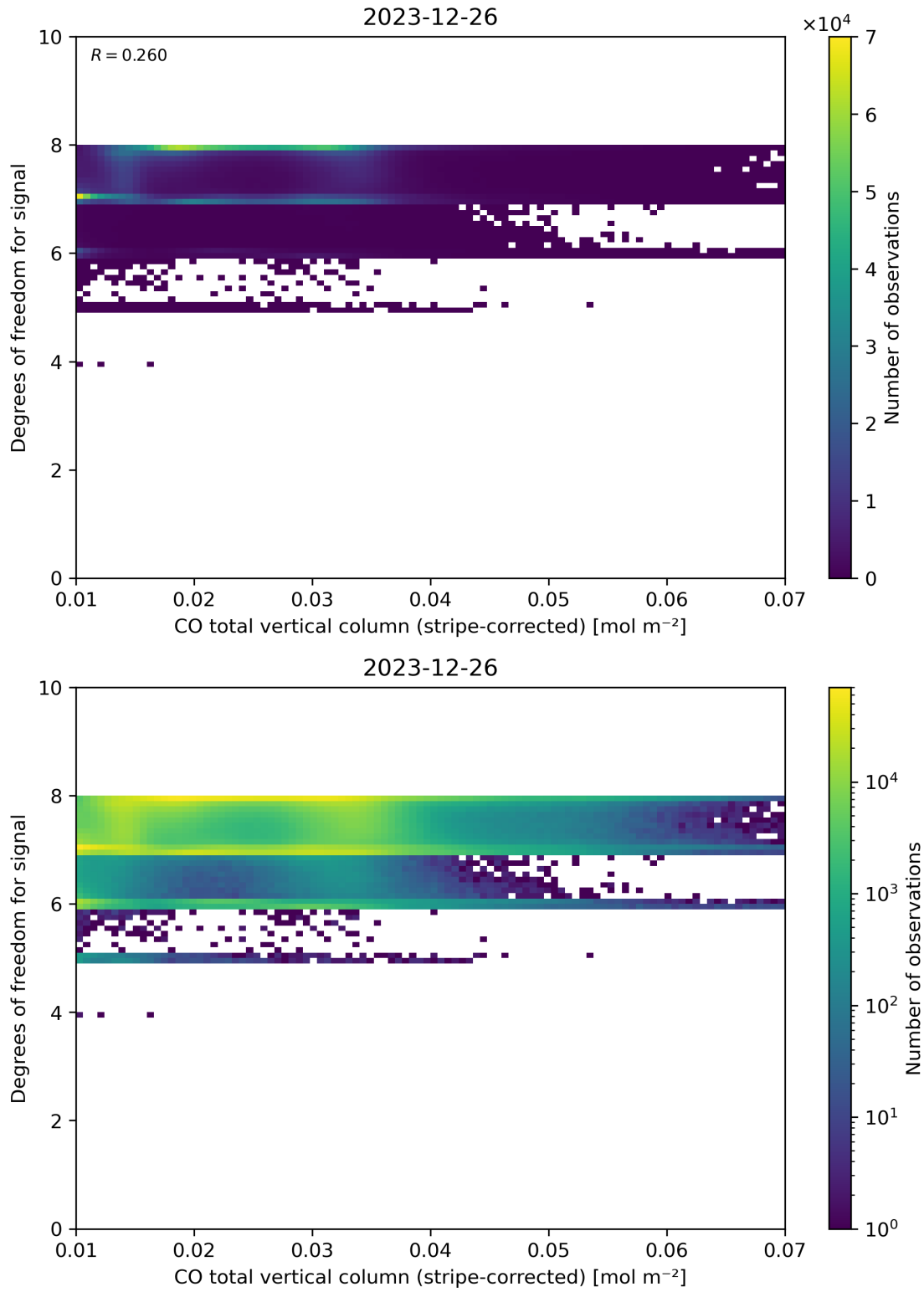
Figure 38: Scatter density plot of “CO total vertical column (stripe-corrected)” against “Degrees of freedom for signal” for 2023-12-25 to 2023-12-27.
