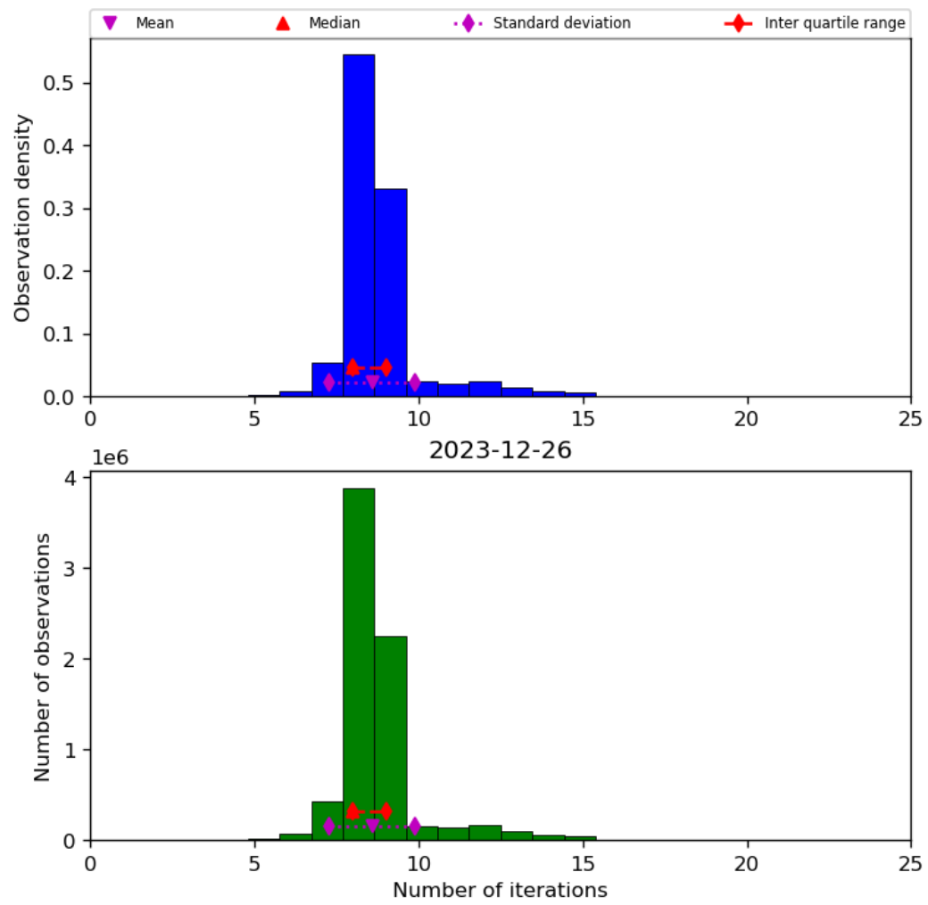
Figure 24: Histogram of “Number of iterations” for 2023-12-25 to 2023-12-27
