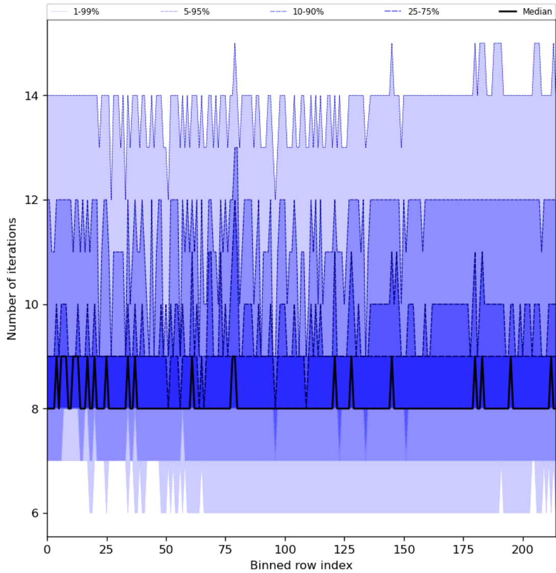
Figure 32: Along track statistics of “Number of iterations” for 2023-12-25 to 2023-12-27
