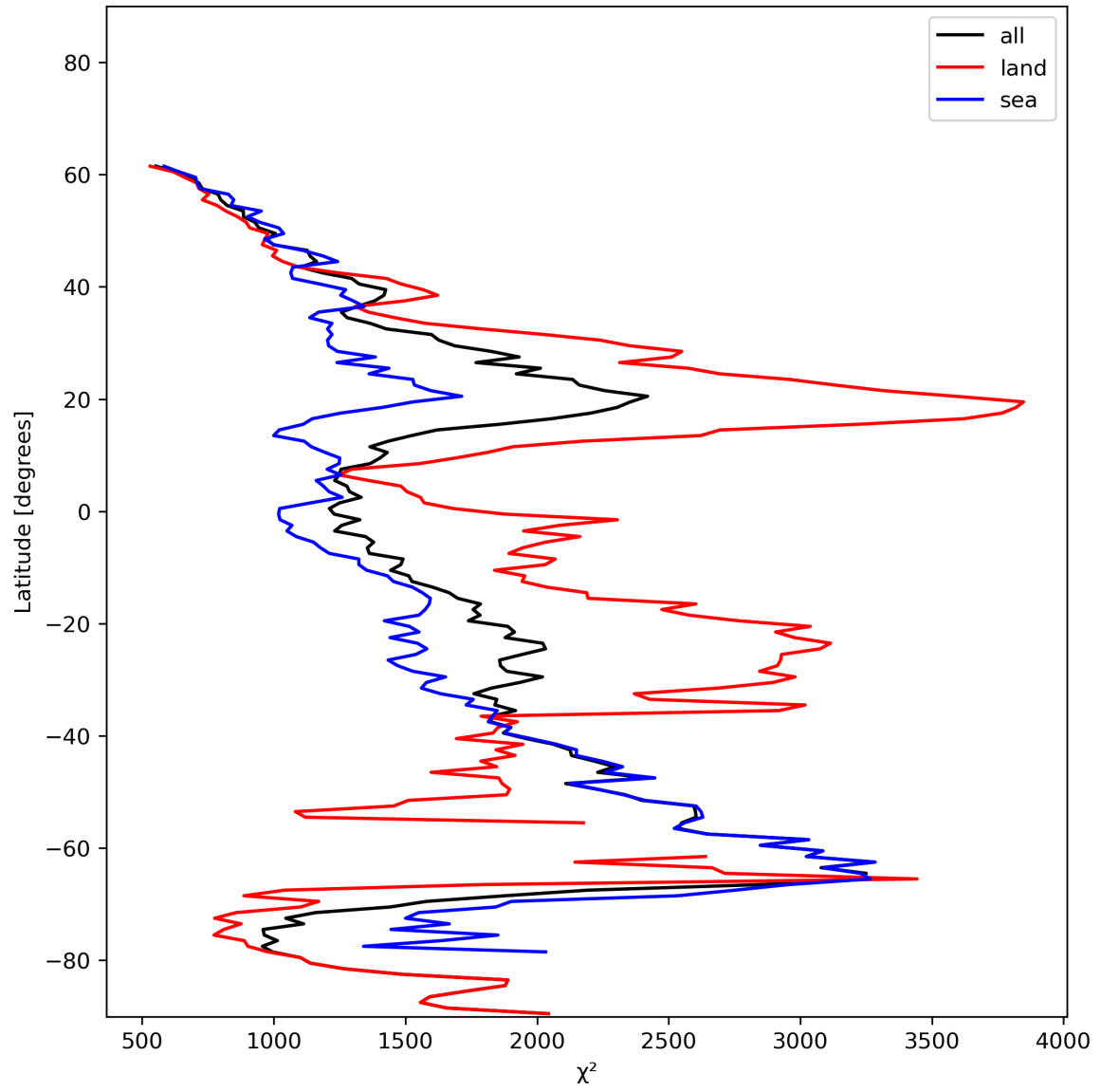
Figure 14: Zonal average of “ \chi^2 ” for 2023-12-25 to 2023-12-27.
