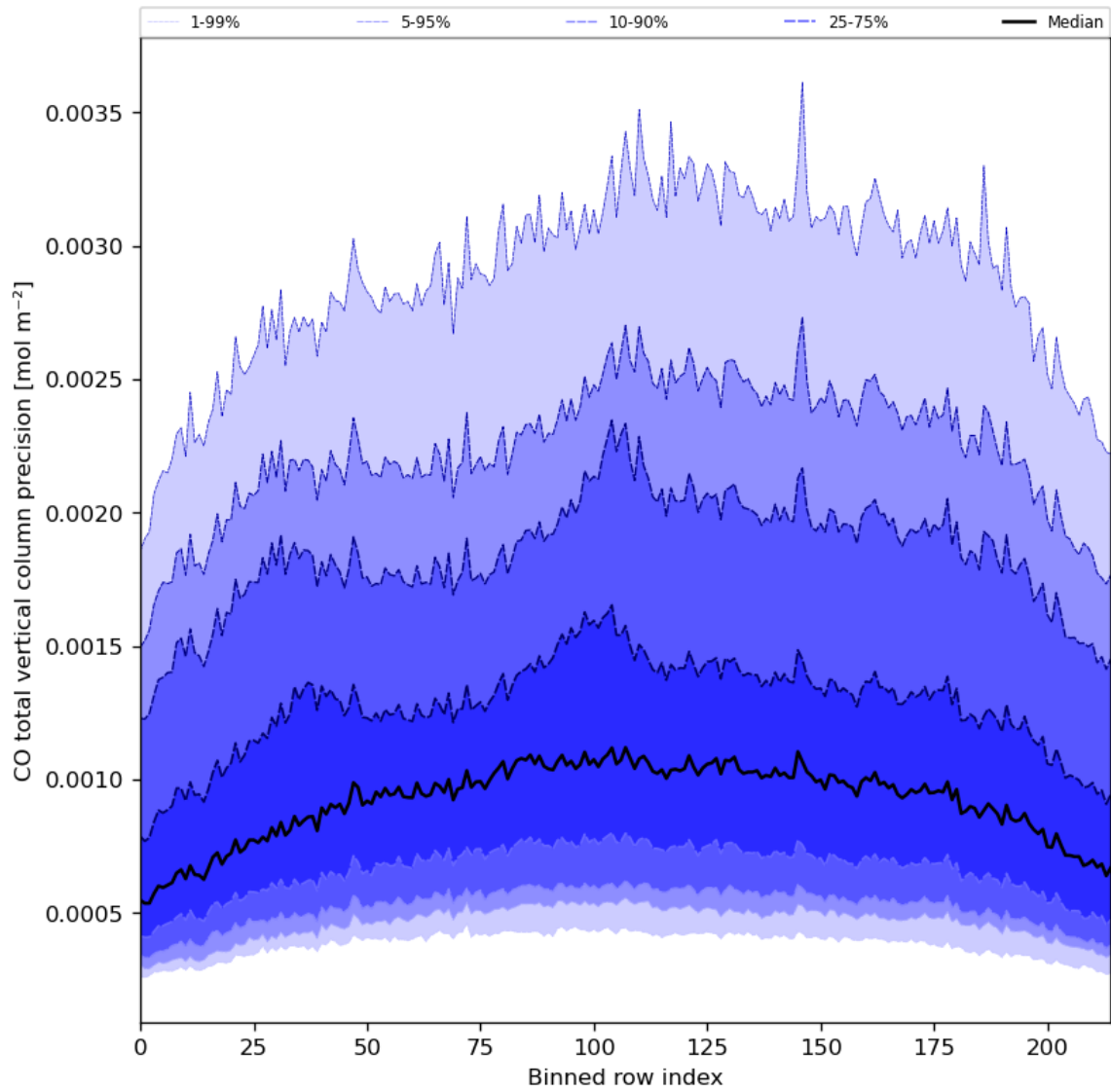
Figure 28: Along track statistics of “CO total vertical column precision” for 2023-12-25 to 2023-12-27
