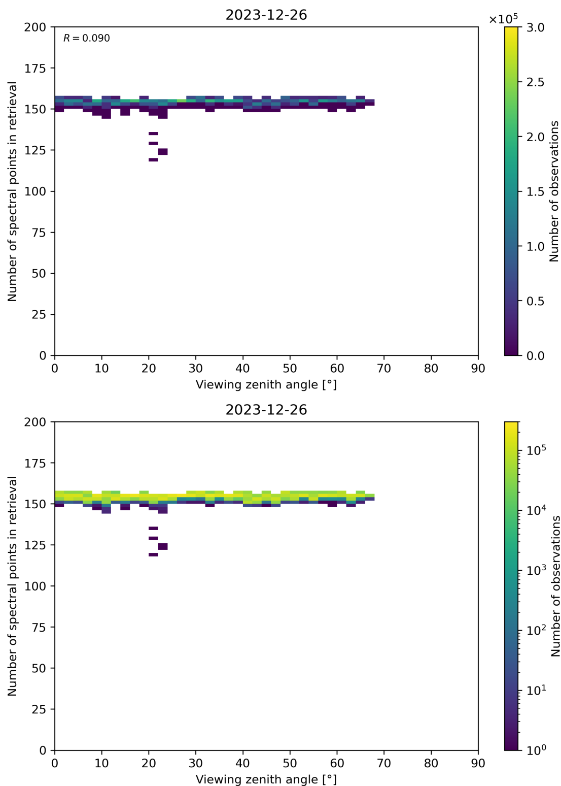
Figure 76: Scatter density plot of “Viewing zenith angle” against “Number of spectral points in retrieval” for 2023-12-25 to 2023-12-27.
