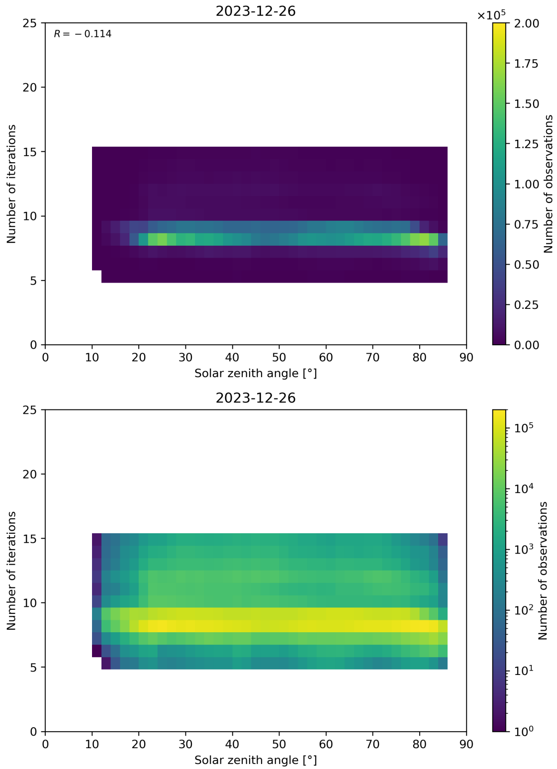
Figure 67: Scatter density plot of “Solar zenith angle” against “Number of iterations” for 2023-12-25 to 2023-12-27.
