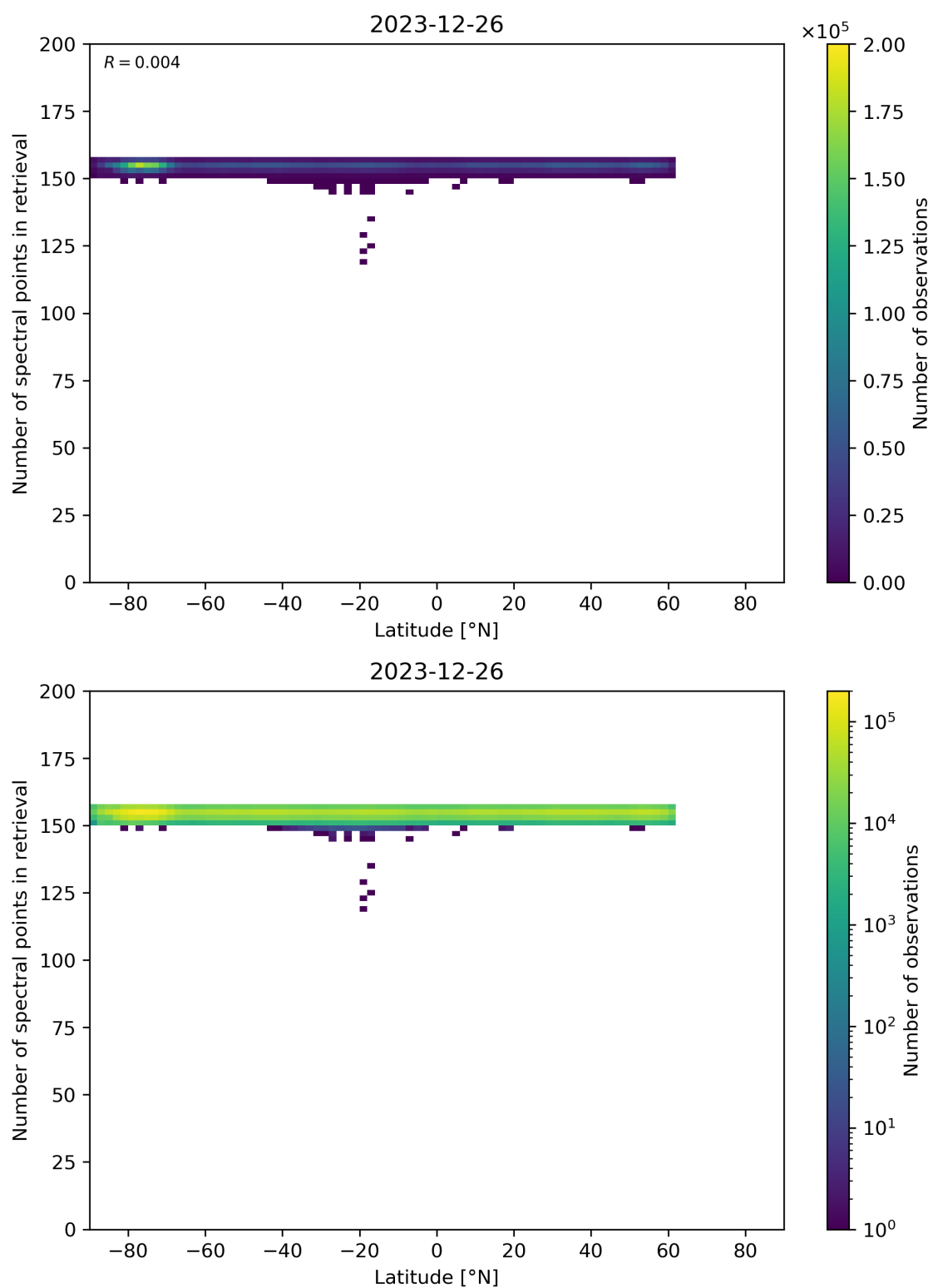
Figure 57: Scatter density plot of “Latitude” against “Number of spectral points in retrieval” for 2023-12-25 to 2023-12-27.
