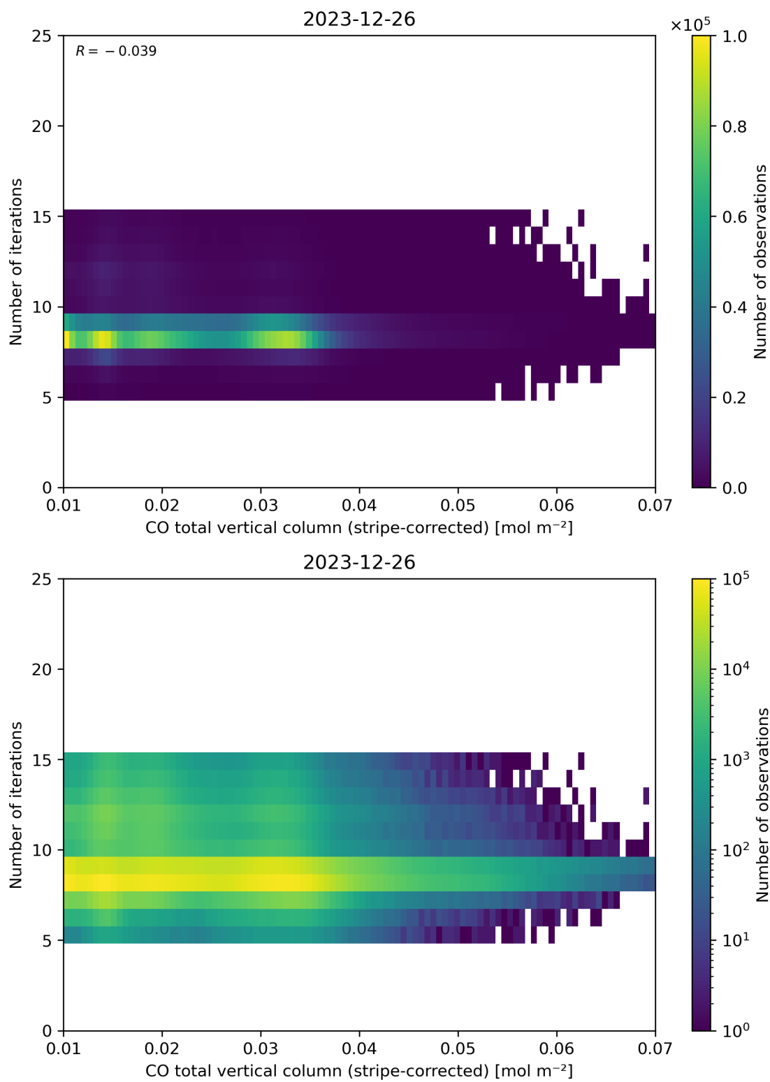
Figure 39: Scatter density plot of “CO total vertical column (stripe-corrected)” against “Number of iterations” for 2023-12-25 to 2023-12-27.
