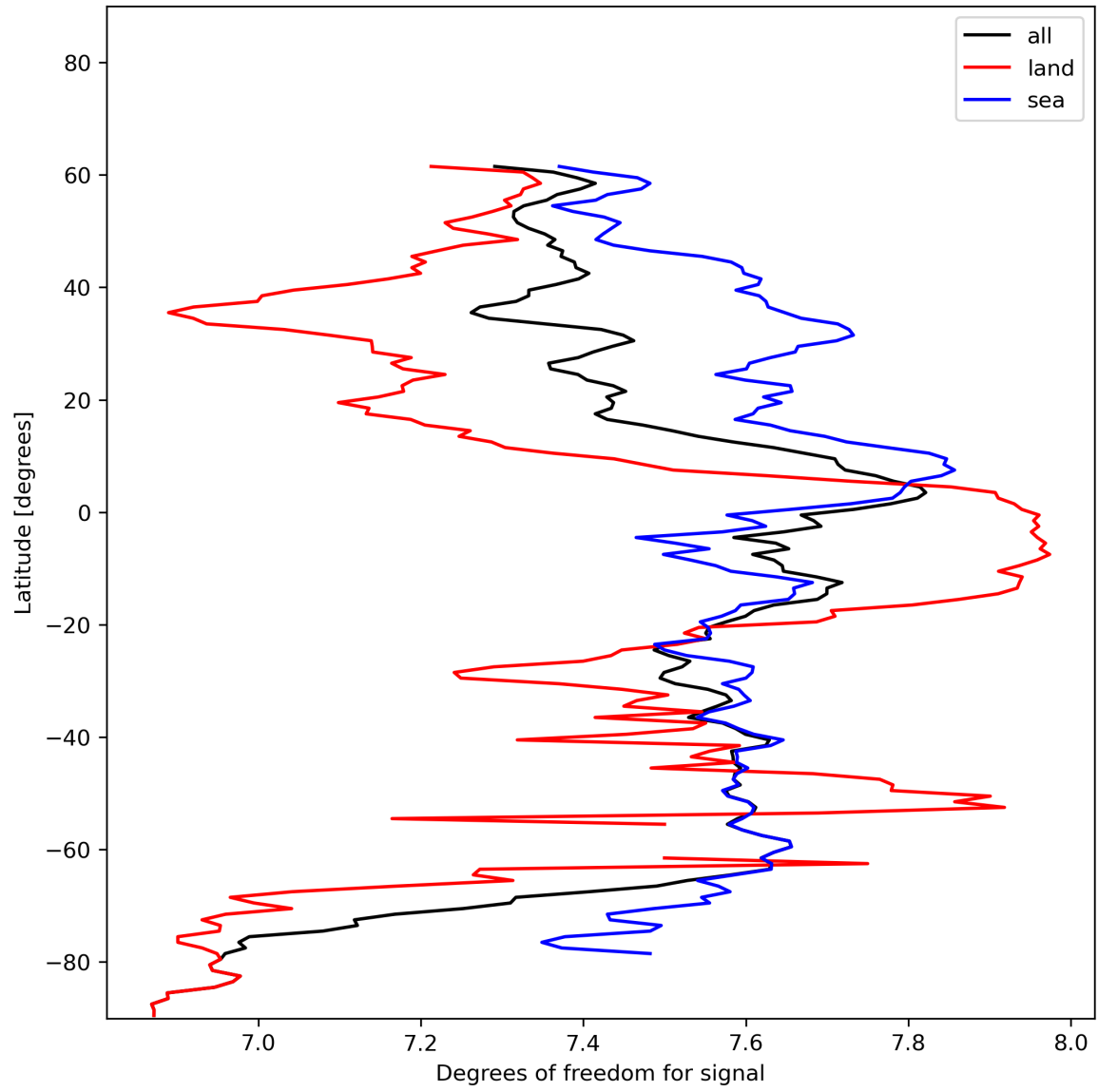
Figure 15: Zonal average of “Degrees of freedom for signal” for 2023-12-25 to 2023-12-27.
