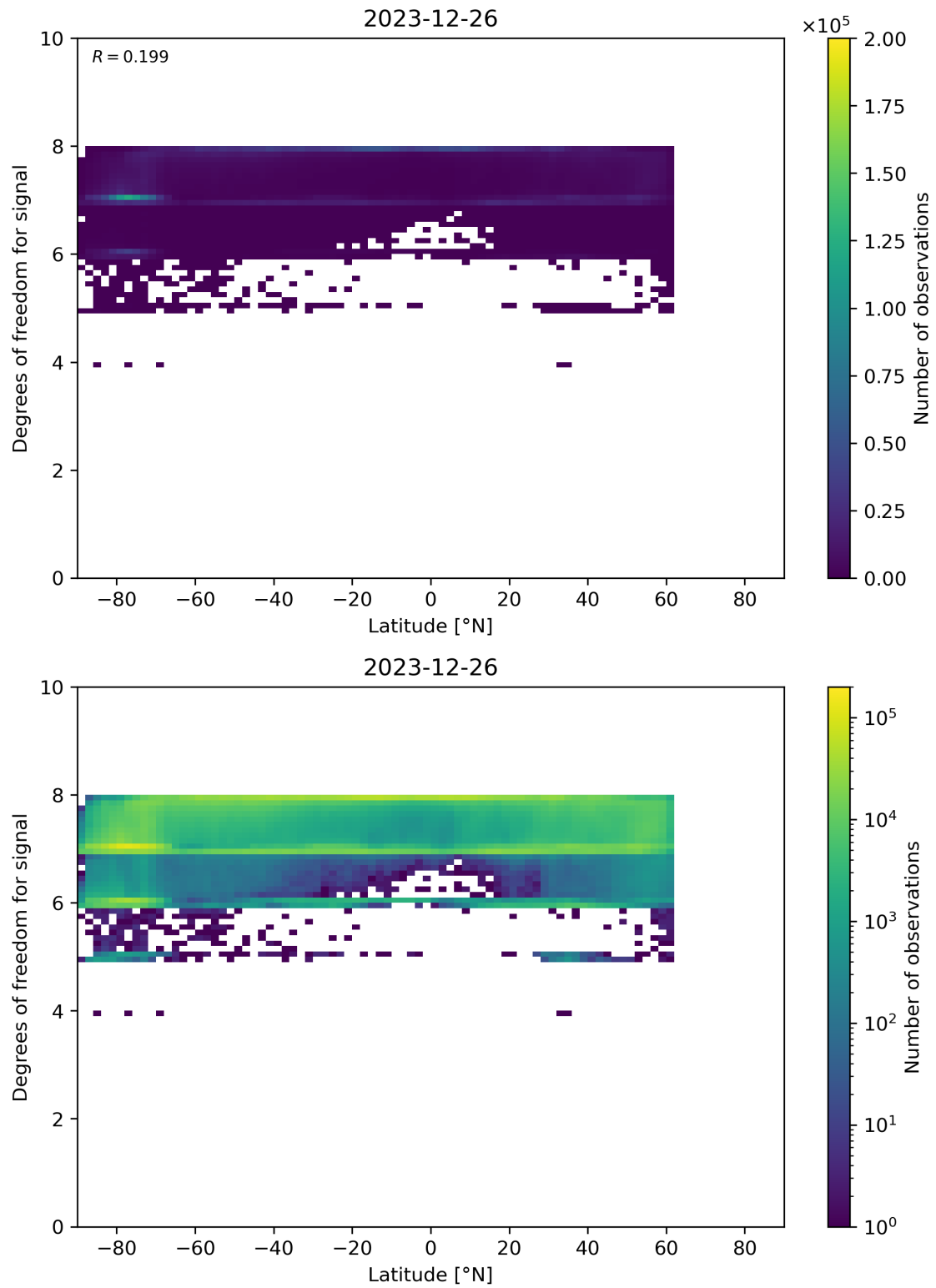
Figure 55: Scatter density plot of “Latitude” against “Degrees of freedom for signal” for 2023-12-25 to 2023-12-27.
