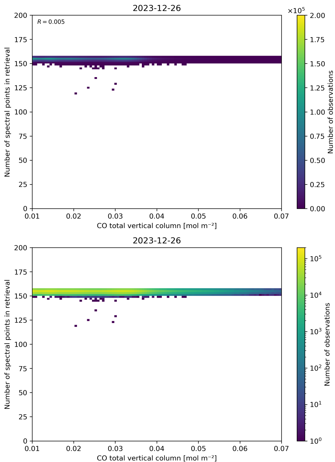
Figure 43: Scatter density plot of “CO total vertical column” against “Number of spectral points in retrieval” for 2023-12-25 to 2023-12-27.
