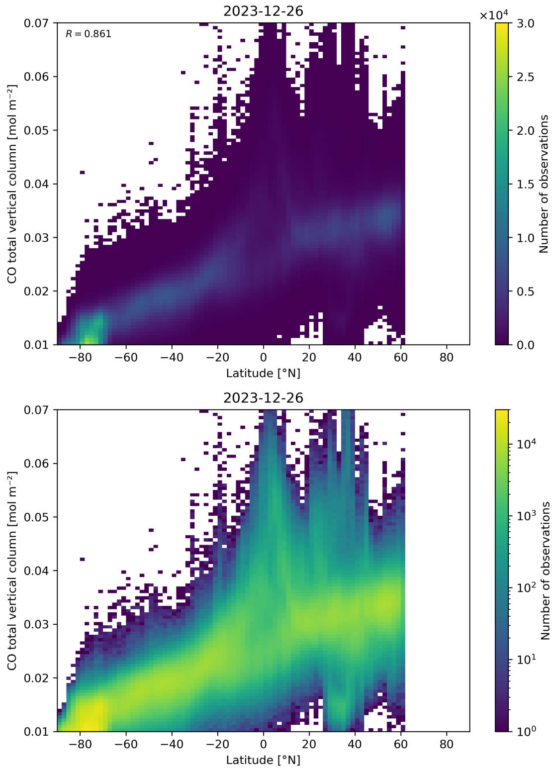
Figure 51: Scatter density plot of “Latitude” against “CO total vertical column” for 2023-12-25 to 2023-12-27.
