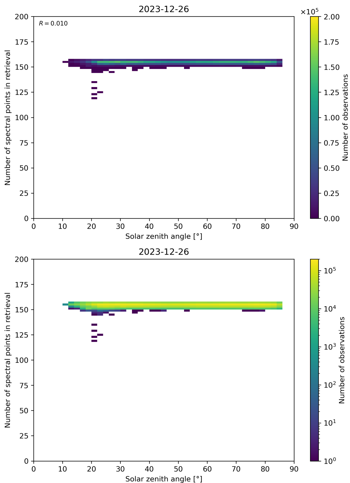
Figure 68: Scatter density plot of “Solar zenith angle” against “Number of spectral points in retrieval” for 2023-12-25 to 2023-12-27.
