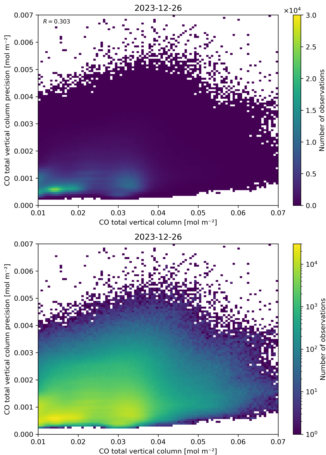
Figure 34: Scatter density plot of “CO total vertical column” against “CO total vertical column precision” for 2023-12-25 to 2023-12-27.
