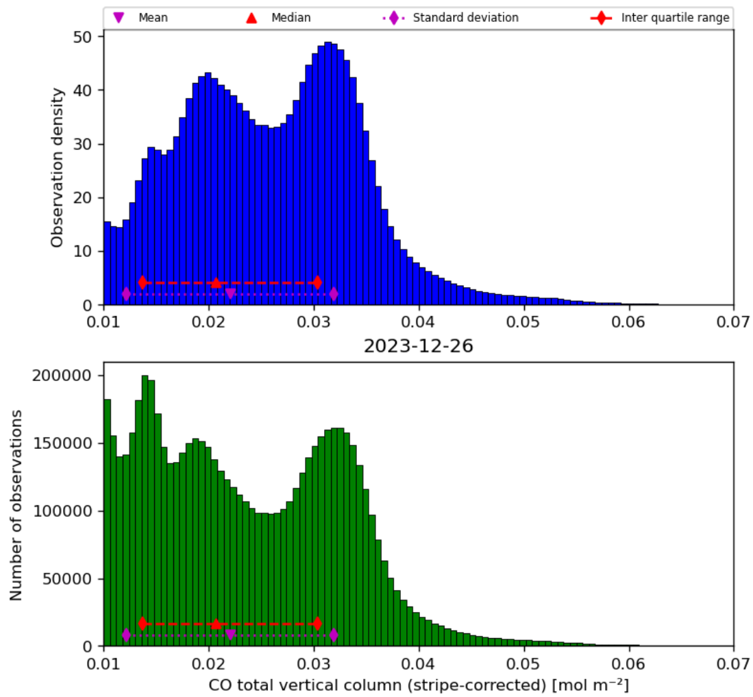
Figure 19: Histogram of “CO total vertical column (stripe-corrected)” for 2023-12-25 to 2023-12-27
