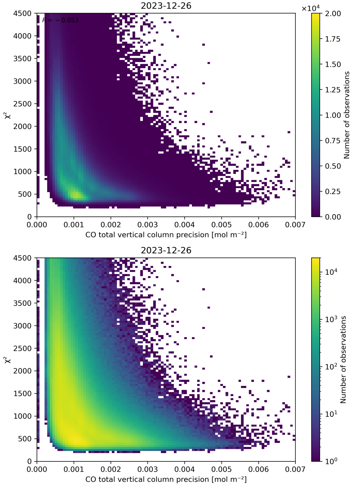
Figure 44: Scatter density plot of “CO total vertical column precision” against “ \chi^2 ” for 2023-12-25 to 2023-12-27.
