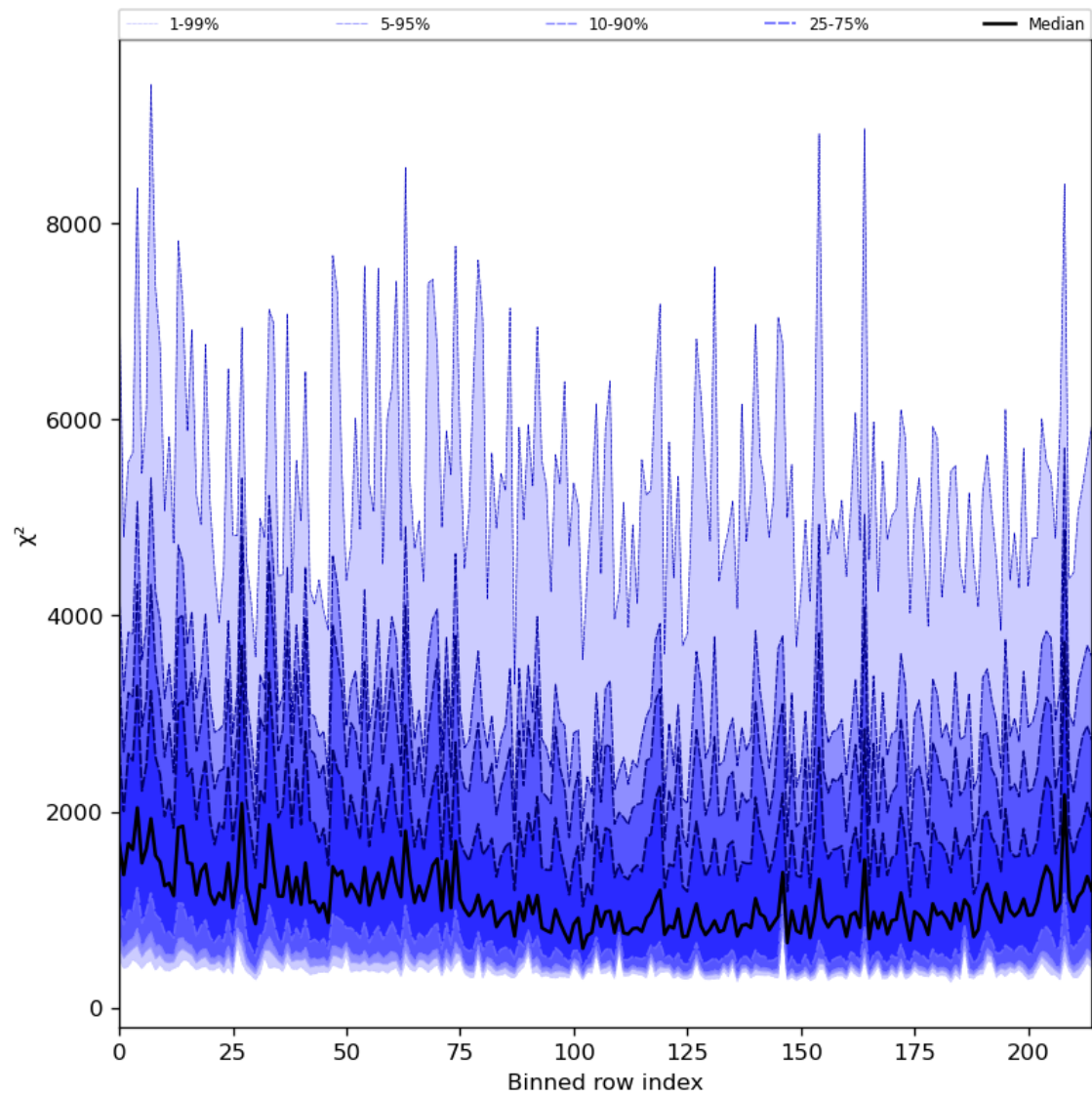
Figure 30: Along track statistics of “ \chi^2 ” for 2023-12-25 to 2023-12-27
