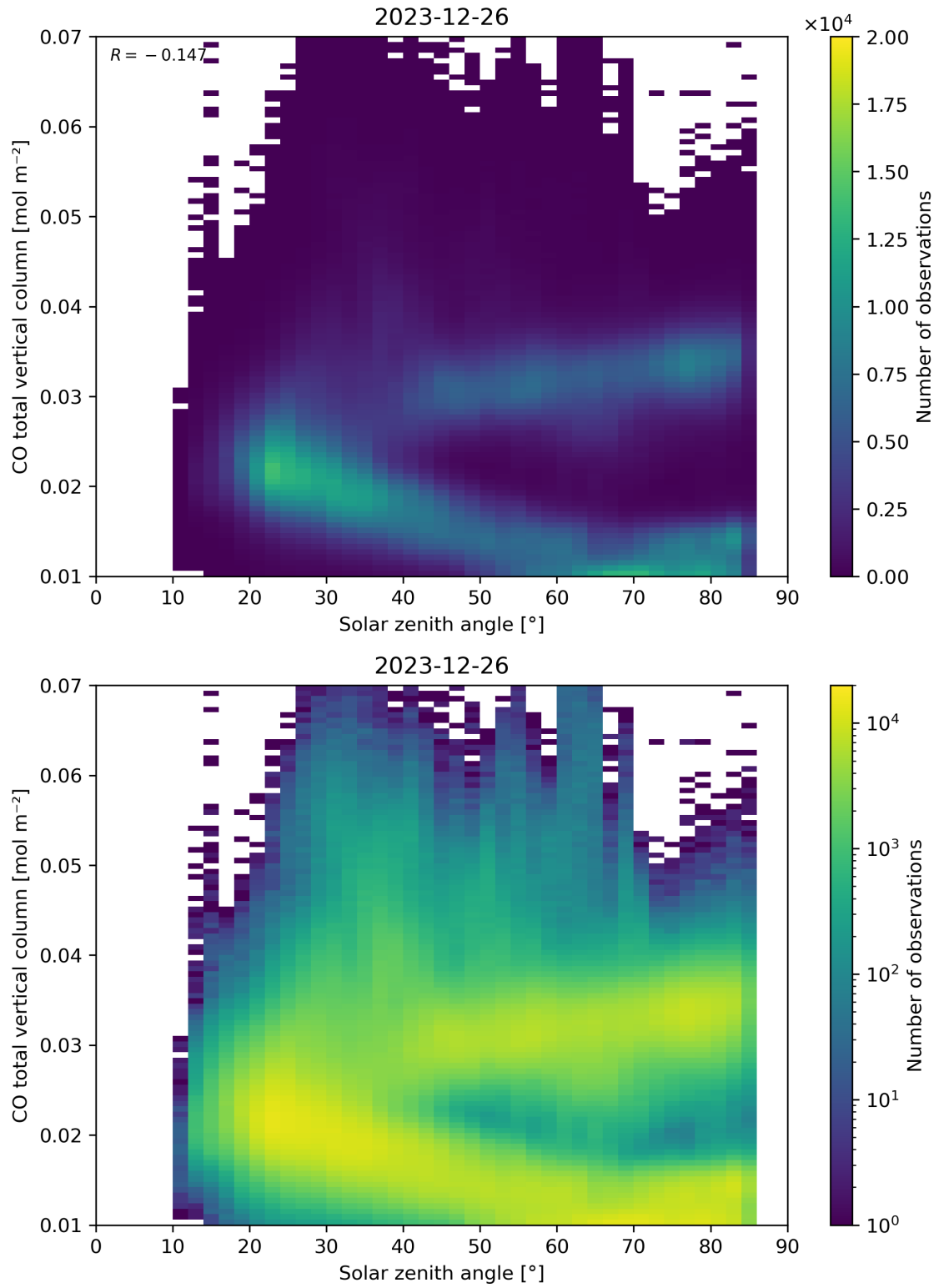
Figure 61: Scatter density plot of “Solar zenith angle” against “CO total vertical column” for 2023-12-25 to 2023-12-27.
