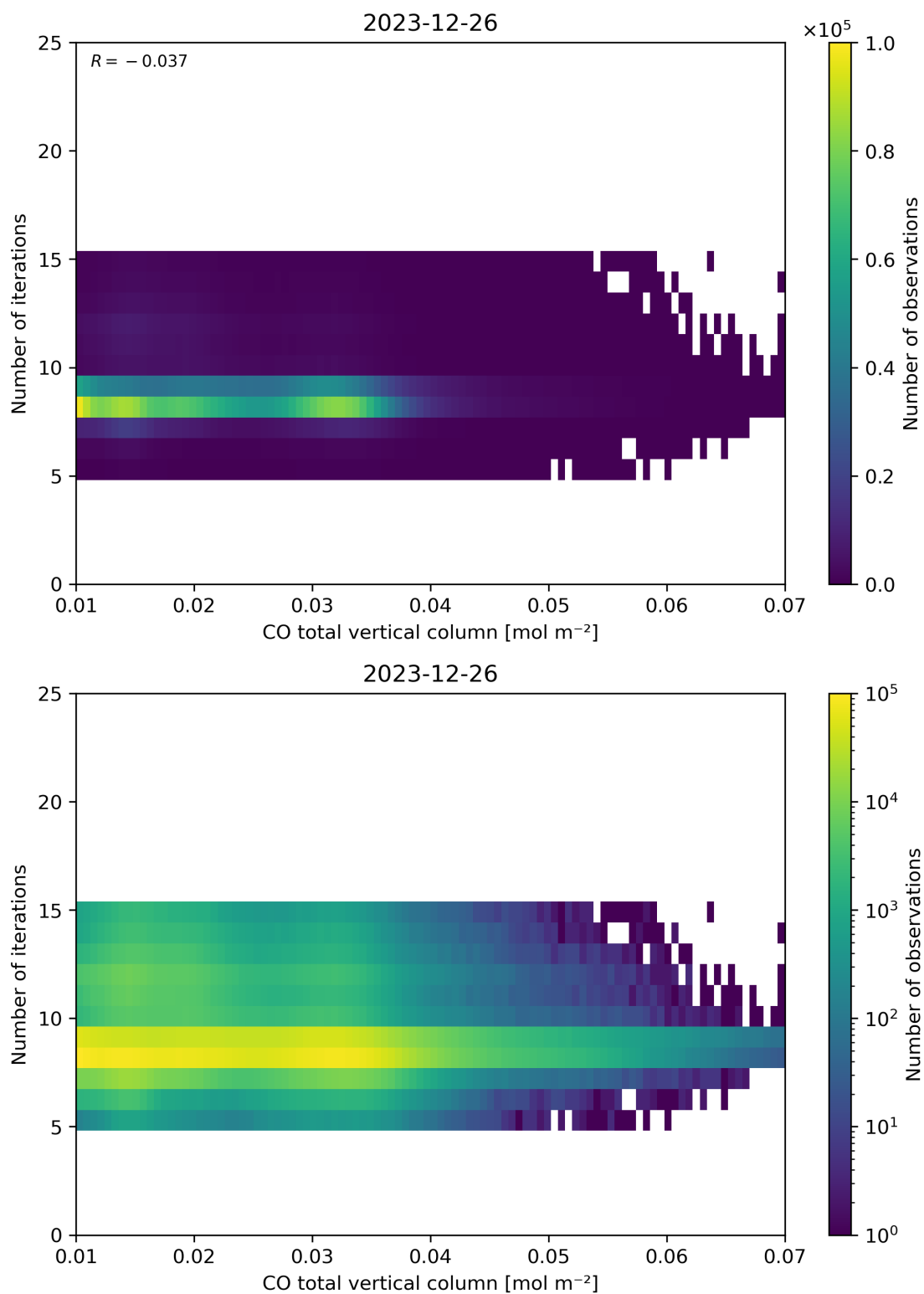
Figure 42: Scatter density plot of “CO total vertical column” against “Number of iterations” for 2023-12-25 to 2023-12-27.
