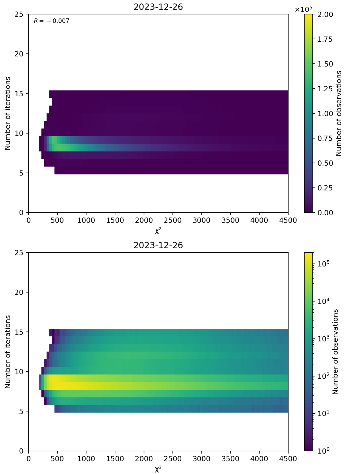
Figure 49: Scatter density plot of “ \chi^2 ” against “Number of iterations” for 2023-12-25 to 2023-12-27.
