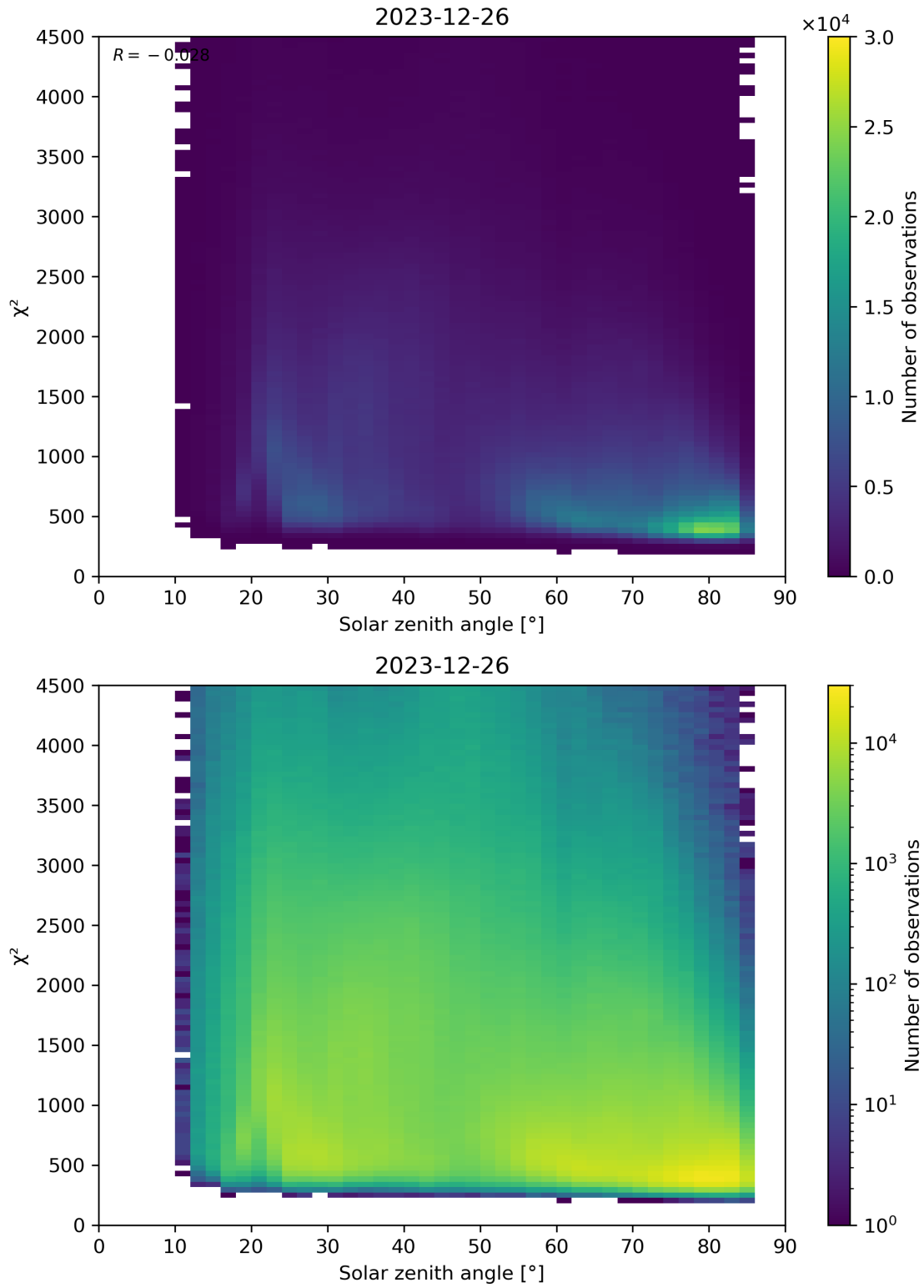
Figure 64: Scatter density plot of “Solar zenith angle” against “ \chi^2 ” for 2023-12-25 to 2023-12-27.
