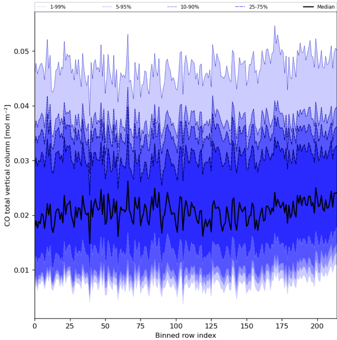
Figure 26: Along track statistics of “CO total vertical column” for 2023-12-25 to 2023-12-27
