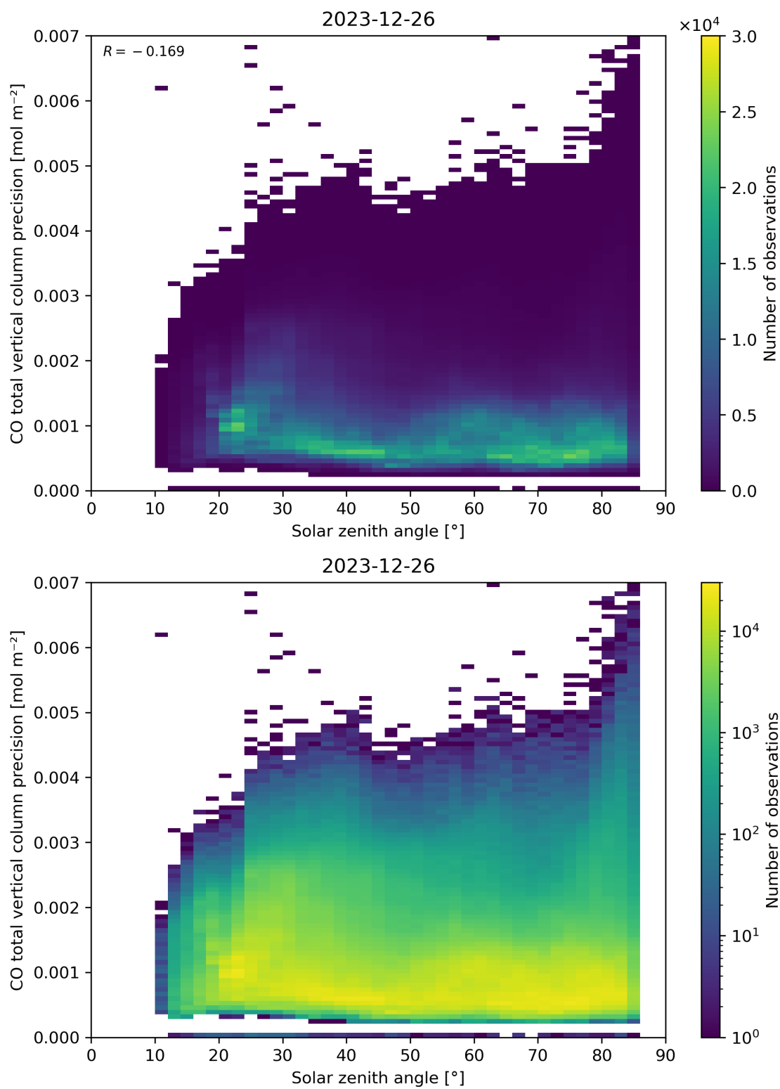
Figure 63: Scatter density plot of “Solar zenith angle” against “CO total vertical column precision” for 2023-12-25 to 2023-12-27.
