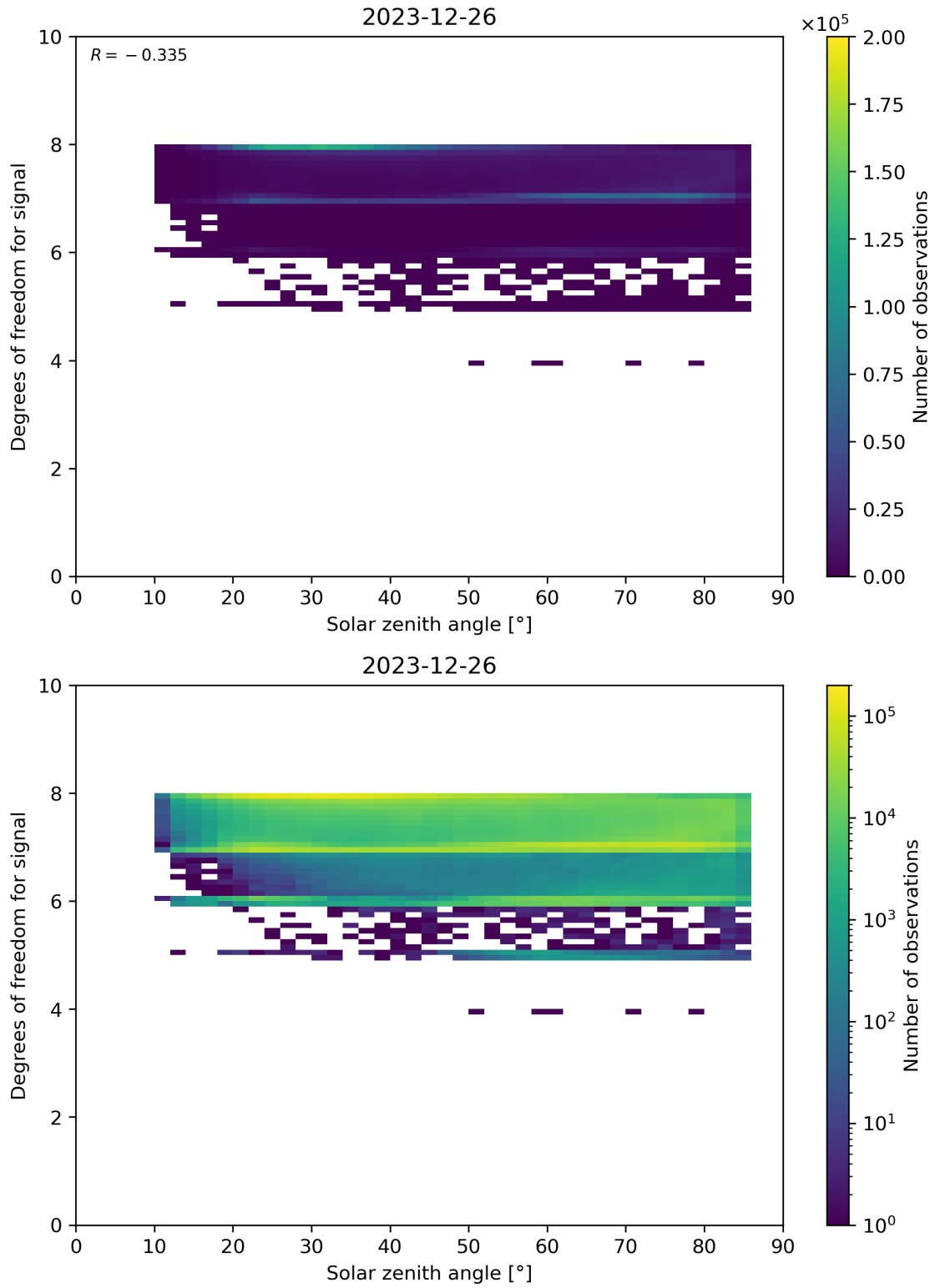
Figure 65: Scatter density plot of “Solar zenith angle” against “Degrees of freedom for signal” for 2023-12-25 to 2023-12-27.
