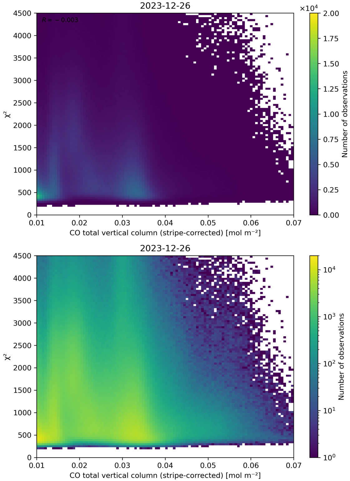
Figure 37: Scatter density plot of “CO total vertical column (stripe-corrected)” against “ \chi^2 ” for 2023-12-25 to 2023-12-27.
