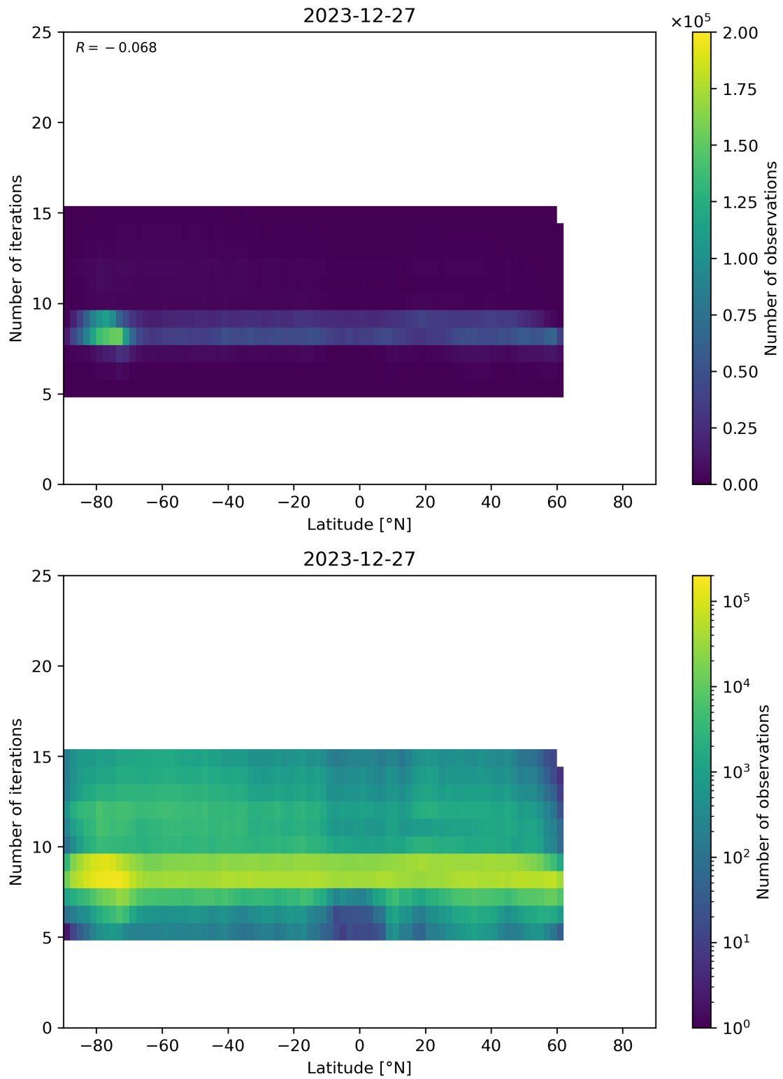
Figure 56: Scatter density plot of “Latitude” against “Number of iterations” for 2023-12-26 to 2023-12-28.
