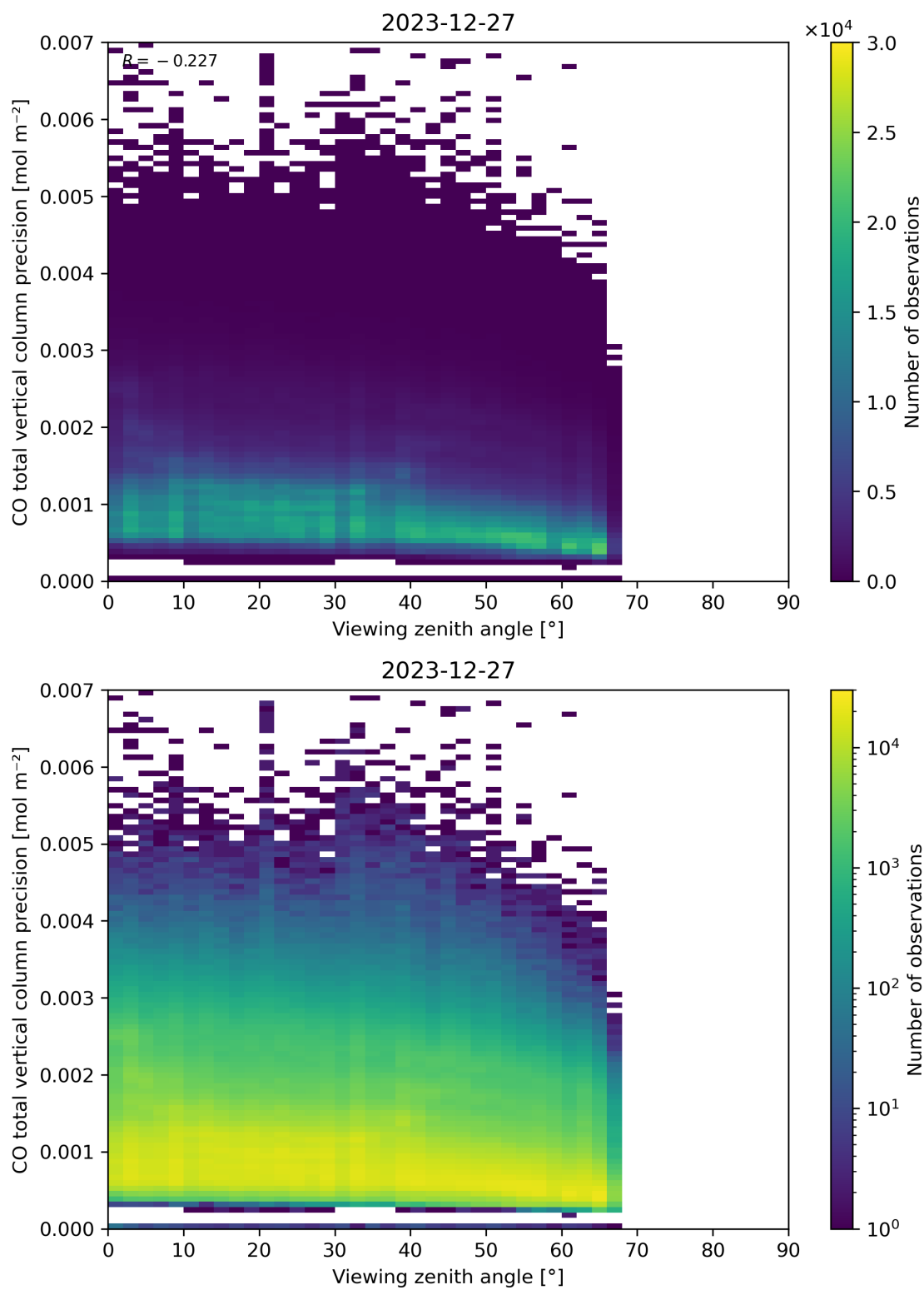
Figure 71: Scatter density plot of “Viewing zenith angle” against “CO total vertical column precision” for 2023-12-26 to 2023-12-28.
