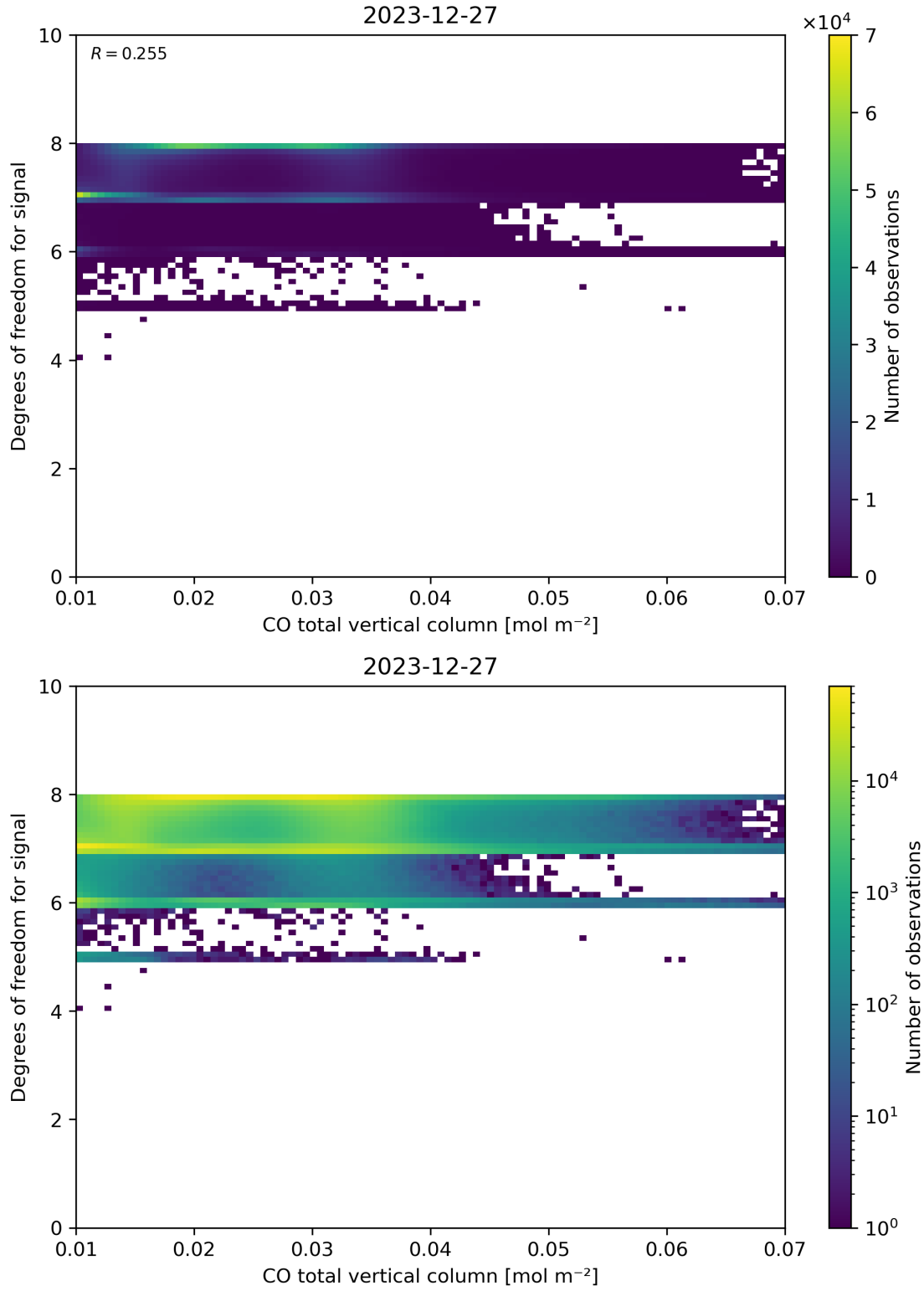
Figure 41: Scatter density plot of “CO total vertical column” against “Degrees of freedom for signal” for 2023-12-26 to 2023-12-28.
