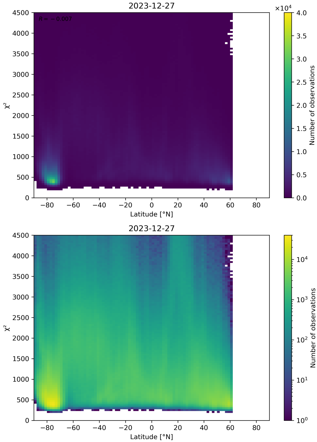
Figure 54: Scatter density plot of “Latitude” against “ \chi^2 ” for 2023-12-26 to 2023-12-28.
