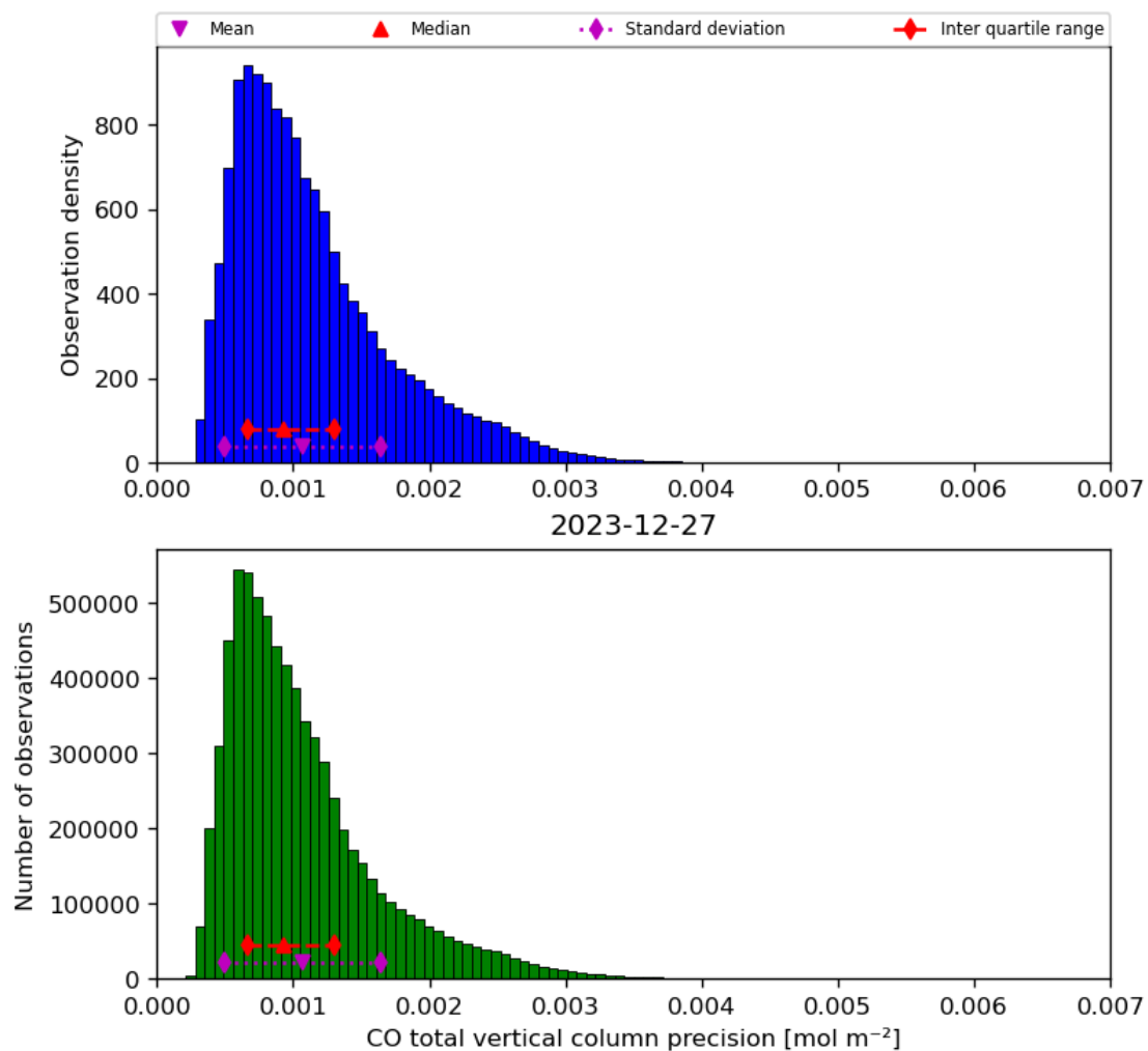
Figure 20: Histogram of “CO total vertical column precision” for 2023-12-26 to 2023-12-28
