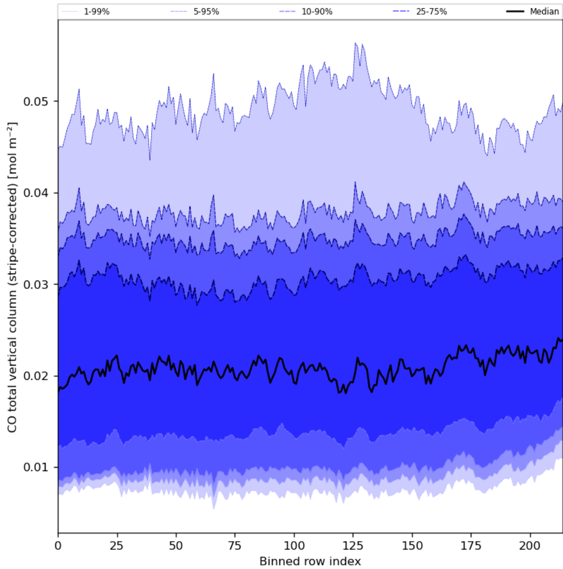
Figure 27: Along track statistics of “CO total vertical column (stripe-corrected)” for 2023-12-26 to 2023-12-28
