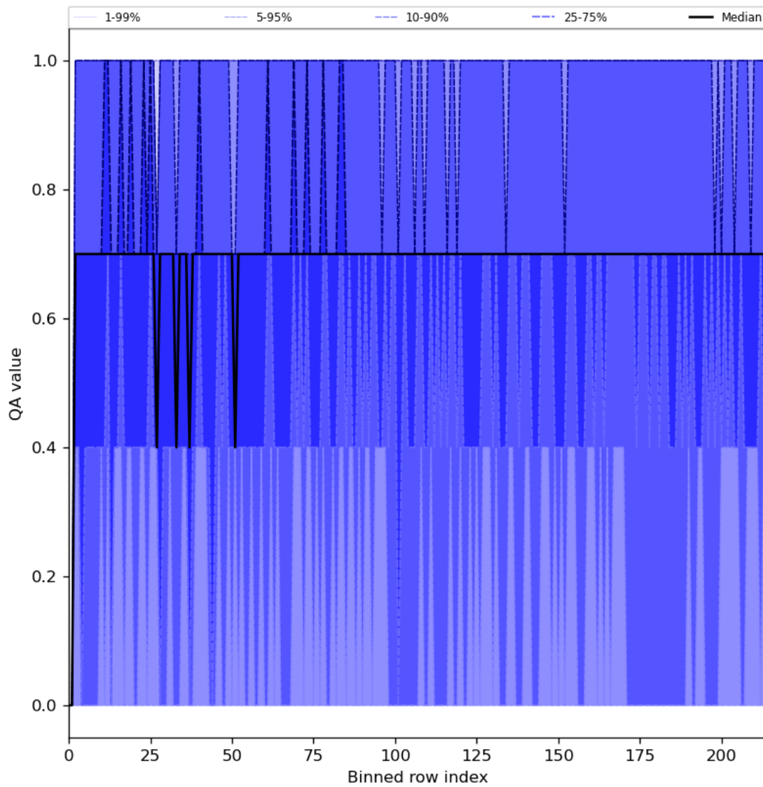
Figure 25: Along track statistics of “QA value” for 2023-12-26 to 2023-12-28
