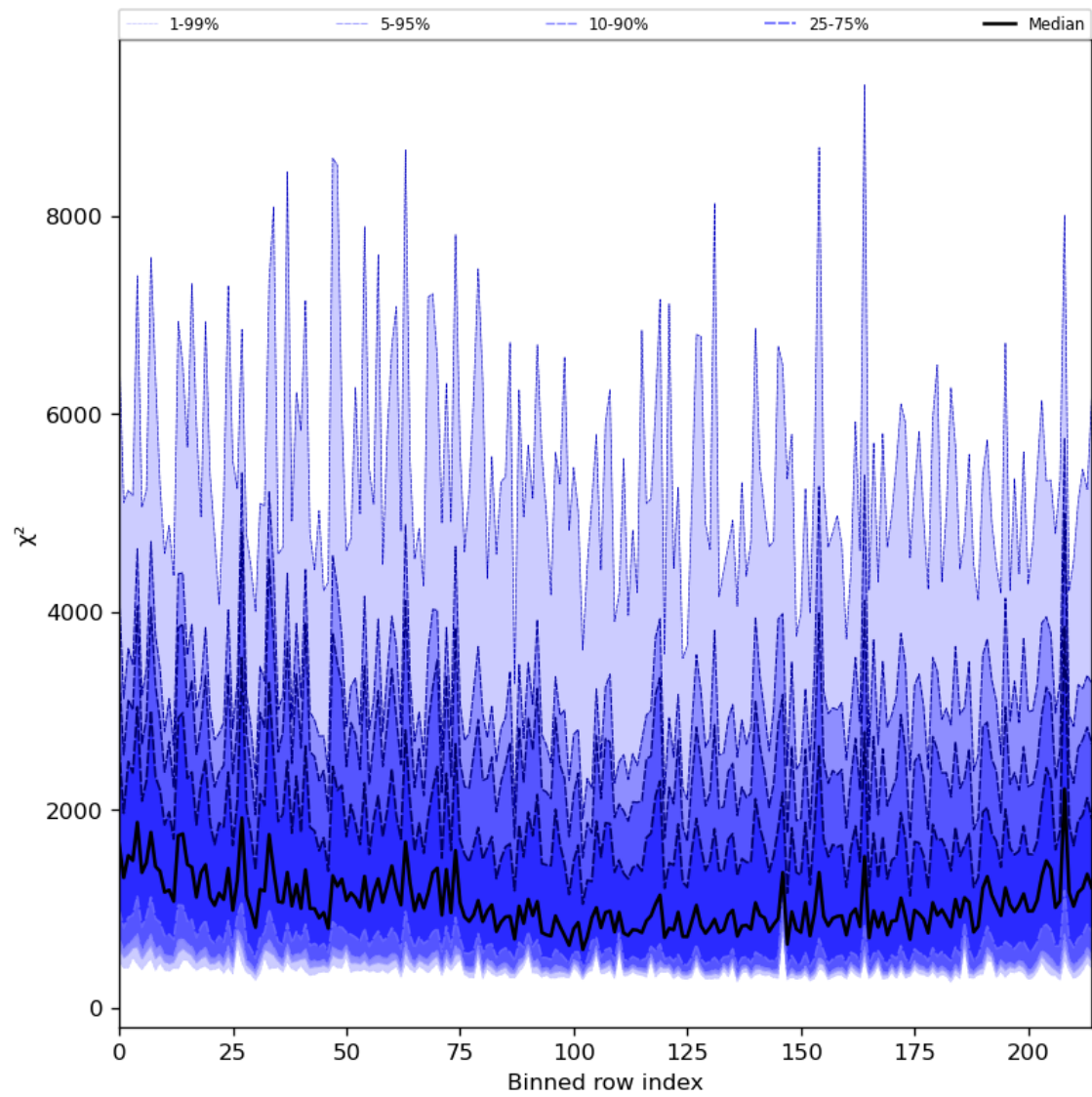
Figure 30: Along track statistics of “ \chi^2 ” for 2023-12-26 to 2023-12-28
