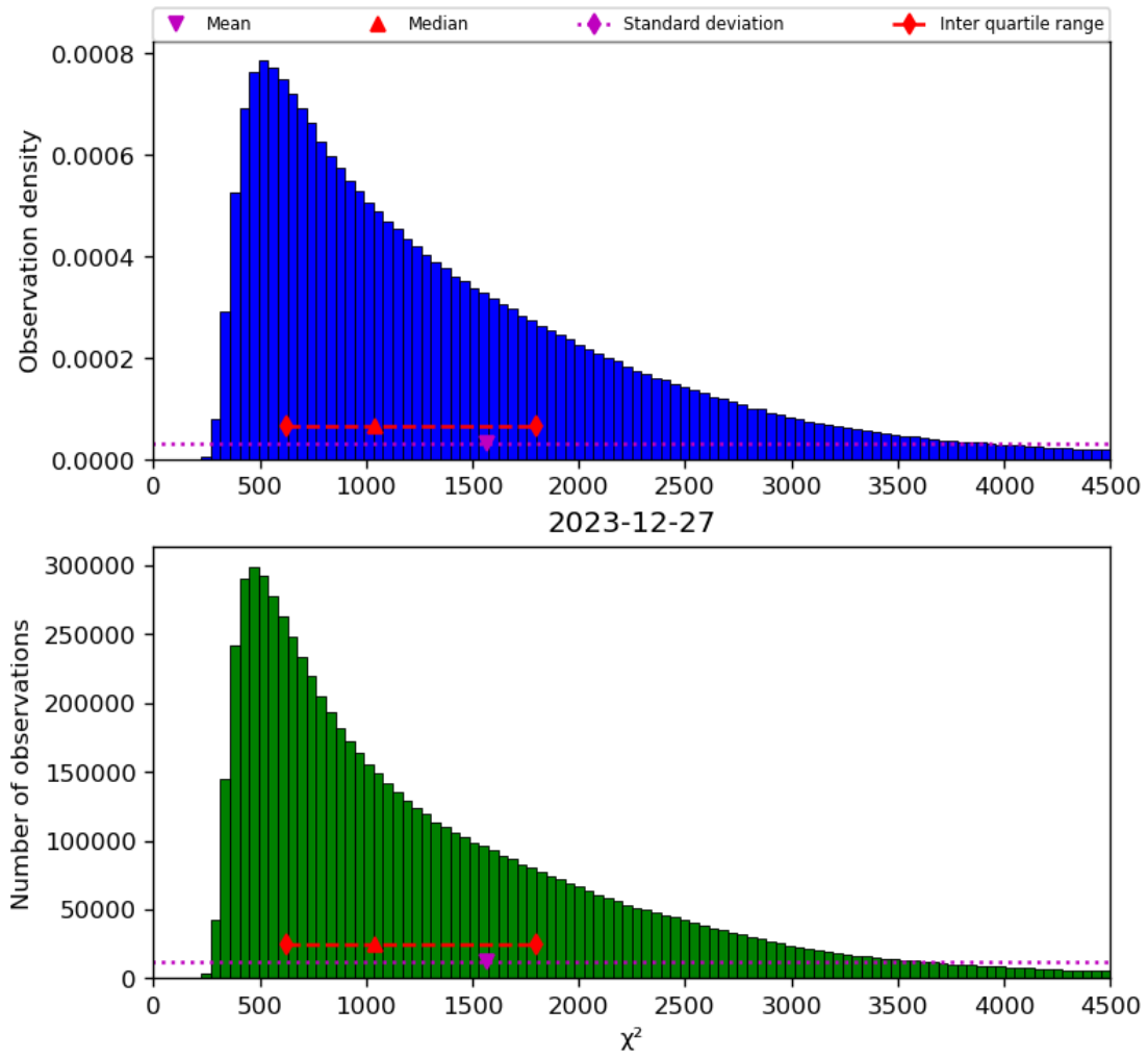
Figure 22: Histogram of “ \chi^2 ” for 2023-12-26 to 2023-12-28
