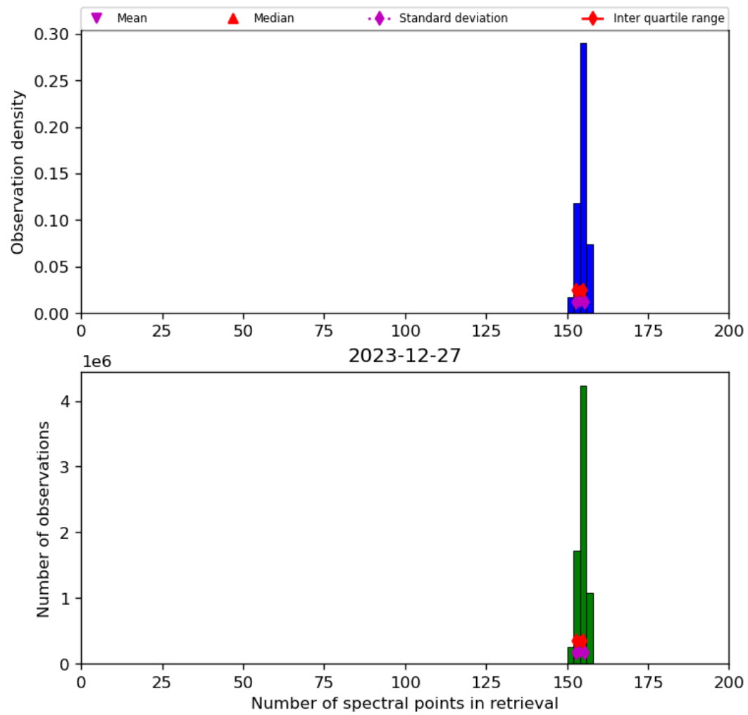
Figure 21: Histogram of “Number of spectral points in retrieval” for 2023-12-26 to 2023-12-28
