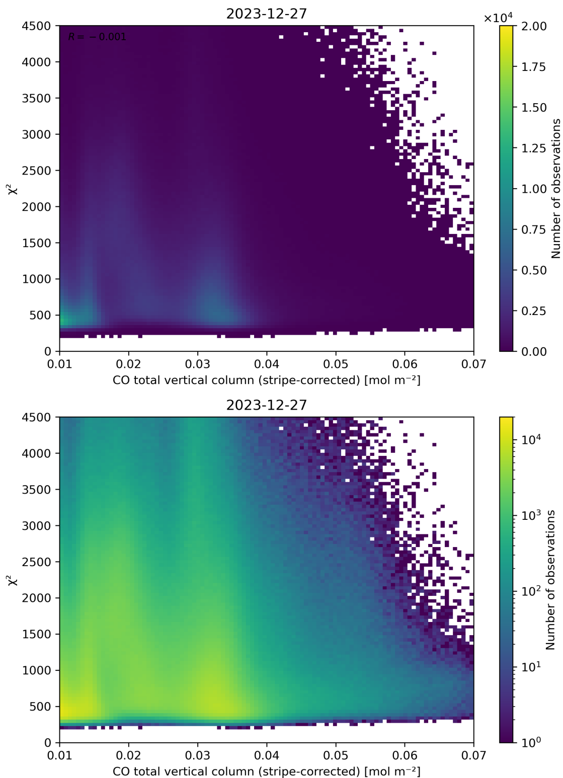
Figure 37: Scatter density plot of “CO total vertical column (stripe-corrected)” against “ \chi^2 ” for 2023-12-26 to 2023-12-28.
