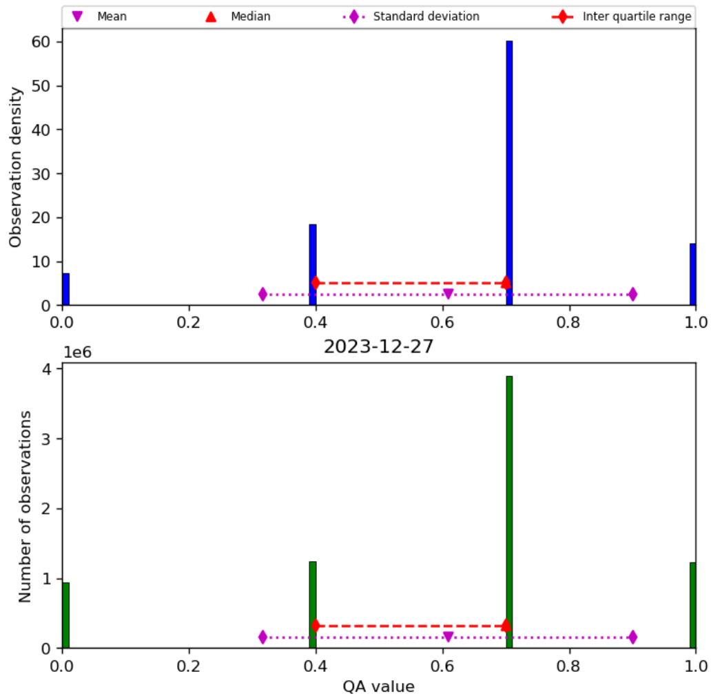
Figure 17: Histogram of “QA value” for 2023-12-26 to 2023-12-28
