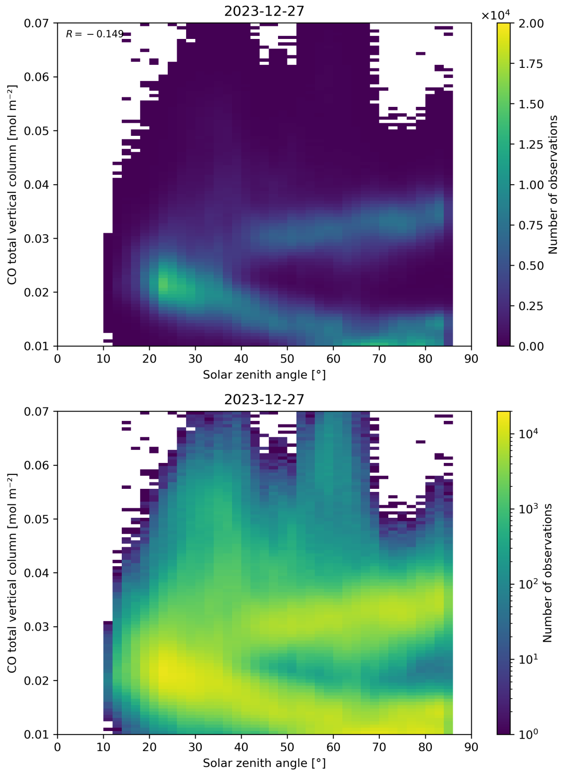
Figure 61: Scatter density plot of “Solar zenith angle” against “CO total vertical column” for 2023-12-26 to 2023-12-28.
