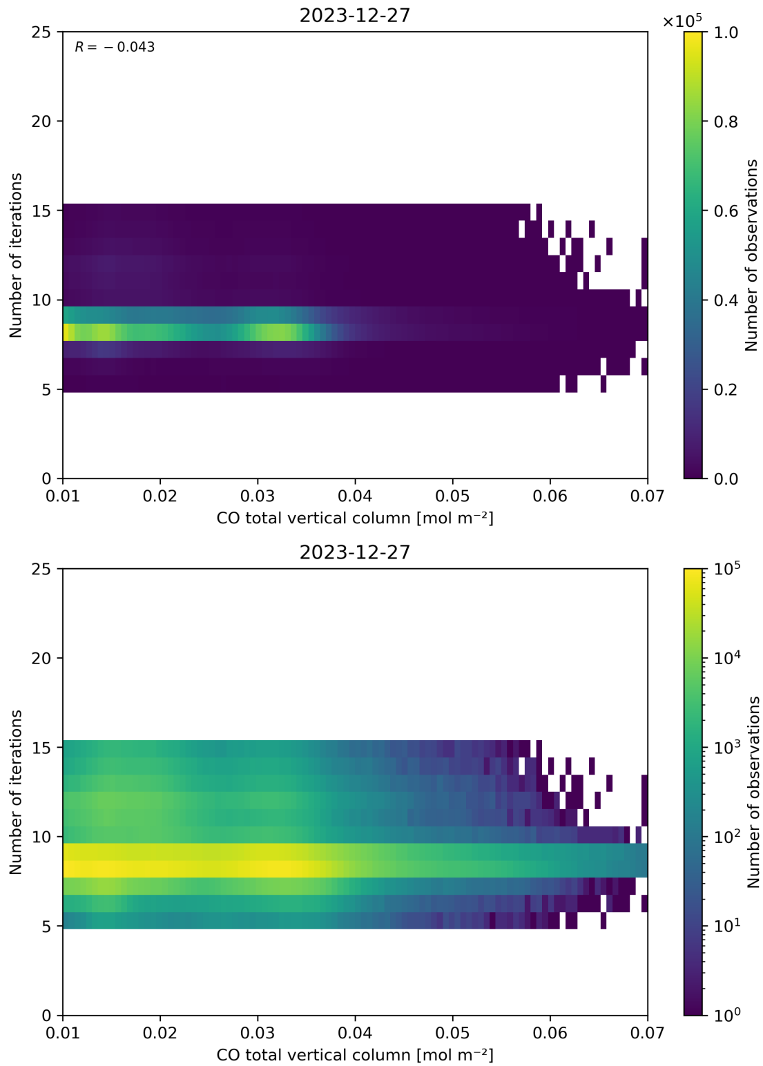
Figure 42: Scatter density plot of “CO total vertical column” against “Number of iterations” for 2023-12-26 to 2023-12-28.
