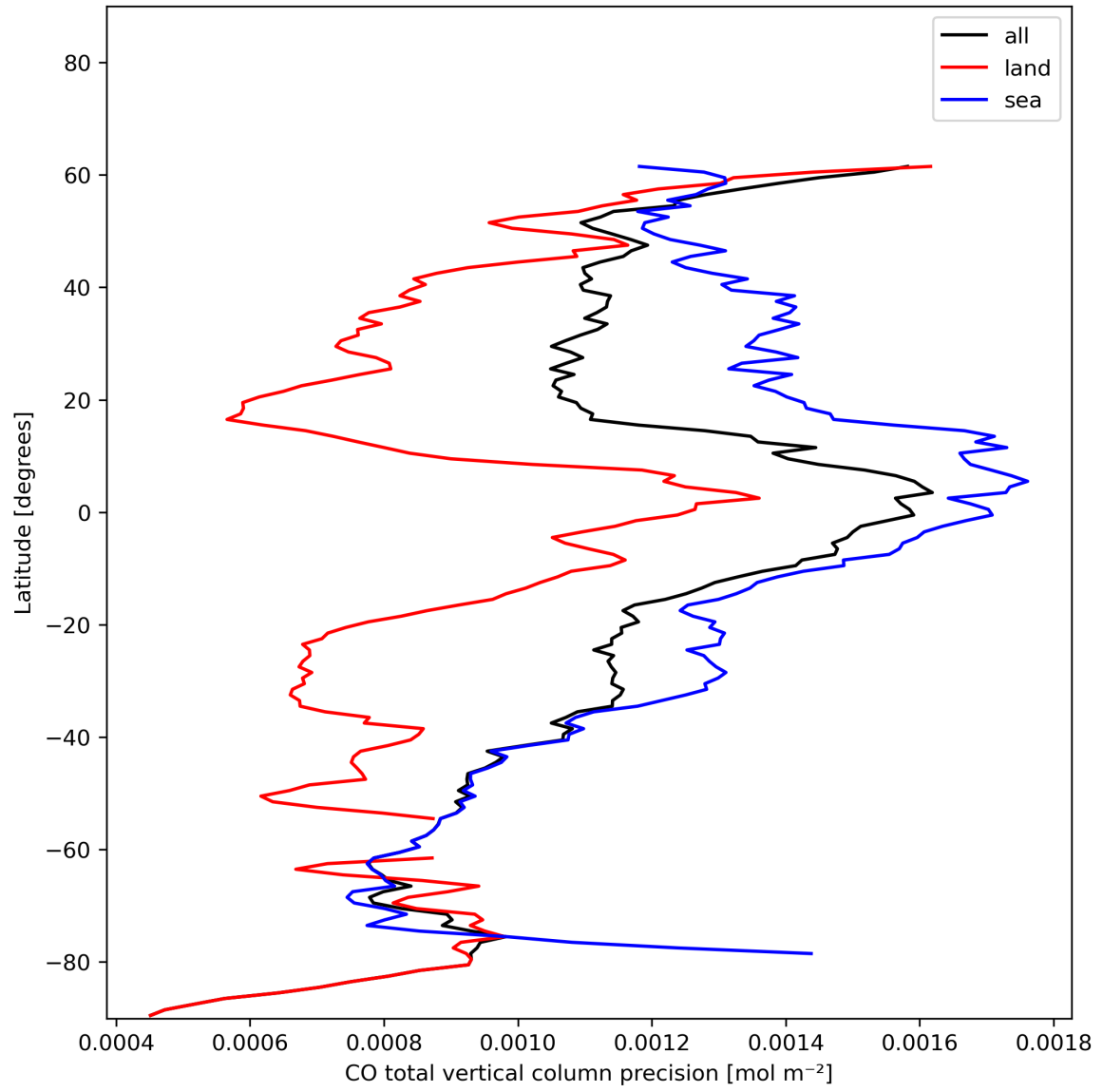
Figure 12: Zonal average of “CO total vertical column precision” for 2023-12-26 to 2023-12-28.
