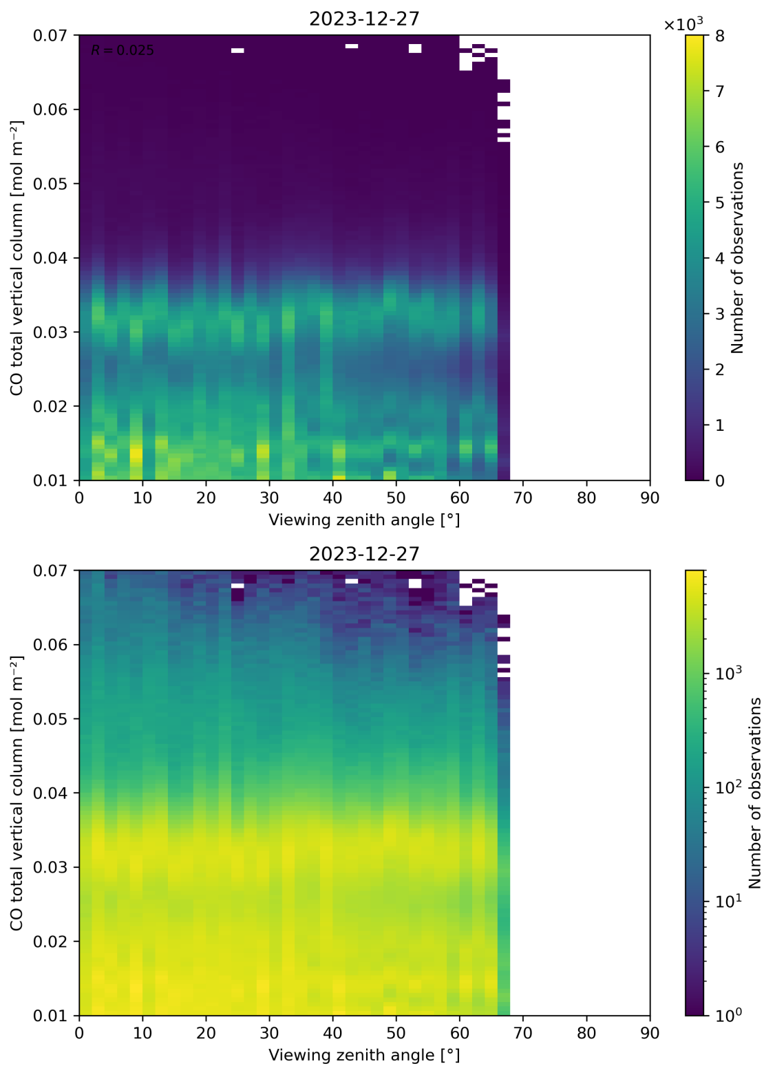
Figure 69: Scatter density plot of “Viewing zenith angle” against “CO total vertical column” for 2023-12-26 to 2023-12-28.
