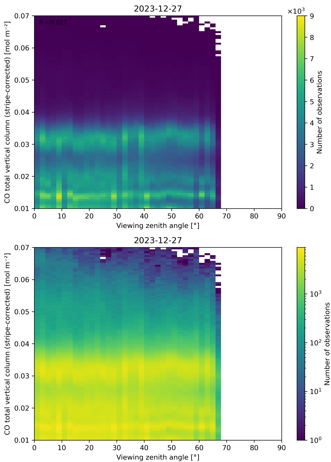
Figure 70: Scatter density plot of “Viewing zenith angle” against “CO total vertical column (stripe-corrected)” for 2023-12-26 to 2023-12-28.
