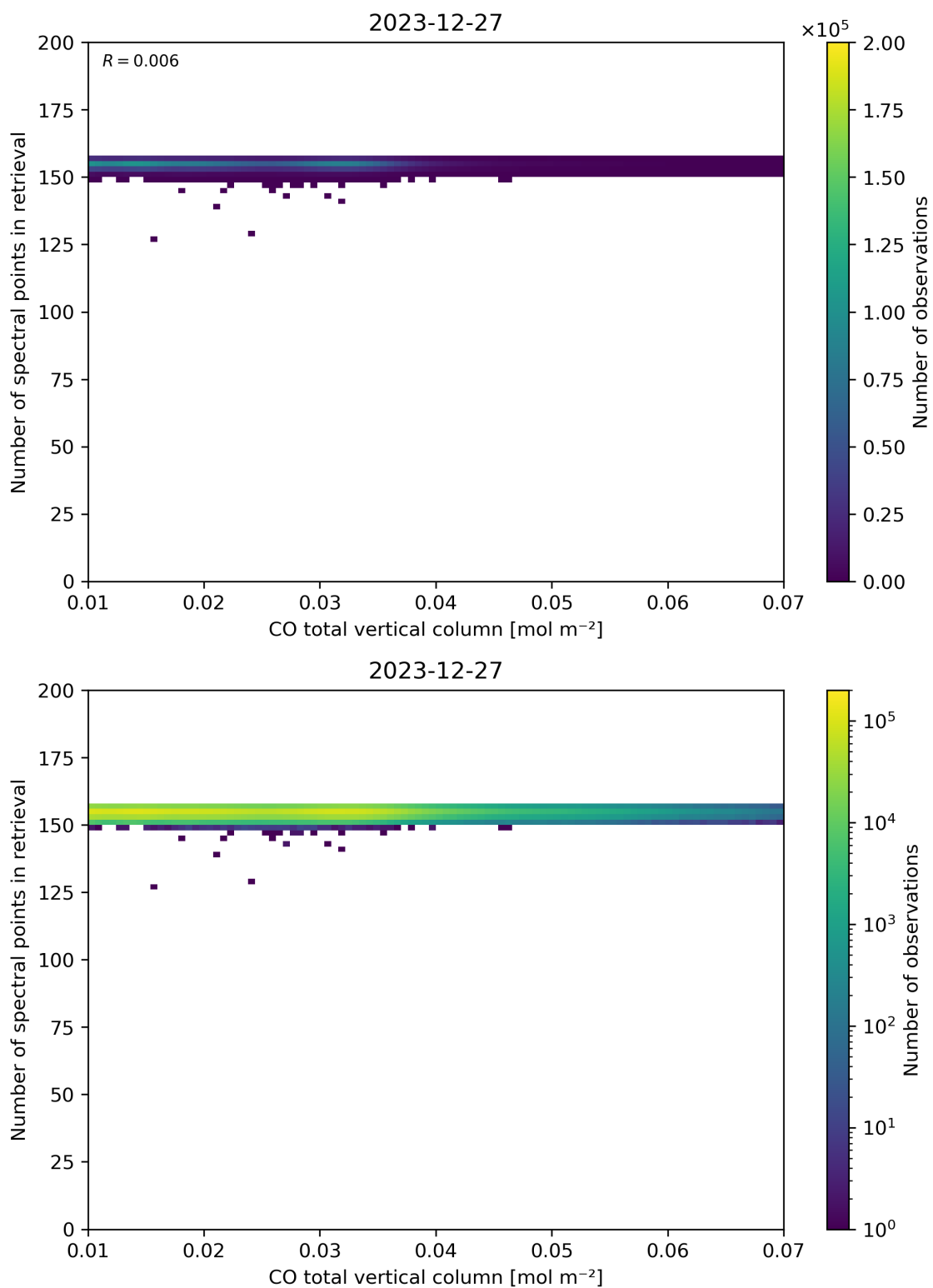
Figure 43: Scatter density plot of “CO total vertical column” against “Number of spectral points in retrieval” for 2023-12-26 to 2023-12-28.
