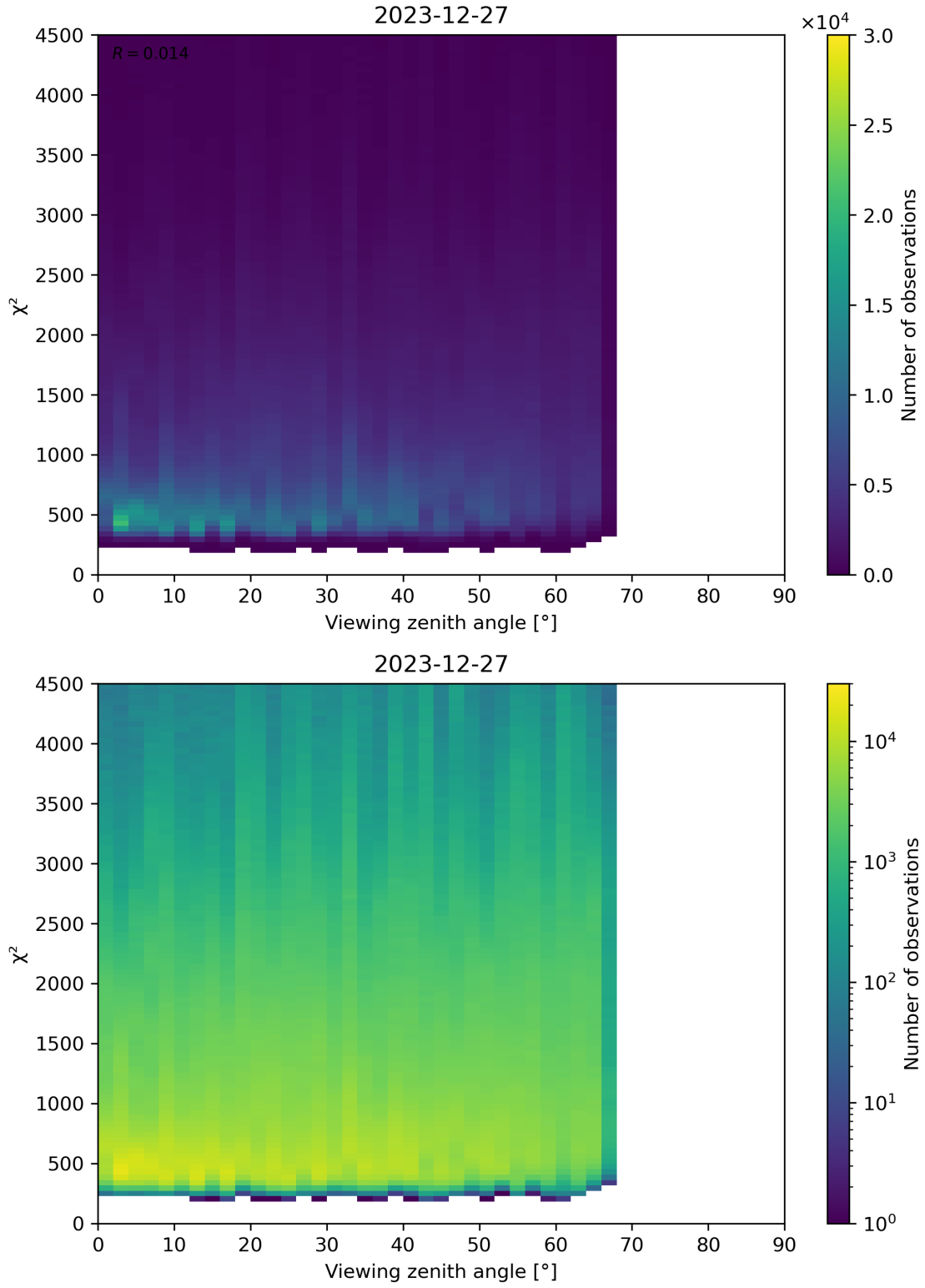
Figure 72: Scatter density plot of “Viewing zenith angle” against “ \chi^2 ” for 2023-12-26 to 2023-12-28.
