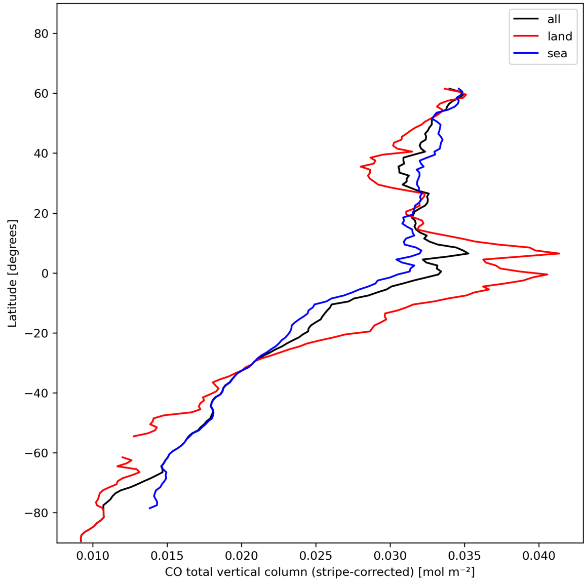
Figure 11: Zonal average of “CO total vertical column (stripe-corrected)” for 2023-12-26 to 2023-12-28.
