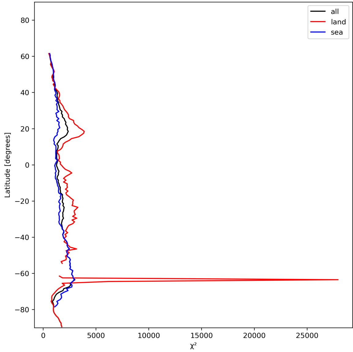
Figure 14: Zonal average of “ \chi^2 ” for 2023-12-26 to 2023-12-28.
