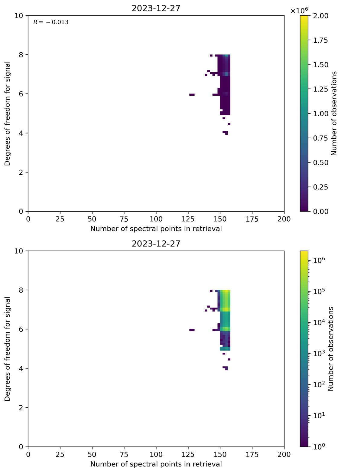
Figure 59: Scatter density plot of “Number of spectral points in retrieval” against “Degrees of freedom for signal” for 2023-12-26 to 2023-12-28.
