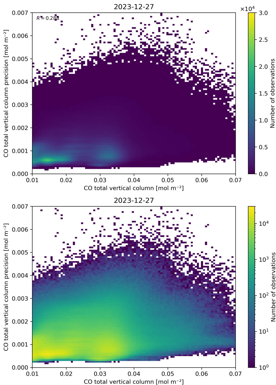
Figure 34: Scatter density plot of “CO total vertical column” against “CO total vertical column precision” for 2023-12-26 to 2023-12-28.
