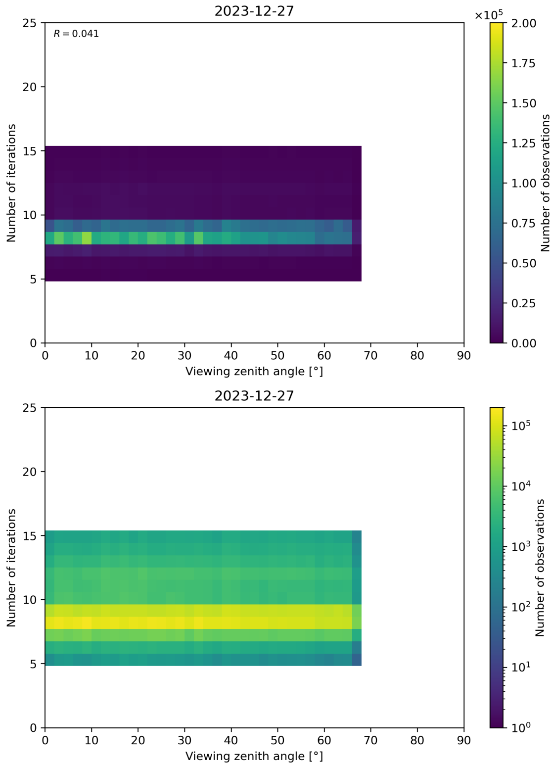
Figure 75: Scatter density plot of “Viewing zenith angle” against “Number of iterations” for 2023-12-26 to 2023-12-28.
