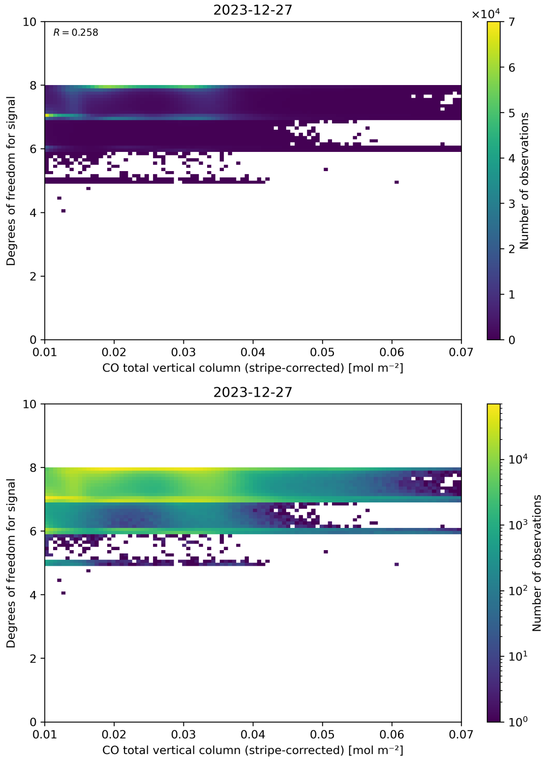
Figure 38: Scatter density plot of “CO total vertical column (stripe-corrected)” against “Degrees of freedom for signal” for 2023-12-26 to 2023-12-28.
