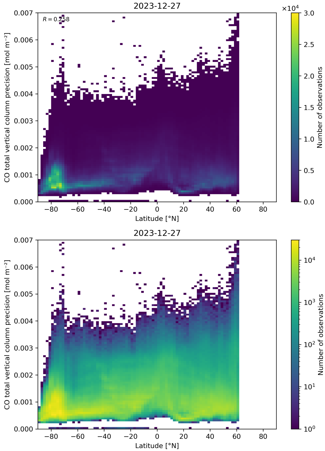
Figure 53: Scatter density plot of “Latitude” against “CO total vertical column precision” for 2023-12-26 to 2023-12-28.
