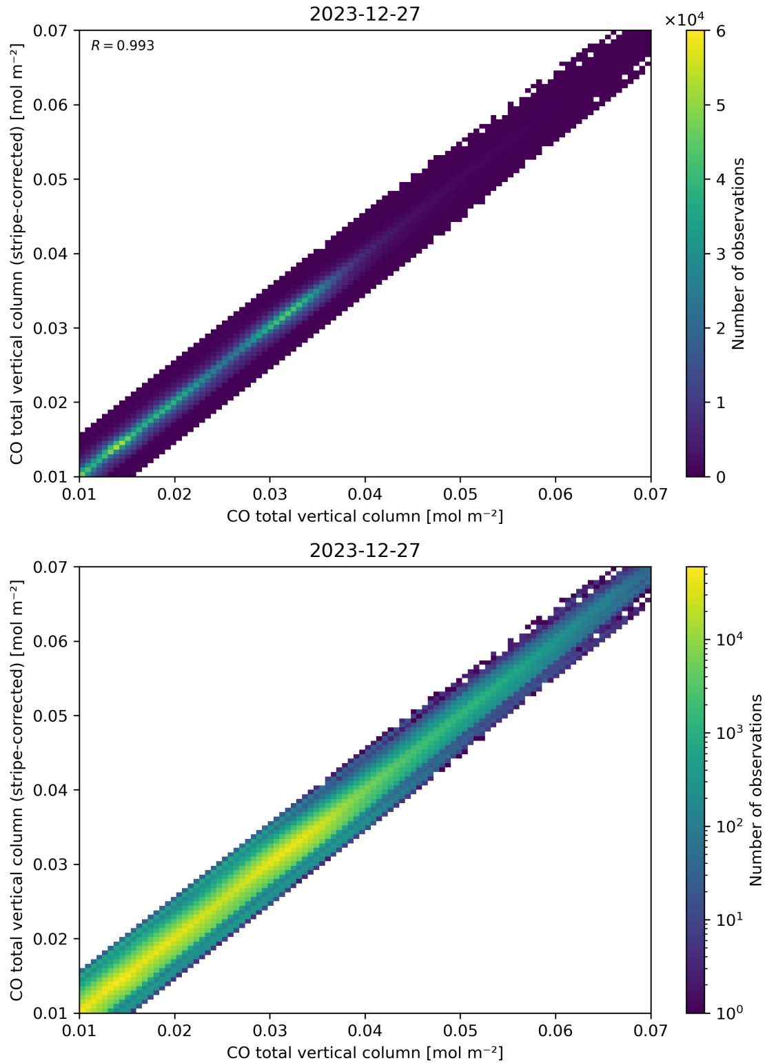
Figure 33: Scatter density plot of “CO total vertical column” against “CO total vertical column (stripe-corrected)” for 2023-12-26 to 2023-12-28.
