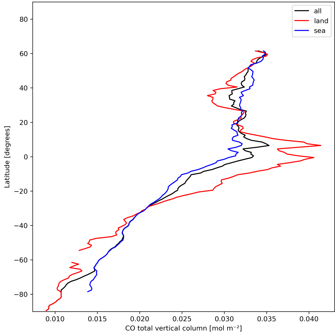
Figure 10: Zonal average of “CO total vertical column” for 2023-12-26 to 2023-12-28.
