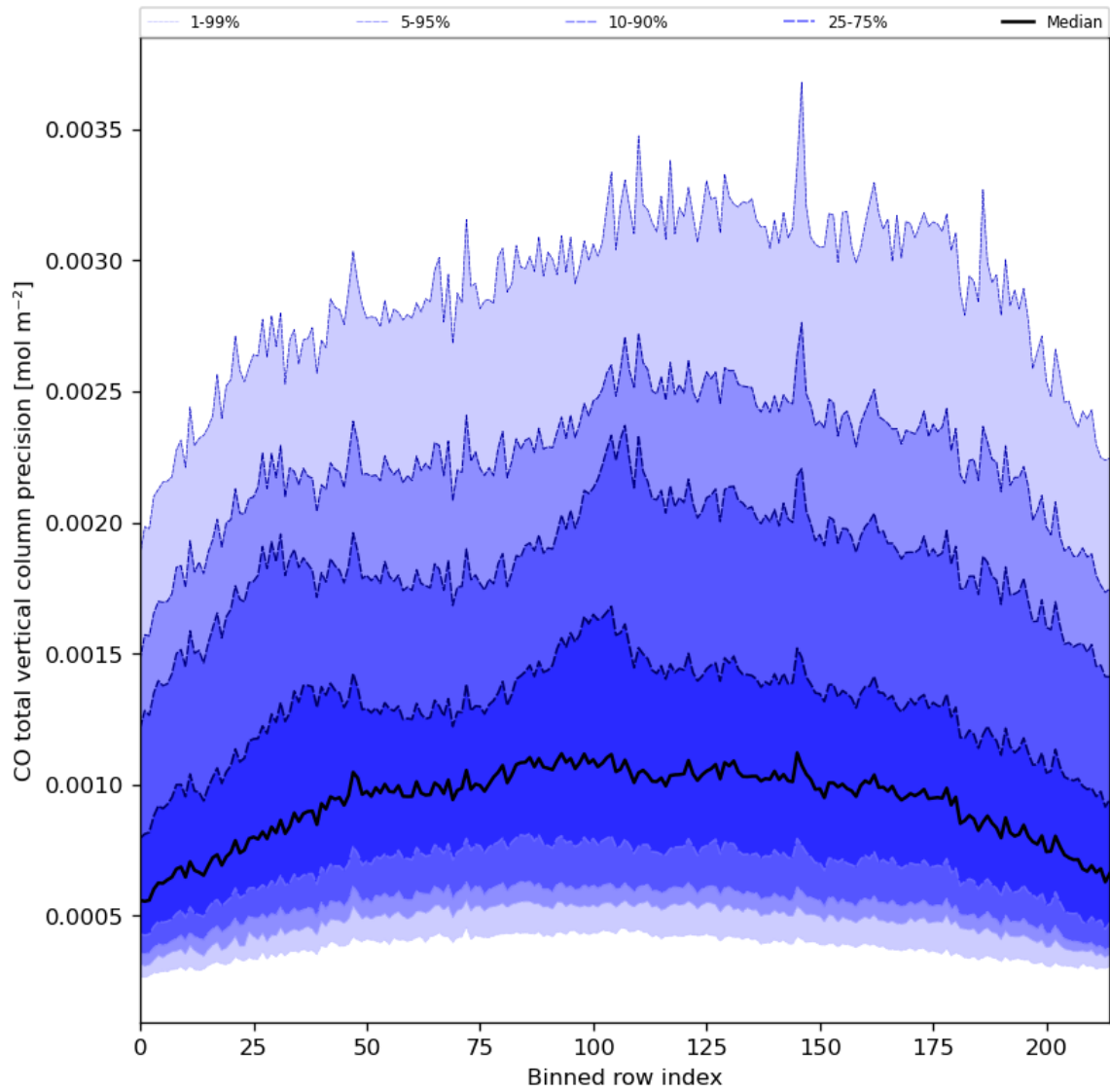
Figure 28: Along track statistics of “CO total vertical column precision” for 2023-12-26 to 2023-12-28
