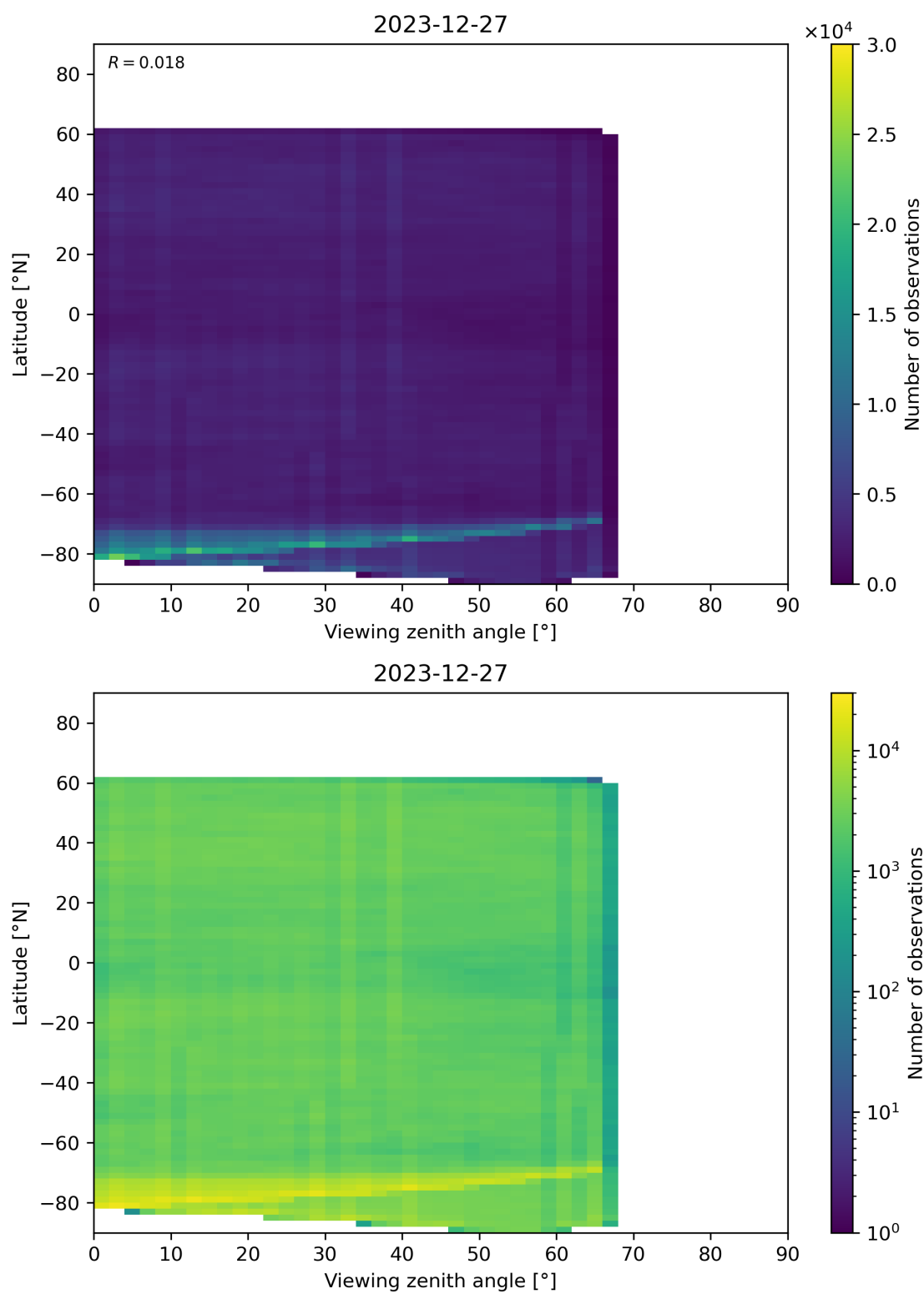
Figure 74: Scatter density plot of “Viewing zenith angle” against “Latitude” for 2023-12-26 to 2023-12-28.
