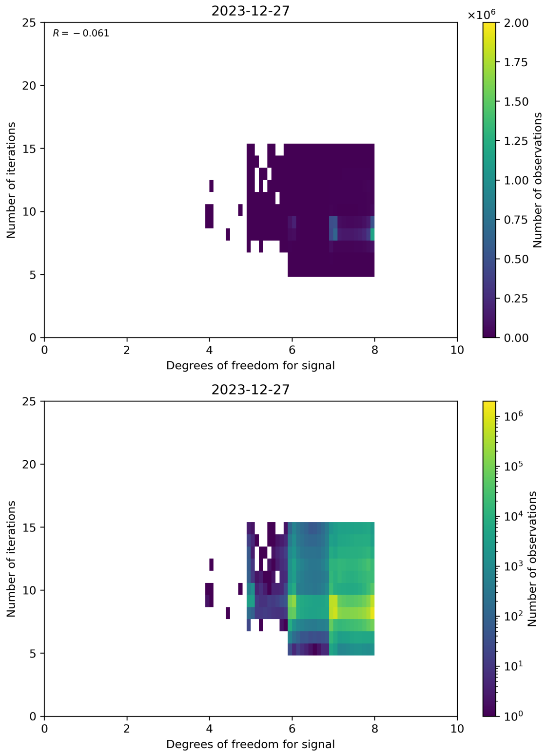
Figure 50: Scatter density plot of “Degrees of freedom for signal” against “Number of iterations” for 2023-12-26 to 2023-12-28.
