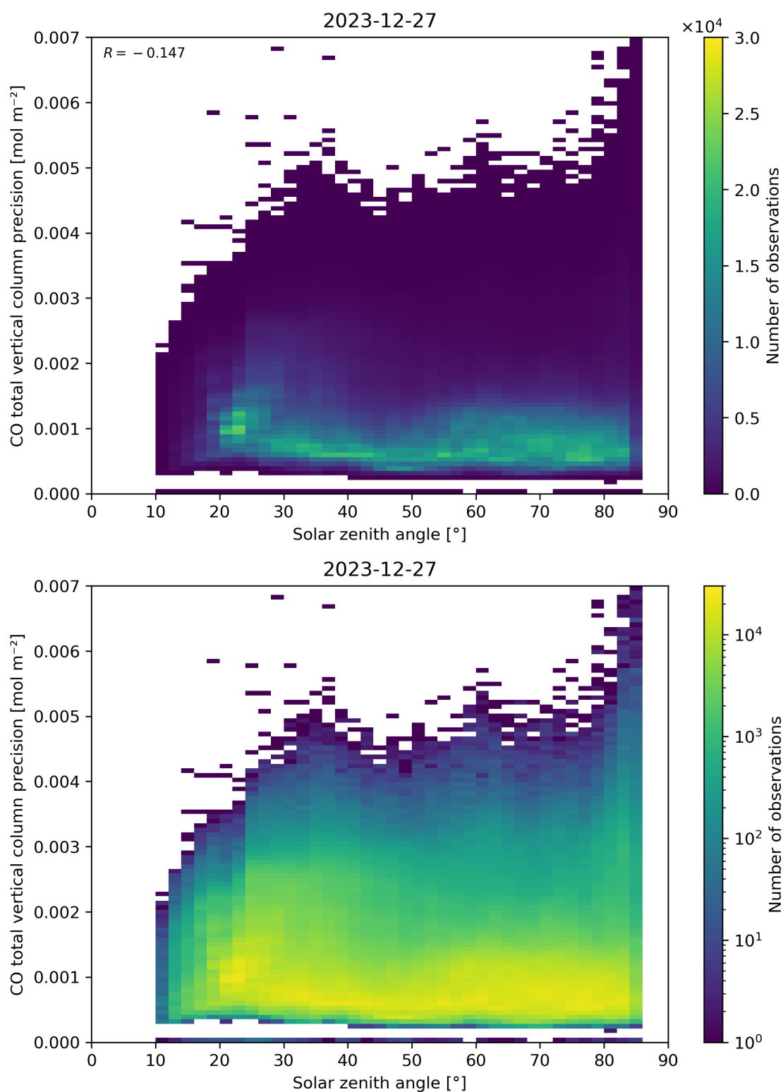
Figure 63: Scatter density plot of “Solar zenith angle” against “CO total vertical column precision” for 2023-12-26 to 2023-12-28.
