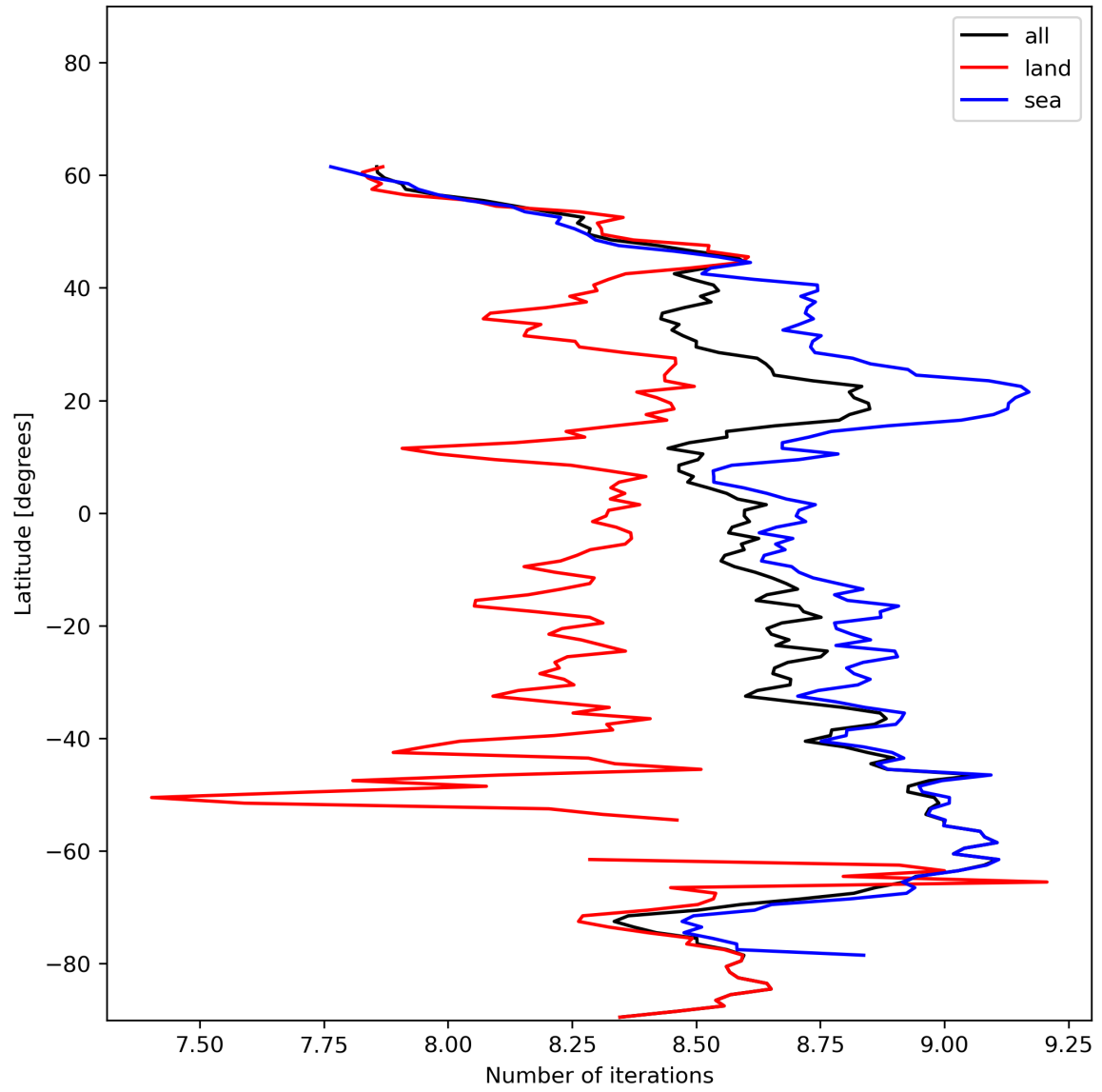
Figure 16: Zonal average of “Number of iterations” for 2023-12-26 to 2023-12-28.
