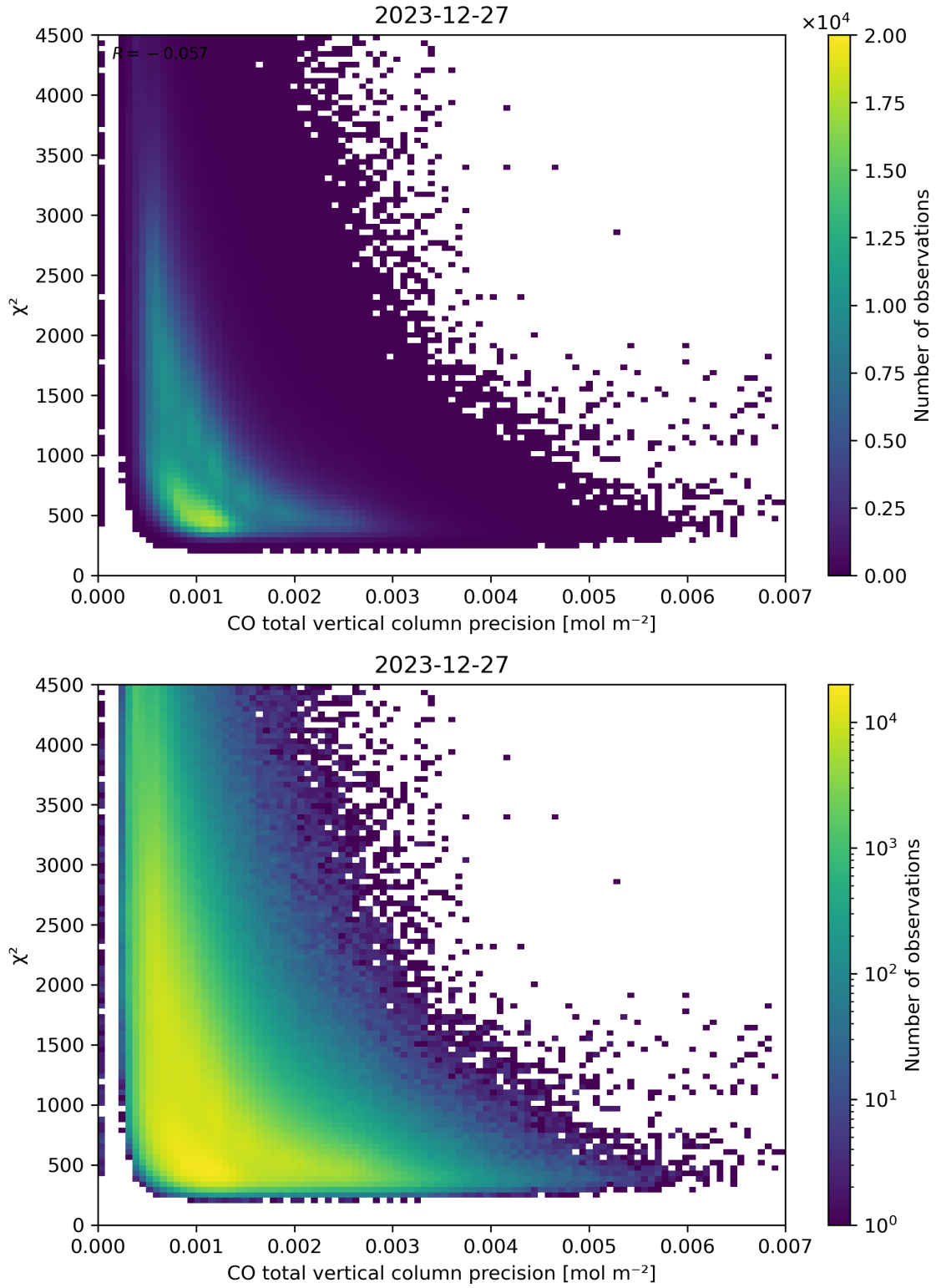
Figure 44: Scatter density plot of “CO total vertical column precision” against “ \chi^2 ” for 2023-12-26 to 2023-12-28.
