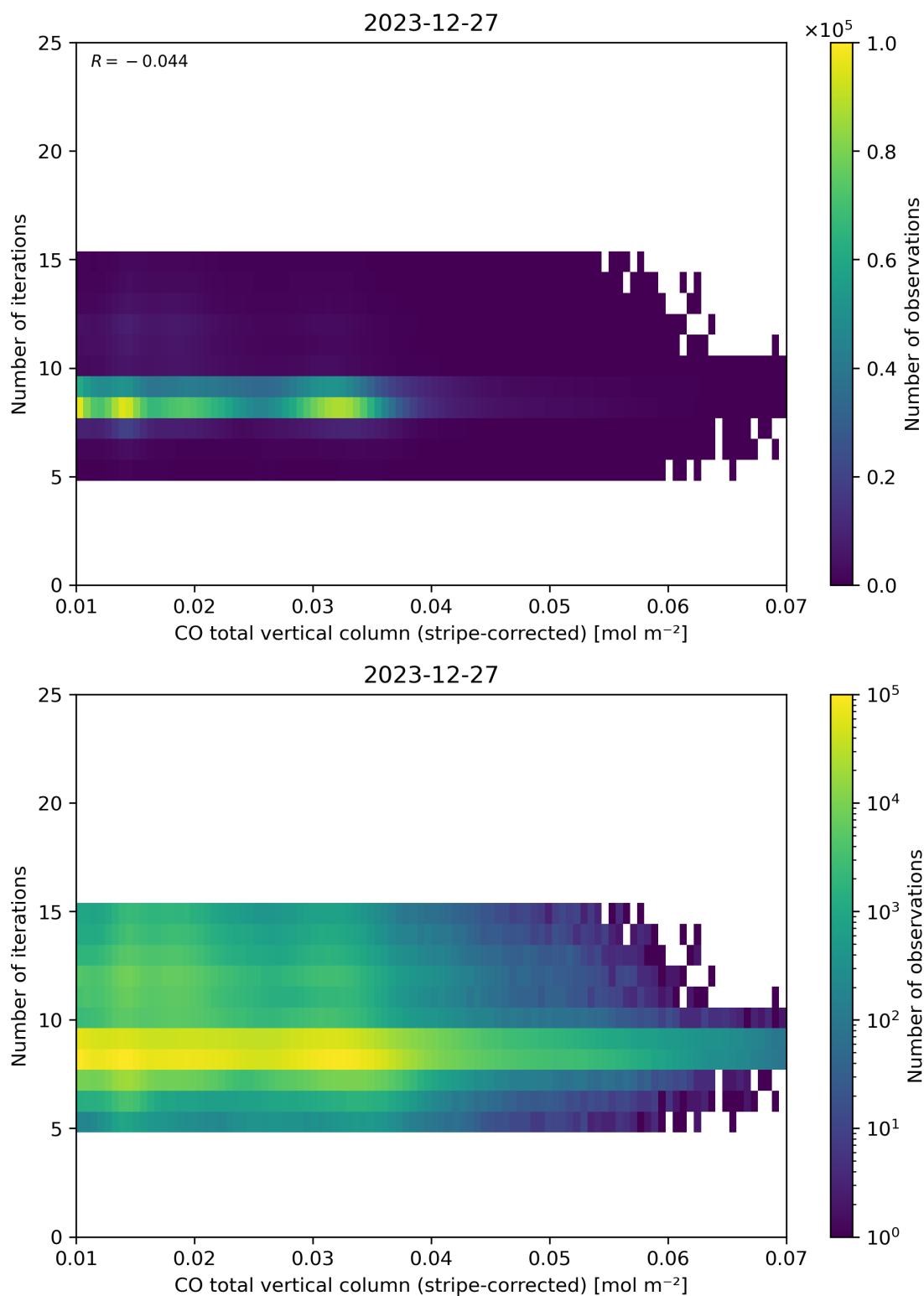
Figure 39: Scatter density plot of “CO total vertical column (stripe-corrected)” against “Number of iterations” for 2023-12-26 to 2023-12-28.
