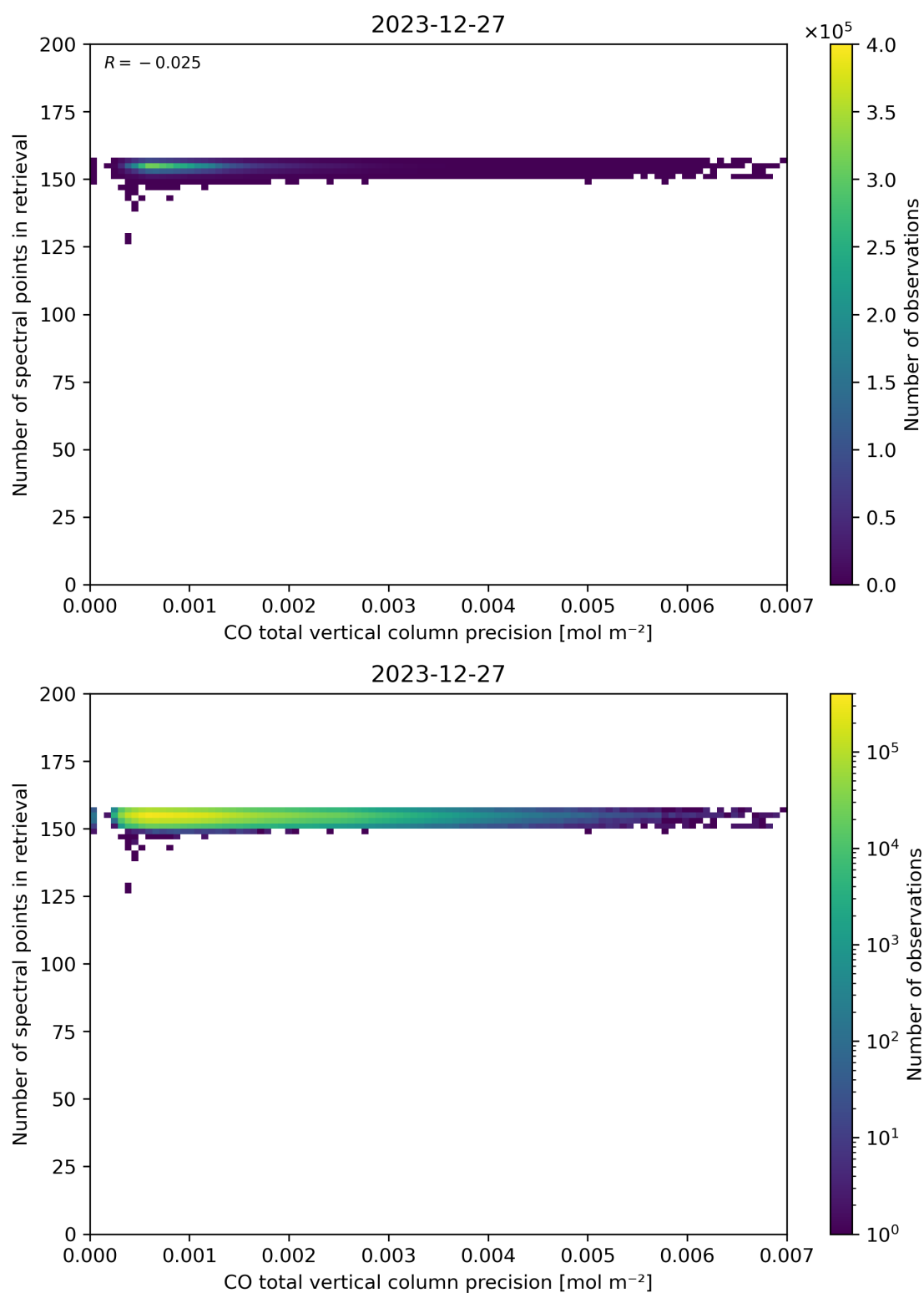
Figure 47: Scatter density plot of “CO total vertical column precision” against “Number of spectral points in retrieval” for 2023-12-26 to 2023-12-28.
