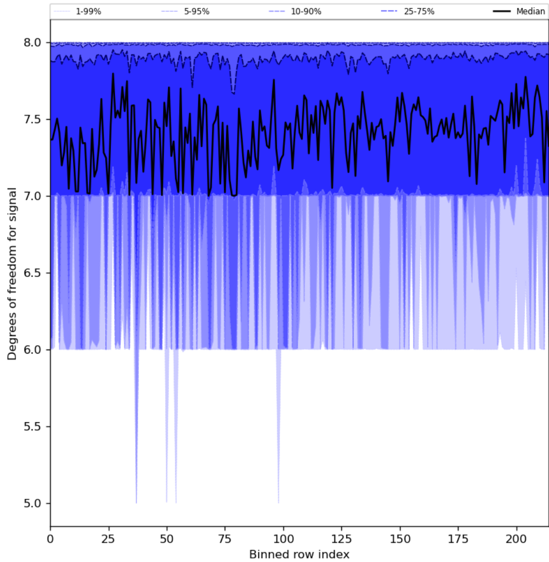
Figure 31: Along track statistics of “Degrees of freedom for signal” for 2023-12-26 to 2023-12-28
