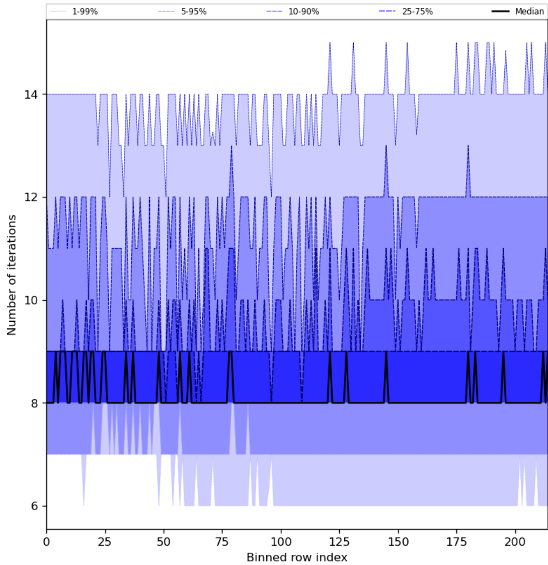
Figure 32: Along track statistics of “Number of iterations” for 2023-12-26 to 2023-12-28
