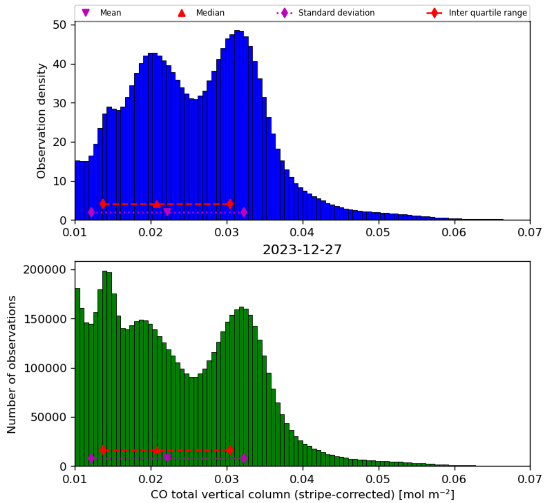
Figure 19: Histogram of “CO total vertical column (stripe-corrected)” for 2023-12-26 to 2023-12-28
