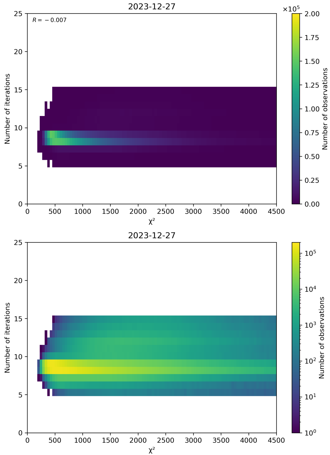
Figure 49: Scatter density plot of “ \chi^2 ” against “Number of iterations” for 2023-12-26 to 2023-12-28.
