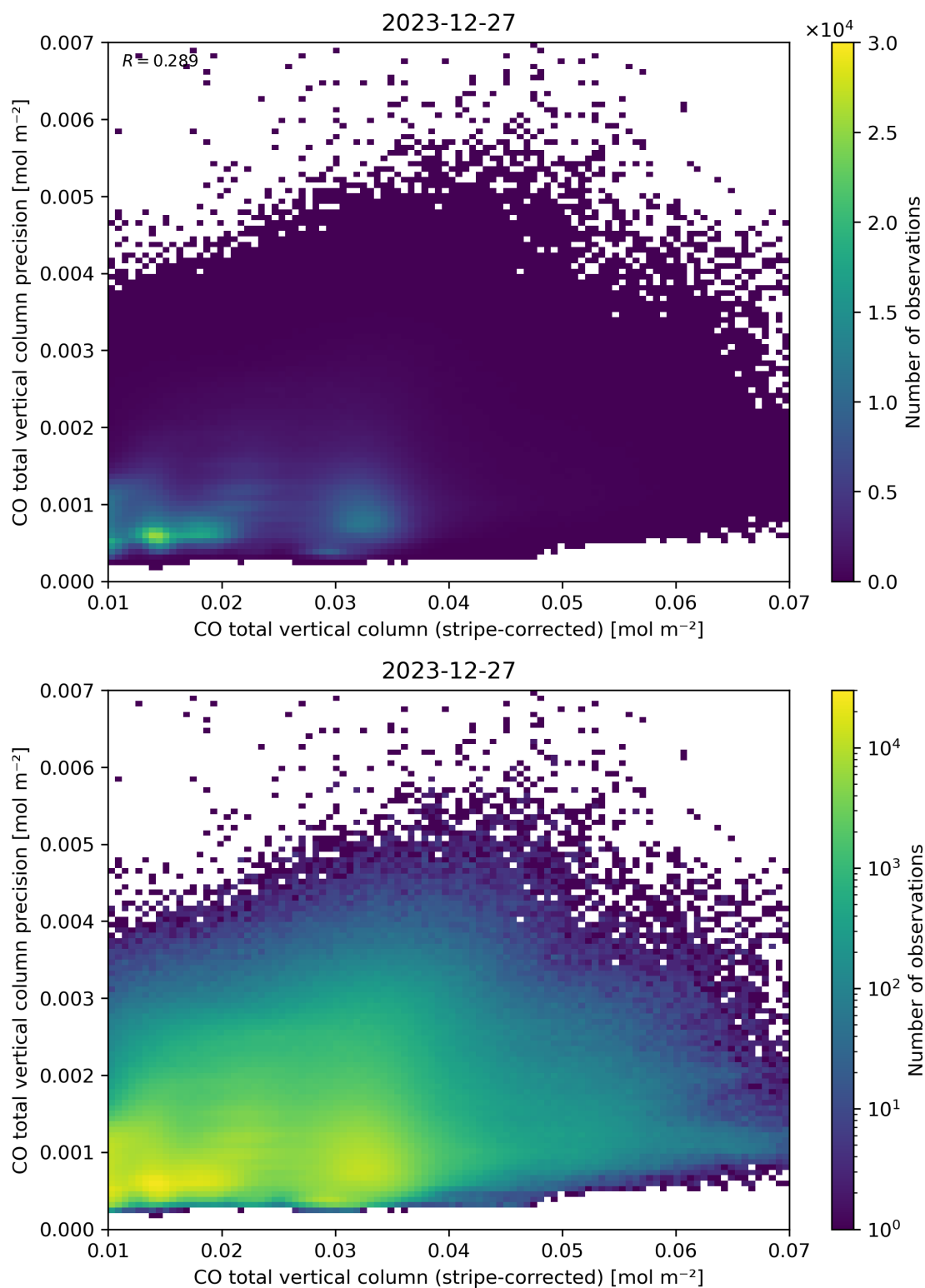
Figure 36: Scatter density plot of “CO total vertical column (stripe-corrected)” against “CO total vertical column precision” for 2023-12-26 to 2023-12-28.
