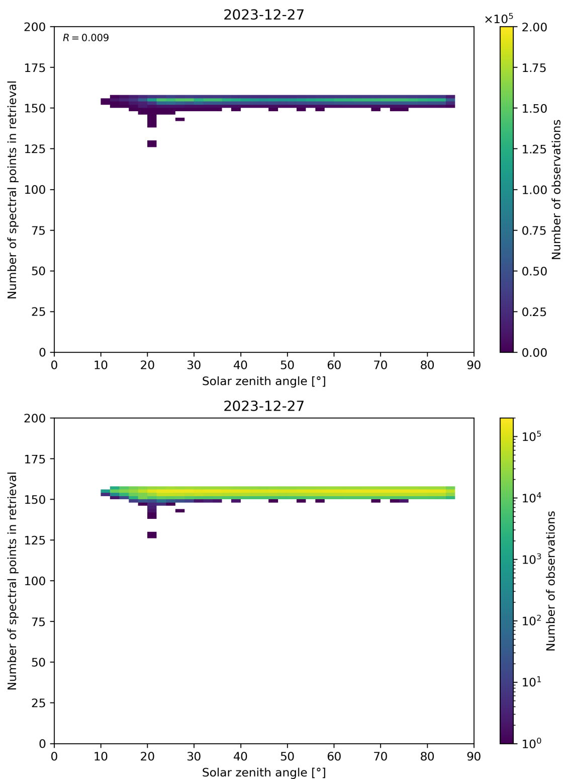
Figure 68: Scatter density plot of “Solar zenith angle” against “Number of spectral points in retrieval” for 2023-12-26 to 2023-12-28.
