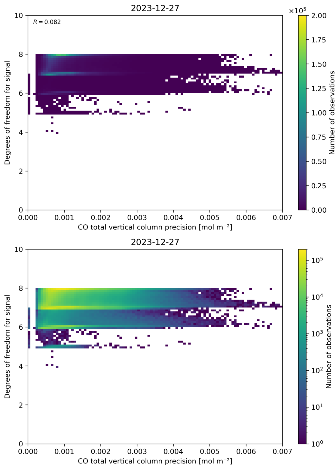
Figure 45: Scatter density plot of “CO total vertical column precision” against “Degrees of freedom for signal” for 2023-12-26 to 2023-12-28.
