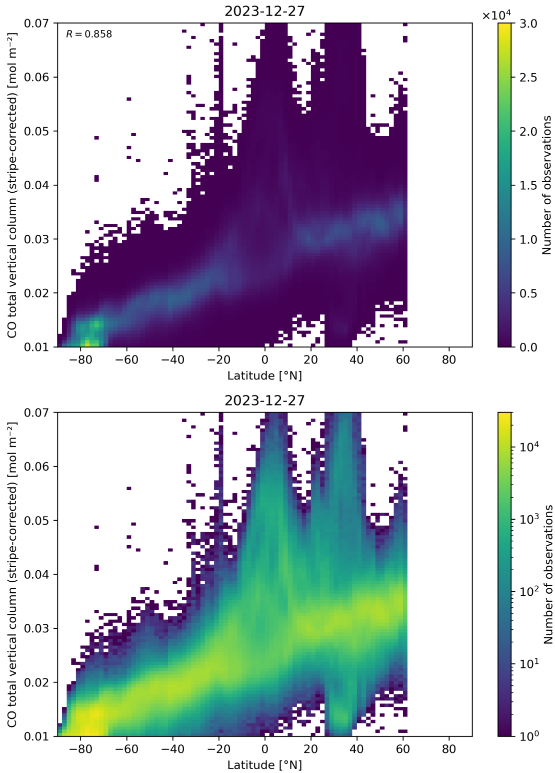
Figure 52: Scatter density plot of “Latitude” against “CO total vertical column (stripe-corrected)” for 2023-12-26 to 2023-12-28.
