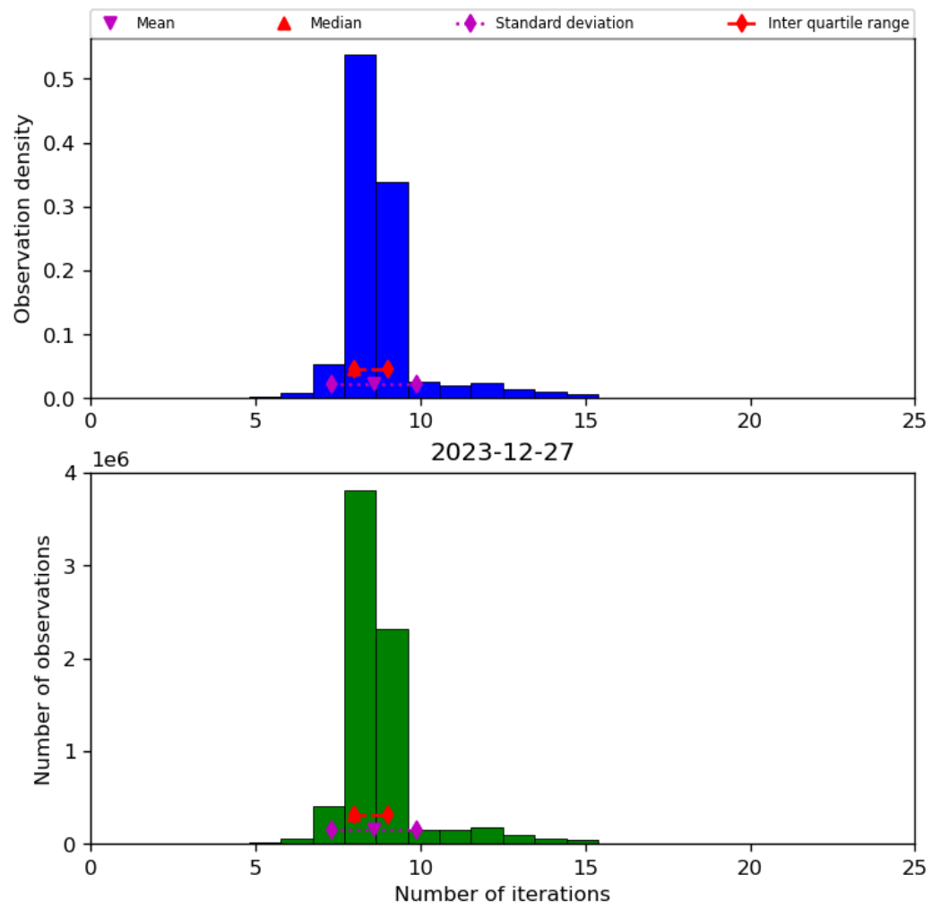
Figure 24: Histogram of “Number of iterations” for 2023-12-26 to 2023-12-28
