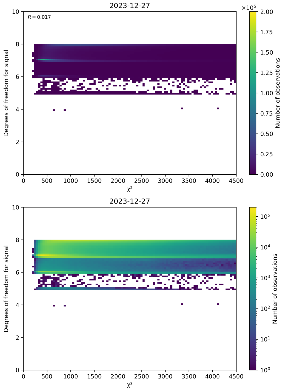
Figure 48: Scatter density plot of “ \chi^2 ” against “Degrees of freedom for signal” for 2023-12-26 to 2023-12-28.
