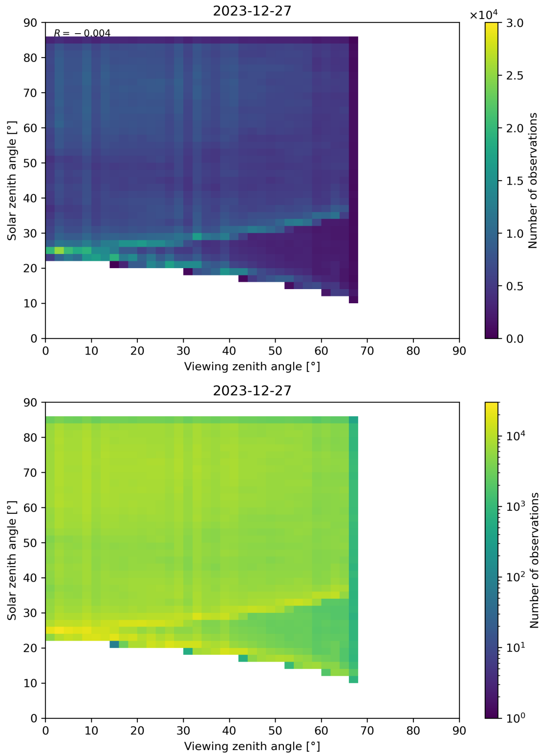
Figure 77: Scatter density plot of “Viewing zenith angle” against “Solar zenith angle” for 2023-12-26 to 2023-12-28.
