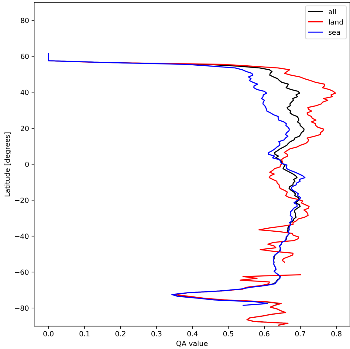
Figure 9: Zonal average of “QA value” for 2023-12-26 to 2023-12-28.
