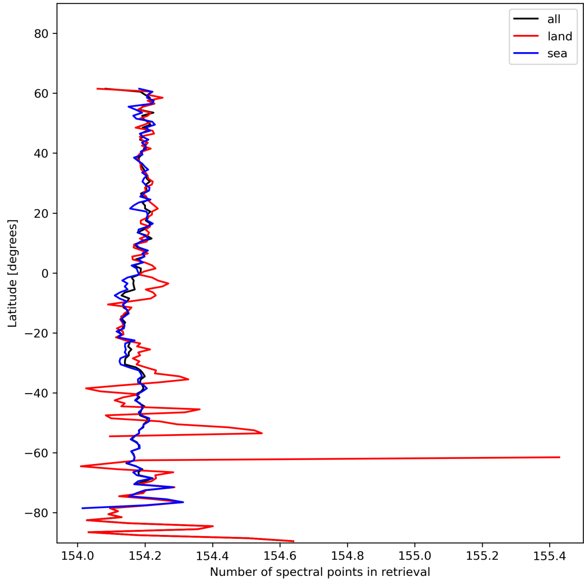
Figure 13: Zonal average of “Number of spectral points in retrieval” for 2023-12-26 to 2023-12-28.
