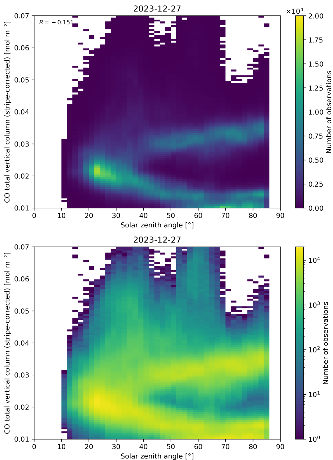
Figure 62: Scatter density plot of “Solar zenith angle” against “CO total vertical column (stripe-corrected)” for 2023-12-26 to 2023-12-28.
