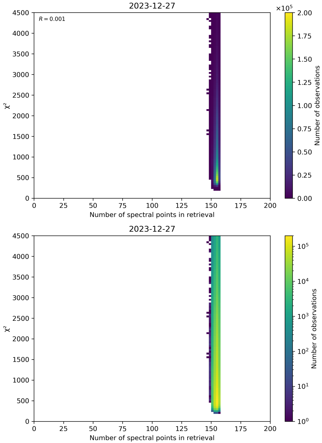
Figure 58: Scatter density plot of “Number of spectral points in retrieval” against “ \chi^2 ” for 2023-12-26 to 2023-12-28.
