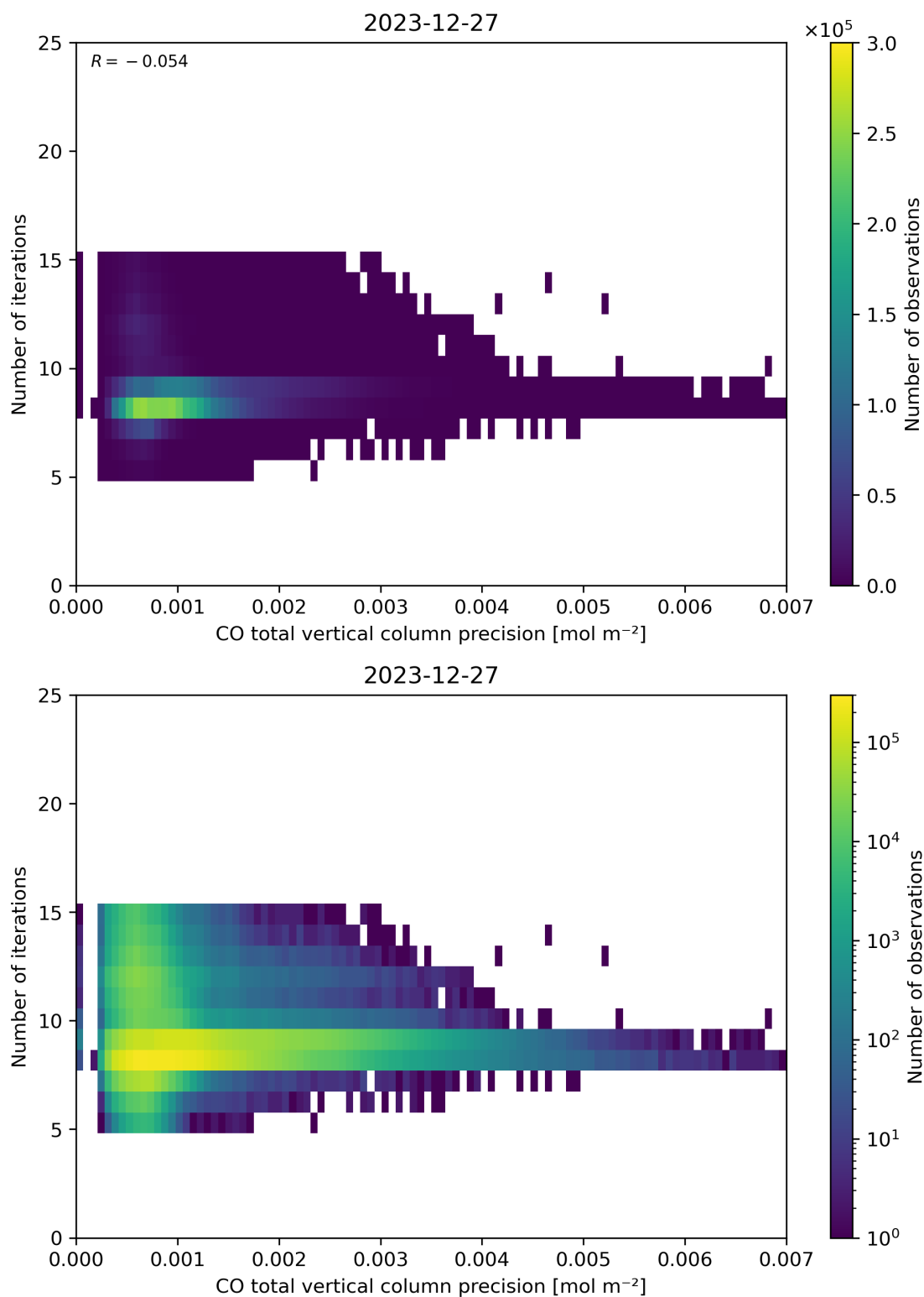
Figure 46: Scatter density plot of “CO total vertical column precision” against “Number of iterations” for 2023-12-26 to 2023-12-28.
