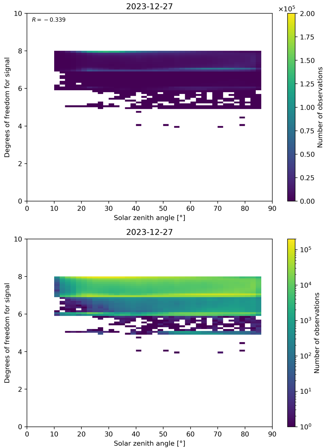
Figure 65: Scatter density plot of “Solar zenith angle” against “Degrees of freedom for signal” for 2023-12-26 to 2023-12-28.
