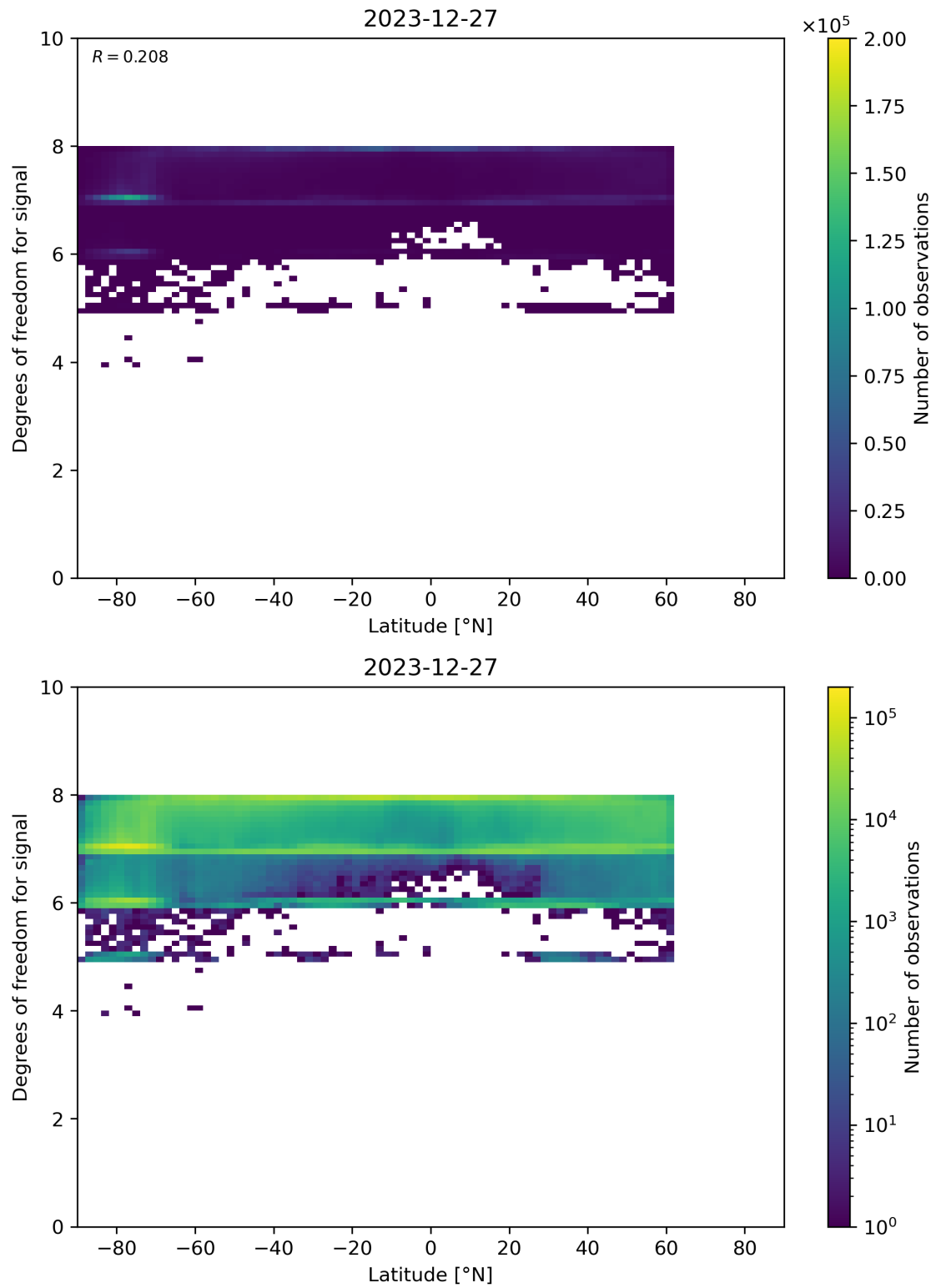
Figure 55: Scatter density plot of “Latitude” against “Degrees of freedom for signal” for 2023-12-26 to 2023-12-28.
