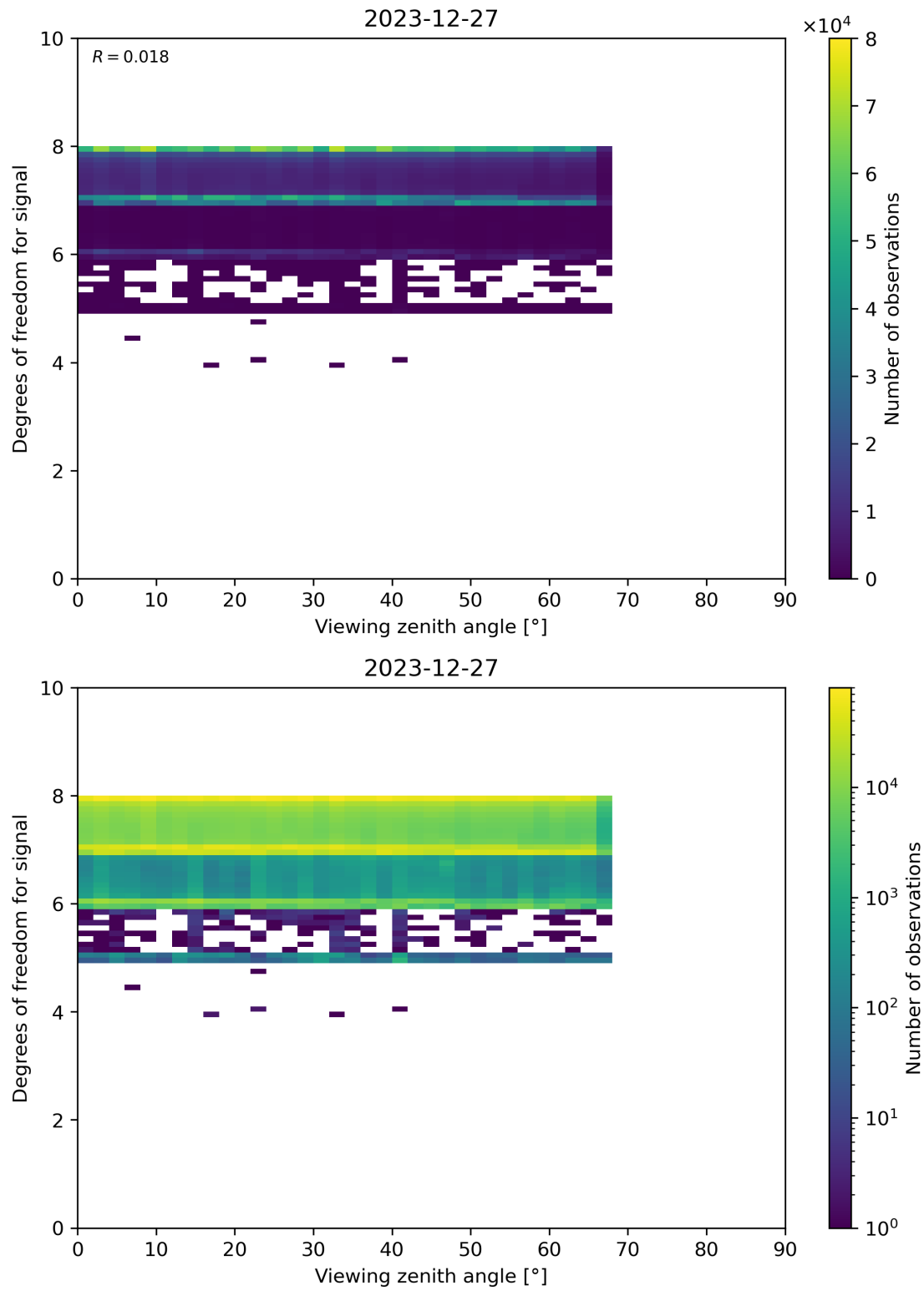
Figure 73: Scatter density plot of “Viewing zenith angle” against “Degrees of freedom for signal” for 2023-12-26 to 2023-12-28.
