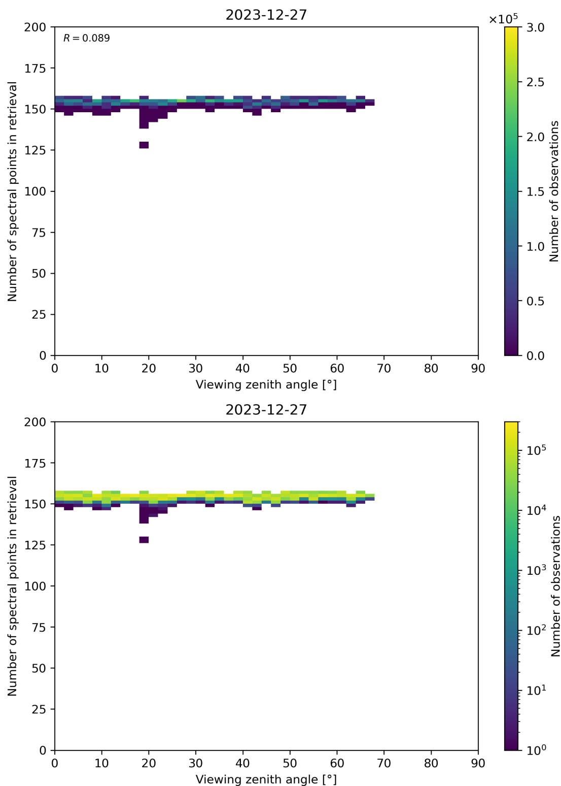
Figure 76: Scatter density plot of “Viewing zenith angle” against “Number of spectral points in retrieval” for 2023-12-26 to 2023-12-28.
