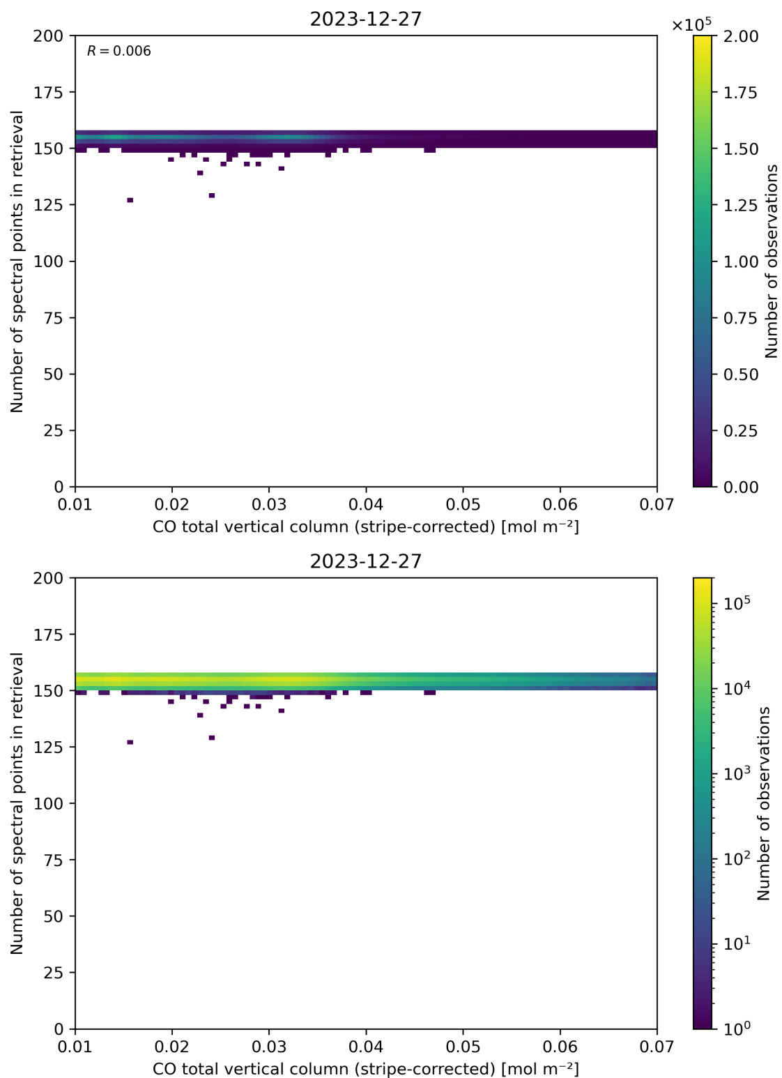
Figure 40: Scatter density plot of “CO total vertical column (stripe-corrected)” against “Number of spectral points in retrieval” for 2023-12-26 to 2023-12-28.
