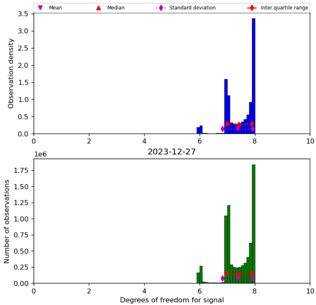
Figure 23: Histogram of “Degrees of freedom for signal” for 2023-12-26 to 2023-12-28
