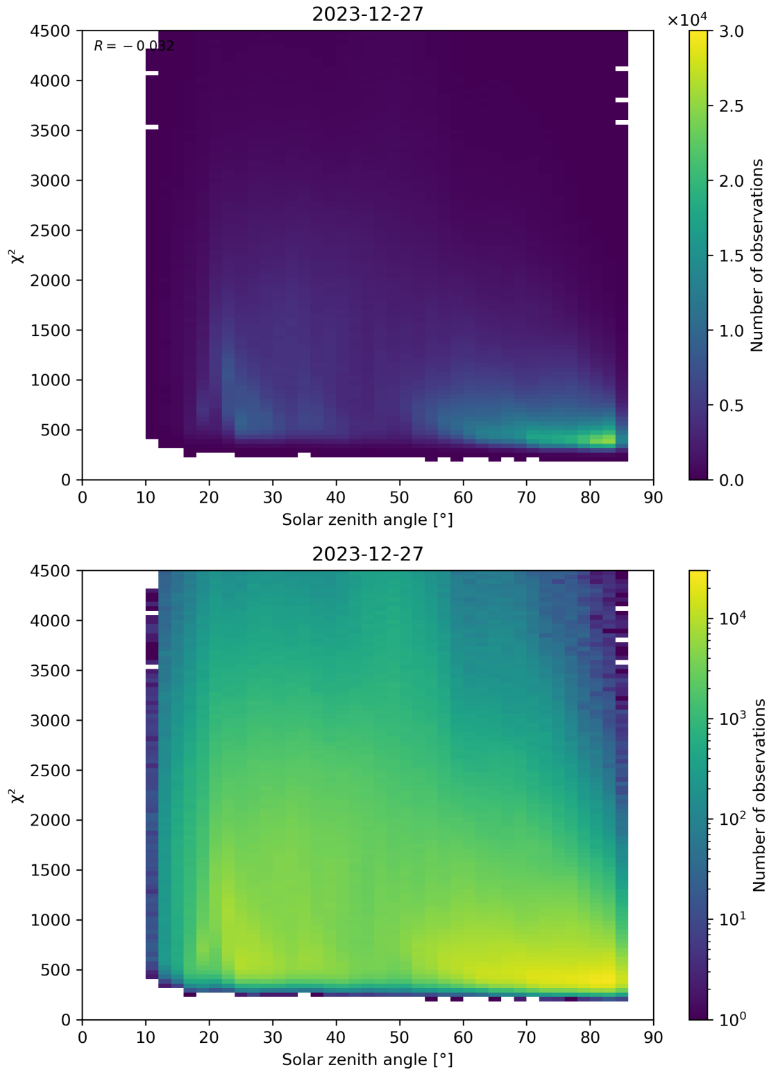
Figure 64: Scatter density plot of “Solar zenith angle” against “ \chi^2 ” for 2023-12-26 to 2023-12-28.
