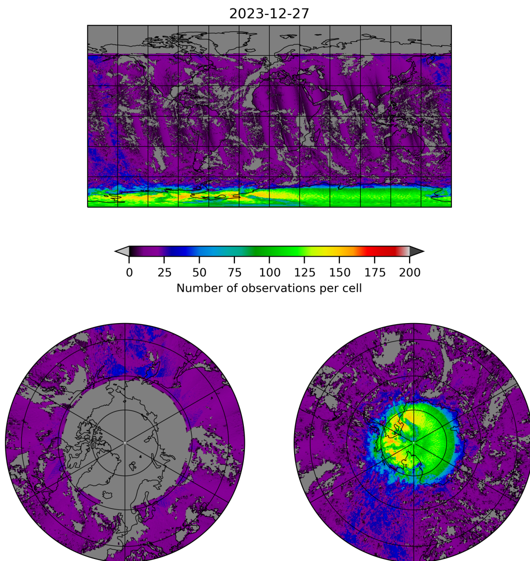
Figure 8: Map of the number of observations for 2023-12-26 to 2023-12-28
