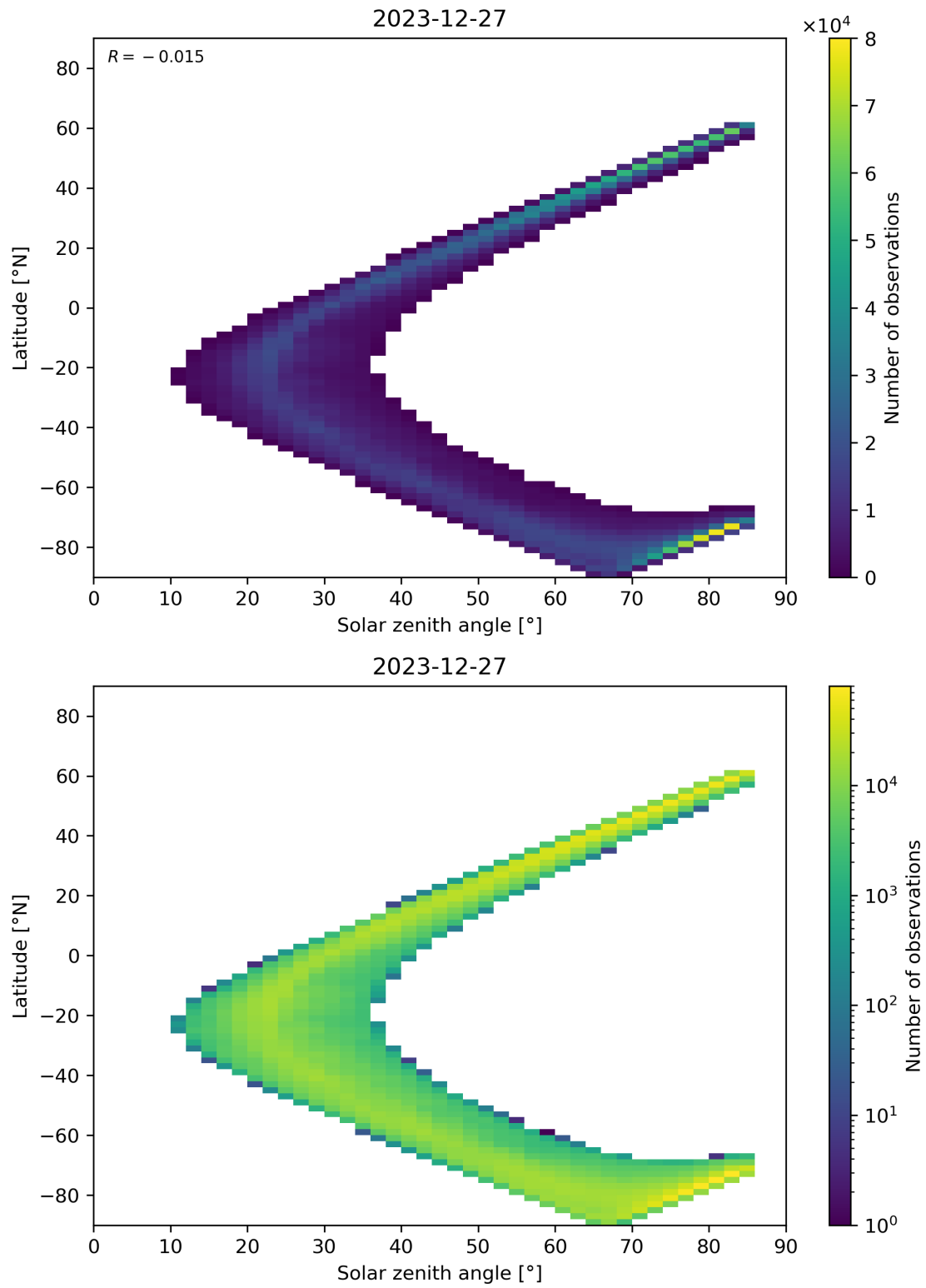
Figure 66: Scatter density plot of “Solar zenith angle” against “Latitude” for 2023-12-26 to 2023-12-28.
