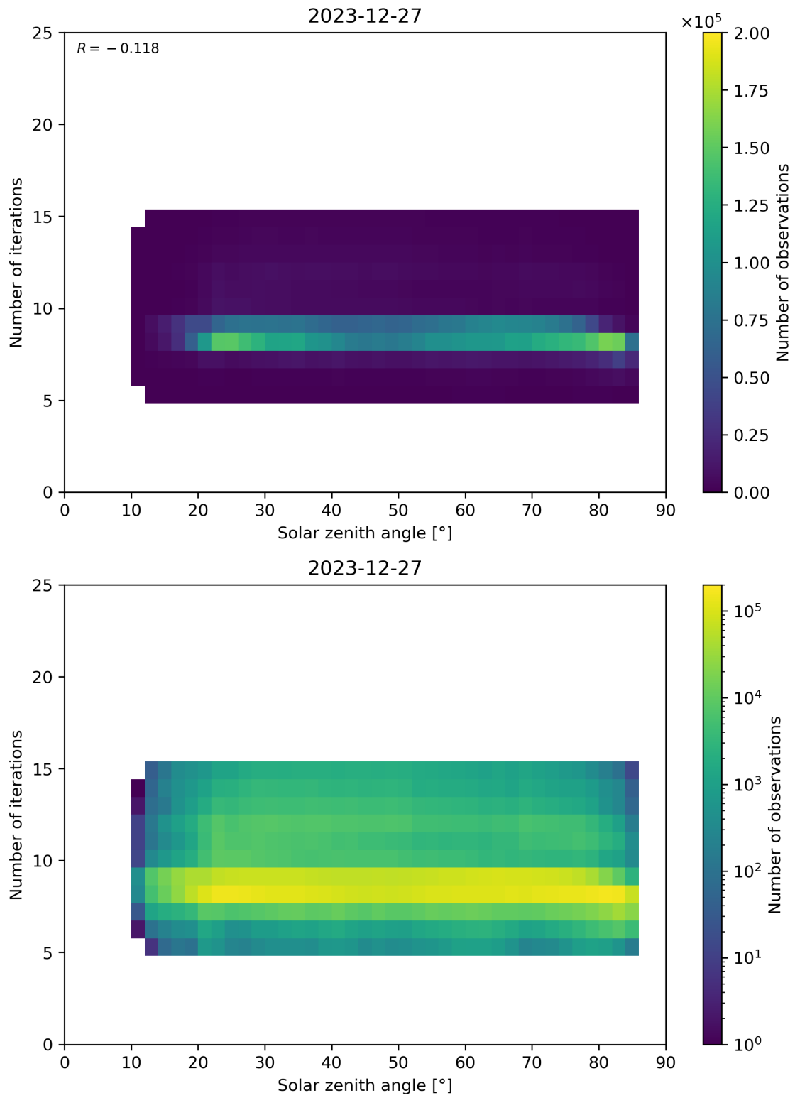
Figure 67: Scatter density plot of “Solar zenith angle” against “Number of iterations” for 2023-12-26 to 2023-12-28.
