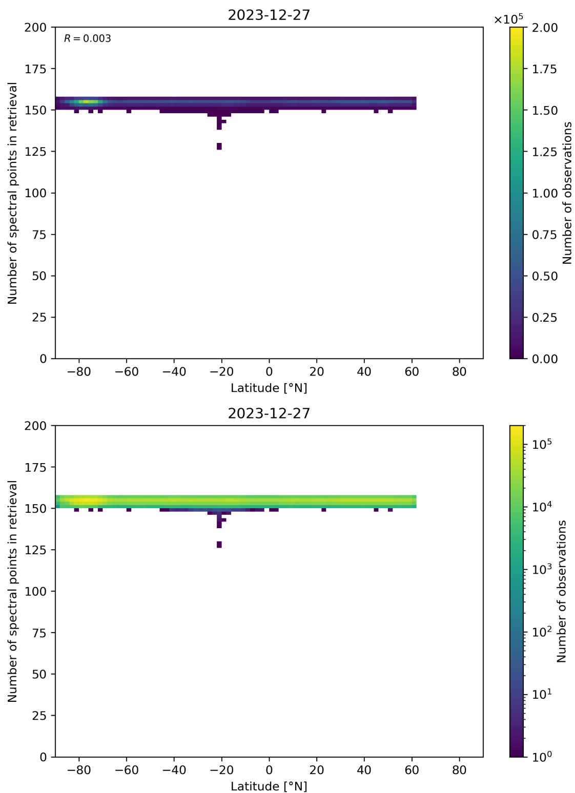
Figure 57: Scatter density plot of “Latitude” against “Number of spectral points in retrieval” for 2023-12-26 to 2023-12-28.
