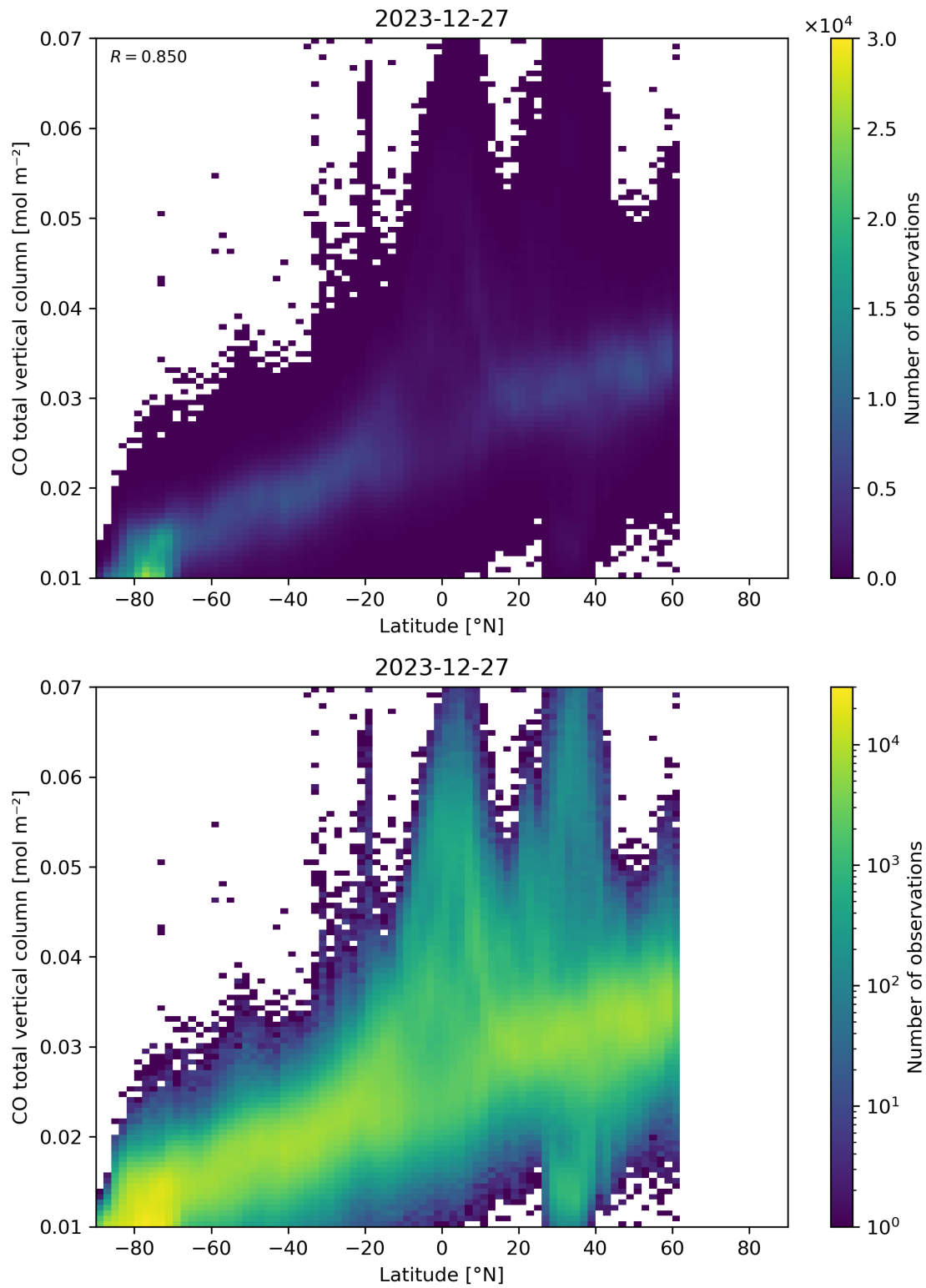
Figure 51: Scatter density plot of “Latitude” against “CO total vertical column” for 2023-12-26 to 2023-12-28.
