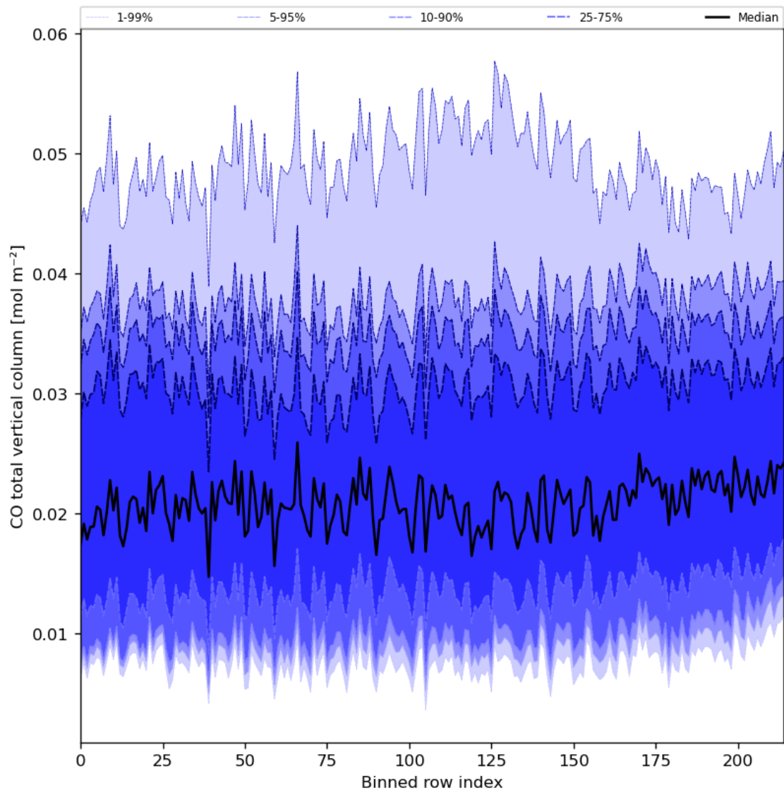
Figure 26: Along track statistics of “CO total vertical column” for 2023-12-26 to 2023-12-28
