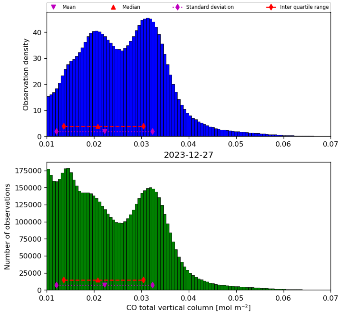
Figure 18: Histogram of “CO total vertical column” for 2023-12-26 to 2023-12-28
