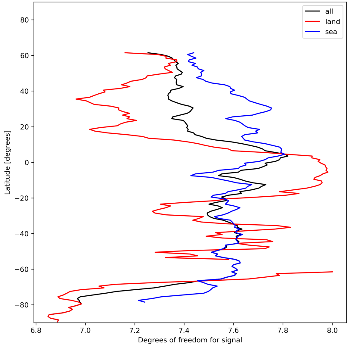
Figure 15: Zonal average of “Degrees of freedom for signal” for 2023-12-26 to 2023-12-28.
