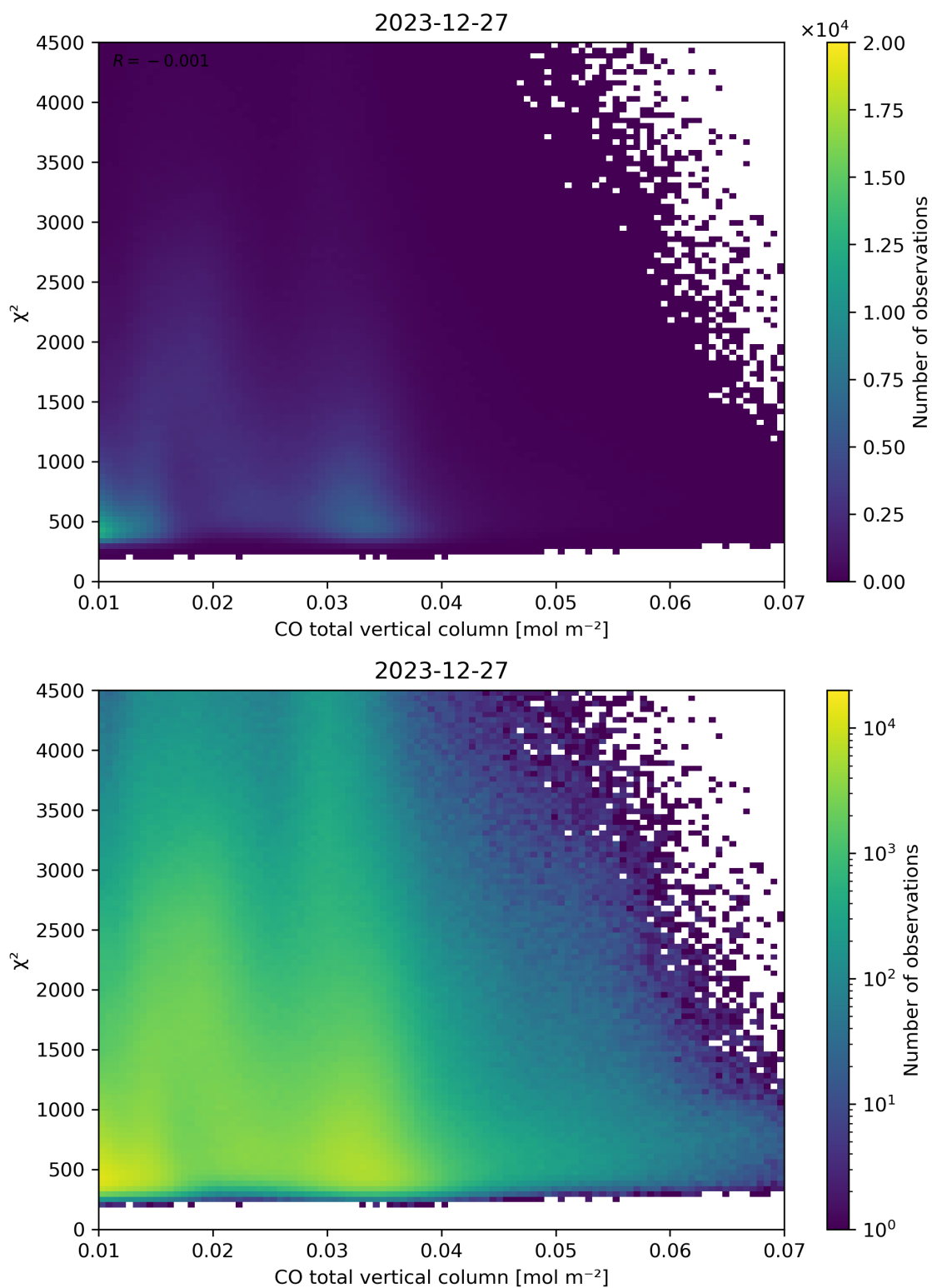
Figure 35: Scatter density plot of “CO total vertical column” against “ \chi^2 ” for 2023-12-26 to 2023-12-28.
