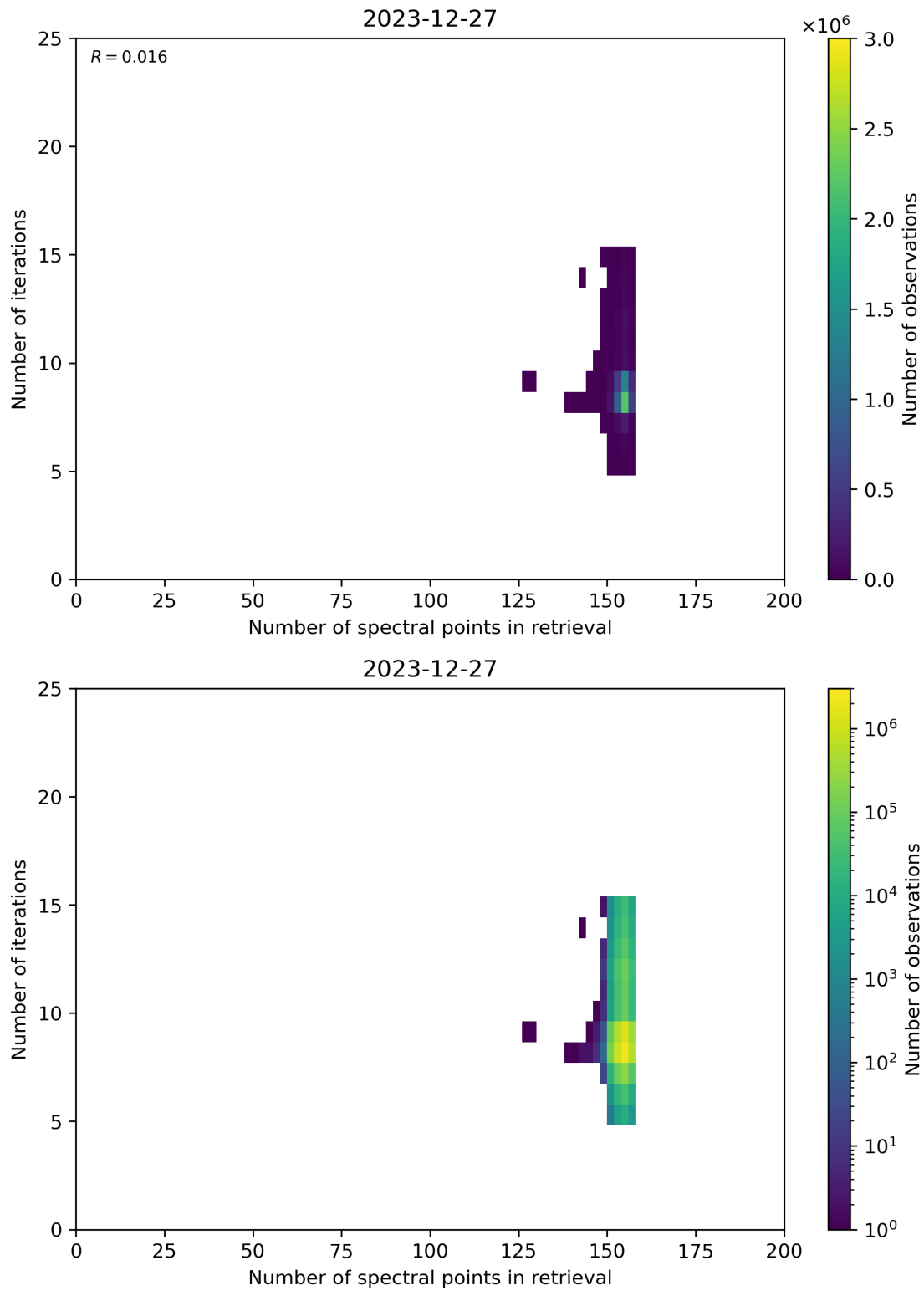
Figure 60: Scatter density plot of “Number of spectral points in retrieval” against “Number of iterations” for 2023-12-26 to 2023-12-28.
