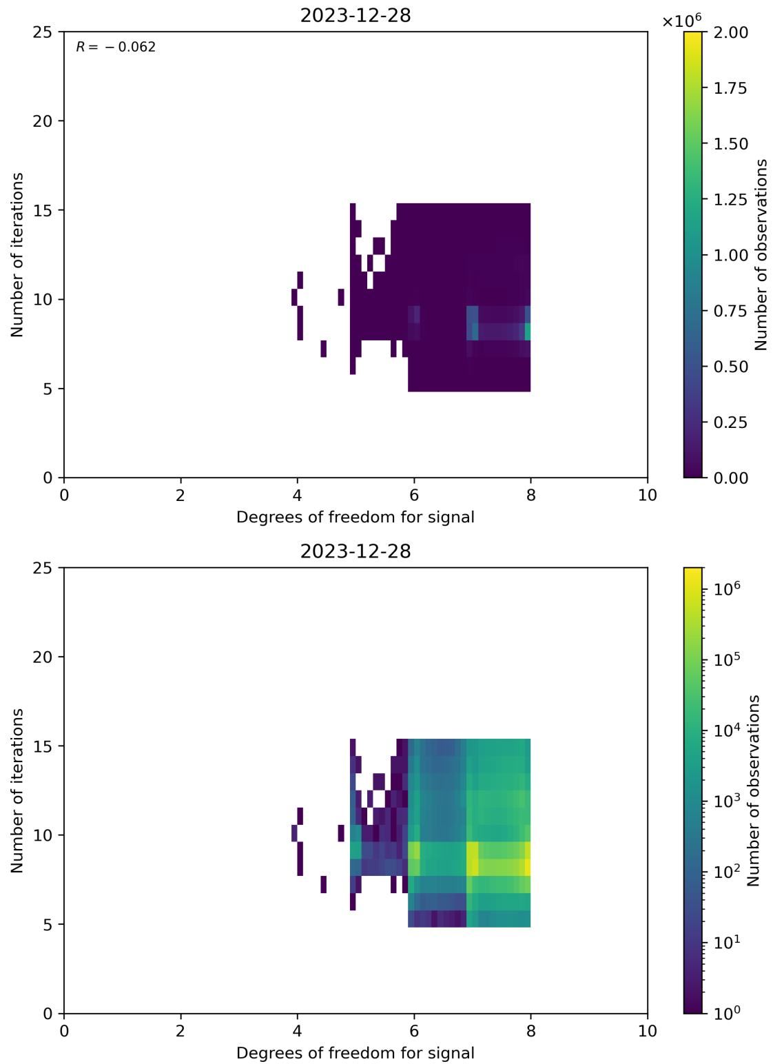
Figure 50: Scatter density plot of “Degrees of freedom for signal” against “Number of iterations” for 2023-12-27 to 2023-12-29.
