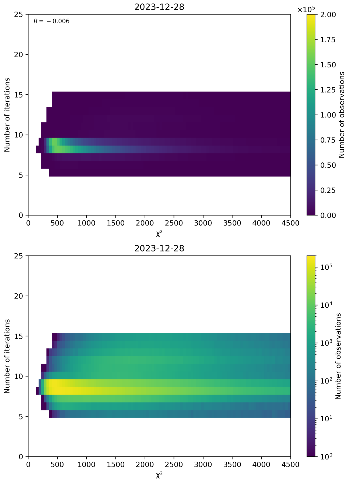
Figure 49: Scatter density plot of “ \chi^2 ” against “Number of iterations” for 2023-12-27 to 2023-12-29.
