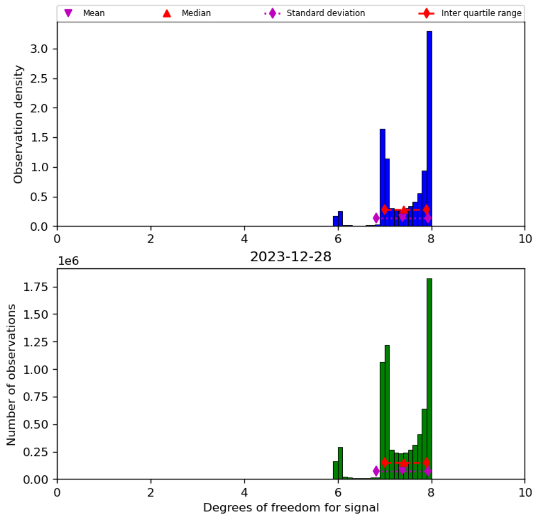
Figure 23: Histogram of “Degrees of freedom for signal” for 2023-12-27 to 2023-12-29
