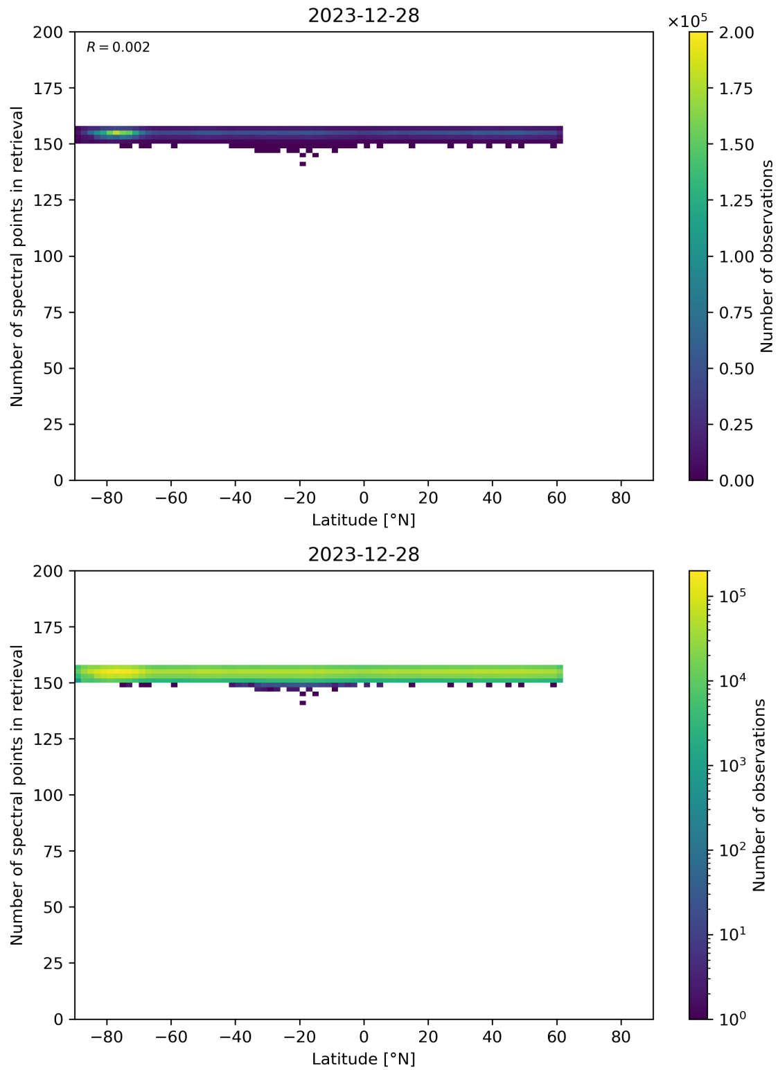
Figure 57: Scatter density plot of “Latitude” against “Number of spectral points in retrieval” for 2023-12-27 to 2023-12-29.
