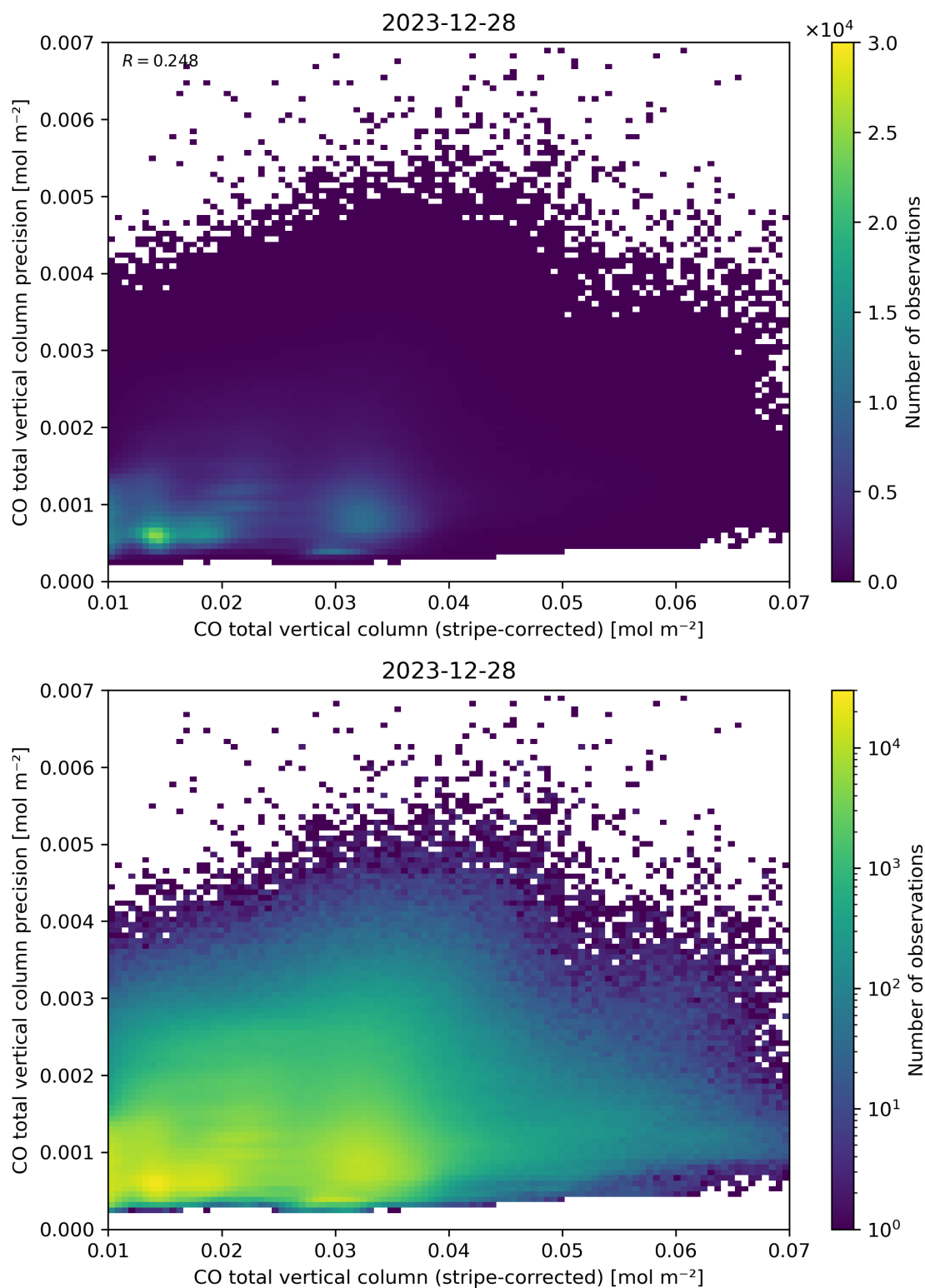
Figure 36: Scatter density plot of “CO total vertical column (stripe-corrected)” against “CO total vertical column precision” for 2023-12-27 to 2023-12-29.
