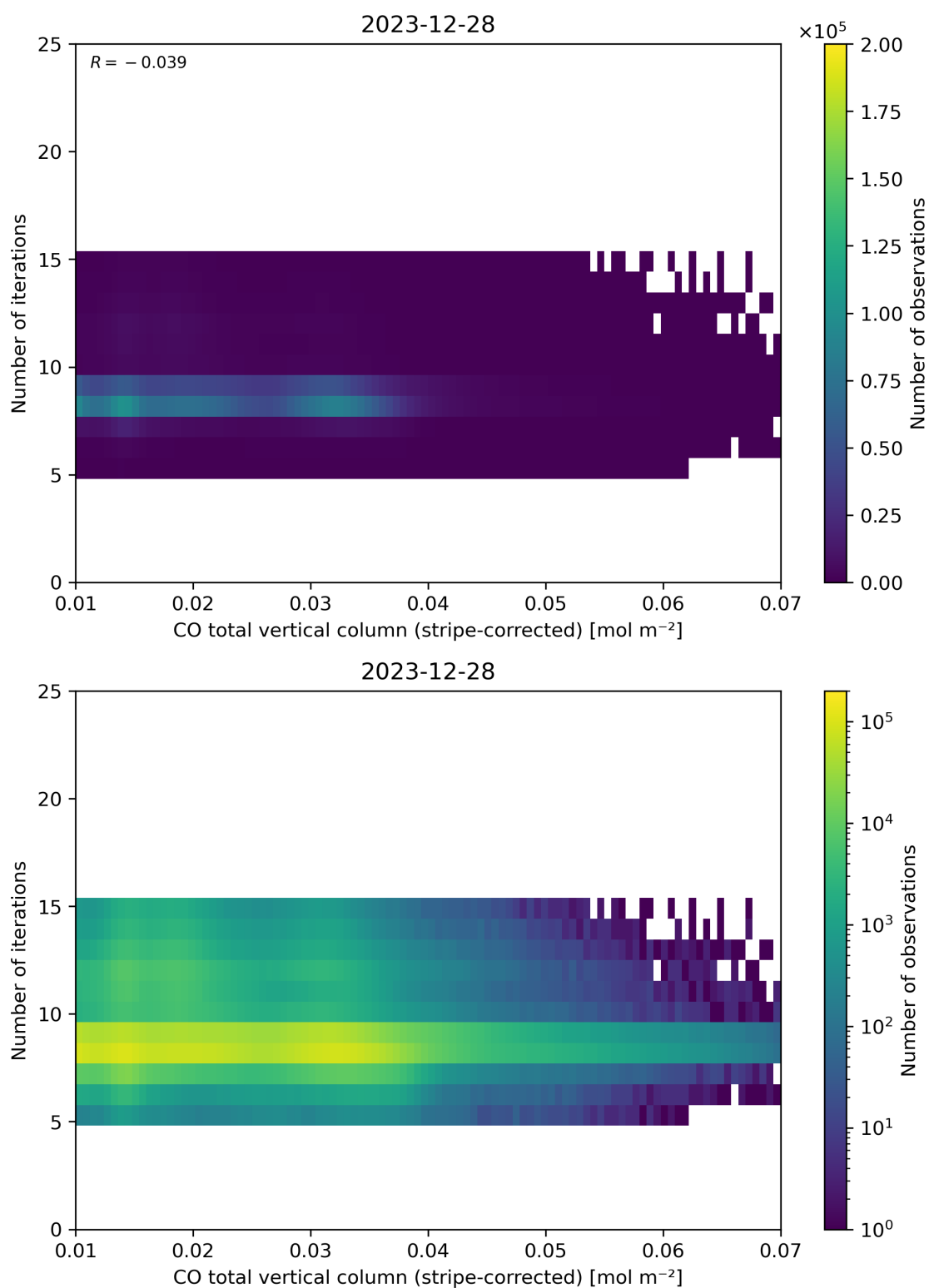
Figure 39: Scatter density plot of “CO total vertical column (stripe-corrected)” against “Number of iterations” for 2023-12-27 to 2023-12-29.
