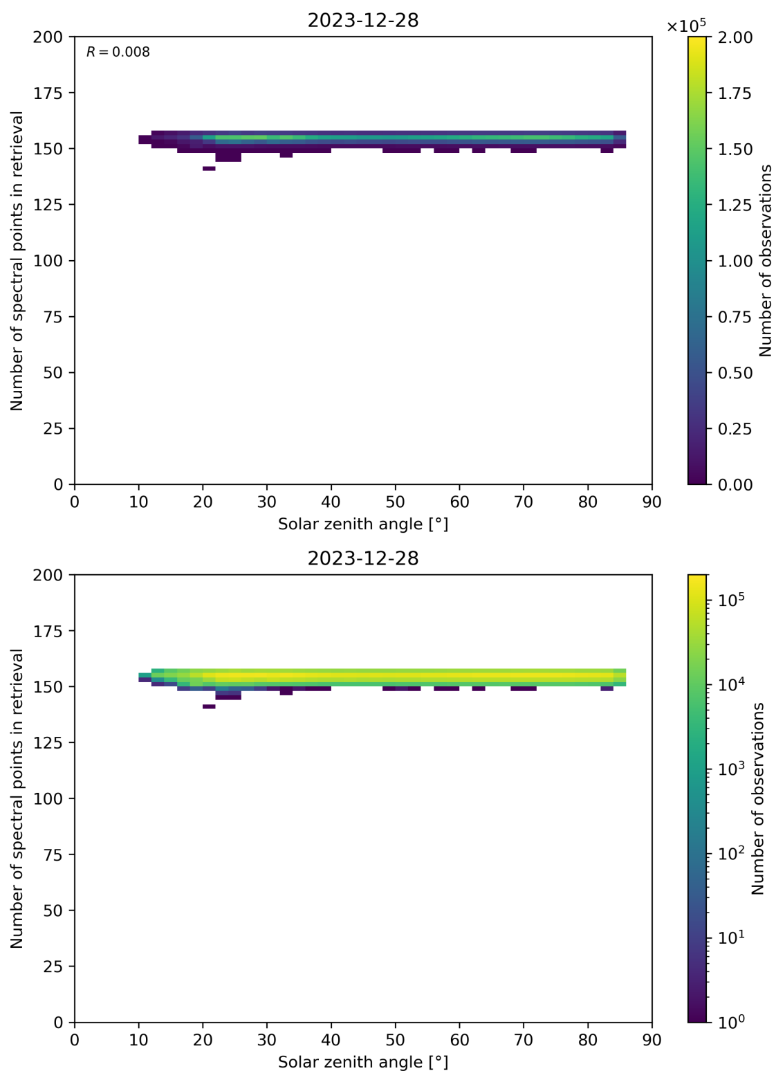
Figure 68: Scatter density plot of “Solar zenith angle” against “Number of spectral points in retrieval” for 2023-12-27 to 2023-12-29.
