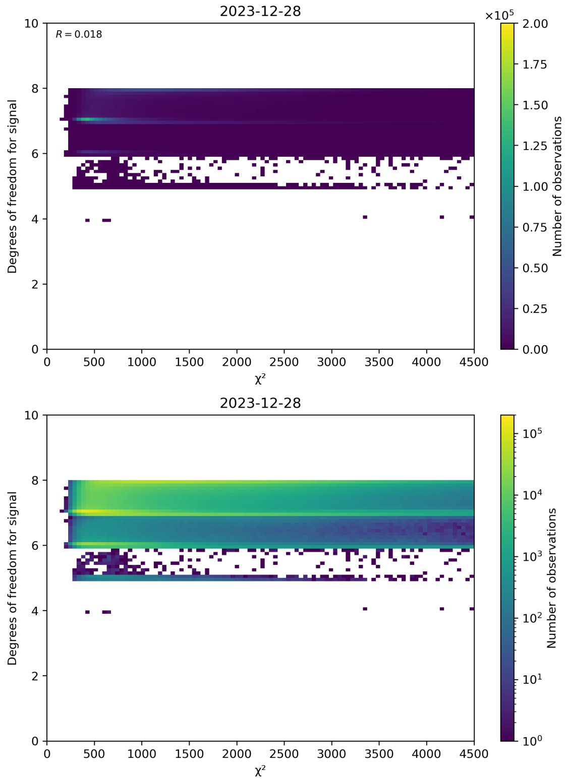
Figure 48: Scatter density plot of “ \chi^2 ” against “Degrees of freedom for signal” for 2023-12-27 to 2023-12-29.
