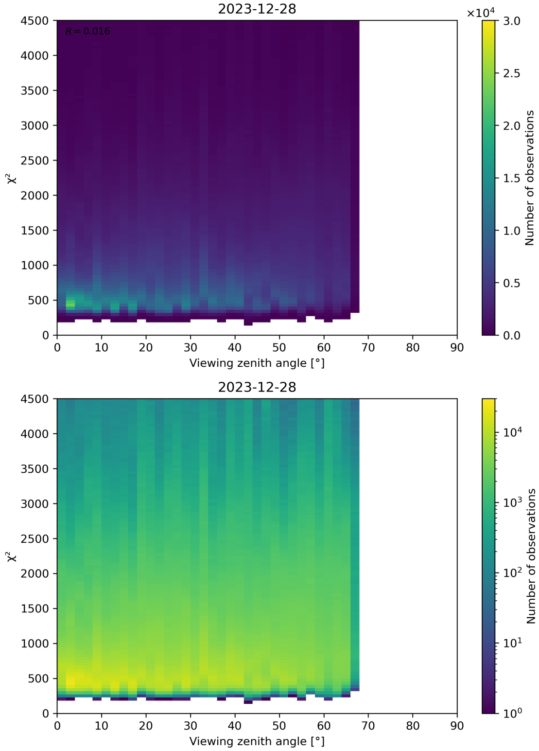
Figure 72: Scatter density plot of “Viewing zenith angle” against “ \chi^2 ” for 2023-12-27 to 2023-12-29.
