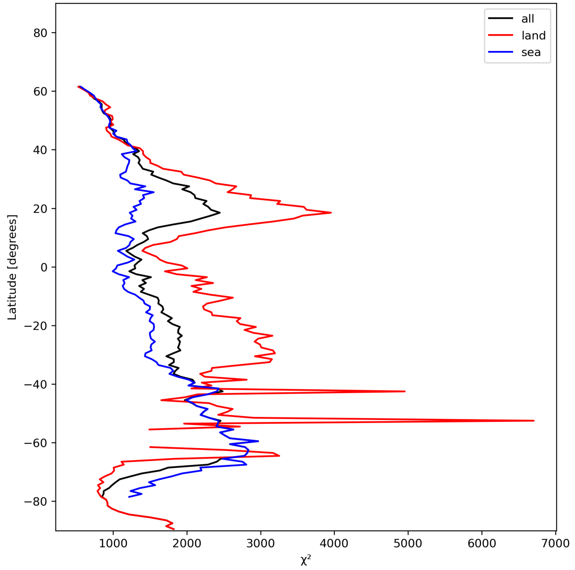
Figure 14: Zonal average of “ \chi^2 ” for 2023-12-27 to 2023-12-29.
