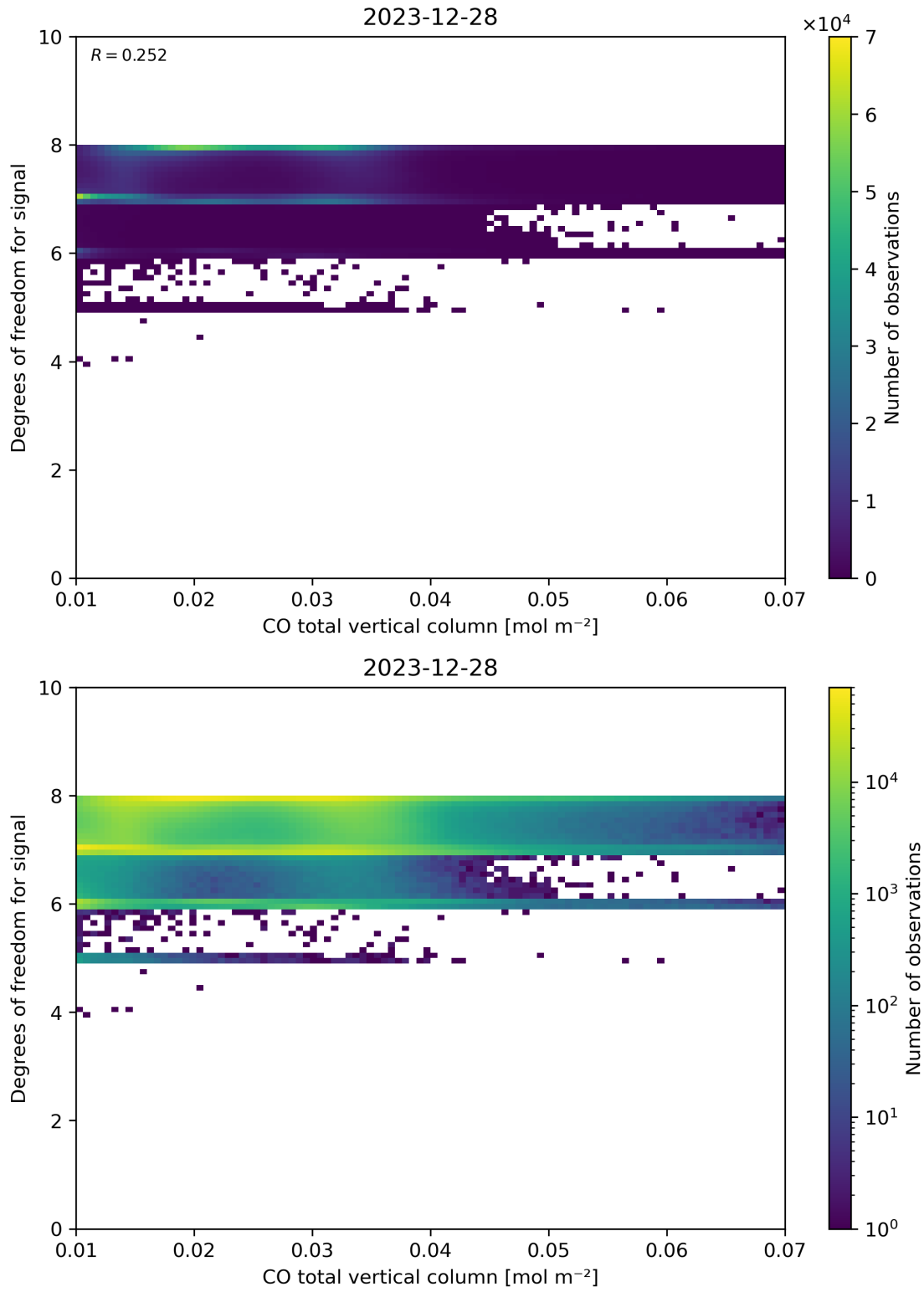
Figure 41: Scatter density plot of “CO total vertical column” against “Degrees of freedom for signal” for 2023-12-27 to 2023-12-29.
