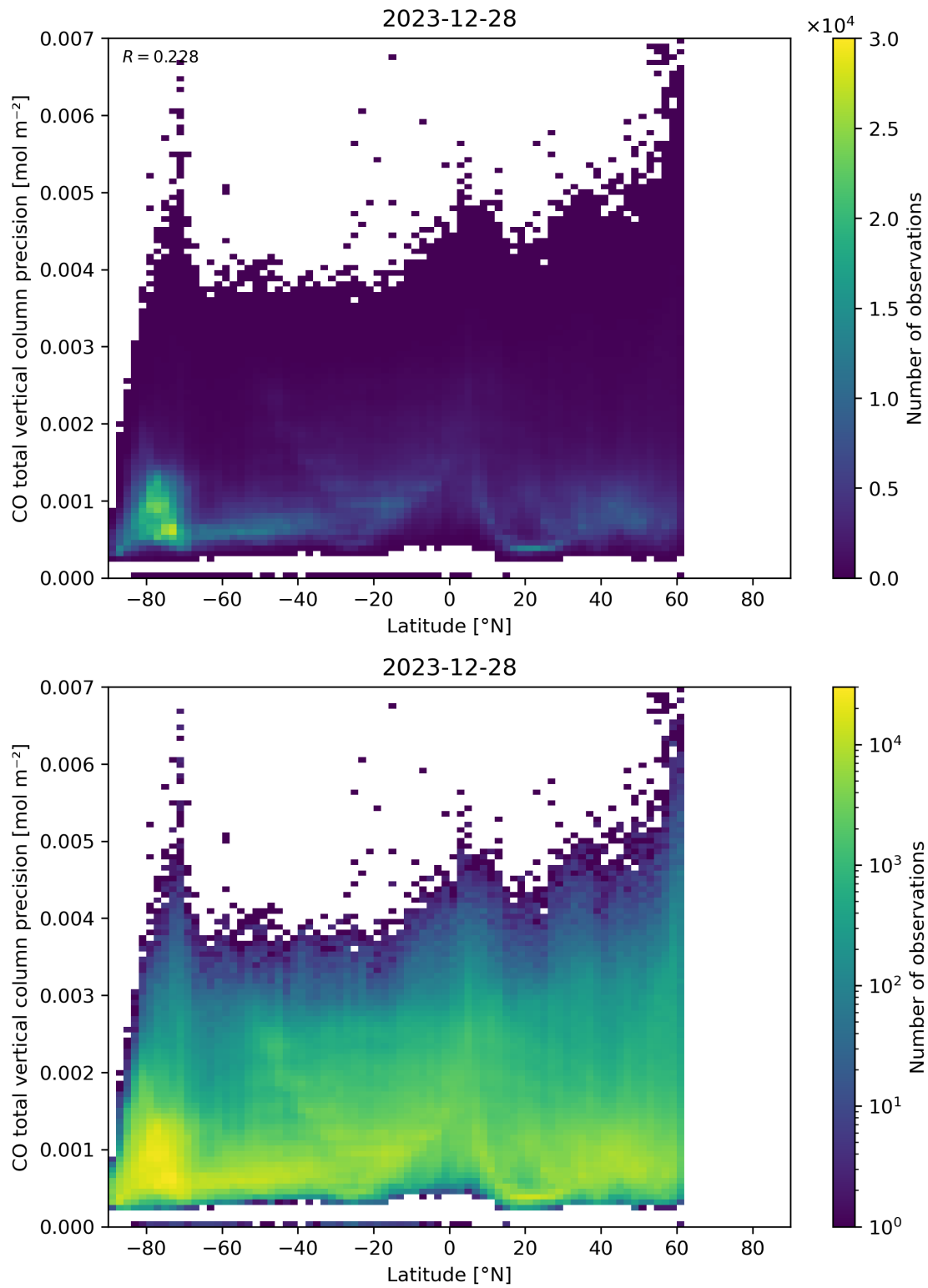
Figure 53: Scatter density plot of “Latitude” against “CO total vertical column precision” for 2023-12-27 to 2023-12-29.
