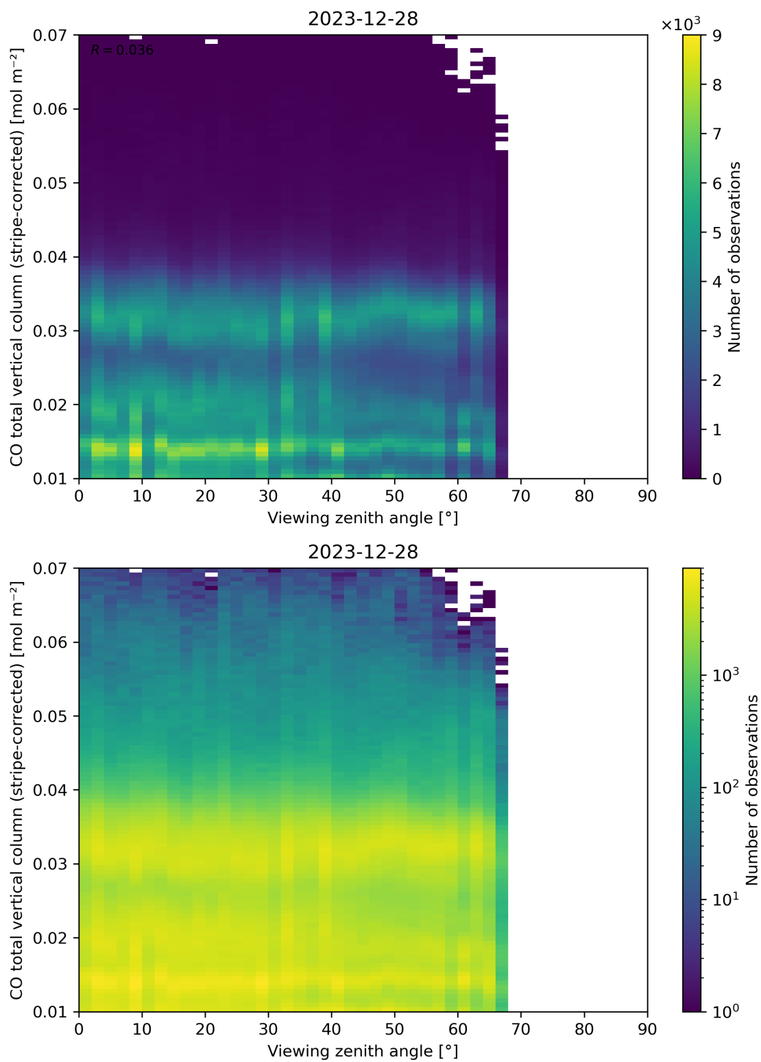
Figure 70: Scatter density plot of “Viewing zenith angle” against “CO total vertical column (stripe-corrected)” for 2023-12-27 to 2023-12-29.
