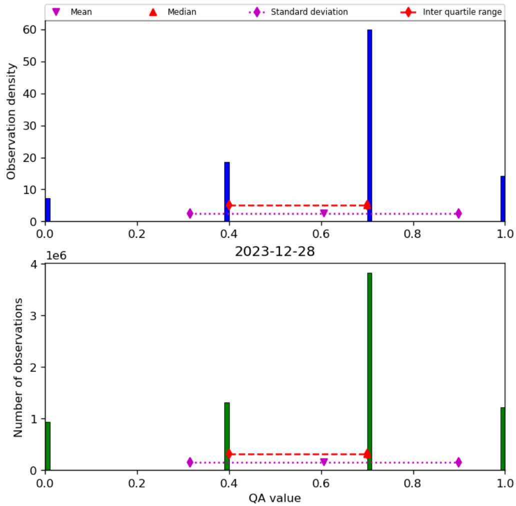
Figure 17: Histogram of “QA value” for 2023-12-27 to 2023-12-29
