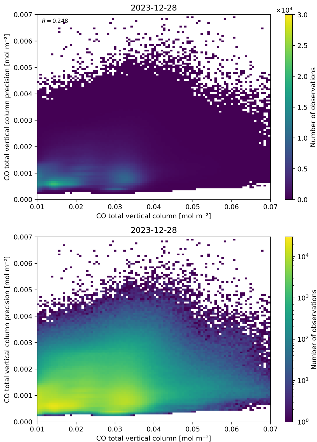
Figure 34: Scatter density plot of “CO total vertical column” against “CO total vertical column precision” for 2023-12-27 to 2023-12-29.
