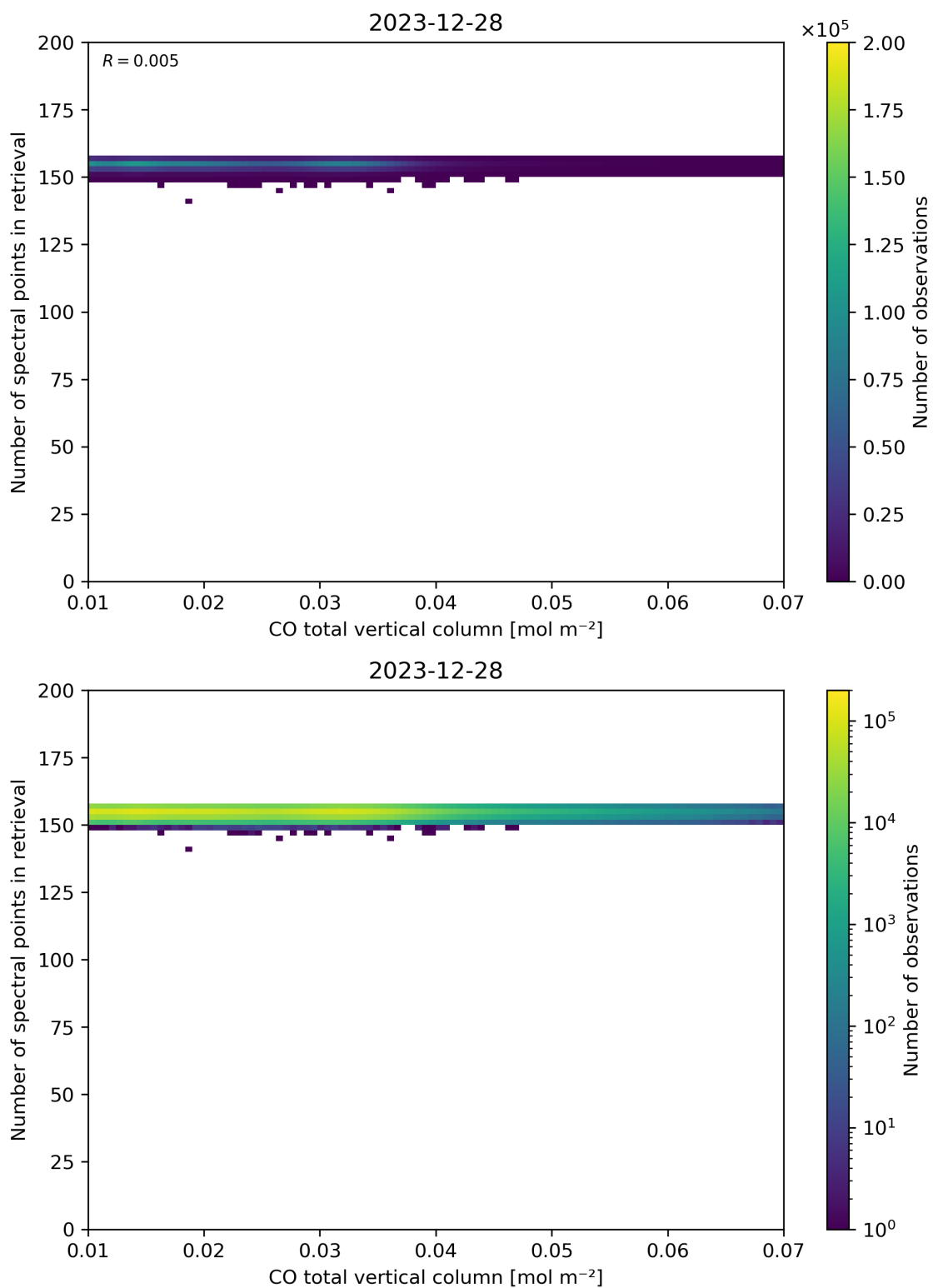
Figure 43: Scatter density plot of “CO total vertical column” against “Number of spectral points in retrieval” for 2023-12-27 to 2023-12-29.
