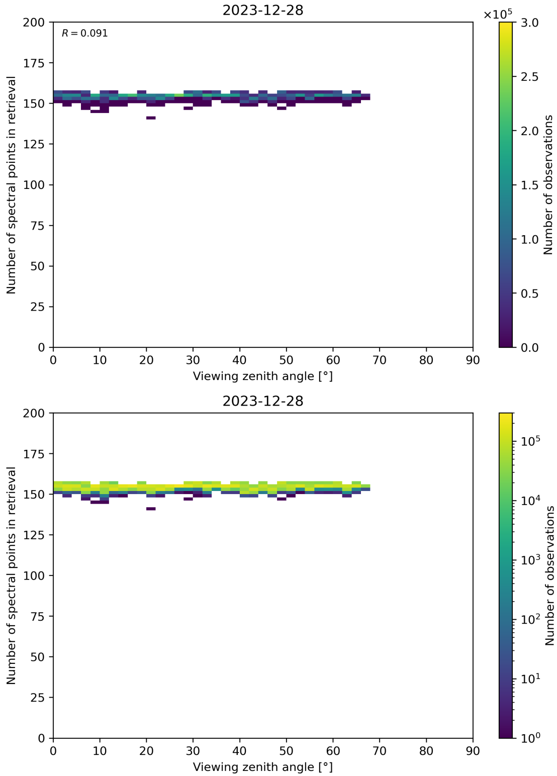
Figure 76: Scatter density plot of “Viewing zenith angle” against “Number of spectral points in retrieval” for 2023-12-27 to 2023-12-29.
