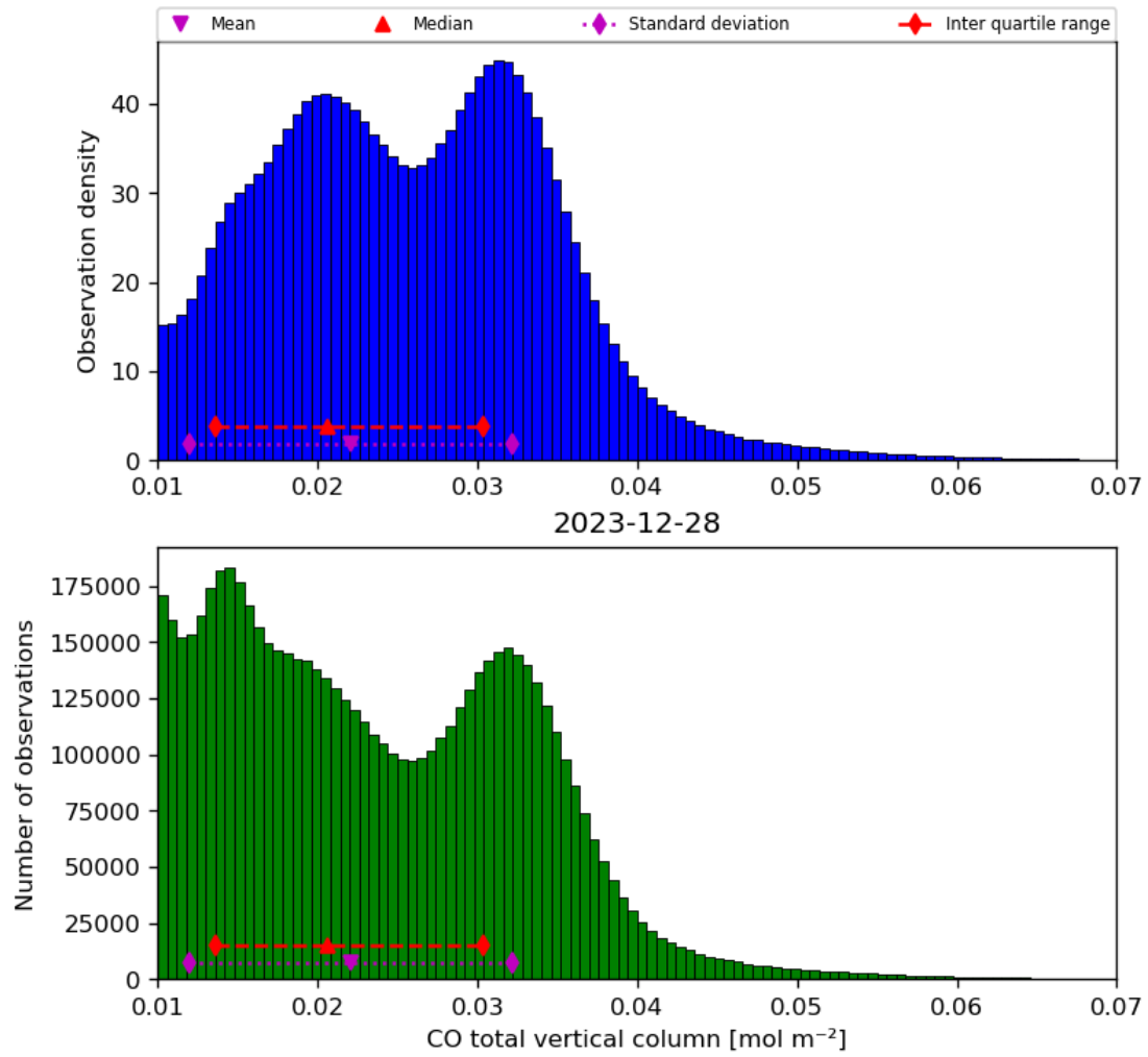
Figure 18: Histogram of “CO total vertical column” for 2023-12-27 to 2023-12-29
