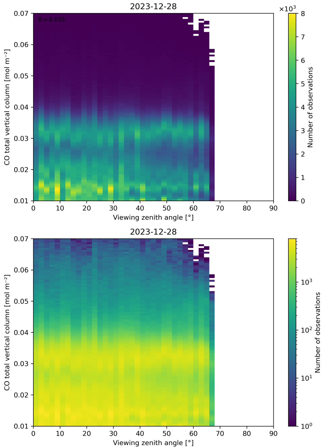
Figure 69: Scatter density plot of “Viewing zenith angle” against “CO total vertical column” for 2023-12-27 to 2023-12-29.
