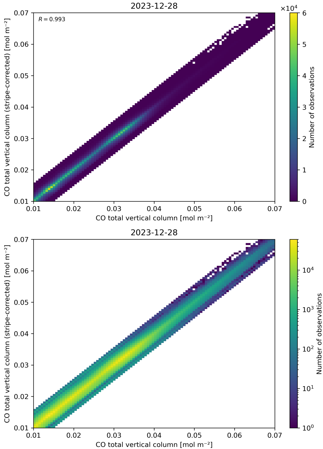
Figure 33: Scatter density plot of “CO total vertical column” against “CO total vertical column (stripe-corrected)” for 2023-12-27 to 2023-12-29.
