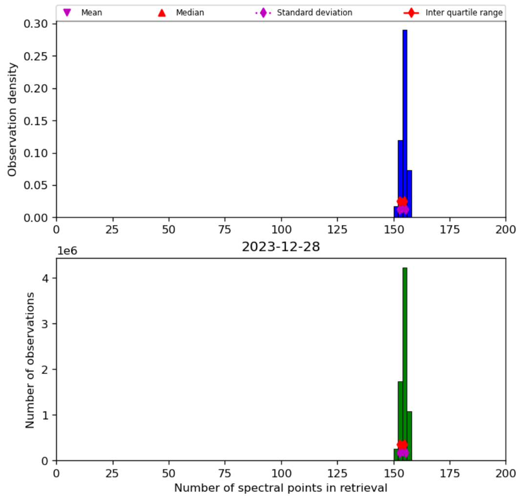
Figure 21: Histogram of “Number of spectral points in retrieval” for 2023-12-27 to 2023-12-29
