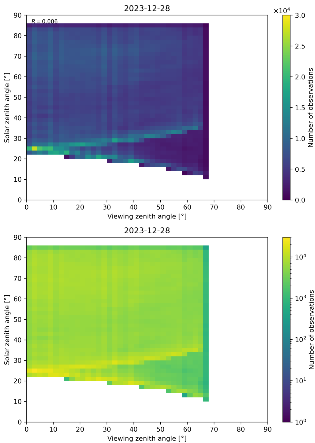
Figure 77: Scatter density plot of “Viewing zenith angle” against “Solar zenith angle” for 2023-12-27 to 2023-12-29.
