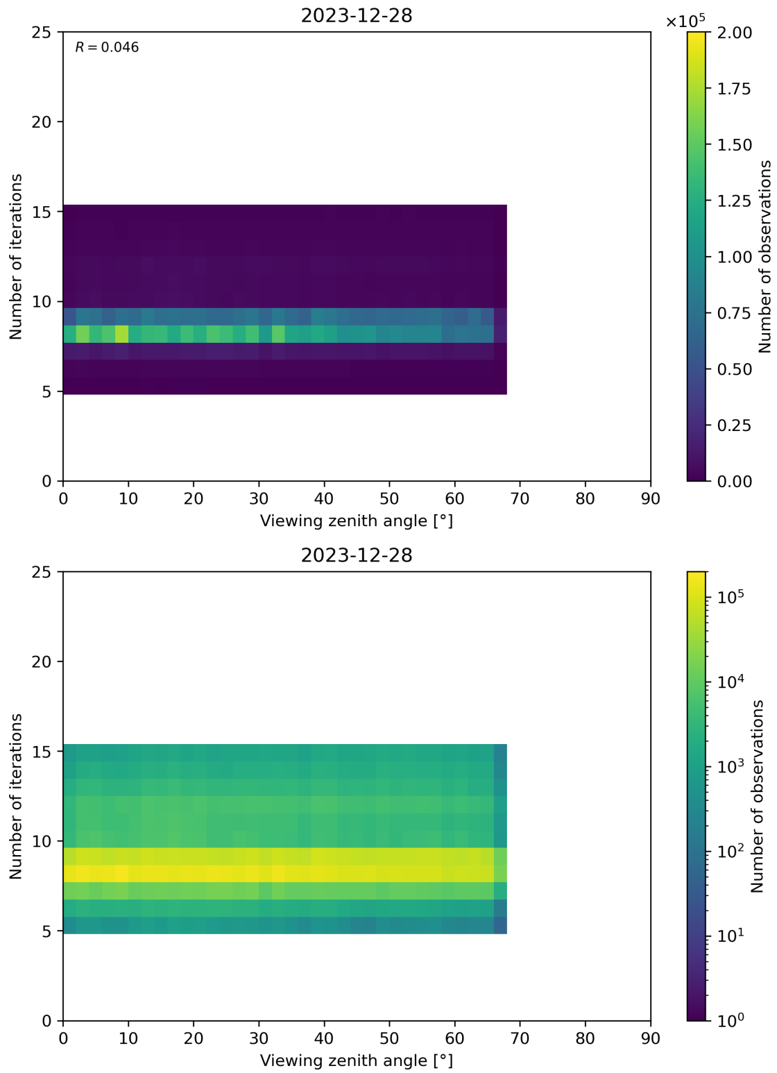
Figure 75: Scatter density plot of “Viewing zenith angle” against “Number of iterations” for 2023-12-27 to 2023-12-29.
