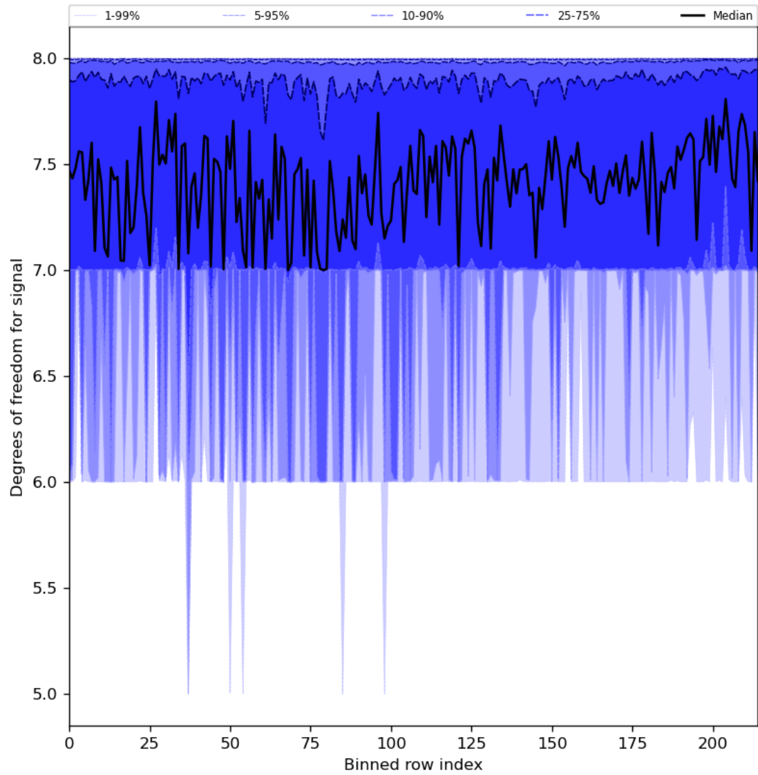
Figure 31: Along track statistics of “Degrees of freedom for signal” for 2023-12-27 to 2023-12-29
