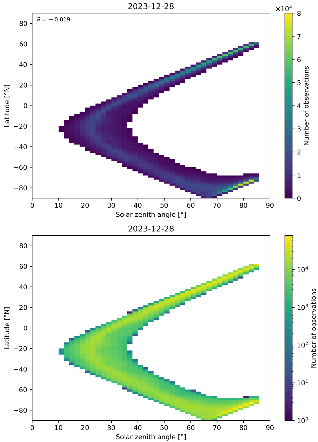
Figure 66: Scatter density plot of “Solar zenith angle” against “Latitude” for 2023-12-27 to 2023-12-29.
