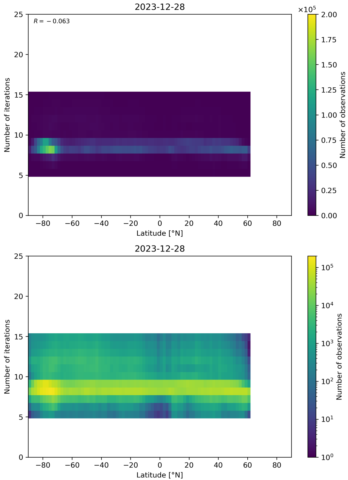
Figure 56: Scatter density plot of “Latitude” against “Number of iterations” for 2023-12-27 to 2023-12-29.
