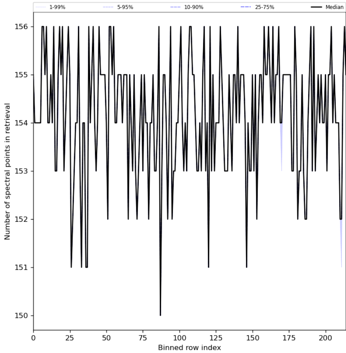
Figure 29: Along track statistics of “Number of spectral points in retrieval” for 2023-12-27 to 2023-12-29
