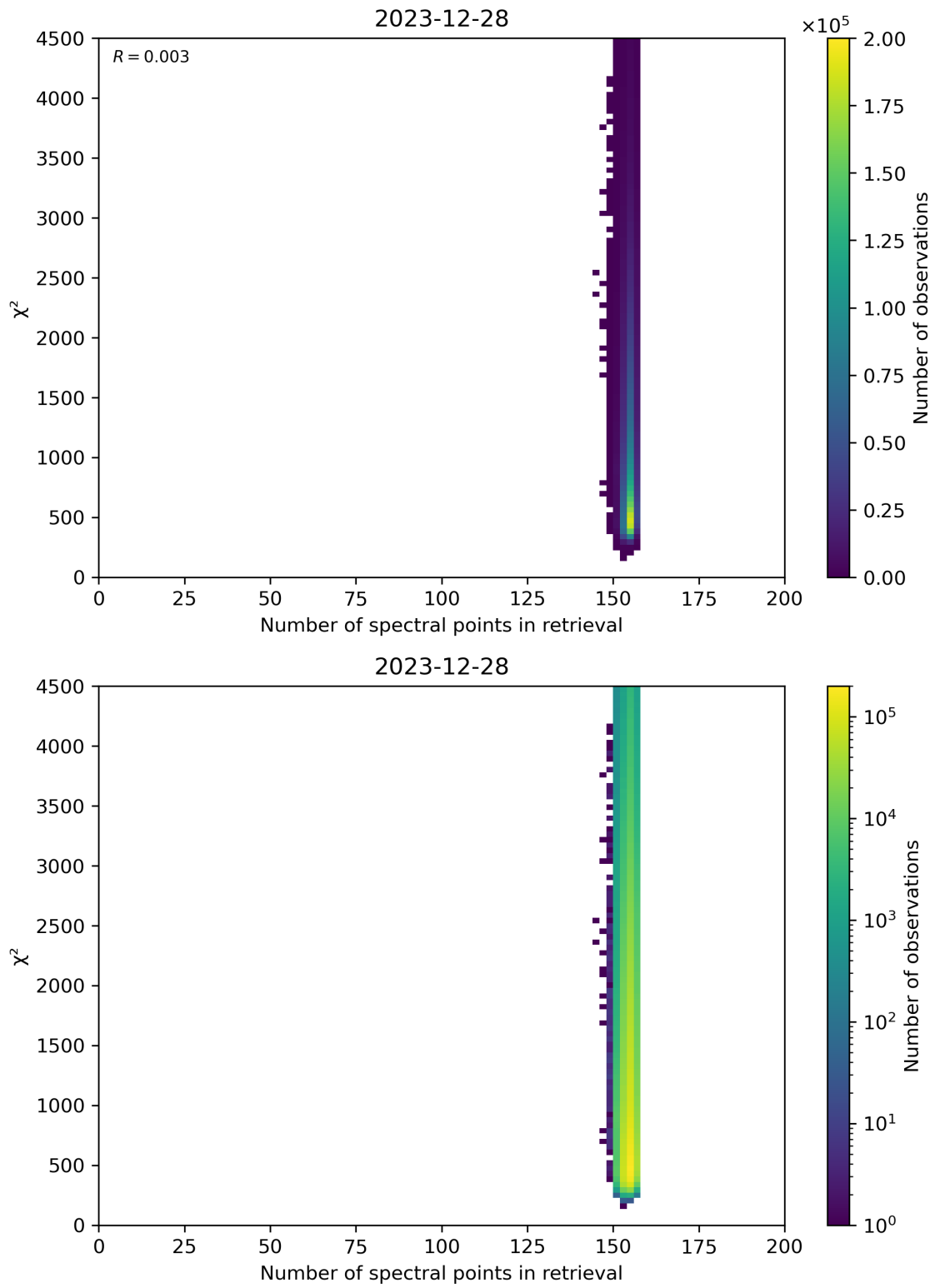
Figure 58: Scatter density plot of “Number of spectral points in retrieval” against “ \chi^2 ” for 2023-12-27 to 2023-12-29.
