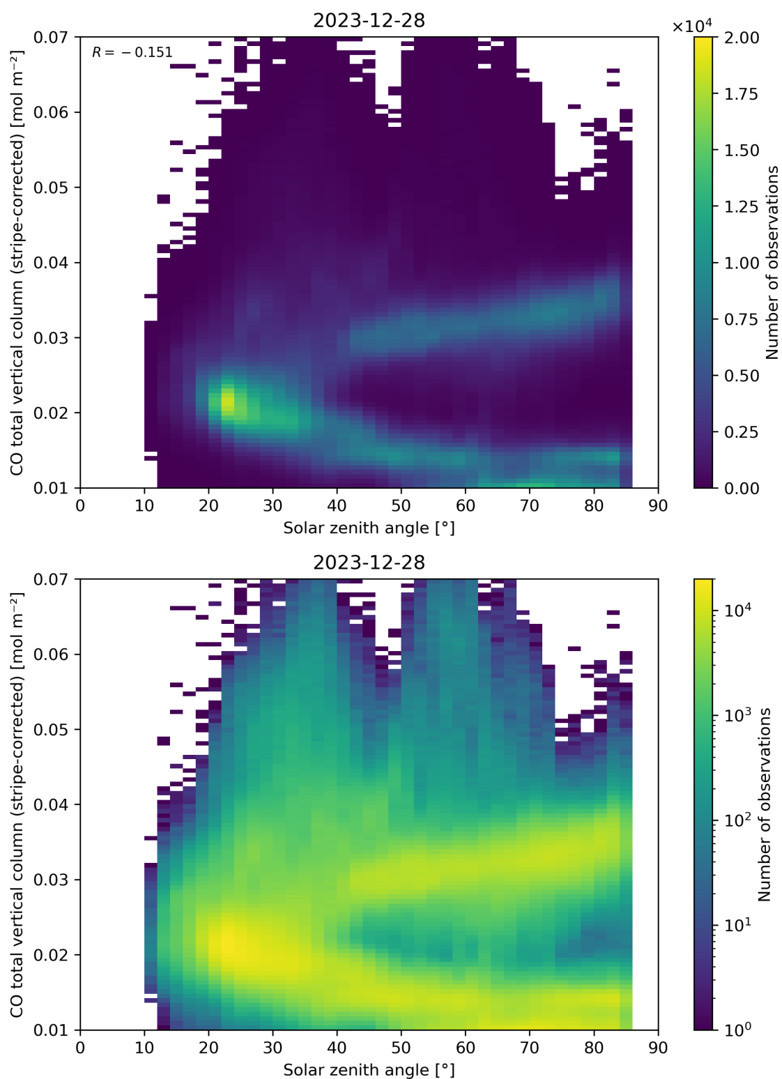
Figure 62: Scatter density plot of “Solar zenith angle” against “CO total vertical column (stripe-corrected)” for 2023-12-27 to 2023-12-29.
