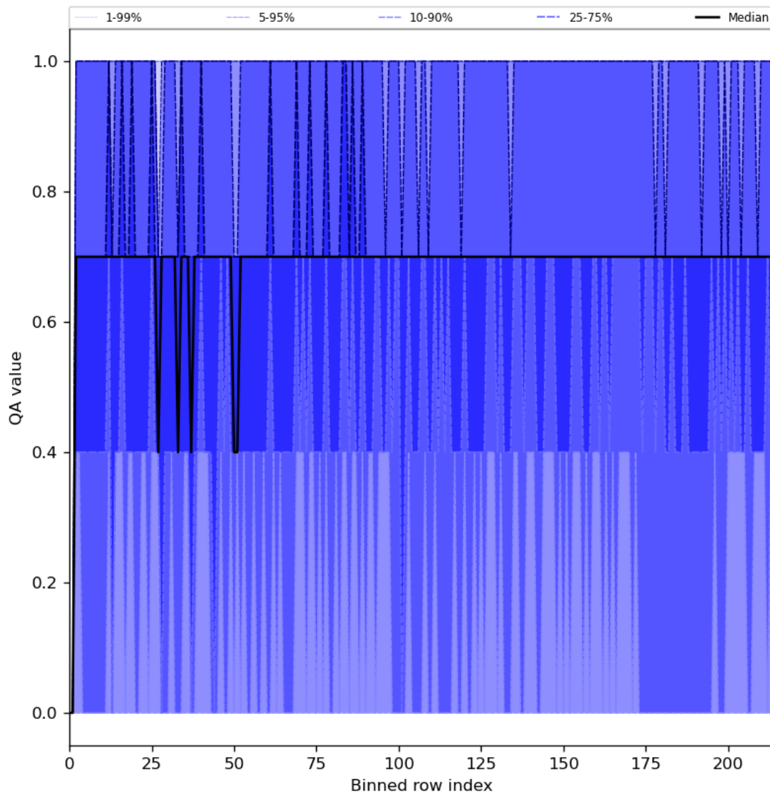
Figure 25: Along track statistics of “QA value” for 2023-12-27 to 2023-12-29
