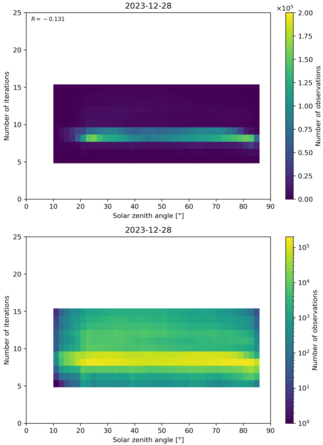
Figure 67: Scatter density plot of “Solar zenith angle” against “Number of iterations” for 2023-12-27 to 2023-12-29.
