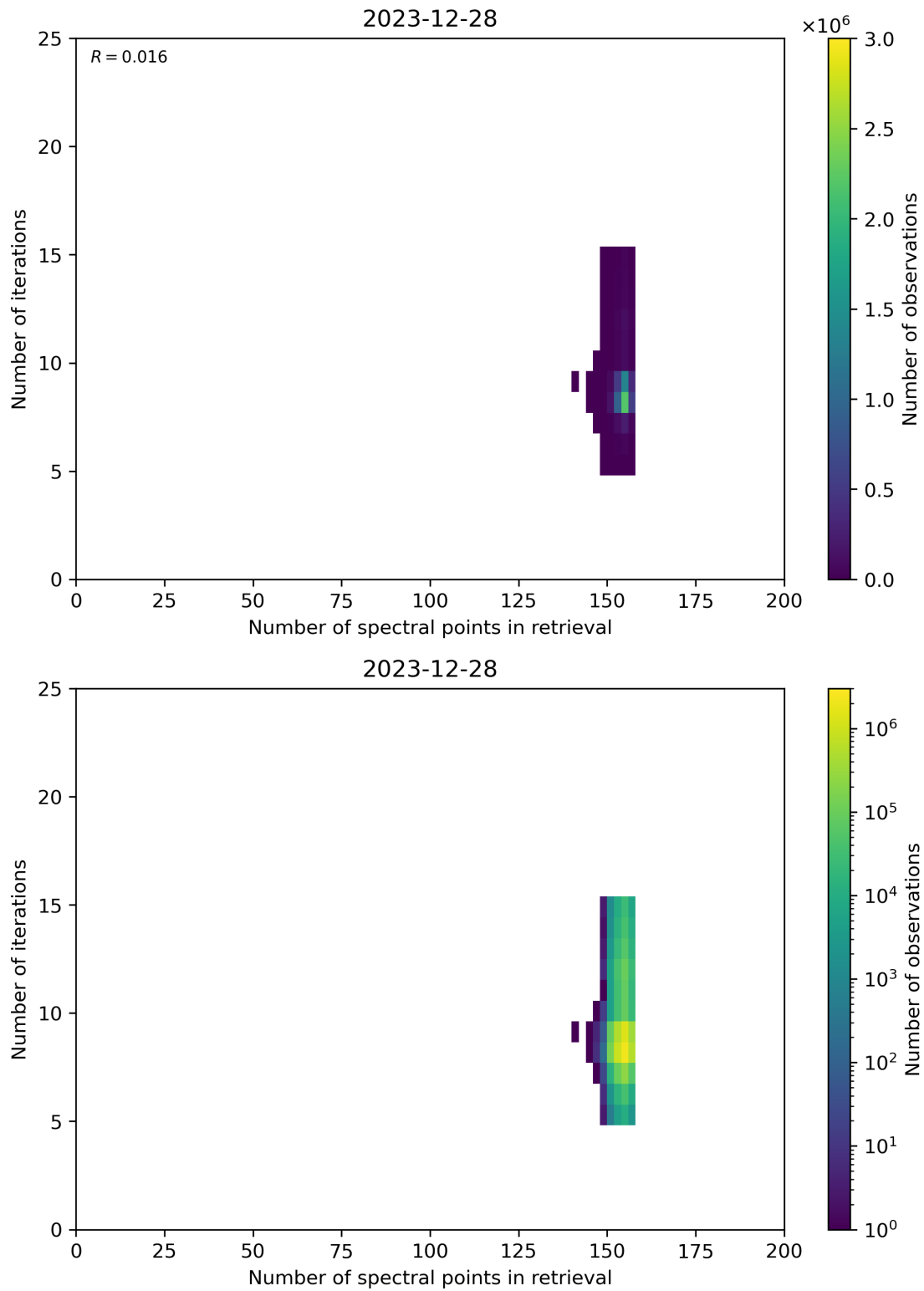
Figure 60: Scatter density plot of “Number of spectral points in retrieval” against “Number of iterations” for 2023-12-27 to 2023-12-29.
