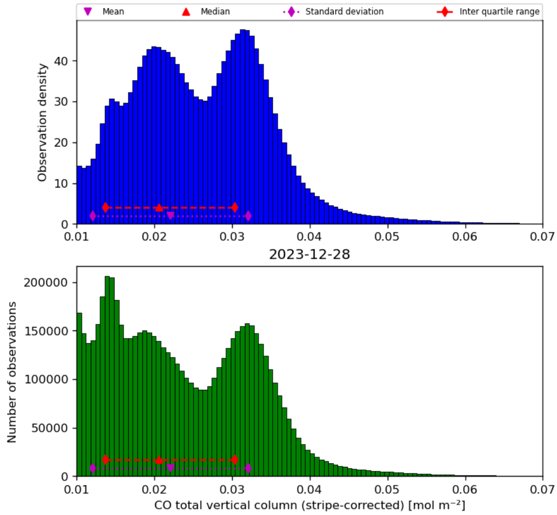
Figure 19: Histogram of “CO total vertical column (stripe-corrected)” for 2023-12-27 to 2023-12-29
