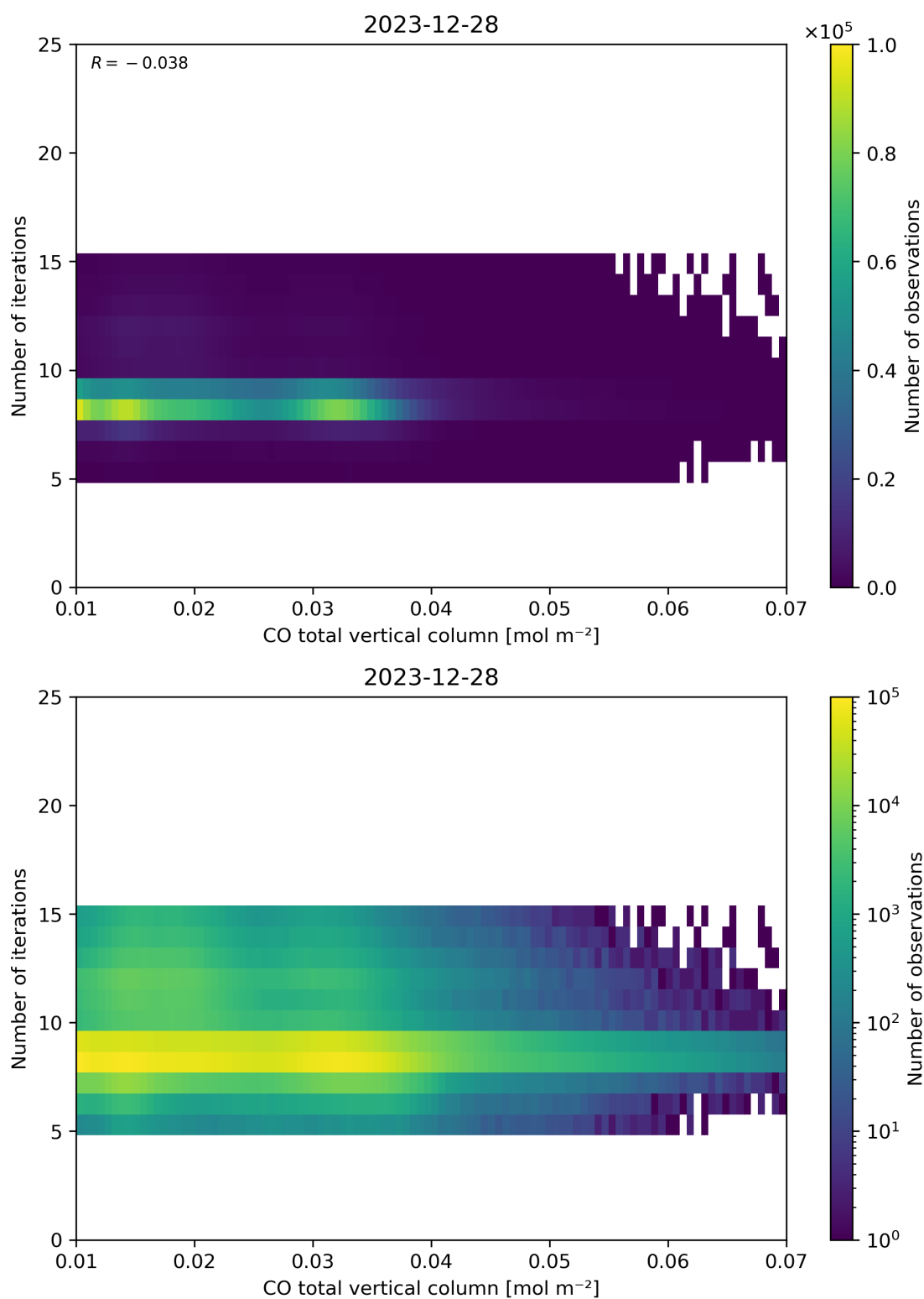
Figure 42: Scatter density plot of “CO total vertical column” against “Number of iterations” for 2023-12-27 to 2023-12-29.
