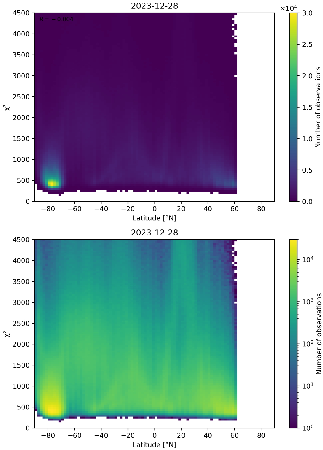
Figure 54: Scatter density plot of “Latitude” against “ \chi^2 ” for 2023-12-27 to 2023-12-29.
