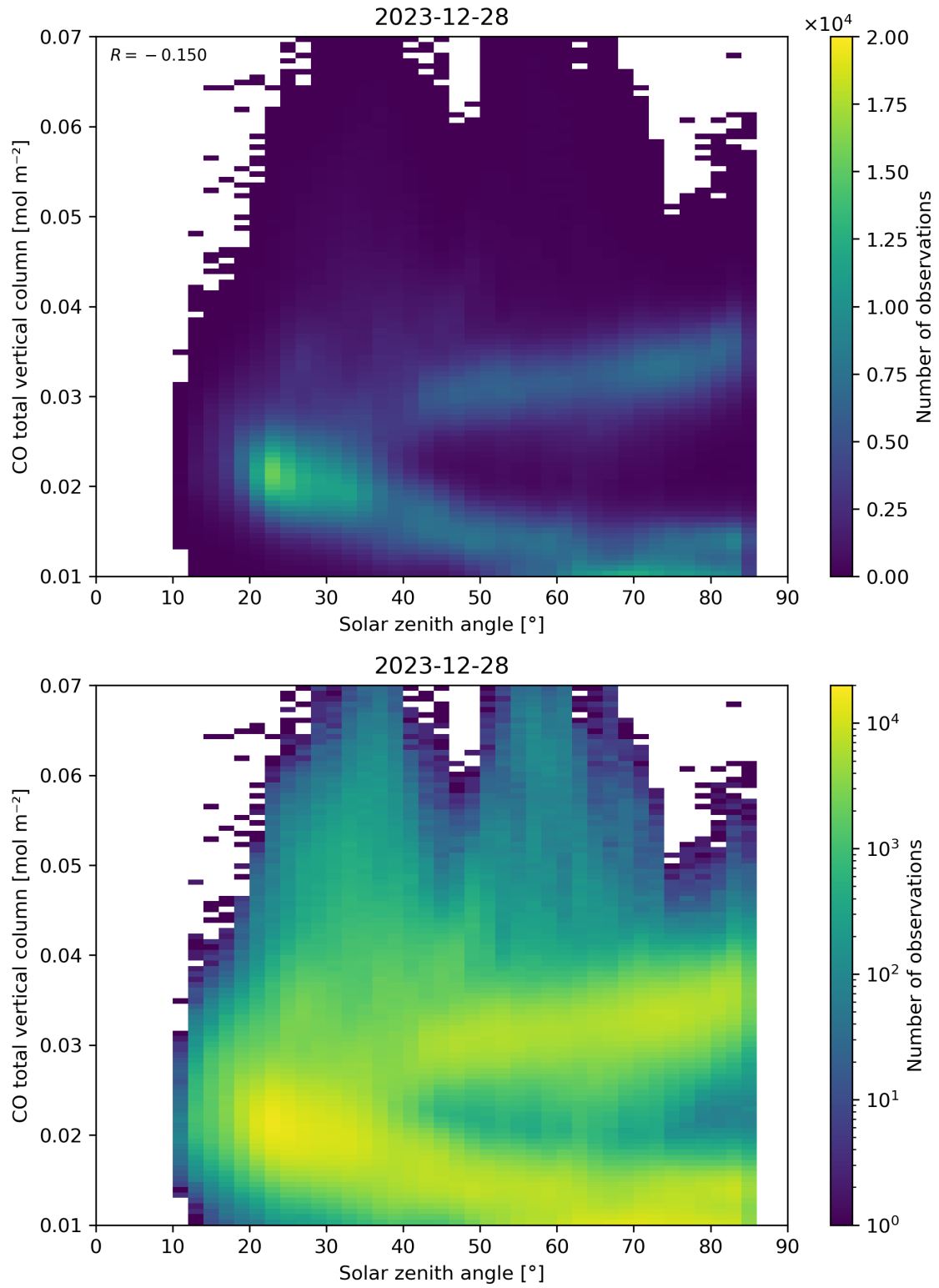
Figure 61: Scatter density plot of “Solar zenith angle” against “CO total vertical column” for 2023-12-27 to 2023-12-29.
