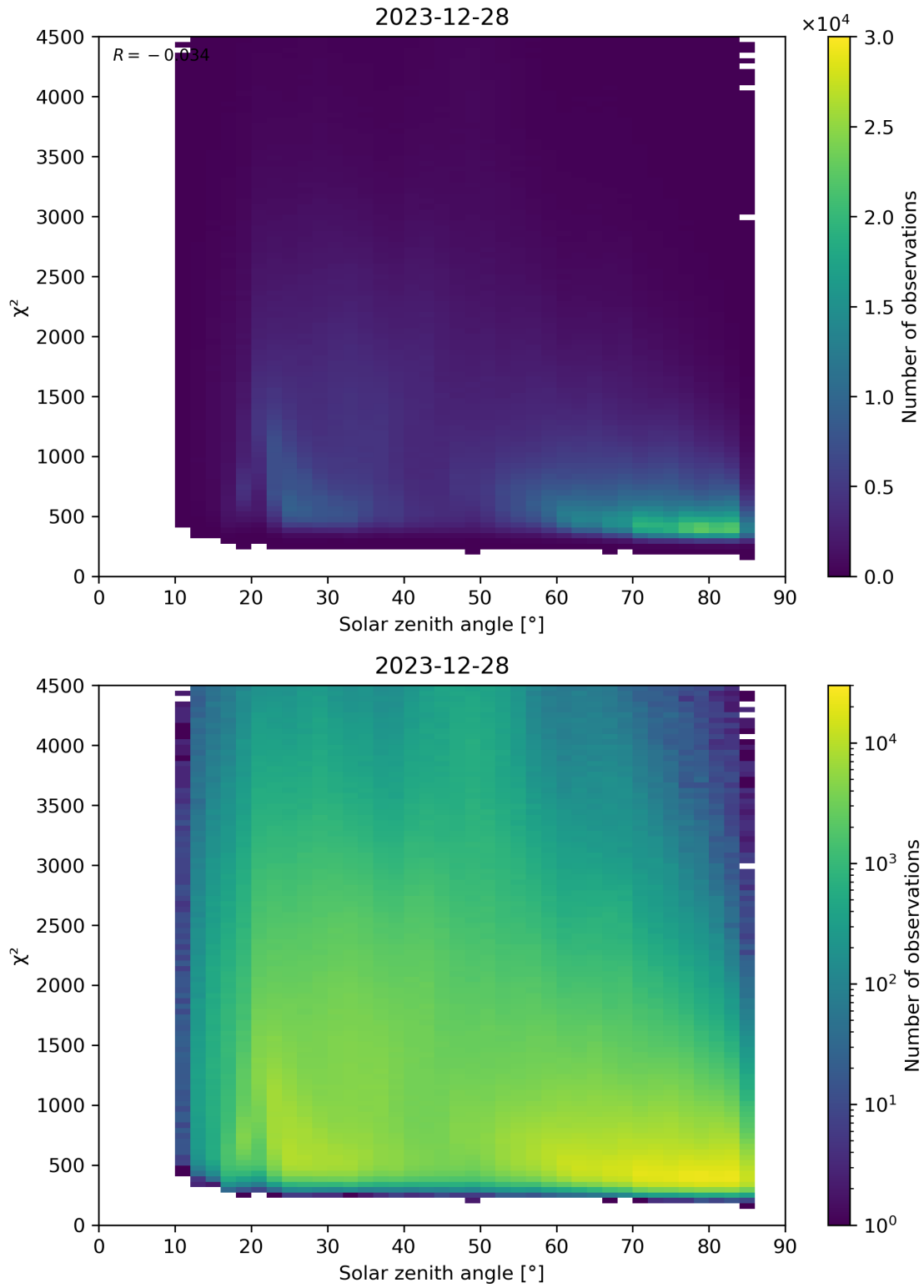
Figure 64: Scatter density plot of “Solar zenith angle” against “ \chi^2 ” for 2023-12-27 to 2023-12-29.
