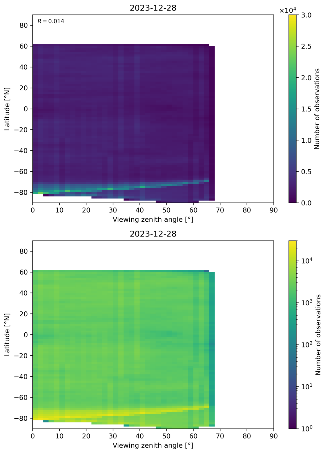
Figure 74: Scatter density plot of “Viewing zenith angle” against “Latitude” for 2023-12-27 to 2023-12-29.
