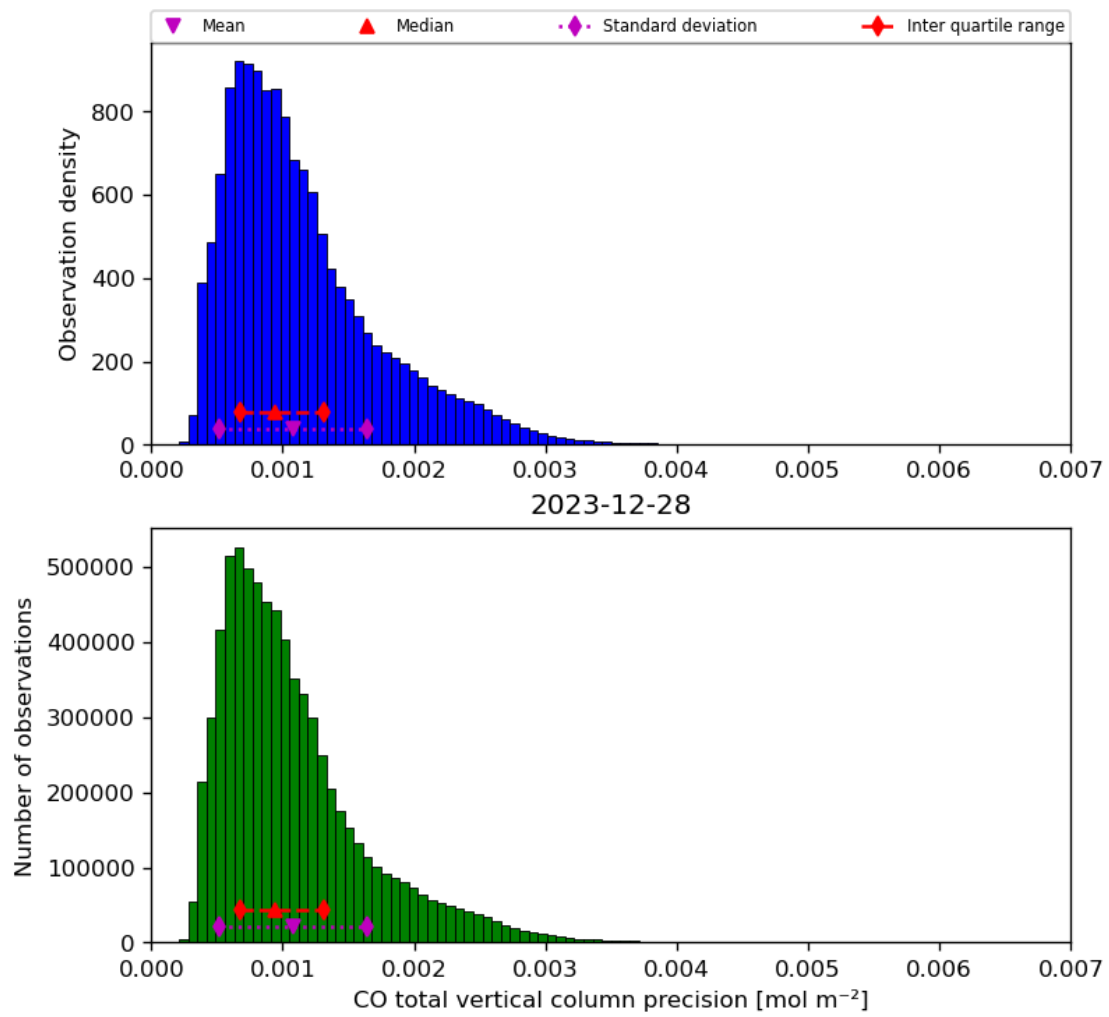
Figure 20: Histogram of “CO total vertical column precision” for 2023-12-27 to 2023-12-29
