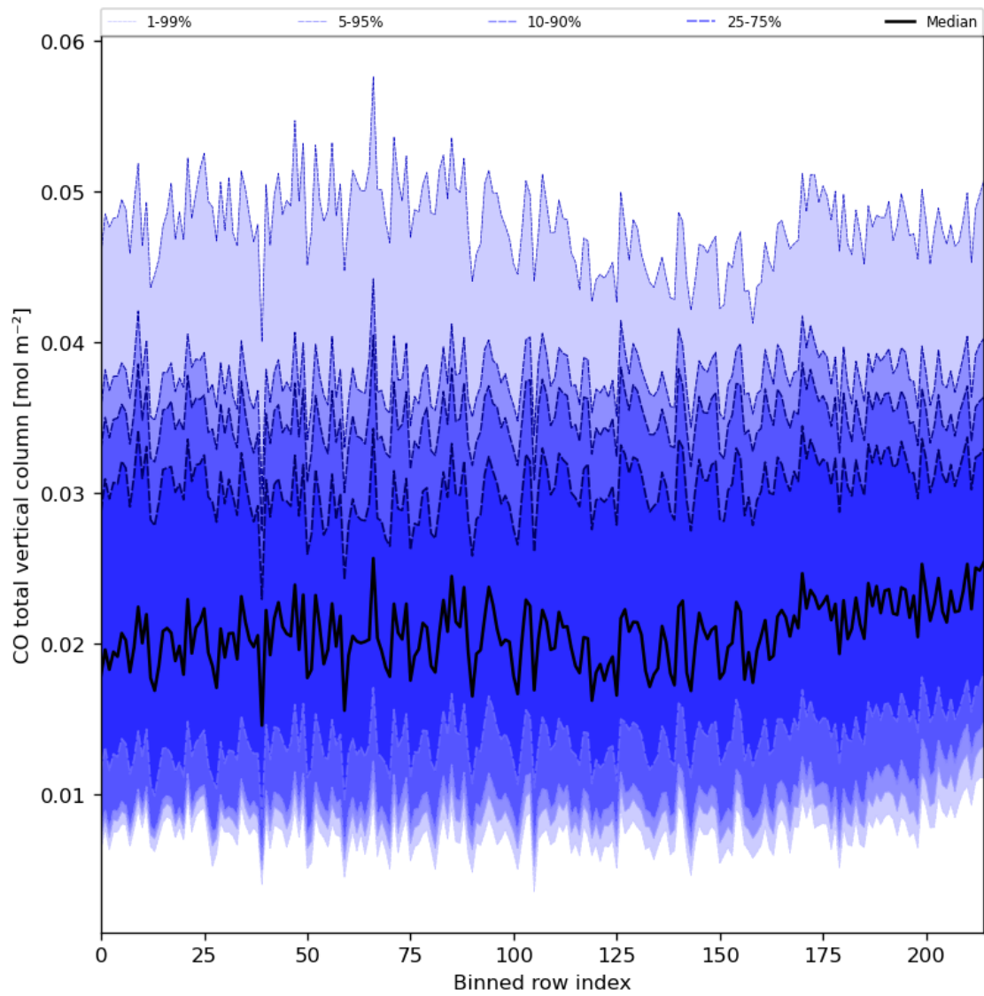
Figure 26: Along track statistics of “CO total vertical column” for 2023-12-27 to 2023-12-29
