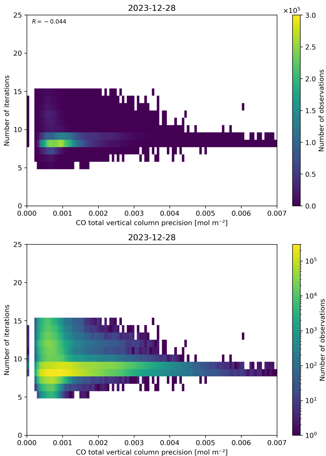
Figure 46: Scatter density plot of “CO total vertical column precision” against “Number of iterations” for 2023-12-27 to 2023-12-29.
