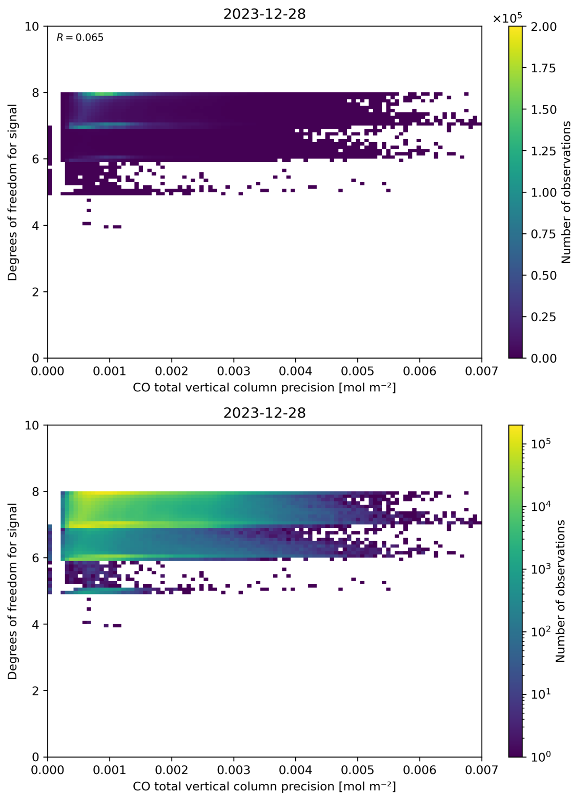
Figure 45: Scatter density plot of “CO total vertical column precision” against “Degrees of freedom for signal” for 2023-12-27 to 2023-12-29.
