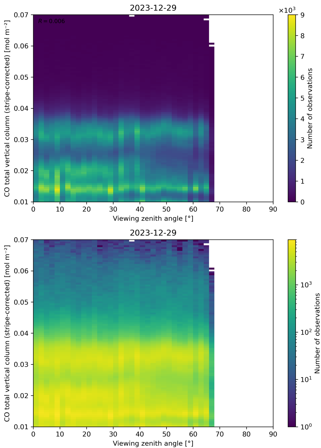
Figure 70: Scatter density plot of “Viewing zenith angle” against “CO total vertical column (stripe-corrected)” for 2023-12-28 to 2023-12-30.
