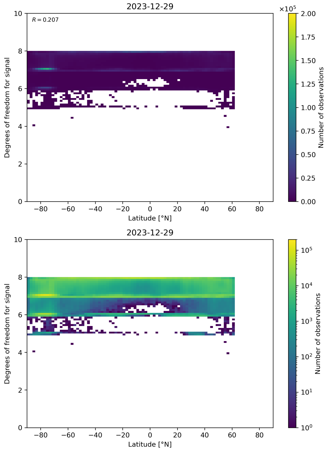
Figure 55: Scatter density plot of “Latitude” against “Degrees of freedom for signal” for 2023-12-28 to 2023-12-30.
