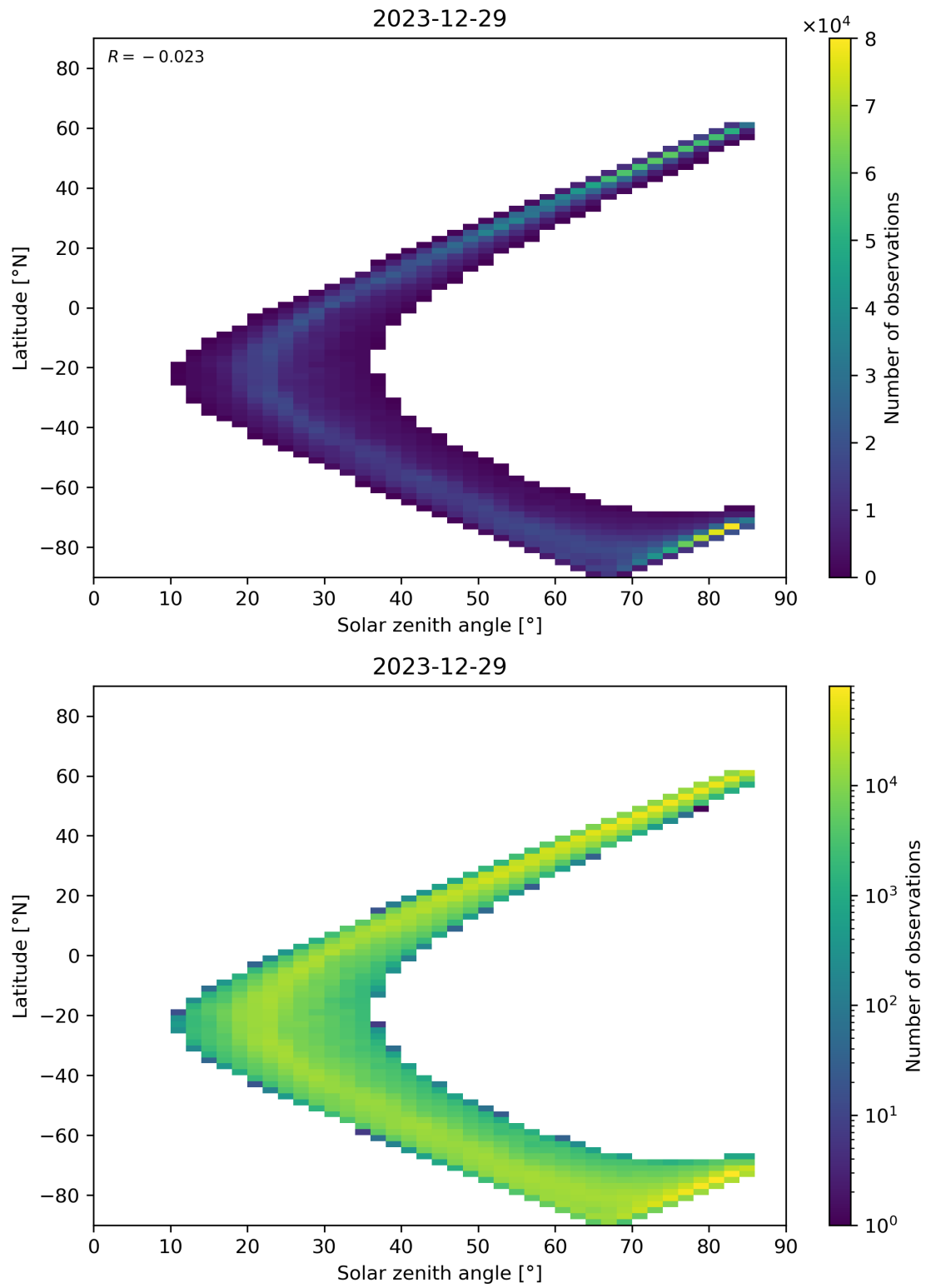
Figure 66: Scatter density plot of “Solar zenith angle” against “Latitude” for 2023-12-28 to 2023-12-30.
