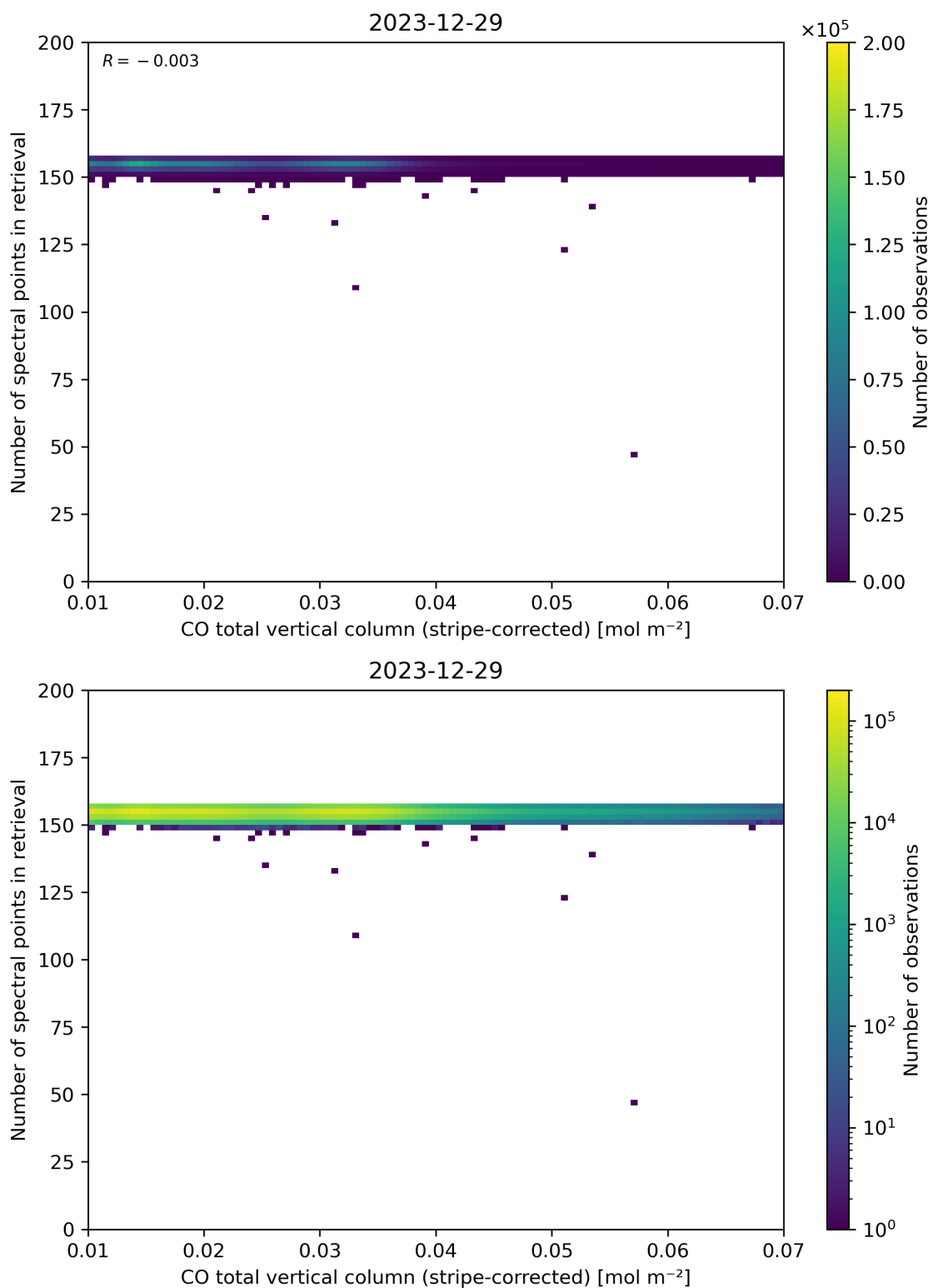
Figure 40: Scatter density plot of “CO total vertical column (stripe-corrected)” against “Number of spectral points in retrieval” for 2023-12-28 to 2023-12-30.
