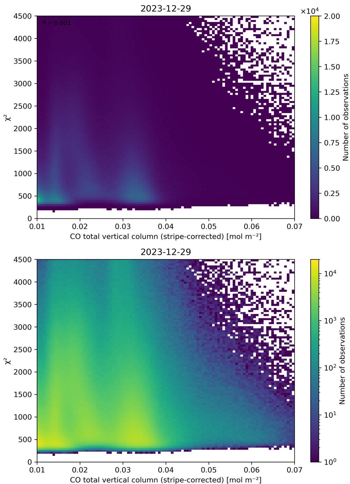
Figure 37: Scatter density plot of “CO total vertical column (stripe-corrected)” against “ \chi^2 ” for 2023-12-28 to 2023-12-30.
