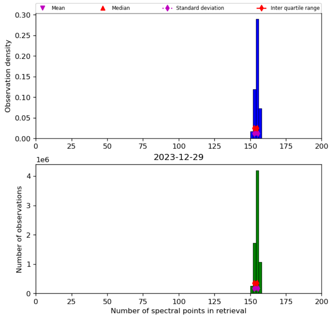
Figure 21: Histogram of “Number of spectral points in retrieval” for 2023-12-28 to 2023-12-30
