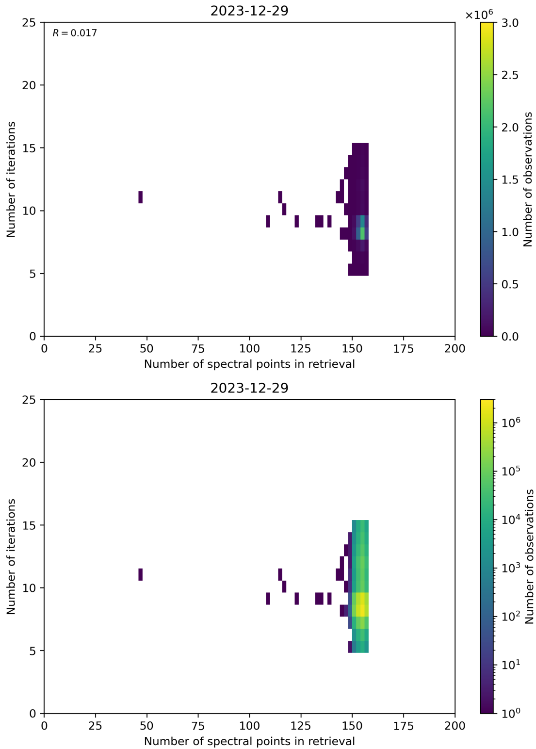
Figure 60: Scatter density plot of “Number of spectral points in retrieval” against “Number of iterations” for 2023-12-28 to 2023-12-30.
