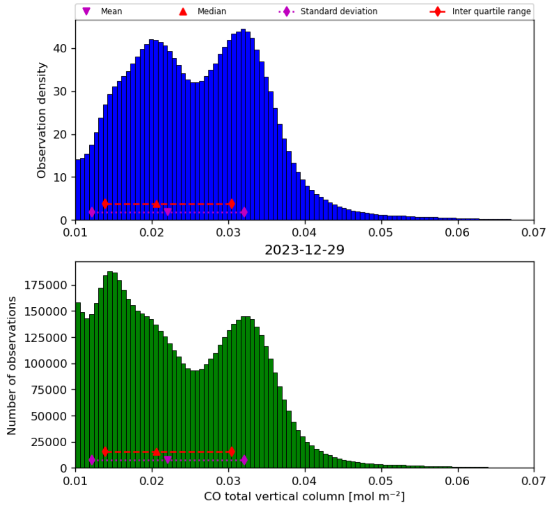
Figure 18: Histogram of “CO total vertical column” for 2023-12-28 to 2023-12-30
