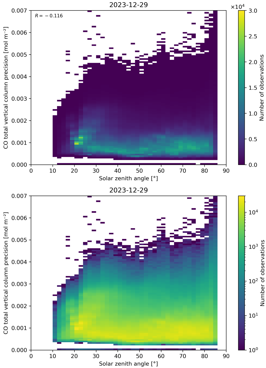
Figure 63: Scatter density plot of “Solar zenith angle” against “CO total vertical column precision” for 2023-12-28 to 2023-12-30.
