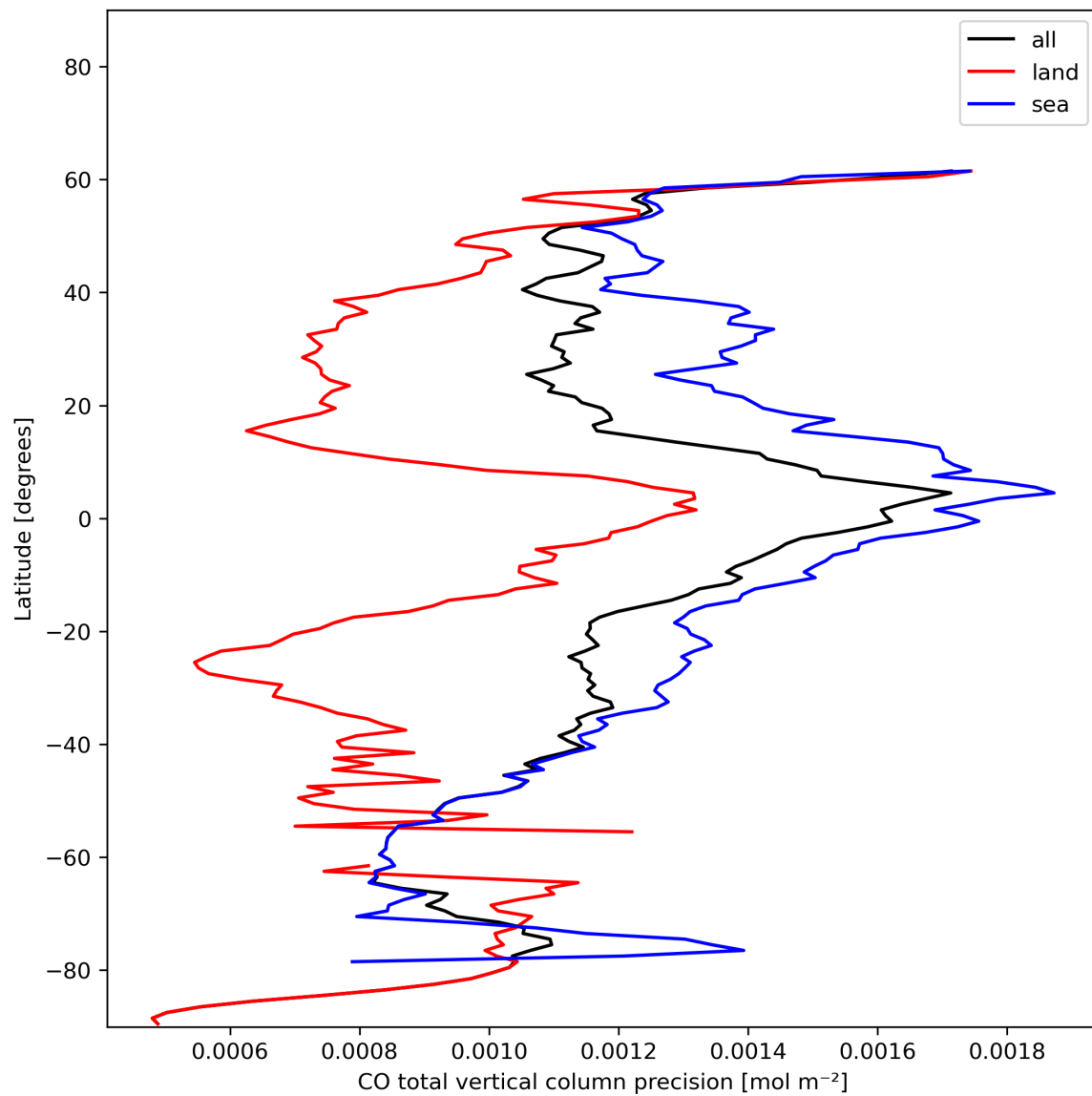
Figure 12: Zonal average of “CO total vertical column precision” for 2023-12-28 to 2023-12-30.
