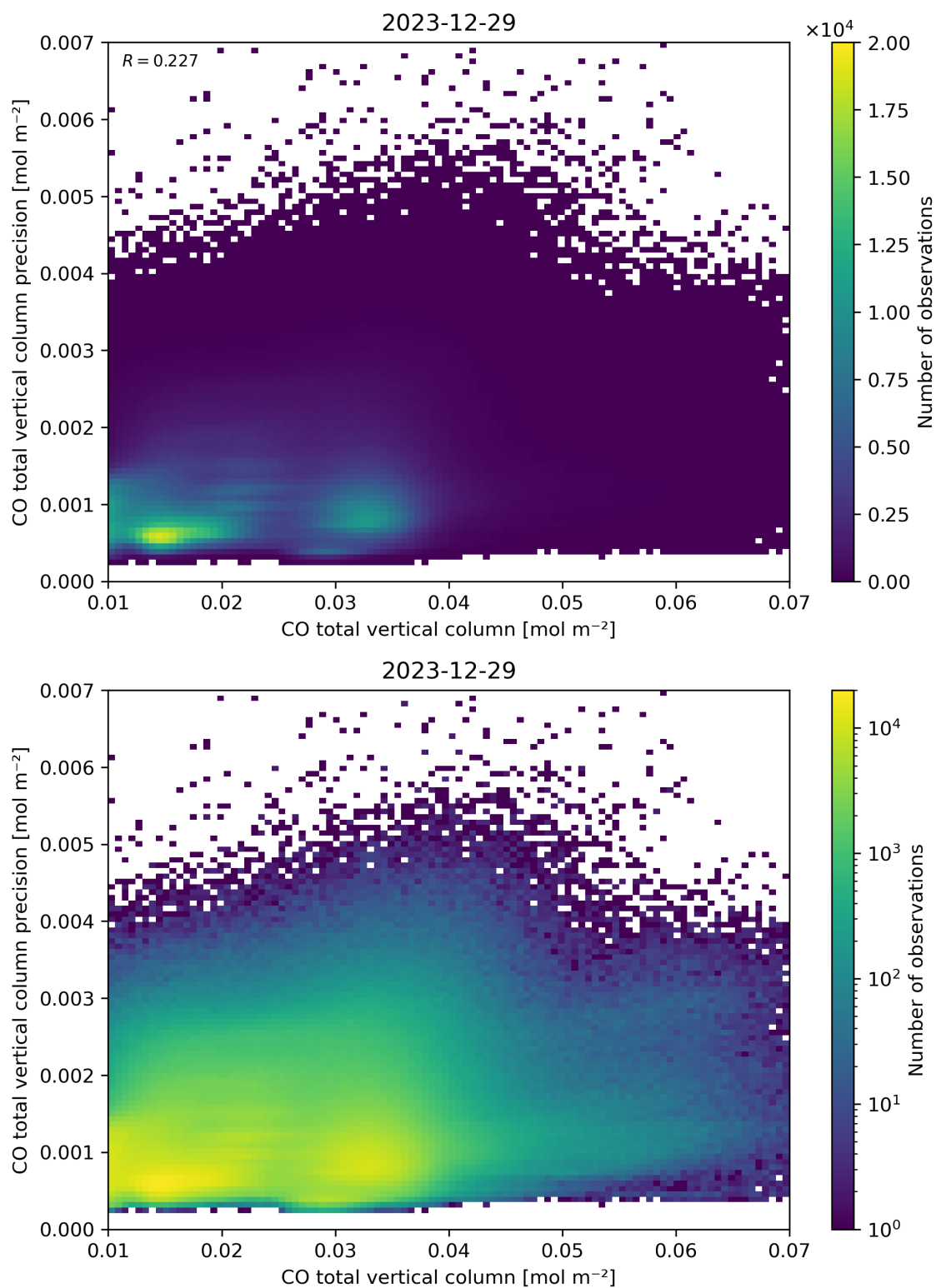
Figure 34: Scatter density plot of “CO total vertical column” against “CO total vertical column precision” for 2023-12-28 to 2023-12-30.
