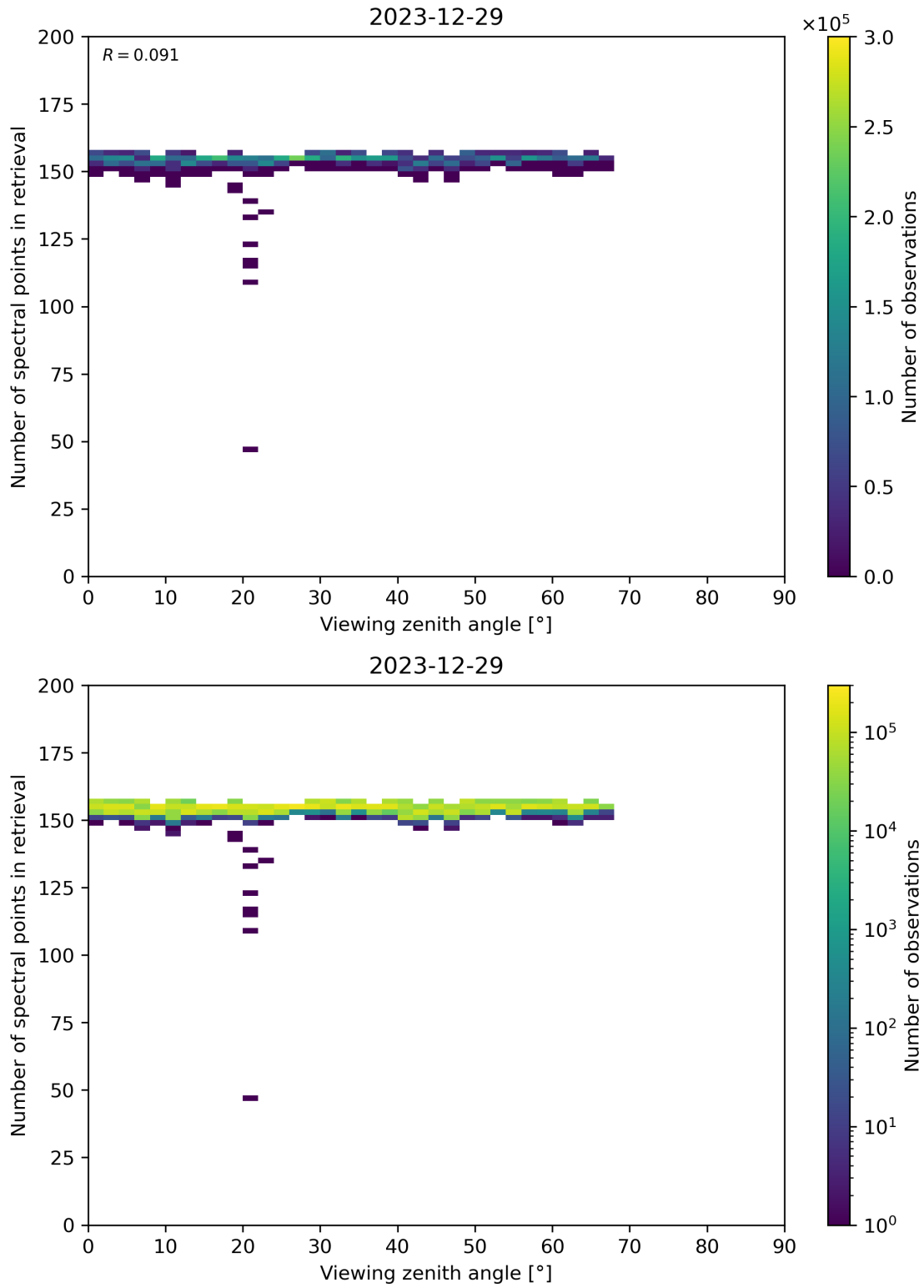
Figure 76: Scatter density plot of “Viewing zenith angle” against “Number of spectral points in retrieval” for 2023-12-28 to 2023-12-30.
