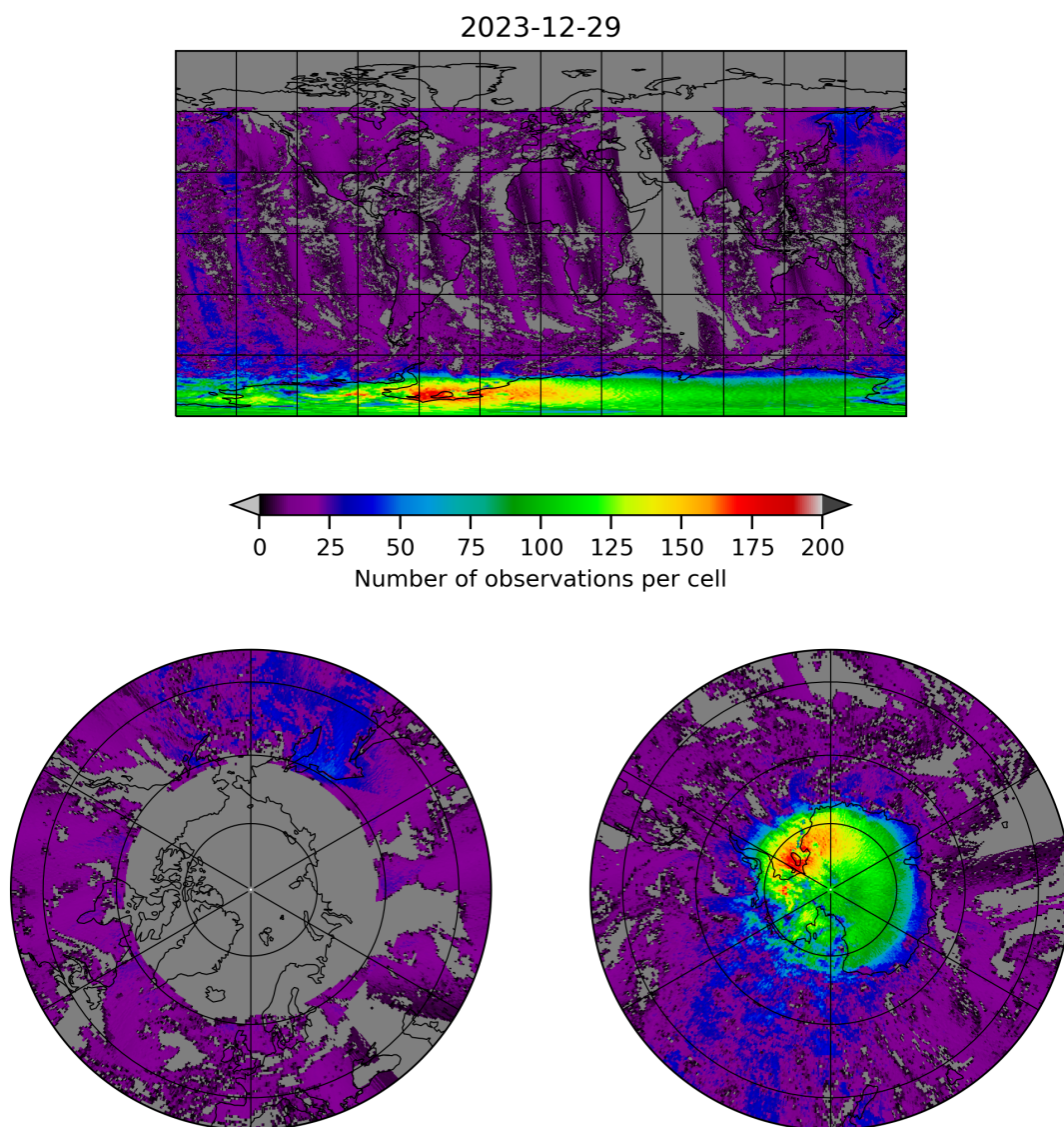
Figure 8: Map of the number of observations for 2023-12-28 to 2023-12-30
