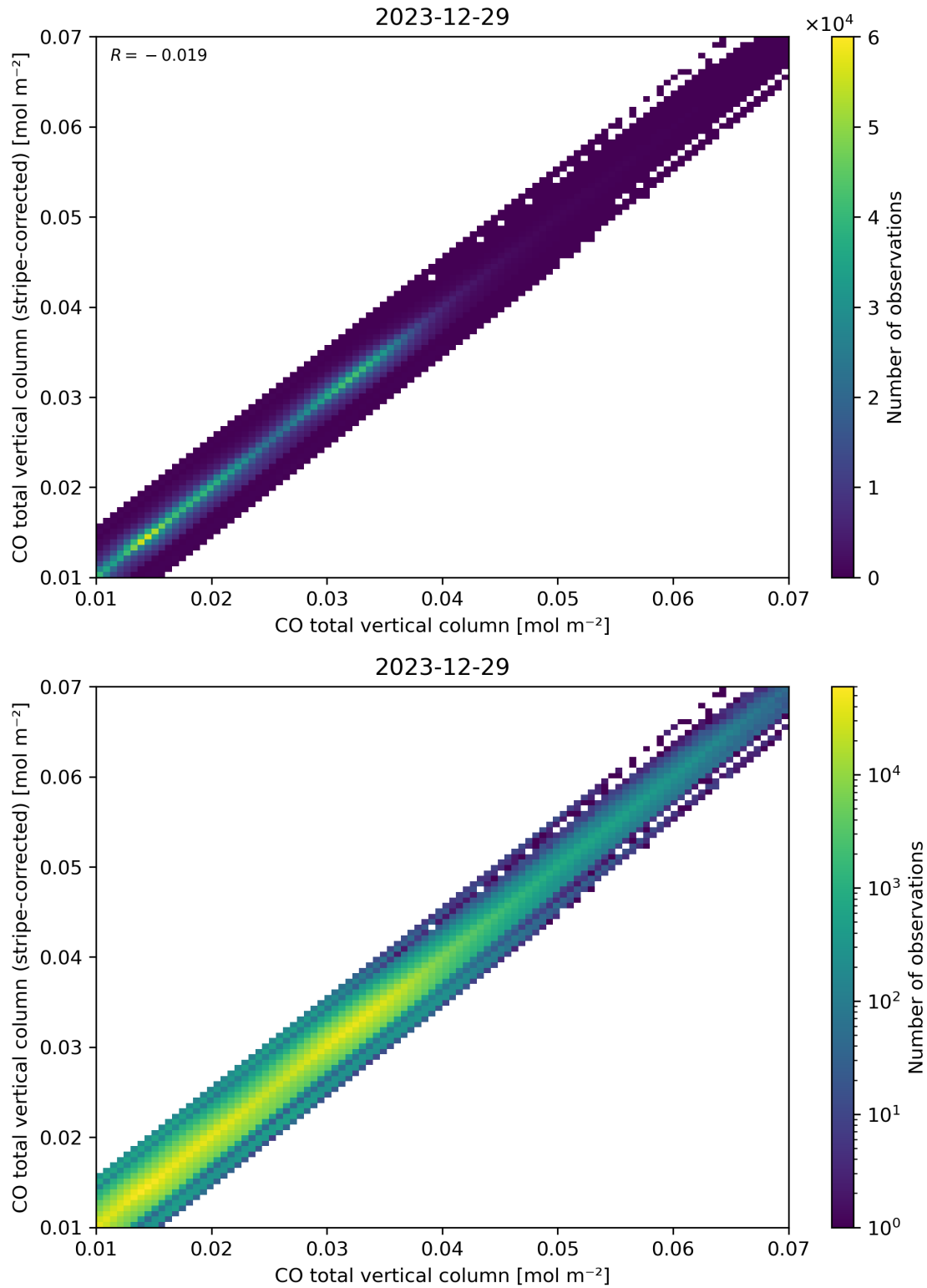
Figure 33: Scatter density plot of “CO total vertical column” against “CO total vertical column (stripe-corrected)” for 2023-12-28 to 2023-12-30.
