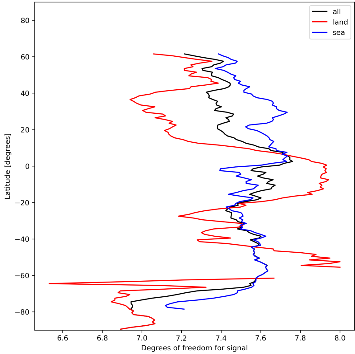
Figure 15: Zonal average of “Degrees of freedom for signal” for 2023-12-28 to 2023-12-30.
