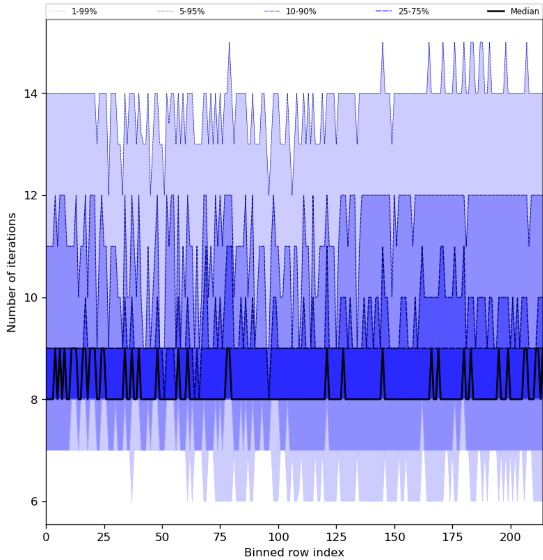
Figure 32: Along track statistics of “Number of iterations” for 2023-12-28 to 2023-12-30
