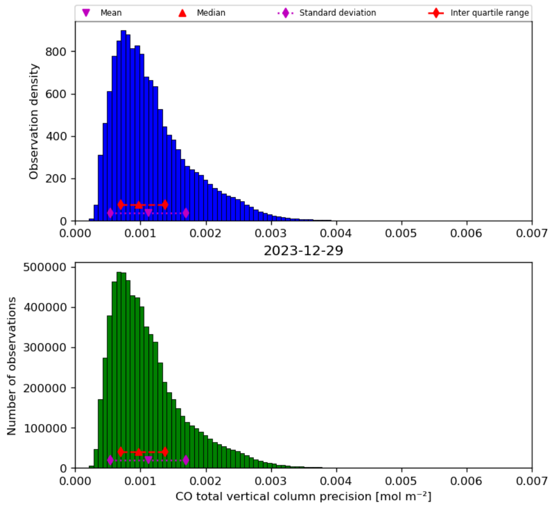
Figure 20: Histogram of “CO total vertical column precision” for 2023-12-28 to 2023-12-30
