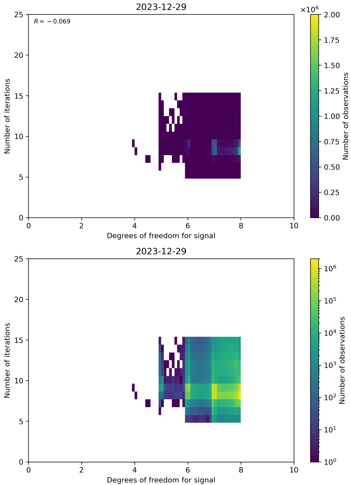
Figure 50: Scatter density plot of “Degrees of freedom for signal” against “Number of iterations” for 2023-12-28 to 2023-12-30.
