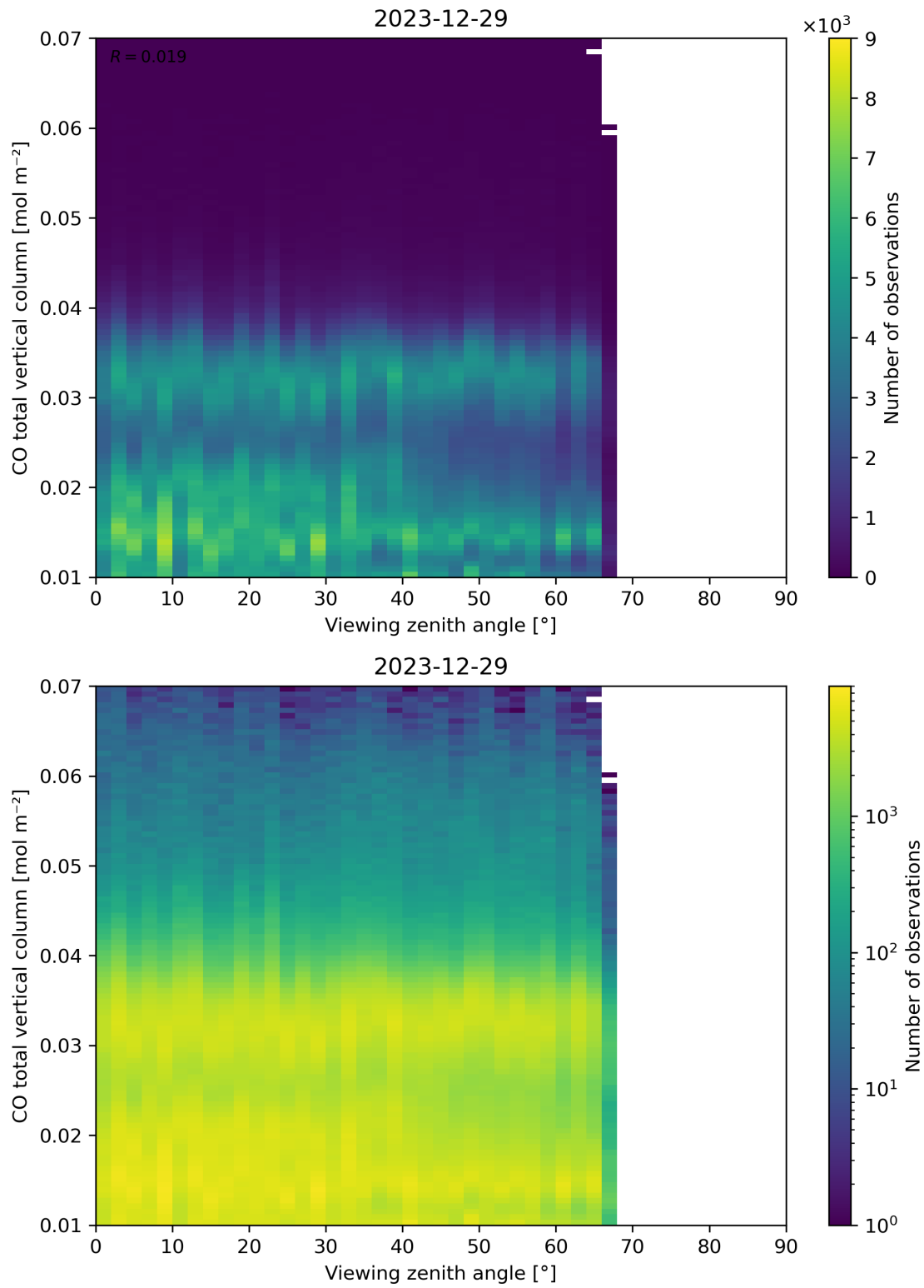
Figure 69: Scatter density plot of “Viewing zenith angle” against “CO total vertical column” for 2023-12-28 to 2023-12-30.
