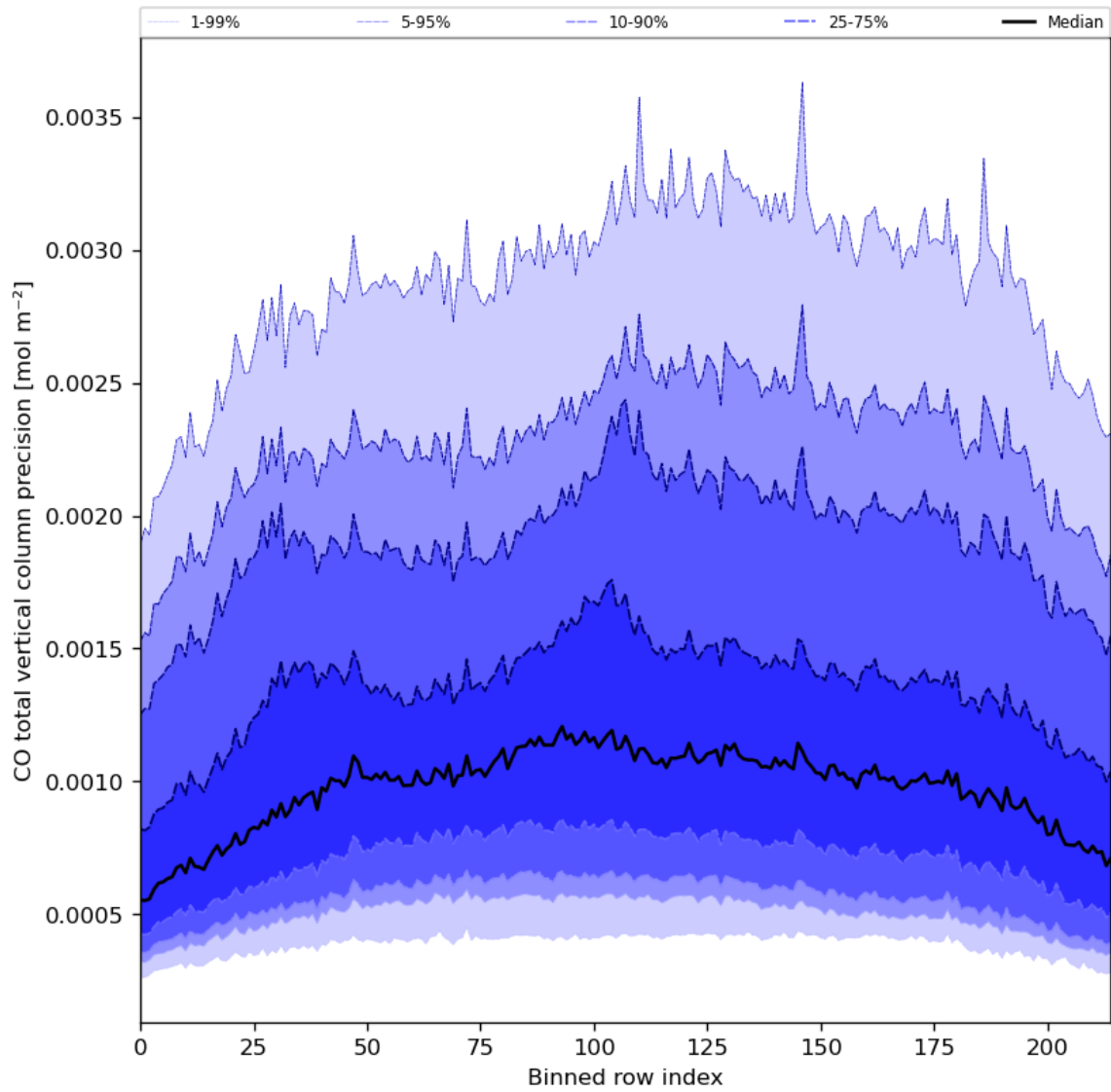
Figure 28: Along track statistics of “CO total vertical column precision” for 2023-12-28 to 2023-12-30
