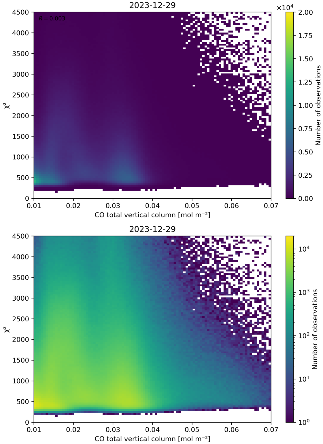
Figure 35: Scatter density plot of “CO total vertical column” against “ \chi^2 ” for 2023-12-28 to 2023-12-30.
