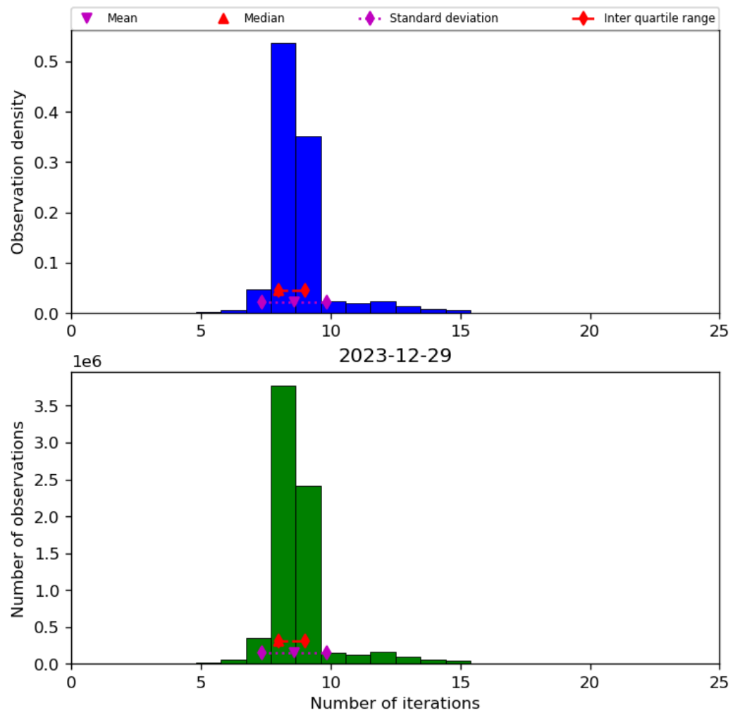
Figure 24: Histogram of “Number of iterations” for 2023-12-28 to 2023-12-30
