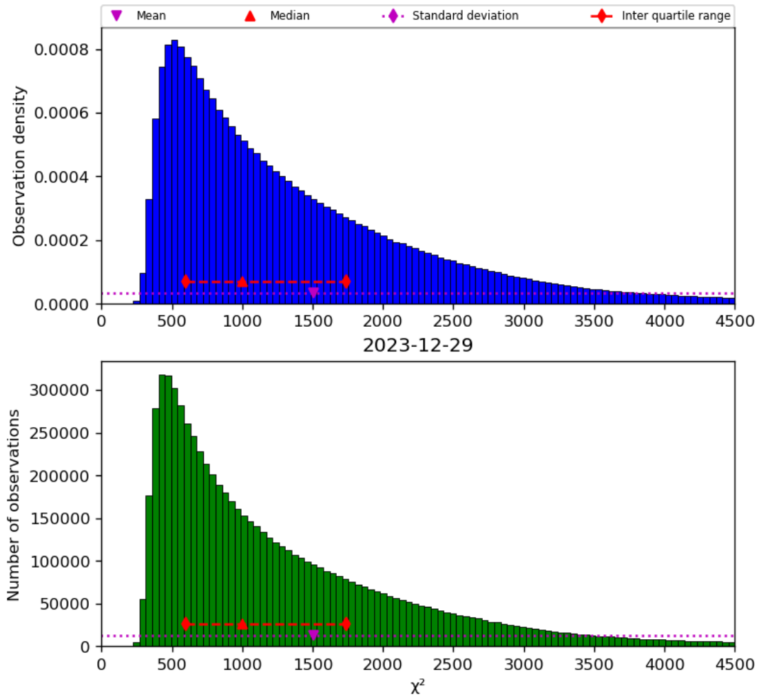
Figure 22: Histogram of “ \chi^2 ” for 2023-12-28 to 2023-12-30
