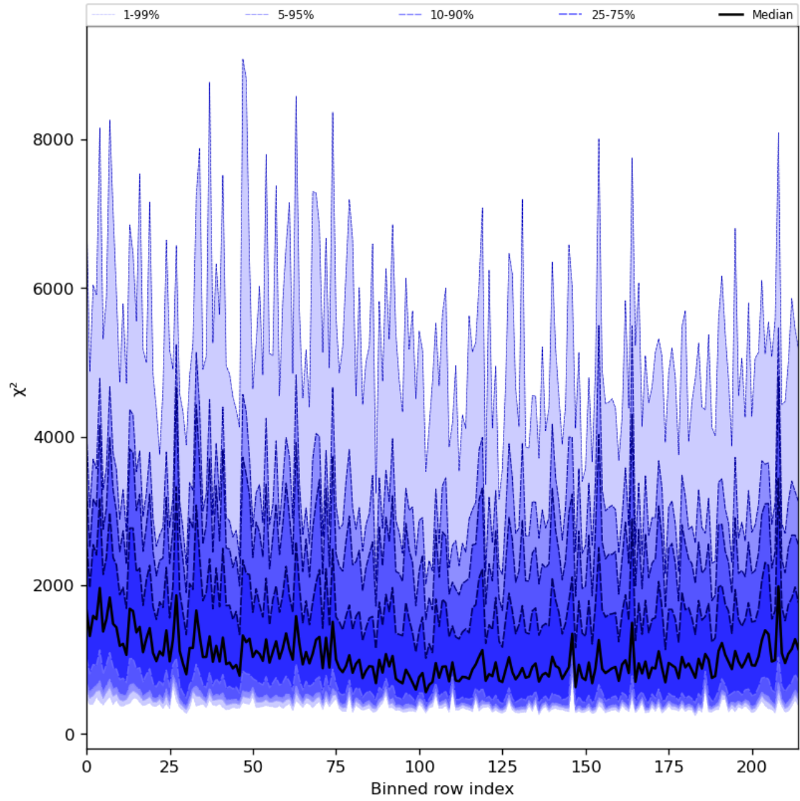
Figure 30: Along track statistics of “ \chi^2 ” for 2023-12-28 to 2023-12-30
