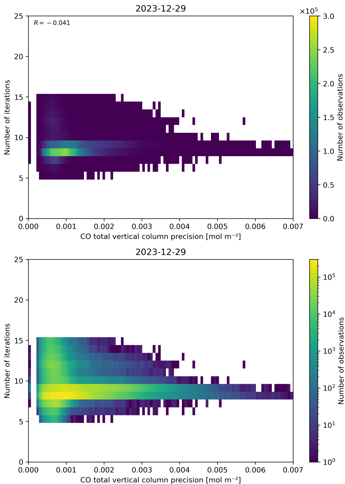
Figure 46: Scatter density plot of “CO total vertical column precision” against “Number of iterations” for 2023-12-28 to 2023-12-30.
