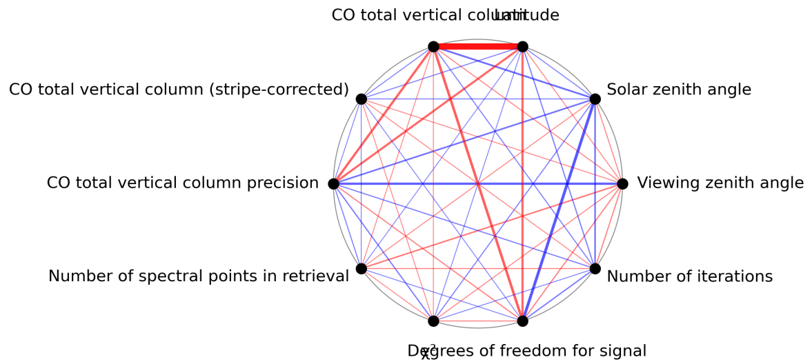
Figure 1: Map of correlation graph for 2023-12-28 to 2023-12-30.
