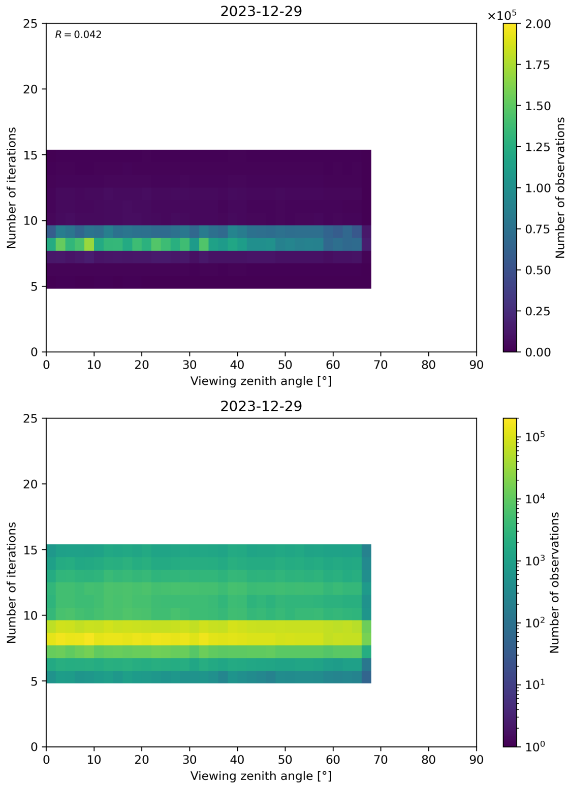
Figure 75: Scatter density plot of “Viewing zenith angle” against “Number of iterations” for 2023-12-28 to 2023-12-30.
