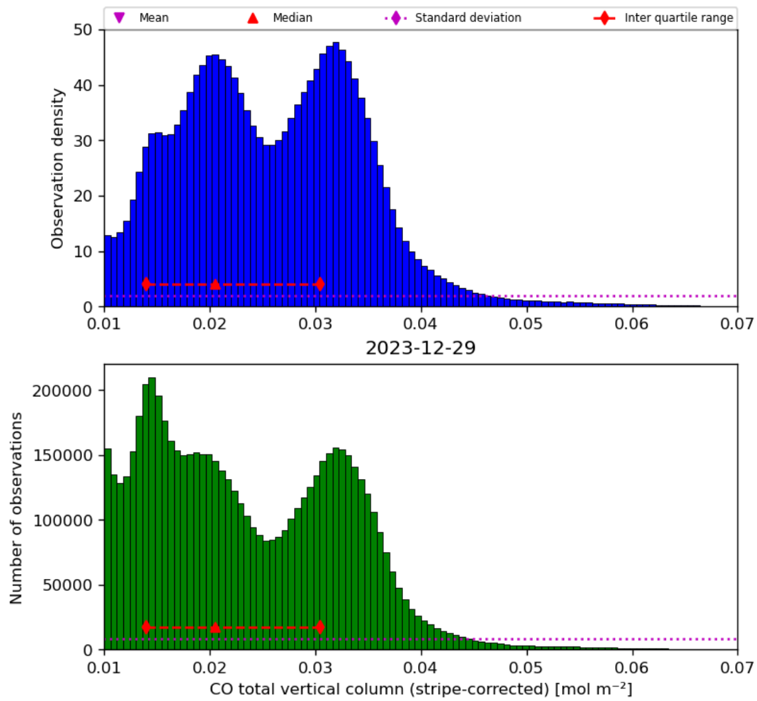
Figure 19: Histogram of “CO total vertical column (stripe-corrected)” for 2023-12-28 to 2023-12-30
