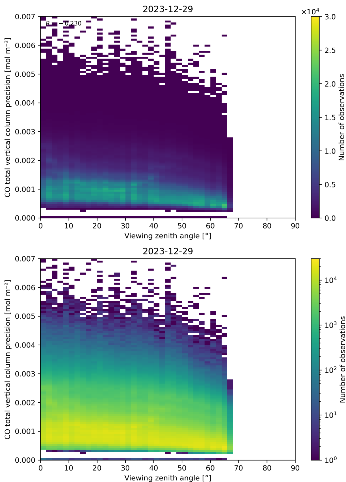
Figure 71: Scatter density plot of “Viewing zenith angle” against “CO total vertical column precision” for 2023-12-28 to 2023-12-30.
