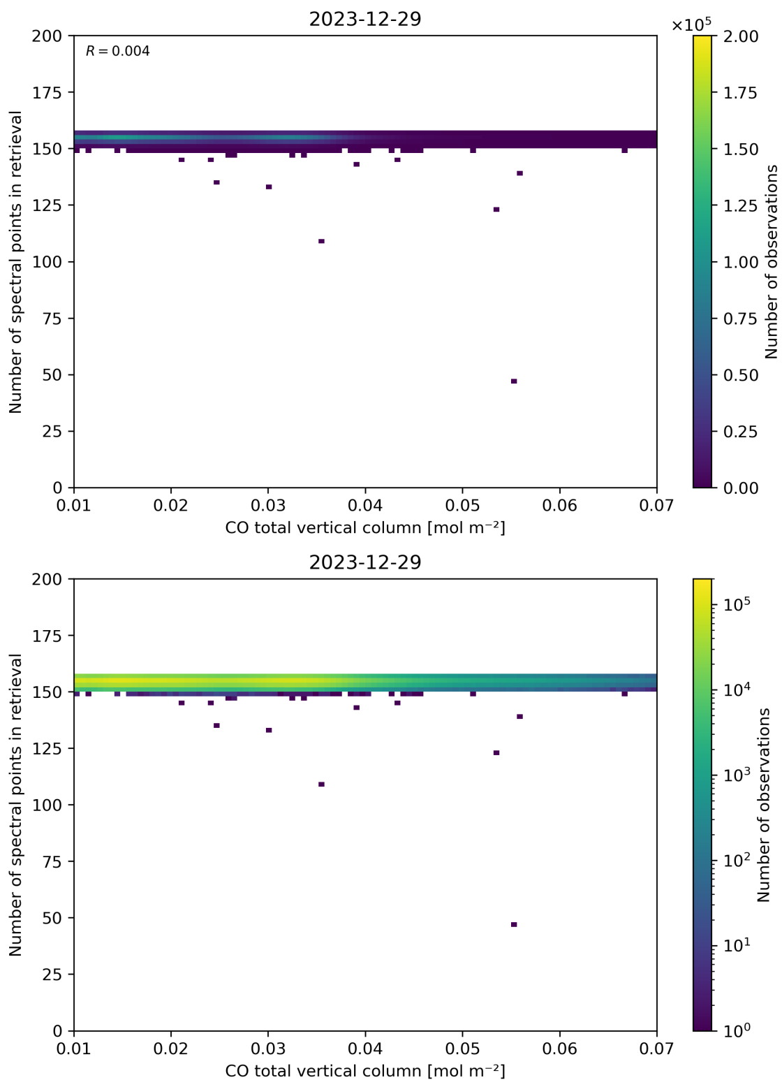
Figure 43: Scatter density plot of “CO total vertical column” against “Number of spectral points in retrieval” for 2023-12-28 to 2023-12-30.
