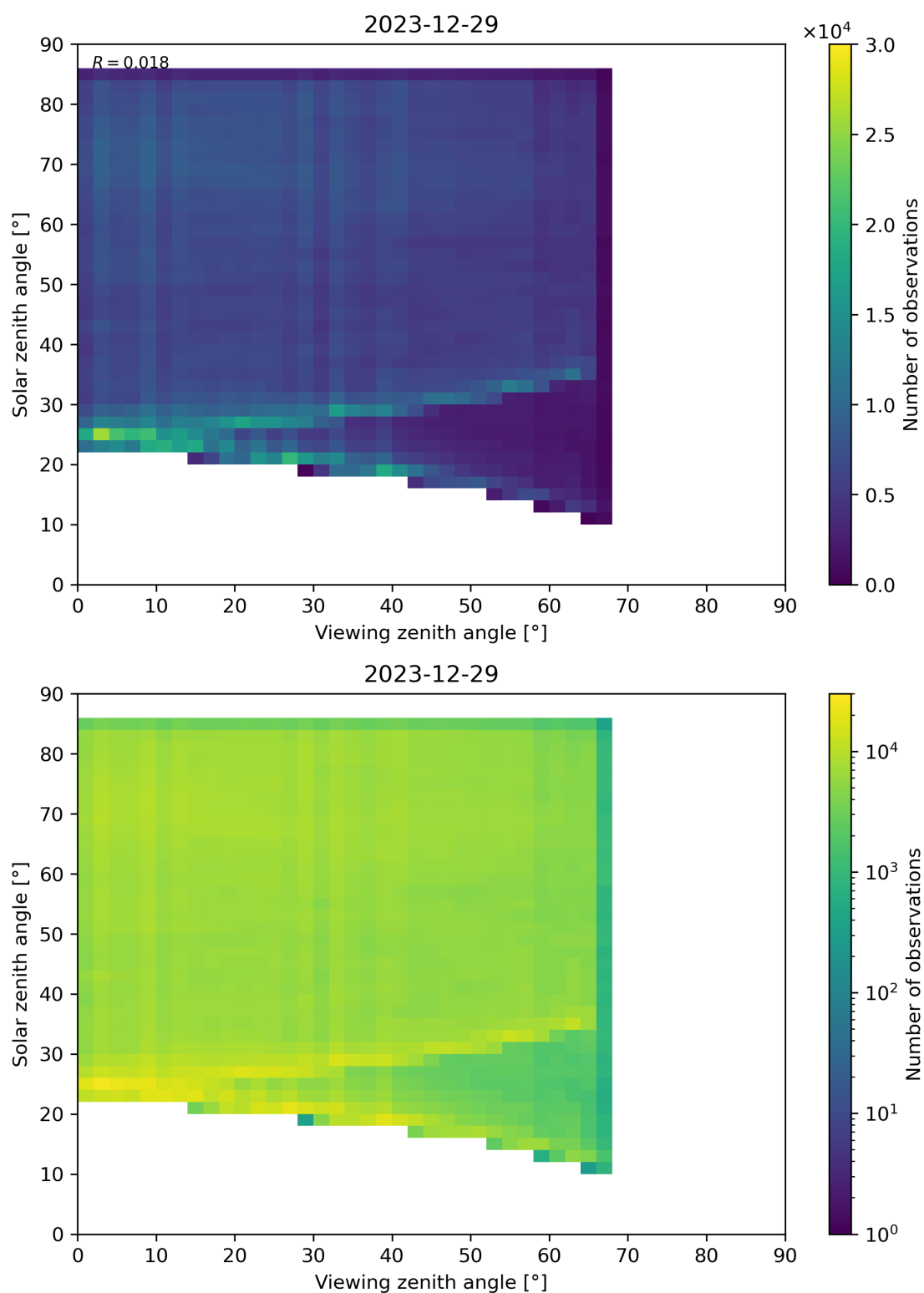
Figure 77: Scatter density plot of “Viewing zenith angle” against “Solar zenith angle” for 2023-12-28 to 2023-12-30.
