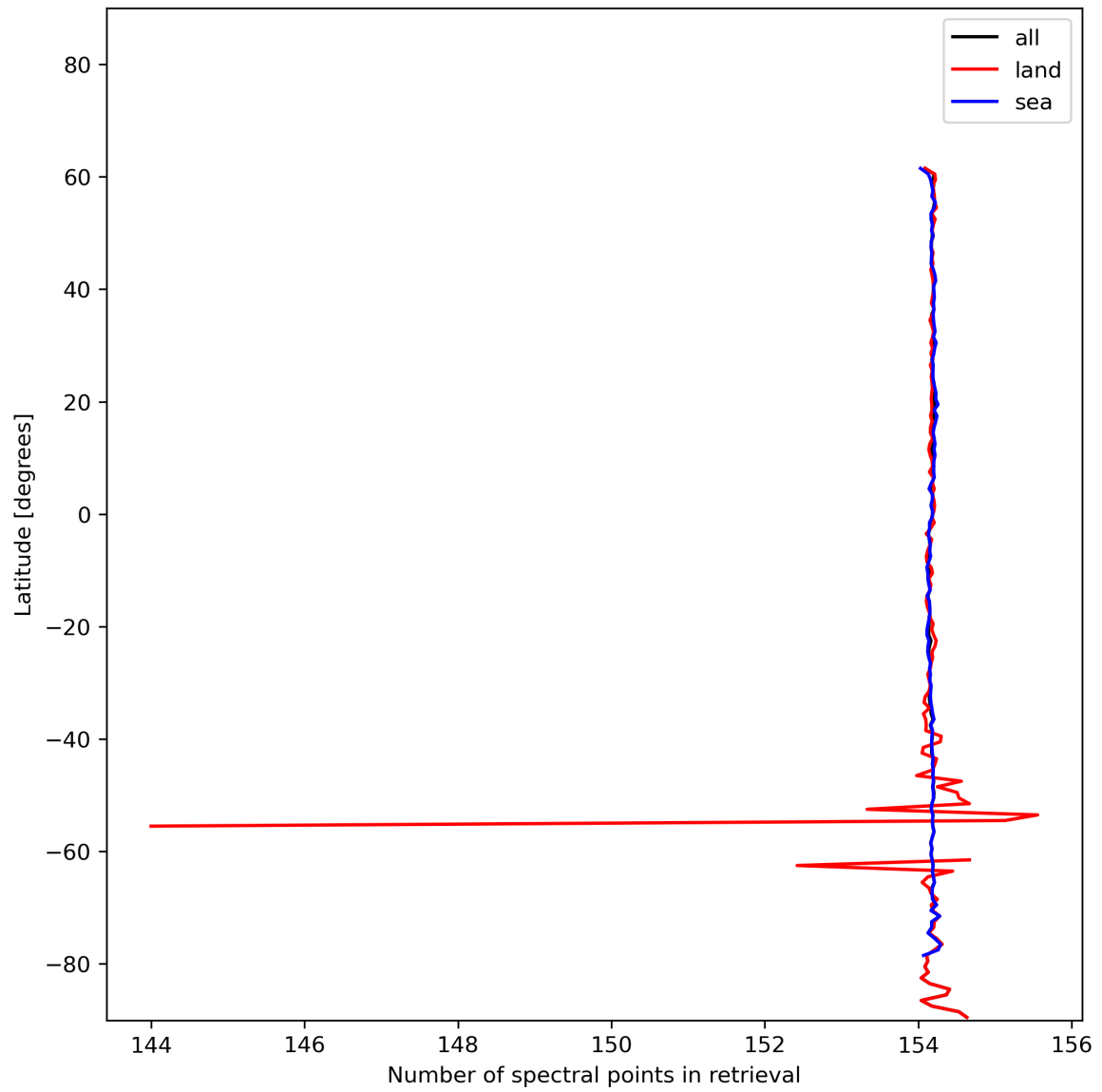
Figure 13: Zonal average of “Number of spectral points in retrieval” for 2023-12-28 to 2023-12-30.
