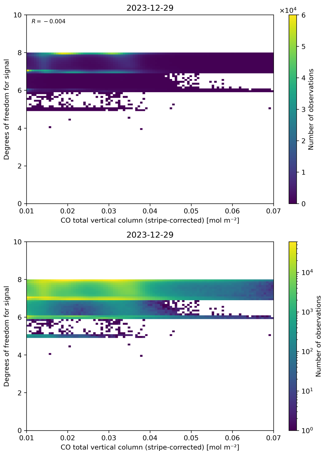
Figure 38: Scatter density plot of “CO total vertical column (stripe-corrected)” against “Degrees of freedom for signal” for 2023-12-28 to 2023-12-30.
