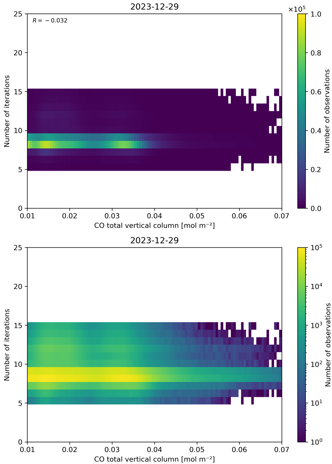
Figure 42: Scatter density plot of “CO total vertical column” against “Number of iterations” for 2023-12-28 to 2023-12-30.
