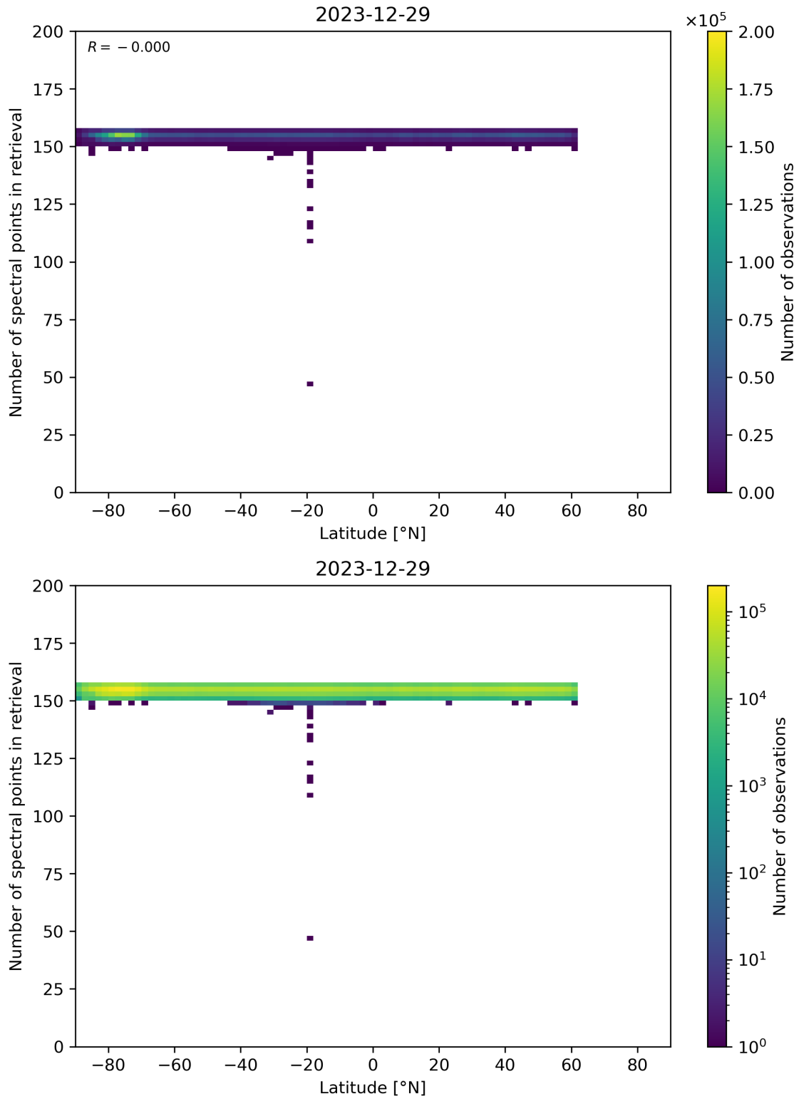
Figure 57: Scatter density plot of “Latitude” against “Number of spectral points in retrieval” for 2023-12-28 to 2023-12-30.
