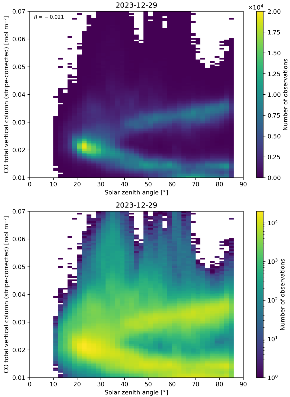
Figure 62: Scatter density plot of “Solar zenith angle” against “CO total vertical column (stripe-corrected)” for 2023-12-28 to 2023-12-30.
