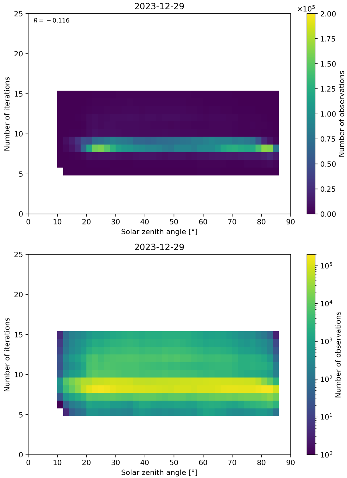
Figure 67: Scatter density plot of “Solar zenith angle” against “Number of iterations” for 2023-12-28 to 2023-12-30.
