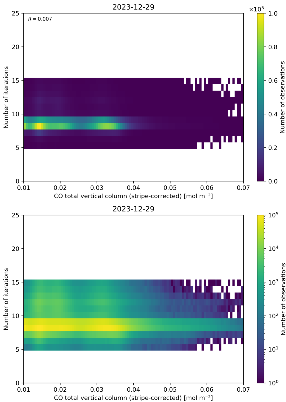
Figure 39: Scatter density plot of “CO total vertical column (stripe-corrected)” against “Number of iterations” for 2023-12-28 to 2023-12-30.
