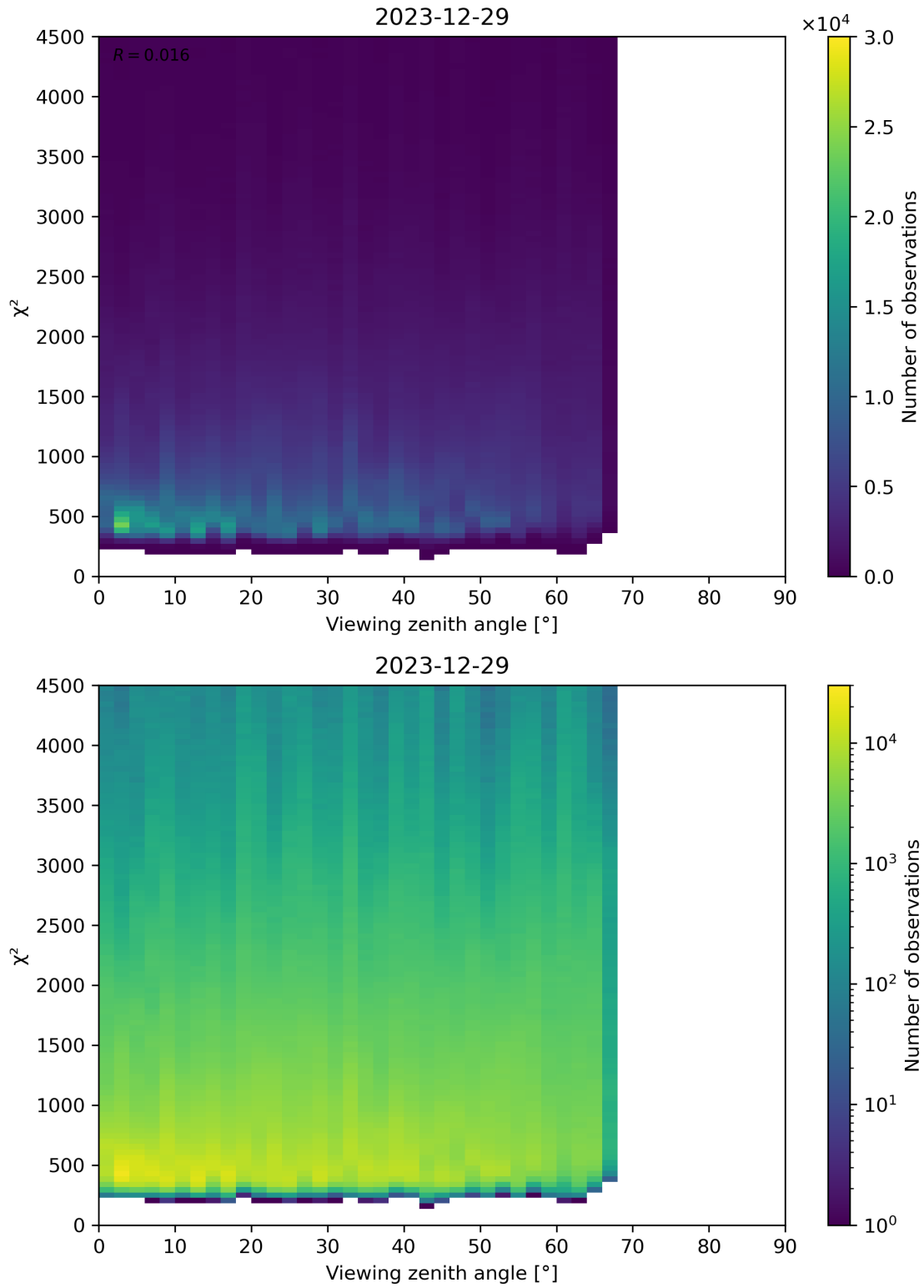
Figure 72: Scatter density plot of “Viewing zenith angle” against “ \chi^2 ” for 2023-12-28 to 2023-12-30.
