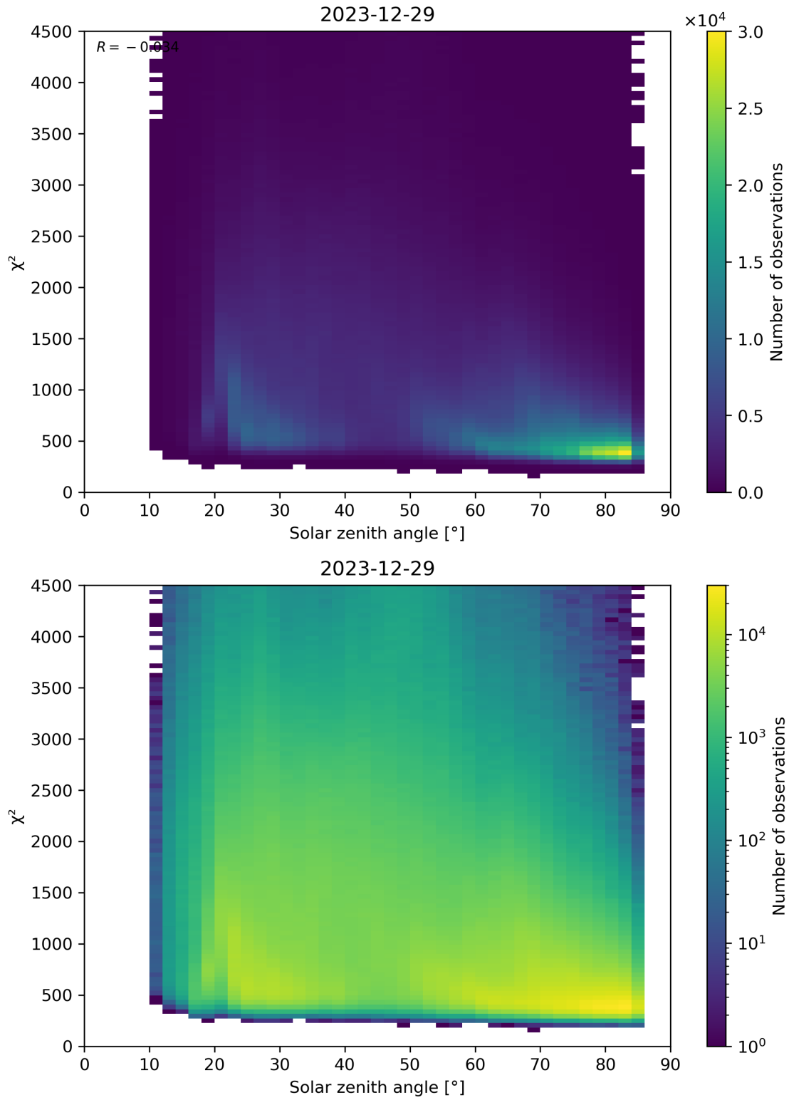
Figure 64: Scatter density plot of “Solar zenith angle” against “ \chi^2 ” for 2023-12-28 to 2023-12-30.
