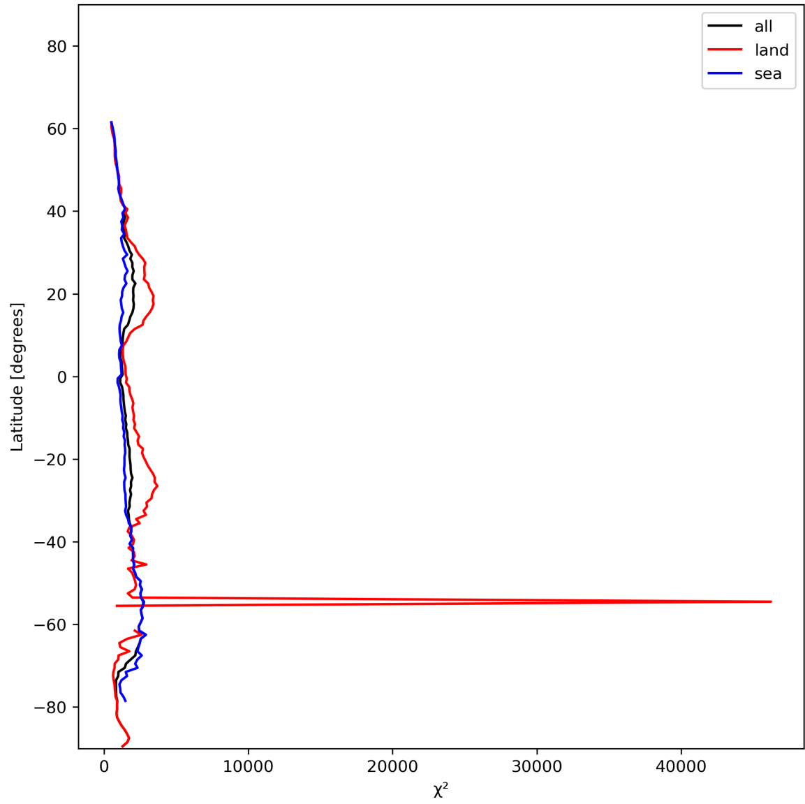
Figure 14: Zonal average of “ \chi^2 ” for 2023-12-28 to 2023-12-30.
