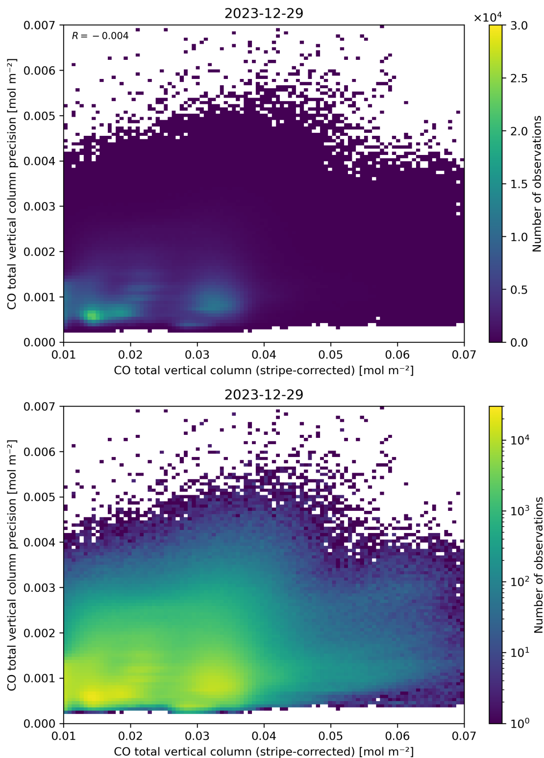
Figure 36: Scatter density plot of “CO total vertical column (stripe-corrected)” against “CO total vertical column precision” for 2023-12-28 to 2023-12-30.
