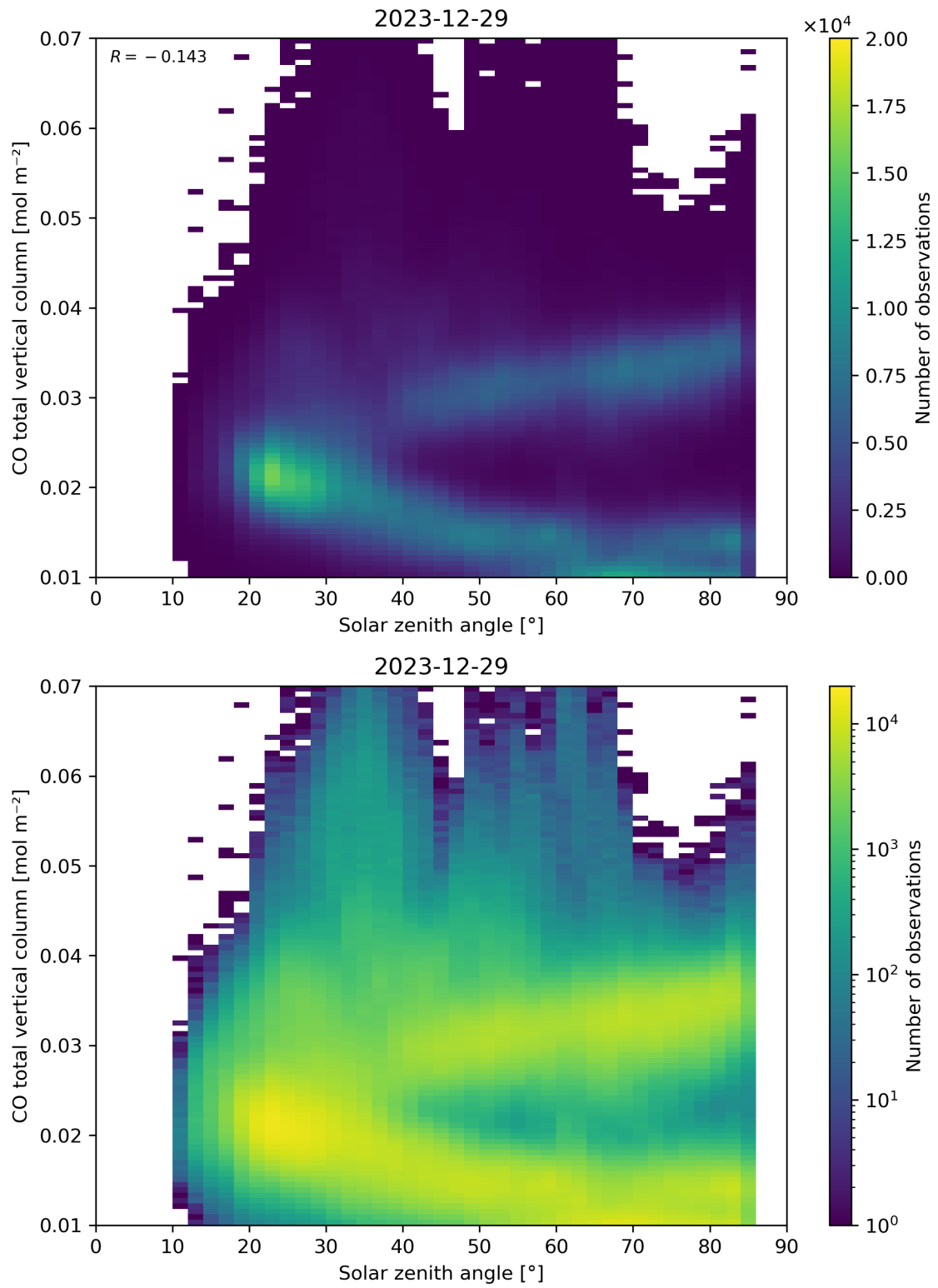
Figure 61: Scatter density plot of “Solar zenith angle” against “CO total vertical column” for 2023-12-28 to 2023-12-30.
