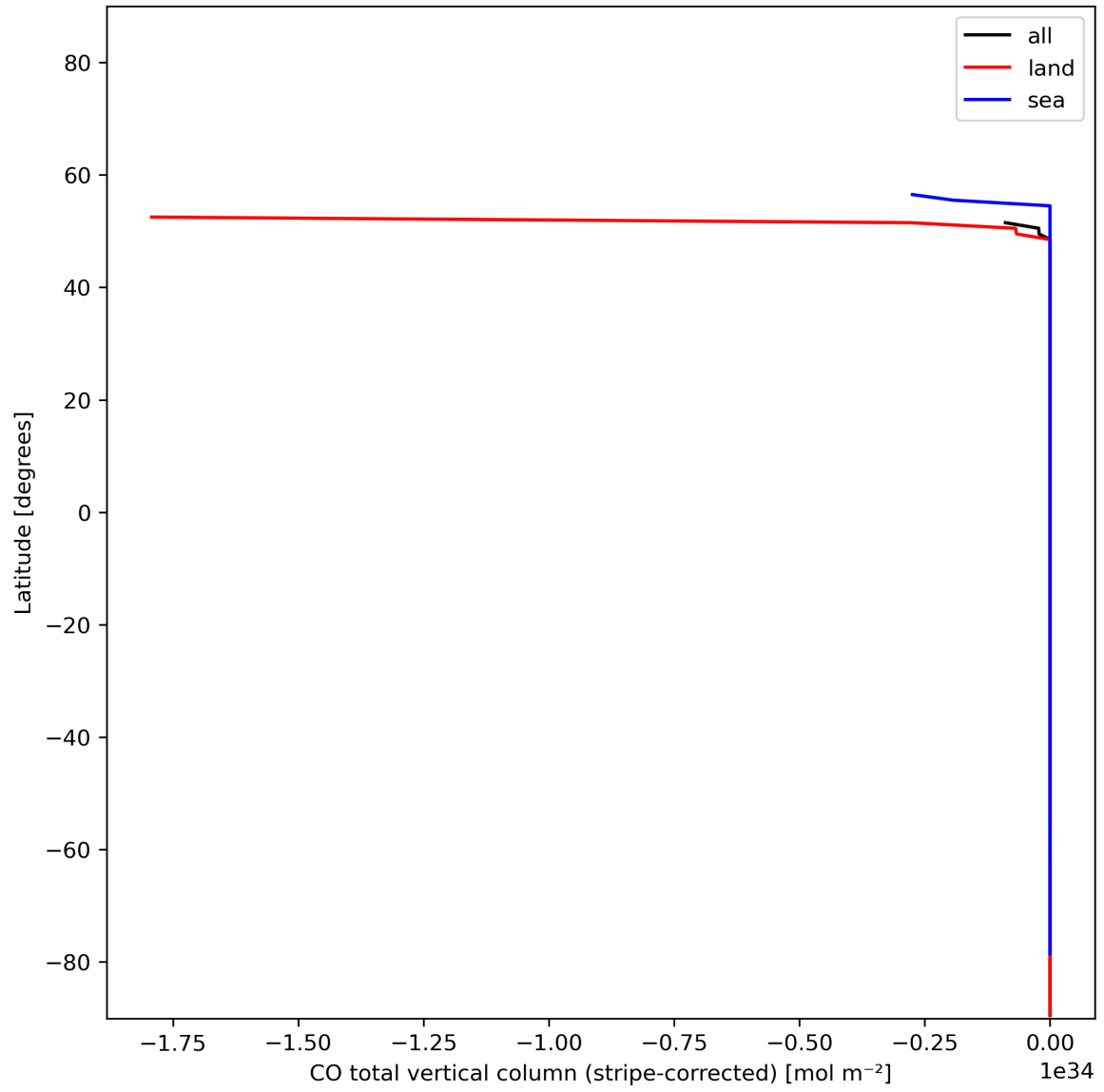
Figure 11: Zonal average of “CO total vertical column (stripe-corrected)” for 2023-12-28 to 2023-12-30.
