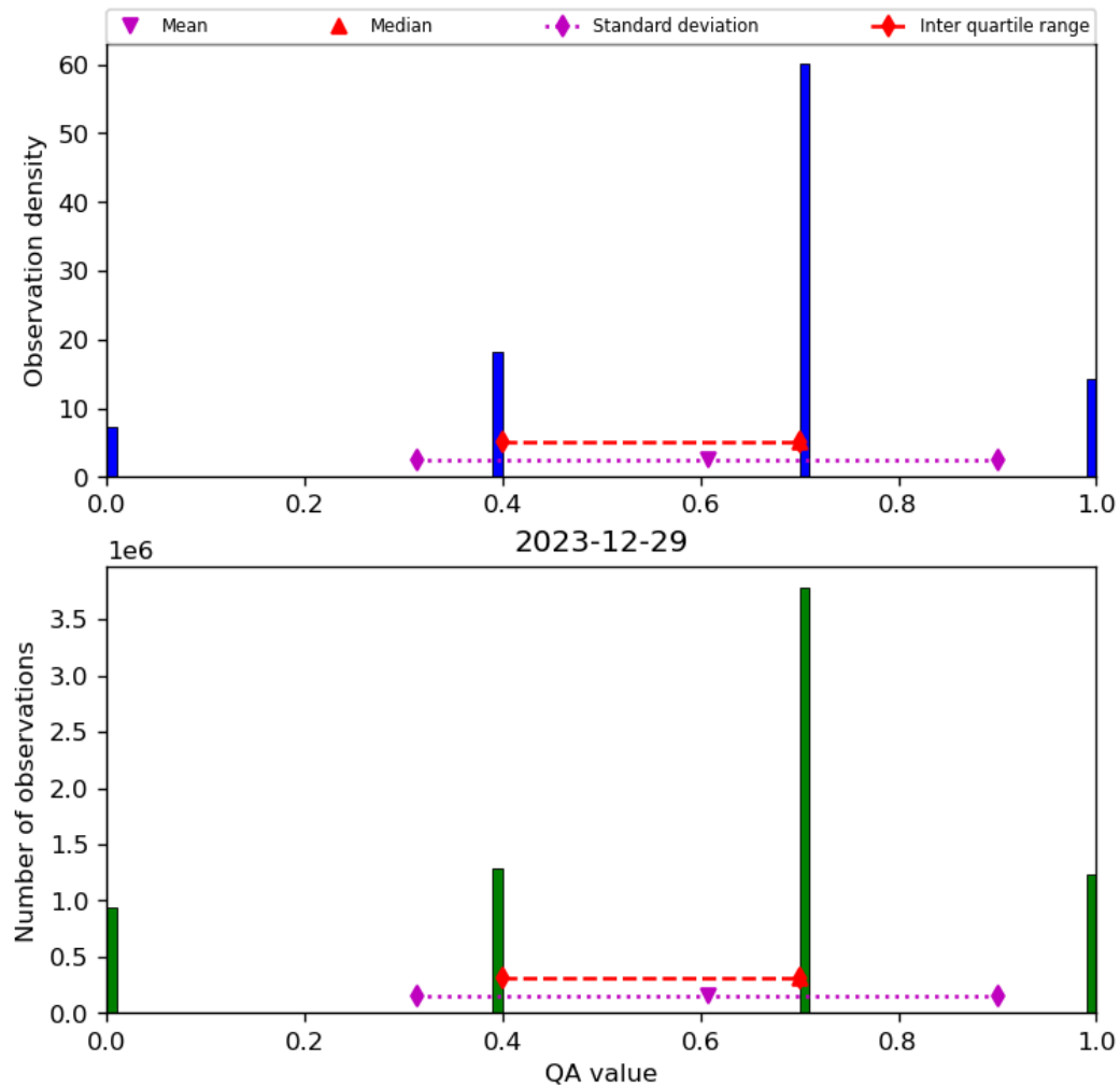
Figure 17: Histogram of “QA value” for 2023-12-28 to 2023-12-30
