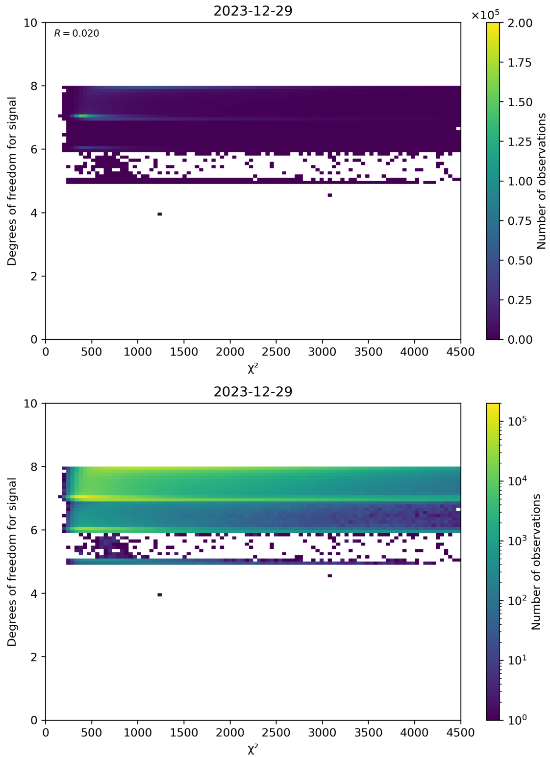
Figure 48: Scatter density plot of “ \chi^2 ” against “Degrees of freedom for signal” for 2023-12-28 to 2023-12-30.
