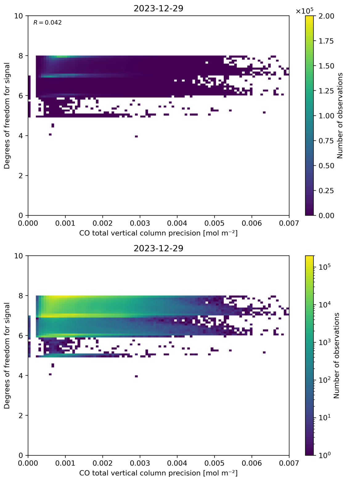
Figure 45: Scatter density plot of “CO total vertical column precision” against “Degrees of freedom for signal” for 2023-12-28 to 2023-12-30.
