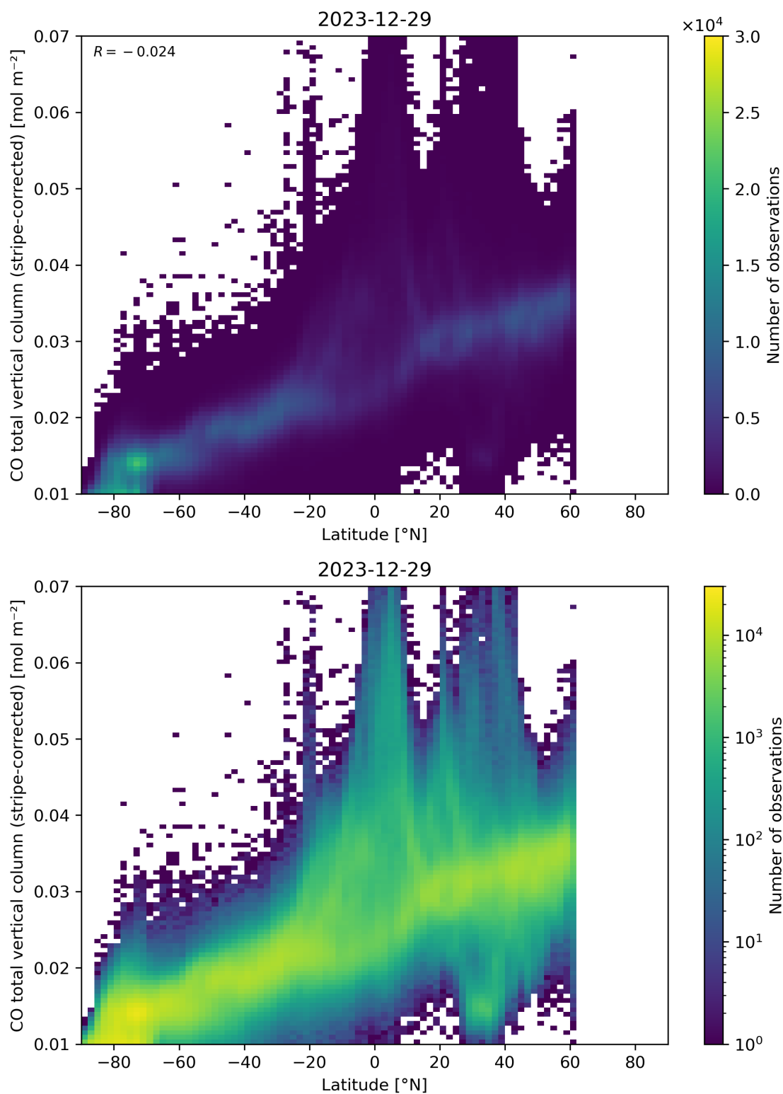
Figure 52: Scatter density plot of “Latitude” against “CO total vertical column (stripe-corrected)” for 2023-12-28 to 2023-12-30.
