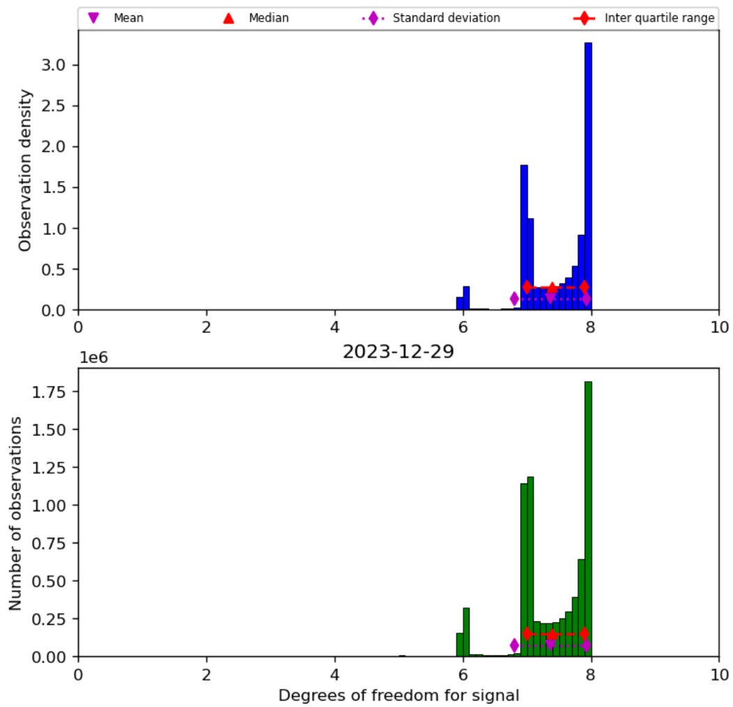
Figure 23: Histogram of “Degrees of freedom for signal” for 2023-12-28 to 2023-12-30
