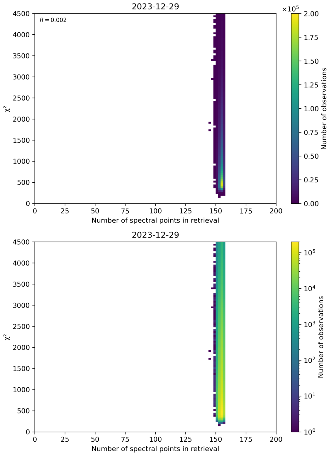
Figure 58: Scatter density plot of “Number of spectral points in retrieval” against “ \chi^2 ” for 2023-12-28 to 2023-12-30.
