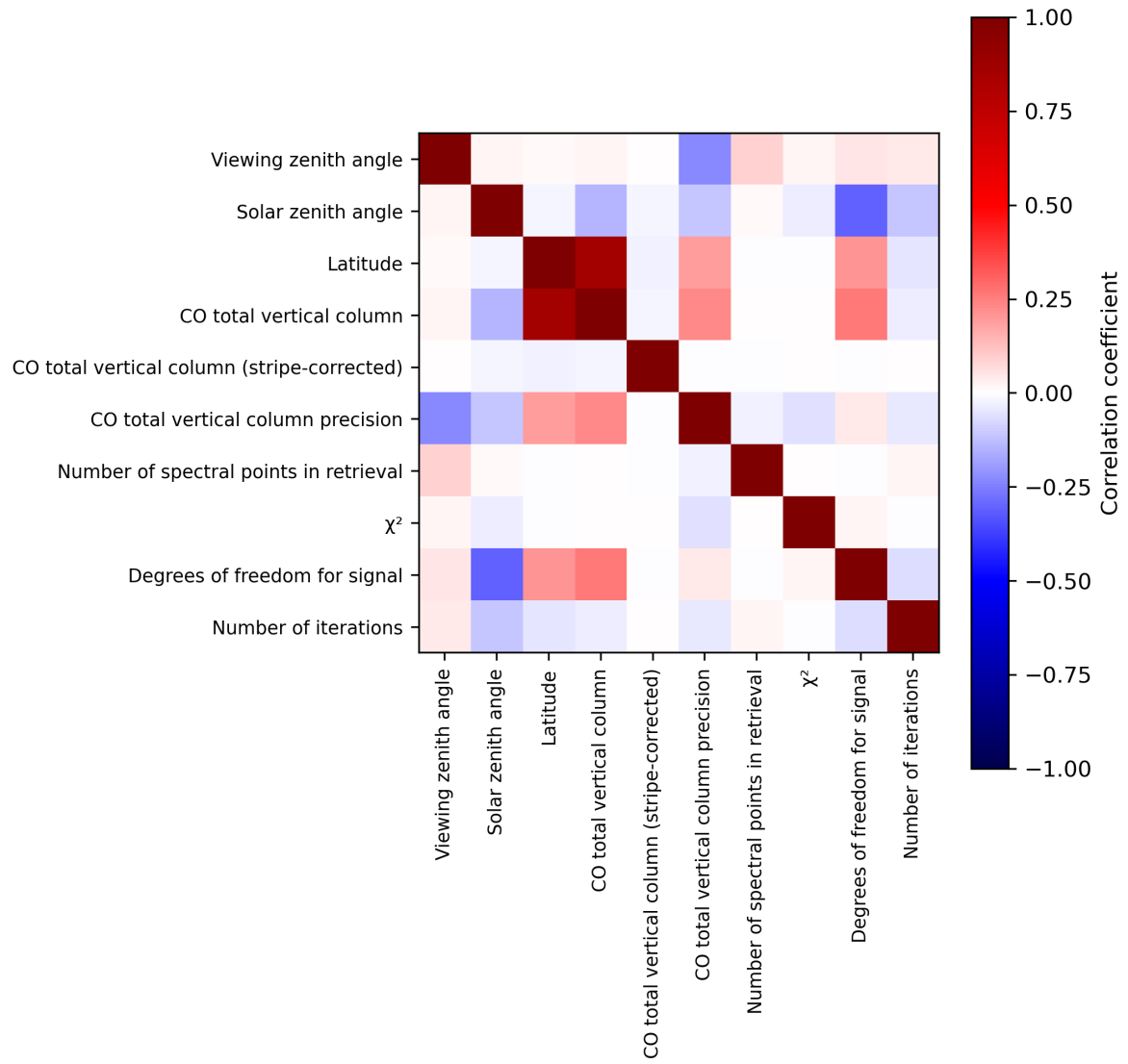
Figure 2: Map of correlation matrix for 2023-12-28 to 2023-12-30.
