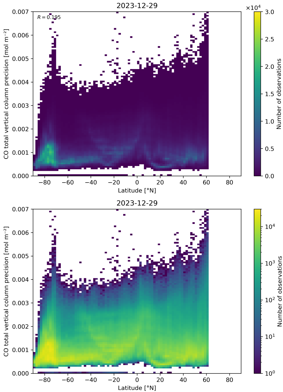
Figure 53: Scatter density plot of “Latitude” against “CO total vertical column precision” for 2023-12-28 to 2023-12-30.
