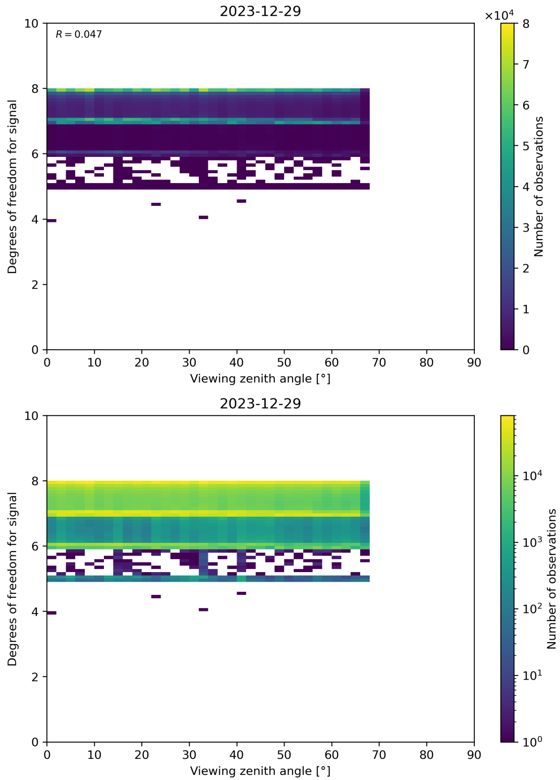
Figure 73: Scatter density plot of “Viewing zenith angle” against “Degrees of freedom for signal” for 2023-12-28 to 2023-12-30.
