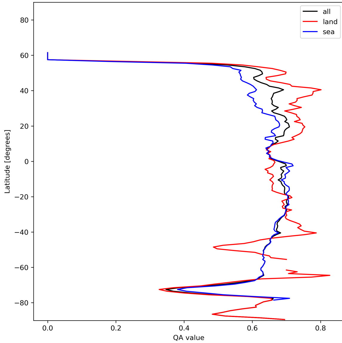
Figure 9: Zonal average of “QA value” for 2023-12-28 to 2023-12-30.
