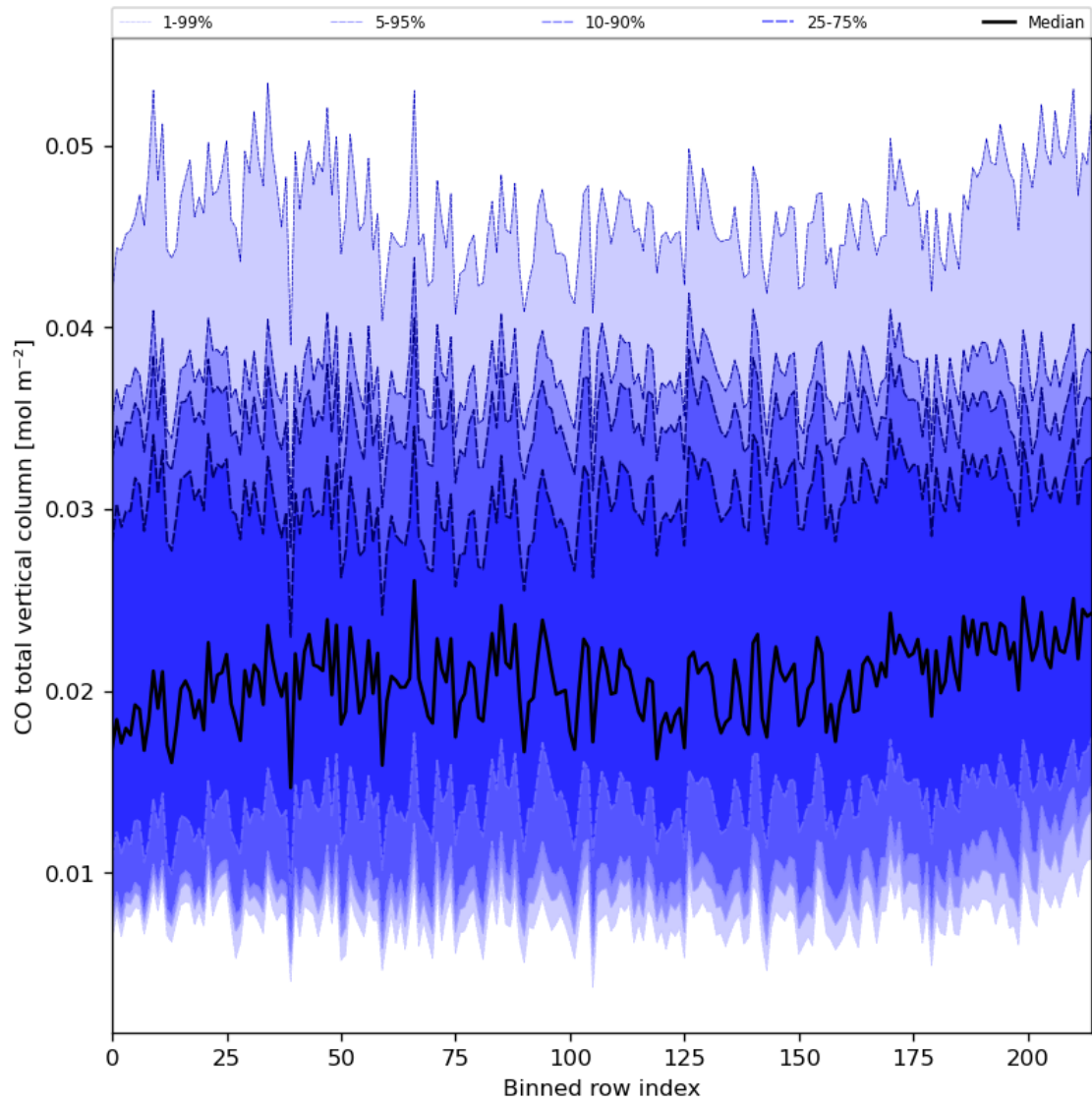
Figure 26: Along track statistics of “CO total vertical column” for 2023-12-28 to 2023-12-30
