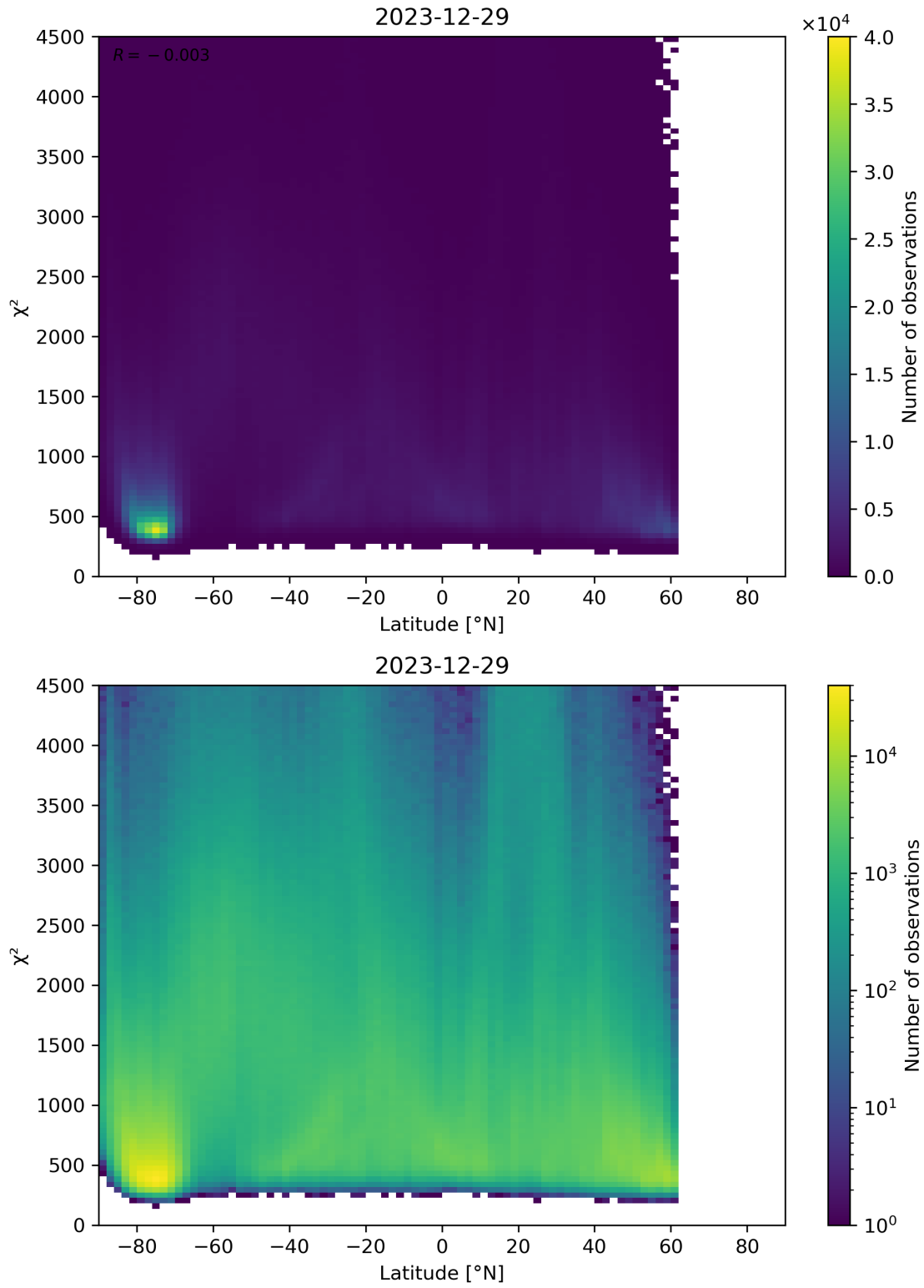
Figure 54: Scatter density plot of “Latitude” against “ \chi^2 ” for 2023-12-28 to 2023-12-30.
