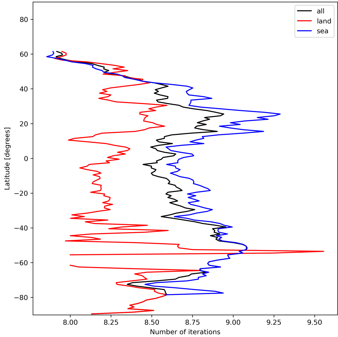
Figure 16: Zonal average of “Number of iterations” for 2023-12-28 to 2023-12-30.
