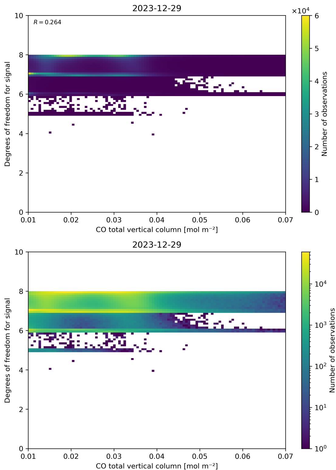
Figure 41: Scatter density plot of “CO total vertical column” against “Degrees of freedom for signal” for 2023-12-28 to 2023-12-30.
