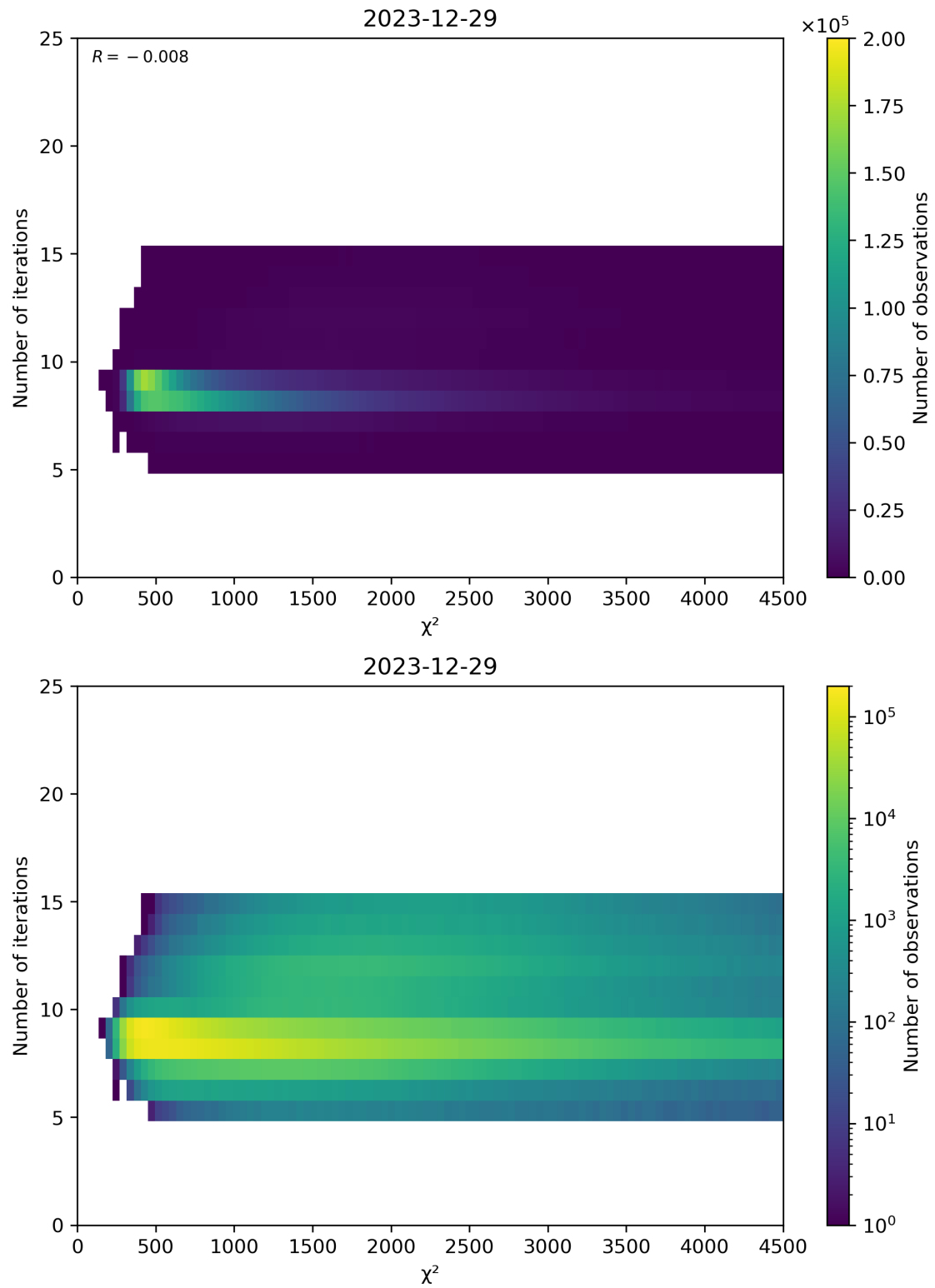
Figure 49: Scatter density plot of “ \chi^2 ” against “Number of iterations” for 2023-12-28 to 2023-12-30.
