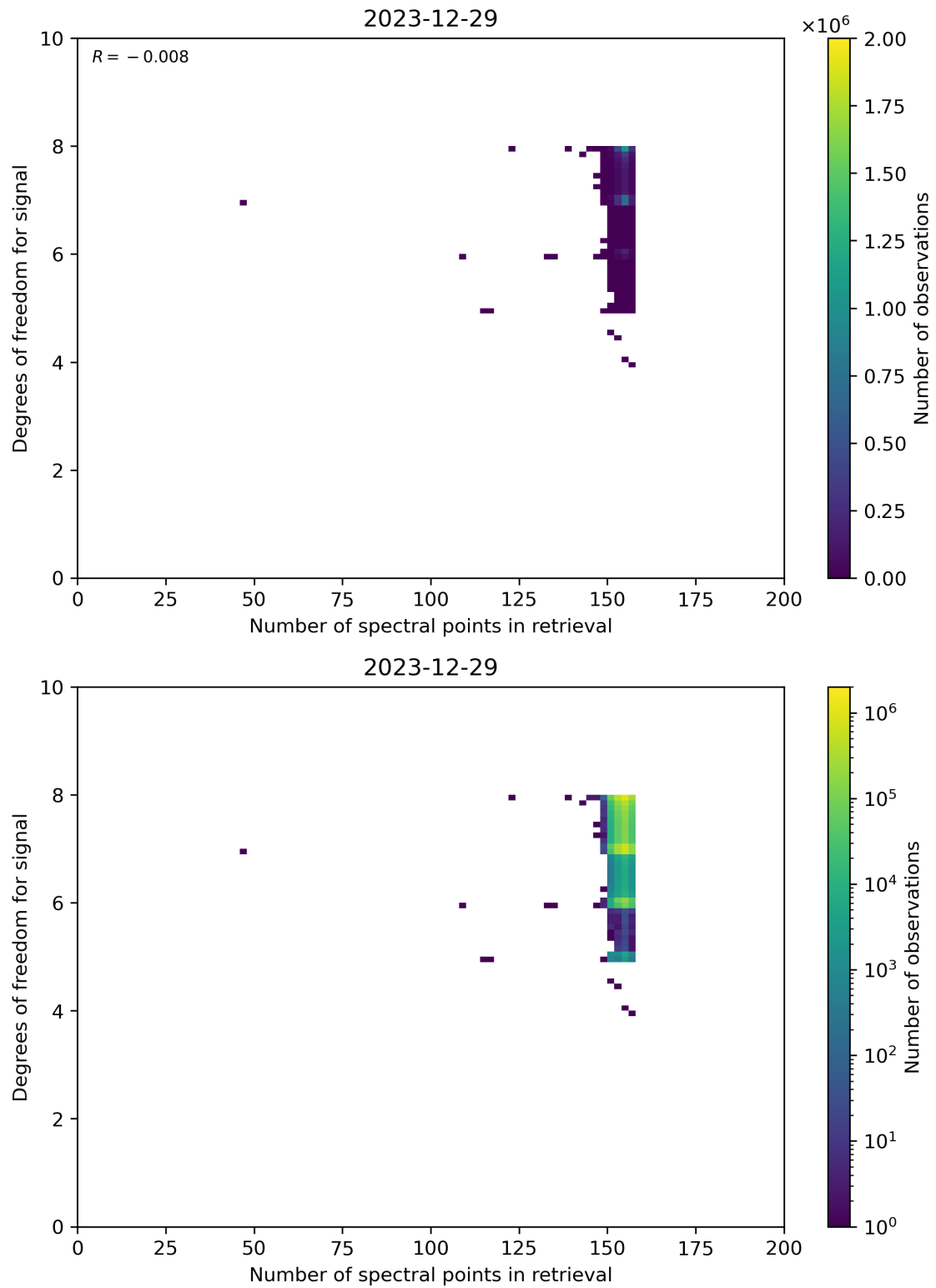
Figure 59: Scatter density plot of “Number of spectral points in retrieval” against “Degrees of freedom for signal” for 2023-12-28 to 2023-12-30.
