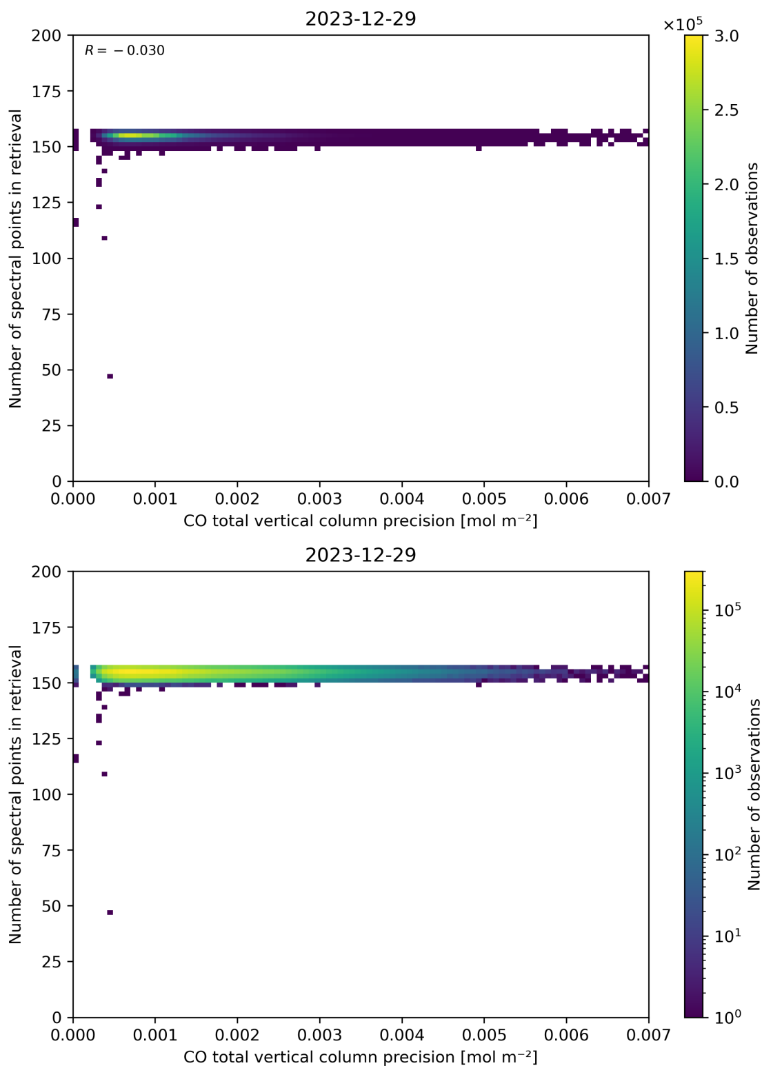
Figure 47: Scatter density plot of “CO total vertical column precision” against “Number of spectral points in retrieval” for 2023-12-28 to 2023-12-30.
