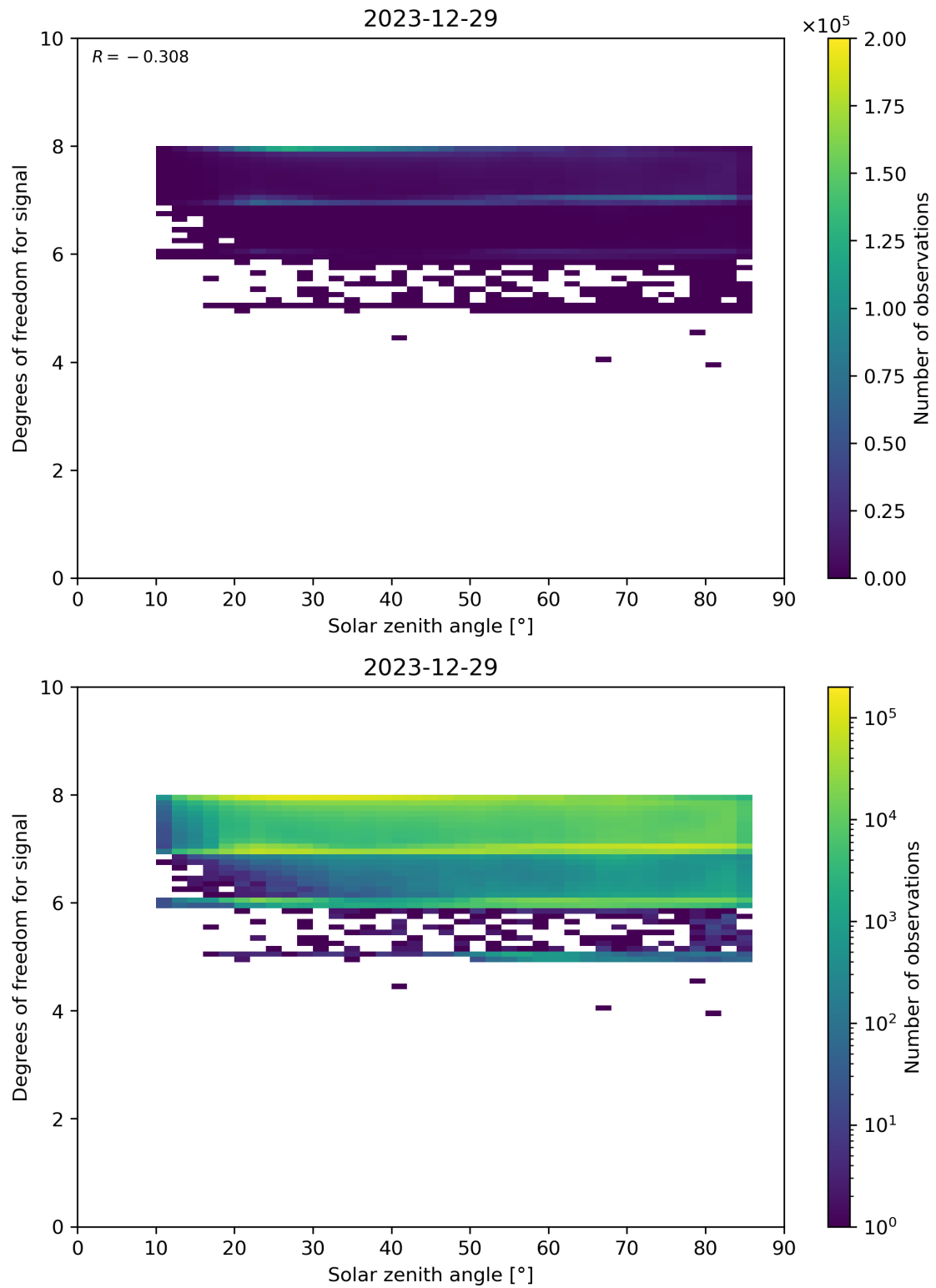
Figure 65: Scatter density plot of “Solar zenith angle” against “Degrees of freedom for signal” for 2023-12-28 to 2023-12-30.
