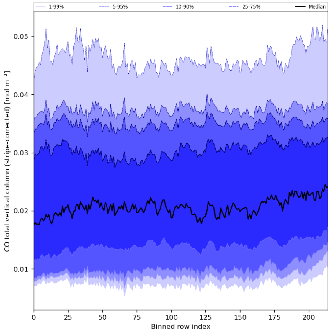
Figure 27: Along track statistics of “CO total vertical column (stripe-corrected)” for 2023-12-28 to 2023-12-30
