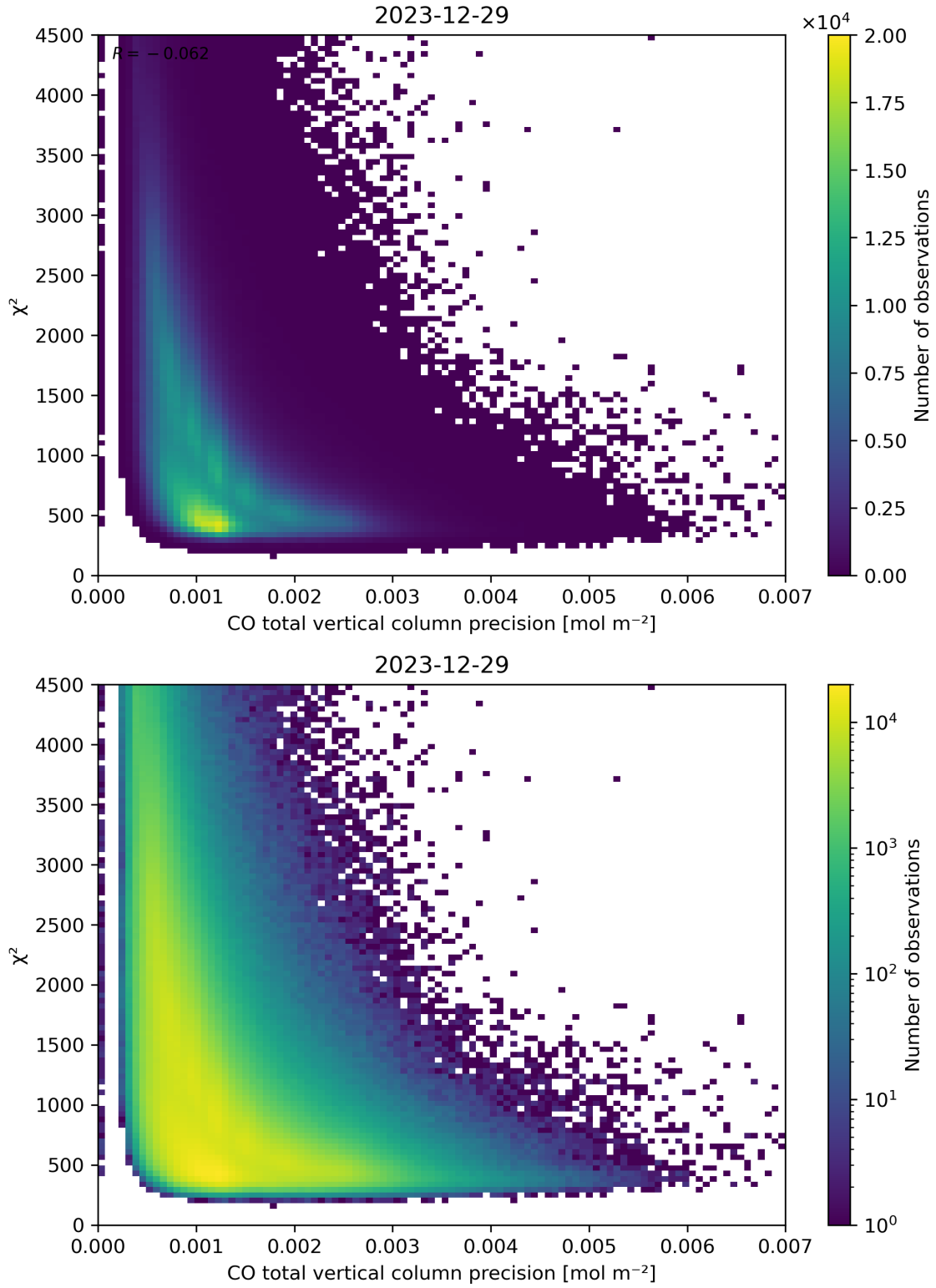
Figure 44: Scatter density plot of “CO total vertical column precision” against “ \chi^2 ” for 2023-12-28 to 2023-12-30.
