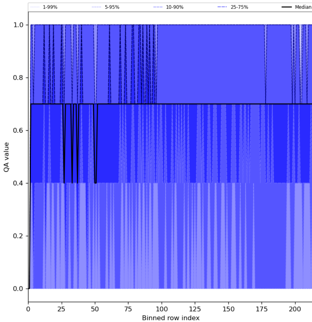
Figure 25: Along track statistics of “QA value” for 2023-12-28 to 2023-12-30
