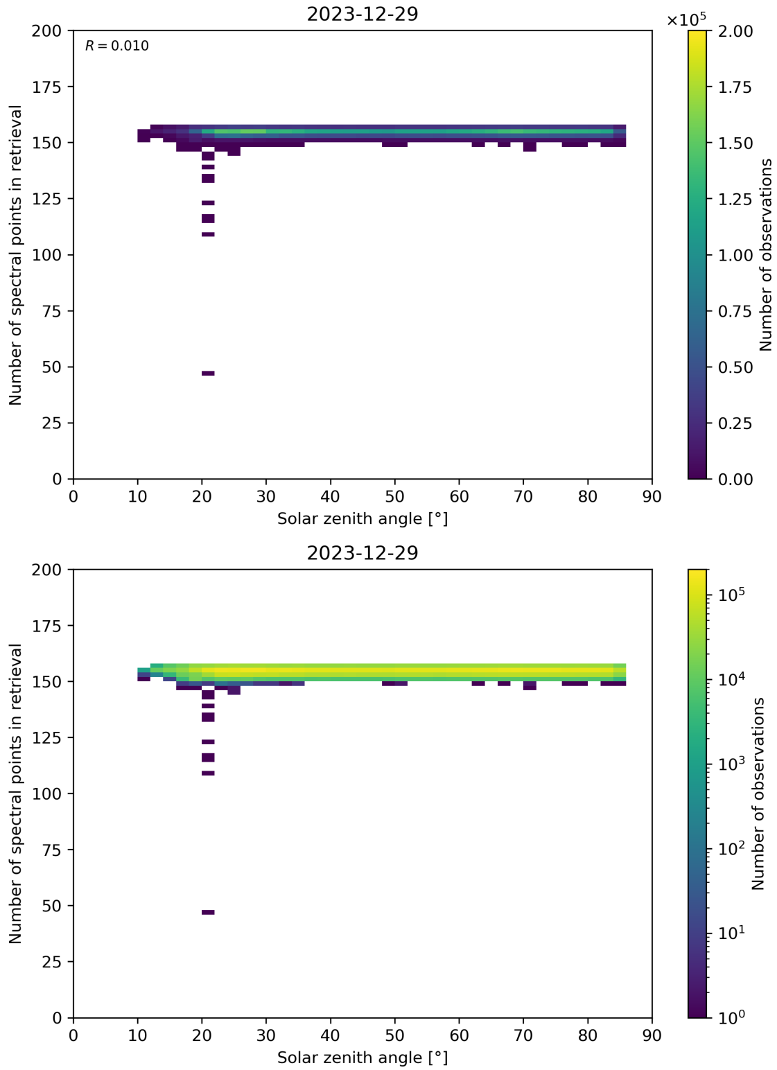
Figure 68: Scatter density plot of “Solar zenith angle” against “Number of spectral points in retrieval” for 2023-12-28 to 2023-12-30.
