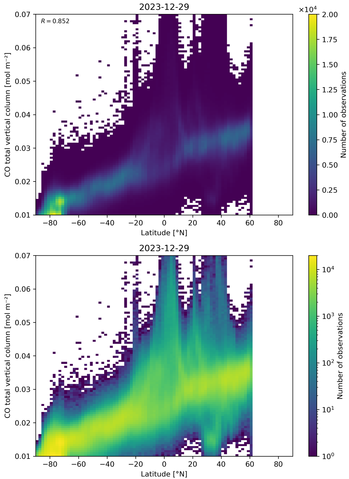
Figure 51: Scatter density plot of “Latitude” against “CO total vertical column” for 2023-12-28 to 2023-12-30.
