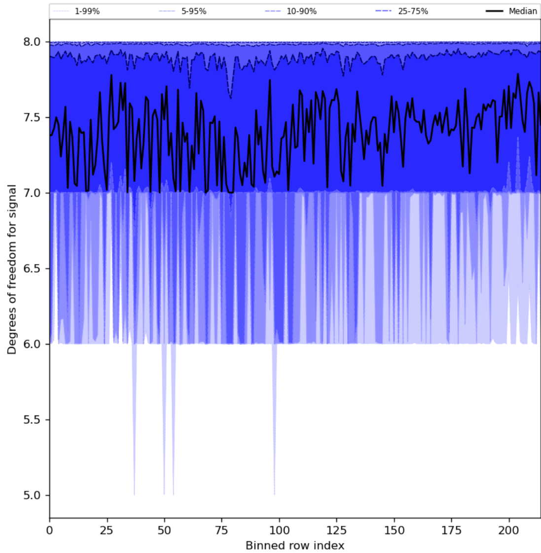
Figure 31: Along track statistics of “Degrees of freedom for signal” for 2023-12-28 to 2023-12-30
