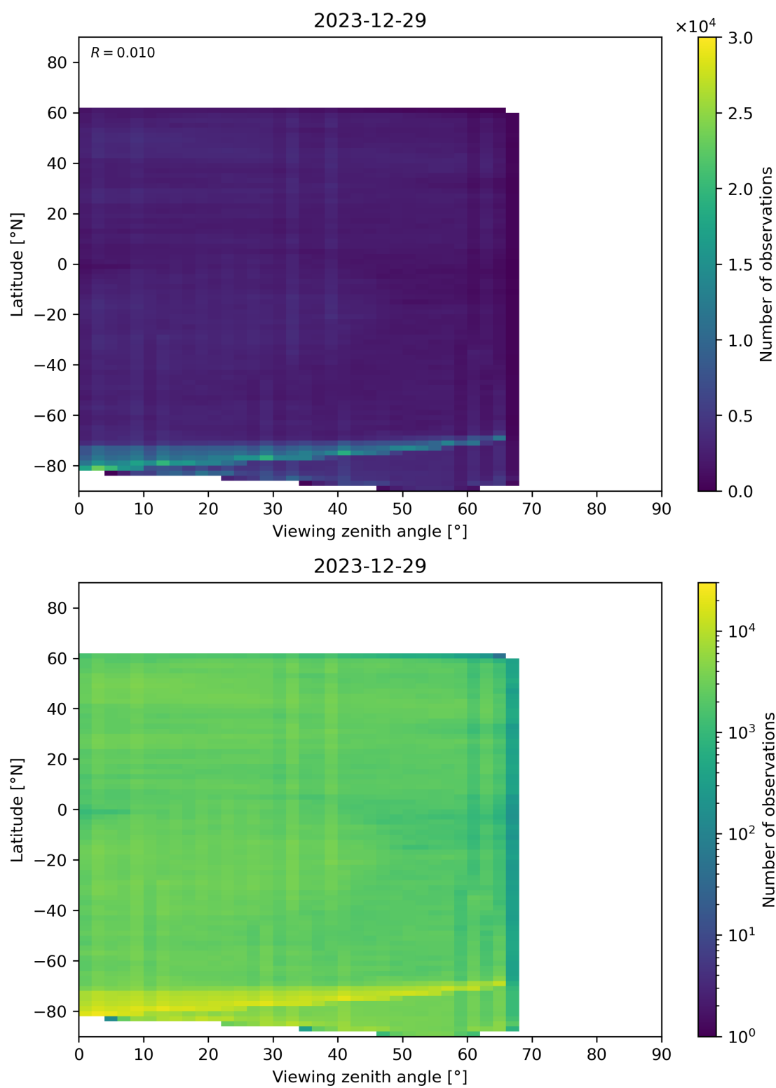
Figure 74: Scatter density plot of “Viewing zenith angle” against “Latitude” for 2023-12-28 to 2023-12-30.
