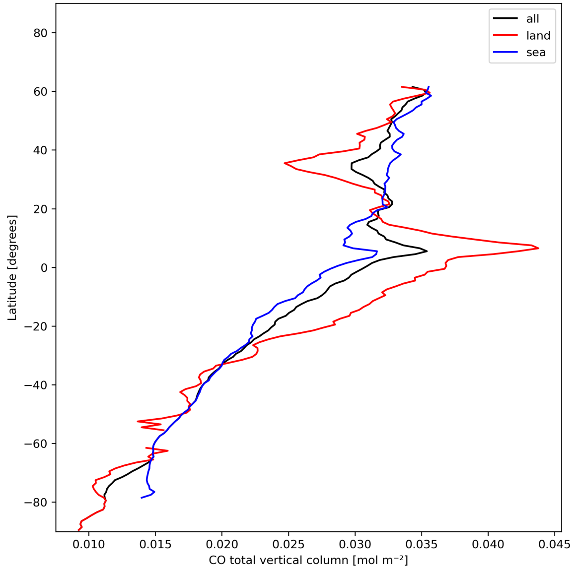
Figure 10: Zonal average of “CO total vertical column” for 2023-12-28 to 2023-12-30.
