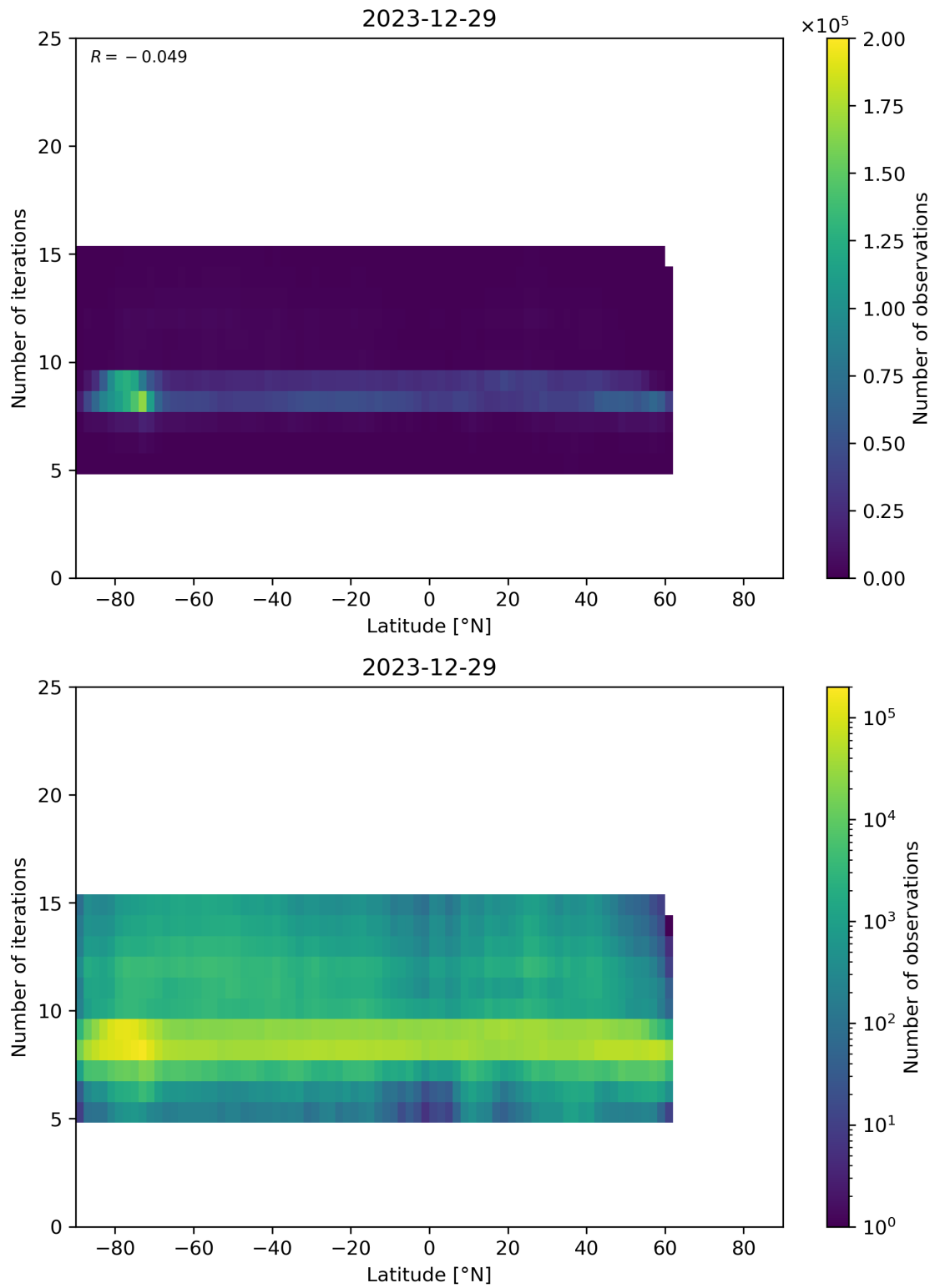
Figure 56: Scatter density plot of “Latitude” against “Number of iterations” for 2023-12-28 to 2023-12-30.
