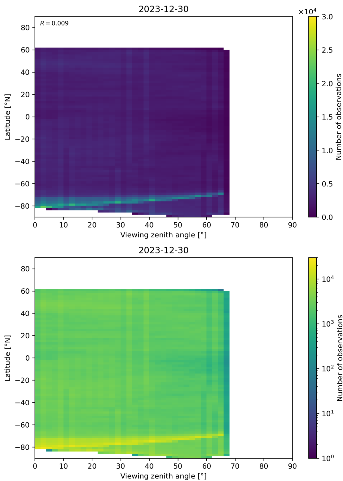
Figure 74: Scatter density plot of “Viewing zenith angle” against “Latitude” for 2023-12-30 to 2023-12-31.
