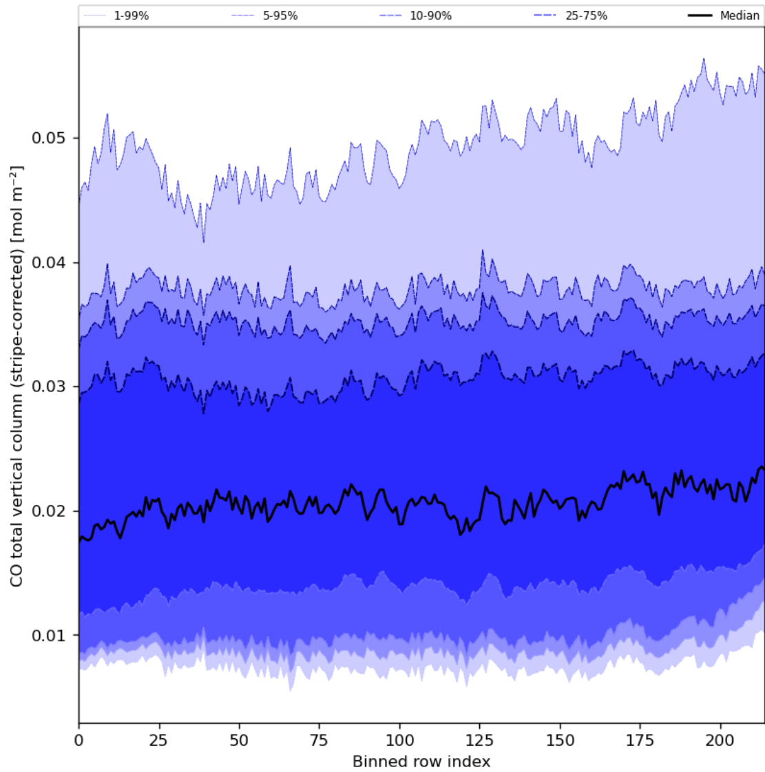
Figure 27: Along track statistics of "CO total vertical column (stripe-corrected)" for 2023-12-30 to 2023-12-31
