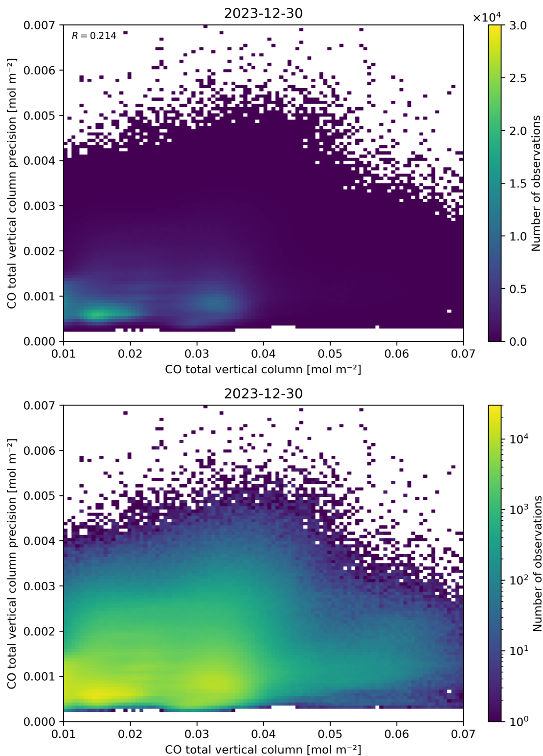
Figure 34: Scatter density plot of “CO total vertical column” against “CO total vertical column precision” for 2023-12-30 to 2023-12-31.
