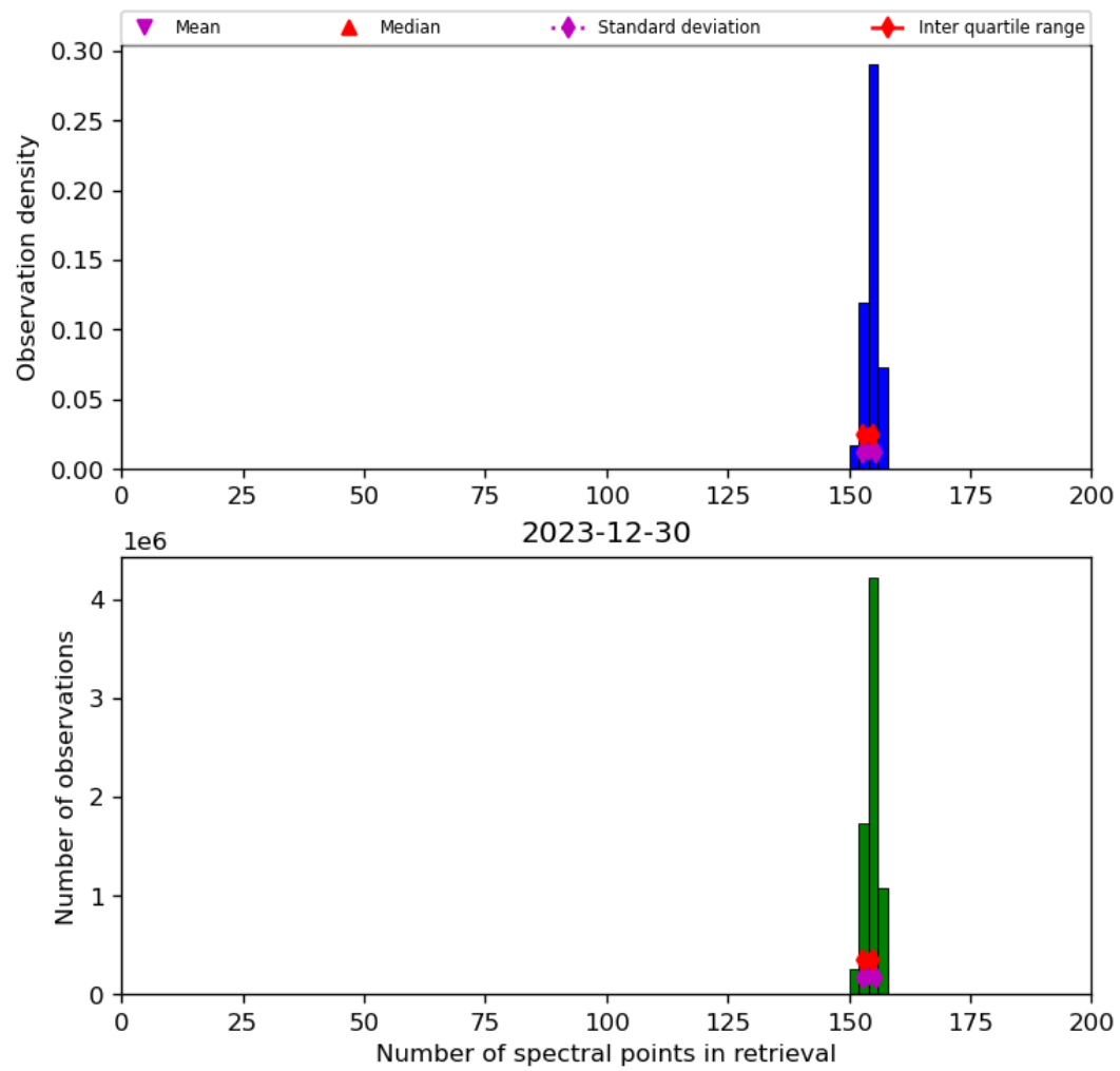
Figure 21: Histogram of “Number of spectral points in retrieval” for 2023-12-30 to 2023-12-31
