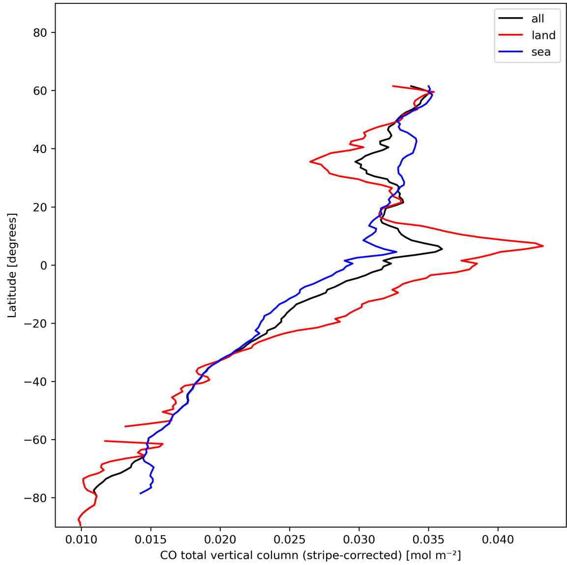
Figure 11: Zonal average of “CO total vertical column (stripe-corrected)” for 2023-12-30 to 2023-12-31.
