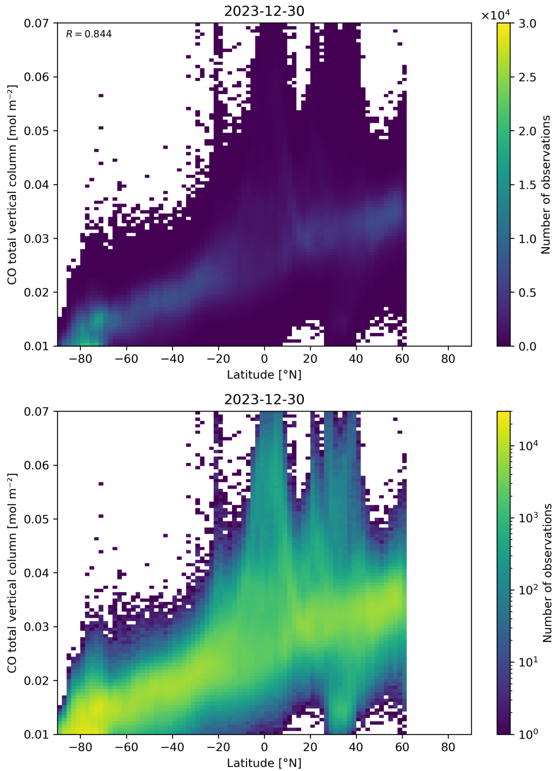
Figure 51: Scatter density plot of “Latitude” against “CO total vertical column” for 2023-12-30 to 2023-12-31.
