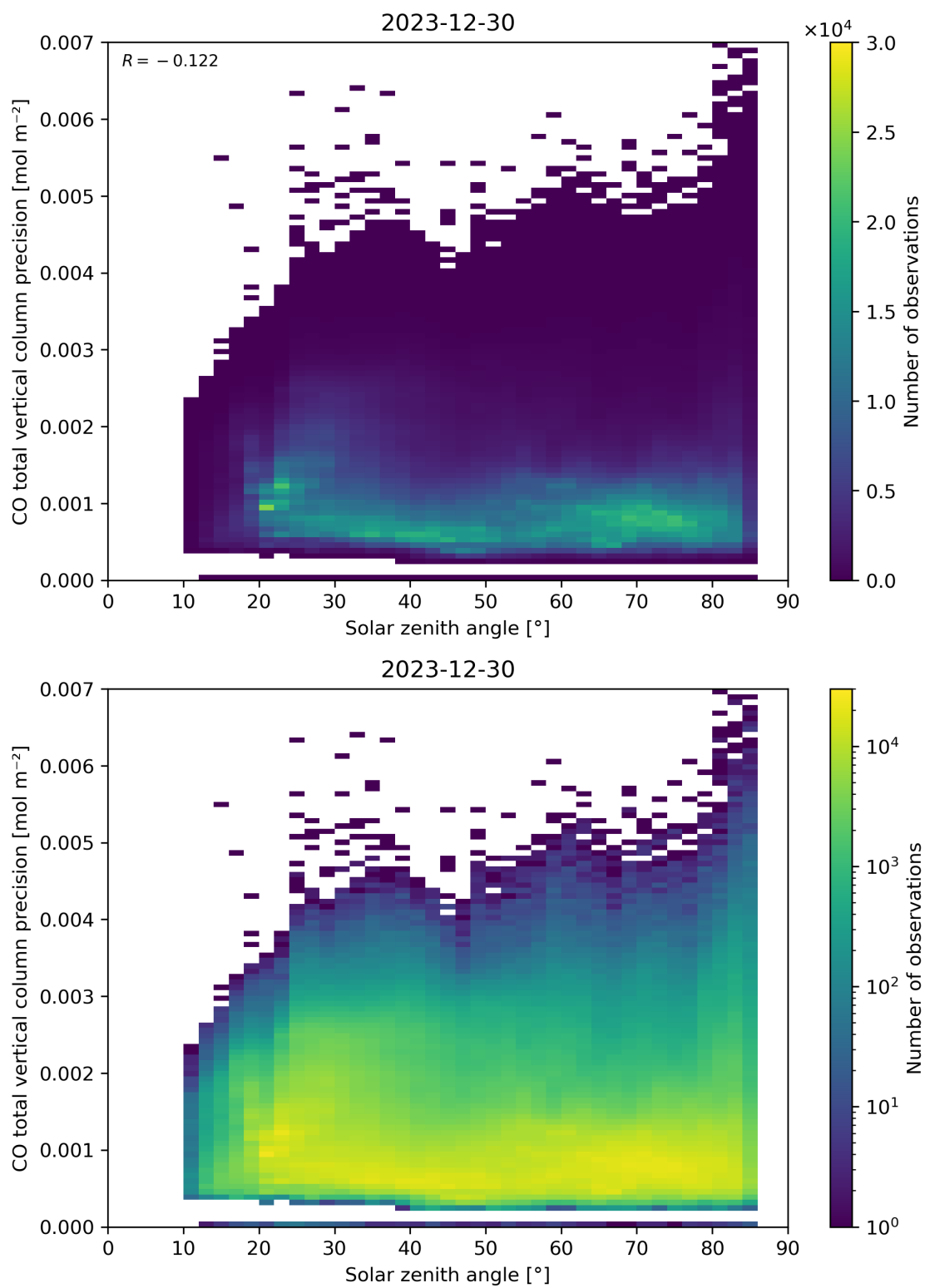
Figure 63: Scatter density plot of “Solar zenith angle” against “CO total vertical column precision” for 2023-12-30 to 2023-12-31.
