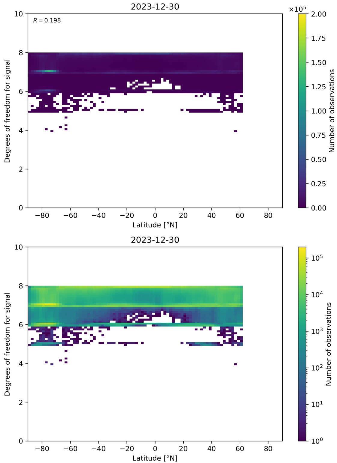
Figure 55: Scatter density plot of “Latitude” against “Degrees of freedom for signal” for 2023-12-30 to 2023-12-31.
