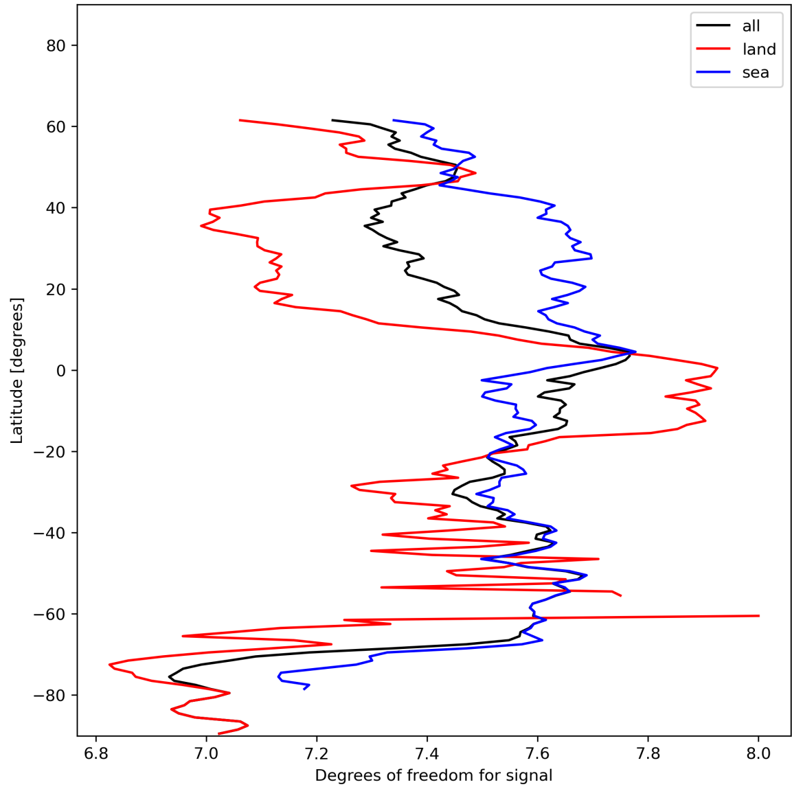
Figure 15: Zonal average of “Degrees of freedom for signal” for 2023-12-30 to 2023-12-31.
