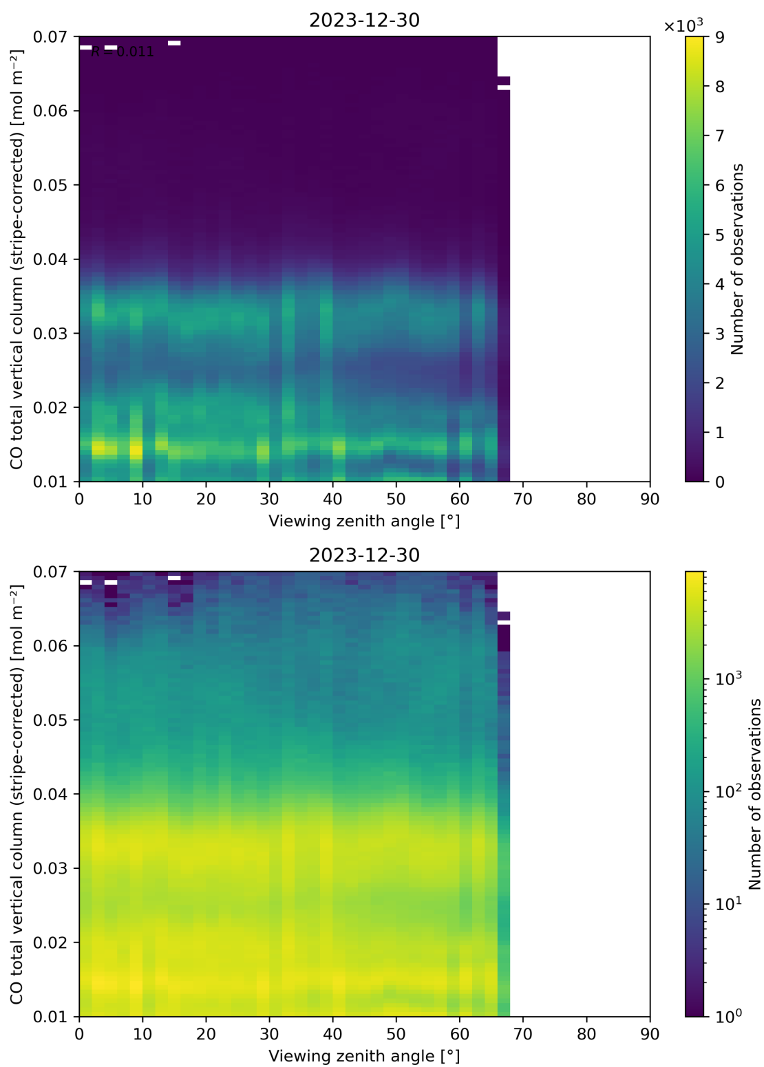
Figure 70: Scatter density plot of “Viewing zenith angle” against “CO total vertical column (stripe-corrected)” for 2023-12-30 to 2023-12-31.
