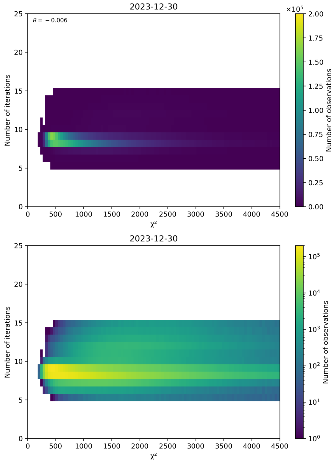
Figure 49: Scatter density plot of “ \chi^2 ” against “Number of iterations” for 2023-12-30 to 2023-12-31.
