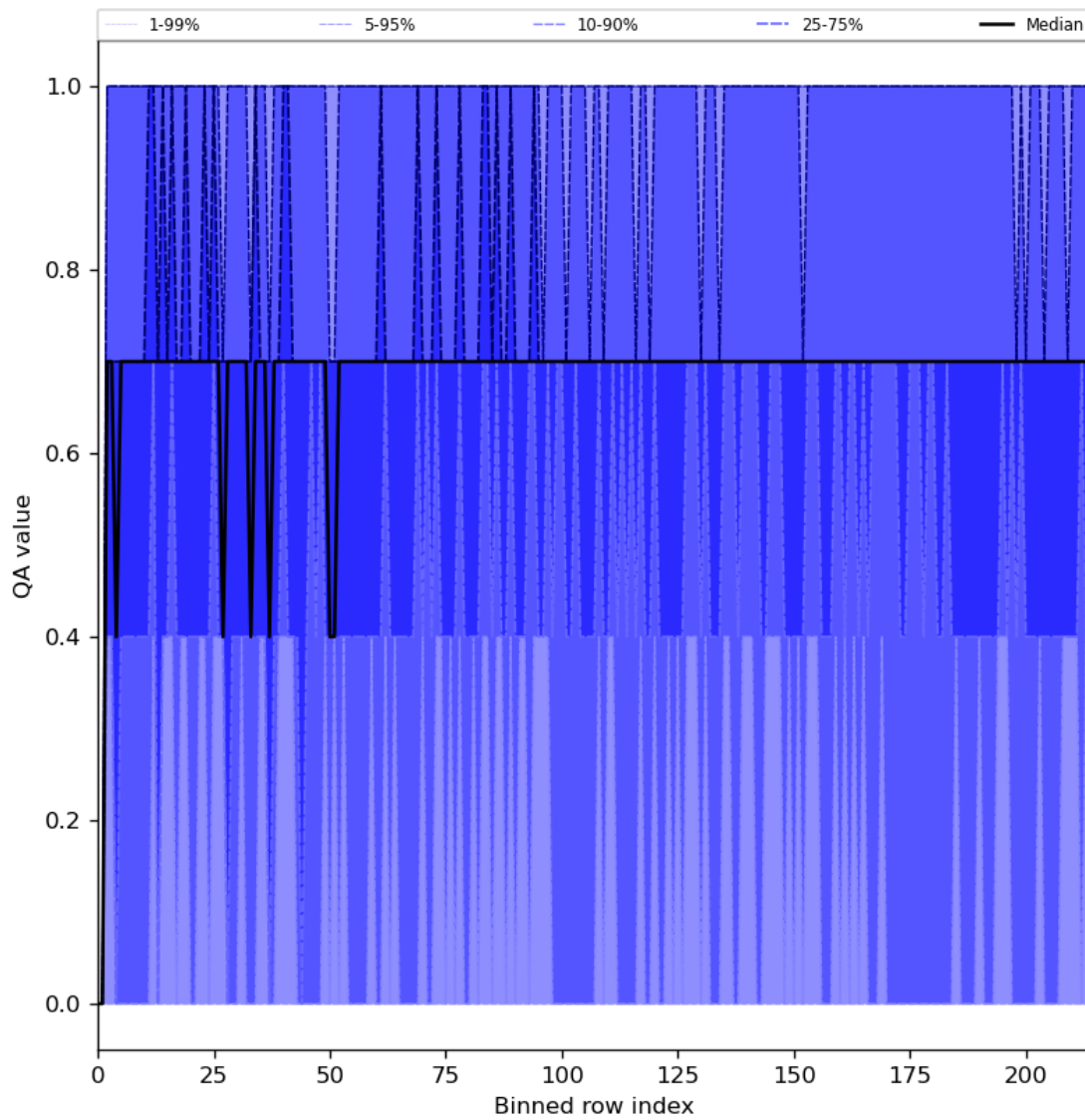
Figure 25: Along track statistics of “QA value” for 2023-12-30 to 2023-12-31
