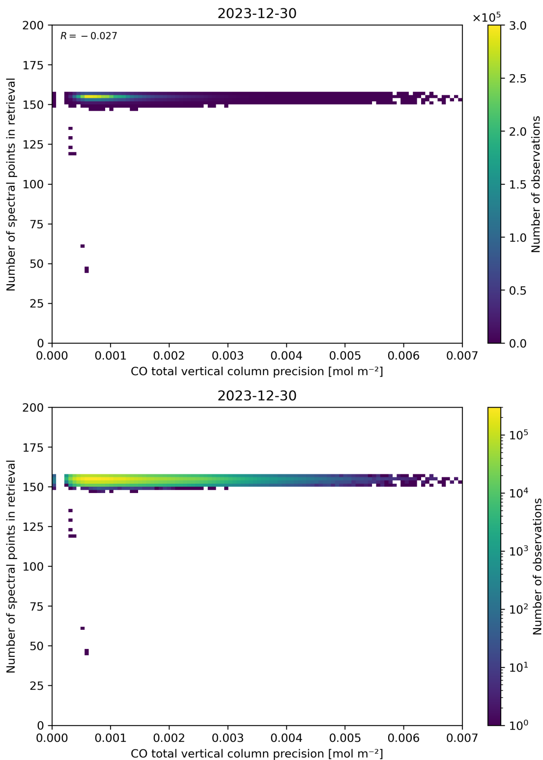
Figure 47: Scatter density plot of “CO total vertical column precision” against “Number of spectral points in retrieval” for 2023-12-30 to 2023-12-31.
