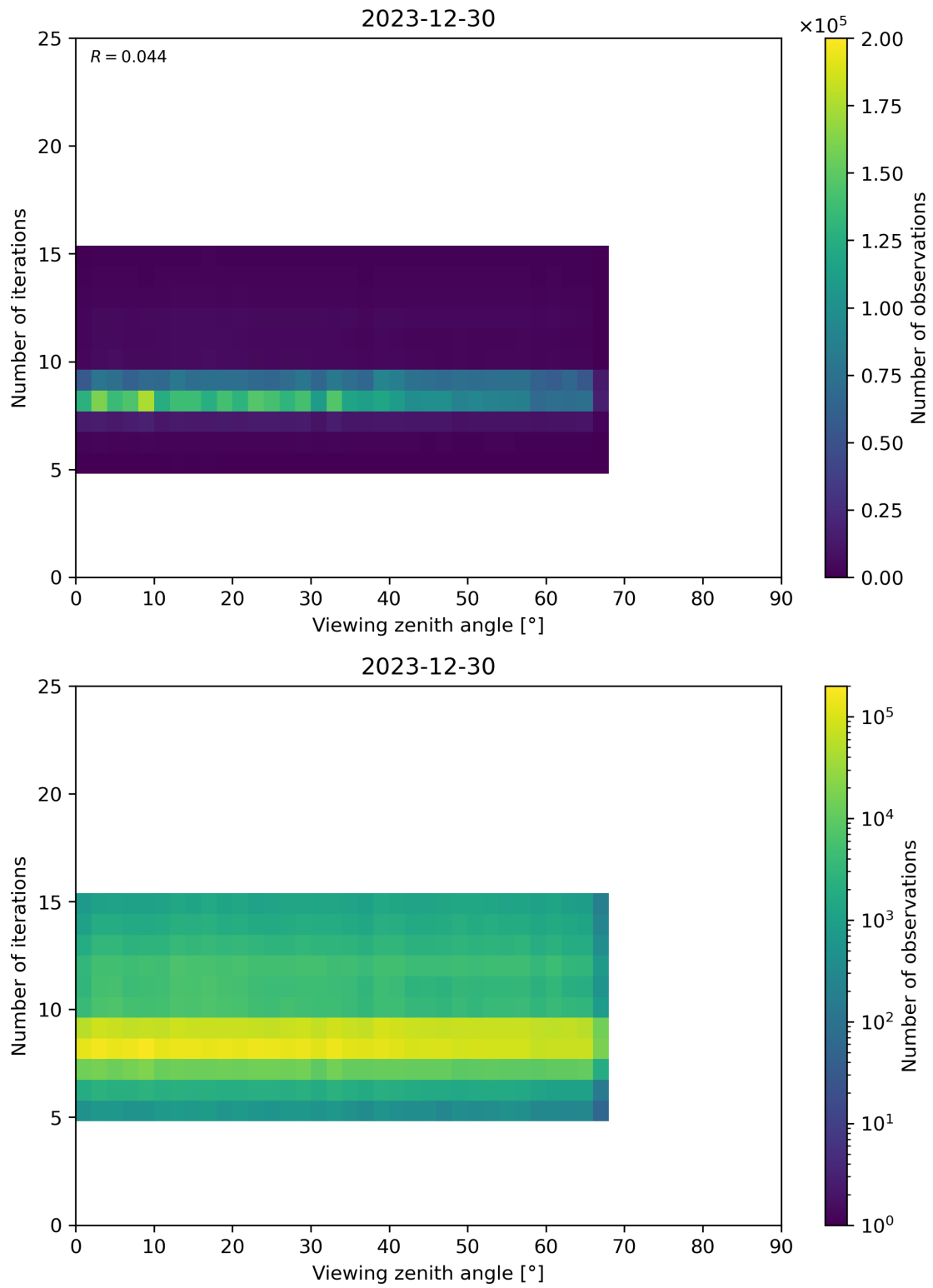
Figure 75: Scatter density plot of “Viewing zenith angle” against “Number of iterations” for 2023-12-30 to 2023-12-31.
