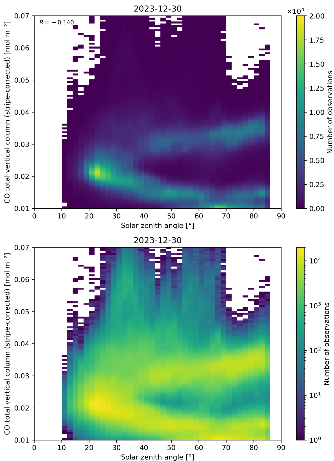
Figure 62: Scatter density plot of “Solar zenith angle” against “CO total vertical column (stripe-corrected)” for 2023-12-30 to 2023-12-31.
