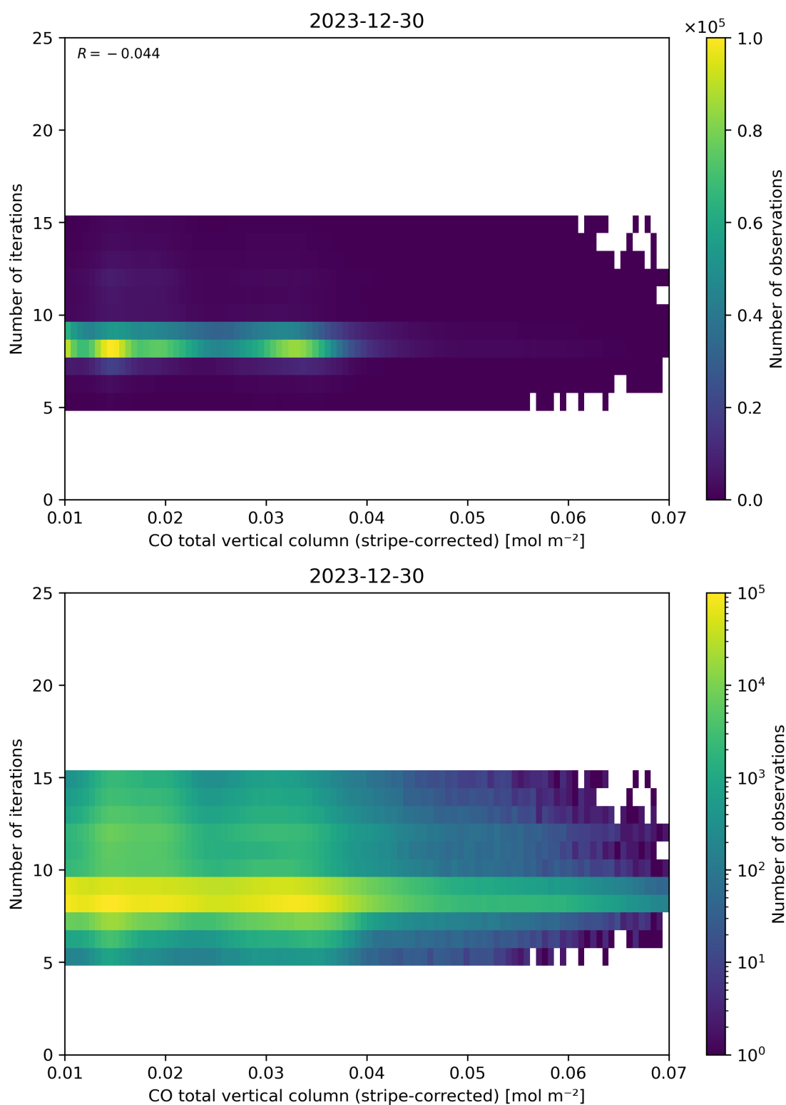
Figure 39: Scatter density plot of “CO total vertical column (stripe-corrected)” against “Number of iterations” for 2023-12-30 to 2023-12-31.
