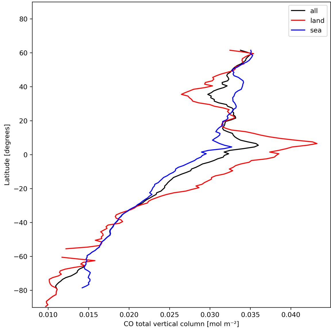
Figure 10: Zonal average of “CO total vertical column” for 2023-12-30 to 2023-12-31.
