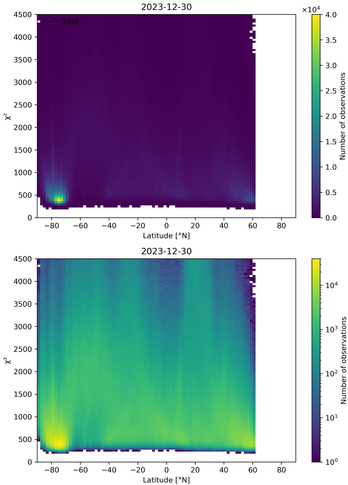
Figure 54: Scatter density plot of “Latitude” against “ \chi^2 ” for 2023-12-30 to 2023-12-31.
