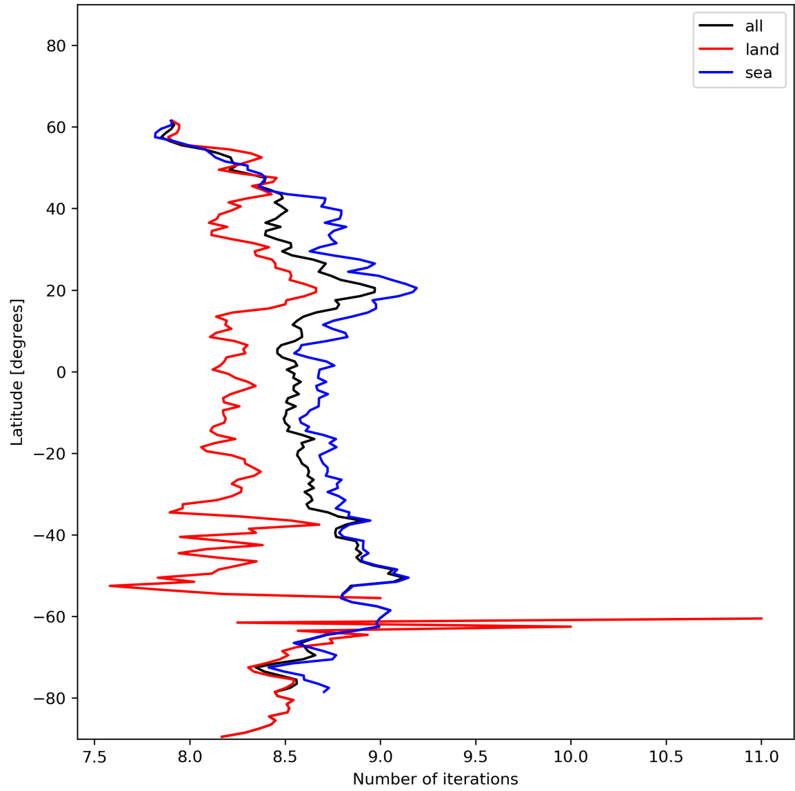
Figure 16: Zonal average of “Number of iterations” for 2023-12-30 to 2023-12-31.
