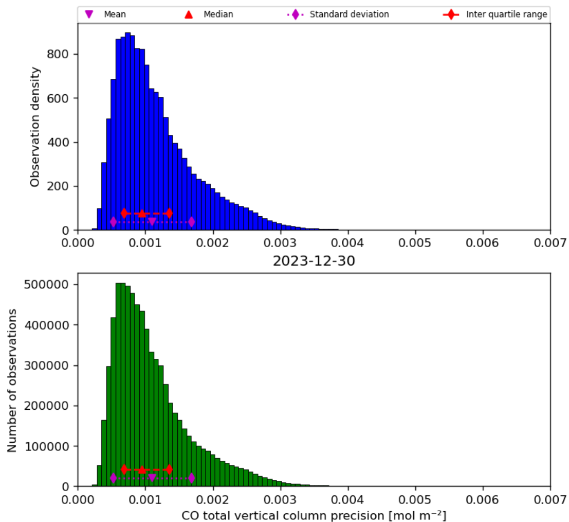
Figure 20: Histogram of “CO total vertical column precision” for 2023-12-30 to 2023-12-31
