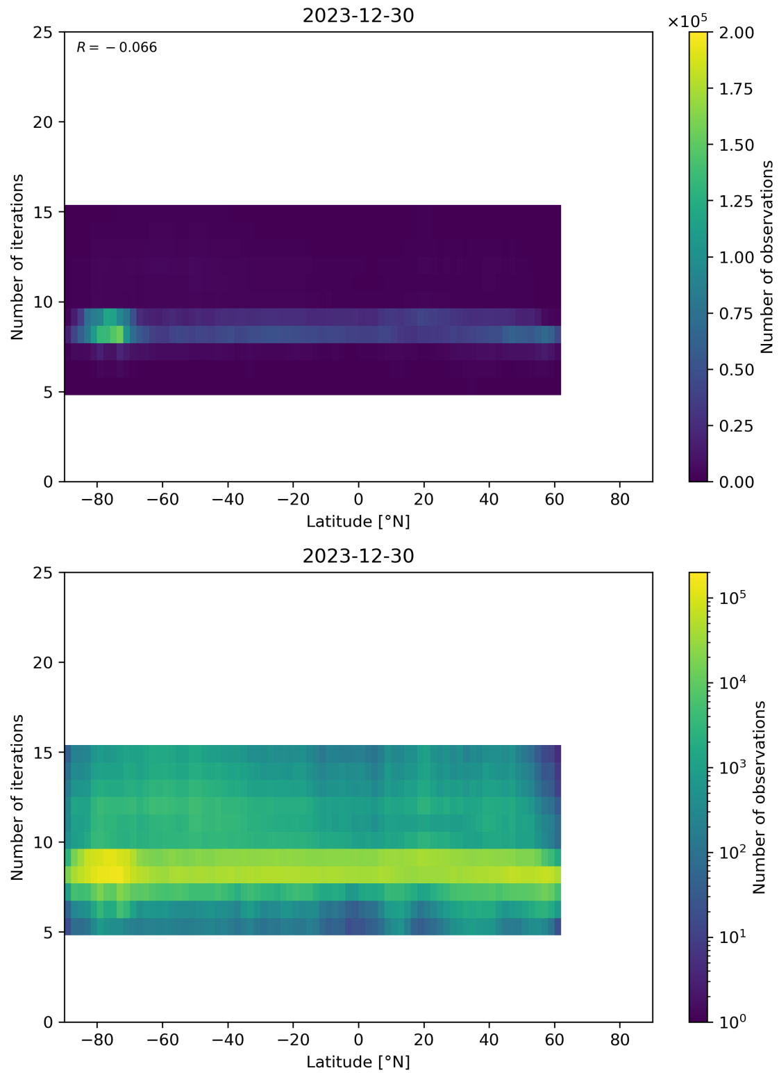
Figure 56: Scatter density plot of “Latitude” against “Number of iterations” for 2023-12-30 to 2023-12-31.
