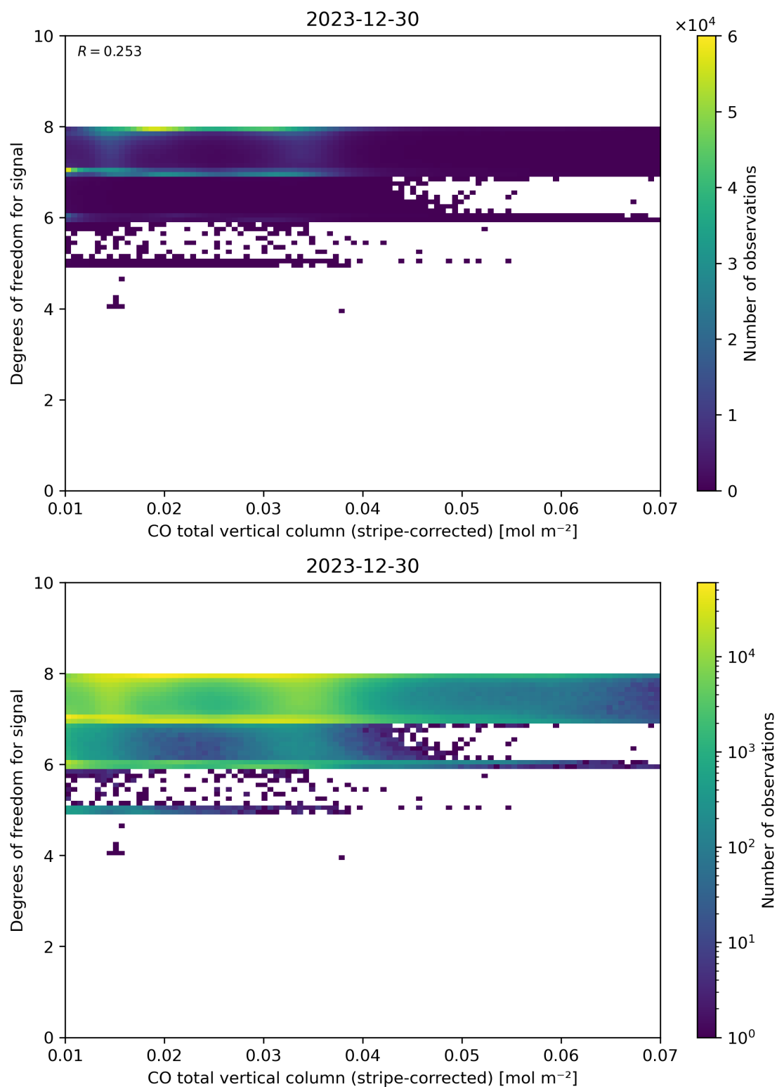
Figure 38: Scatter density plot of “CO total vertical column (stripe-corrected)” against “Degrees of freedom for signal” for 2023-12-30 to 2023-12-31.
