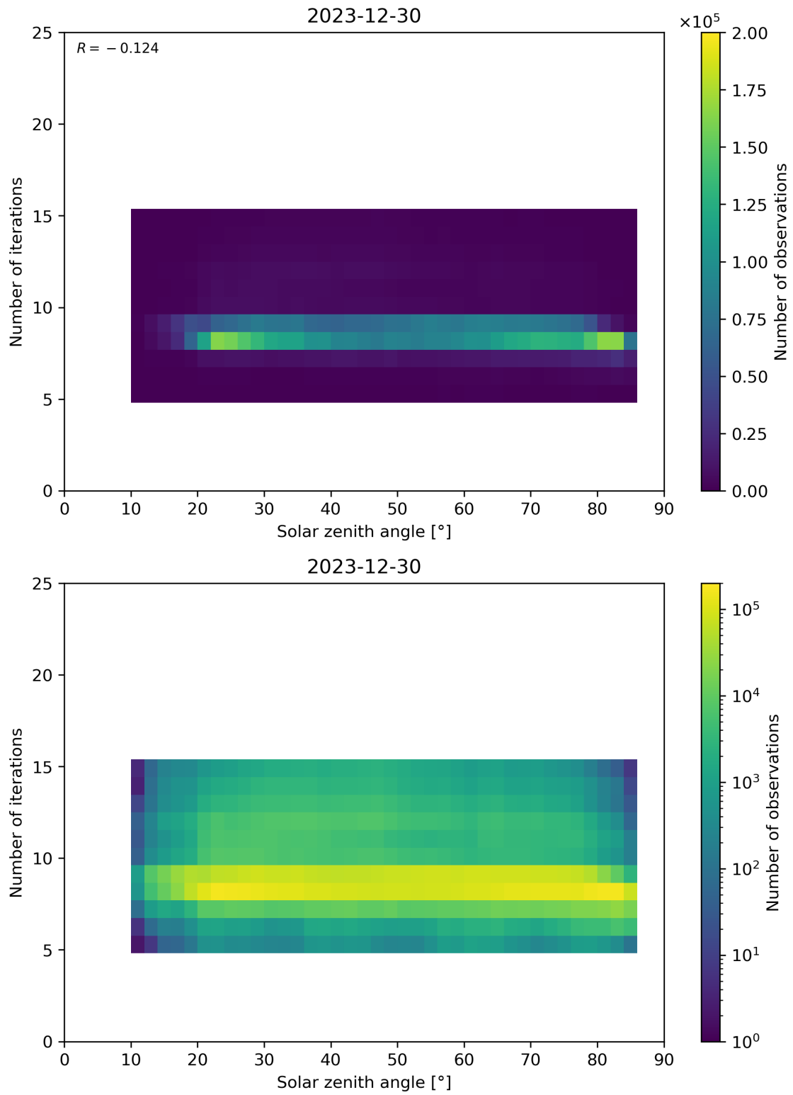
Figure 67: Scatter density plot of “Solar zenith angle” against “Number of iterations” for 2023-12-30 to 2023-12-31.
