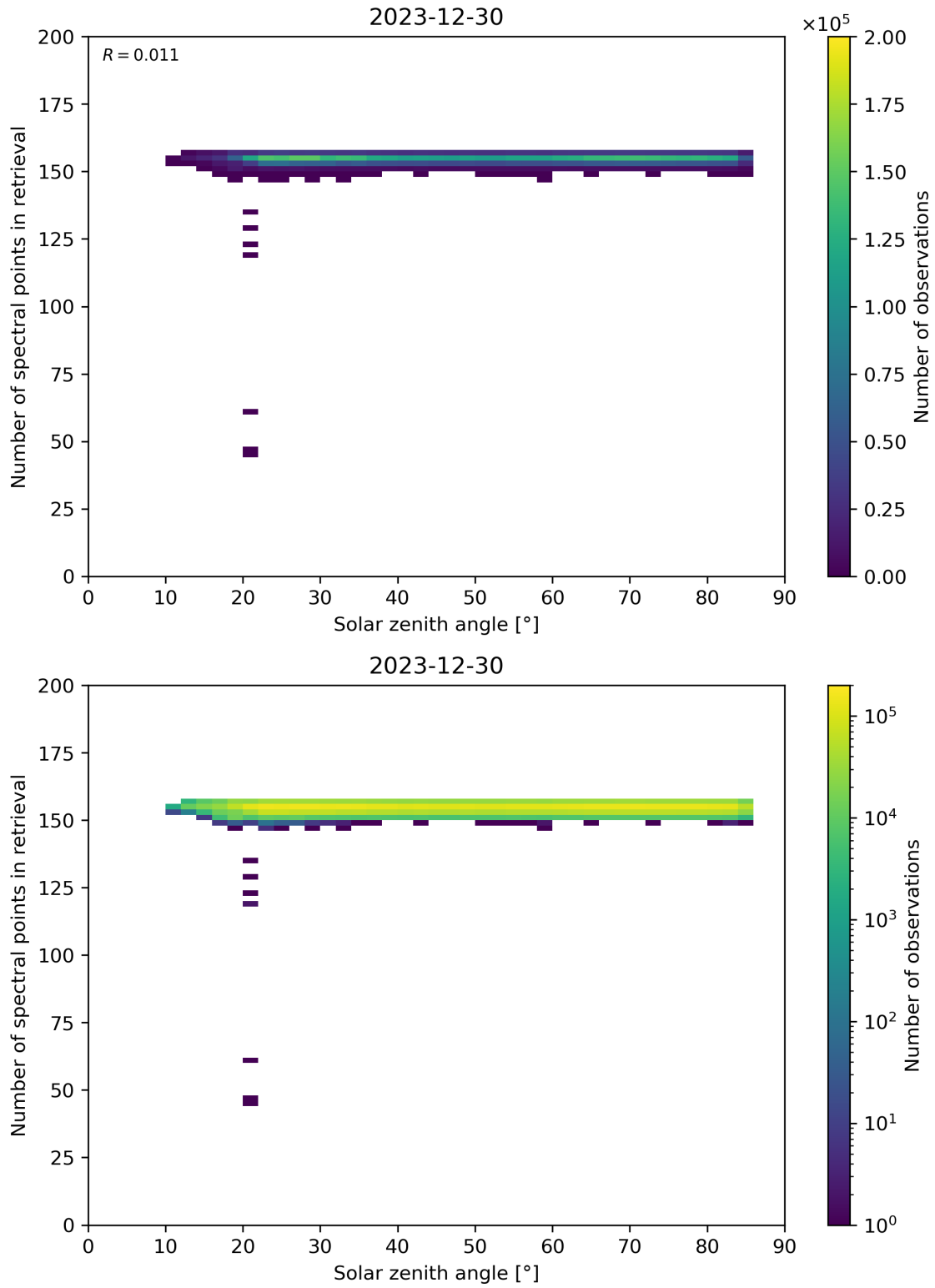
Figure 68: Scatter density plot of “Solar zenith angle” against “Number of spectral points in retrieval” for 2023-12-30 to 2023-12-31.
