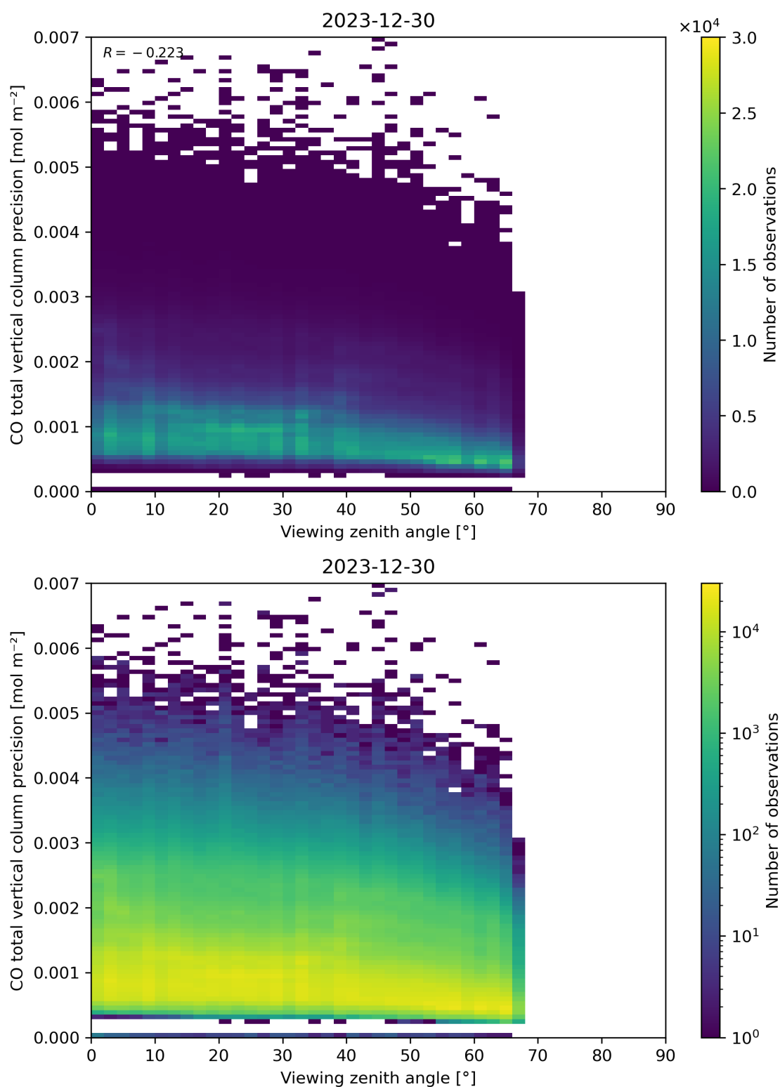
Figure 71: Scatter density plot of “Viewing zenith angle” against “CO total vertical column precision” for 2023-12-30 to 2023-12-31.
