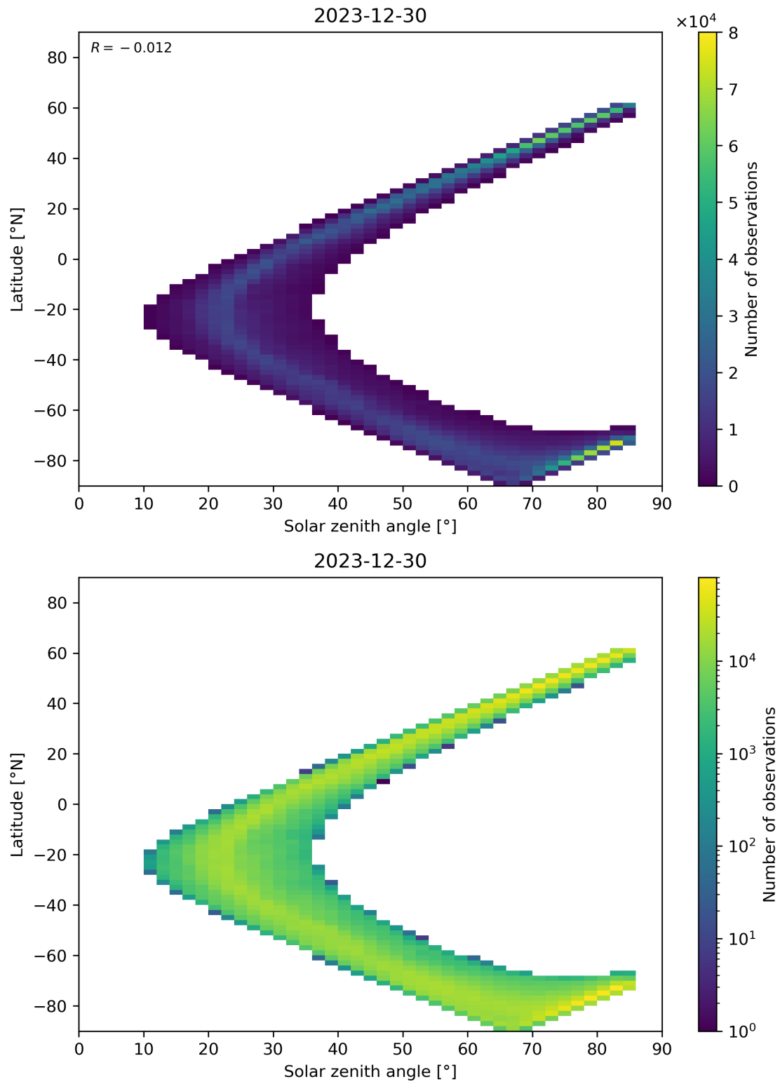
Figure 66: Scatter density plot of “Solar zenith angle” against “Latitude” for 2023-12-30 to 2023-12-31.
