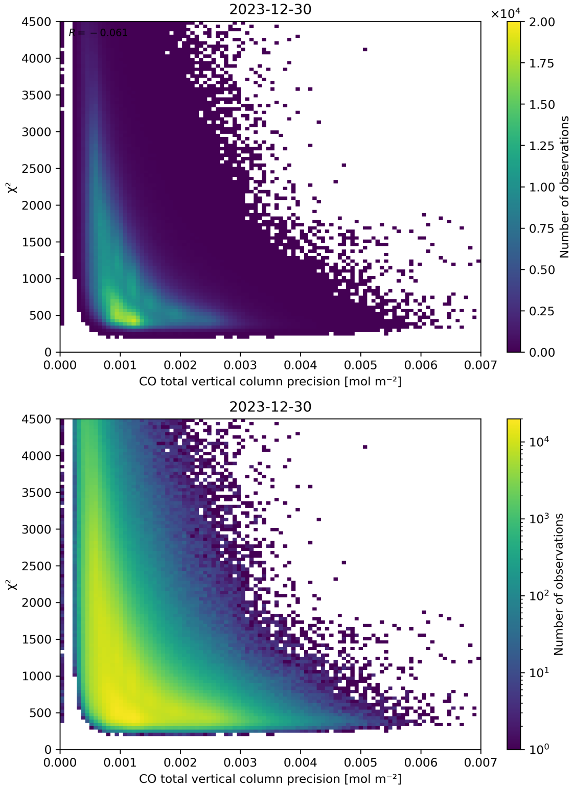
Figure 44: Scatter density plot of “CO total vertical column precision” against “ \chi^2 ” for 2023-12-30 to 2023-12-31.
