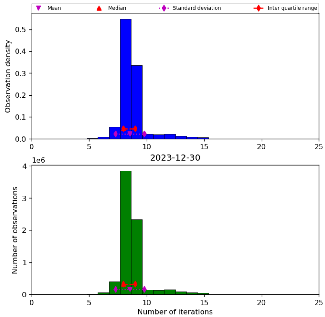
Figure 24: Histogram of “Number of iterations” for 2023-12-30 to 2023-12-31
