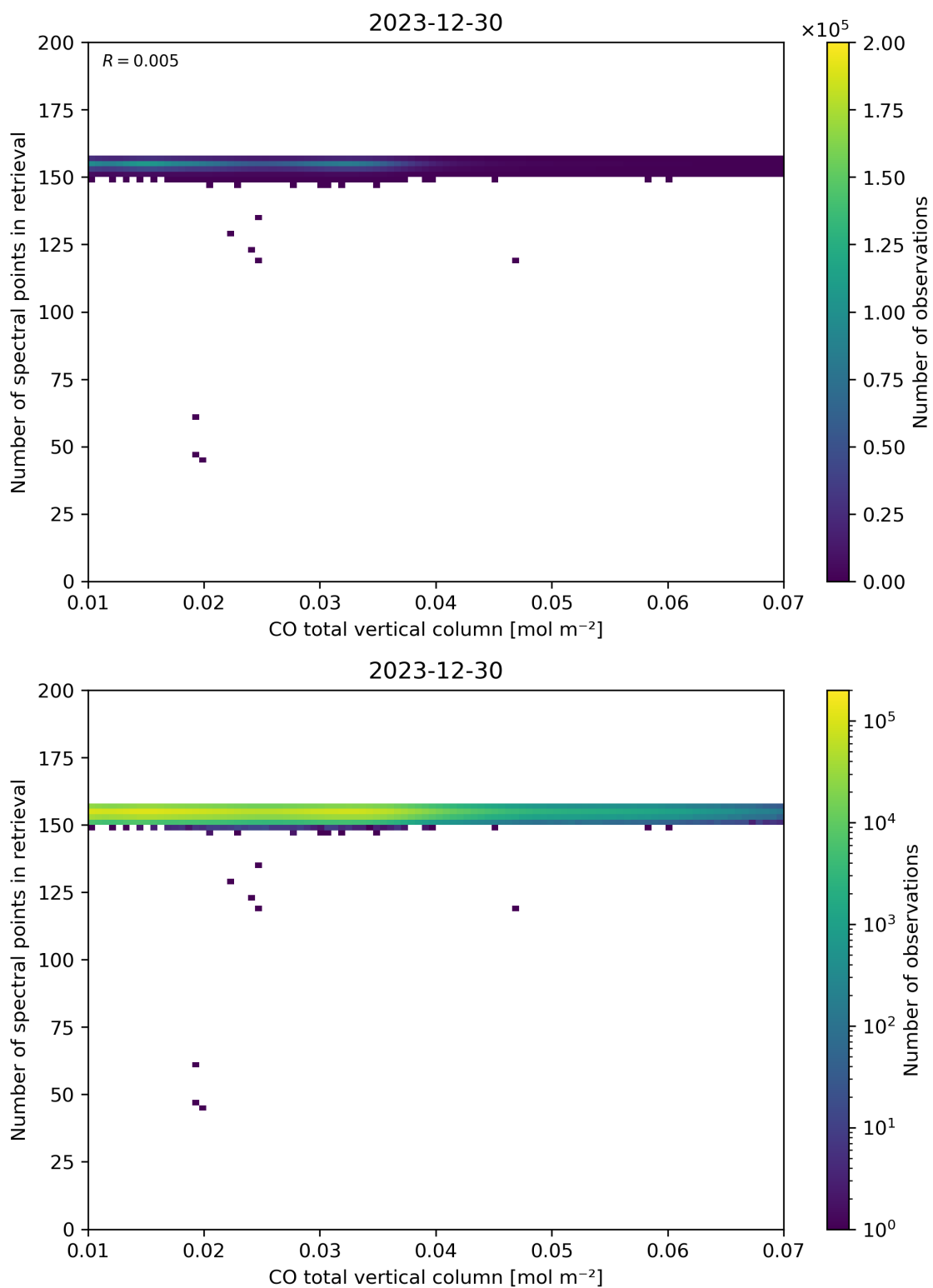
Figure 43: Scatter density plot of “CO total vertical column” against “Number of spectral points in retrieval” for 2023-12-30 to 2023-12-31.
