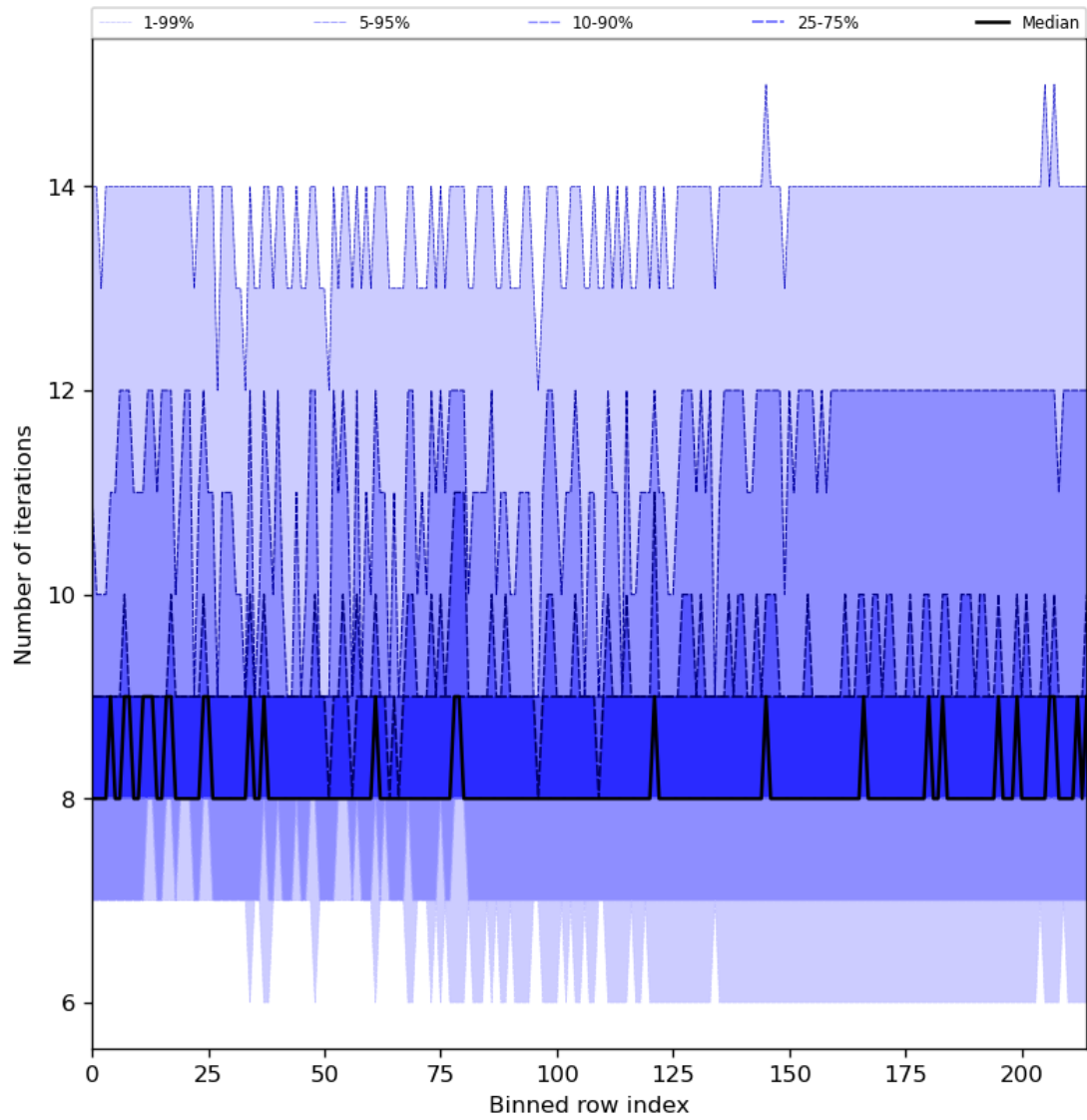
Figure 32: Along track statistics of “Number of iterations” for 2023-12-30 to 2023-12-31
