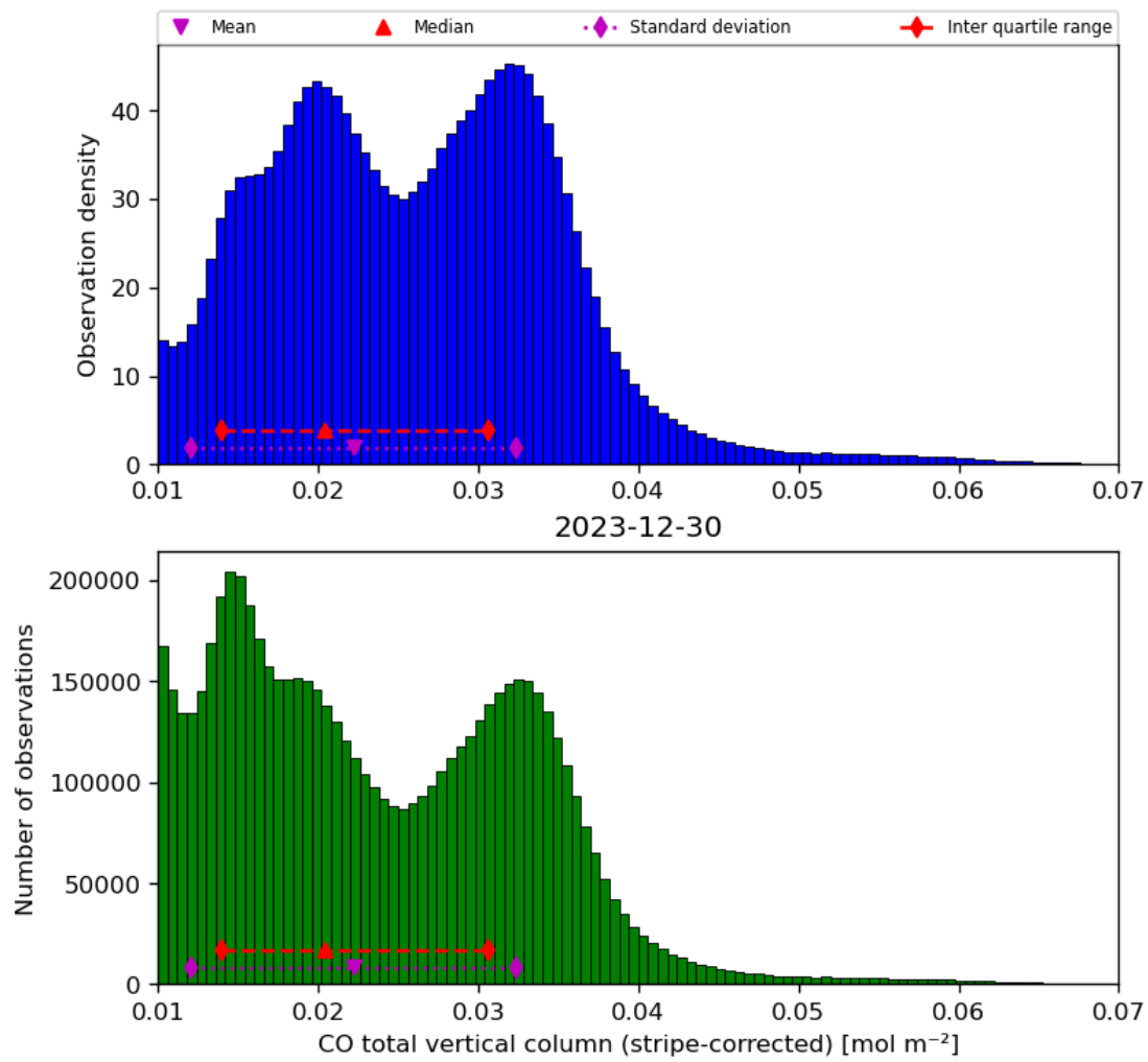
Figure 19: Histogram of “CO total vertical column (stripe-corrected)” for 2023-12-30 to 2023-12-31
