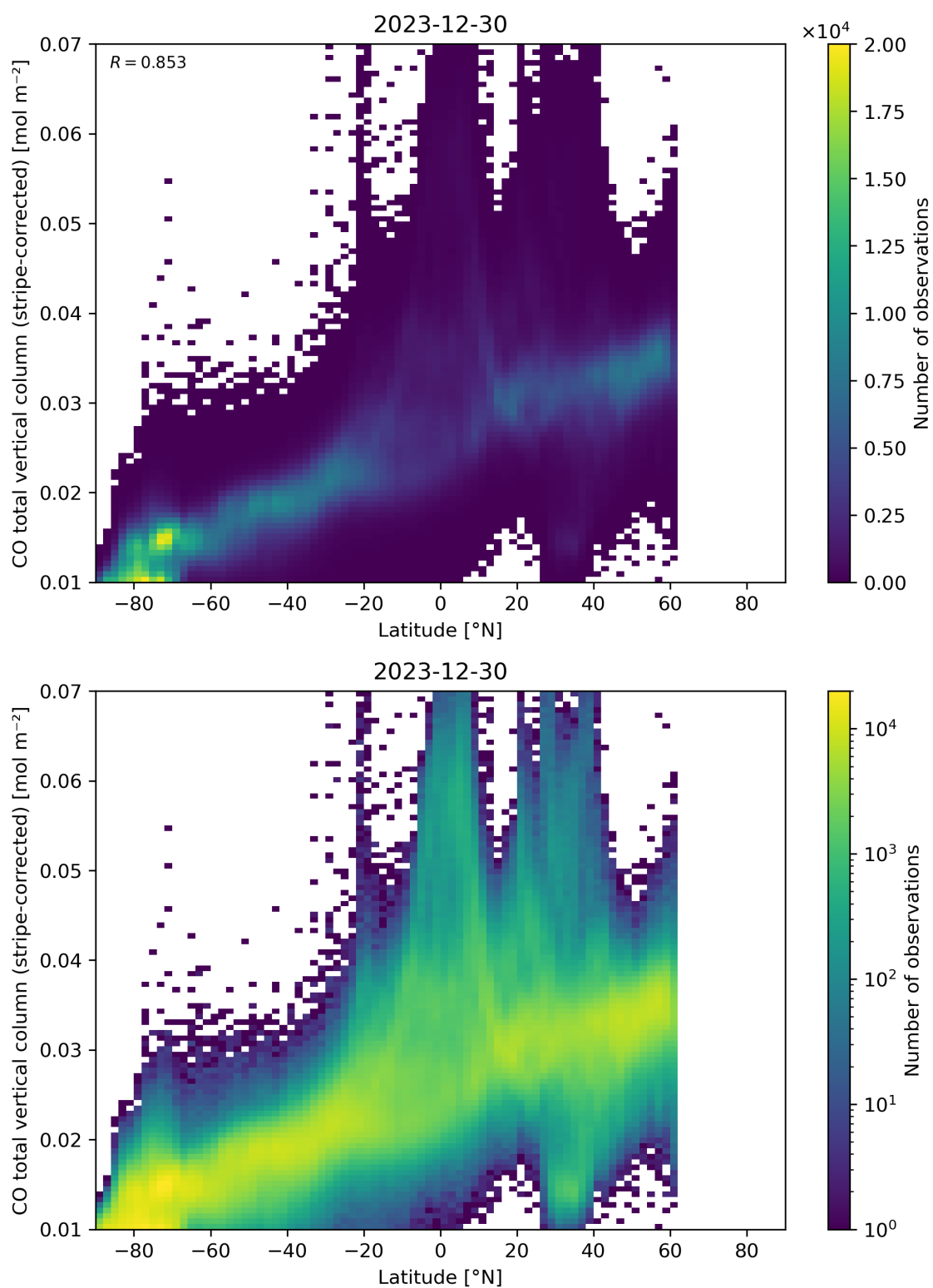
Figure 52: Scatter density plot of “Latitude” against “CO total vertical column (stripe-corrected)” for 2023-12-30 to 2023-12-31.
