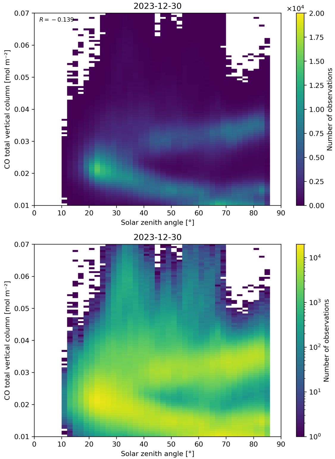
Figure 61: Scatter density plot of “Solar zenith angle” against “CO total vertical column” for 2023-12-30 to 2023-12-31.
