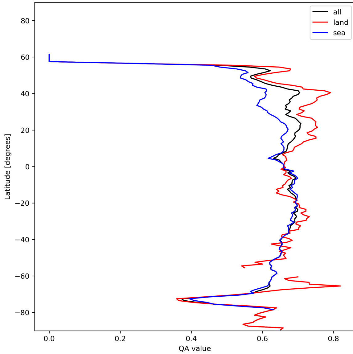
Figure 9: Zonal average of “QA value” for 2023-12-30 to 2023-12-31.
