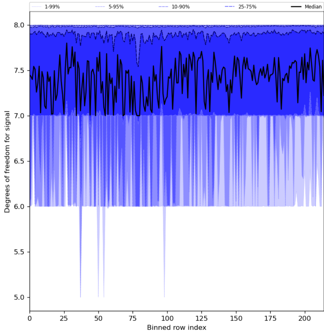
Figure 31: Along track statistics of “Degrees of freedom for signal” for 2023-12-30 to 2023-12-31
