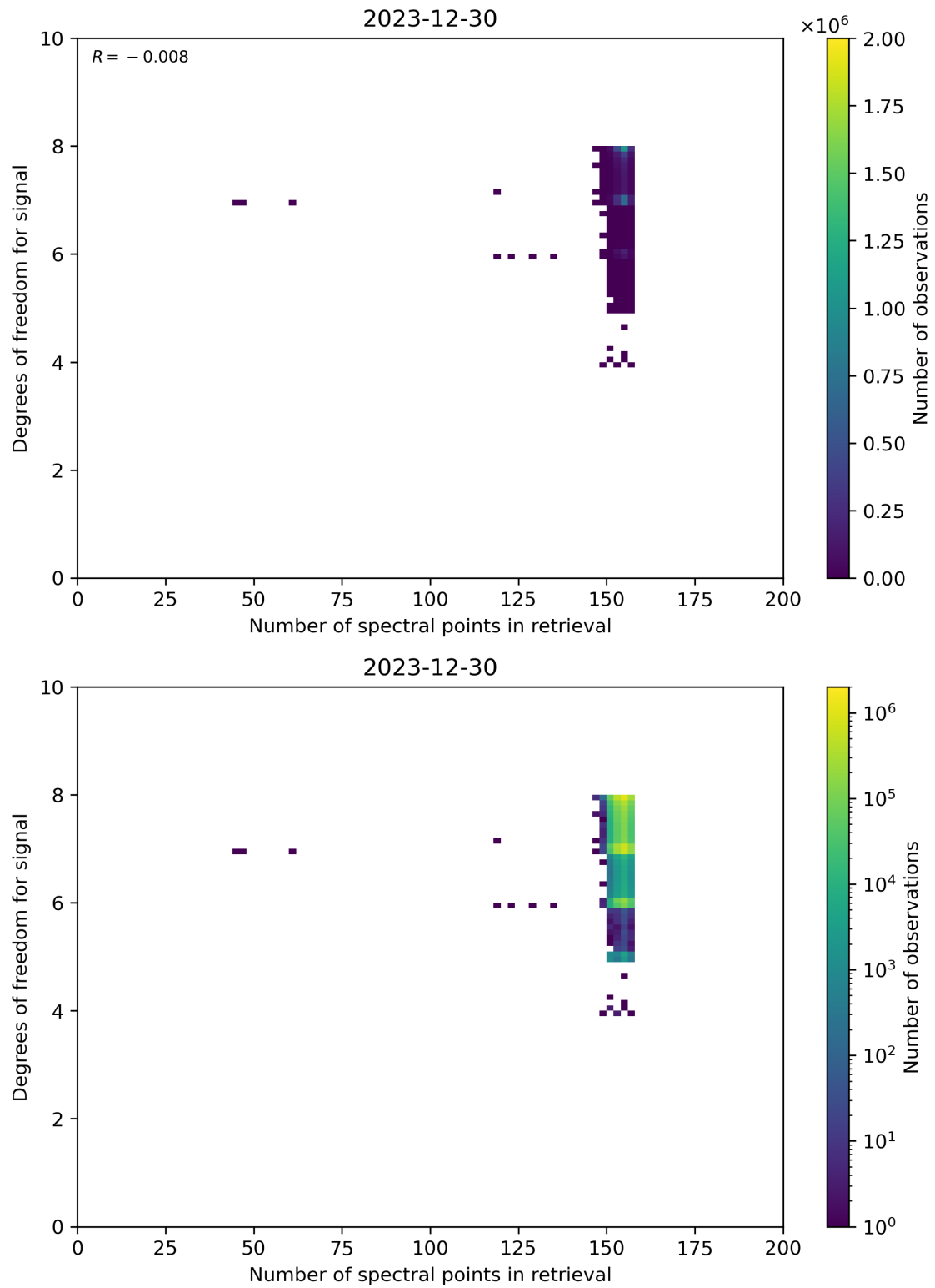
Figure 59: Scatter density plot of “Number of spectral points in retrieval” against “Degrees of freedom for signal” for 2023-12-30 to 2023-12-31.
