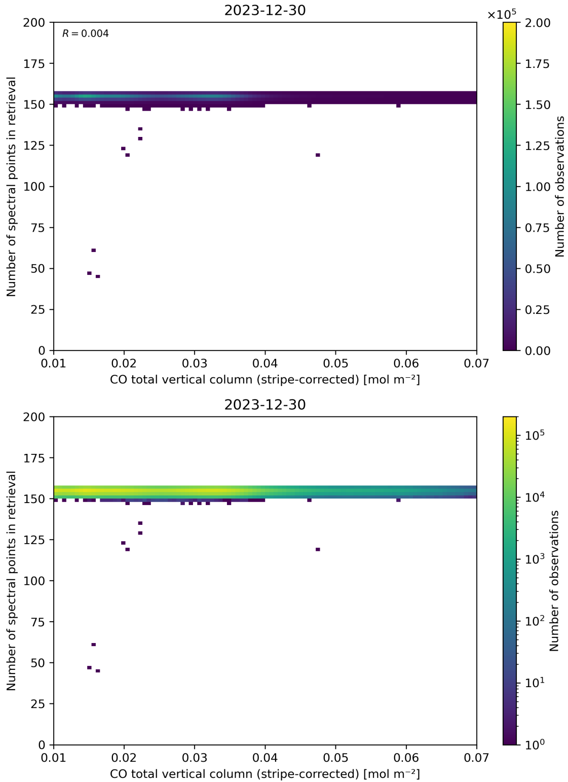
Figure 40: Scatter density plot of “CO total vertical column (stripe-corrected)” against “Number of spectral points in retrieval” for 2023-12-30 to 2023-12-31.
