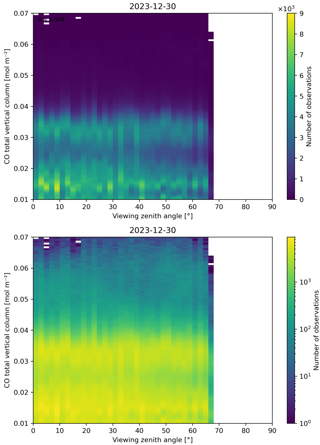
Figure 69: Scatter density plot of “Viewing zenith angle” against “CO total vertical column” for 2023-12-30 to 2023-12-31.
