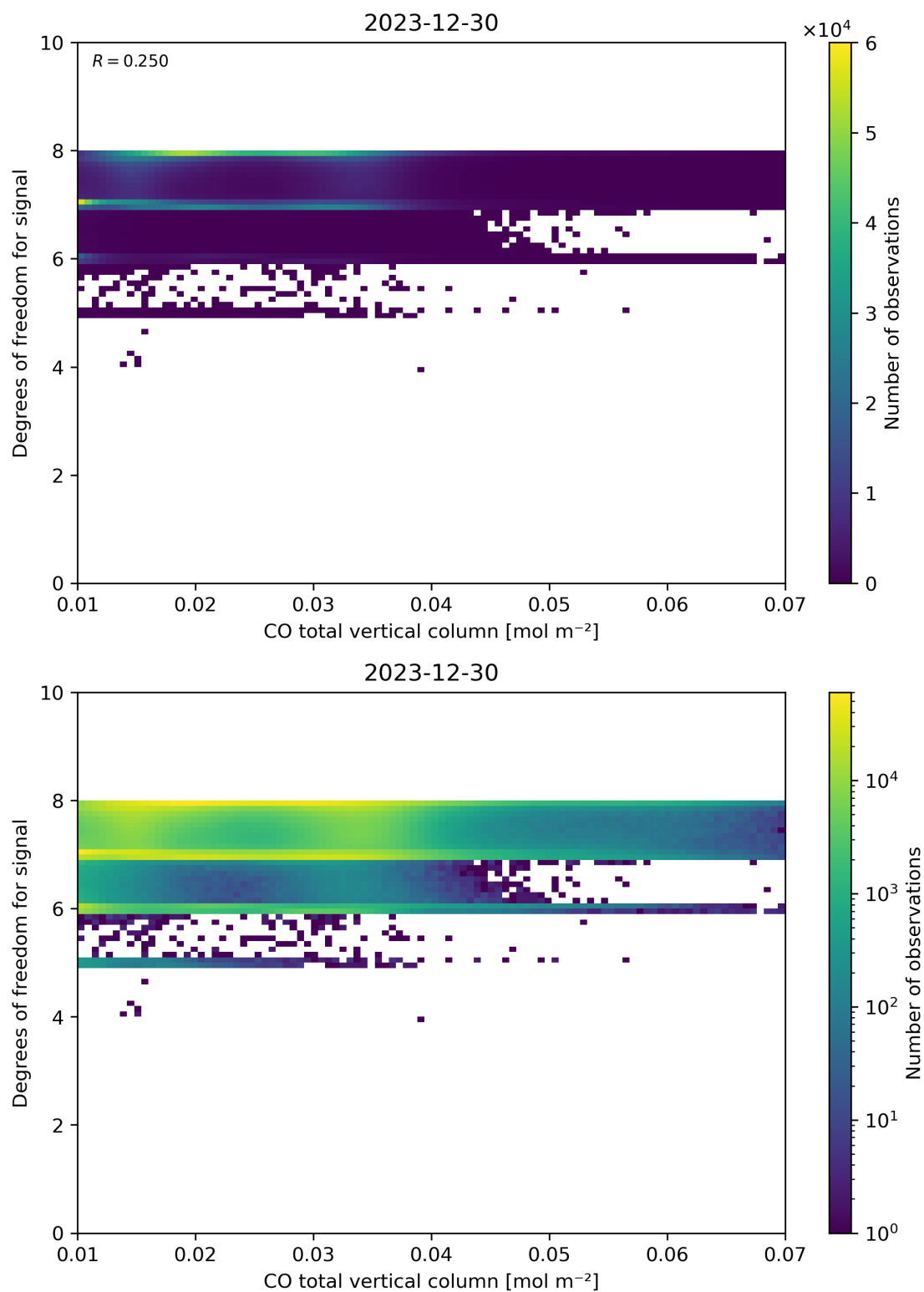
Figure 41: Scatter density plot of “CO total vertical column” against “Degrees of freedom for signal” for 2023-12-30 to 2023-12-31.
