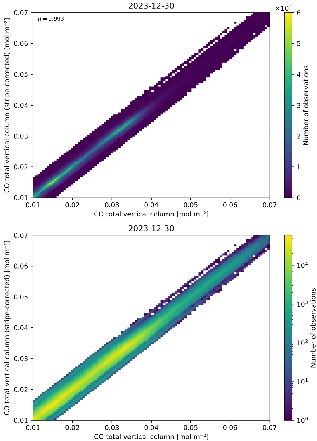
Figure 33: Scatter density plot of “CO total vertical column” against “CO total vertical column (stripe-corrected)” for 2023-12-30 to 2023-12-31.
