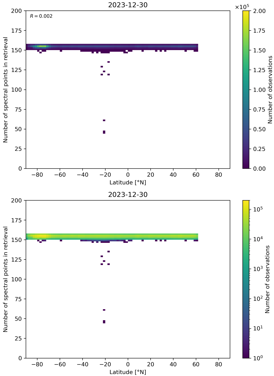
Figure 57: Scatter density plot of “Latitude” against “Number of spectral points in retrieval” for 2023-12-30 to 2023-12-31.
