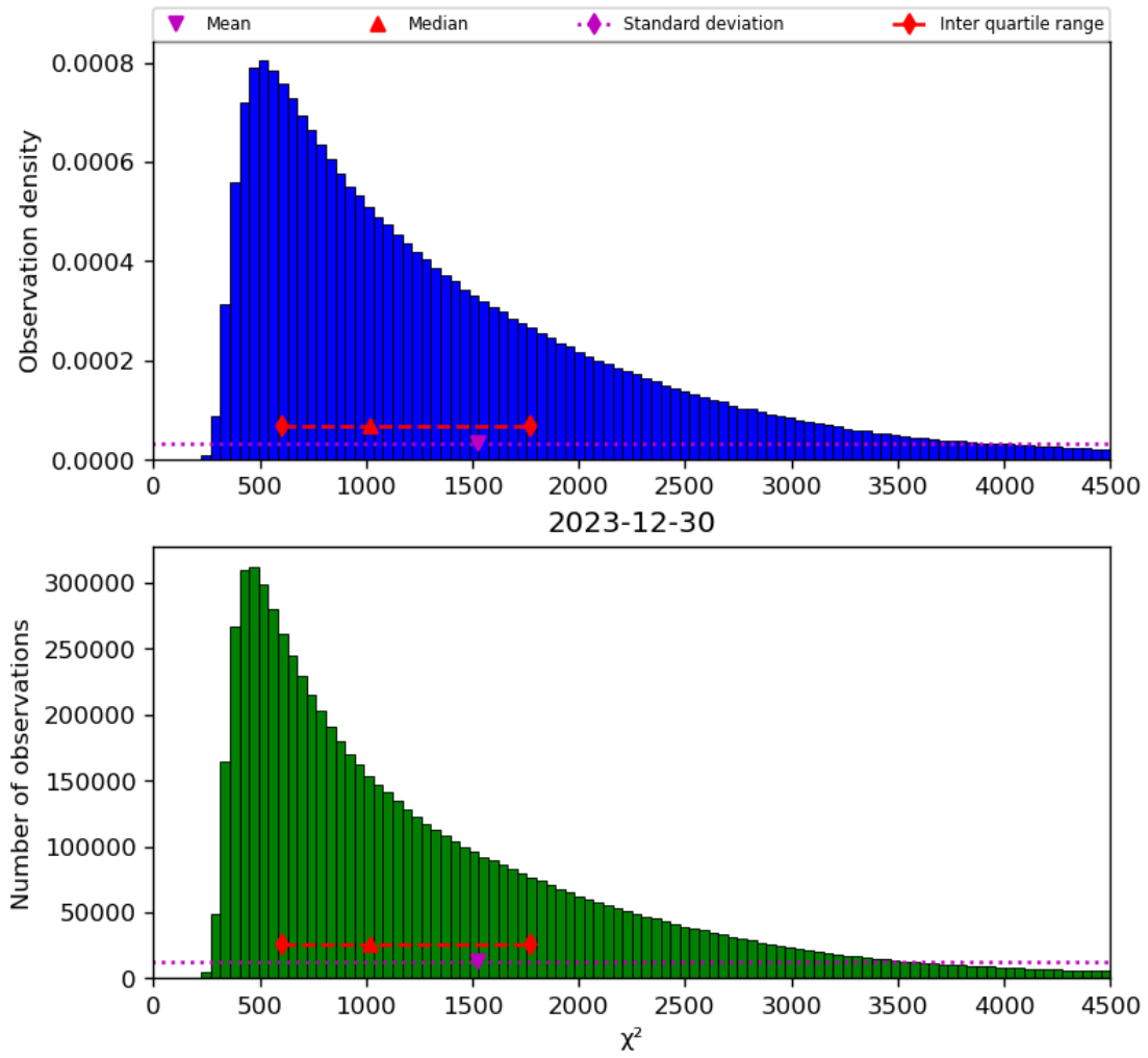
Figure 22: Histogram of “ \chi^2 ” for 2023-12-30 to 2023-12-31
