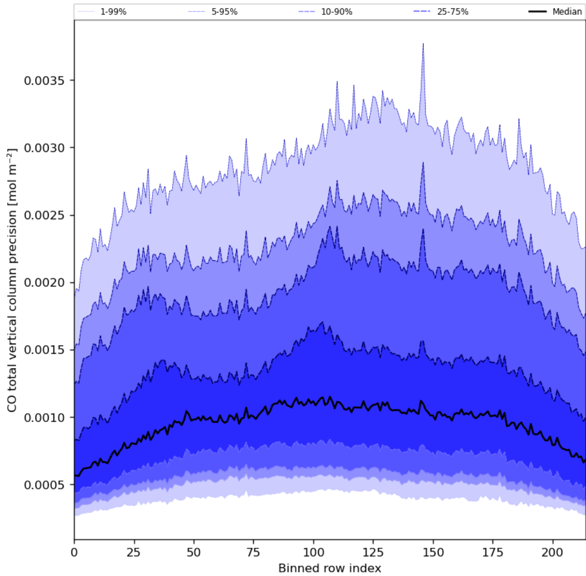
Figure 28: Along track statistics of “CO total vertical column precision” for 2023-12-30 to 2023-12-31
