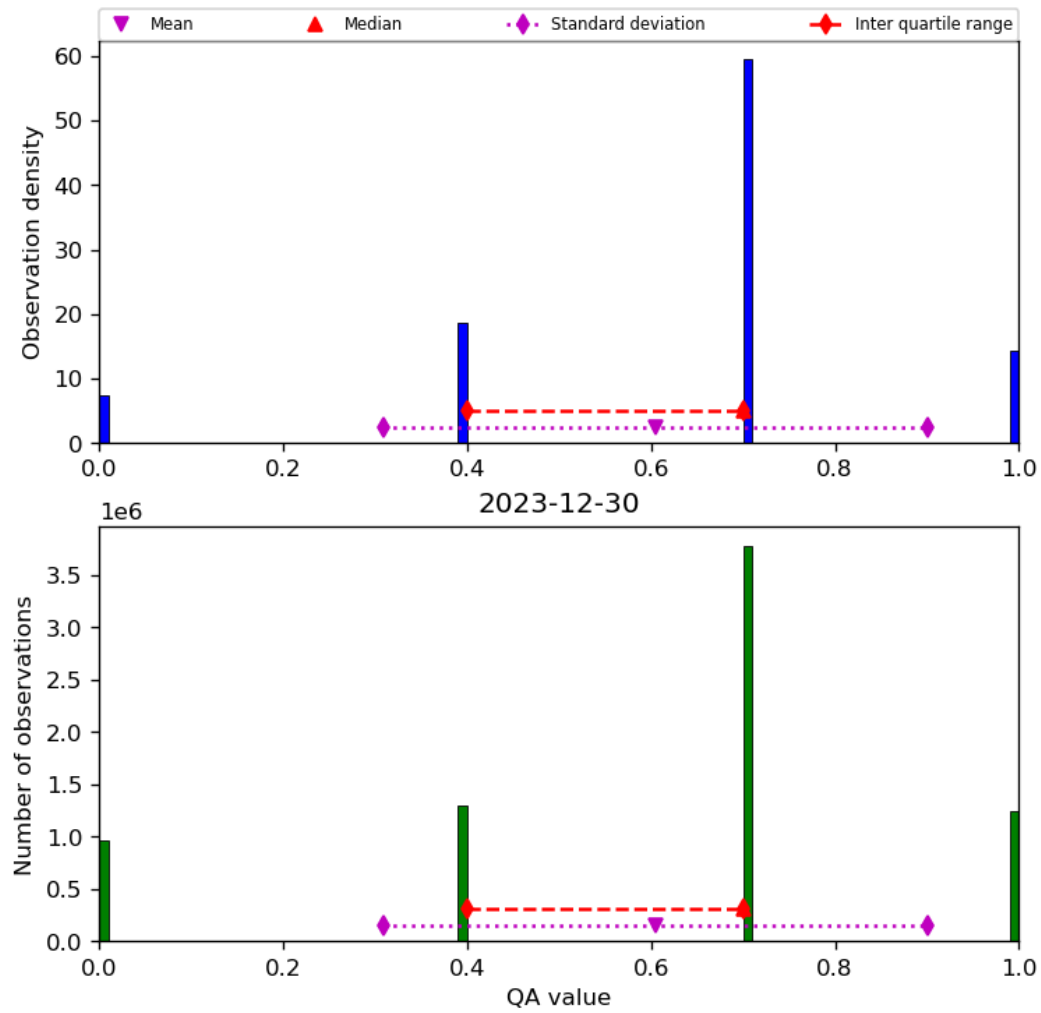
Figure 17: Histogram of “QA value” for 2023-12-30 to 2023-12-31
