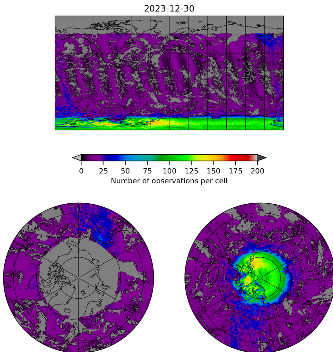
Figure 8: Map of the number of observations for 2023-12-30 to 2023-12-31
