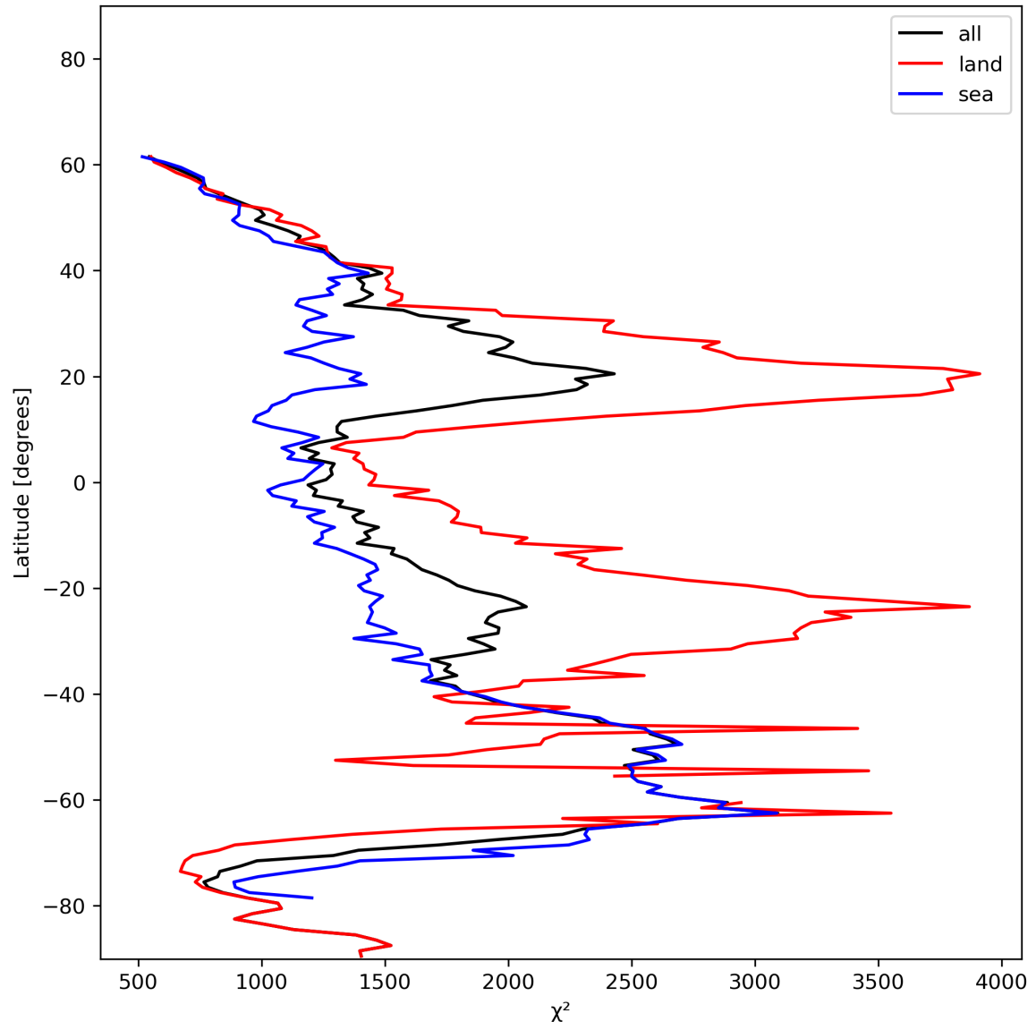
Figure 14: Zonal average of “ \chi^2 ” for 2023-12-30 to 2023-12-31.
