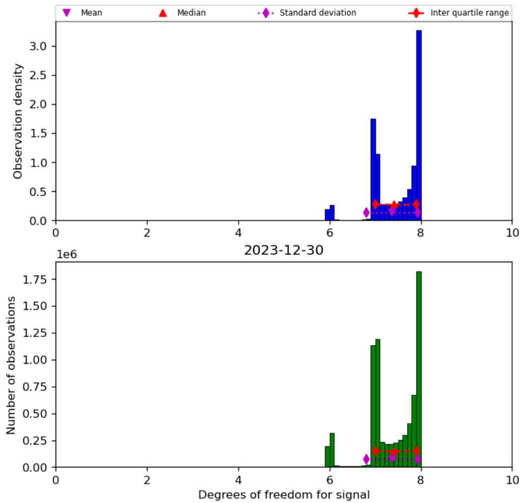
Figure 23: Histogram of “Degrees of freedom for signal” for 2023-12-30 to 2023-12-31
