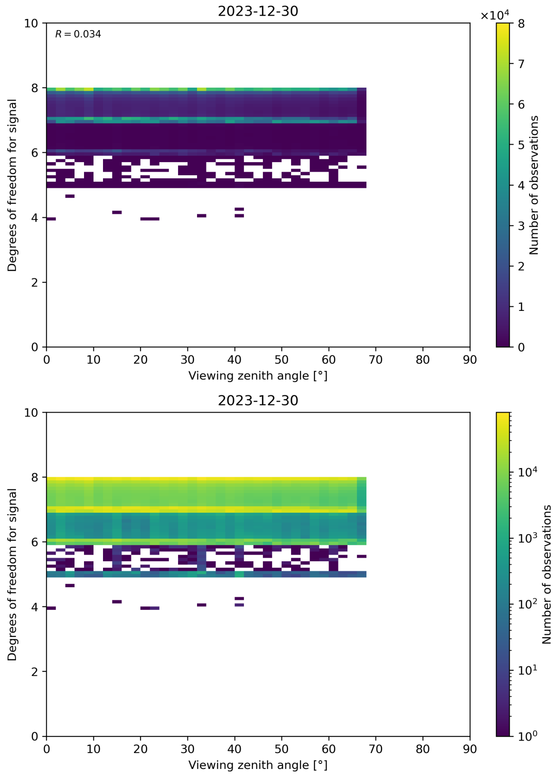
Figure 73: Scatter density plot of “Viewing zenith angle” against “Degrees of freedom for signal” for 2023-12-30 to 2023-12-31.
