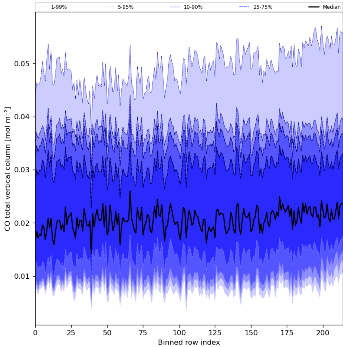
Figure 26: Along track statistics of “CO total vertical column” for 2023-12-30 to 2023-12-31
