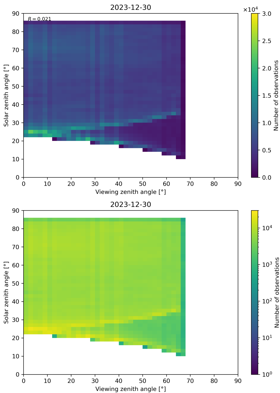
Figure 77: Scatter density plot of “Viewing zenith angle” against “Solar zenith angle” for 2023-12-30 to 2023-12-31.
