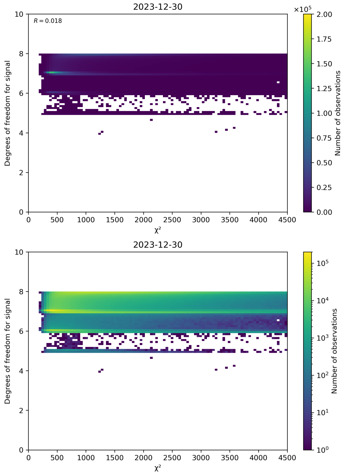
Figure 48: Scatter density plot of “ \chi^2 ” against “Degrees of freedom for signal” for 2023-12-30 to 2023-12-31.
