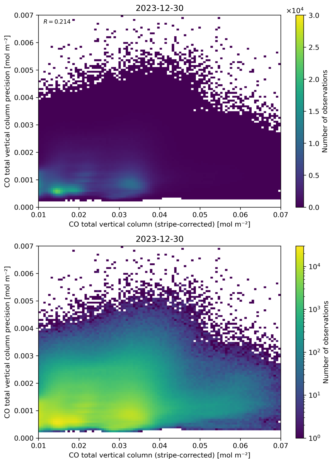
Figure 36: Scatter density plot of “CO total vertical column (stripe-corrected)” against “CO total vertical column precision” for 2023-12-30 to 2023-12-31.
