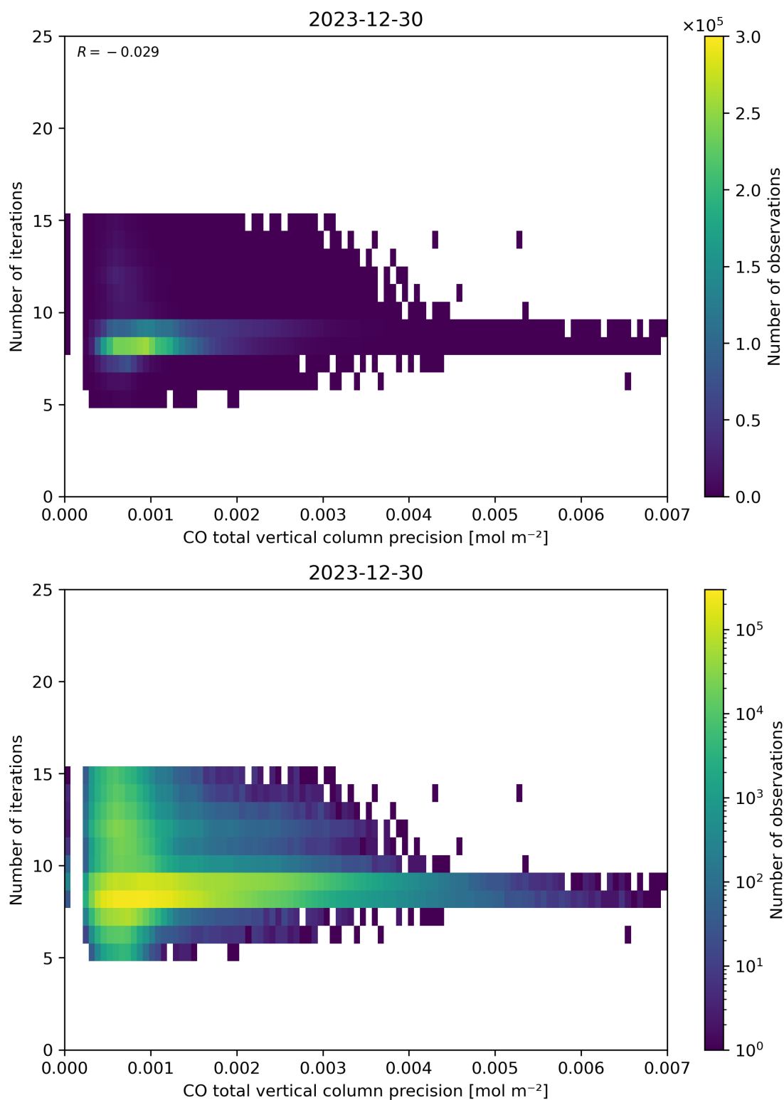
Figure 46: Scatter density plot of “CO total vertical column precision” against “Number of iterations” for 2023-12-30 to 2023-12-31.
