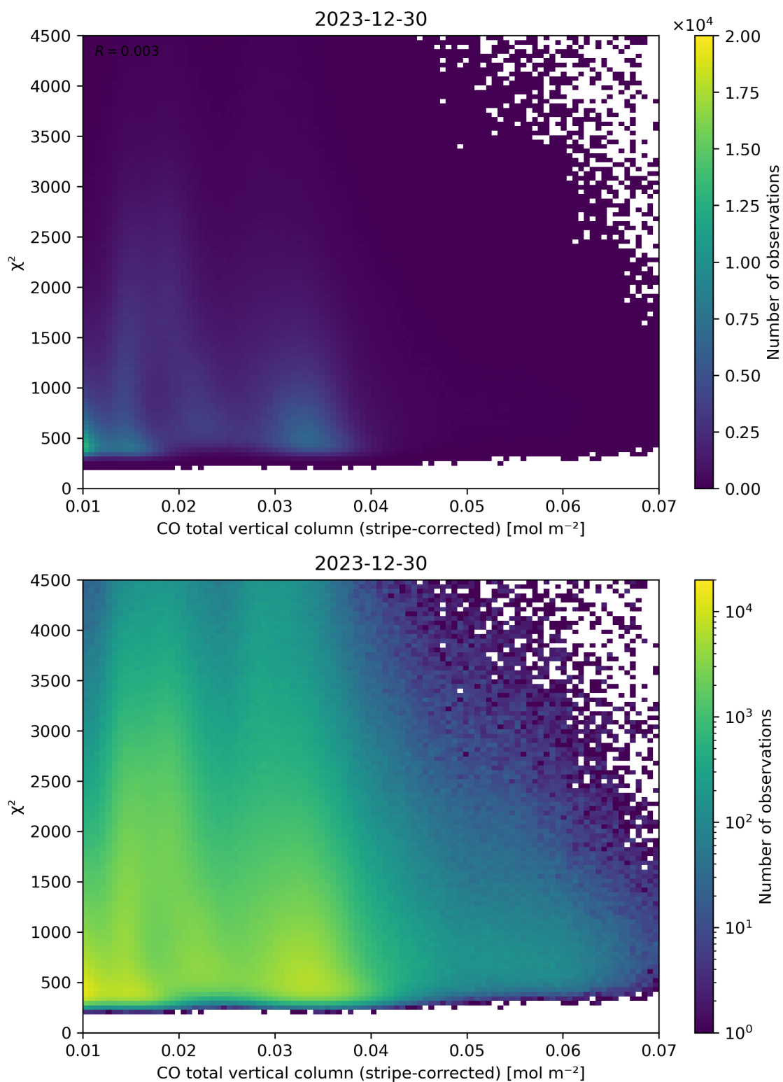
Figure 37: Scatter density plot of “CO total vertical column (stripe-corrected)” against “ \chi^2 ” for 2023-12-30 to 2023-12-31.
