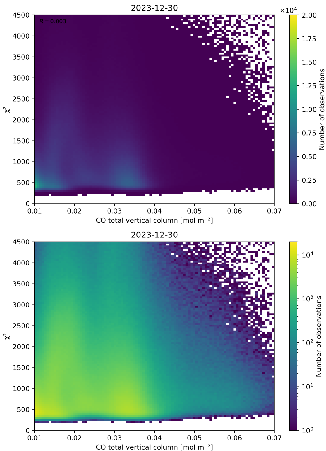
Figure 35: Scatter density plot of “CO total vertical column” against “ \chi^2 ” for 2023-12-30 to 2023-12-31.
