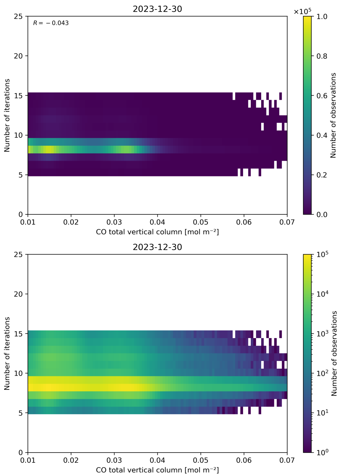
Figure 42: Scatter density plot of “CO total vertical column” against “Number of iterations” for 2023-12-30 to 2023-12-31.
