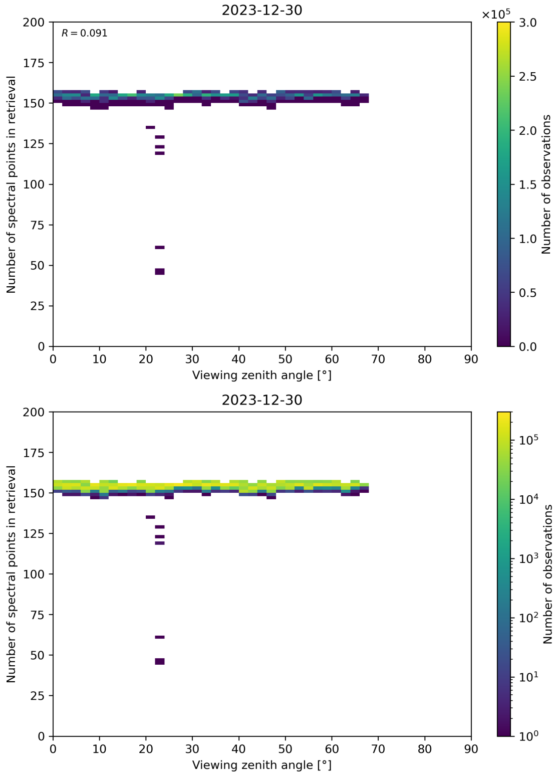
Figure 76: Scatter density plot of “Viewing zenith angle” against “Number of spectral points in retrieval” for 2023-12-30 to 2023-12-31.
