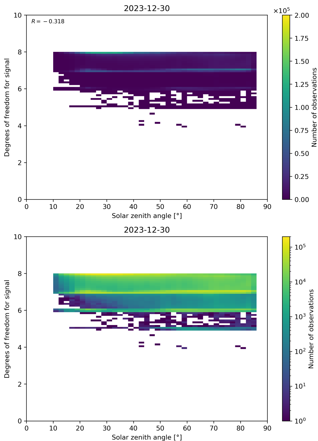
Figure 65: Scatter density plot of “Solar zenith angle” against “Degrees of freedom for signal” for 2023-12-30 to 2023-12-31.
