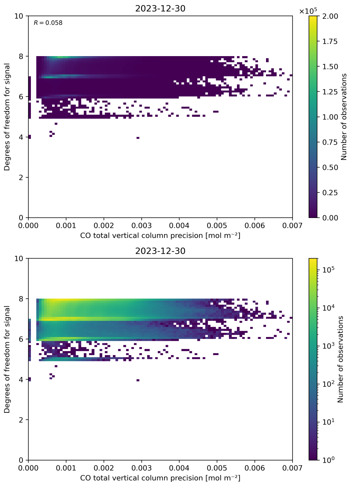
Figure 45: Scatter density plot of “CO total vertical column precision” against “Degrees of freedom for signal” for 2023-12-30 to 2023-12-31.
