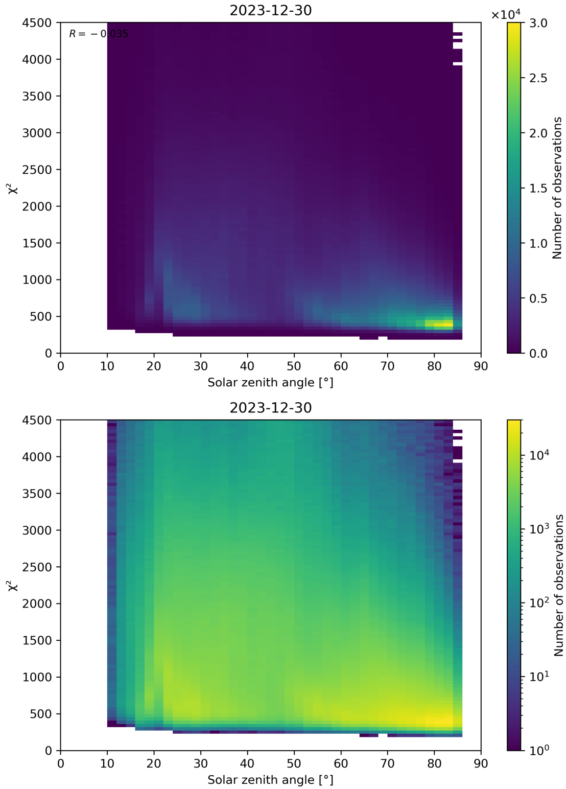
Figure 64: Scatter density plot of “Solar zenith angle” against “ \chi^2 ” for 2023-12-30 to 2023-12-31.
