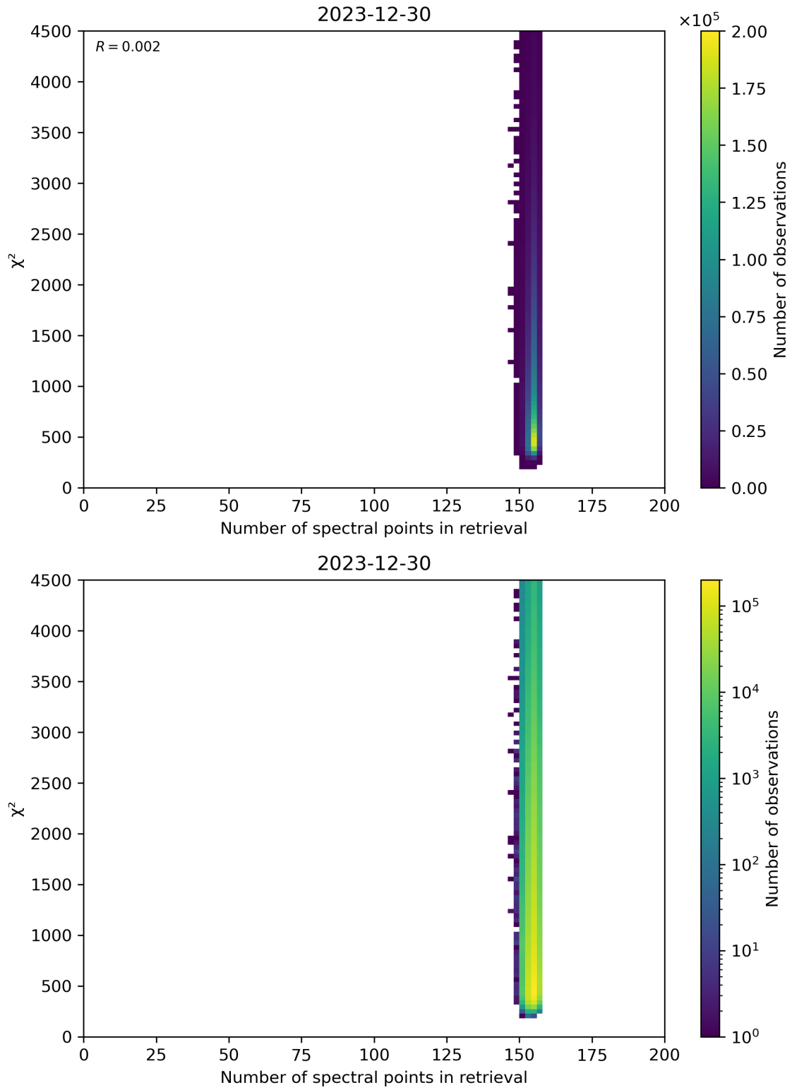
Figure 58: Scatter density plot of “Number of spectral points in retrieval” against “ \chi^2 ” for 2023-12-30 to 2023-12-31.
