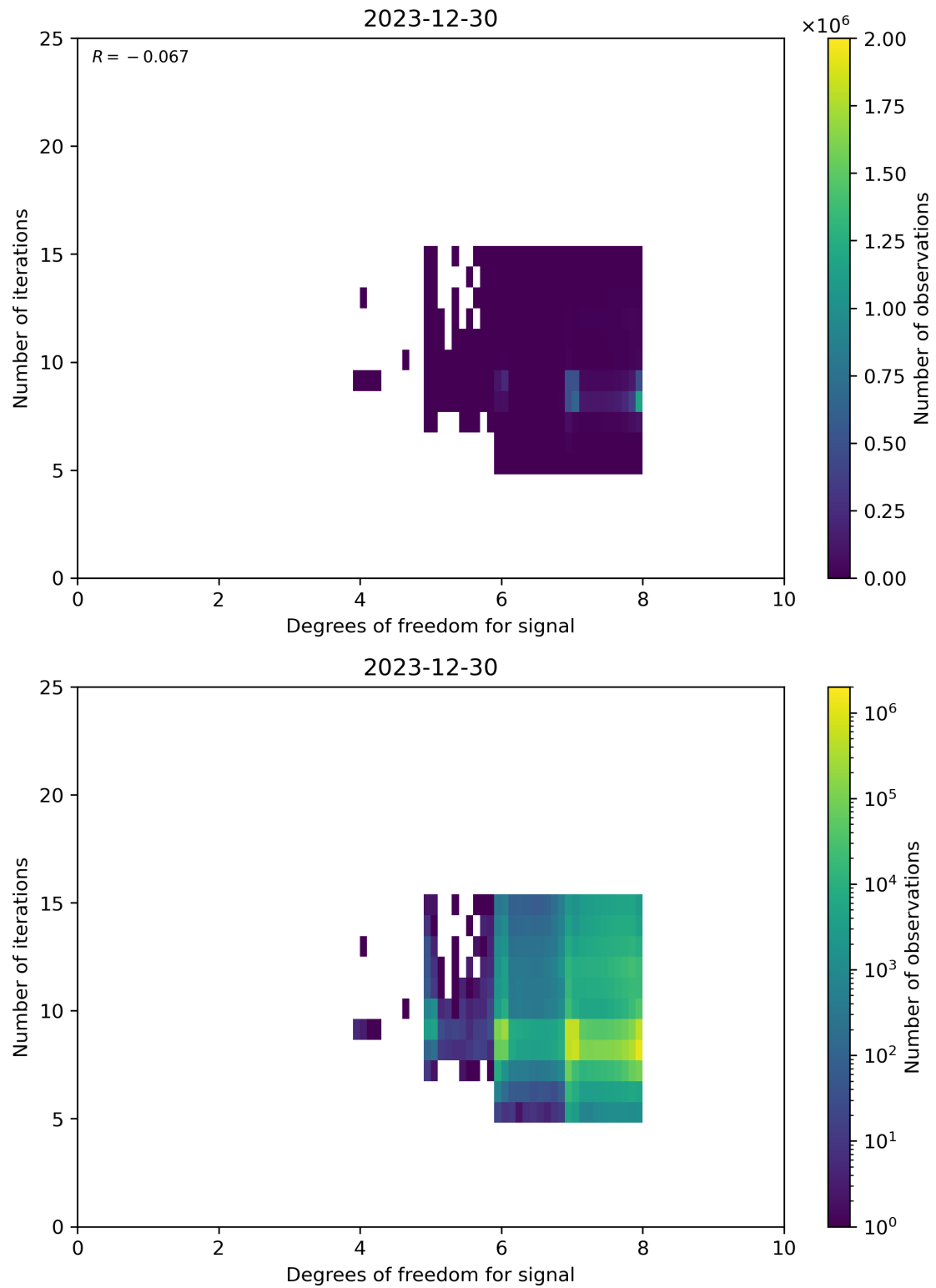
Figure 50: Scatter density plot of “Degrees of freedom for signal” against “Number of iterations” for 2023-12-30 to 2023-12-31.
