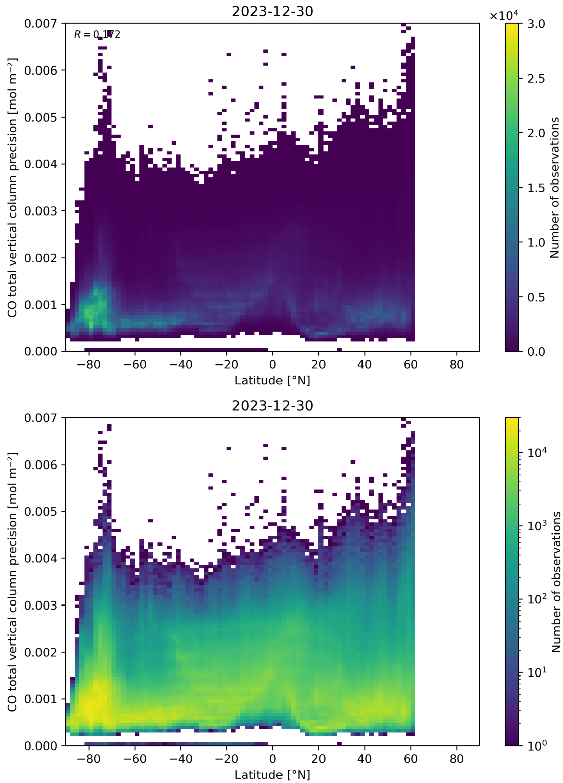
Figure 53: Scatter density plot of “Latitude” against “CO total vertical column precision” for 2023-12-30 to 2023-12-31.
