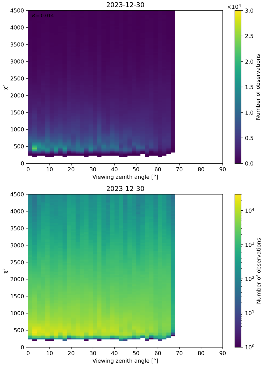
Figure 72: Scatter density plot of “Viewing zenith angle” against “ \chi^2 ” for 2023-12-30 to 2023-12-31.
