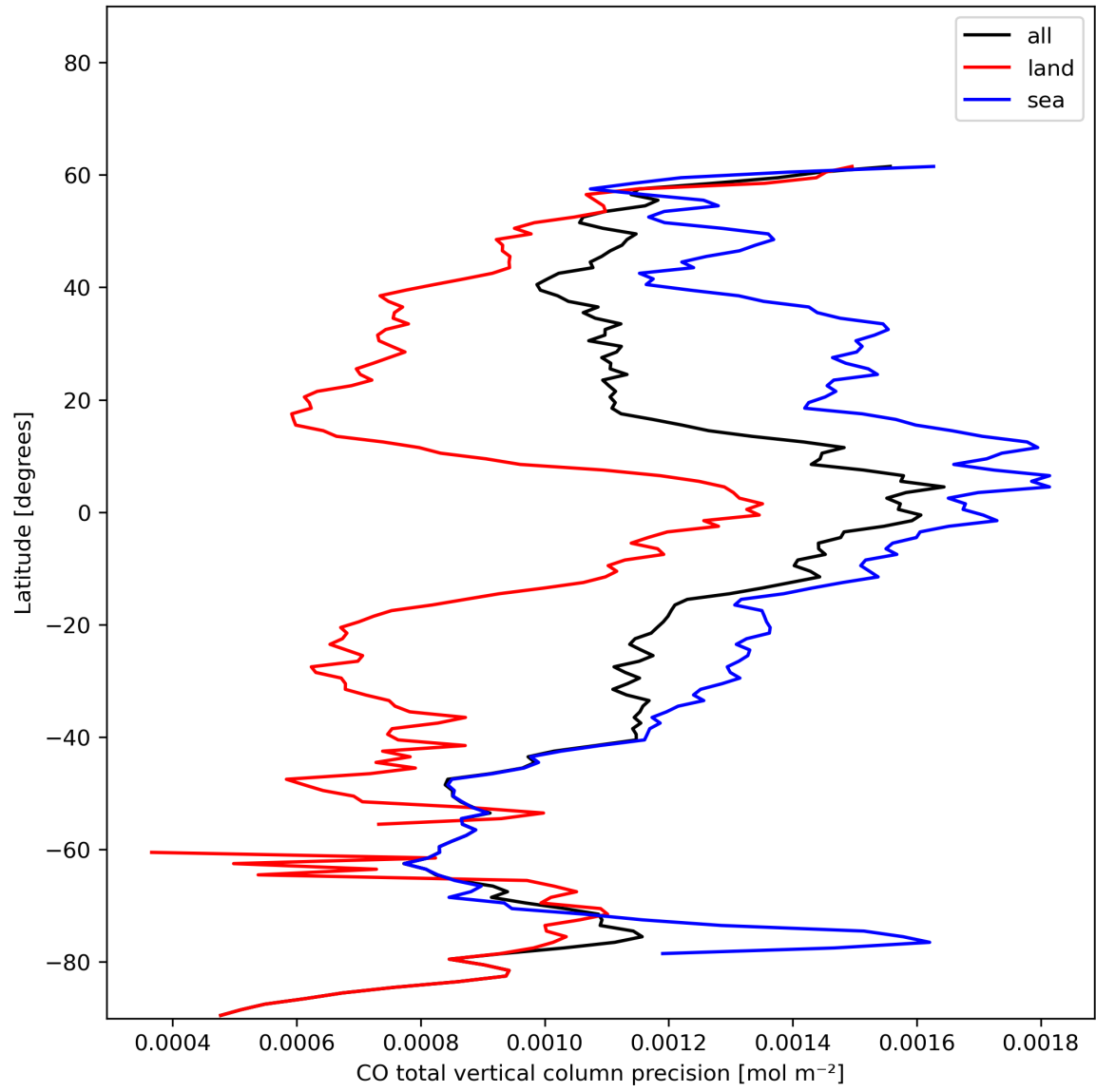
Figure 12: Zonal average of “CO total vertical column precision” for 2023-12-30 to 2023-12-31.
