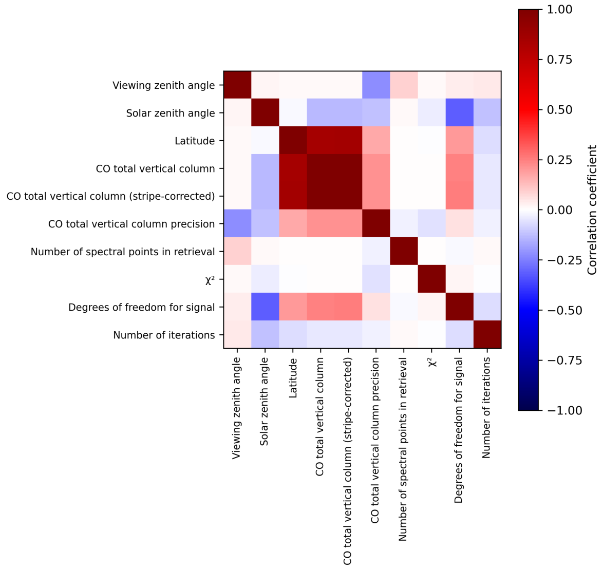
Figure 2: Map of correlation matrix for 2023-12-30 to 2023-12-31.
