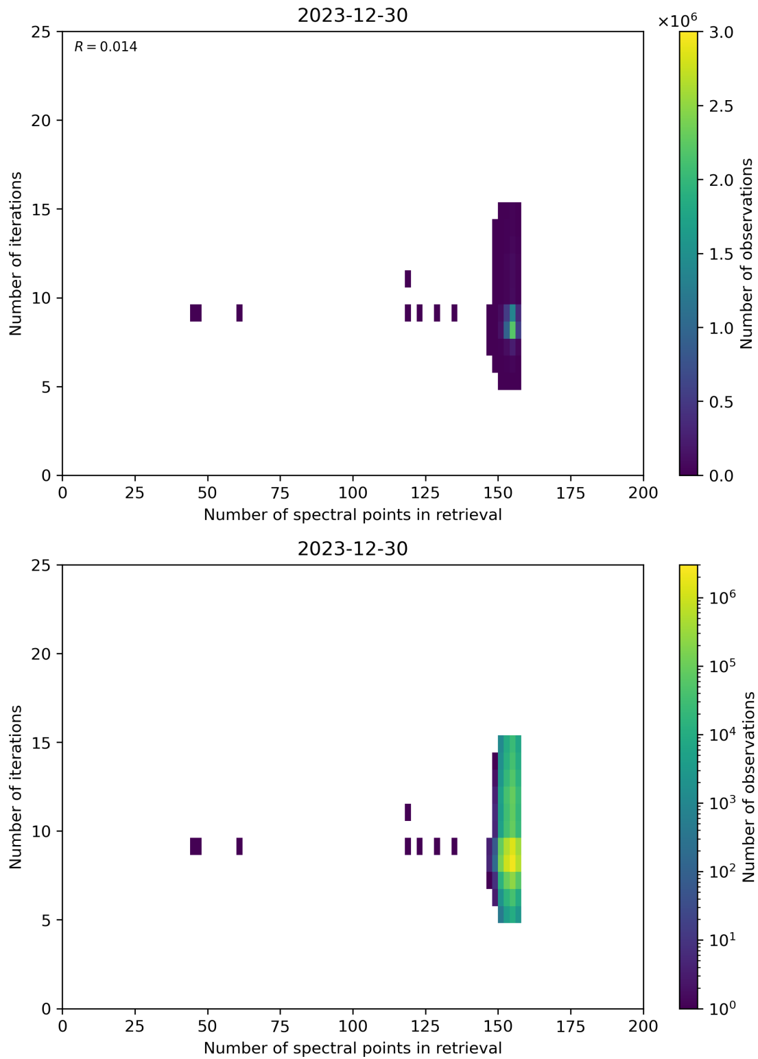
Figure 60: Scatter density plot of “Number of spectral points in retrieval” against “Number of iterations” for 2023-12-30 to 2023-12-31.
