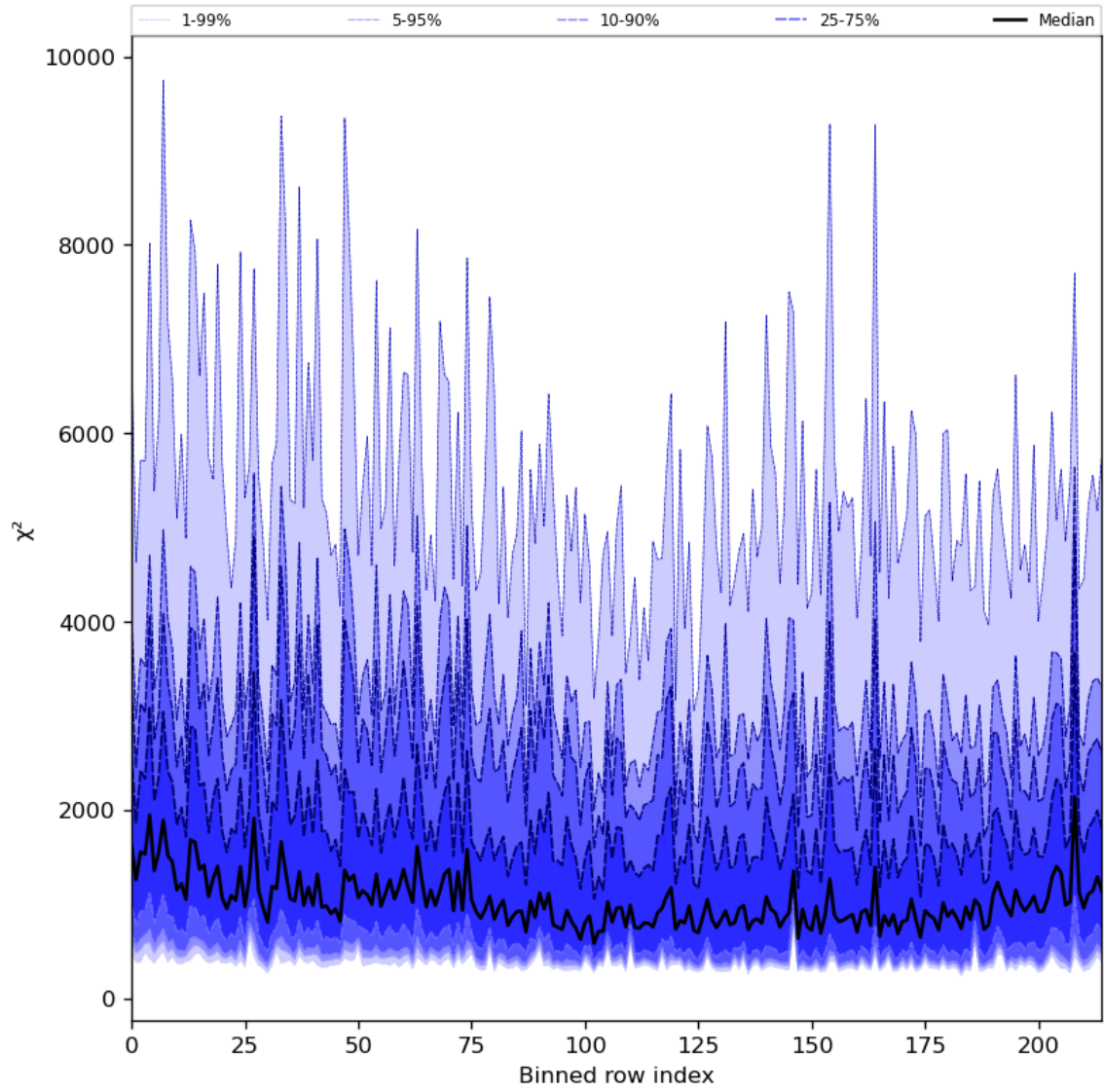
Figure 30: Along track statistics of “ \chi^2 ” for 2023-12-30 to 2023-12-31
