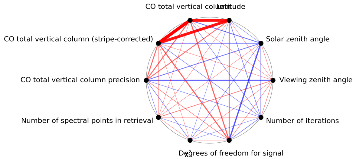
Figure 1: Map of correlation graph for 2023-12-30 to 2023-12-31.
