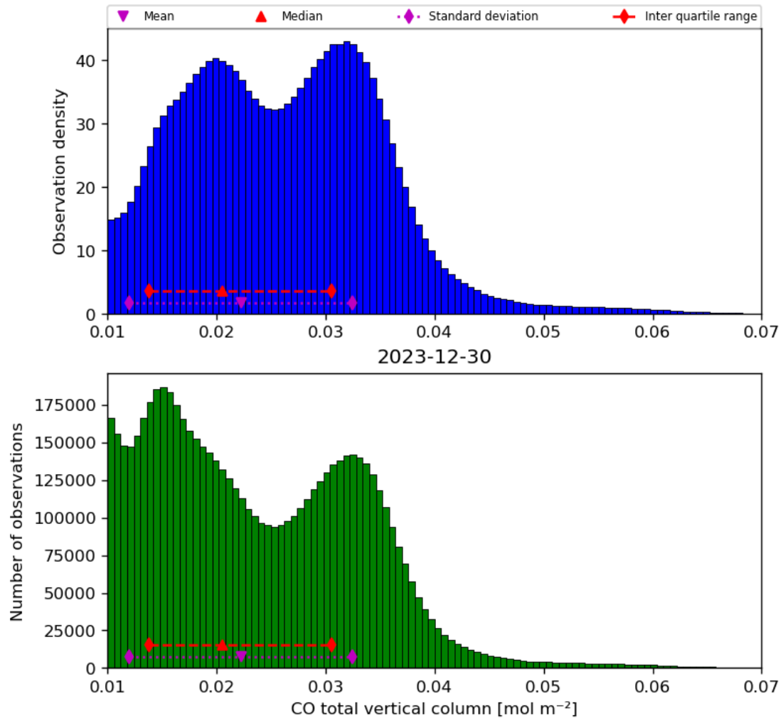
Figure 18: Histogram of “CO total vertical column” for 2023-12-30 to 2023-12-31
