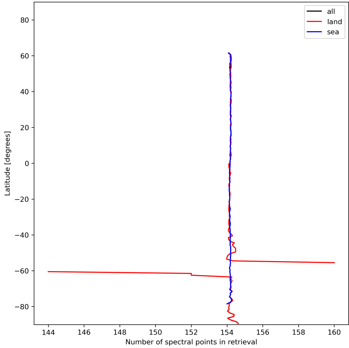
Figure 13: Zonal average of “Number of spectral points in retrieval” for 2023-12-30 to 2023-12-31.
