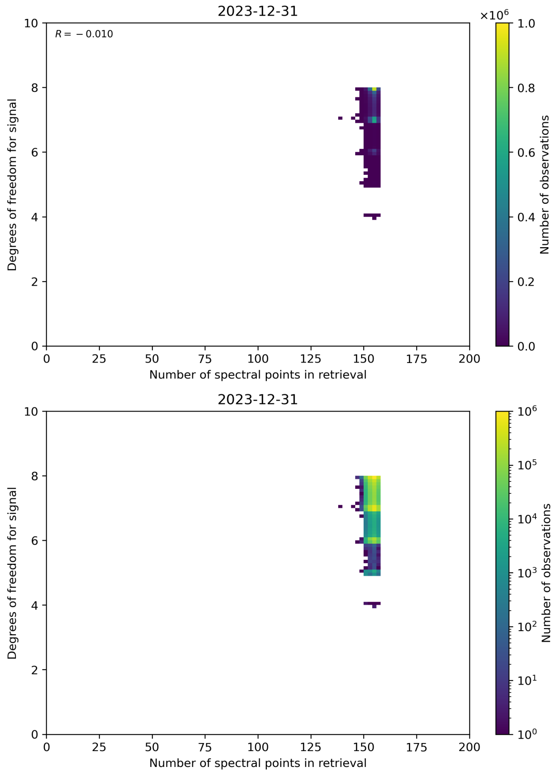
Figure 59: Scatter density plot of “Number of spectral points in retrieval” against “Degrees of freedom for signal” for 2023-12-30 to 2023-12-31.
