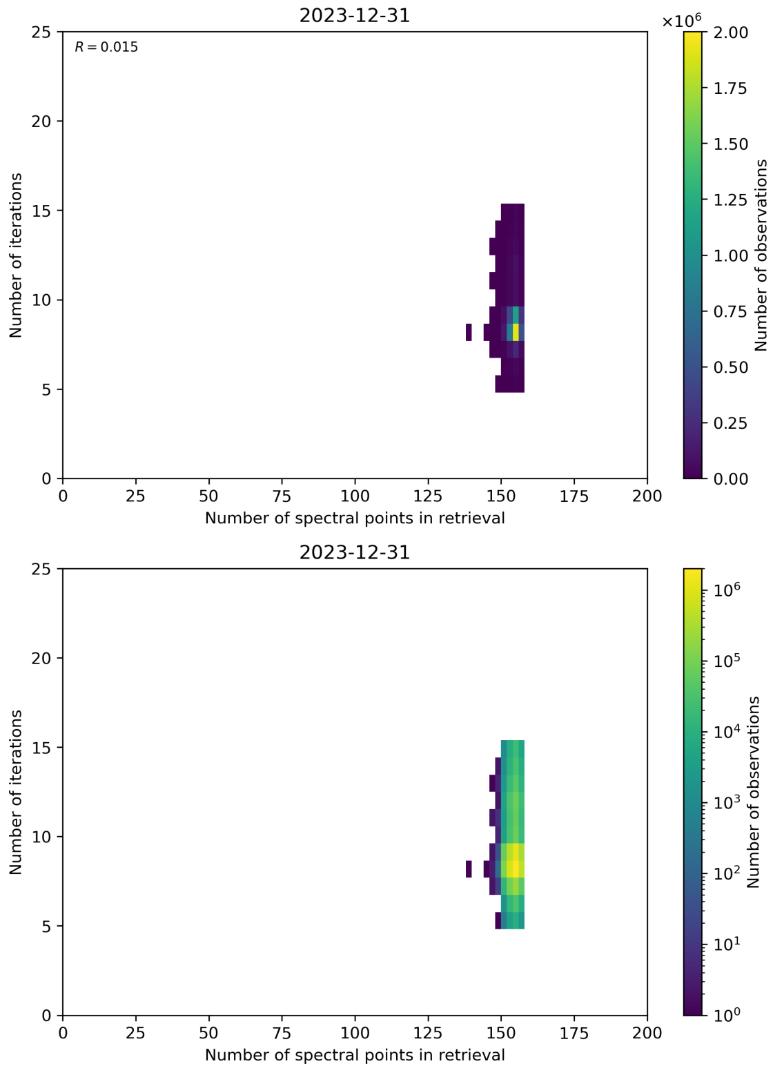
Figure 60: Scatter density plot of “Number of spectral points in retrieval” against “Number of iterations” for 2023-12-30 to 2023-12-31.
