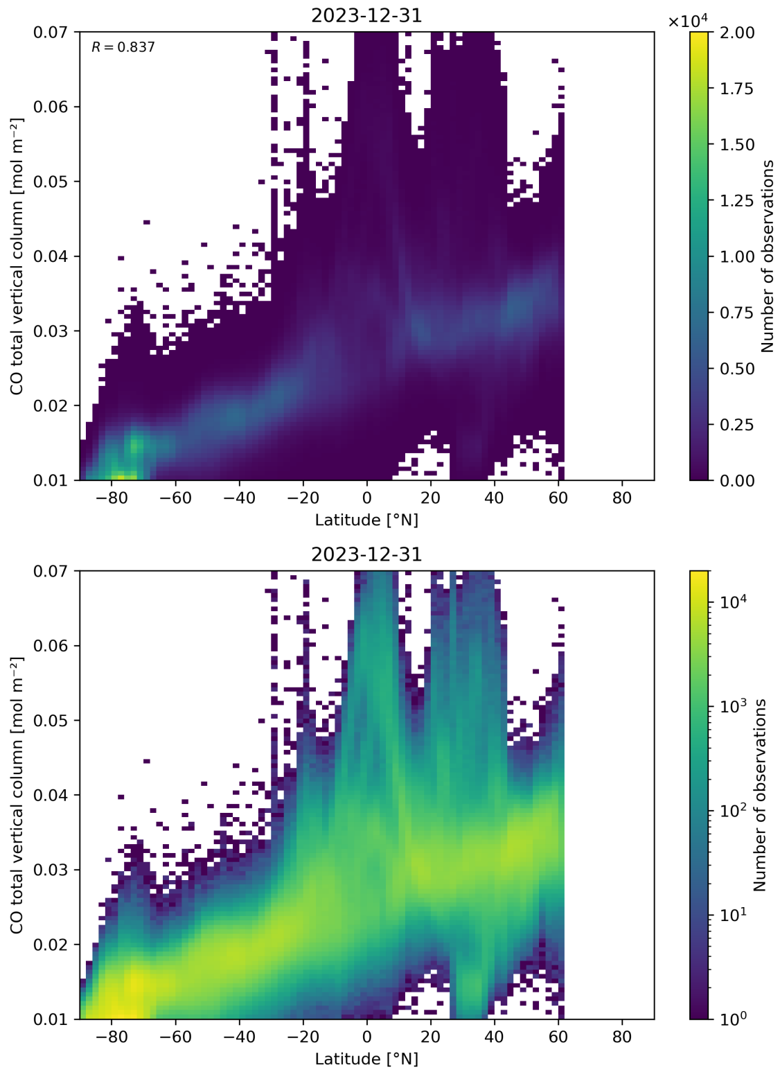
Figure 51: Scatter density plot of “Latitude” against “CO total vertical column” for 2023-12-30 to 2023-12-31.
