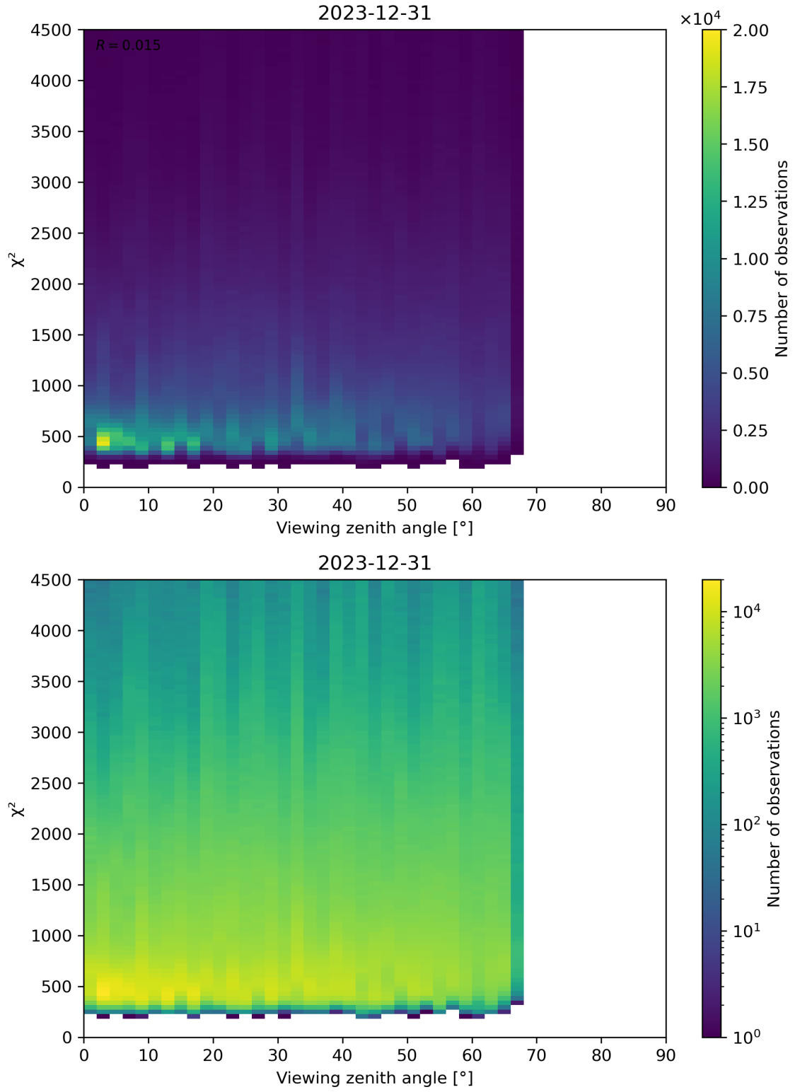
Figure 72: Scatter density plot of “Viewing zenith angle” against “ \chi^2 ” for 2023-12-30 to 2023-12-31.
