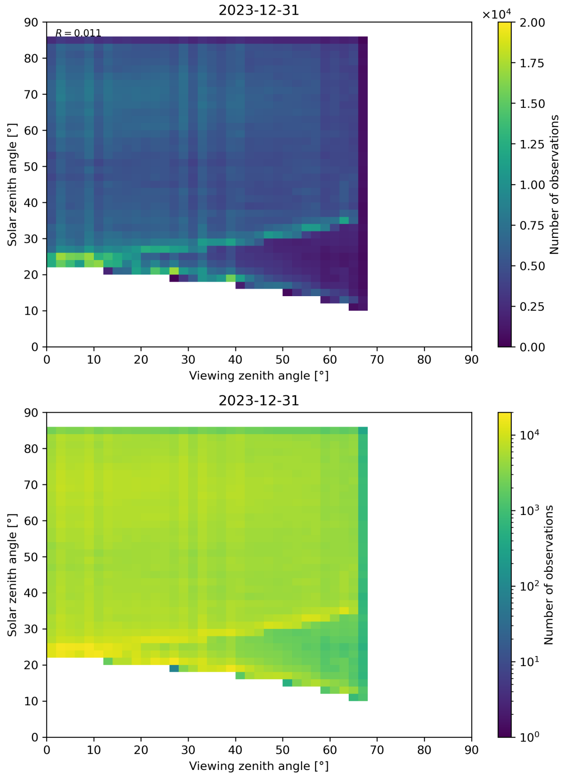
Figure 77: Scatter density plot of “Viewing zenith angle” against “Solar zenith angle” for 2023-12-30 to 2023-12-31.
