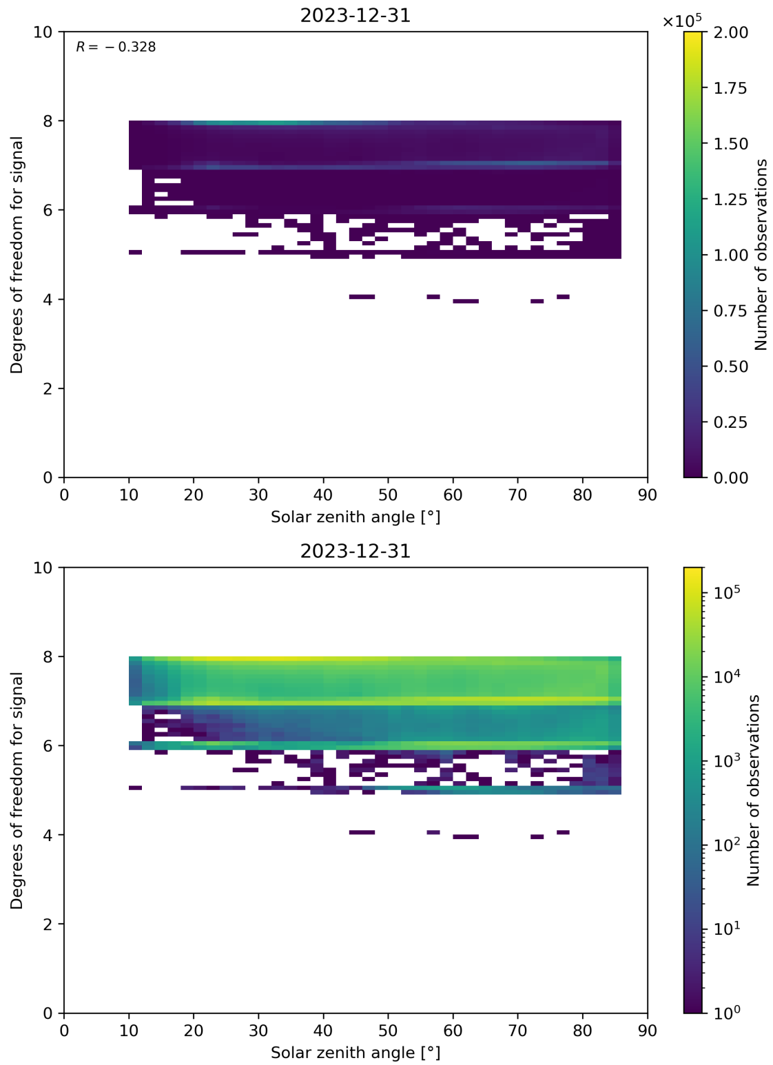
Figure 65: Scatter density plot of “Solar zenith angle” against “Degrees of freedom for signal” for 2023-12-30 to 2023-12-31.
