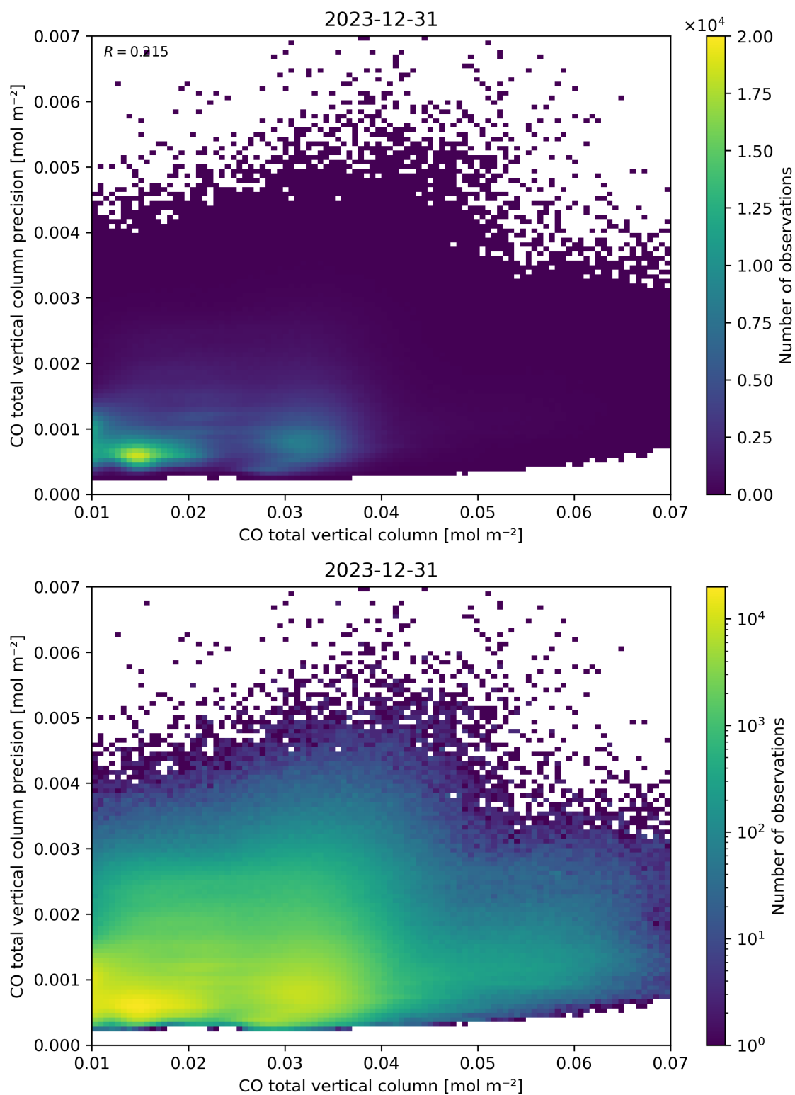
Figure 34: Scatter density plot of “CO total vertical column” against “CO total vertical column precision” for 2023-12-30 to 2023-12-31.
