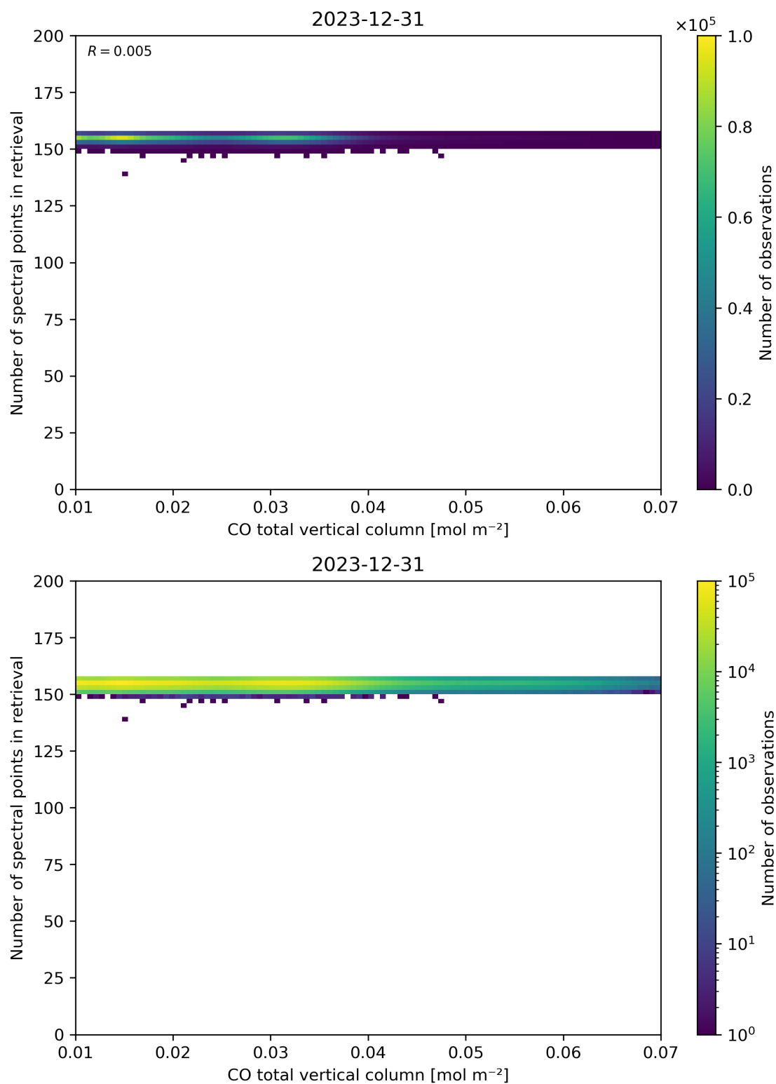
Figure 43: Scatter density plot of “CO total vertical column” against “Number of spectral points in retrieval” for 2023-12-30 to 2023-12-31.
