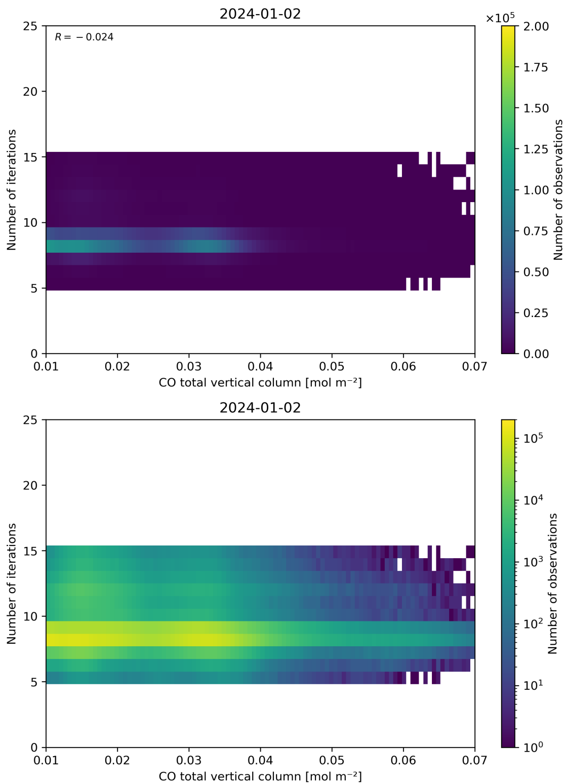
Figure 42: Scatter density plot of “CO total vertical column” against “Number of iterations” for 2024-01-01 to 2024-01-03.
