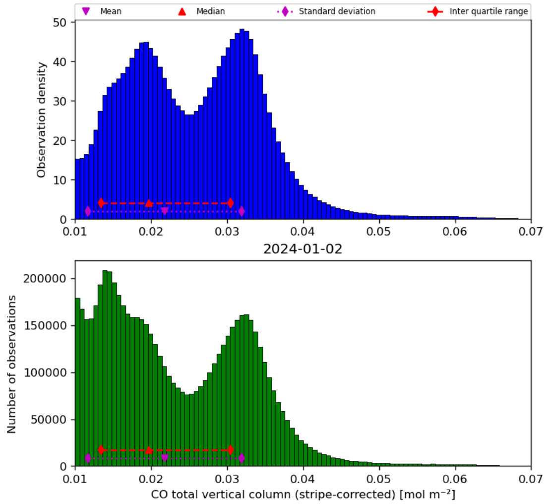
Figure 19: Histogram of “CO total vertical column (stripe-corrected)” for 2024-01-01 to 2024-01-03
