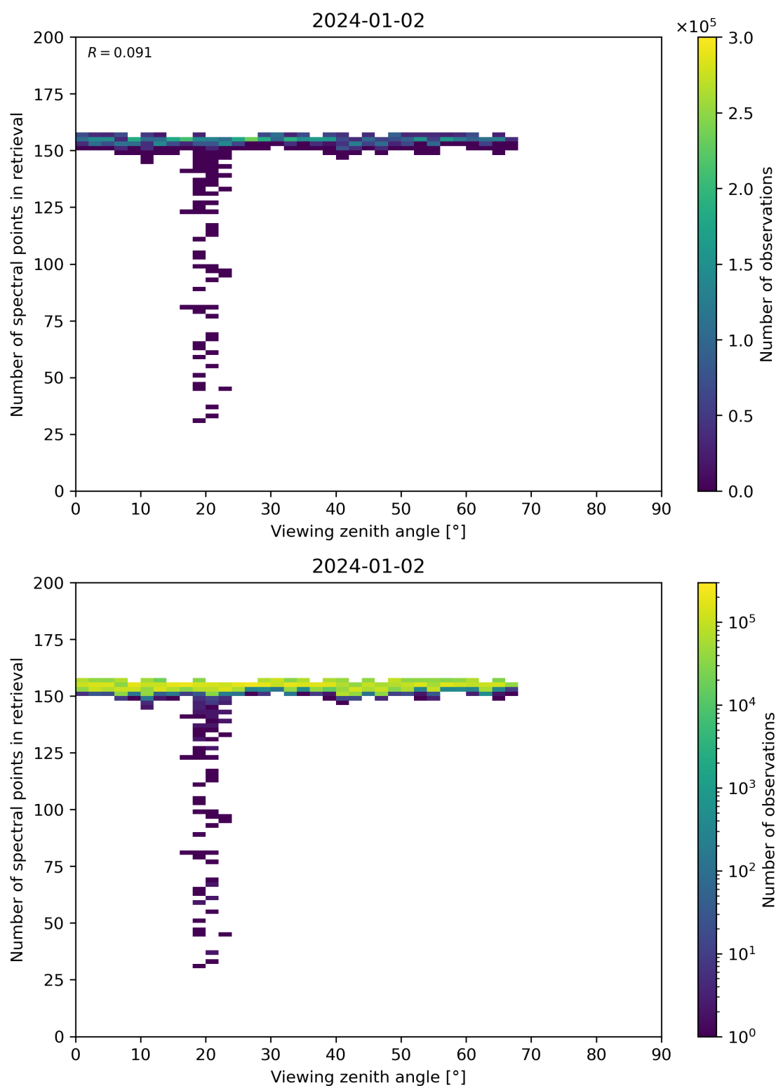
Figure 76: Scatter density plot of “Viewing zenith angle” against “Number of spectral points in retrieval” for 2024-01-01 to 2024-01-03.
