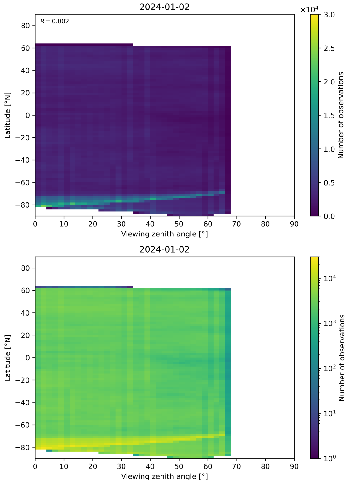
Figure 74: Scatter density plot of “Viewing zenith angle” against “Latitude” for 2024-01-01 to 2024-01-03.
