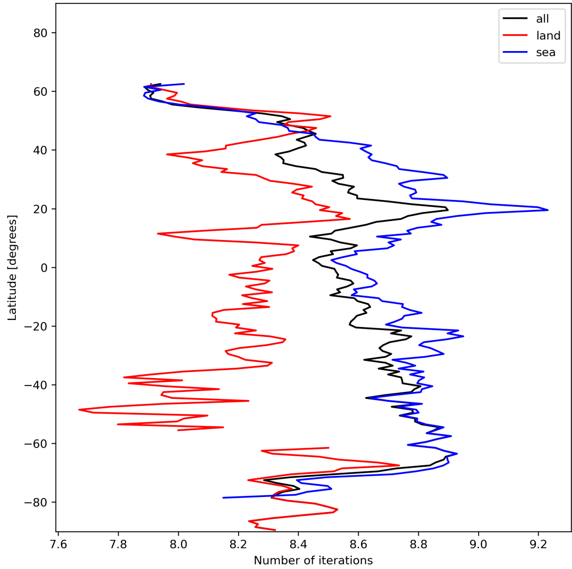
Figure 16: Zonal average of “Number of iterations” for 2024-01-01 to 2024-01-03.
