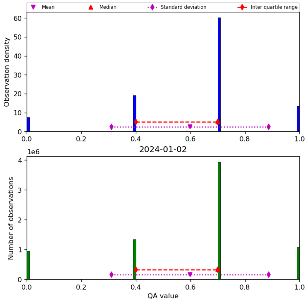
Figure 17: Histogram of “QA value” for 2024-01-01 to 2024-01-03
