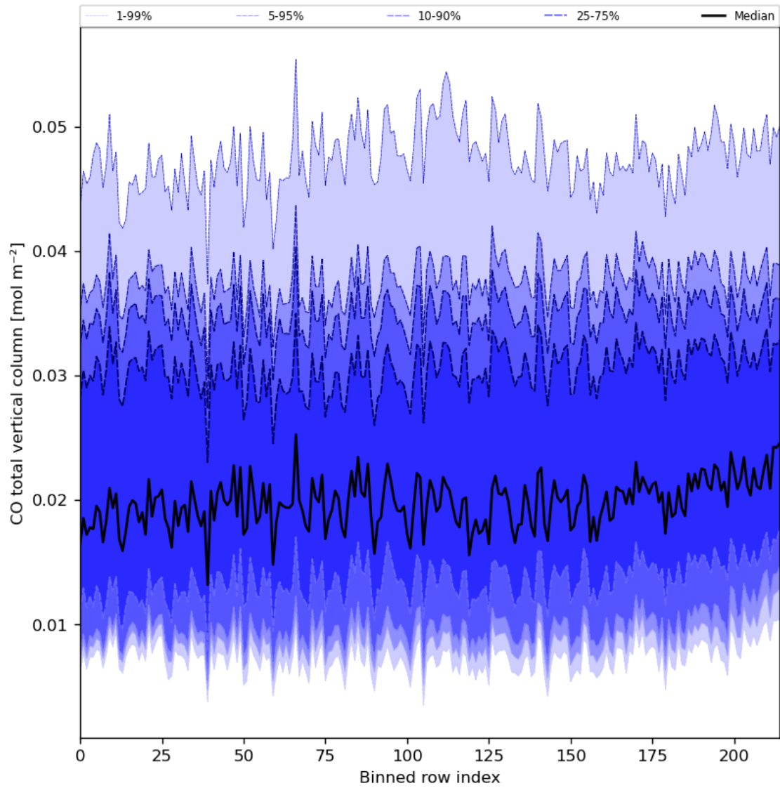
Figure 26: Along track statistics of “CO total vertical column” for 2024-01-01 to 2024-01-03
