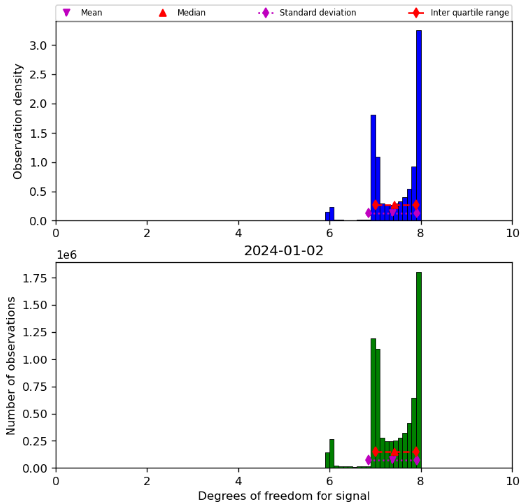
Figure 23: Histogram of “Degrees of freedom for signal” for 2024-01-01 to 2024-01-03
