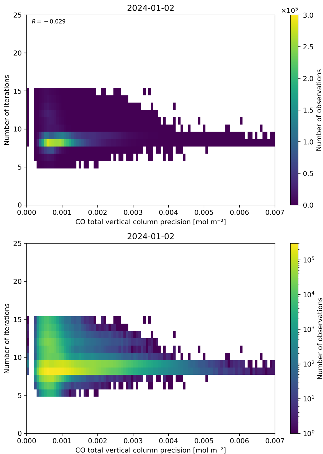
Figure 46: Scatter density plot of “CO total vertical column precision” against “Number of iterations” for 2024-01-01 to 2024-01-03.
