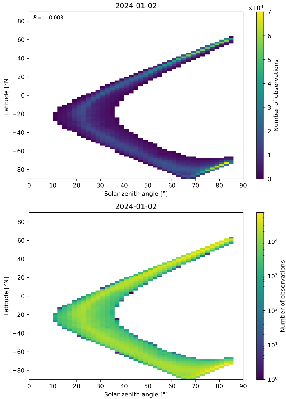
Figure 66: Scatter density plot of “Solar zenith angle” against “Latitude” for 2024-01-01 to 2024-01-03.
