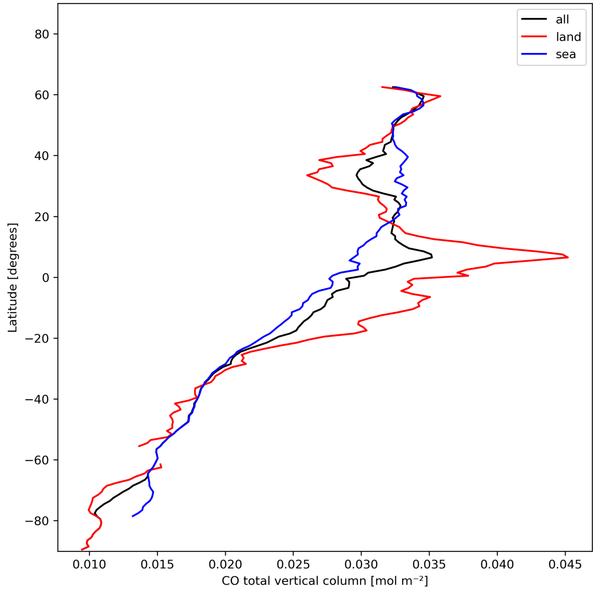
Figure 10: Zonal average of “CO total vertical column” for 2024-01-01 to 2024-01-03.
