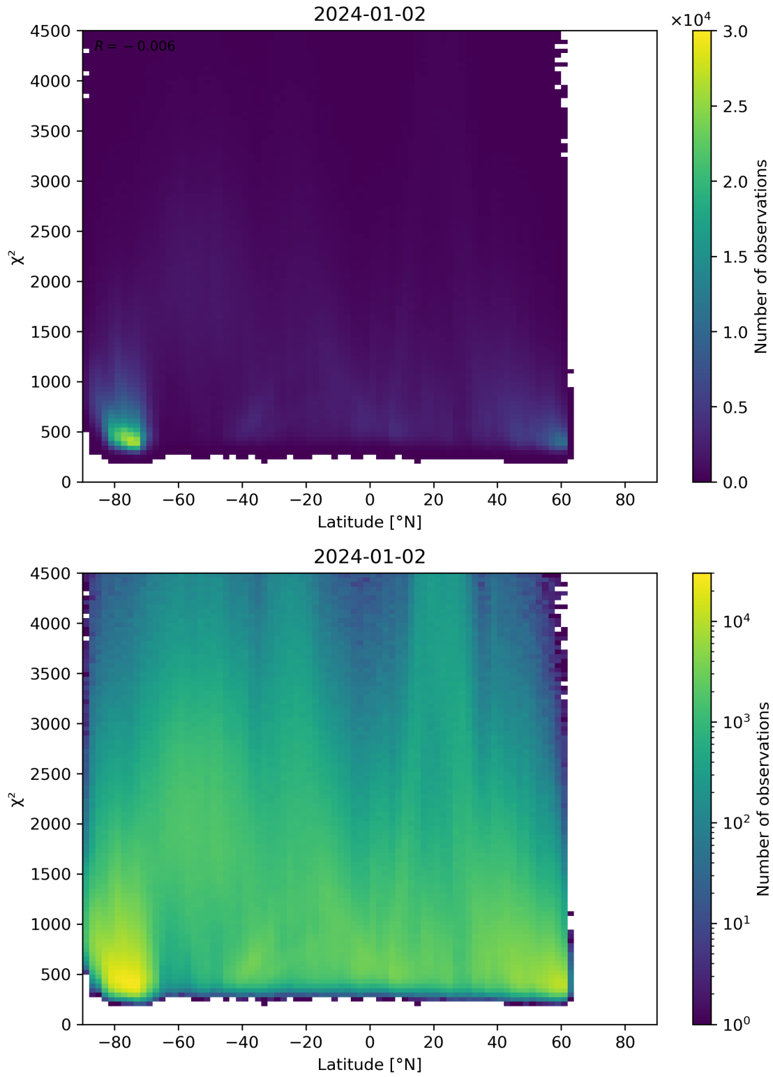
Figure 54: Scatter density plot of “Latitude” against “ \chi^2 ” for 2024-01-01 to 2024-01-03.
