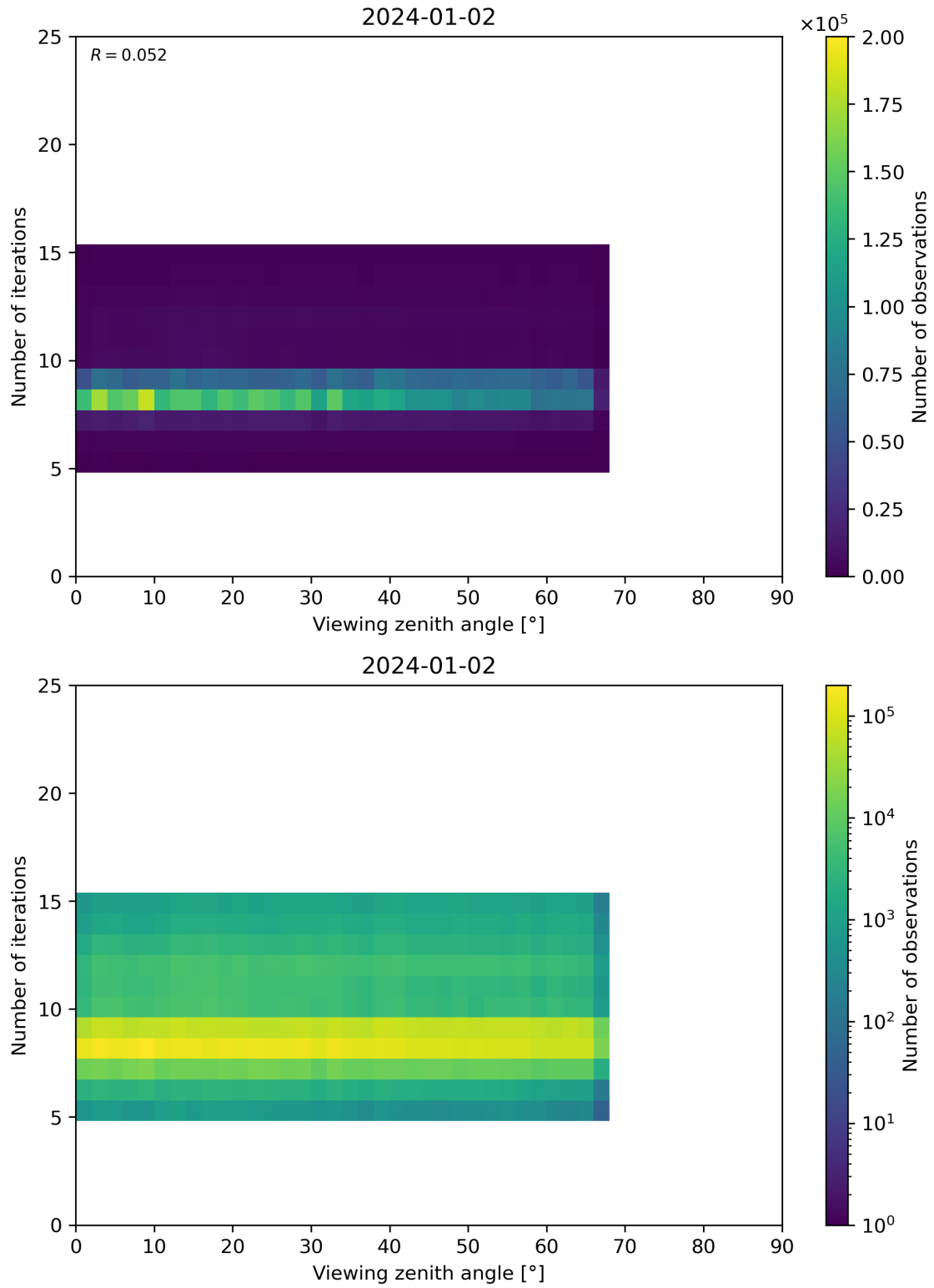
Figure 75: Scatter density plot of “Viewing zenith angle” against “Number of iterations” for 2024-01-01 to 2024-01-03.
