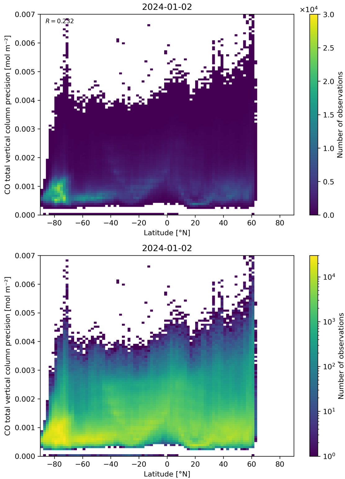
Figure 53: Scatter density plot of “Latitude” against “CO total vertical column precision” for 2024-01-01 to 2024-01-03.
