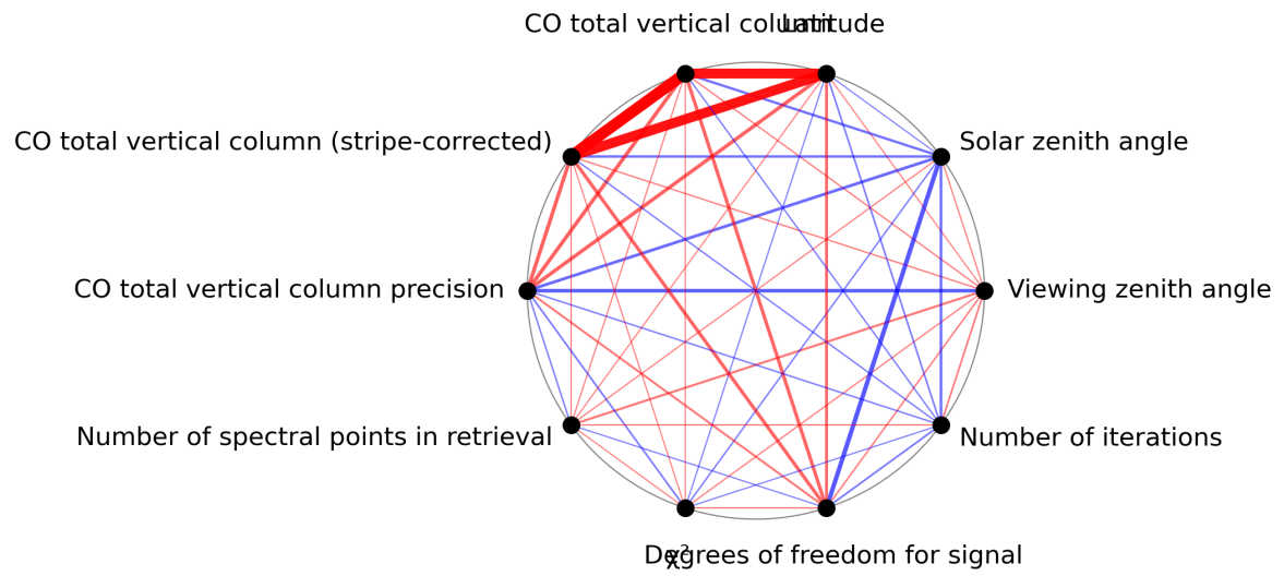
Figure 1: Map of correlation graph for 2024-01-01 to 2024-01-03.
