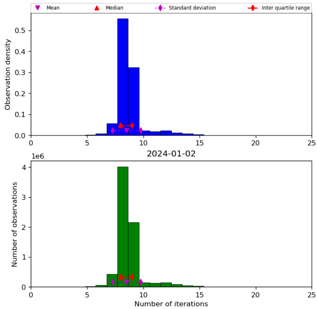
Figure 24: Histogram of “Number of iterations” for 2024-01-01 to 2024-01-03
