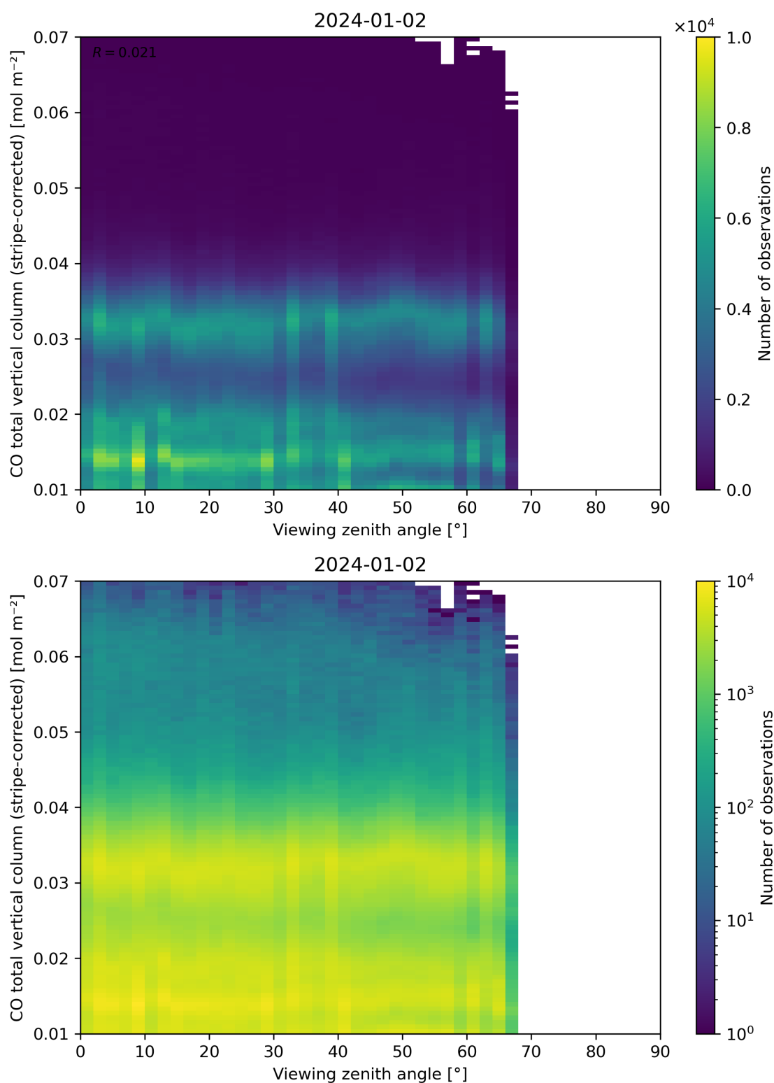
Figure 70: Scatter density plot of “Viewing zenith angle” against “CO total vertical column (stripe-corrected)” for 2024-01-01 to 2024-01-03.
