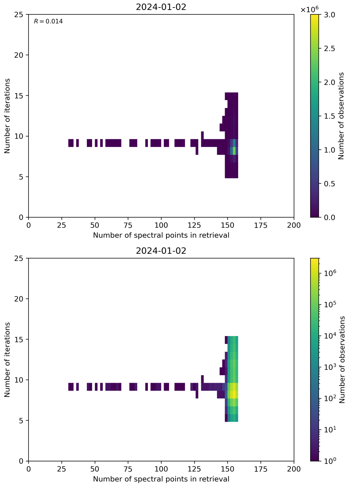
Figure 60: Scatter density plot of “Number of spectral points in retrieval” against “Number of iterations” for 2024-01-01 to 2024-01-03.
