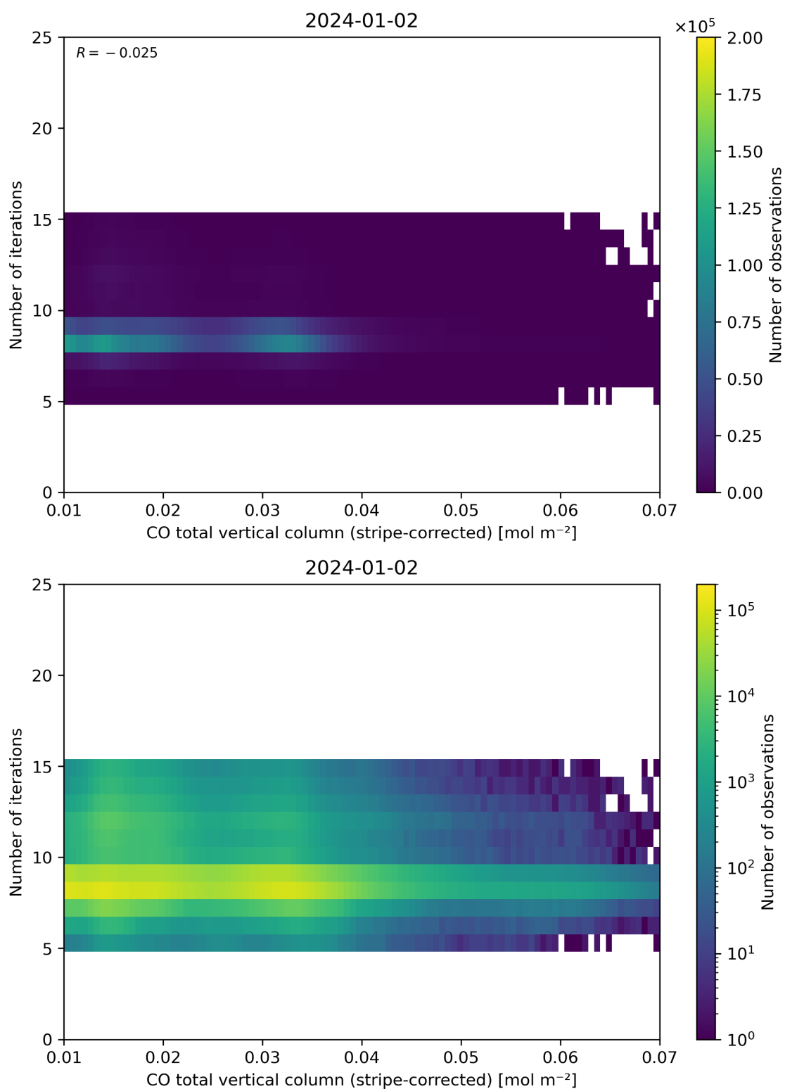
Figure 39: Scatter density plot of “CO total vertical column (stripe-corrected)” against “Number of iterations” for 2024-01-01 to 2024-01-03.
