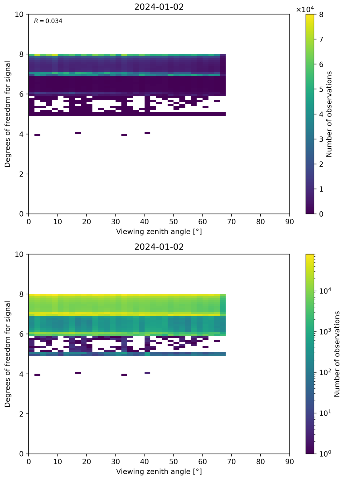
Figure 73: Scatter density plot of “Viewing zenith angle” against “Degrees of freedom for signal” for 2024-01-01 to 2024-01-03.
