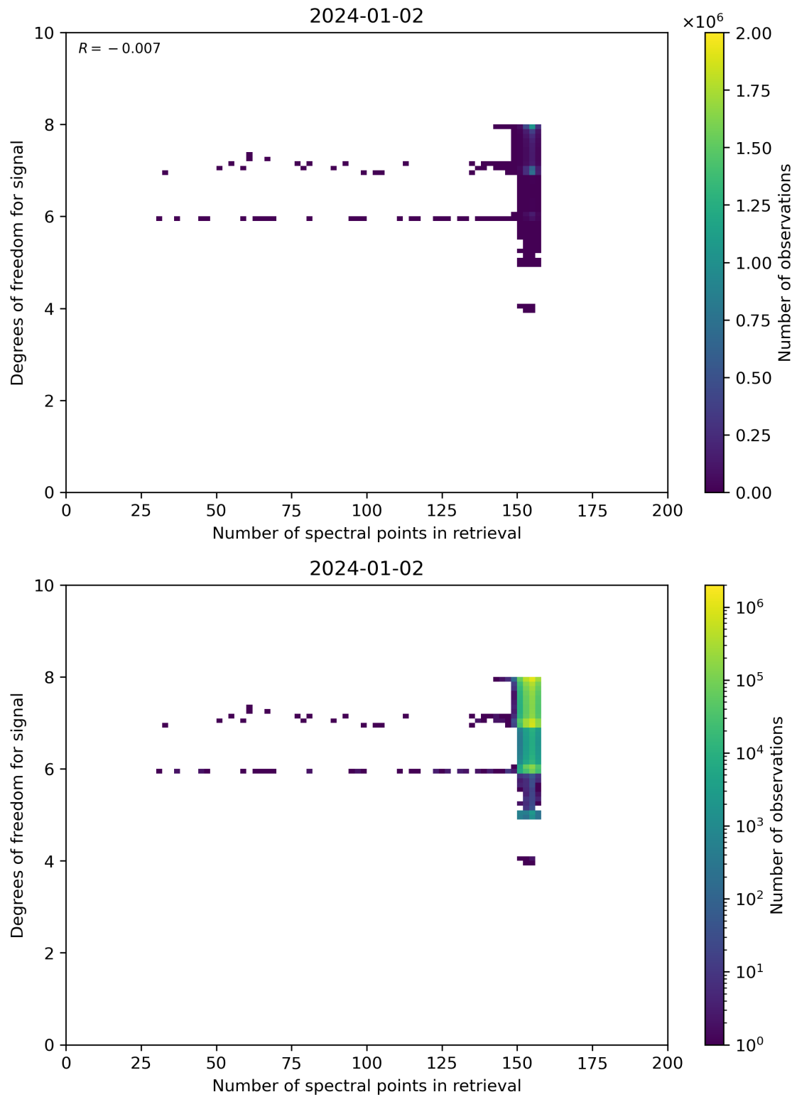
Figure 59: Scatter density plot of “Number of spectral points in retrieval” against “Degrees of freedom for signal” for 2024-01-01 to 2024-01-03.
