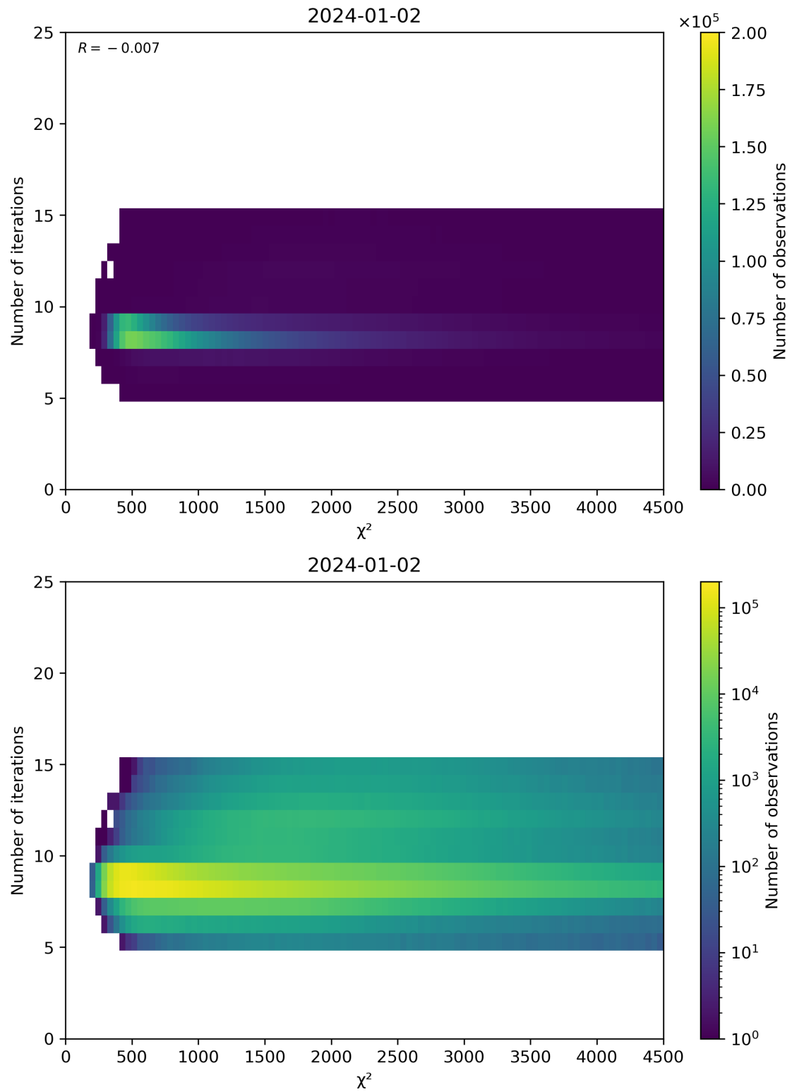
Figure 49: Scatter density plot of “ \chi^2 ” against “Number of iterations” for 2024-01-01 to 2024-01-03.
