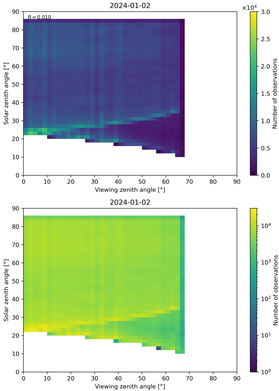
Figure 77: Scatter density plot of “Viewing zenith angle” against “Solar zenith angle” for 2024-01-01 to 2024-01-03.
