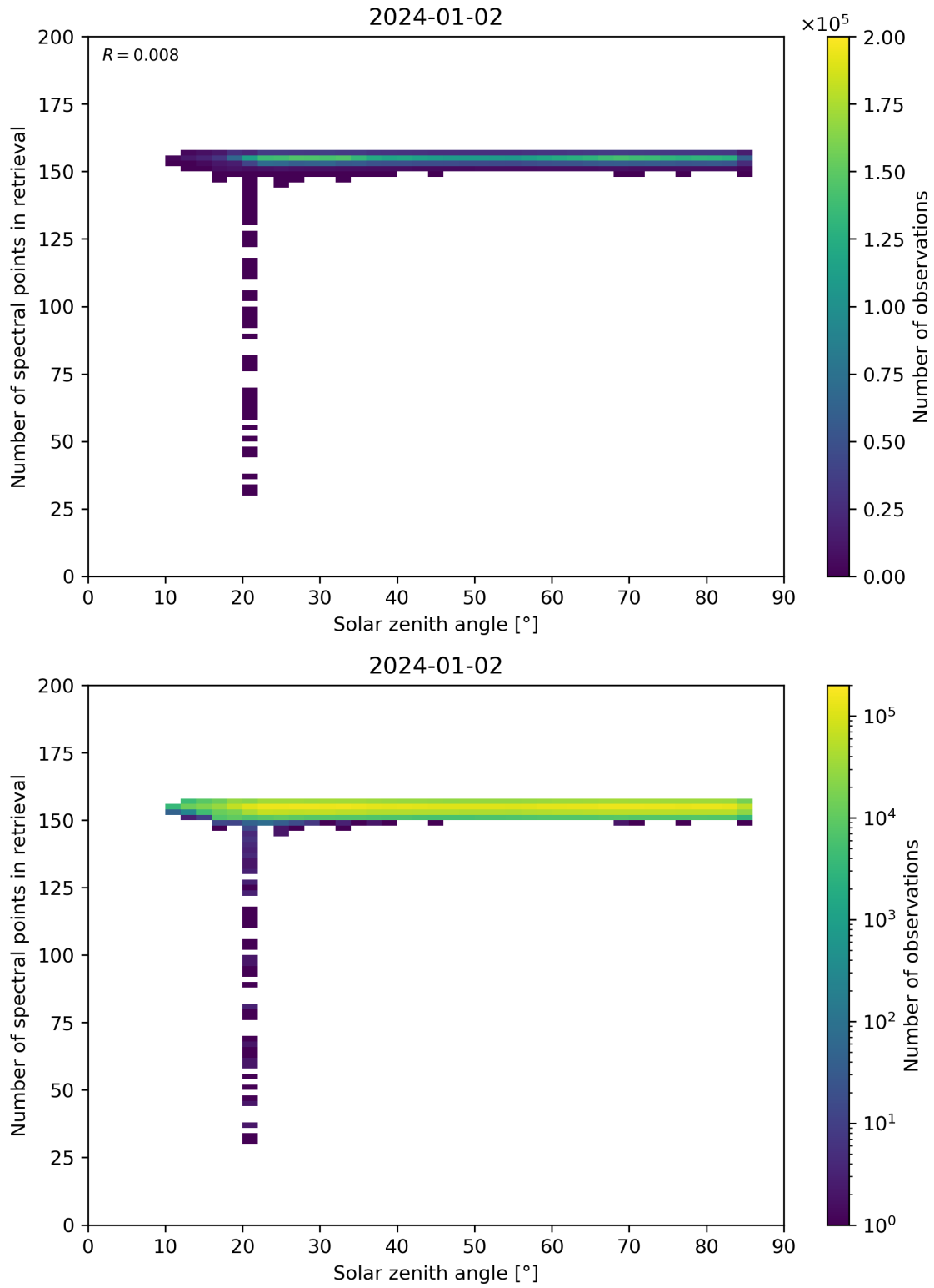
Figure 68: Scatter density plot of “Solar zenith angle” against “Number of spectral points in retrieval” for 2024-01-01 to 2024-01-03.
