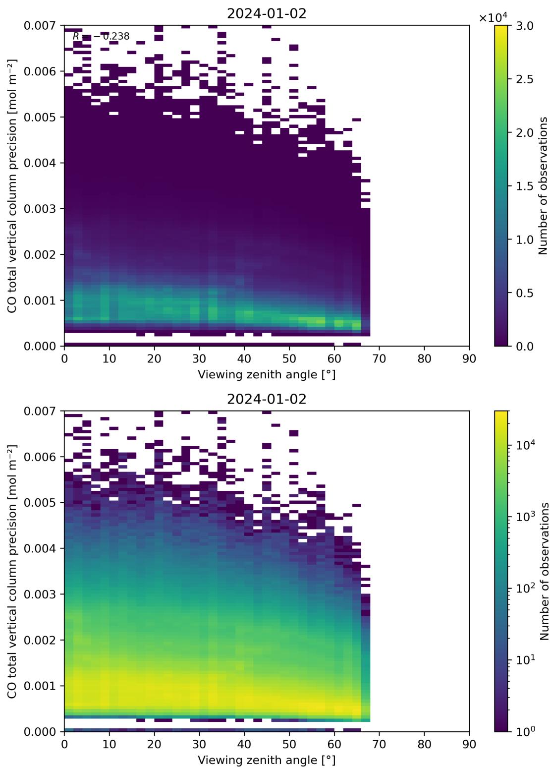
Figure 71: Scatter density plot of “Viewing zenith angle” against “CO total vertical column precision” for 2024-01-01 to 2024-01-03.
