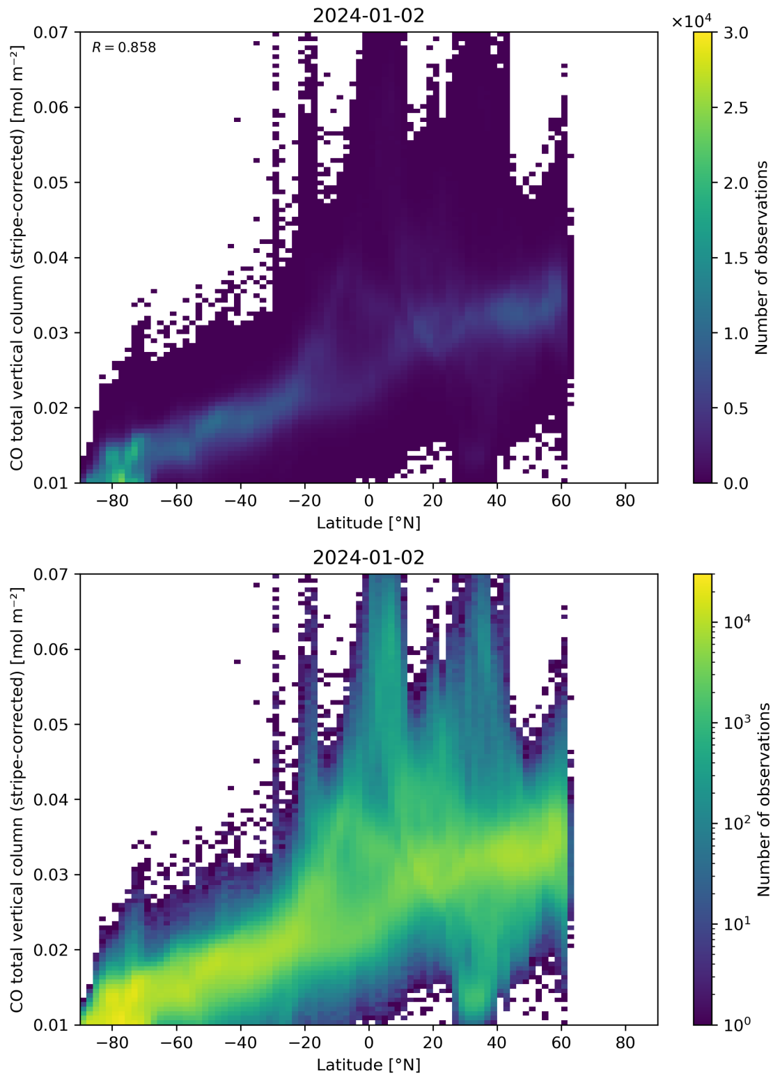
Figure 52: Scatter density plot of “Latitude” against “CO total vertical column (stripe-corrected)” for 2024-01-01 to 2024-01-03.
