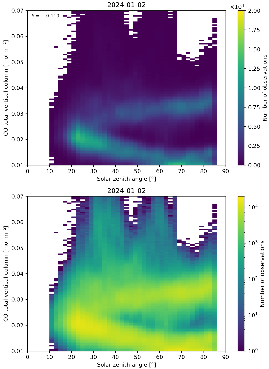
Figure 61: Scatter density plot of “Solar zenith angle” against “CO total vertical column” for 2024-01-01 to 2024-01-03.
