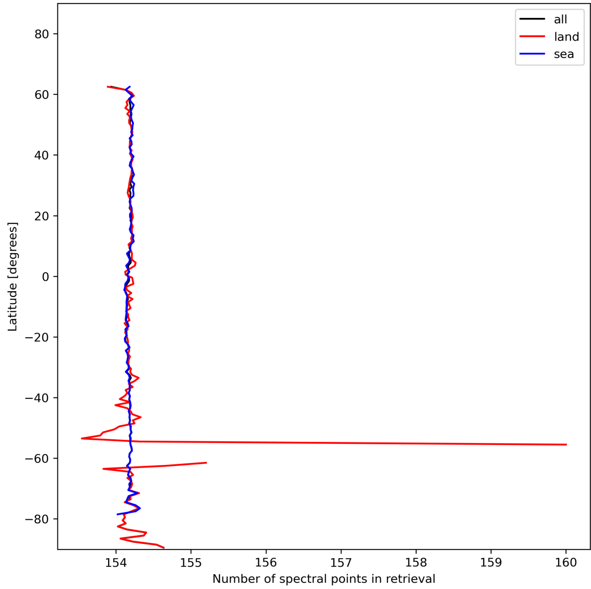
Figure 13: Zonal average of “Number of spectral points in retrieval” for 2024-01-01 to 2024-01-03.
