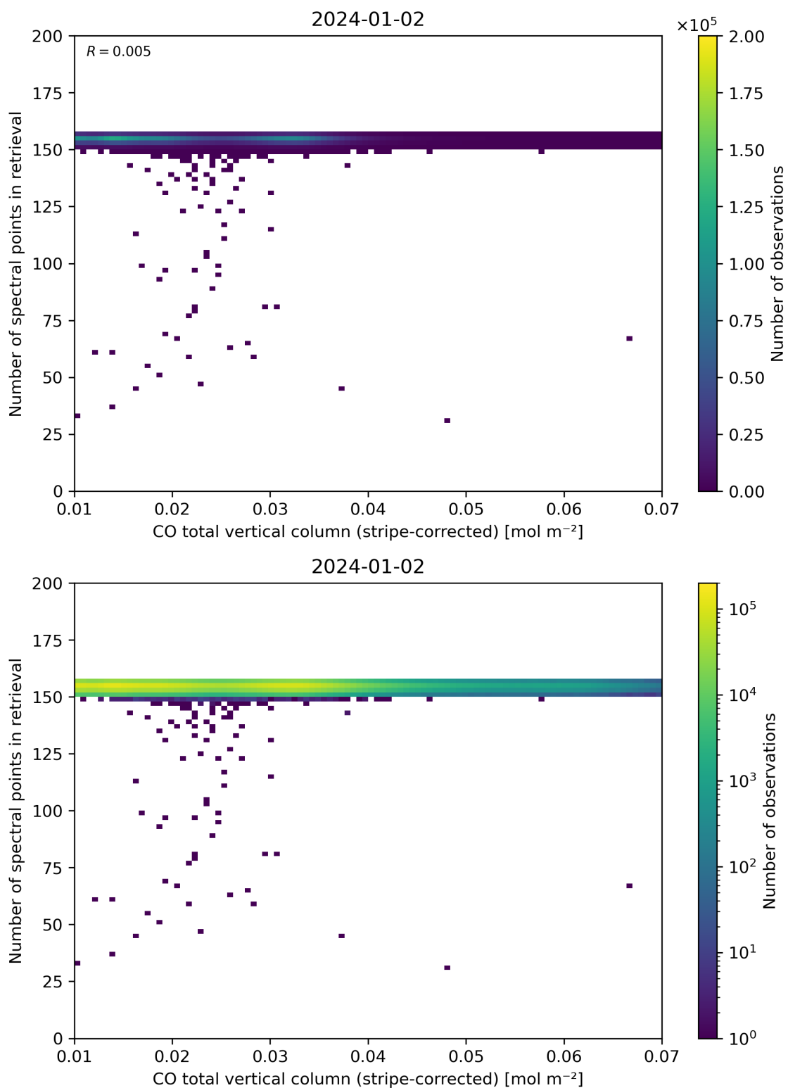
Figure 40: Scatter density plot of “CO total vertical column (stripe-corrected)” against “Number of spectral points in retrieval” for 2024-01-01 to 2024-01-03.
