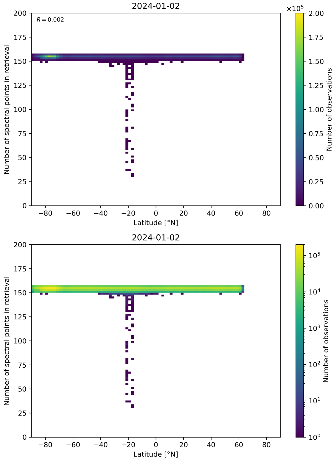
Figure 57: Scatter density plot of “Latitude” against “Number of spectral points in retrieval” for 2024-01-01 to 2024-01-03.
