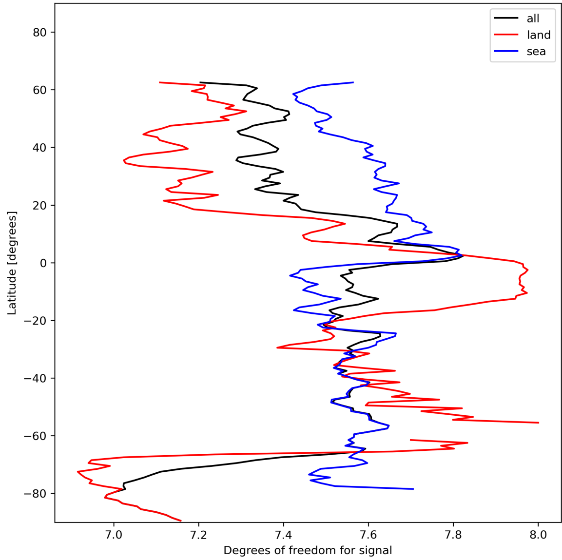
Figure 15: Zonal average of “Degrees of freedom for signal” for 2024-01-01 to 2024-01-03.
