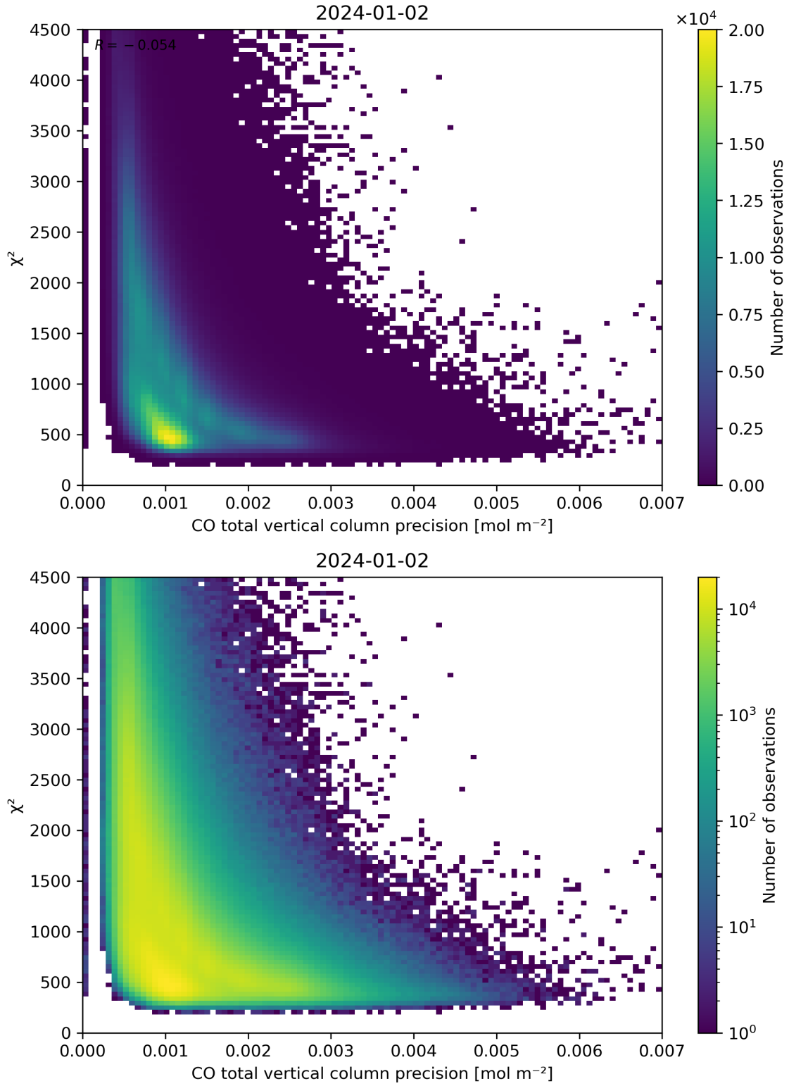
Figure 44: Scatter density plot of “CO total vertical column precision” against “ \chi^2 ” for 2024-01-01 to 2024-01-03.
