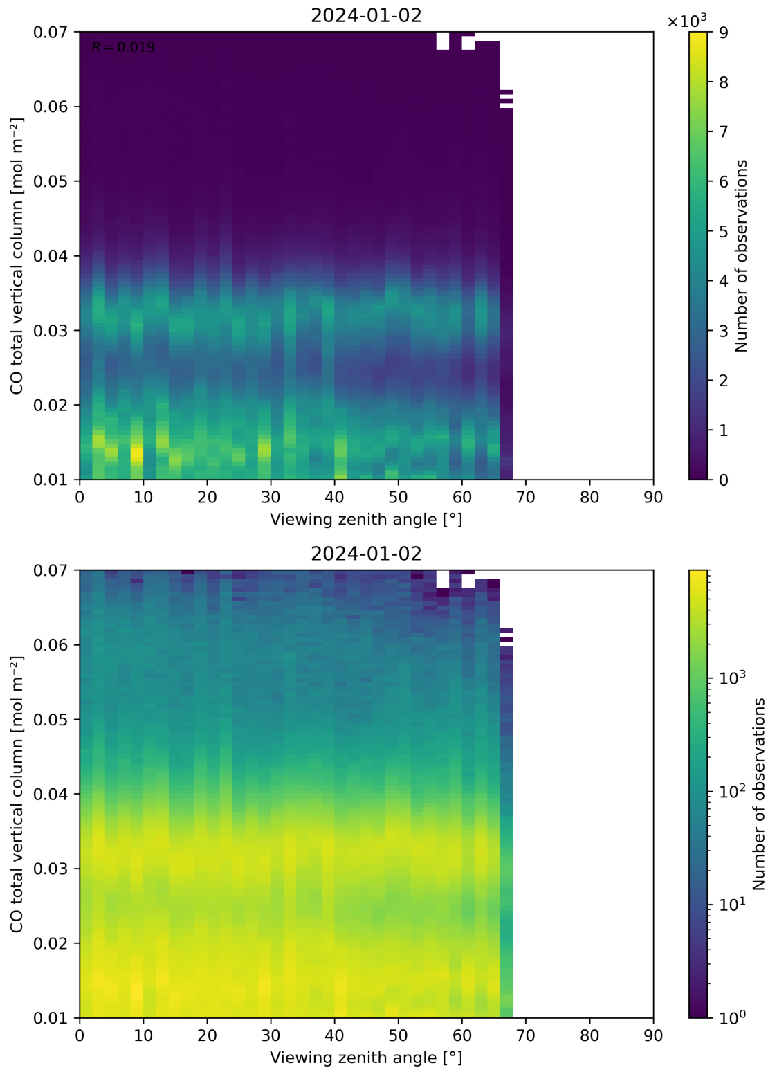
Figure 69: Scatter density plot of “Viewing zenith angle” against “CO total vertical column” for 2024-01-01 to 2024-01-03.
