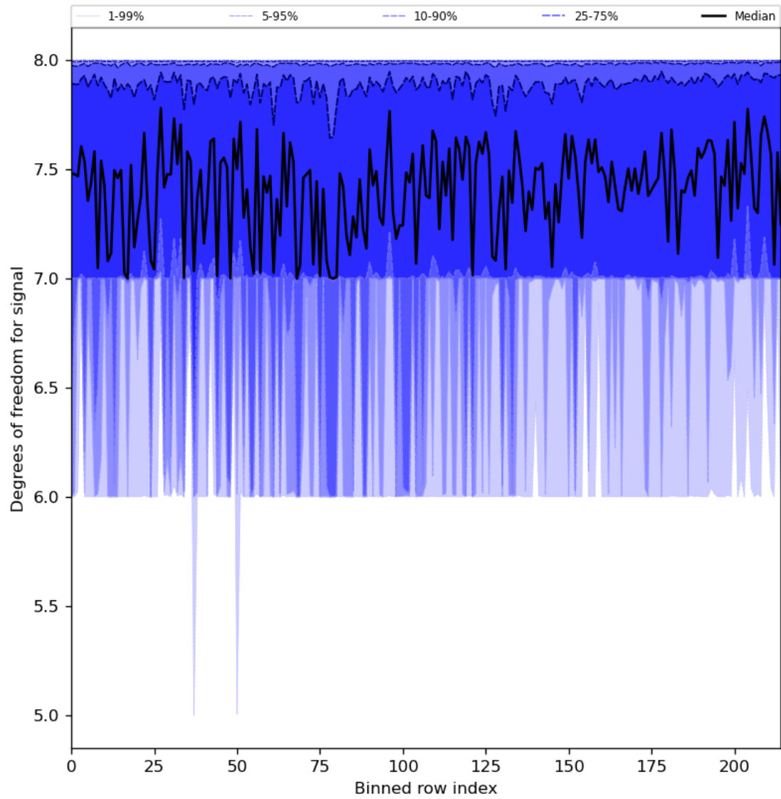
Figure 31: Along track statistics of “Degrees of freedom for signal” for 2024-01-01 to 2024-01-03
