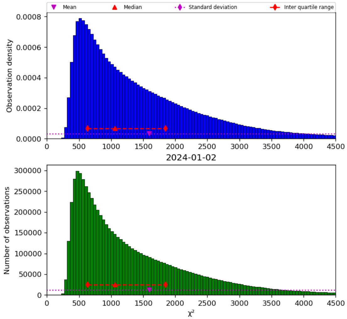
Figure 22: Histogram of “ \chi^2 ” for 2024-01-01 to 2024-01-03
