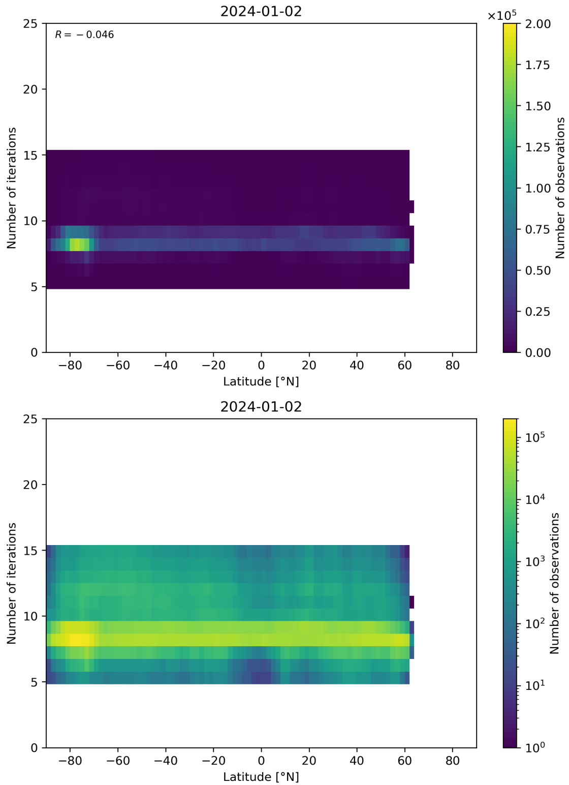
Figure 56: Scatter density plot of “Latitude” against “Number of iterations” for 2024-01-01 to 2024-01-03.
