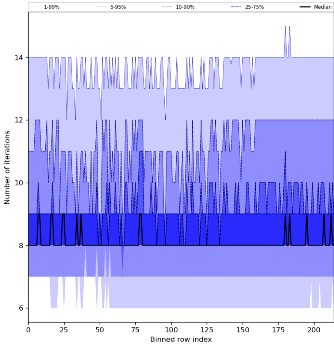
Figure 32: Along track statistics of “Number of iterations” for 2024-01-01 to 2024-01-03
