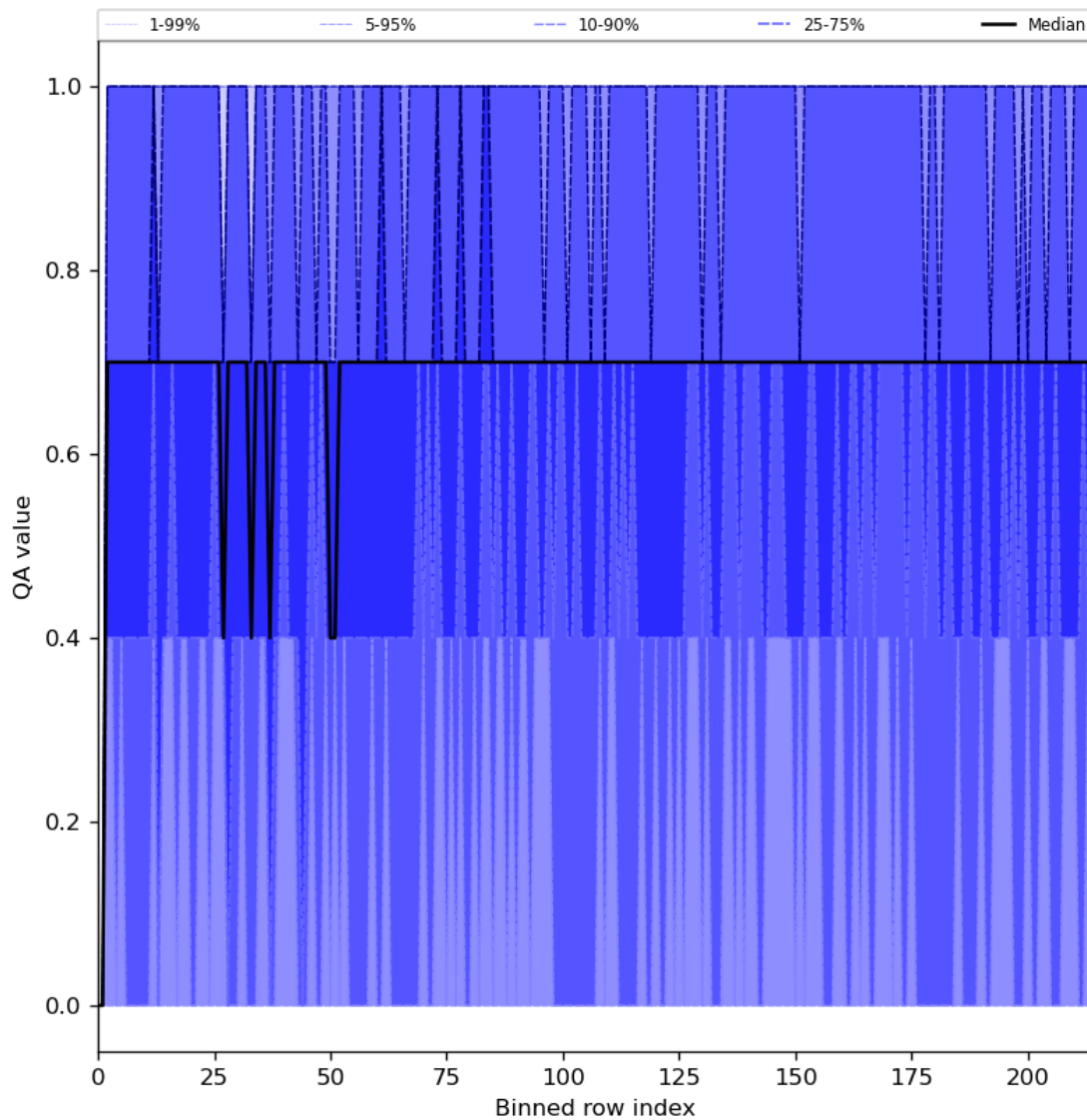
Figure 25: Along track statistics of “QA value” for 2024-01-01 to 2024-01-03
