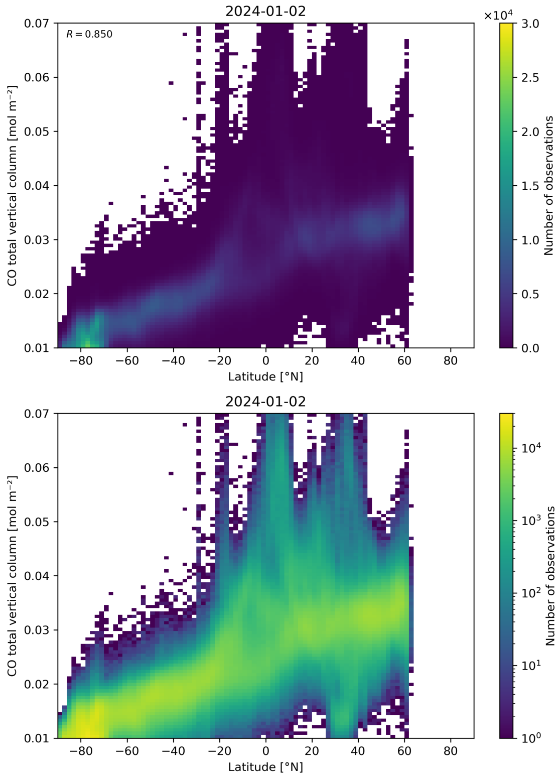
Figure 51: Scatter density plot of “Latitude” against “CO total vertical column” for 2024-01-01 to 2024-01-03.
