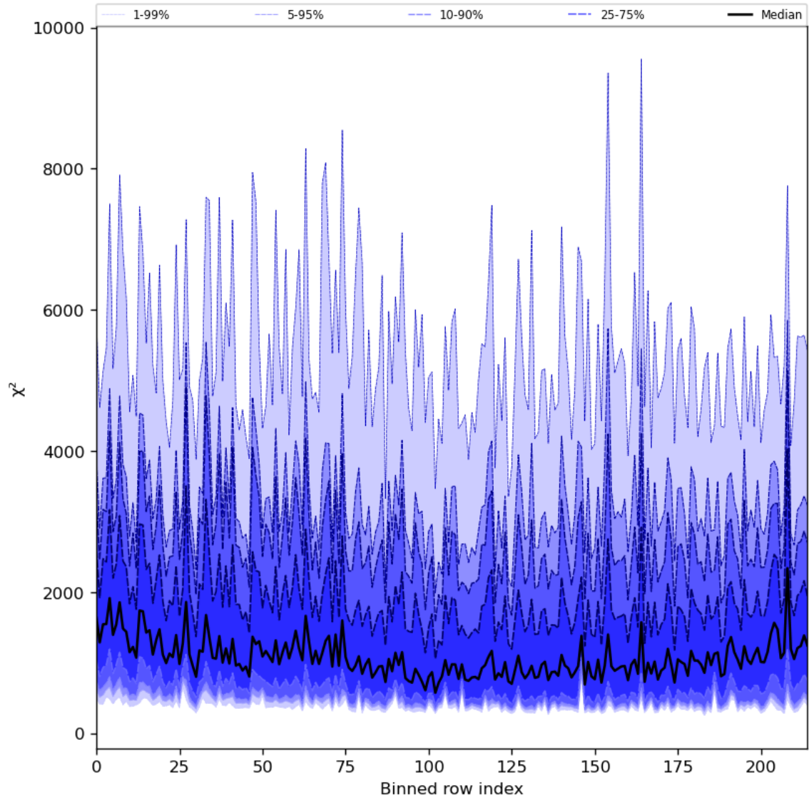
Figure 30: Along track statistics of “ \chi^2 ” for 2024-01-01 to 2024-01-03
