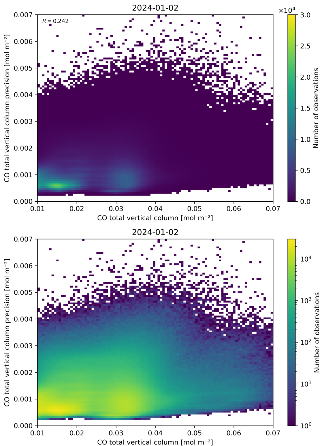
Figure 34: Scatter density plot of “CO total vertical column” against “CO total vertical column precision” for 2024-01-01 to 2024-01-03.
