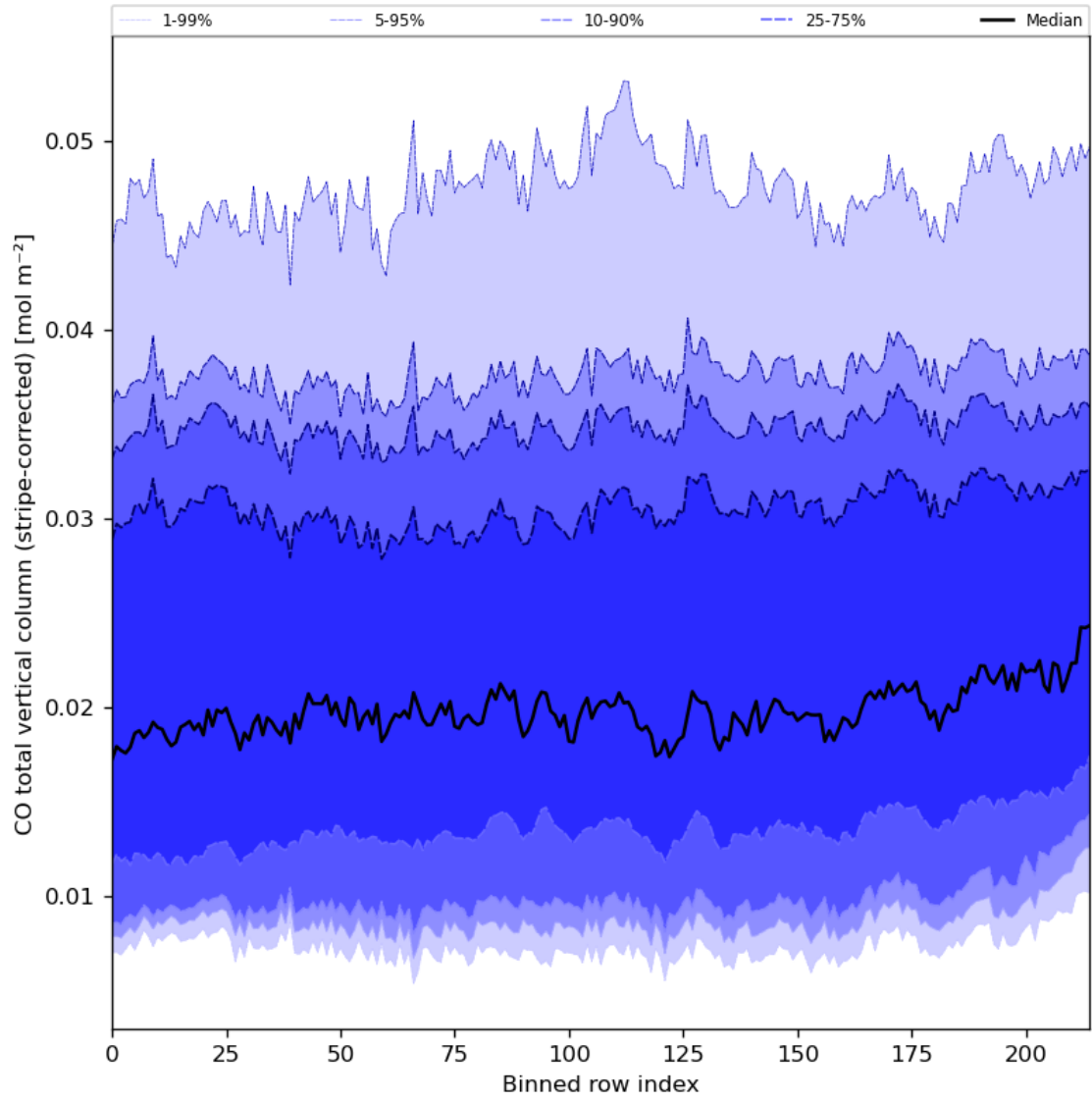
Figure 27: Along track statistics of “CO total vertical column (stripe-corrected)” for 2024-01-01 to 2024-01-03
