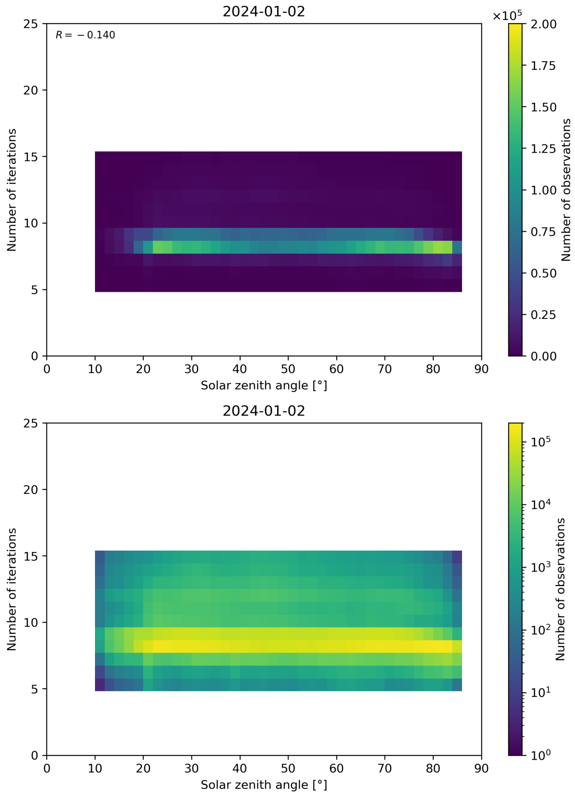
Figure 67: Scatter density plot of “Solar zenith angle” against “Number of iterations” for 2024-01-01 to 2024-01-03.
