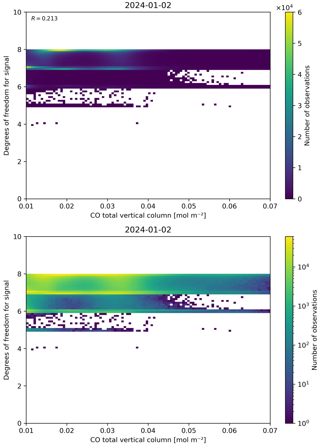
Figure 41: Scatter density plot of “CO total vertical column” against “Degrees of freedom for signal” for 2024-01-01 to 2024-01-03.
