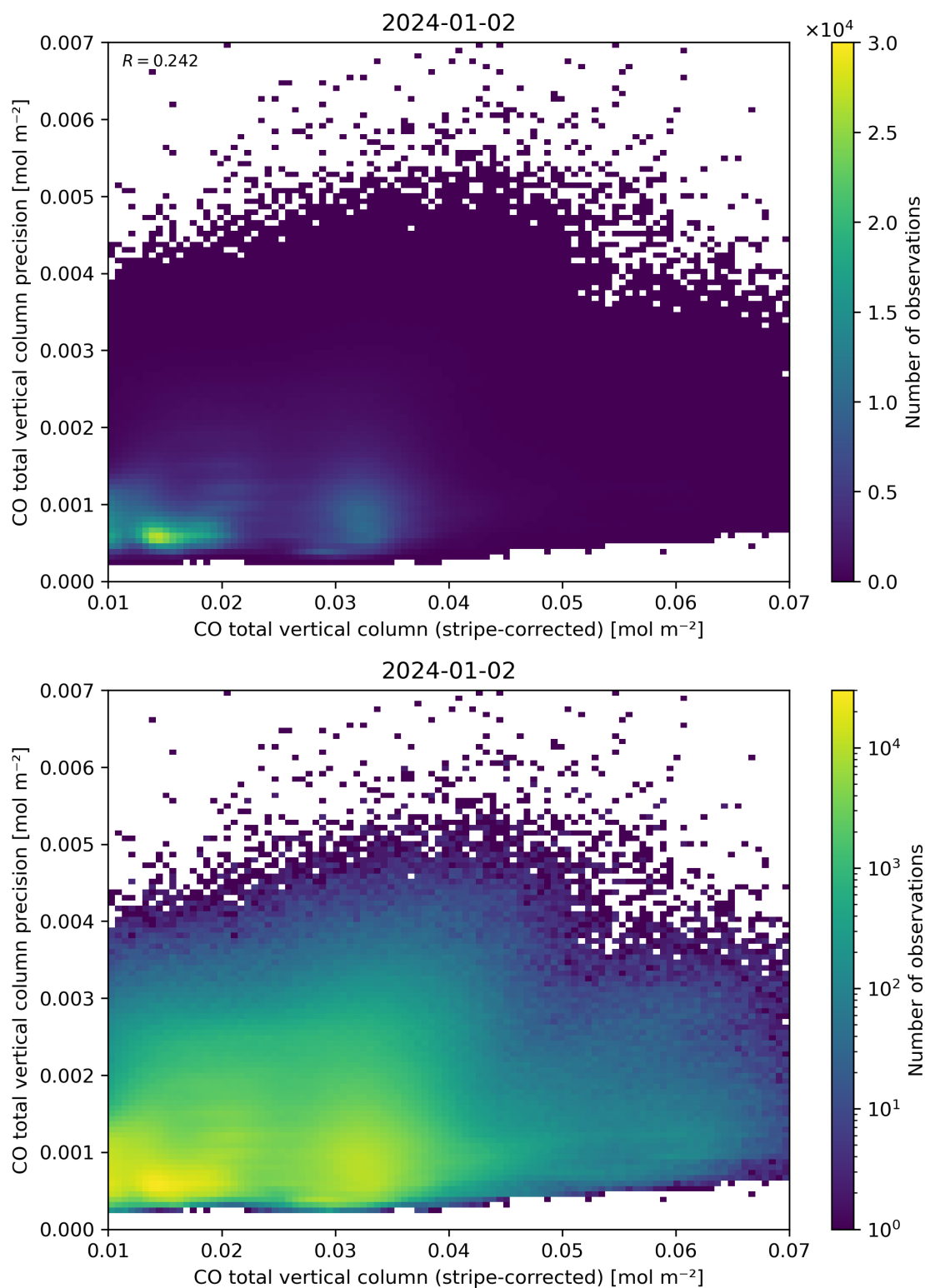
Figure 36: Scatter density plot of “CO total vertical column (stripe-corrected)” against “CO total vertical column precision” for 2024-01-01 to 2024-01-03.
