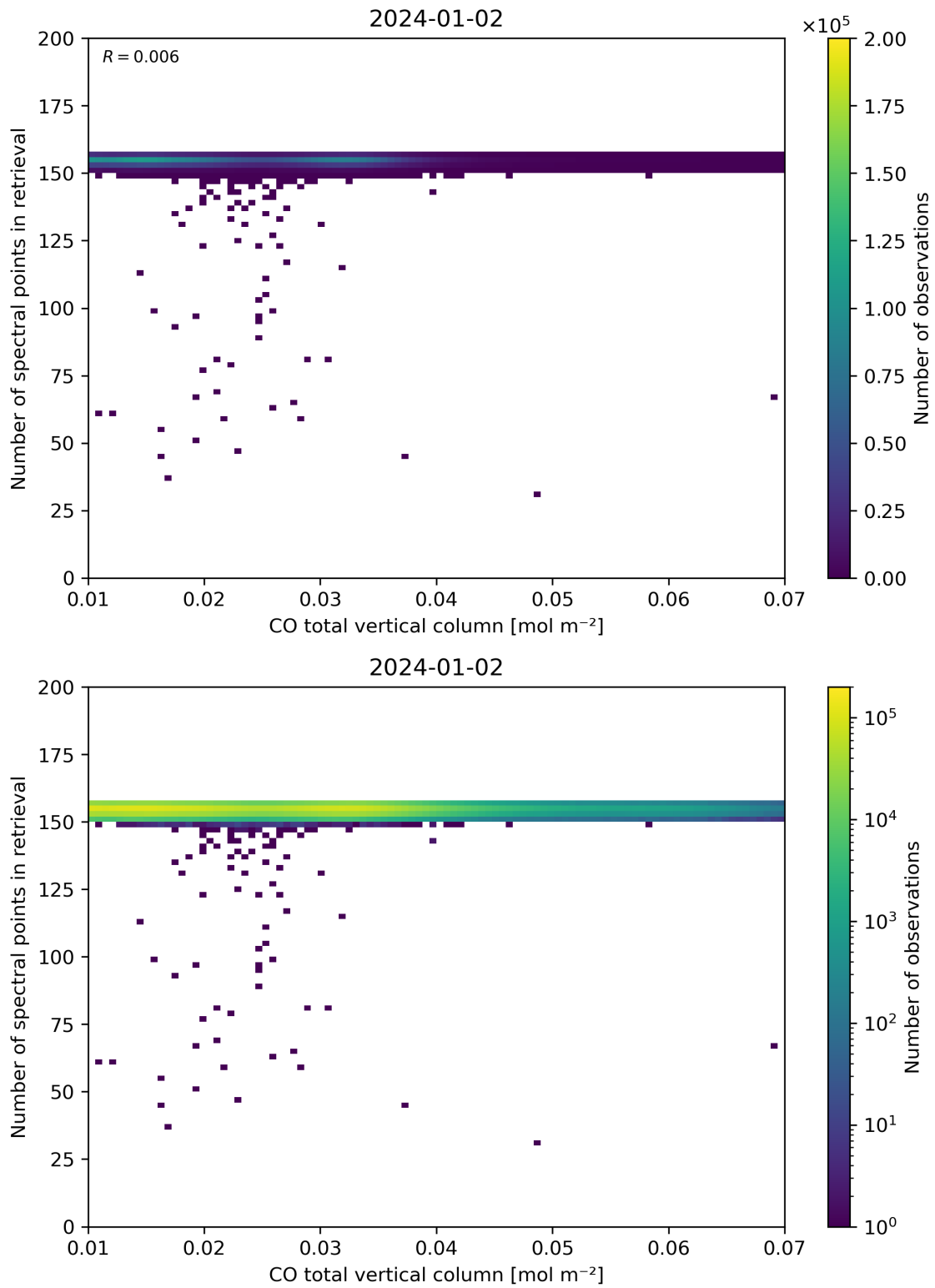
Figure 43: Scatter density plot of “CO total vertical column” against “Number of spectral points in retrieval” for 2024-01-01 to 2024-01-03.
