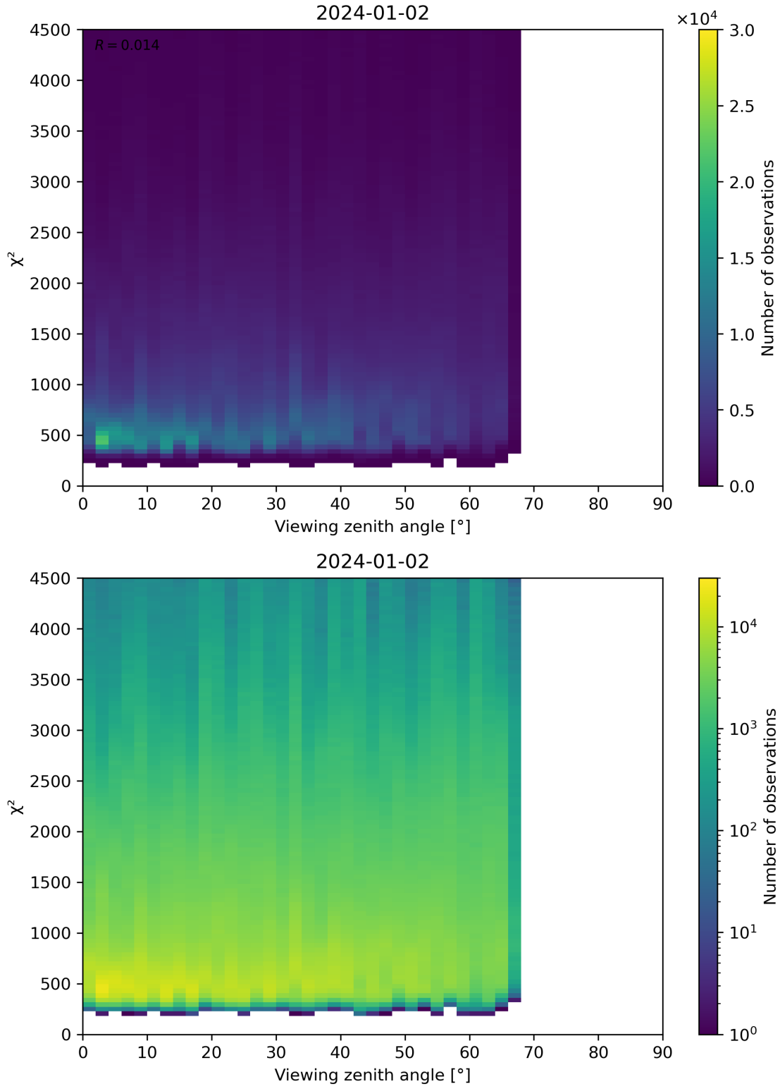
Figure 72: Scatter density plot of “Viewing zenith angle” against “ \chi^2 ” for 2024-01-01 to 2024-01-03.
