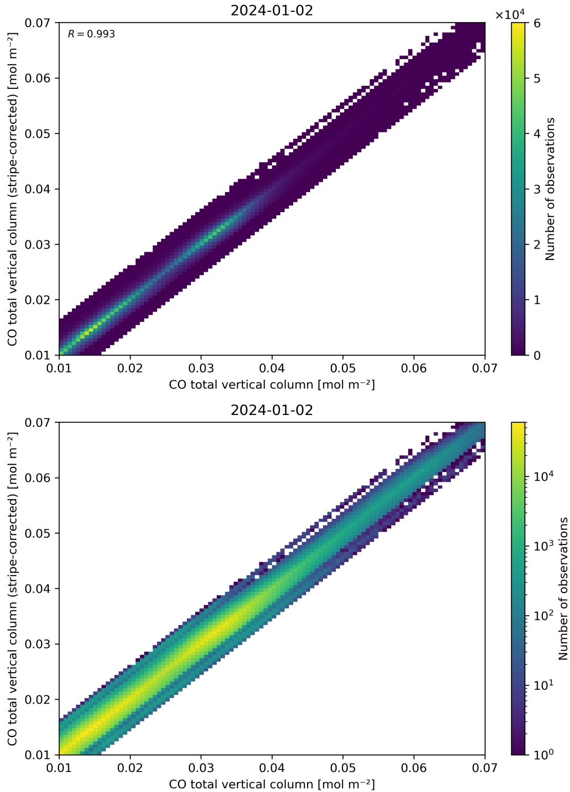
Figure 33: Scatter density plot of “CO total vertical column” against “CO total vertical column (stripe-corrected)” for 2024-01-01 to 2024-01-03.
