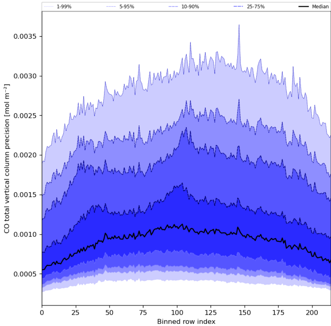
Figure 28: Along track statistics of “CO total vertical column precision” for 2024-01-01 to 2024-01-03
