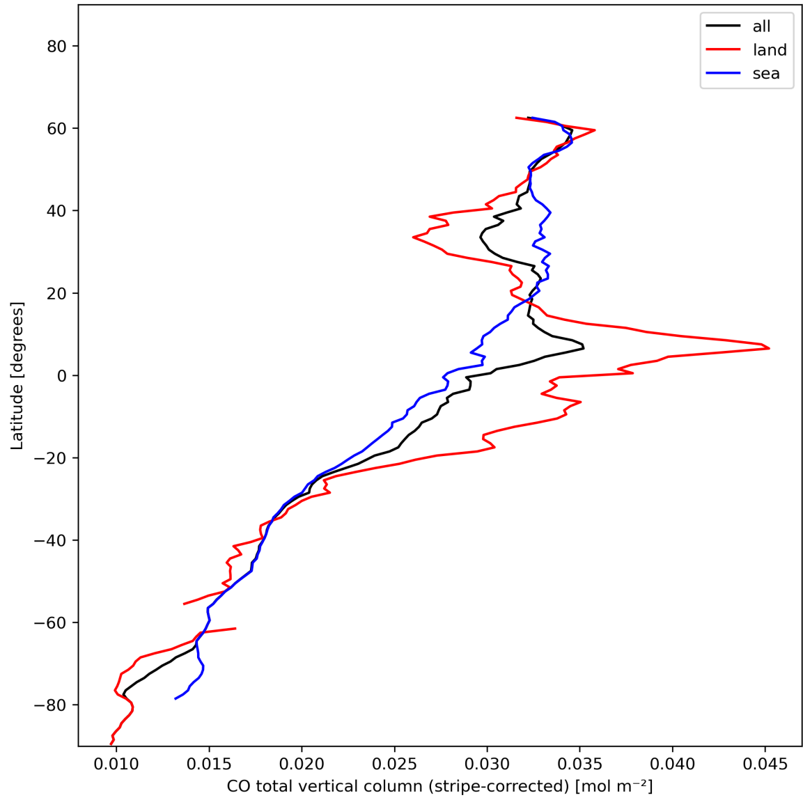
Figure 11: Zonal average of “CO total vertical column (stripe-corrected)” for 2024-01-01 to 2024-01-03.
