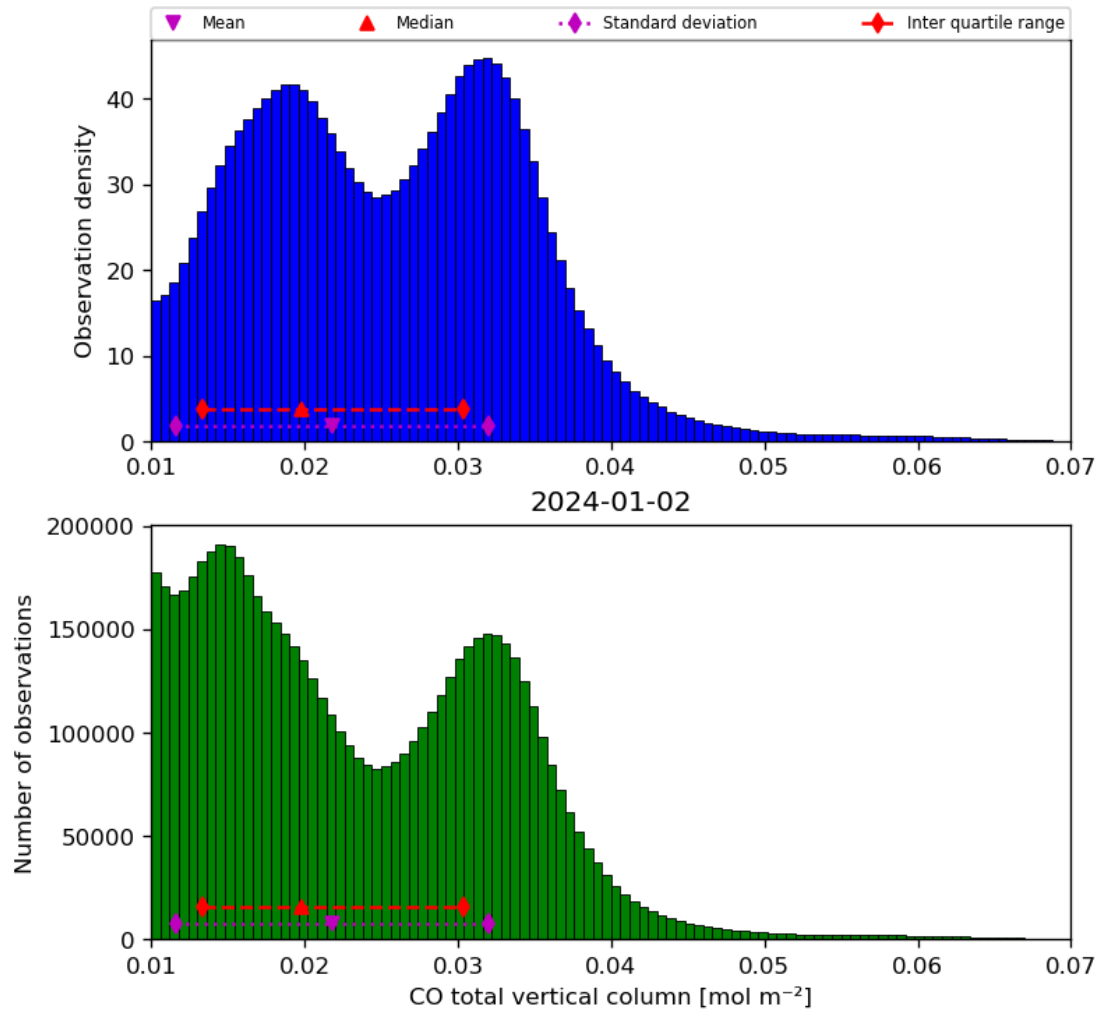
Figure 18: Histogram of “CO total vertical column” for 2024-01-01 to 2024-01-03
