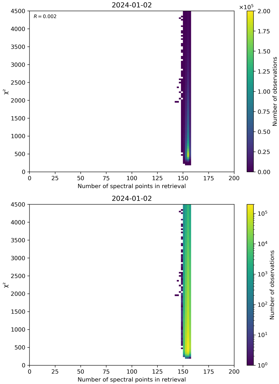
Figure 58: Scatter density plot of “Number of spectral points in retrieval” against “ \chi^2 ” for 2024-01-01 to 2024-01-03.
