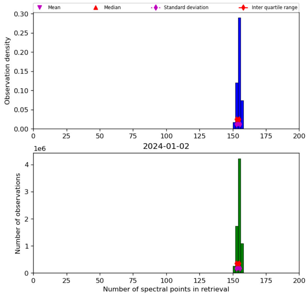
Figure 21: Histogram of “Number of spectral points in retrieval” for 2024-01-01 to 2024-01-03
