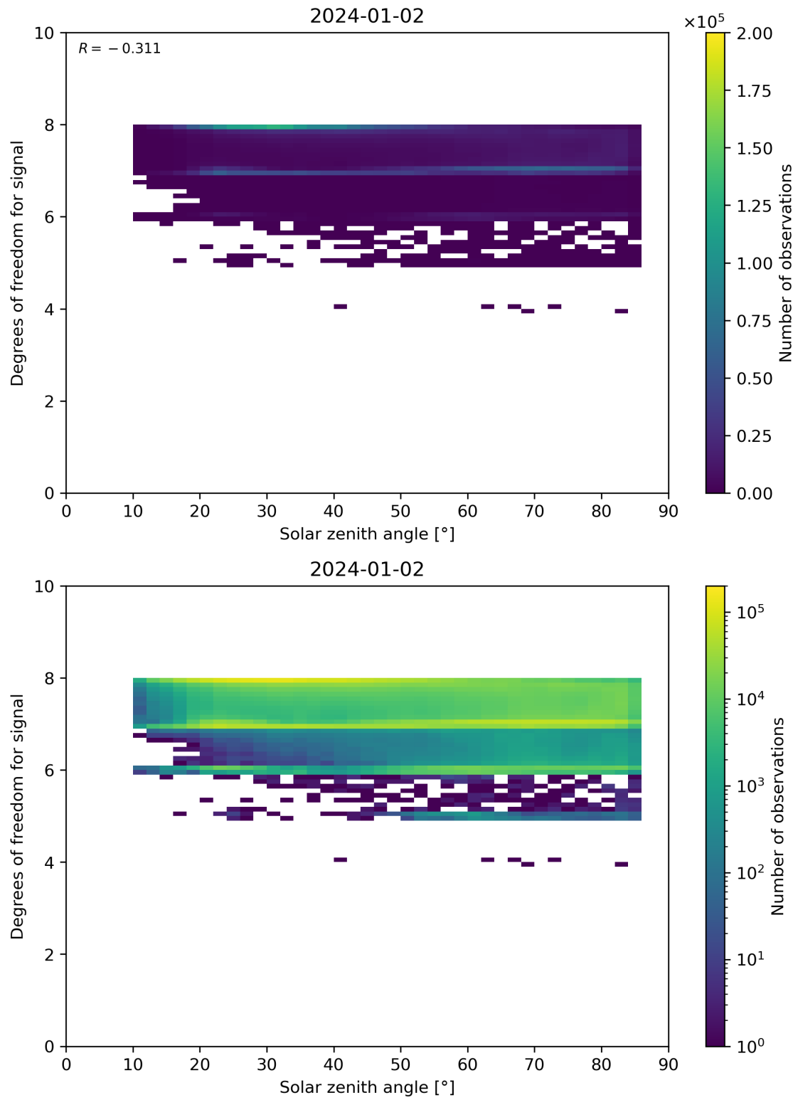
Figure 65: Scatter density plot of “Solar zenith angle” against “Degrees of freedom for signal” for 2024-01-01 to 2024-01-03.
