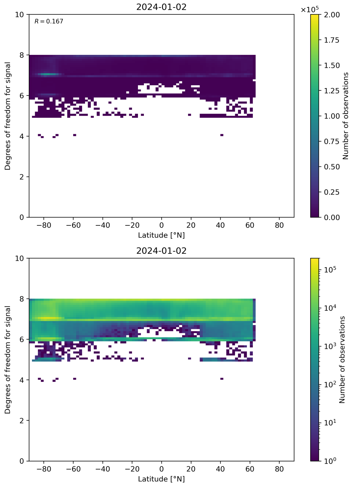
Figure 55: Scatter density plot of “Latitude” against “Degrees of freedom for signal” for 2024-01-01 to 2024-01-03.
