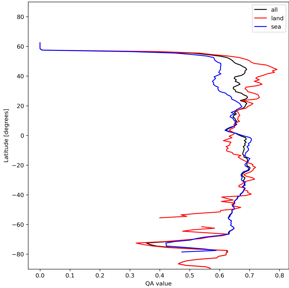
Figure 9: Zonal average of “QA value” for 2024-01-01 to 2024-01-03.
