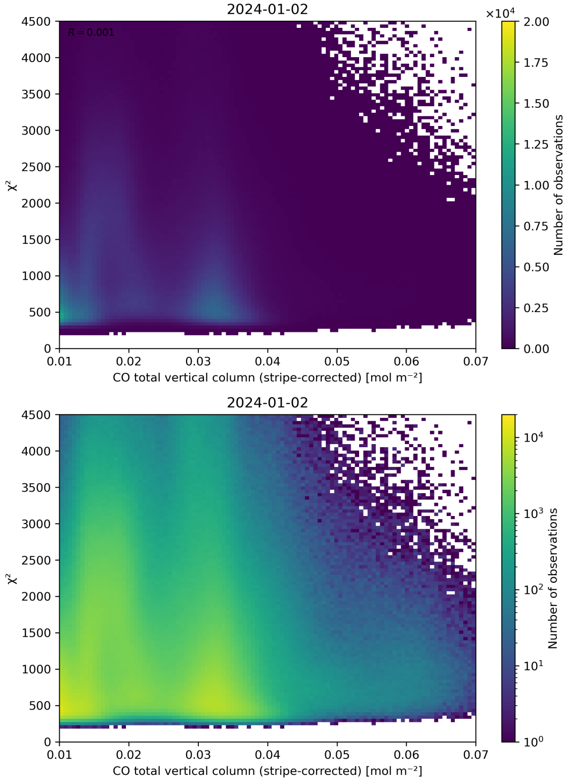
Figure 37: Scatter density plot of “CO total vertical column (stripe-corrected)” against “ \chi^2 ” for 2024-01-01 to 2024-01-03.
