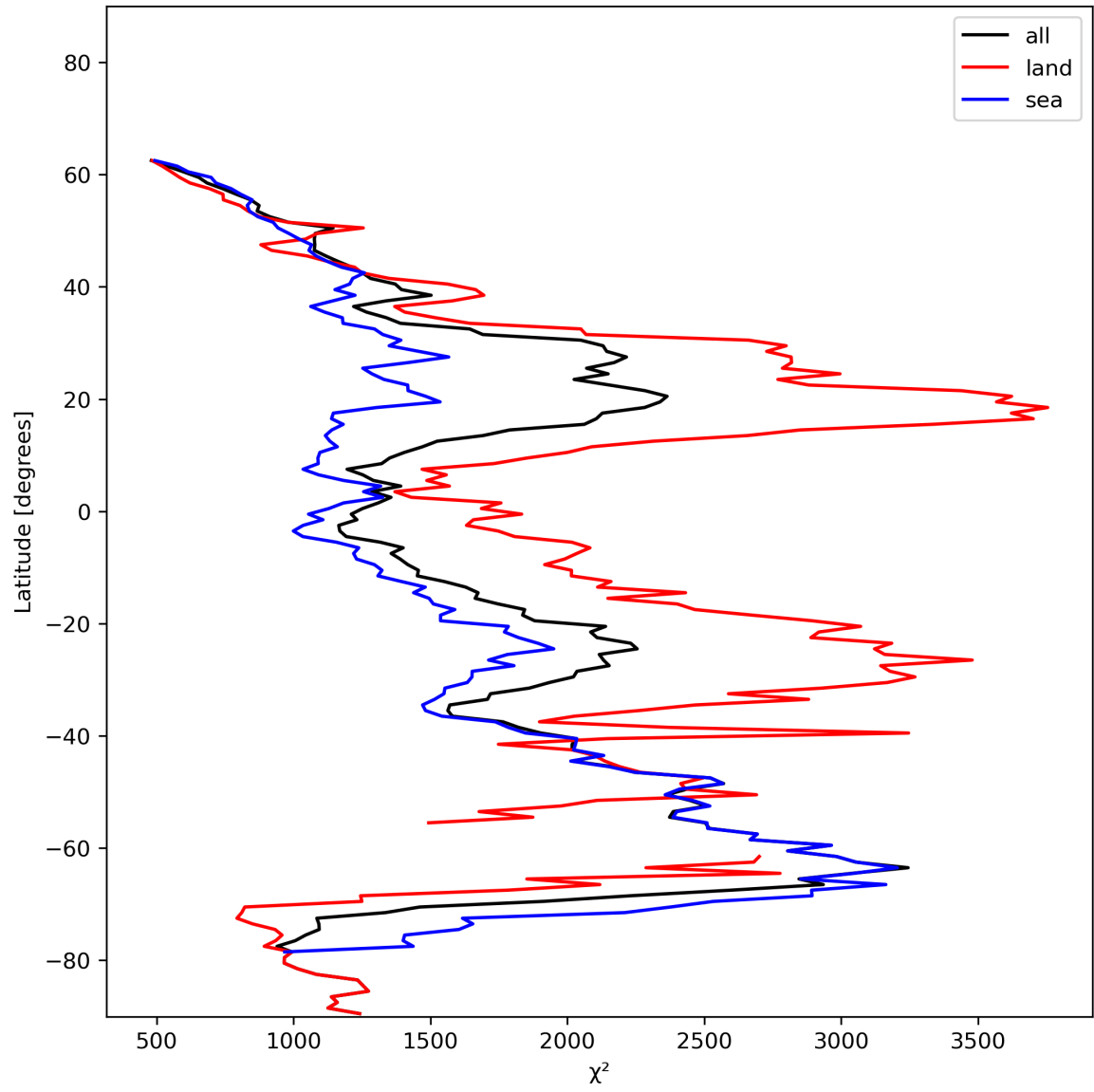
Figure 14: Zonal average of “ \chi^2 ” for 2024-01-01 to 2024-01-03.
