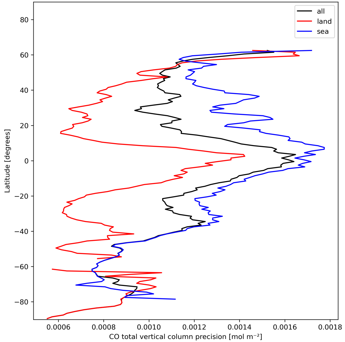
Figure 12: Zonal average of “CO total vertical column precision” for 2024-01-01 to 2024-01-03.
