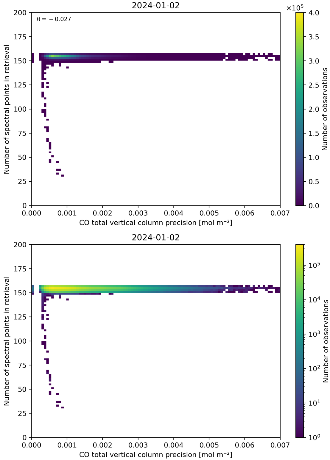
Figure 47: Scatter density plot of “CO total vertical column precision” against “Number of spectral points in retrieval” for 2024-01-01 to 2024-01-03.
