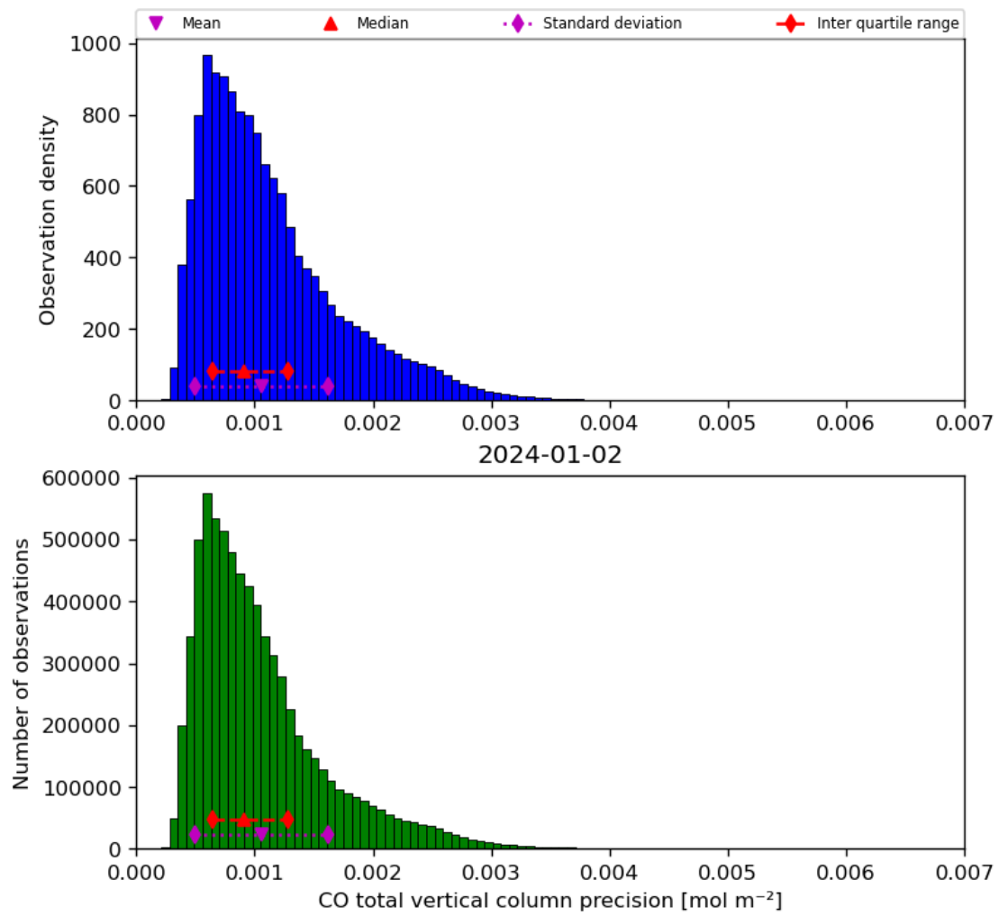
Figure 20: Histogram of “CO total vertical column precision” for 2024-01-01 to 2024-01-03
