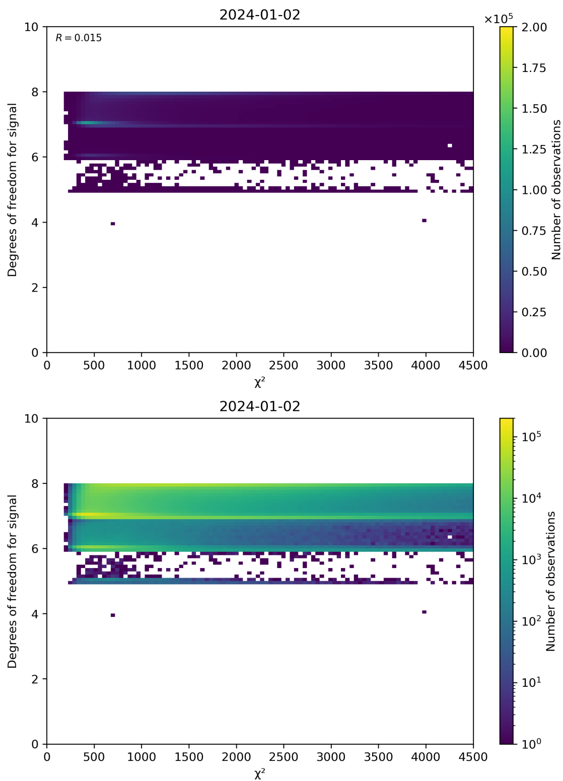
Figure 48: Scatter density plot of “ \chi^2 ” against “Degrees of freedom for signal” for 2024-01-01 to 2024-01-03.
