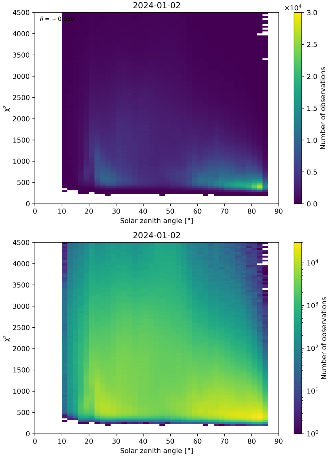
Figure 64: Scatter density plot of “Solar zenith angle” against “ \chi^2 ” for 2024-01-01 to 2024-01-03.
