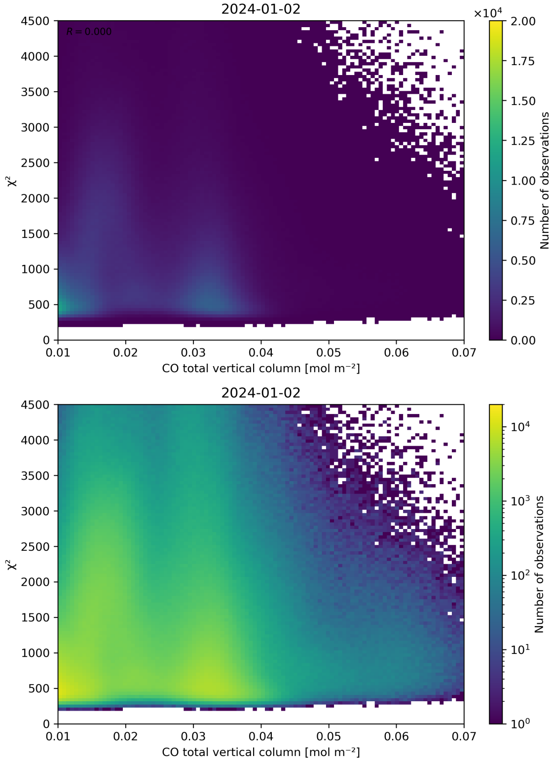
Figure 35: Scatter density plot of “CO total vertical column” against “ \chi^2 ” for 2024-01-01 to 2024-01-03.
