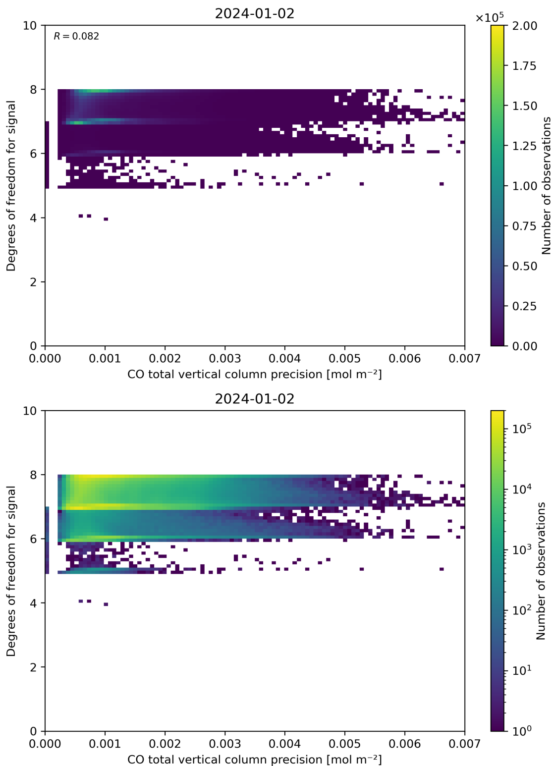
Figure 45: Scatter density plot of “CO total vertical column precision” against “Degrees of freedom for signal” for 2024-01-01 to 2024-01-03.
