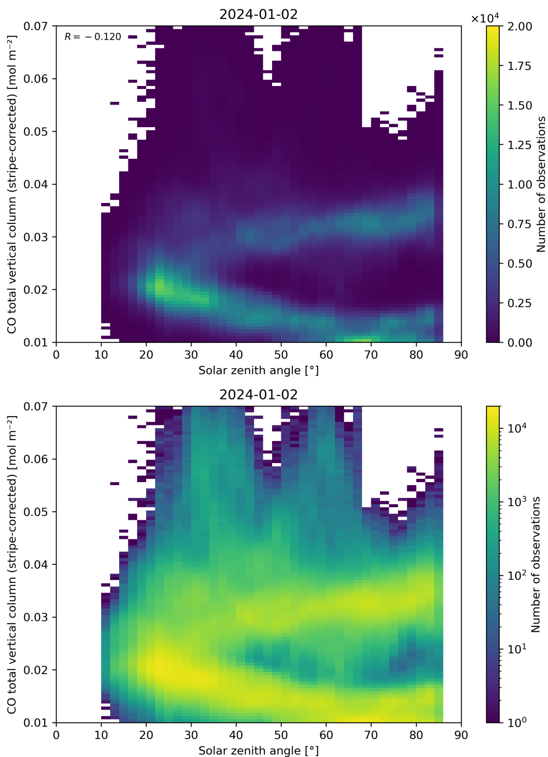
Figure 62: Scatter density plot of “Solar zenith angle” against “CO total vertical column (stripe-corrected)” for 2024-01-01 to 2024-01-03.
