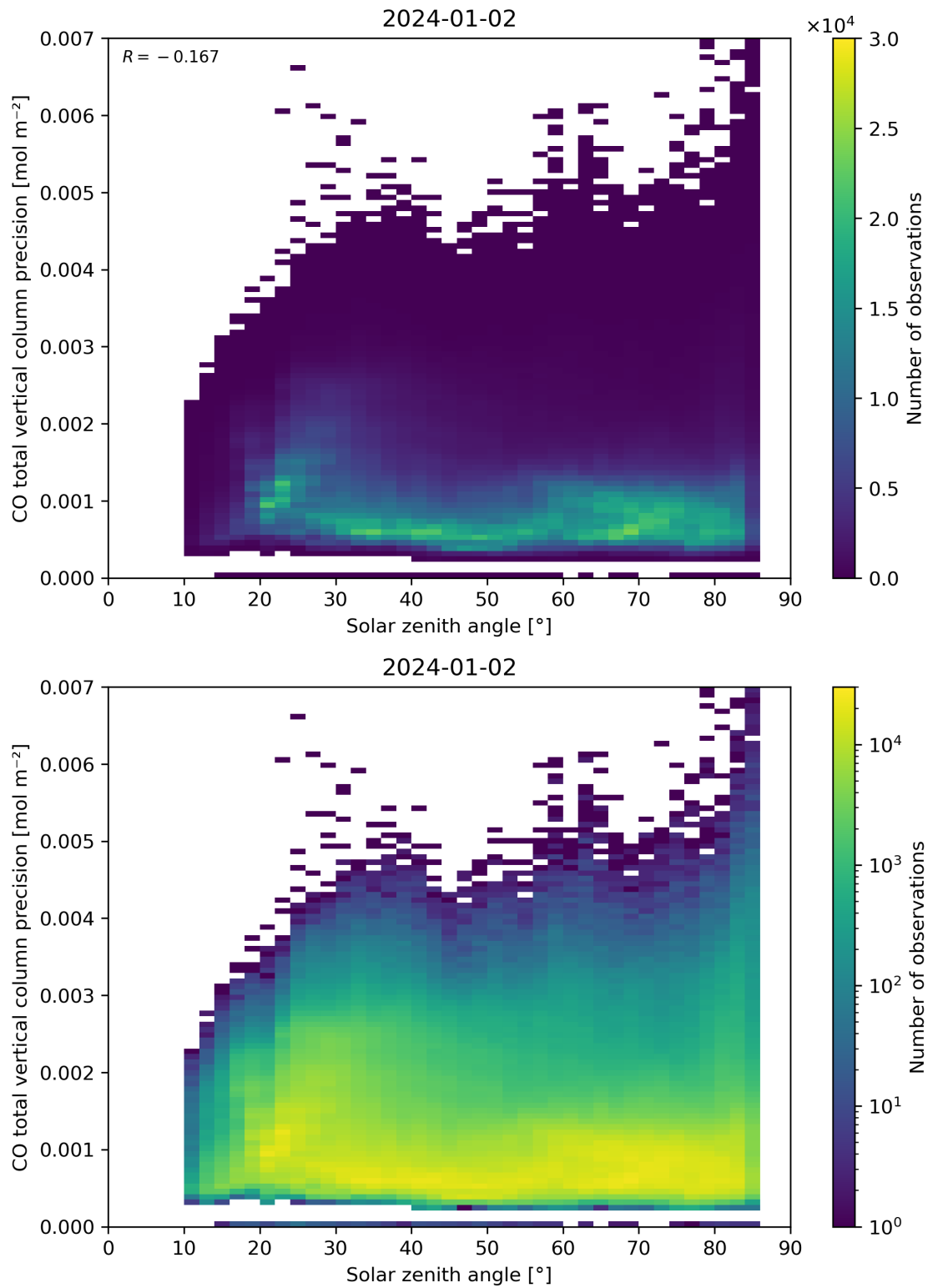
Figure 63: Scatter density plot of “Solar zenith angle” against “CO total vertical column precision” for 2024-01-01 to 2024-01-03.
