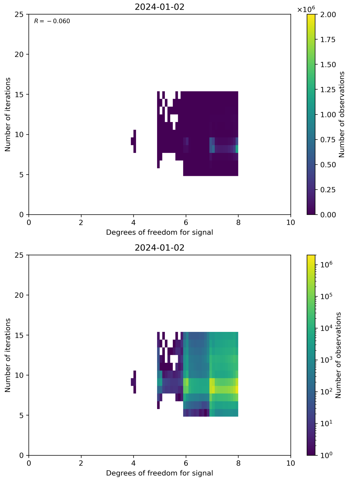
Figure 50: Scatter density plot of “Degrees of freedom for signal” against “Number of iterations” for 2024-01-01 to 2024-01-03.
