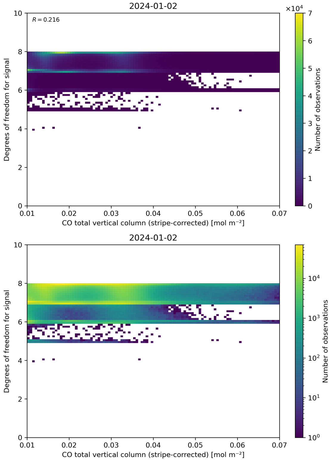
Figure 38: Scatter density plot of “CO total vertical column (stripe-corrected)” against “Degrees of freedom for signal” for 2024-01-01 to 2024-01-03.
