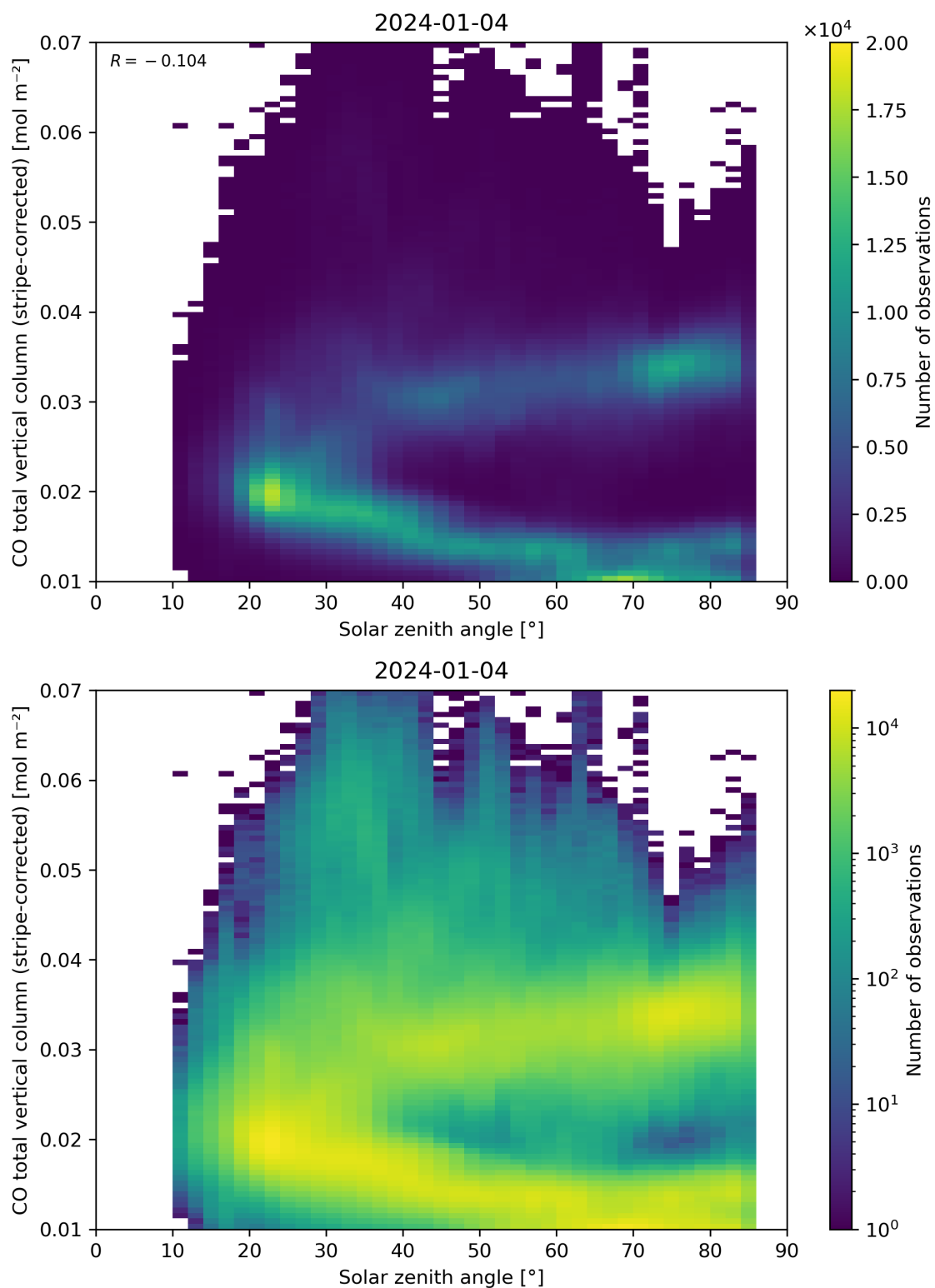
Figure 62: Scatter density plot of “Solar zenith angle” against “CO total vertical column (stripe-corrected)” for 2024-01-03 to 2024-01-05.
