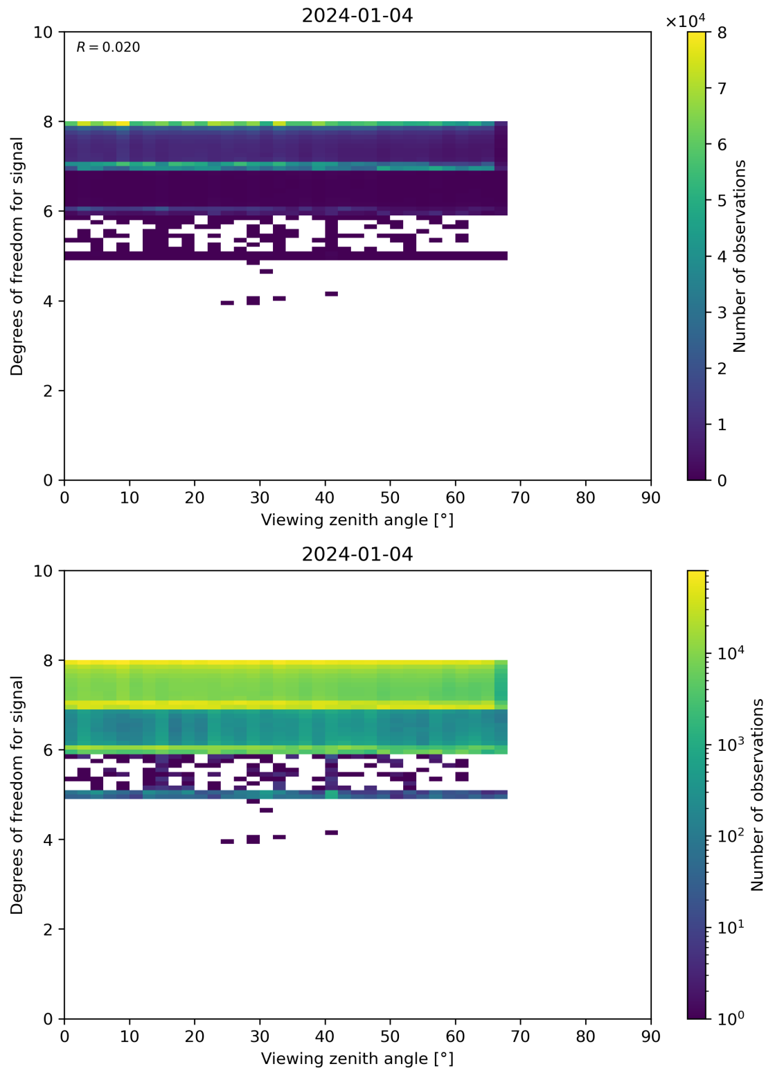
Figure 73: Scatter density plot of “Viewing zenith angle” against “Degrees of freedom for signal” for 2024-01-03 to 2024-01-05.
