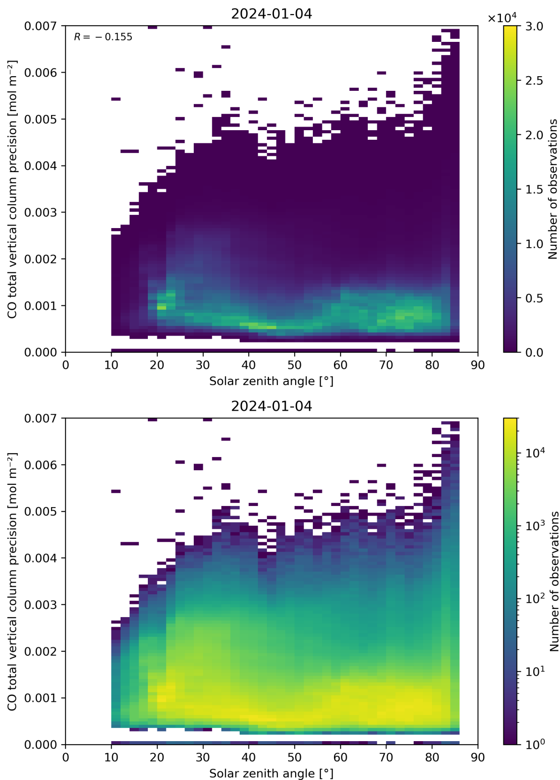
Figure 63: Scatter density plot of “Solar zenith angle” against “CO total vertical column precision” for 2024-01-03 to 2024-01-05.
