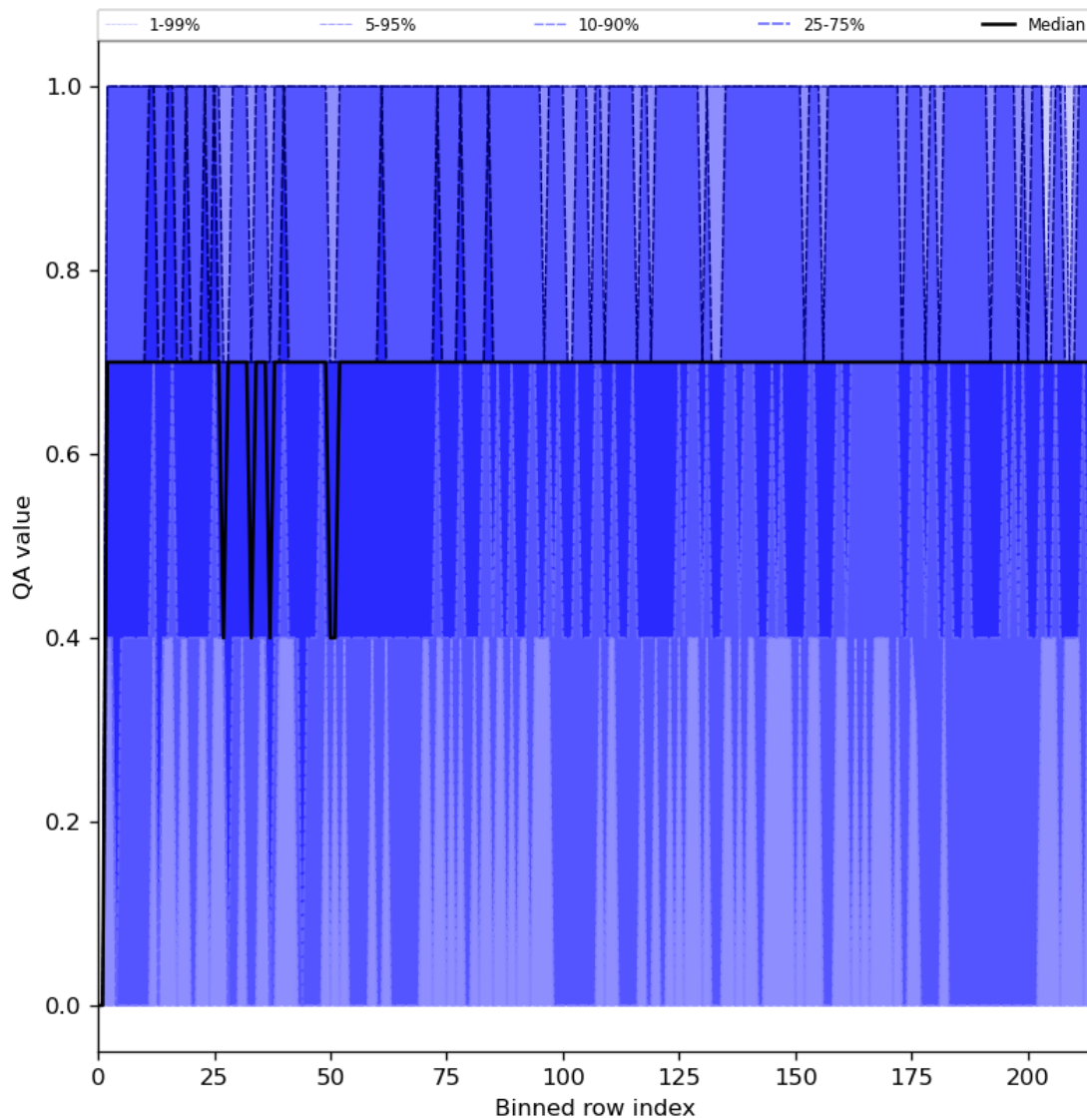
Figure 25: Along track statistics of “QA value” for 2024-01-03 to 2024-01-05
