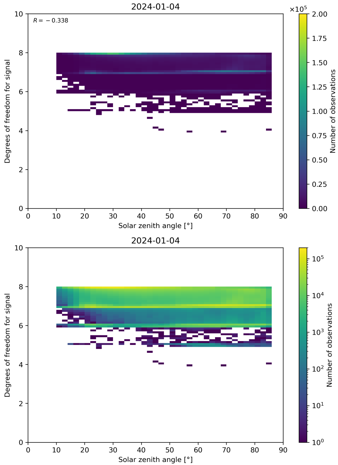
Figure 65: Scatter density plot of “Solar zenith angle” against “Degrees of freedom for signal” for 2024-01-03 to 2024-01-05.
