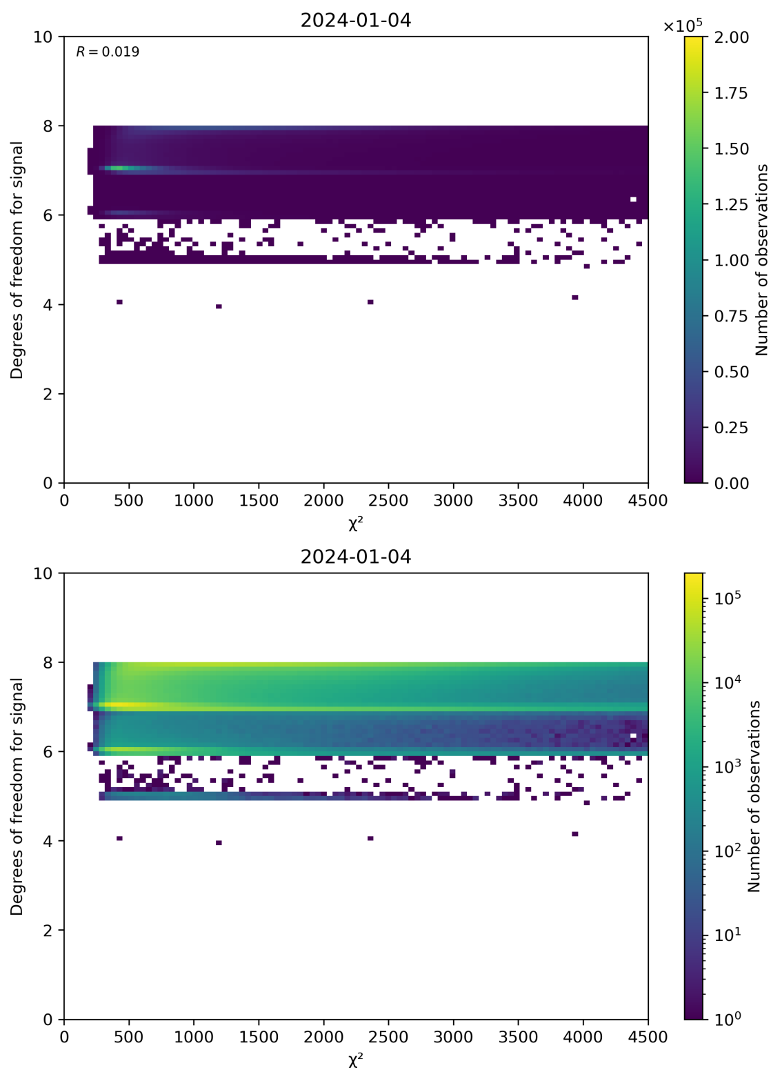
Figure 48: Scatter density plot of “ \chi^2 ” against “Degrees of freedom for signal” for 2024-01-03 to 2024-01-05.
