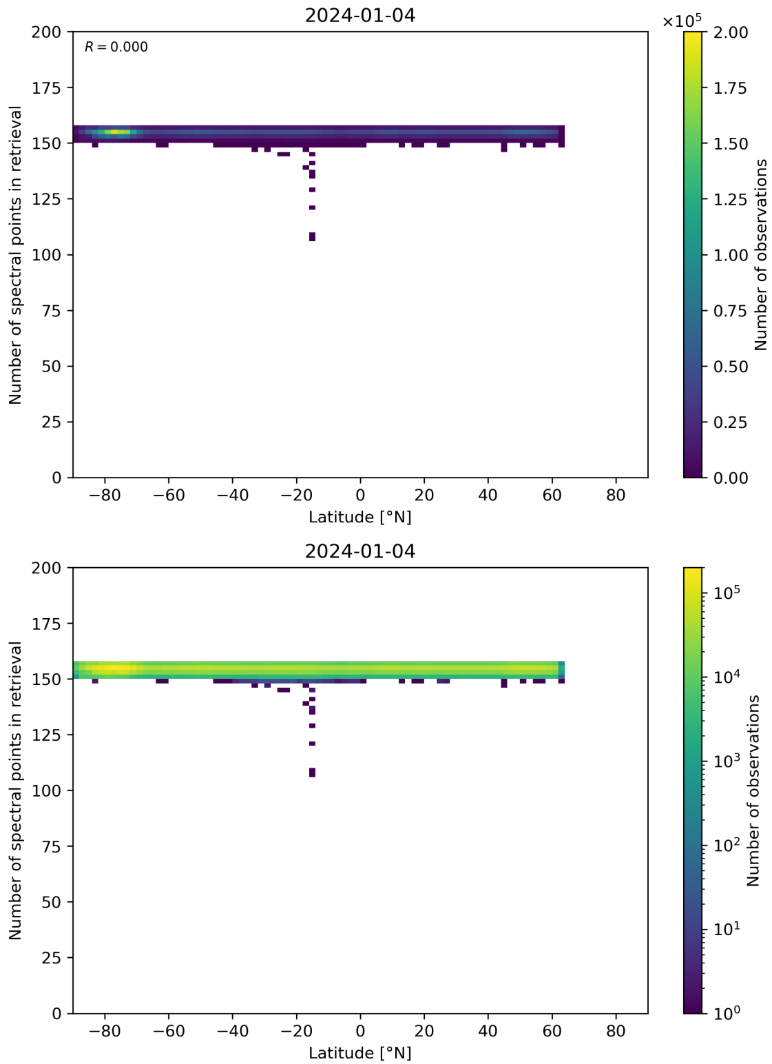
Figure 57: Scatter density plot of “Latitude” against “Number of spectral points in retrieval” for 2024-01-03 to 2024-01-05.
