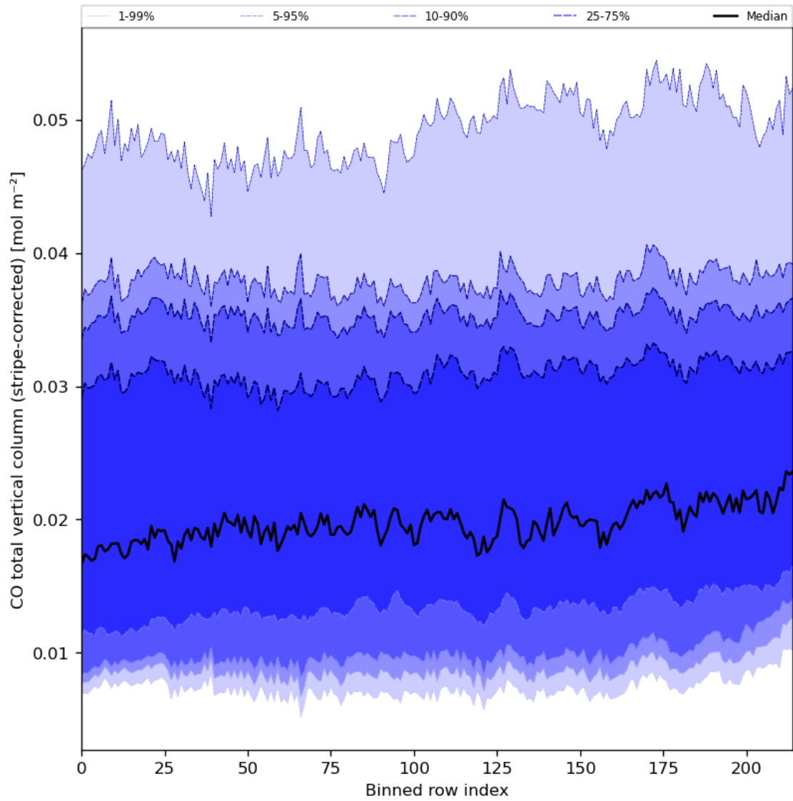
Figure 27: Along track statistics of “CO total vertical column (stripe-corrected)” for 2024-01-03 to 2024-01-05
