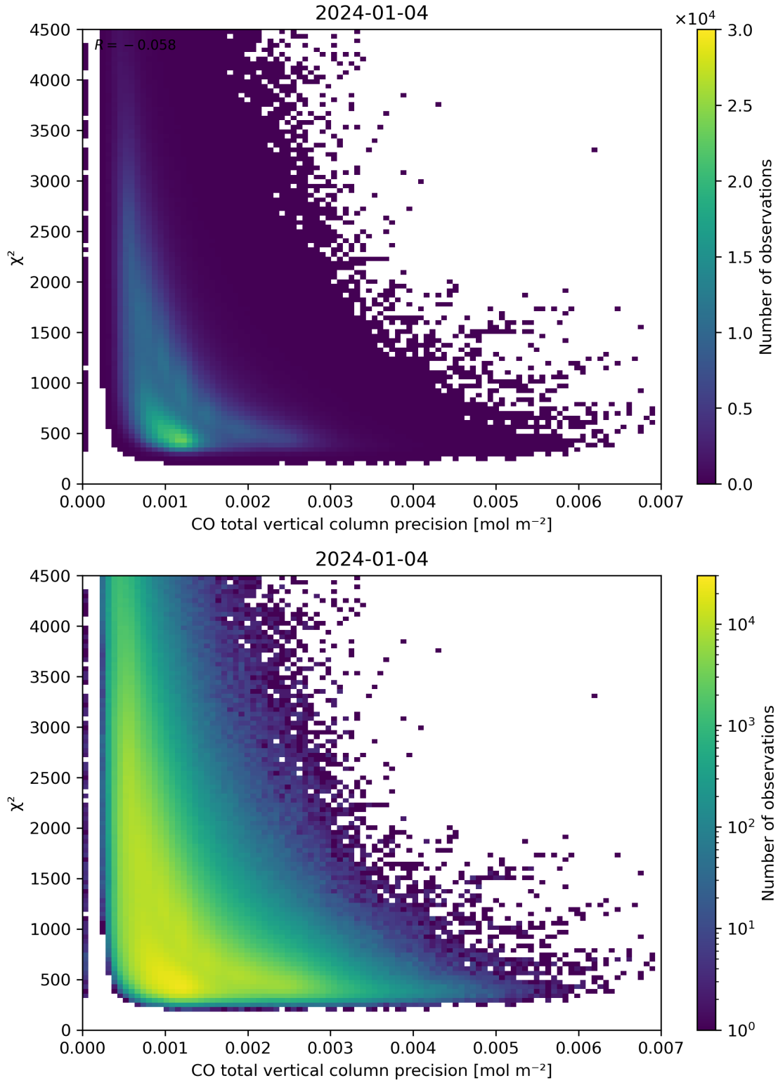
Figure 44: Scatter density plot of “CO total vertical column precision” against “ \chi^2 ” for 2024-01-03 to 2024-01-05.
