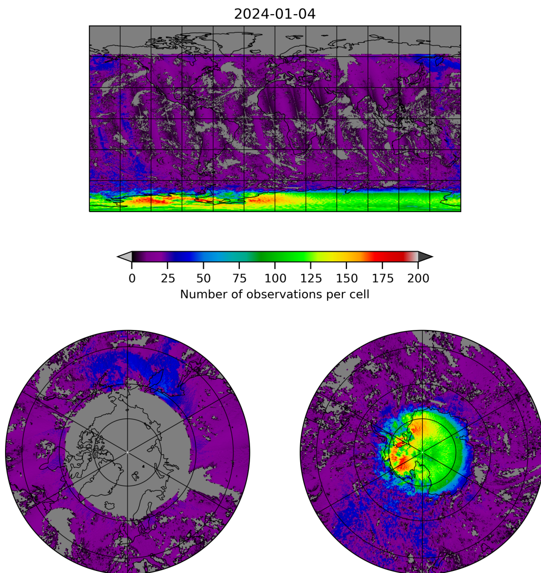
Figure 8: Map of the number of observations for 2024-01-03 to 2024-01-05
