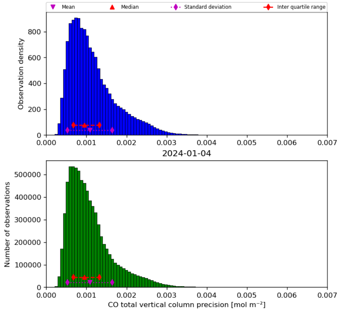
Figure 20: Histogram of “CO total vertical column precision” for 2024-01-03 to 2024-01-05
