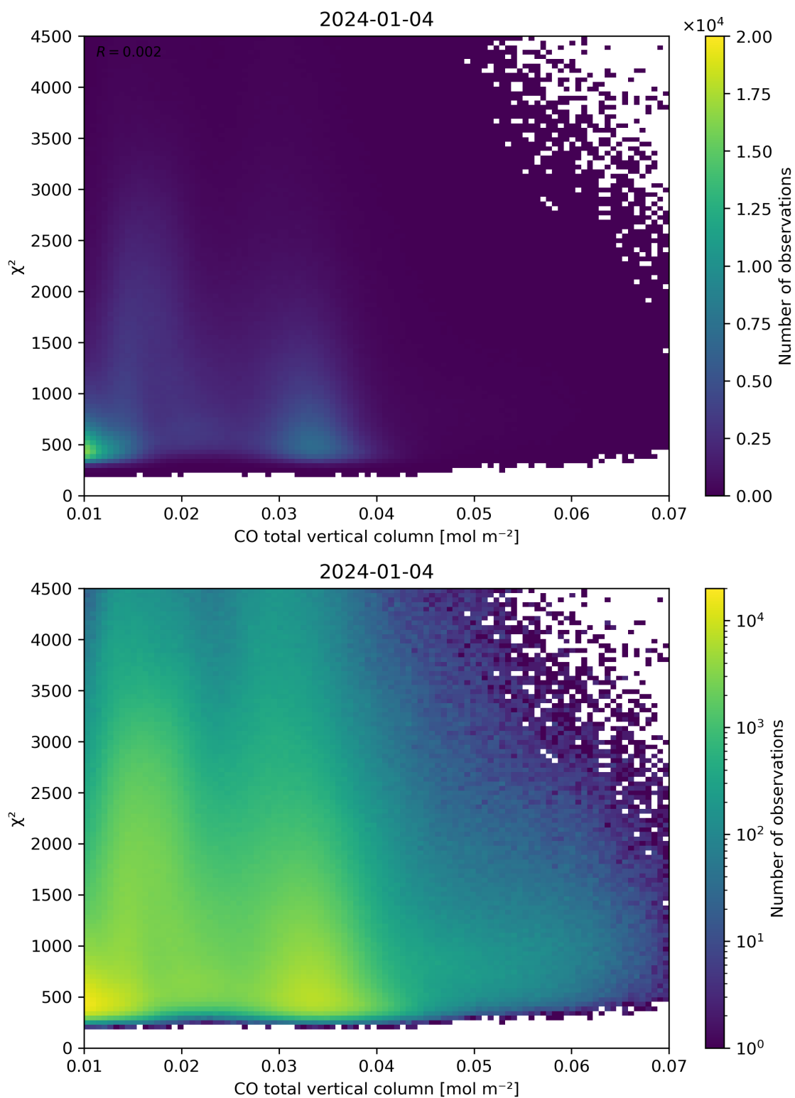
Figure 35: Scatter density plot of “CO total vertical column” against “ \chi^2 ” for 2024-01-03 to 2024-01-05.
