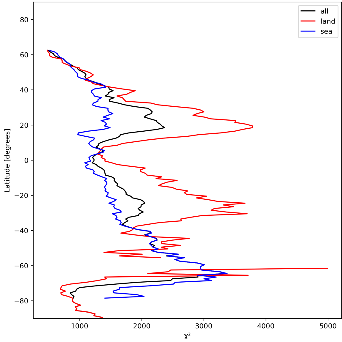
Figure 14: Zonal average of “ \chi^2 ” for 2024-01-03 to 2024-01-05.
