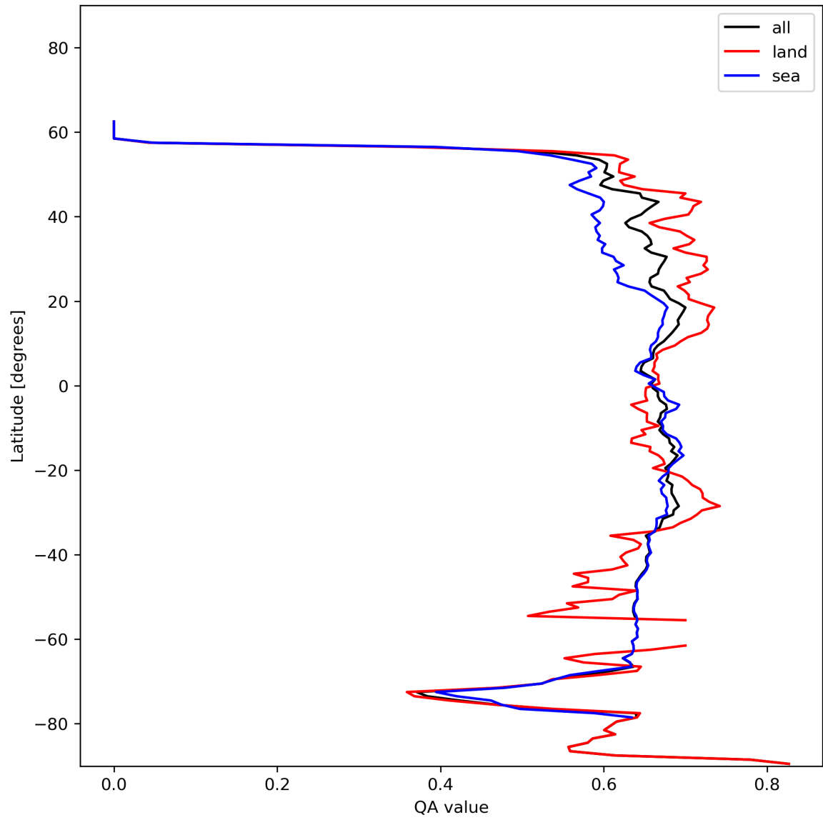
Figure 9: Zonal average of “QA value” for 2024-01-03 to 2024-01-05.
