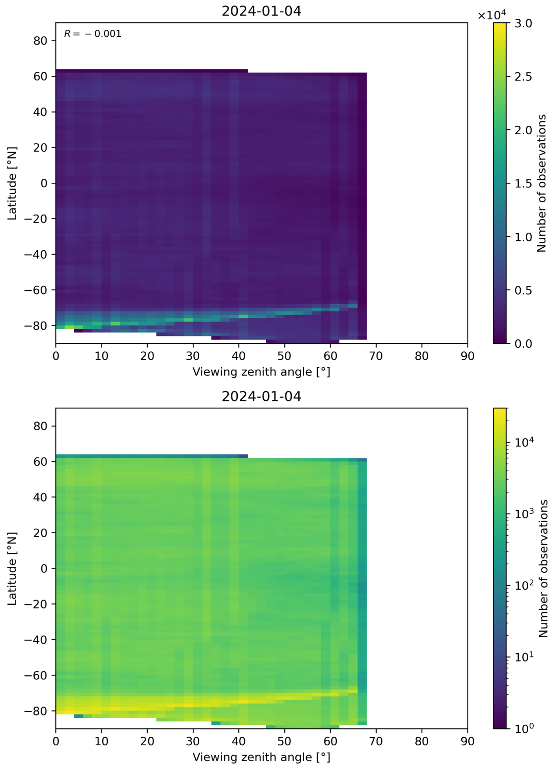
Figure 74: Scatter density plot of “Viewing zenith angle” against “Latitude” for 2024-01-03 to 2024-01-05.
