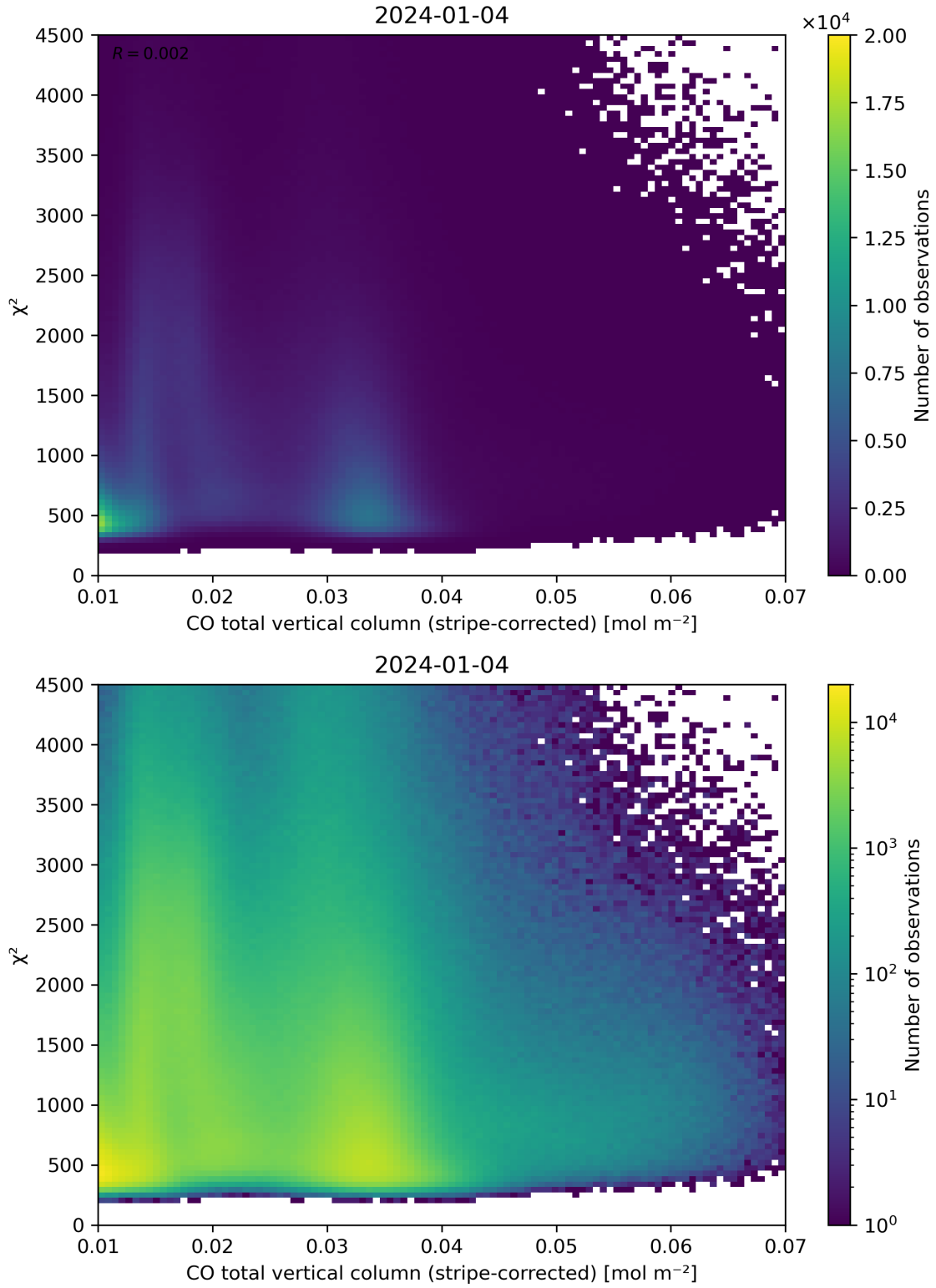
Figure 37: Scatter density plot of “CO total vertical column (stripe-corrected)” against “ \chi^2 ” for 2024-01-03 to 2024-01-05.
