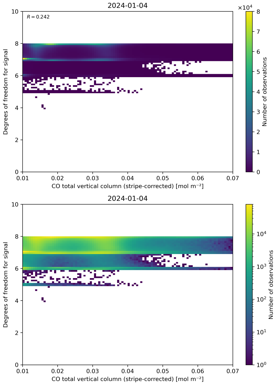
Figure 38: Scatter density plot of “CO total vertical column (stripe-corrected)” against “Degrees of freedom for signal” for 2024-01-03 to 2024-01-05.
