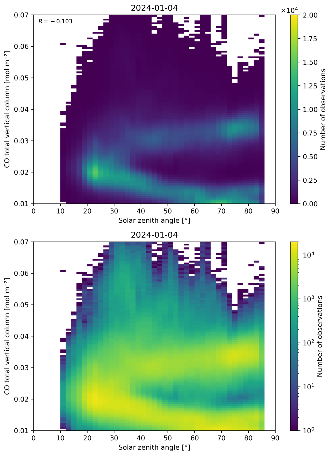
Figure 61: Scatter density plot of “Solar zenith angle” against “CO total vertical column” for 2024-01-03 to 2024-01-05.
