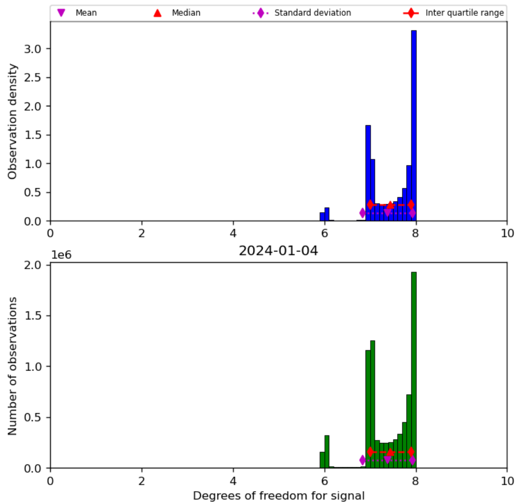
Figure 23: Histogram of “Degrees of freedom for signal” for 2024-01-03 to 2024-01-05
