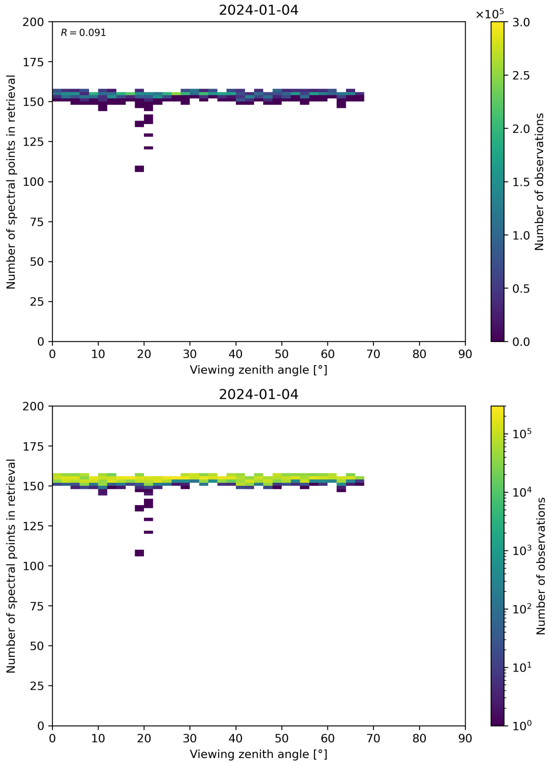
Figure 76: Scatter density plot of “Viewing zenith angle” against “Number of spectral points in retrieval” for 2024-01-03 to 2024-01-05.
