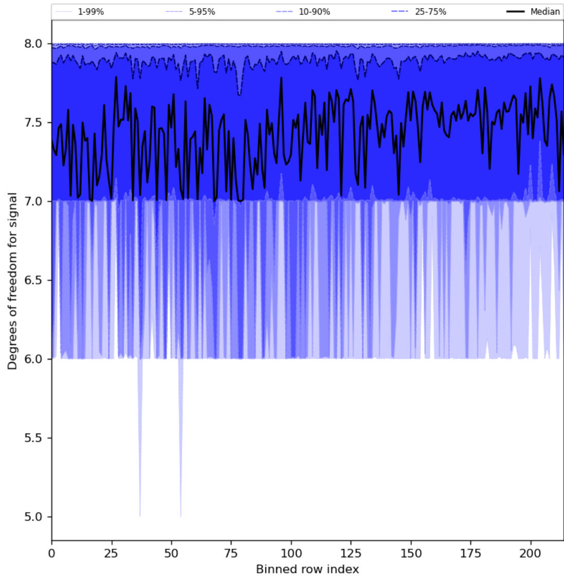
Figure 31: Along track statistics of “Degrees of freedom for signal” for 2024-01-03 to 2024-01-05
