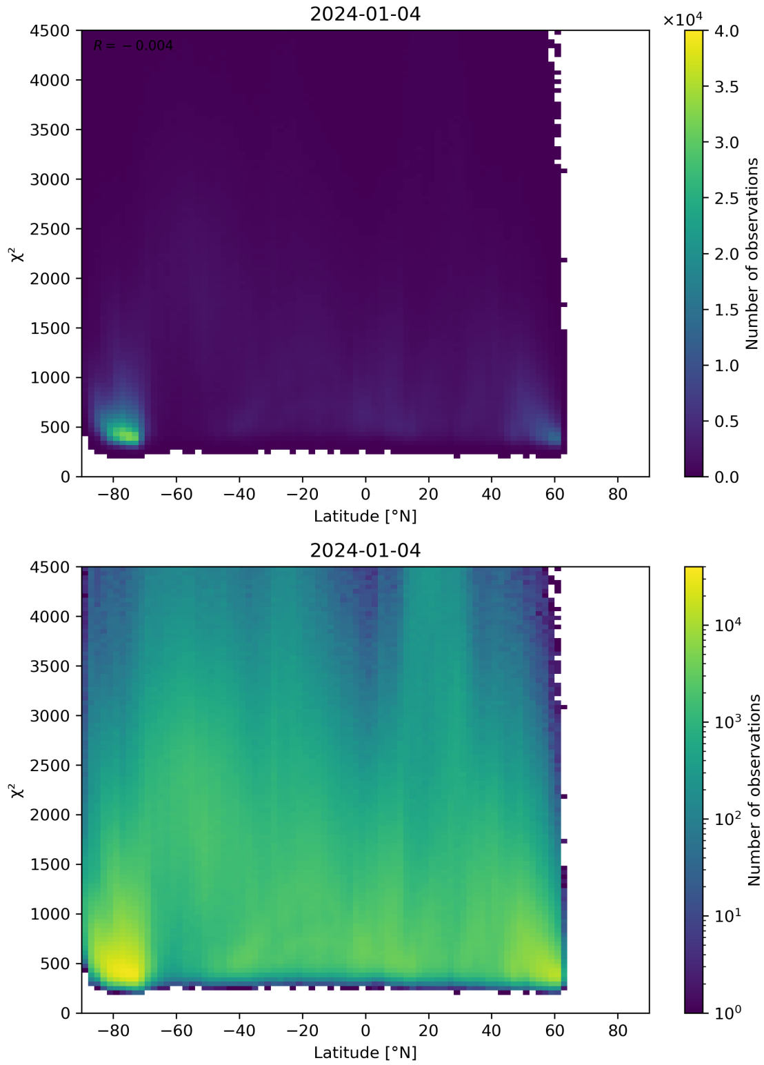
Figure 54: Scatter density plot of “Latitude” against “ \chi^2 ” for 2024-01-03 to 2024-01-05.
