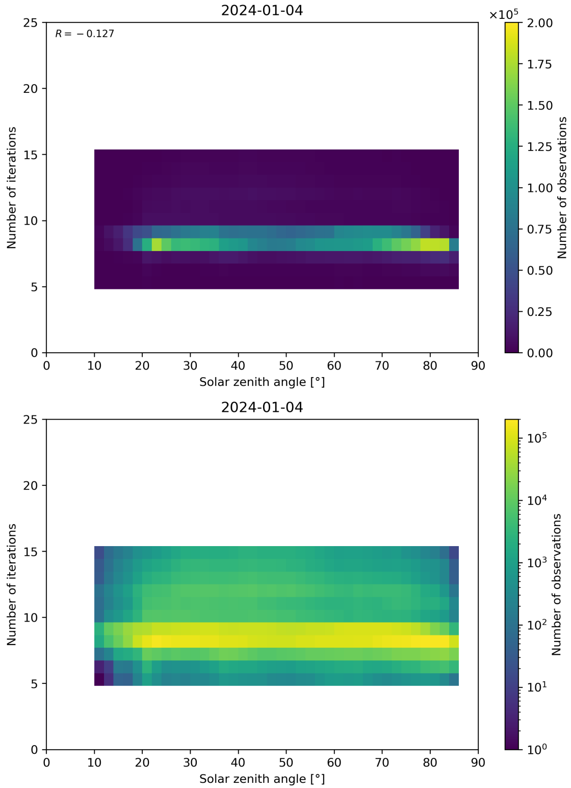
Figure 67: Scatter density plot of “Solar zenith angle” against “Number of iterations” for 2024-01-03 to 2024-01-05.
