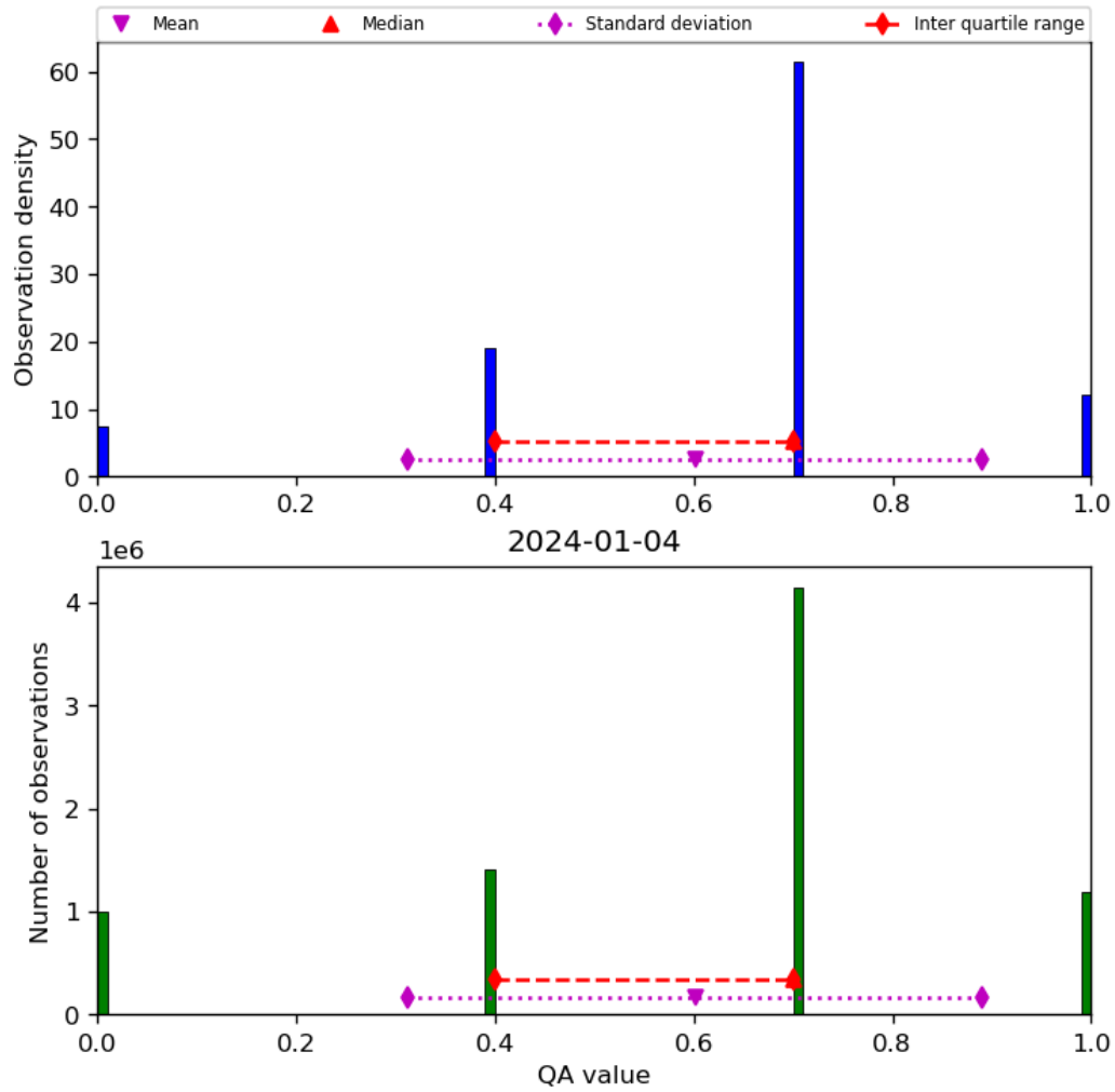
Figure 17: Histogram of “QA value” for 2024-01-03 to 2024-01-05
