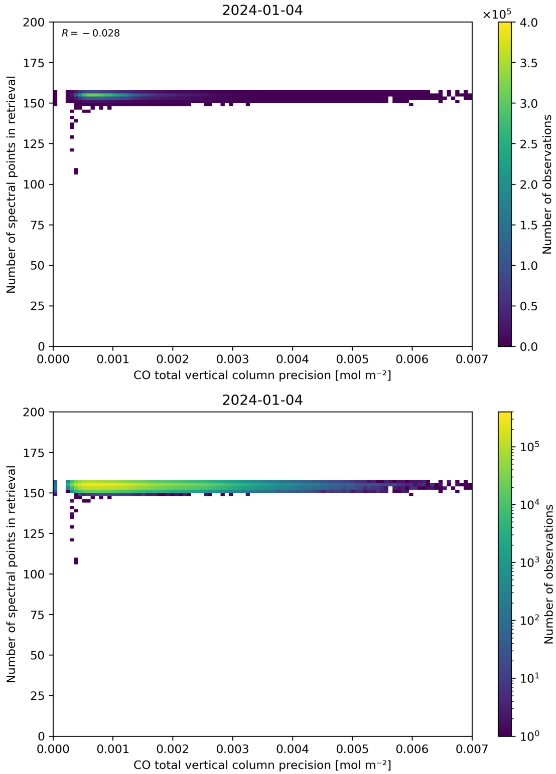
Figure 47: Scatter density plot of “CO total vertical column precision” against “Number of spectral points in retrieval” for 2024-01-03 to 2024-01-05.
