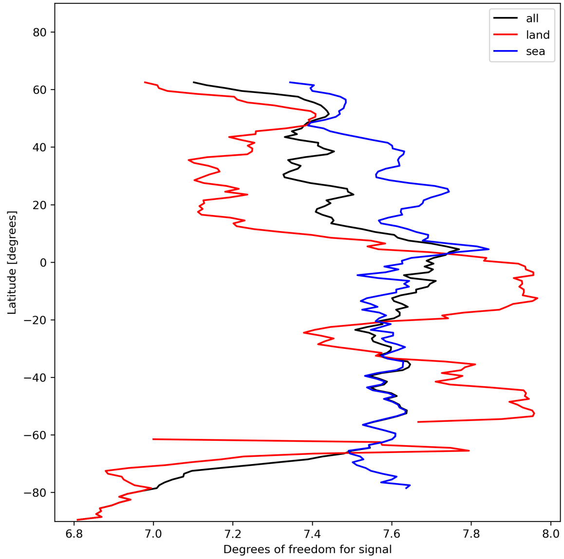
Figure 15: Zonal average of “Degrees of freedom for signal” for 2024-01-03 to 2024-01-05.
