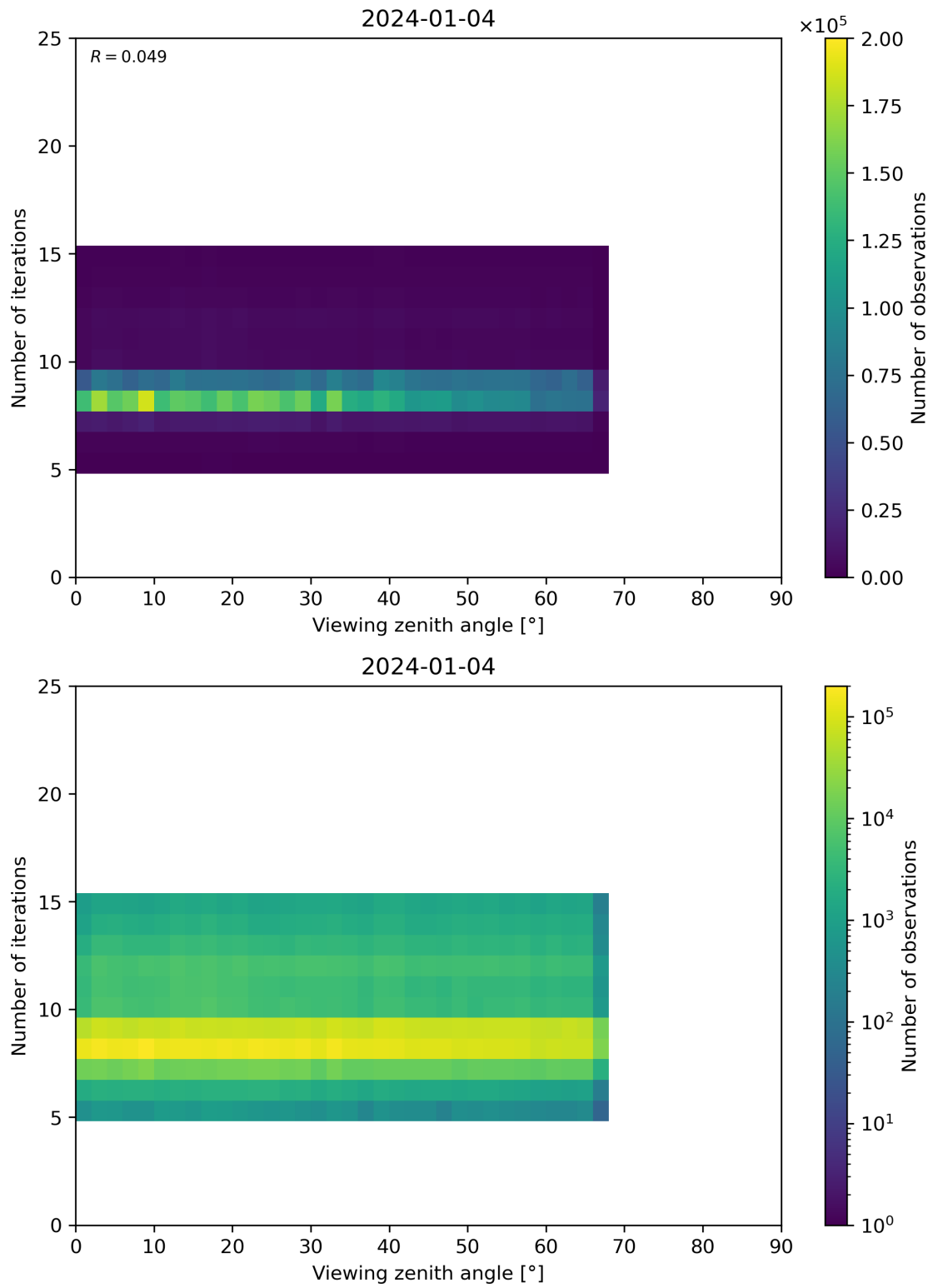
Figure 75: Scatter density plot of “Viewing zenith angle” against “Number of iterations” for 2024-01-03 to 2024-01-05.
