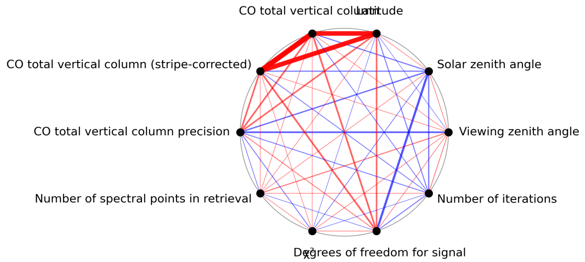
Figure 1: Map of correlation graph for 2024-01-03 to 2024-01-05.
