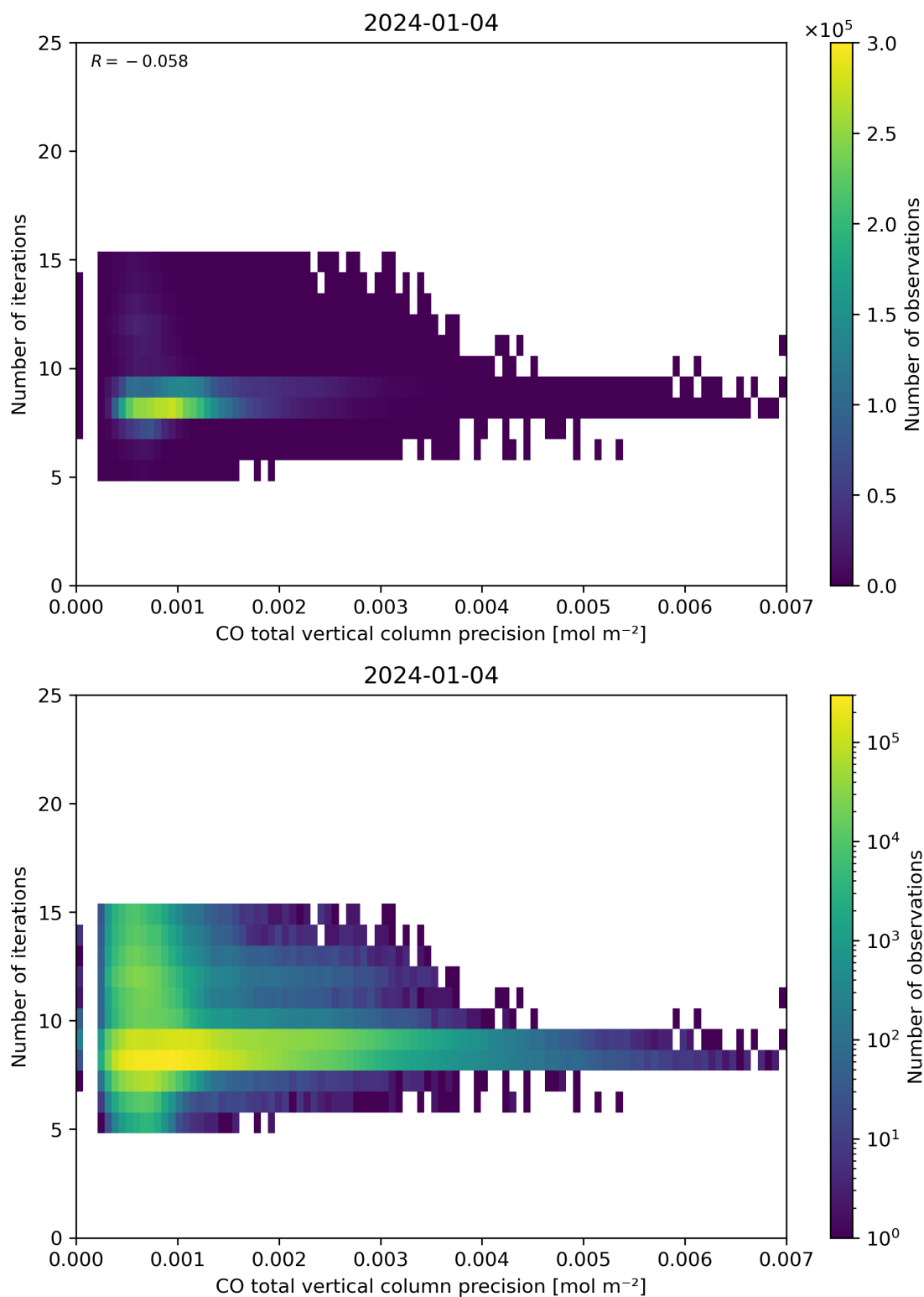
Figure 46: Scatter density plot of “CO total vertical column precision” against “Number of iterations” for 2024-01-03 to 2024-01-05.
