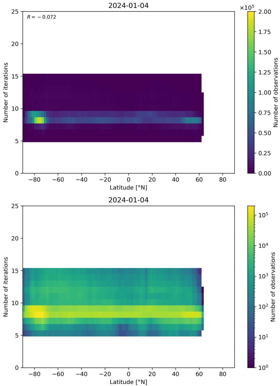
Figure 56: Scatter density plot of “Latitude” against “Number of iterations” for 2024-01-03 to 2024-01-05.
