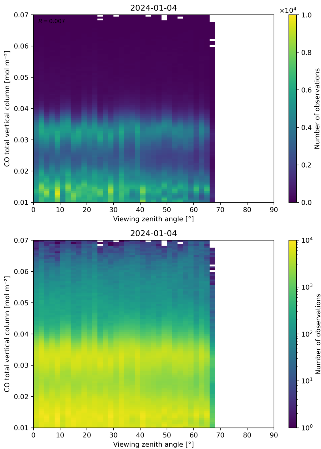
Figure 69: Scatter density plot of “Viewing zenith angle” against “CO total vertical column” for 2024-01-03 to 2024-01-05.
