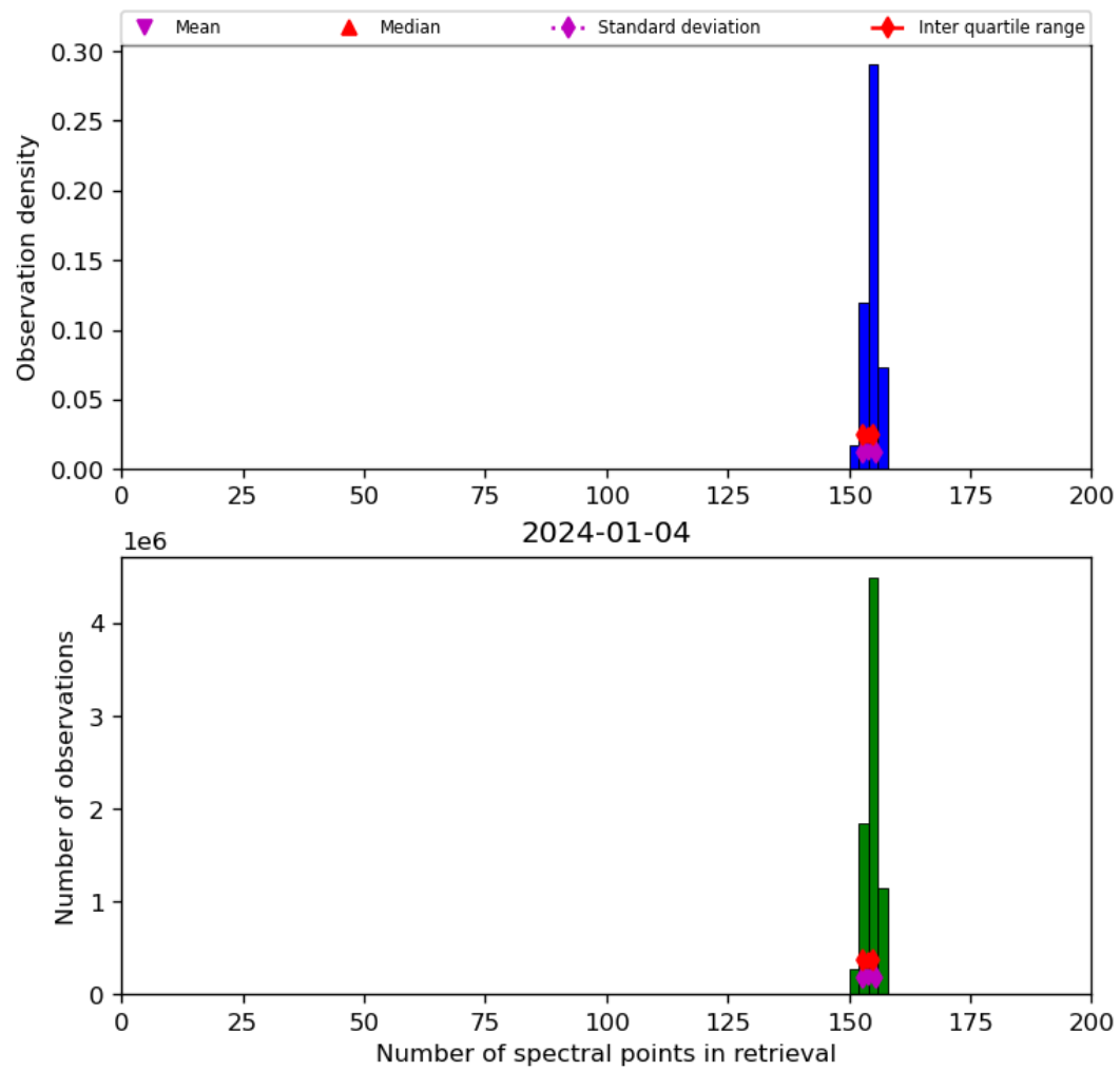
Figure 21: Histogram of “Number of spectral points in retrieval” for 2024-01-03 to 2024-01-05
