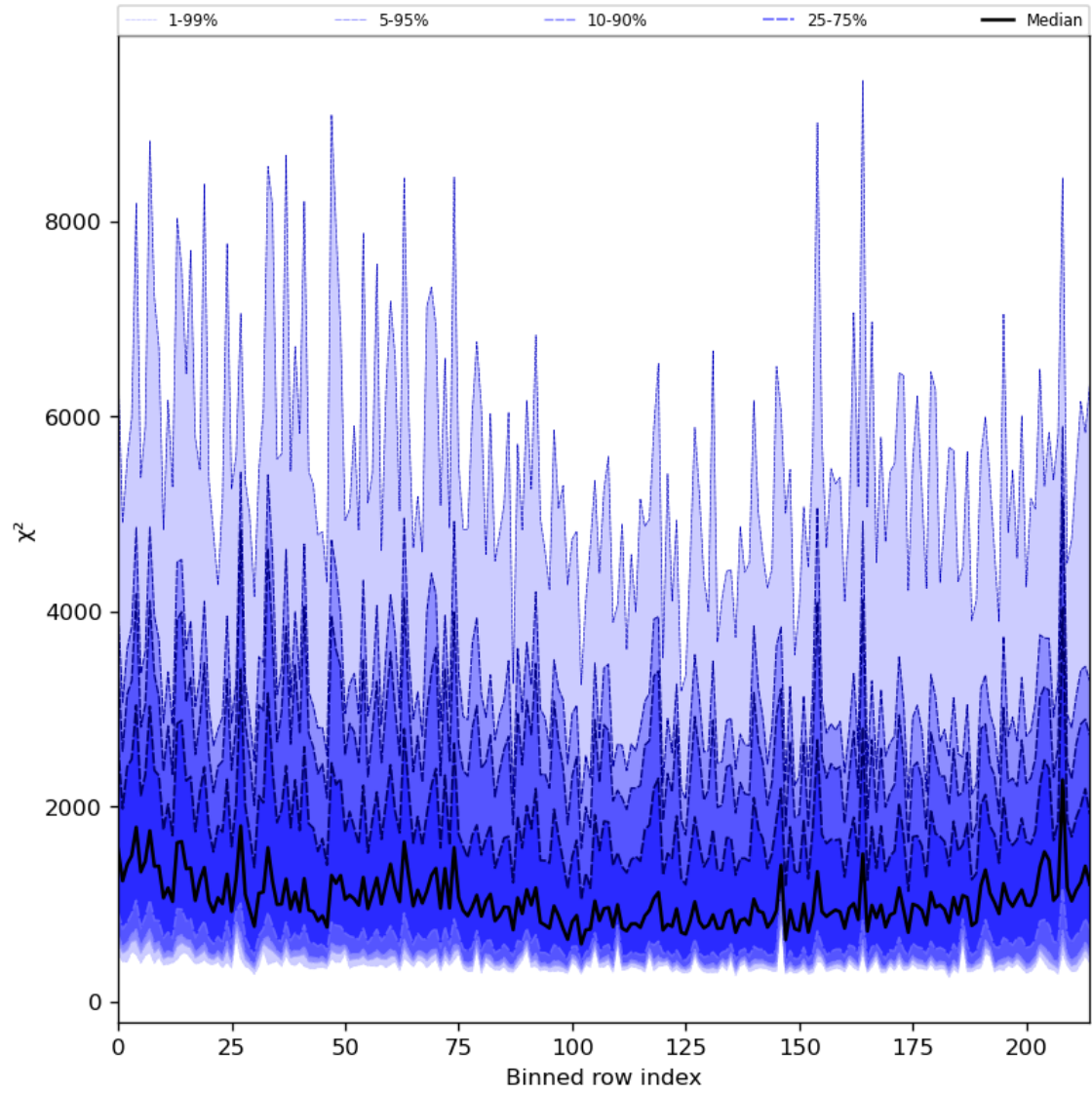
Figure 30: Along track statistics of “ \chi^2 ” for 2024-01-03 to 2024-01-05
