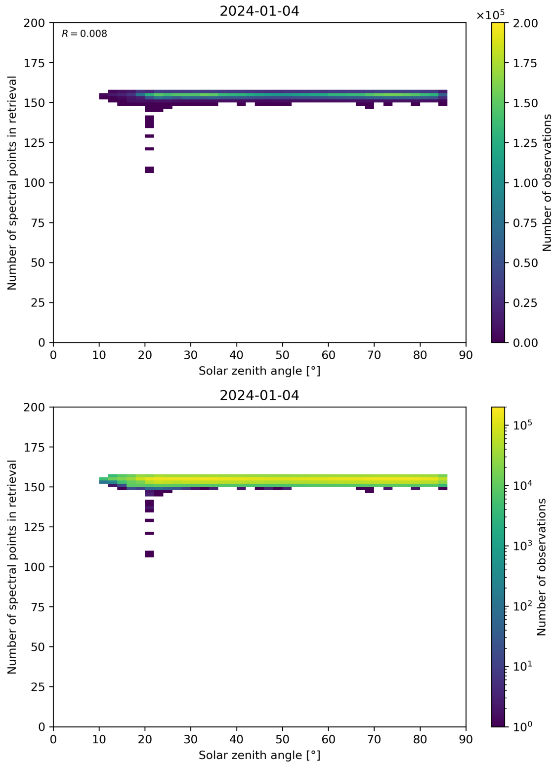
Figure 68: Scatter density plot of “Solar zenith angle” against “Number of spectral points in retrieval” for 2024-01-03 to 2024-01-05.
