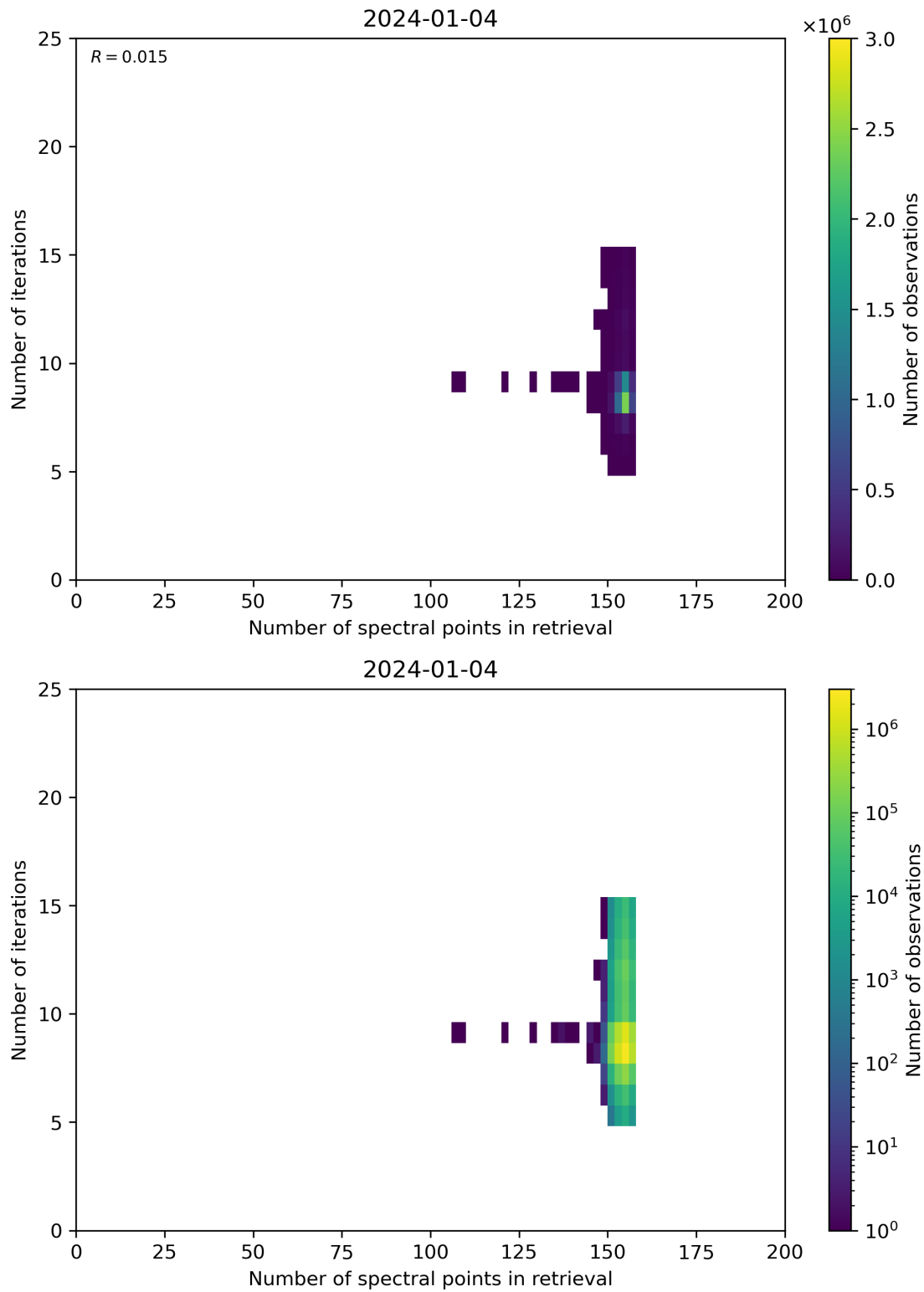
Figure 60: Scatter density plot of “Number of spectral points in retrieval” against “Number of iterations” for 2024-01-03 to 2024-01-05.
