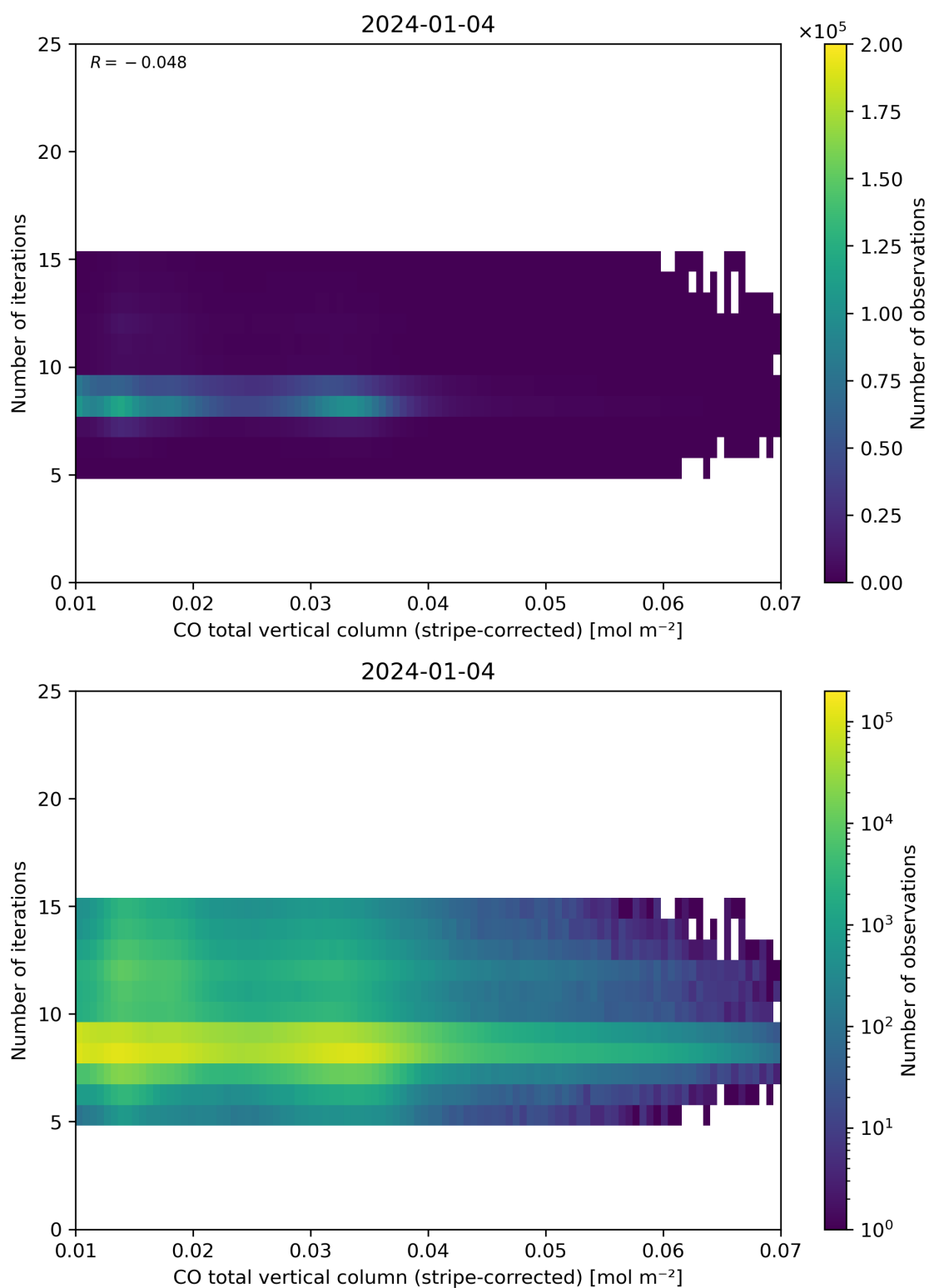
Figure 39: Scatter density plot of “CO total vertical column (stripe-corrected)” against “Number of iterations” for 2024-01-03 to 2024-01-05.
