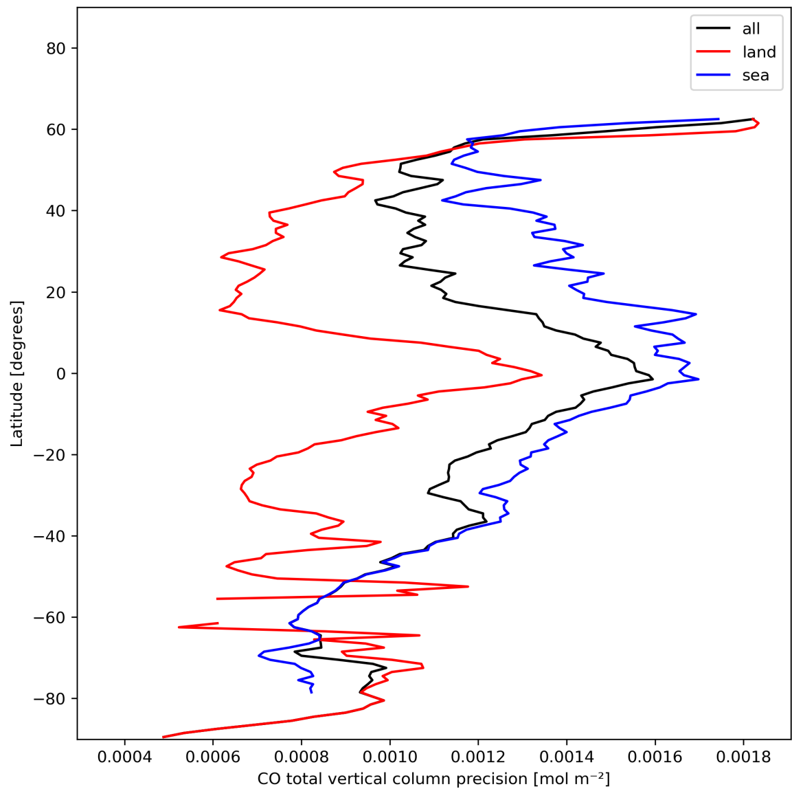
Figure 12: Zonal average of “CO total vertical column precision” for 2024-01-03 to 2024-01-05.
