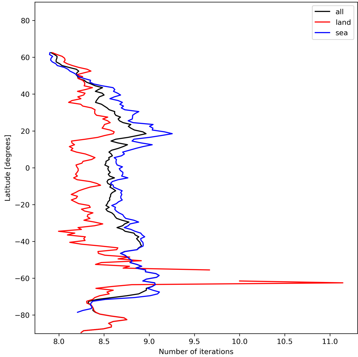
Figure 16: Zonal average of “Number of iterations” for 2024-01-03 to 2024-01-05.
