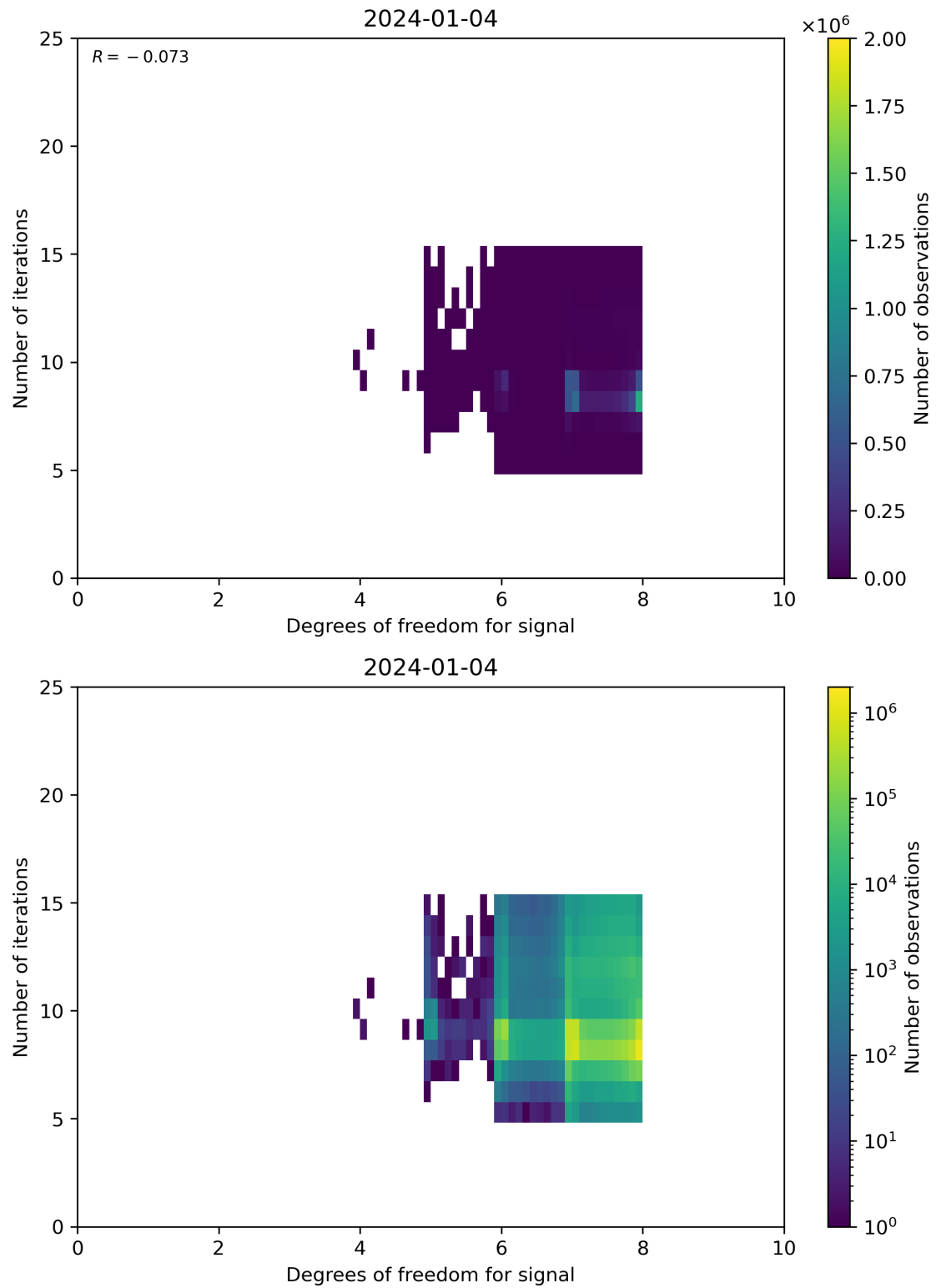
Figure 50: Scatter density plot of “Degrees of freedom for signal” against “Number of iterations” for 2024-01-03 to 2024-01-05.
