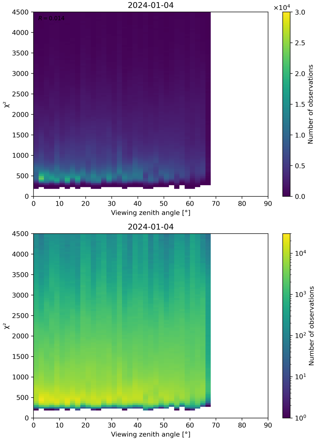
Figure 72: Scatter density plot of “Viewing zenith angle” against “ \chi^2 ” for 2024-01-03 to 2024-01-05.
