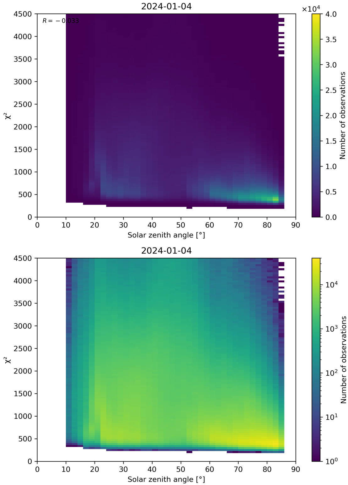
Figure 64: Scatter density plot of “Solar zenith angle” against “ \chi^2 ” for 2024-01-03 to 2024-01-05.
