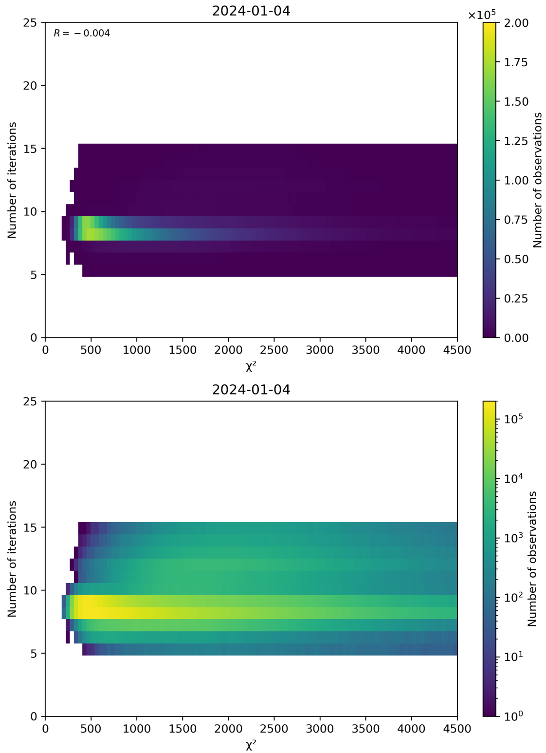
Figure 49: Scatter density plot of “ \chi^2 ” against “Number of iterations” for 2024-01-03 to 2024-01-05.
