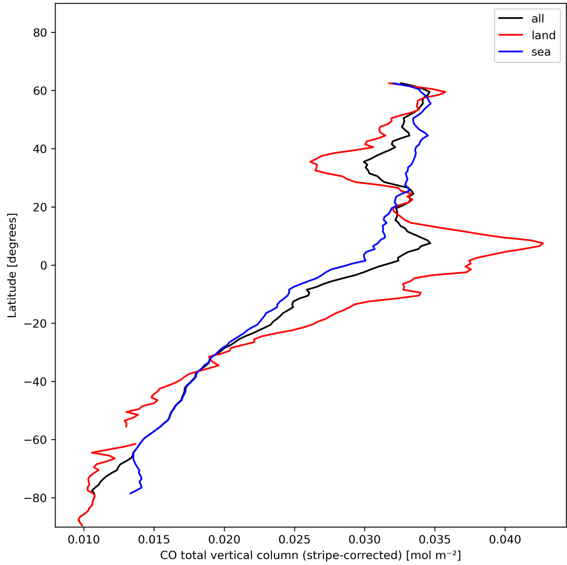
Figure 11: Zonal average of “CO total vertical column (stripe-corrected)” for 2024-01-03 to 2024-01-05.
