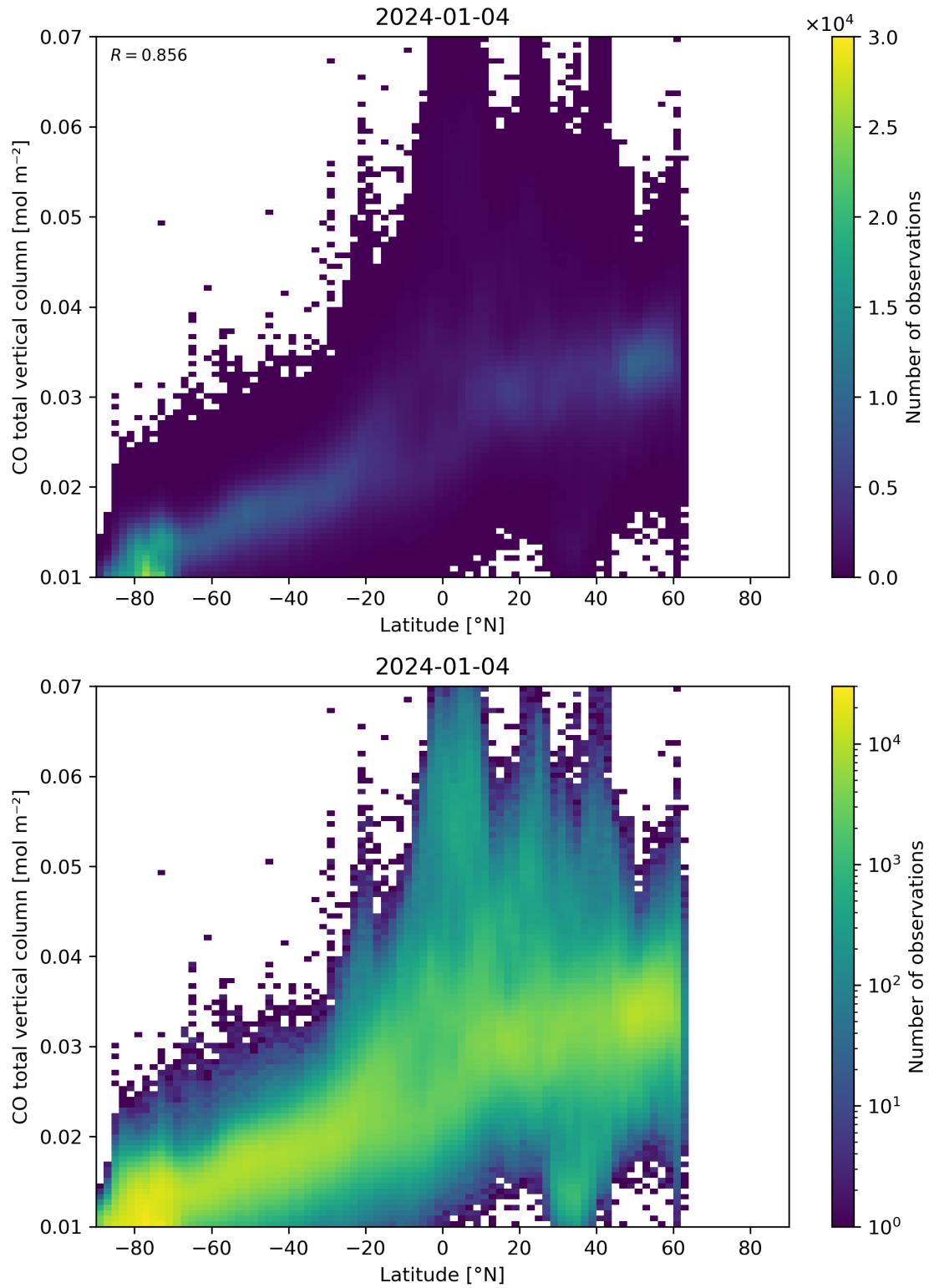
Figure 51: Scatter density plot of “Latitude” against “CO total vertical column” for 2024-01-03 to 2024-01-05.
