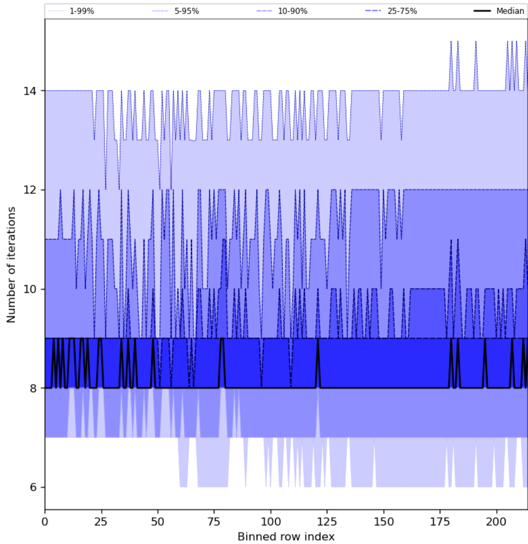
Figure 32: Along track statistics of “Number of iterations” for 2024-01-03 to 2024-01-05
