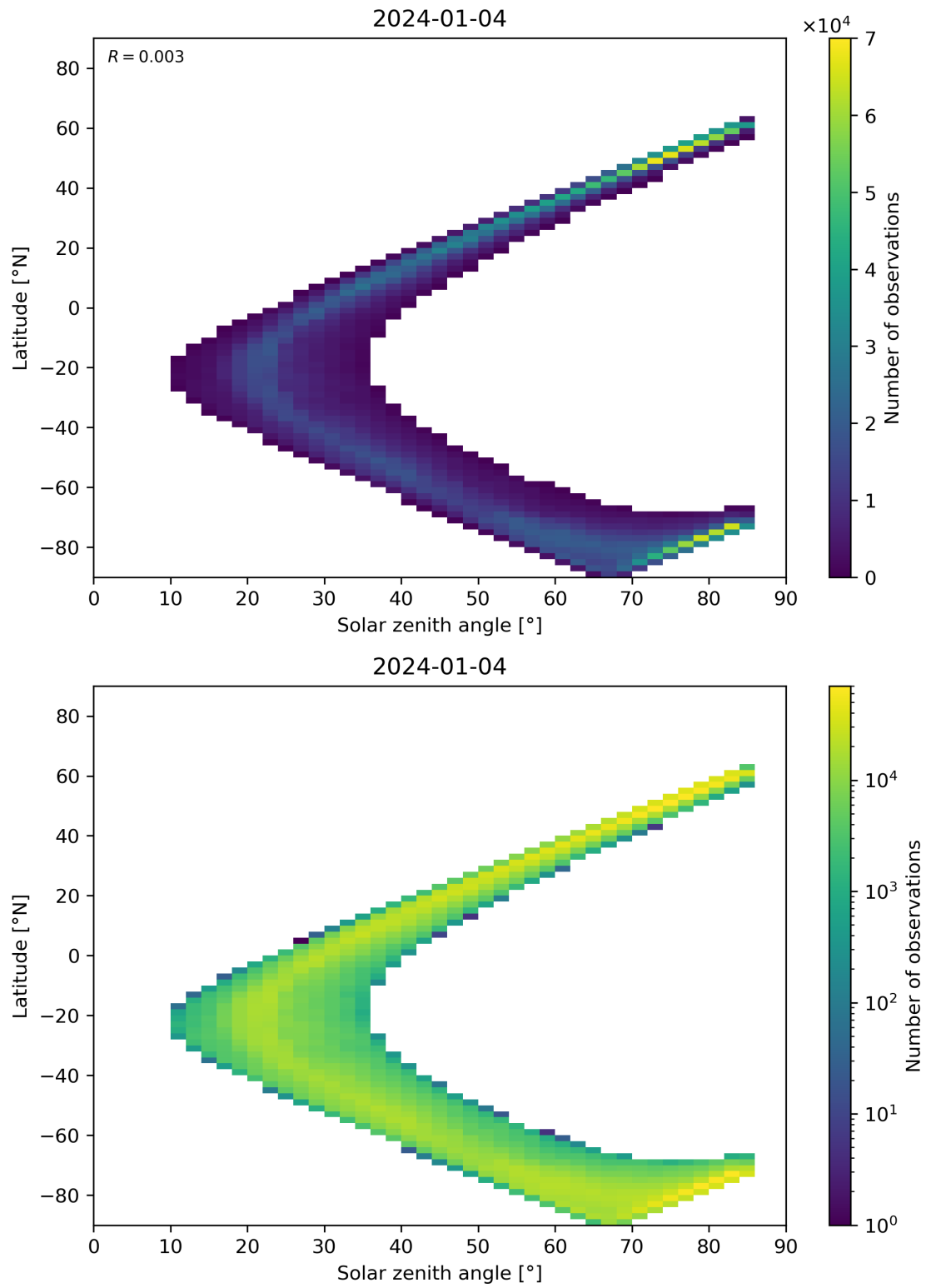
Figure 66: Scatter density plot of “Solar zenith angle” against “Latitude” for 2024-01-03 to 2024-01-05.
