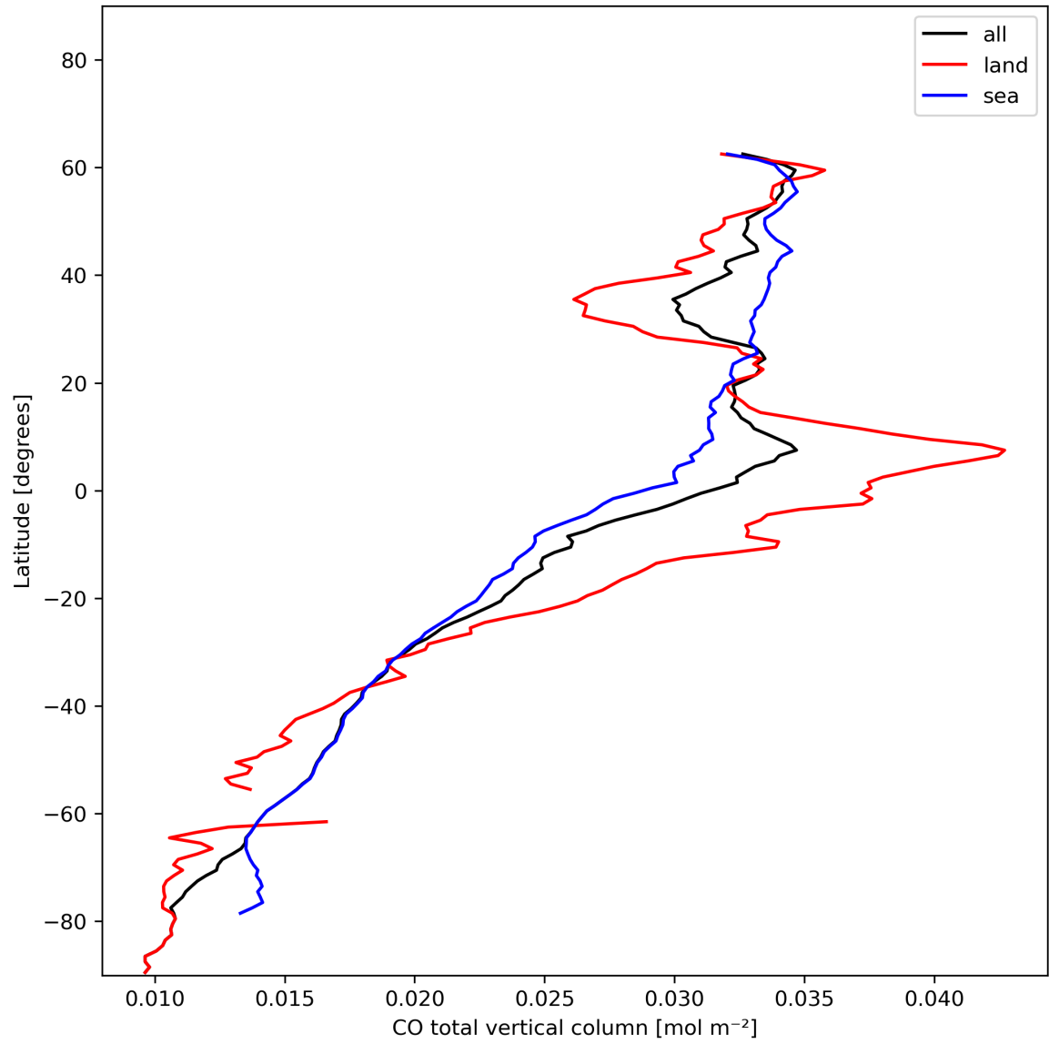
Figure 10: Zonal average of “CO total vertical column” for 2024-01-03 to 2024-01-05.
