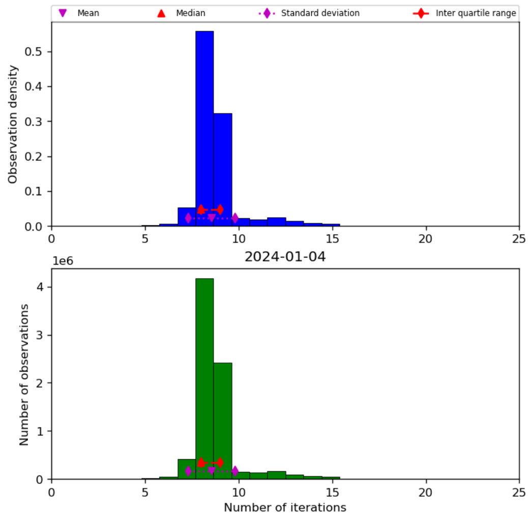
Figure 24: Histogram of “Number of iterations” for 2024-01-03 to 2024-01-05
