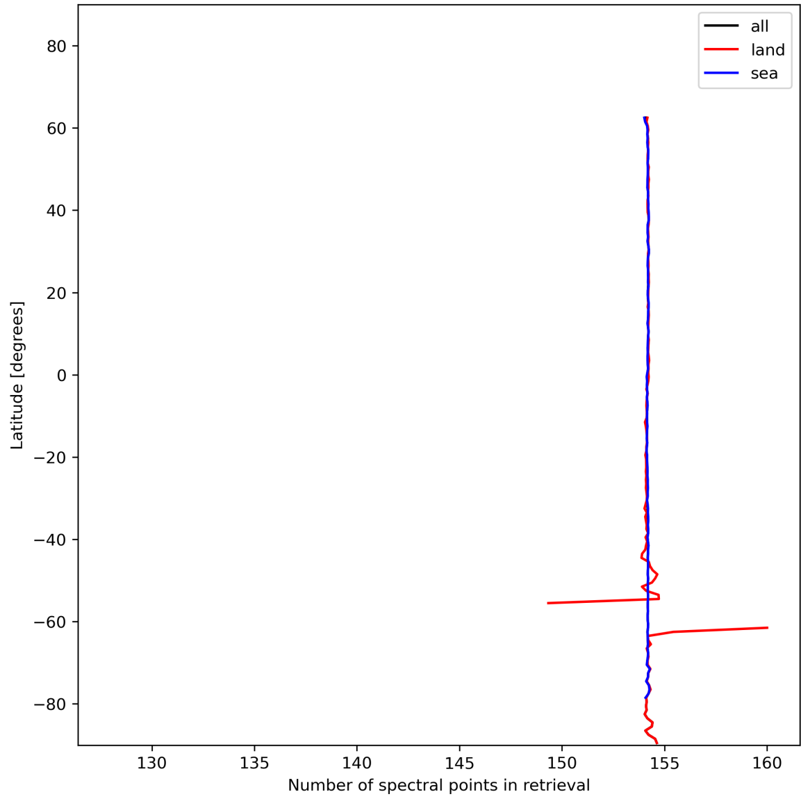
Figure 13: Zonal average of “Number of spectral points in retrieval” for 2024-01-03 to 2024-01-05.
