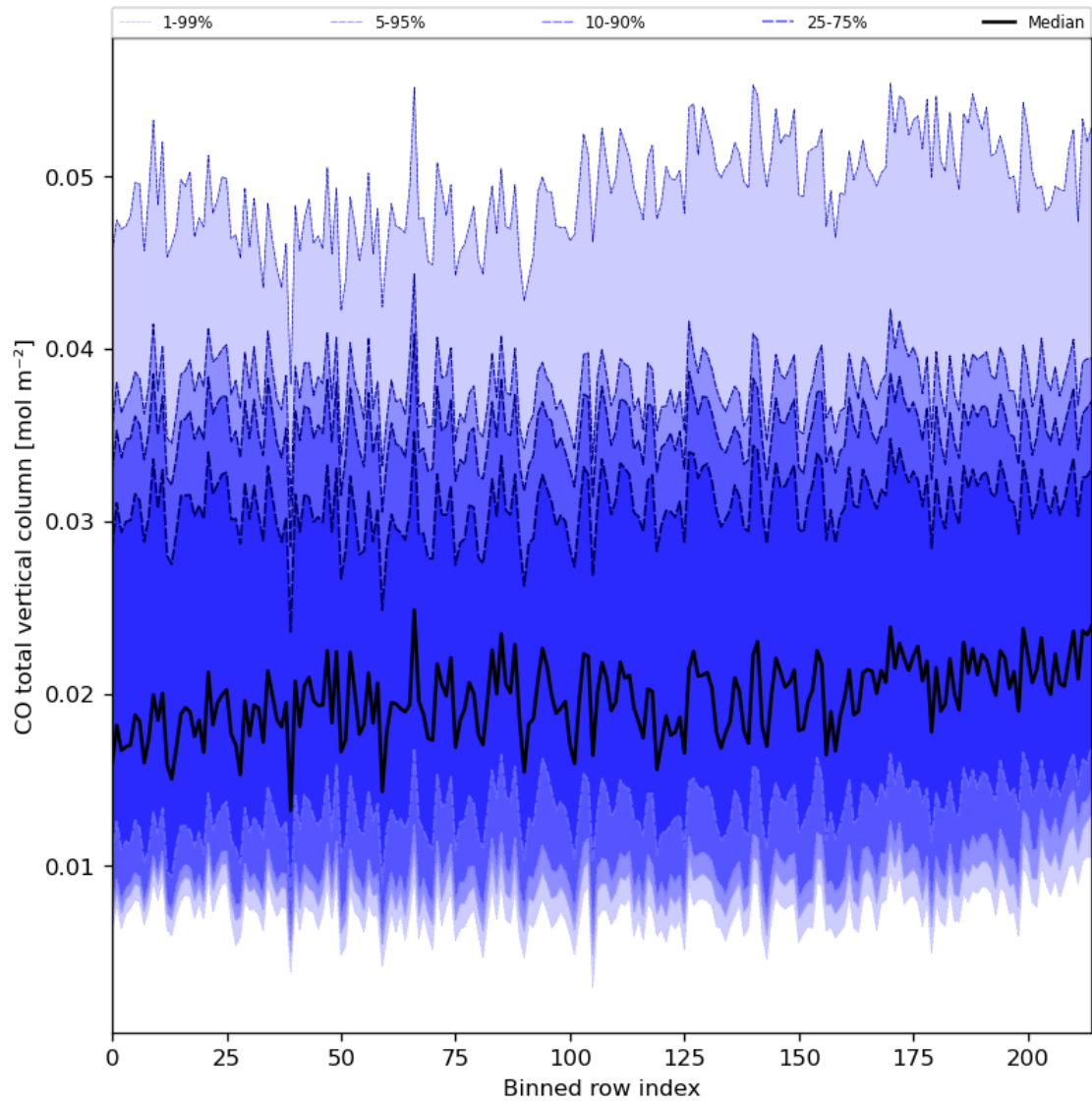
Figure 26: Along track statistics of “CO total vertical column” for 2024-01-03 to 2024-01-05
