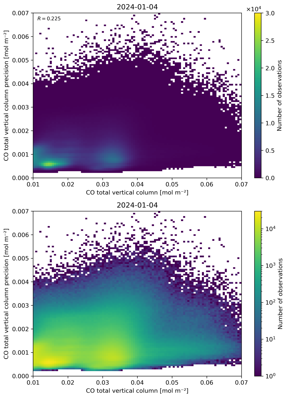
Figure 34: Scatter density plot of “CO total vertical column” against “CO total vertical column precision” for 2024-01-03 to 2024-01-05.
