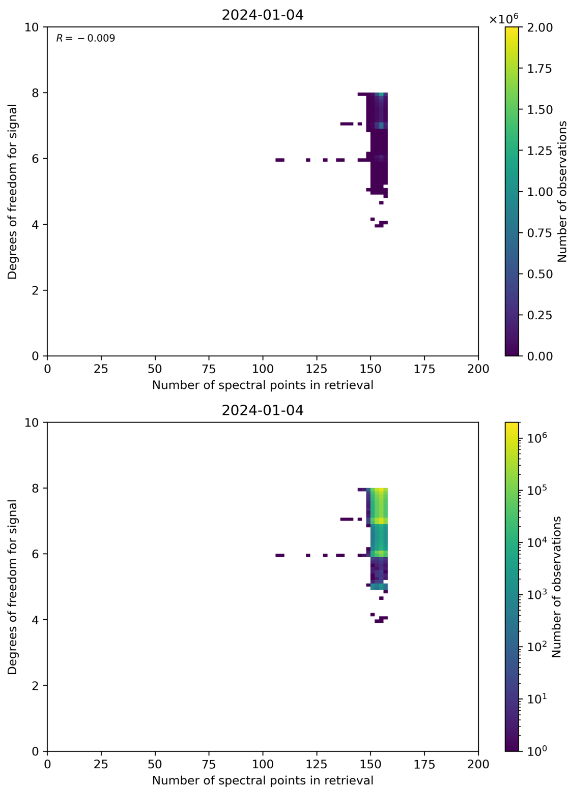
Figure 59: Scatter density plot of “Number of spectral points in retrieval” against “Degrees of freedom for signal” for 2024-01-03 to 2024-01-05.
