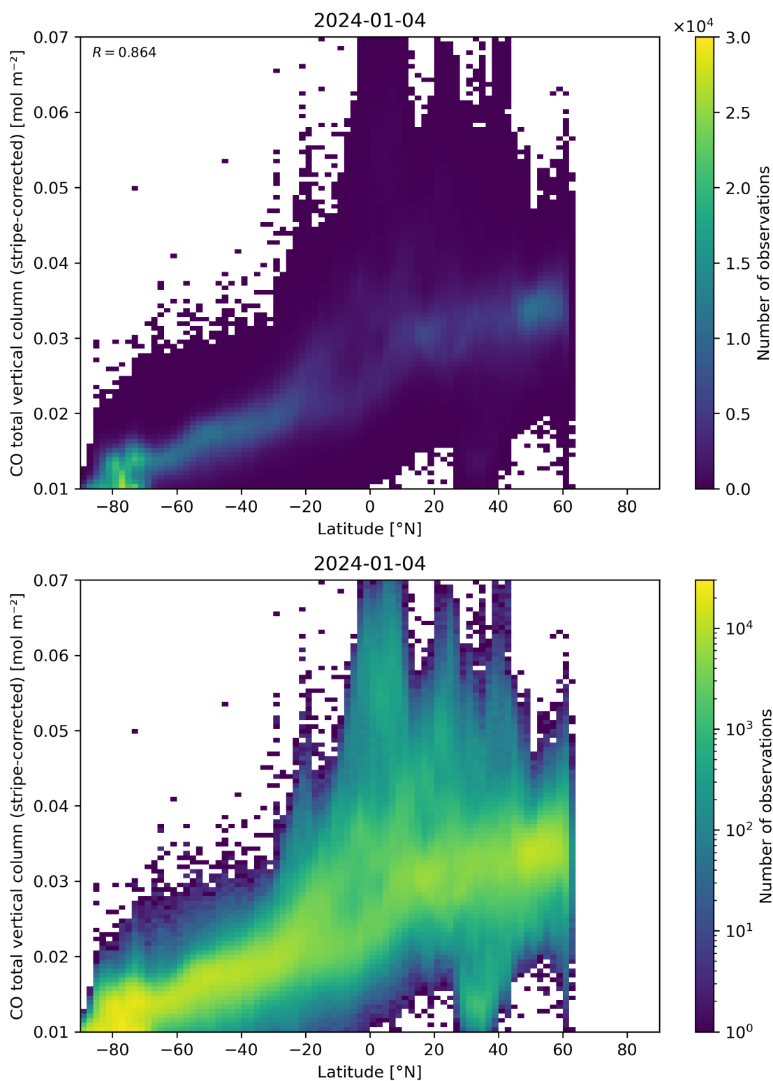
Figure 52: Scatter density plot of “Latitude” against “CO total vertical column (stripe-corrected)” for 2024-01-03 to 2024-01-05.
