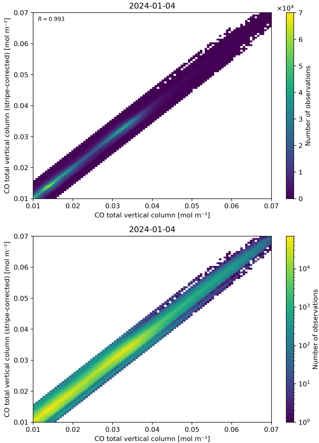
Figure 33: Scatter density plot of “CO total vertical column” against “CO total vertical column (stripe-corrected)” for 2024-01-03 to 2024-01-05.
