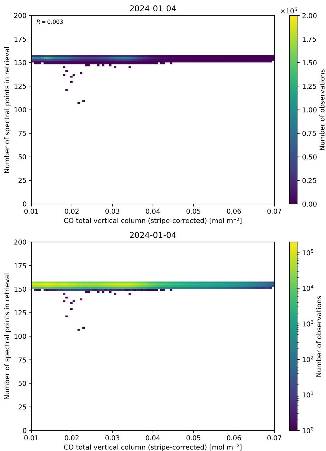
Figure 40: Scatter density plot of “CO total vertical column (stripe-corrected)” against “Number of spectral points in retrieval” for 2024-01-03 to 2024-01-05.
