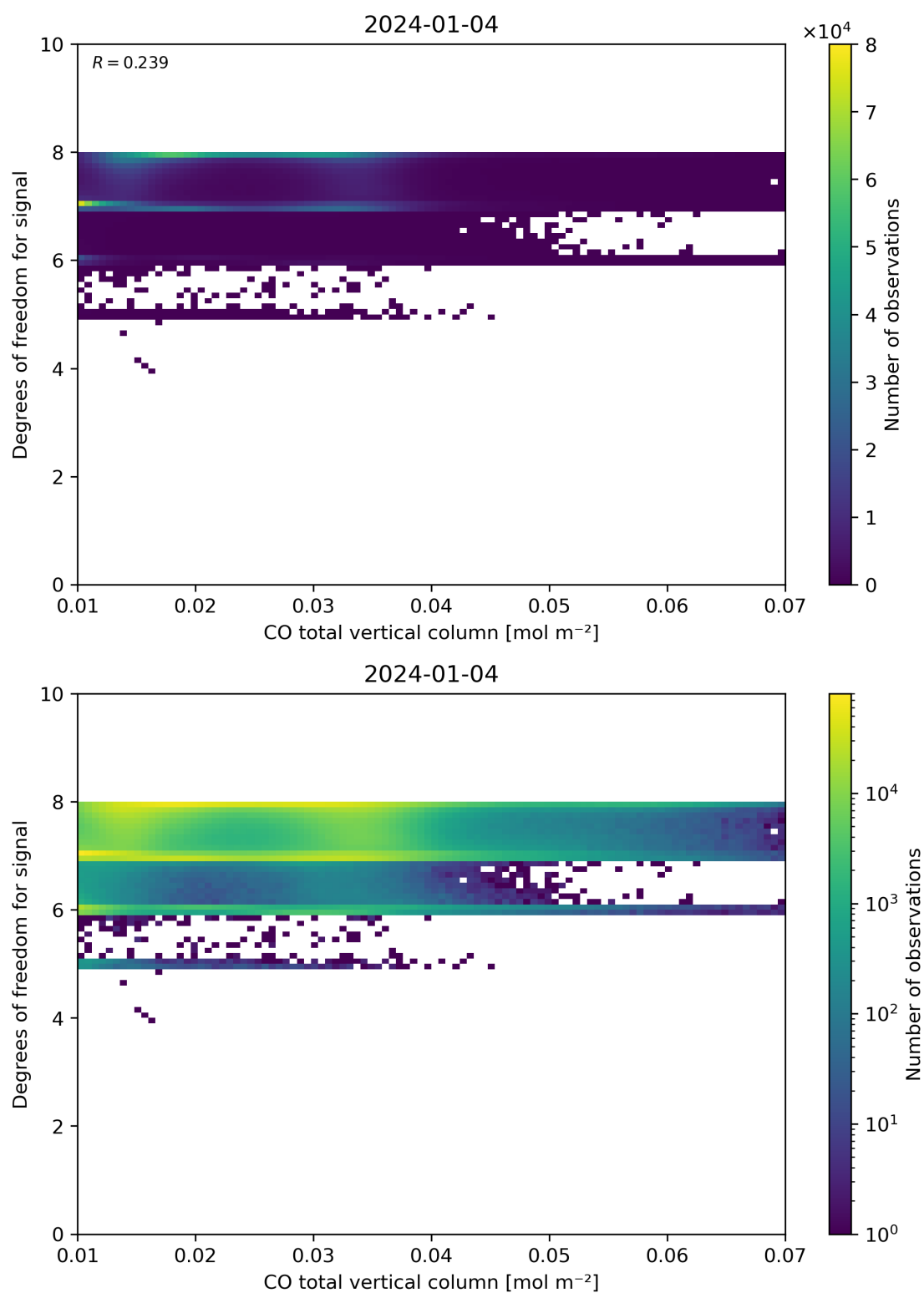
Figure 41: Scatter density plot of “CO total vertical column” against “Degrees of freedom for signal” for 2024-01-03 to 2024-01-05.
