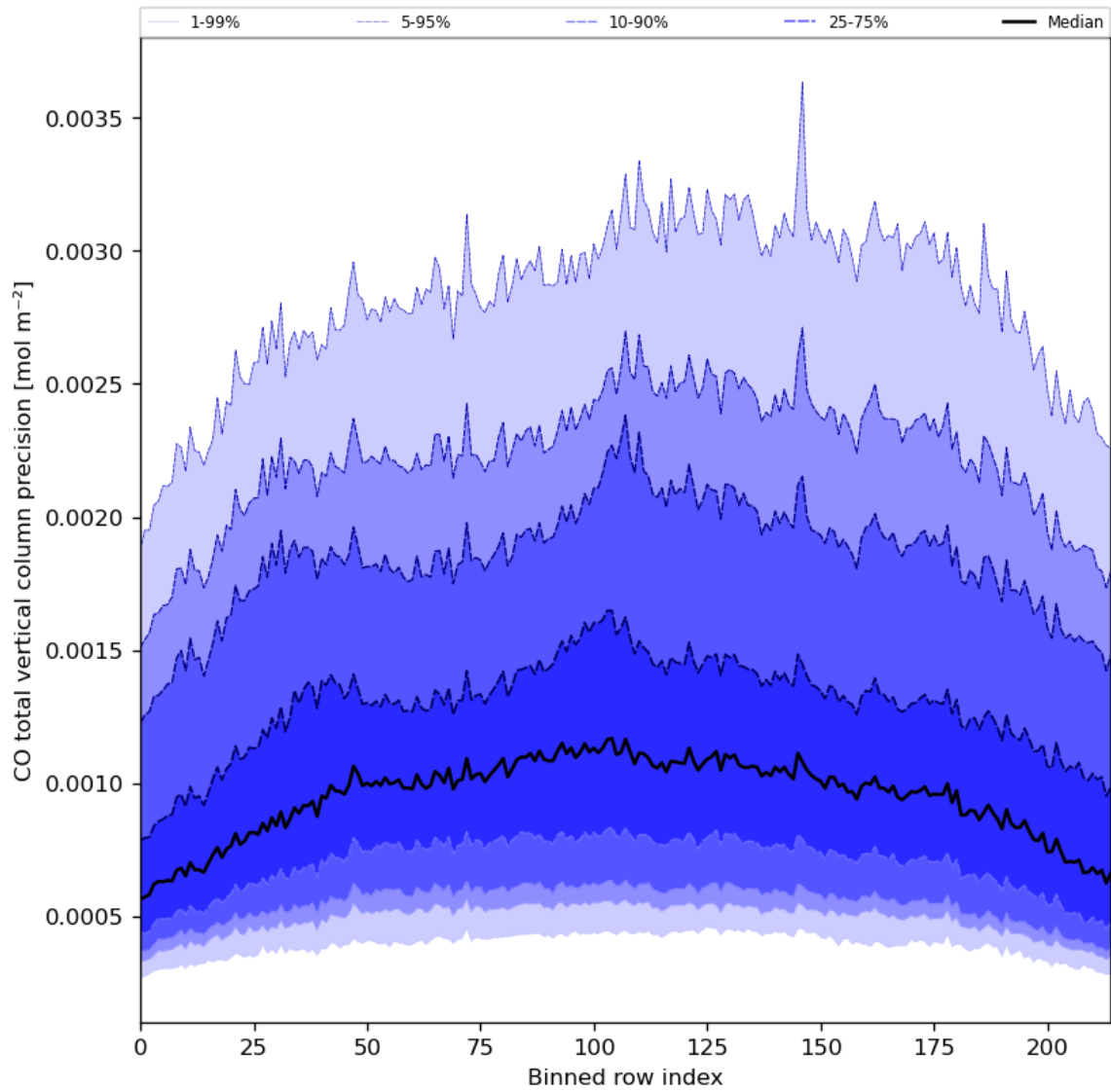
Figure 28: Along track statistics of “CO total vertical column precision” for 2024-01-03 to 2024-01-05
