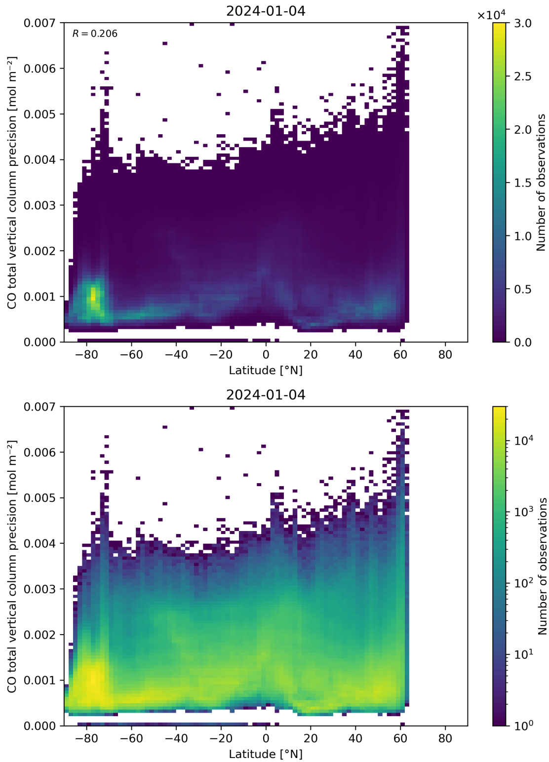
Figure 53: Scatter density plot of “Latitude” against “CO total vertical column precision” for 2024-01-03 to 2024-01-05.
