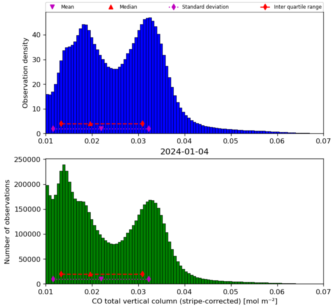
Figure 19: Histogram of “CO total vertical column (stripe-corrected)” for 2024-01-03 to 2024-01-05
