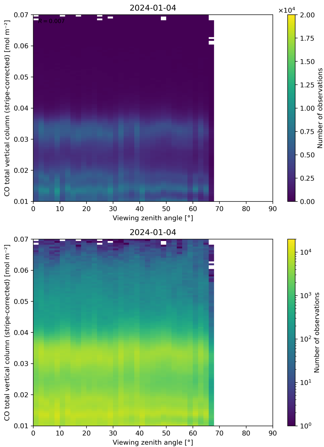
Figure 70: Scatter density plot of “Viewing zenith angle” against “CO total vertical column (stripe-corrected)” for 2024-01-03 to 2024-01-05.
