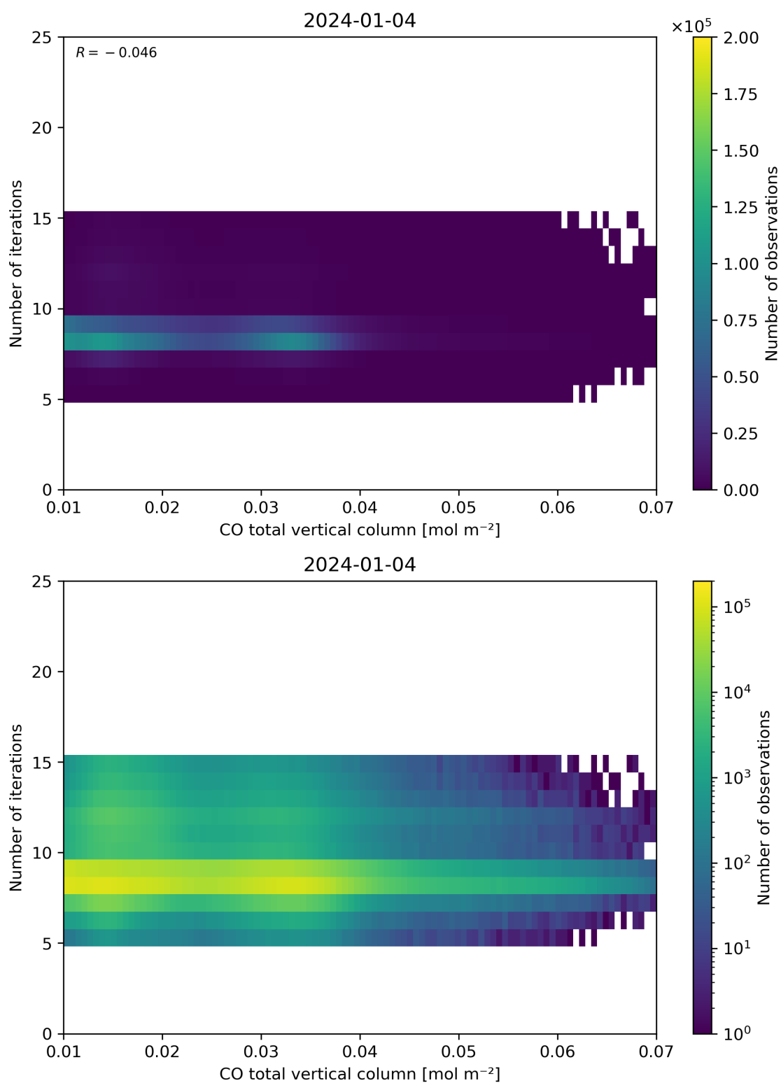
Figure 42: Scatter density plot of “CO total vertical column” against “Number of iterations” for 2024-01-03 to 2024-01-05.
