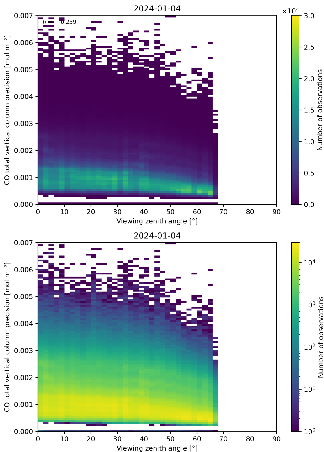
Figure 71: Scatter density plot of “Viewing zenith angle” against “CO total vertical column precision” for 2024-01-03 to 2024-01-05.
