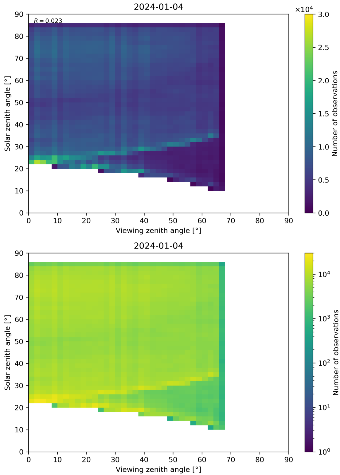
Figure 77: Scatter density plot of “Viewing zenith angle” against “Solar zenith angle” for 2024-01-03 to 2024-01-05.
