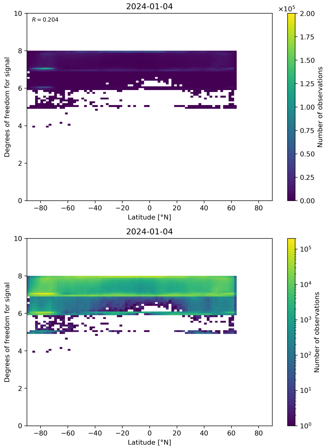
Figure 55: Scatter density plot of “Latitude” against “Degrees of freedom for signal” for 2024-01-03 to 2024-01-05.
