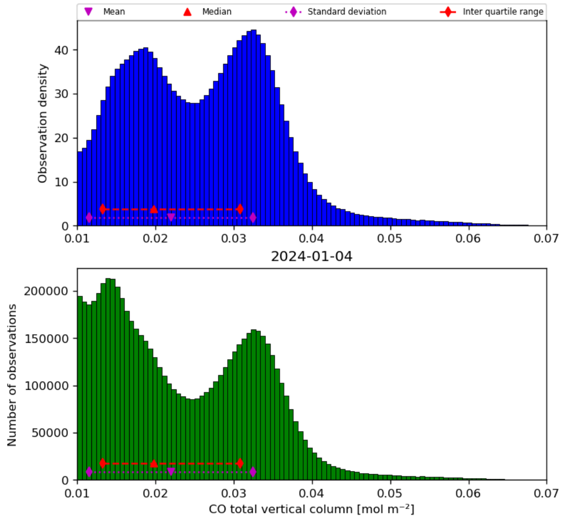
Figure 18: Histogram of “CO total vertical column” for 2024-01-03 to 2024-01-05
