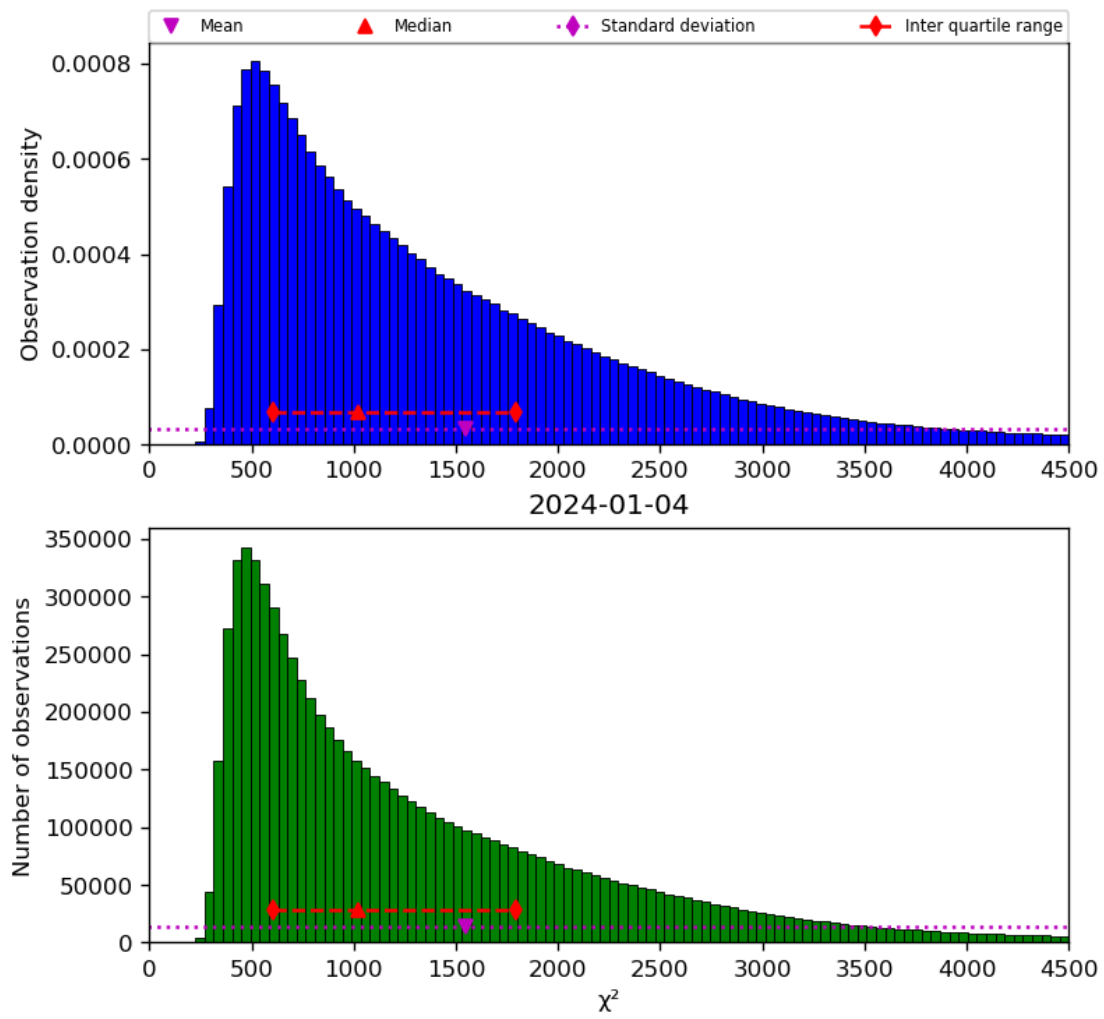
Figure 22: Histogram of “ \chi^2 ” for 2024-01-03 to 2024-01-05
