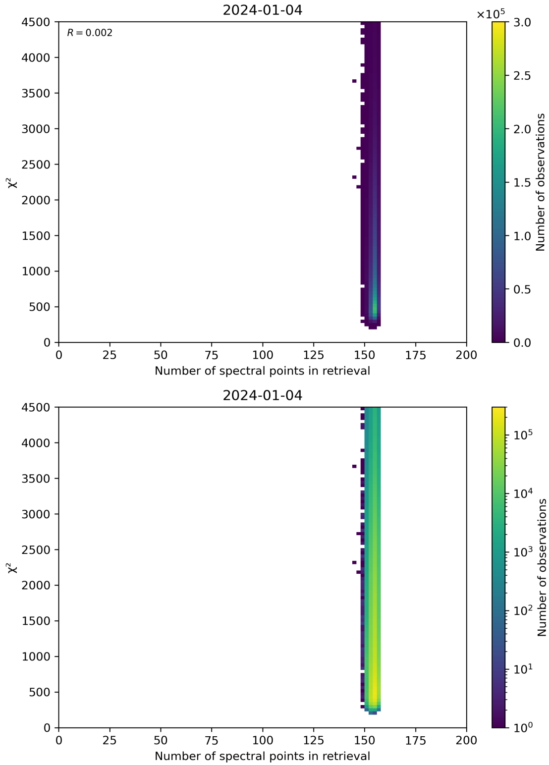
Figure 58: Scatter density plot of “Number of spectral points in retrieval” against “ \chi^2 ” for 2024-01-03 to 2024-01-05.
