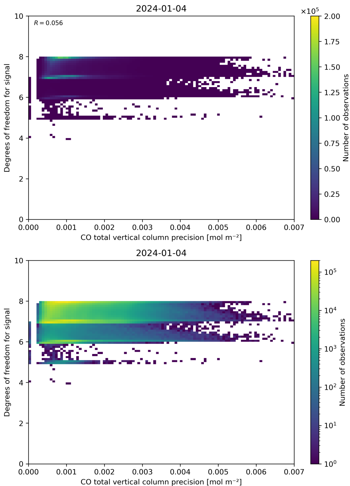
Figure 45: Scatter density plot of “CO total vertical column precision” against “Degrees of freedom for signal” for 2024-01-03 to 2024-01-05.
