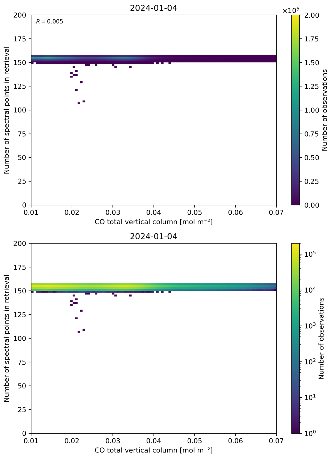
Figure 43: Scatter density plot of “CO total vertical column” against “Number of spectral points in retrieval” for 2024-01-03 to 2024-01-05.
