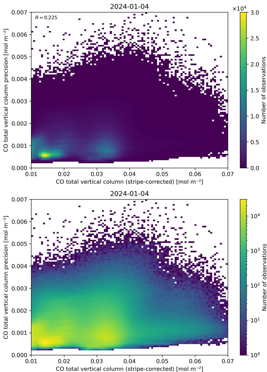
Figure 36: Scatter density plot of “CO total vertical column (stripe-corrected)” against “CO total vertical column precision” for 2024-01-03 to 2024-01-05.
