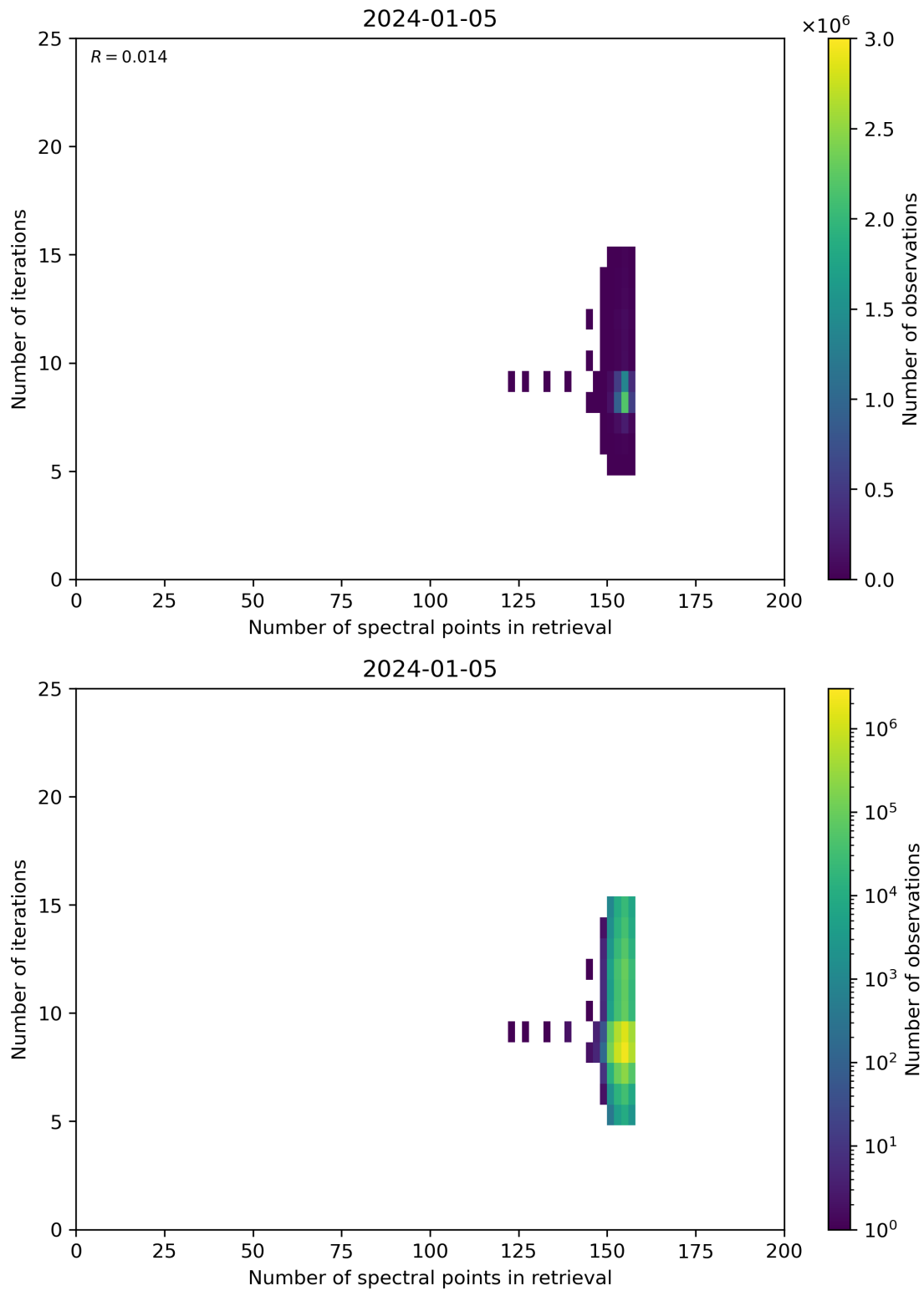
Figure 60: Scatter density plot of “Number of spectral points in retrieval” against “Number of iterations” for 2024-01-05 to 2024-01-06.
