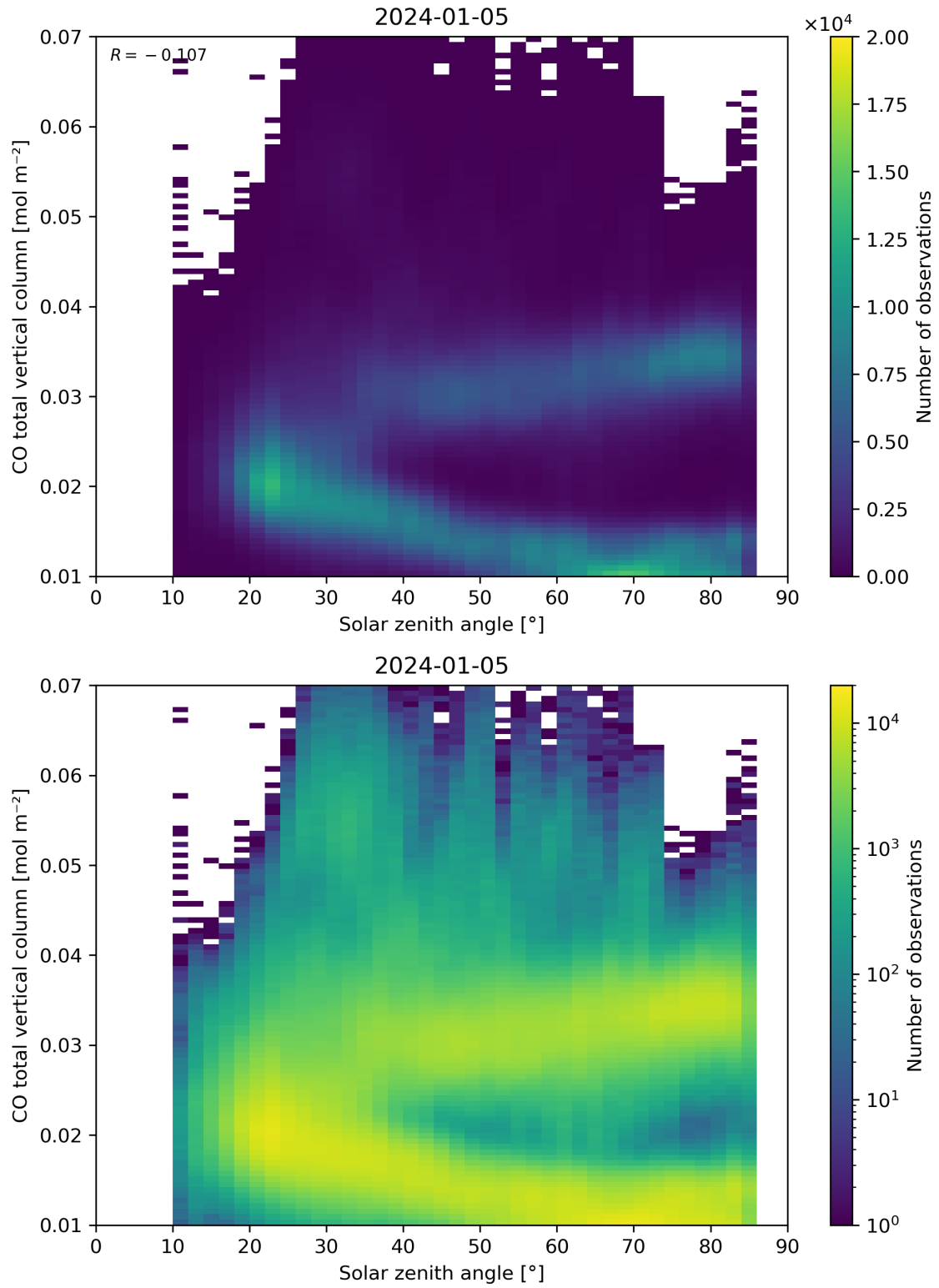
Figure 61: Scatter density plot of “Solar zenith angle” against “CO total vertical column” for 2024-01-05 to 2024-01-06.
