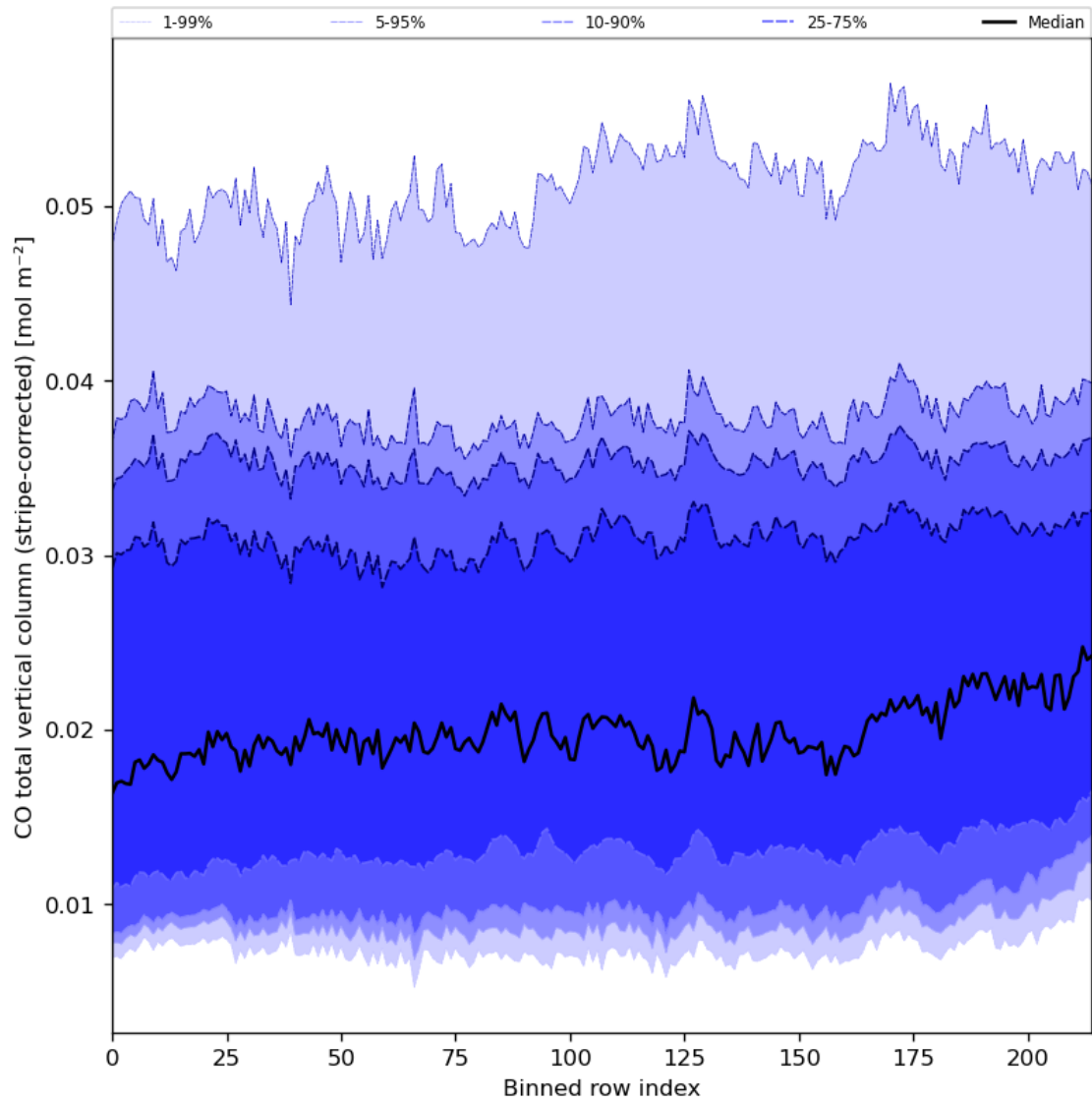
Figure 27: Along track statistics of “CO total vertical column (stripe-corrected)” for 2024-01-05 to 2024-01-06
