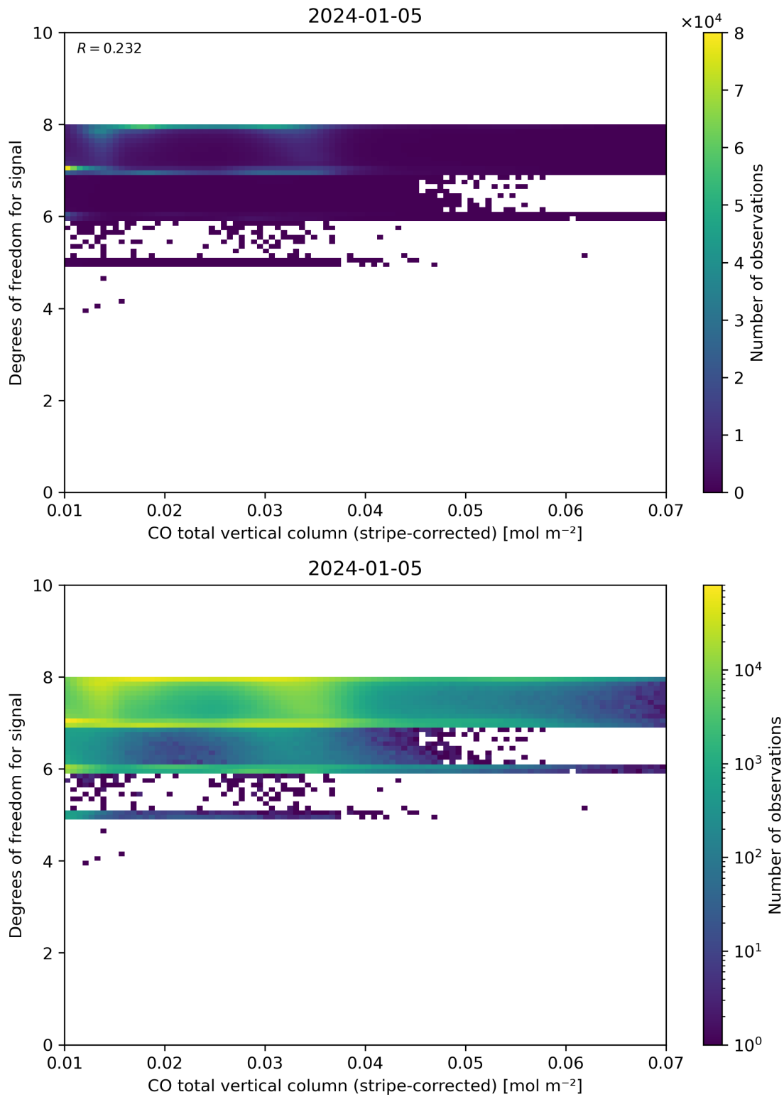
Figure 38: Scatter density plot of “CO total vertical column (stripe-corrected)” against “Degrees of freedom for signal” for 2024-01-05 to 2024-01-06.
