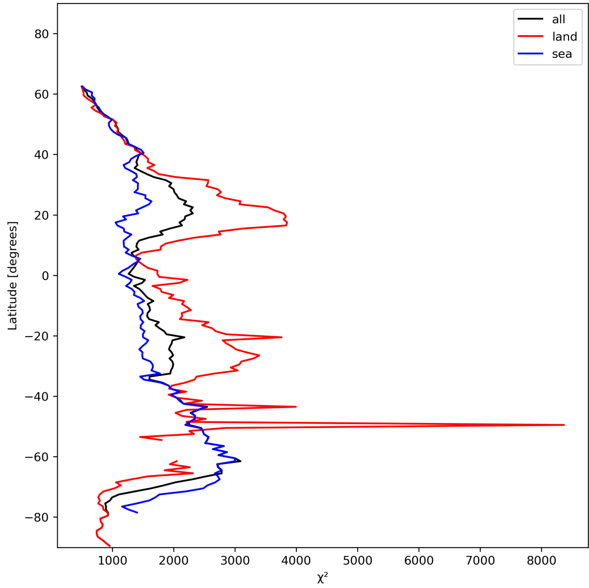
Figure 14: Zonal average of “ \chi^2 ” for 2024-01-05 to 2024-01-06.
