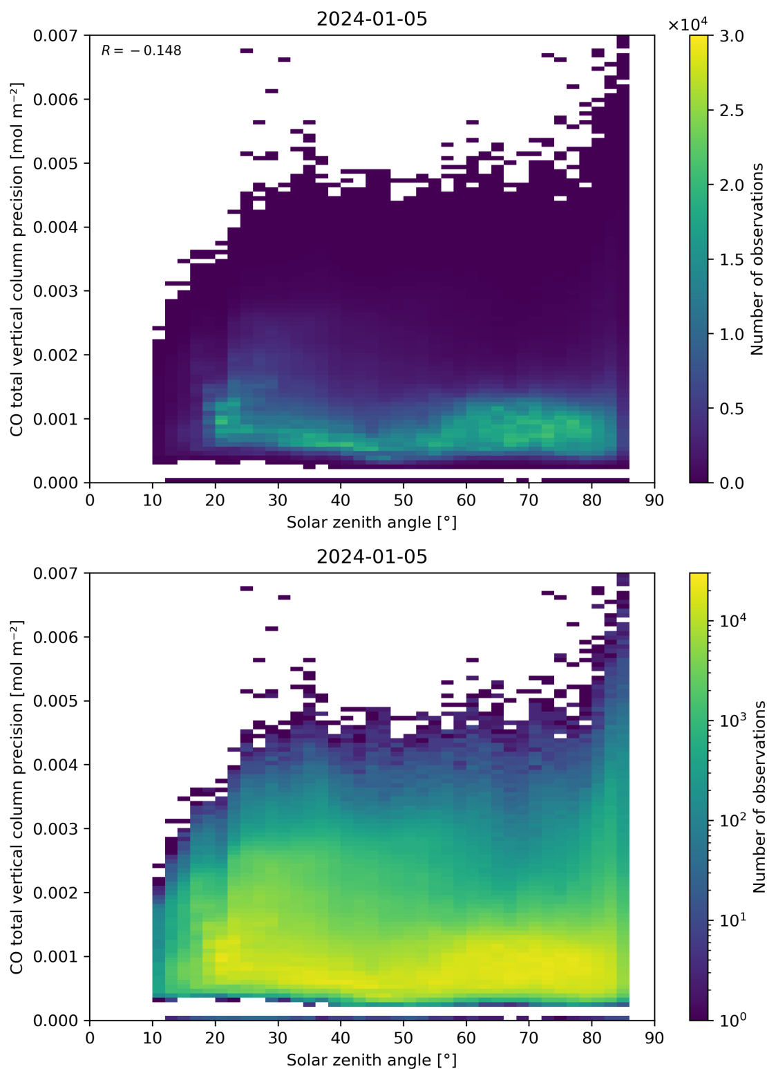
Figure 63: Scatter density plot of “Solar zenith angle” against “CO total vertical column precision” for 2024-01-05 to 2024-01-06.
