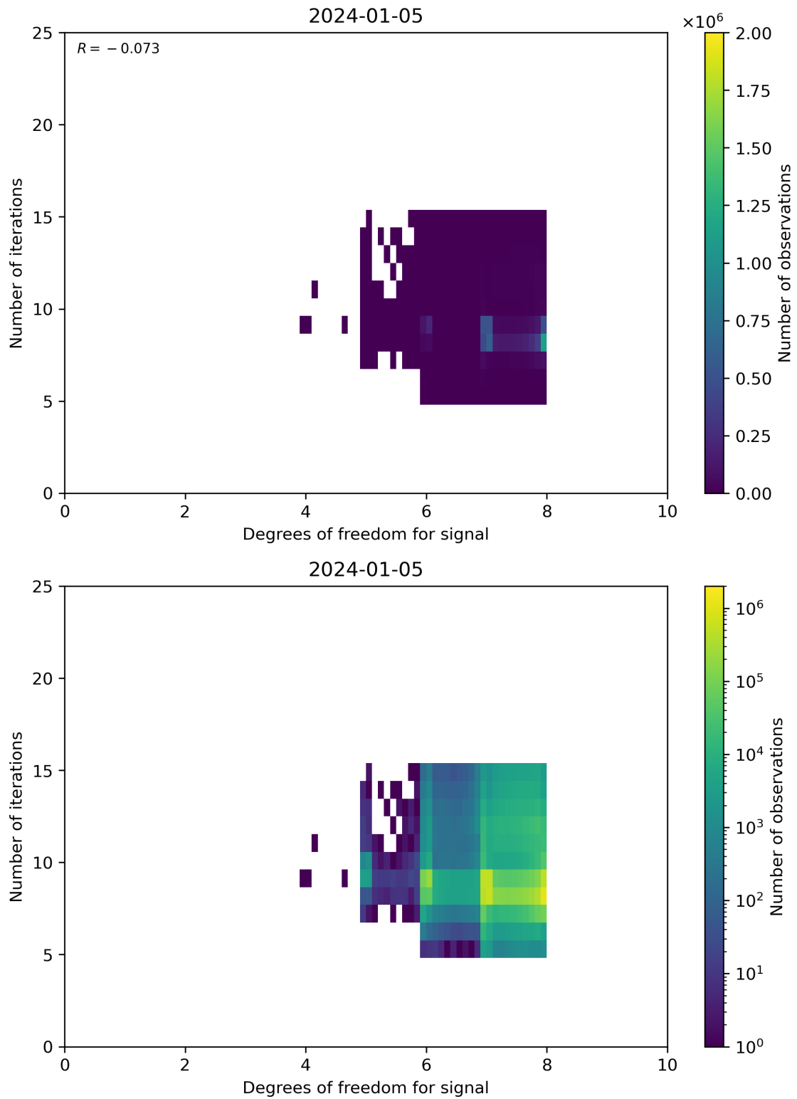
Figure 50: Scatter density plot of “Degrees of freedom for signal” against “Number of iterations” for 2024-01-05 to 2024-01-06.
