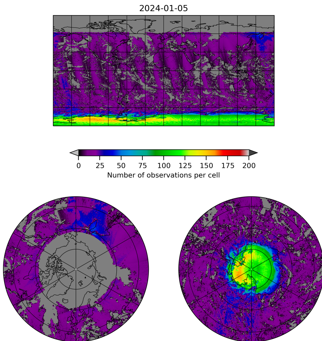
Figure 8: Map of the number of observations for 2024-01-05 to 2024-01-06
