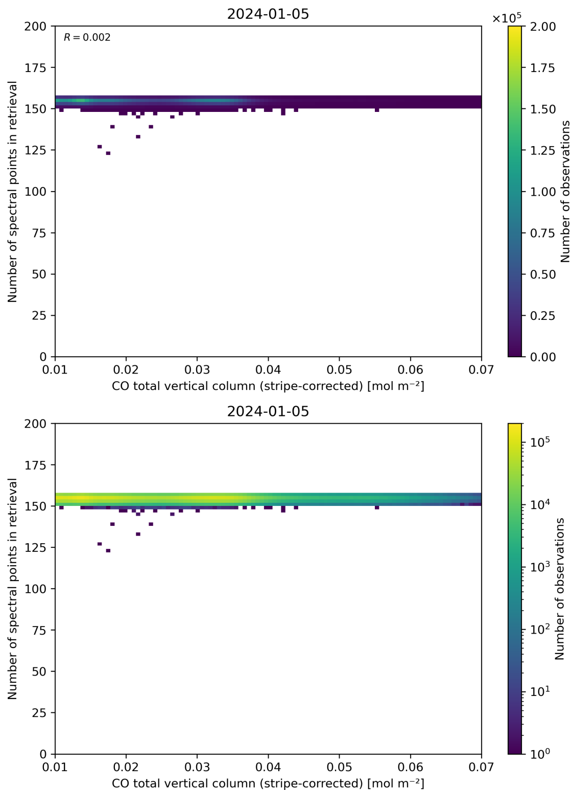
Figure 40: Scatter density plot of “CO total vertical column (stripe-corrected)” against “Number of spectral points in retrieval” for 2024-01-05 to 2024-01-06.
