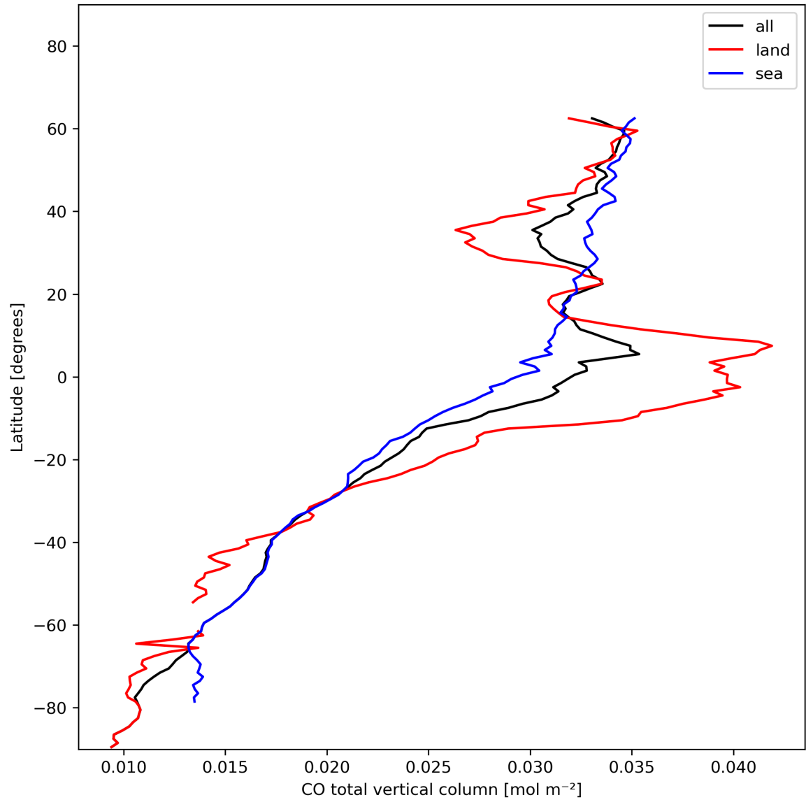
Figure 10: Zonal average of “CO total vertical column” for 2024-01-05 to 2024-01-06.
