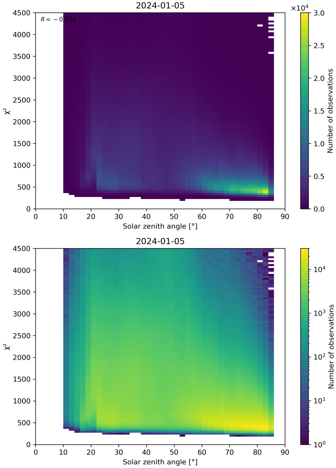
Figure 64: Scatter density plot of “Solar zenith angle” against “ \chi^2 ” for 2024-01-05 to 2024-01-06.
