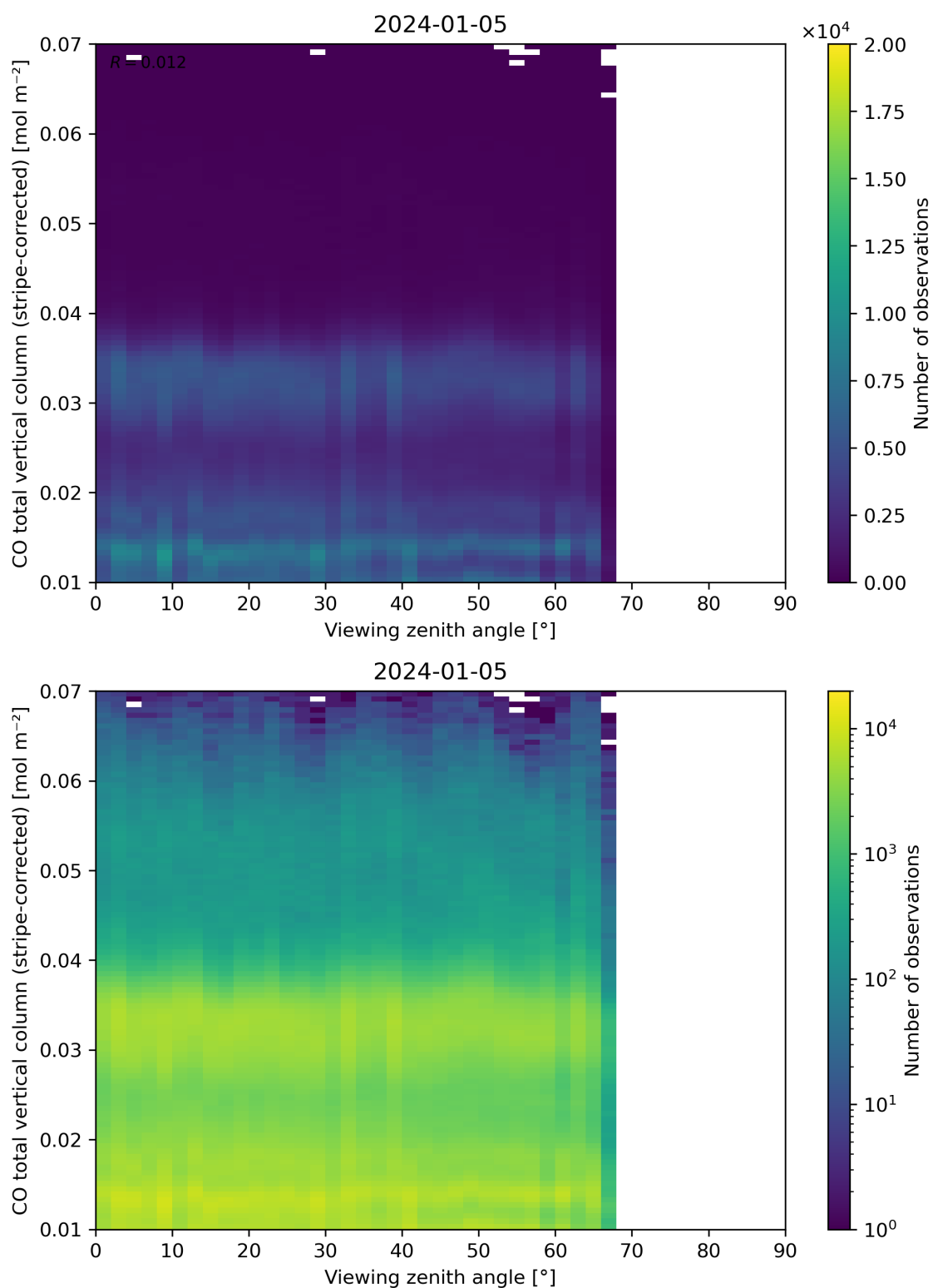
Figure 70: Scatter density plot of “Viewing zenith angle” against “CO total vertical column (stripe-corrected)” for 2024-01-05 to 2024-01-06.
