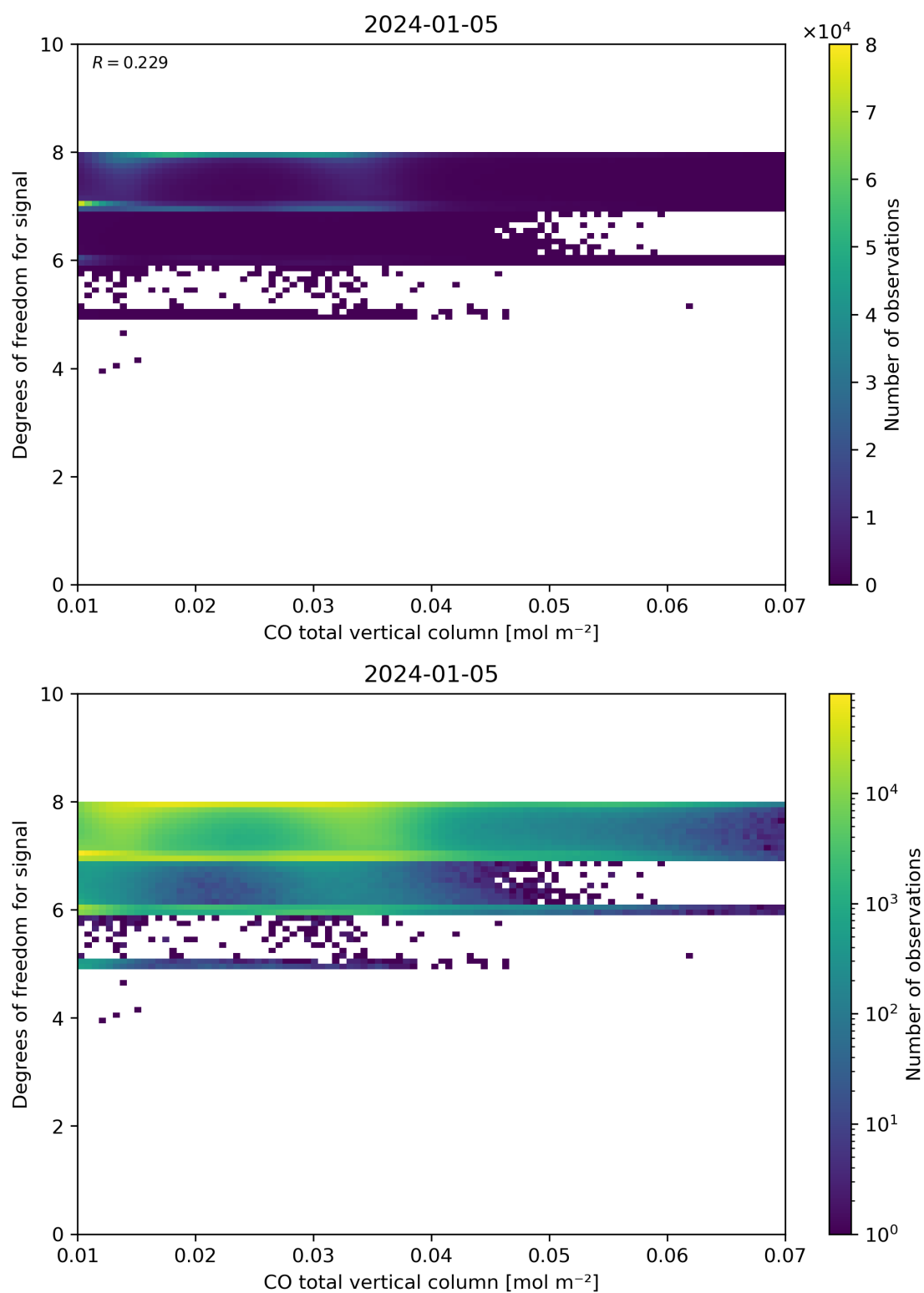
Figure 41: Scatter density plot of “CO total vertical column” against “Degrees of freedom for signal” for 2024-01-05 to 2024-01-06.
