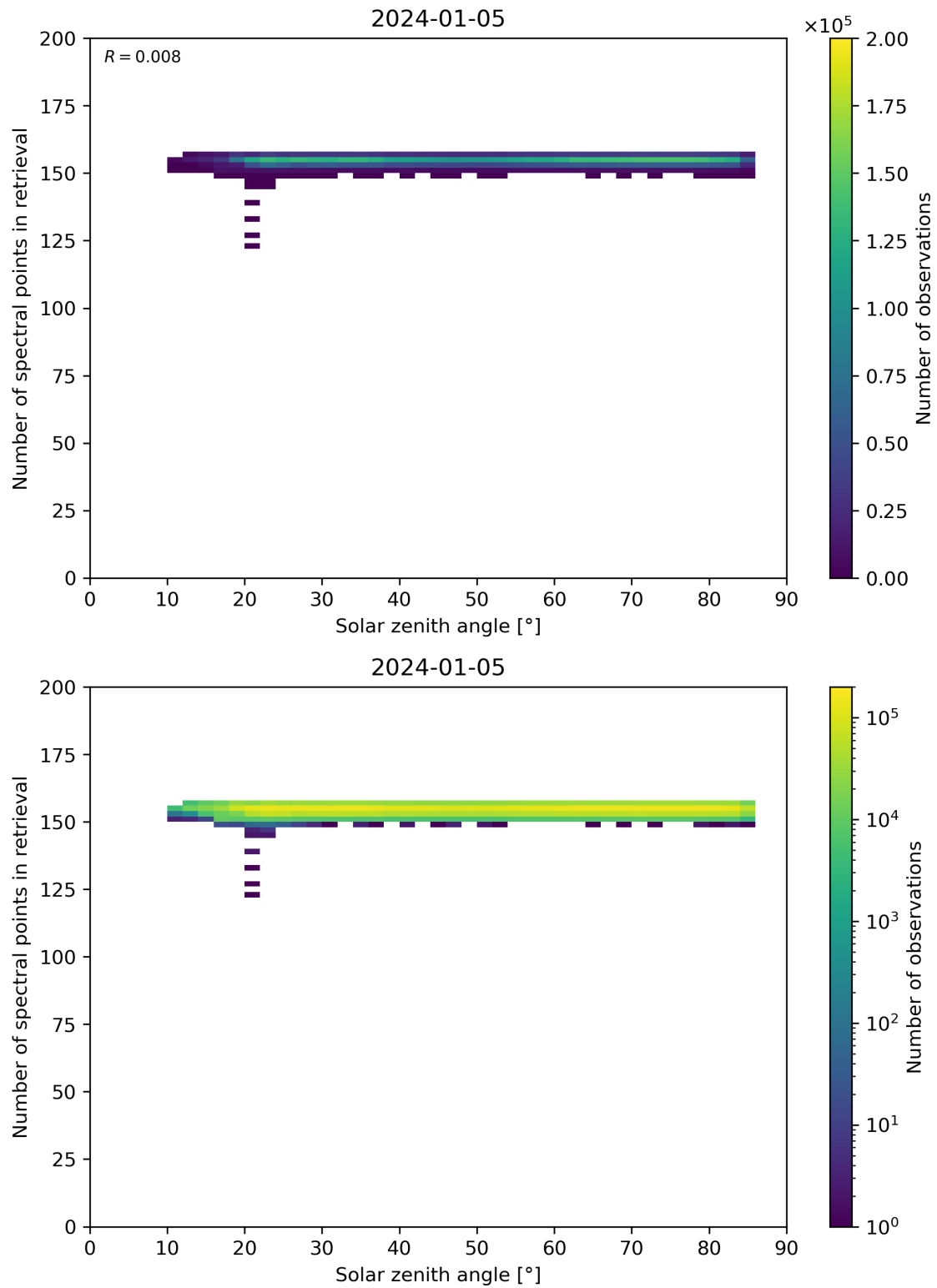
Figure 68: Scatter density plot of “Solar zenith angle” against “Number of spectral points in retrieval” for 2024-01-05 to 2024-01-06.
