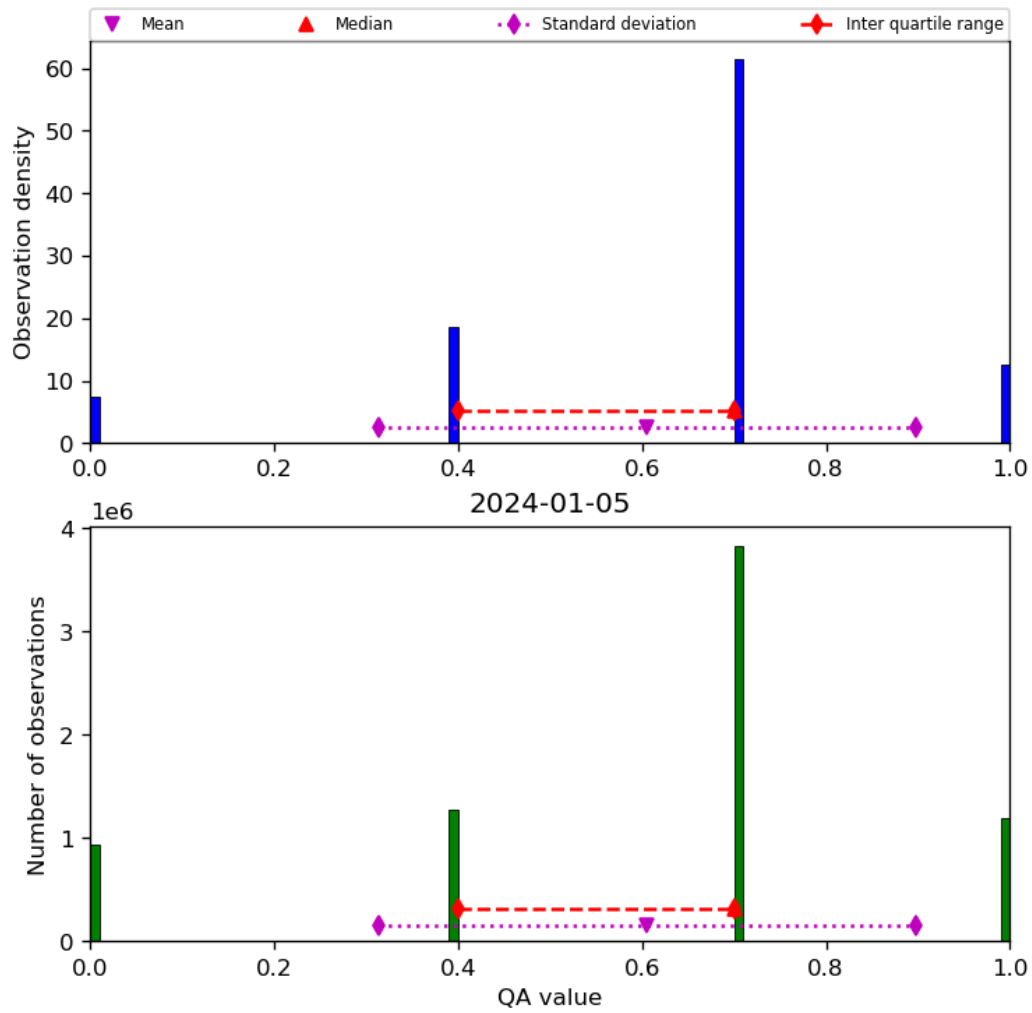
Figure 17: Histogram of “QA value” for 2024-01-05 to 2024-01-06
