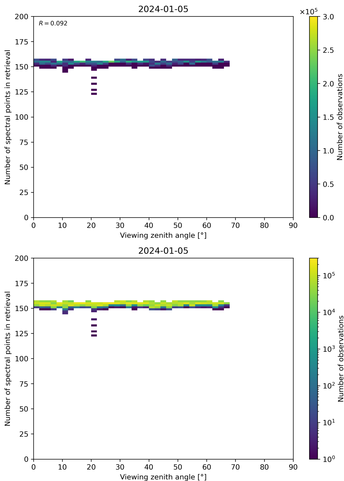
Figure 76: Scatter density plot of “Viewing zenith angle” against “Number of spectral points in retrieval” for 2024-01-05 to 2024-01-06.
