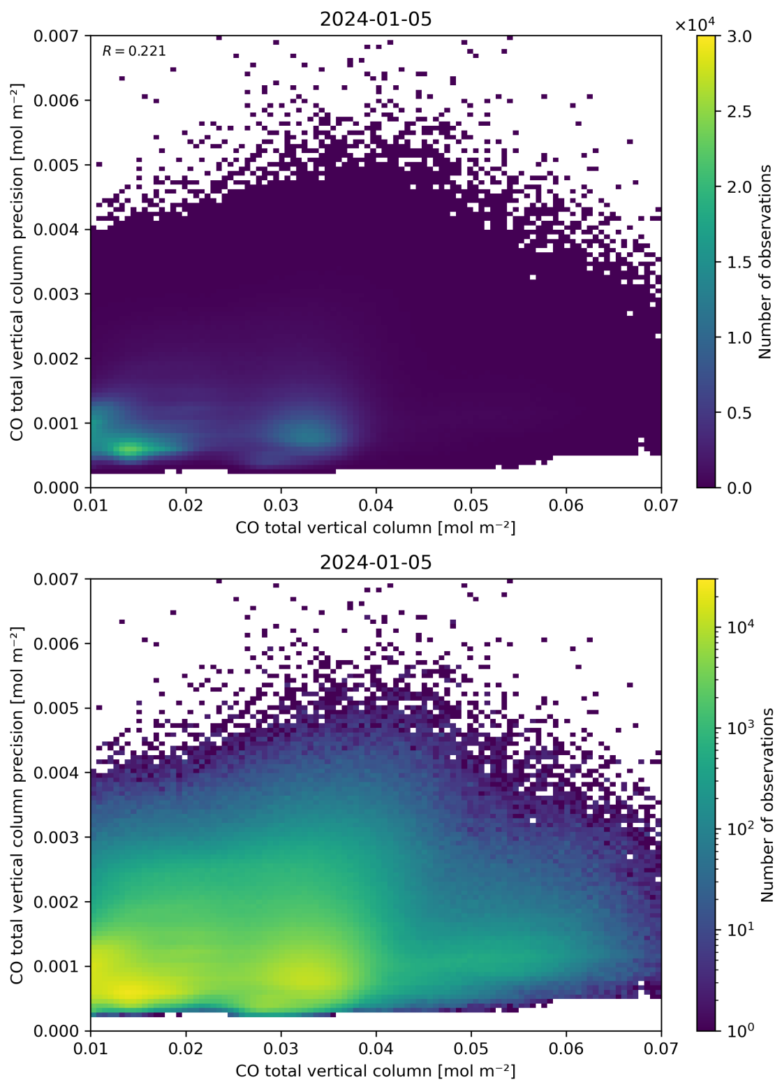
Figure 34: Scatter density plot of “CO total vertical column” against “CO total vertical column precision” for 2024-01-05 to 2024-01-06.
