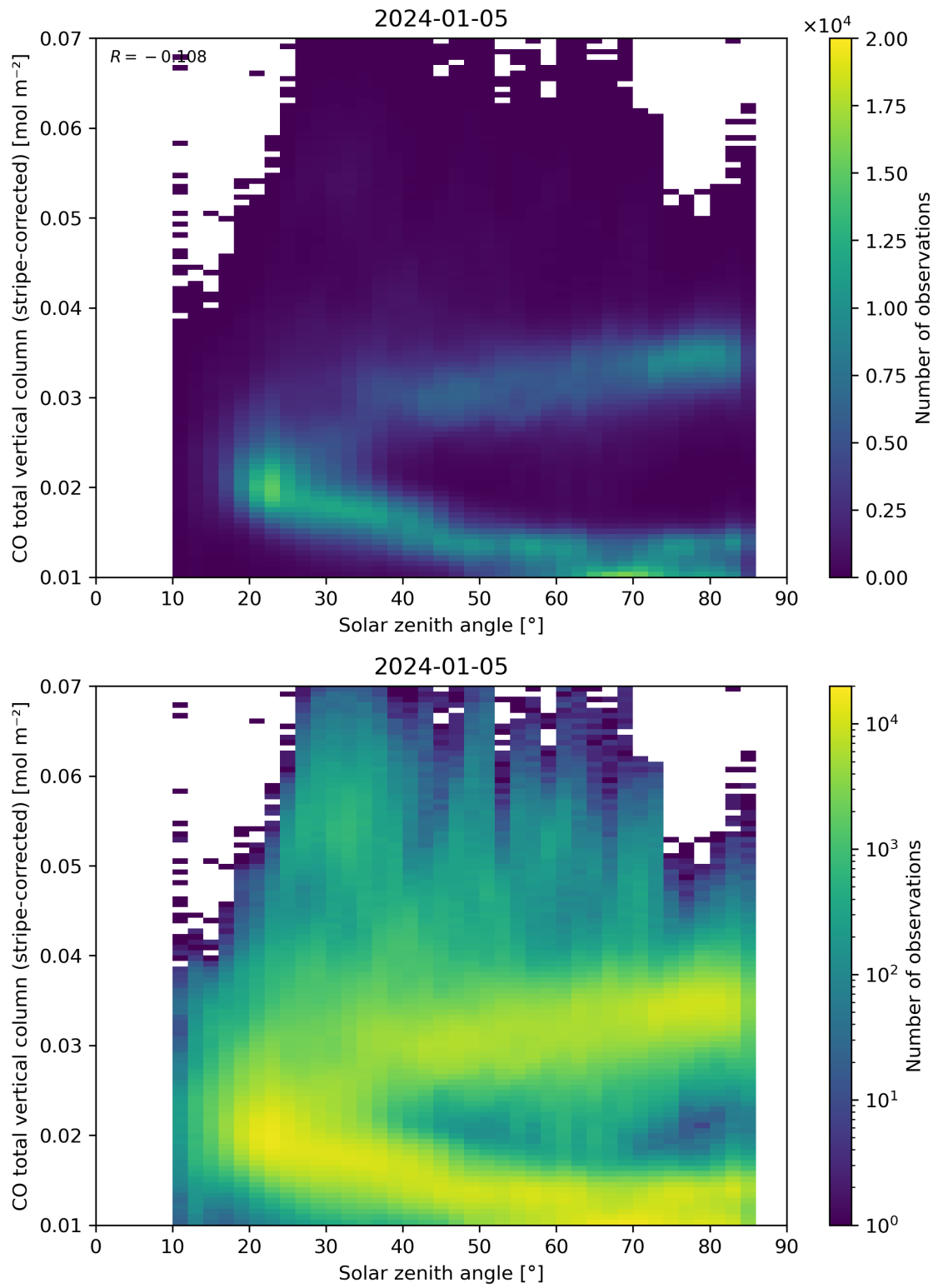
Figure 62: Scatter density plot of “Solar zenith angle” against “CO total vertical column (stripe-corrected)” for 2024-01-05 to 2024-01-06.
