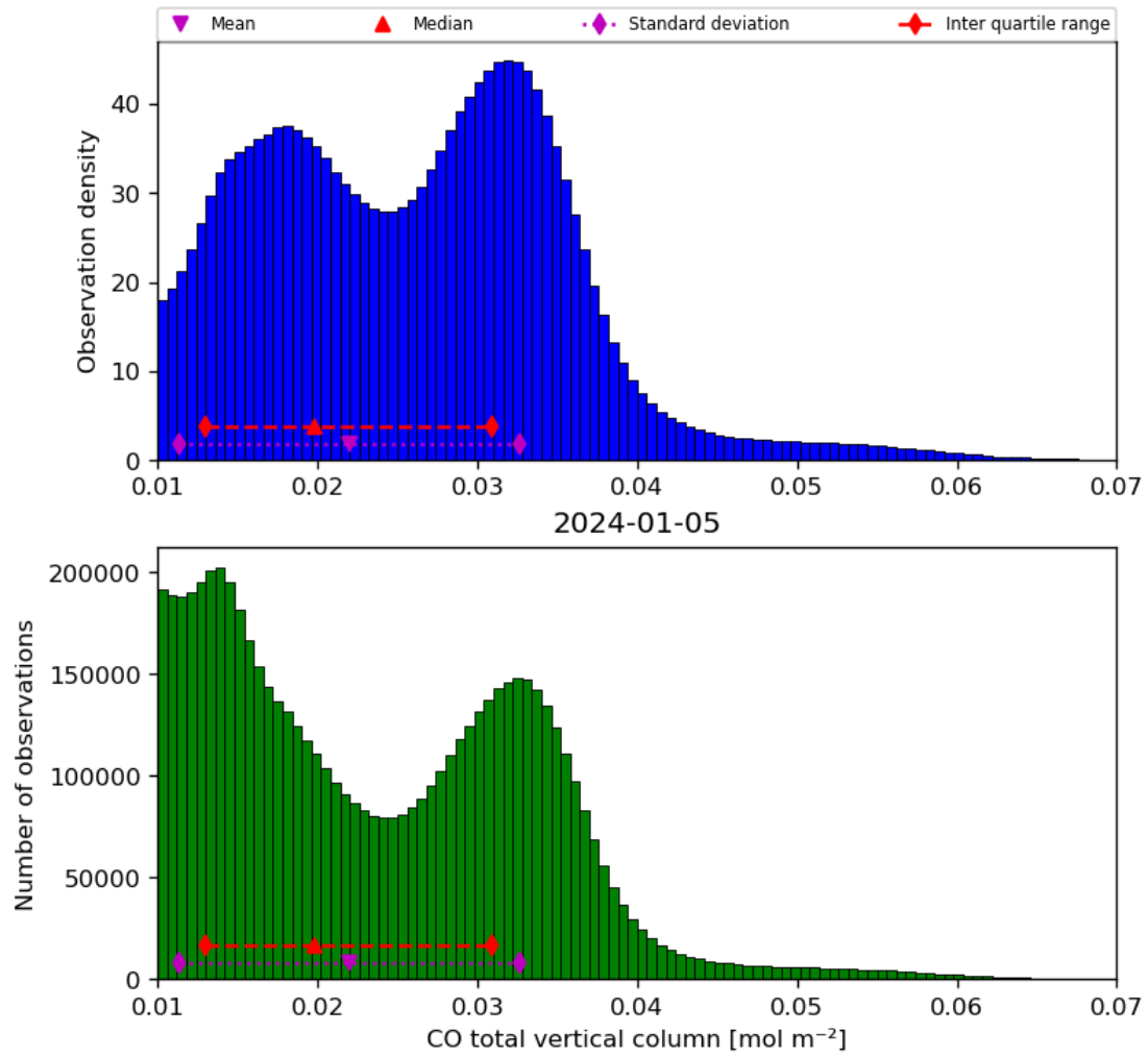
Figure 18: Histogram of “CO total vertical column” for 2024-01-05 to 2024-01-06
