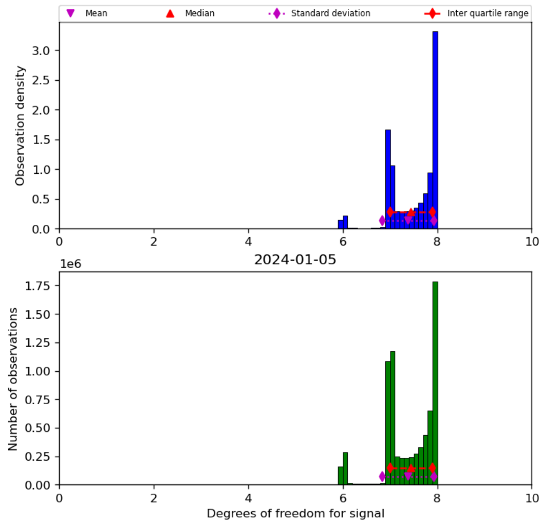
Figure 23: Histogram of “Degrees of freedom for signal” for 2024-01-05 to 2024-01-06
