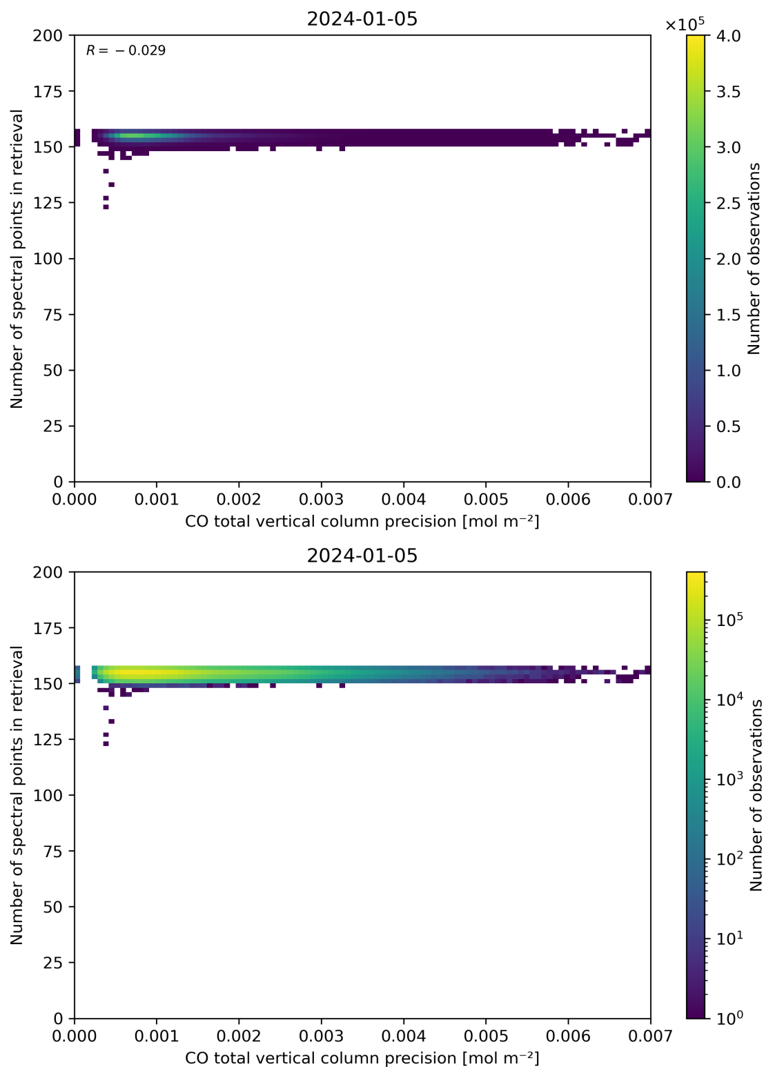
Figure 47: Scatter density plot of “CO total vertical column precision” against “Number of spectral points in retrieval” for 2024-01-05 to 2024-01-06.
