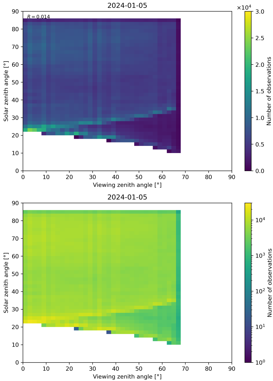
Figure 77: Scatter density plot of “Viewing zenith angle” against “Solar zenith angle” for 2024-01-05 to 2024-01-06.
