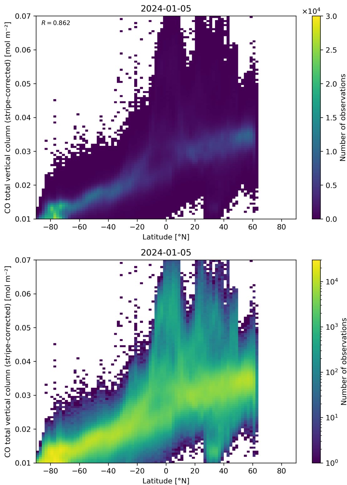
Figure 52: Scatter density plot of “Latitude” against “CO total vertical column (stripe-corrected)” for 2024-01-05 to 2024-01-06.
