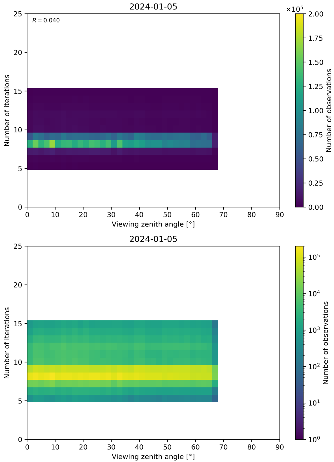
Figure 75: Scatter density plot of “Viewing zenith angle” against “Number of iterations” for 2024-01-05 to 2024-01-06.
