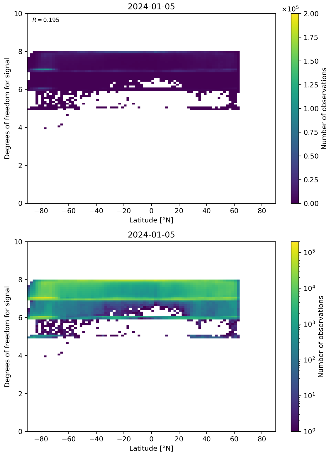
Figure 55: Scatter density plot of “Latitude” against “Degrees of freedom for signal” for 2024-01-05 to 2024-01-06.
