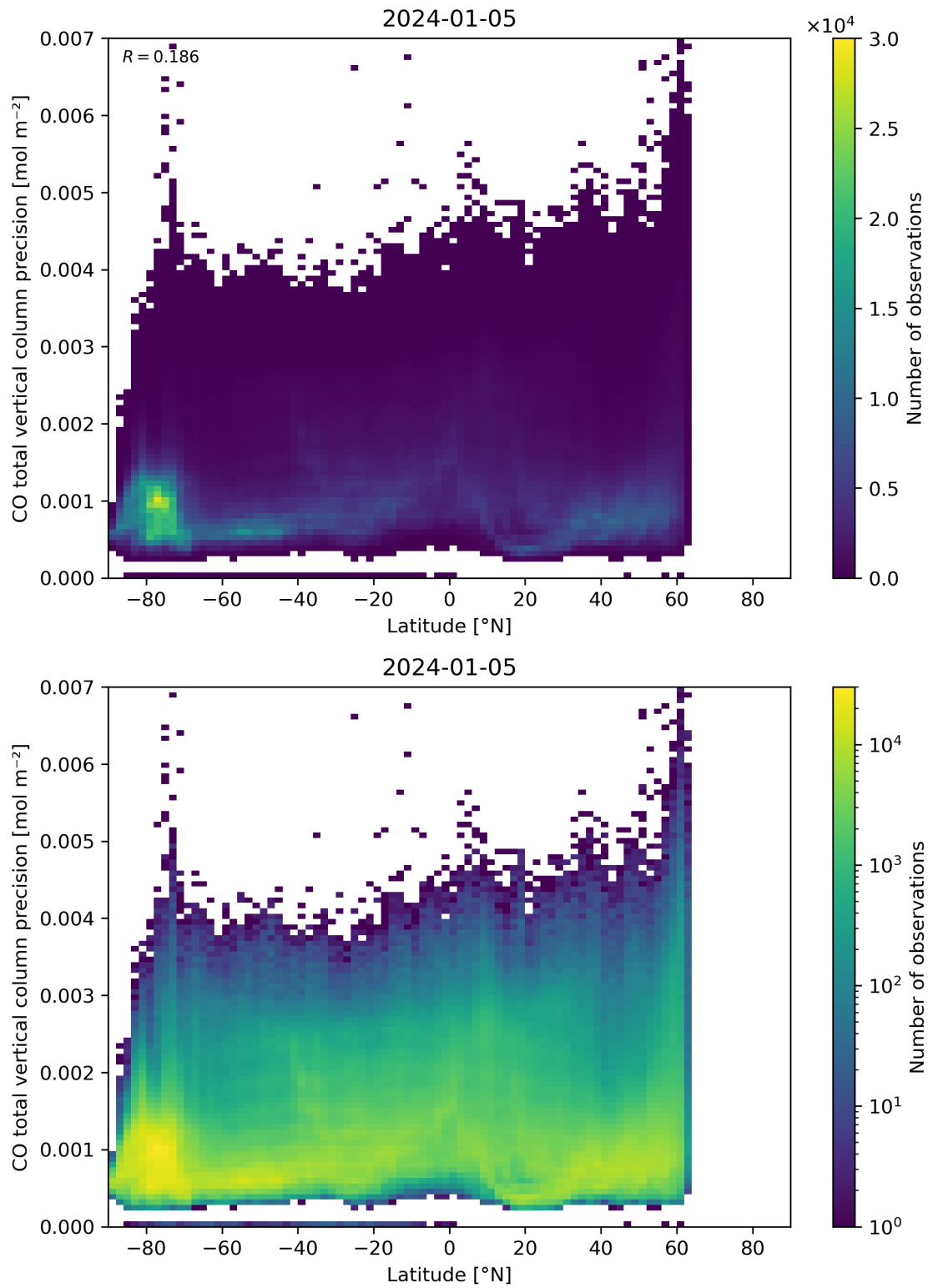
Figure 53: Scatter density plot of “Latitude” against “CO total vertical column precision” for 2024-01-05 to 2024-01-06.
