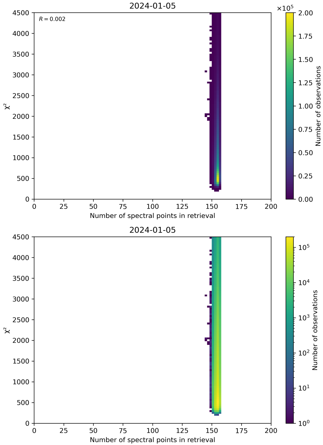
Figure 58: Scatter density plot of “Number of spectral points in retrieval” against “ \chi^2 ” for 2024-01-05 to 2024-01-06.
