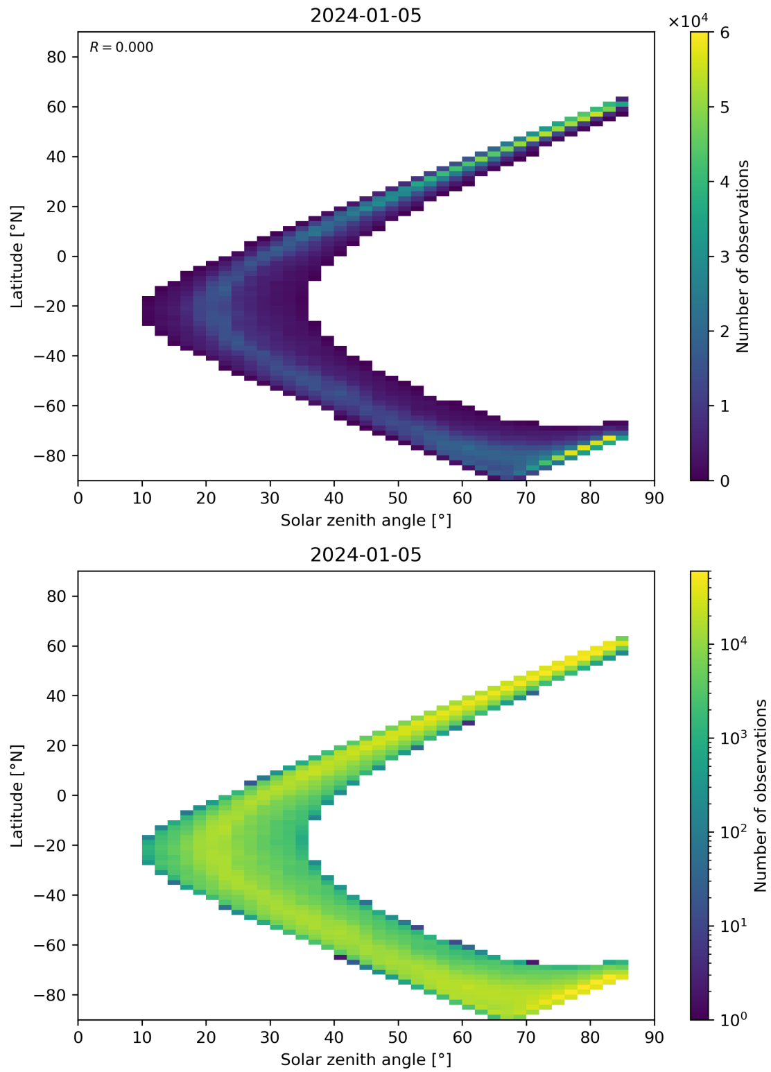
Figure 66: Scatter density plot of “Solar zenith angle” against “Latitude” for 2024-01-05 to 2024-01-06.
