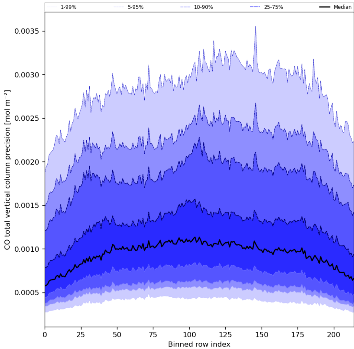
Figure 28: Along track statistics of “CO total vertical column precision” for 2024-01-05 to 2024-01-06
