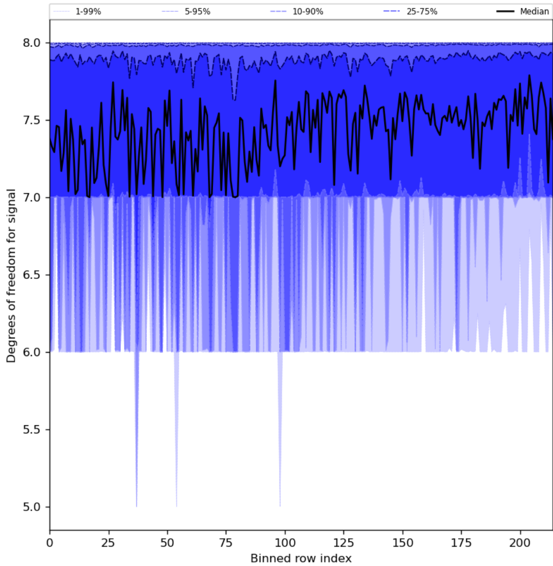
Figure 31: Along track statistics of “Degrees of freedom for signal” for 2024-01-05 to 2024-01-06
