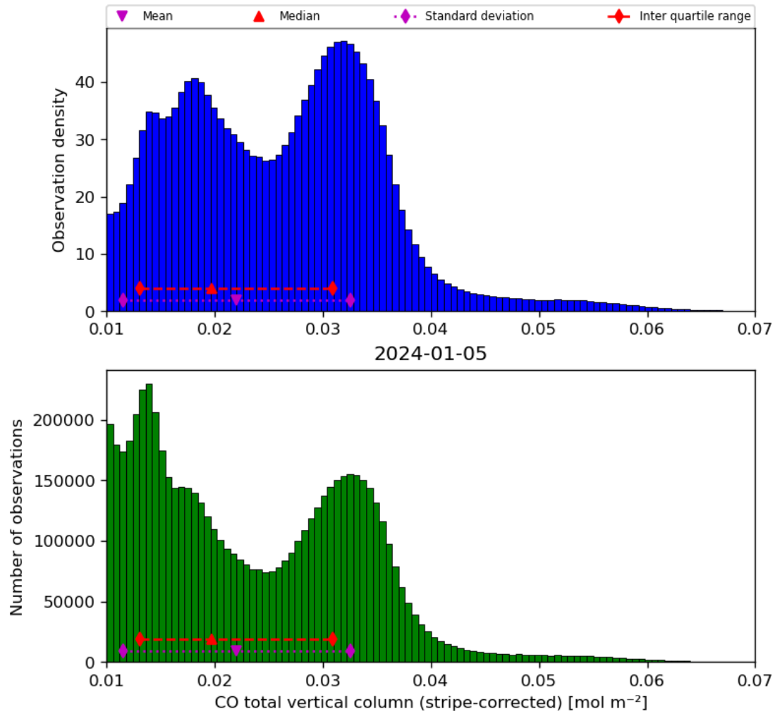
Figure 19: Histogram of “CO total vertical column (stripe-corrected)” for 2024-01-05 to 2024-01-06
