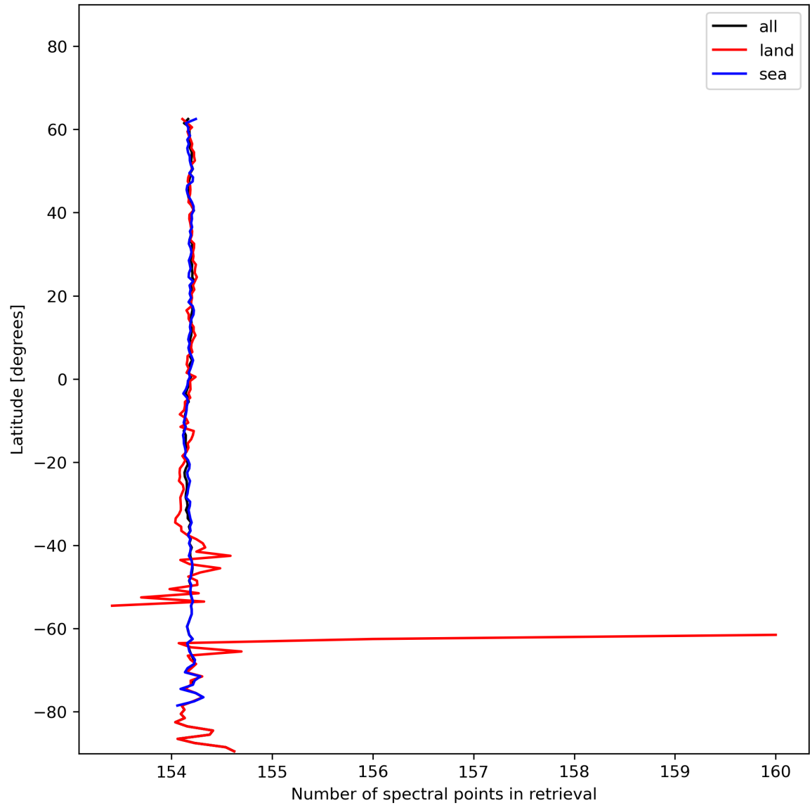
Figure 13: Zonal average of “Number of spectral points in retrieval” for 2024-01-05 to 2024-01-06.
