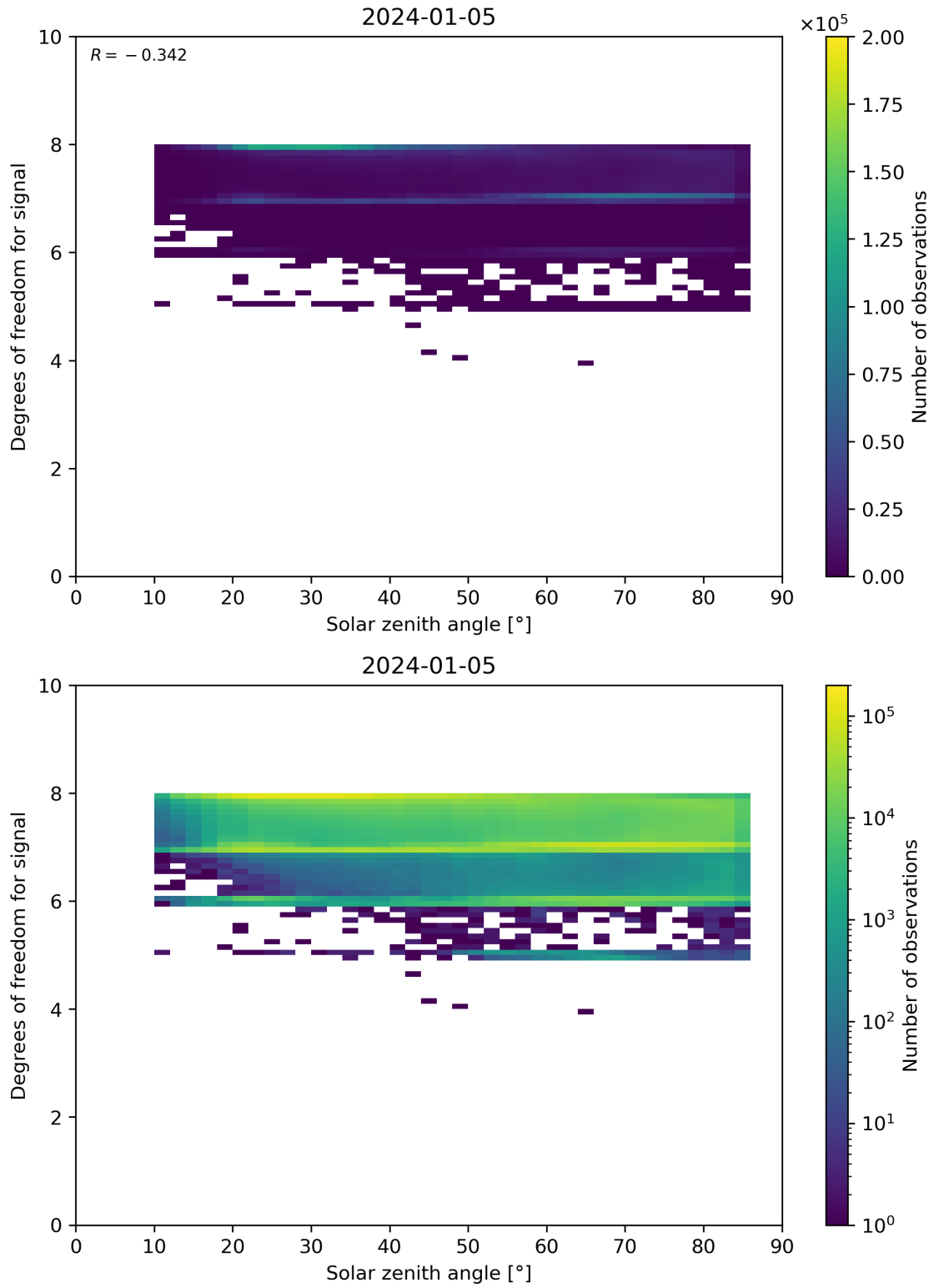
Figure 65: Scatter density plot of “Solar zenith angle” against “Degrees of freedom for signal” for 2024-01-05 to 2024-01-06.
