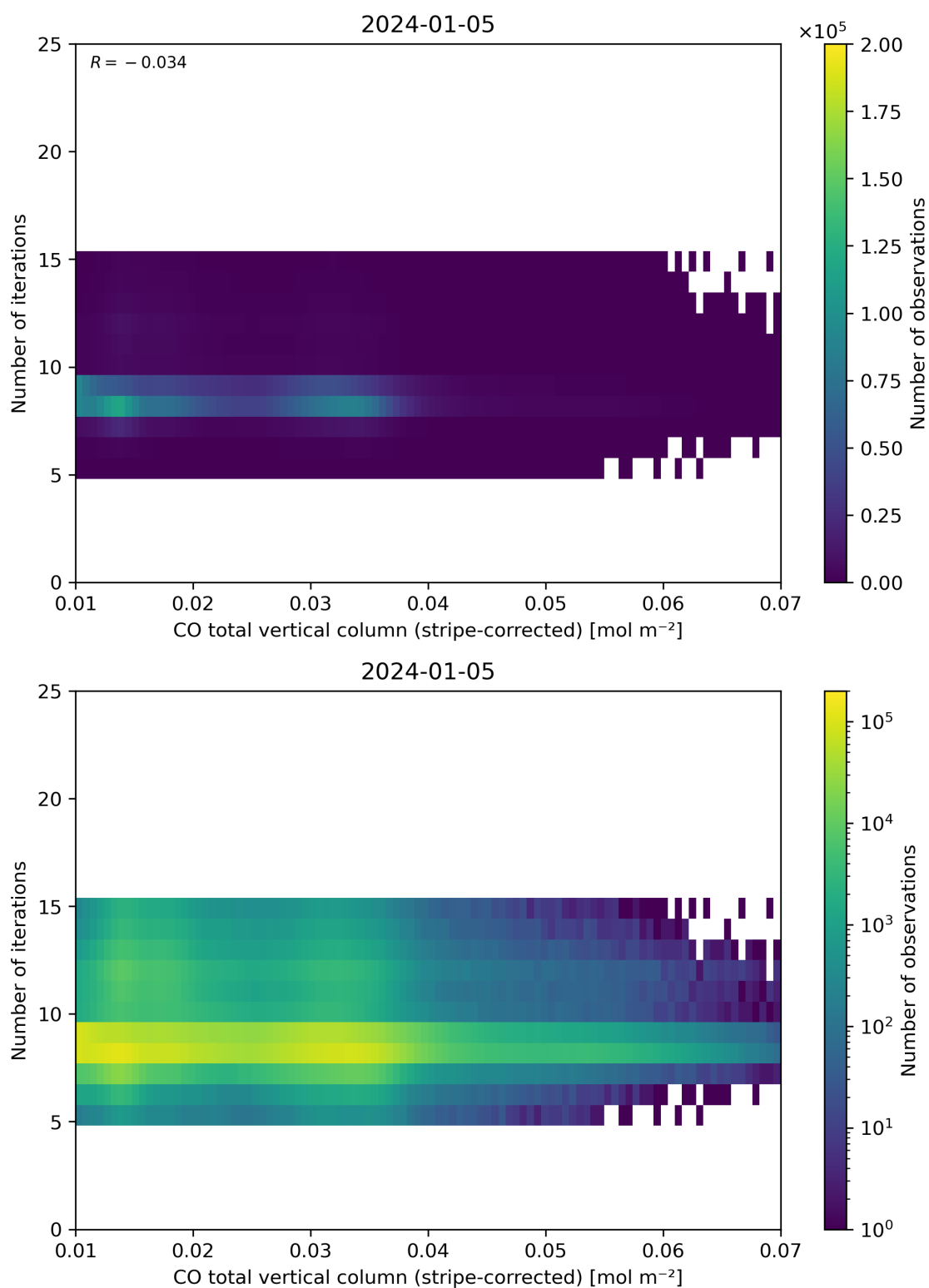
Figure 39: Scatter density plot of “CO total vertical column (stripe-corrected)” against “Number of iterations” for 2024-01-05 to 2024-01-06.
