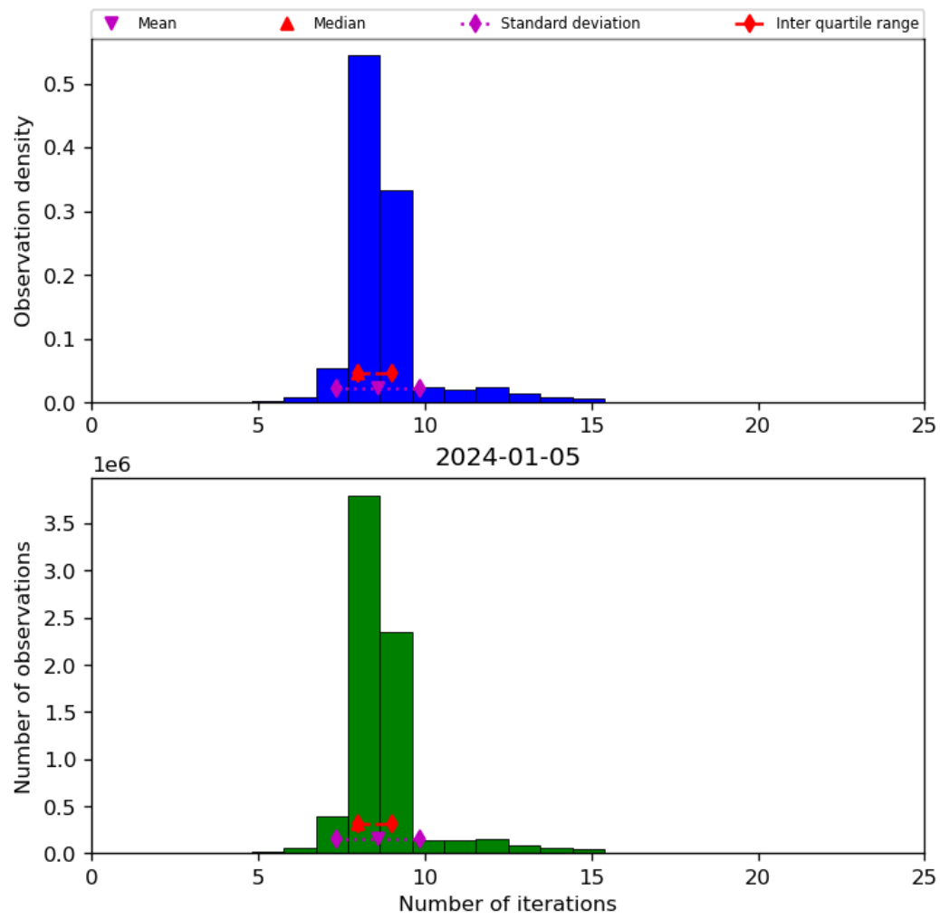
Figure 24: Histogram of “Number of iterations” for 2024-01-05 to 2024-01-06
