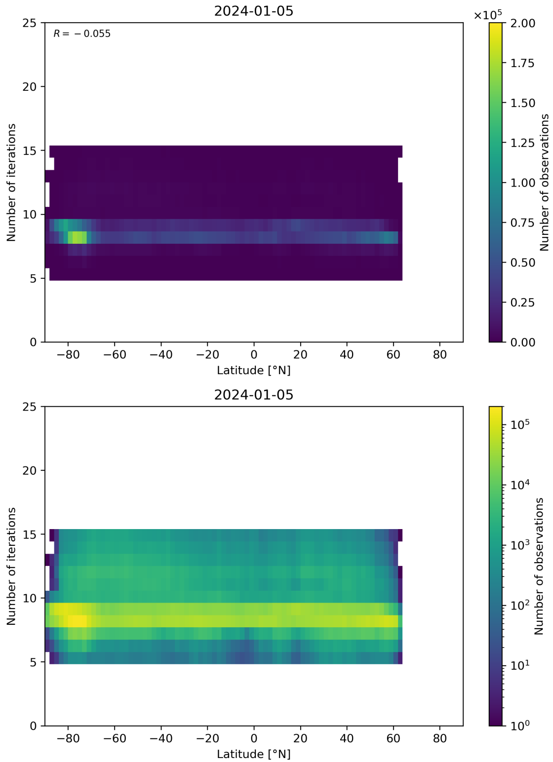
Figure 56: Scatter density plot of “Latitude” against “Number of iterations” for 2024-01-05 to 2024-01-06.
