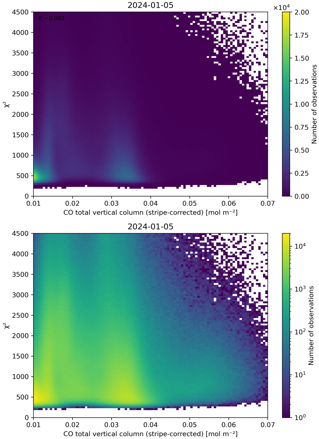
Figure 37: Scatter density plot of “CO total vertical column (stripe-corrected)” against “ \chi^2 ” for 2024-01-05 to 2024-01-06.
