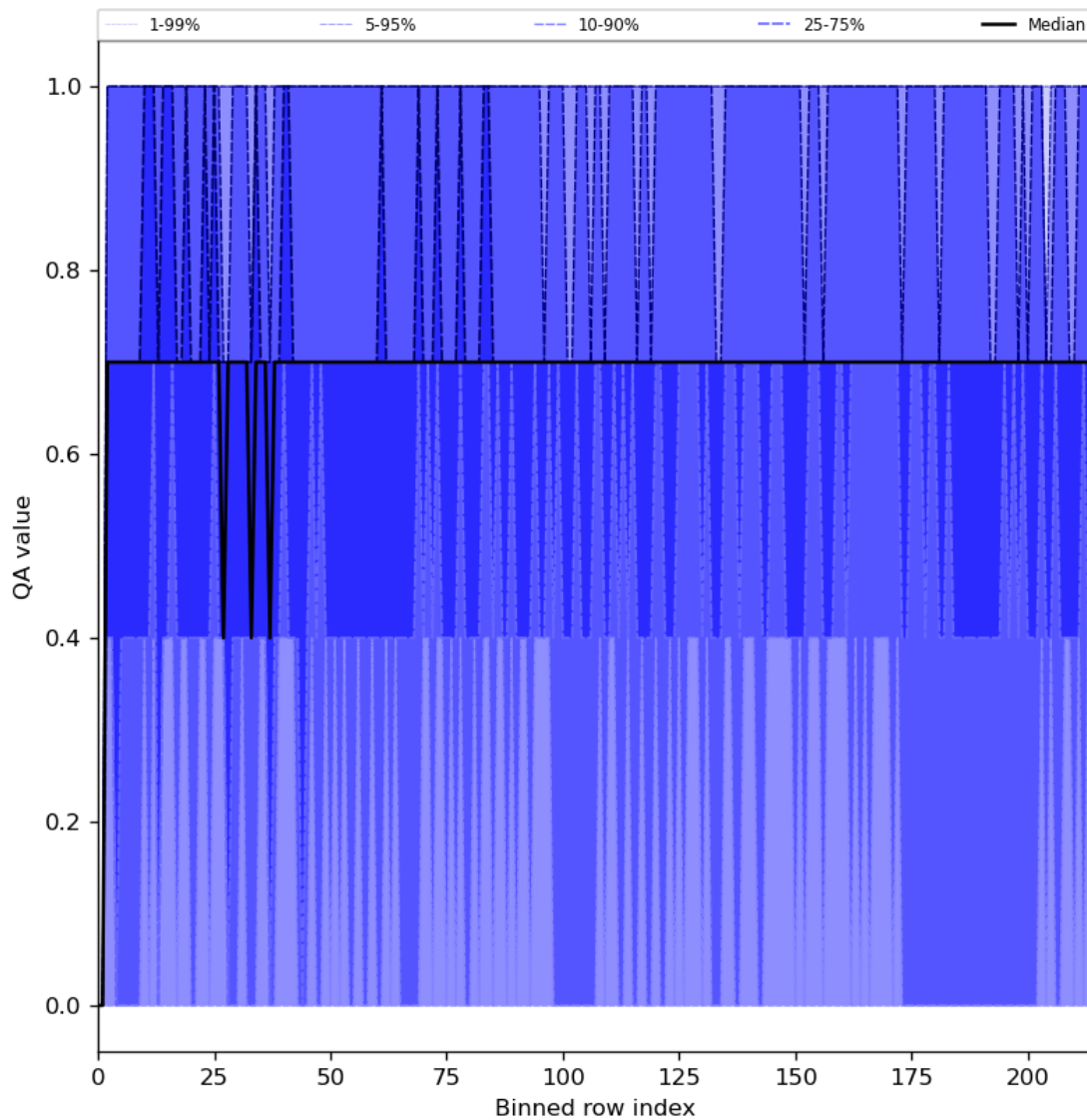
Figure 25: Along track statistics of “QA value” for 2024-01-05 to 2024-01-06
