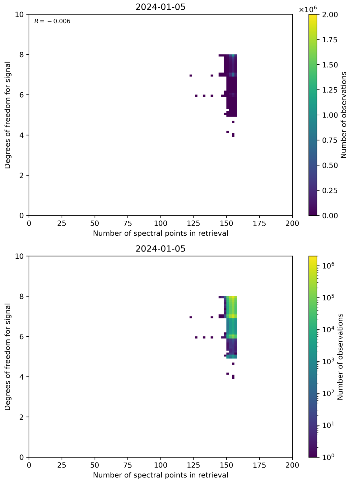
Figure 59: Scatter density plot of “Number of spectral points in retrieval” against “Degrees of freedom for signal” for 2024-01-05 to 2024-01-06.
