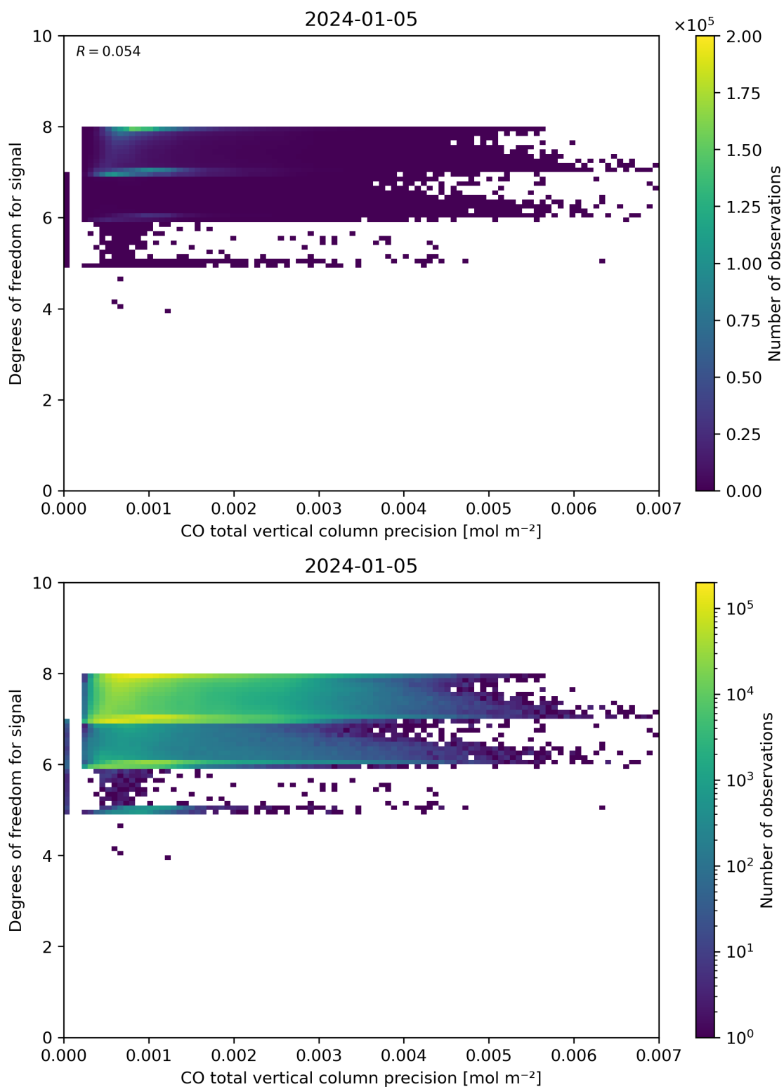
Figure 45: Scatter density plot of “CO total vertical column precision” against “Degrees of freedom for signal” for 2024-01-05 to 2024-01-06.
