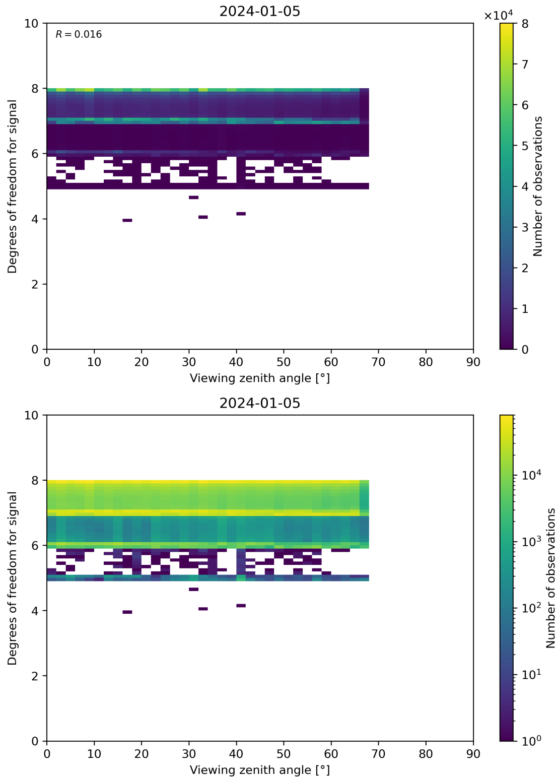
Figure 73: Scatter density plot of “Viewing zenith angle” against “Degrees of freedom for signal” for 2024-01-05 to 2024-01-06.
