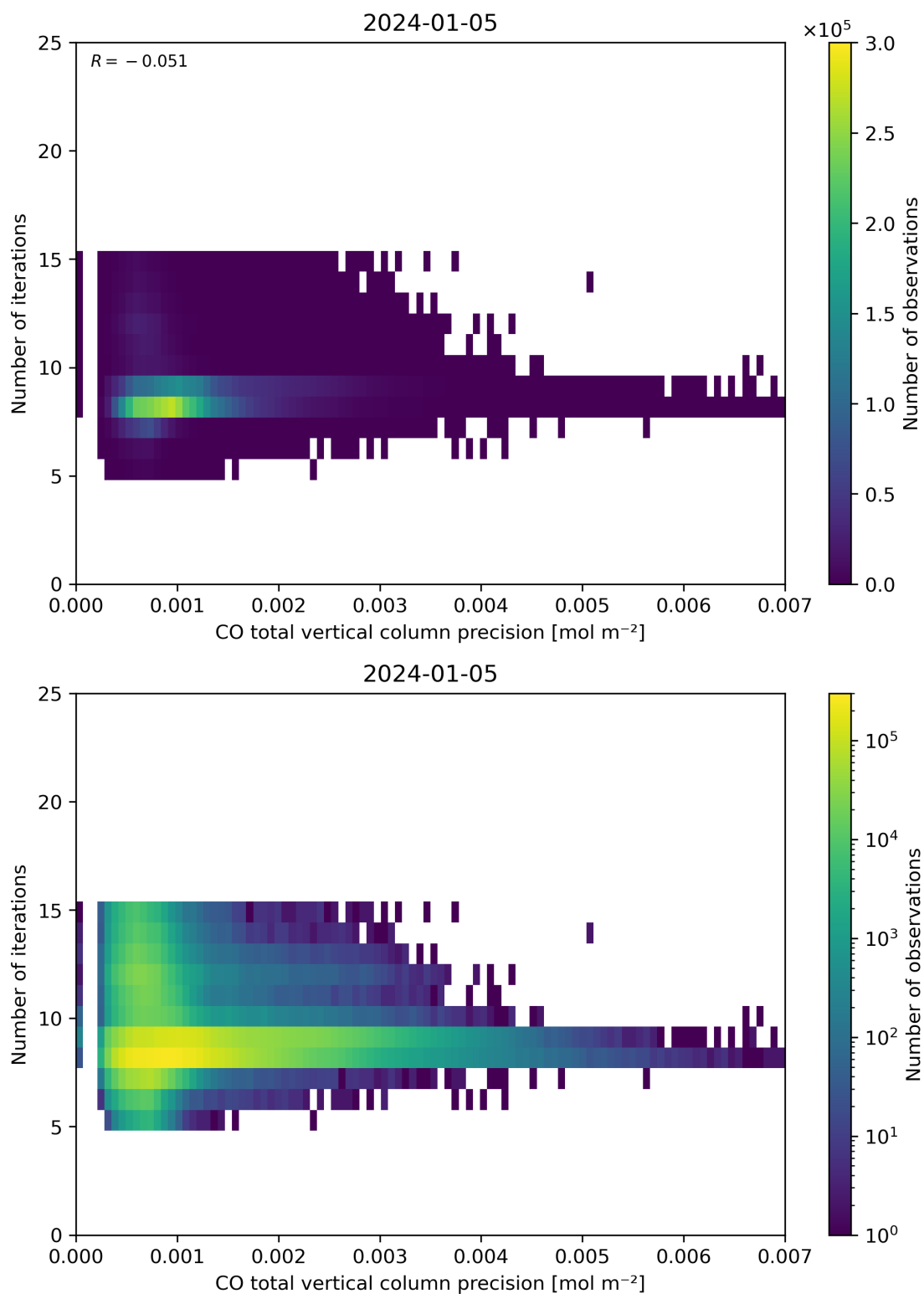
Figure 46: Scatter density plot of “CO total vertical column precision” against “Number of iterations” for 2024-01-05 to 2024-01-06.
