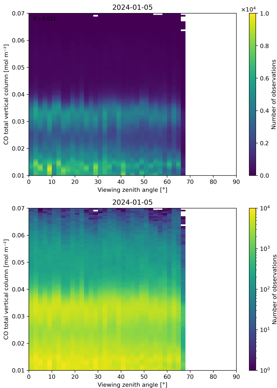
Figure 69: Scatter density plot of “Viewing zenith angle” against “CO total vertical column” for 2024-01-05 to 2024-01-06.
