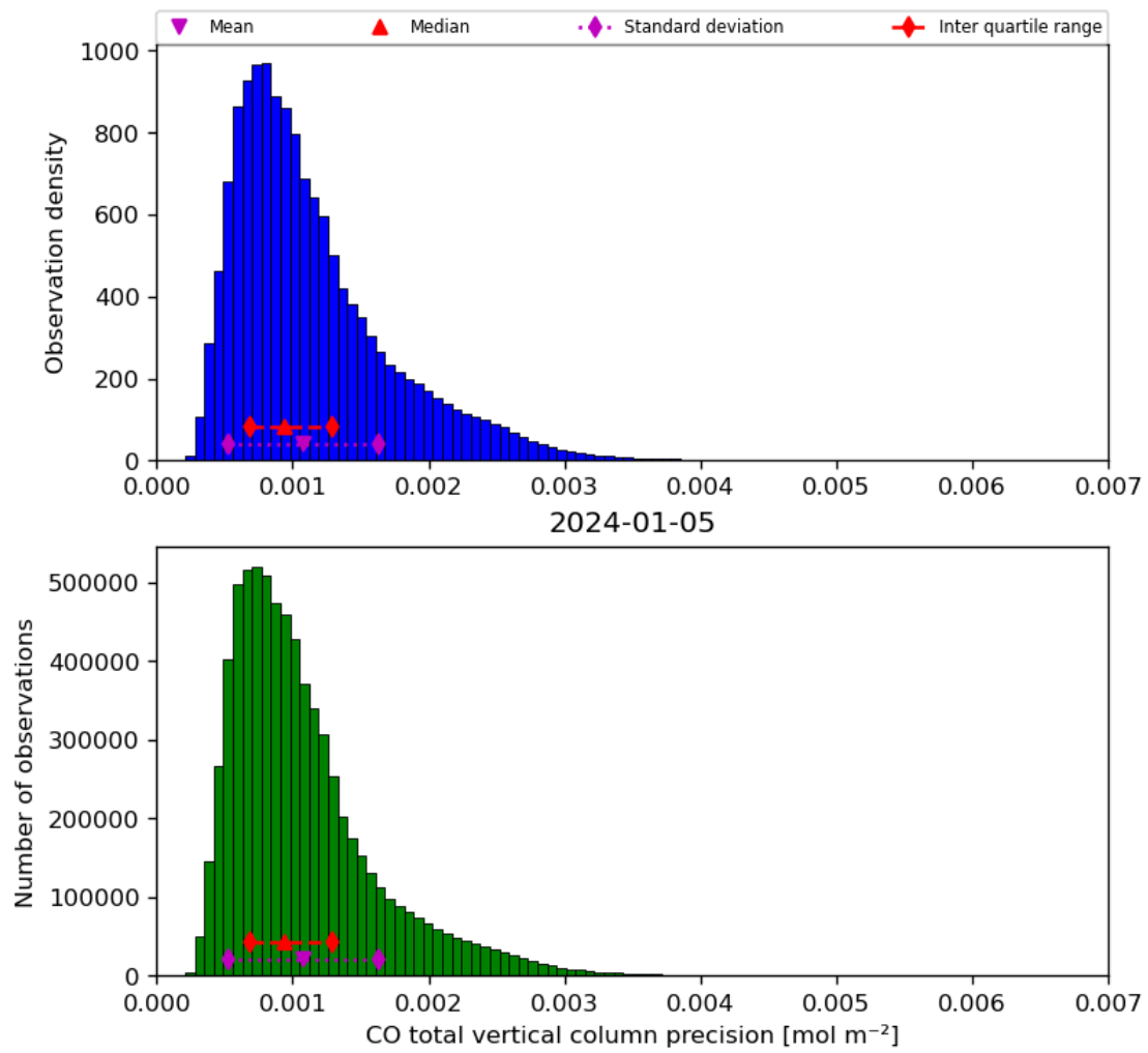
Figure 20: Histogram of “CO total vertical column precision” for 2024-01-05 to 2024-01-06
