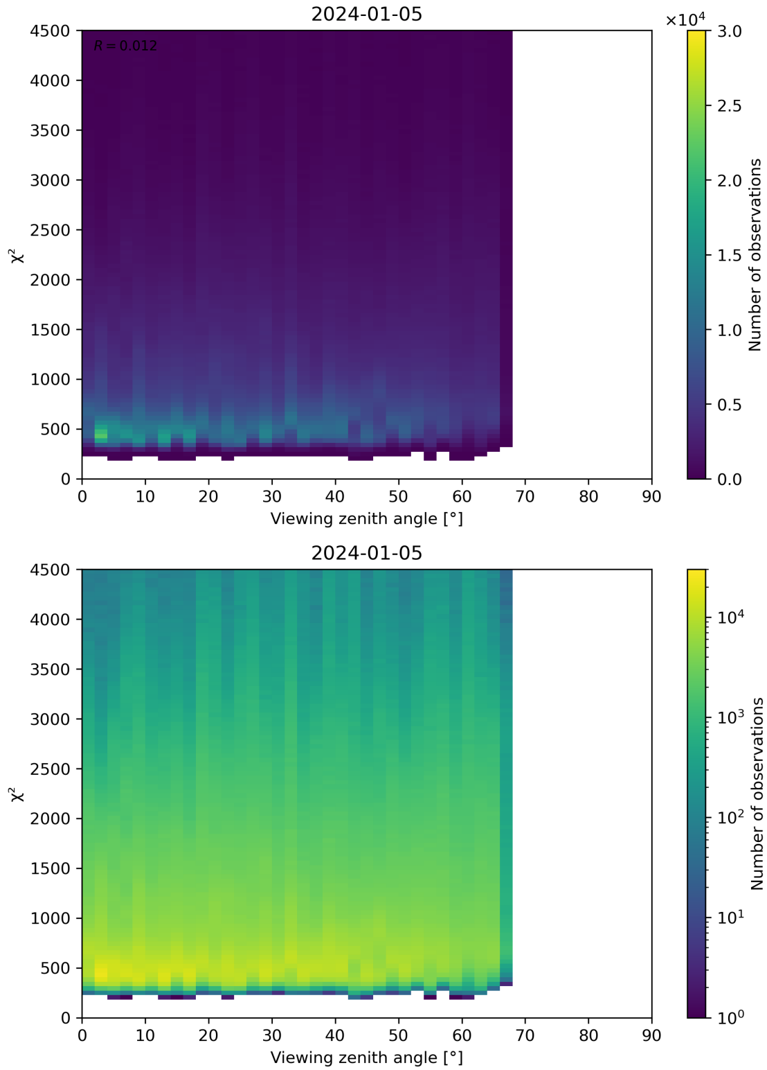
Figure 72: Scatter density plot of “Viewing zenith angle” against “ \chi^2 ” for 2024-01-05 to 2024-01-06.
