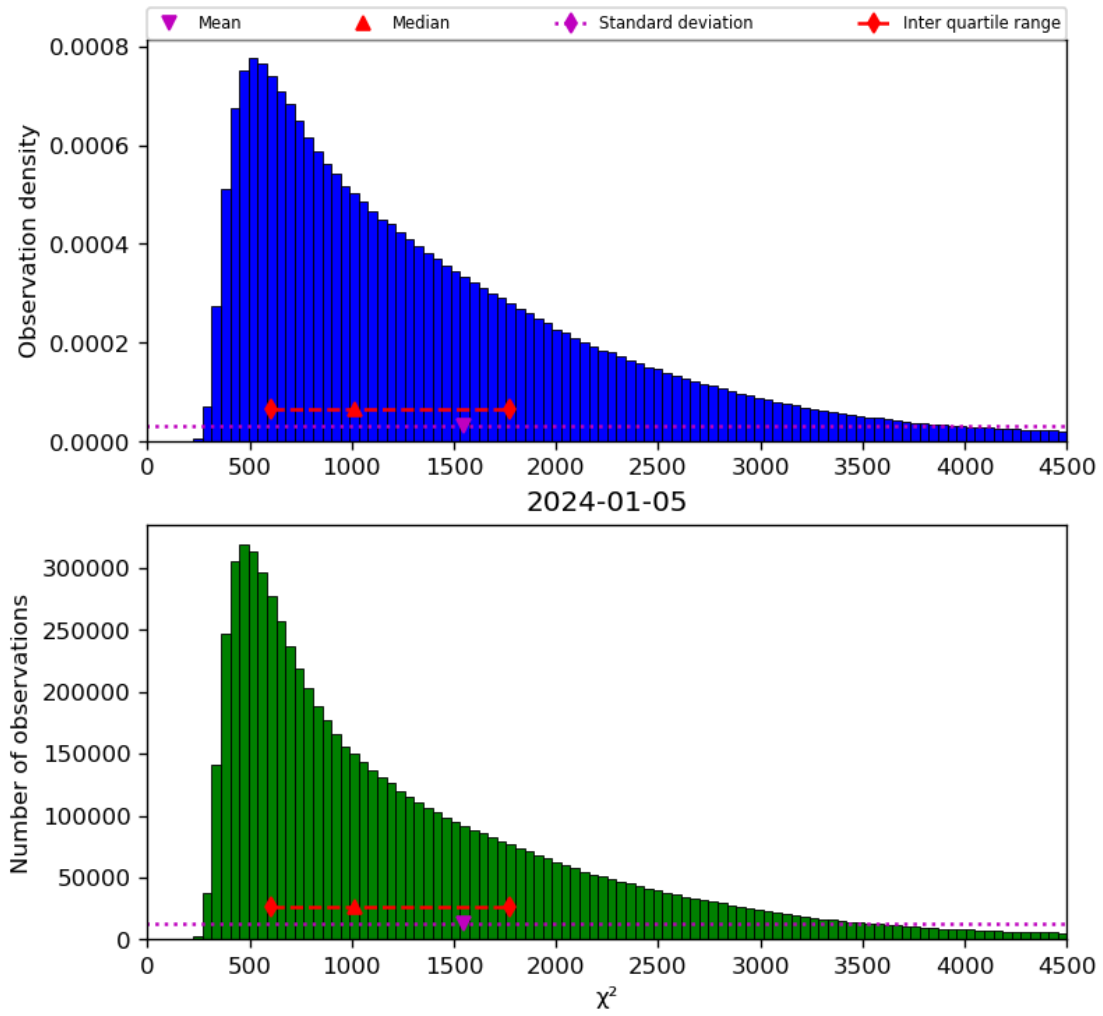
Figure 22: Histogram of “ \chi^2 ” for 2024-01-05 to 2024-01-06
