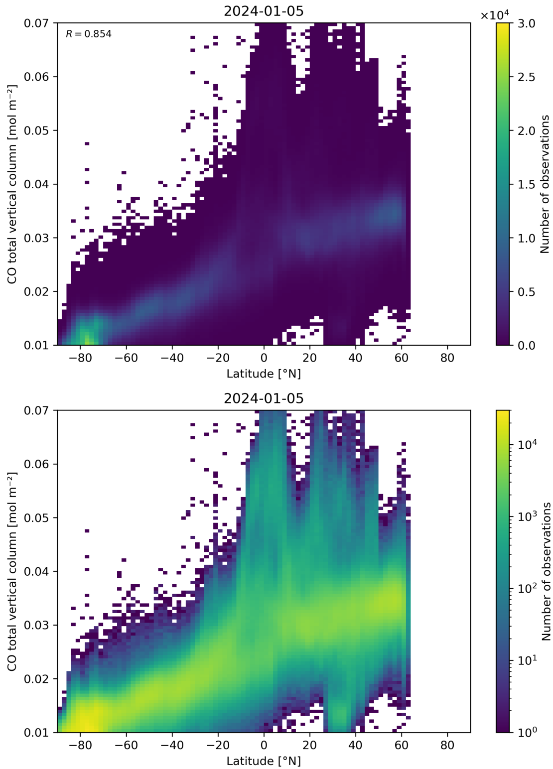
Figure 51: Scatter density plot of “Latitude” against “CO total vertical column” for 2024-01-05 to 2024-01-06.
