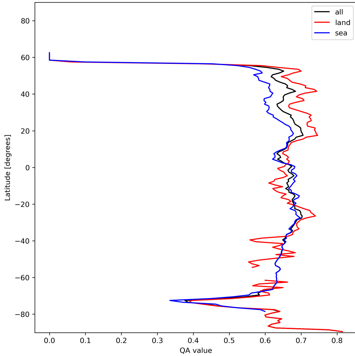
Figure 9: Zonal average of “QA value” for 2024-01-05 to 2024-01-06.
