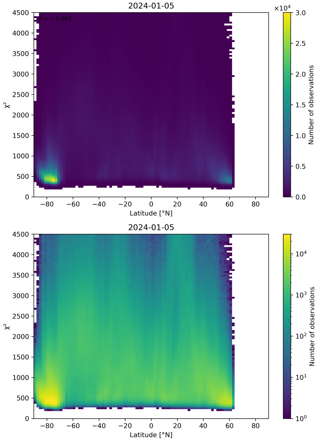
Figure 54: Scatter density plot of “Latitude” against “ \chi^2 ” for 2024-01-05 to 2024-01-06.
