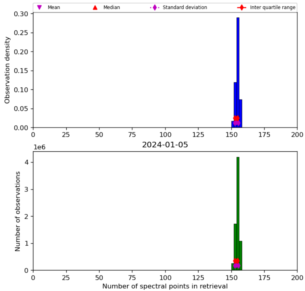
Figure 21: Histogram of “Number of spectral points in retrieval” for 2024-01-05 to 2024-01-06
