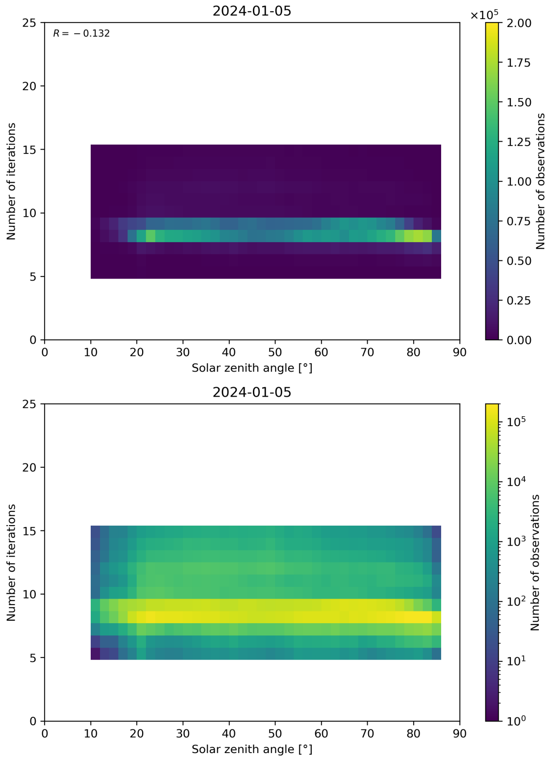
Figure 67: Scatter density plot of “Solar zenith angle” against “Number of iterations” for 2024-01-05 to 2024-01-06.
