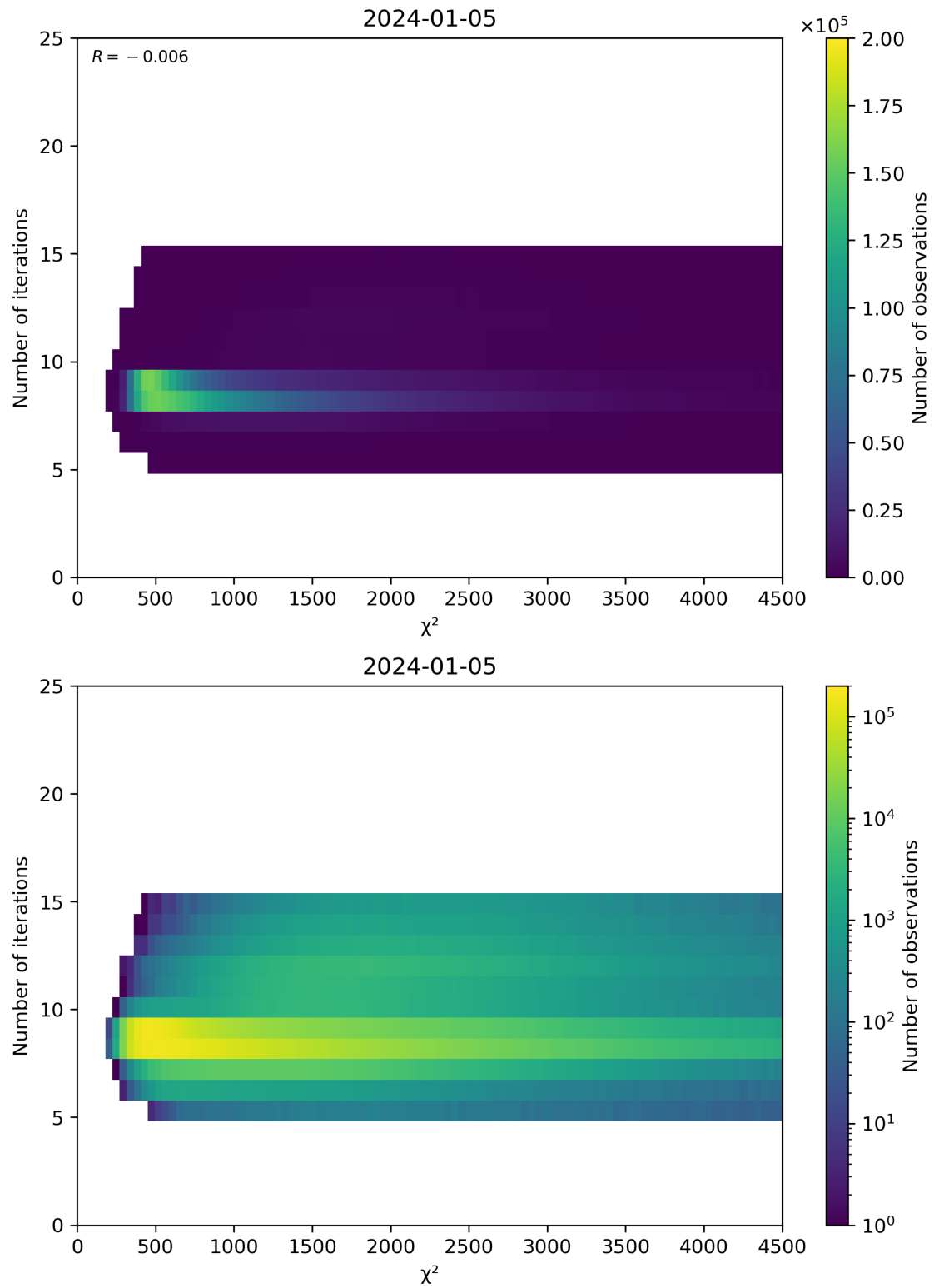
Figure 49: Scatter density plot of “ \chi^2 ” against “Number of iterations” for 2024-01-05 to 2024-01-06.
