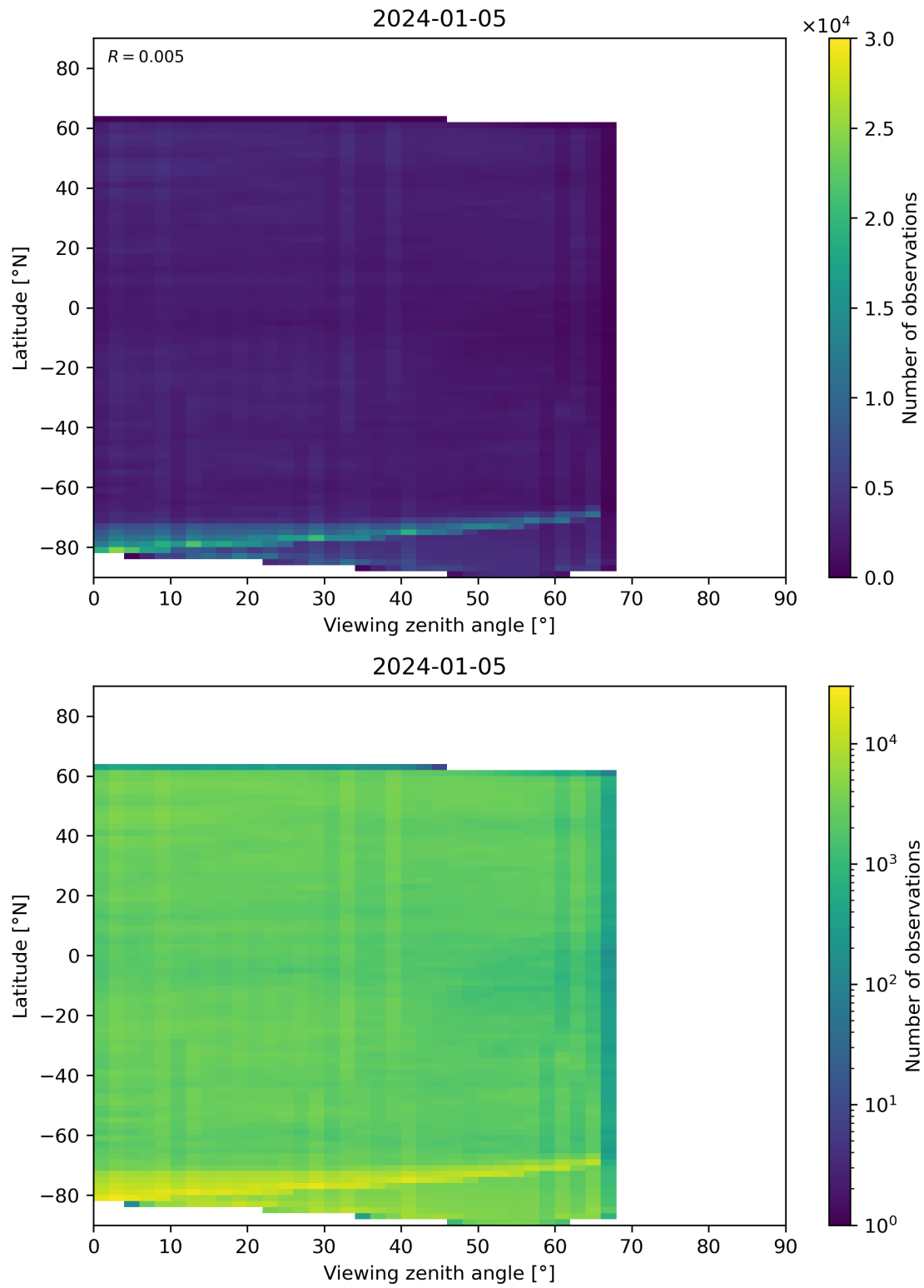
Figure 74: Scatter density plot of “Viewing zenith angle” against “Latitude” for 2024-01-05 to 2024-01-06.
