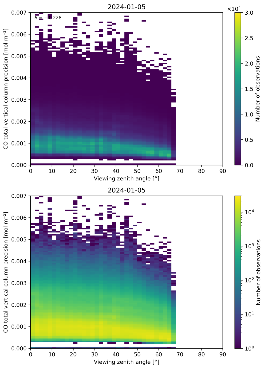
Figure 71: Scatter density plot of “Viewing zenith angle” against “CO total vertical column precision” for 2024-01-05 to 2024-01-06.
