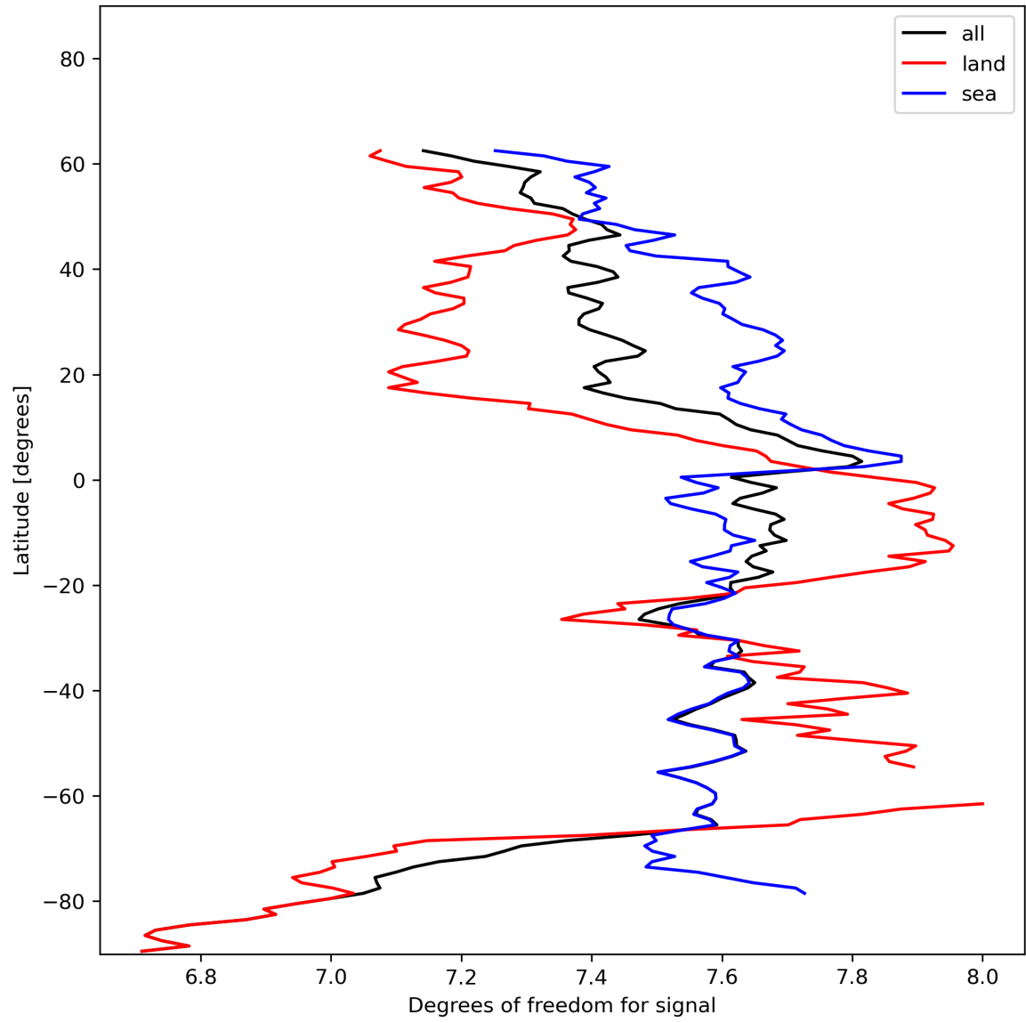
Figure 15: Zonal average of “Degrees of freedom for signal” for 2024-01-05 to 2024-01-06.
