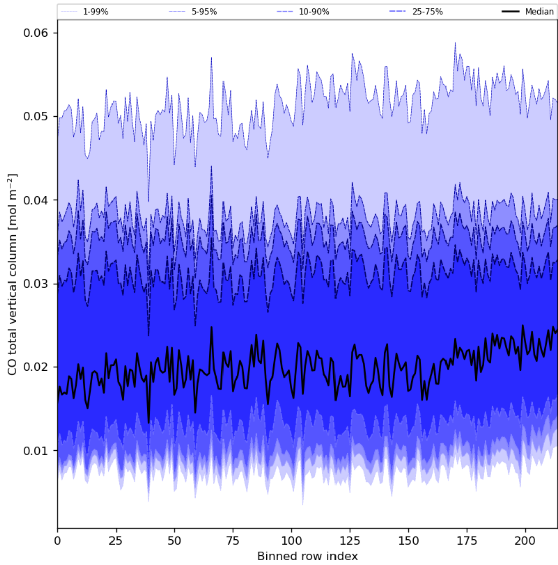
Figure 26: Along track statistics of “CO total vertical column” for 2024-01-05 to 2024-01-06
