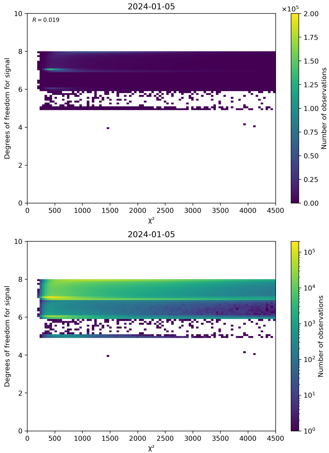
Figure 48: Scatter density plot of " \chi^2 " against "Degrees of freedom for signal" for 2024-01-05 to 2024-01-06.
