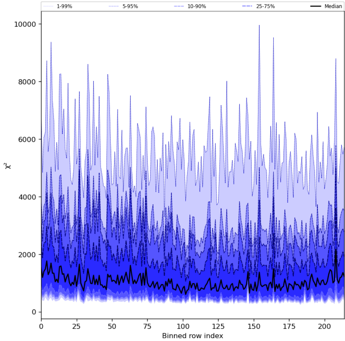
Figure 30: Along track statistics of “ \chi^2 ” for 2024-01-05 to 2024-01-06
