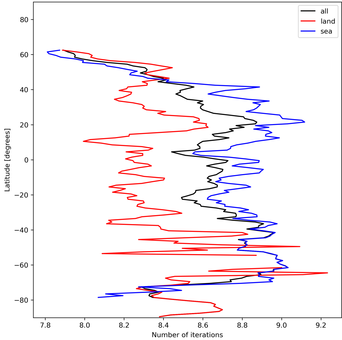
Figure 16: Zonal average of “Number of iterations” for 2024-01-05 to 2024-01-06.
