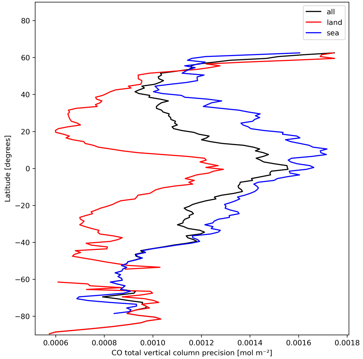
Figure 12: Zonal average of “CO total vertical column precision” for 2024-01-05 to 2024-01-06.
