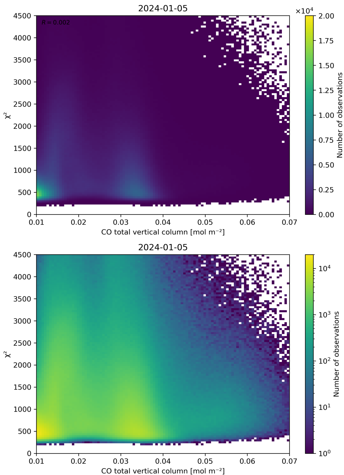
Figure 35: Scatter density plot of “CO total vertical column” against “ \chi^2 ” for 2024-01-05 to 2024-01-06.
