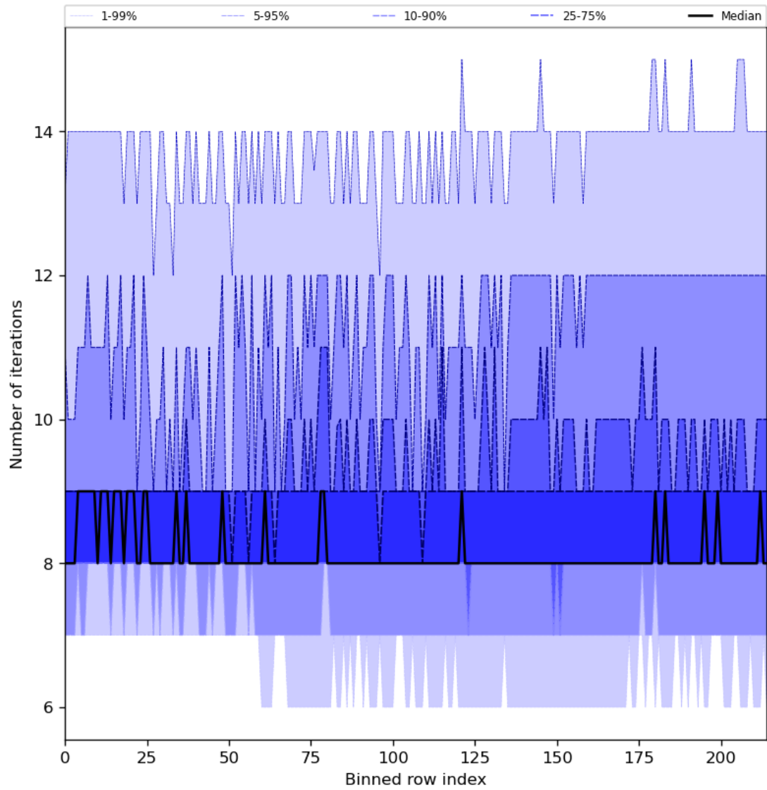
Figure 32: Along track statistics of “Number of iterations” for 2024-01-05 to 2024-01-06
