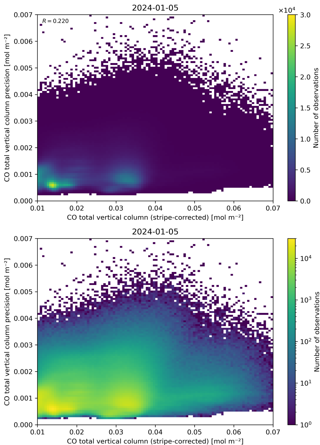
Figure 36: Scatter density plot of “CO total vertical column (stripe-corrected)” against “CO total vertical column precision” for 2024-01-05 to 2024-01-06.
