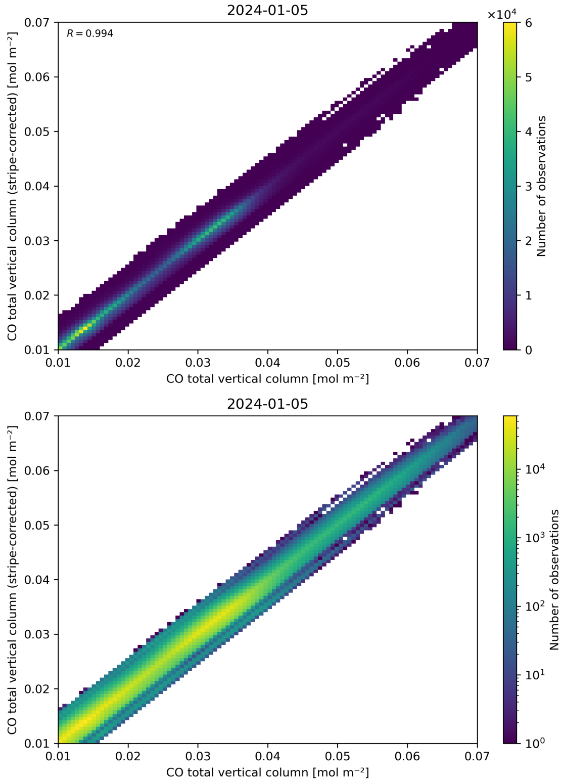
Figure 33: Scatter density plot of “CO total vertical column” against “CO total vertical column (stripe-corrected)” for 2024-01-05 to 2024-01-06.
