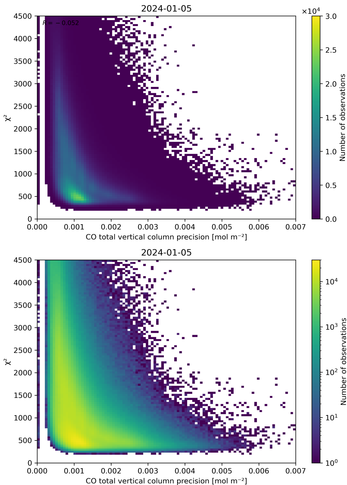
Figure 44: Scatter density plot of “CO total vertical column precision” against “ \chi^2 ” for 2024-01-05 to 2024-01-06.
