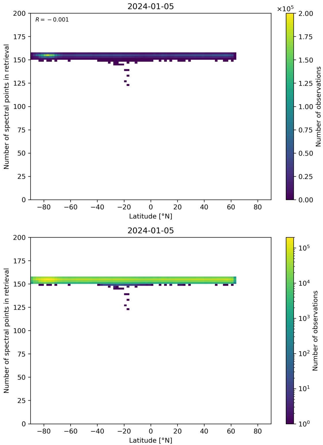
Figure 57: Scatter density plot of “Latitude” against “Number of spectral points in retrieval” for 2024-01-05 to 2024-01-06.
