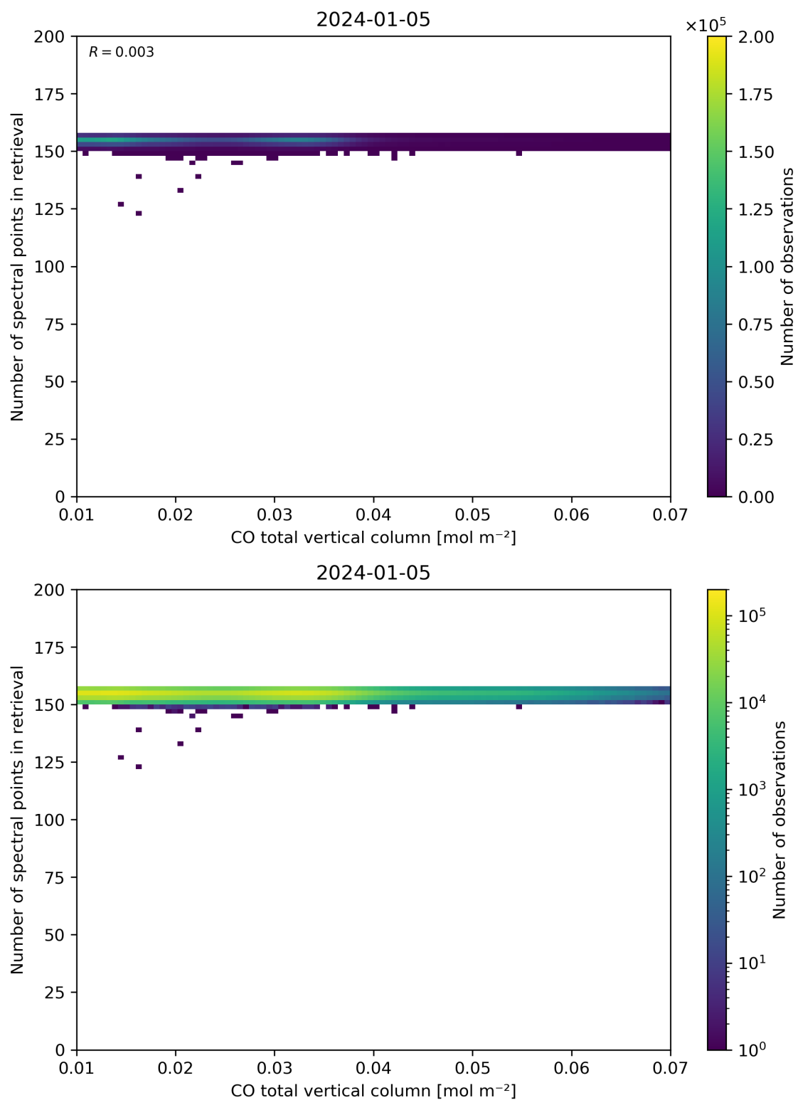
Figure 43: Scatter density plot of “CO total vertical column” against “Number of spectral points in retrieval” for 2024-01-05 to 2024-01-06.
