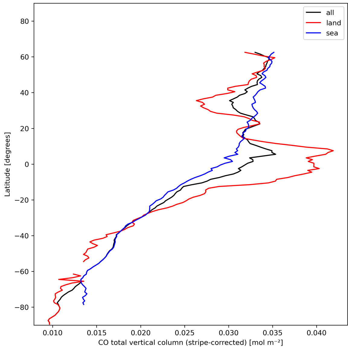
Figure 11: Zonal average of “CO total vertical column (stripe-corrected)” for 2024-01-05 to 2024-01-06.
