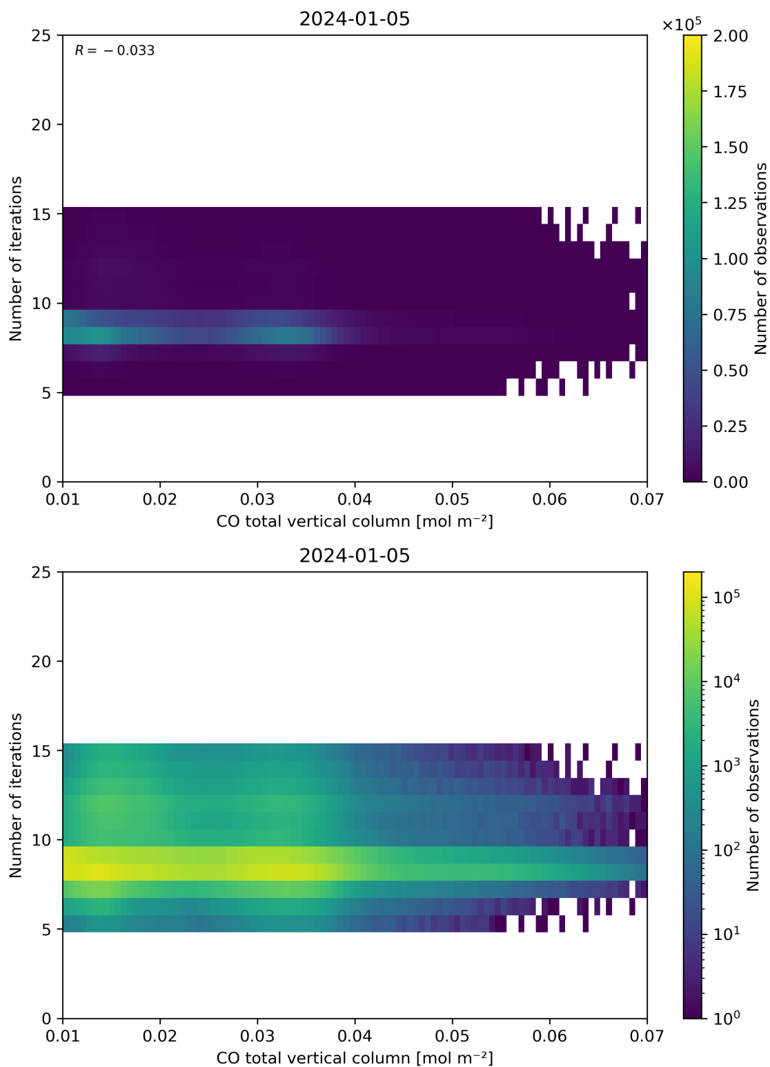
Figure 42: Scatter density plot of “CO total vertical column” against “Number of iterations” for 2024-01-05 to 2024-01-06.
