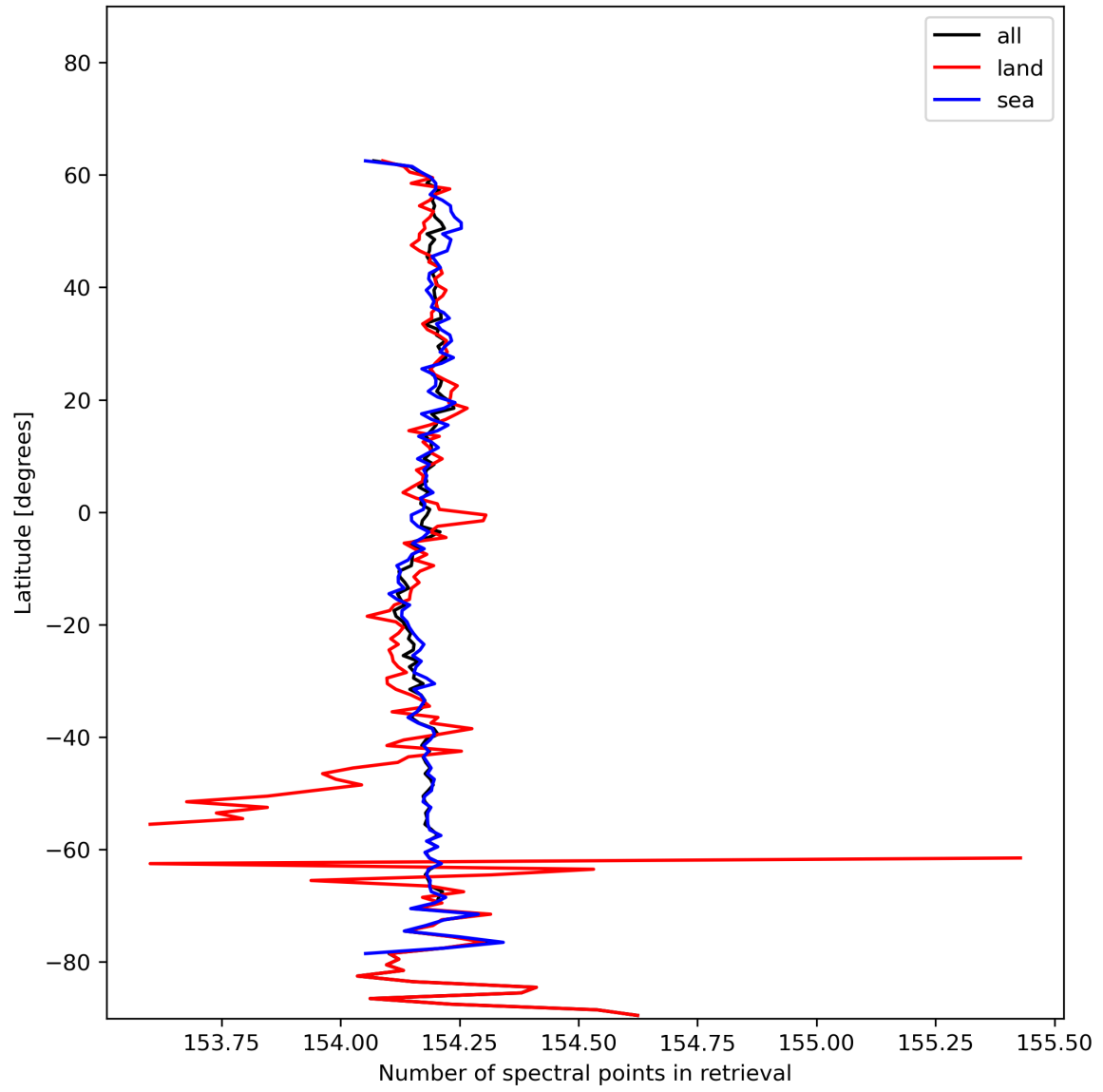
Figure 13: Zonal average of “Number of spectral points in retrieval” for 2024-01-05 to 2024-01-07.
