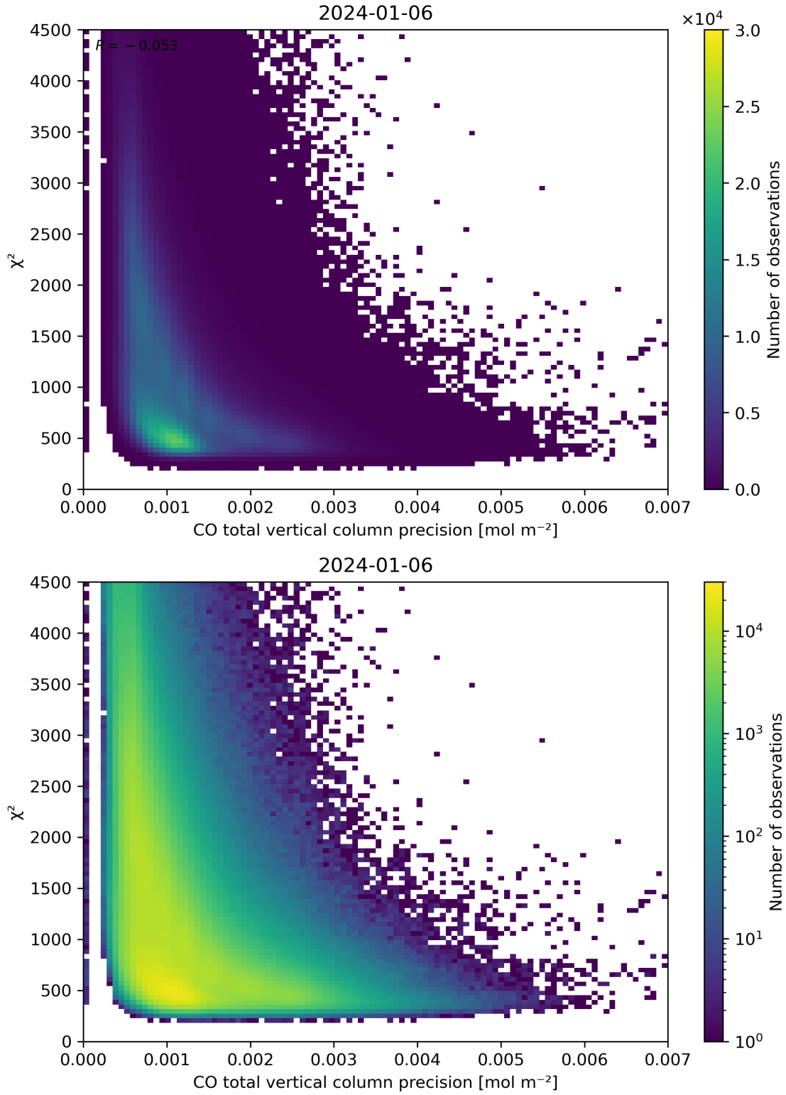
Figure 44: Scatter density plot of “CO total vertical column precision” against “ \chi^2 ” for 2024-01-05 to 2024-01-07.
