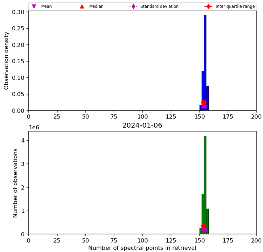
Figure 21: Histogram of “Number of spectral points in retrieval” for 2024-01-05 to 2024-01-07
