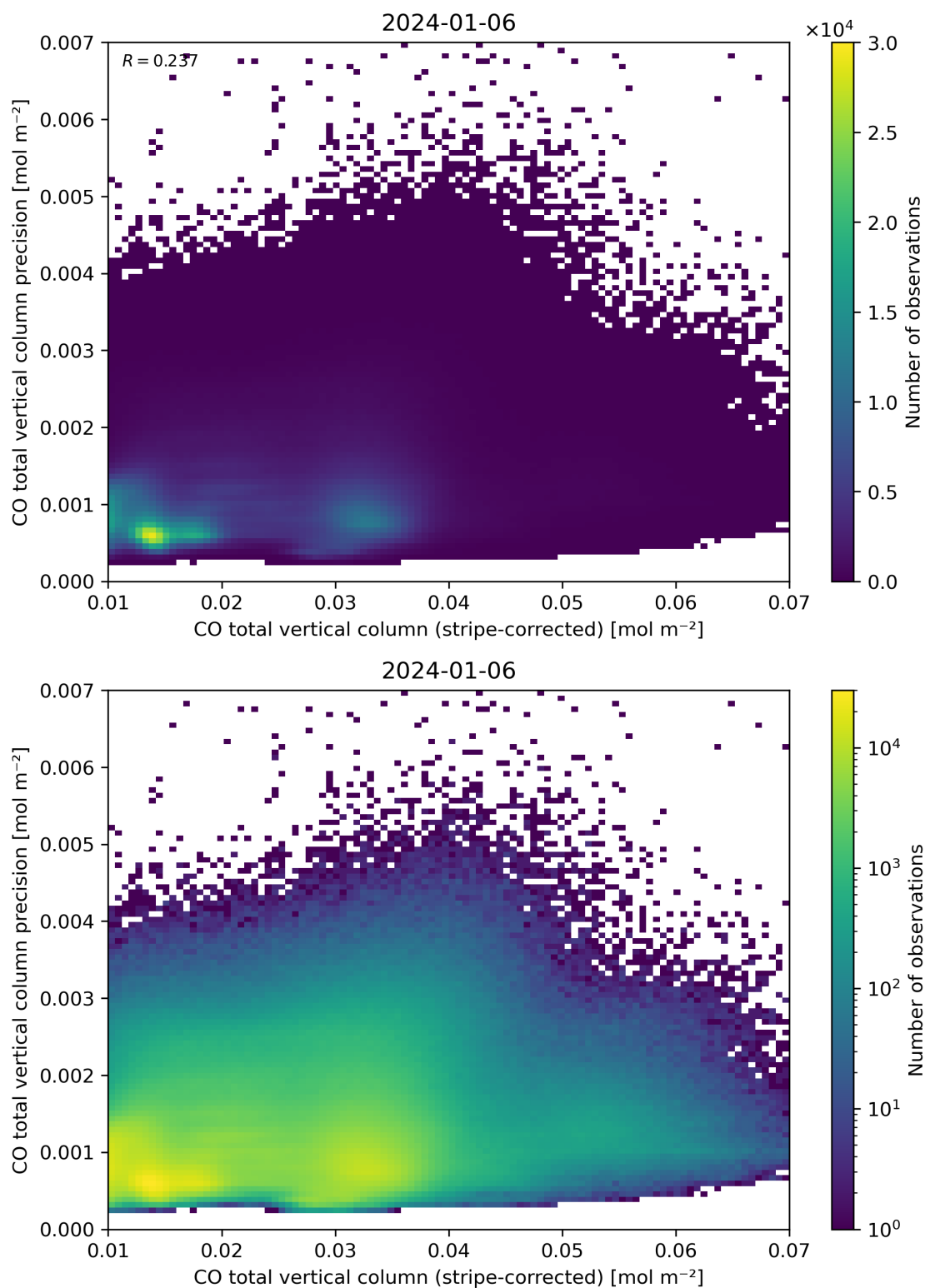
Figure 36: Scatter density plot of “CO total vertical column (stripe-corrected)” against “CO total vertical column precision” for 2024-01-05 to 2024-01-07.
