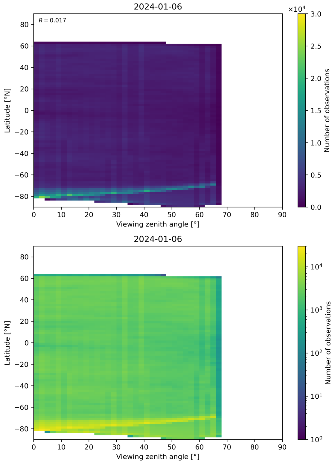
Figure 74: Scatter density plot of “Viewing zenith angle” against “Latitude” for 2024-01-05 to 2024-01-07.
