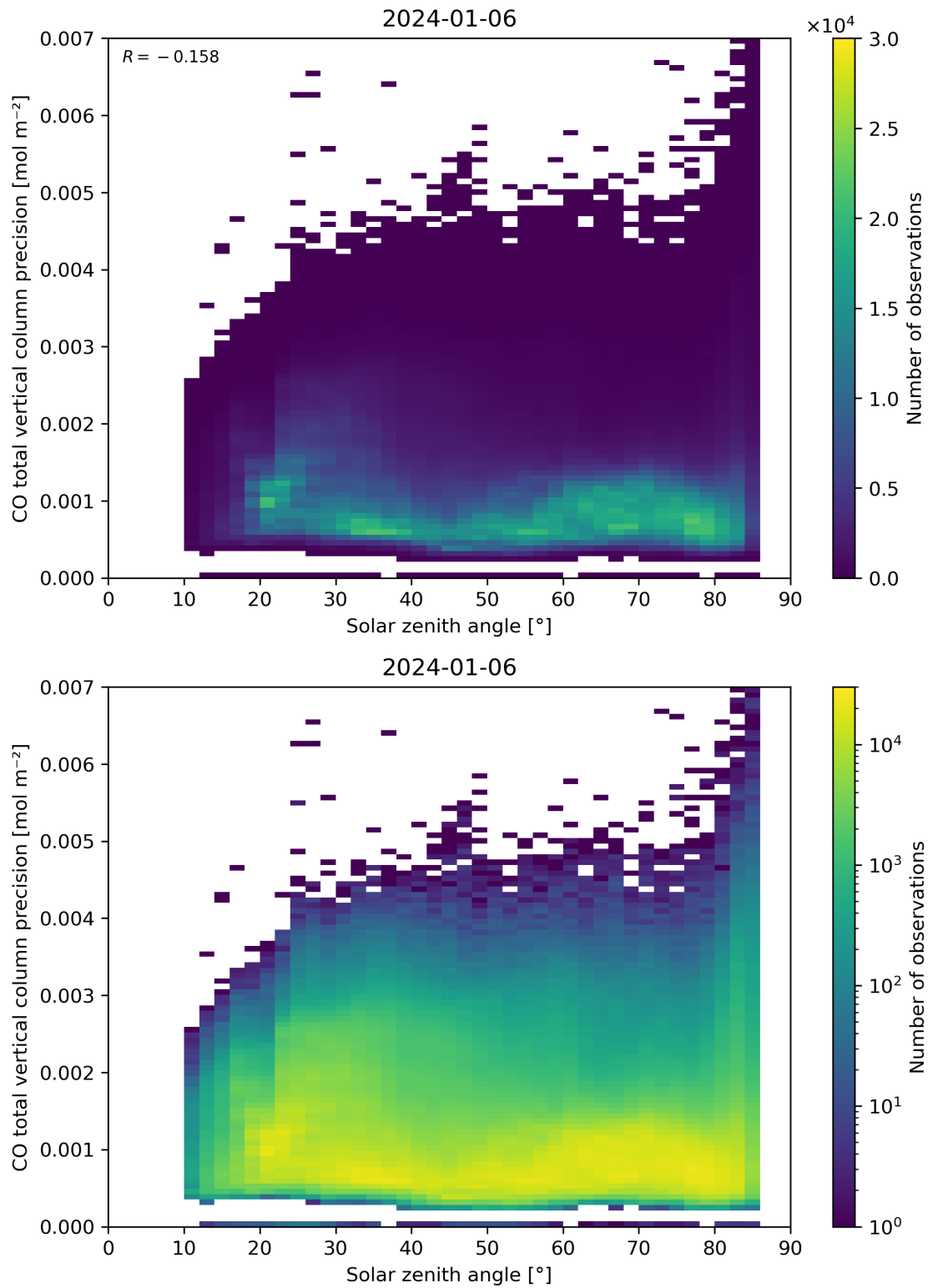
Figure 63: Scatter density plot of “Solar zenith angle” against “CO total vertical column precision” for 2024-01-05 to 2024-01-07.
