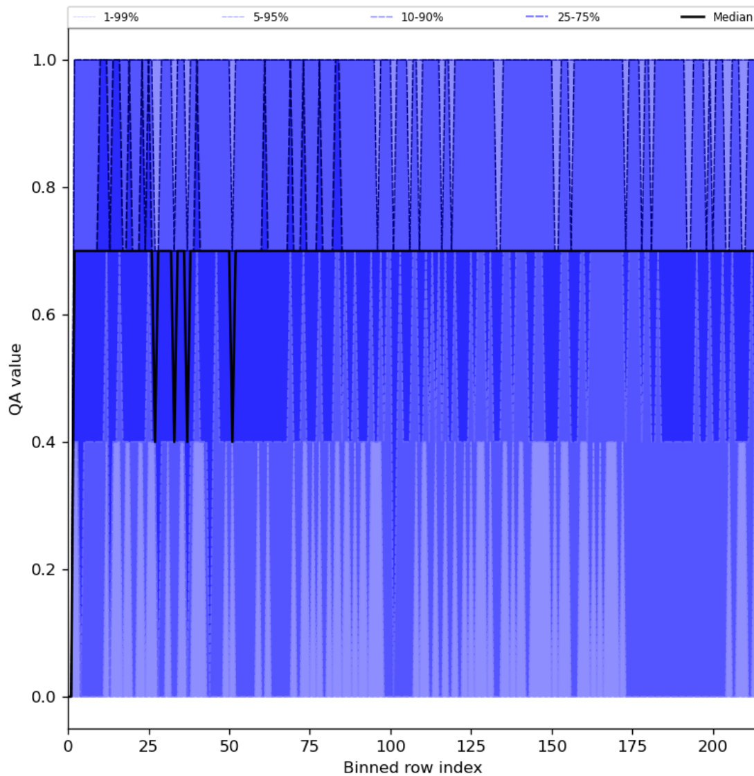
Figure 25: Along track statistics of “QA value” for 2024-01-05 to 2024-01-07
