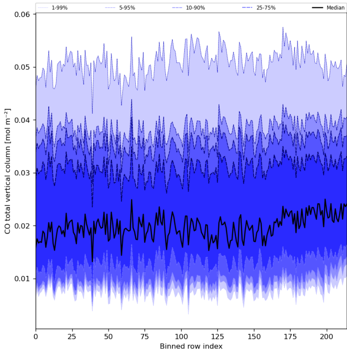
Figure 26: Along track statistics of "CO total vertical column" for 2024-01-05 to 2024-01-07
