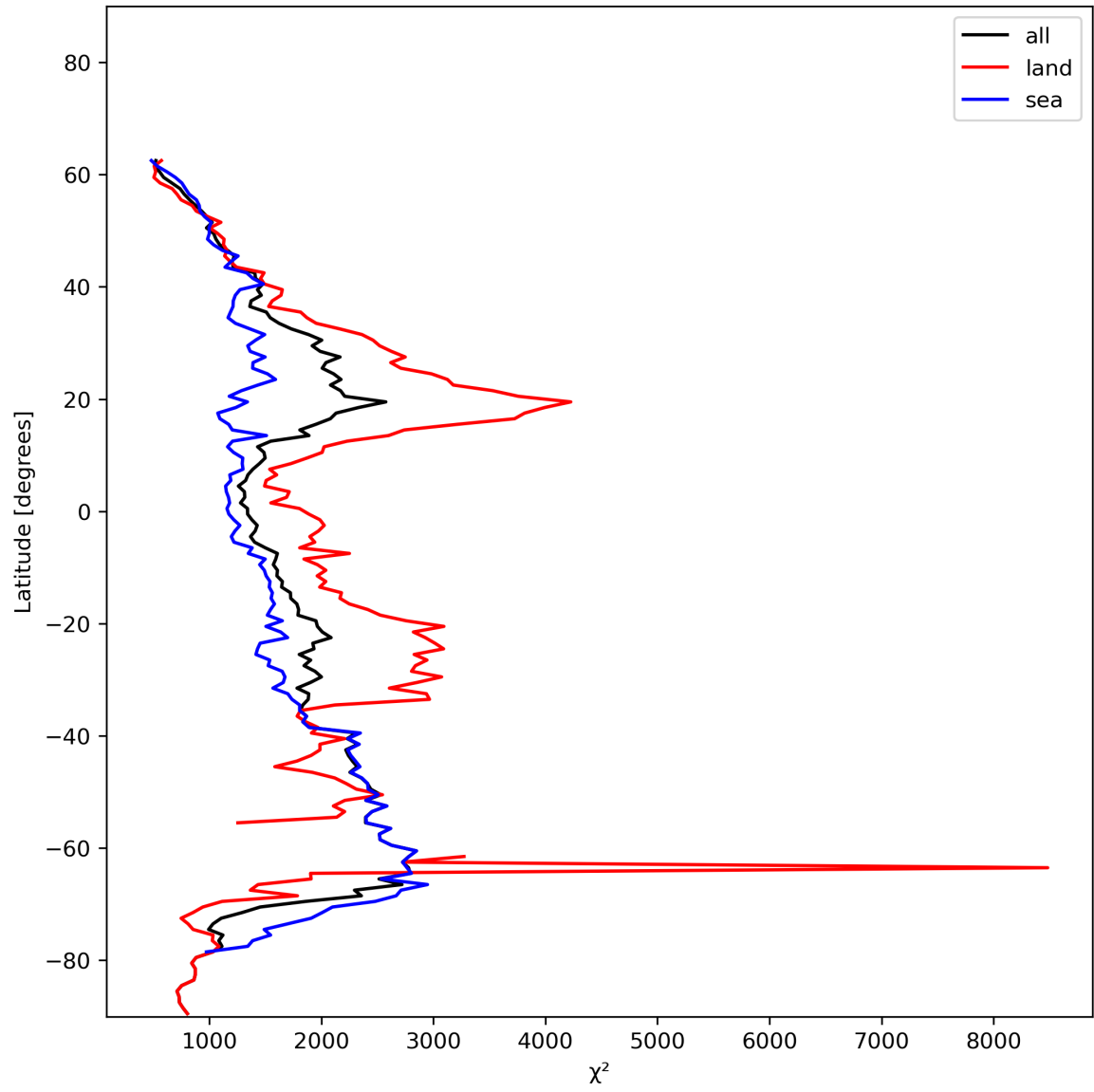
Figure 14: Zonal average of “ \chi^2 ” for 2024-01-05 to 2024-01-07.
