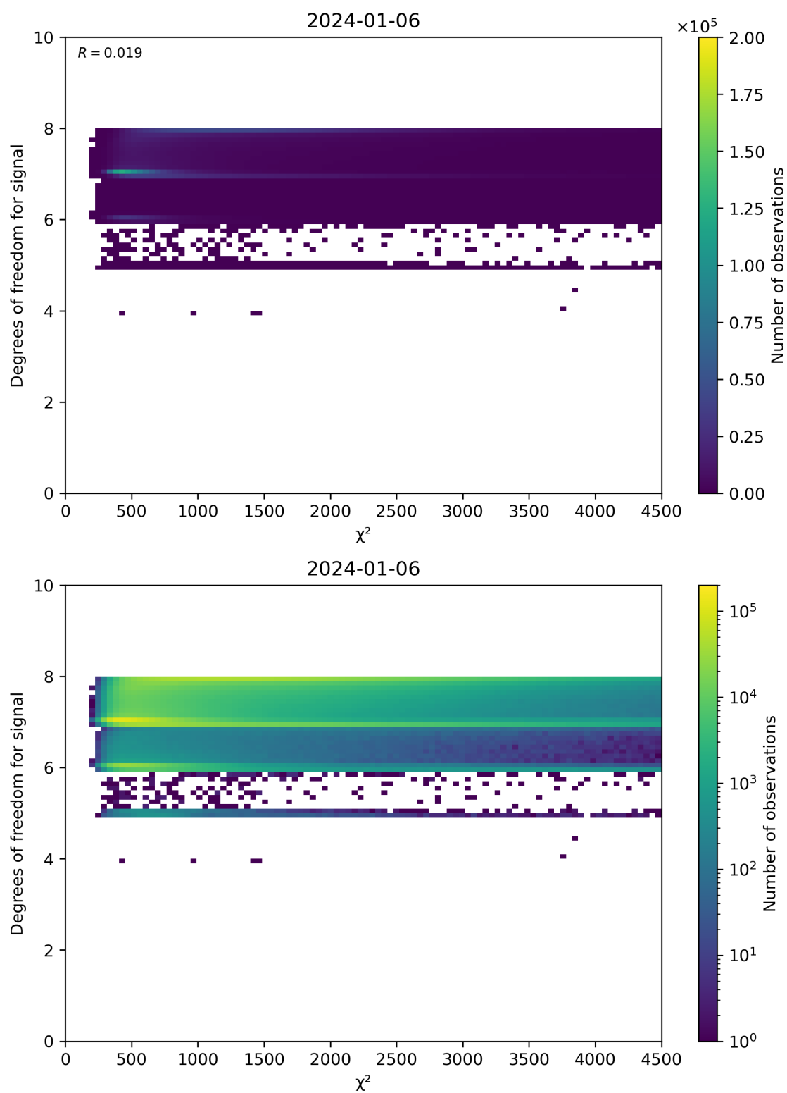
Figure 48: Scatter density plot of “ \chi^2 ” against “Degrees of freedom for signal” for 2024-01-05 to 2024-01-07.
