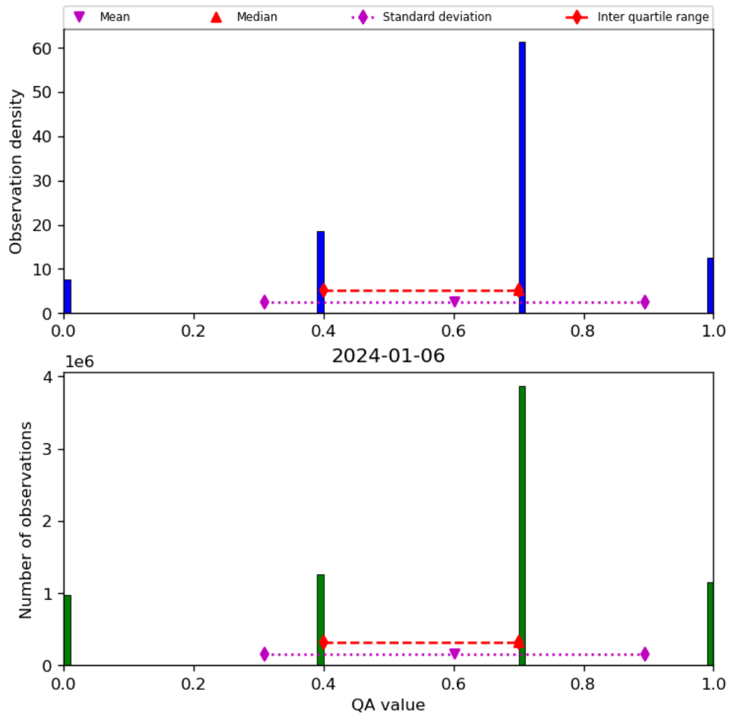
Figure 17: Histogram of “QA value” for 2024-01-05 to 2024-01-07
