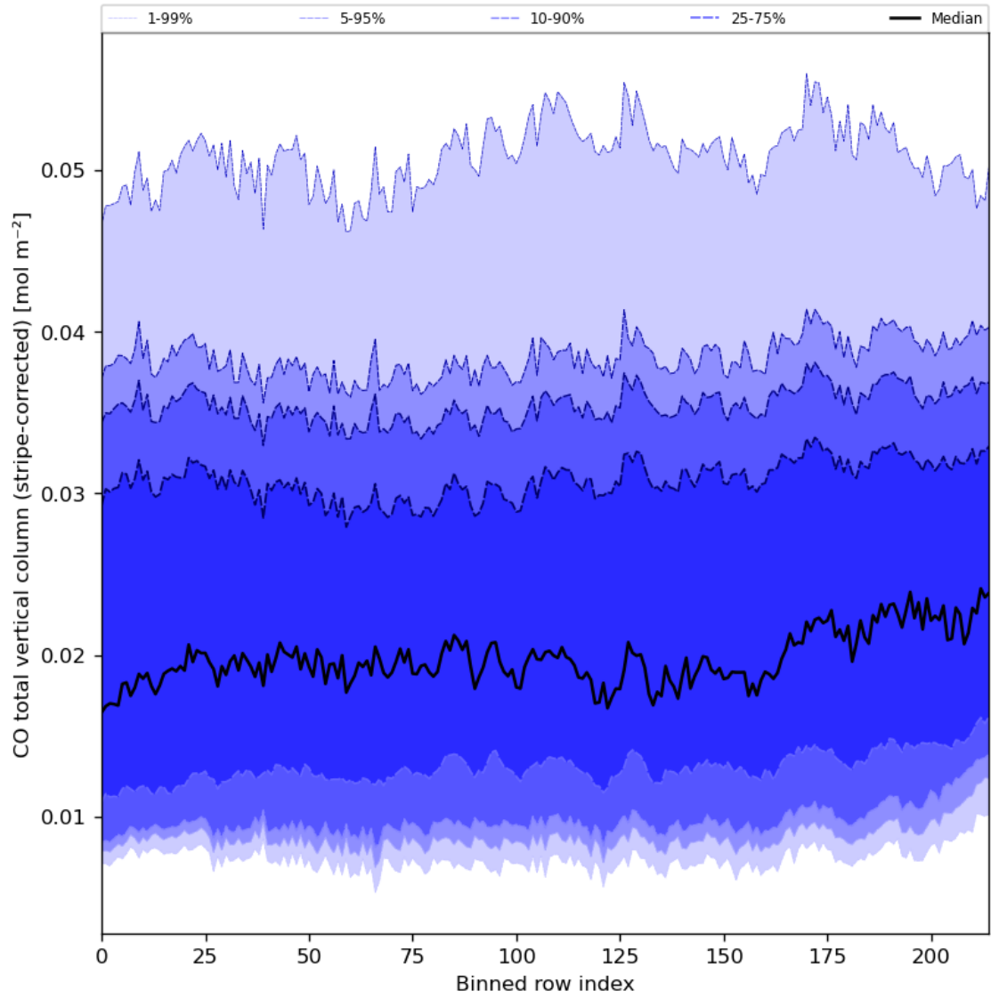
Figure 27: Along track statistics of “CO total vertical column (stripe-corrected)” for 2024-01-05 to 2024-01-07
