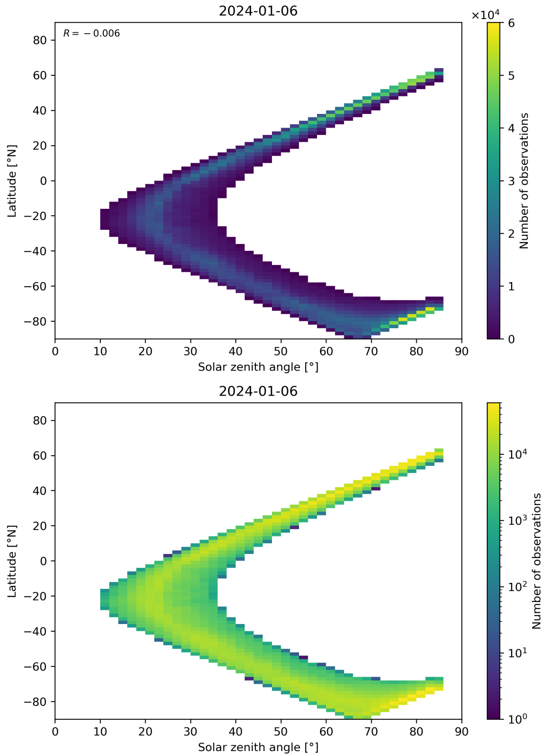
Figure 66: Scatter density plot of “Solar zenith angle” against “Latitude” for 2024-01-05 to 2024-01-07.
