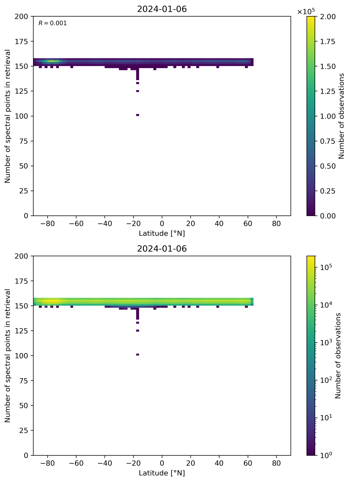
Figure 57: Scatter density plot of “Latitude” against “Number of spectral points in retrieval” for 2024-01-05 to 2024-01-07.
