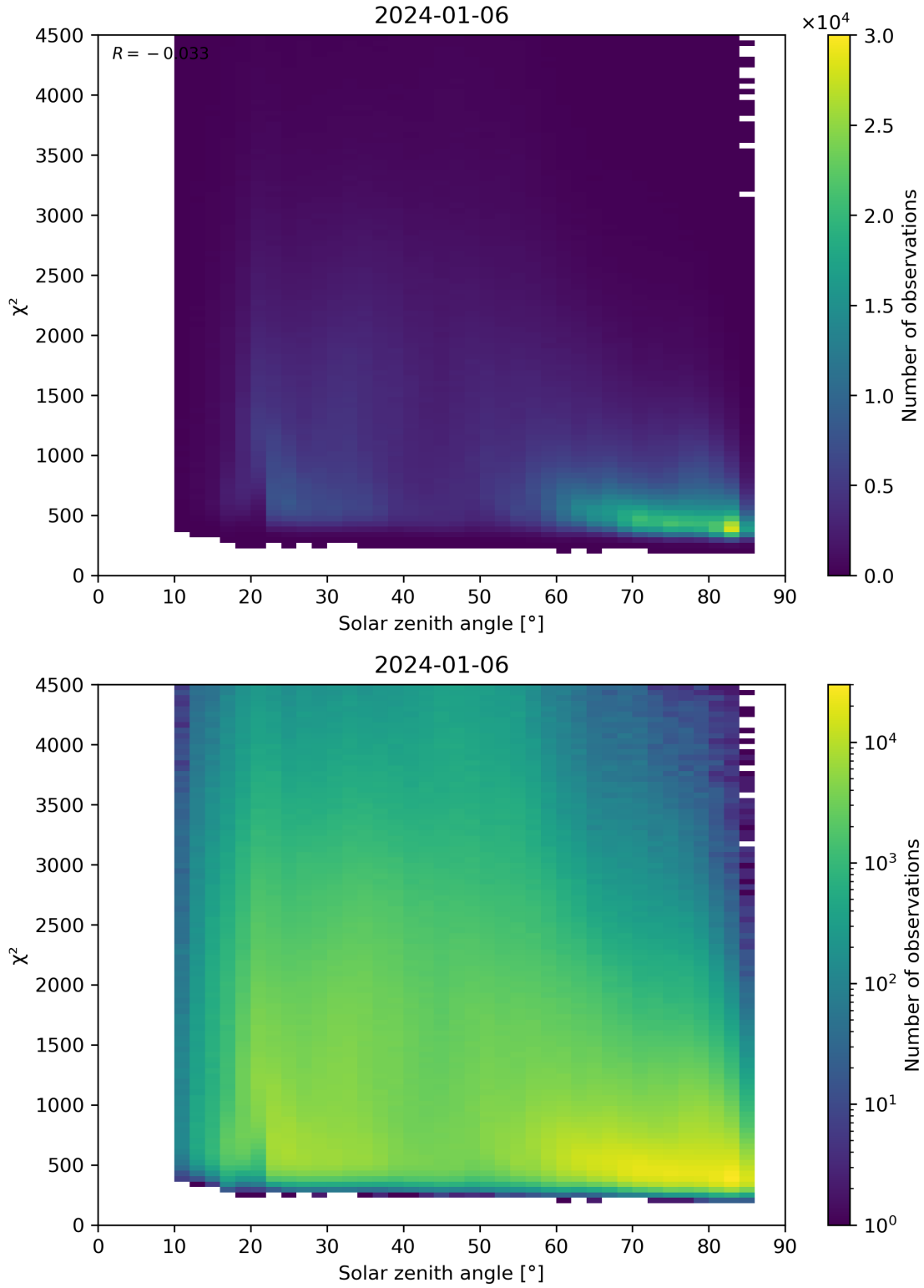
Figure 64: Scatter density plot of “Solar zenith angle” against “ \chi^2 ” for 2024-01-05 to 2024-01-07.
