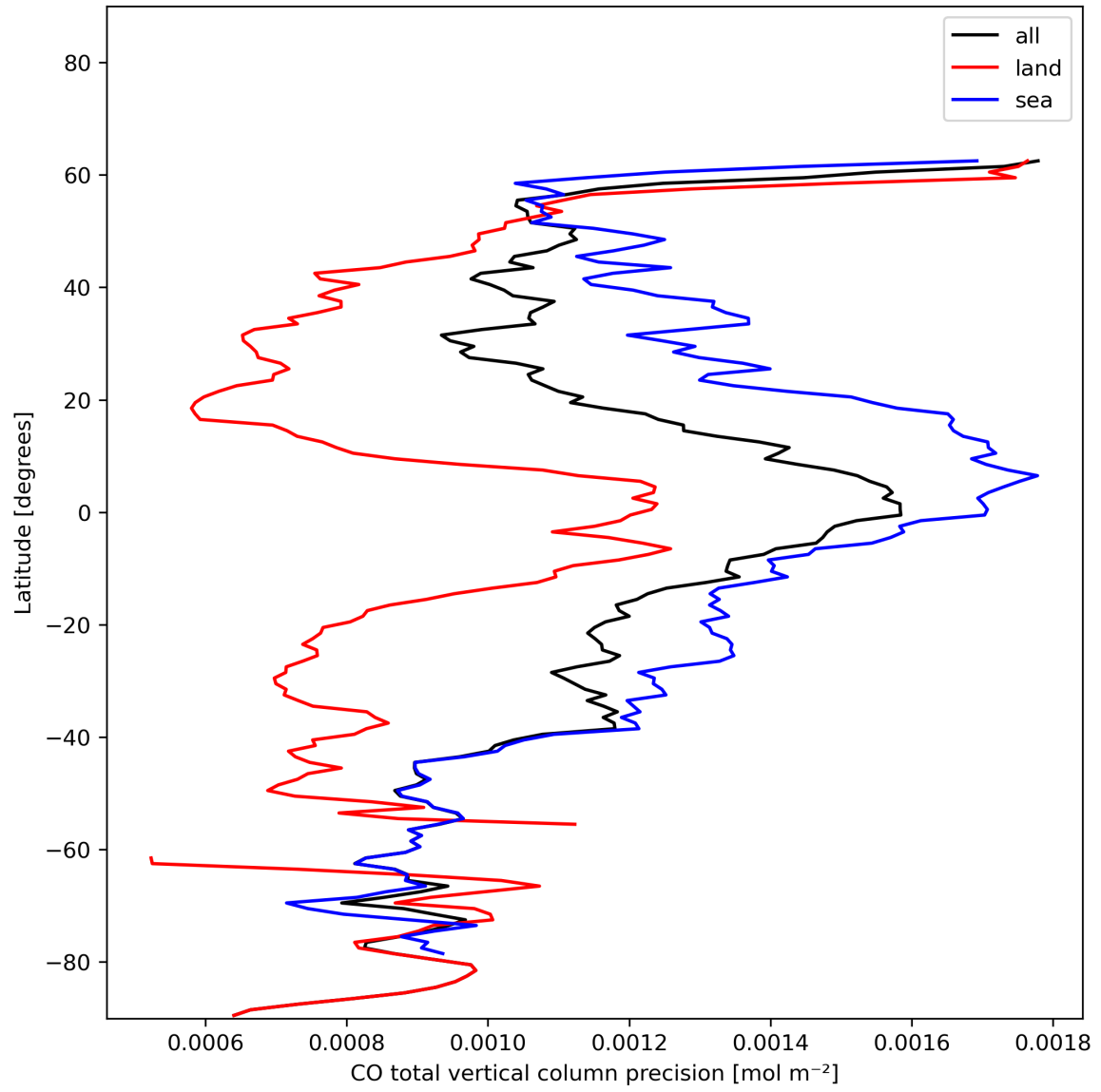
Figure 12: Zonal average of “CO total vertical column precision” for 2024-01-05 to 2024-01-07.
