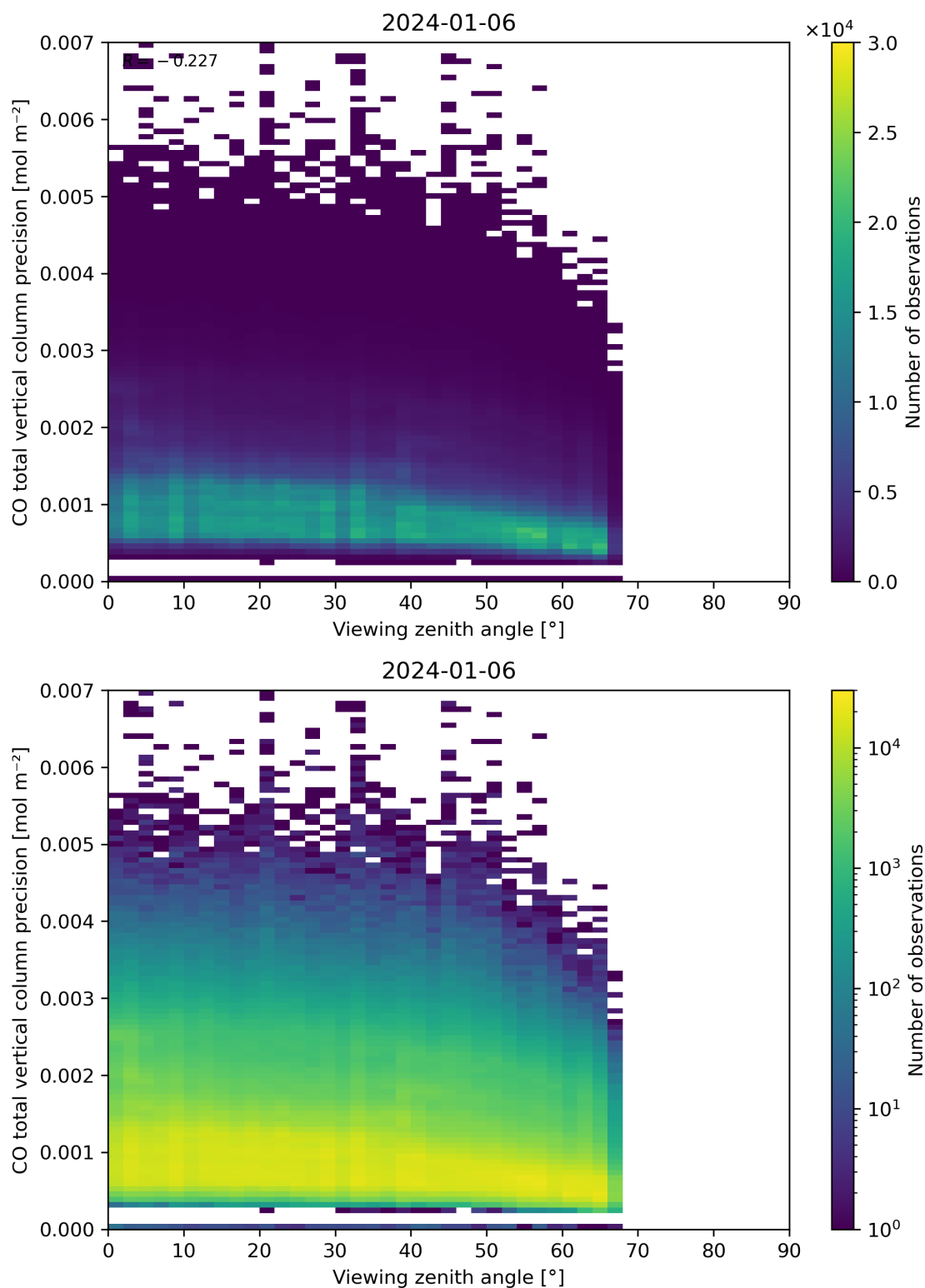
Figure 71: Scatter density plot of “Viewing zenith angle” against “CO total vertical column precision” for 2024-01-05 to 2024-01-07.
