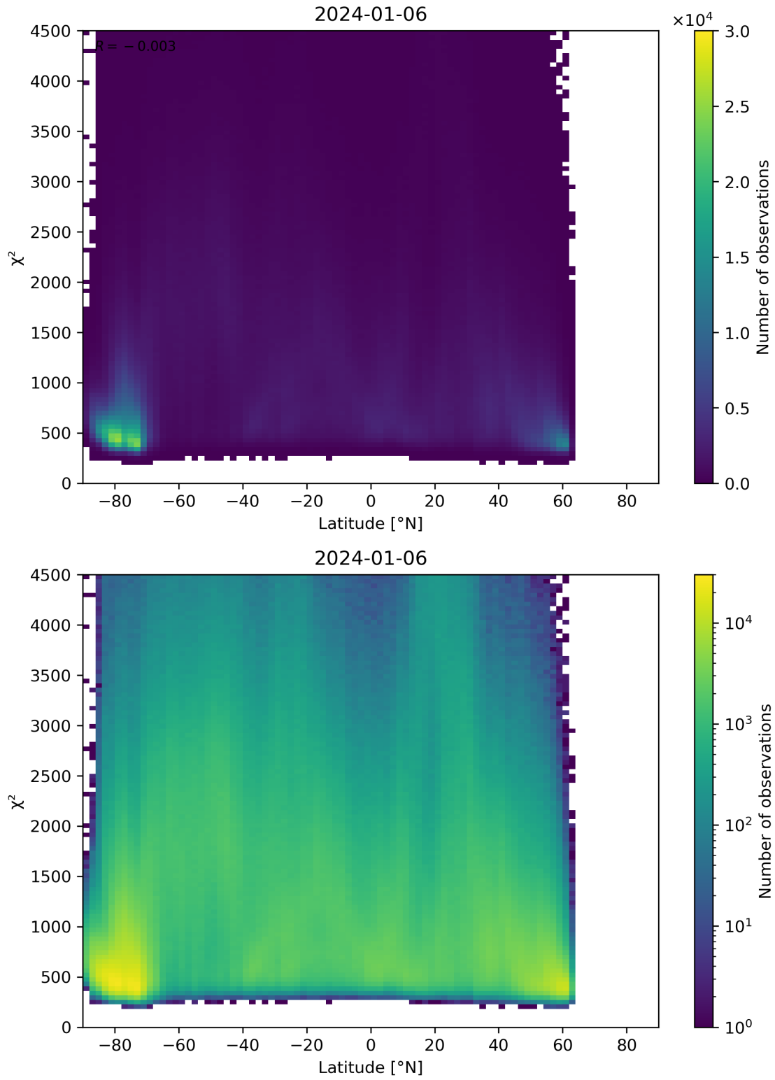
Figure 54: Scatter density plot of “Latitude” against “ \chi^2 ” for 2024-01-05 to 2024-01-07.
