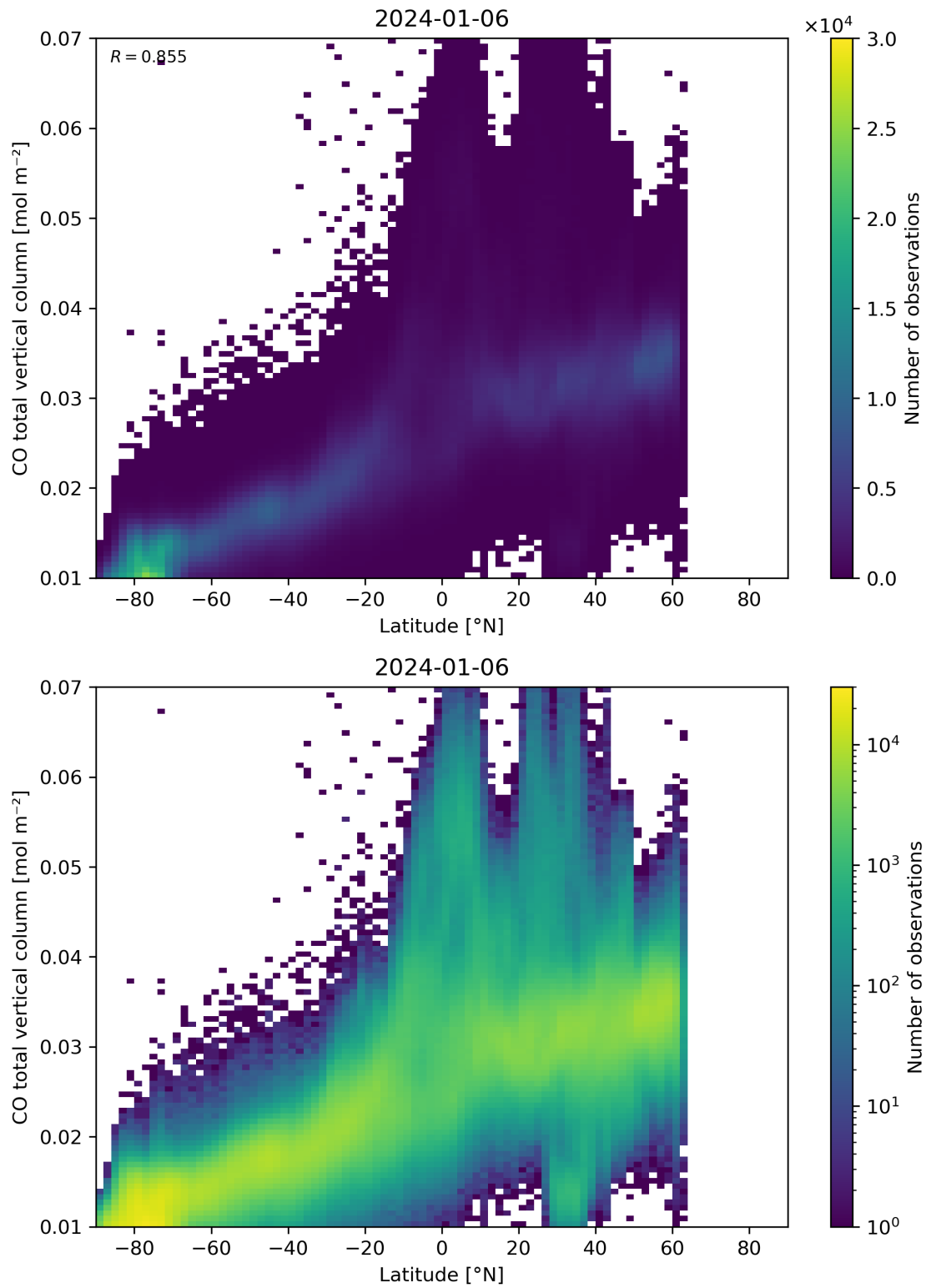
Figure 51: Scatter density plot of “Latitude” against “CO total vertical column” for 2024-01-05 to 2024-01-07.
