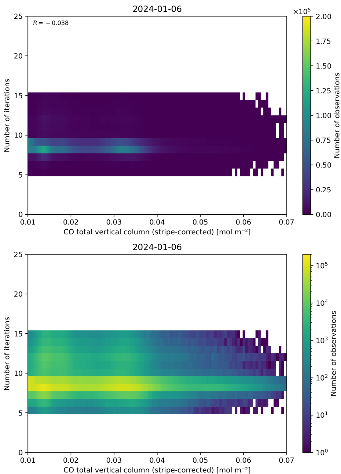
Figure 39: Scatter density plot of “CO total vertical column (stripe-corrected)” against “Number of iterations” for 2024-01-05 to 2024-01-07.
