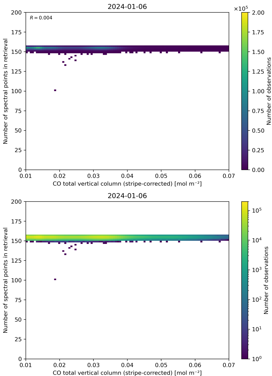
Figure 40: Scatter density plot of “CO total vertical column (stripe-corrected)” against “Number of spectral points in retrieval” for 2024-01-05 to 2024-01-07.
