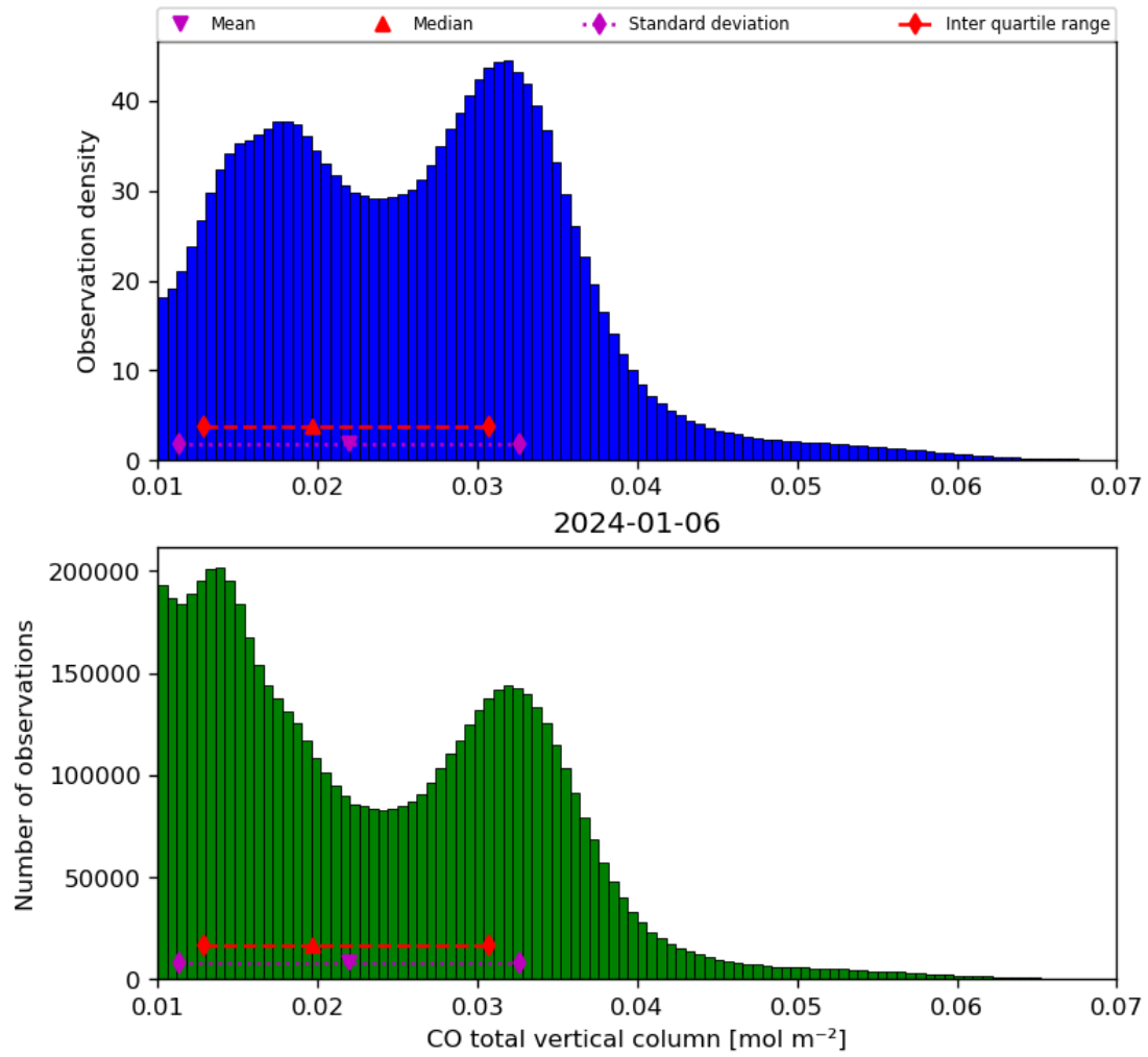
Figure 18: Histogram of “CO total vertical column” for 2024-01-05 to 2024-01-07
