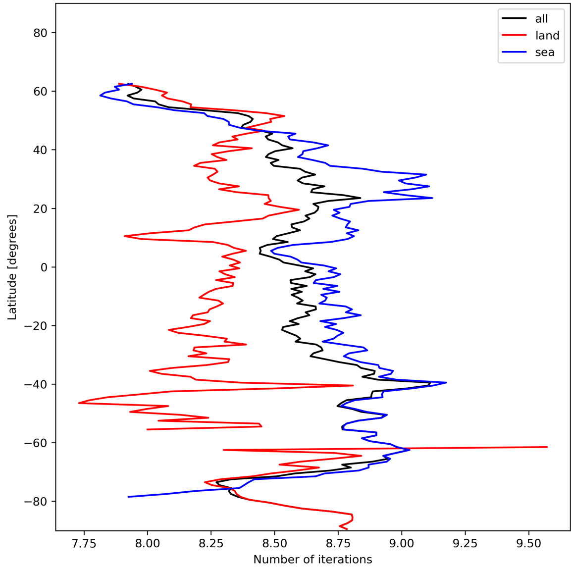
Figure 16: Zonal average of “Number of iterations” for 2024-01-05 to 2024-01-07.
