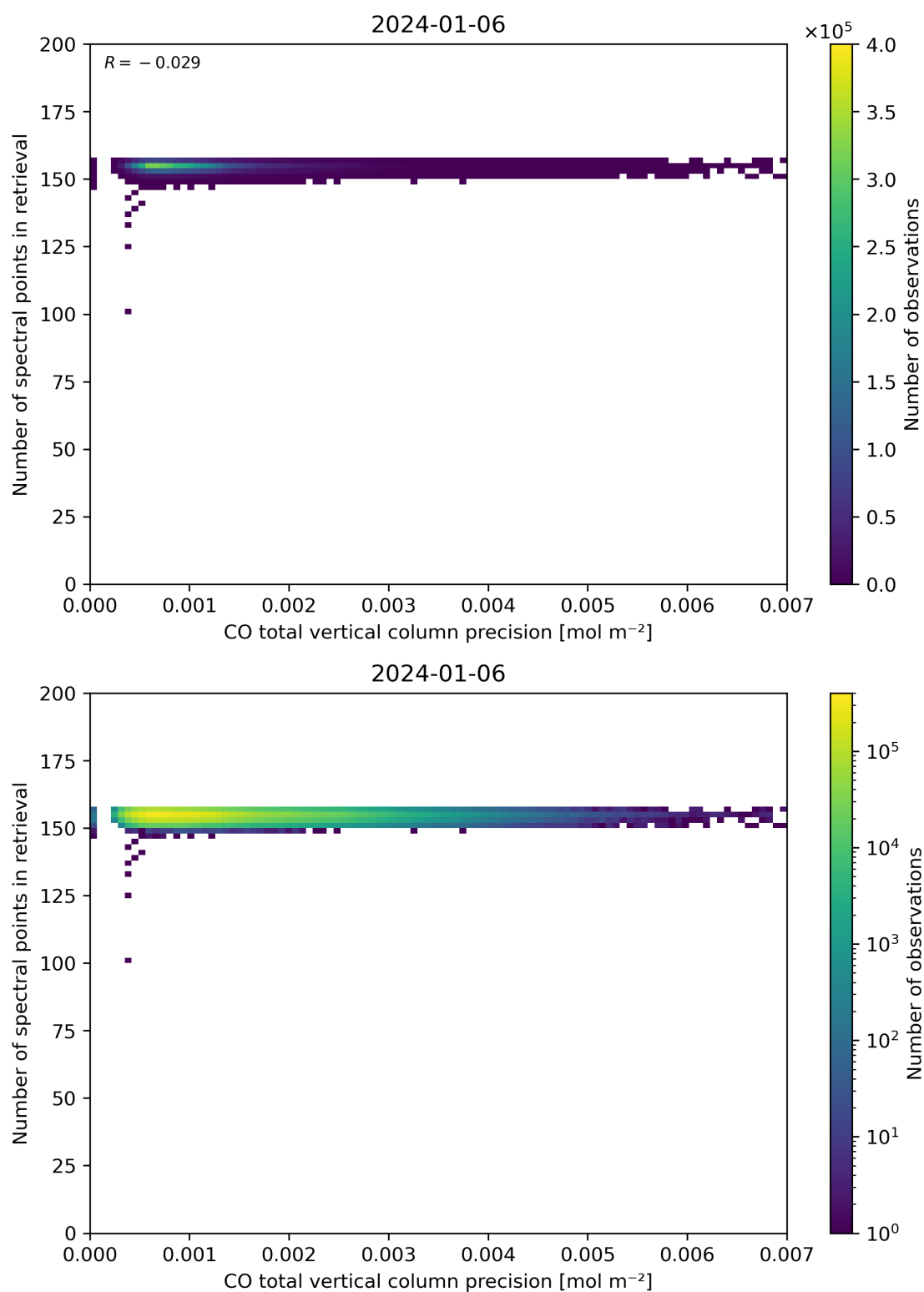
Figure 47: Scatter density plot of “CO total vertical column precision” against “Number of spectral points in retrieval” for 2024-01-05 to 2024-01-07.
