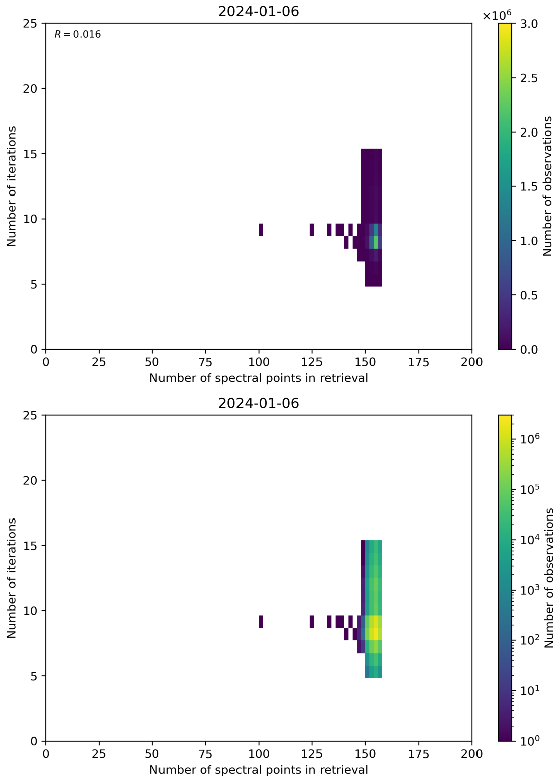
Figure 60: Scatter density plot of “Number of spectral points in retrieval” against “Number of iterations” for 2024-01-05 to 2024-01-07.
