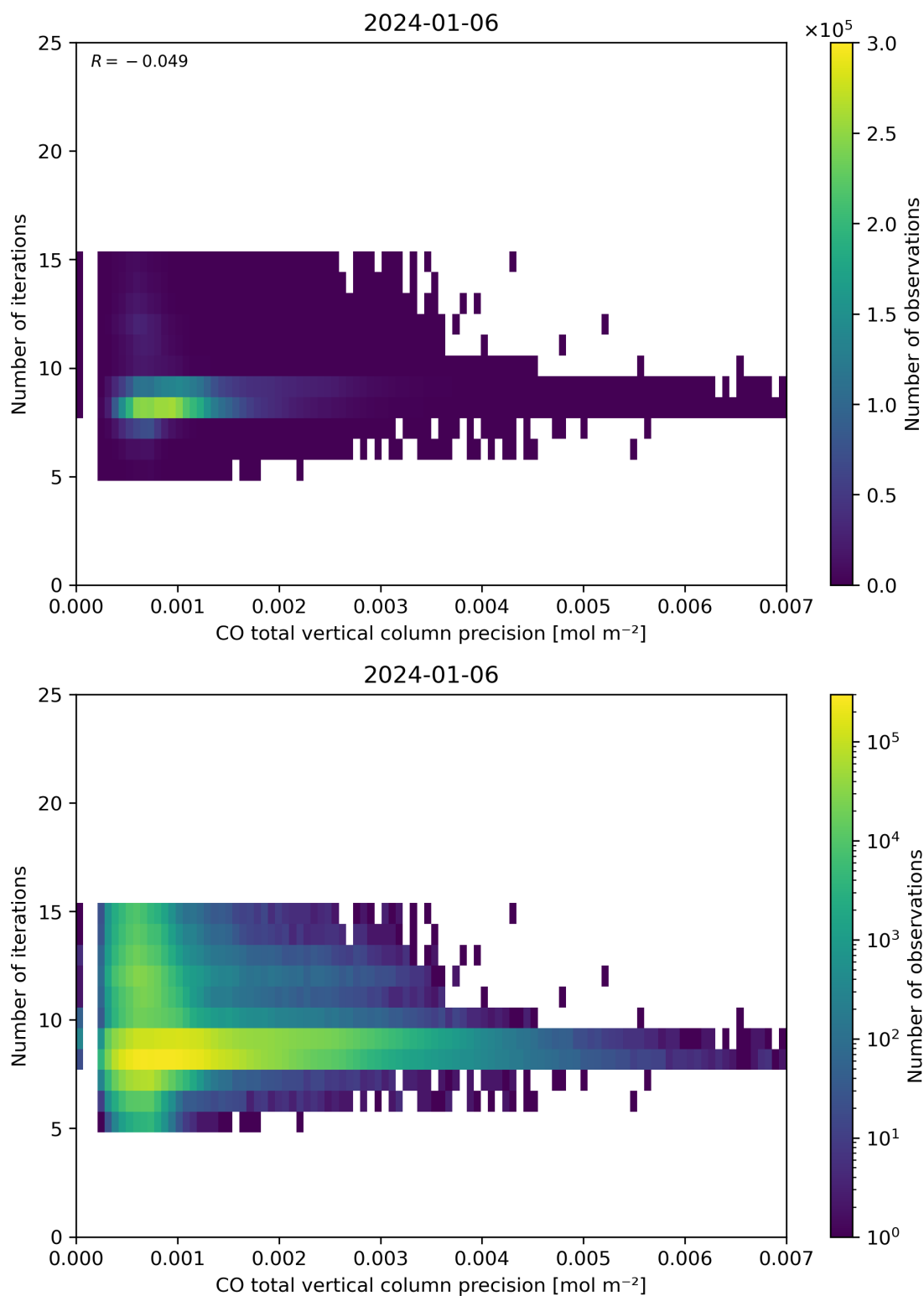
Figure 46: Scatter density plot of “CO total vertical column precision” against “Number of iterations” for 2024-01-05 to 2024-01-07.
