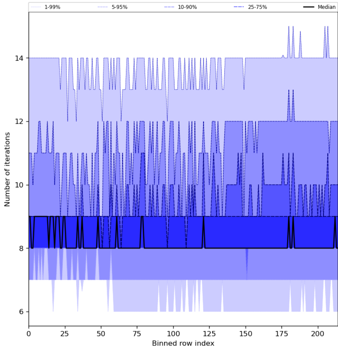
Figure 32: Along track statistics of “Number of iterations” for 2024-01-05 to 2024-01-07
