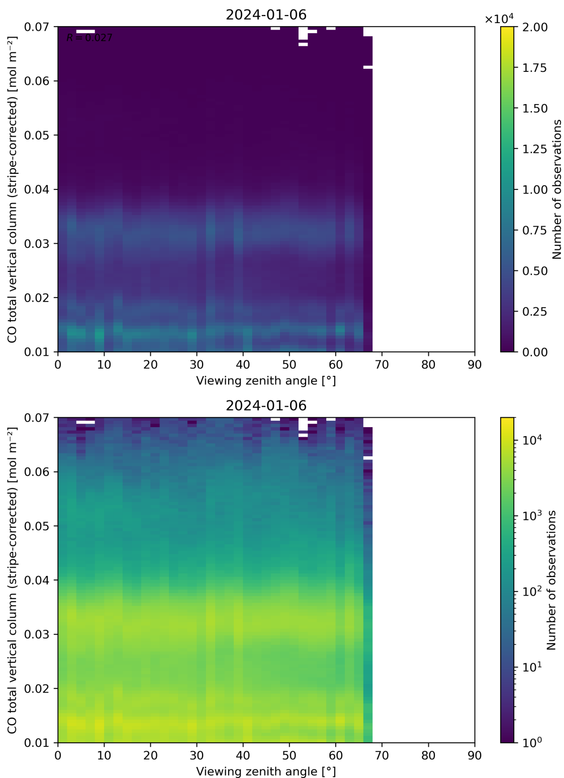
Figure 70: Scatter density plot of “Viewing zenith angle” against “CO total vertical column (stripe-corrected)” for 2024-01-05 to 2024-01-07.
