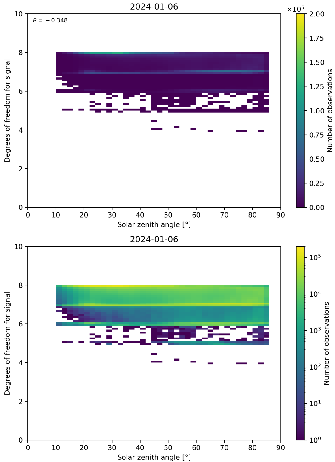
Figure 65: Scatter density plot of “Solar zenith angle” against “Degrees of freedom for signal” for 2024-01-05 to 2024-01-07.
