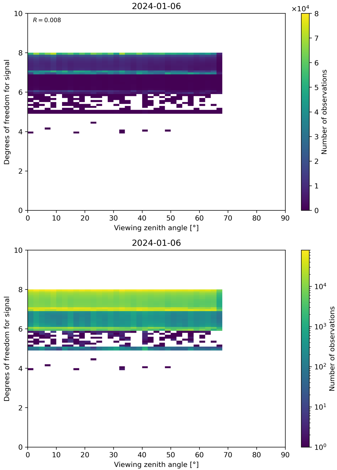
Figure 73: Scatter density plot of “Viewing zenith angle” against “Degrees of freedom for signal” for 2024-01-05 to 2024-01-07.
