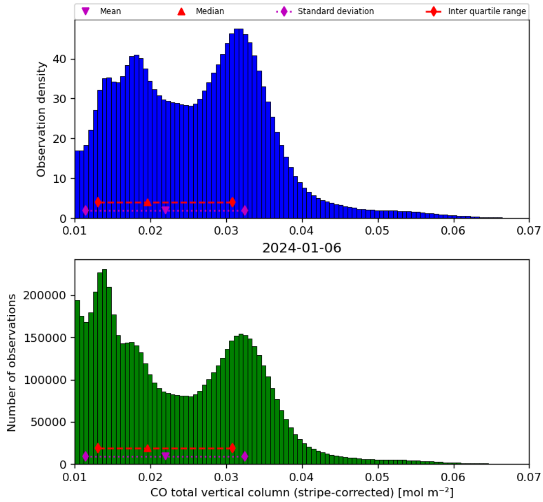
Figure 19: Histogram of “CO total vertical column (stripe-corrected)” for 2024-01-05 to 2024-01-07
