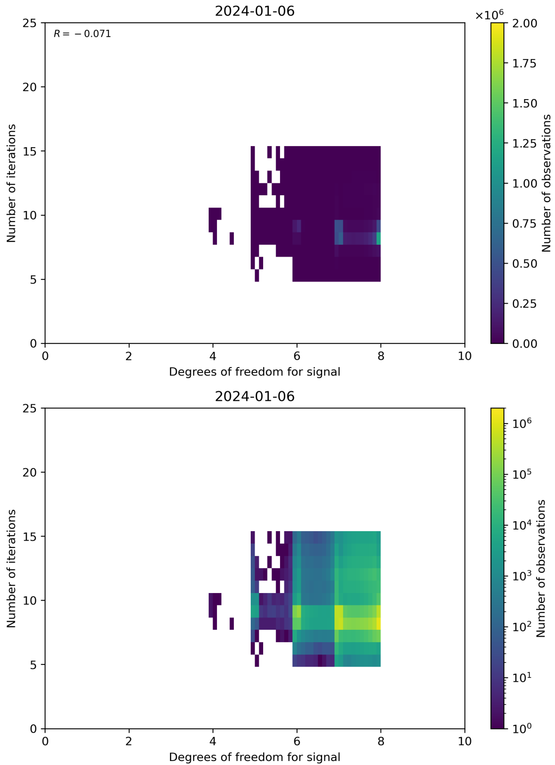
Figure 50: Scatter density plot of “Degrees of freedom for signal” against “Number of iterations” for 2024-01-05 to 2024-01-07.
