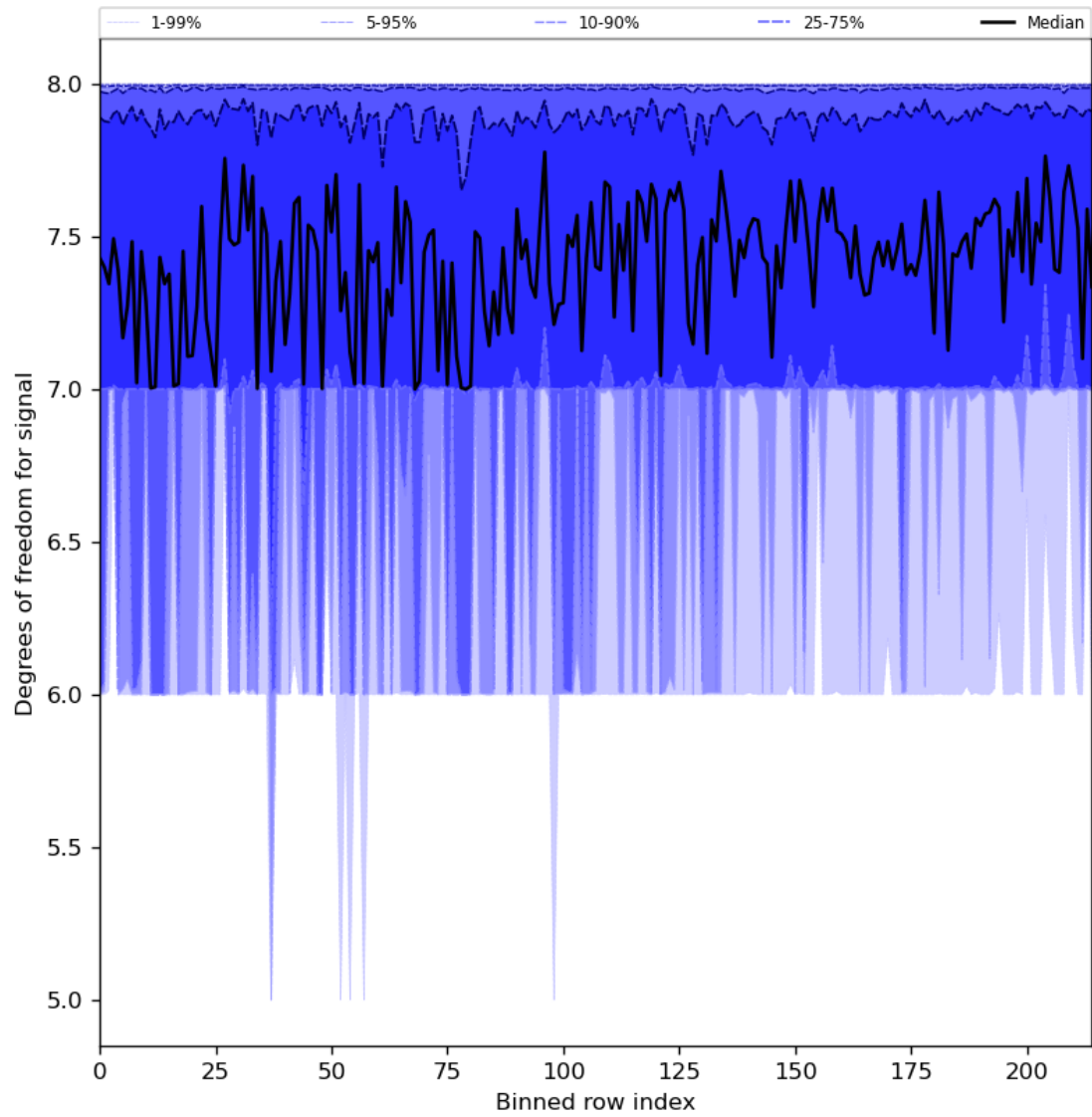
Figure 31: Along track statistics of “Degrees of freedom for signal” for 2024-01-05 to 2024-01-07
