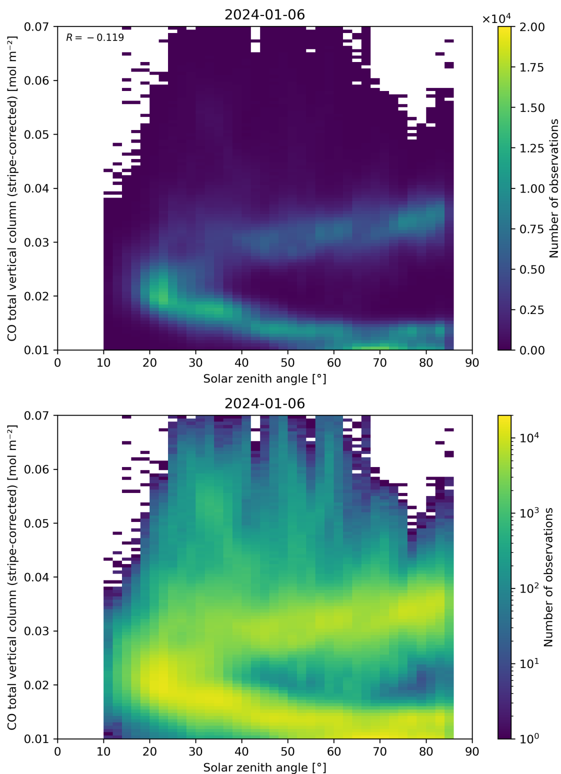
Figure 62: Scatter density plot of “Solar zenith angle” against “CO total vertical column (stripe-corrected)” for 2024-01-05 to 2024-01-07.
