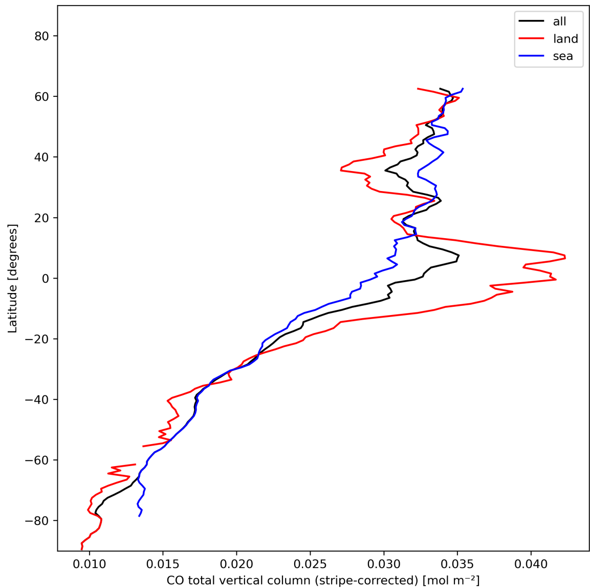
Figure 11: Zonal average of “CO total vertical column (stripe-corrected)” for 2024-01-05 to 2024-01-07.
