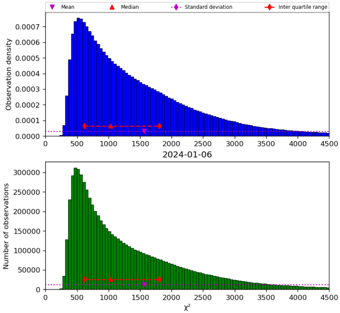
Figure 22: Histogram of “ \chi^2 ” for 2024-01-05 to 2024-01-07
