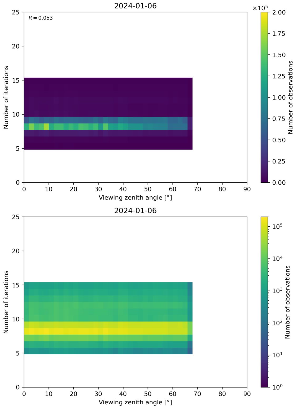
Figure 75: Scatter density plot of “Viewing zenith angle” against “Number of iterations” for 2024-01-05 to 2024-01-07.
