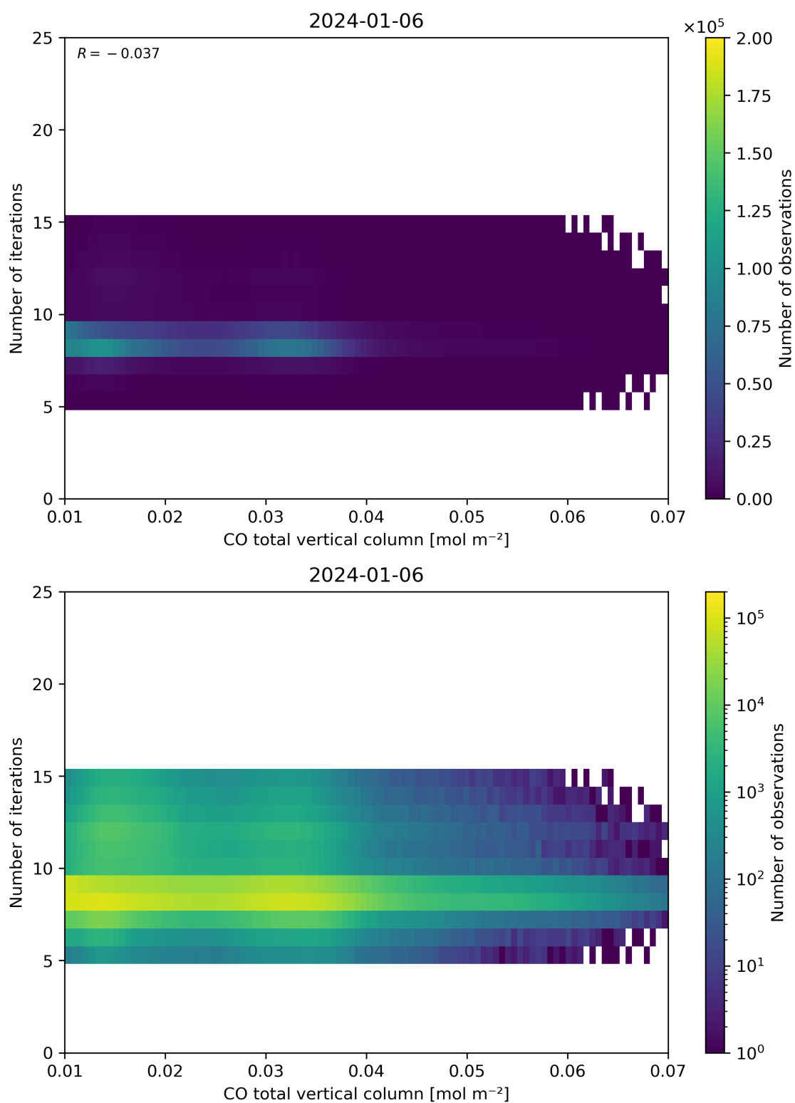
Figure 42: Scatter density plot of “CO total vertical column” against “Number of iterations” for 2024-01-05 to 2024-01-07.
