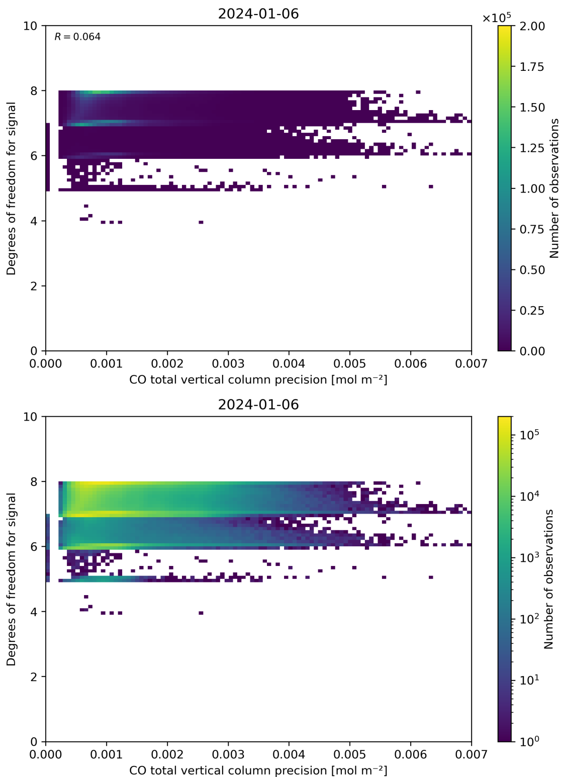
Figure 45: Scatter density plot of “CO total vertical column precision” against “Degrees of freedom for signal” for 2024-01-05 to 2024-01-07.
