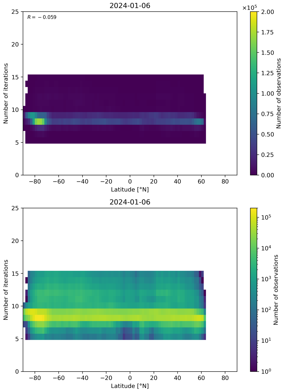
Figure 56: Scatter density plot of “Latitude” against “Number of iterations” for 2024-01-05 to 2024-01-07.
