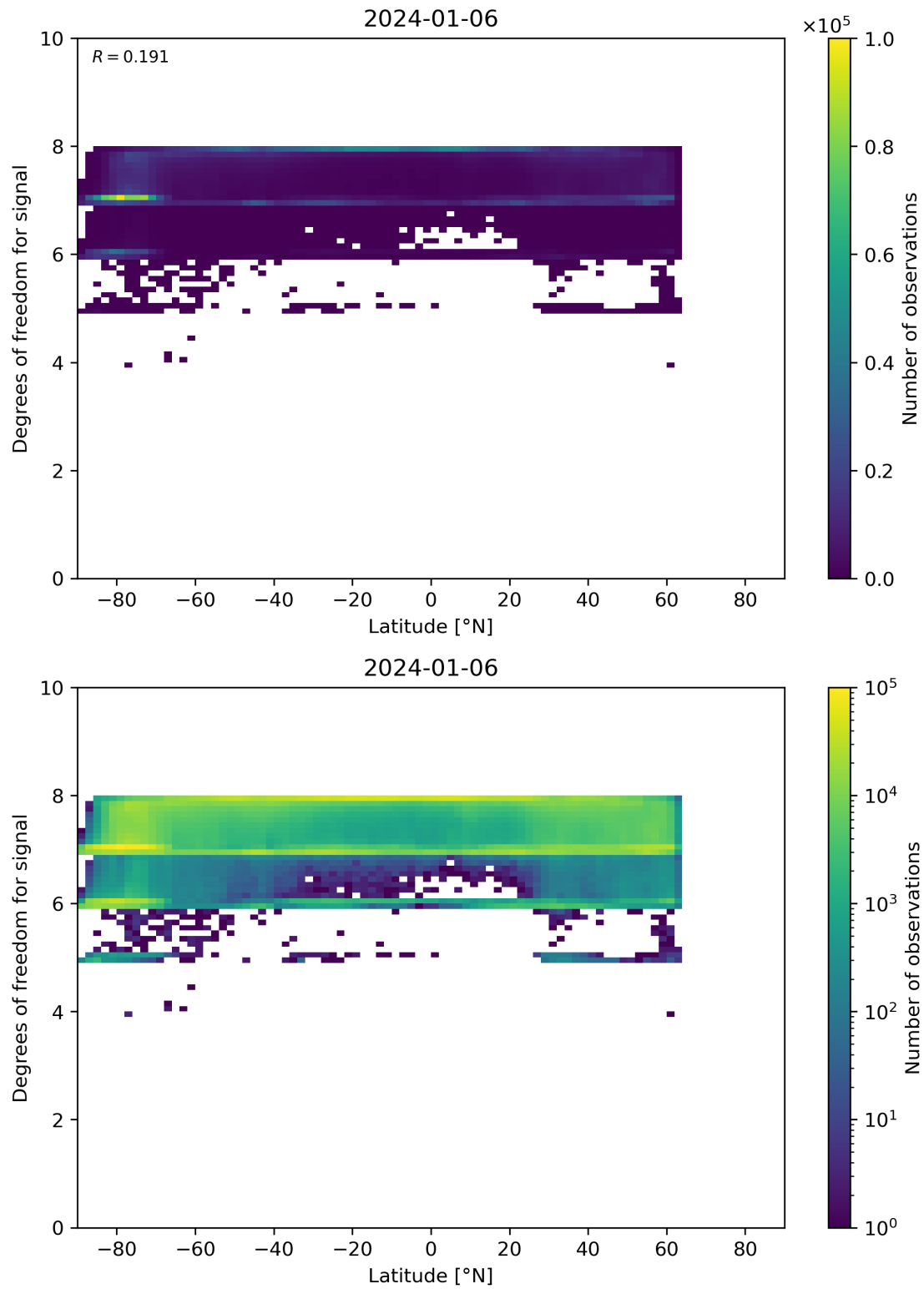
Figure 55: Scatter density plot of “Latitude” against “Degrees of freedom for signal” for 2024-01-05 to 2024-01-07.
