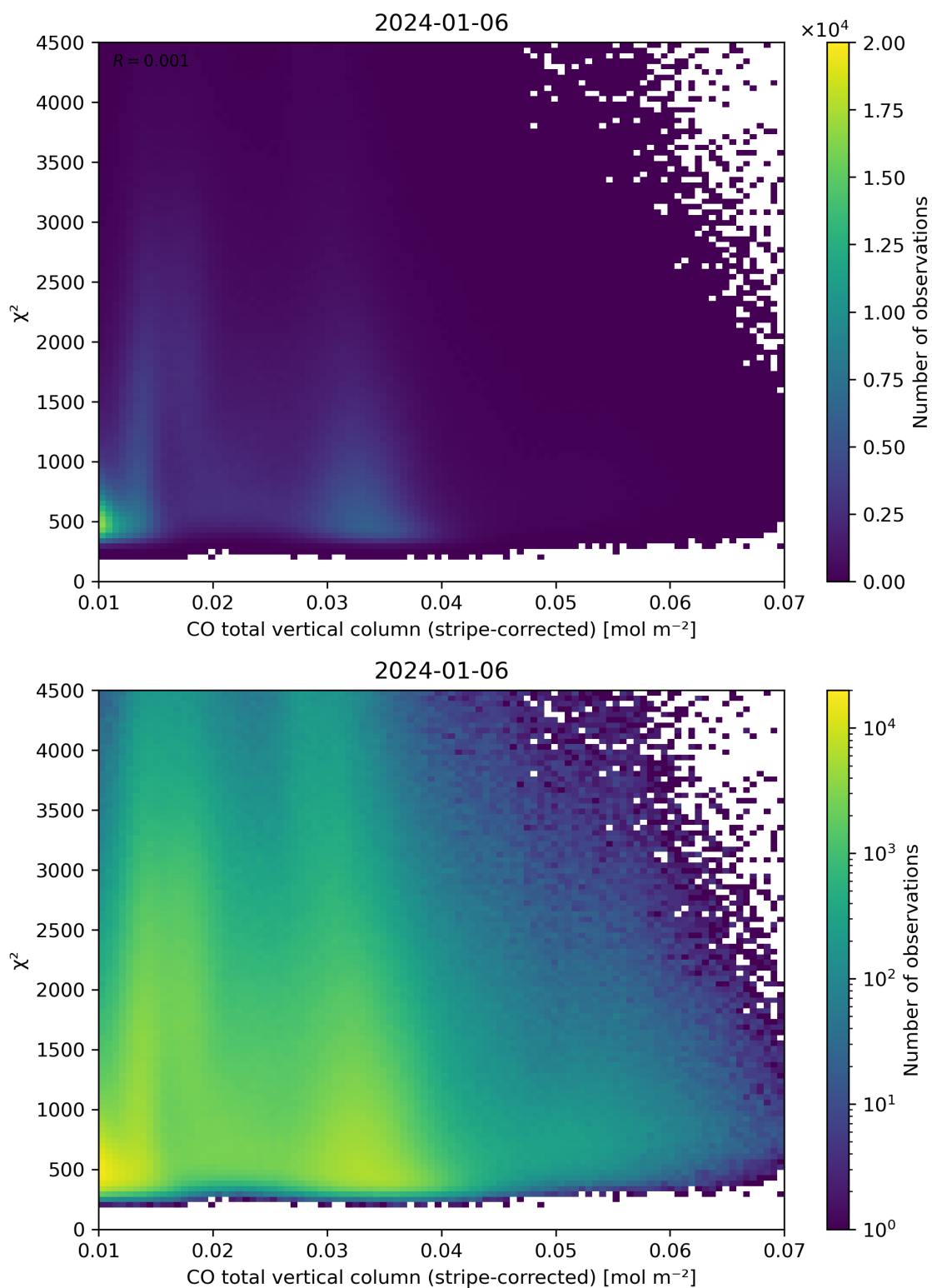
Figure 37: Scatter density plot of “CO total vertical column (stripe-corrected)” against “ \chi^2 ” for 2024-01-05 to 2024-01-07.
