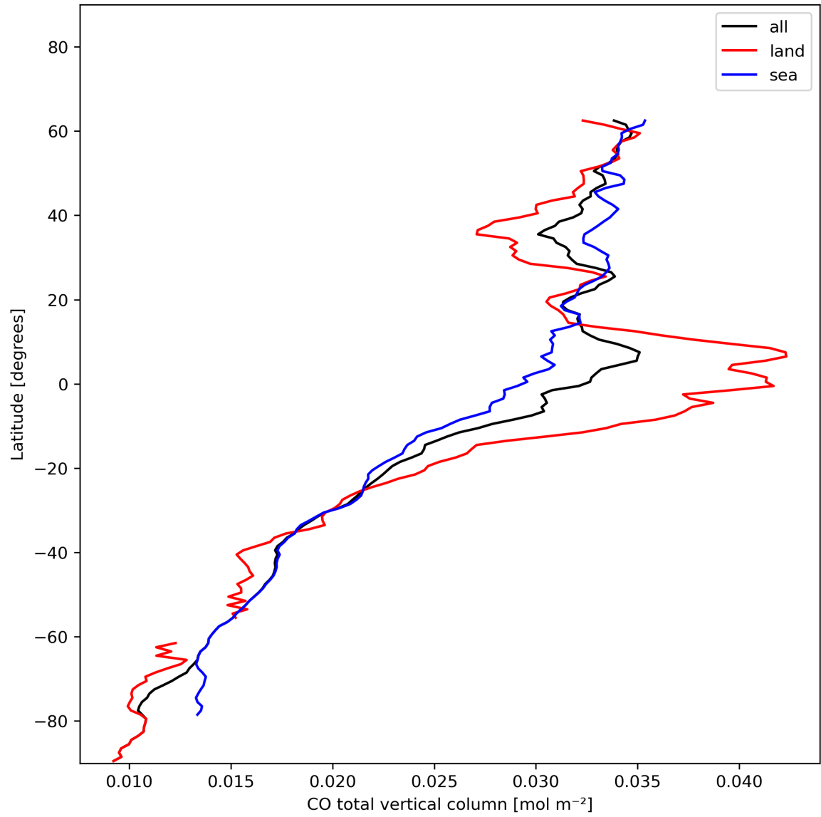
Figure 10: Zonal average of “CO total vertical column” for 2024-01-05 to 2024-01-07.
