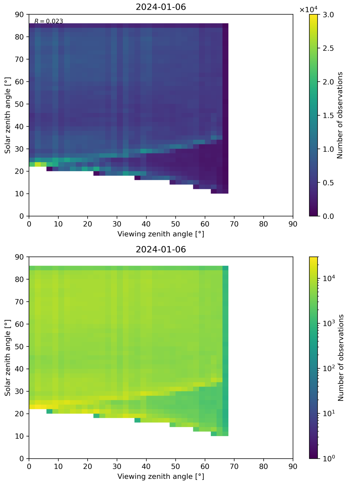
Figure 77: Scatter density plot of “Viewing zenith angle” against “Solar zenith angle” for 2024-01-05 to 2024-01-07.
