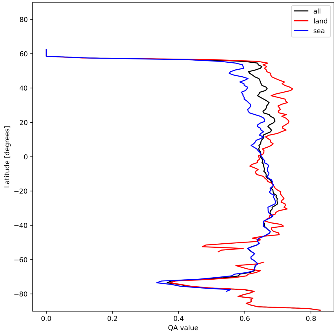
Figure 9: Zonal average of “QA value” for 2024-01-05 to 2024-01-07.
