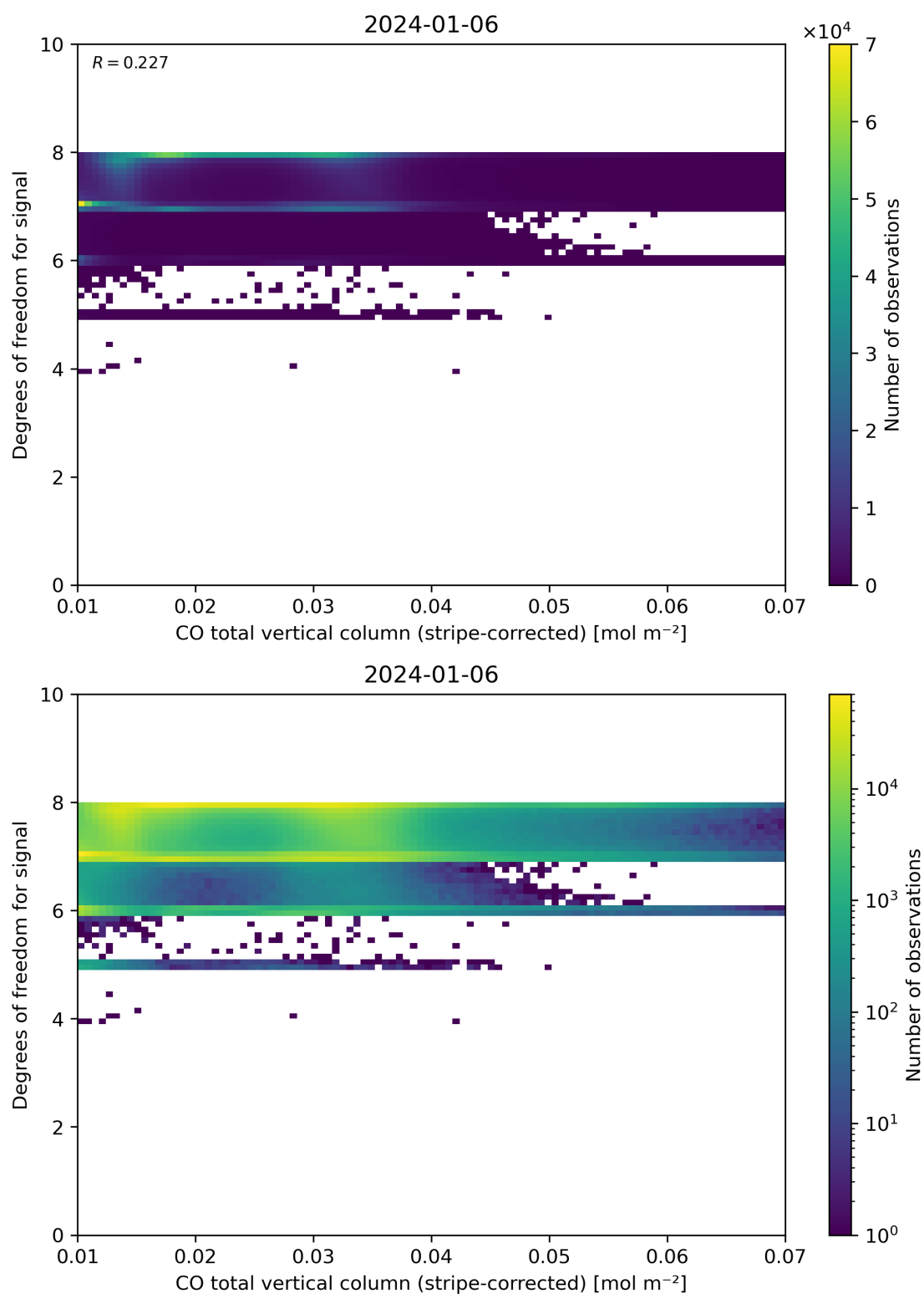
Figure 38: Scatter density plot of “CO total vertical column (stripe-corrected)” against “Degrees of freedom for signal” for 2024-01-05 to 2024-01-07.
