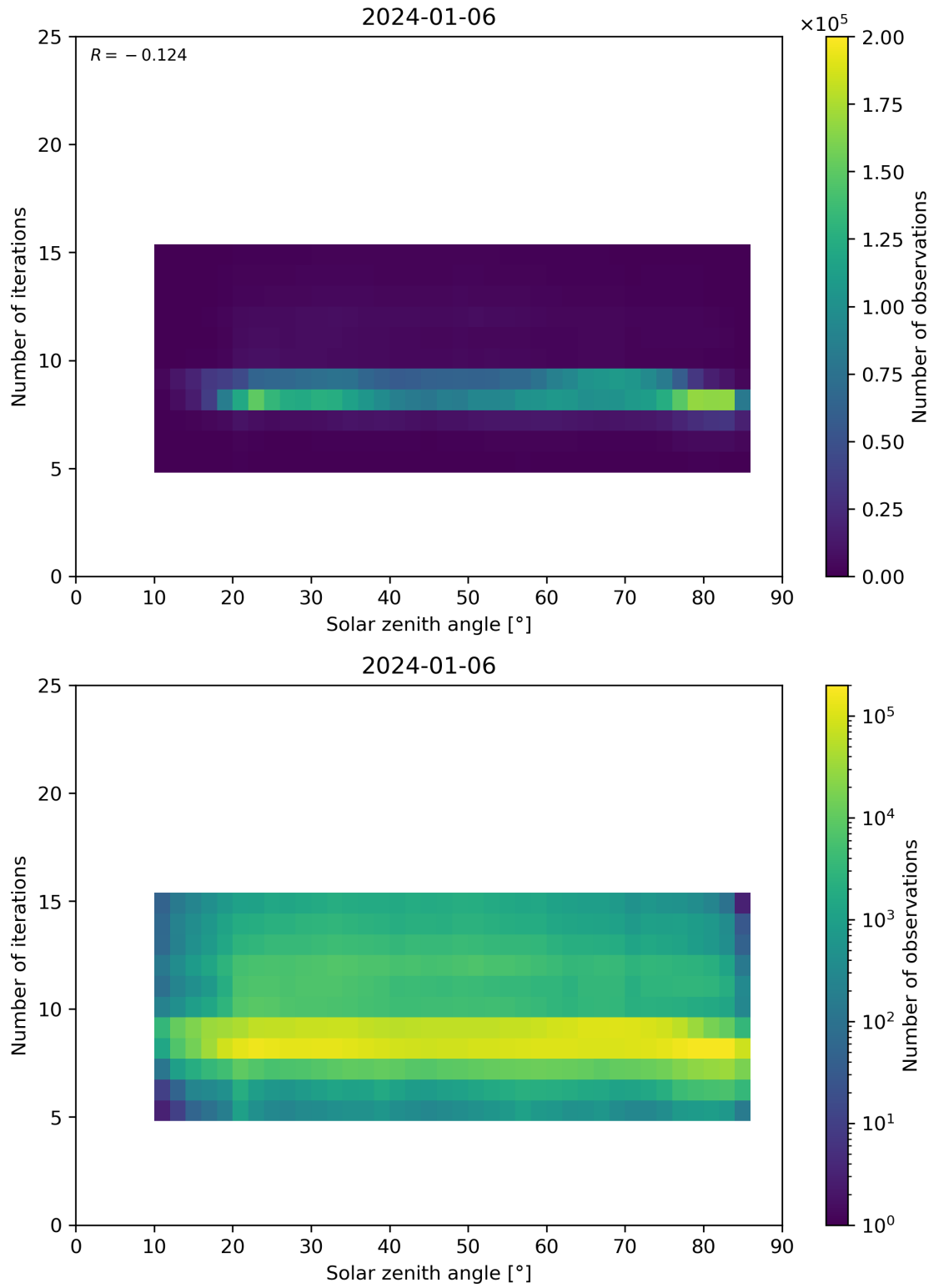
Figure 67: Scatter density plot of “Solar zenith angle” against “Number of iterations” for 2024-01-05 to 2024-01-07.
