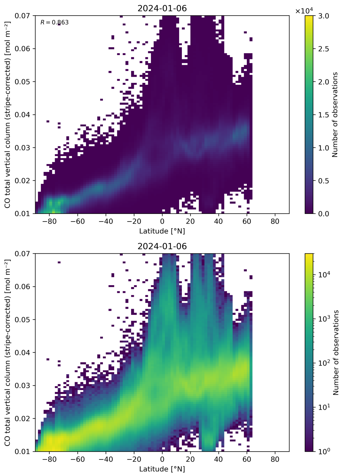
Figure 52: Scatter density plot of “Latitude” against “CO total vertical column (stripe-corrected)” for 2024-01-05 to 2024-01-07.
