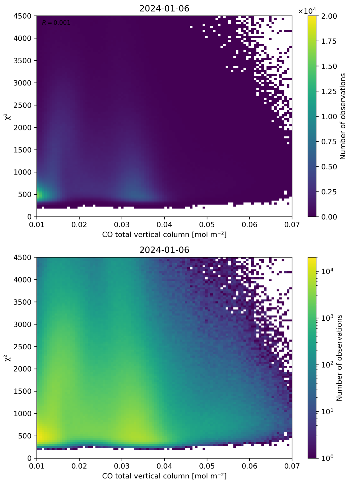
Figure 35: Scatter density plot of “CO total vertical column” against “ \chi^2 ” for 2024-01-05 to 2024-01-07.
