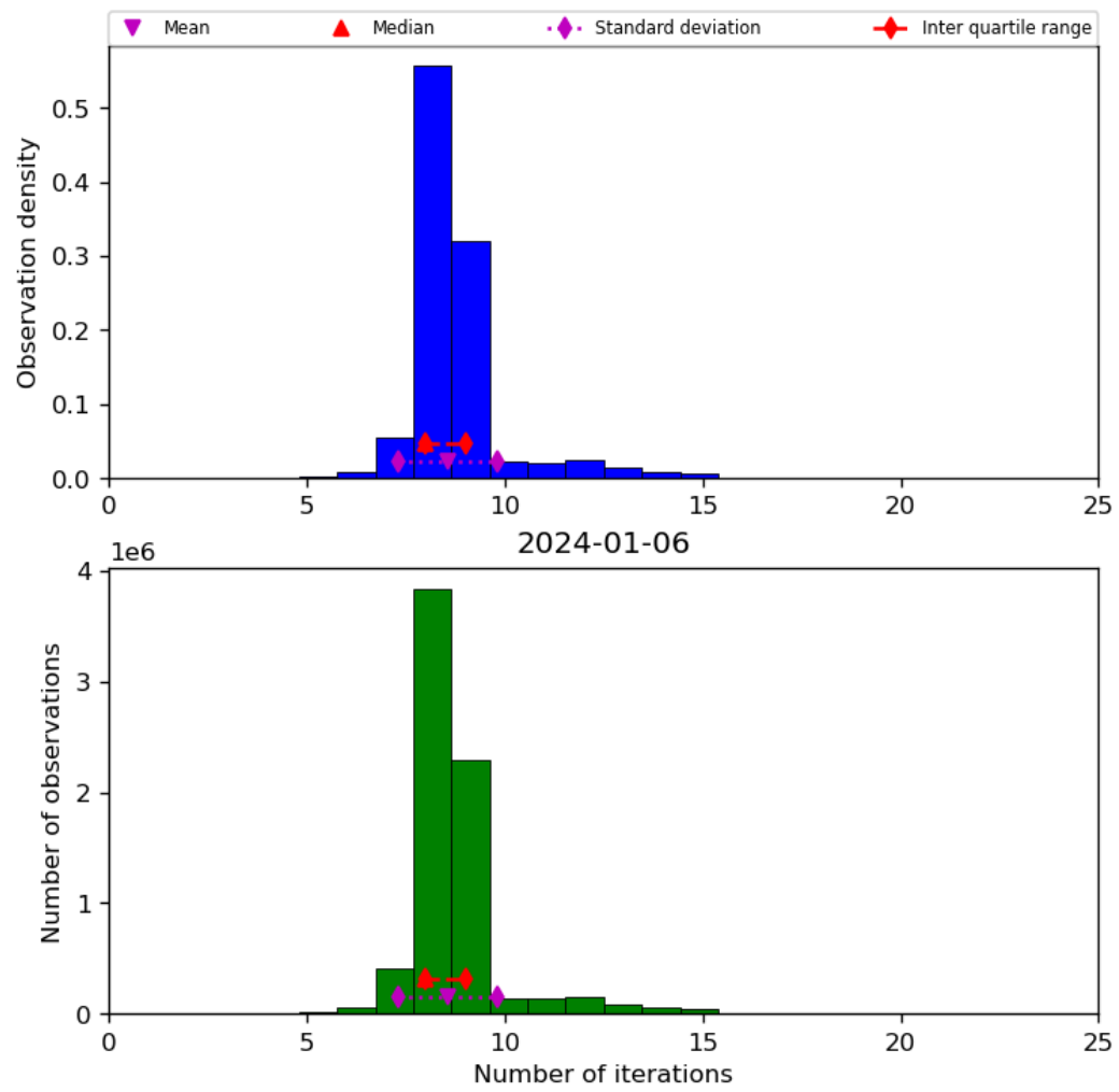
Figure 24: Histogram of “Number of iterations” for 2024-01-05 to 2024-01-07
