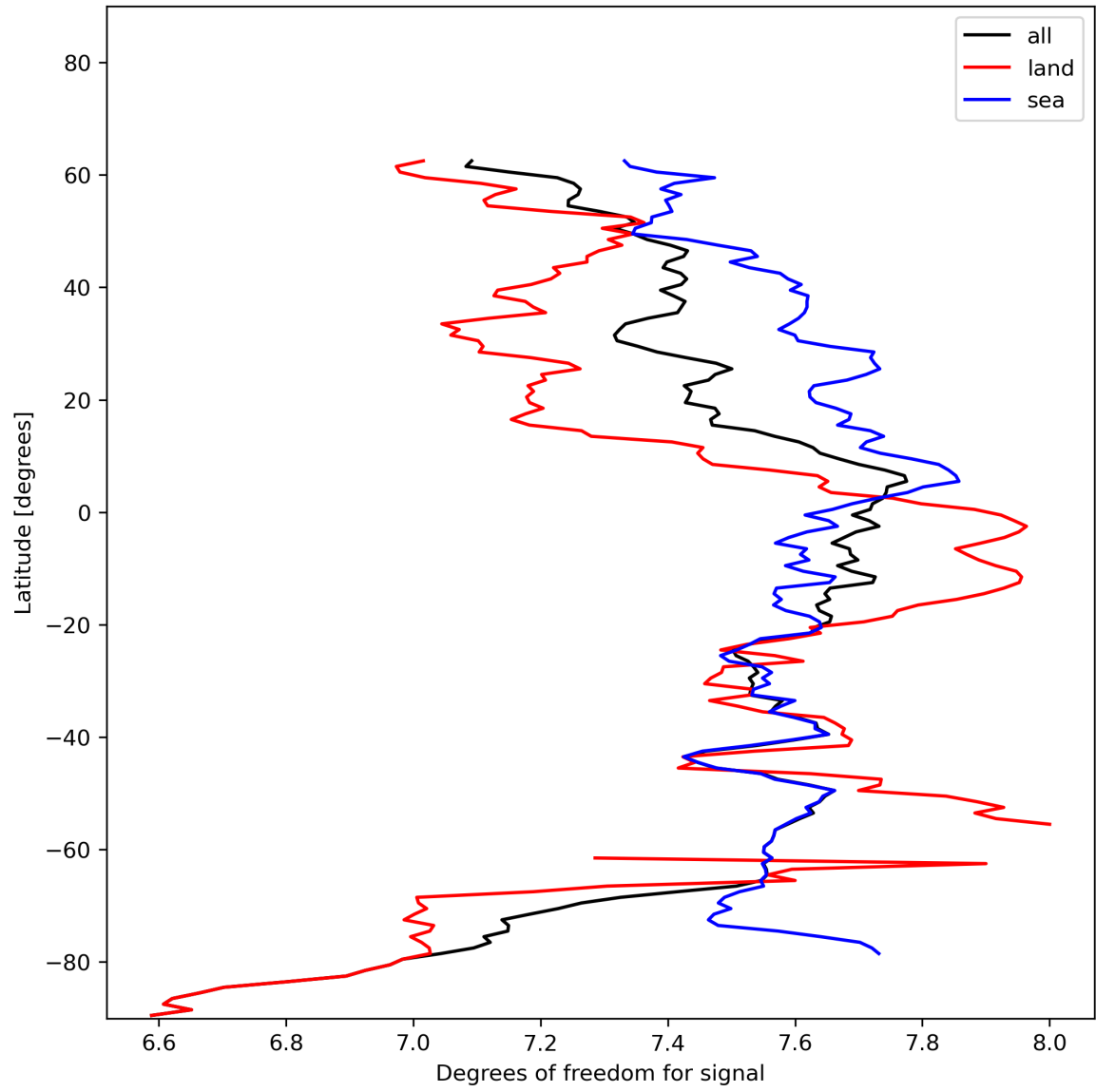
Figure 15: Zonal average of “Degrees of freedom for signal” for 2024-01-05 to 2024-01-07.
