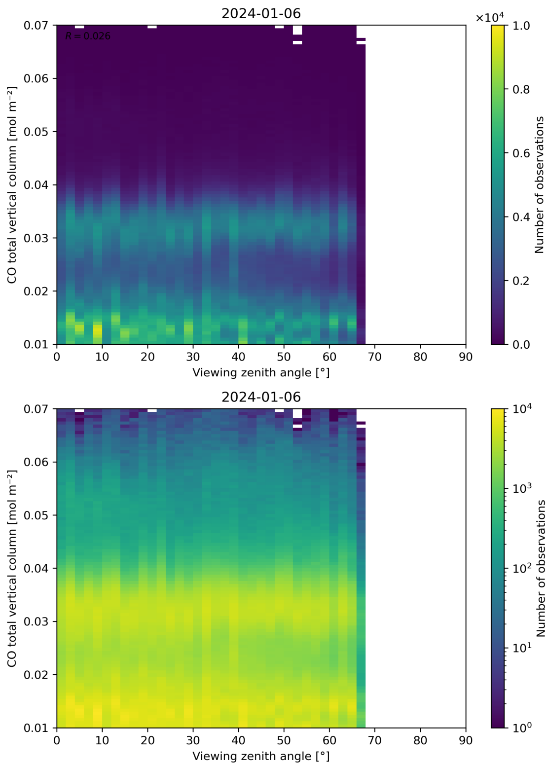
Figure 69: Scatter density plot of “Viewing zenith angle” against “CO total vertical column” for 2024-01-05 to 2024-01-07.
