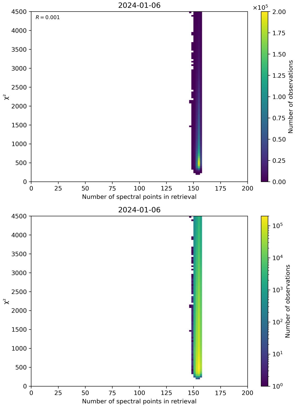
Figure 58: Scatter density plot of “Number of spectral points in retrieval” against “ \chi^2 ” for 2024-01-05 to 2024-01-07.
