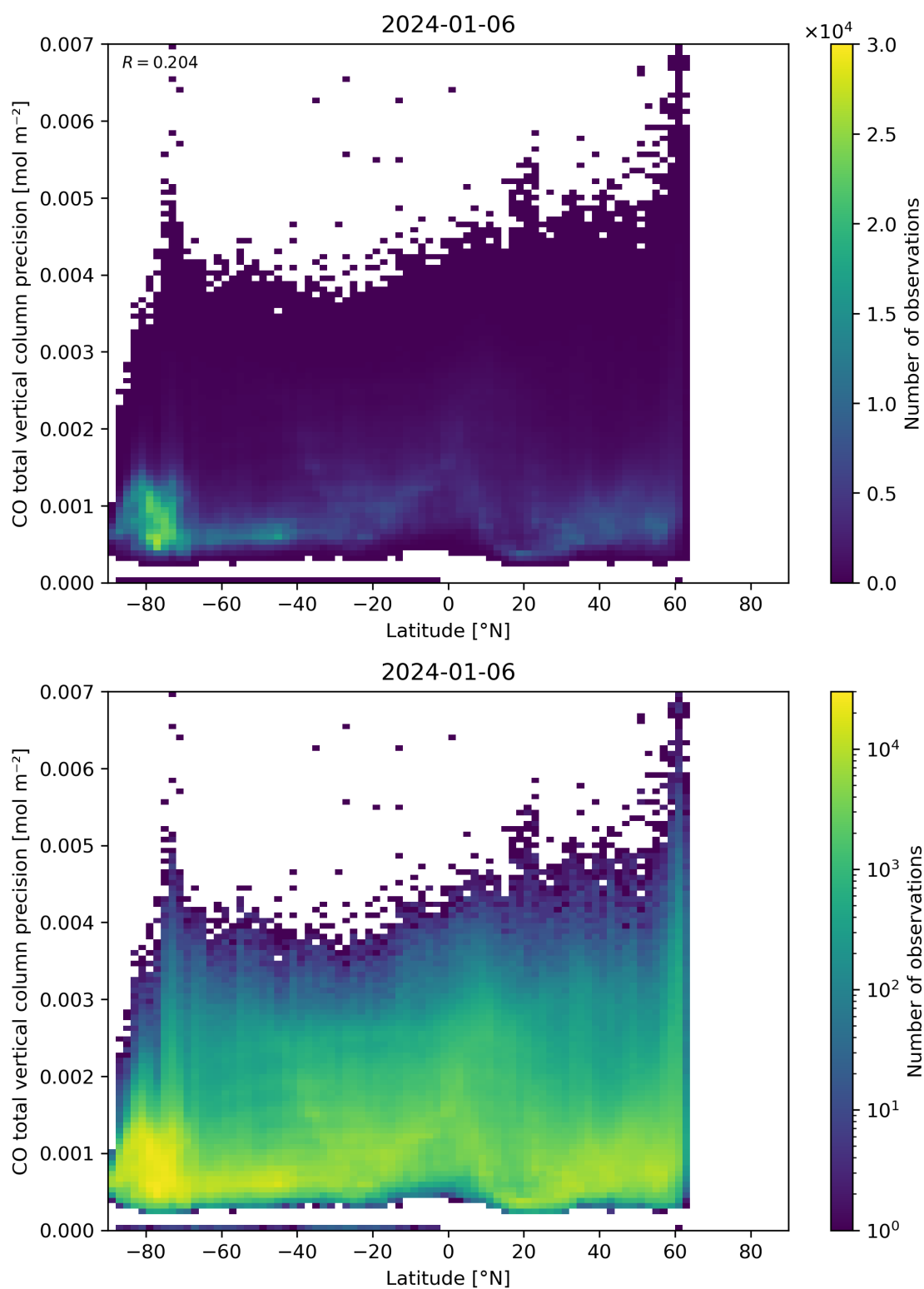
Figure 53: Scatter density plot of “Latitude” against “CO total vertical column precision” for 2024-01-05 to 2024-01-07.
