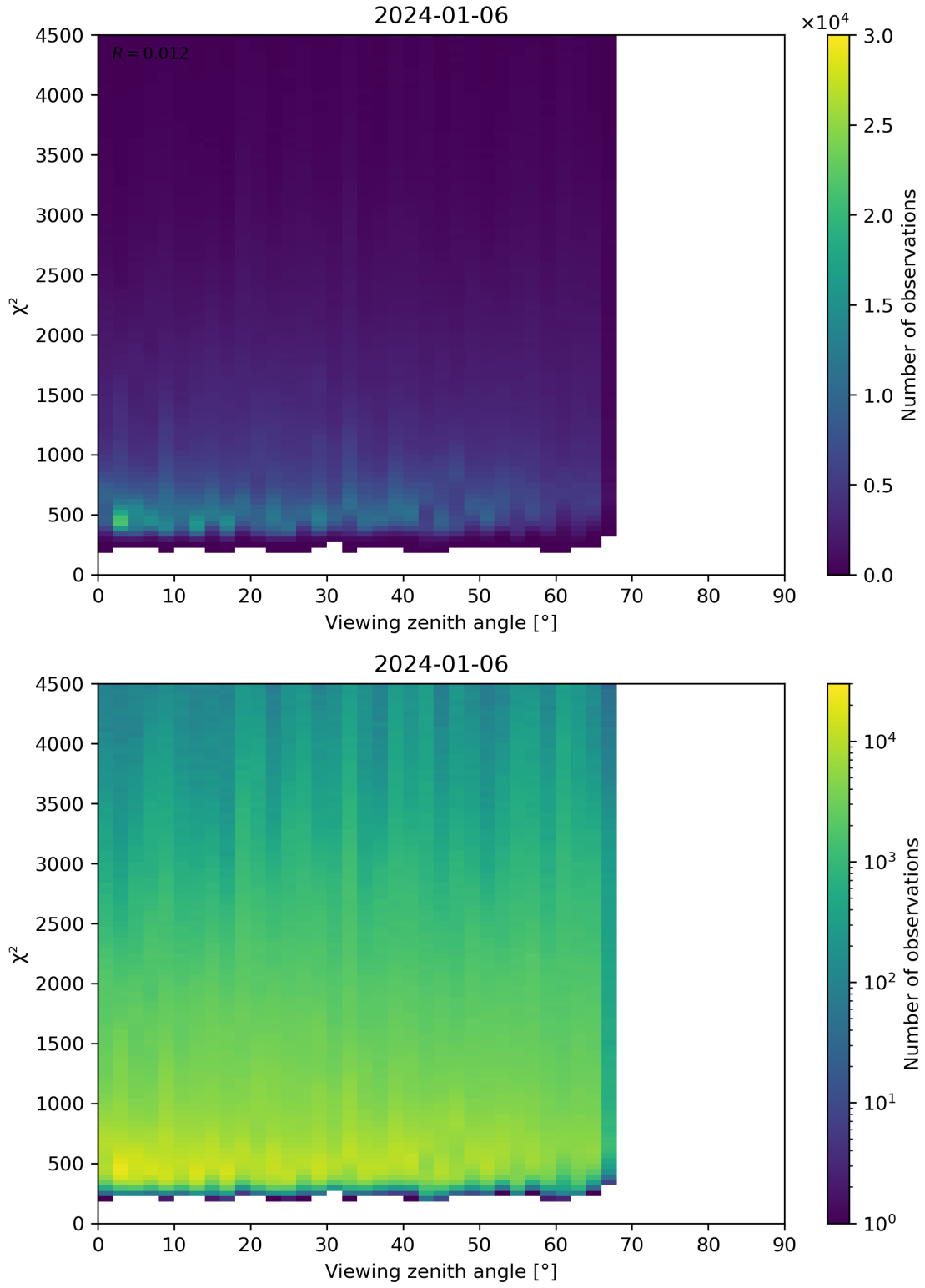
Figure 72: Scatter density plot of “Viewing zenith angle” against “ \chi^2 ” for 2024-01-05 to 2024-01-07.
