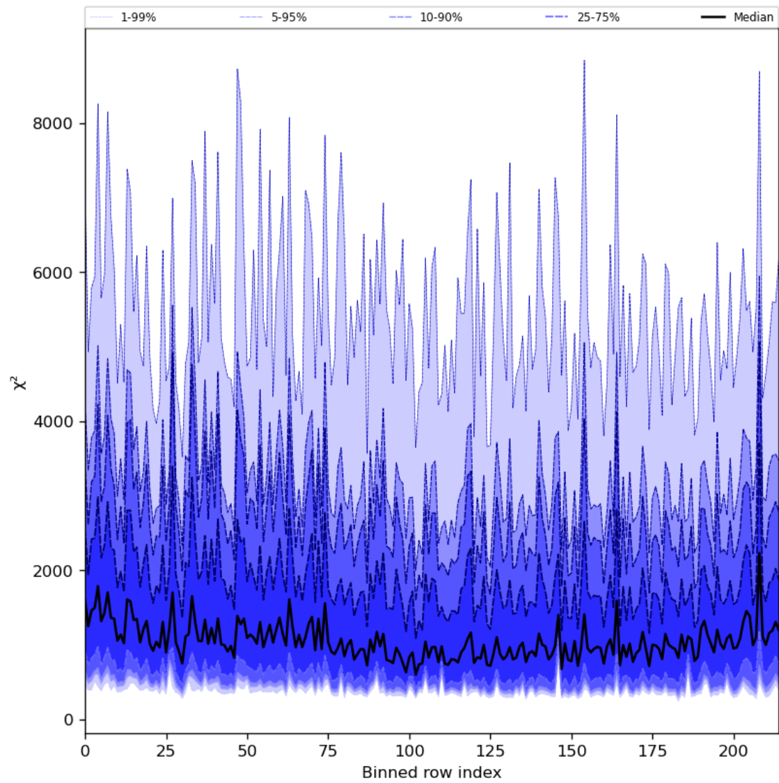
Figure 30: Along track statistics of “ \chi^2 ” for 2024-01-05 to 2024-01-07
