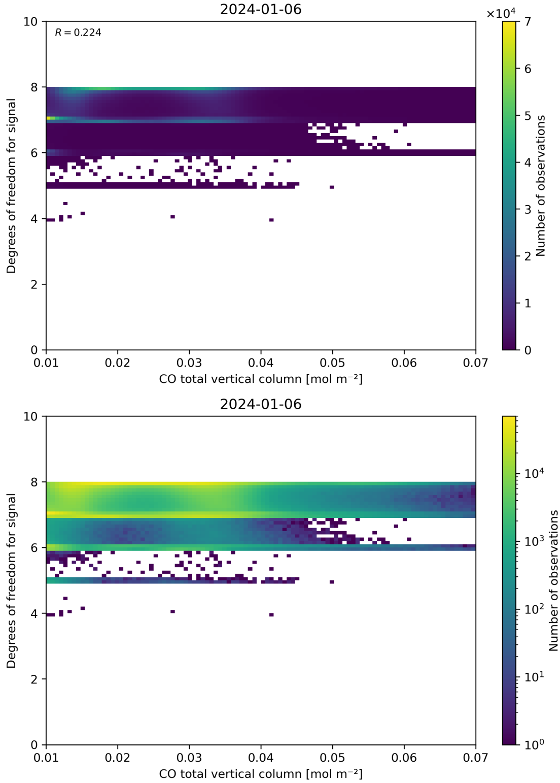
Figure 41: Scatter density plot of “CO total vertical column” against “Degrees of freedom for signal” for 2024-01-05 to 2024-01-07.
