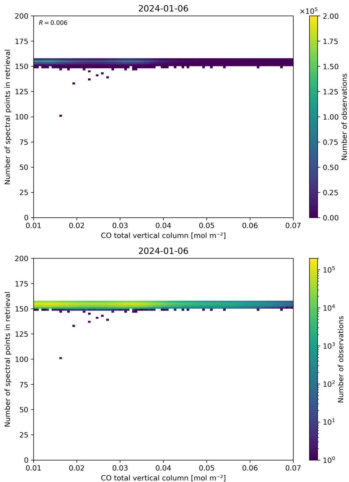
Figure 43: Scatter density plot of “CO total vertical column” against “Number of spectral points in retrieval” for 2024-01-05 to 2024-01-07.
