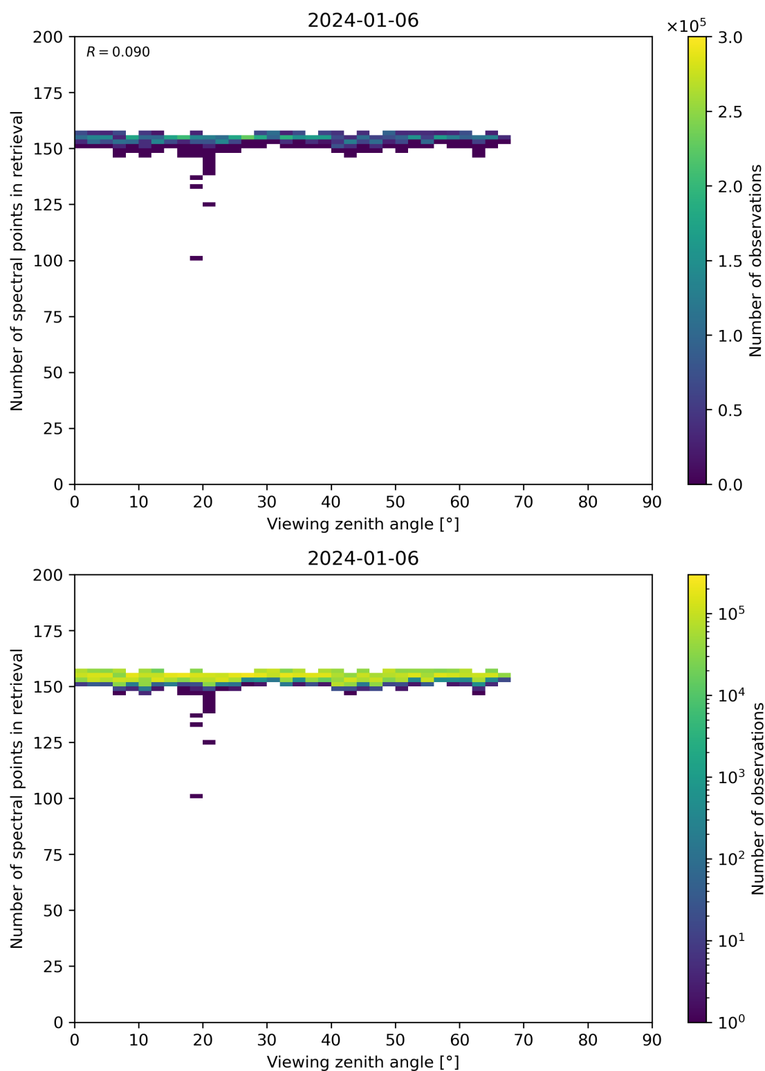
Figure 76: Scatter density plot of “Viewing zenith angle” against “Number of spectral points in retrieval” for 2024-01-05 to 2024-01-07.
