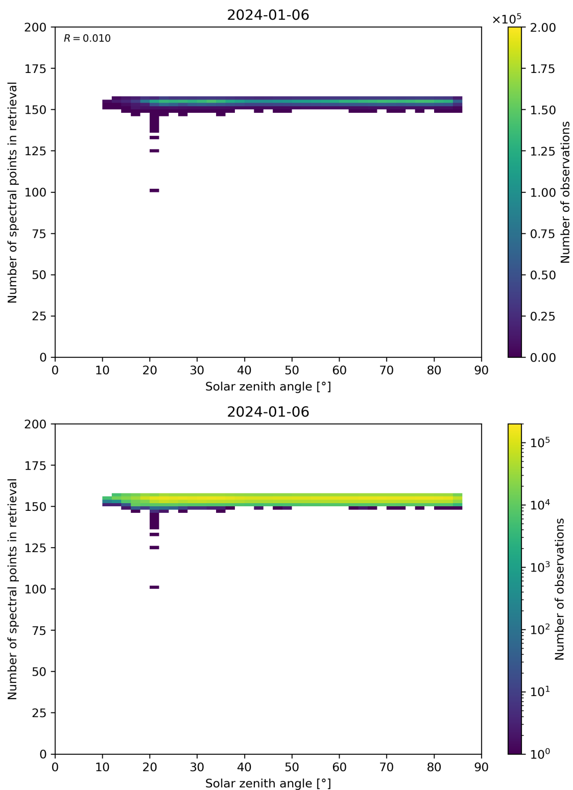
Figure 68: Scatter density plot of “Solar zenith angle” against “Number of spectral points in retrieval” for 2024-01-05 to 2024-01-07.
