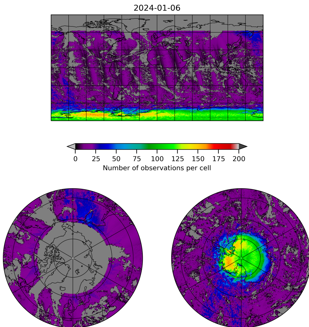
Figure 8: Map of the number of observations for 2024-01-05 to 2024-01-07
