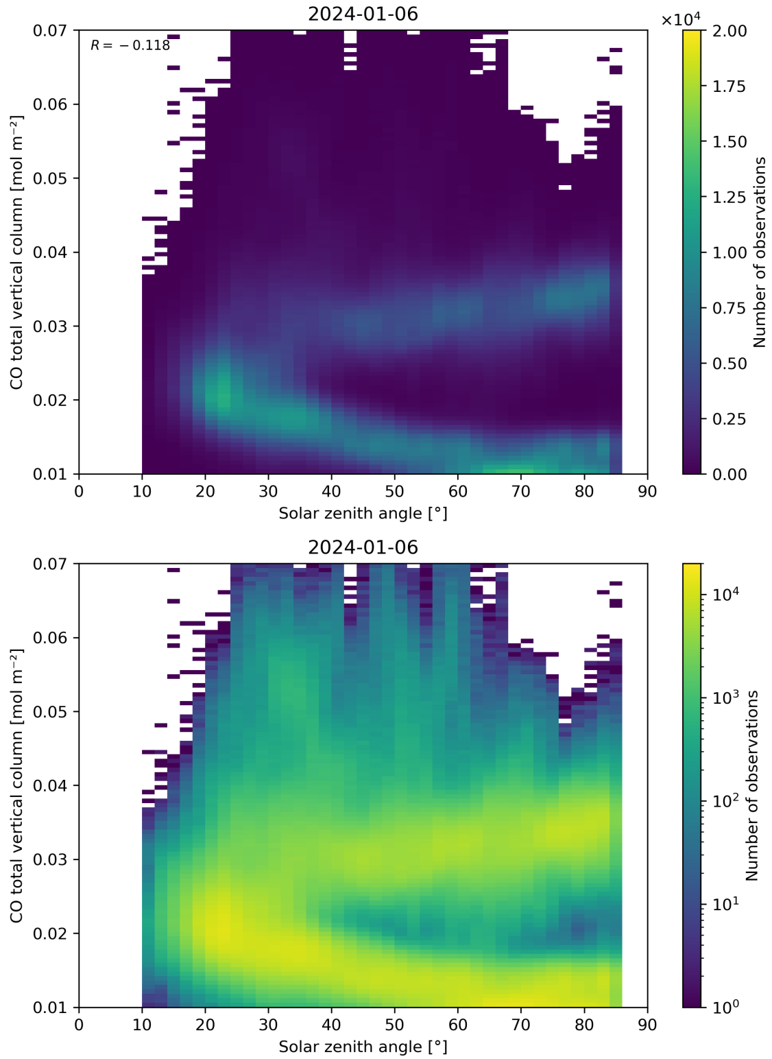
Figure 61: Scatter density plot of “Solar zenith angle” against “CO total vertical column” for 2024-01-05 to 2024-01-07.
