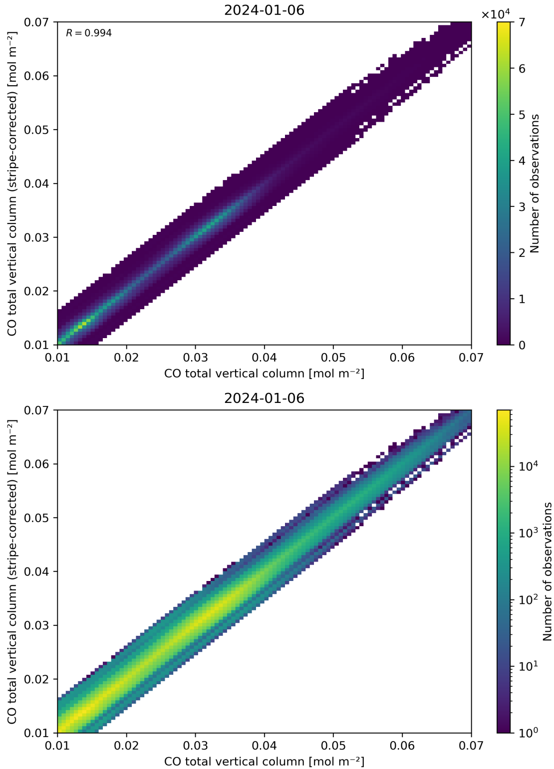
Figure 33: Scatter density plot of “CO total vertical column” against “CO total vertical column (stripe-corrected)” for 2024-01-05 to 2024-01-07.
