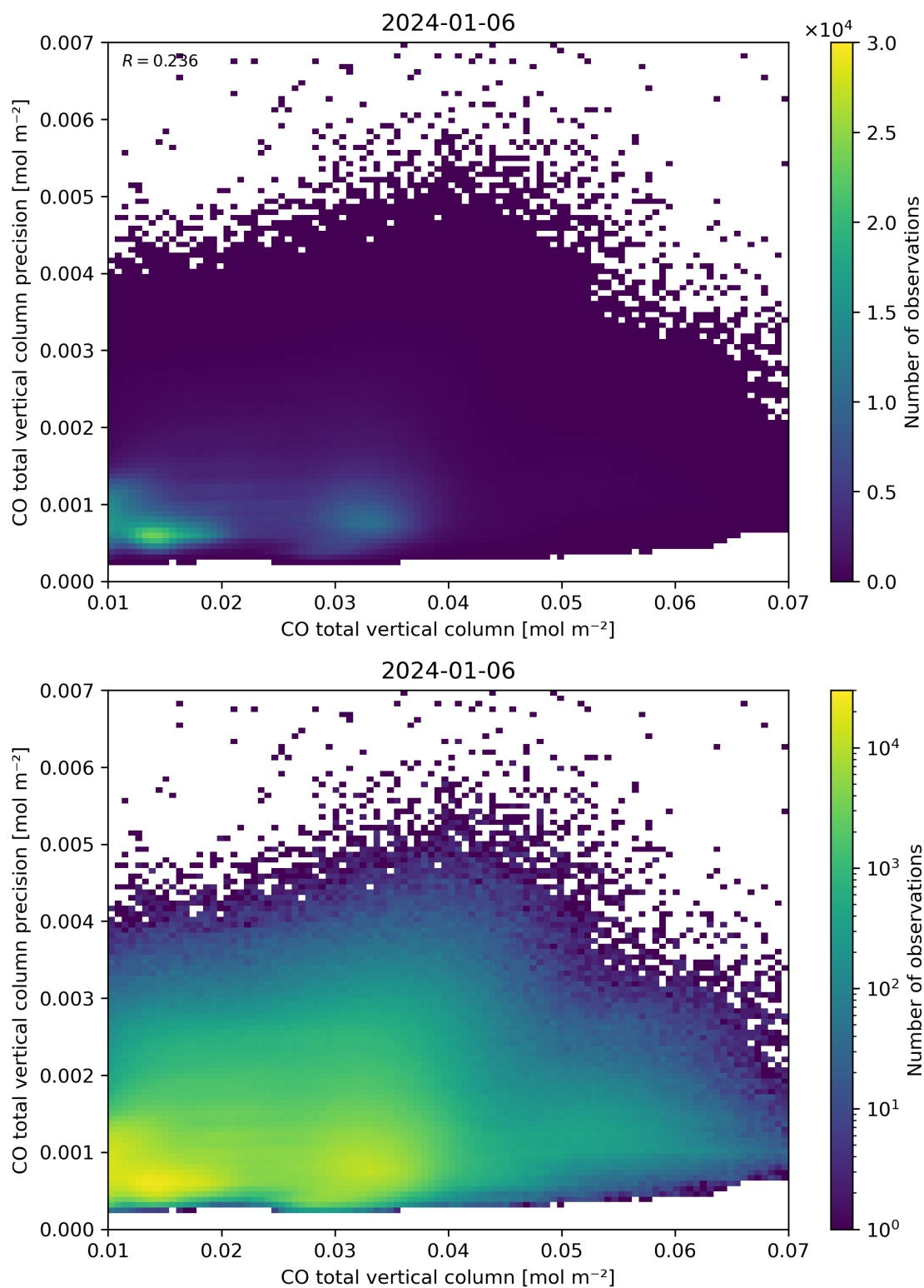
Figure 34: Scatter density plot of “CO total vertical column” against “CO total vertical column precision” for 2024-01-05 to 2024-01-07.
