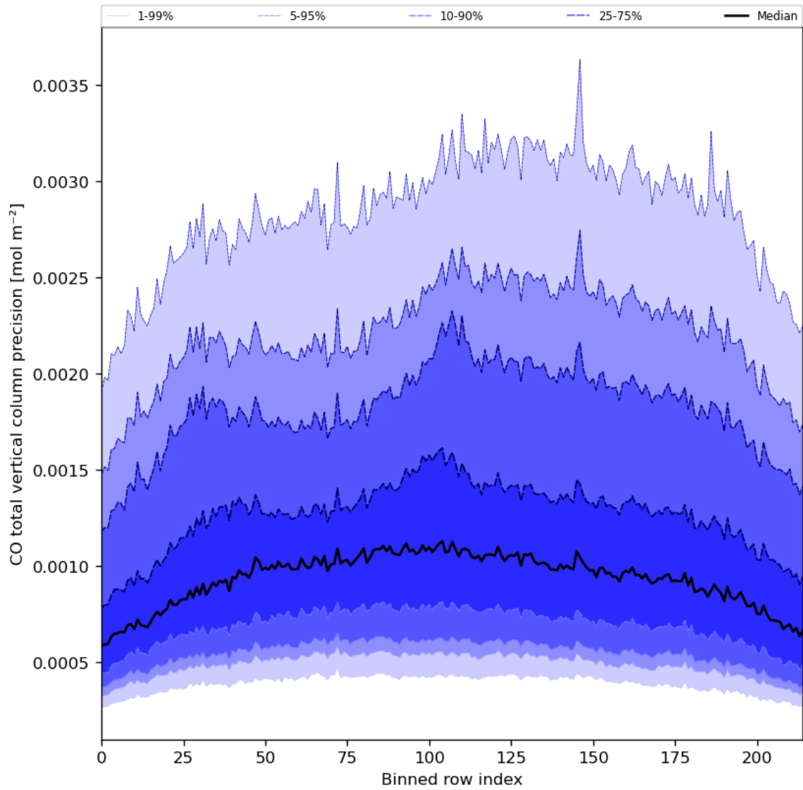
Figure 28: Along track statistics of “CO total vertical column precision” for 2024-01-05 to 2024-01-07
