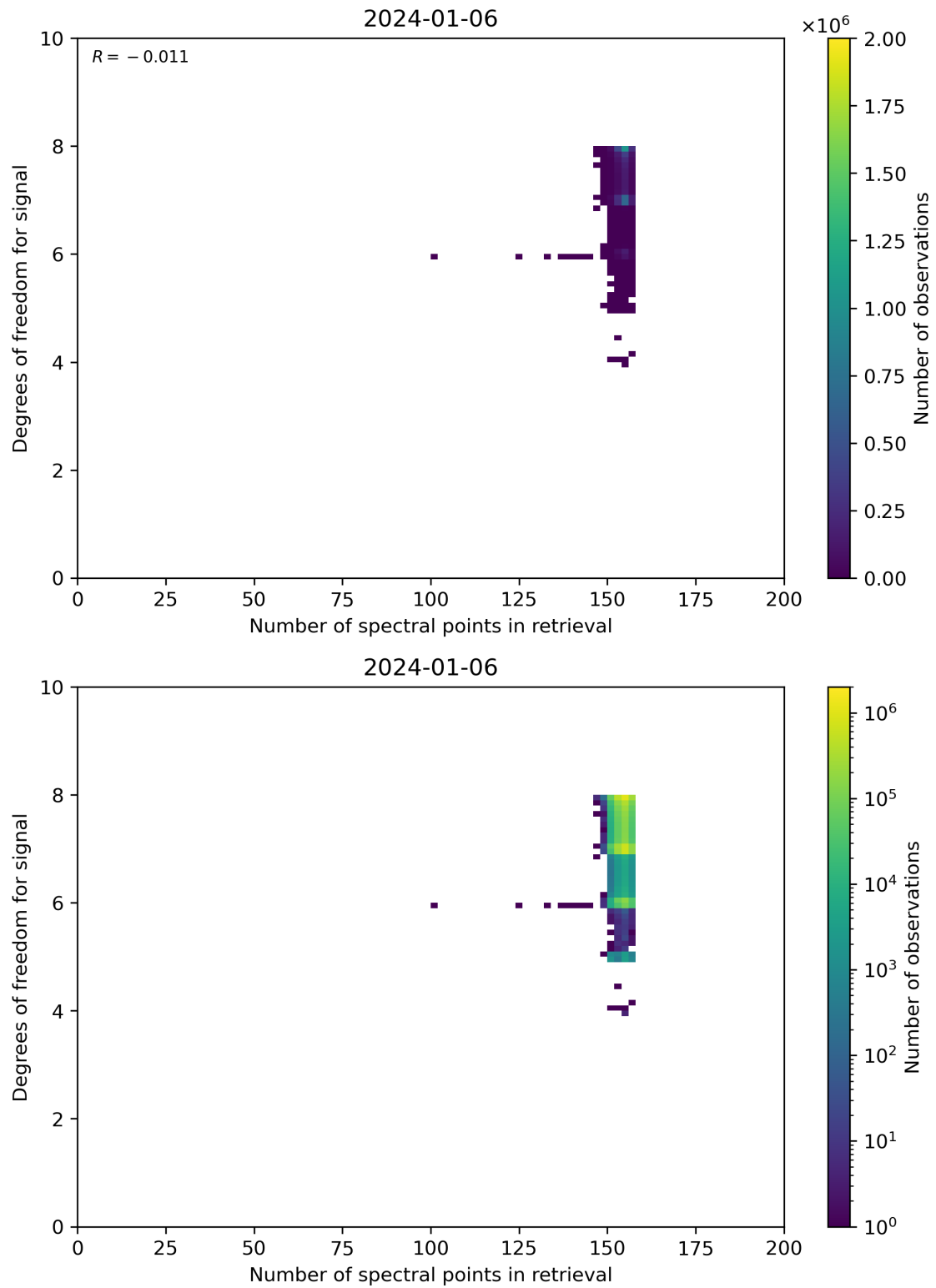
Figure 59: Scatter density plot of “Number of spectral points in retrieval” against “Degrees of freedom for signal” for 2024-01-05 to 2024-01-07.
