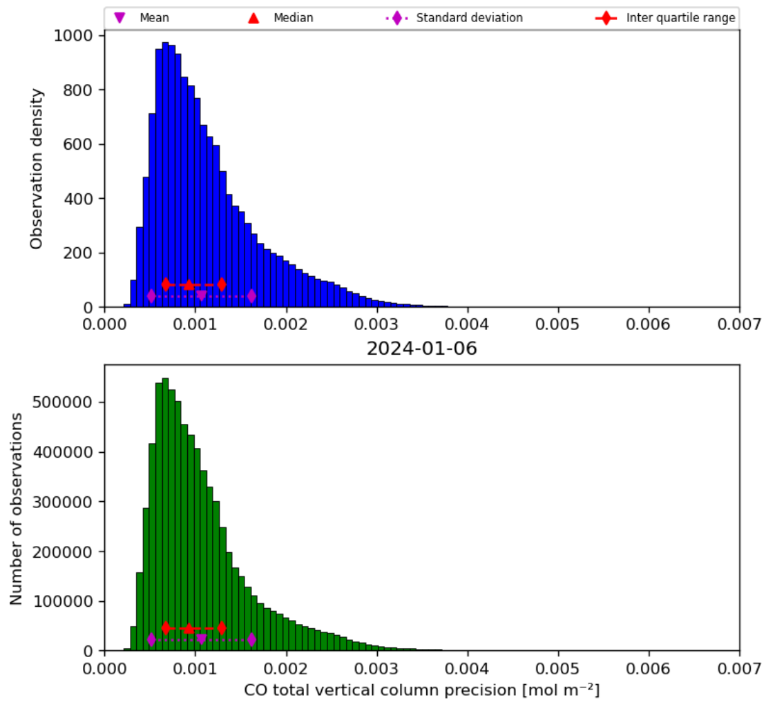
Figure 20: Histogram of “CO total vertical column precision” for 2024-01-05 to 2024-01-07
