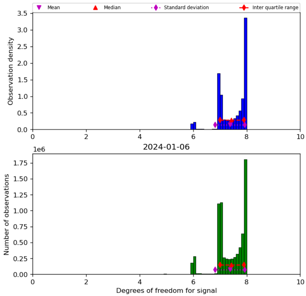
Figure 23: Histogram of “Degrees of freedom for signal” for 2024-01-05 to 2024-01-07
