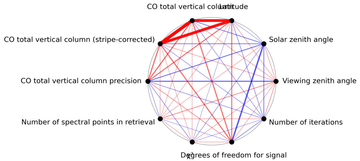
Figure 1: Map of correlation graph for 2024-01-05 to 2024-01-07.
