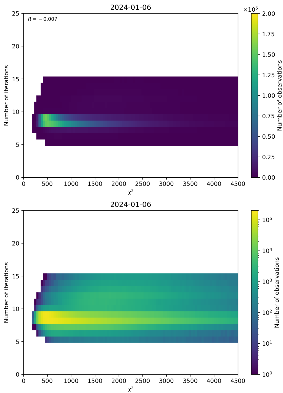
Figure 49: Scatter density plot of “ \chi^2 ” against “Number of iterations” for 2024-01-05 to 2024-01-07.
