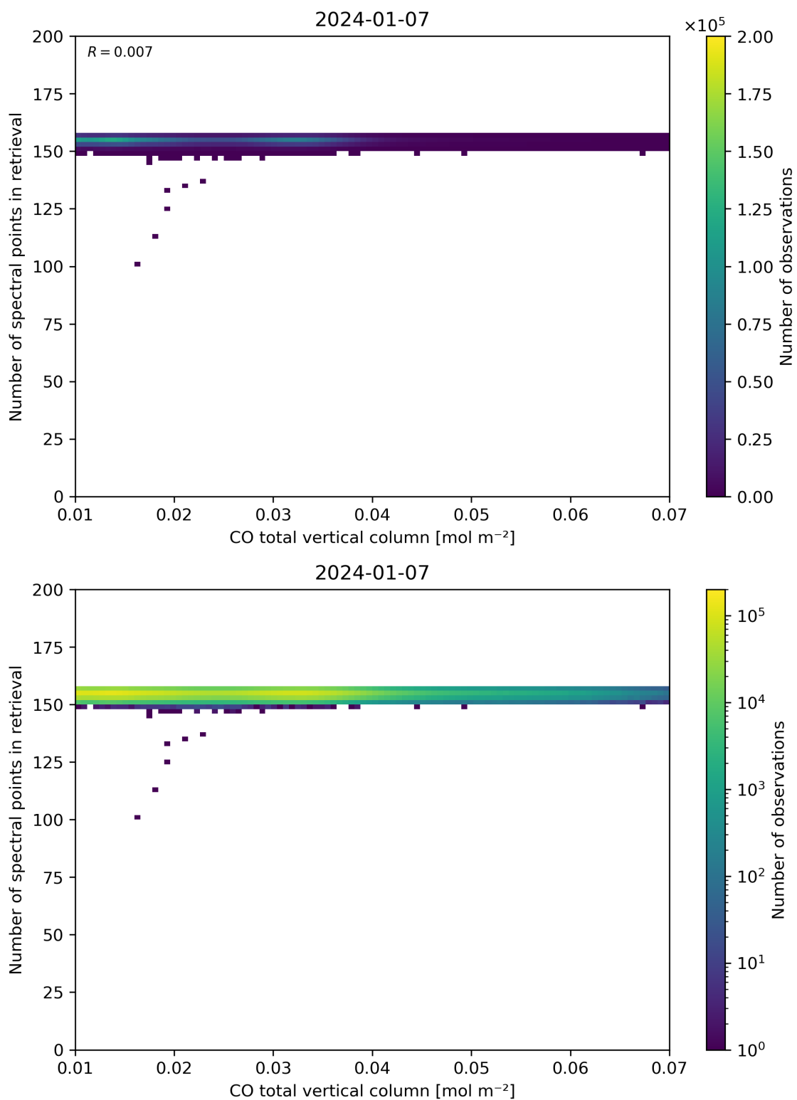
Figure 43: Scatter density plot of “CO total vertical column” against “Number of spectral points in retrieval” for 2024-01-06 to 2024-01-08.
