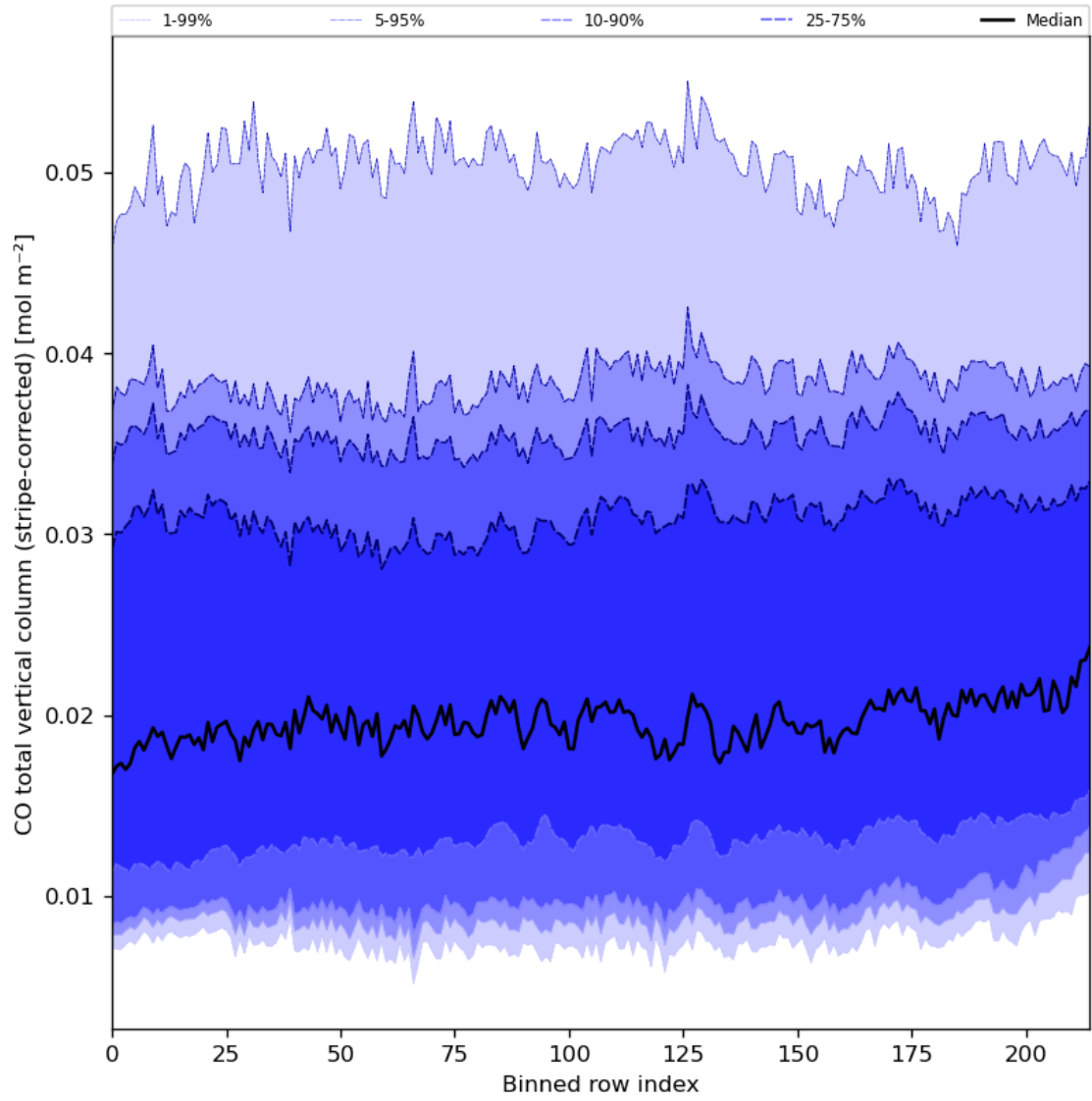
Figure 27: Along track statistics of “CO total vertical column (stripe-corrected)” for 2024-01-06 to 2024-01-08
