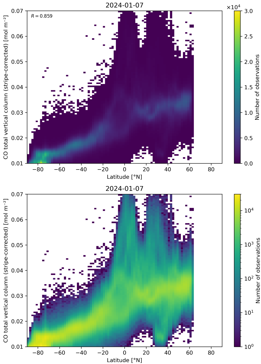
Figure 52: Scatter density plot of “Latitude” against “CO total vertical column (stripe-corrected)” for 2024-01-06 to 2024-01-08.
