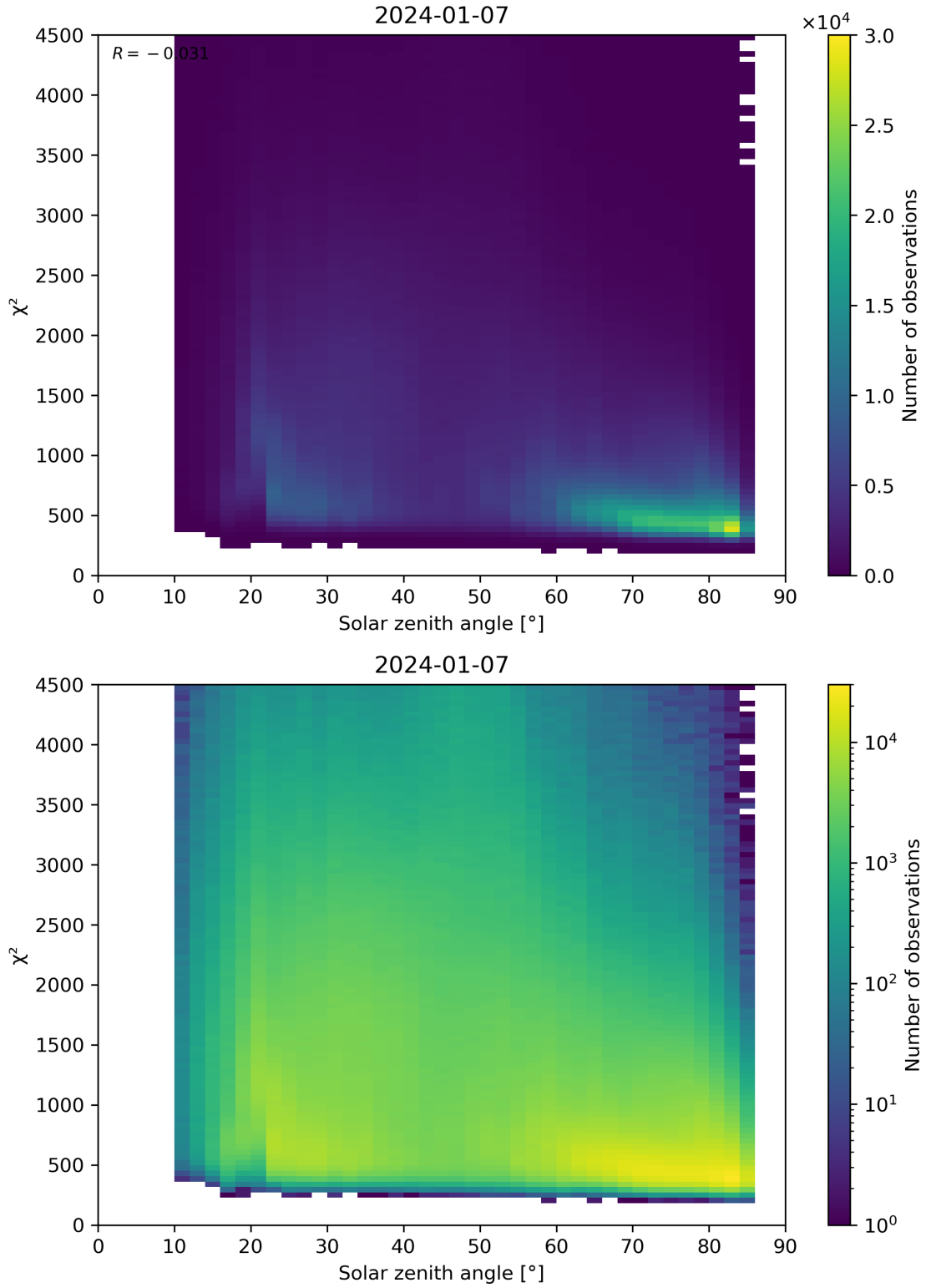
Figure 64: Scatter density plot of “Solar zenith angle” against “ \chi^2 ” for 2024-01-06 to 2024-01-08.
