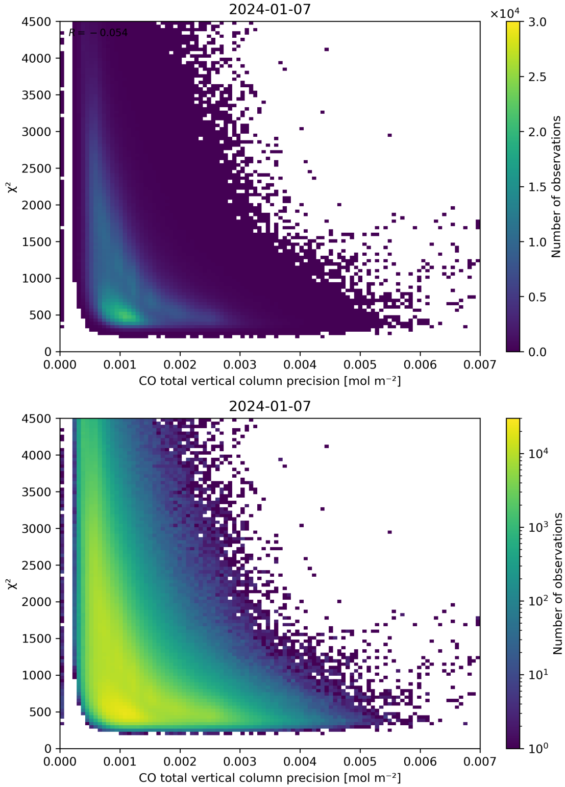
Figure 44: Scatter density plot of “CO total vertical column precision” against “ \chi^2 ” for 2024-01-06 to 2024-01-08.
