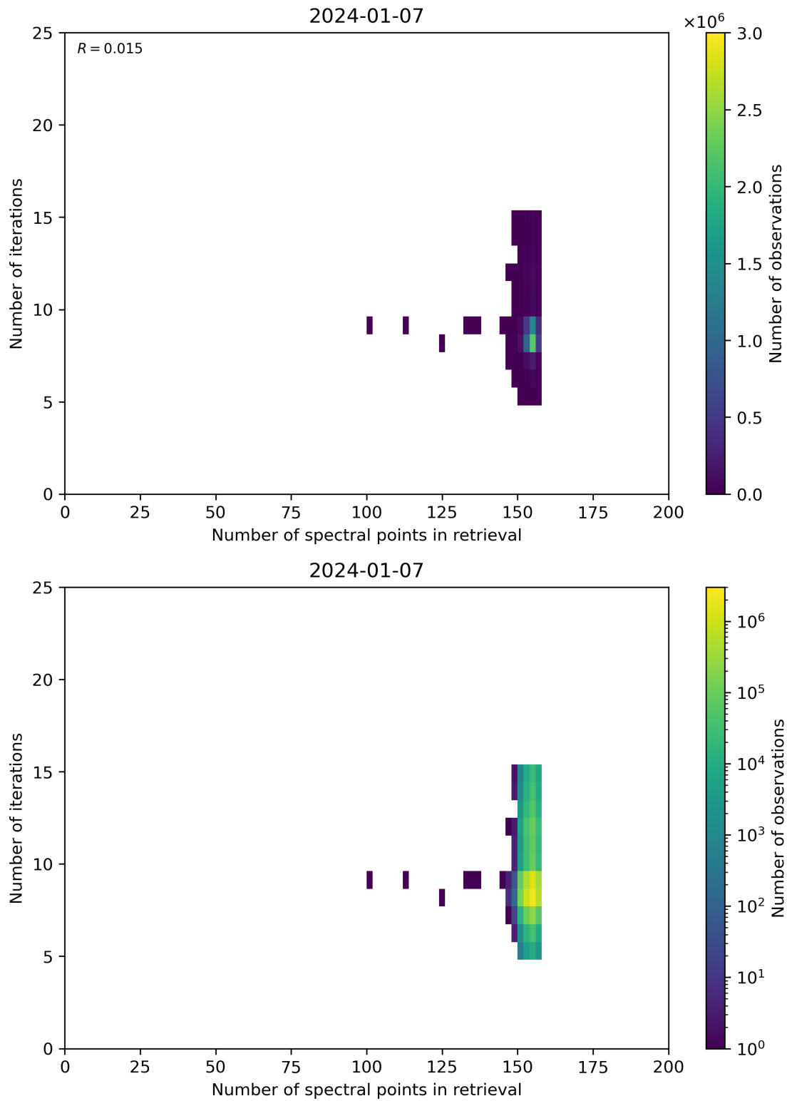
Figure 60: Scatter density plot of “Number of spectral points in retrieval” against “Number of iterations” for 2024-01-06 to 2024-01-08.
