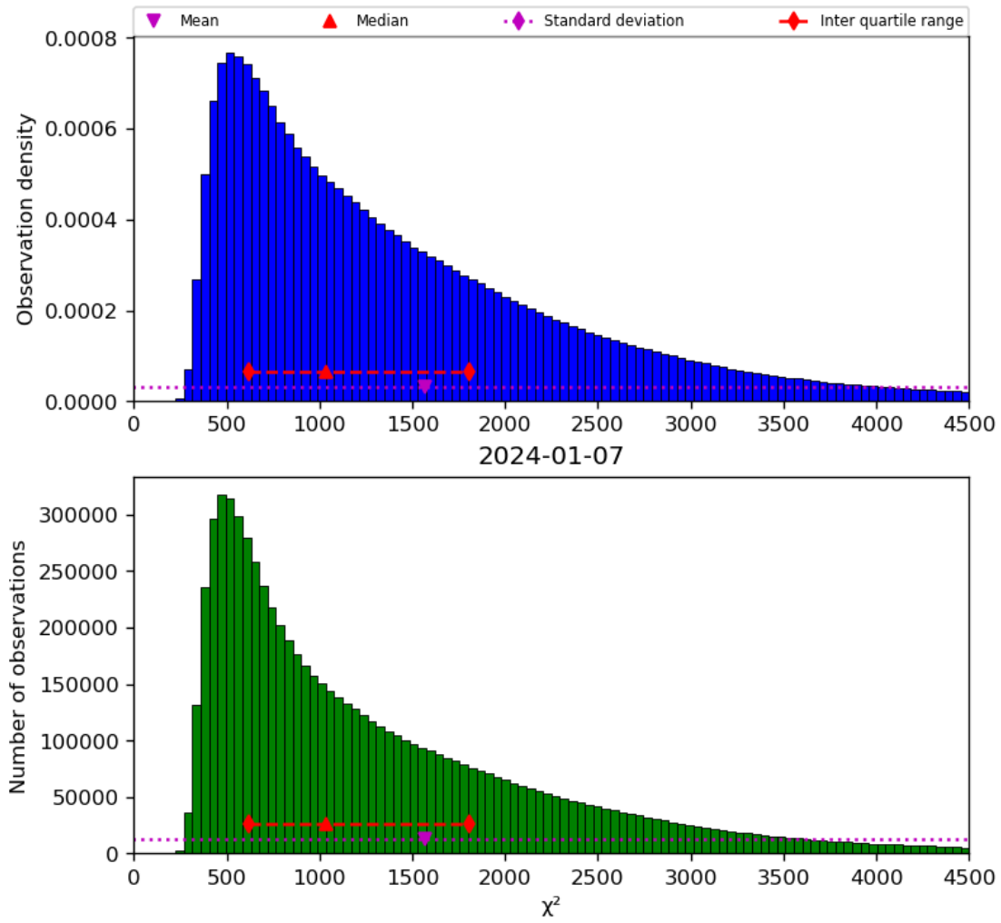
Figure 22: Histogram of “ \chi^2 ” for 2024-01-06 to 2024-01-08
