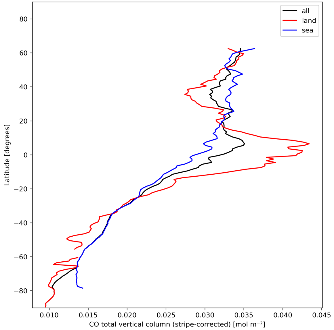
Figure 11: Zonal average of “CO total vertical column (stripe-corrected)” for 2024-01-06 to 2024-01-08.
