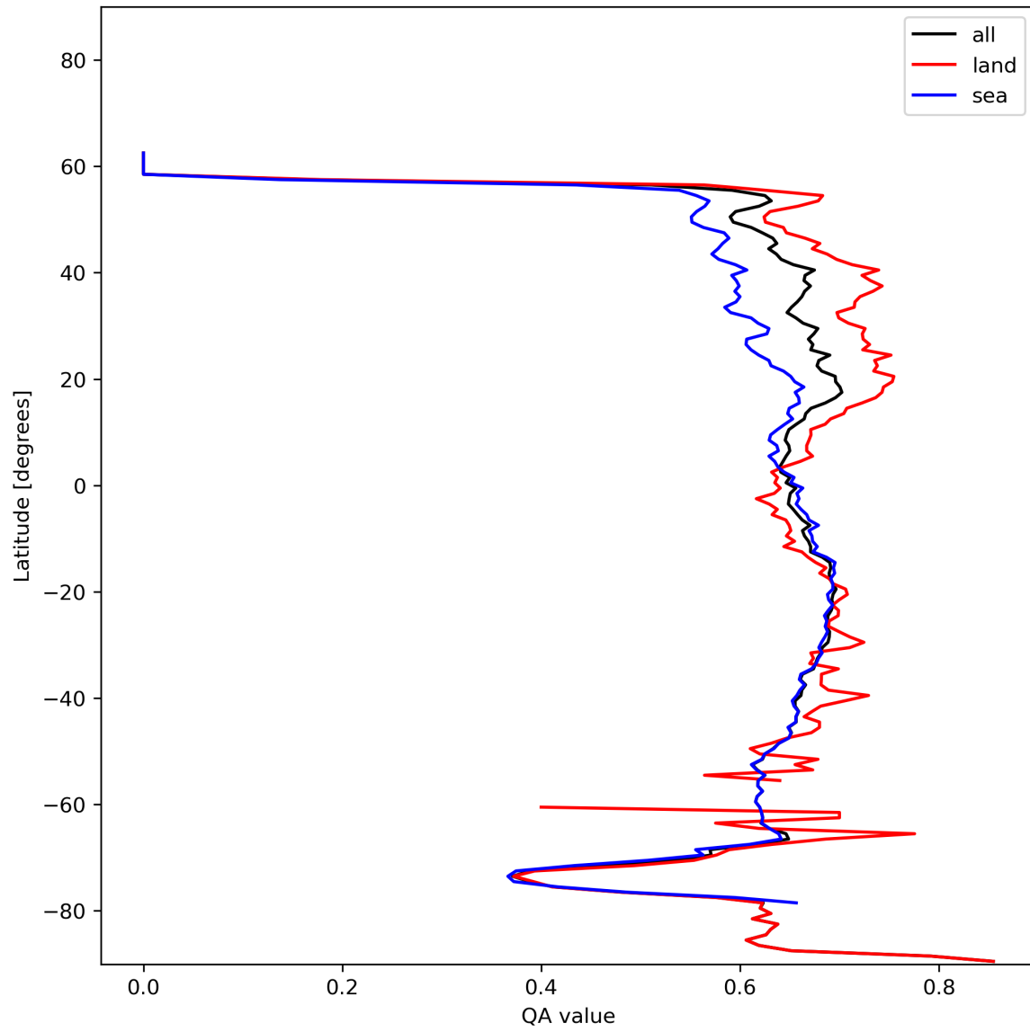
Figure 9: Zonal average of “QA value” for 2024-01-06 to 2024-01-08.
