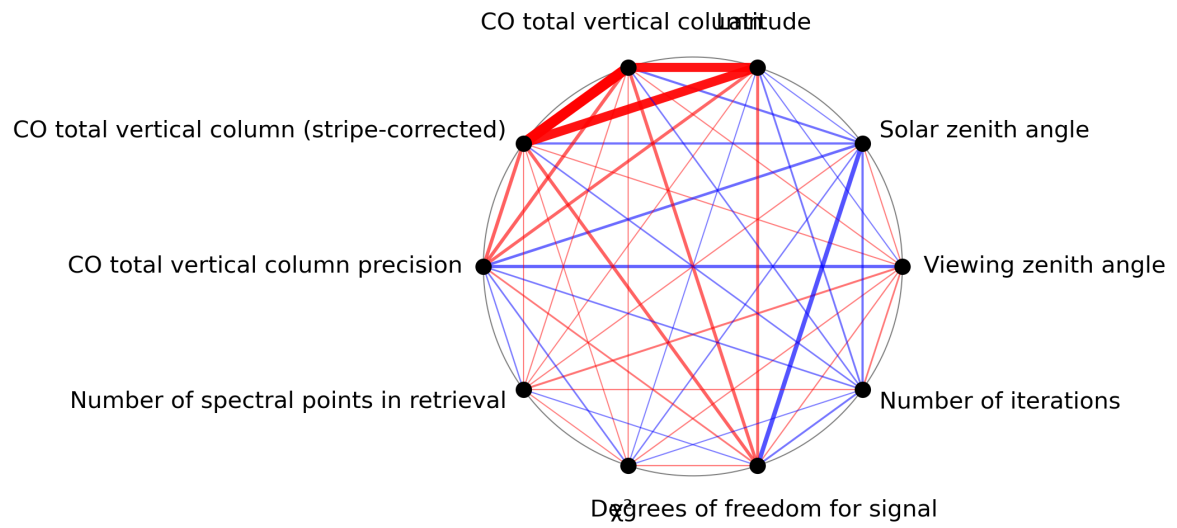
Figure 1: Map of correlation graph for 2024-01-06 to 2024-01-08.
