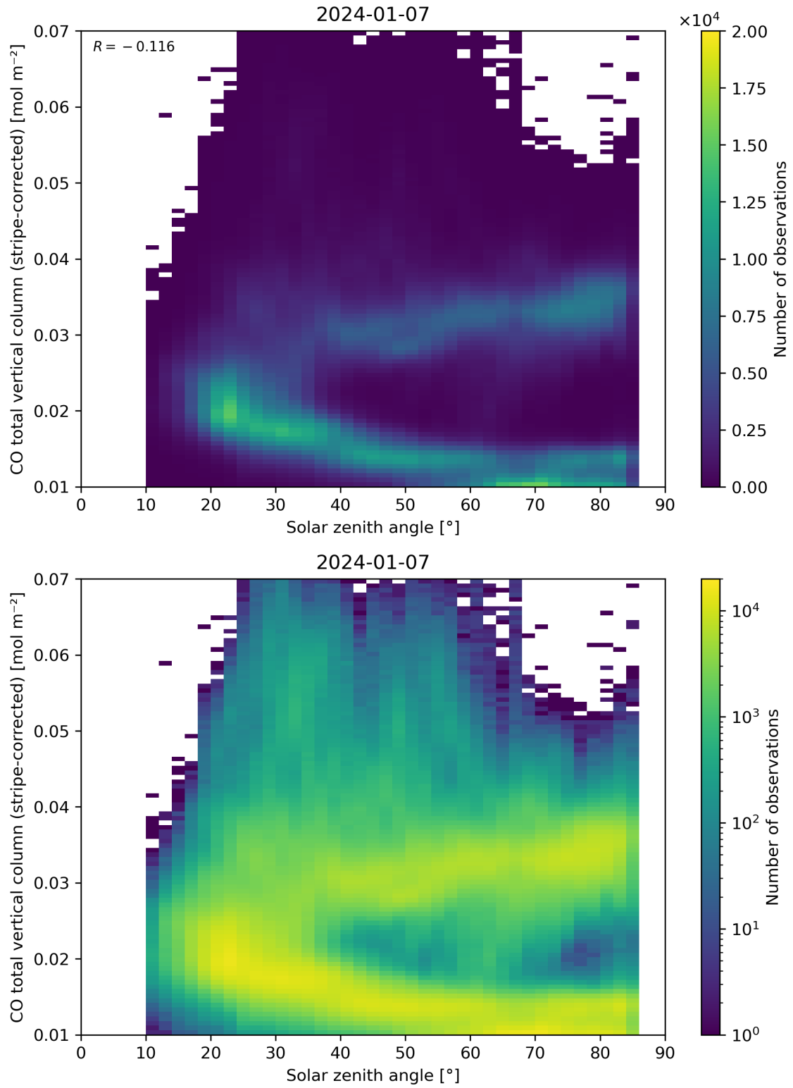
Figure 62: Scatter density plot of “Solar zenith angle” against “CO total vertical column (stripe-corrected)” for 2024-01-06 to 2024-01-08.
