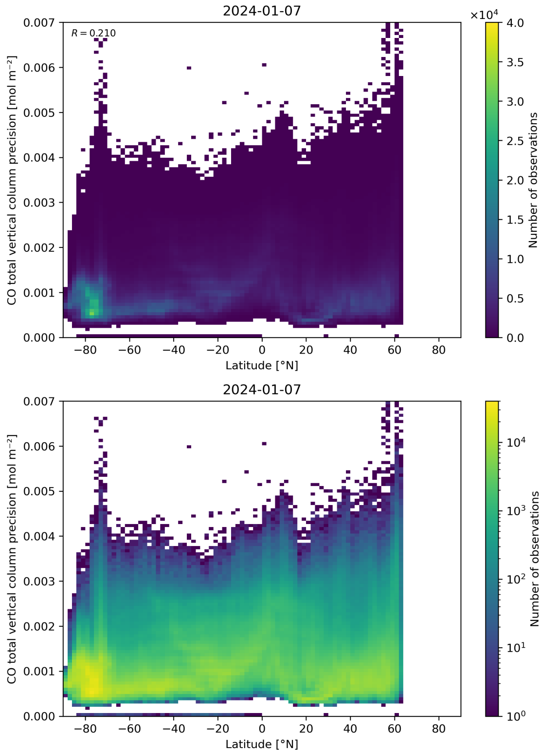
Figure 53: Scatter density plot of “Latitude” against “CO total vertical column precision” for 2024-01-06 to 2024-01-08.
