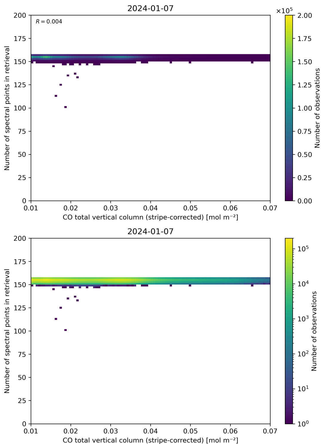
Figure 40: Scatter density plot of “CO total vertical column (stripe-corrected)” against “Number of spectral points in retrieval” for 2024-01-06 to 2024-01-08.
