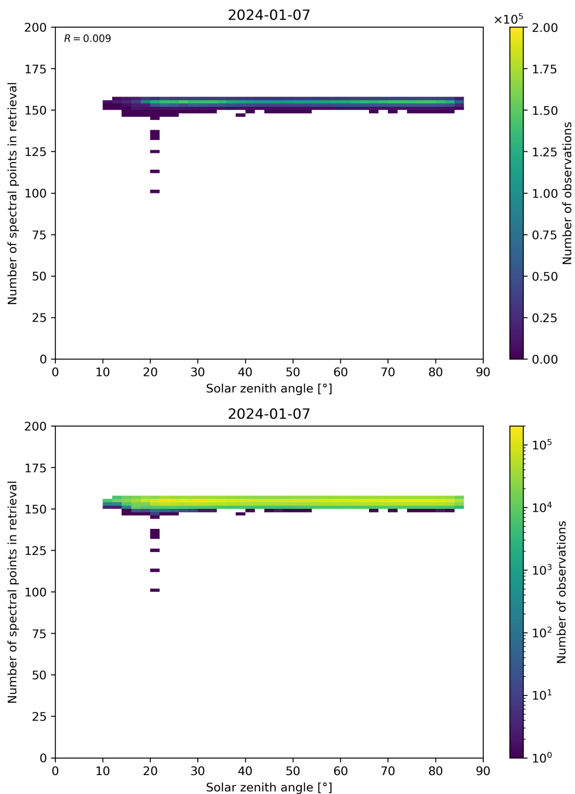
Figure 68: Scatter density plot of “Solar zenith angle” against “Number of spectral points in retrieval” for 2024-01-06 to 2024-01-08.
