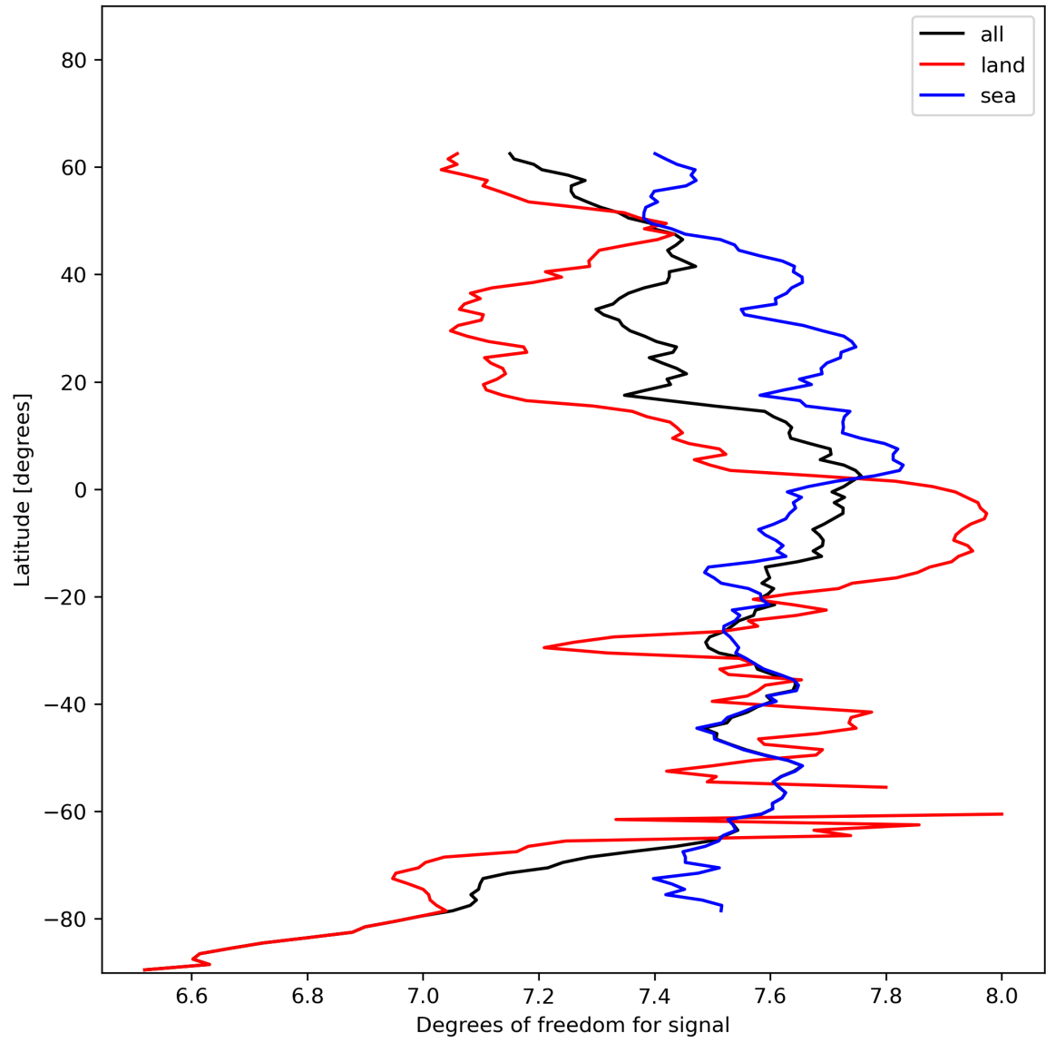
Figure 15: Zonal average of “Degrees of freedom for signal” for 2024-01-06 to 2024-01-08.
