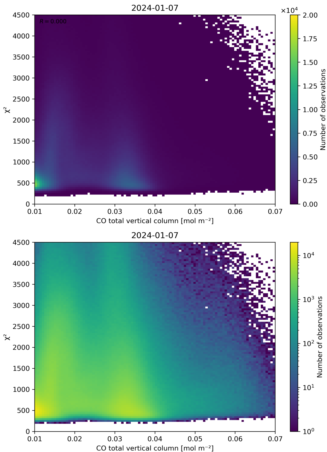
Figure 35: Scatter density plot of “CO total vertical column” against “ \chi^2 ” for 2024-01-06 to 2024-01-08.
