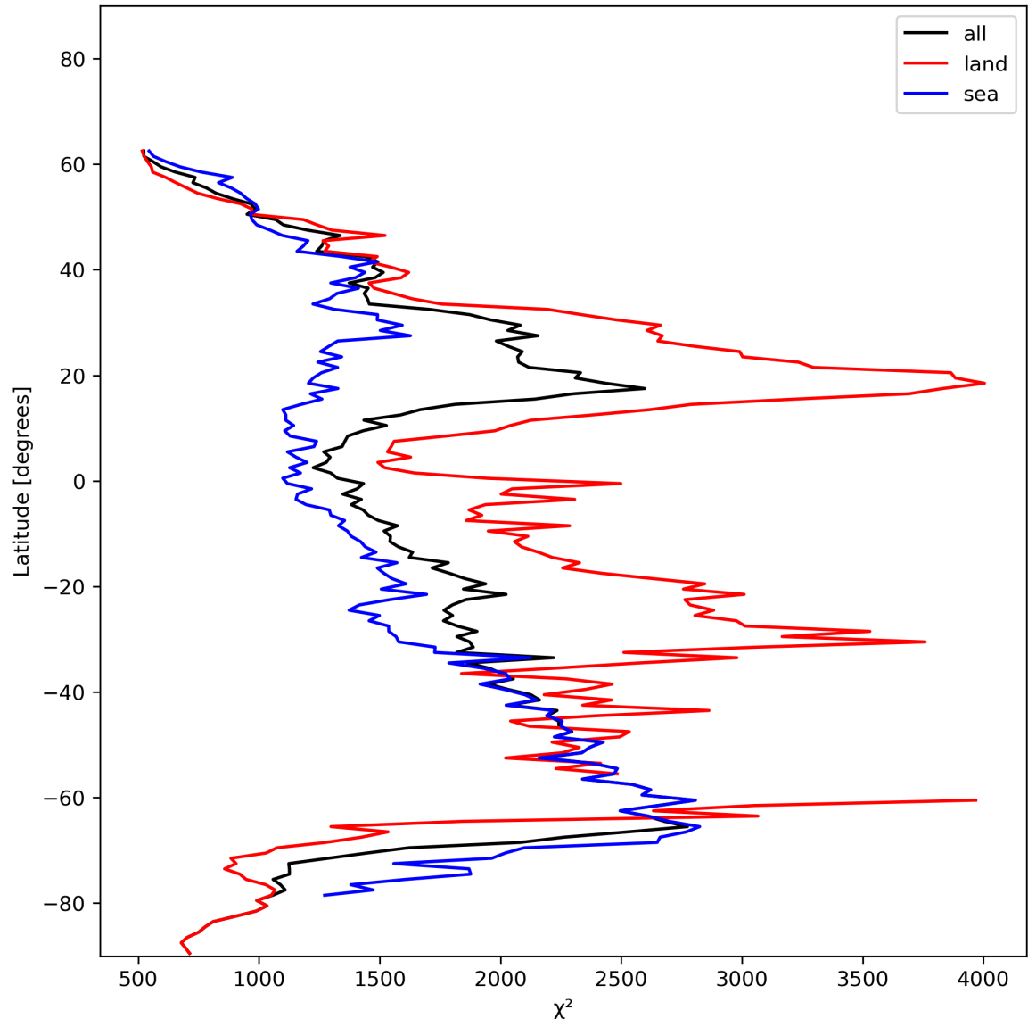
Figure 14: Zonal average of “ \chi^2 ” for 2024-01-06 to 2024-01-08.
