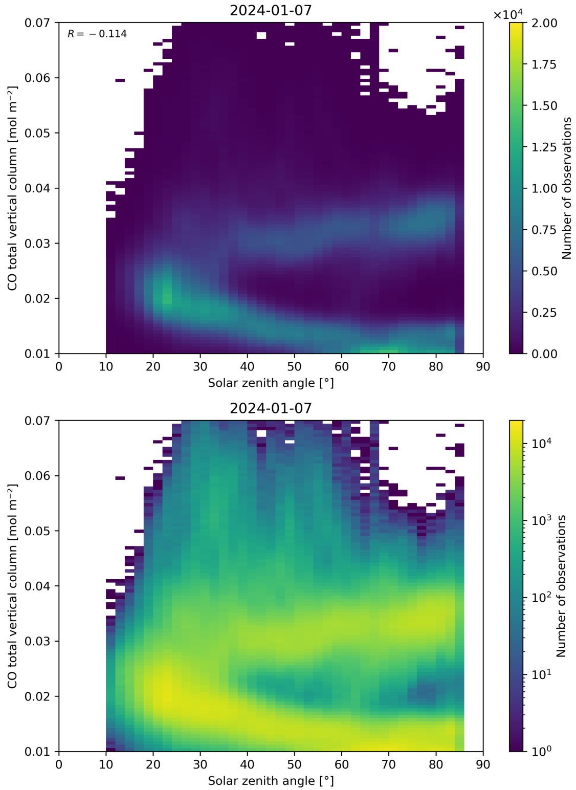
Figure 61: Scatter density plot of “Solar zenith angle” against “CO total vertical column” for 2024-01-06 to 2024-01-08.
