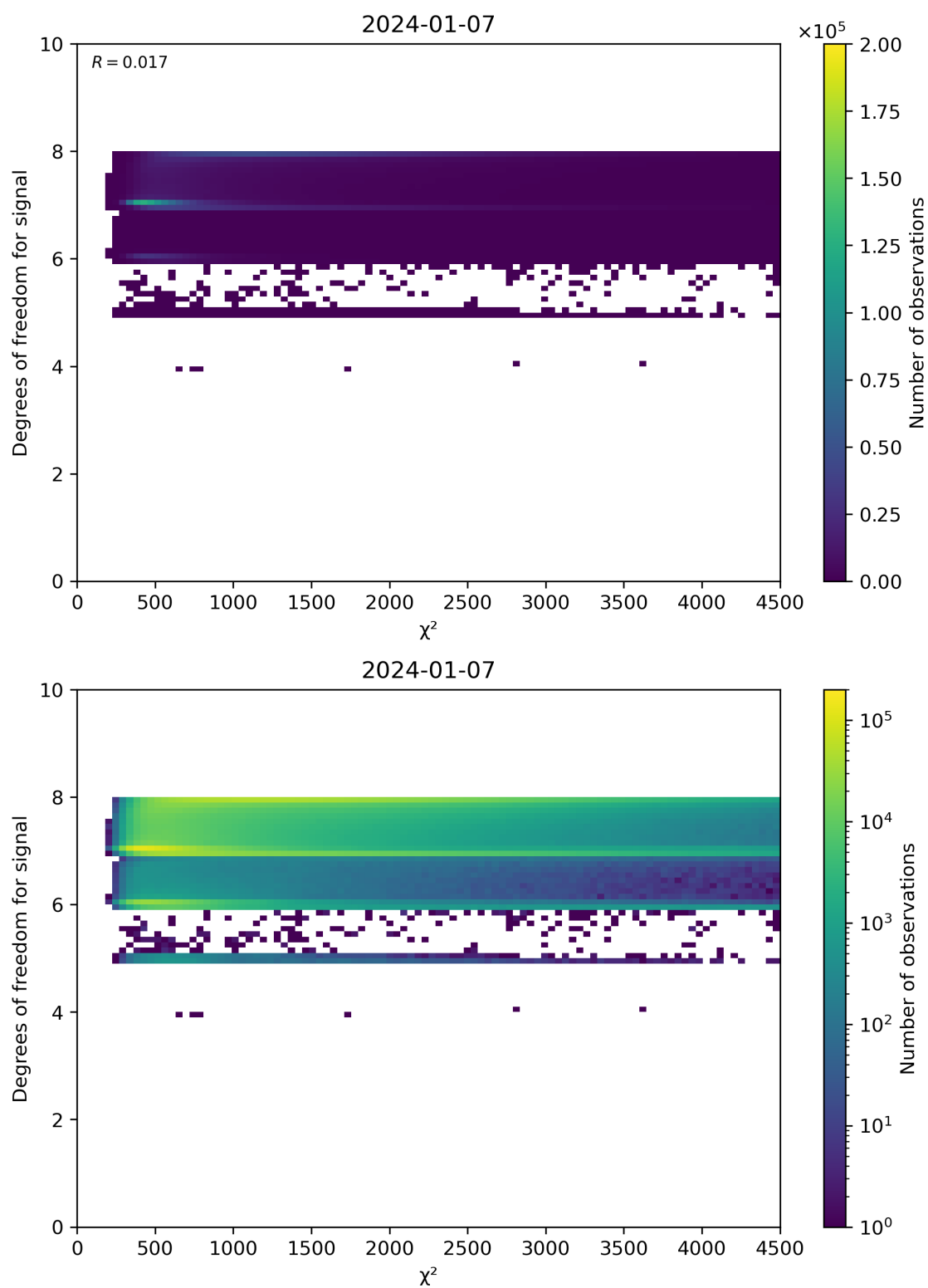
Figure 48: Scatter density plot of “ \chi^2 ” against “Degrees of freedom for signal” for 2024-01-06 to 2024-01-08.
