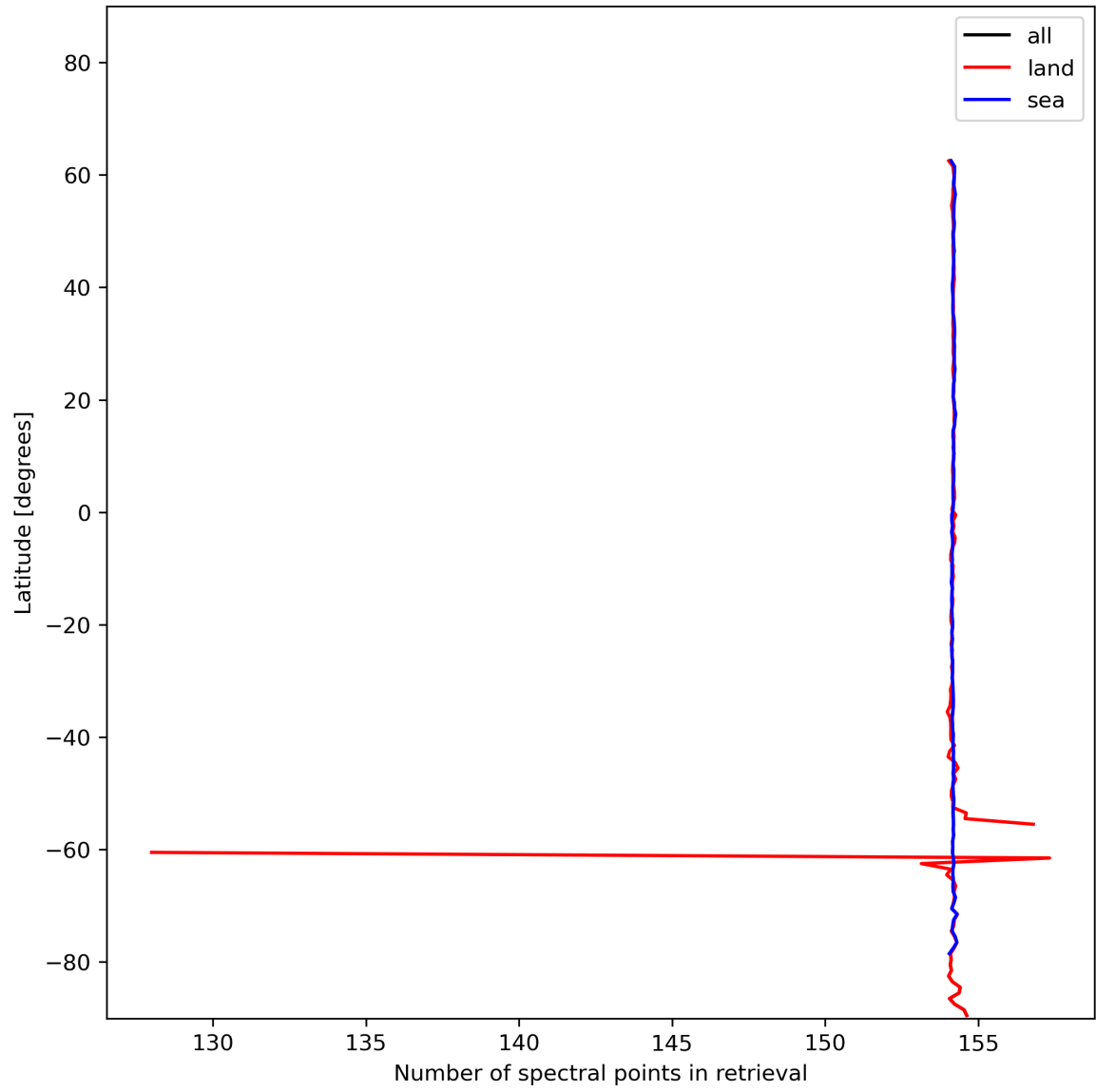
Figure 13: Zonal average of “Number of spectral points in retrieval” for 2024-01-06 to 2024-01-08.
