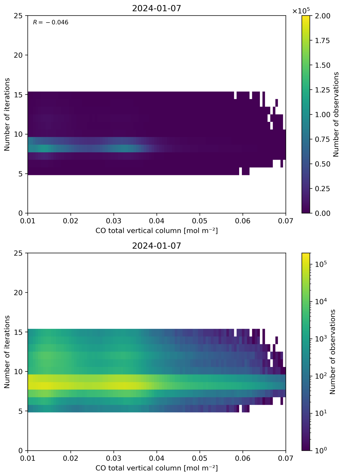
Figure 42: Scatter density plot of “CO total vertical column” against “Number of iterations” for 2024-01-06 to 2024-01-08.
