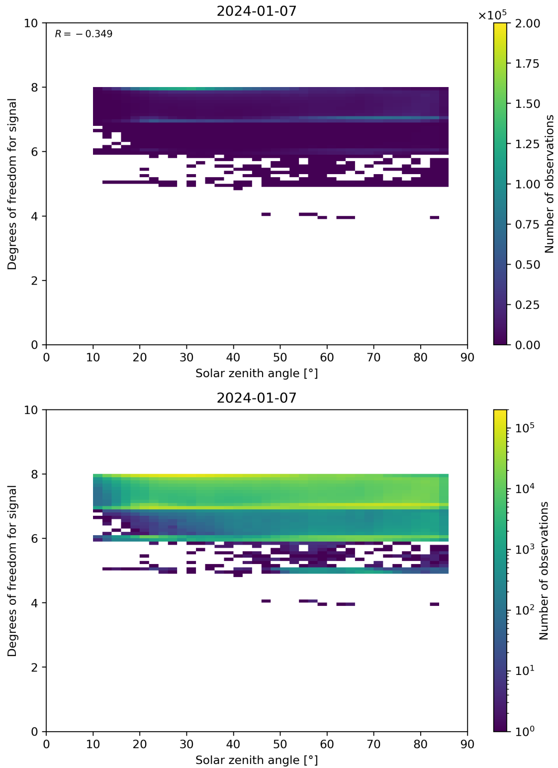
Figure 65: Scatter density plot of “Solar zenith angle” against “Degrees of freedom for signal” for 2024-01-06 to 2024-01-08.
