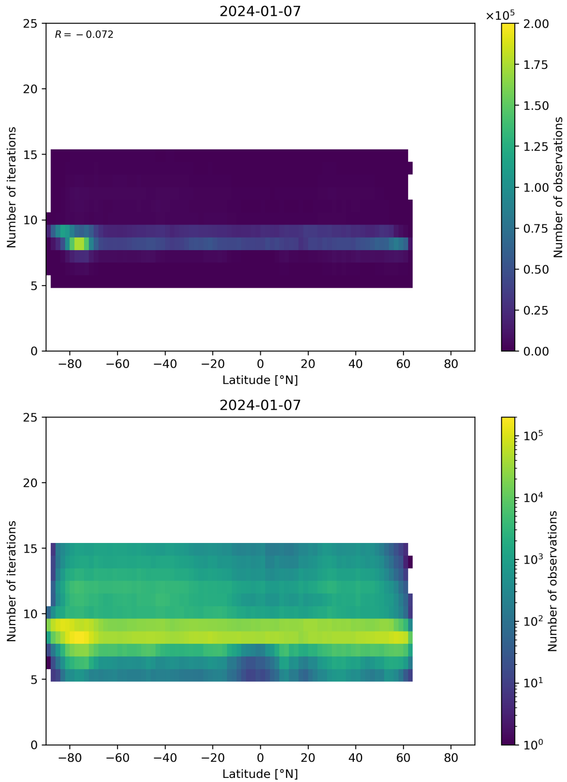
Figure 56: Scatter density plot of “Latitude” against “Number of iterations” for 2024-01-06 to 2024-01-08.
