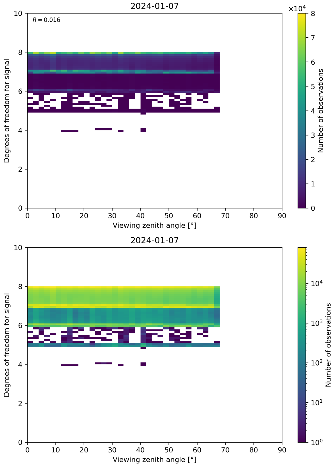
Figure 73: Scatter density plot of “Viewing zenith angle” against “Degrees of freedom for signal” for 2024-01-06 to 2024-01-08.
