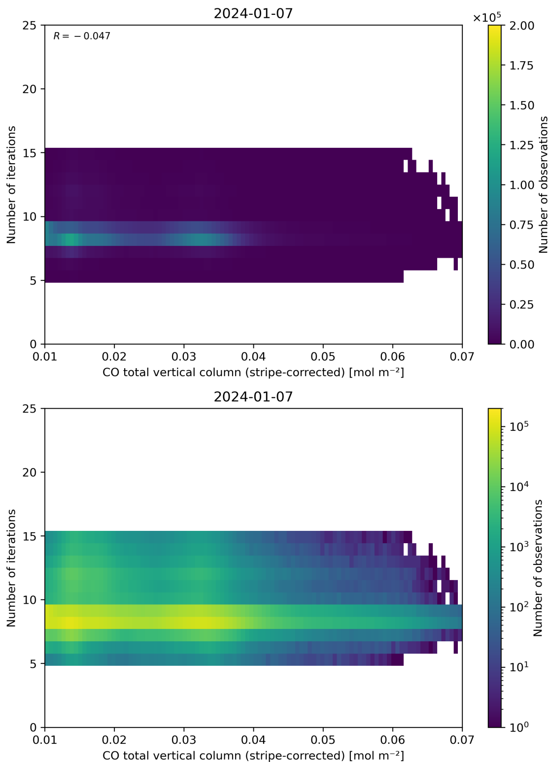
Figure 39: Scatter density plot of “CO total vertical column (stripe-corrected)” against “Number of iterations” for 2024-01-06 to 2024-01-08.
