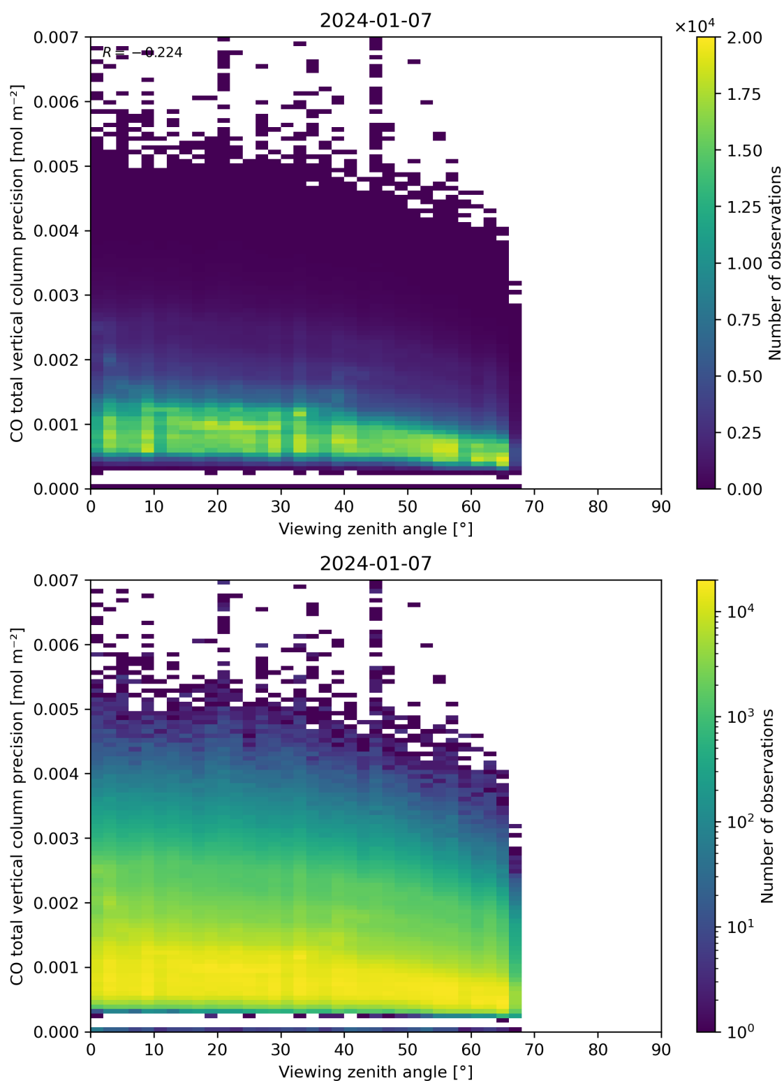
Figure 71: Scatter density plot of “Viewing zenith angle” against “CO total vertical column precision” for 2024-01-06 to 2024-01-08.
