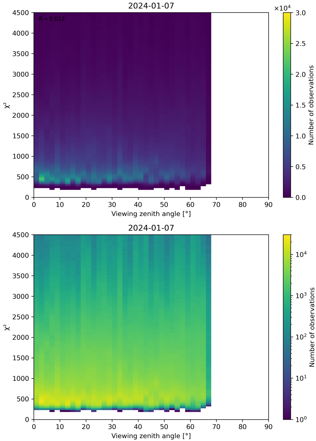
Figure 72: Scatter density plot of “Viewing zenith angle” against “ \chi^2 ” for 2024-01-06 to 2024-01-08.
