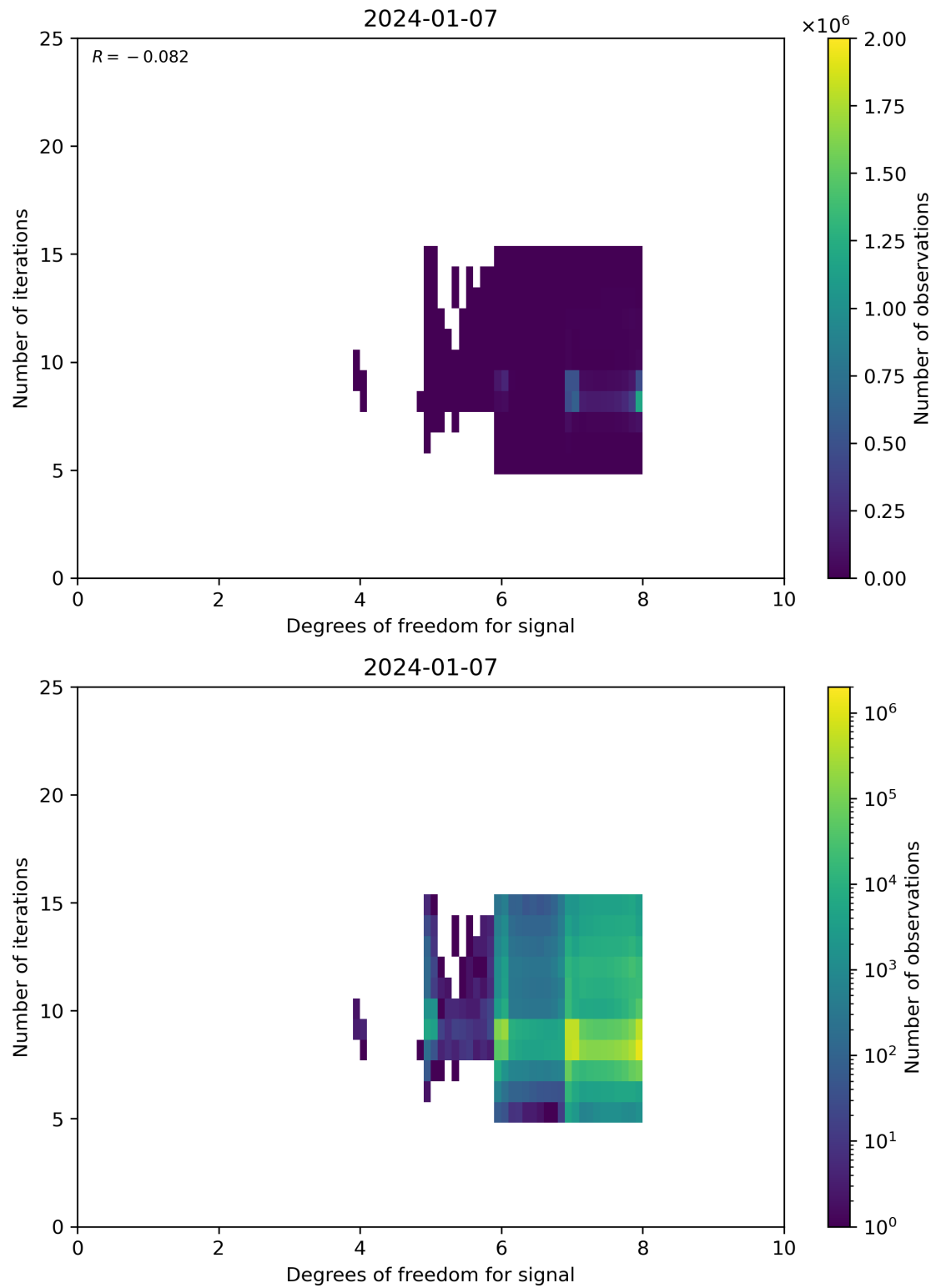
Figure 50: Scatter density plot of “Degrees of freedom for signal” against “Number of iterations” for 2024-01-06 to 2024-01-08.
