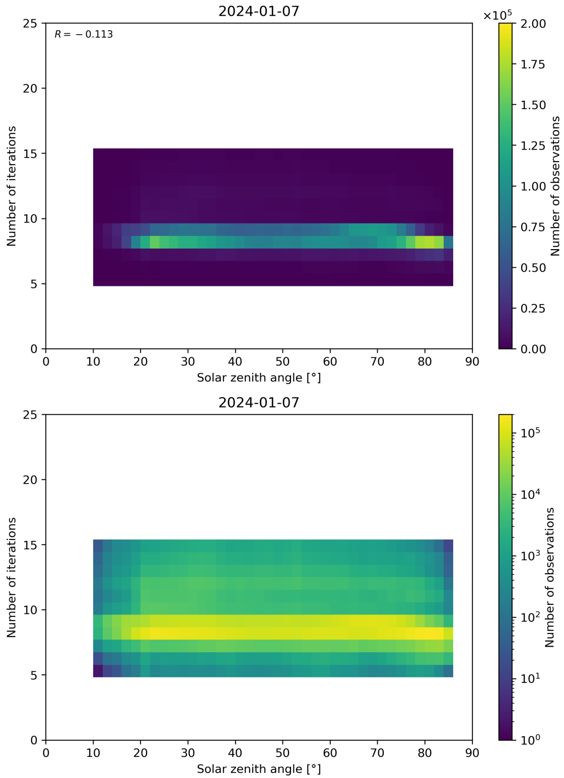
Figure 67: Scatter density plot of “Solar zenith angle” against “Number of iterations” for 2024-01-06 to 2024-01-08.
