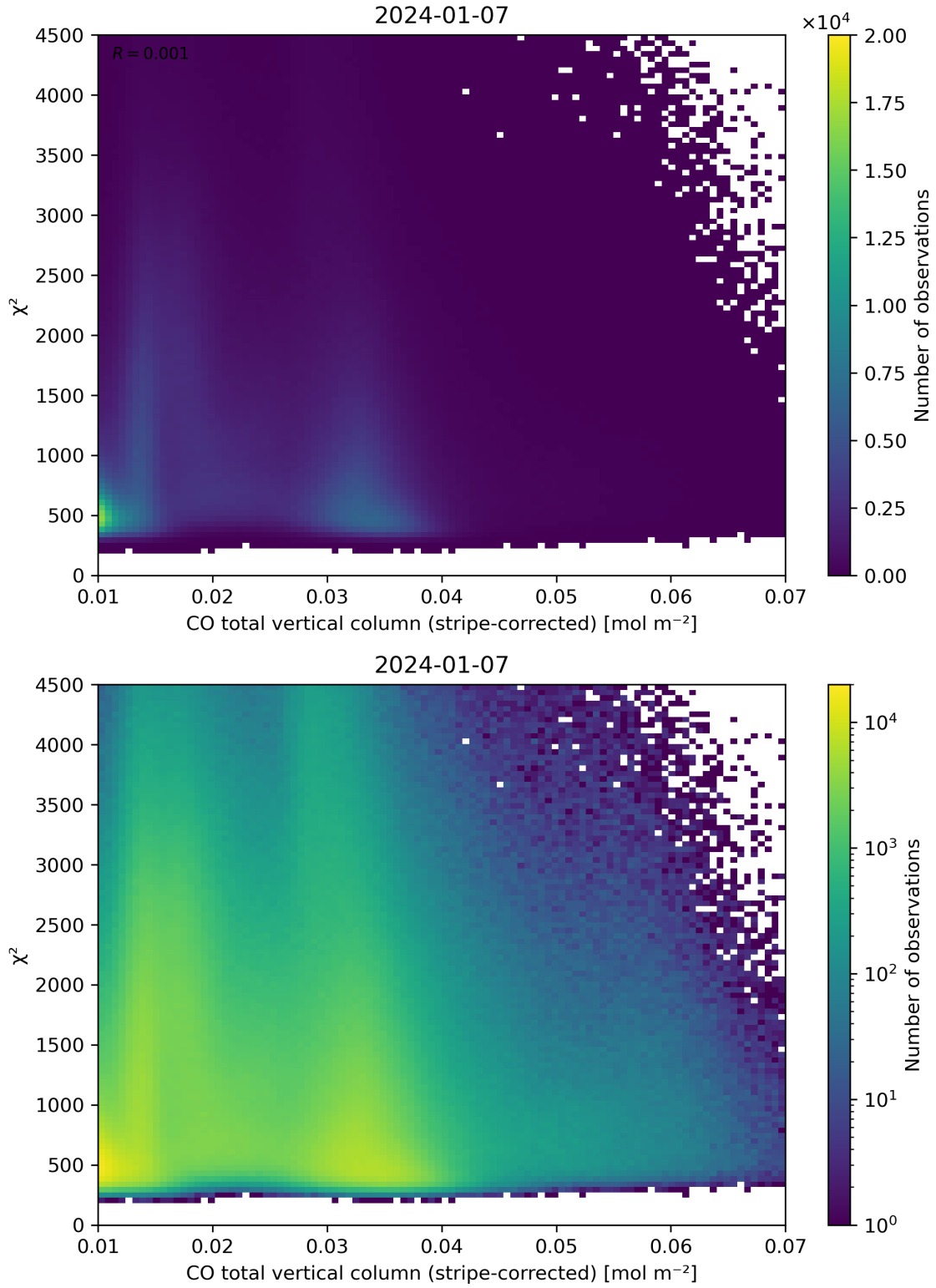
Figure 37: Scatter density plot of “CO total vertical column (stripe-corrected)” against “ \chi^2 ” for 2024-01-06 to 2024-01-08.
