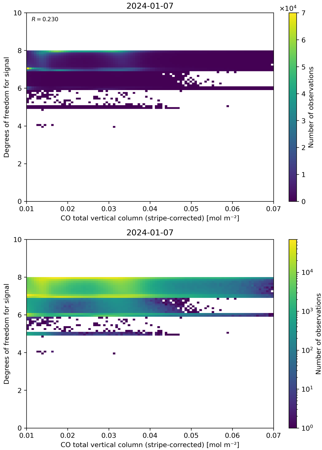
Figure 38: Scatter density plot of “CO total vertical column (stripe-corrected)” against “Degrees of freedom for signal” for 2024-01-06 to 2024-01-08.
