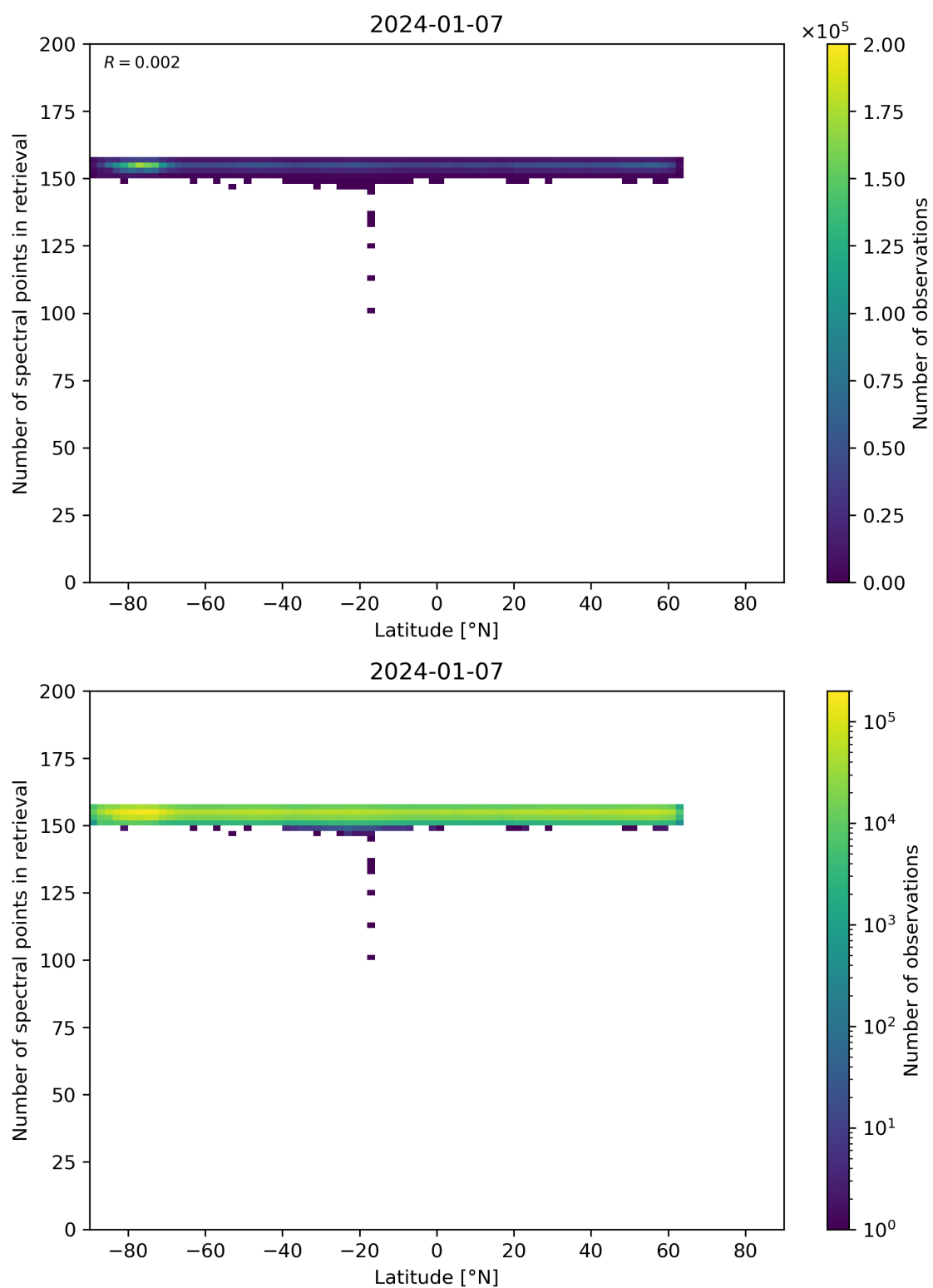
Figure 57: Scatter density plot of “Latitude” against “Number of spectral points in retrieval” for 2024-01-06 to 2024-01-08.
