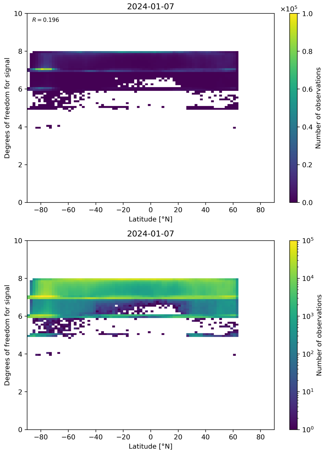
Figure 55: Scatter density plot of “Latitude” against “Degrees of freedom for signal” for 2024-01-06 to 2024-01-08.
