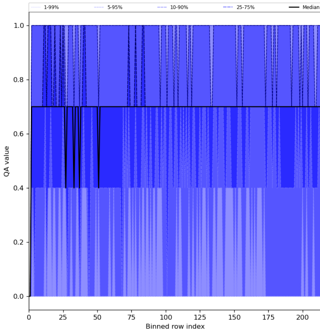
Figure 25: Along track statistics of “QA value” for 2024-01-06 to 2024-01-08
