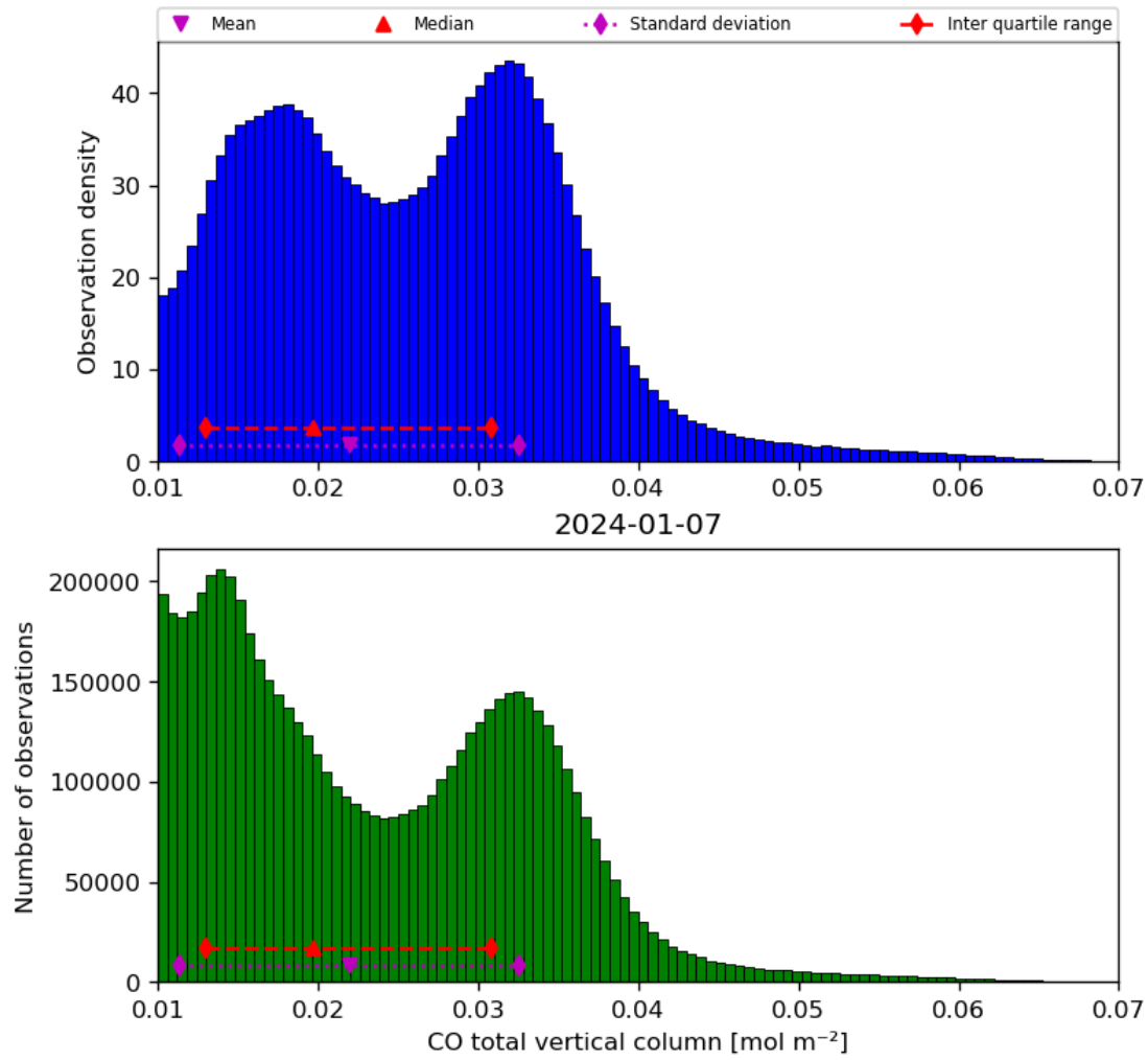
Figure 18: Histogram of “CO total vertical column” for 2024-01-06 to 2024-01-08
