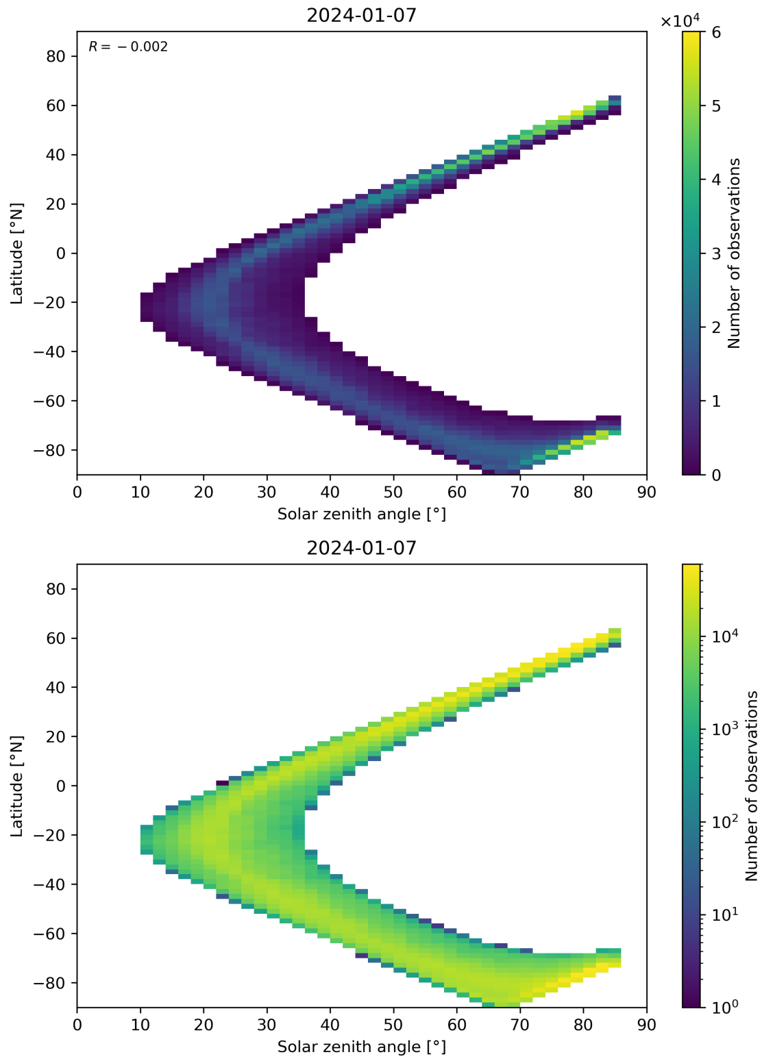
Figure 66: Scatter density plot of “Solar zenith angle” against “Latitude” for 2024-01-06 to 2024-01-08.
