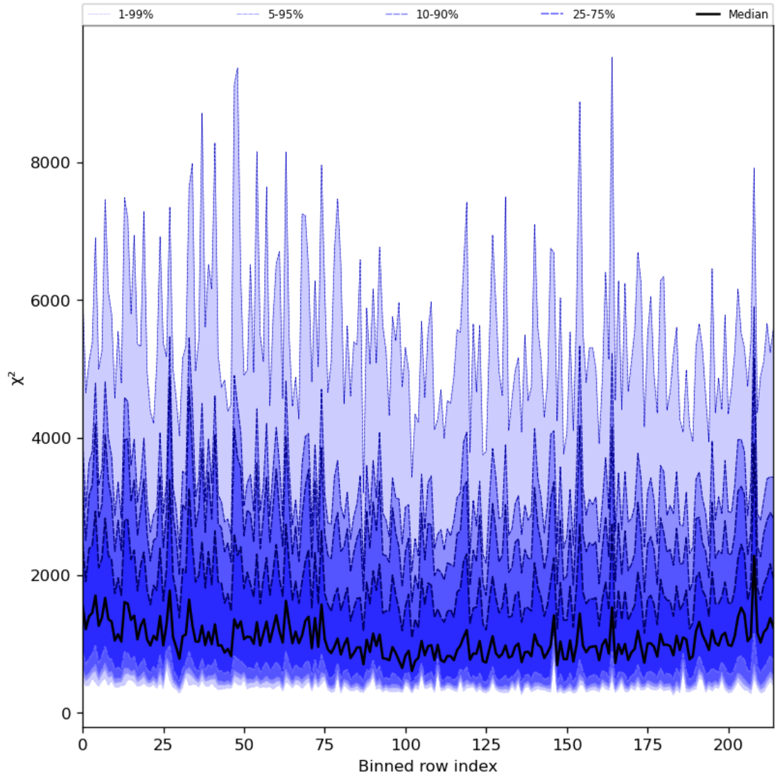
Figure 30: Along track statistics of “ \chi^2 ” for 2024-01-06 to 2024-01-08
