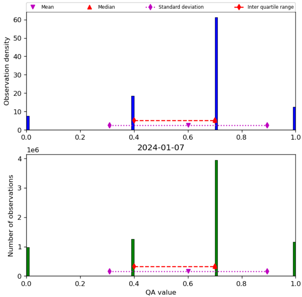
Figure 17: Histogram of “QA value” for 2024-01-06 to 2024-01-08
