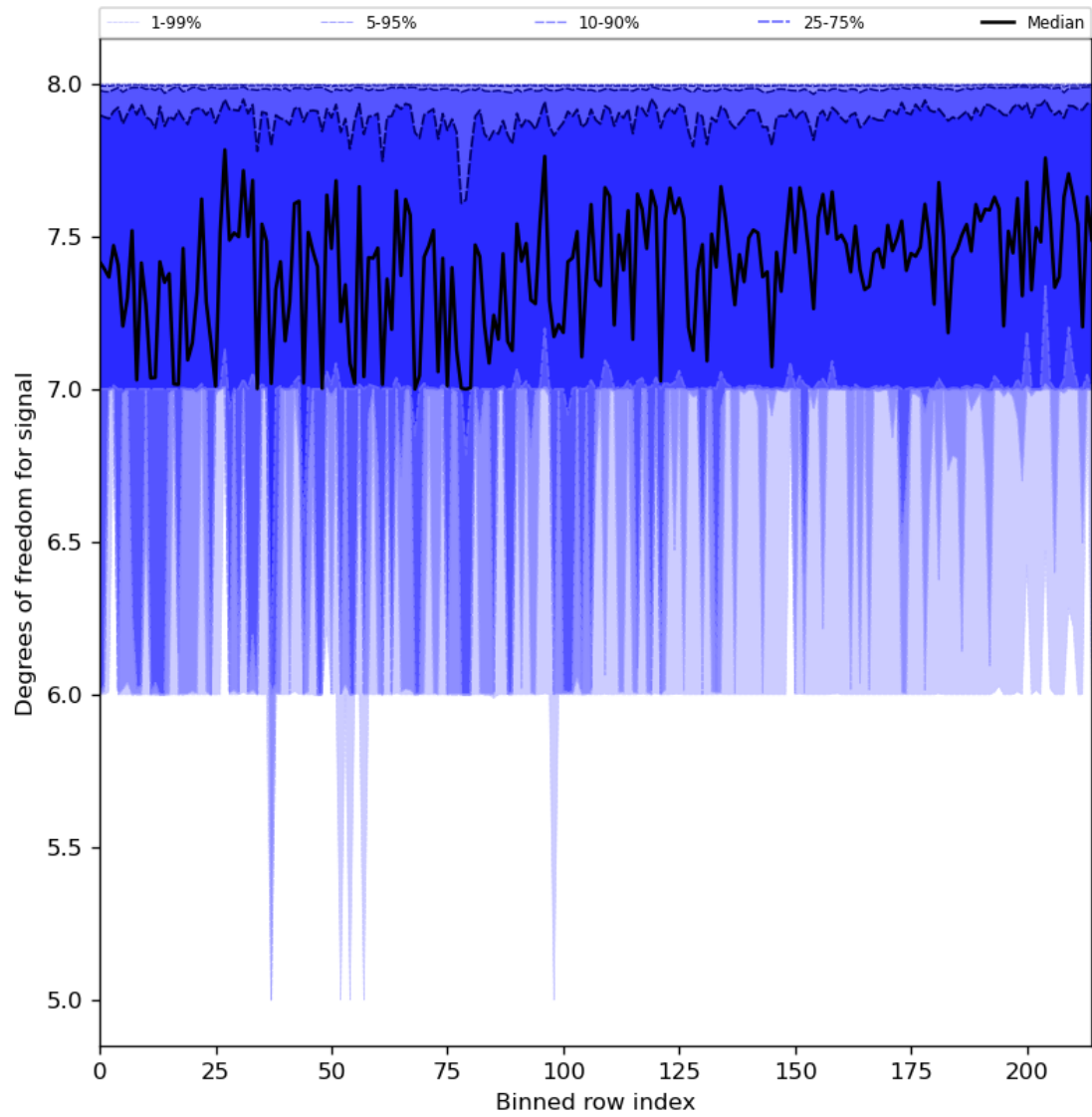
Figure 31: Along track statistics of “Degrees of freedom for signal” for 2024-01-06 to 2024-01-08
