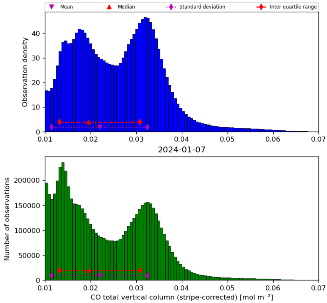
Figure 19: Histogram of “CO total vertical column (stripe-corrected)” for 2024-01-06 to 2024-01-08
