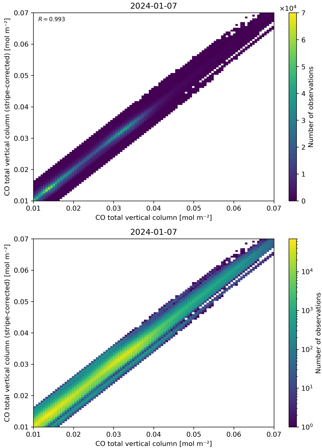
Figure 33: Scatter density plot of “CO total vertical column” against “CO total vertical column (stripe-corrected)” for 2024-01-06 to 2024-01-08.
