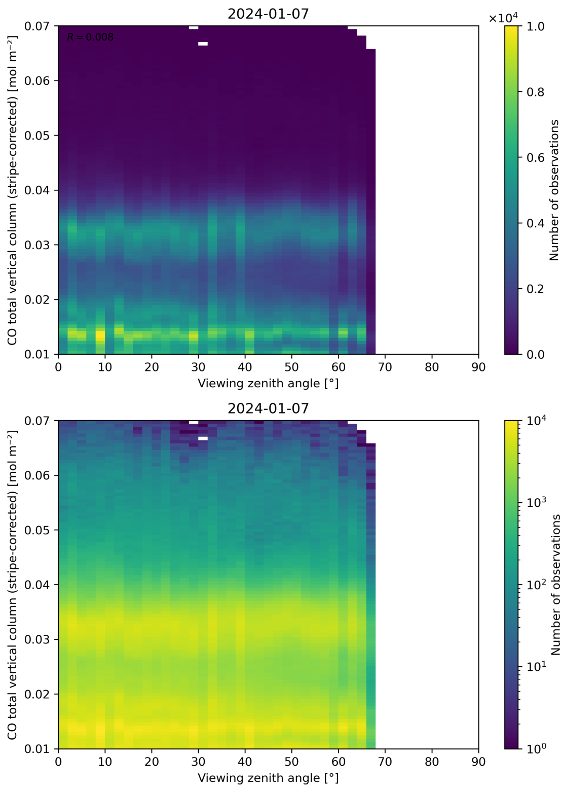
Figure 70: Scatter density plot of “Viewing zenith angle” against “CO total vertical column (stripe-corrected)” for 2024-01-06 to 2024-01-08.
