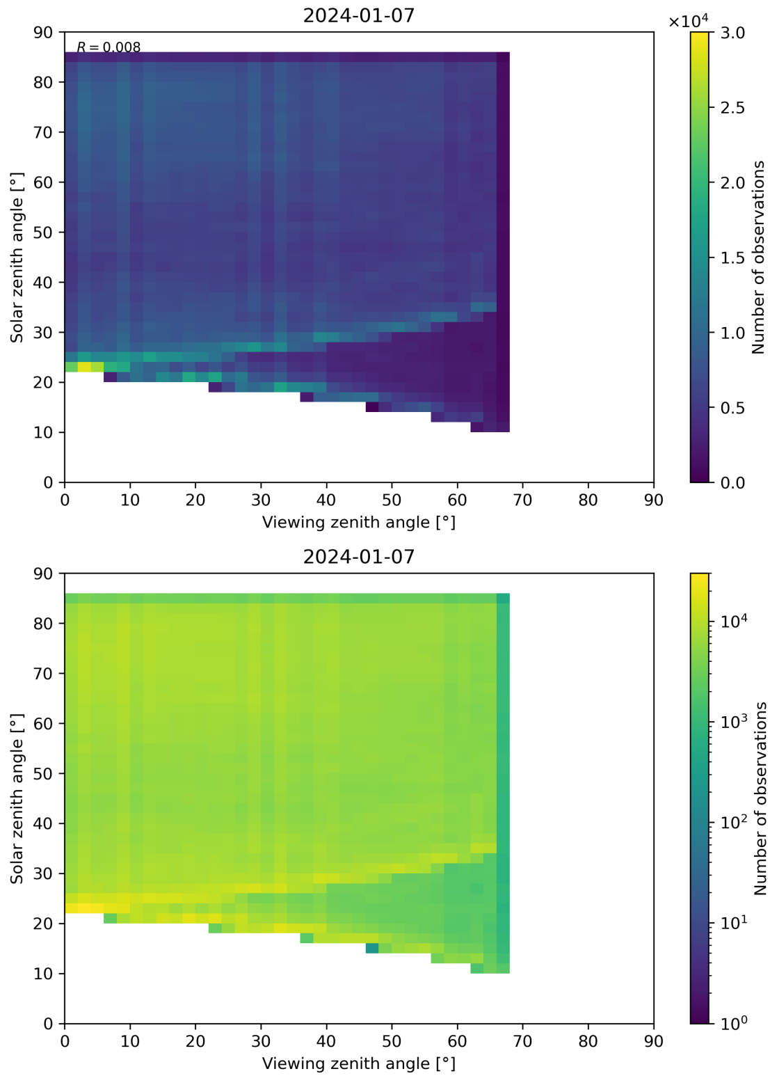
Figure 77: Scatter density plot of “Viewing zenith angle” against “Solar zenith angle” for 2024-01-06 to 2024-01-08.
