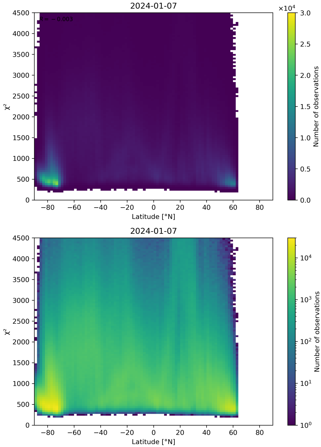
Figure 54: Scatter density plot of “Latitude” against “ \chi^2 ” for 2024-01-06 to 2024-01-08.
