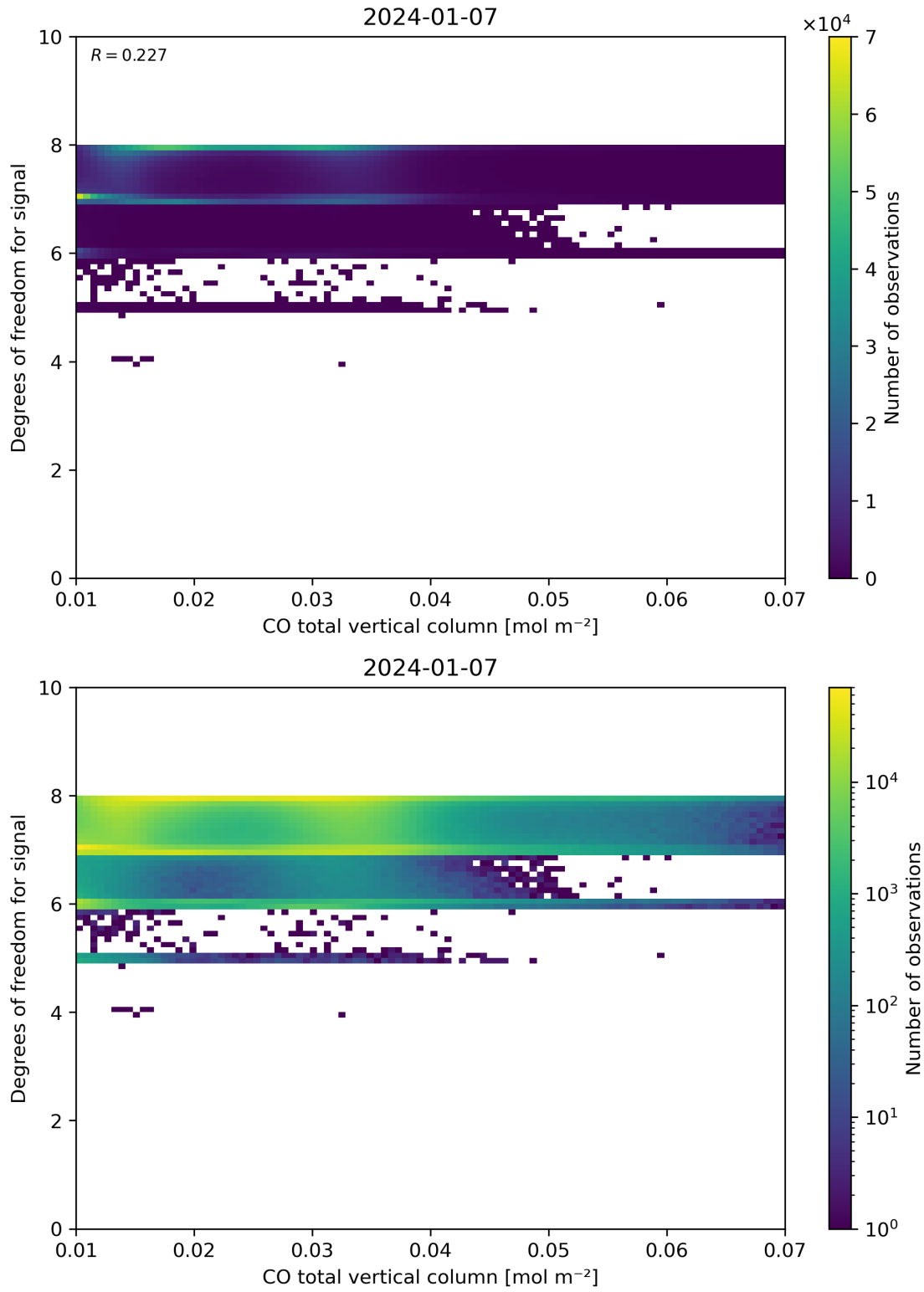
Figure 41: Scatter density plot of “CO total vertical column” against “Degrees of freedom for signal” for 2024-01-06 to 2024-01-08.
