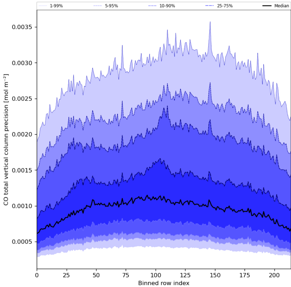
Figure 28: Along track statistics of “CO total vertical column precision” for 2024-01-06 to 2024-01-08
