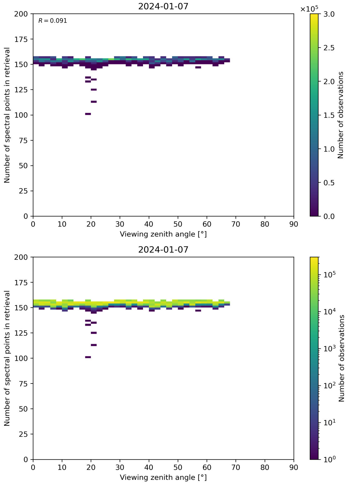
Figure 76: Scatter density plot of “Viewing zenith angle” against “Number of spectral points in retrieval” for 2024-01-06 to 2024-01-08.
