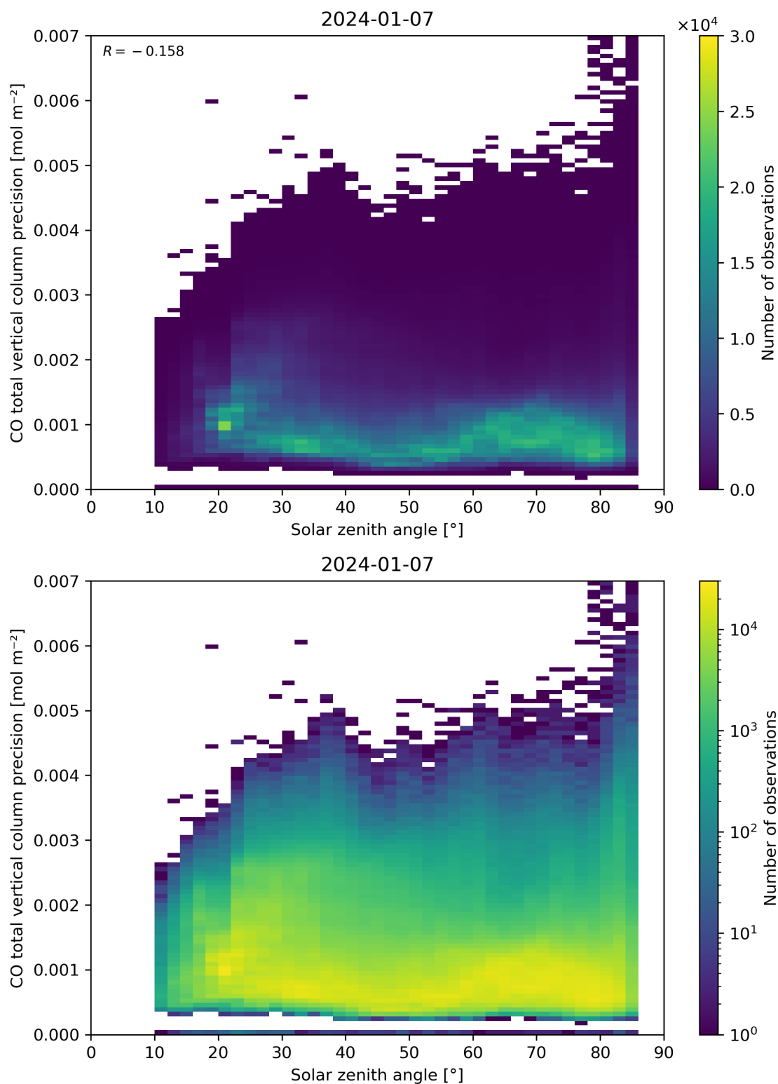
Figure 63: Scatter density plot of “Solar zenith angle” against “CO total vertical column precision” for 2024-01-06 to 2024-01-08.
