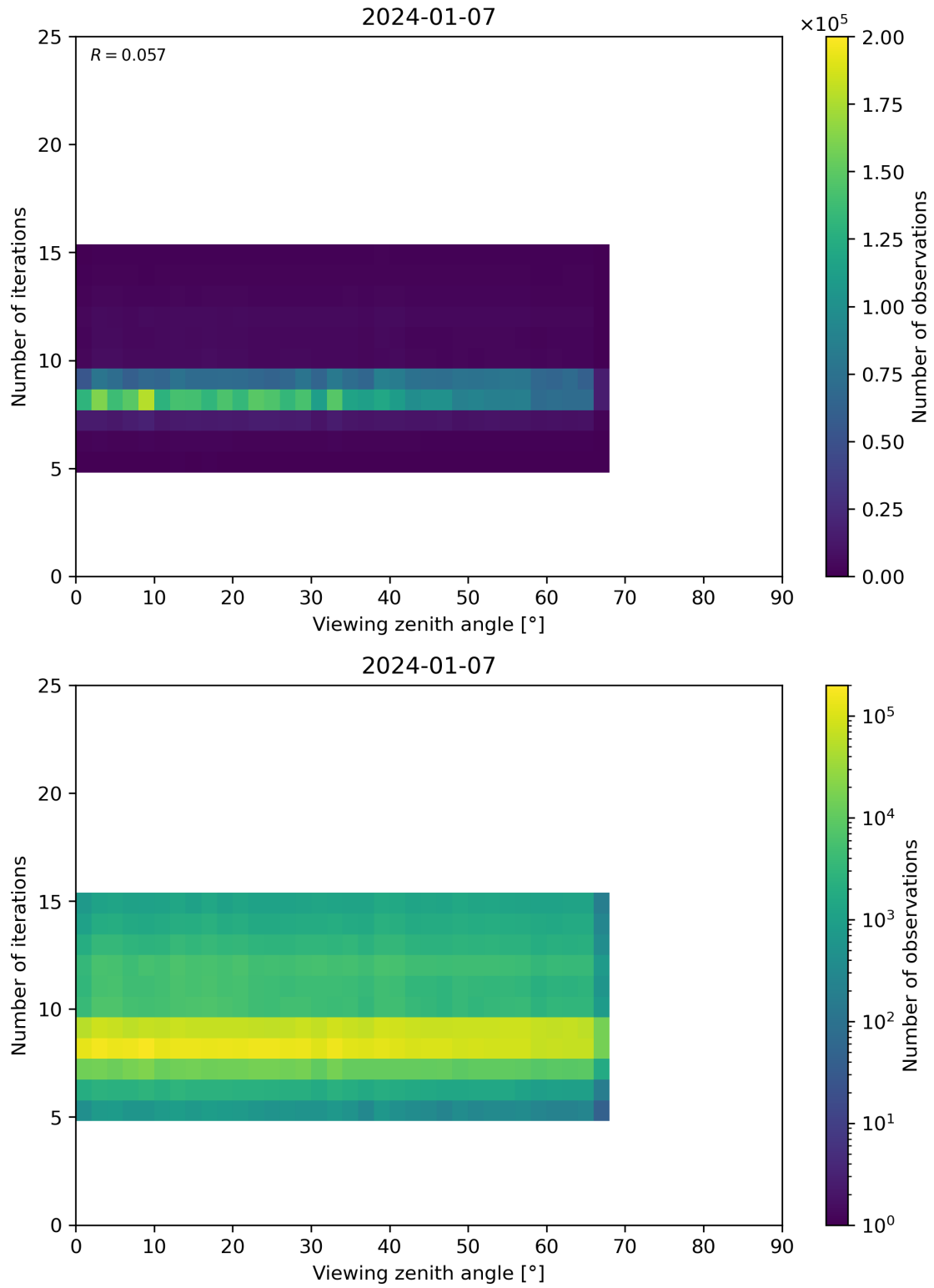
Figure 75: Scatter density plot of “Viewing zenith angle” against “Number of iterations” for 2024-01-06 to 2024-01-08.
