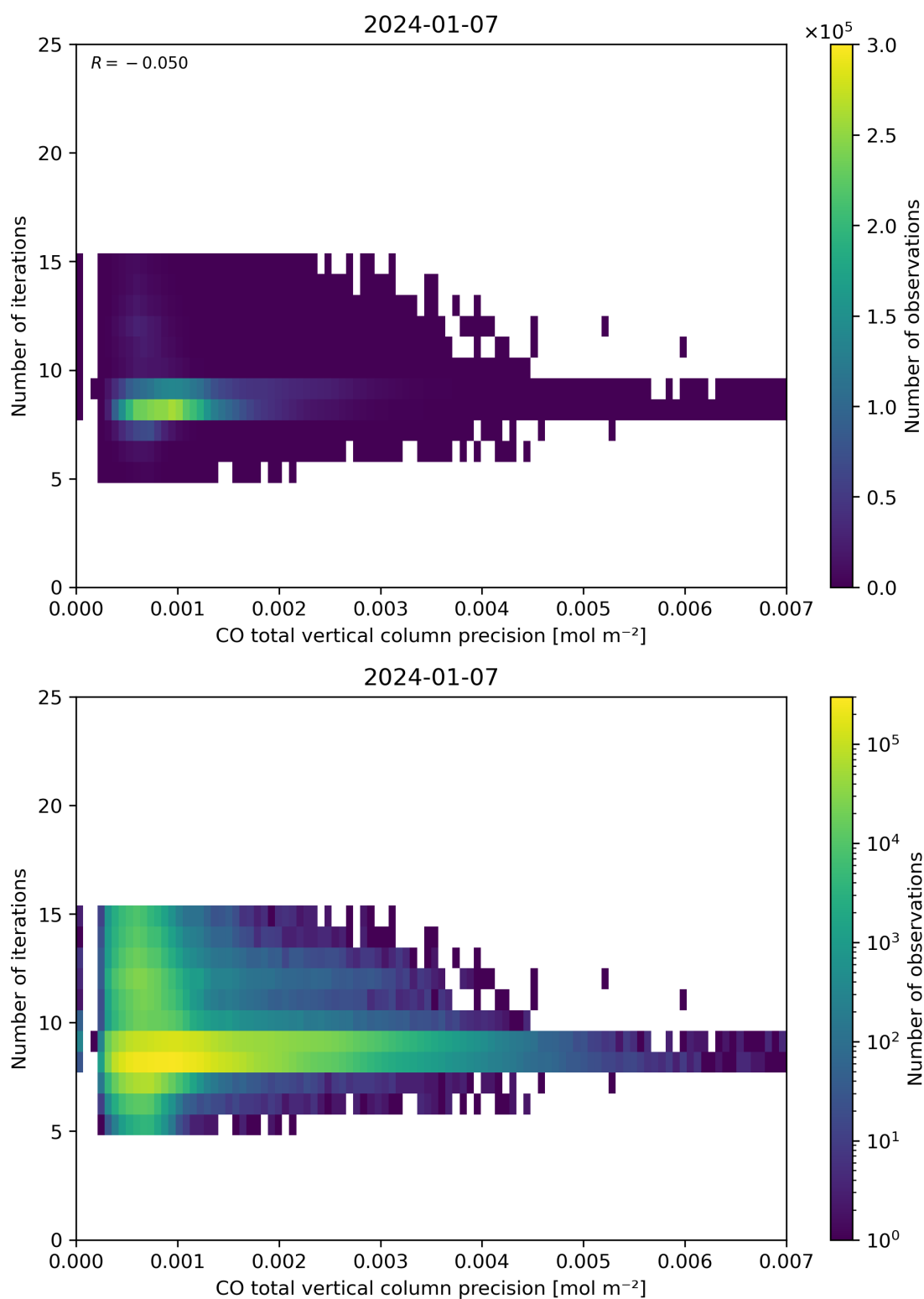
Figure 46: Scatter density plot of “CO total vertical column precision” against “Number of iterations” for 2024-01-06 to 2024-01-08.
