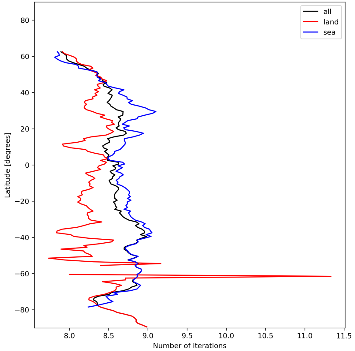
Figure 16: Zonal average of “Number of iterations” for 2024-01-06 to 2024-01-08.
