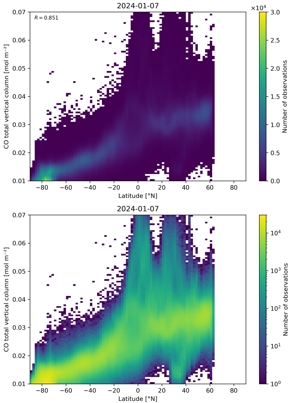
Figure 51: Scatter density plot of “Latitude” against “CO total vertical column” for 2024-01-06 to 2024-01-08.
