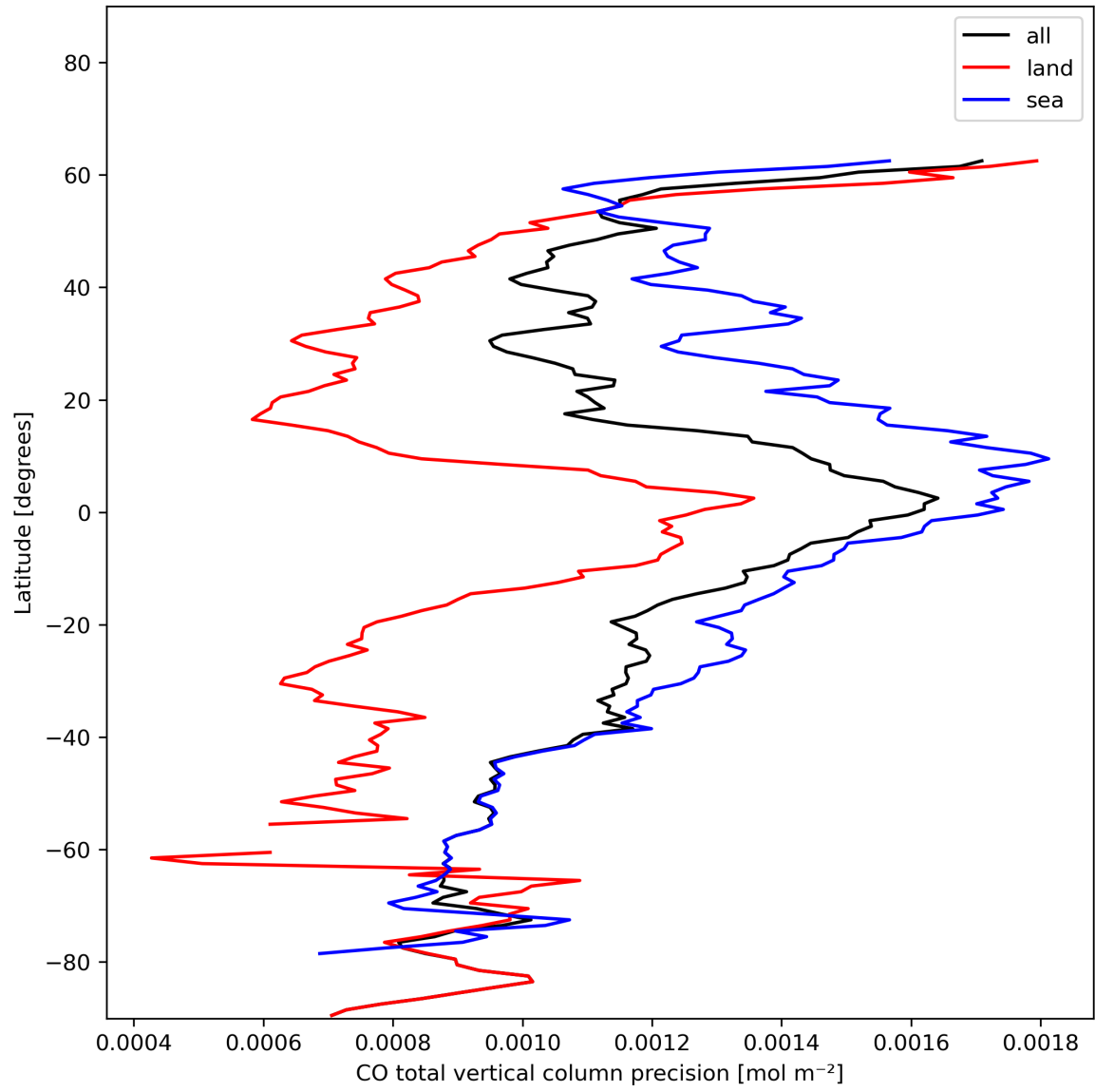
Figure 12: Zonal average of “CO total vertical column precision” for 2024-01-06 to 2024-01-08.
