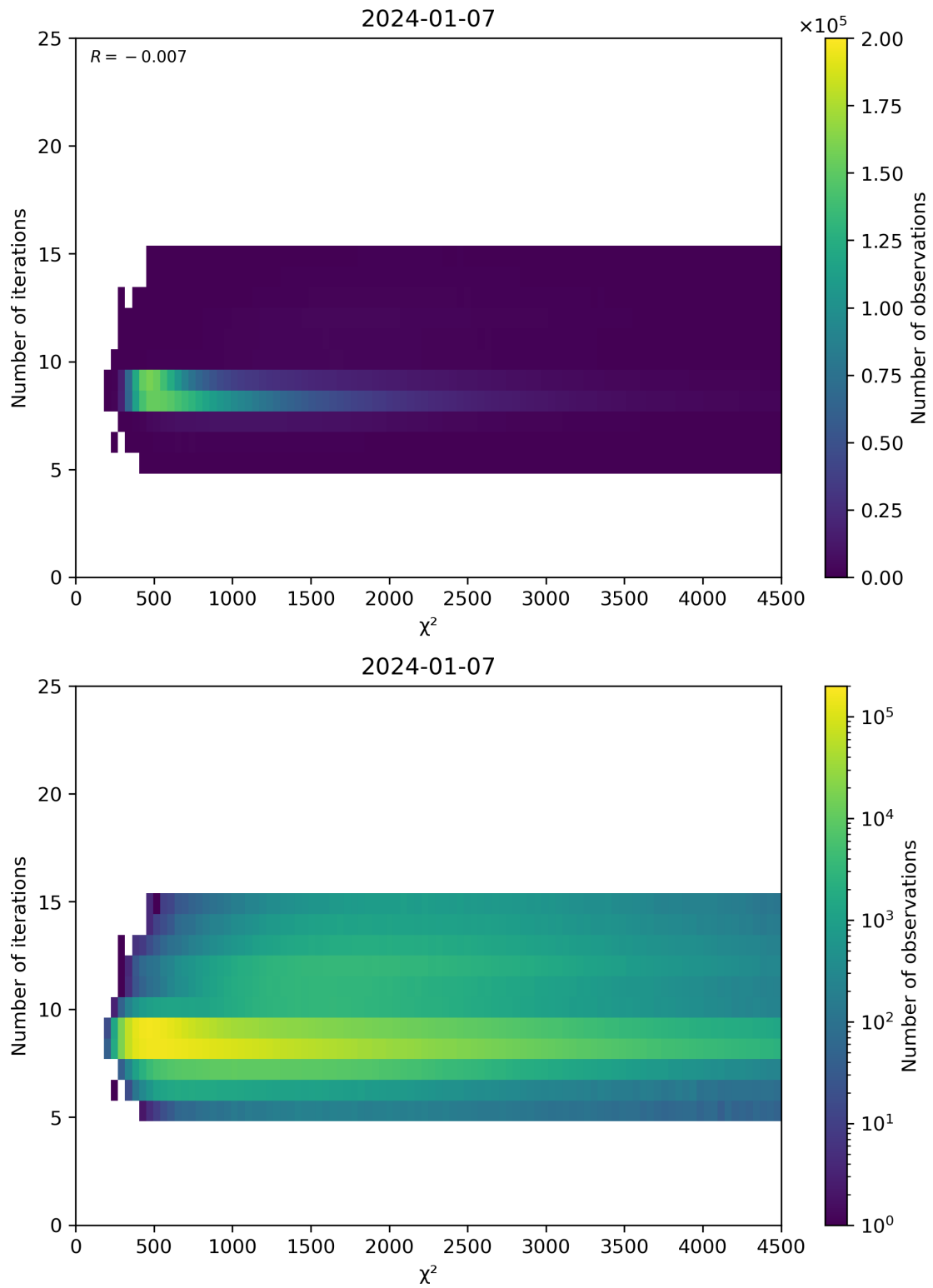
Figure 49: Scatter density plot of “ \chi^2 ” against “Number of iterations” for 2024-01-06 to 2024-01-08.
