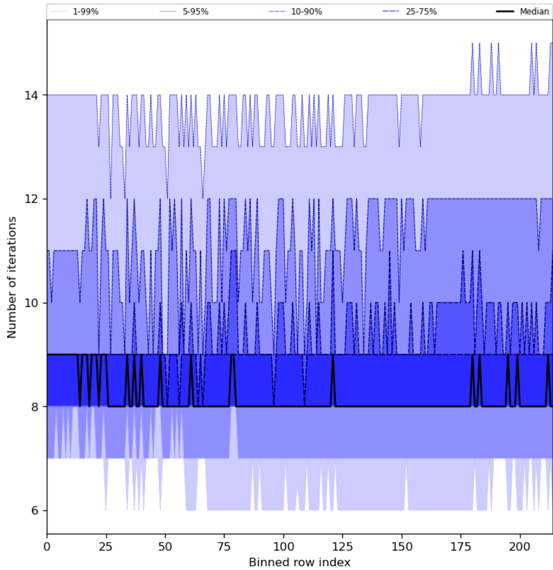
Figure 32: Along track statistics of “Number of iterations” for 2024-01-06 to 2024-01-08
