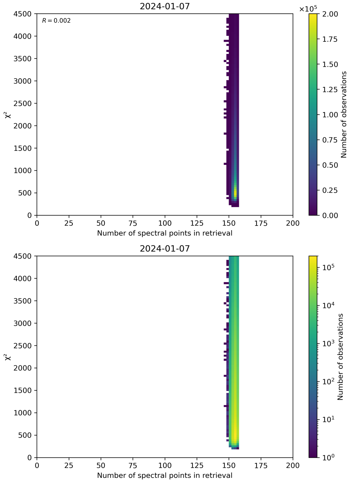
Figure 58: Scatter density plot of “Number of spectral points in retrieval” against “ \chi^2 ” for 2024-01-06 to 2024-01-08.
