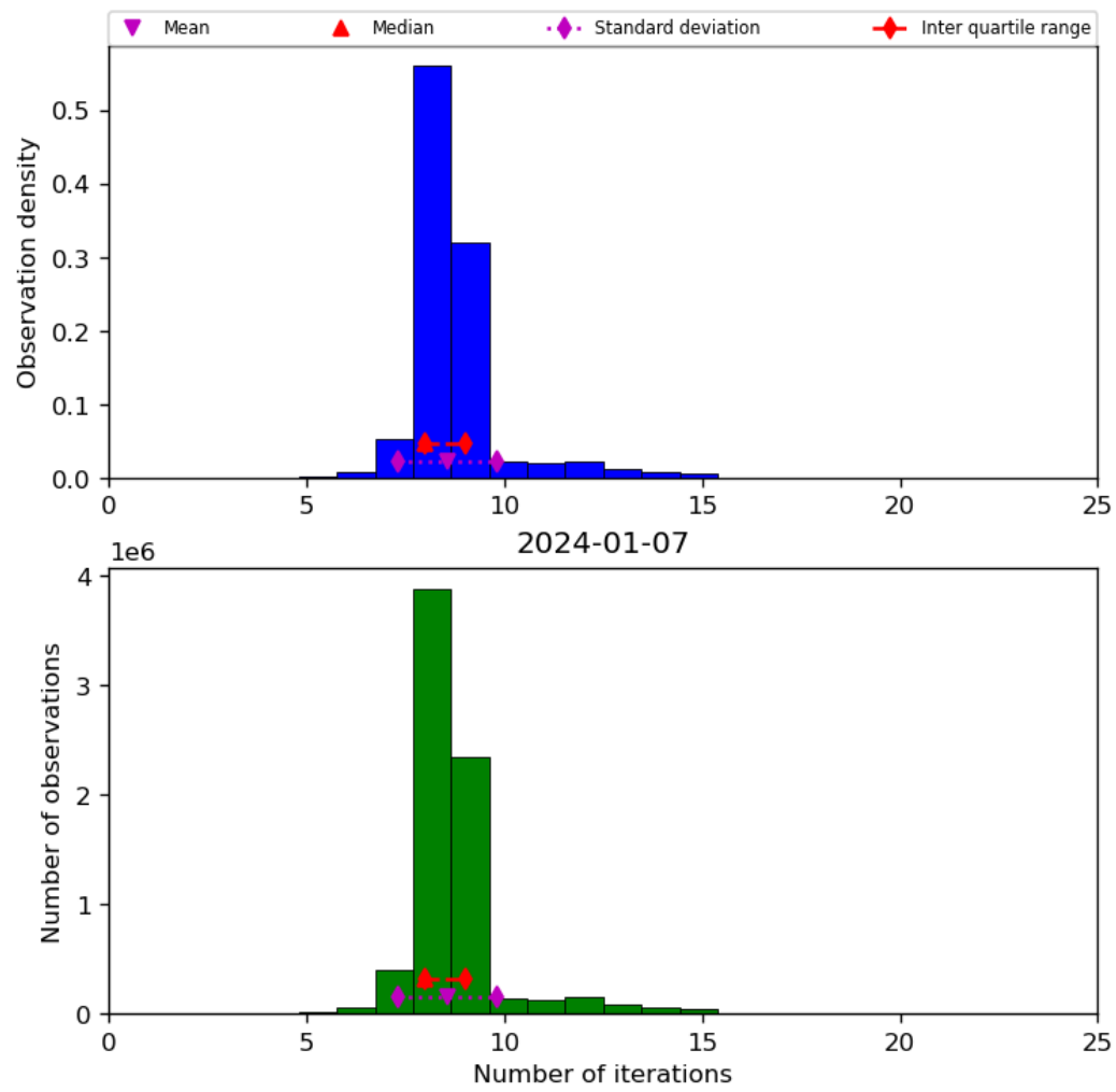
Figure 24: Histogram of “Number of iterations” for 2024-01-06 to 2024-01-08
