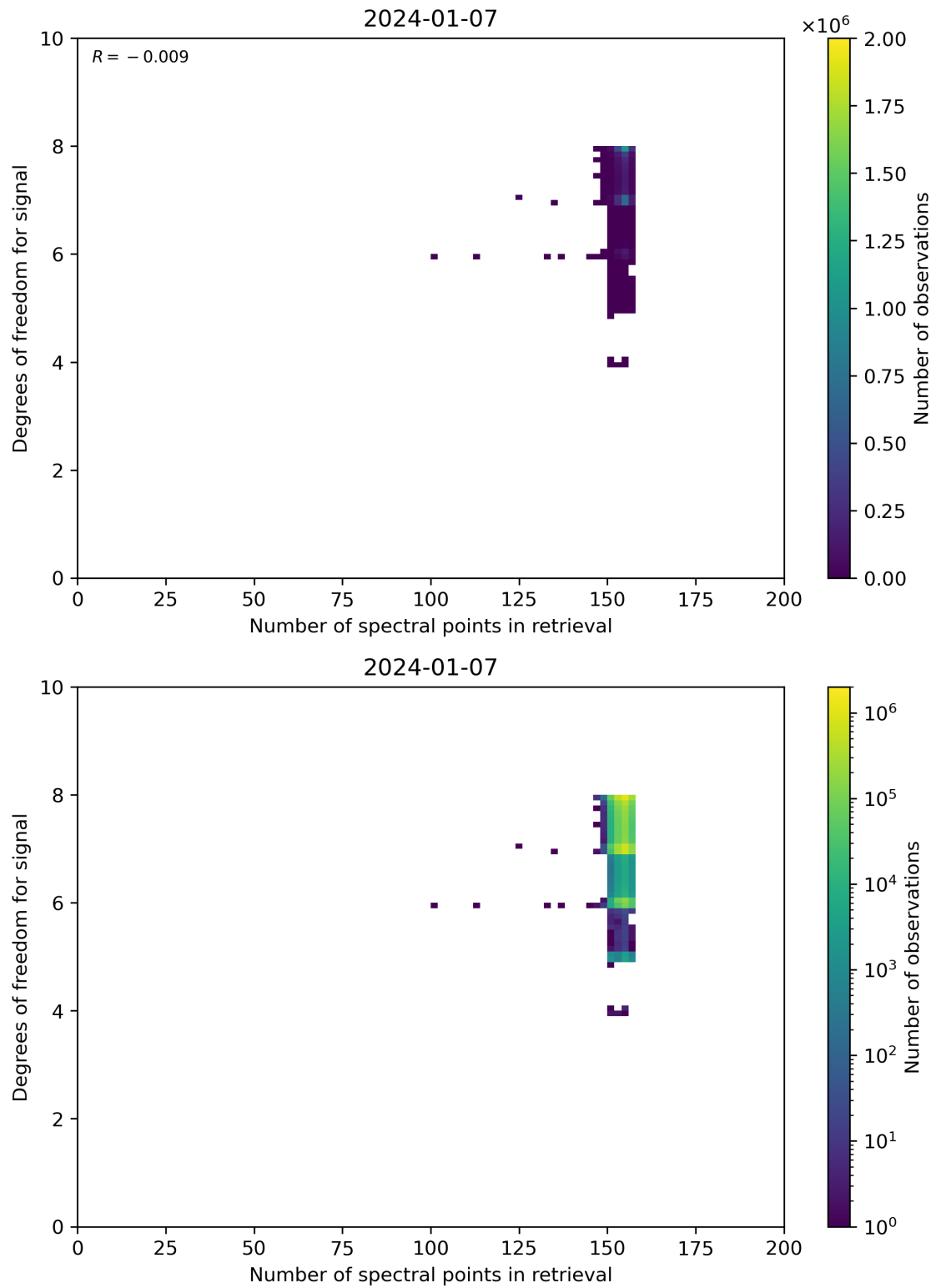
Figure 59: Scatter density plot of “Number of spectral points in retrieval” against “Degrees of freedom for signal” for 2024-01-06 to 2024-01-08.
