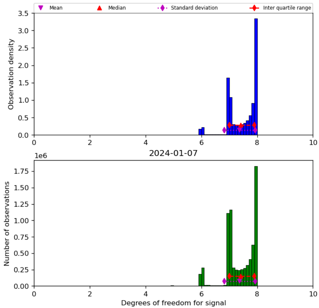
Figure 23: Histogram of “Degrees of freedom for signal” for 2024-01-06 to 2024-01-08
