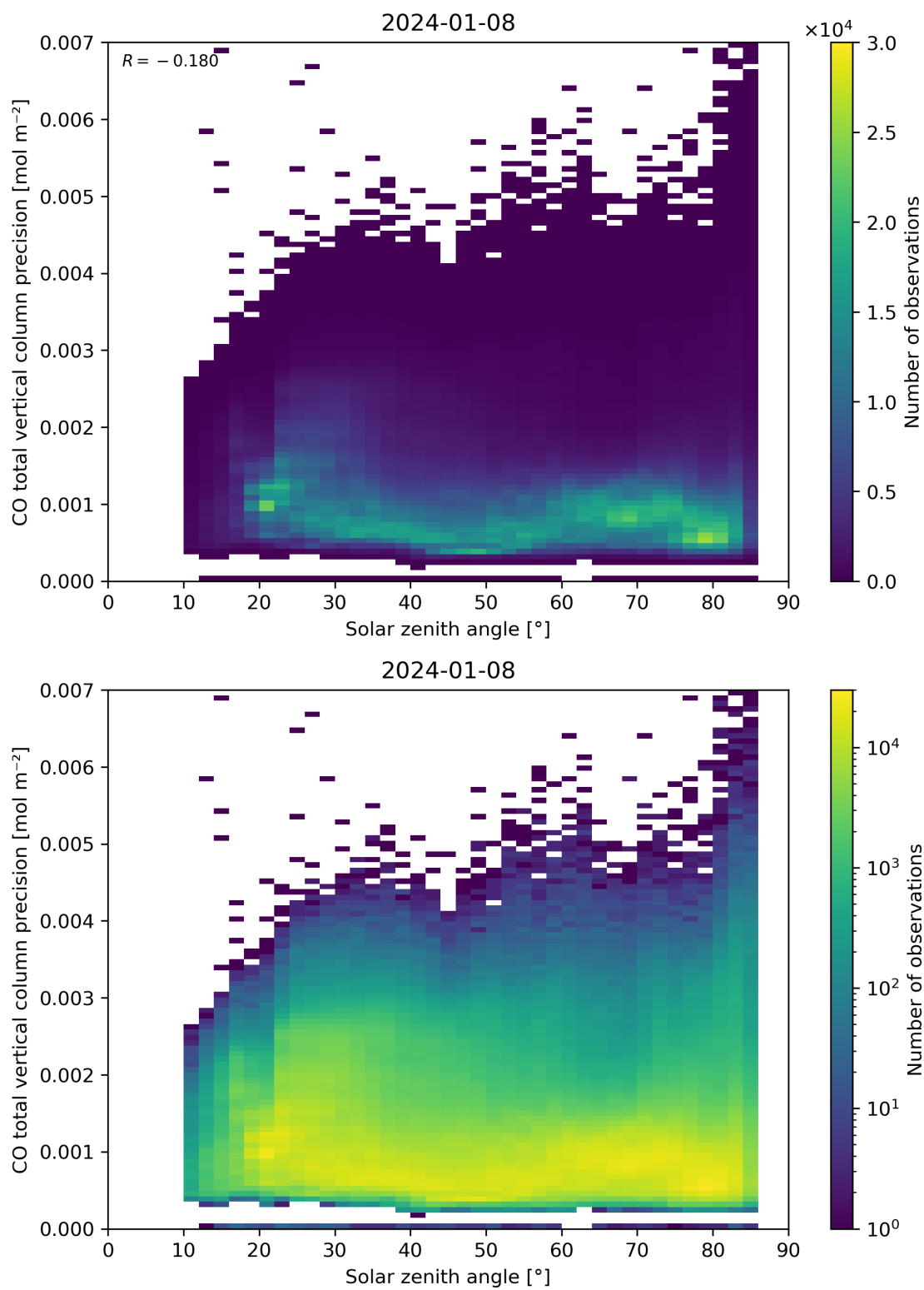
Figure 63: Scatter density plot of “Solar zenith angle” against “CO total vertical column precision” for 2024-01-07 to 2024-01-09.
