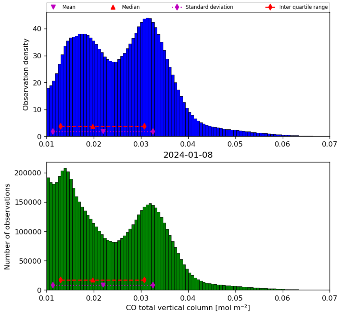
Figure 18: Histogram of “CO total vertical column” for 2024-01-07 to 2024-01-09
