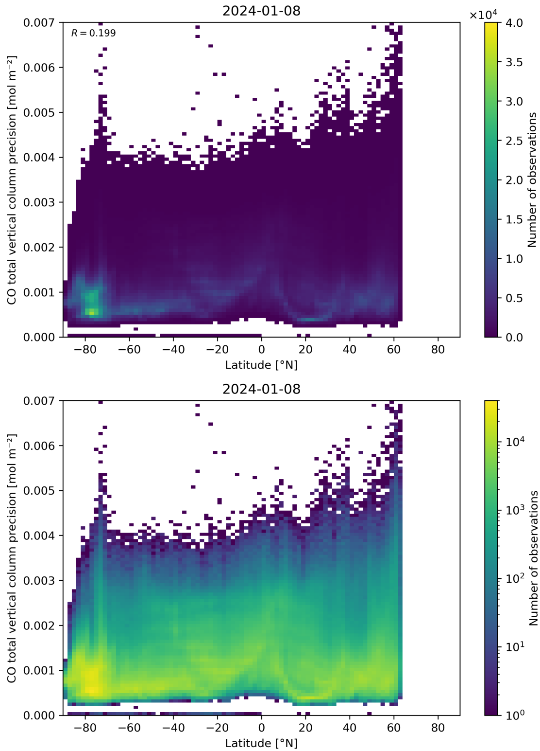
Figure 53: Scatter density plot of “Latitude” against “CO total vertical column precision” for 2024-01-07 to 2024-01-09.
