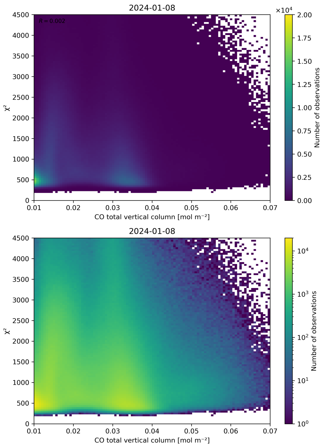
Figure 35: Scatter density plot of “CO total vertical column” against “ \chi^2 ” for 2024-01-07 to 2024-01-09.
