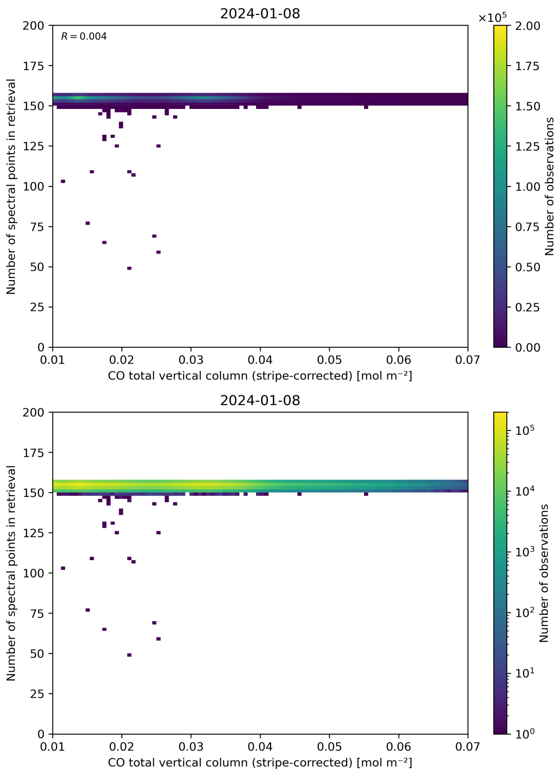
Figure 40: Scatter density plot of “CO total vertical column (stripe-corrected)” against “Number of spectral points in retrieval” for 2024-01-07 to 2024-01-09.
