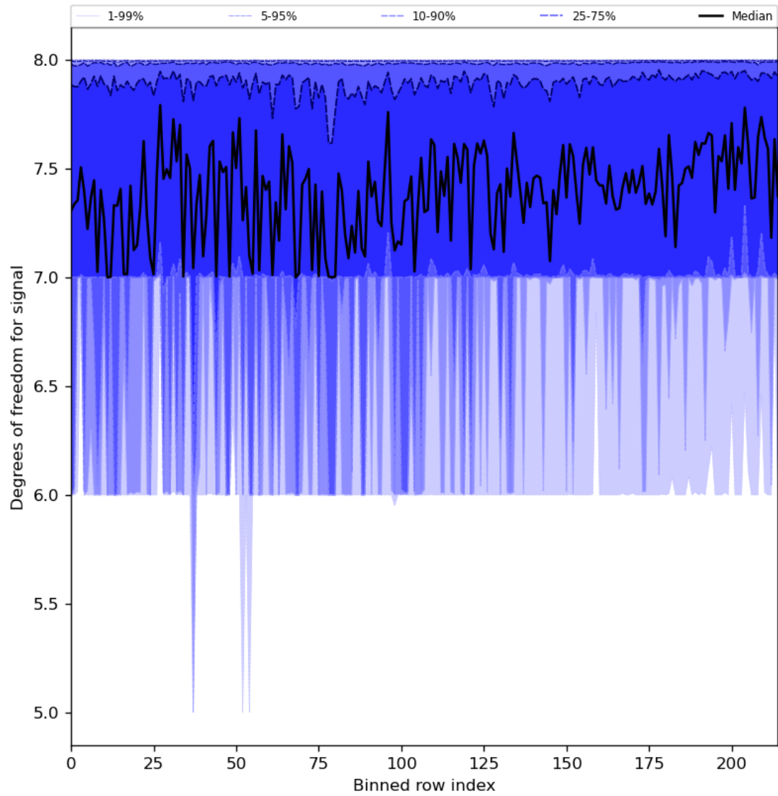
Figure 31: Along track statistics of “Degrees of freedom for signal” for 2024-01-07 to 2024-01-09
