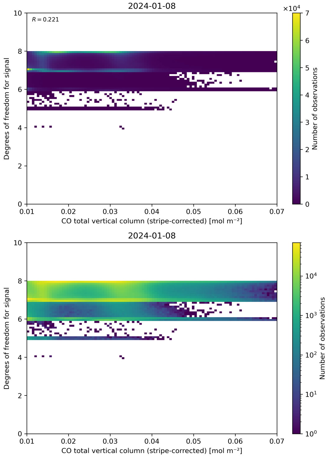
Figure 38: Scatter density plot of “CO total vertical column (stripe-corrected)” against “Degrees of freedom for signal” for 2024-01-07 to 2024-01-09.
