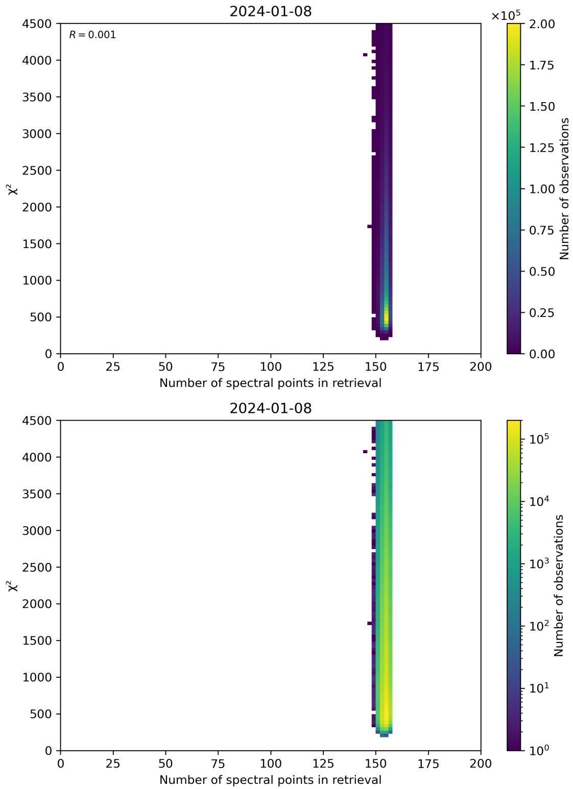
Figure 58: Scatter density plot of “Number of spectral points in retrieval” against “ \chi^2 ” for 2024-01-07 to 2024-01-09.
