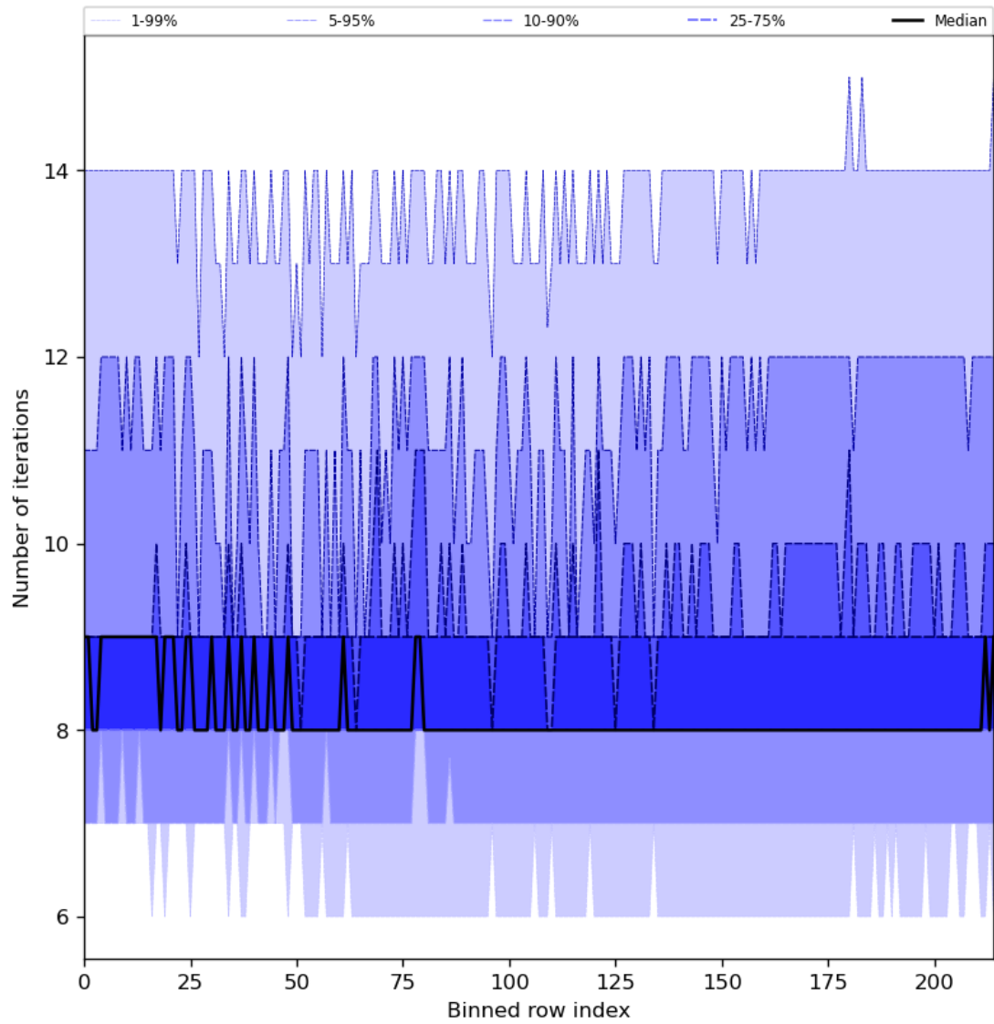
Figure 32: Along track statistics of “Number of iterations” for 2024-01-07 to 2024-01-09
