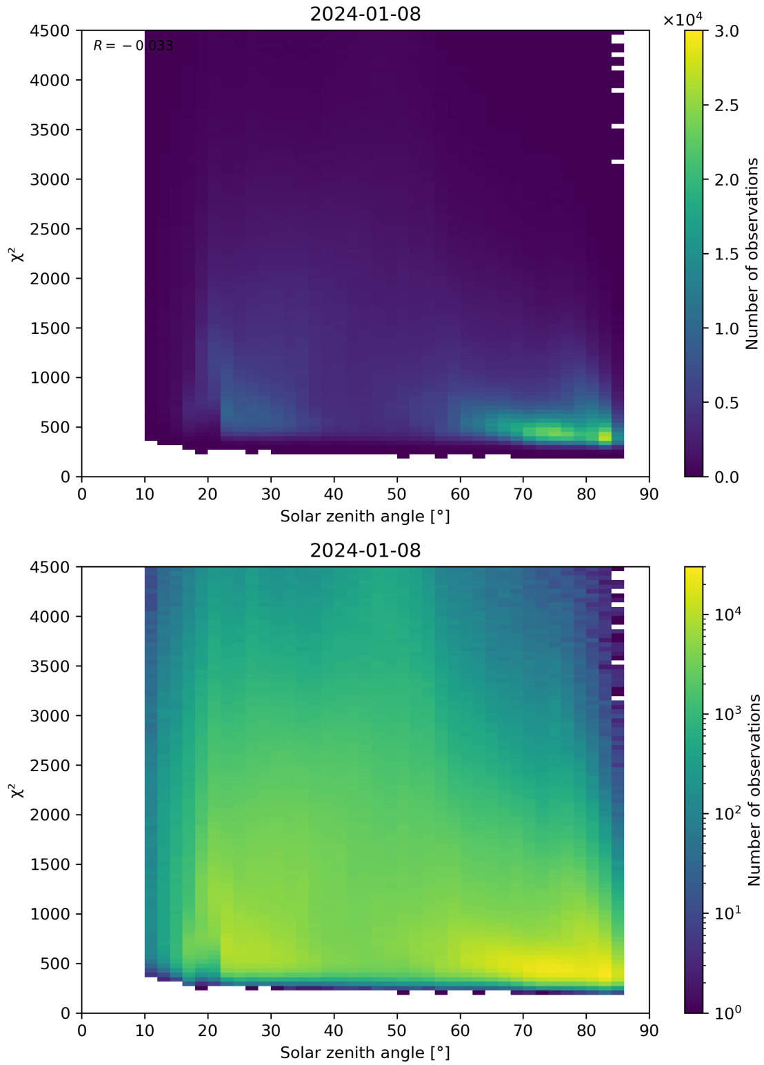
Figure 64: Scatter density plot of “Solar zenith angle” against “ \chi^2 ” for 2024-01-07 to 2024-01-09.
