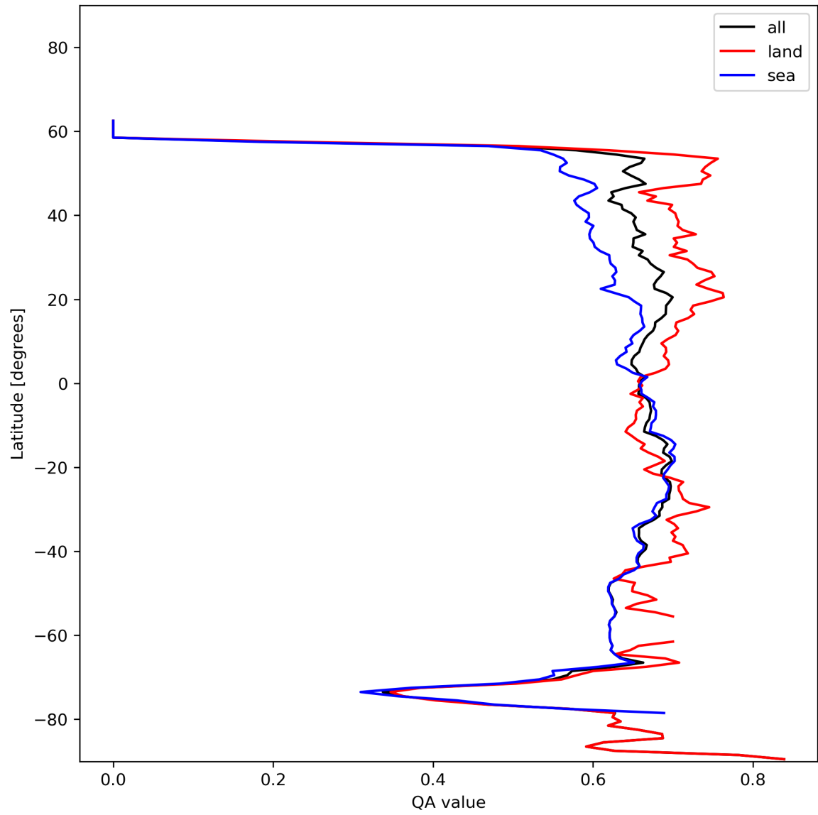
Figure 9: Zonal average of “QA value” for 2024-01-07 to 2024-01-09.
