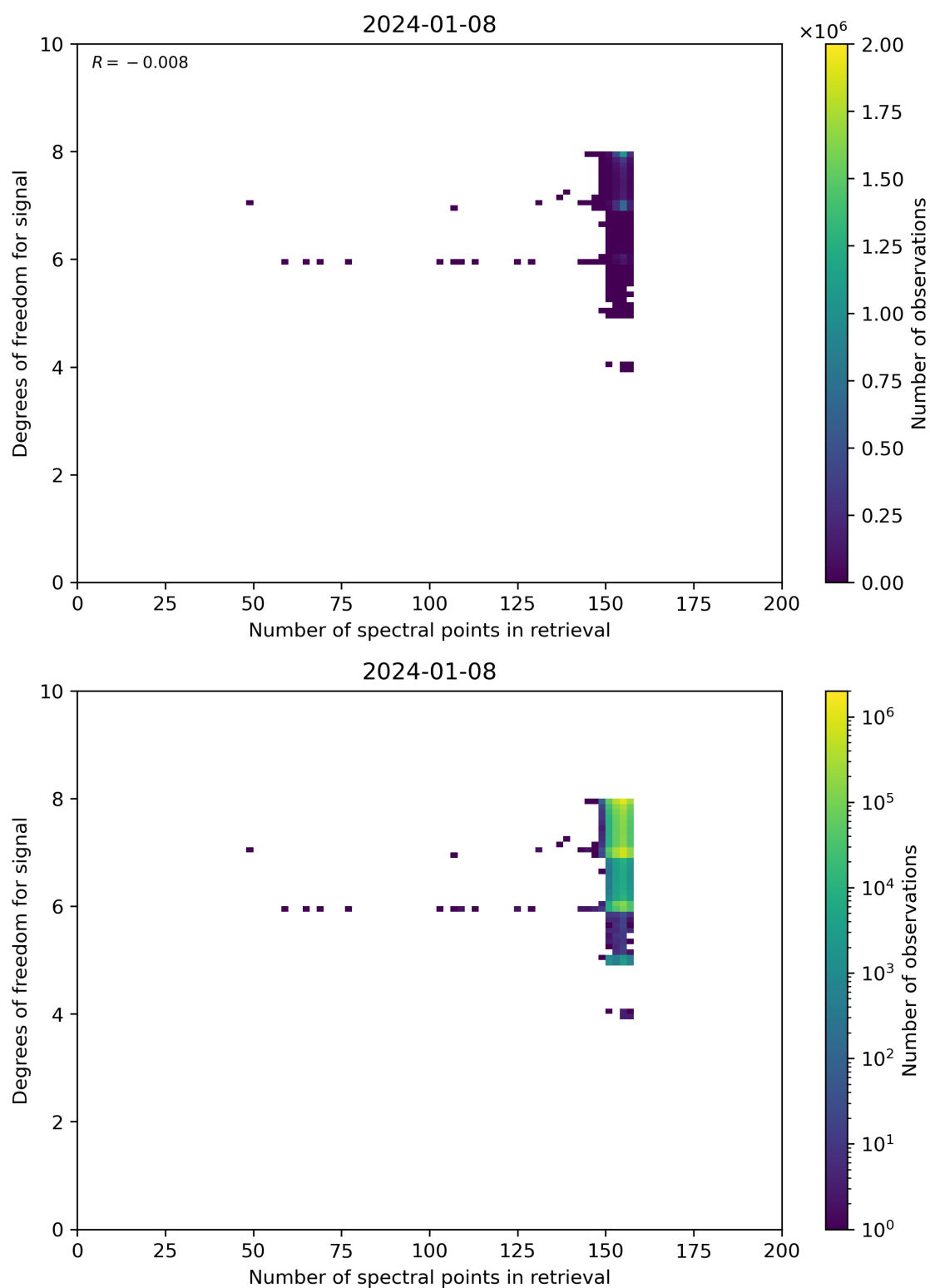
Figure 59: Scatter density plot of “Number of spectral points in retrieval” against “Degrees of freedom for signal” for 2024-01-07 to 2024-01-09.
