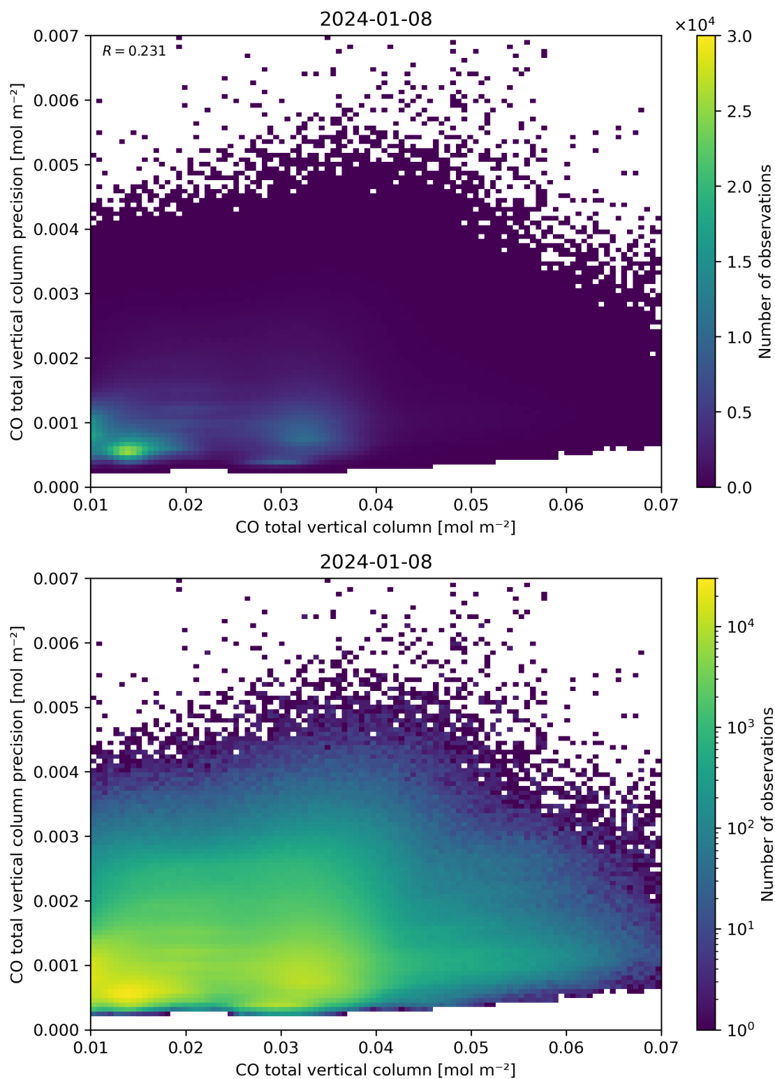
Figure 34: Scatter density plot of “CO total vertical column” against “CO total vertical column precision” for 2024-01-07 to 2024-01-09.
