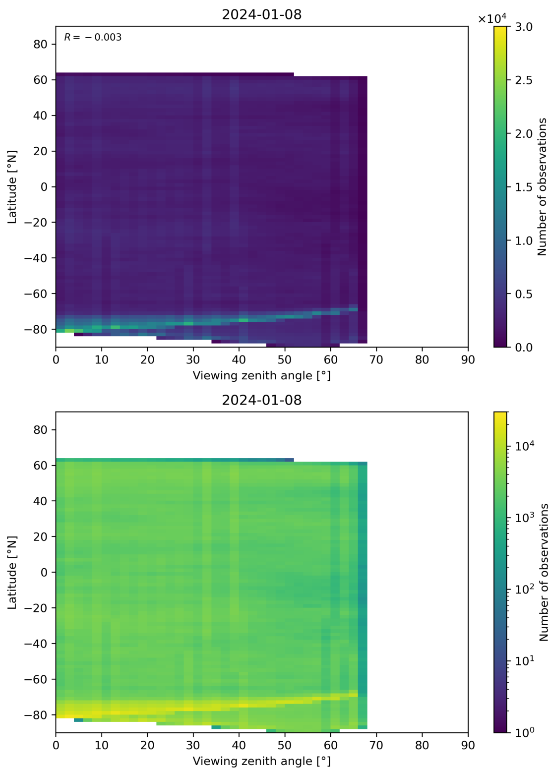
Figure 74: Scatter density plot of “Viewing zenith angle” against “Latitude” for 2024-01-07 to 2024-01-09.
