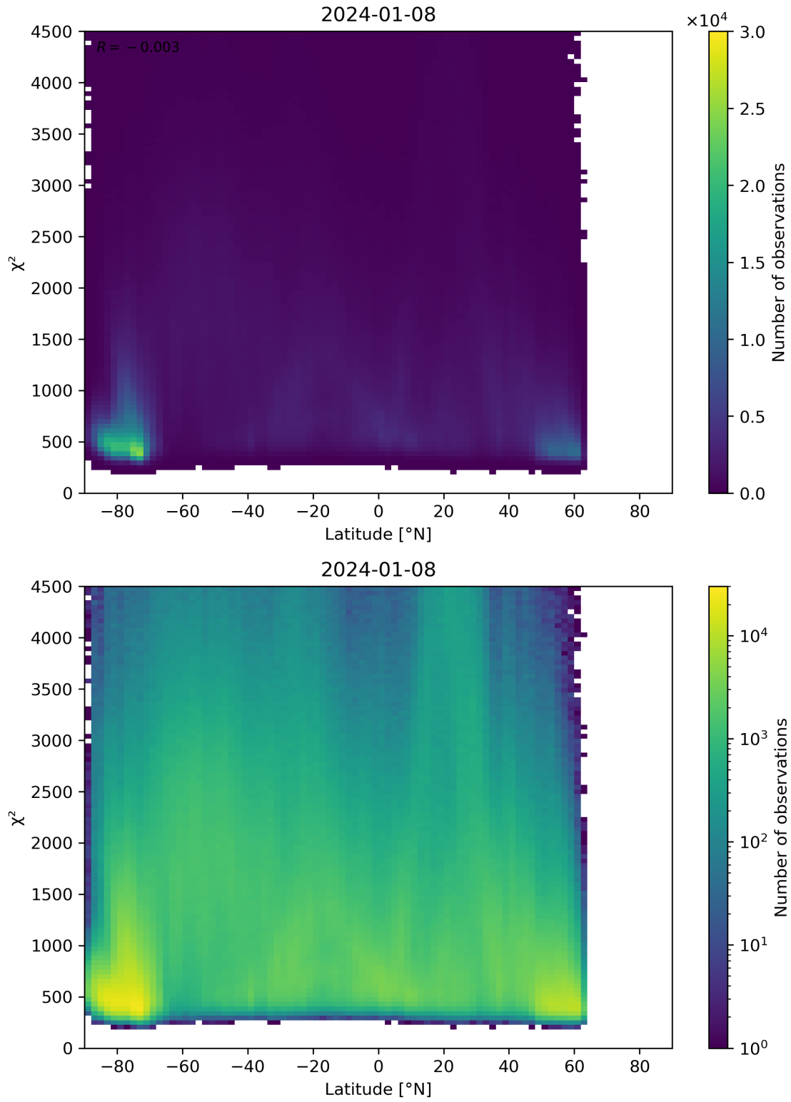
Figure 54: Scatter density plot of “Latitude” against “ \chi^2 ” for 2024-01-07 to 2024-01-09.
