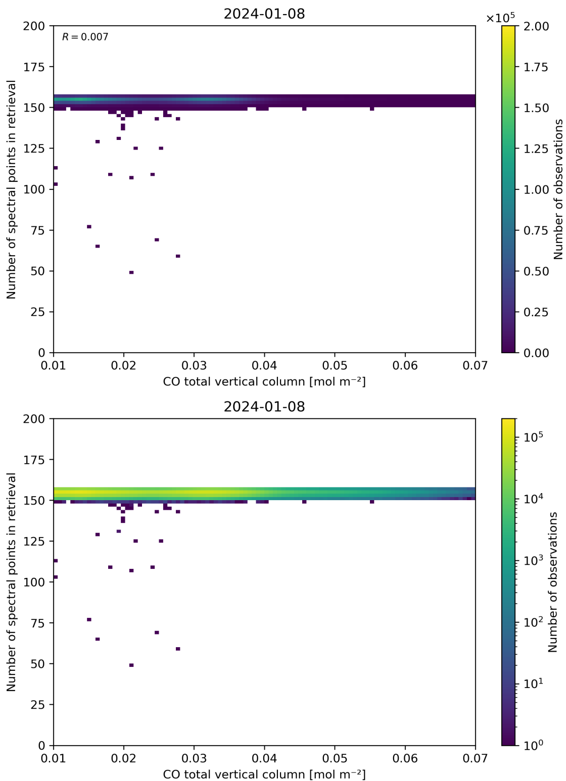
Figure 43: Scatter density plot of “CO total vertical column” against “Number of spectral points in retrieval” for 2024-01-07 to 2024-01-09.
