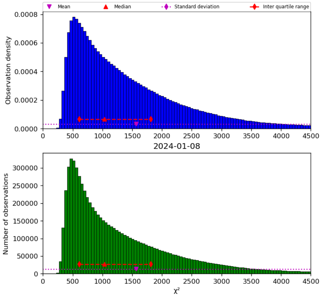
Figure 22: Histogram of “ \chi^2 ” for 2024-01-07 to 2024-01-09
