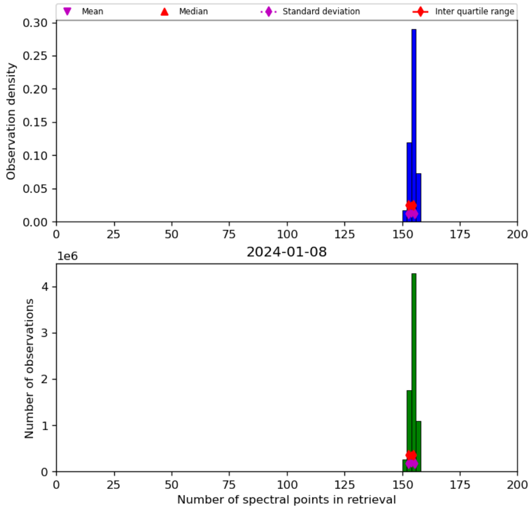
Figure 21: Histogram of “Number of spectral points in retrieval” for 2024-01-07 to 2024-01-09
