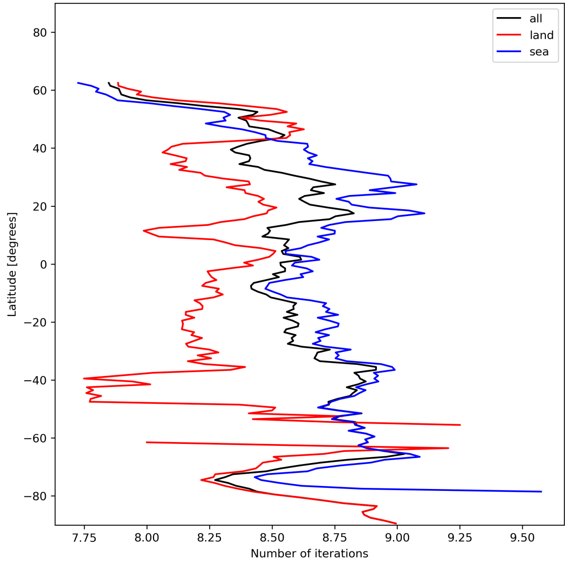
Figure 16: Zonal average of “Number of iterations” for 2024-01-07 to 2024-01-09.
