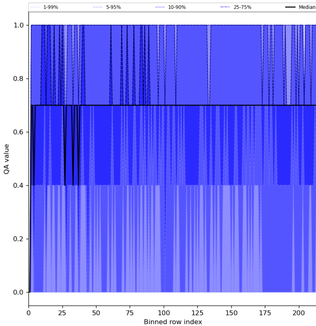
Figure 25: Along track statistics of “QA value” for 2024-01-07 to 2024-01-09
