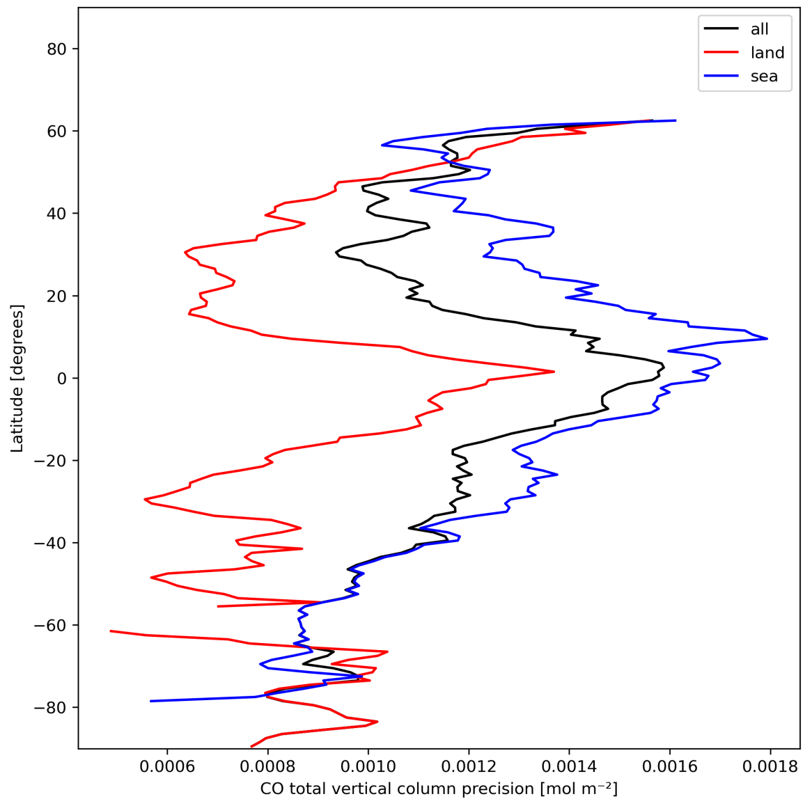
Figure 12: Zonal average of “CO total vertical column precision” for 2024-01-07 to 2024-01-09.
