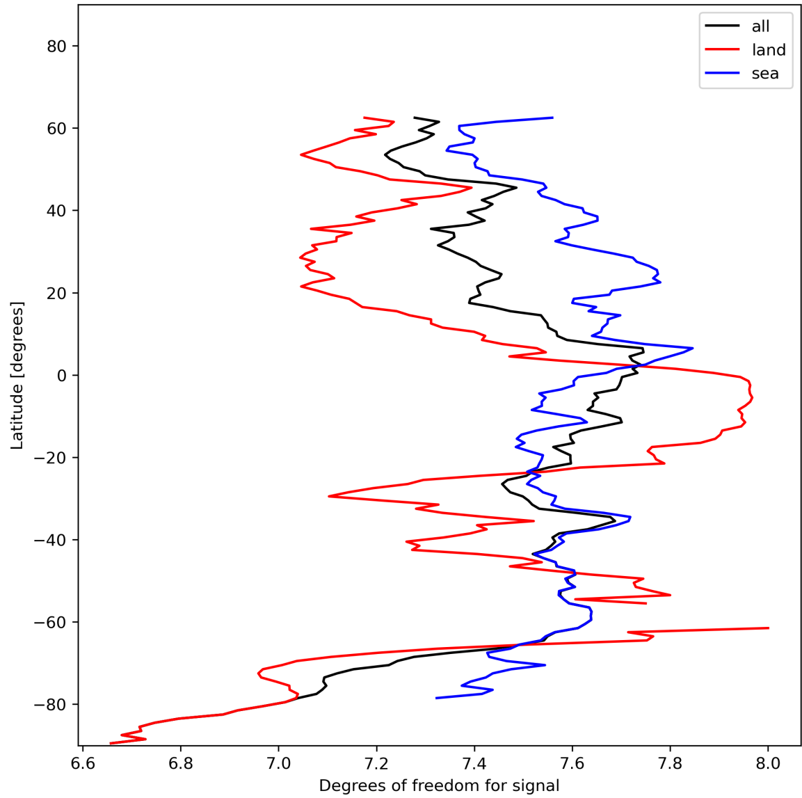
Figure 15: Zonal average of “Degrees of freedom for signal” for 2024-01-07 to 2024-01-09.
