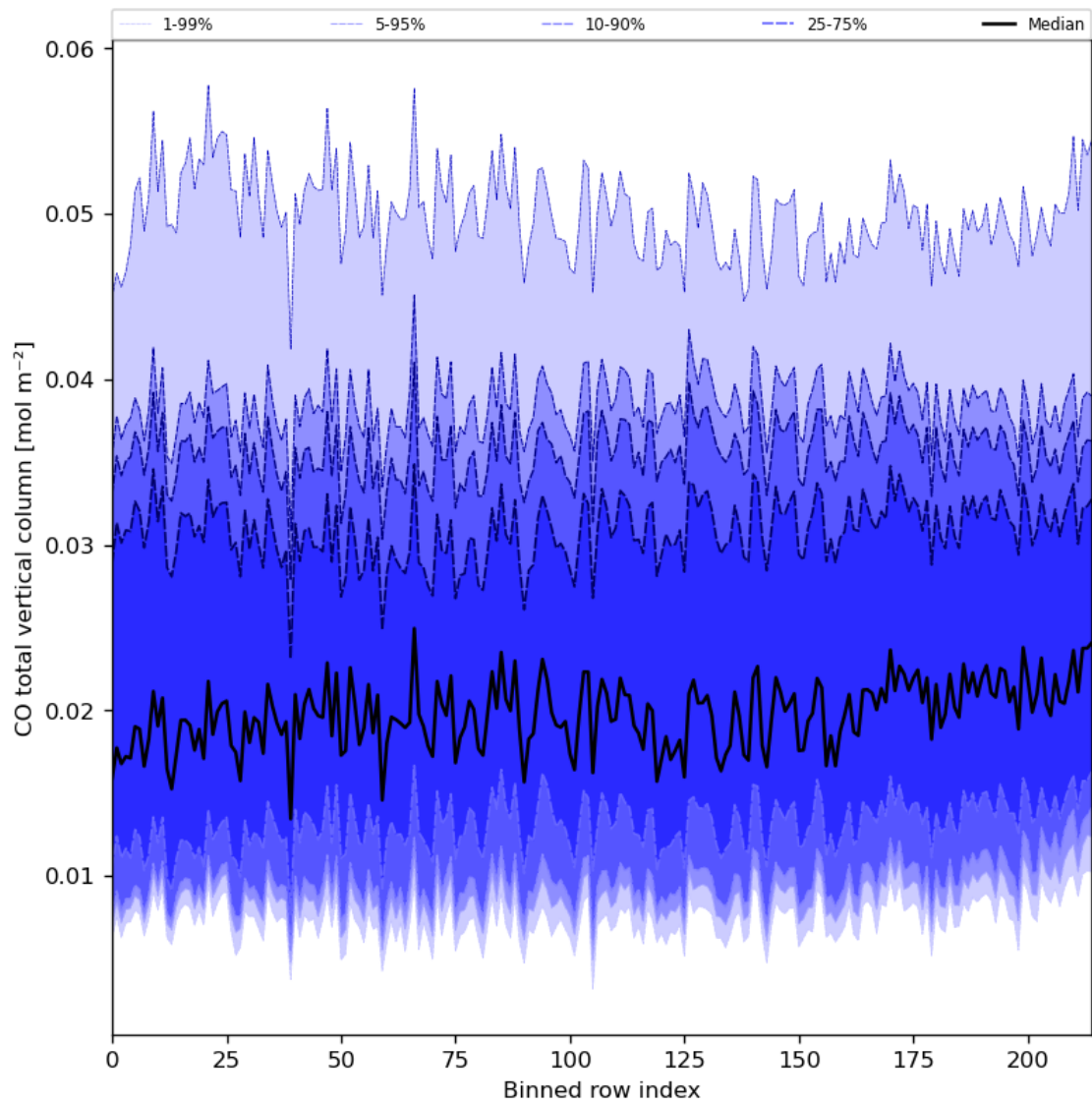
Figure 26: Along track statistics of “CO total vertical column” for 2024-01-07 to 2024-01-09
