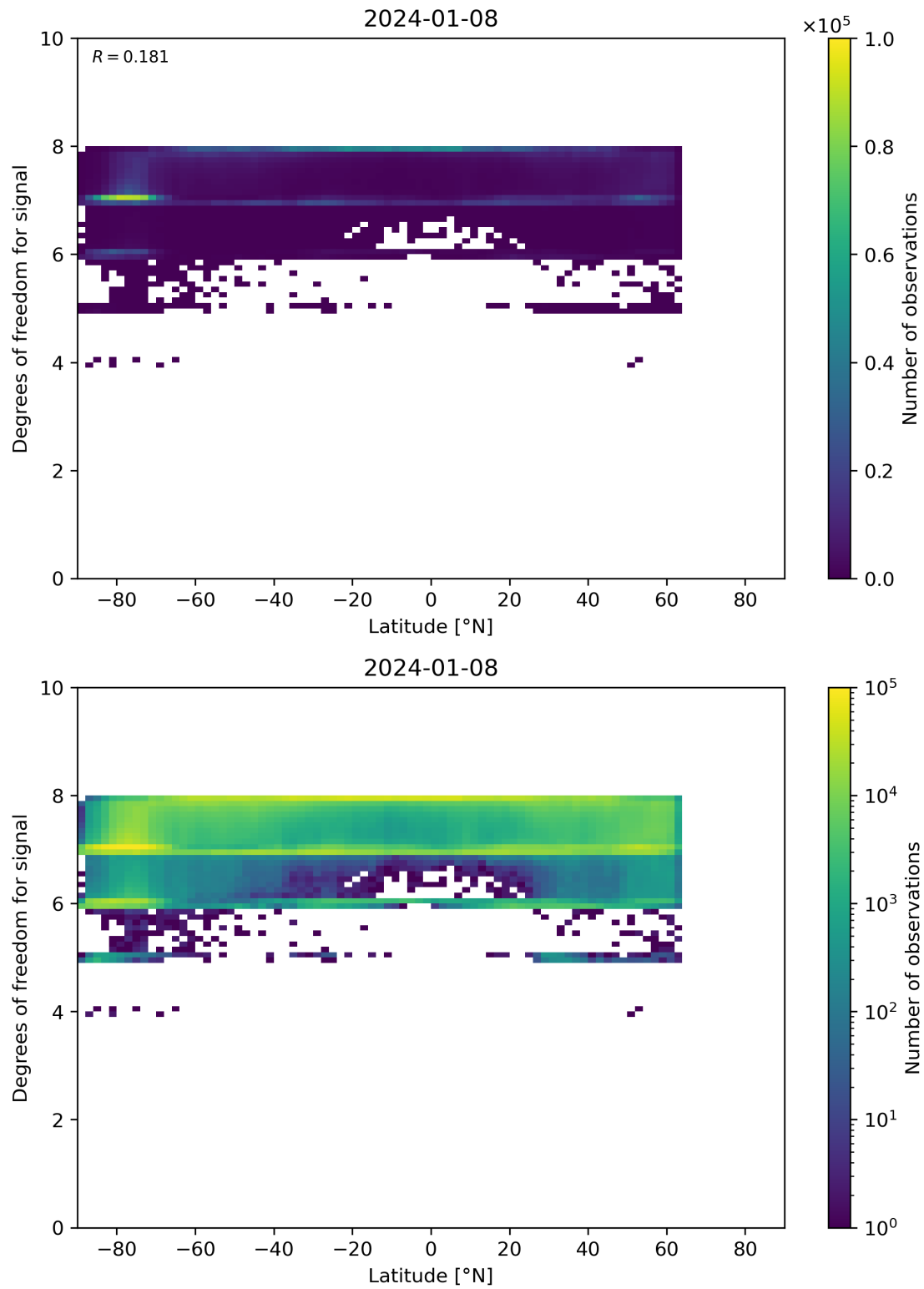
Figure 55: Scatter density plot of “Latitude” against “Degrees of freedom for signal” for 2024-01-07 to 2024-01-09.
