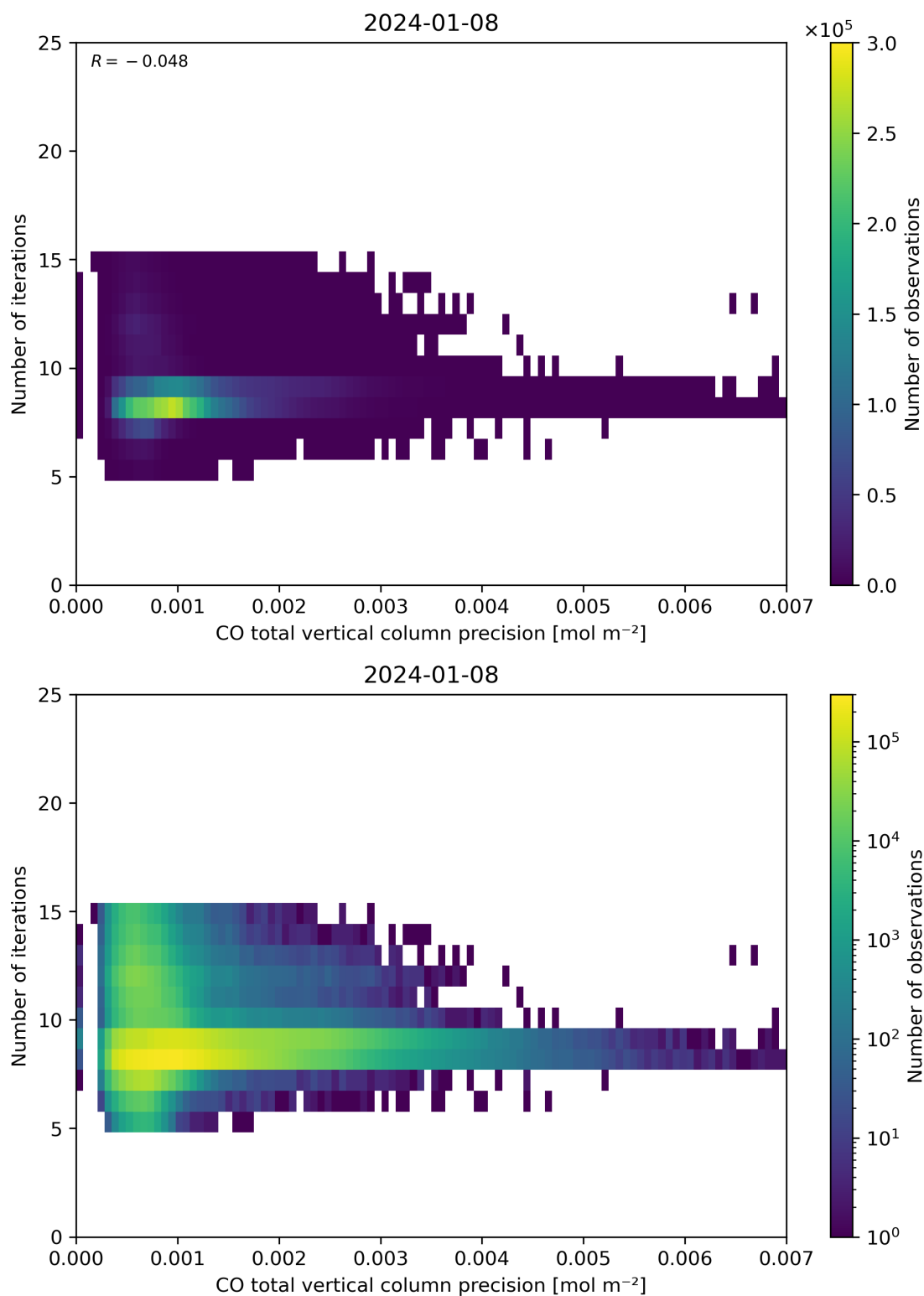
Figure 46: Scatter density plot of “CO total vertical column precision” against “Number of iterations” for 2024-01-07 to 2024-01-09.
