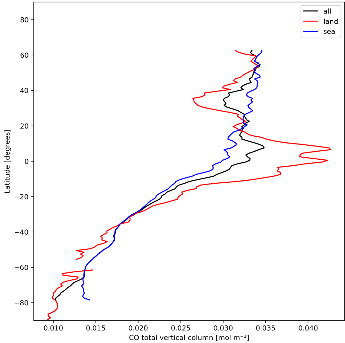
Figure 10: Zonal average of “CO total vertical column” for 2024-01-07 to 2024-01-09.
