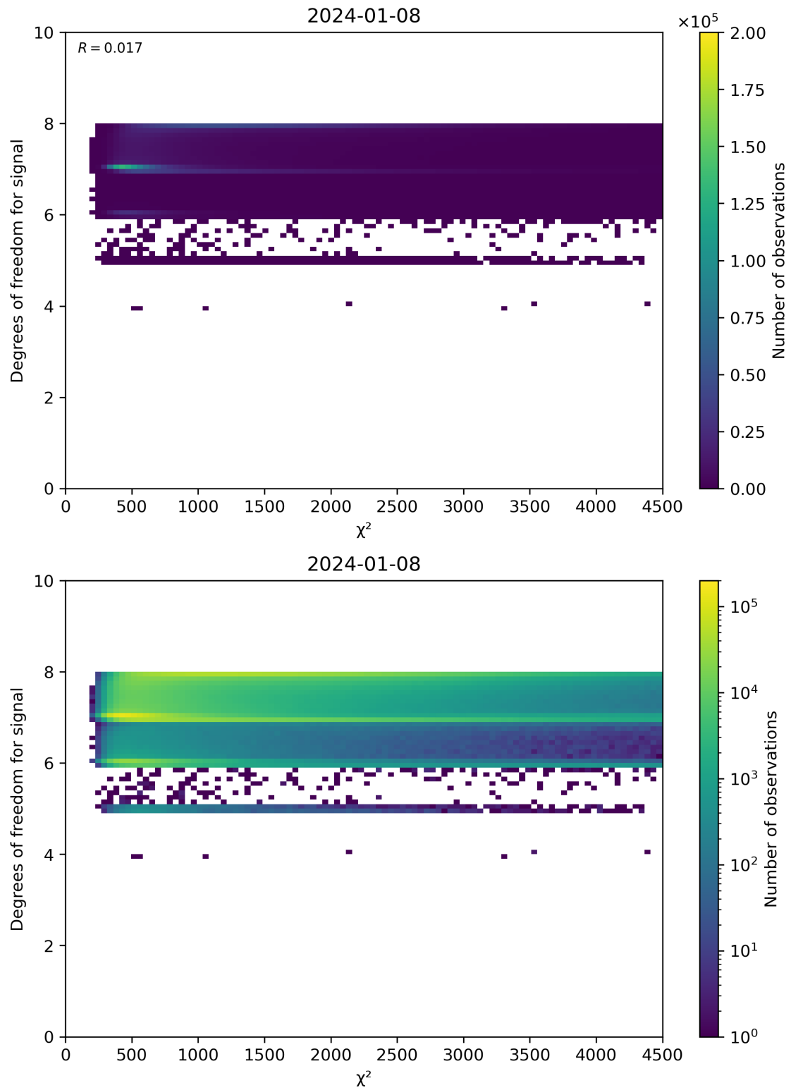
Figure 48: Scatter density plot of “ \chi^2 ” against “Degrees of freedom for signal” for 2024-01-07 to 2024-01-09.
