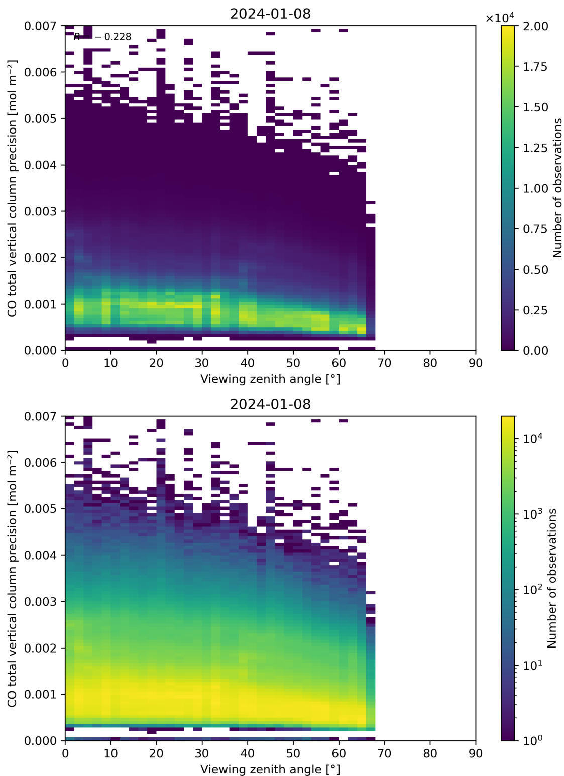
Figure 71: Scatter density plot of “Viewing zenith angle” against “CO total vertical column precision” for 2024-01-07 to 2024-01-09.
