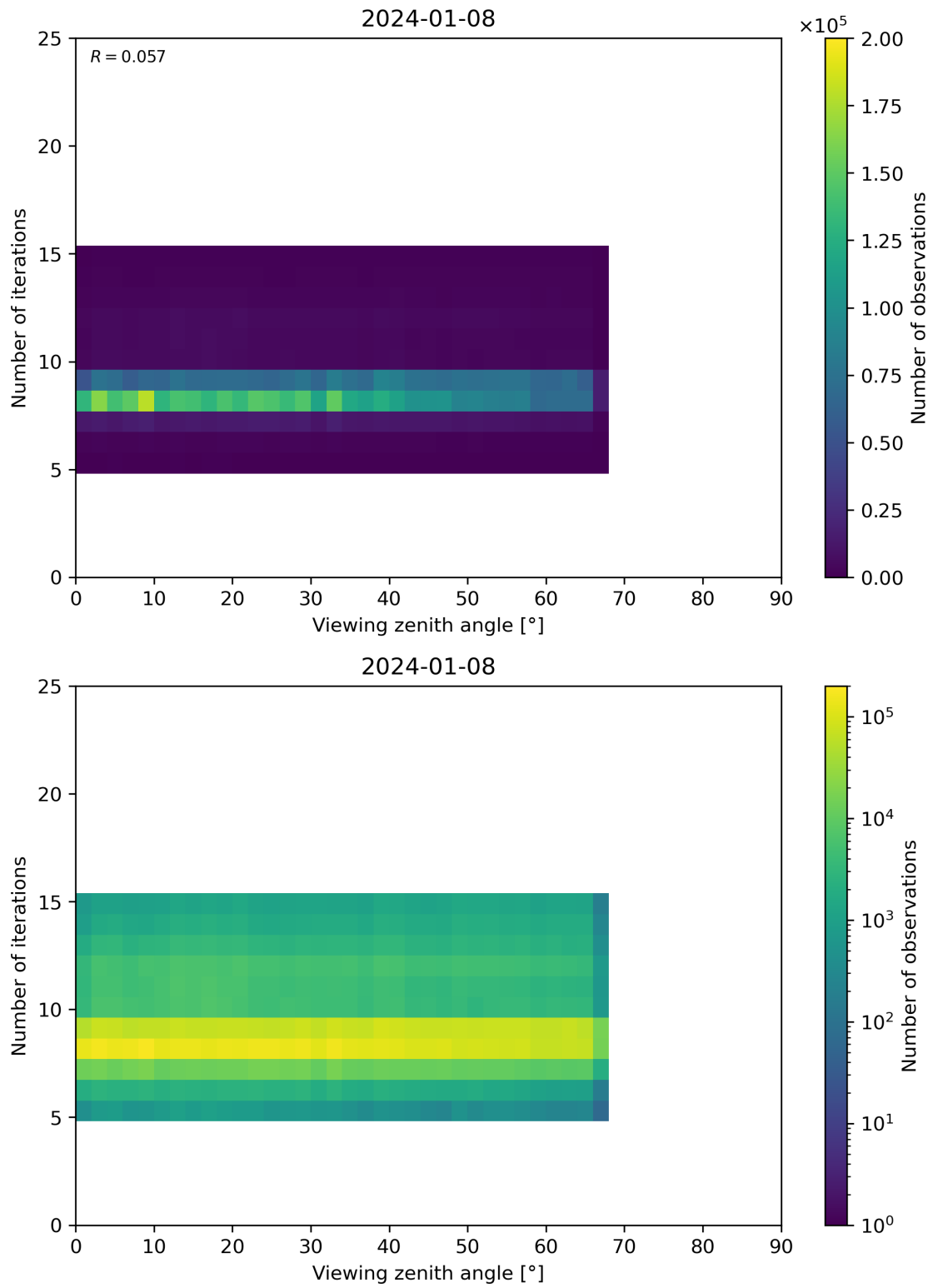
Figure 75: Scatter density plot of “Viewing zenith angle” against “Number of iterations” for 2024-01-07 to 2024-01-09.
