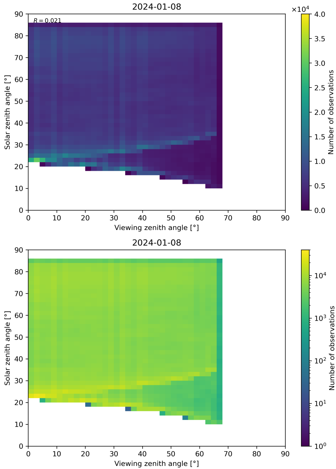
Figure 77: Scatter density plot of “Viewing zenith angle” against “Solar zenith angle” for 2024-01-07 to 2024-01-09.
