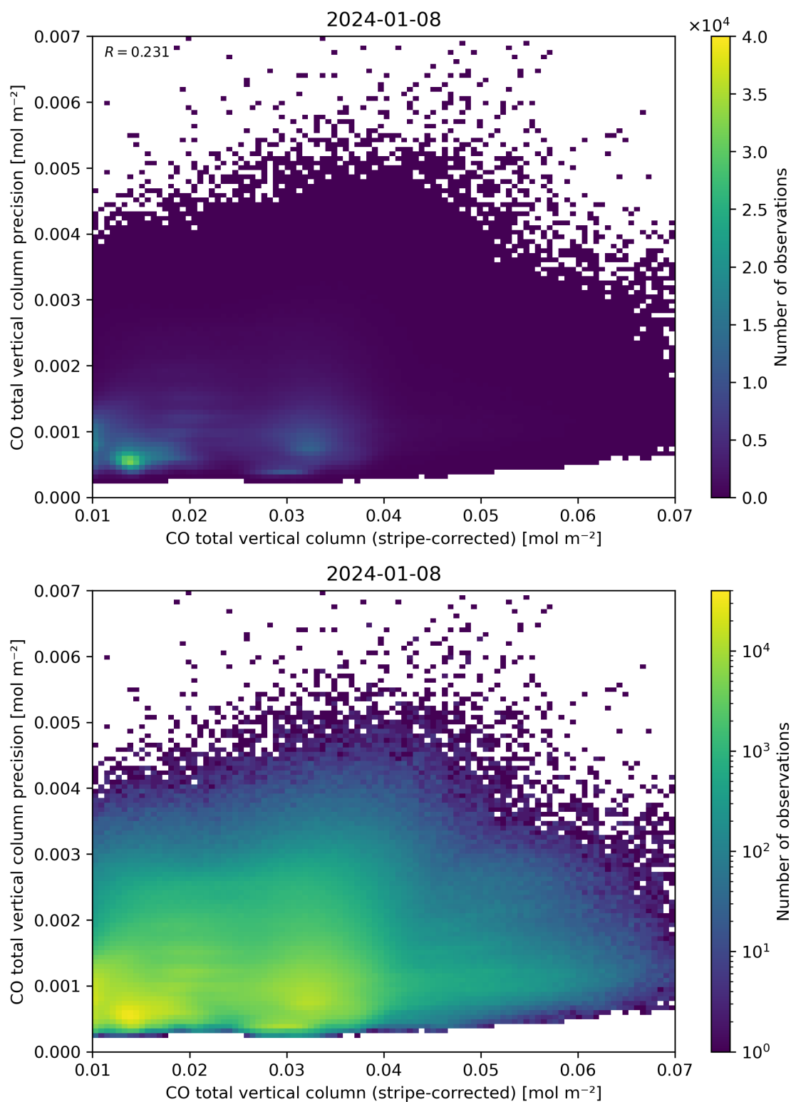
Figure 36: Scatter density plot of “CO total vertical column (stripe-corrected)” against “CO total vertical column precision” for 2024-01-07 to 2024-01-09.
