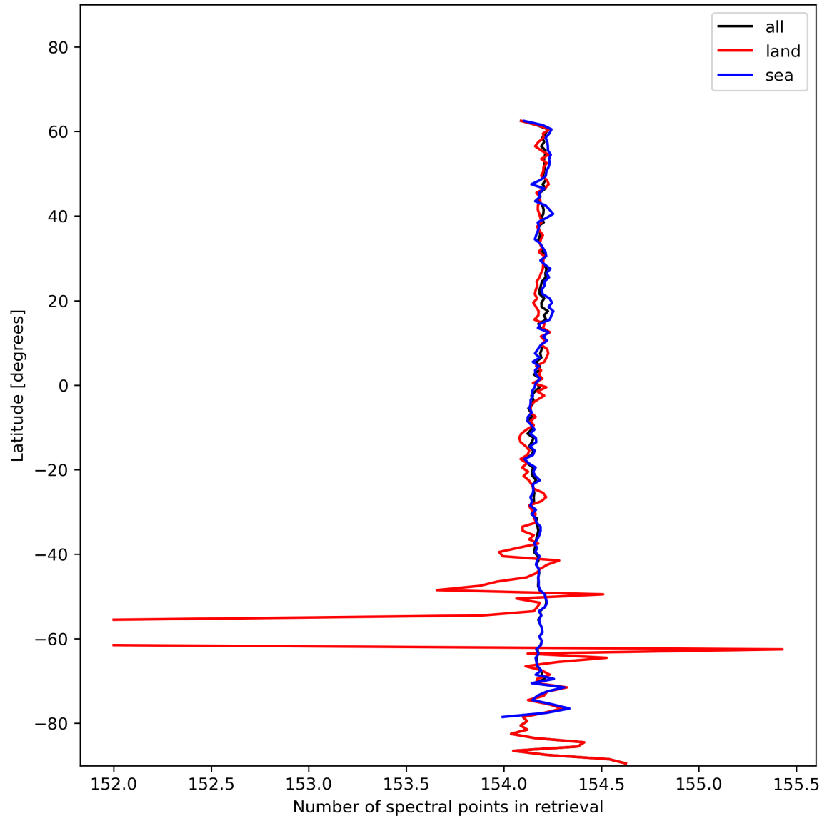
Figure 13: Zonal average of “Number of spectral points in retrieval” for 2024-01-07 to 2024-01-09.
