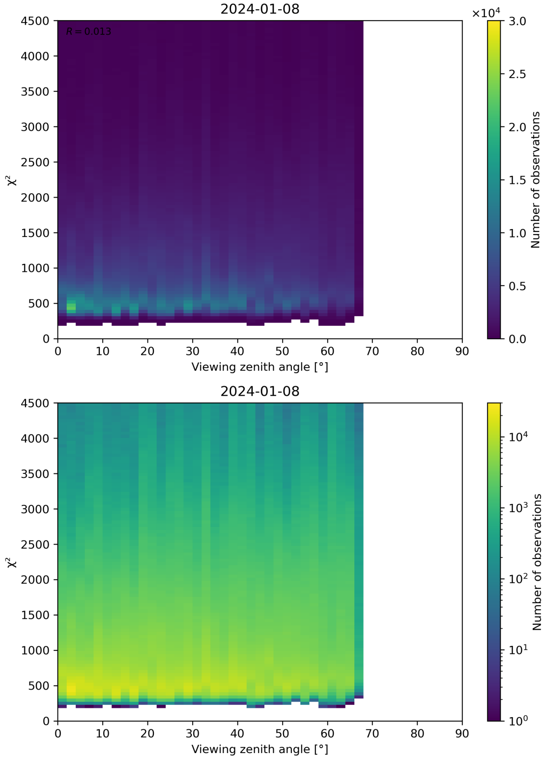
Figure 72: Scatter density plot of “Viewing zenith angle” against “ \chi^2 ” for 2024-01-07 to 2024-01-09.
