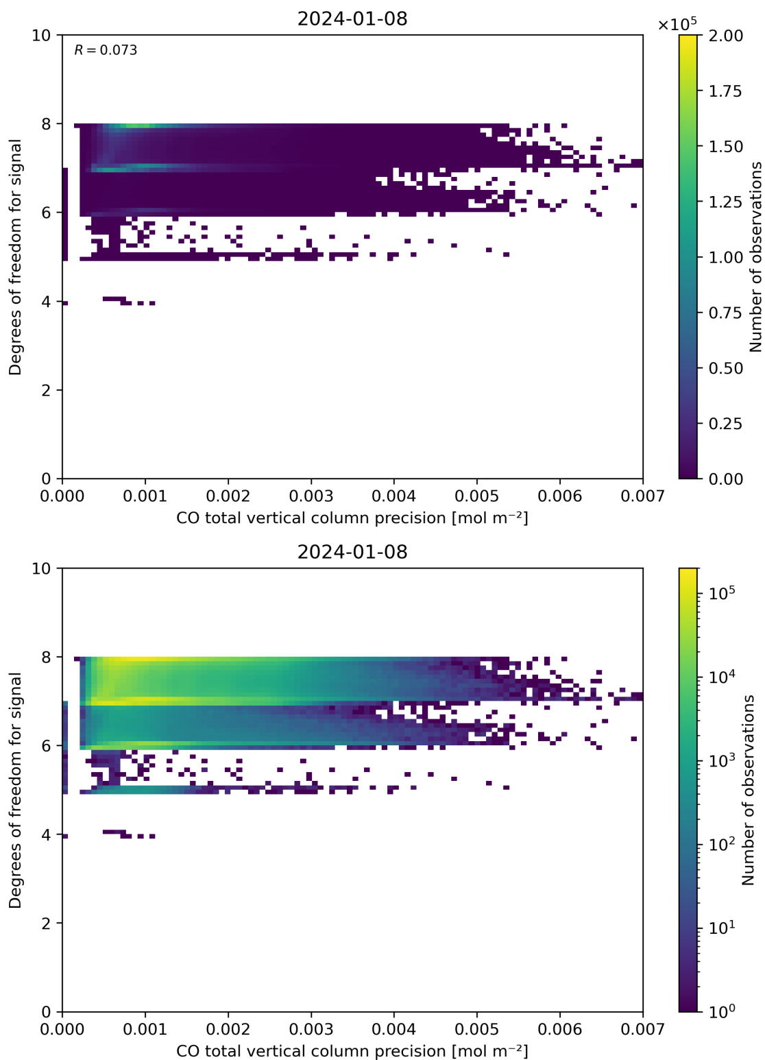
Figure 45: Scatter density plot of “CO total vertical column precision” against “Degrees of freedom for signal” for 2024-01-07 to 2024-01-09.
