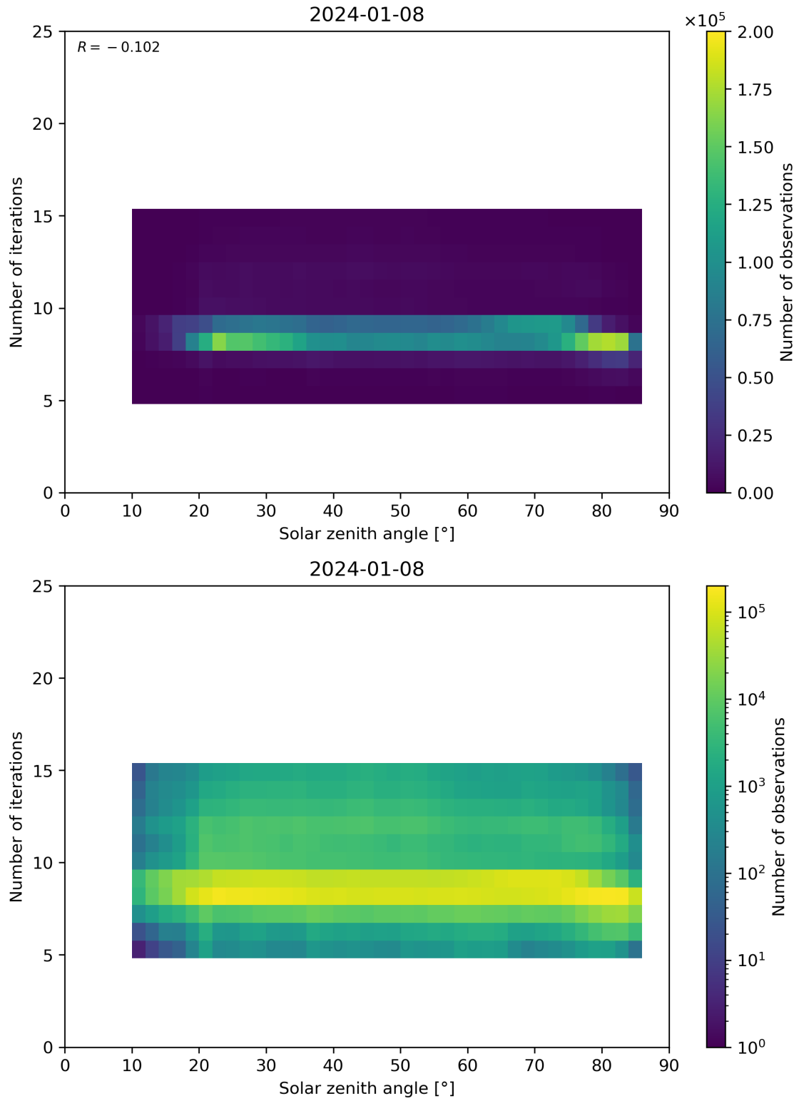
Figure 67: Scatter density plot of “Solar zenith angle” against “Number of iterations” for 2024-01-07 to 2024-01-09.
