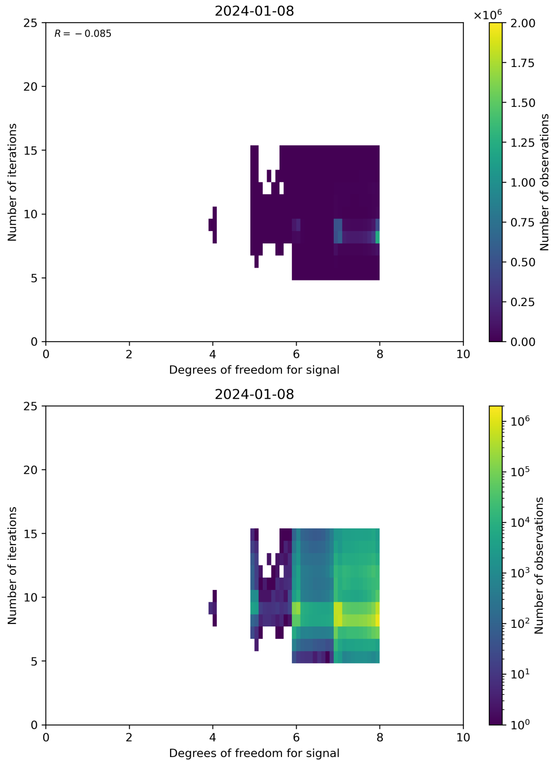
Figure 50: Scatter density plot of “Degrees of freedom for signal” against “Number of iterations” for 2024-01-07 to 2024-01-09.
