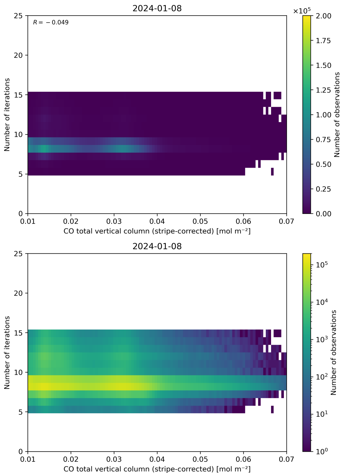
Figure 39: Scatter density plot of “CO total vertical column (stripe-corrected)” against “Number of iterations” for 2024-01-07 to 2024-01-09.
