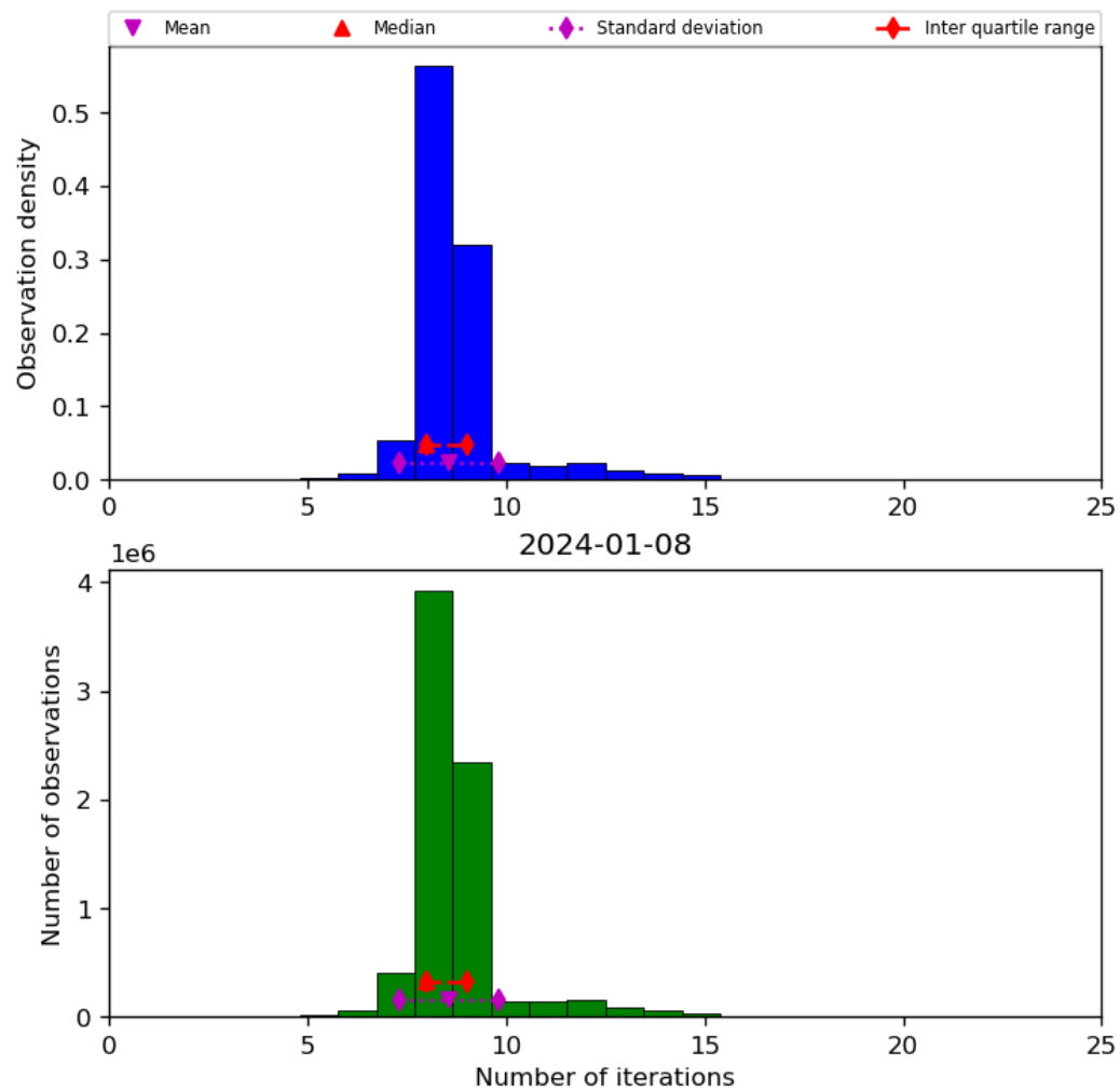
Figure 24: Histogram of “Number of iterations” for 2024-01-07 to 2024-01-09
