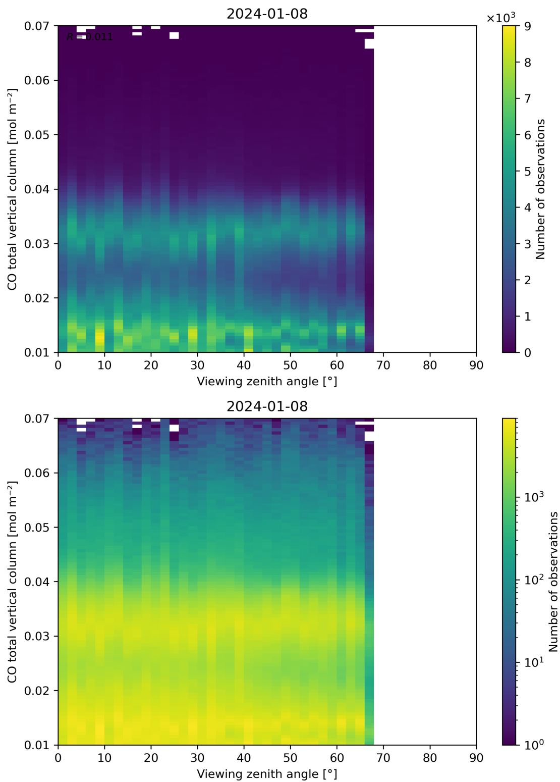
Figure 69: Scatter density plot of “Viewing zenith angle” against “CO total vertical column” for 2024-01-07 to 2024-01-09.
