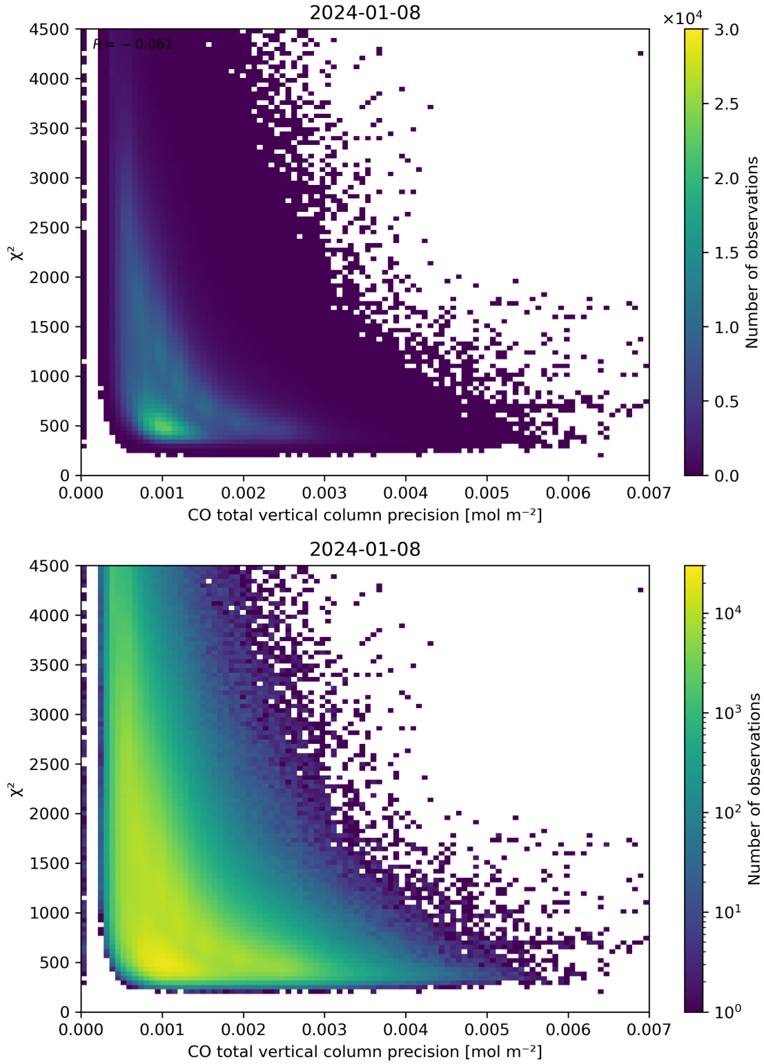
Figure 44: Scatter density plot of “CO total vertical column precision” against “ \chi^2 ” for 2024-01-07 to 2024-01-09.
