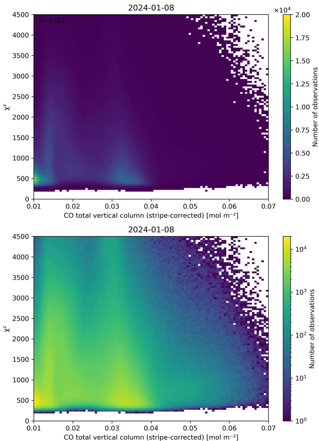
Figure 37: Scatter density plot of “CO total vertical column (stripe-corrected)” against “ \chi^2 ” for 2024-01-07 to 2024-01-09.
