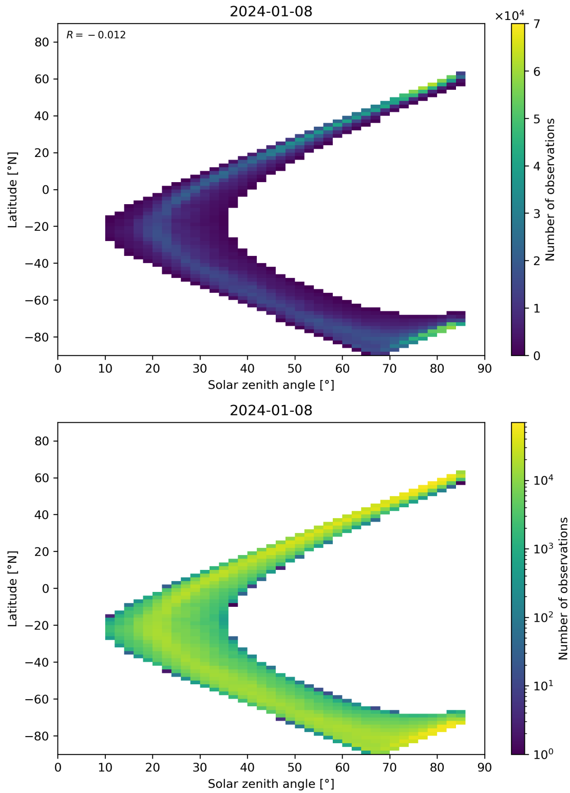
Figure 66: Scatter density plot of “Solar zenith angle” against “Latitude” for 2024-01-07 to 2024-01-09.
