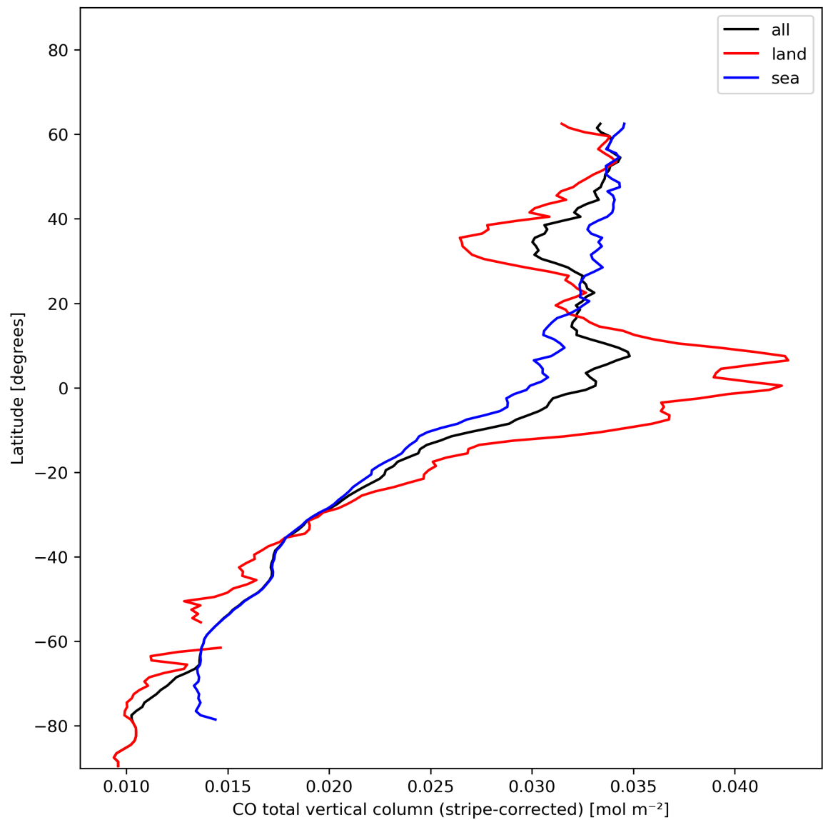
Figure 11: Zonal average of “CO total vertical column (stripe-corrected)” for 2024-01-07 to 2024-01-09.
