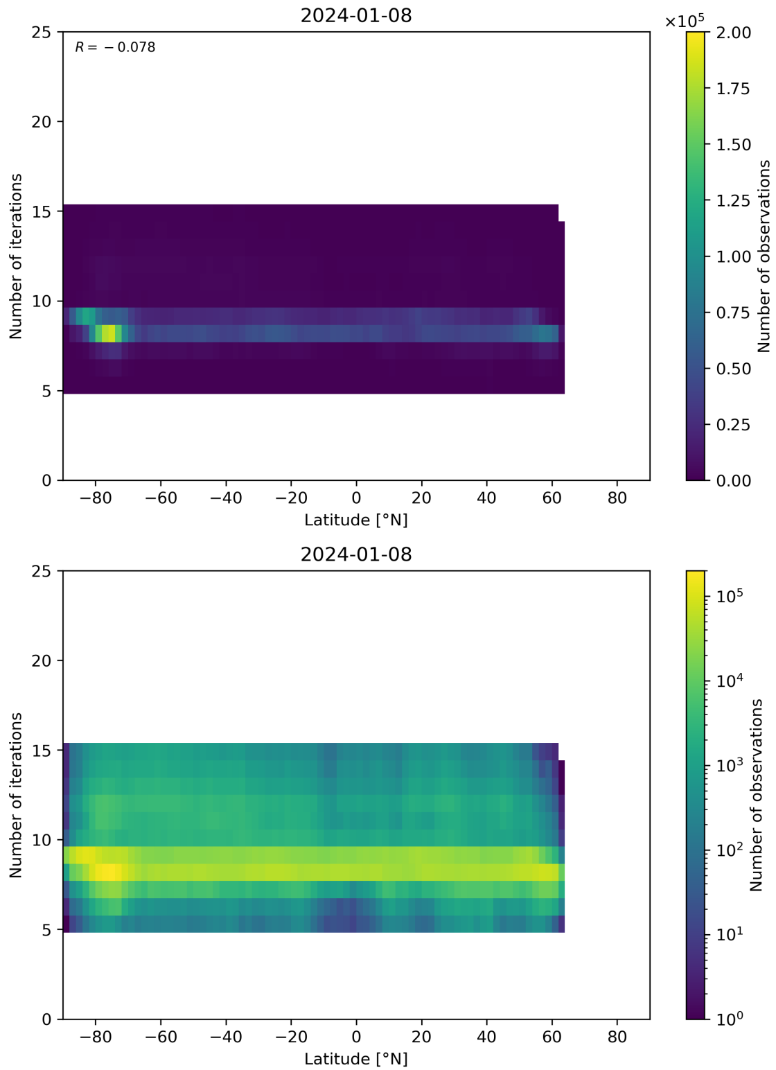
Figure 56: Scatter density plot of “Latitude” against “Number of iterations” for 2024-01-07 to 2024-01-09.
