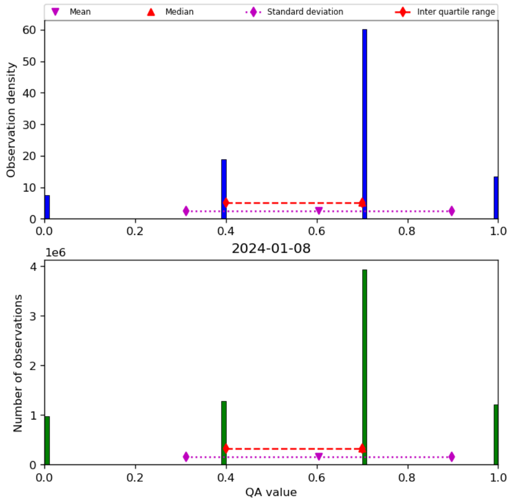
Figure 17: Histogram of “QA value” for 2024-01-07 to 2024-01-09
