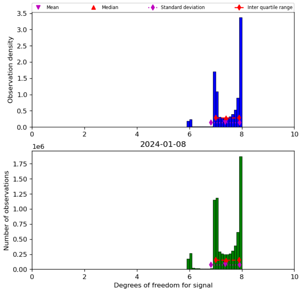
Figure 23: Histogram of “Degrees of freedom for signal” for 2024-01-07 to 2024-01-09
