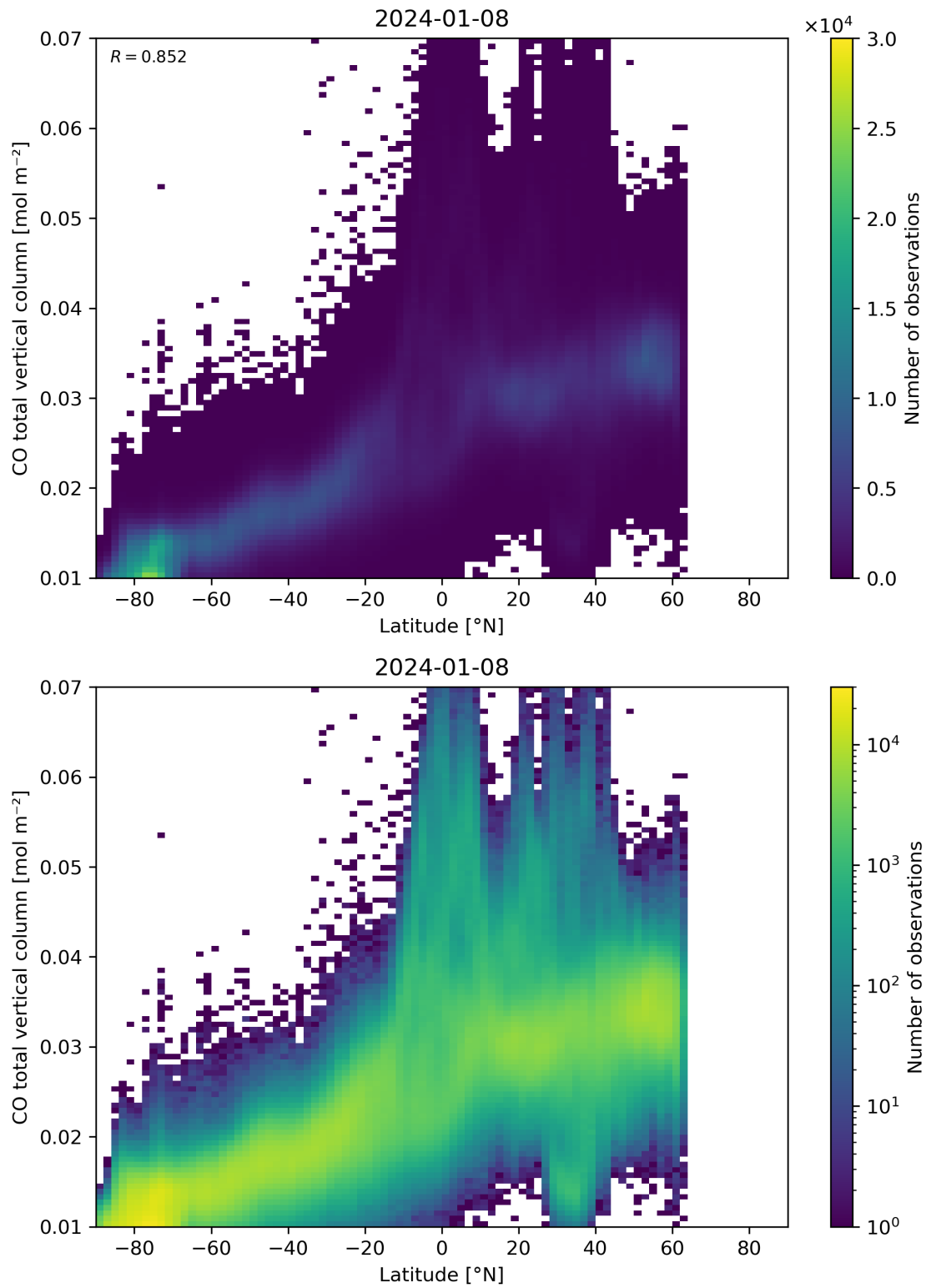
Figure 51: Scatter density plot of “Latitude” against “CO total vertical column” for 2024-01-07 to 2024-01-09.
