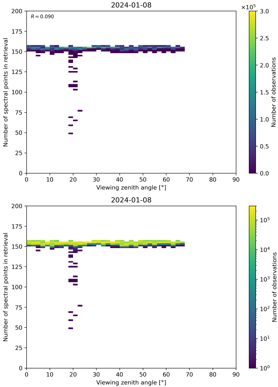
Figure 76: Scatter density plot of “Viewing zenith angle” against “Number of spectral points in retrieval” for 2024-01-07 to 2024-01-09.
