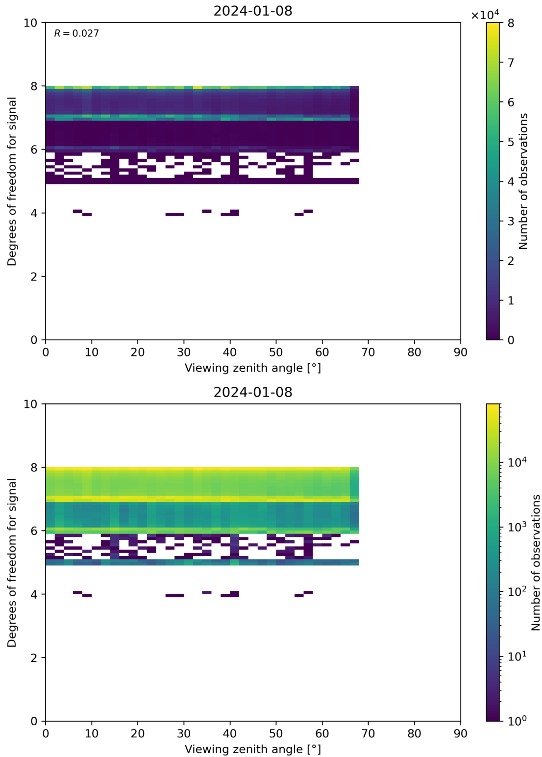
Figure 73: Scatter density plot of “Viewing zenith angle” against “Degrees of freedom for signal” for 2024-01-07 to 2024-01-09.
