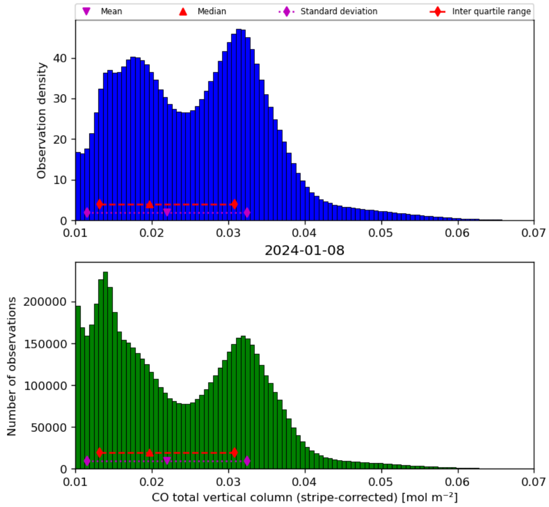
Figure 19: Histogram of “CO total vertical column (stripe-corrected)” for 2024-01-07 to 2024-01-09
