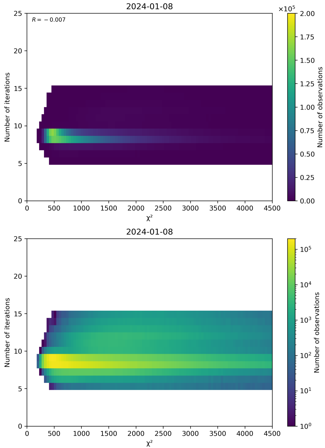
Figure 49: Scatter density plot of “ \chi^2 ” against “Number of iterations” for 2024-01-07 to 2024-01-09.
