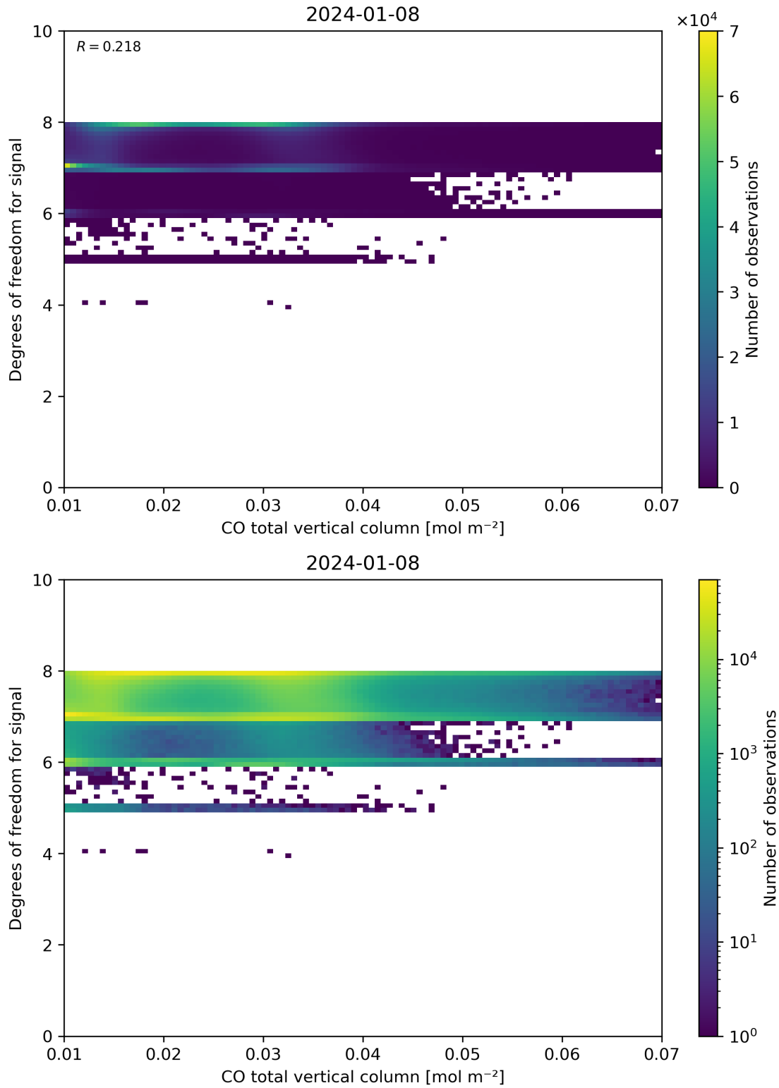
Figure 41: Scatter density plot of “CO total vertical column” against “Degrees of freedom for signal” for 2024-01-07 to 2024-01-09.
