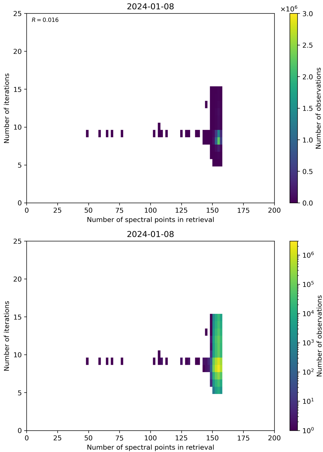
Figure 60: Scatter density plot of “Number of spectral points in retrieval” against “Number of iterations” for 2024-01-07 to 2024-01-09.
