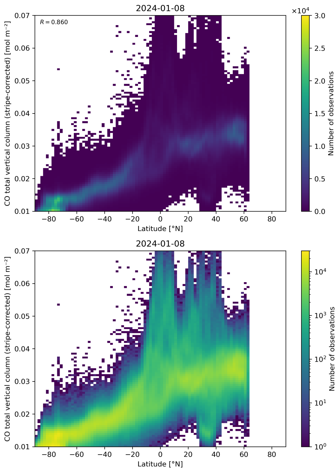
Figure 52: Scatter density plot of “Latitude” against “CO total vertical column (stripe-corrected)” for 2024-01-07 to 2024-01-09.
