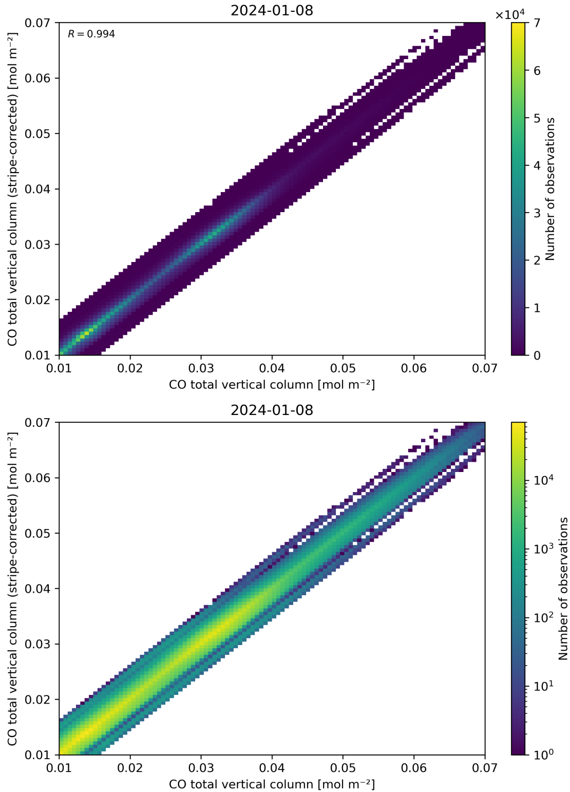
Figure 33: Scatter density plot of “CO total vertical column” against “CO total vertical column (stripe-corrected)” for 2024-01-07 to 2024-01-09.
