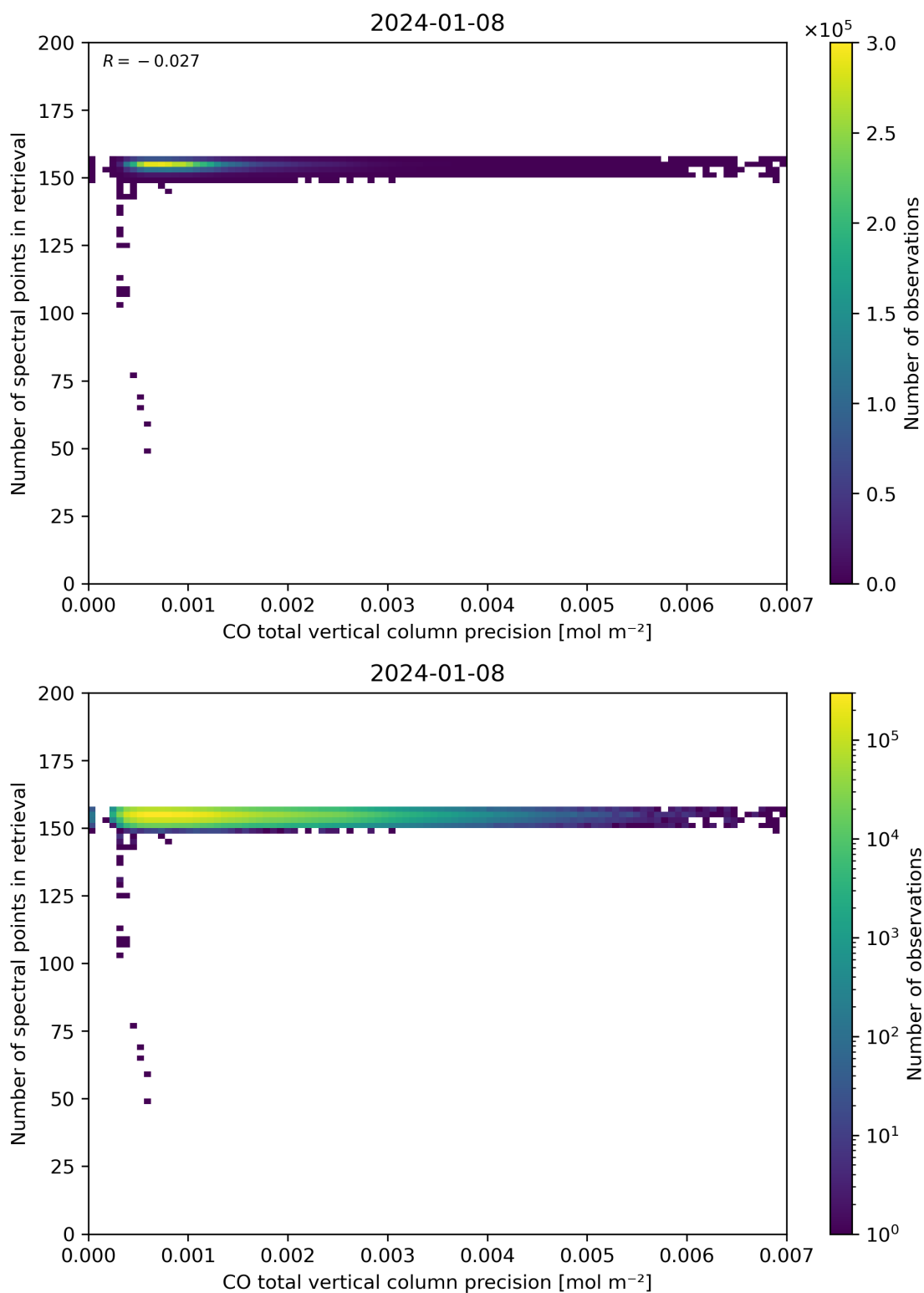
Figure 47: Scatter density plot of “CO total vertical column precision” against “Number of spectral points in retrieval” for 2024-01-07 to 2024-01-09.
