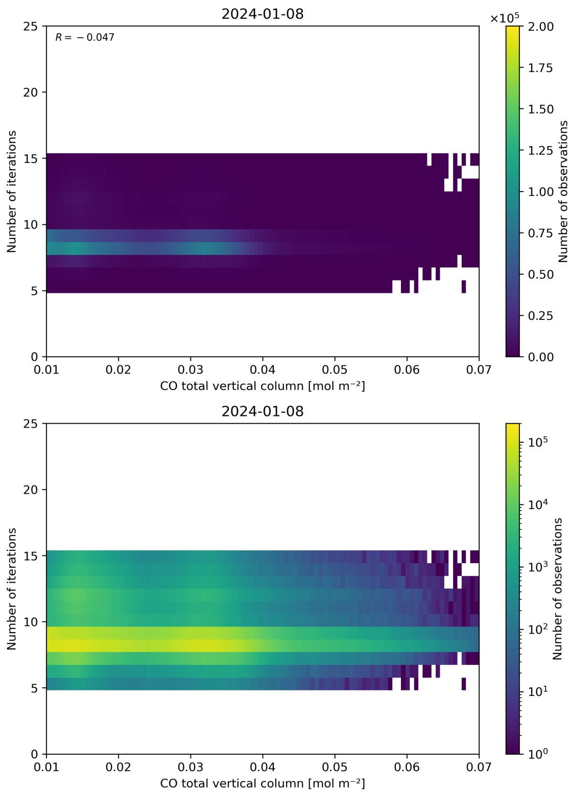
Figure 42: Scatter density plot of “CO total vertical column” against “Number of iterations” for 2024-01-07 to 2024-01-09.
