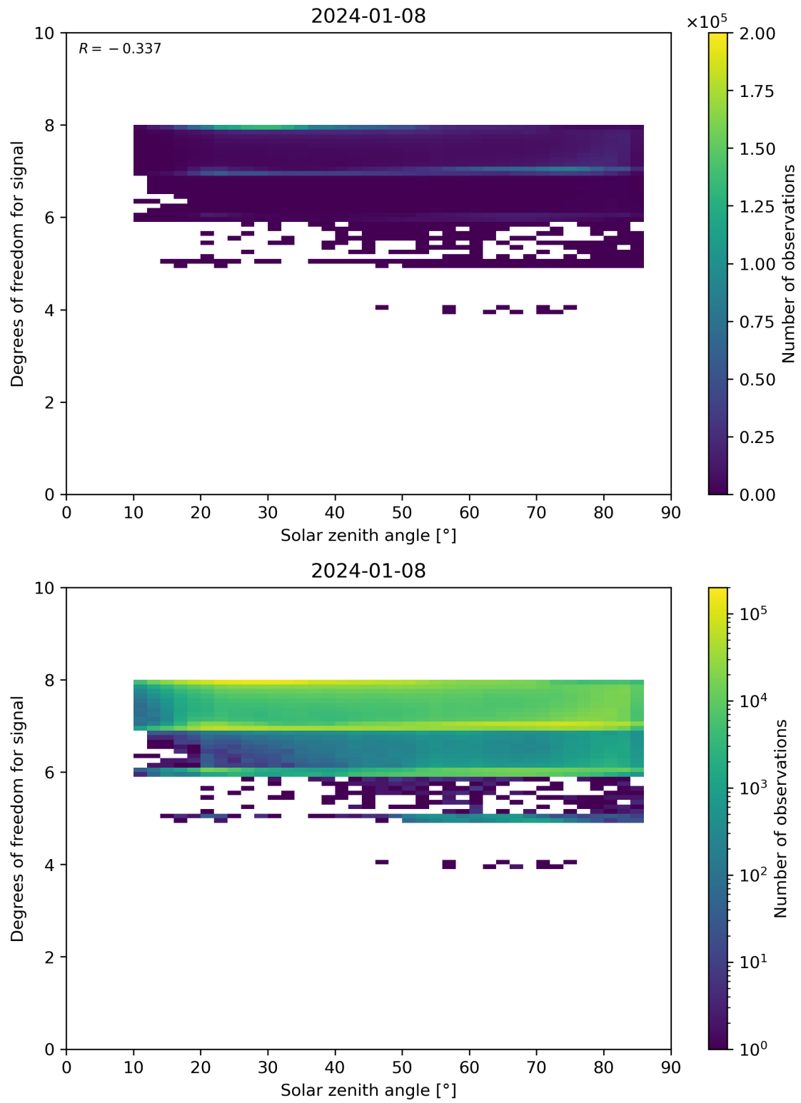
Figure 65: Scatter density plot of “Solar zenith angle” against “Degrees of freedom for signal” for 2024-01-07 to 2024-01-09.
