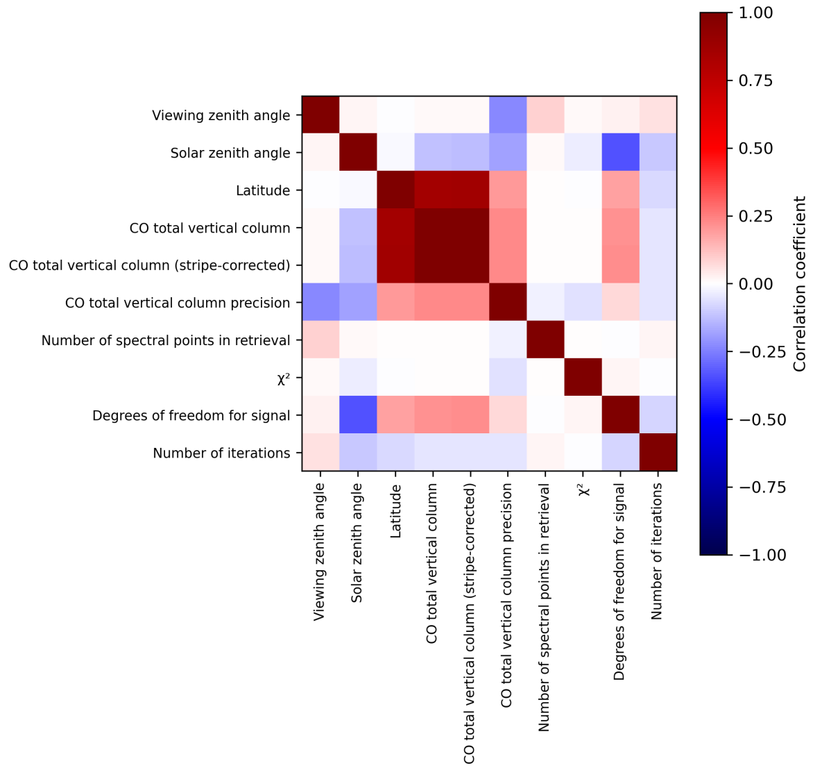
Figure 2: Map of correlation matrix for 2024-01-07 to 2024-01-09.
