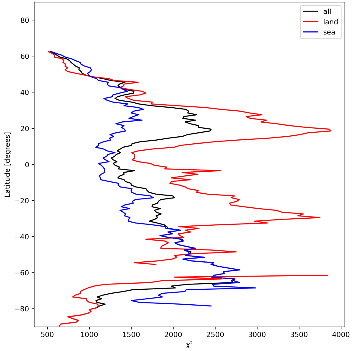
Figure 14: Zonal average of “ \chi^2 ” for 2024-01-07 to 2024-01-09.
