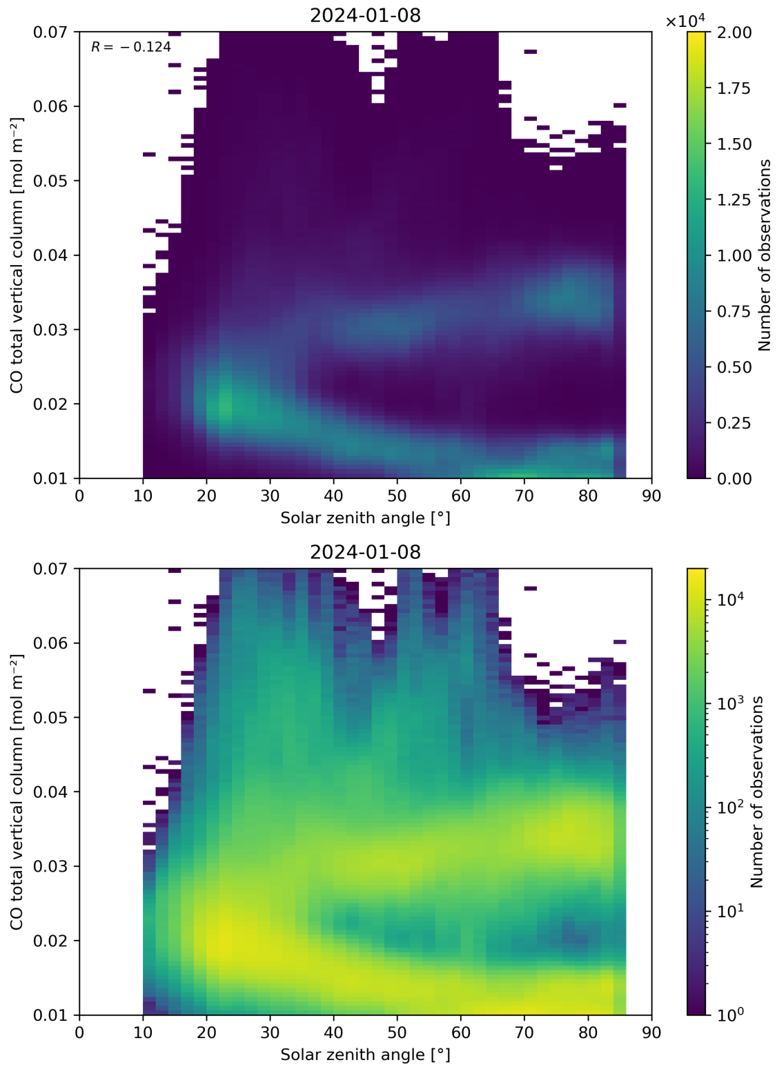
Figure 61: Scatter density plot of “Solar zenith angle” against “CO total vertical column” for 2024-01-07 to 2024-01-09.
