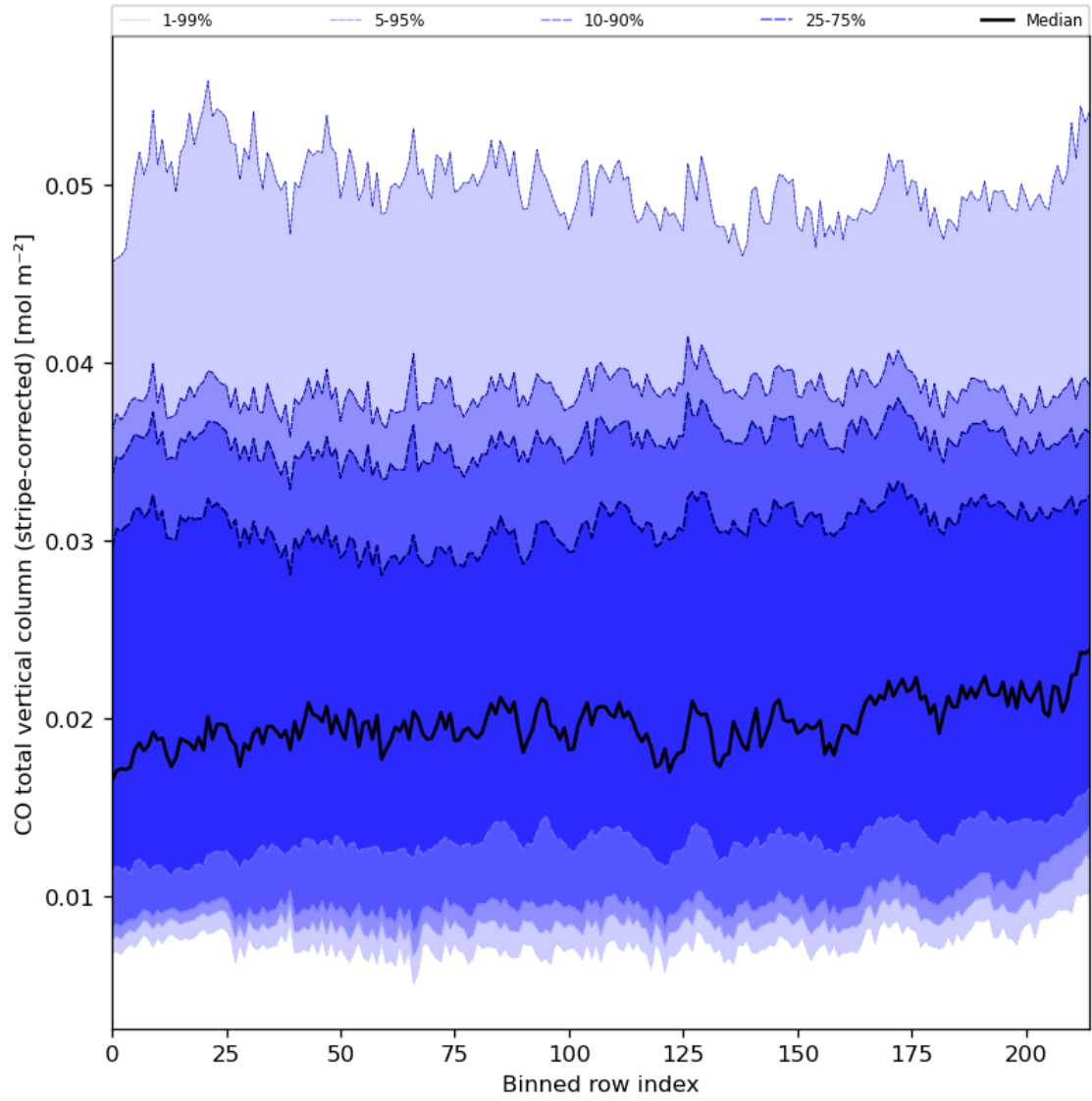
Figure 27: Along track statistics of “CO total vertical column (stripe-corrected)” for 2024-01-07 to 2024-01-09
