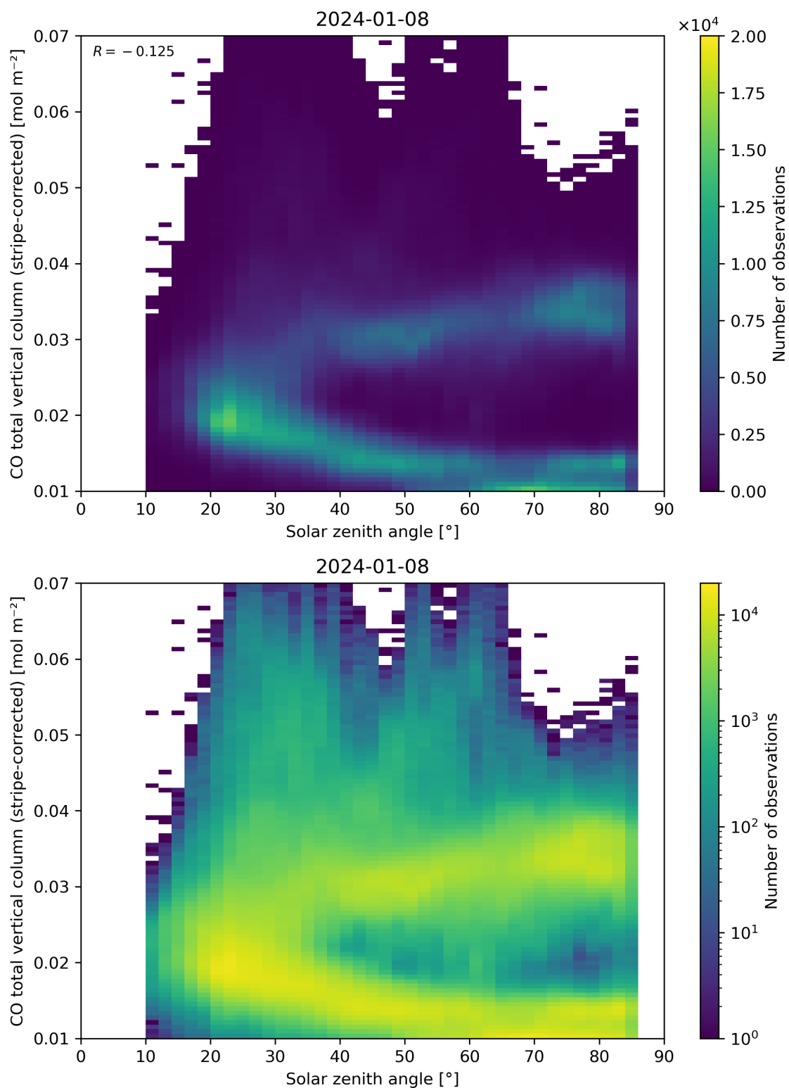
Figure 62: Scatter density plot of “Solar zenith angle” against “CO total vertical column (stripe-corrected)” for 2024-01-07 to 2024-01-09.
