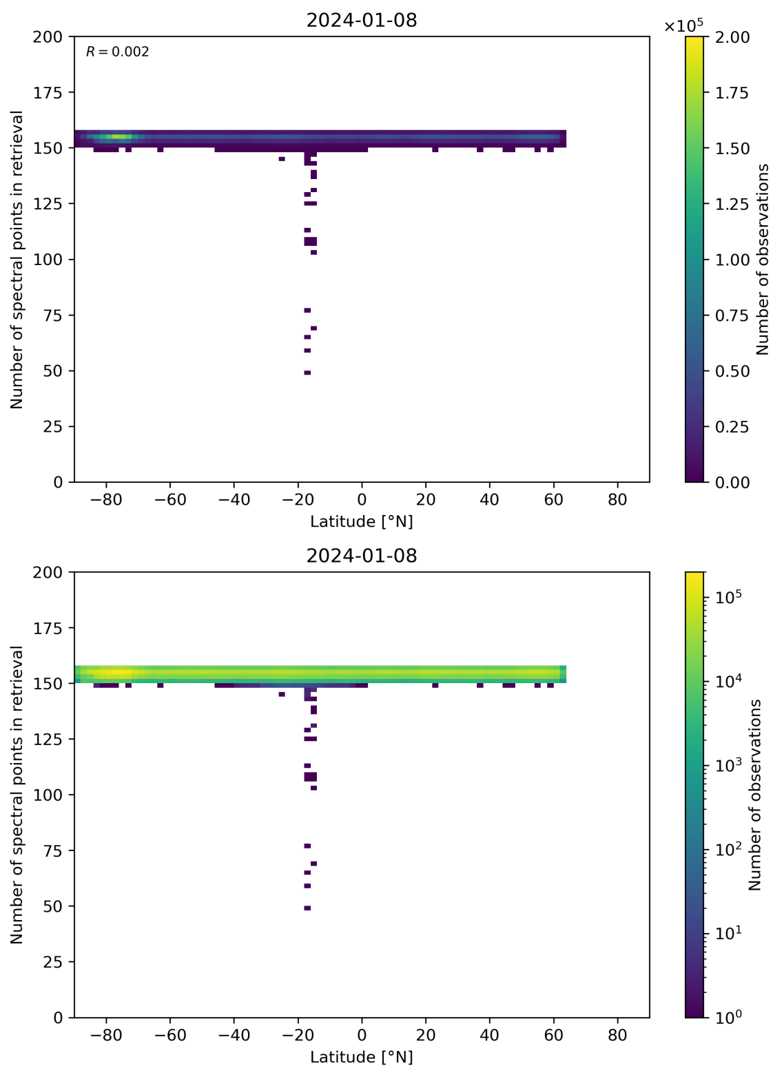
Figure 57: Scatter density plot of “Latitude” against “Number of spectral points in retrieval” for 2024-01-07 to 2024-01-09.
