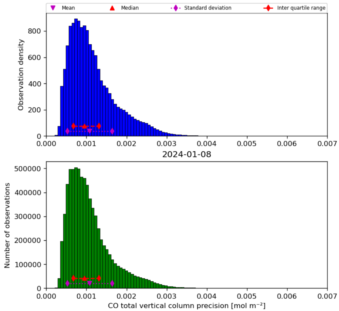
Figure 20: Histogram of “CO total vertical column precision” for 2024-01-07 to 2024-01-09
