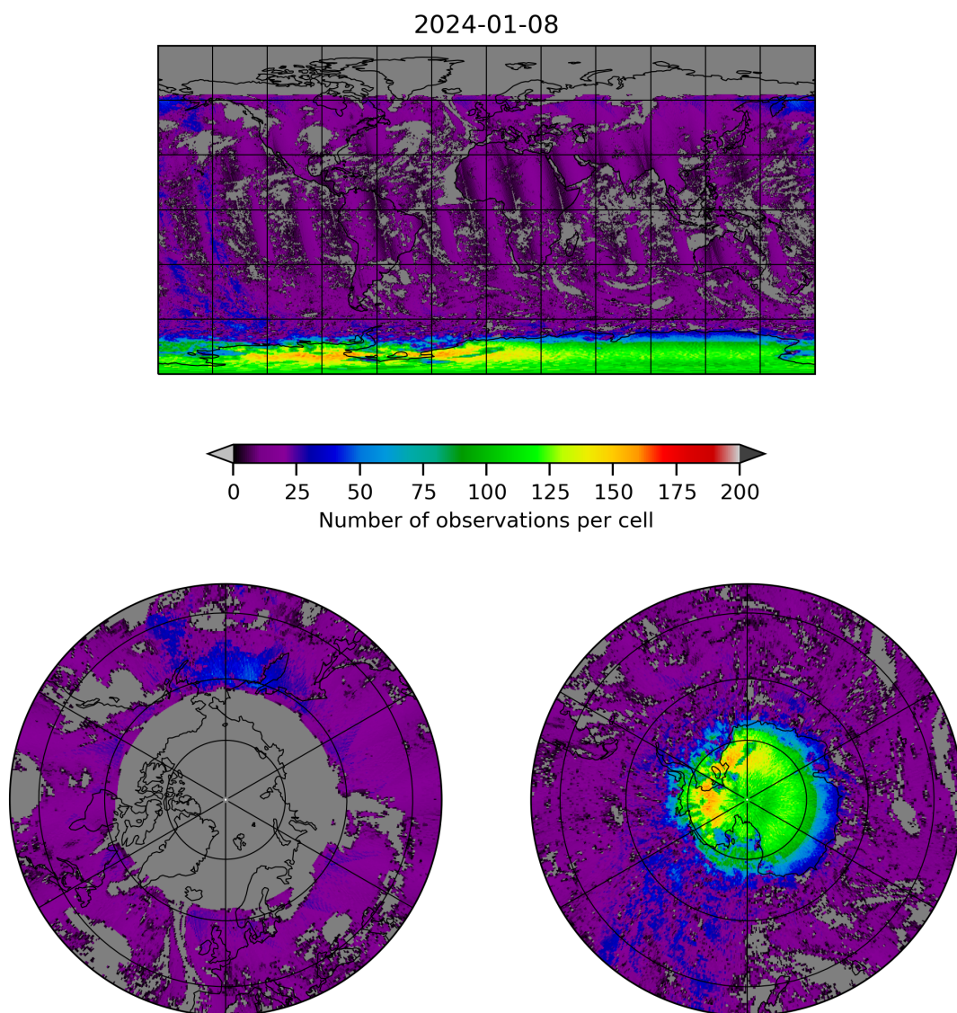
Figure 8: Map of the number of observations for 2024-01-07 to 2024-01-09
