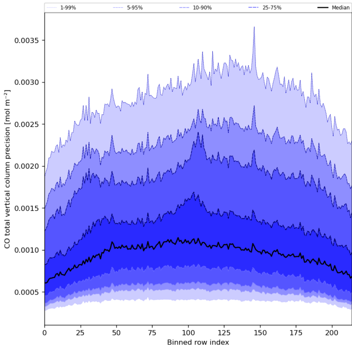
Figure 28: Along track statistics of “CO total vertical column precision” for 2024-01-07 to 2024-01-09
