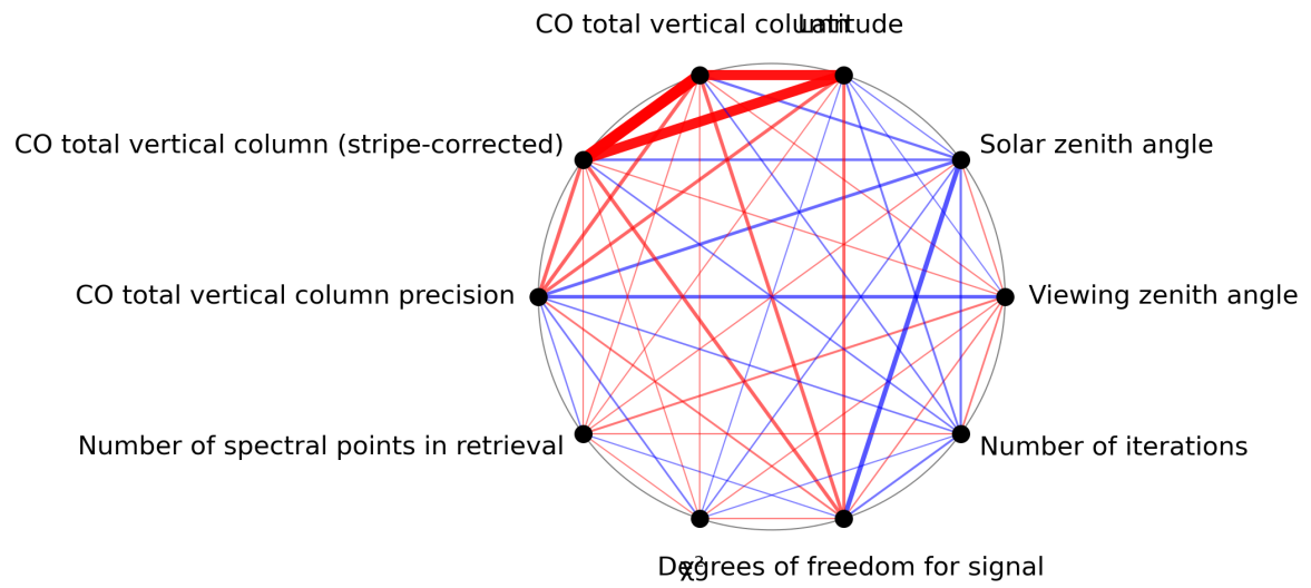
Figure 1: Map of correlation graph for 2024-01-07 to 2024-01-09.
