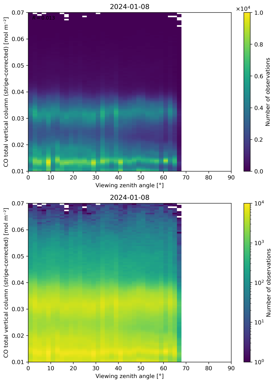
Figure 70: Scatter density plot of “Viewing zenith angle” against “CO total vertical column (stripe-corrected)” for 2024-01-07 to 2024-01-09.
