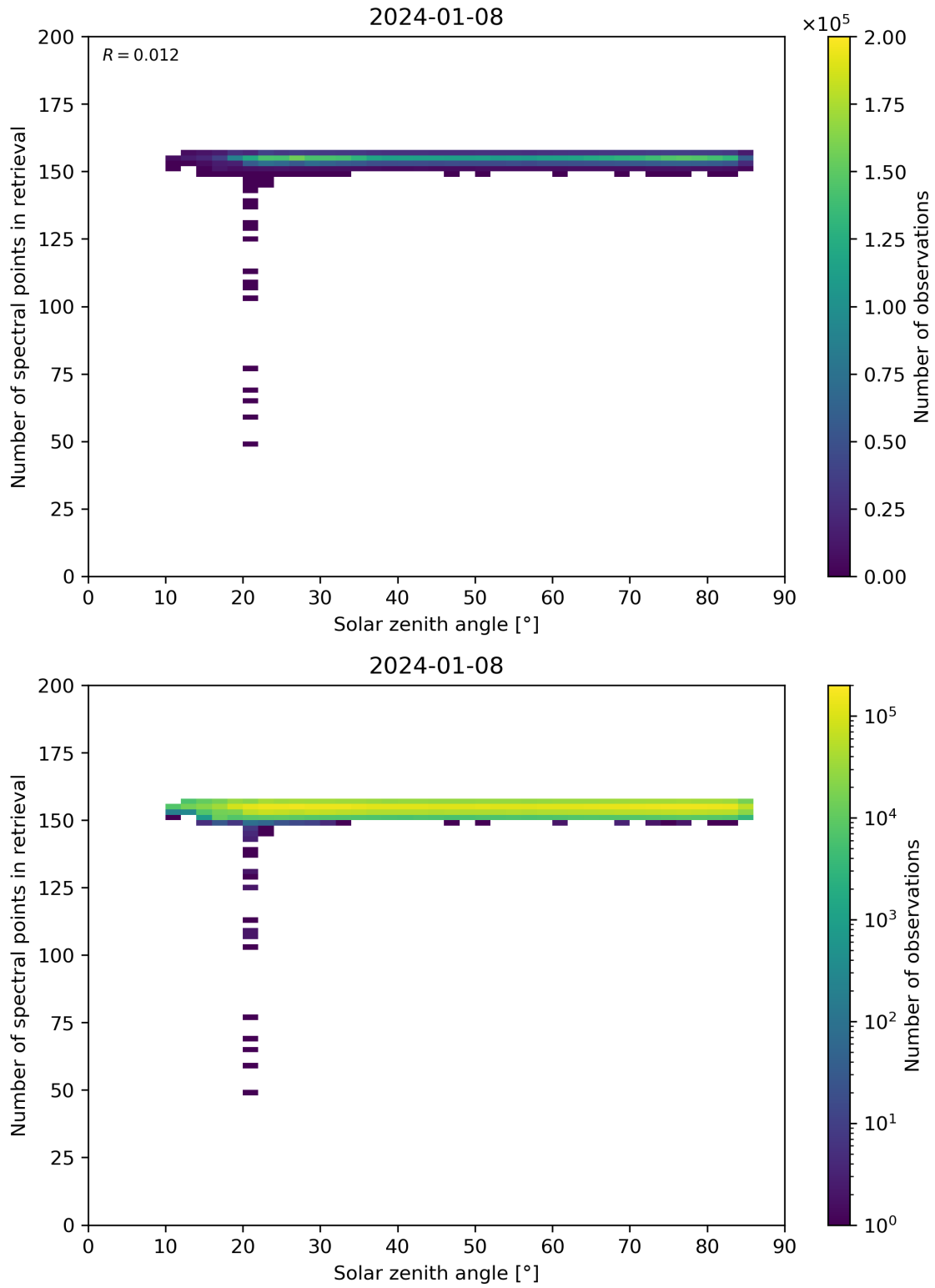
Figure 68: Scatter density plot of “Solar zenith angle” against “Number of spectral points in retrieval” for 2024-01-07 to 2024-01-09.
