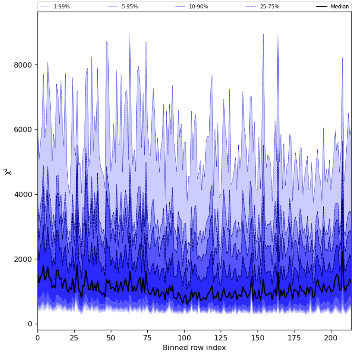
Figure 30: Along track statistics of “ \chi^2 ” for 2024-01-07 to 2024-01-09
