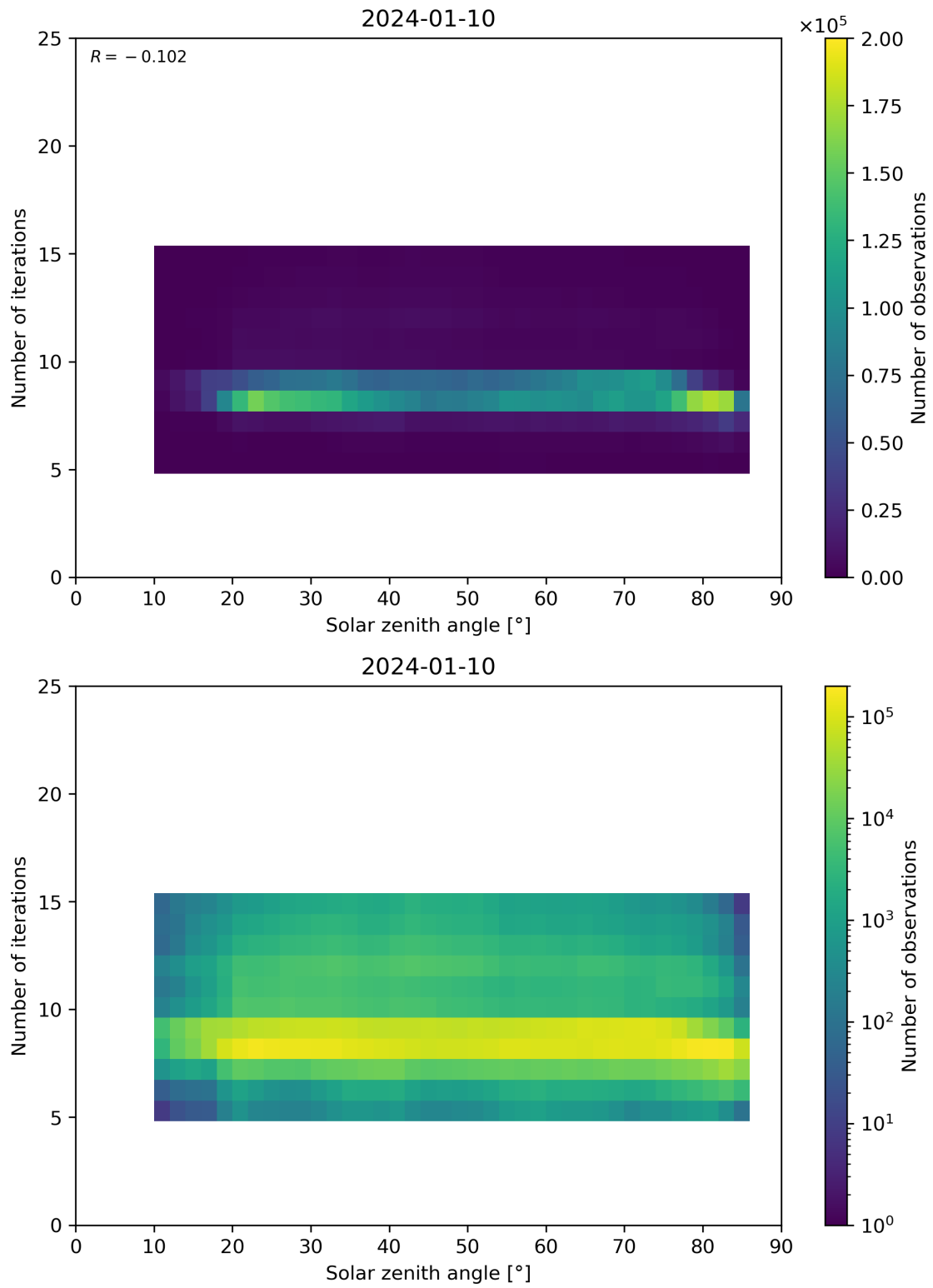
Figure 67: Scatter density plot of “Solar zenith angle” against “Number of iterations” for 2024-01-10 to 2024-01-11.
