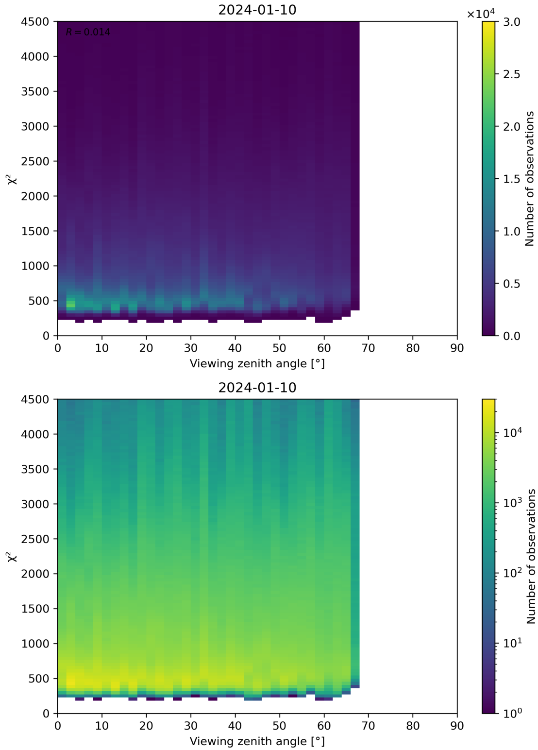
Figure 72: Scatter density plot of “Viewing zenith angle” against “ \chi^2 ” for 2024-01-10 to 2024-01-11.
