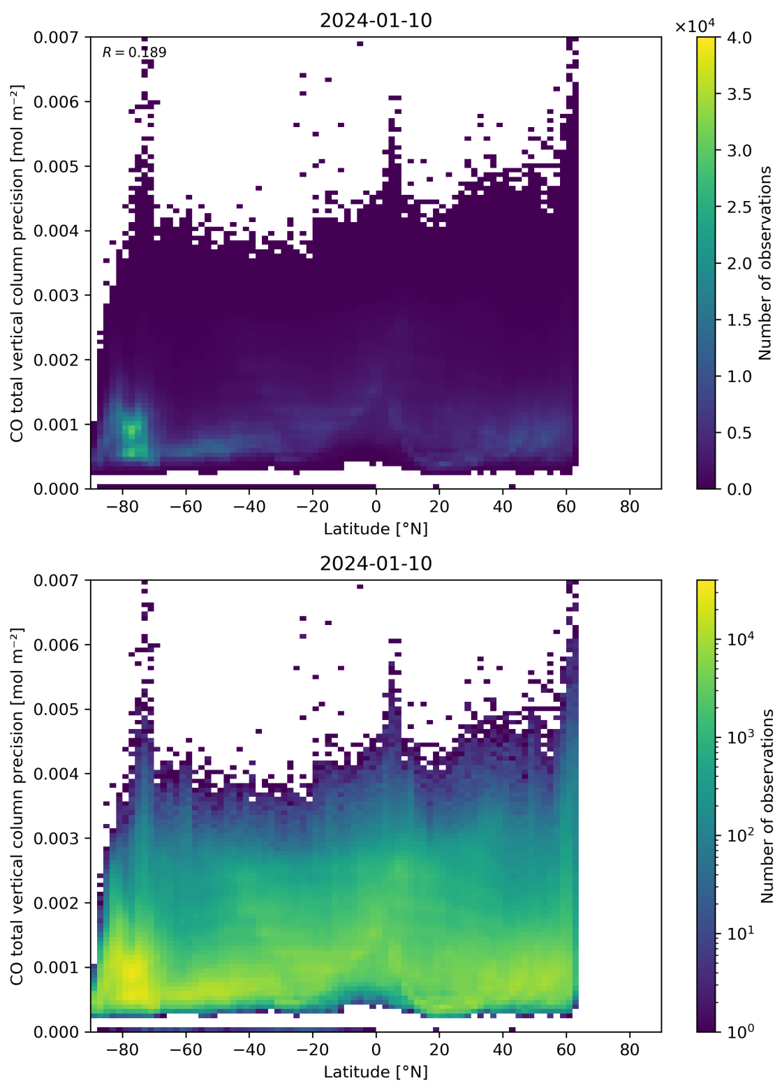
Figure 53: Scatter density plot of “Latitude” against “CO total vertical column precision” for 2024-01-10 to 2024-01-11.
