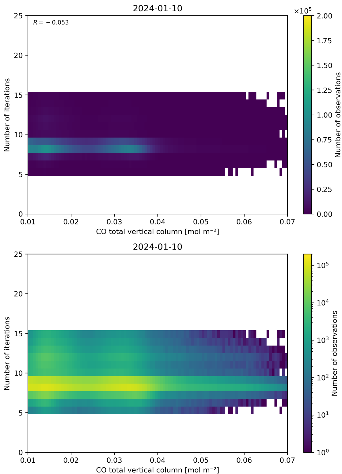
Figure 42: Scatter density plot of “CO total vertical column” against “Number of iterations” for 2024-01-10 to 2024-01-11.
