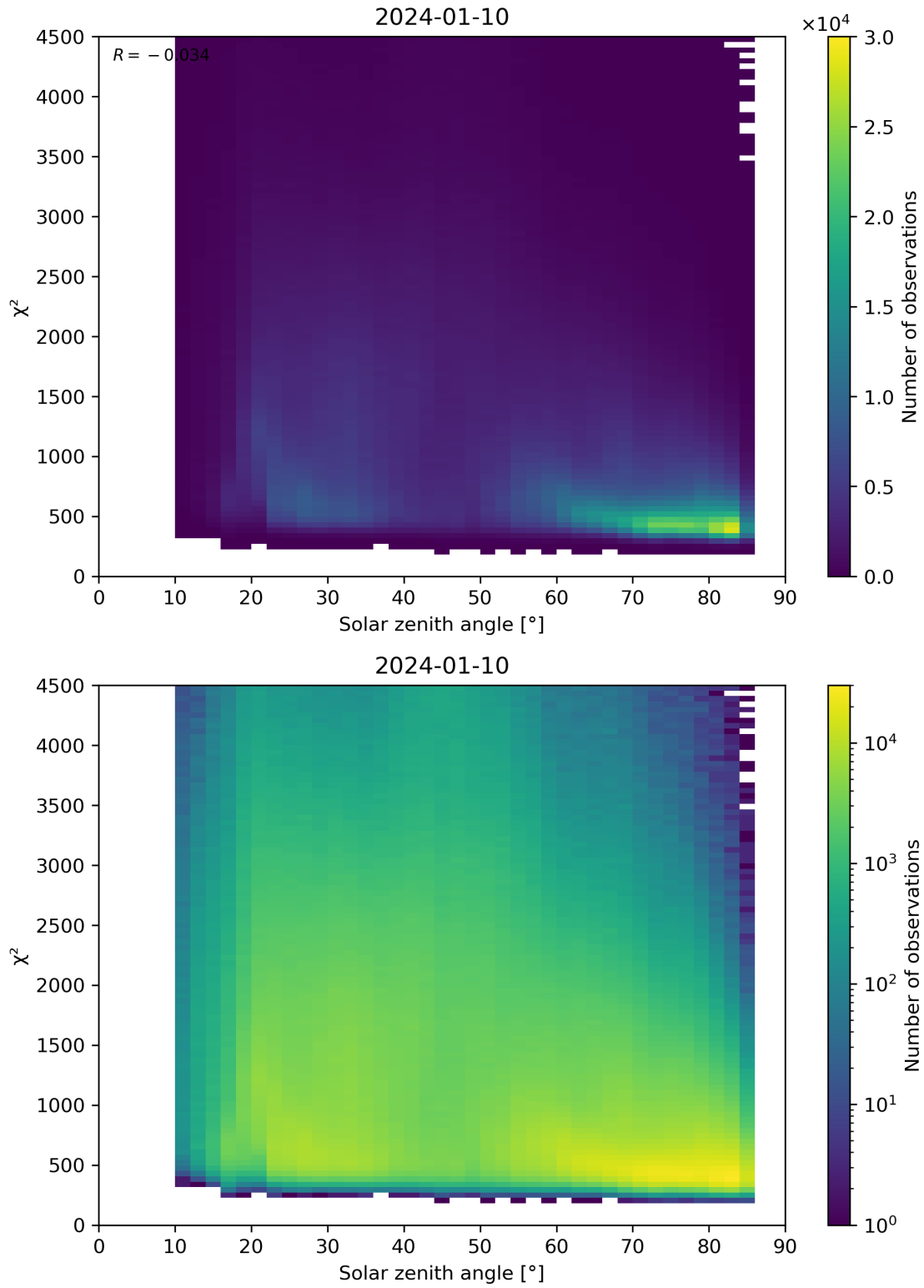
Figure 64: Scatter density plot of “Solar zenith angle” against “ \chi^2 ” for 2024-01-10 to 2024-01-11.
