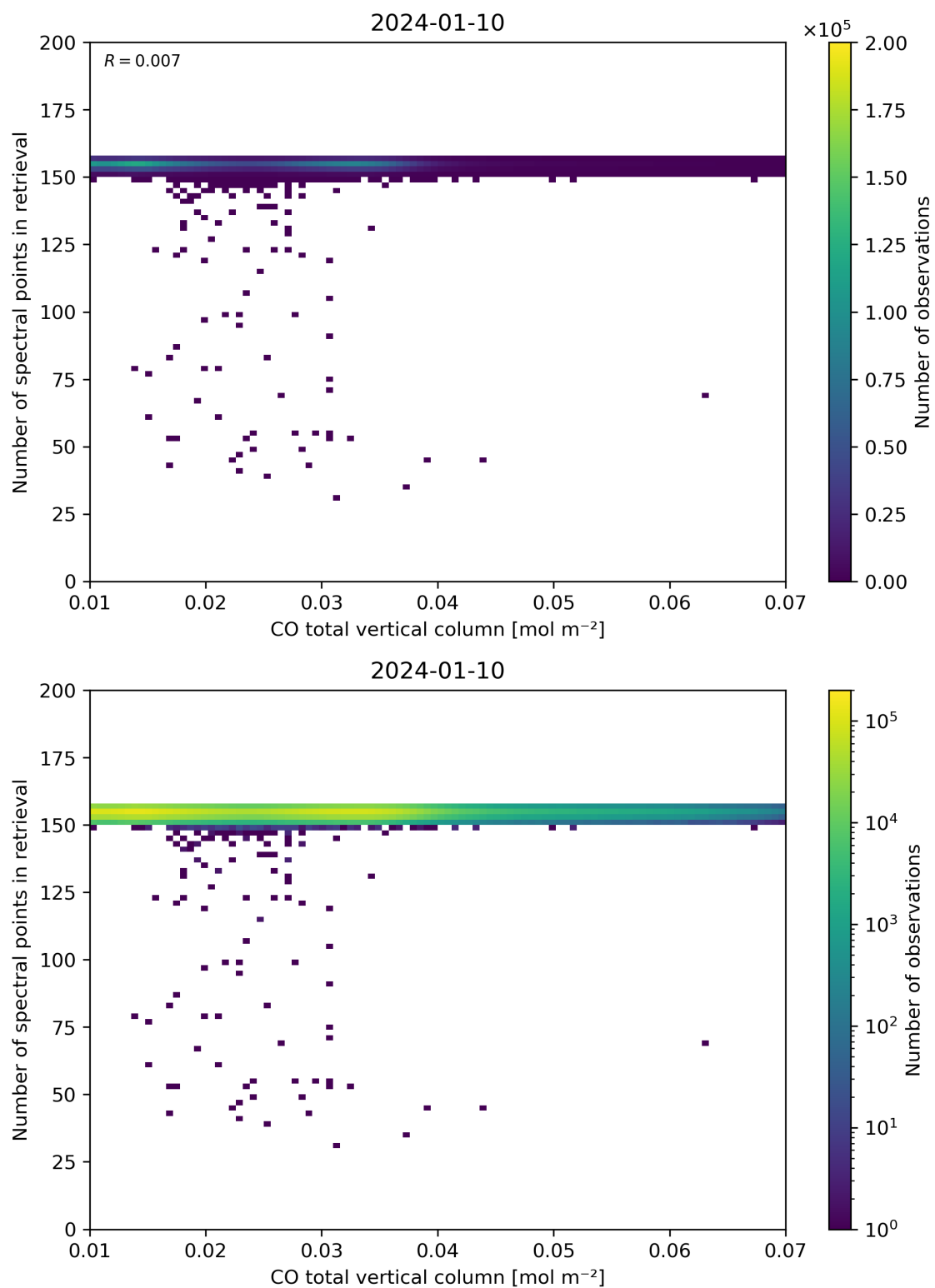
Figure 43: Scatter density plot of “CO total vertical column” against “Number of spectral points in retrieval” for 2024-01-10 to 2024-01-11.
