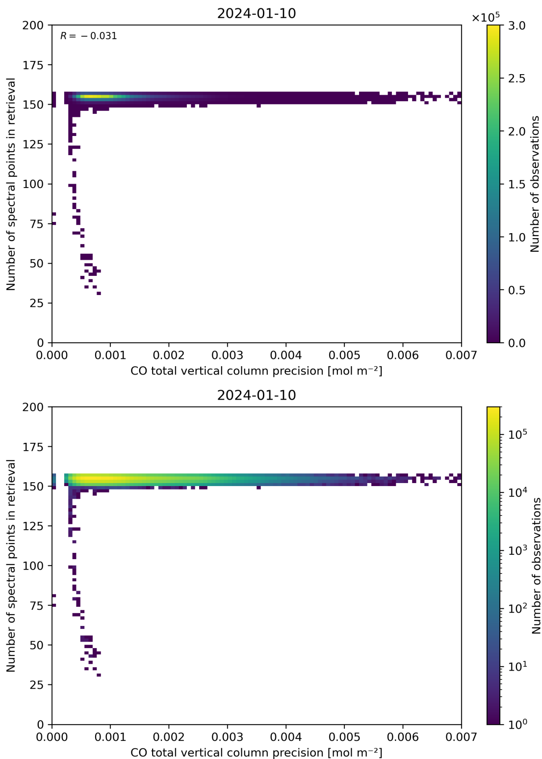
Figure 47: Scatter density plot of “CO total vertical column precision” against “Number of spectral points in retrieval” for 2024-01-10 to 2024-01-11.
