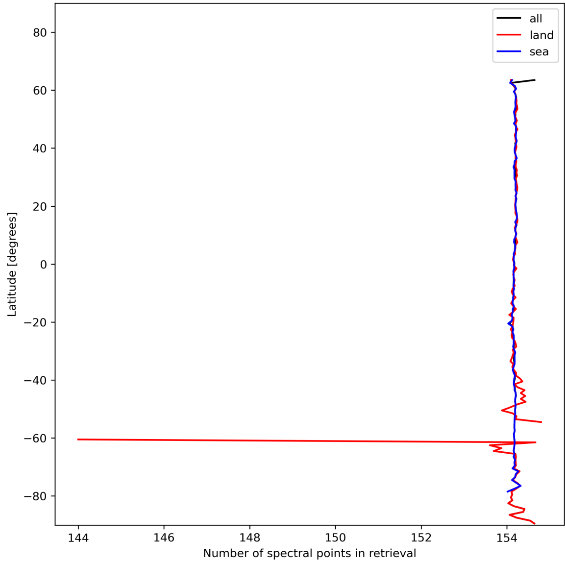
Figure 13: Zonal average of “Number of spectral points in retrieval” for 2024-01-10 to 2024-01-11.
