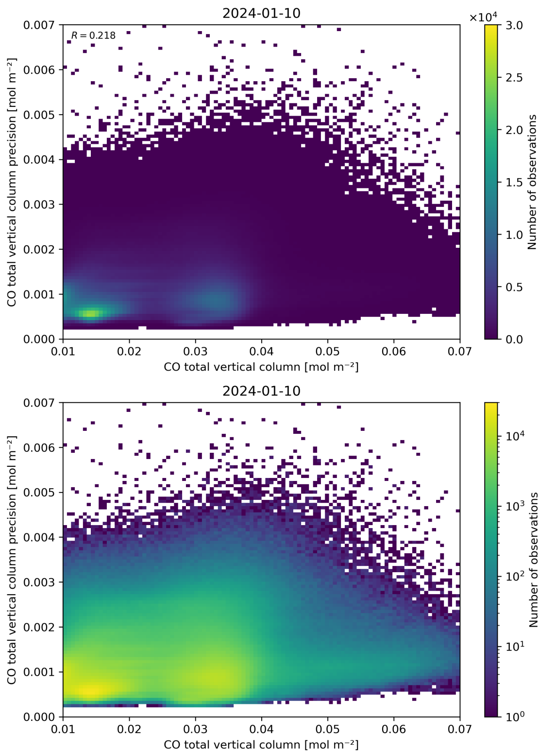
Figure 34: Scatter density plot of “CO total vertical column” against “CO total vertical column precision” for 2024-01-10 to 2024-01-11.
