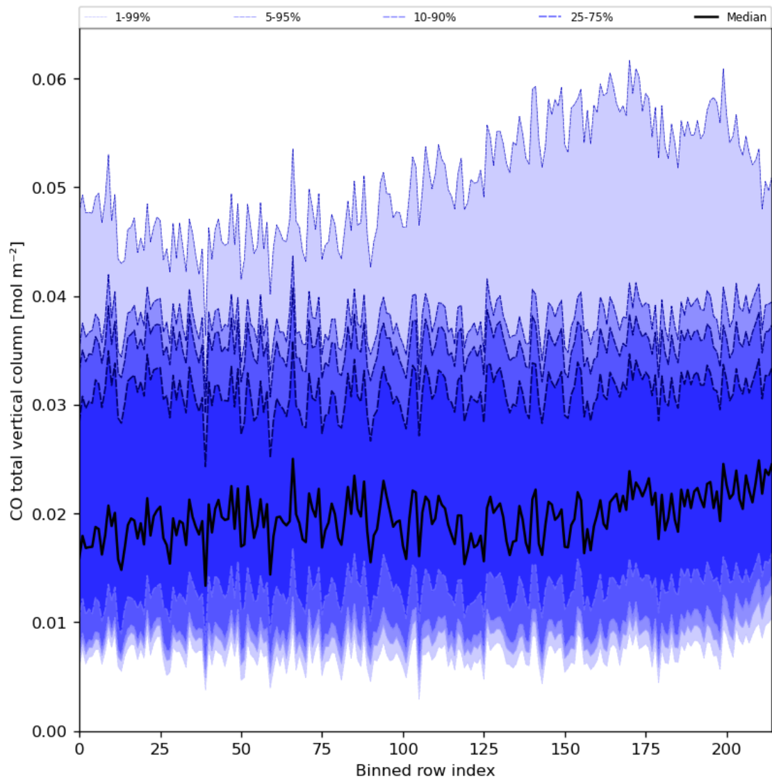
Figure 26: Along track statistics of “CO total vertical column” for 2024-01-10 to 2024-01-11
