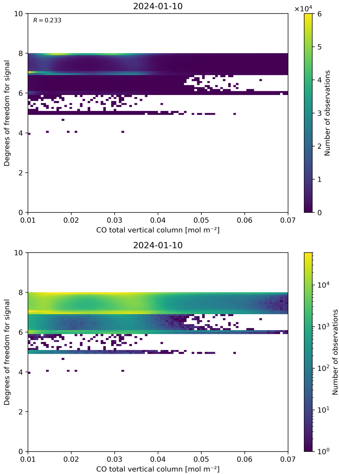
Figure 41: Scatter density plot of “CO total vertical column” against “Degrees of freedom for signal” for 2024-01-10 to 2024-01-11.
