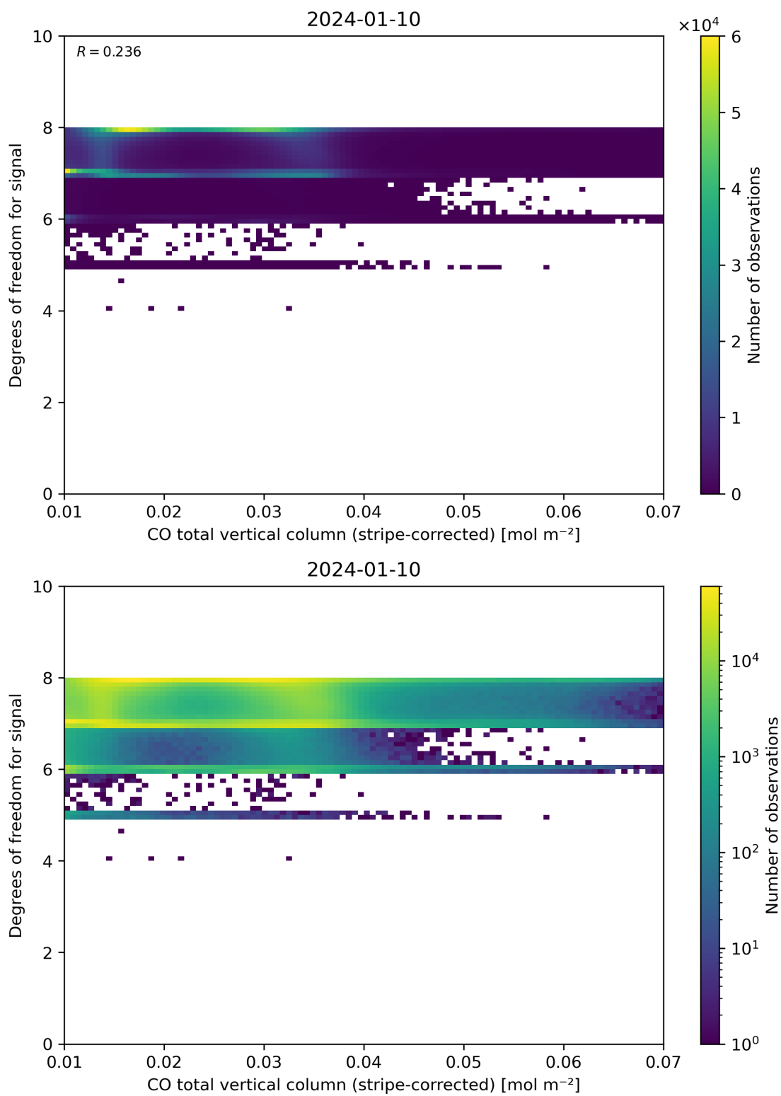
Figure 38: Scatter density plot of “CO total vertical column (stripe-corrected)” against “Degrees of freedom for signal” for 2024-01-10 to 2024-01-11.
