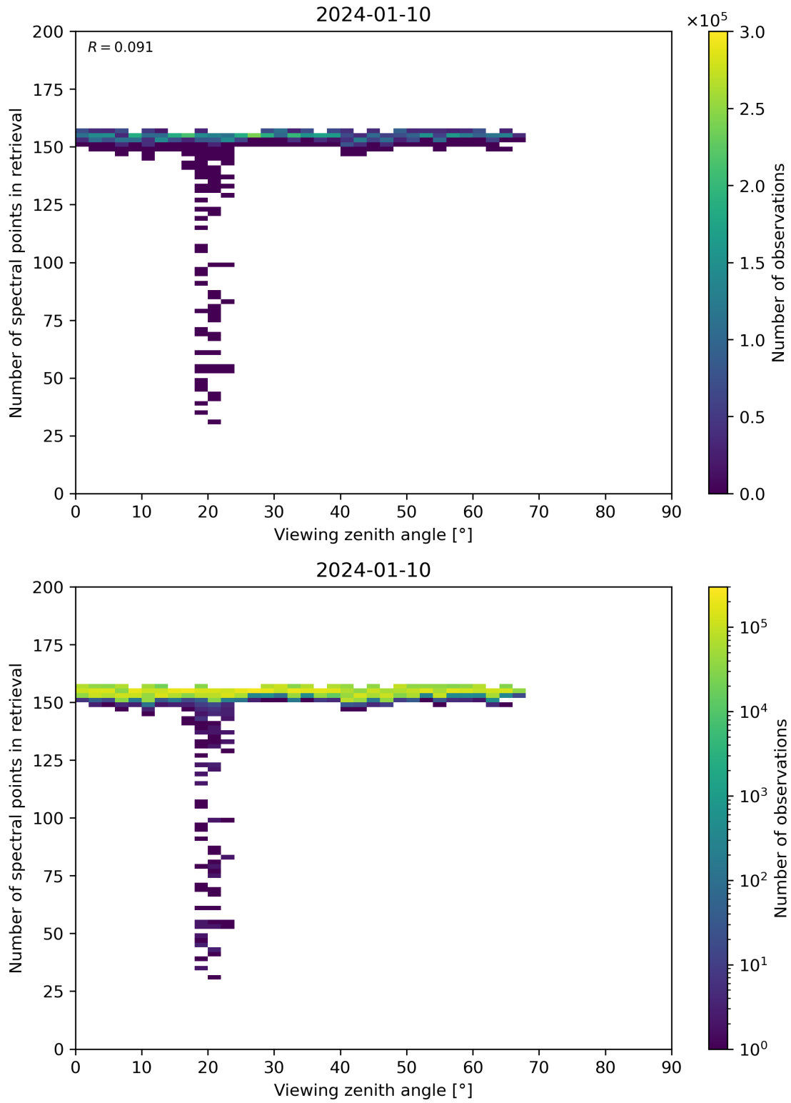
Figure 76: Scatter density plot of “Viewing zenith angle” against “Number of spectral points in retrieval” for 2024-01-10 to 2024-01-11.
