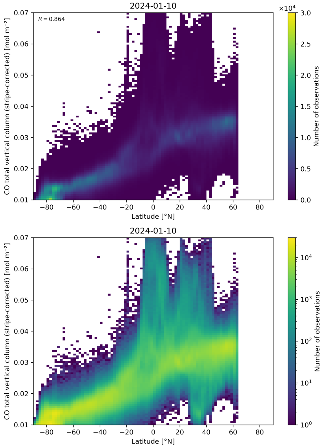
Figure 52: Scatter density plot of “Latitude” against “CO total vertical column (stripe-corrected)” for 2024-01-10 to 2024-01-11.
