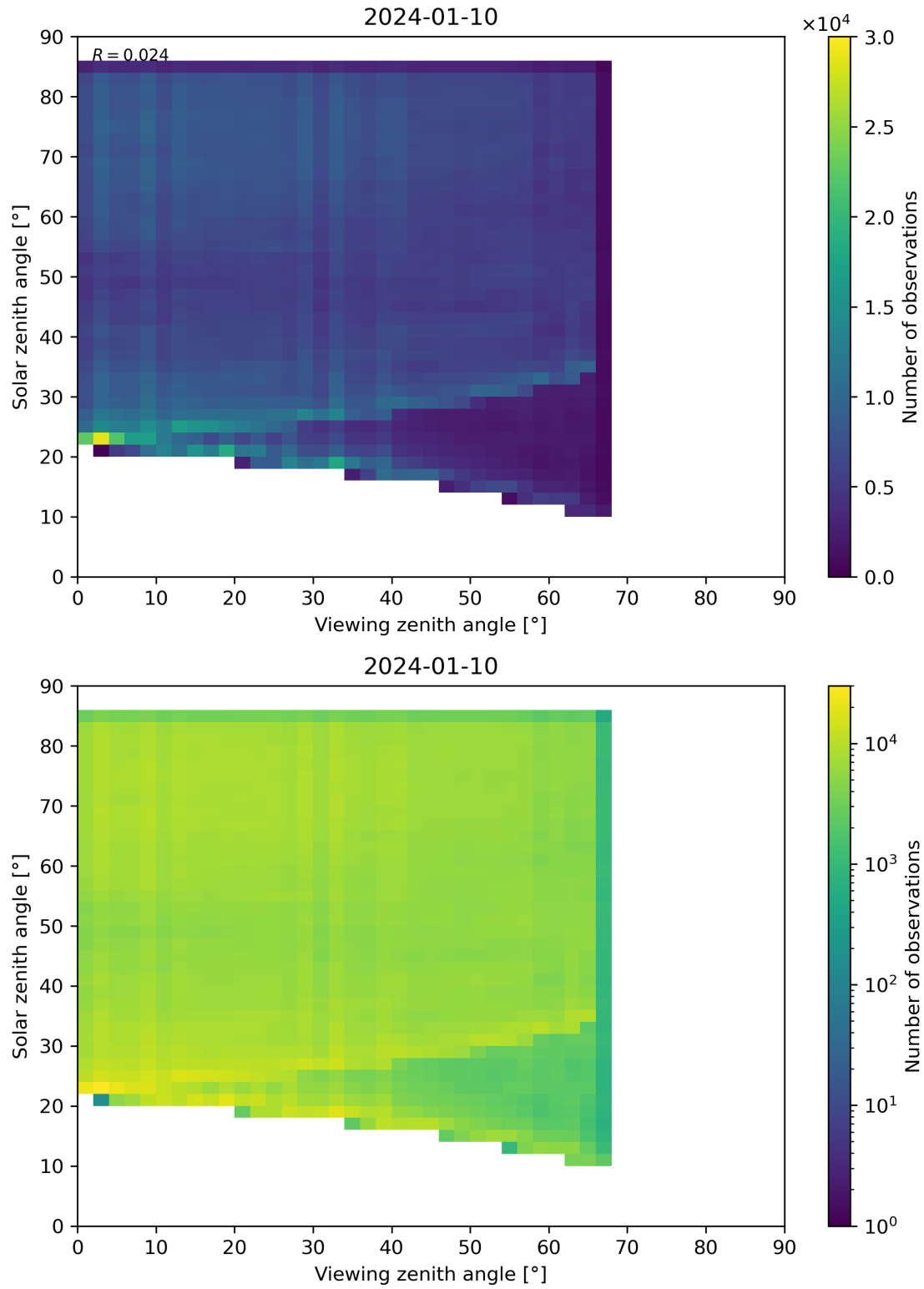
Figure 77: Scatter density plot of “Viewing zenith angle” against “Solar zenith angle” for 2024-01-10 to 2024-01-11.
