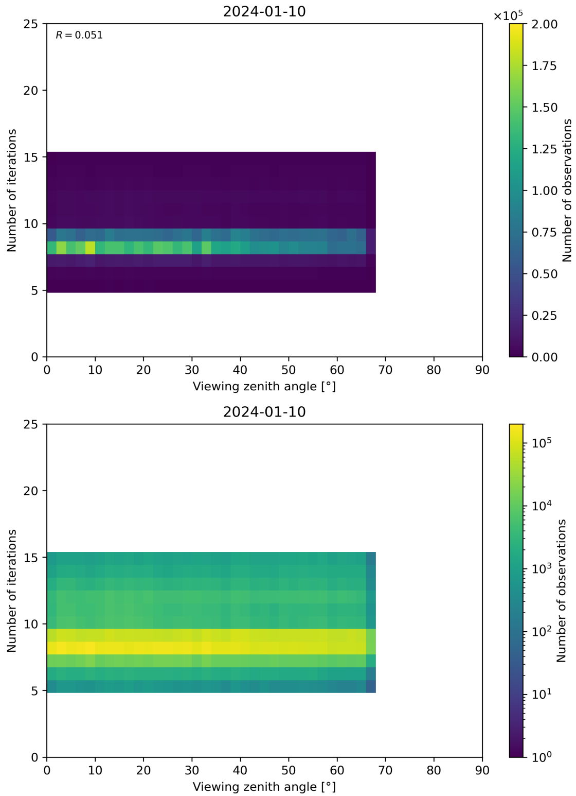
Figure 75: Scatter density plot of “Viewing zenith angle” against “Number of iterations” for 2024-01-10 to 2024-01-11.
