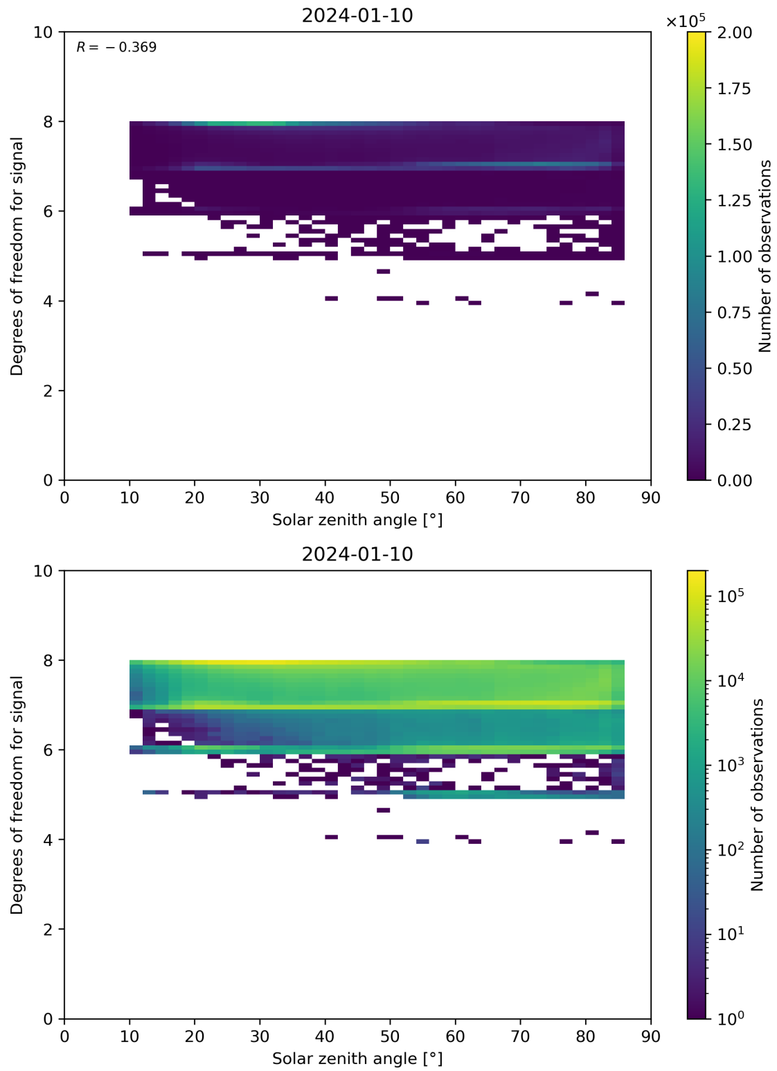
Figure 65: Scatter density plot of “Solar zenith angle” against “Degrees of freedom for signal” for 2024-01-10 to 2024-01-11.
