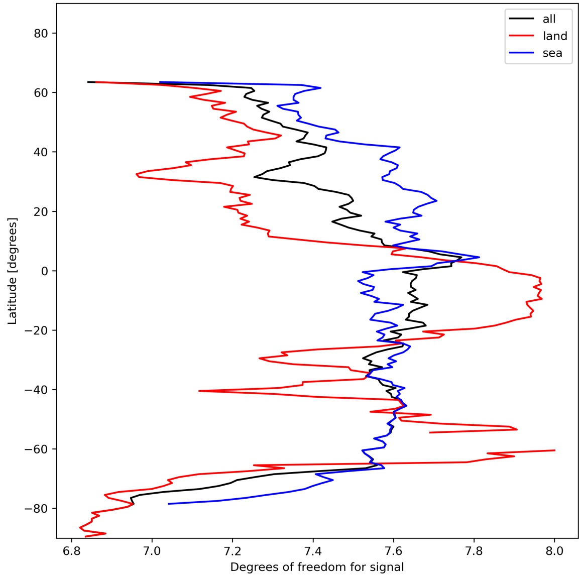
Figure 15: Zonal average of “Degrees of freedom for signal” for 2024-01-10 to 2024-01-11.
