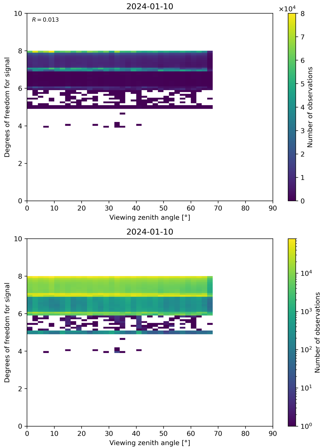
Figure 73: Scatter density plot of “Viewing zenith angle” against “Degrees of freedom for signal” for 2024-01-10 to 2024-01-11.
