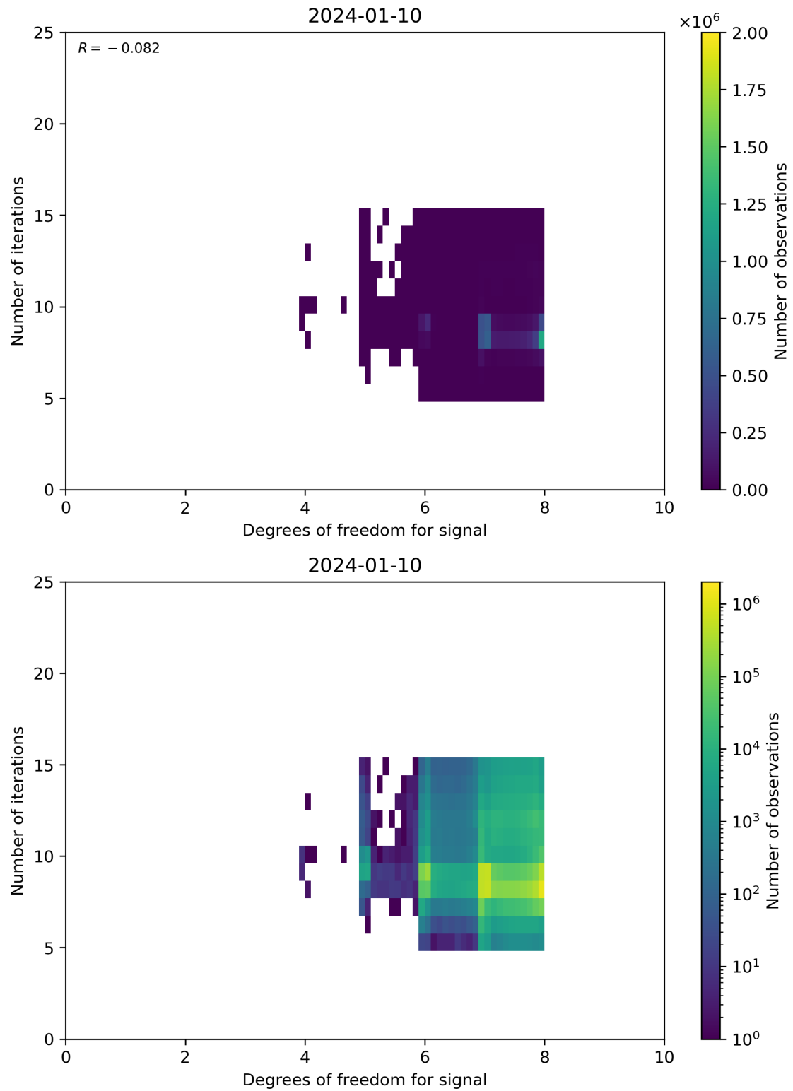
Figure 50: Scatter density plot of “Degrees of freedom for signal” against “Number of iterations” for 2024-01-10 to 2024-01-11.
