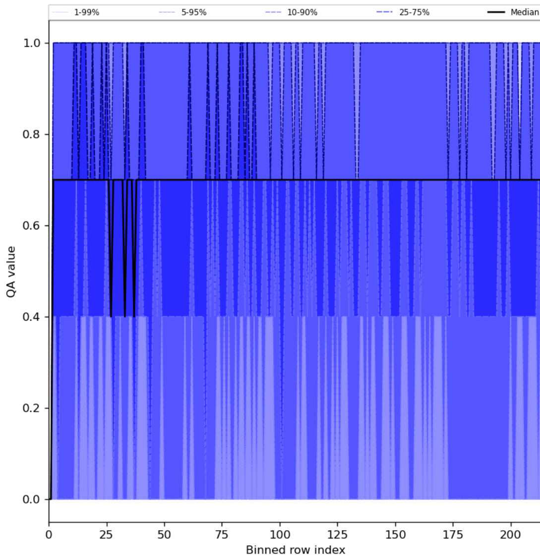
Figure 25: Along track statistics of “QA value” for 2024-01-10 to 2024-01-11
