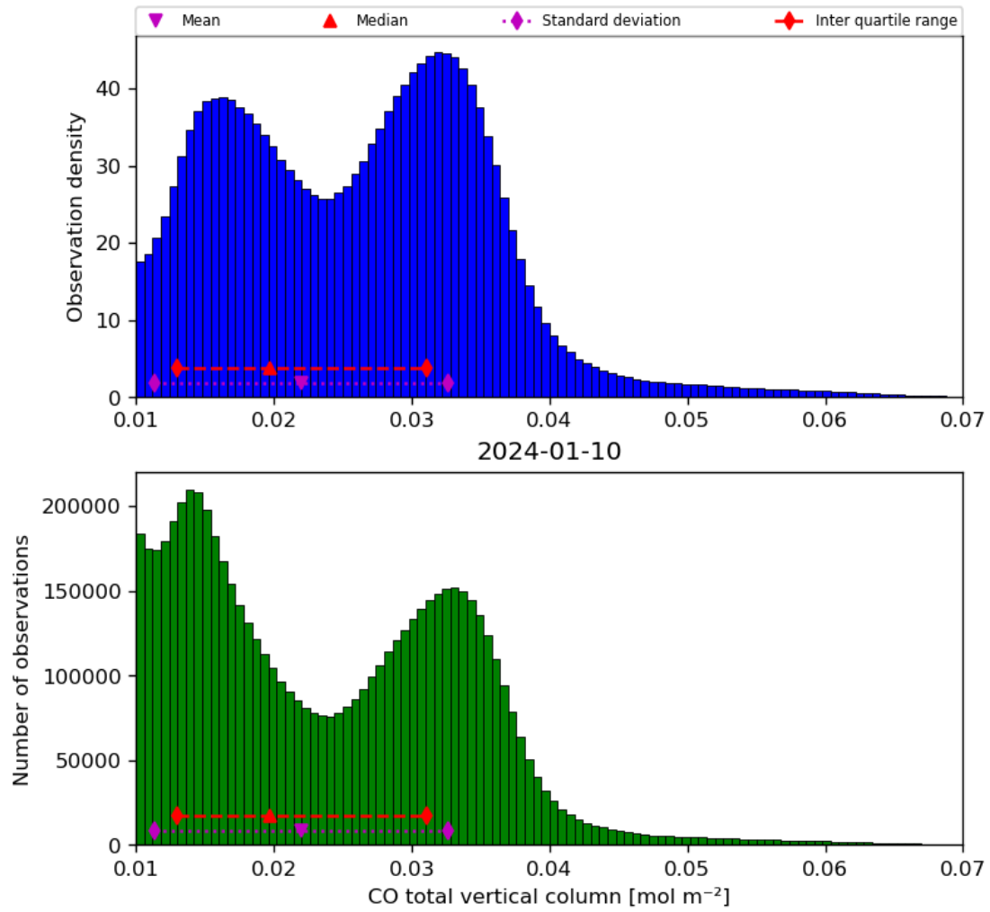
Figure 18: Histogram of “CO total vertical column” for 2024-01-10 to 2024-01-11
