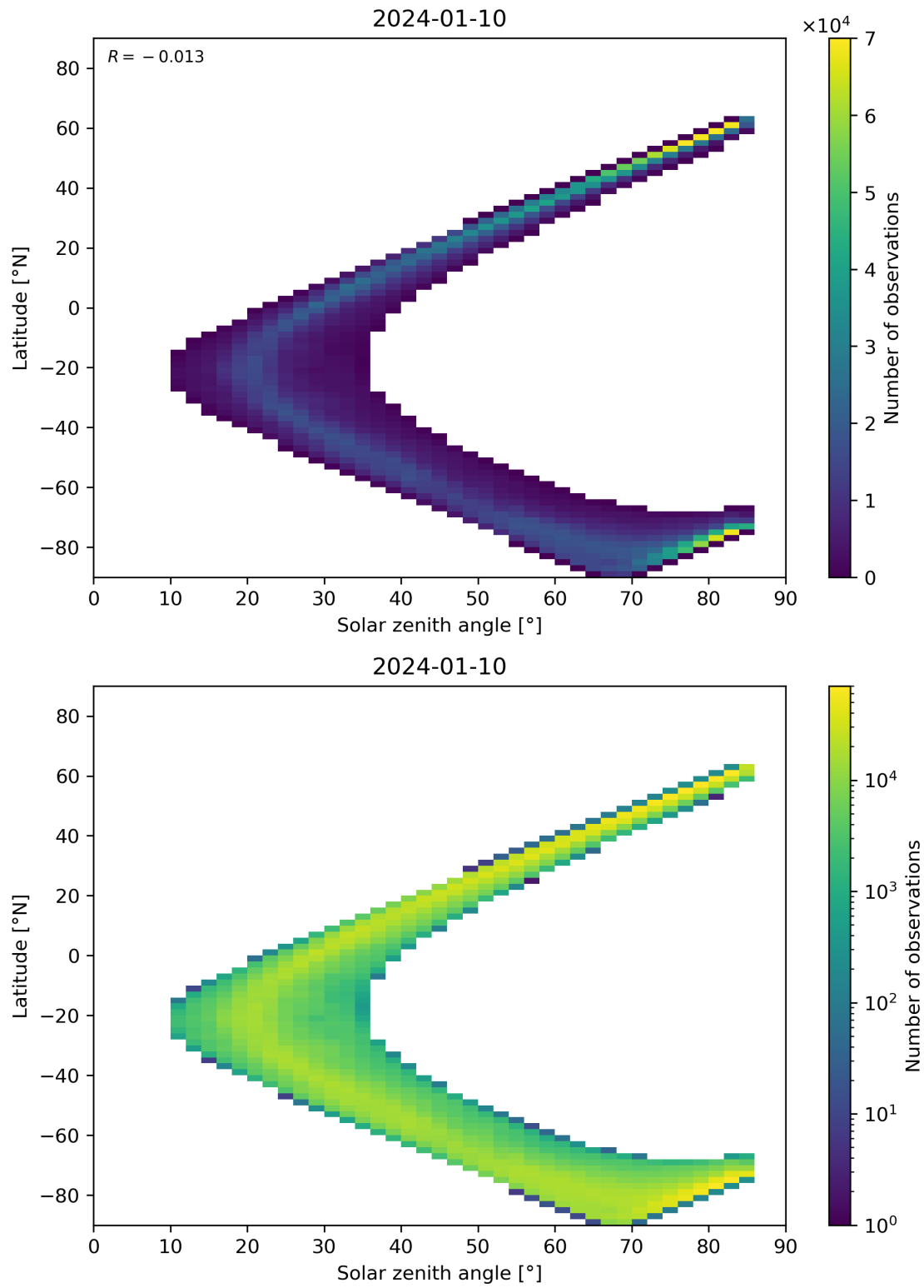
Figure 66: Scatter density plot of “Solar zenith angle” against “Latitude” for 2024-01-10 to 2024-01-11.
