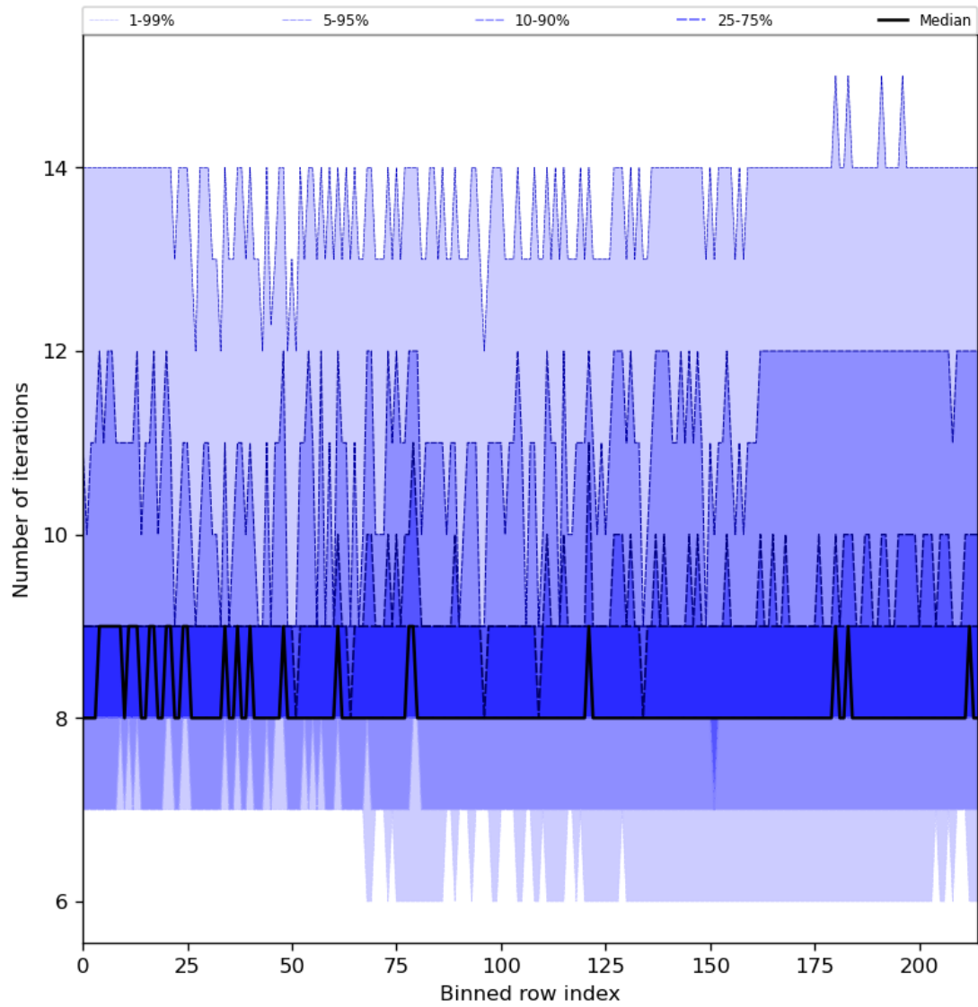
Figure 32: Along track statistics of “Number of iterations” for 2024-01-10 to 2024-01-11
