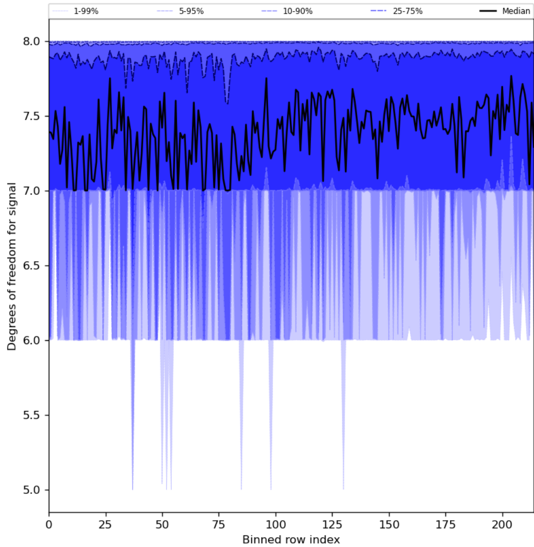
Figure 31: Along track statistics of “Degrees of freedom for signal” for 2024-01-10 to 2024-01-11
