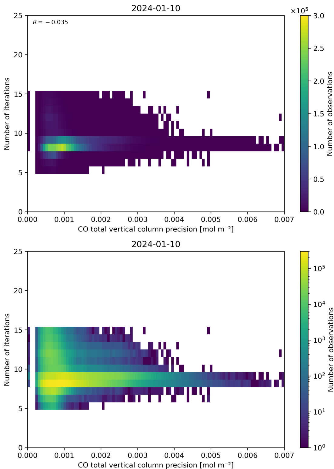
Figure 46: Scatter density plot of “CO total vertical column precision” against “Number of iterations” for 2024-01-10 to 2024-01-11.
