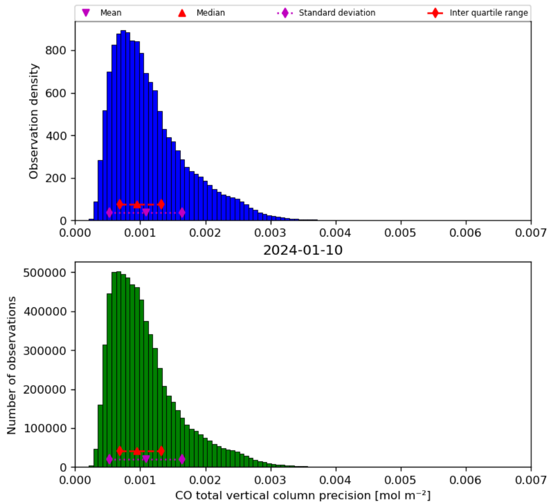
Figure 20: Histogram of “CO total vertical column precision” for 2024-01-10 to 2024-01-11
