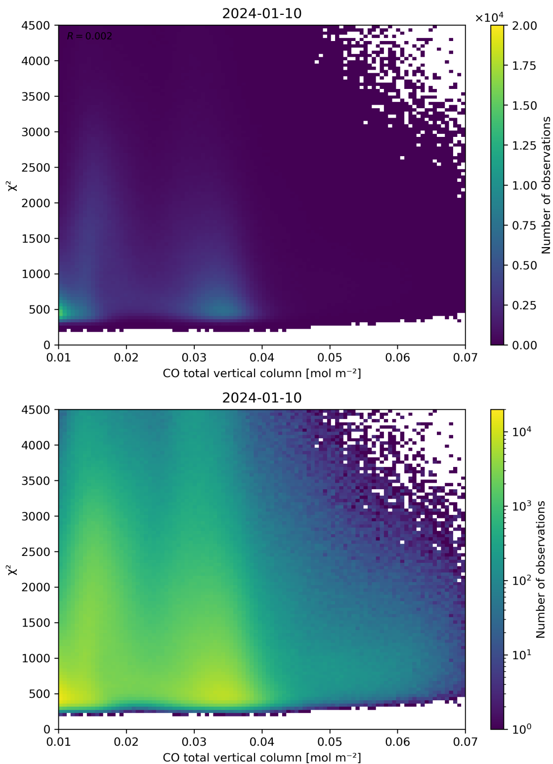
Figure 35: Scatter density plot of “CO total vertical column” against “ \chi^2 ” for 2024-01-10 to 2024-01-11.
