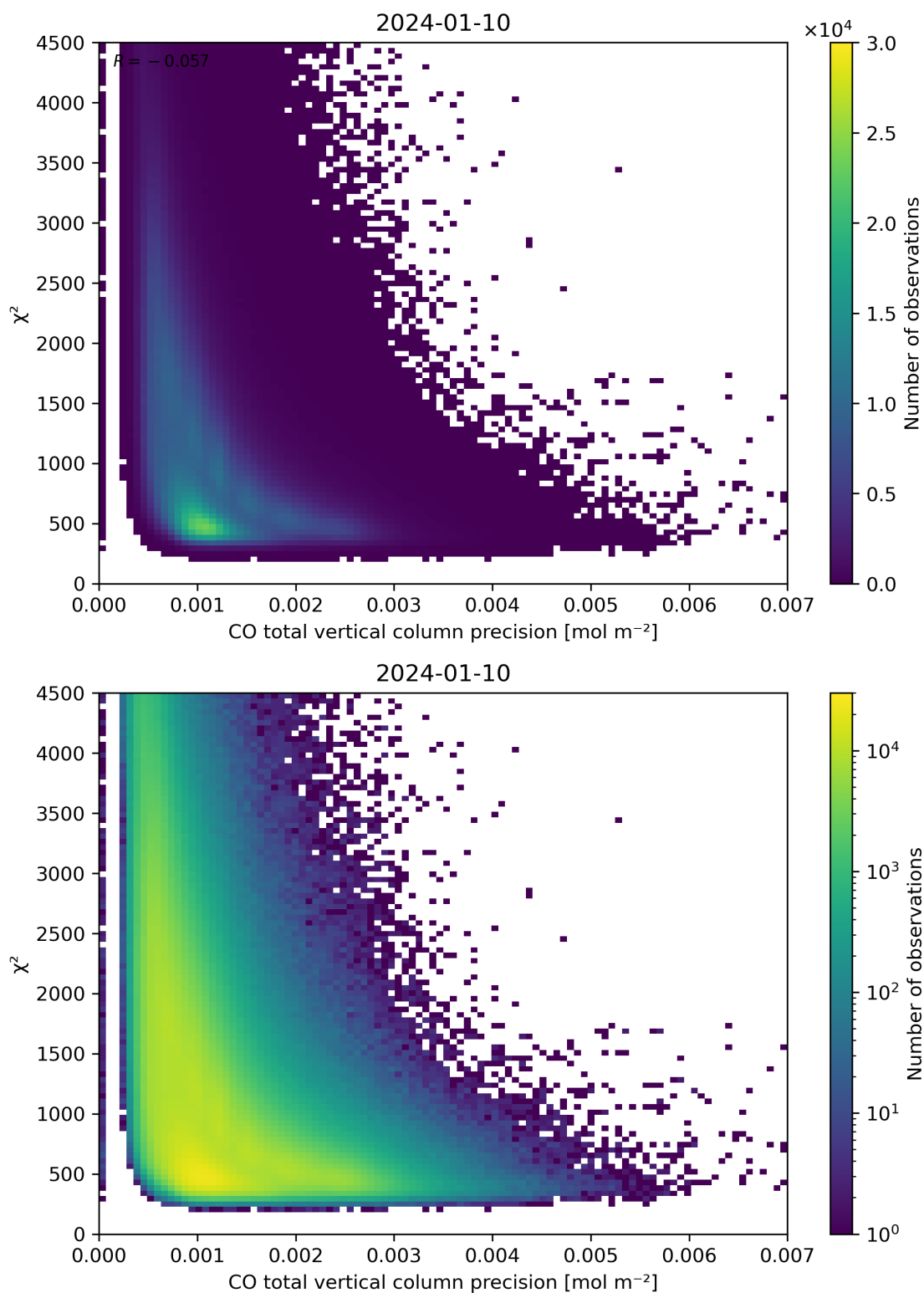
Figure 44: Scatter density plot of “CO total vertical column precision” against “ \chi^2 ” for 2024-01-10 to 2024-01-11.
