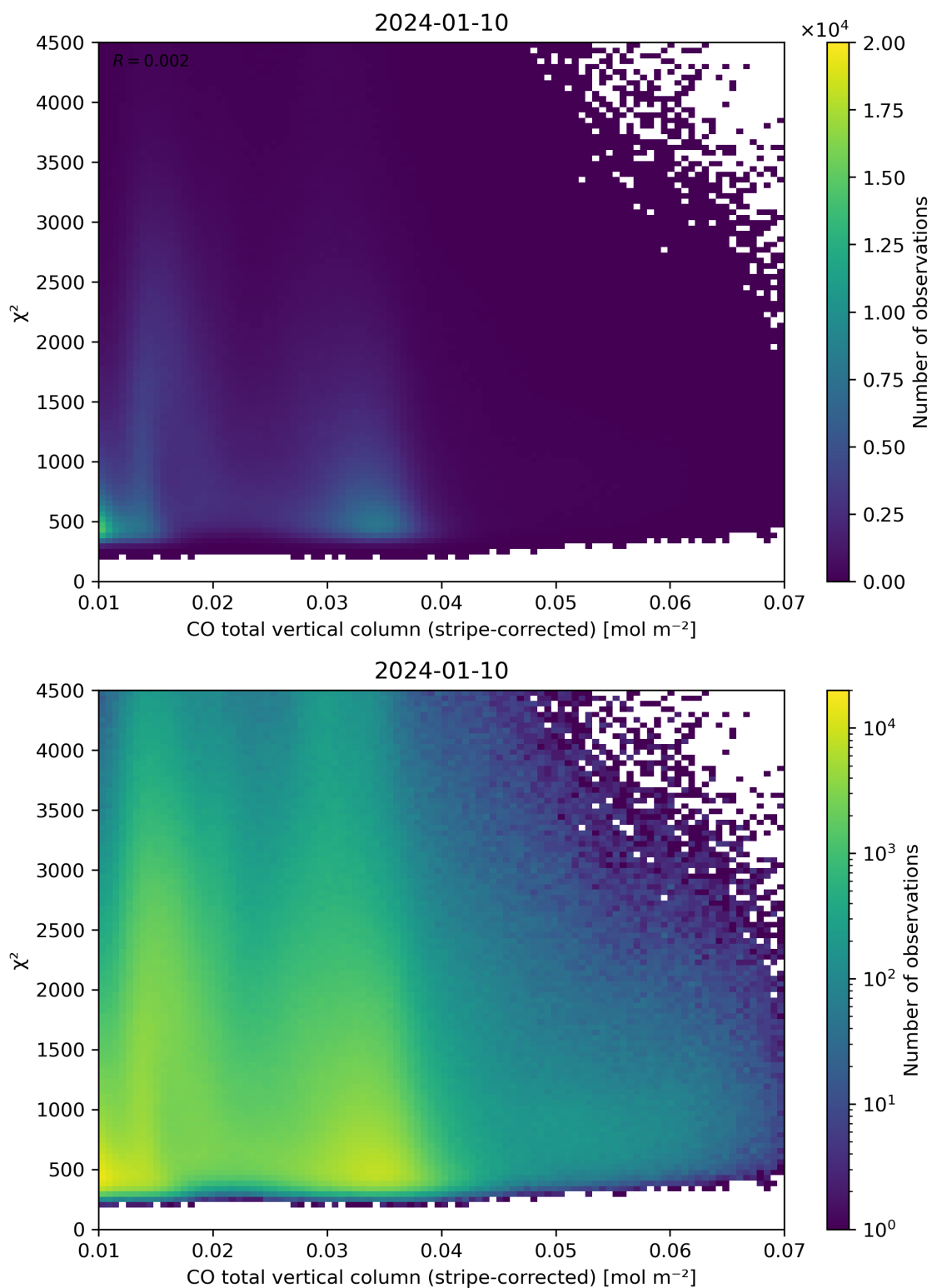
Figure 37: Scatter density plot of “CO total vertical column (stripe-corrected)” against “ \chi^2 ” for 2024-01-10 to 2024-01-11.
