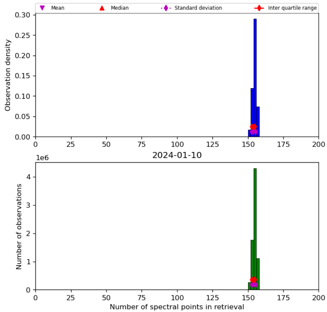
Figure 21: Histogram of “Number of spectral points in retrieval” for 2024-01-10 to 2024-01-11
