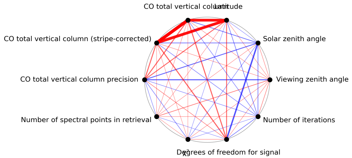
Figure 1: Map of correlation graph for 2024-01-10 to 2024-01-11.
