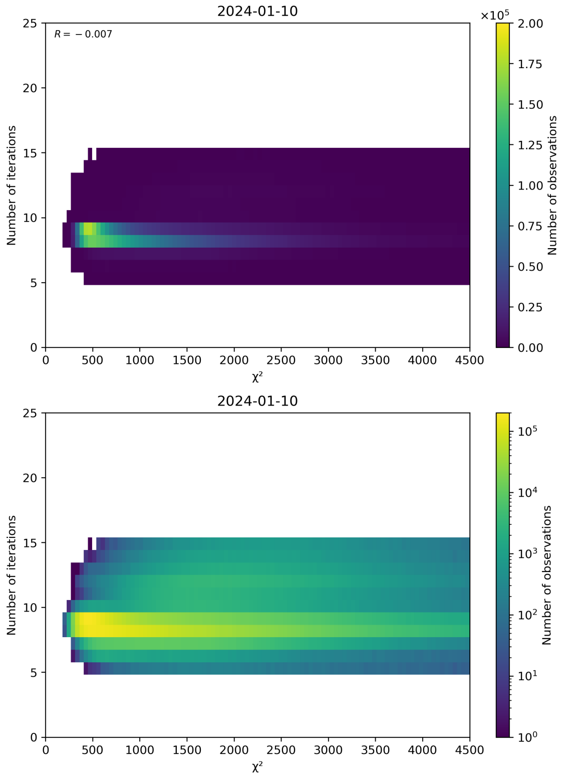
Figure 49: Scatter density plot of “ \chi^2 ” against “Number of iterations” for 2024-01-10 to 2024-01-11.
