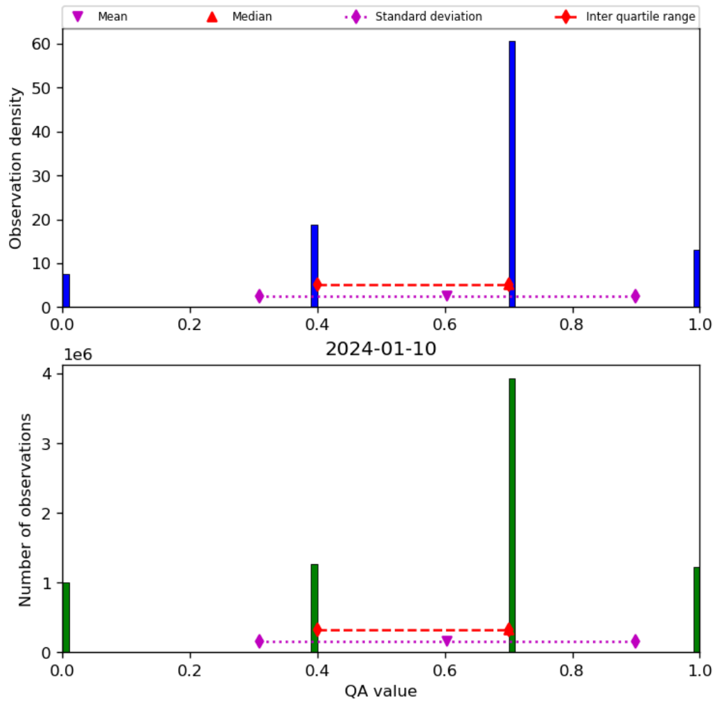
Figure 17: Histogram of “QA value” for 2024-01-10 to 2024-01-11
