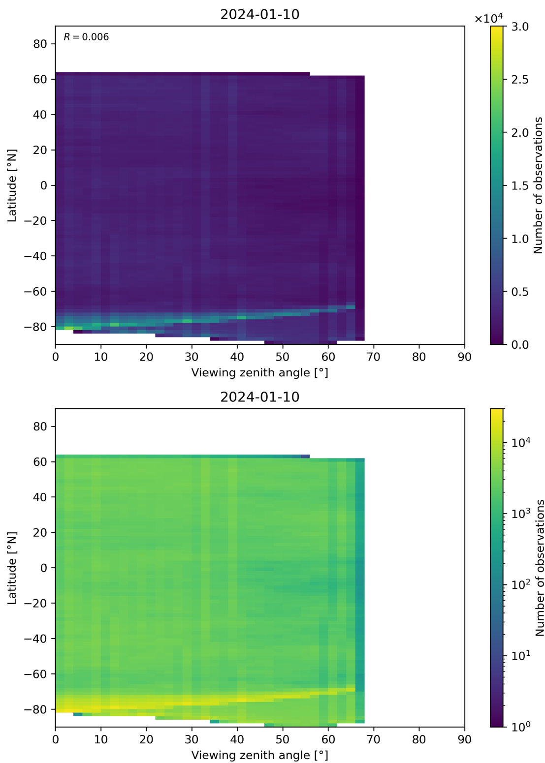
Figure 74: Scatter density plot of “Viewing zenith angle” against “Latitude” for 2024-01-10 to 2024-01-11.
