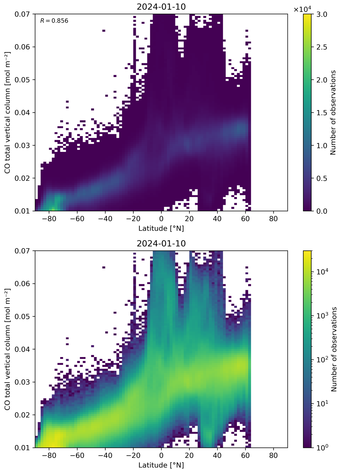
Figure 51: Scatter density plot of “Latitude” against “CO total vertical column” for 2024-01-10 to 2024-01-11.
