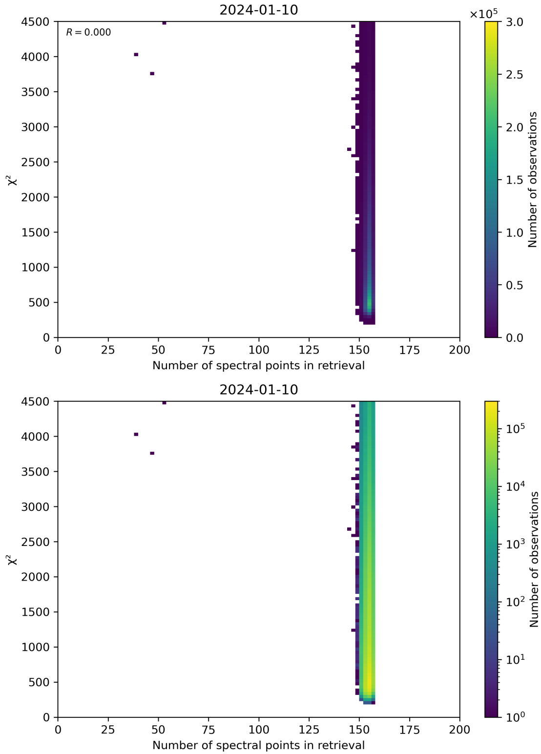
Figure 58: Scatter density plot of “Number of spectral points in retrieval” against “ \chi^2 ” for 2024-01-10 to 2024-01-11.
