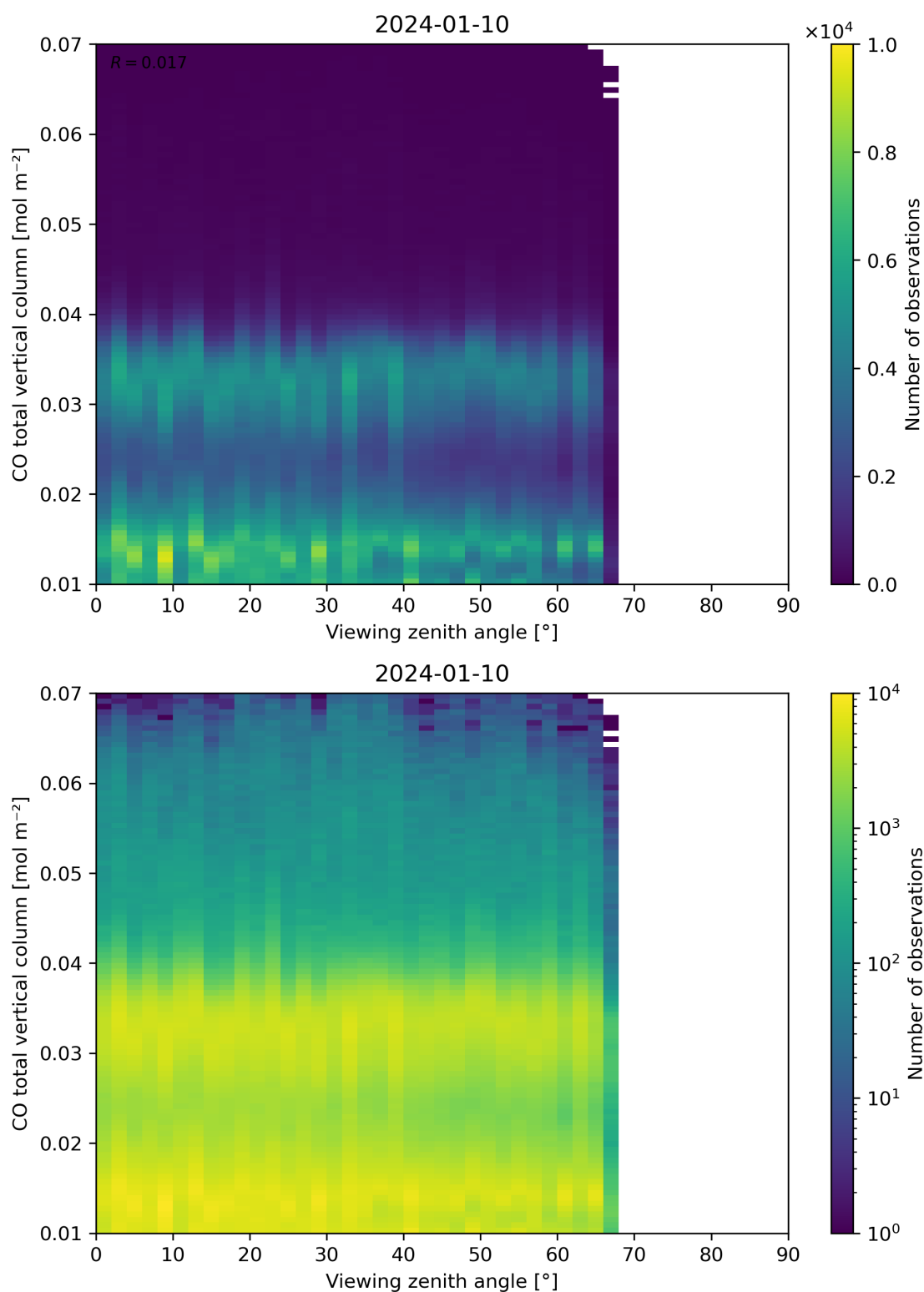
Figure 69: Scatter density plot of “Viewing zenith angle” against “CO total vertical column” for 2024-01-10 to 2024-01-11.
