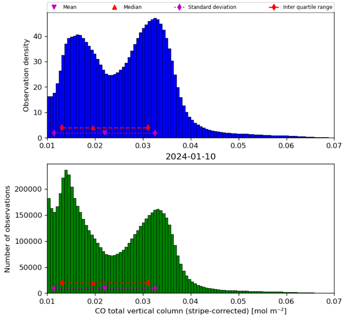
Figure 19: Histogram of “CO total vertical column (stripe-corrected)” for 2024-01-10 to 2024-01-11
