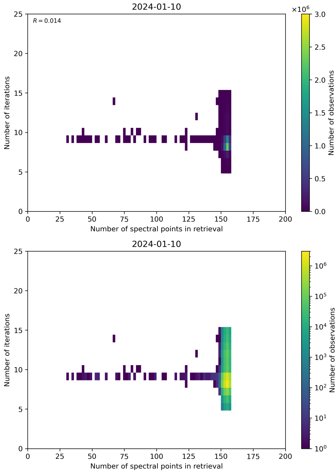
Figure 60: Scatter density plot of “Number of spectral points in retrieval” against “Number of iterations” for 2024-01-10 to 2024-01-11.
