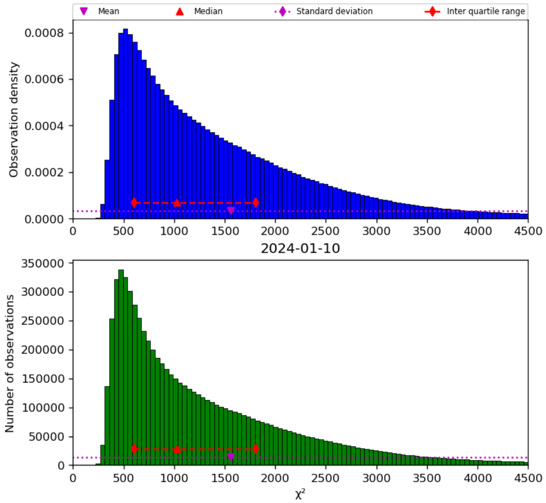
Figure 22: Histogram of “ \chi^2 ” for 2024-01-10 to 2024-01-11
