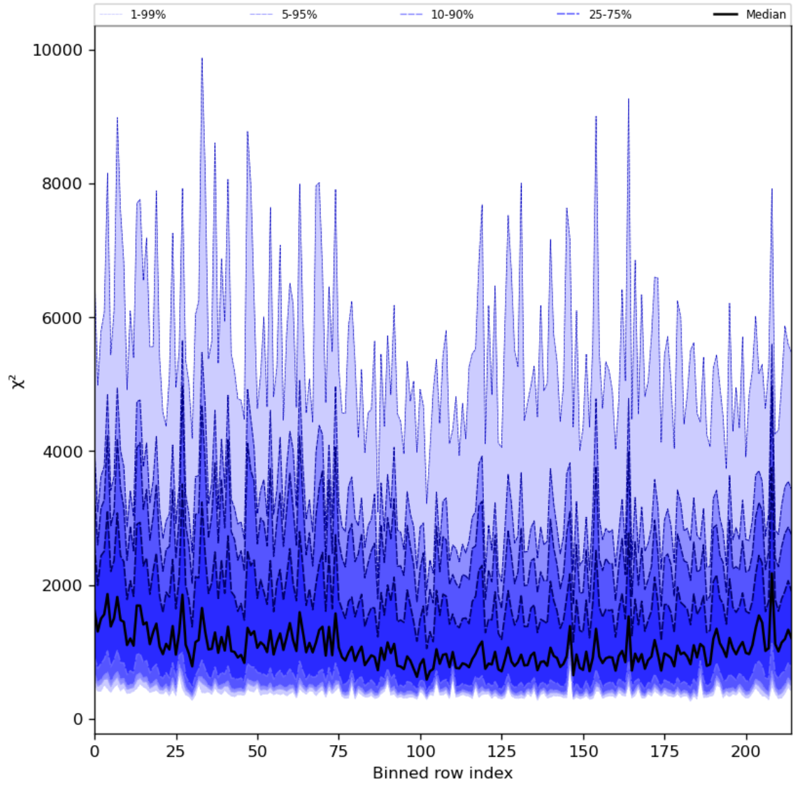
Figure 30: Along track statistics of “ \chi^2 ” for 2024-01-10 to 2024-01-11
