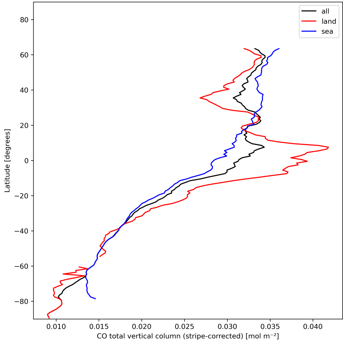
Figure 11: Zonal average of “CO total vertical column (stripe-corrected)” for 2024-01-10 to 2024-01-11.
