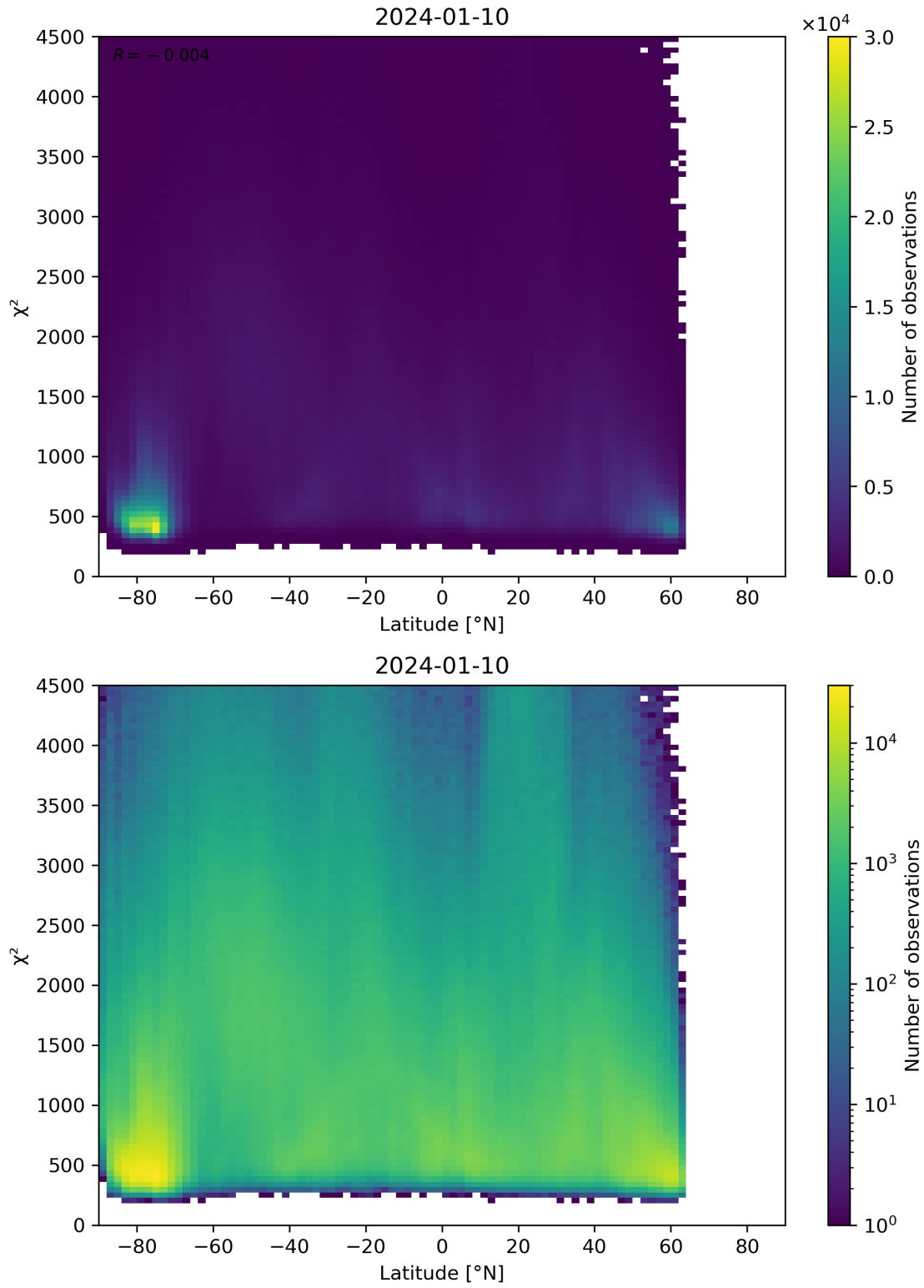
Figure 54: Scatter density plot of “Latitude” against “ \chi^2 ” for 2024-01-10 to 2024-01-11.
