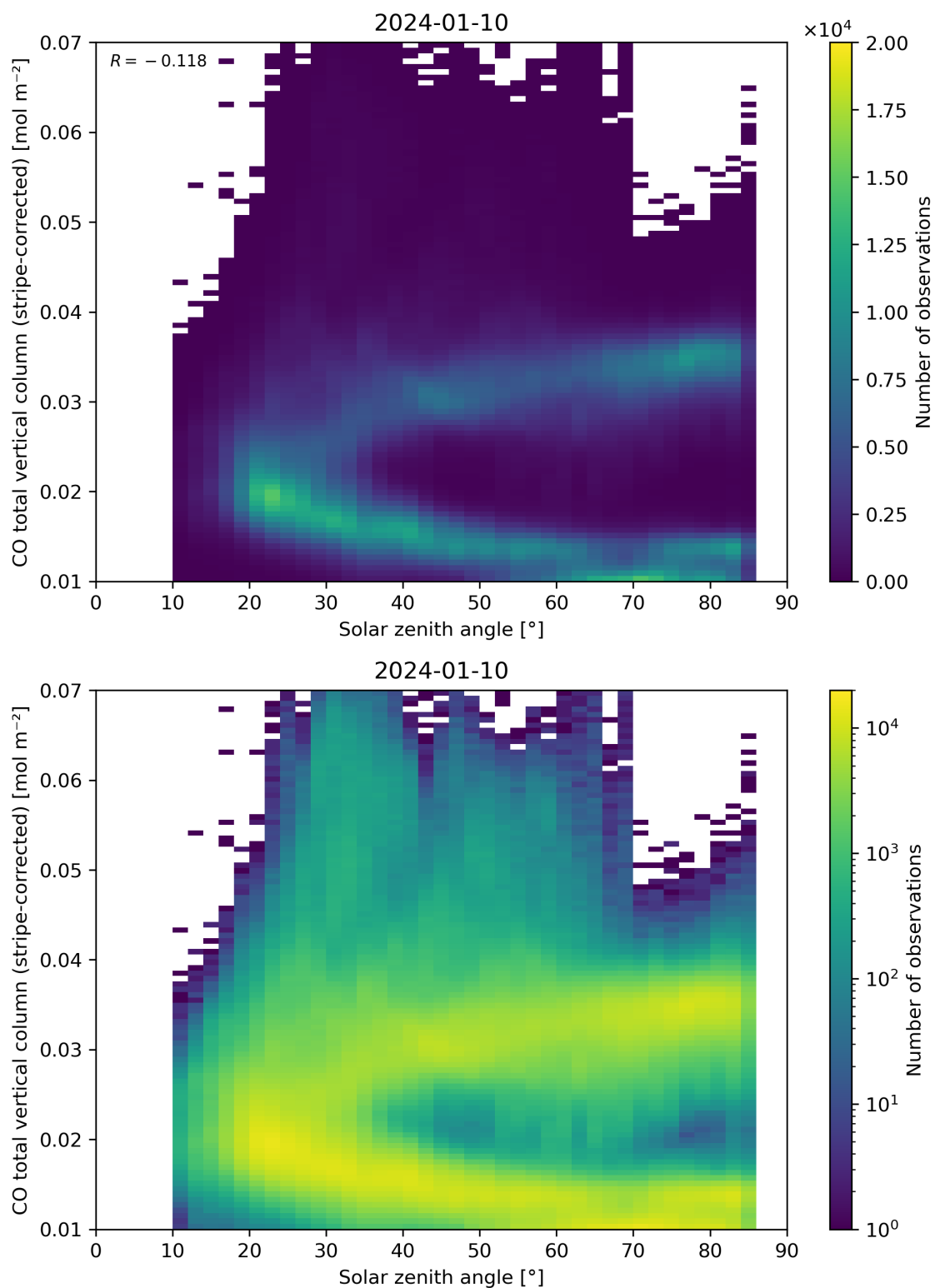
Figure 62: Scatter density plot of “Solar zenith angle” against “CO total vertical column (stripe-corrected)” for 2024-01-10 to 2024-01-11.
