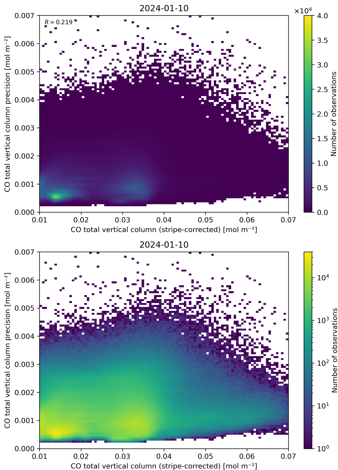
Figure 36: Scatter density plot of “CO total vertical column (stripe-corrected)” against “CO total vertical column precision” for 2024-01-10 to 2024-01-11.
