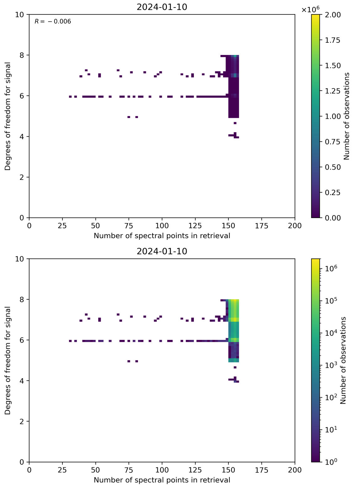
Figure 59: Scatter density plot of “Number of spectral points in retrieval” against “Degrees of freedom for signal” for 2024-01-10 to 2024-01-11.
