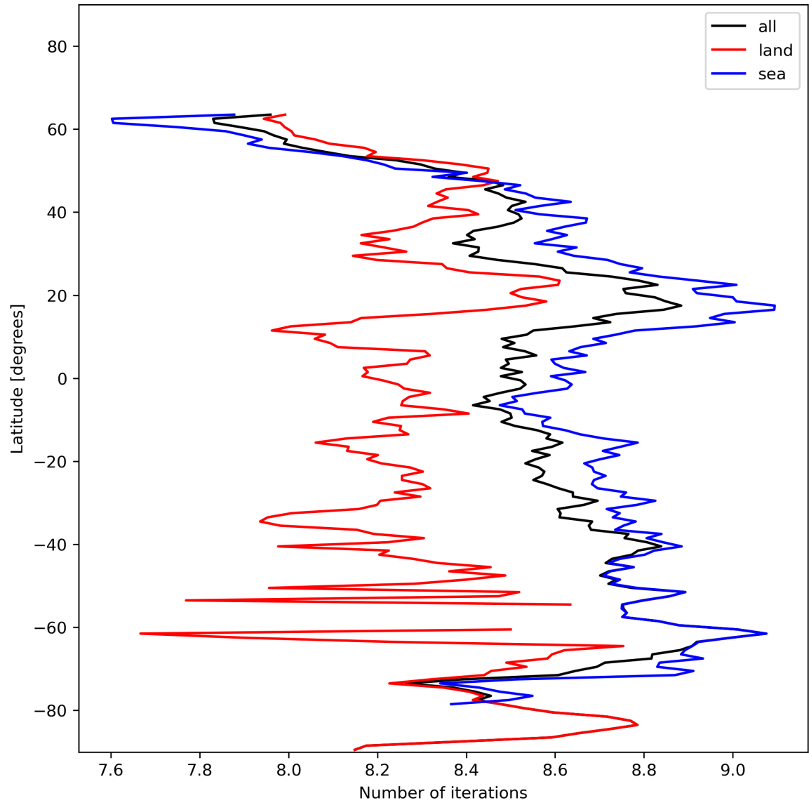
Figure 16: Zonal average of “Number of iterations” for 2024-01-10 to 2024-01-11.
