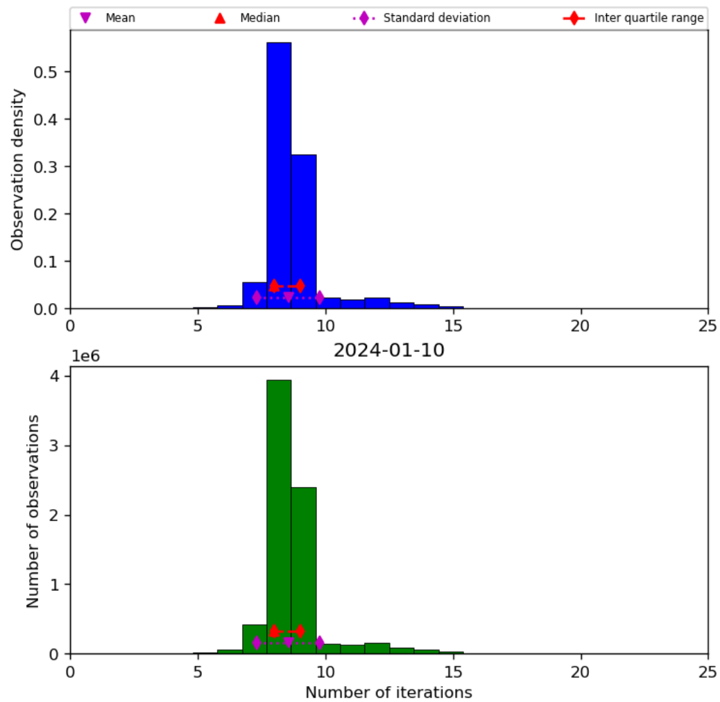
Figure 24: Histogram of “Number of iterations” for 2024-01-10 to 2024-01-11
