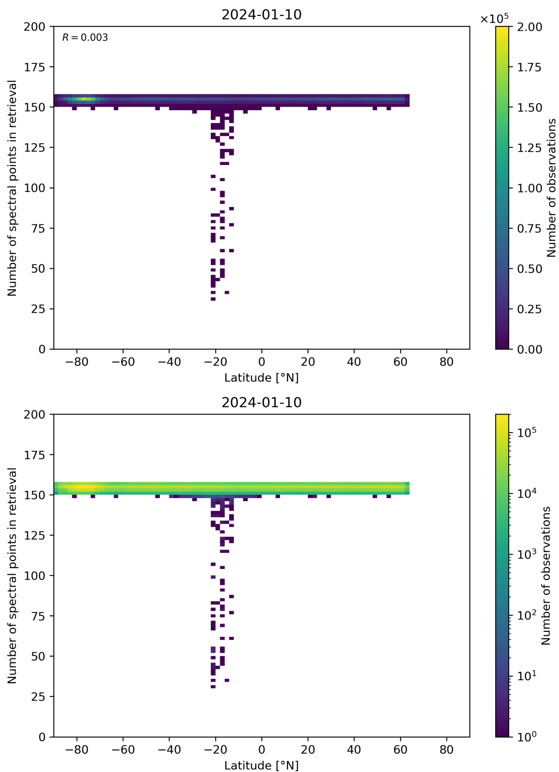
Figure 57: Scatter density plot of “Latitude” against “Number of spectral points in retrieval” for 2024-01-10 to 2024-01-11.
