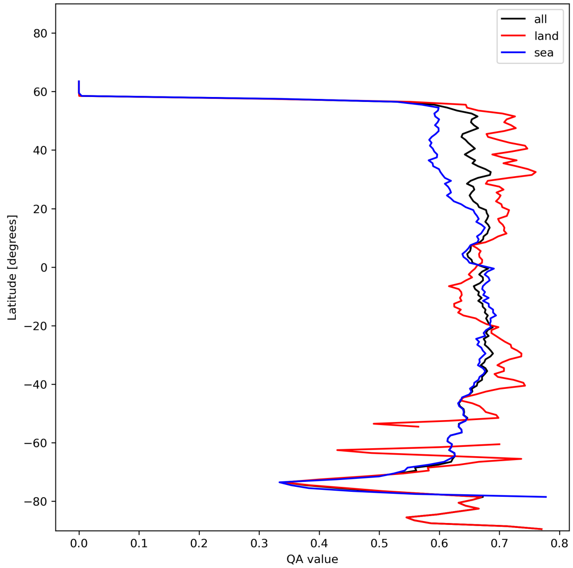
Figure 9: Zonal average of “QA value” for 2024-01-10 to 2024-01-11.
