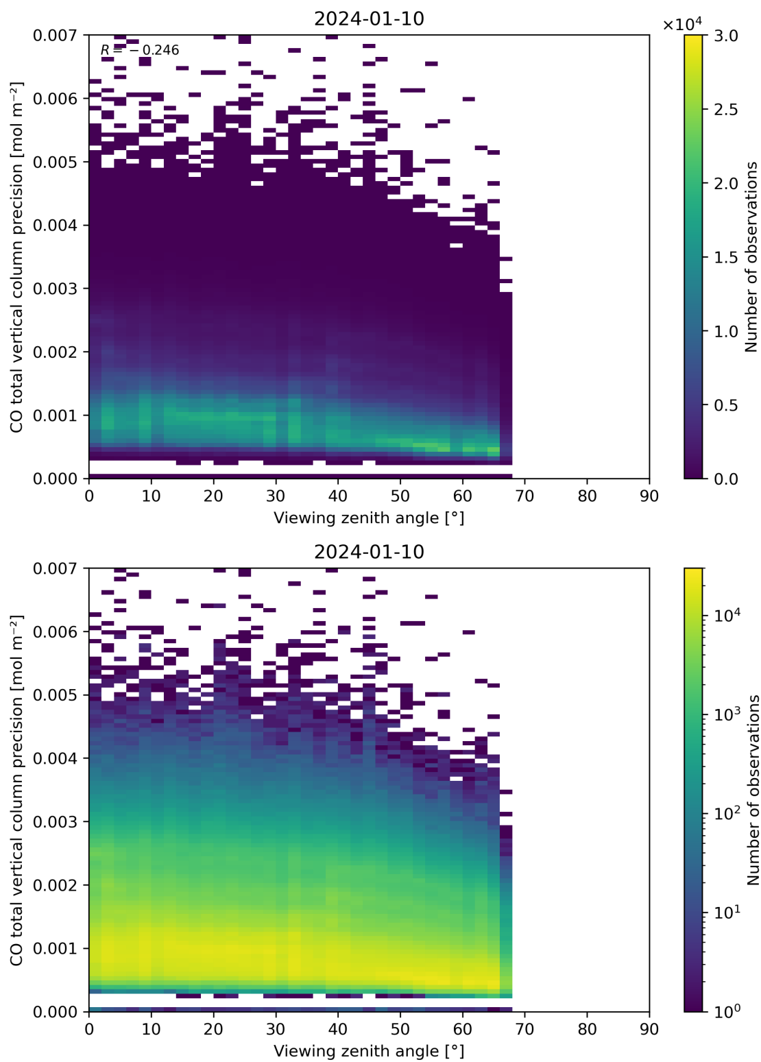
Figure 71: Scatter density plot of “Viewing zenith angle” against “CO total vertical column precision” for 2024-01-10 to 2024-01-11.
