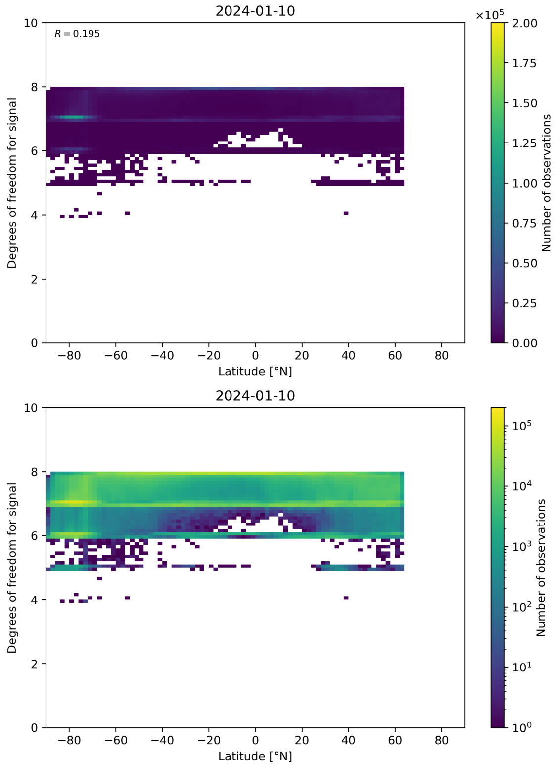
Figure 55: Scatter density plot of “Latitude” against “Degrees of freedom for signal” for 2024-01-10 to 2024-01-11.
