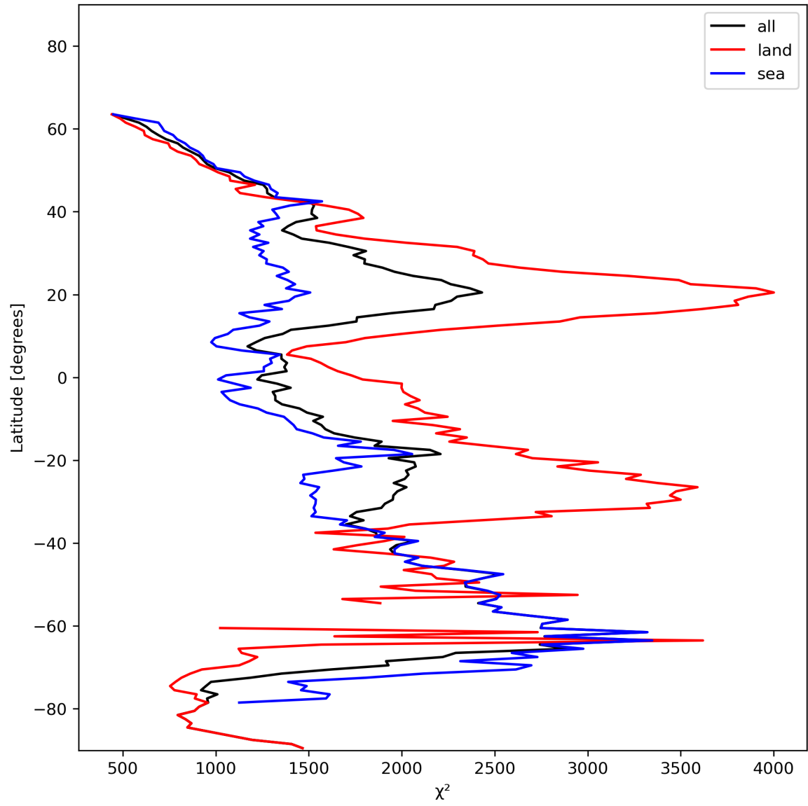
Figure 14: Zonal average of “ \chi^2 ” for 2024-01-10 to 2024-01-11.
