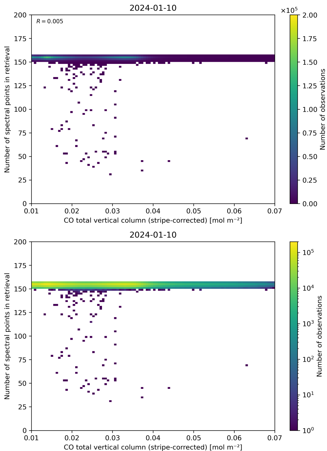
Figure 40: Scatter density plot of “CO total vertical column (stripe-corrected)” against “Number of spectral points in retrieval” for 2024-01-10 to 2024-01-11.
