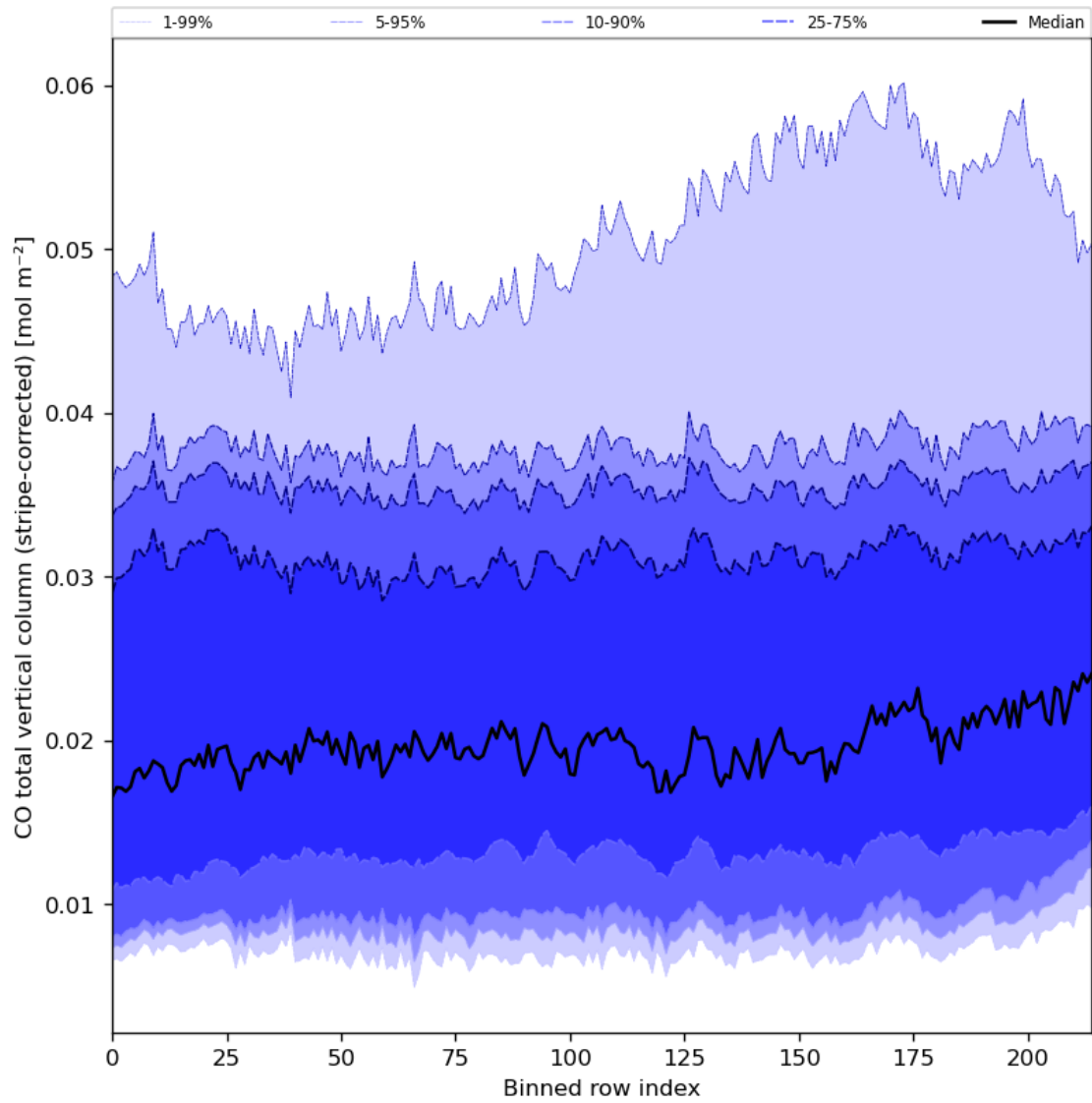
Figure 27: Along track statistics of “CO total vertical column (stripe-corrected)” for 2024-01-10 to 2024-01-11
