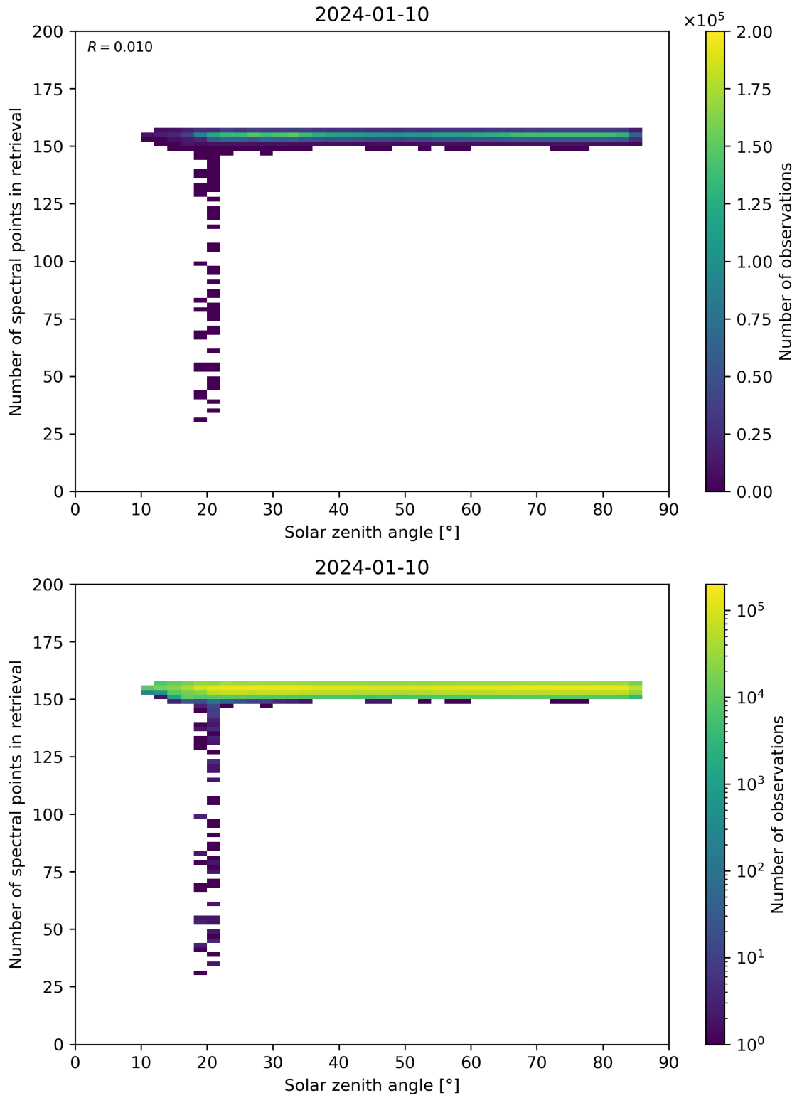
Figure 68: Scatter density plot of “Solar zenith angle” against “Number of spectral points in retrieval” for 2024-01-10 to 2024-01-11.
