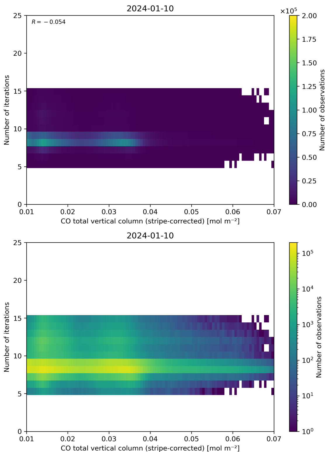
Figure 39: Scatter density plot of “CO total vertical column (stripe-corrected)” against “Number of iterations” for 2024-01-10 to 2024-01-11.
