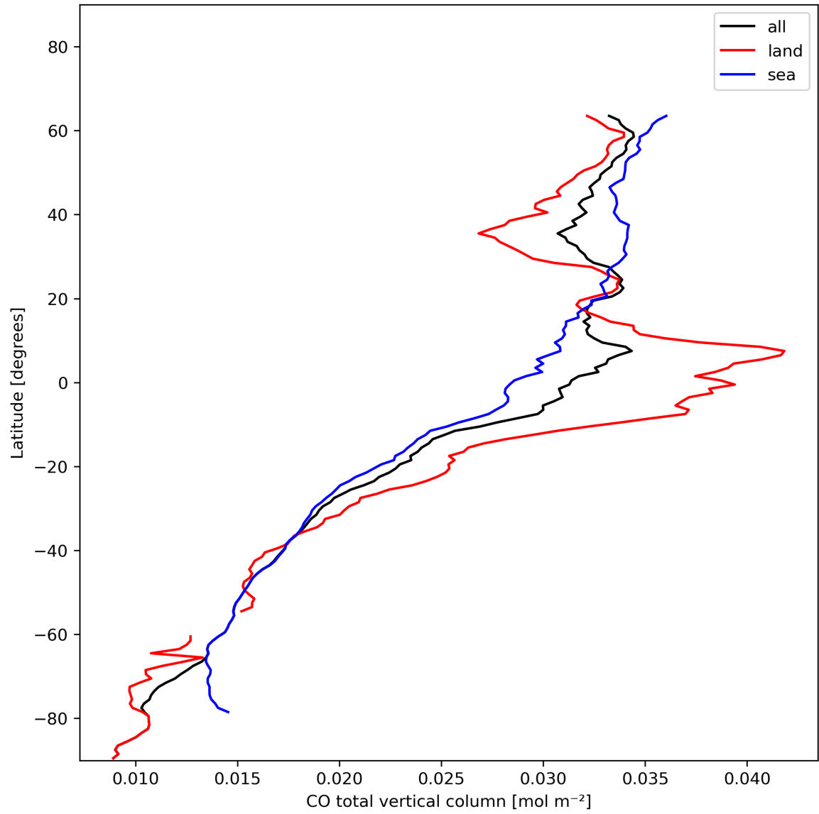
Figure 10: Zonal average of “CO total vertical column” for 2024-01-10 to 2024-01-11.
