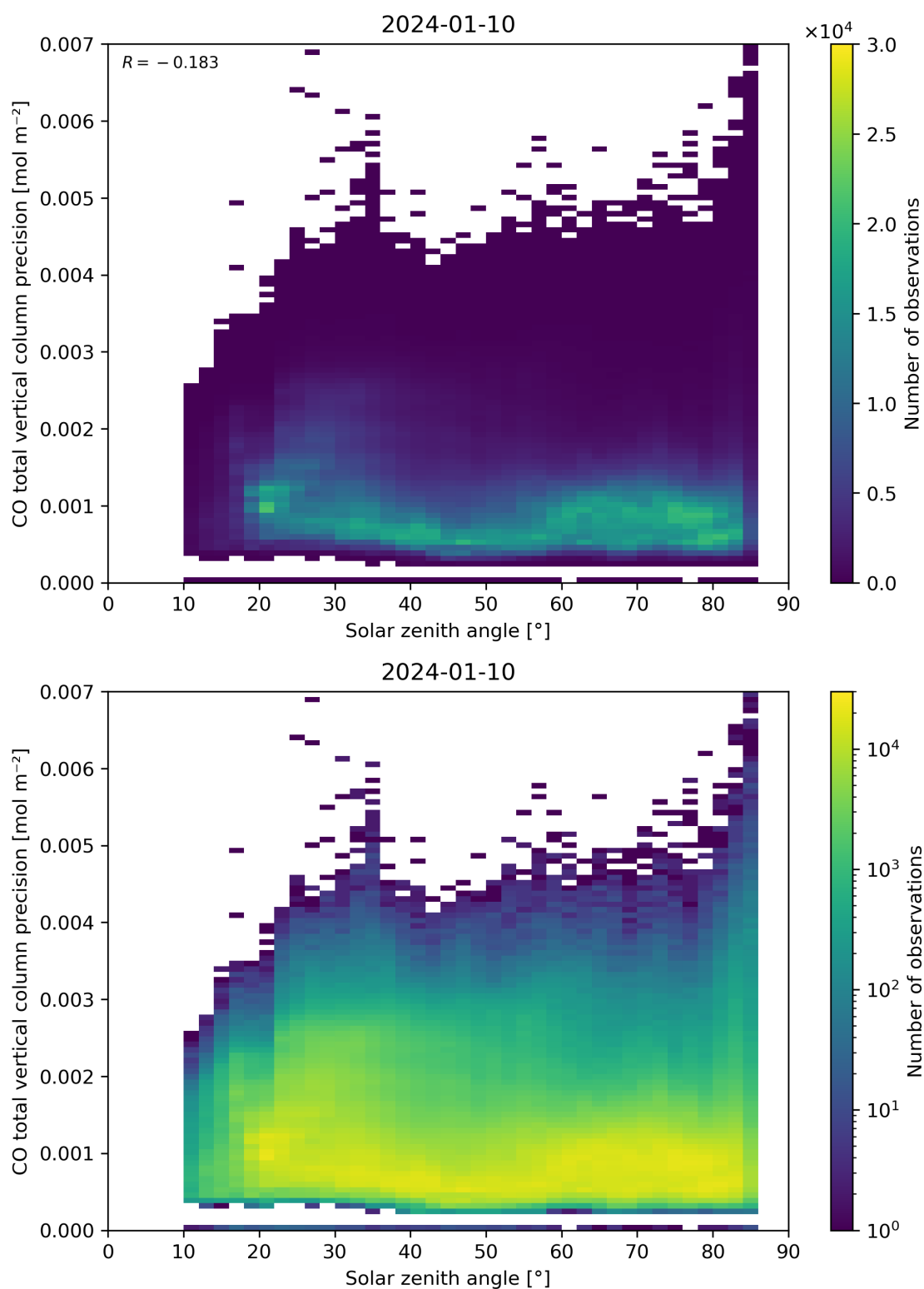
Figure 63: Scatter density plot of “Solar zenith angle” against “CO total vertical column precision” for 2024-01-10 to 2024-01-11.
