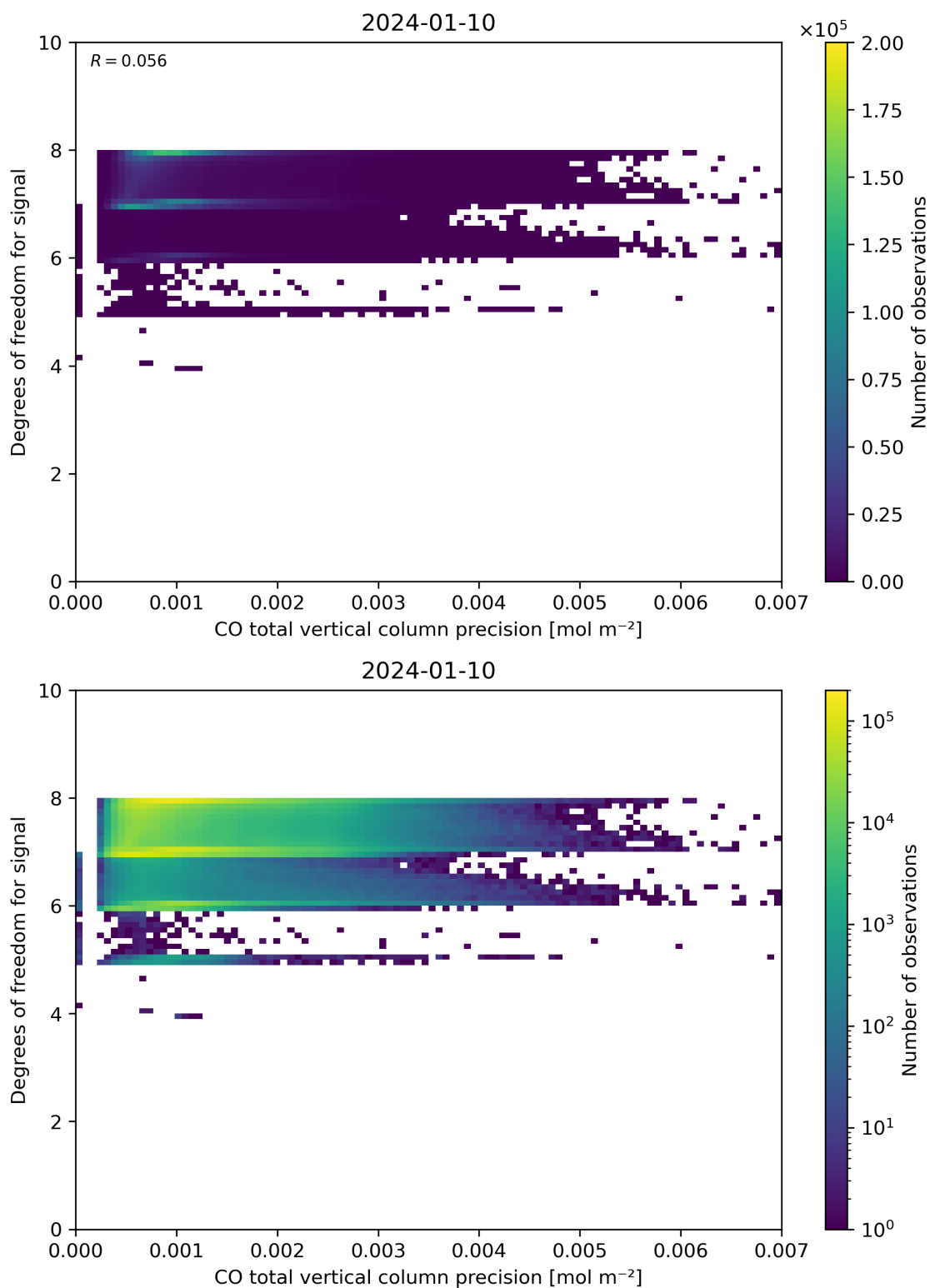
Figure 45: Scatter density plot of “CO total vertical column precision” against “Degrees of freedom for signal” for 2024-01-10 to 2024-01-11.
