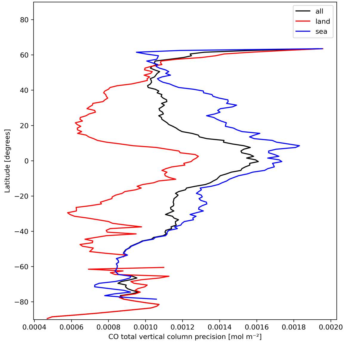
Figure 12: Zonal average of “CO total vertical column precision” for 2024-01-10 to 2024-01-11.
