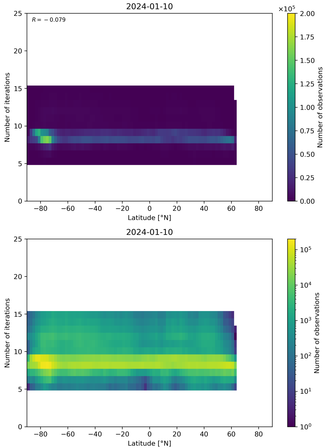
Figure 56: Scatter density plot of “Latitude” against “Number of iterations” for 2024-01-10 to 2024-01-11.
