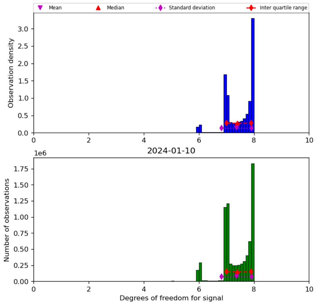
Figure 23: Histogram of “Degrees of freedom for signal” for 2024-01-10 to 2024-01-11
