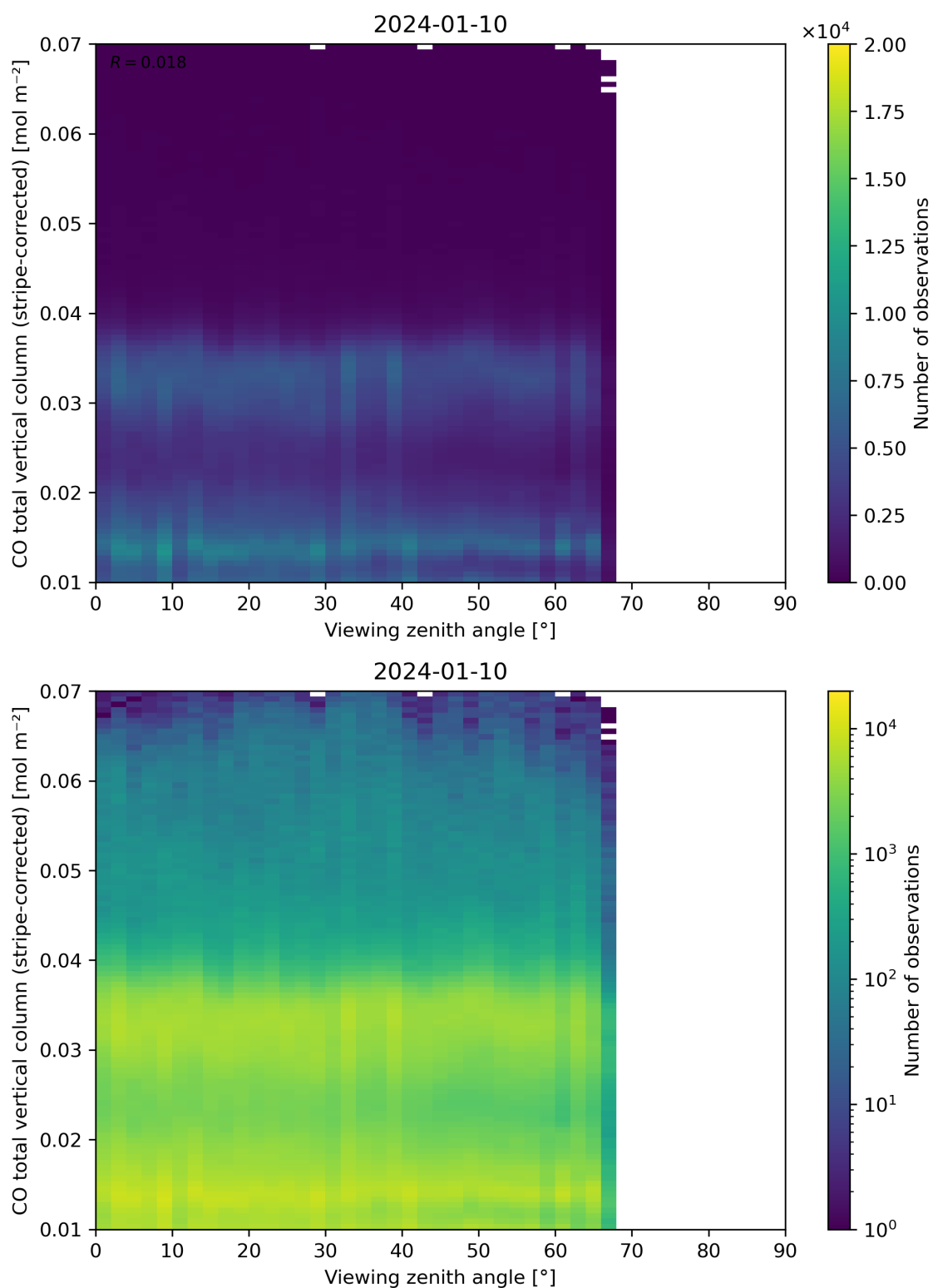
Figure 70: Scatter density plot of “Viewing zenith angle” against “CO total vertical column (stripe-corrected)” for 2024-01-10 to 2024-01-11.
