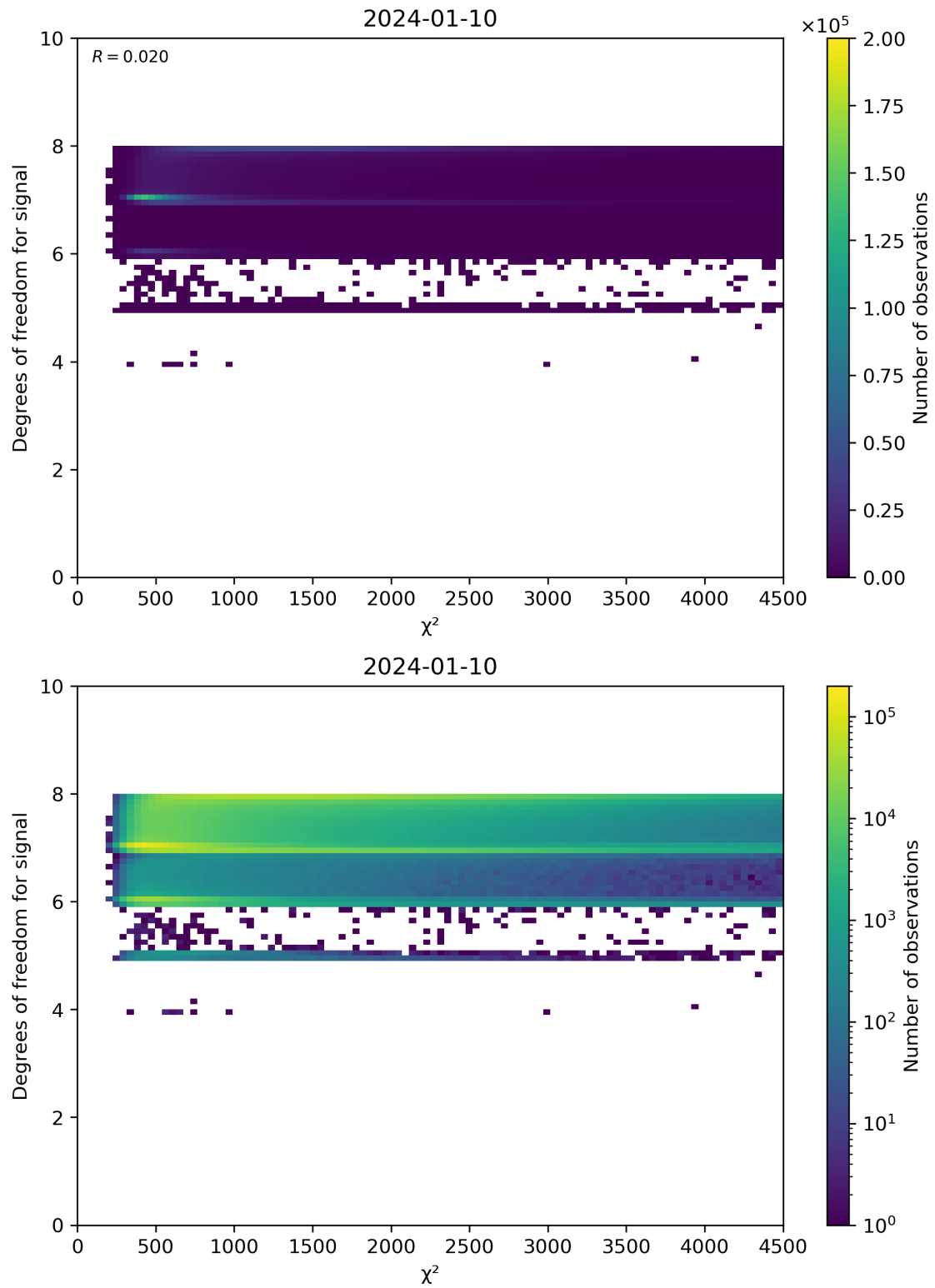
Figure 48: Scatter density plot of “ \chi^2 ” against “Degrees of freedom for signal” for 2024-01-10 to 2024-01-11.
