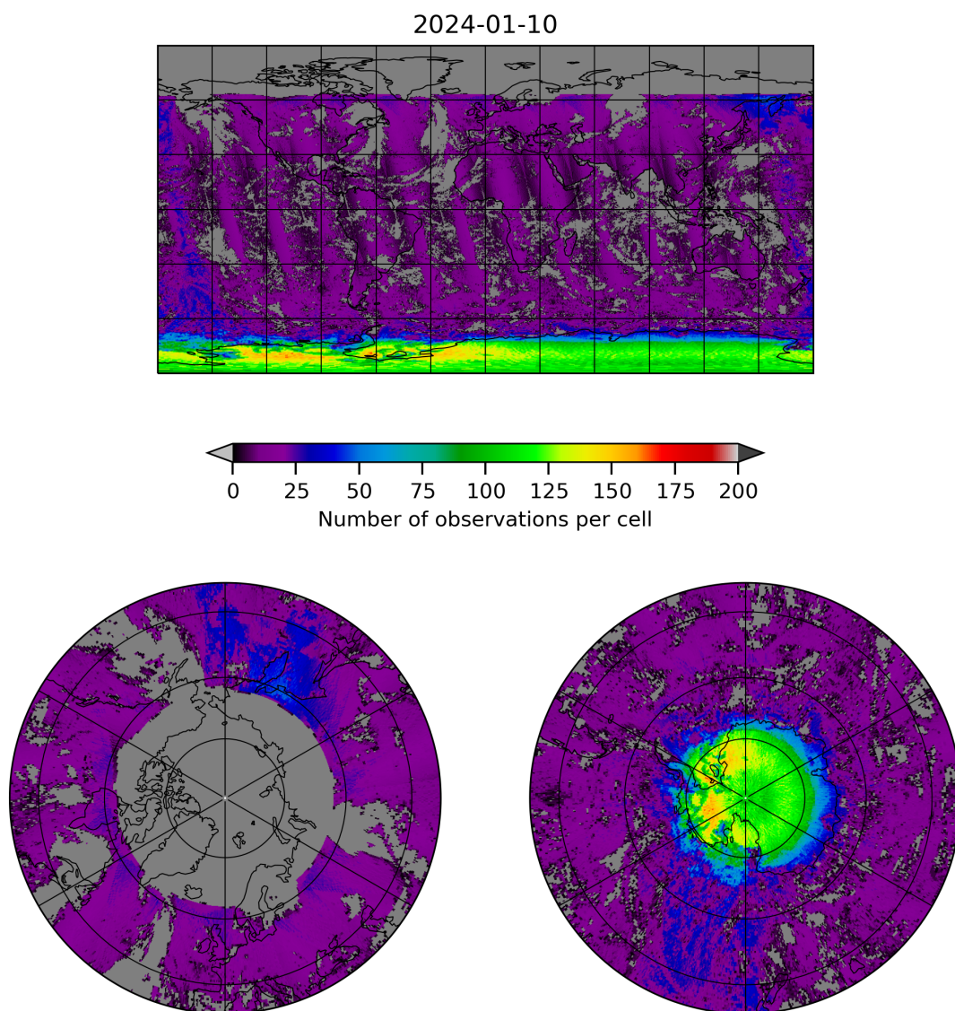
Figure 8: Map of the number of observations for 2024-01-10 to 2024-01-11
