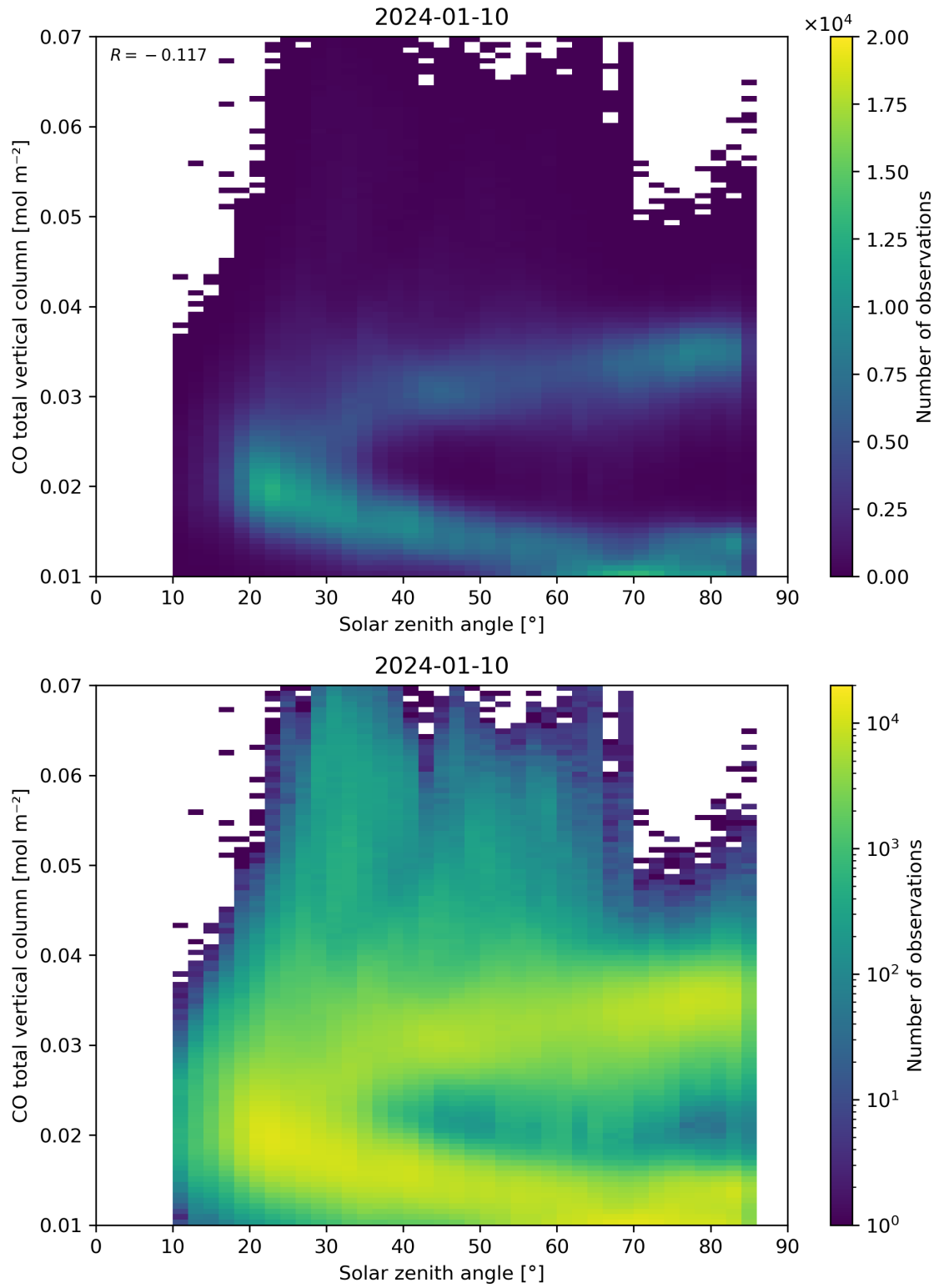
Figure 61: Scatter density plot of “Solar zenith angle” against “CO total vertical column” for 2024-01-10 to 2024-01-11.
