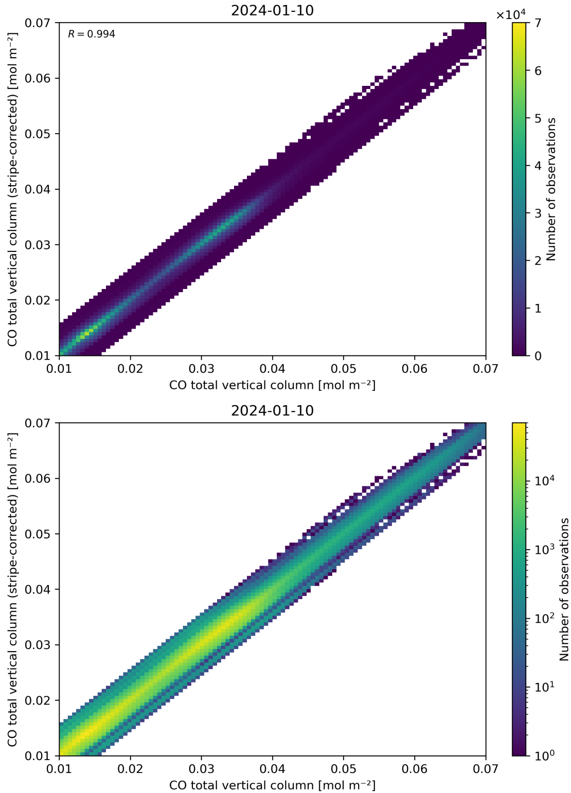
Figure 33: Scatter density plot of “CO total vertical column” against “CO total vertical column (stripe-corrected)” for 2024-01-10 to 2024-01-11.
