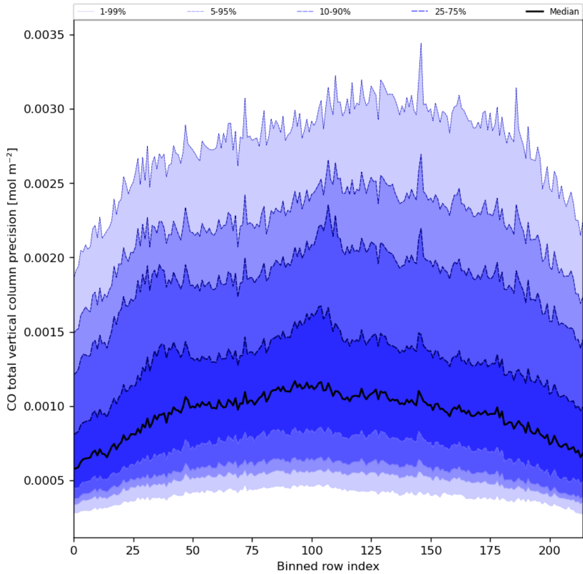
Figure 28: Along track statistics of “CO total vertical column precision” for 2024-01-10 to 2024-01-11
