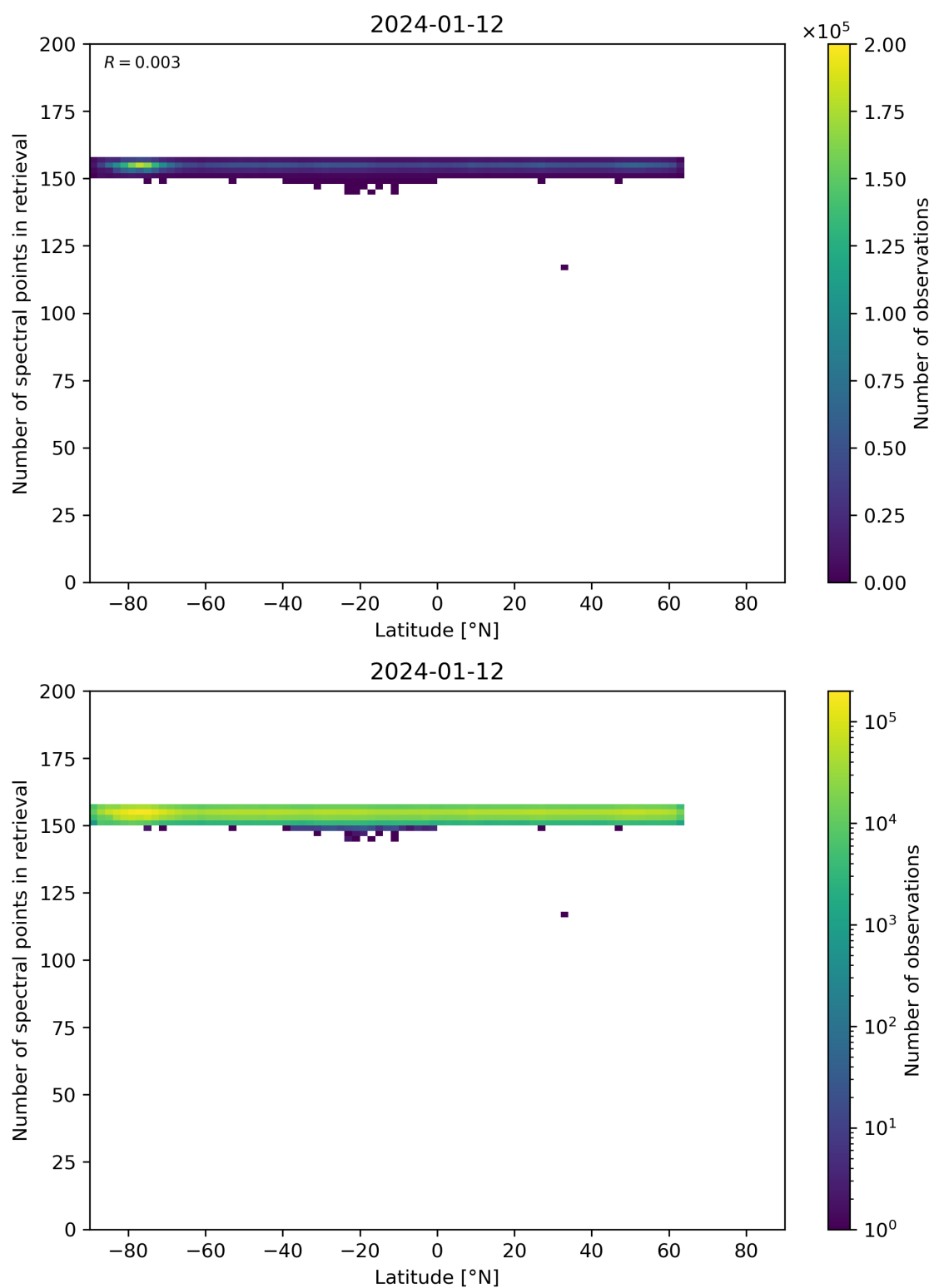
Figure 57: Scatter density plot of “Latitude” against “Number of spectral points in retrieval” for 2024-01-11 to 2024-01-13.
