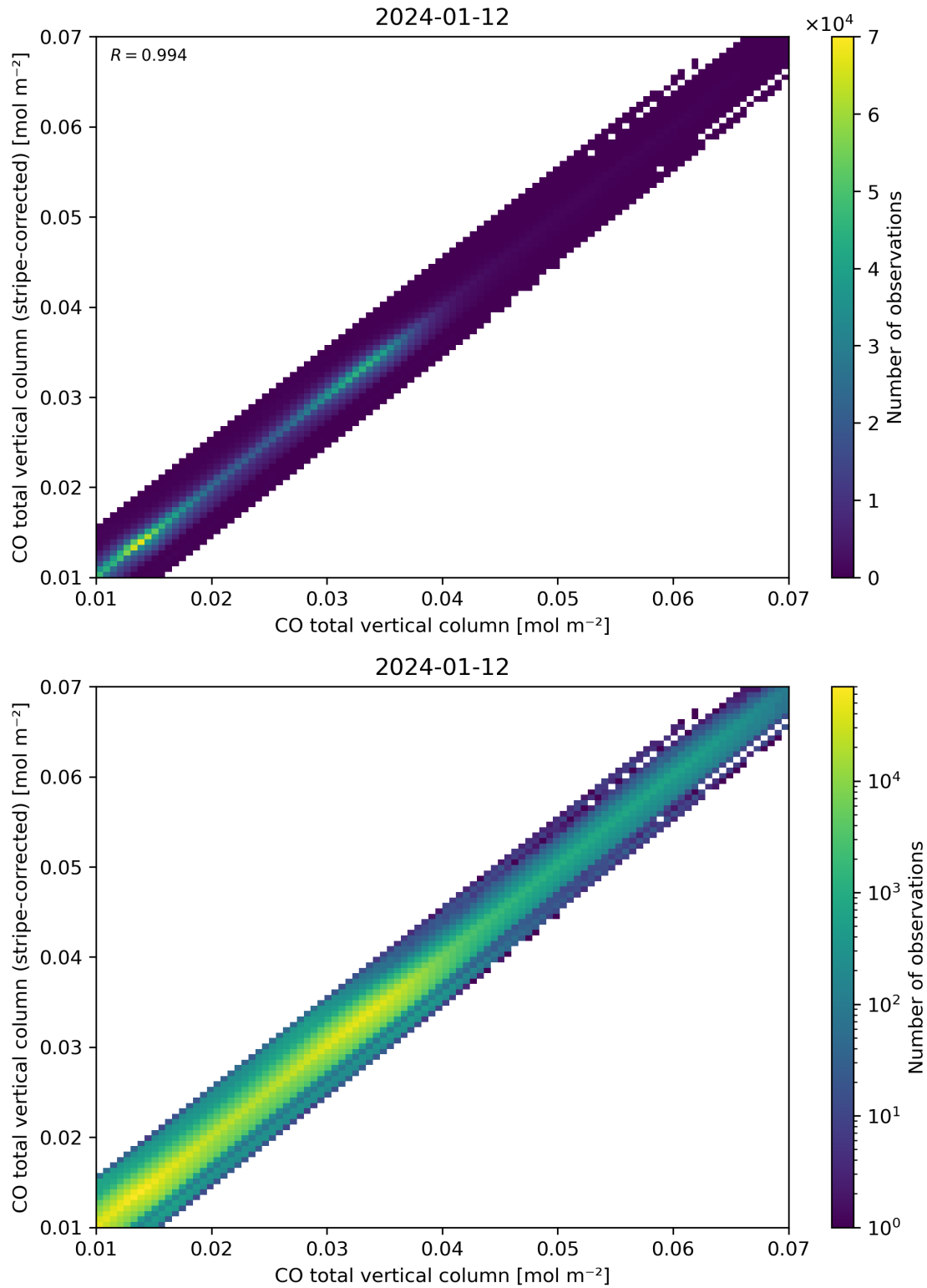
Figure 33: Scatter density plot of “CO total vertical column” against “CO total vertical column (stripe-corrected)” for 2024-01-11 to 2024-01-13.
