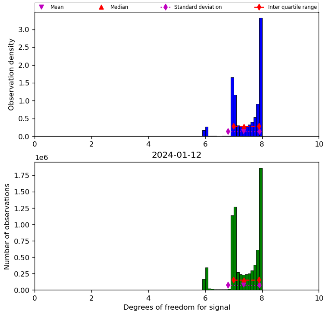
Figure 23: Histogram of “Degrees of freedom for signal” for 2024-01-11 to 2024-01-13
