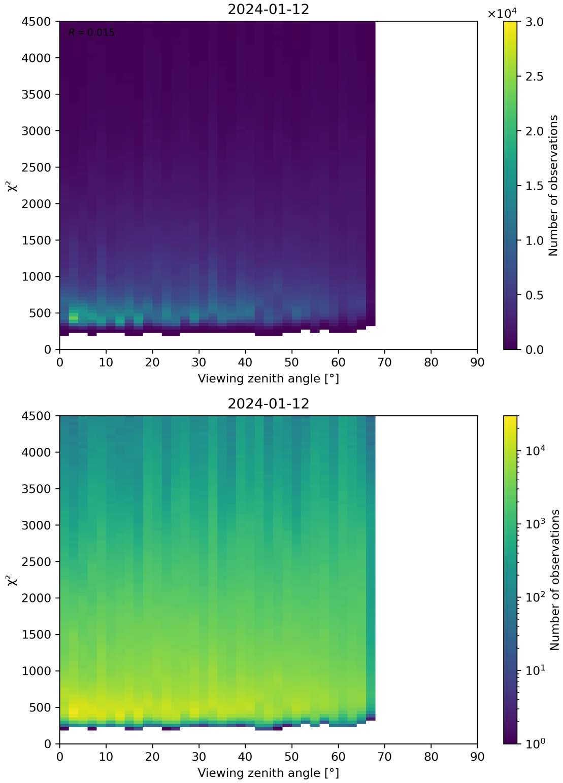
Figure 72: Scatter density plot of “Viewing zenith angle” against “ \chi^2 ” for 2024-01-11 to 2024-01-13.
