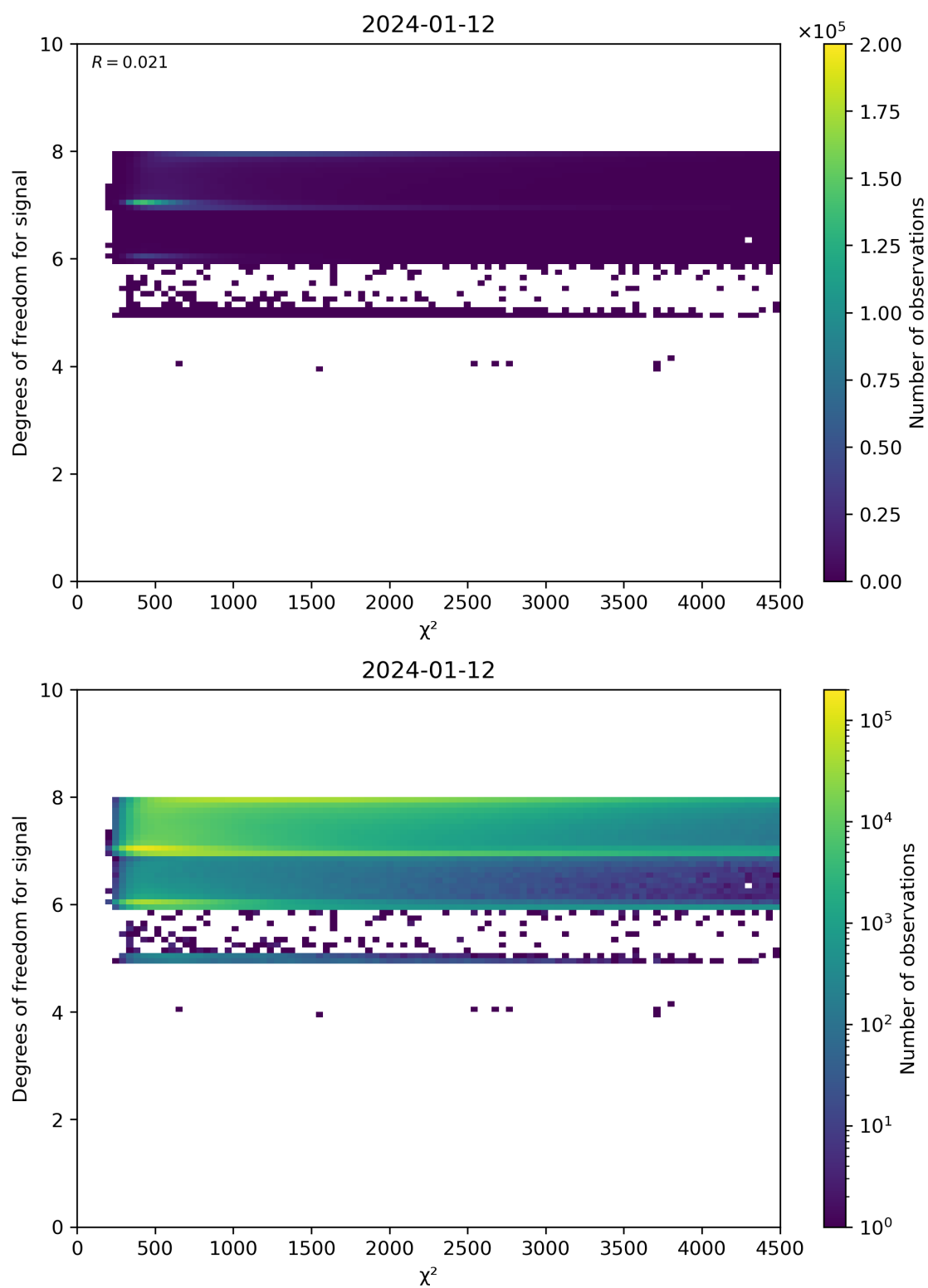
Figure 48: Scatter density plot of “ \chi^2 ” against “Degrees of freedom for signal” for 2024-01-11 to 2024-01-13.
