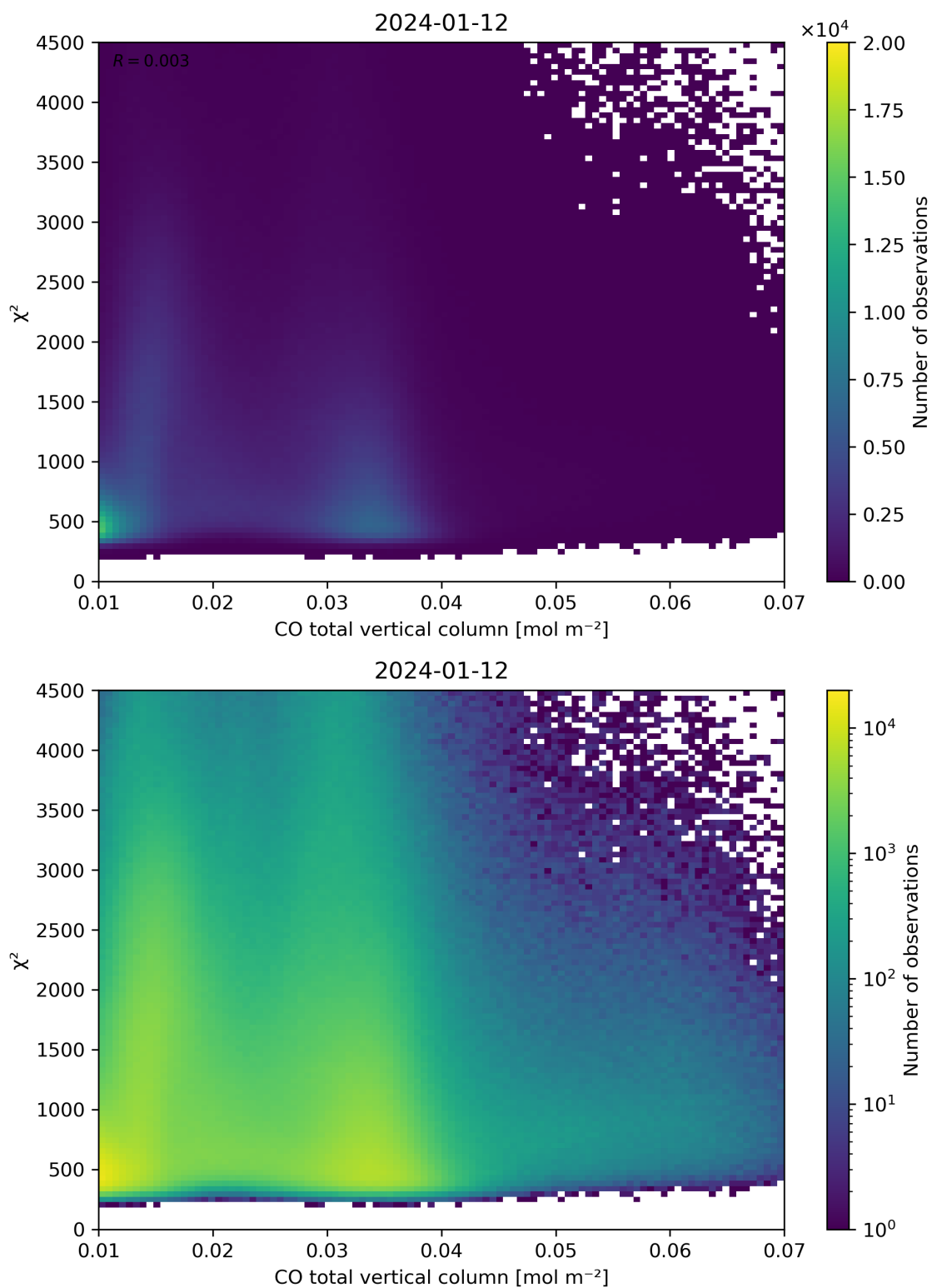
Figure 35: Scatter density plot of “CO total vertical column” against “ \chi^2 ” for 2024-01-11 to 2024-01-13.
