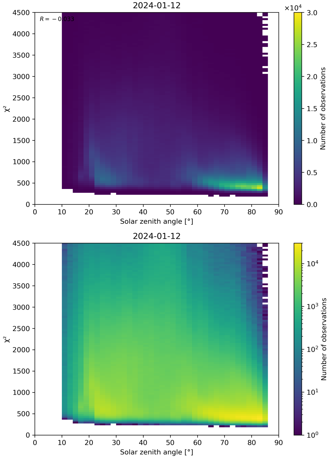
Figure 64: Scatter density plot of “Solar zenith angle” against “ \chi^2 ” for 2024-01-11 to 2024-01-13.
