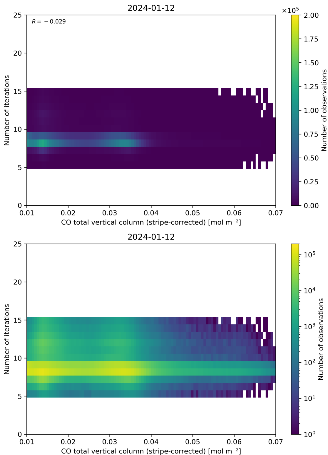
Figure 39: Scatter density plot of “CO total vertical column (stripe-corrected)” against “Number of iterations” for 2024-01-11 to 2024-01-13.
