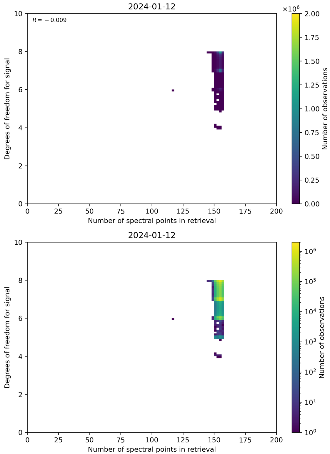
Figure 59: Scatter density plot of “Number of spectral points in retrieval” against “Degrees of freedom for signal” for 2024-01-11 to 2024-01-13.
