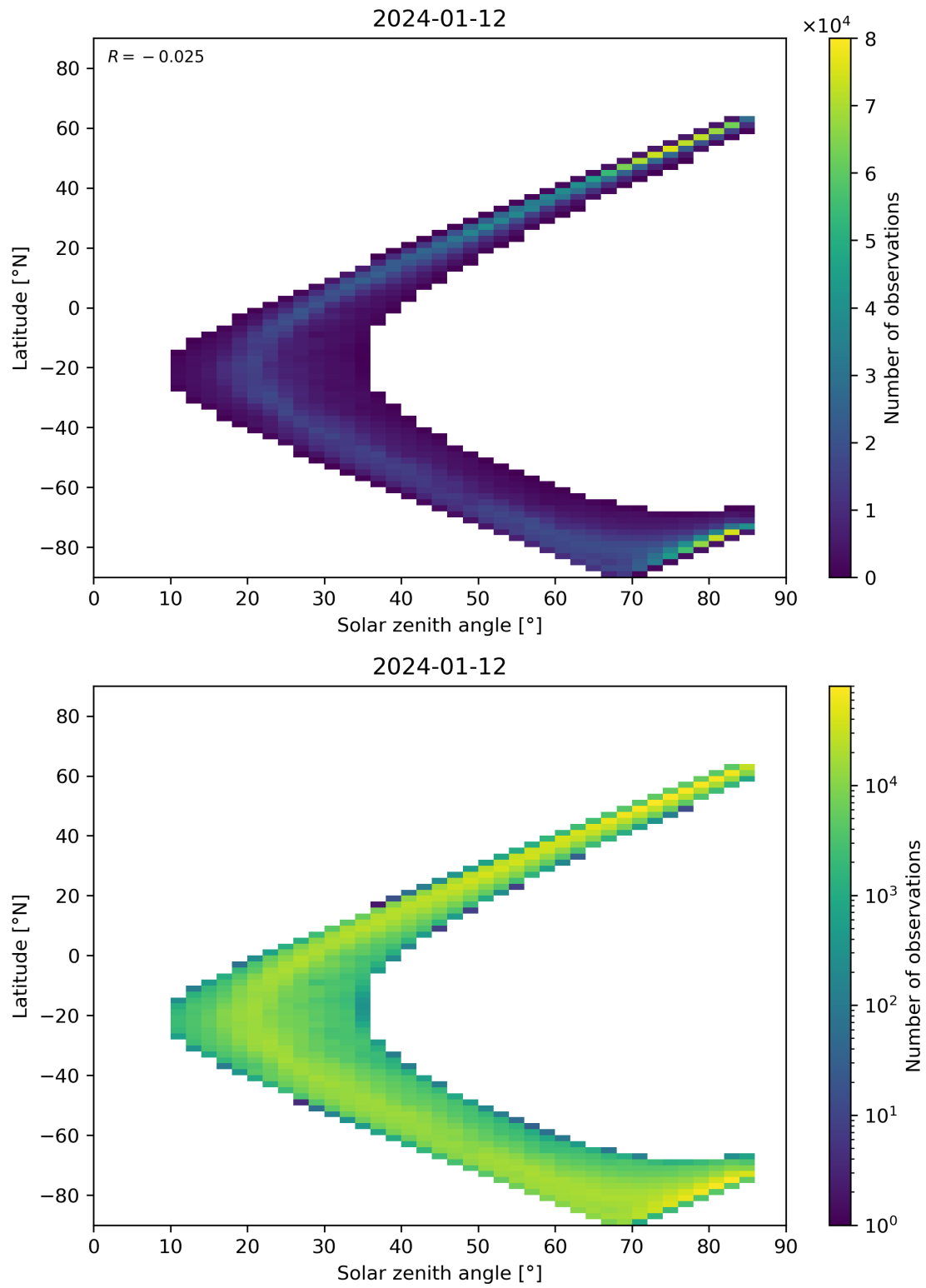
Figure 66: Scatter density plot of “Solar zenith angle” against “Latitude” for 2024-01-11 to 2024-01-13.
