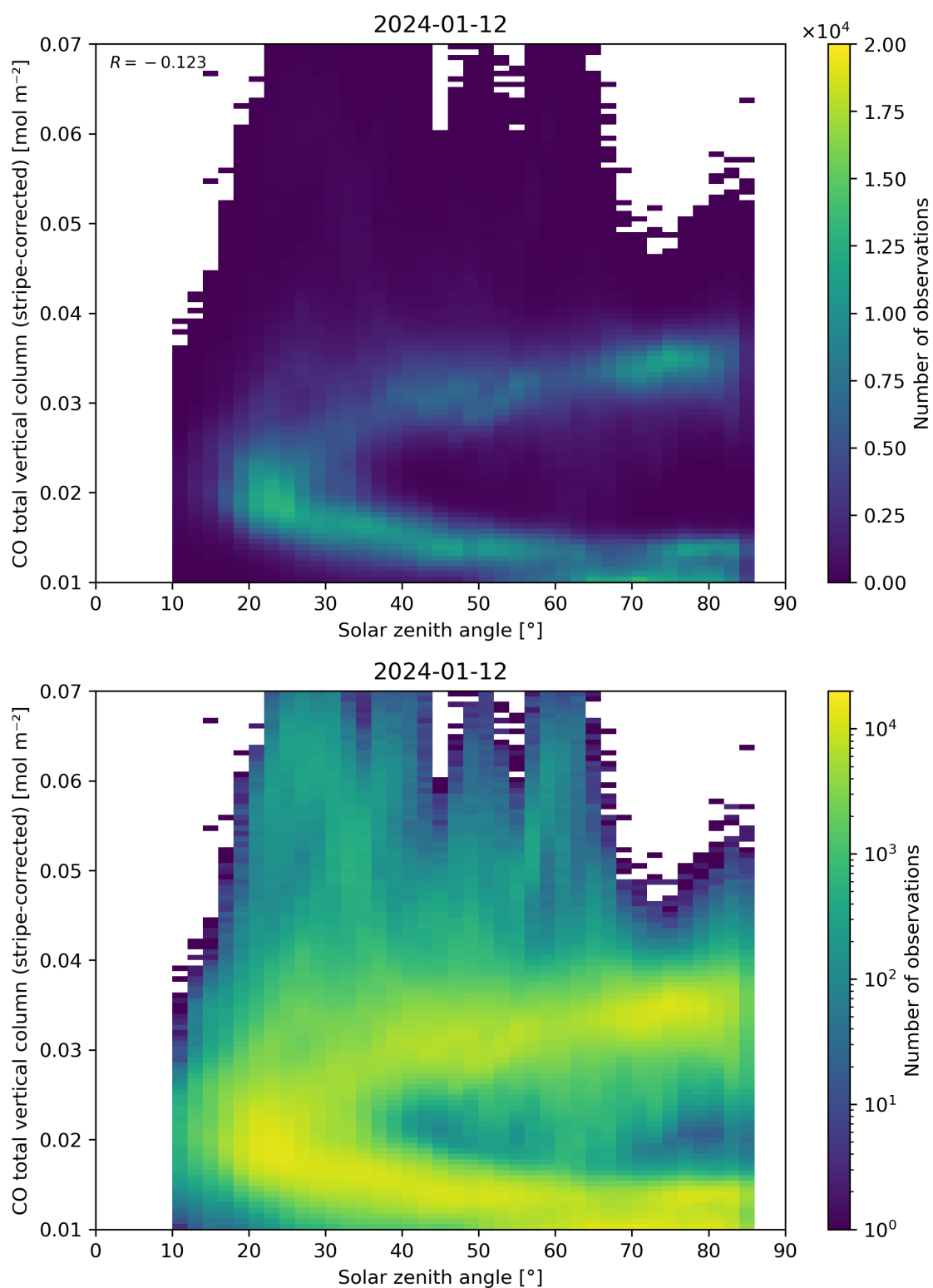
Figure 62: Scatter density plot of “Solar zenith angle” against “CO total vertical column (stripe-corrected)” for 2024-01-11 to 2024-01-13.
