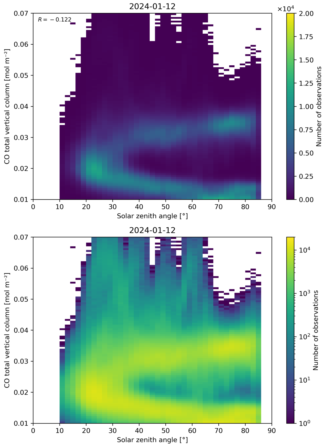
Figure 61: Scatter density plot of “Solar zenith angle” against “CO total vertical column” for 2024-01-11 to 2024-01-13.
