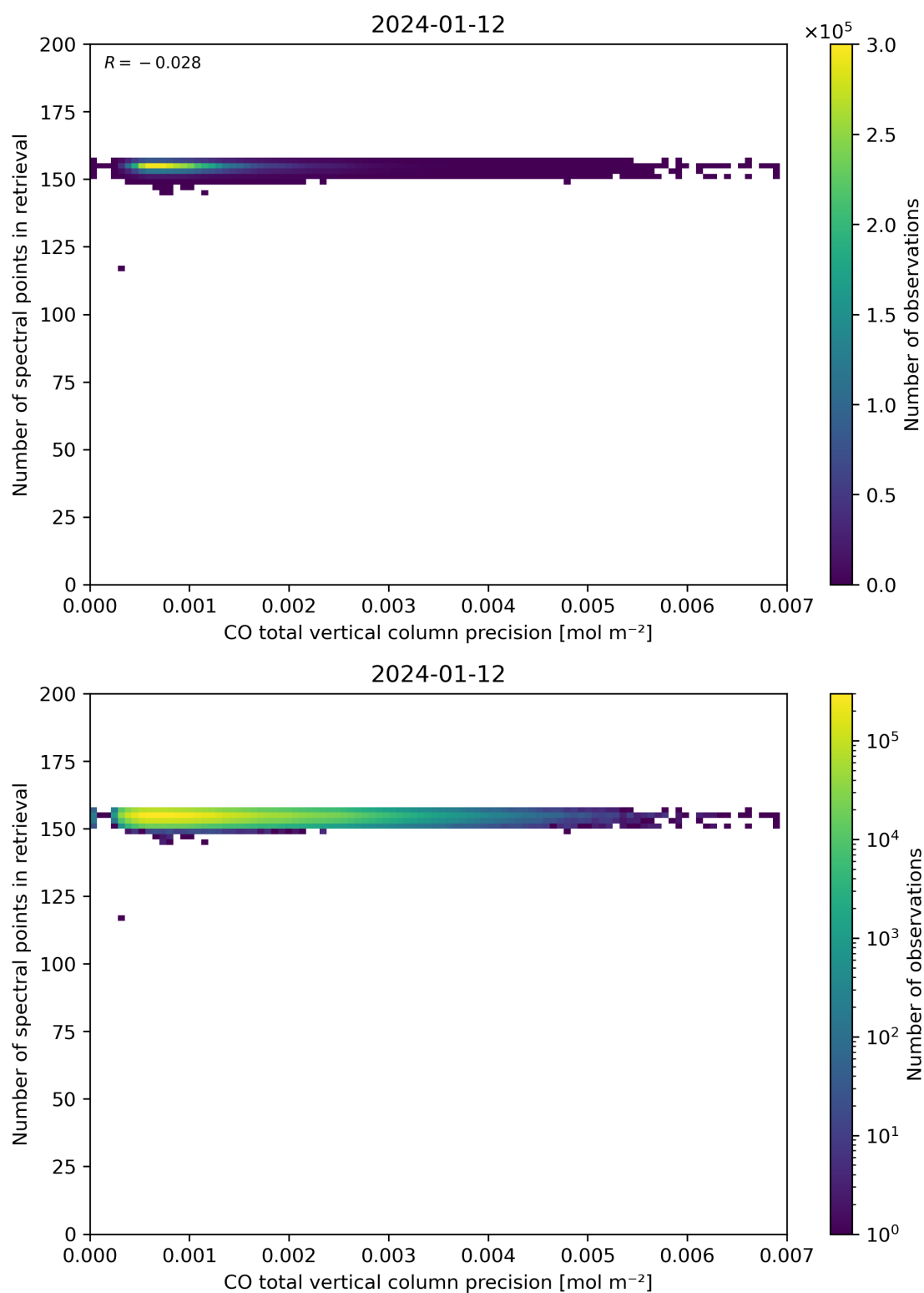
Figure 47: Scatter density plot of “CO total vertical column precision” against “Number of spectral points in retrieval” for 2024-01-11 to 2024-01-13.
