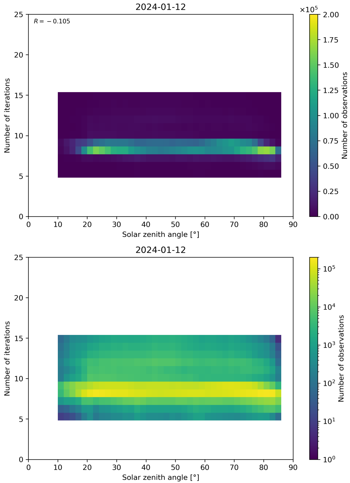
Figure 67: Scatter density plot of “Solar zenith angle” against “Number of iterations” for 2024-01-11 to 2024-01-13.
