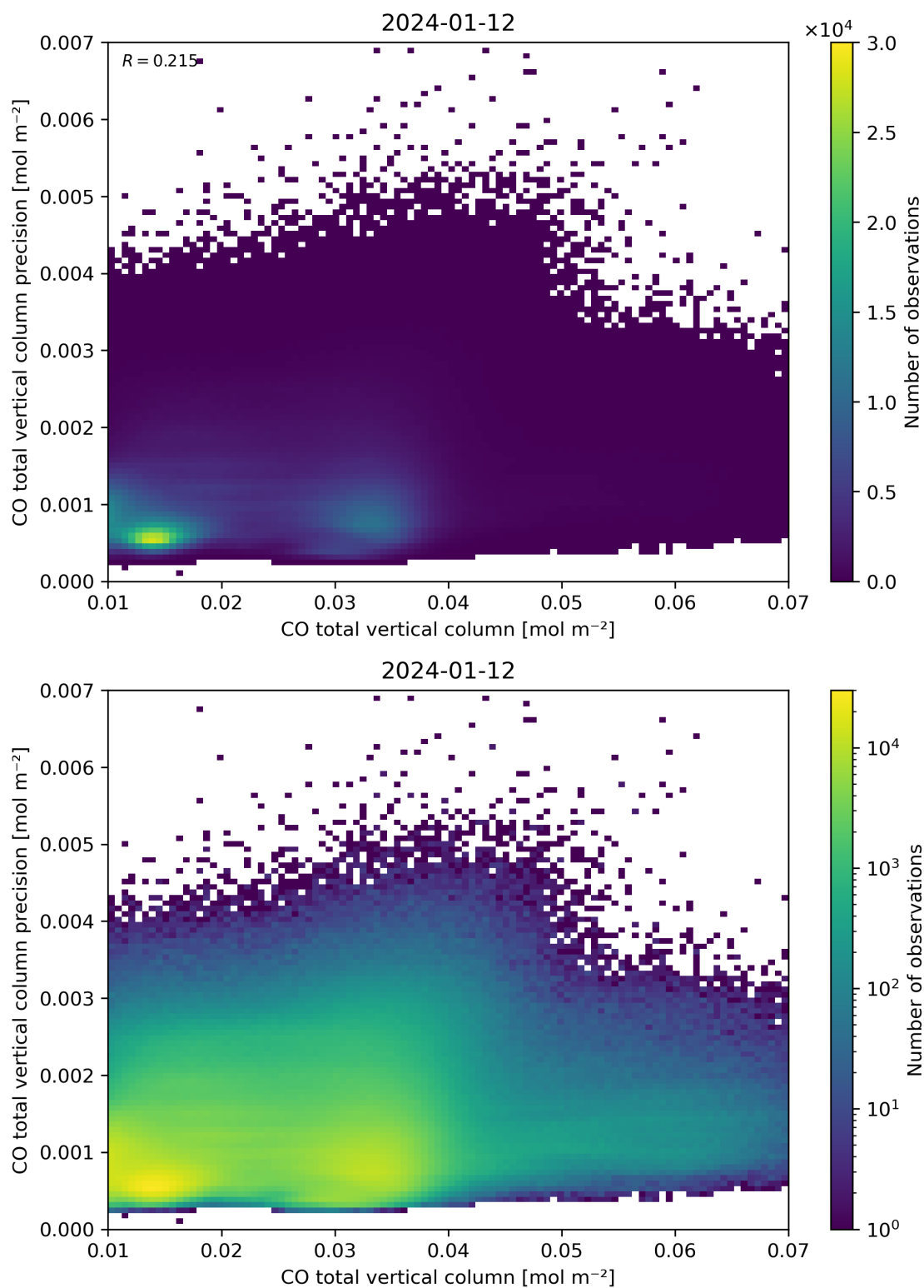
Figure 34: Scatter density plot of “CO total vertical column” against “CO total vertical column precision” for 2024-01-11 to 2024-01-13.
