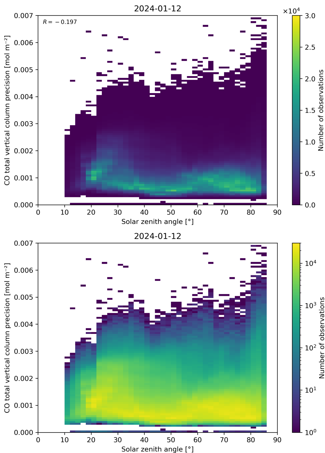
Figure 63: Scatter density plot of “Solar zenith angle” against “CO total vertical column precision” for 2024-01-11 to 2024-01-13.
