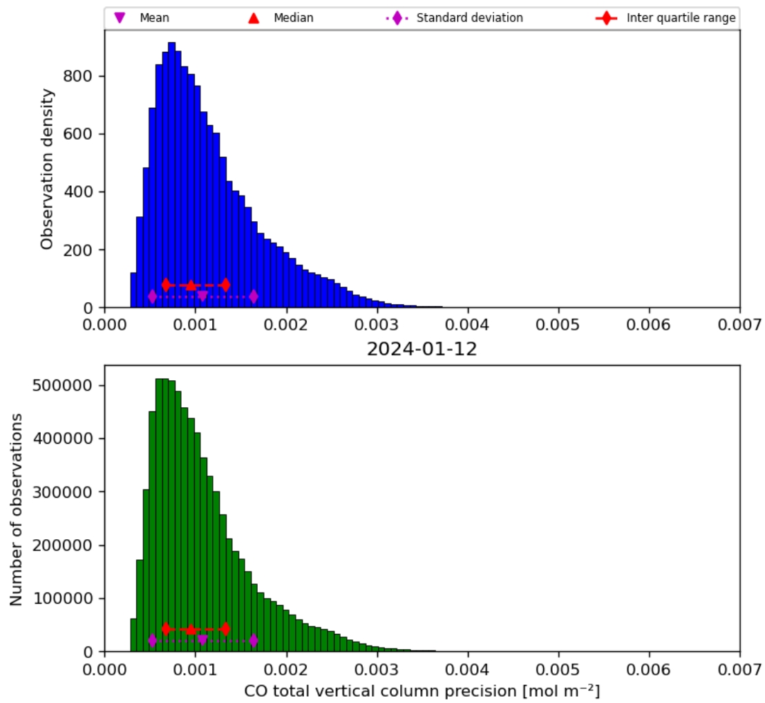
Figure 20: Histogram of “CO total vertical column precision” for 2024-01-11 to 2024-01-13
