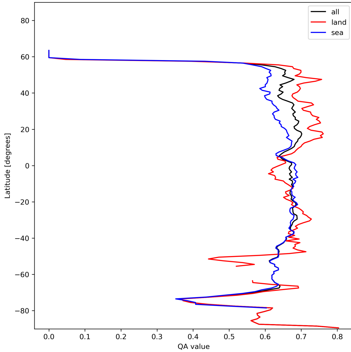
Figure 9: Zonal average of “QA value” for 2024-01-11 to 2024-01-13.
