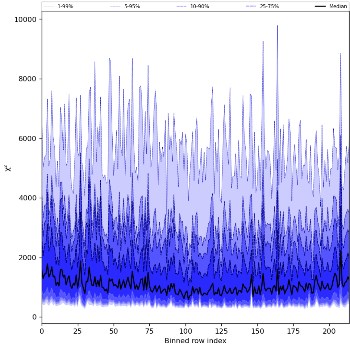
Figure 30: Along track statistics of “ \chi^2 ” for 2024-01-11 to 2024-01-13
