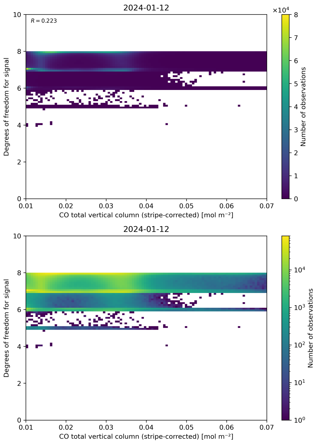
Figure 38: Scatter density plot of “CO total vertical column (stripe-corrected)” against “Degrees of freedom for signal” for 2024-01-11 to 2024-01-13.
