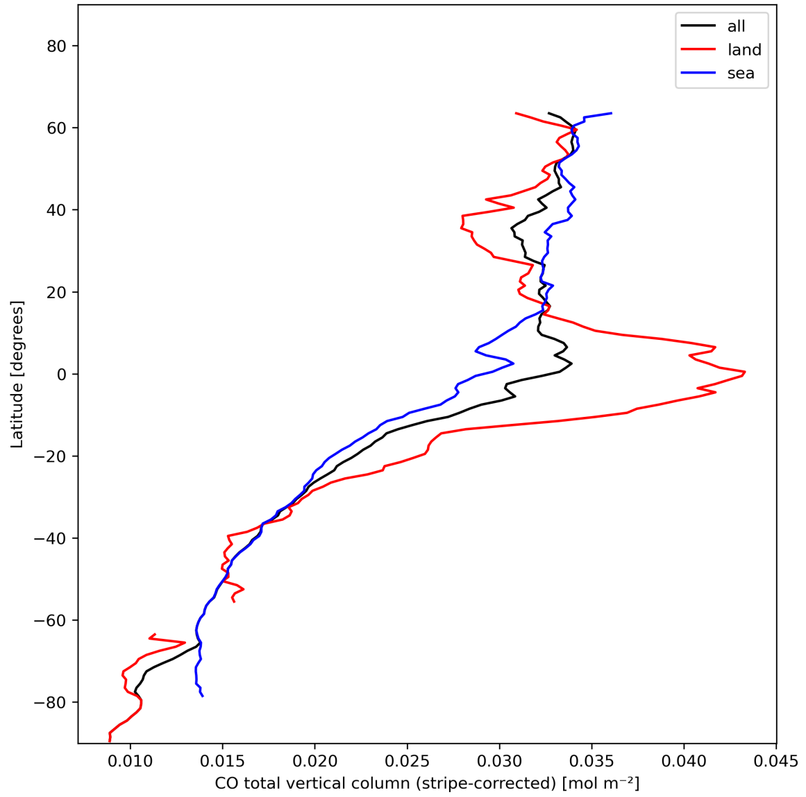
Figure 11: Zonal average of “CO total vertical column (stripe-corrected)” for 2024-01-11 to 2024-01-13.
