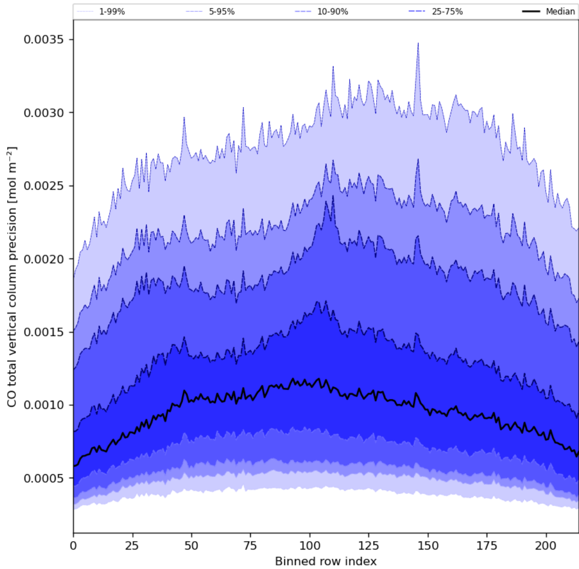
Figure 28: Along track statistics of “CO total vertical column precision” for 2024-01-11 to 2024-01-13
