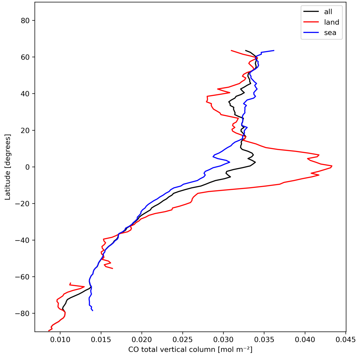
Figure 10: Zonal average of “CO total vertical column” for 2024-01-11 to 2024-01-13.
