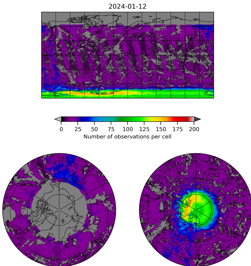
Figure 8: Map of the number of observations for 2024-01-11 to 2024-01-13
