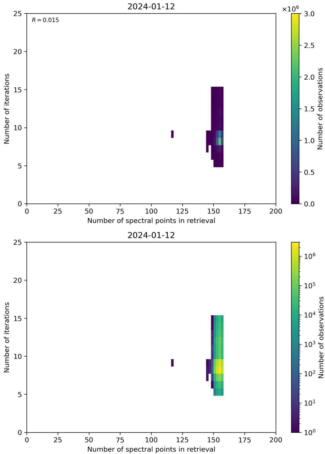
Figure 60: Scatter density plot of “Number of spectral points in retrieval” against “Number of iterations” for 2024-01-11 to 2024-01-13.
