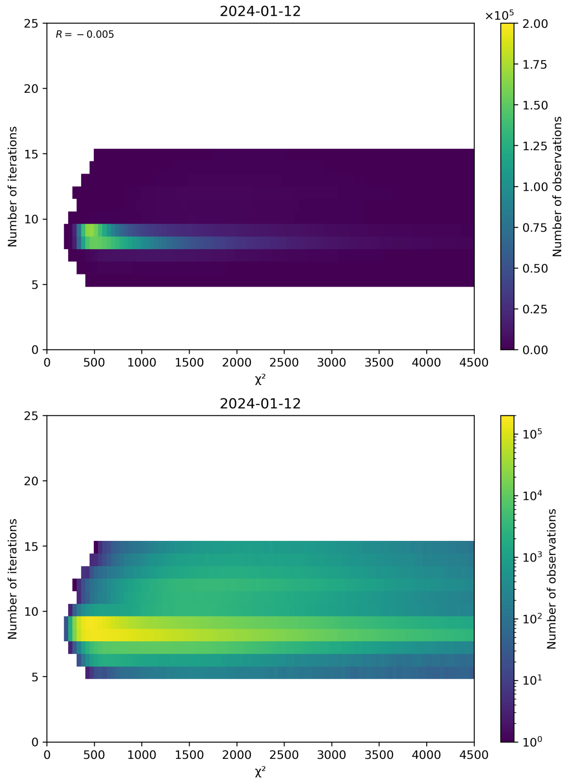
Figure 49: Scatter density plot of “ \chi^2 ” against “Number of iterations” for 2024-01-11 to 2024-01-13.
