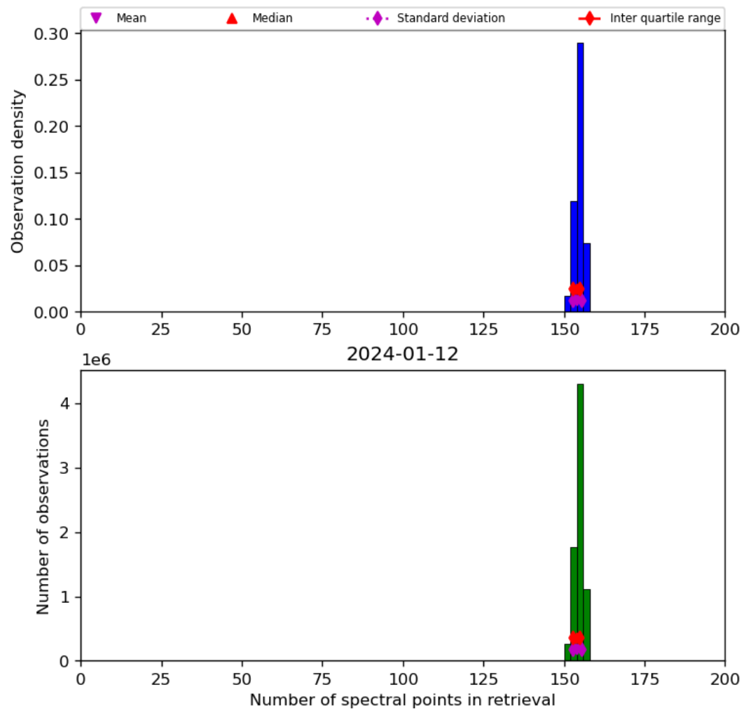
Figure 21: Histogram of “Number of spectral points in retrieval” for 2024-01-11 to 2024-01-13
