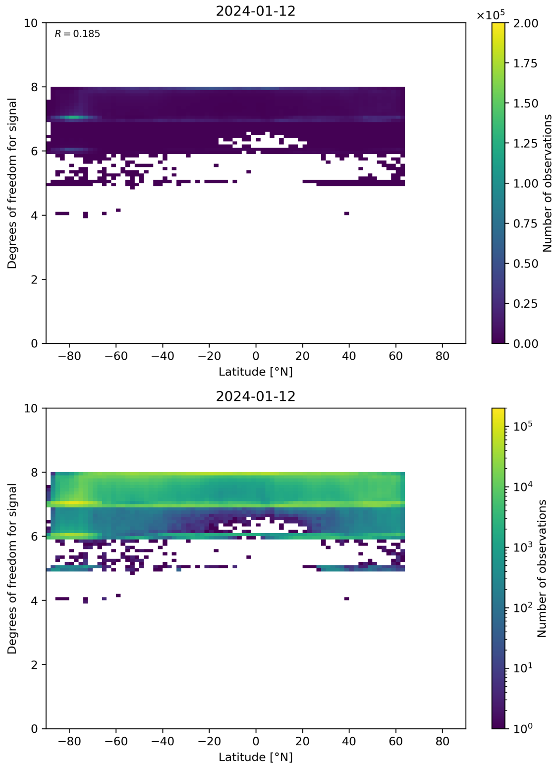
Figure 55: Scatter density plot of “Latitude” against “Degrees of freedom for signal” for 2024-01-11 to 2024-01-13.
