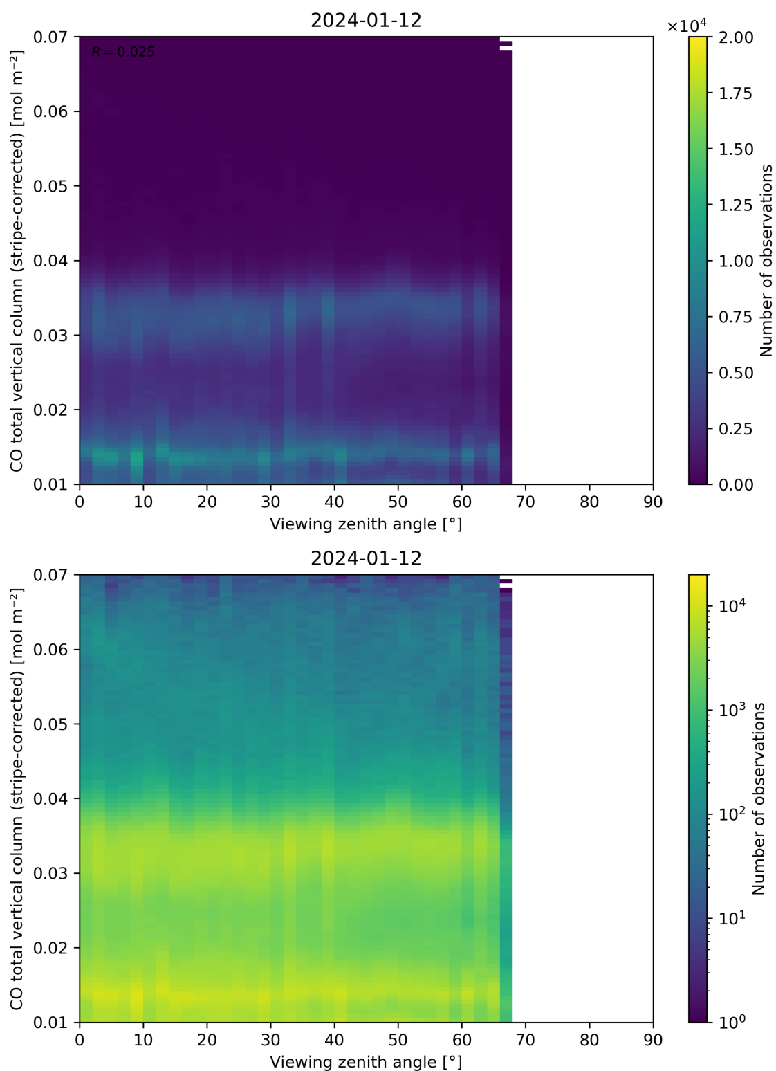
Figure 70: Scatter density plot of “Viewing zenith angle” against “CO total vertical column (stripe-corrected)” for 2024-01-11 to 2024-01-13.
