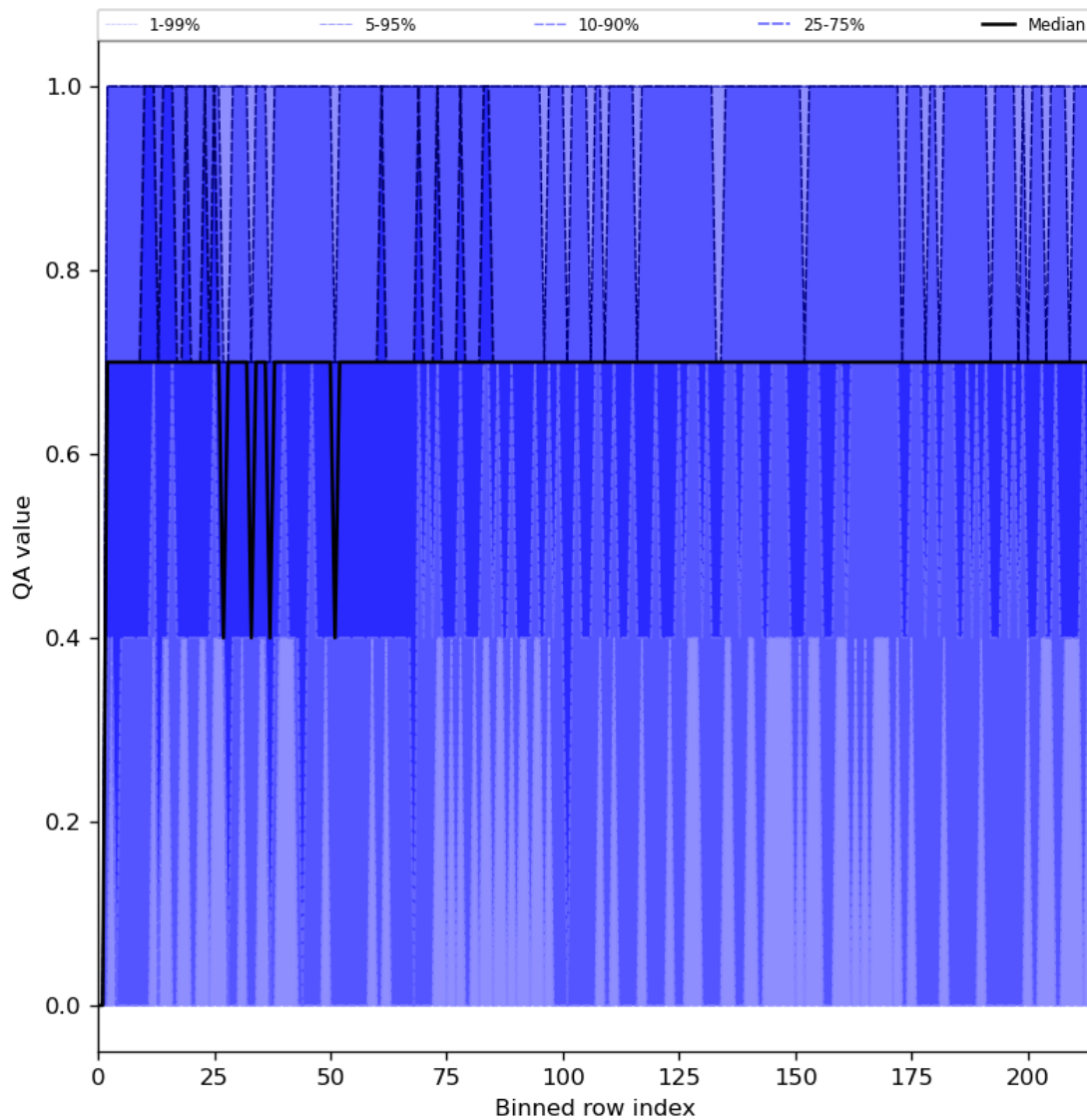
Figure 25: Along track statistics of “QA value” for 2024-01-11 to 2024-01-13
