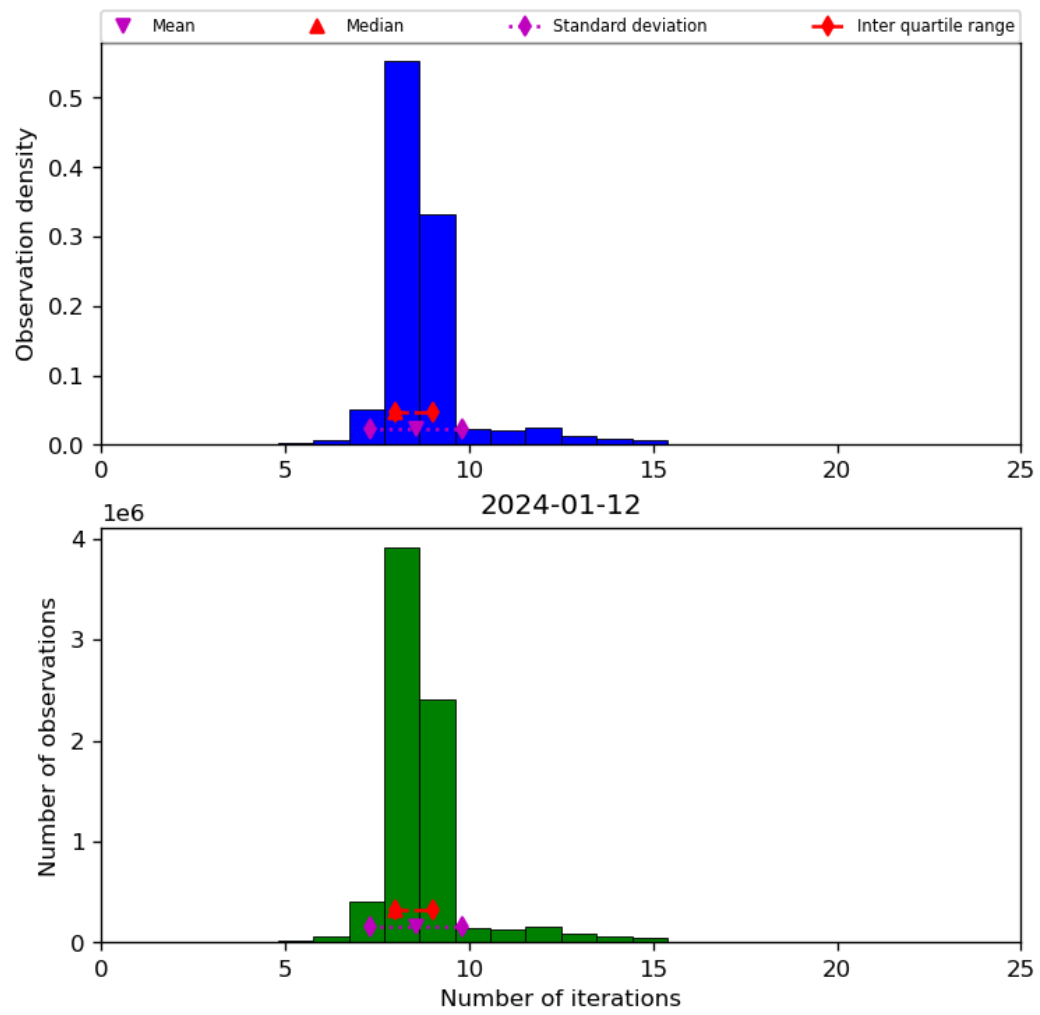
Figure 24: Histogram of “Number of iterations” for 2024-01-11 to 2024-01-13
