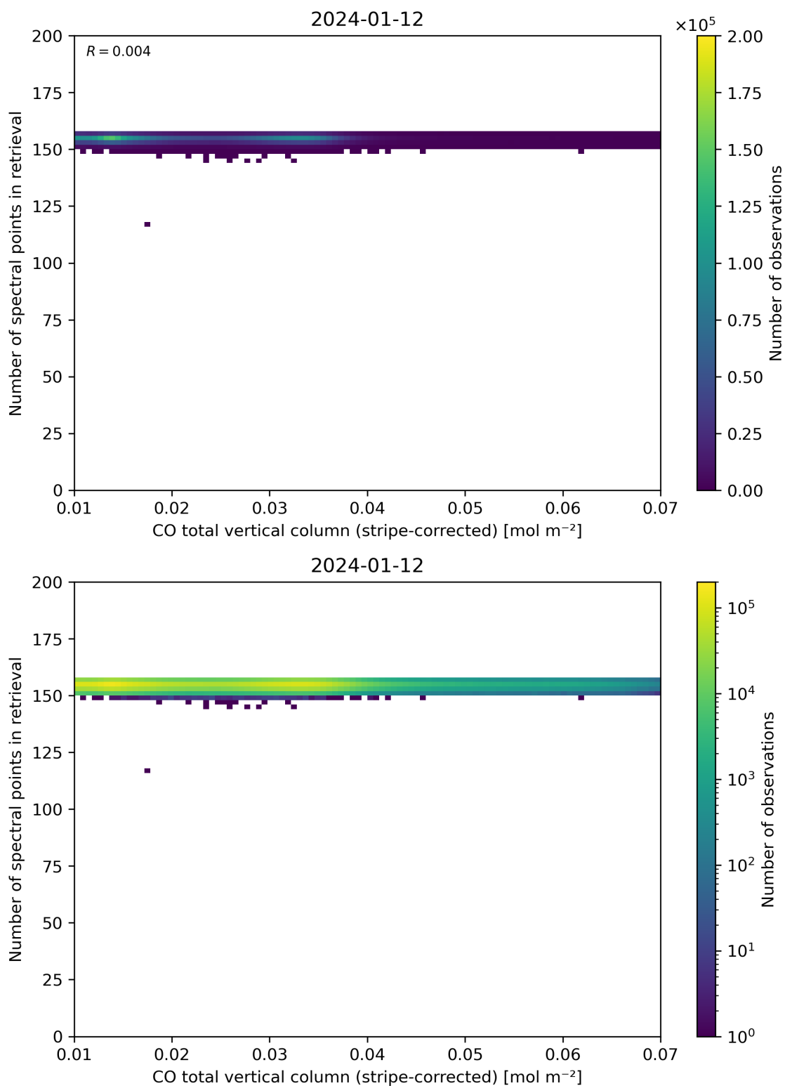
Figure 40: Scatter density plot of “CO total vertical column (stripe-corrected)” against “Number of spectral points in retrieval” for 2024-01-11 to 2024-01-13.
