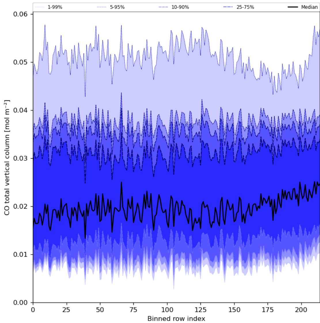
Figure 26: Along track statistics of “CO total vertical column” for 2024-01-11 to 2024-01-13
