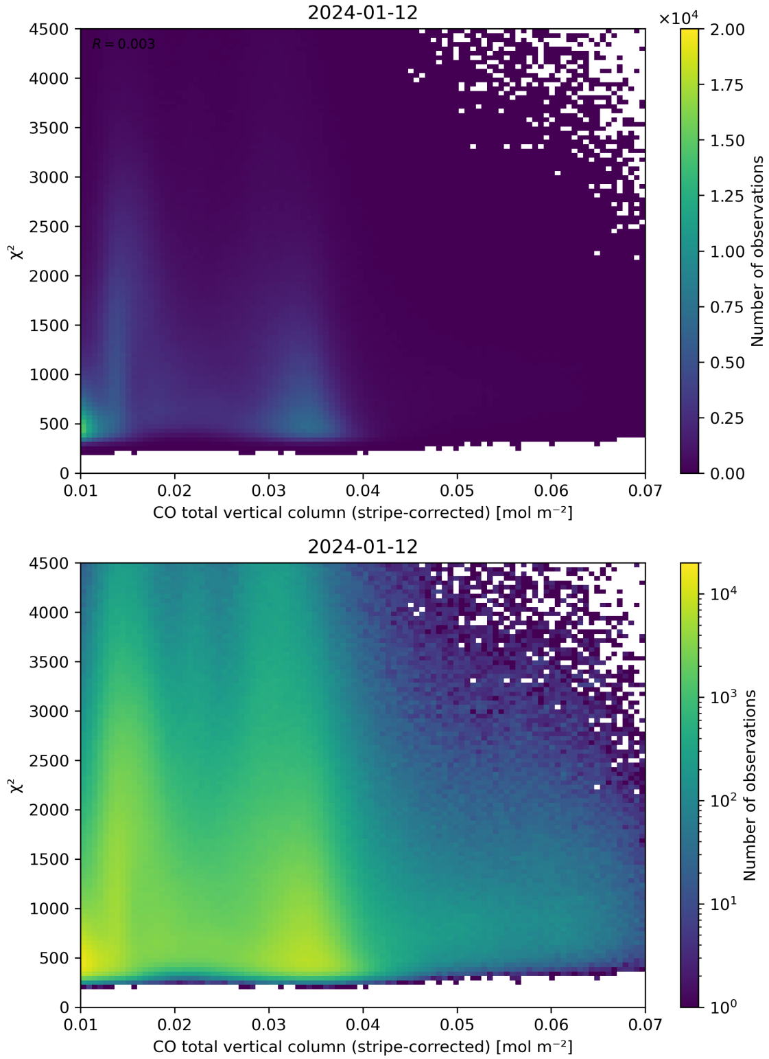
Figure 37: Scatter density plot of “CO total vertical column (stripe-corrected)” against “ \chi^2 ” for 2024-01-11 to 2024-01-13.
