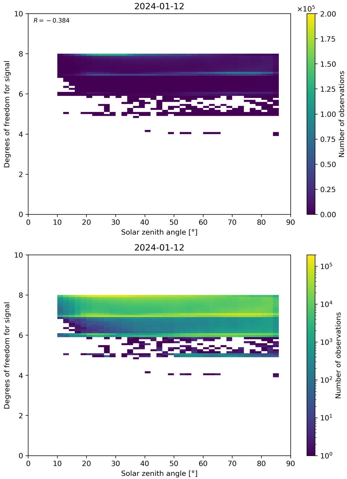
Figure 65: Scatter density plot of “Solar zenith angle” against “Degrees of freedom for signal” for 2024-01-11 to 2024-01-13.
