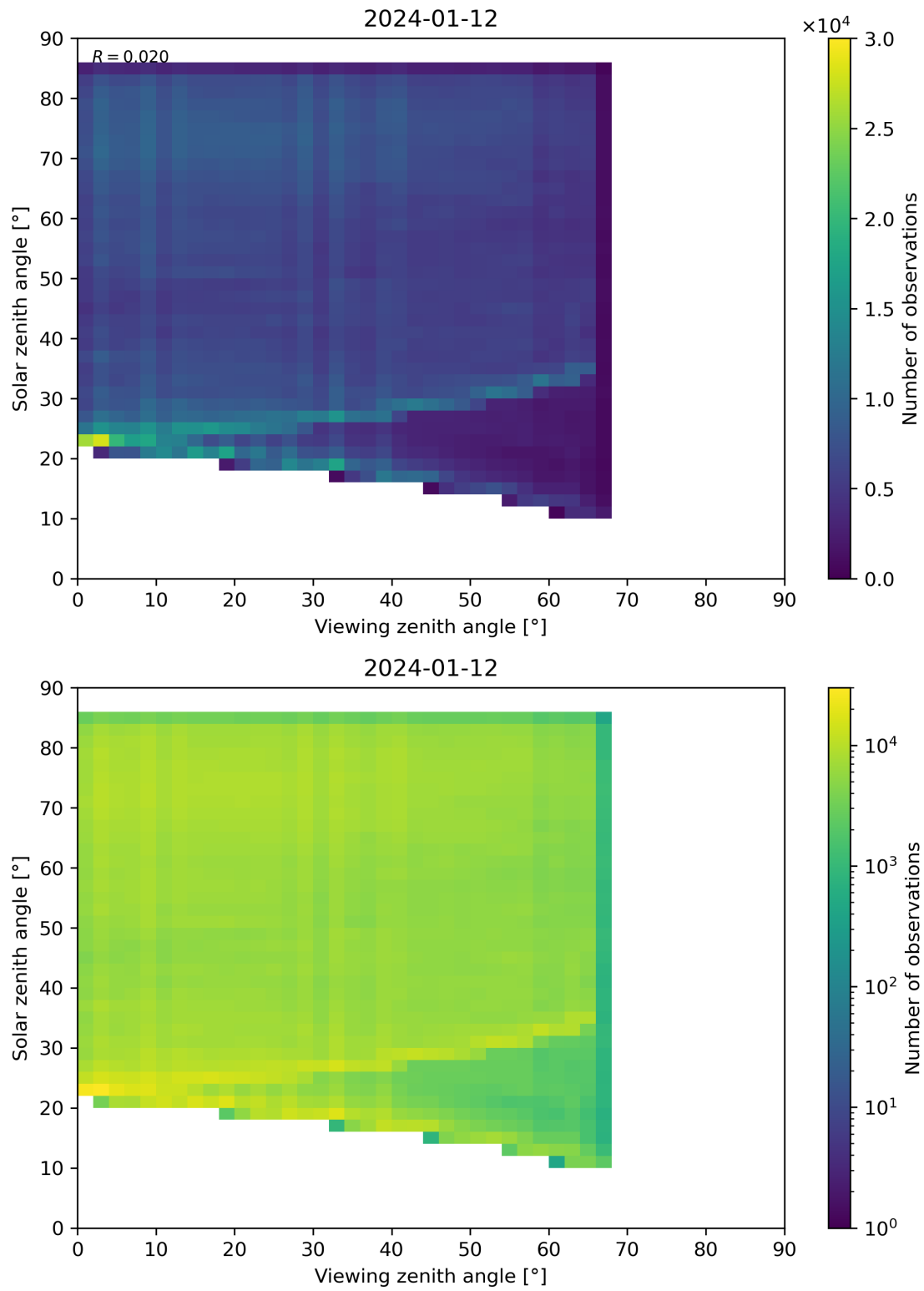
Figure 77: Scatter density plot of “Viewing zenith angle” against “Solar zenith angle” for 2024-01-11 to 2024-01-13.
