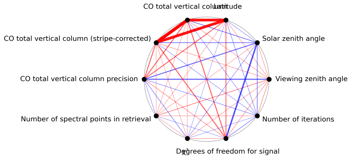
Figure 1: Map of correlation graph for 2024-01-11 to 2024-01-13.
