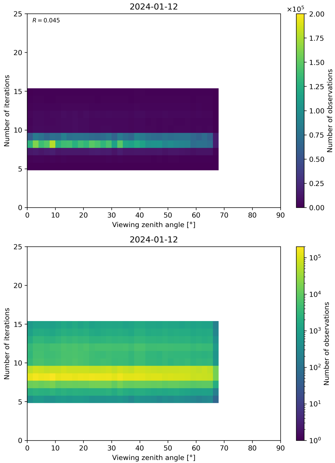
Figure 75: Scatter density plot of “Viewing zenith angle” against “Number of iterations” for 2024-01-11 to 2024-01-13.
