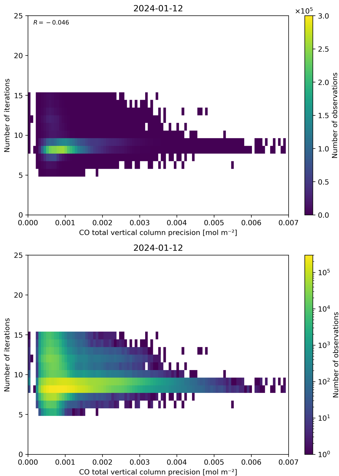
Figure 46: Scatter density plot of “CO total vertical column precision” against “Number of iterations” for 2024-01-11 to 2024-01-13.
