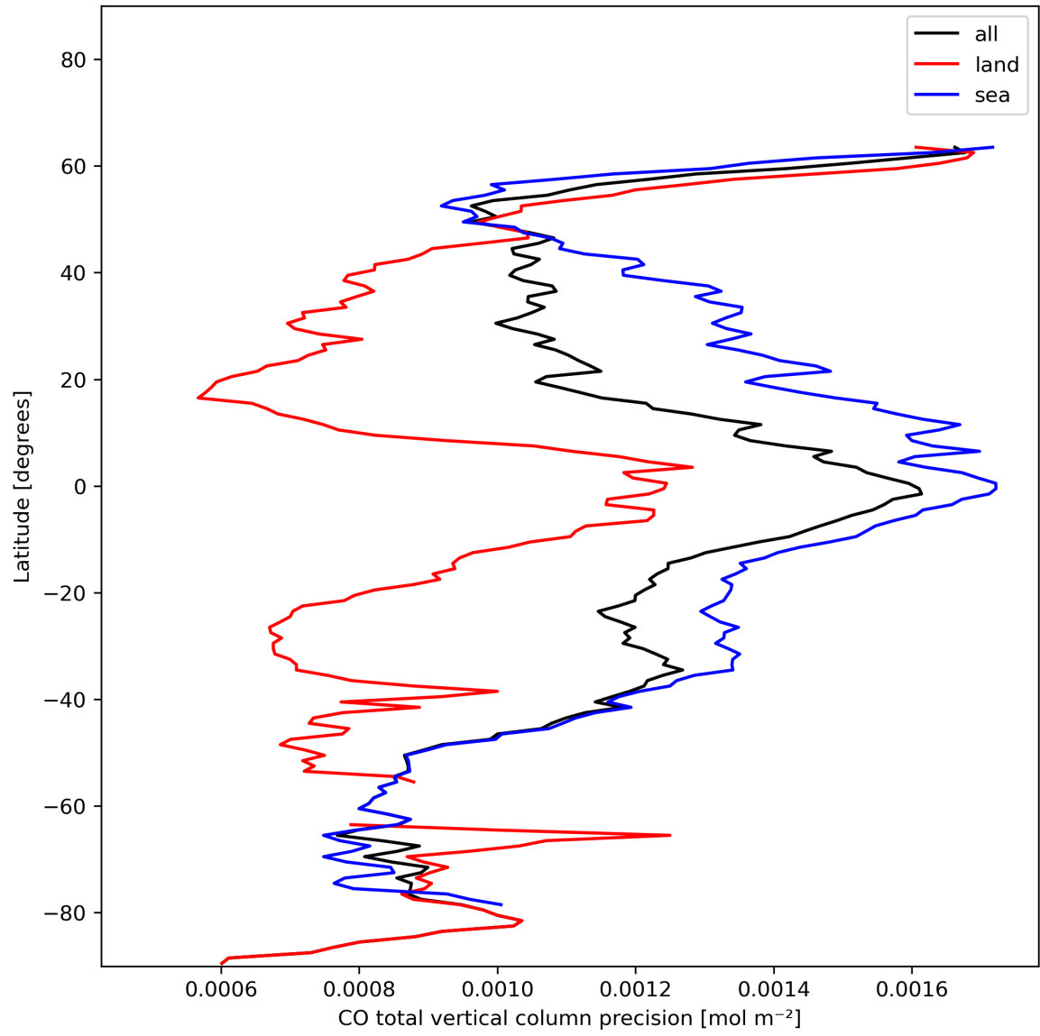
Figure 12: Zonal average of “CO total vertical column precision” for 2024-01-11 to 2024-01-13.
