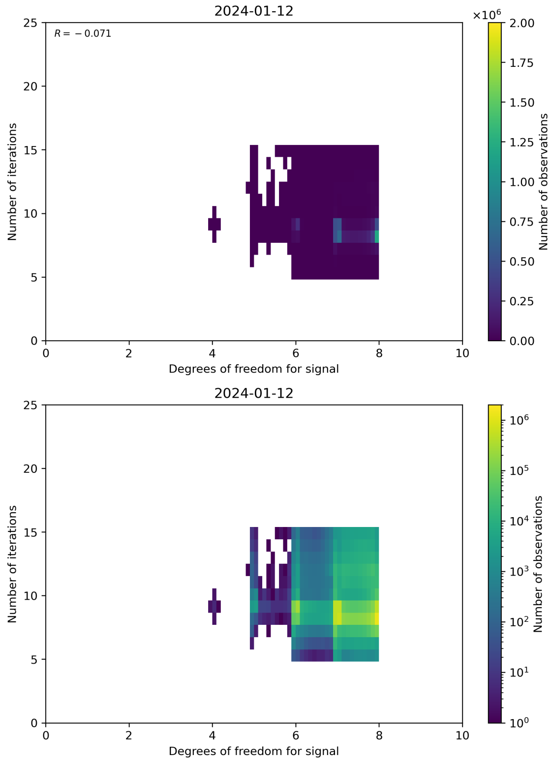
Figure 50: Scatter density plot of “Degrees of freedom for signal” against “Number of iterations” for 2024-01-11 to 2024-01-13.
