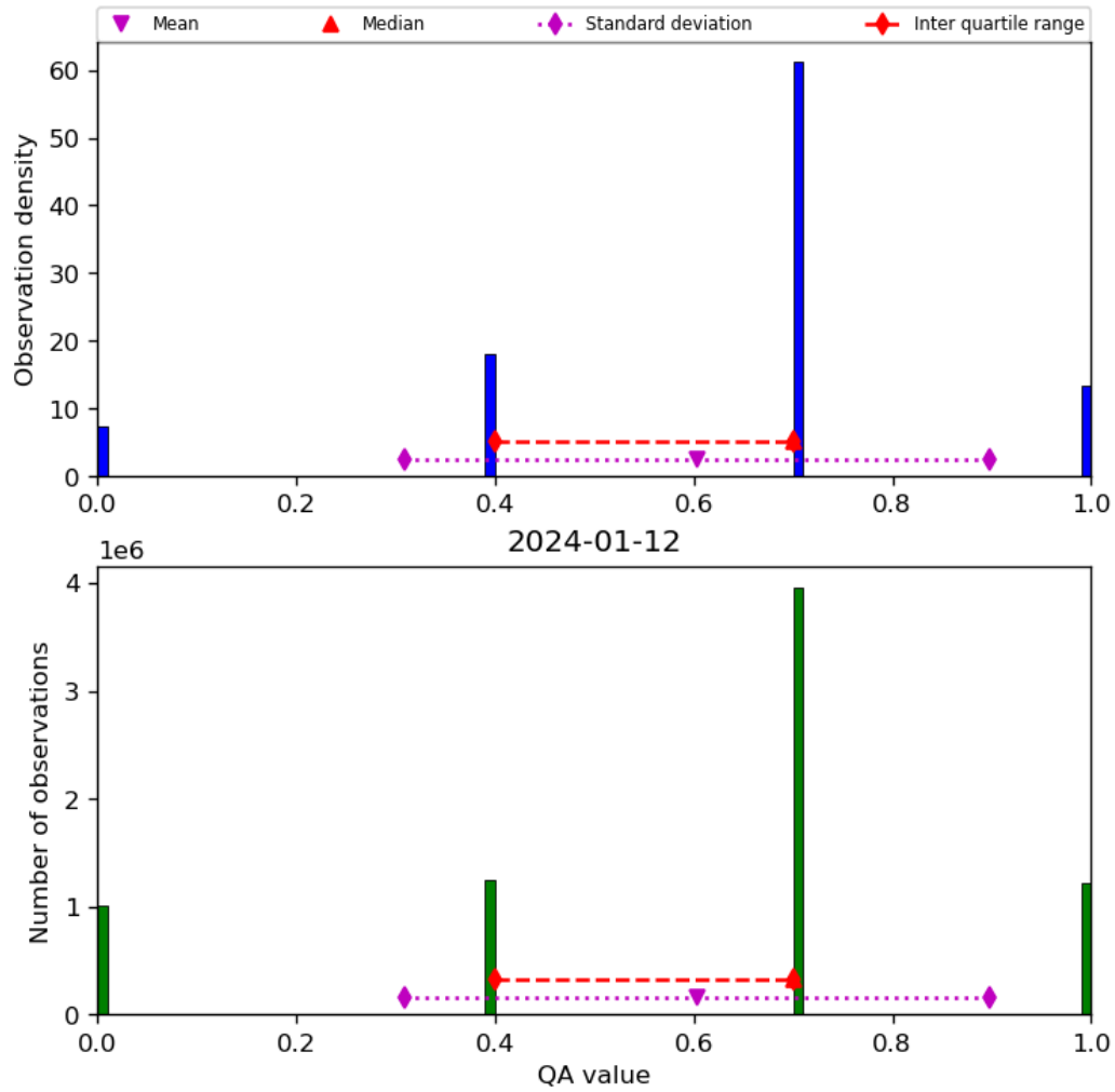
Figure 17: Histogram of “QA value” for 2024-01-11 to 2024-01-13
