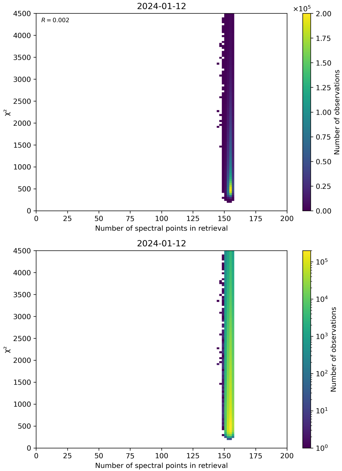
Figure 58: Scatter density plot of “Number of spectral points in retrieval” against “ \chi^2 ” for 2024-01-11 to 2024-01-13.
