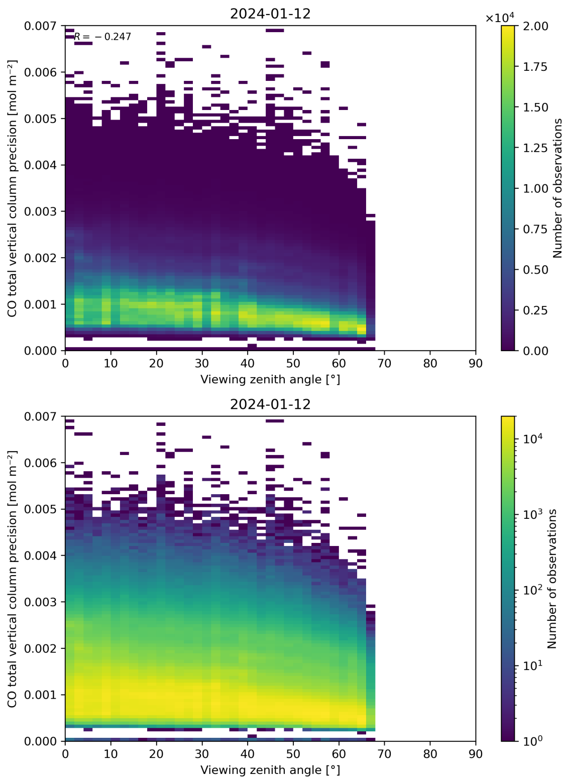
Figure 71: Scatter density plot of “Viewing zenith angle” against “CO total vertical column precision” for 2024-01-11 to 2024-01-13.
