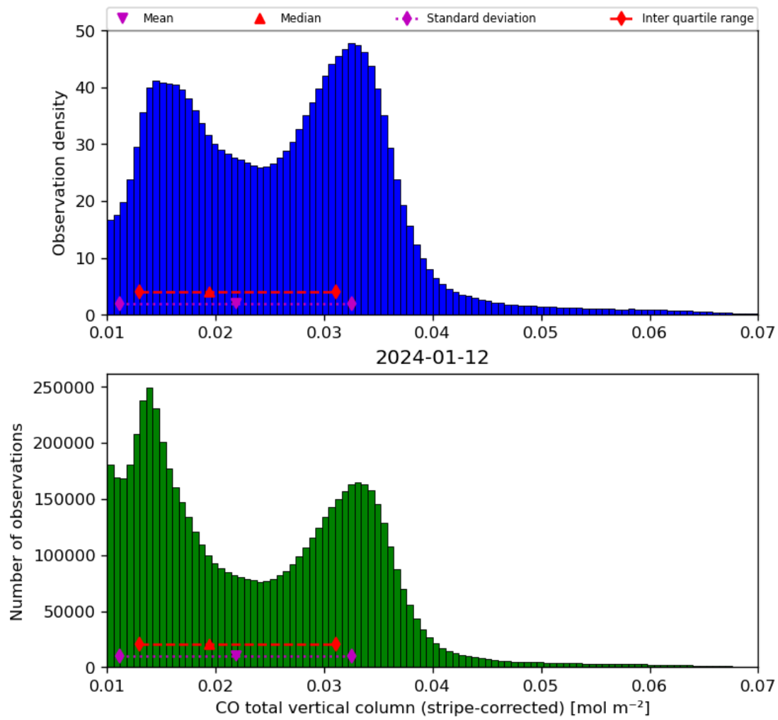
Figure 19: Histogram of “CO total vertical column (stripe-corrected)” for 2024-01-11 to 2024-01-13
