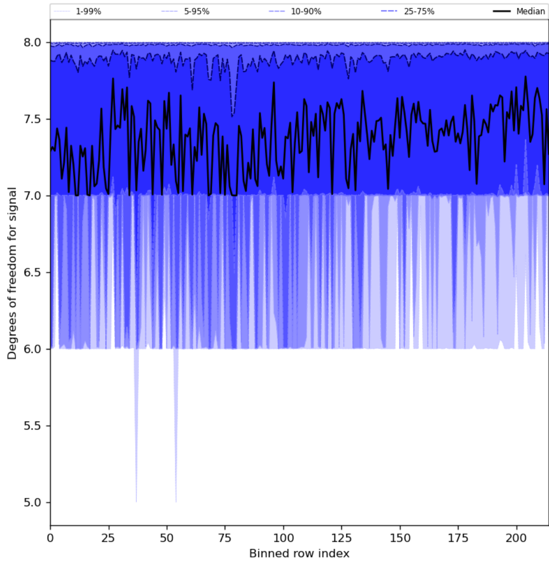
Figure 31: Along track statistics of “Degrees of freedom for signal” for 2024-01-11 to 2024-01-13
