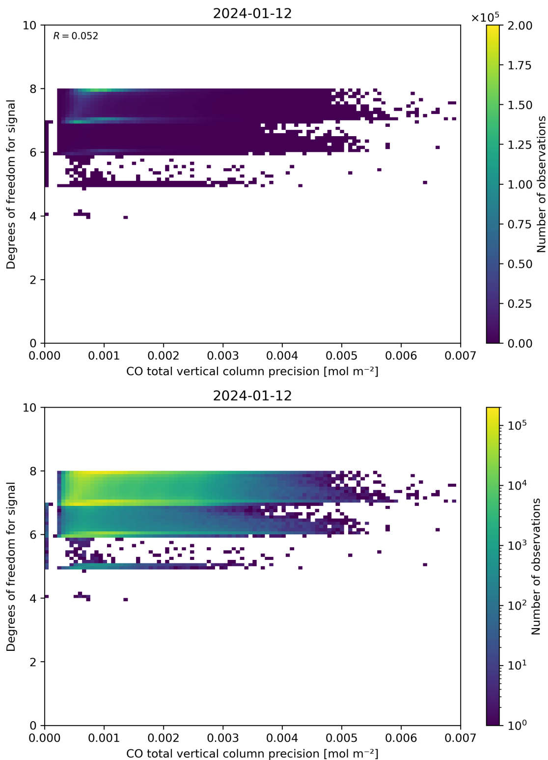
Figure 45: Scatter density plot of “CO total vertical column precision” against “Degrees of freedom for signal” for 2024-01-11 to 2024-01-13.
