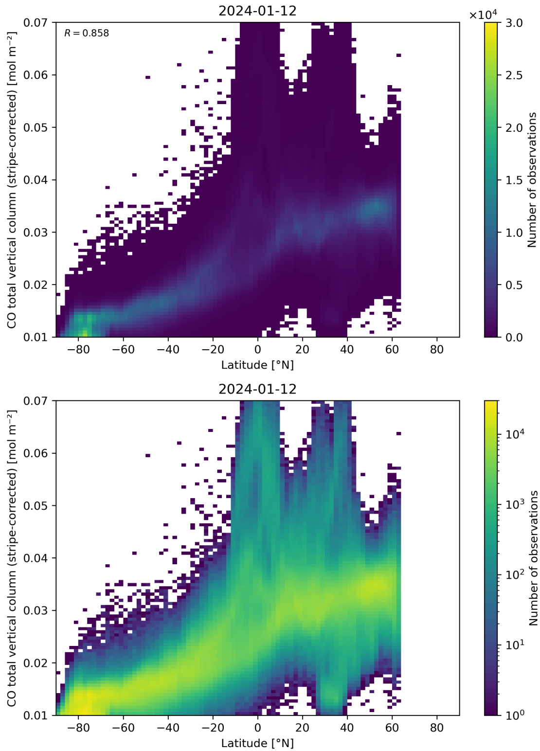
Figure 52: Scatter density plot of “Latitude” against “CO total vertical column (stripe-corrected)” for 2024-01-11 to 2024-01-13.
