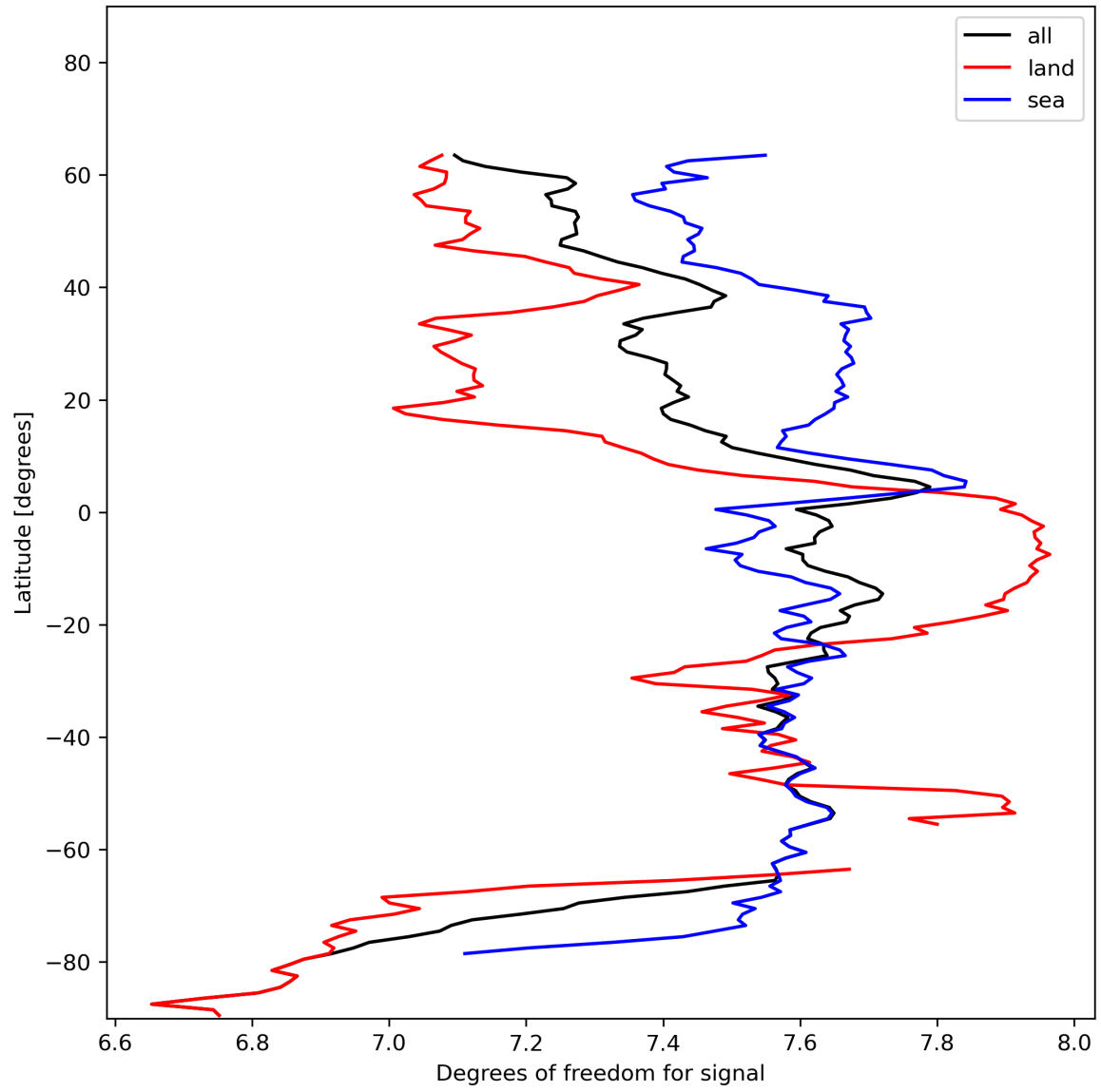
Figure 15: Zonal average of “Degrees of freedom for signal” for 2024-01-11 to 2024-01-13.
