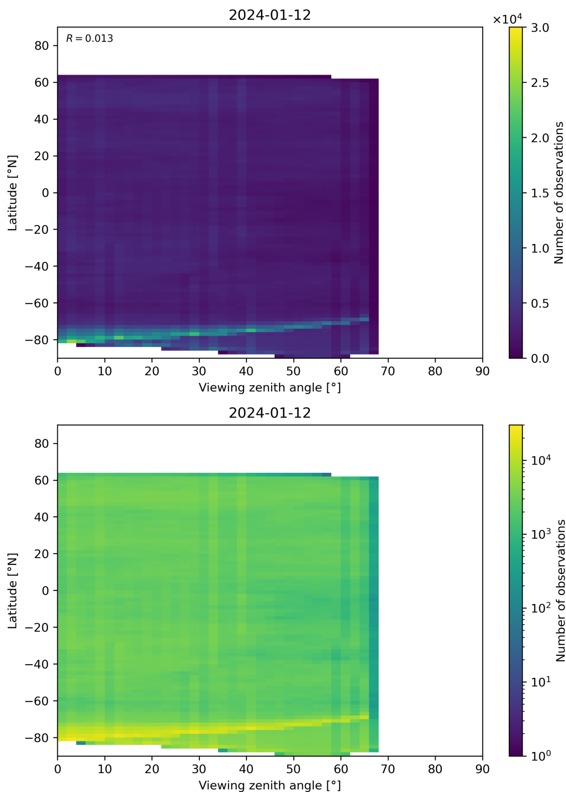
Figure 74: Scatter density plot of “Viewing zenith angle” against “Latitude” for 2024-01-11 to 2024-01-13.
