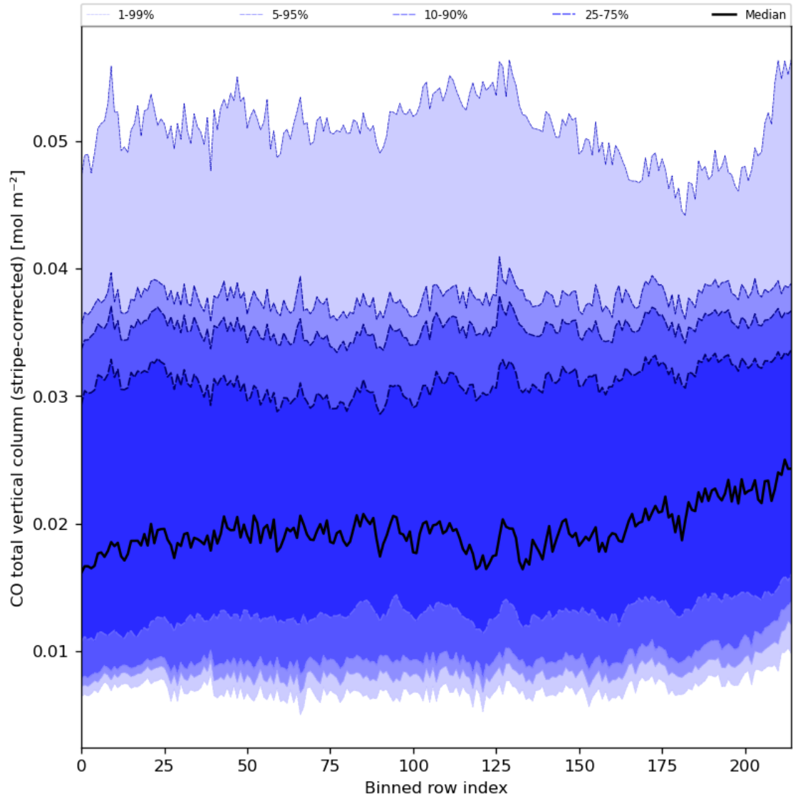
Figure 27: Along track statistics of “CO total vertical column (stripe-corrected)” for 2024-01-11 to 2024-01-13
