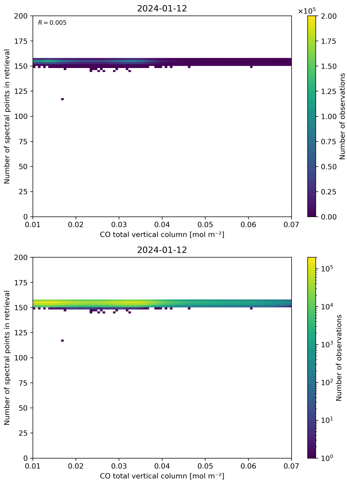
Figure 43: Scatter density plot of “CO total vertical column” against “Number of spectral points in retrieval” for 2024-01-11 to 2024-01-13.
