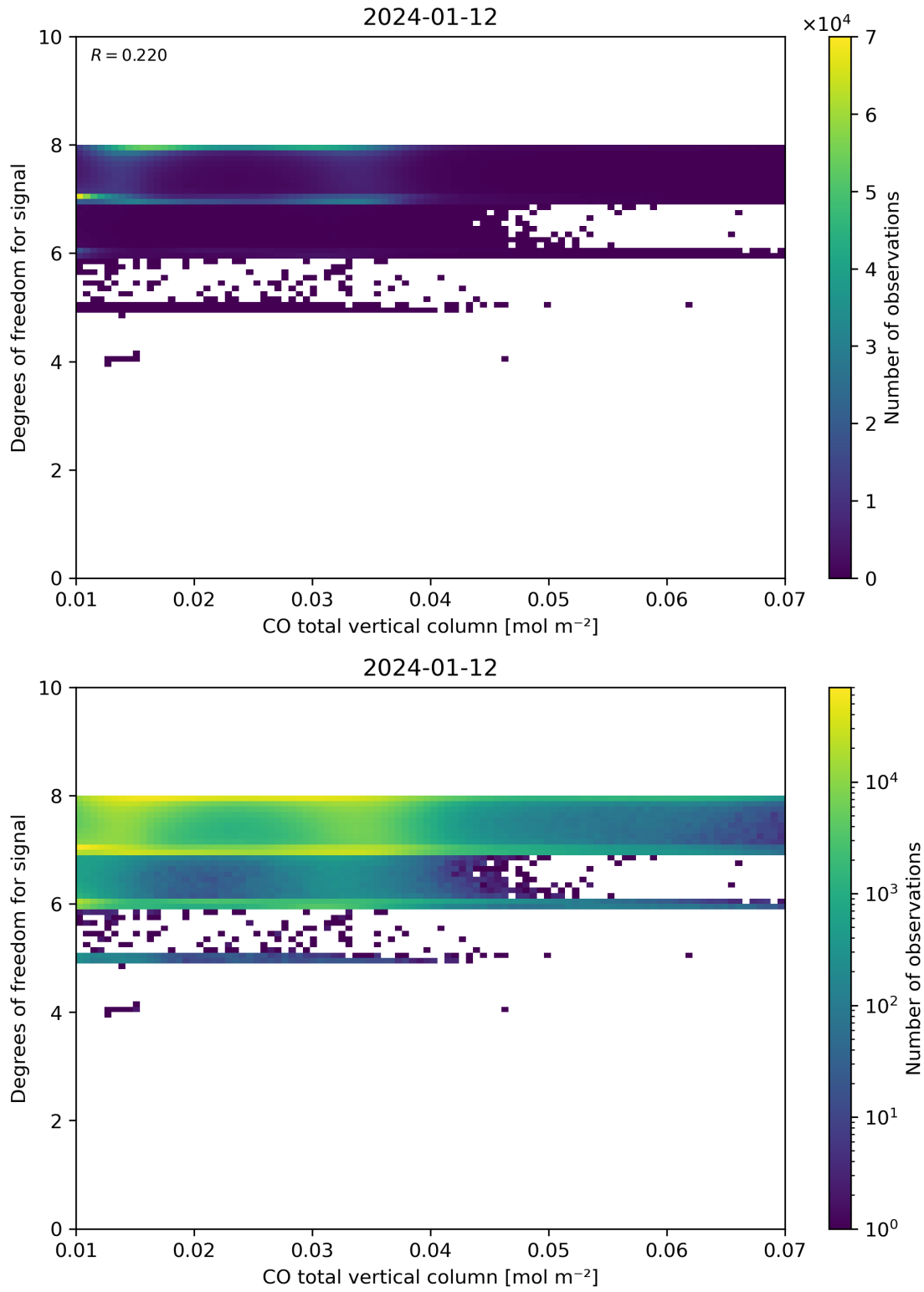
Figure 41: Scatter density plot of “CO total vertical column” against “Degrees of freedom for signal” for 2024-01-11 to 2024-01-13.
