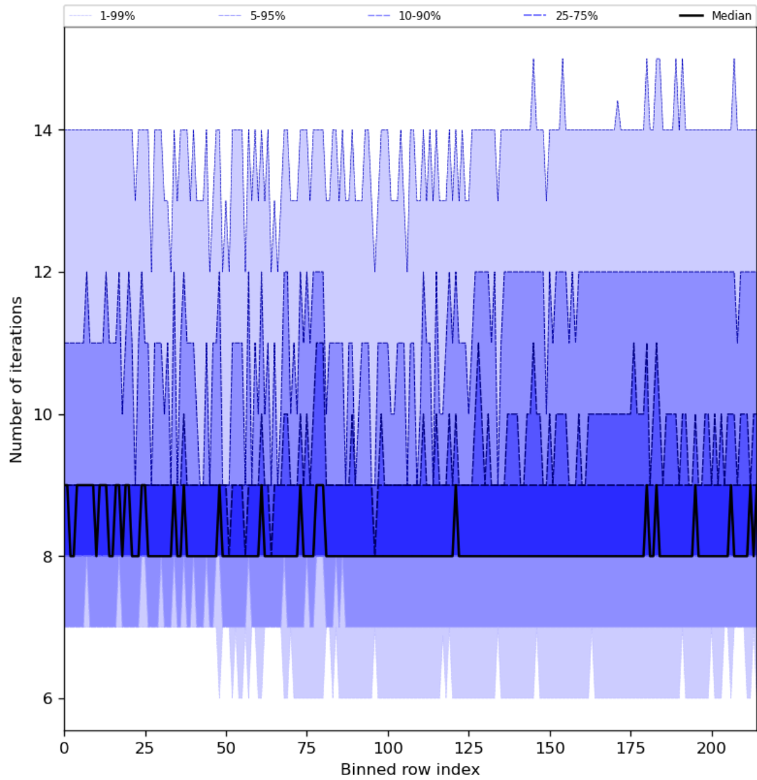
Figure 32: Along track statistics of “Number of iterations” for 2024-01-11 to 2024-01-13
