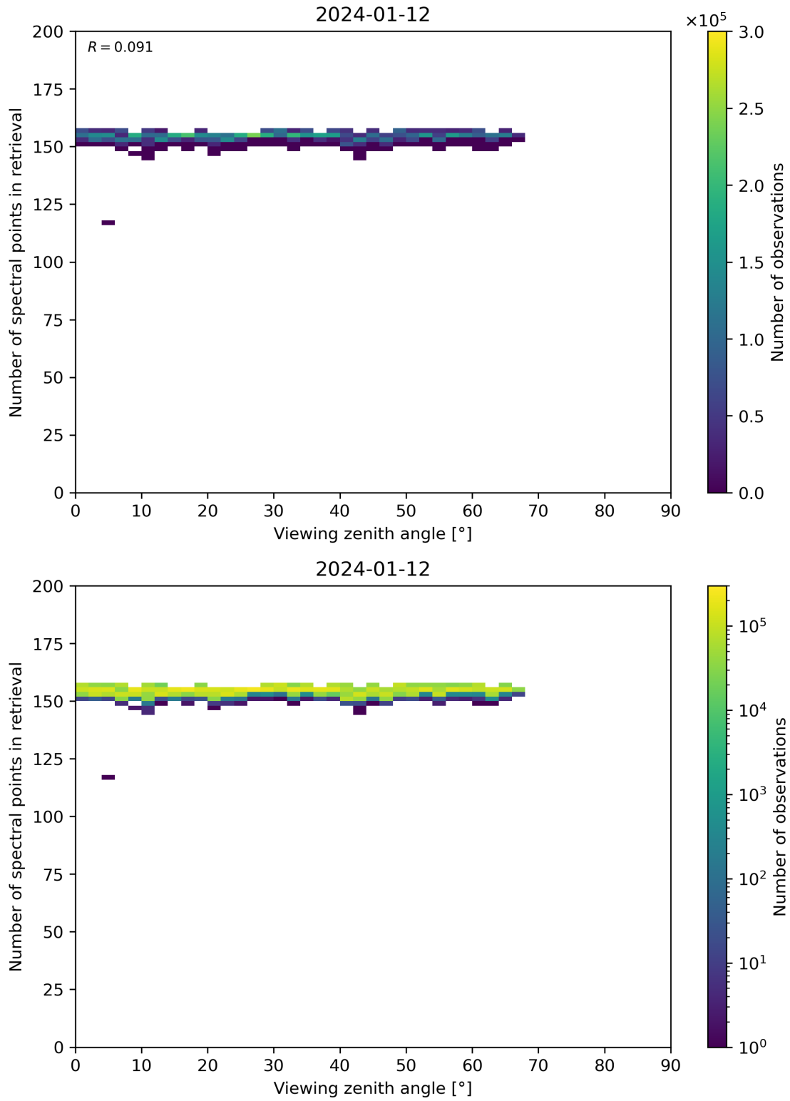
Figure 76: Scatter density plot of “Viewing zenith angle” against “Number of spectral points in retrieval” for 2024-01-11 to 2024-01-13.
