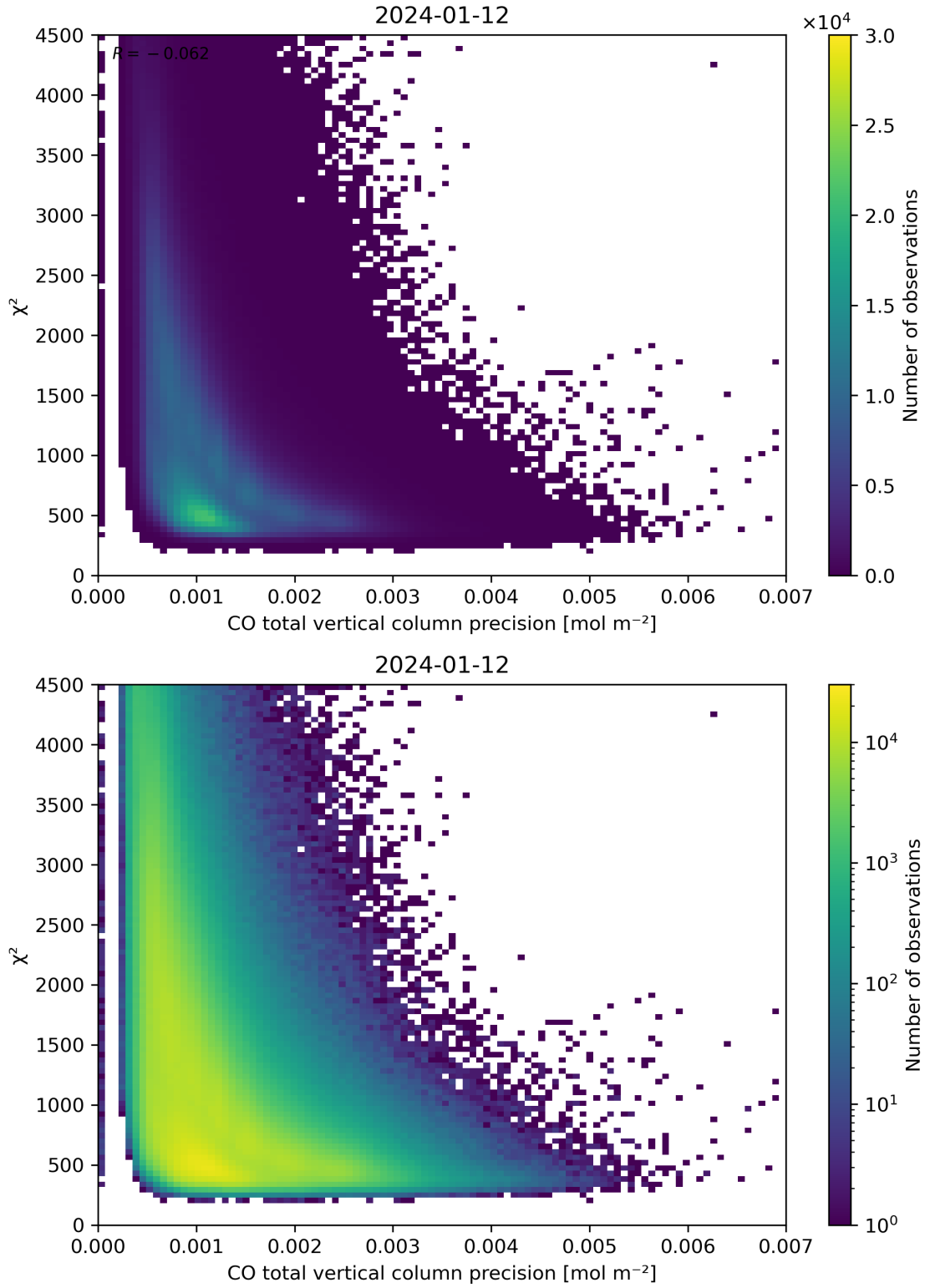
Figure 44: Scatter density plot of “CO total vertical column precision” against “ \chi^2 ” for 2024-01-11 to 2024-01-13.
