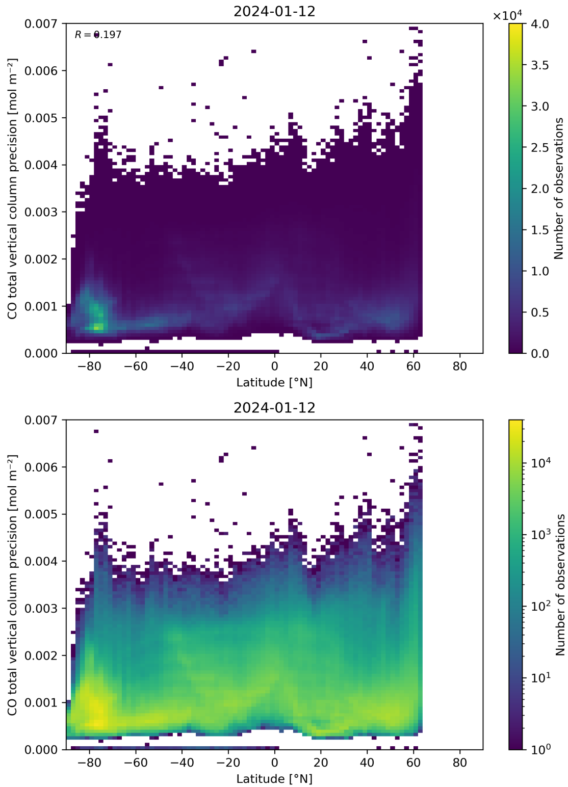
Figure 53: Scatter density plot of “Latitude” against “CO total vertical column precision” for 2024-01-11 to 2024-01-13.
