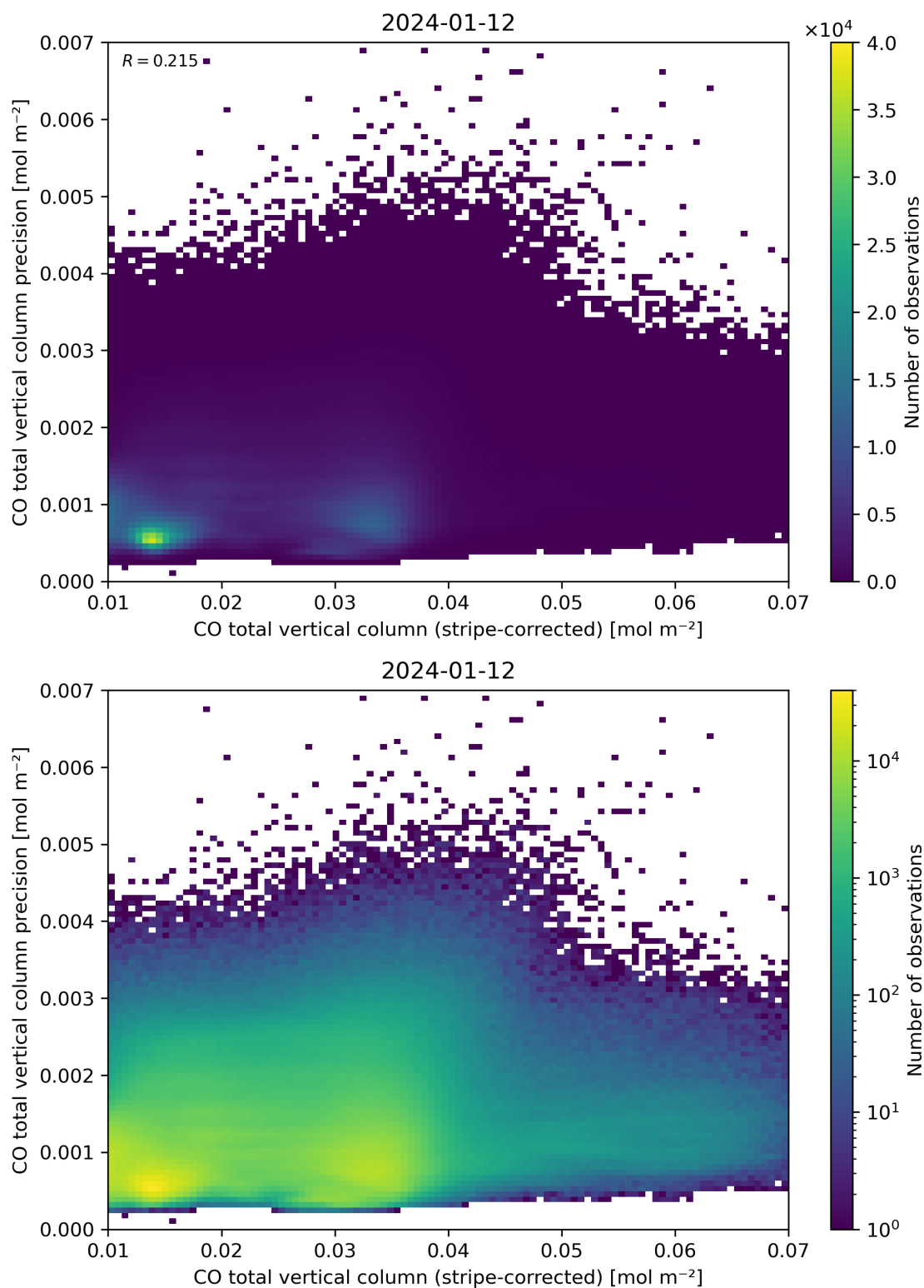
Figure 36: Scatter density plot of “CO total vertical column (stripe-corrected)” against “CO total vertical column precision” for 2024-01-11 to 2024-01-13.
