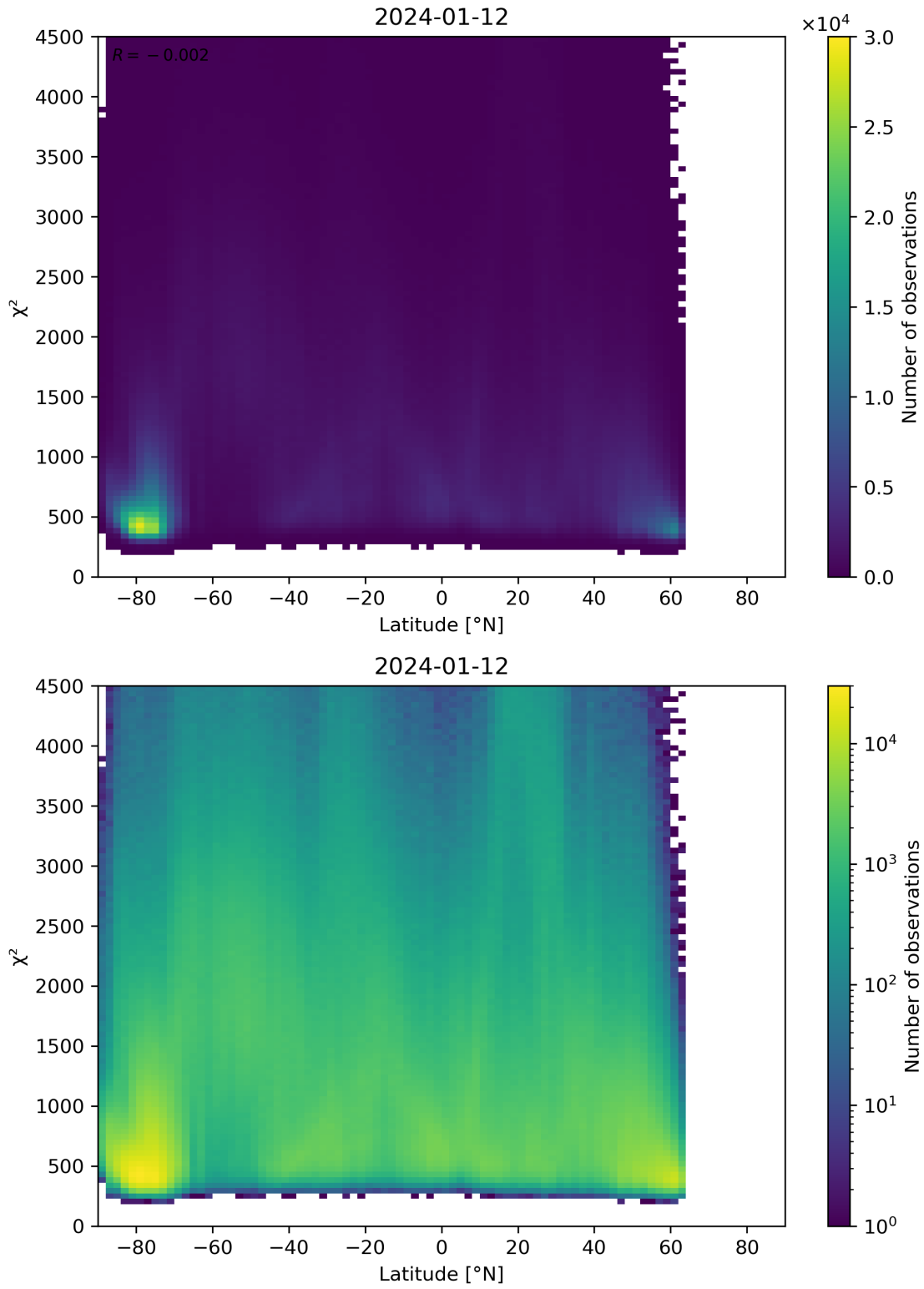
Figure 54: Scatter density plot of “Latitude” against “ \chi^2 ” for 2024-01-11 to 2024-01-13.
