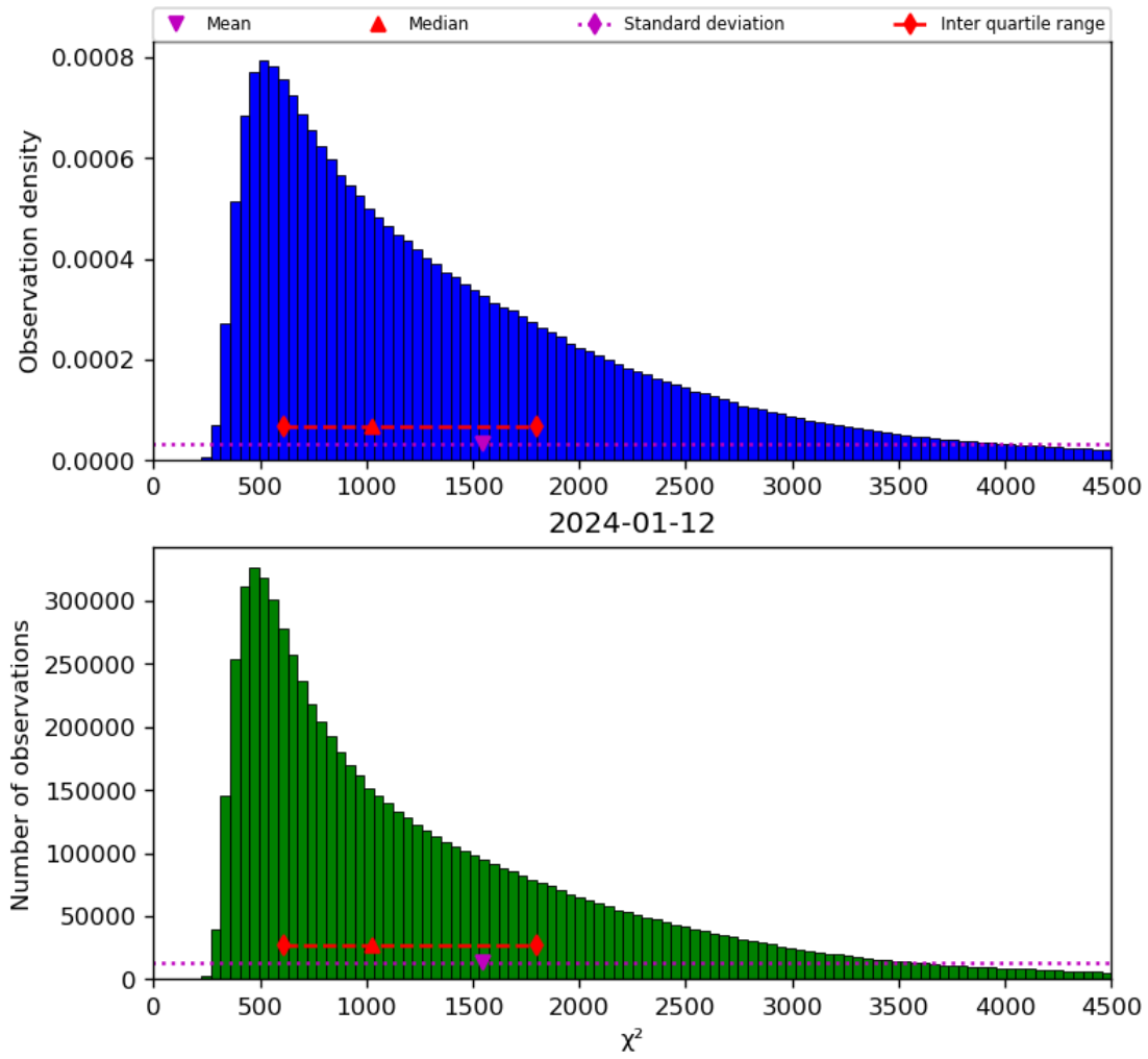
Figure 22: Histogram of “ \chi^2 ” for 2024-01-11 to 2024-01-13
