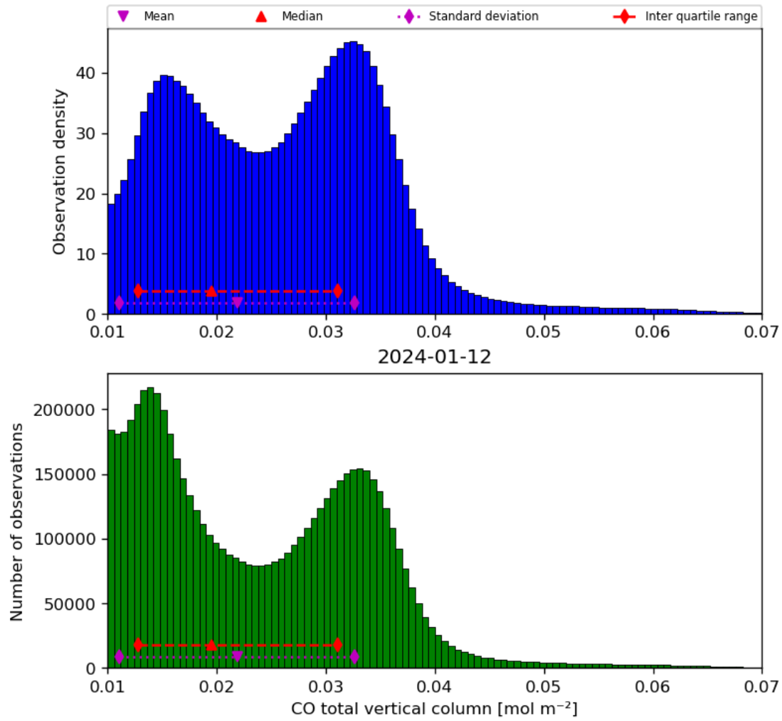
Figure 18: Histogram of “CO total vertical column” for 2024-01-11 to 2024-01-13
