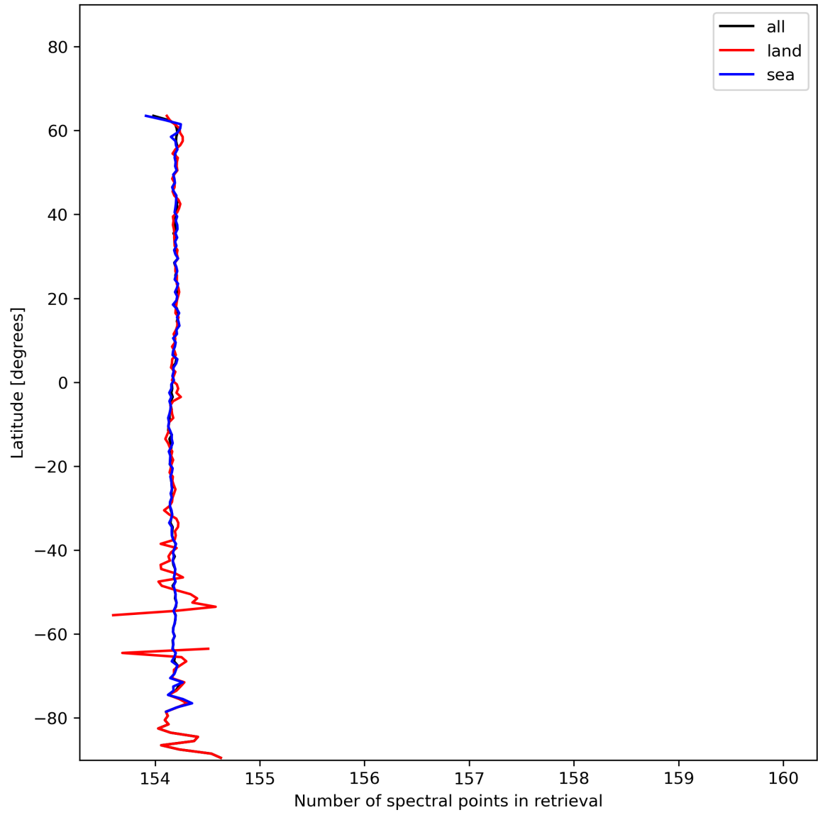
Figure 13: Zonal average of “Number of spectral points in retrieval” for 2024-01-11 to 2024-01-13.
