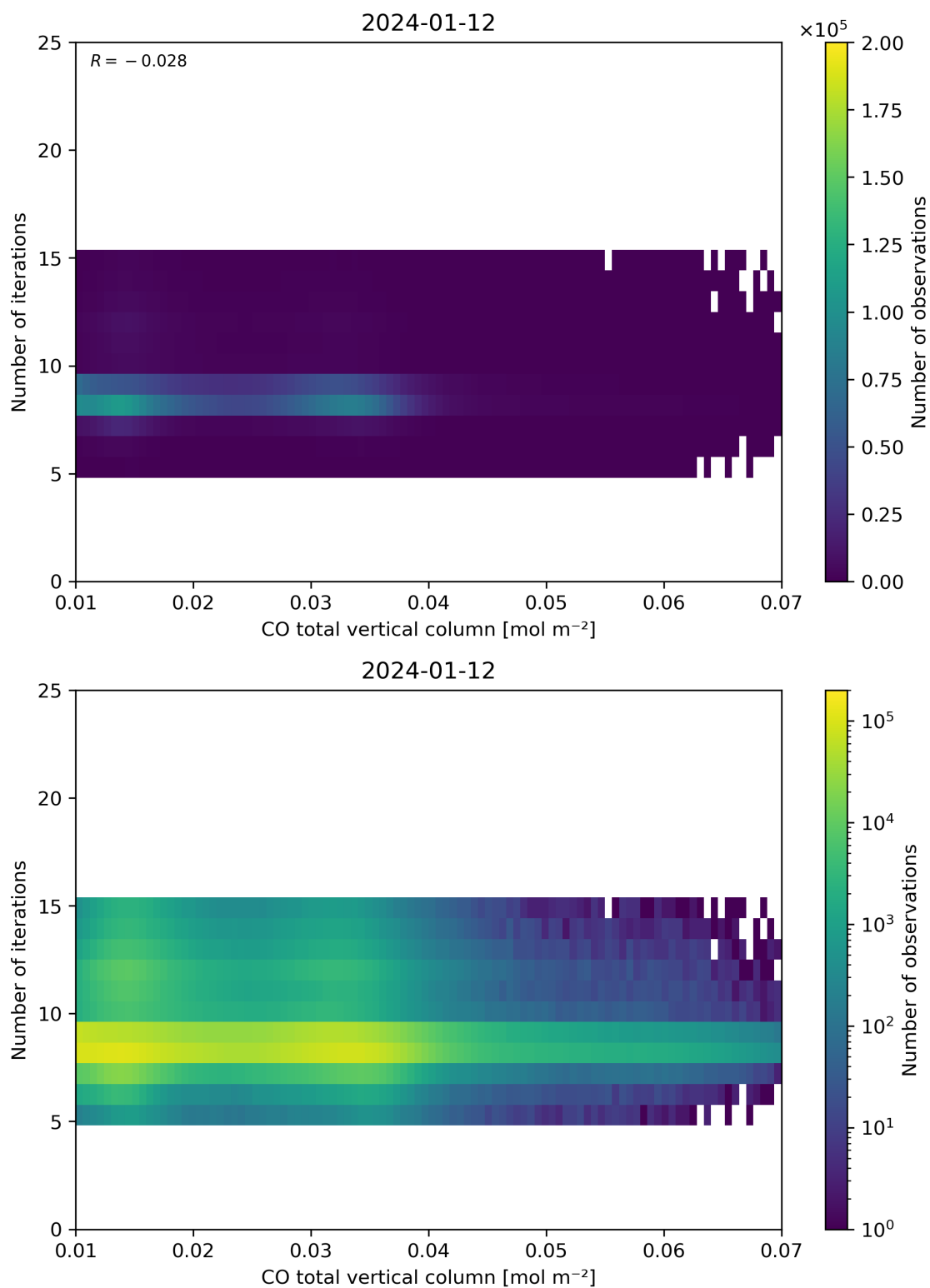
Figure 42: Scatter density plot of “CO total vertical column” against “Number of iterations” for 2024-01-11 to 2024-01-13.
