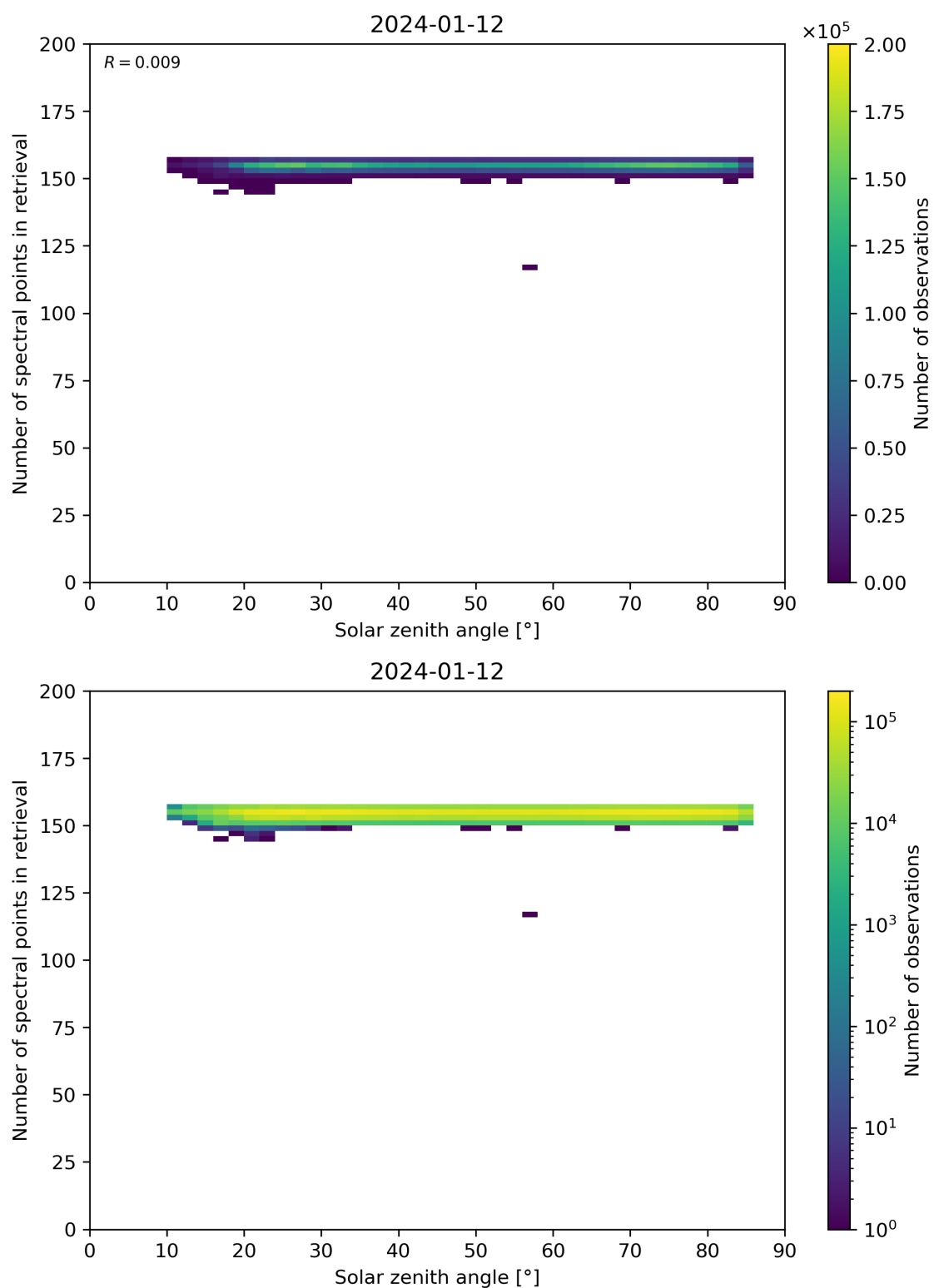
Figure 68: Scatter density plot of “Solar zenith angle” against “Number of spectral points in retrieval” for 2024-01-11 to 2024-01-13.
