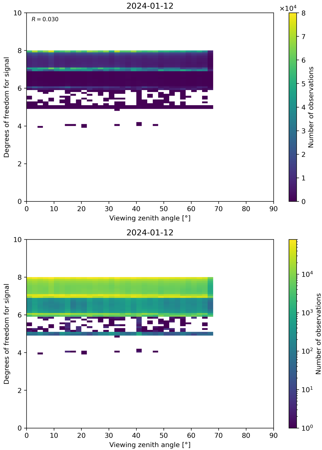
Figure 73: Scatter density plot of “Viewing zenith angle” against “Degrees of freedom for signal” for 2024-01-11 to 2024-01-13.
