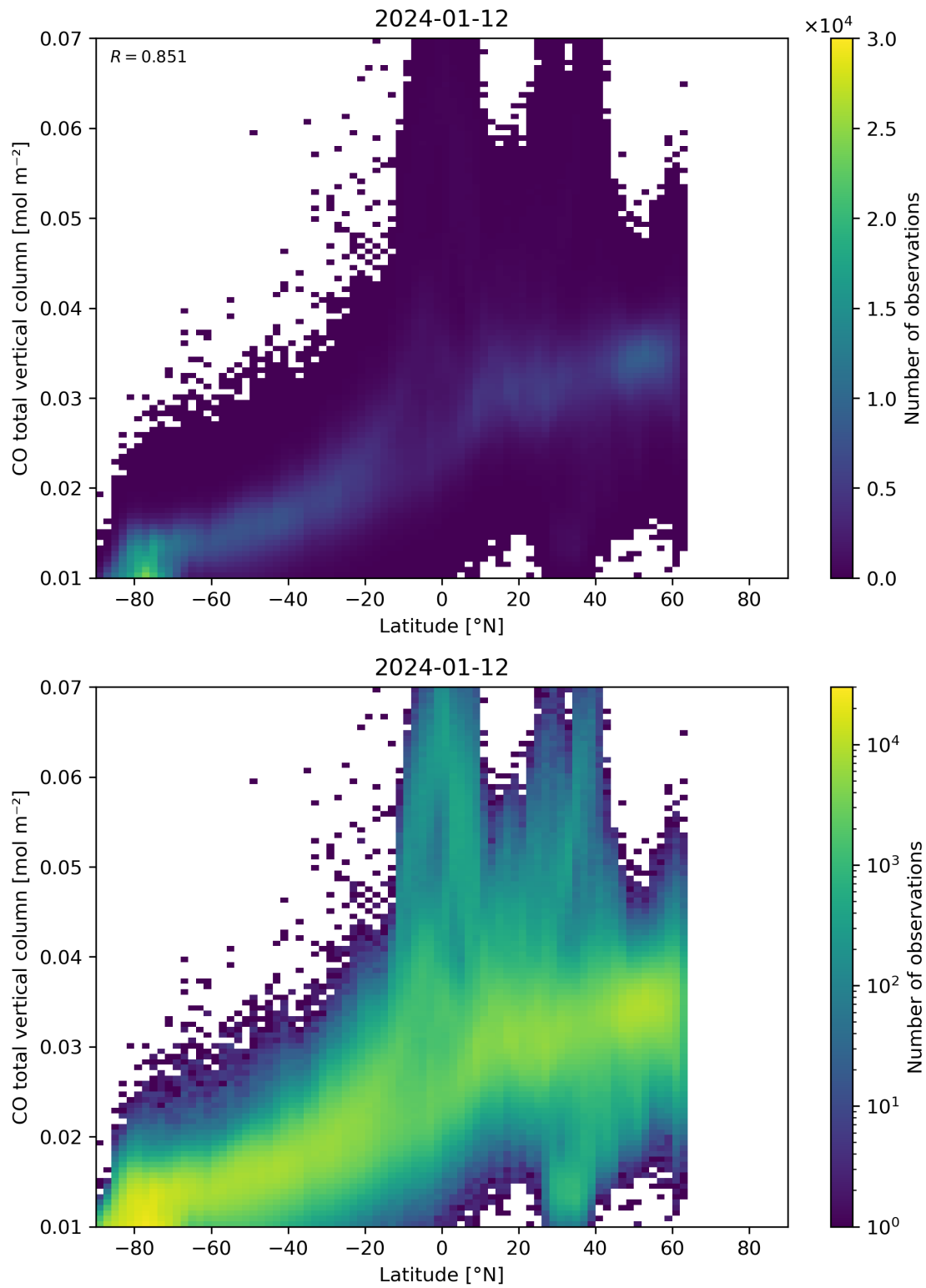
Figure 51: Scatter density plot of “Latitude” against “CO total vertical column” for 2024-01-11 to 2024-01-13.
