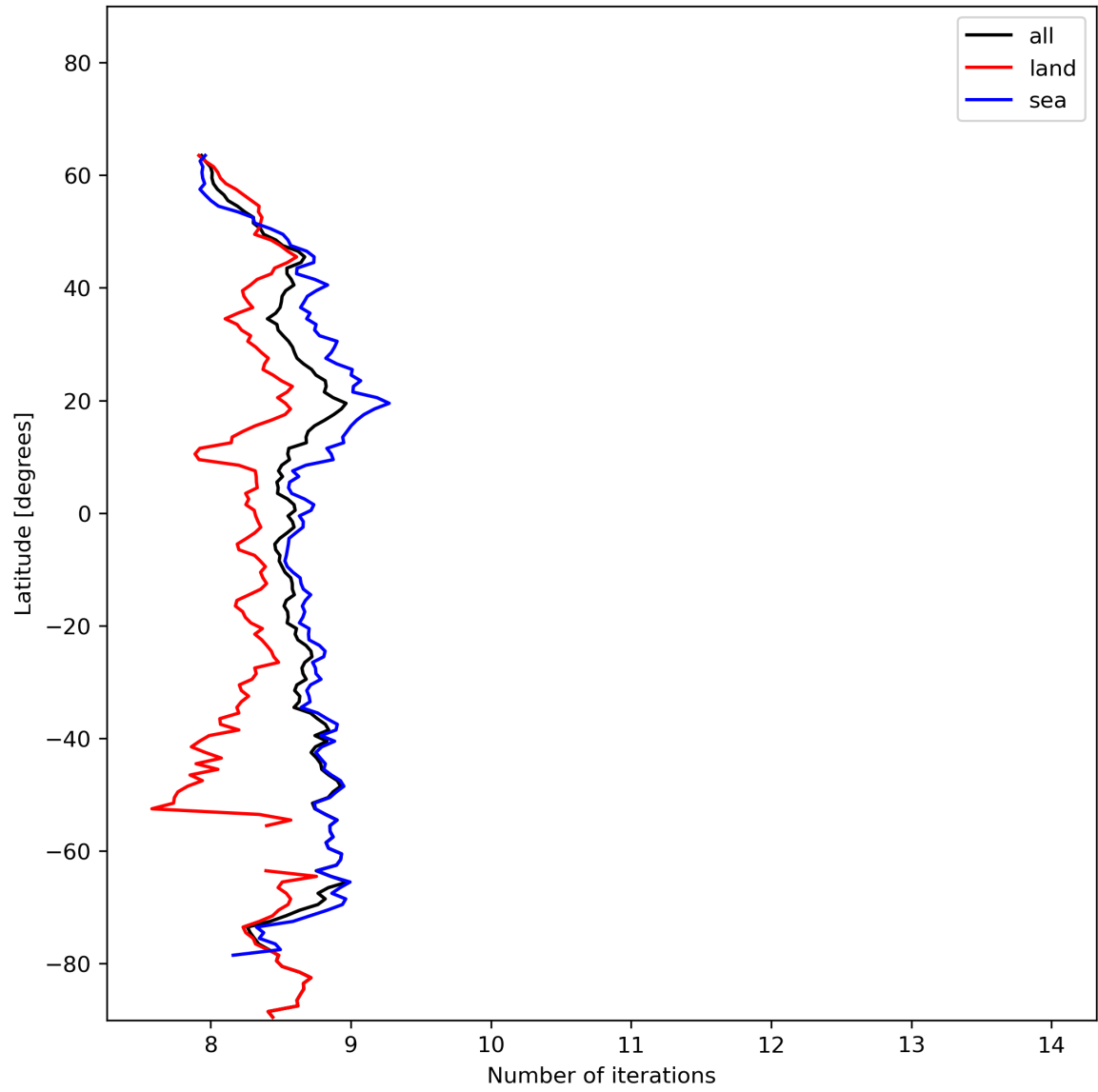
Figure 16: Zonal average of “Number of iterations” for 2024-01-11 to 2024-01-13.
