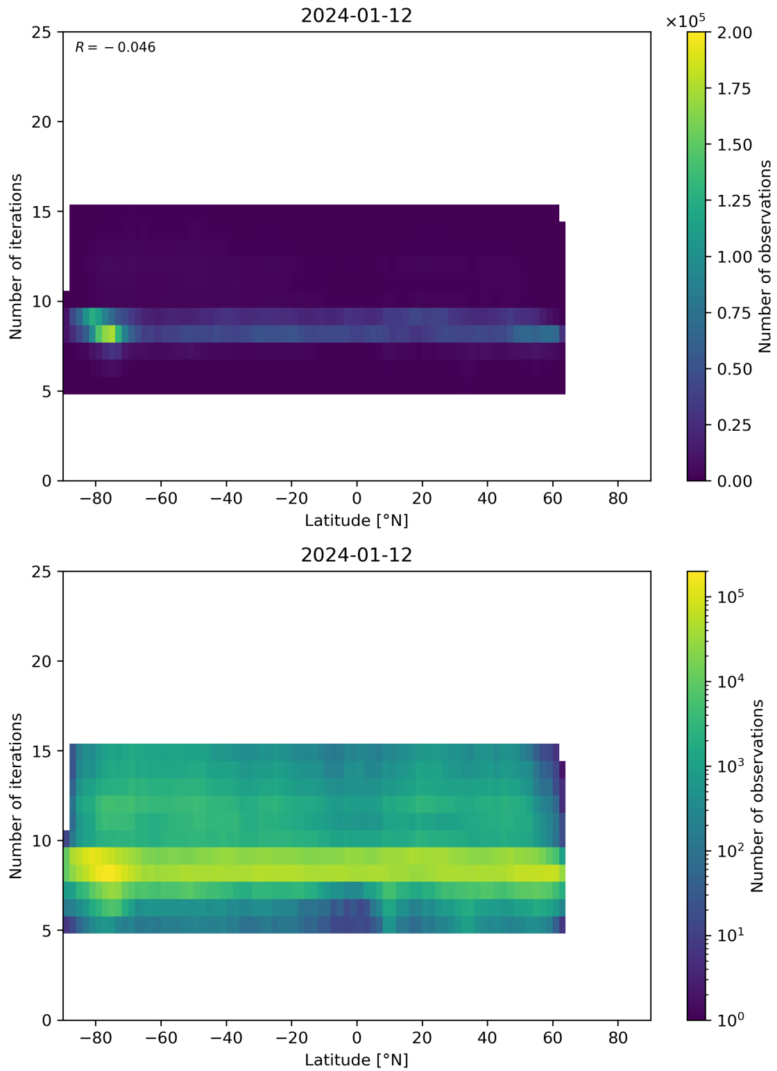
Figure 56: Scatter density plot of “Latitude” against “Number of iterations” for 2024-01-11 to 2024-01-13.
