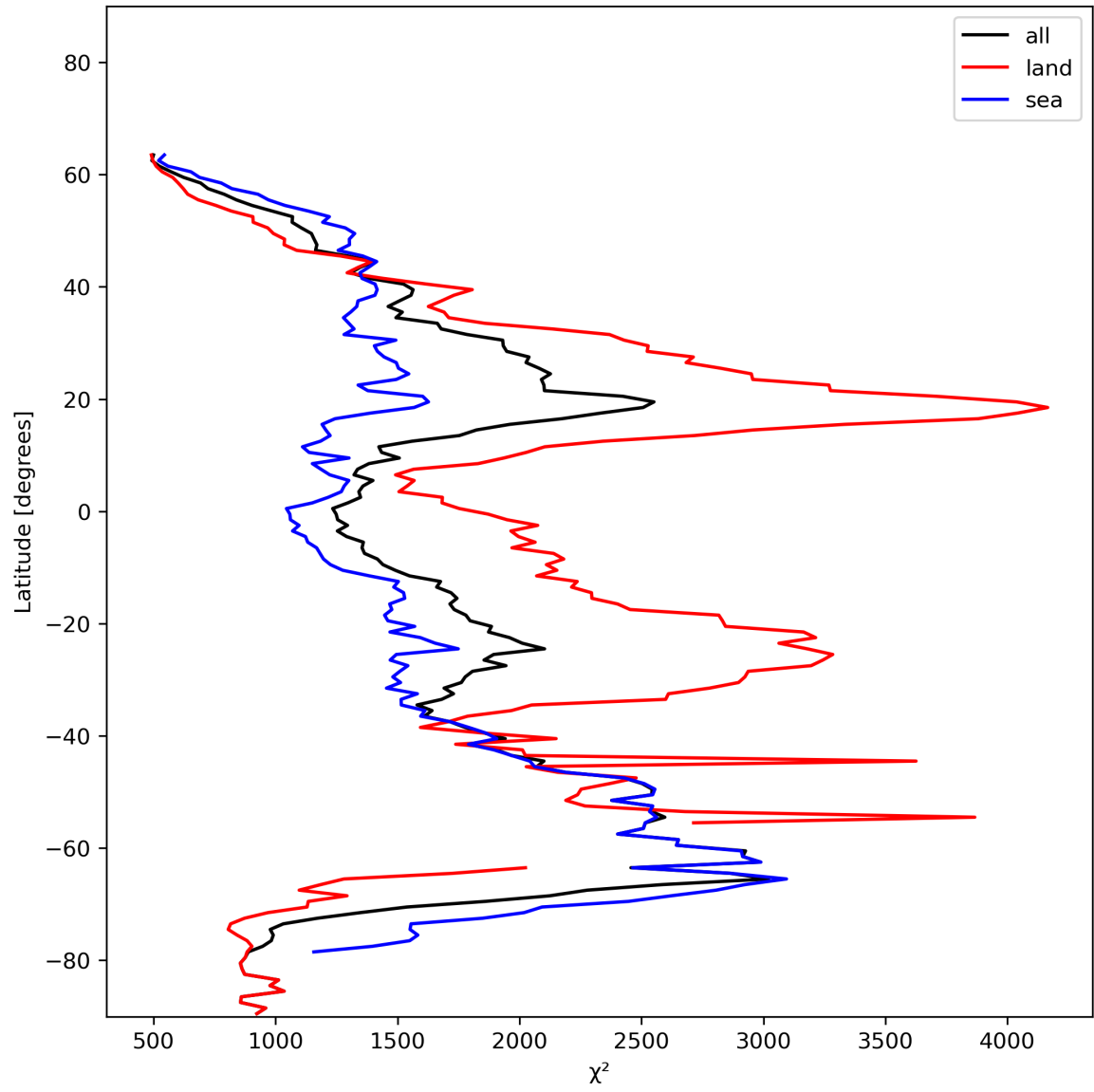
Figure 14: Zonal average of “ \chi^2 ” for 2024-01-11 to 2024-01-13.
