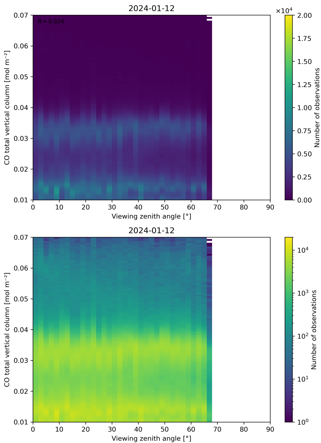
Figure 69: Scatter density plot of “Viewing zenith angle” against “CO total vertical column” for 2024-01-11 to 2024-01-13.
