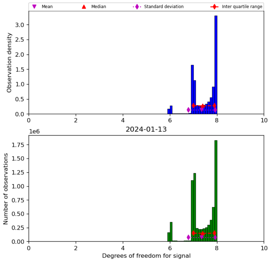
Figure 23: Histogram of “Degrees of freedom for signal” for 2024-01-12 to 2024-01-14
