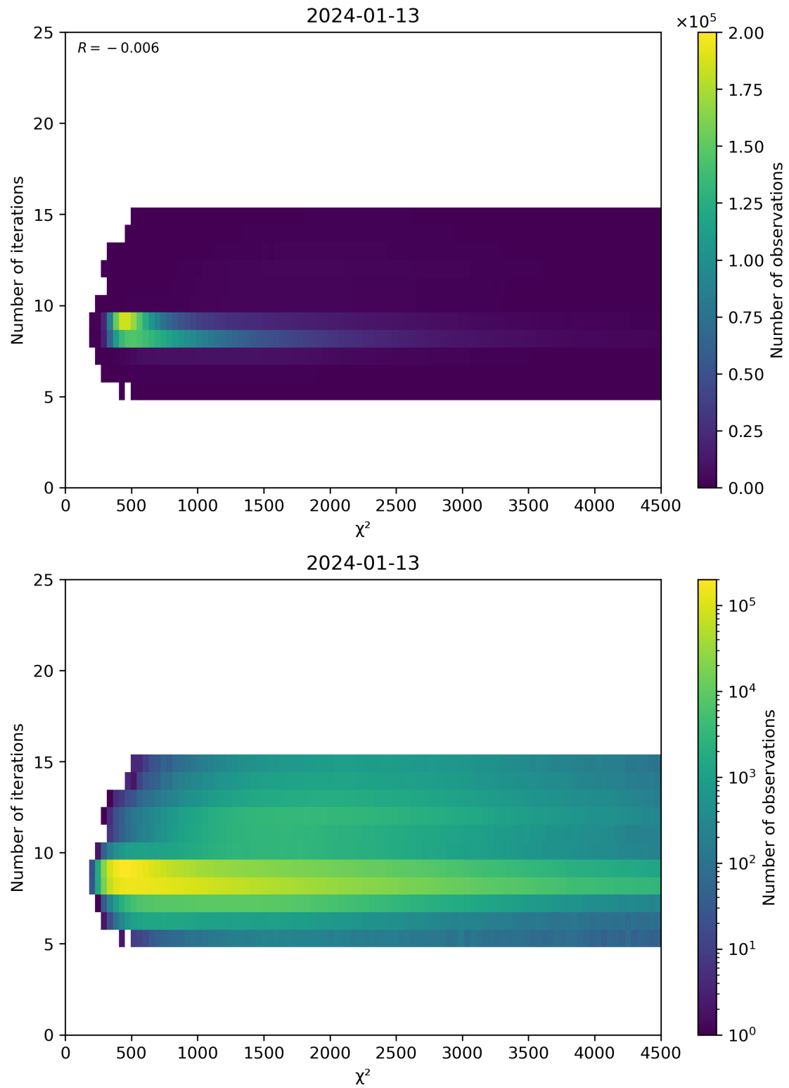
Figure 49: Scatter density plot of “ \chi^2 ” against “Number of iterations” for 2024-01-12 to 2024-01-14.
