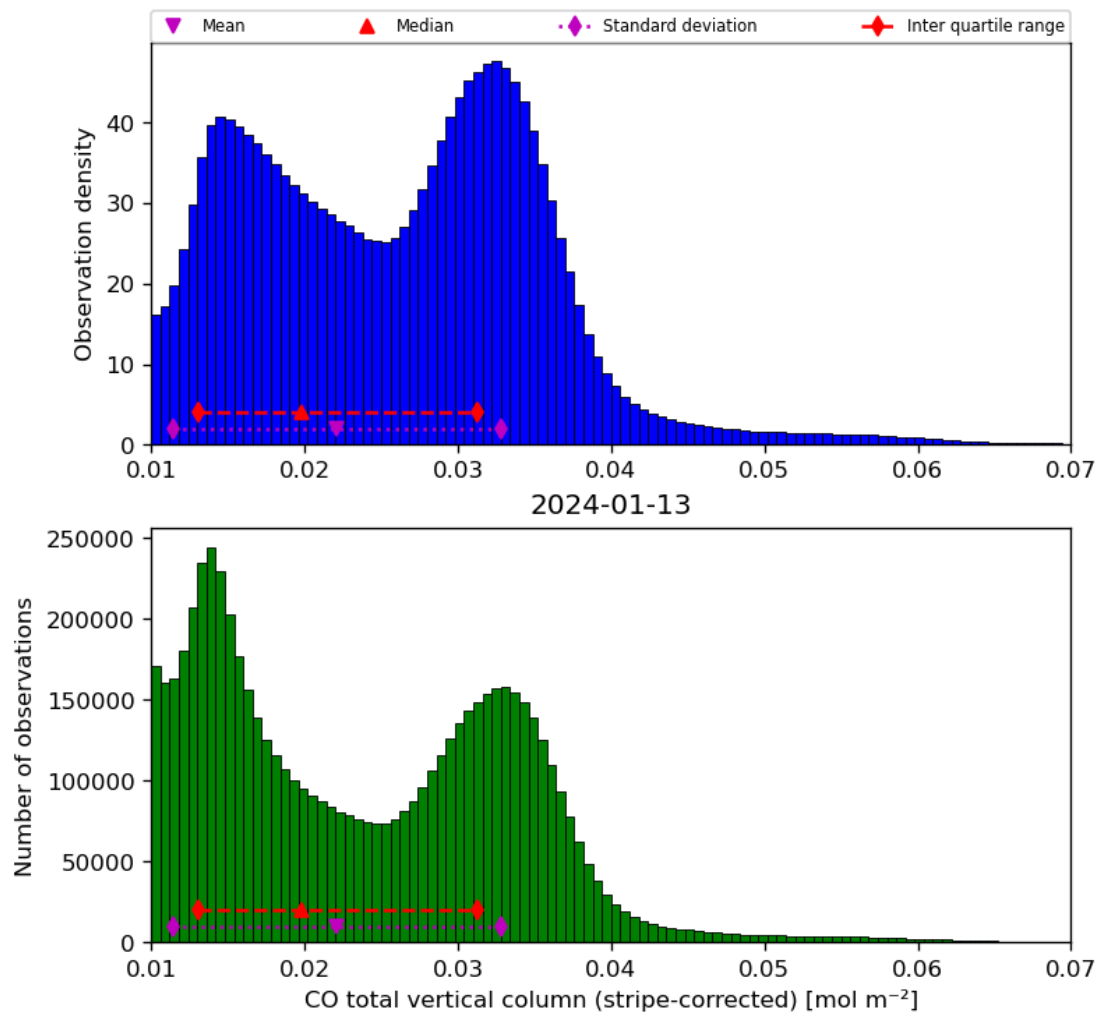
Figure 19: Histogram of “CO total vertical column (stripe-corrected)” for 2024-01-12 to 2024-01-14
