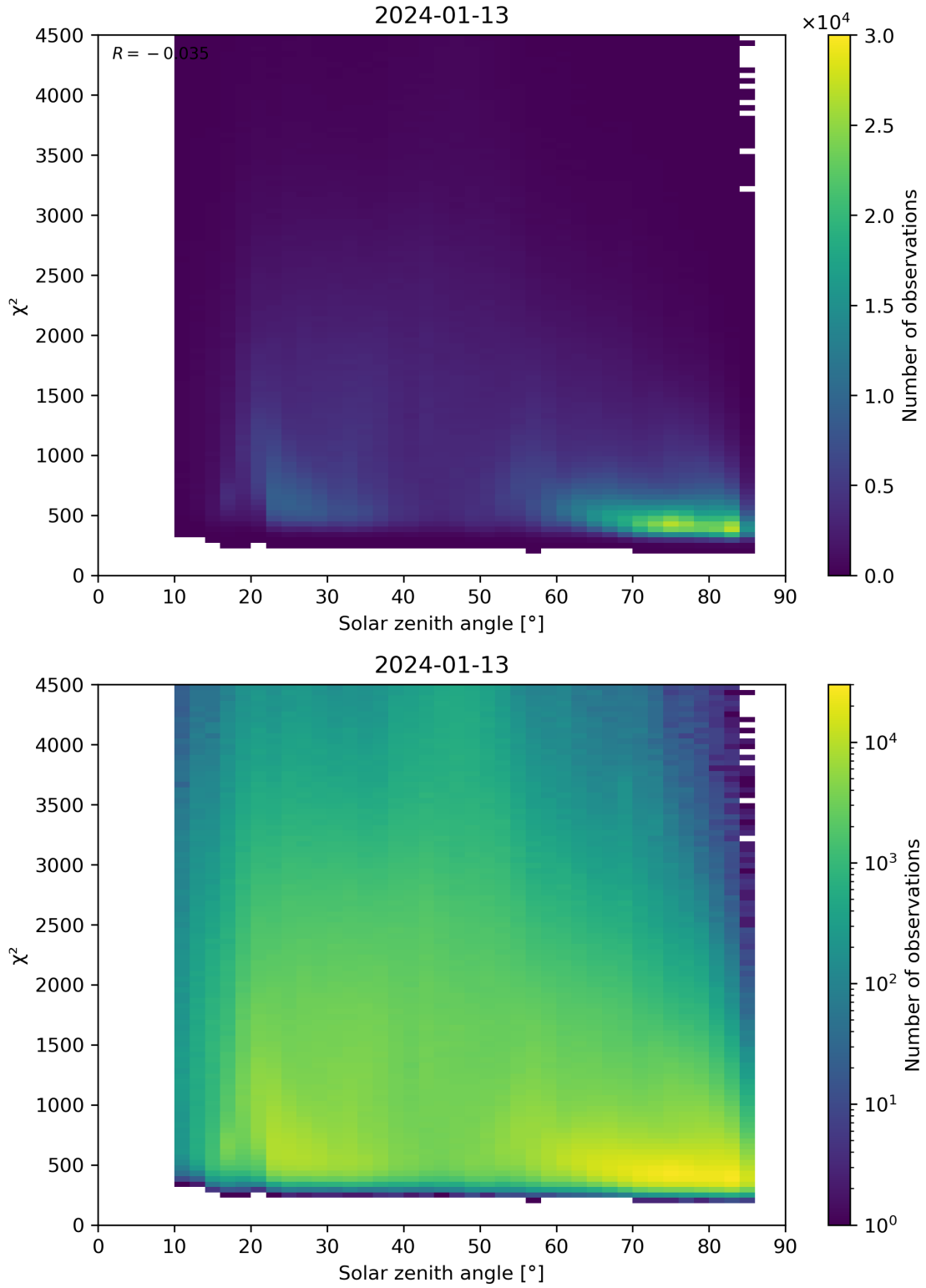
Figure 64: Scatter density plot of “Solar zenith angle” against “ \chi^2 ” for 2024-01-12 to 2024-01-14.
