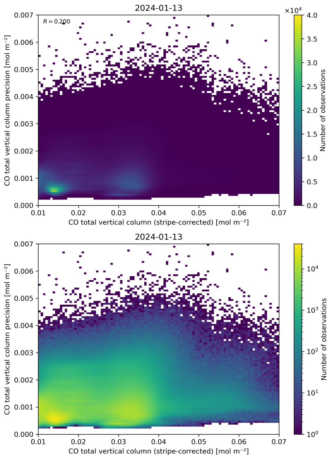
Figure 36: Scatter density plot of “CO total vertical column (stripe-corrected)” against “CO total vertical column precision” for 2024-01-12 to 2024-01-14.
