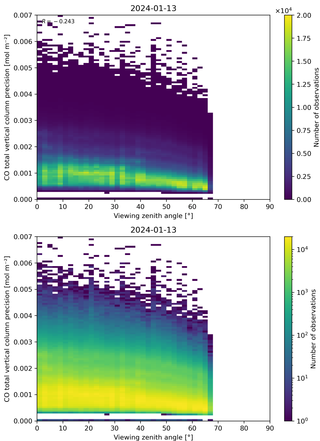
Figure 71: Scatter density plot of “Viewing zenith angle” against “CO total vertical column precision” for 2024-01-12 to 2024-01-14.
