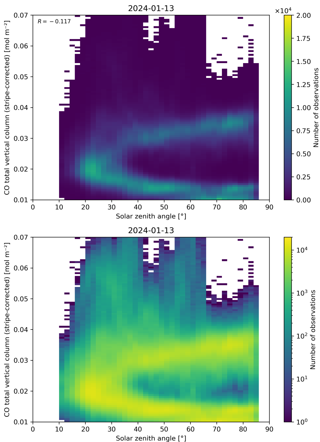
Figure 62: Scatter density plot of “Solar zenith angle” against “CO total vertical column (stripe-corrected)” for 2024-01-12 to 2024-01-14.
