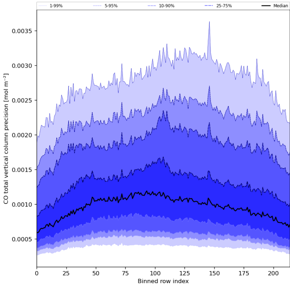
Figure 28: Along track statistics of “CO total vertical column precision” for 2024-01-12 to 2024-01-14
