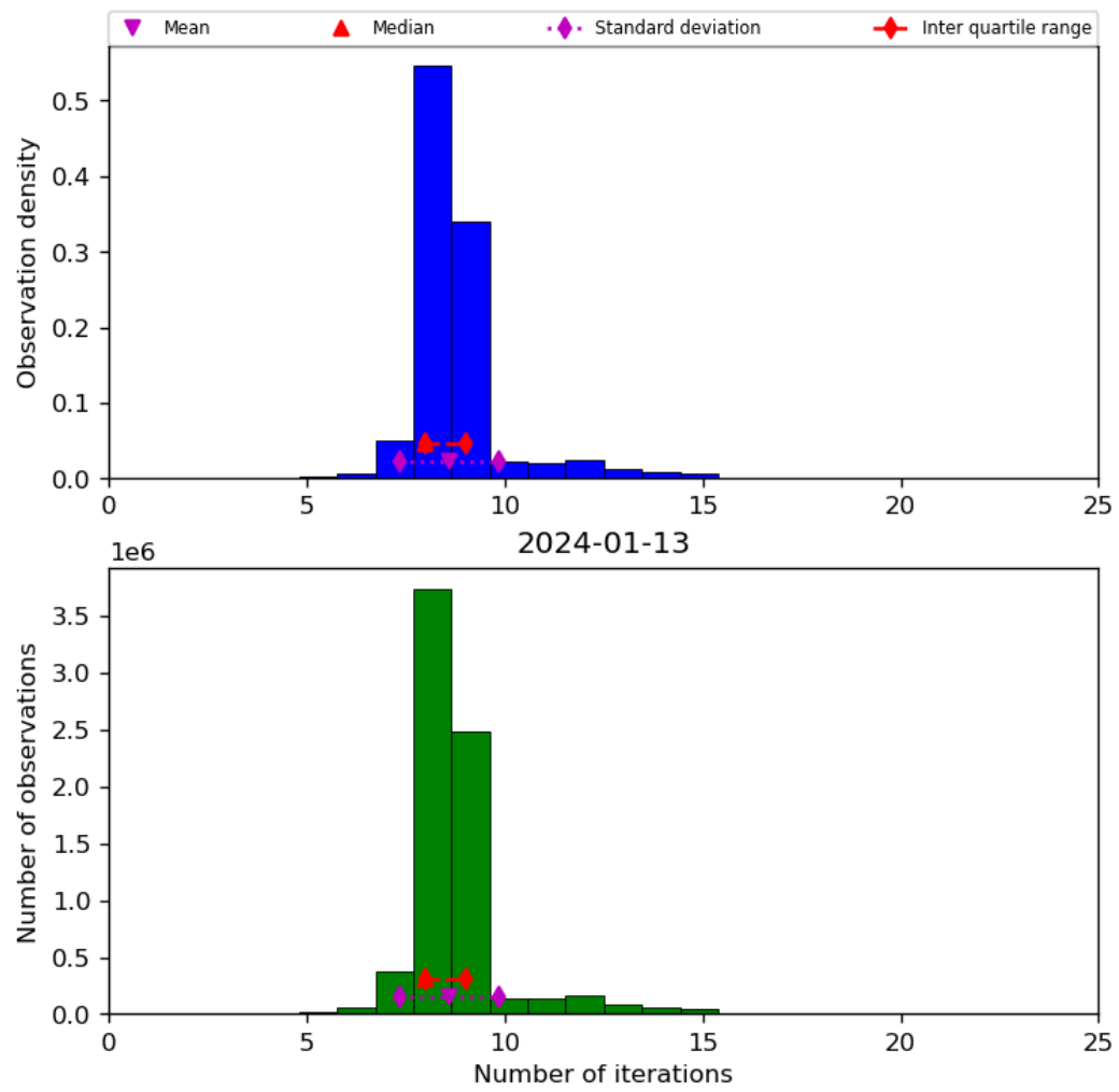
Figure 24: Histogram of “Number of iterations” for 2024-01-12 to 2024-01-14
