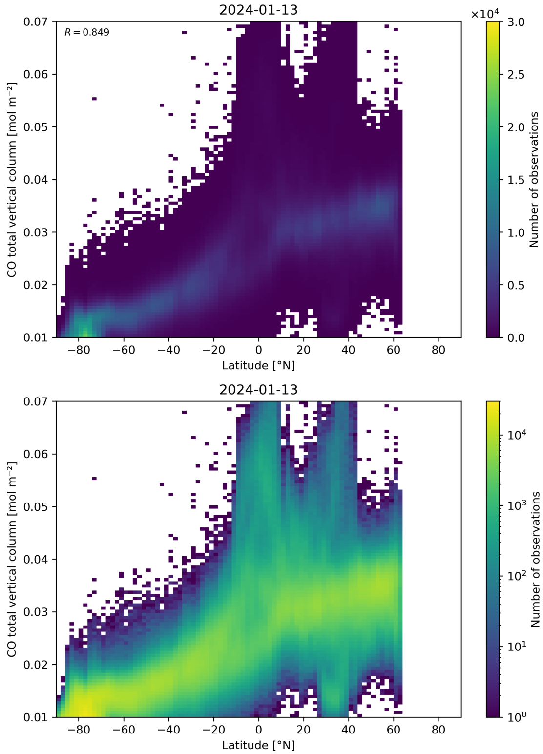
Figure 51: Scatter density plot of “Latitude” against “CO total vertical column” for 2024-01-12 to 2024-01-14.
