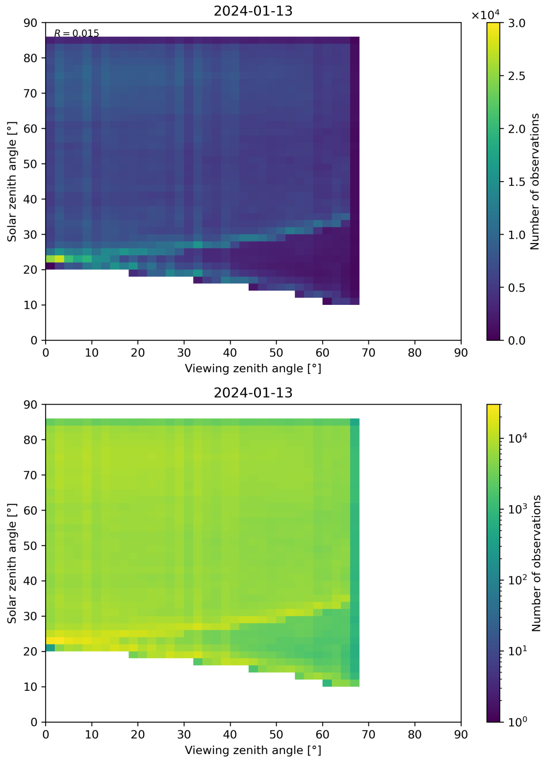
Figure 77: Scatter density plot of “Viewing zenith angle” against “Solar zenith angle” for 2024-01-12 to 2024-01-14.
