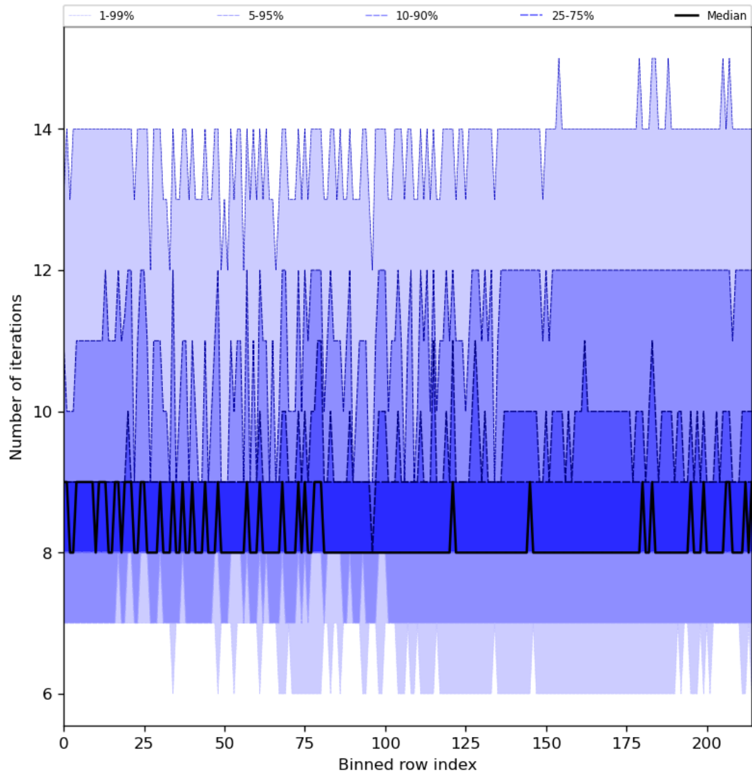
Figure 32: Along track statistics of “Number of iterations” for 2024-01-12 to 2024-01-14
