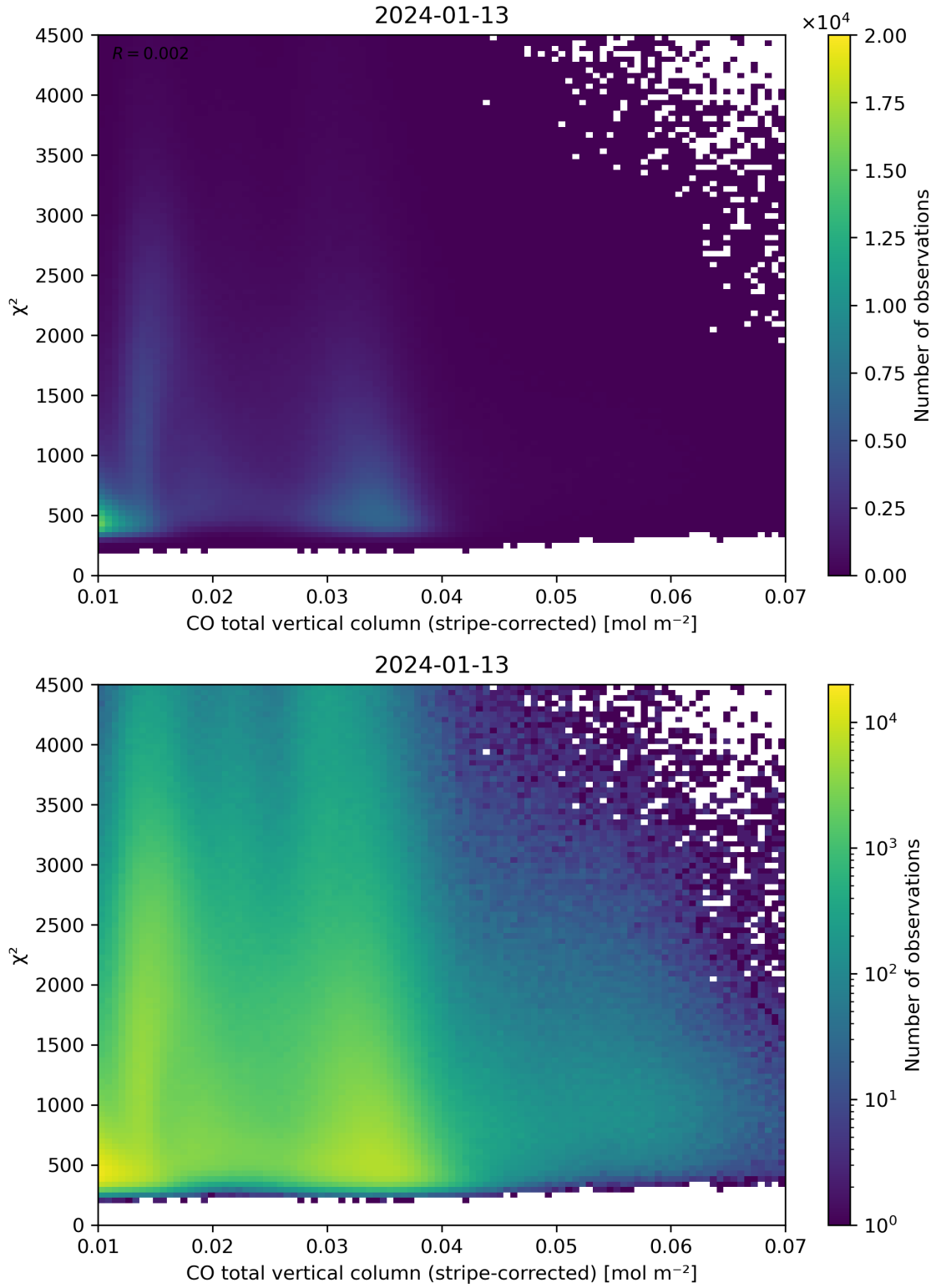
Figure 37: Scatter density plot of “CO total vertical column (stripe-corrected)” against “ \chi^2 ” for 2024-01-12 to 2024-01-14.
