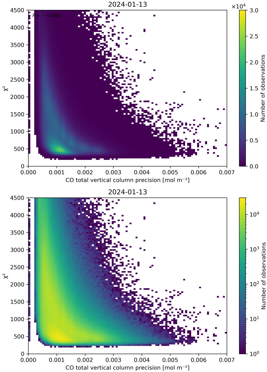
Figure 44: Scatter density plot of “CO total vertical column precision” against “ \chi^2 ” for 2024-01-12 to 2024-01-14.
