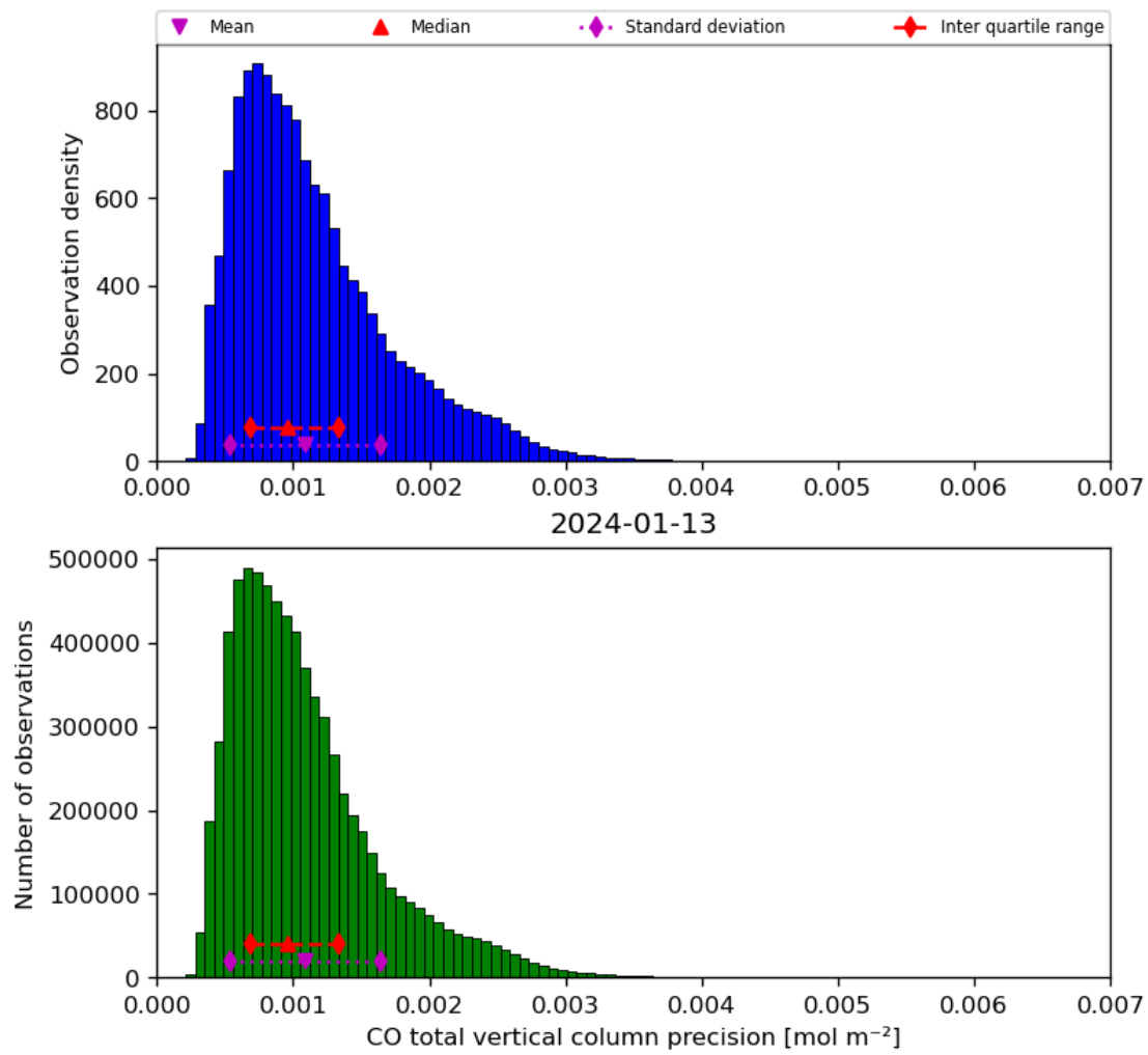
Figure 20: Histogram of “CO total vertical column precision” for 2024-01-12 to 2024-01-14
