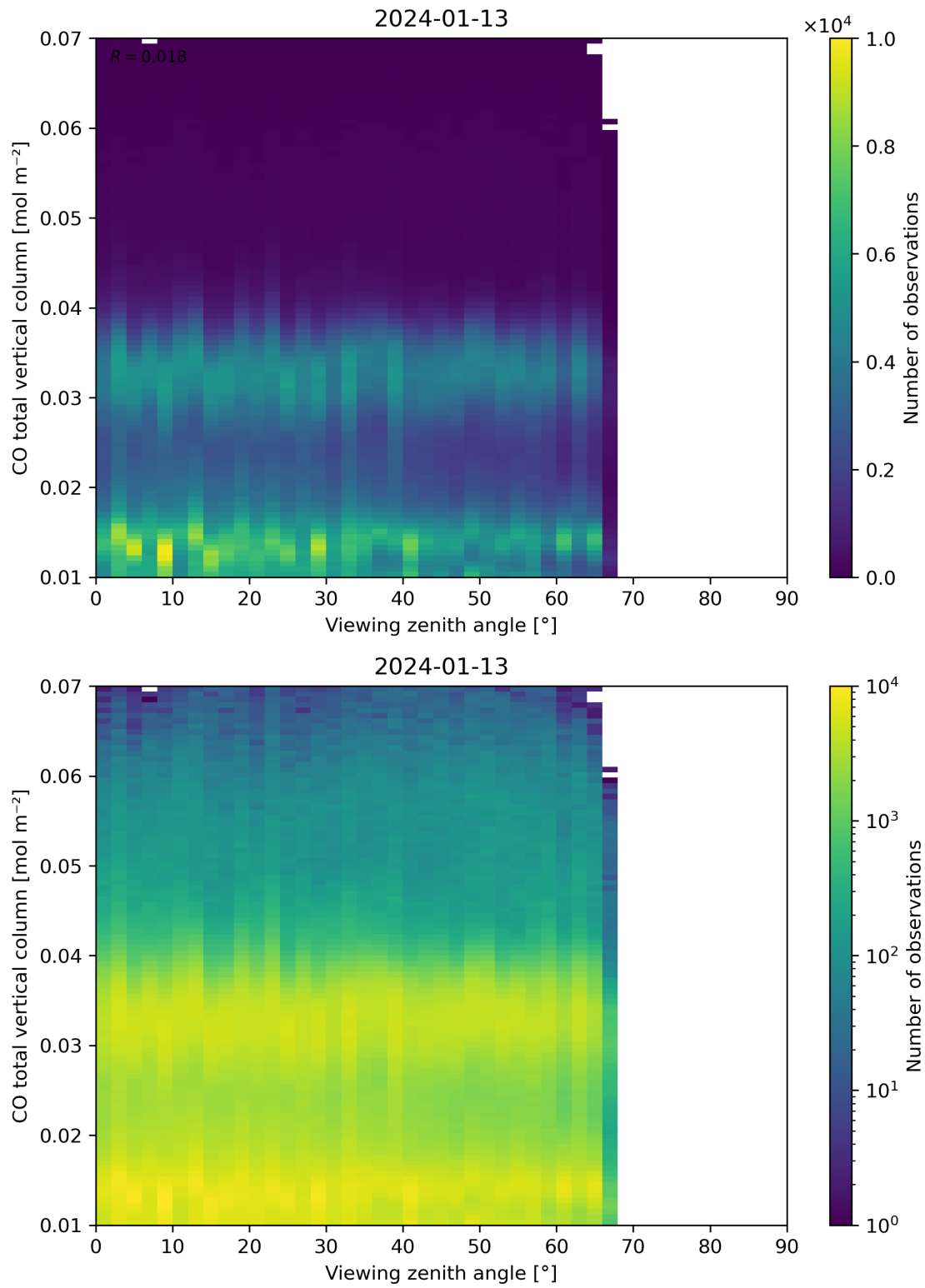
Figure 69: Scatter density plot of “Viewing zenith angle” against “CO total vertical column” for 2024-01-12 to 2024-01-14.
