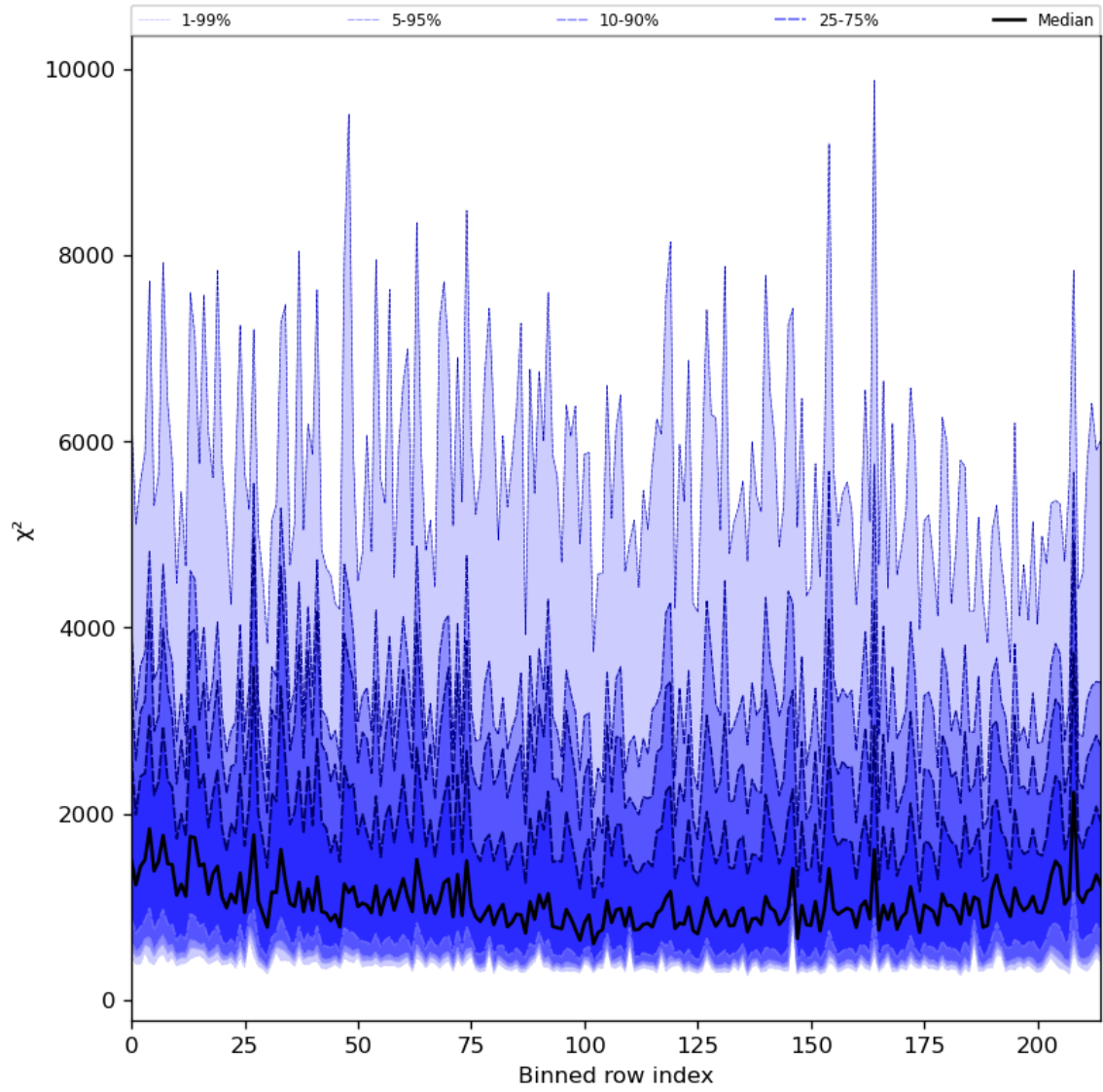
Figure 30: Along track statistics of “ \chi^2 ” for 2024-01-12 to 2024-01-14
