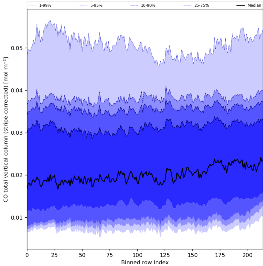
Figure 27: Along track statistics of “CO total vertical column (stripe-corrected)” for 2024-01-12 to 2024-01-14
