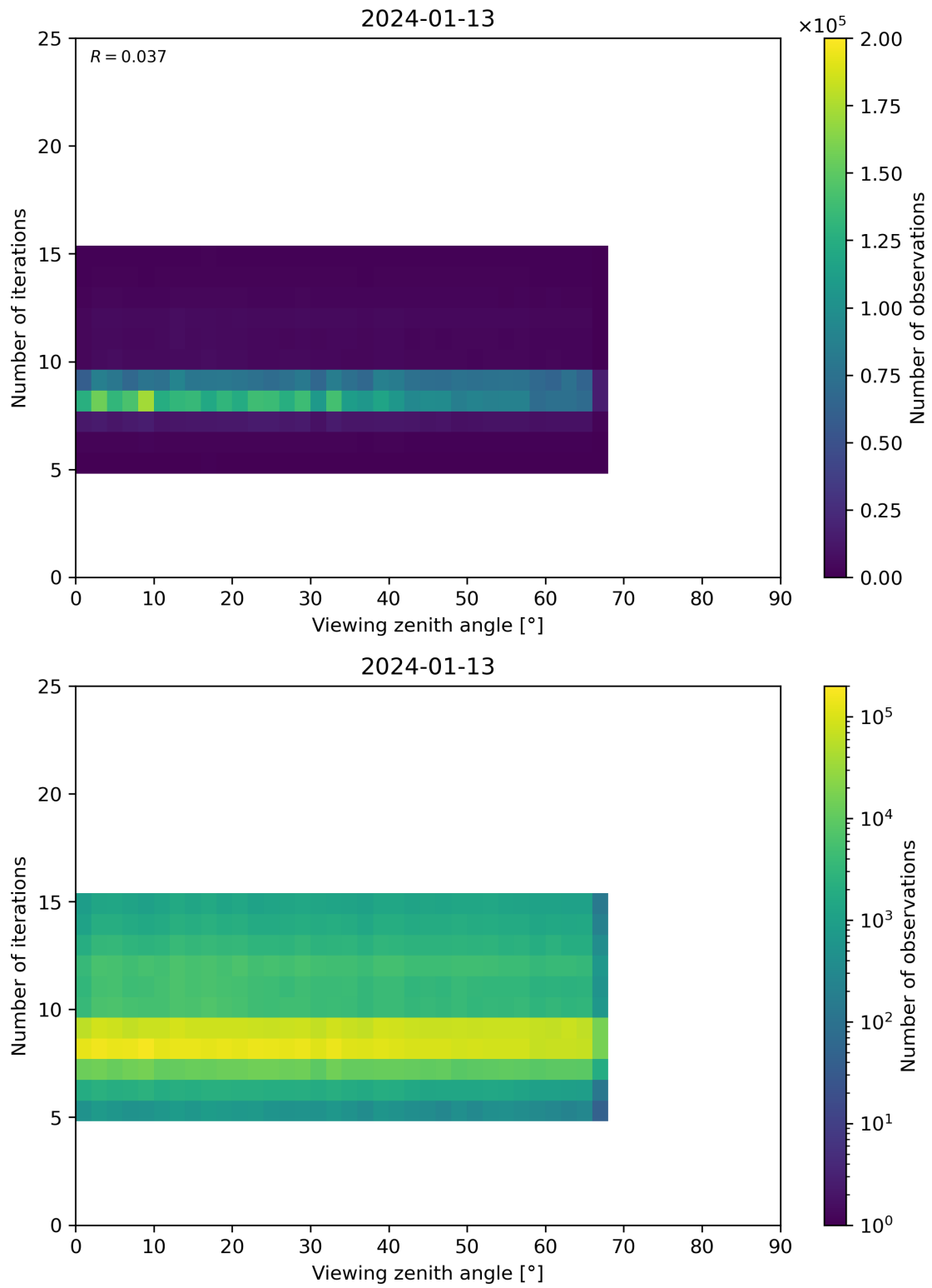
Figure 75: Scatter density plot of “Viewing zenith angle” against “Number of iterations” for 2024-01-12 to 2024-01-14.
