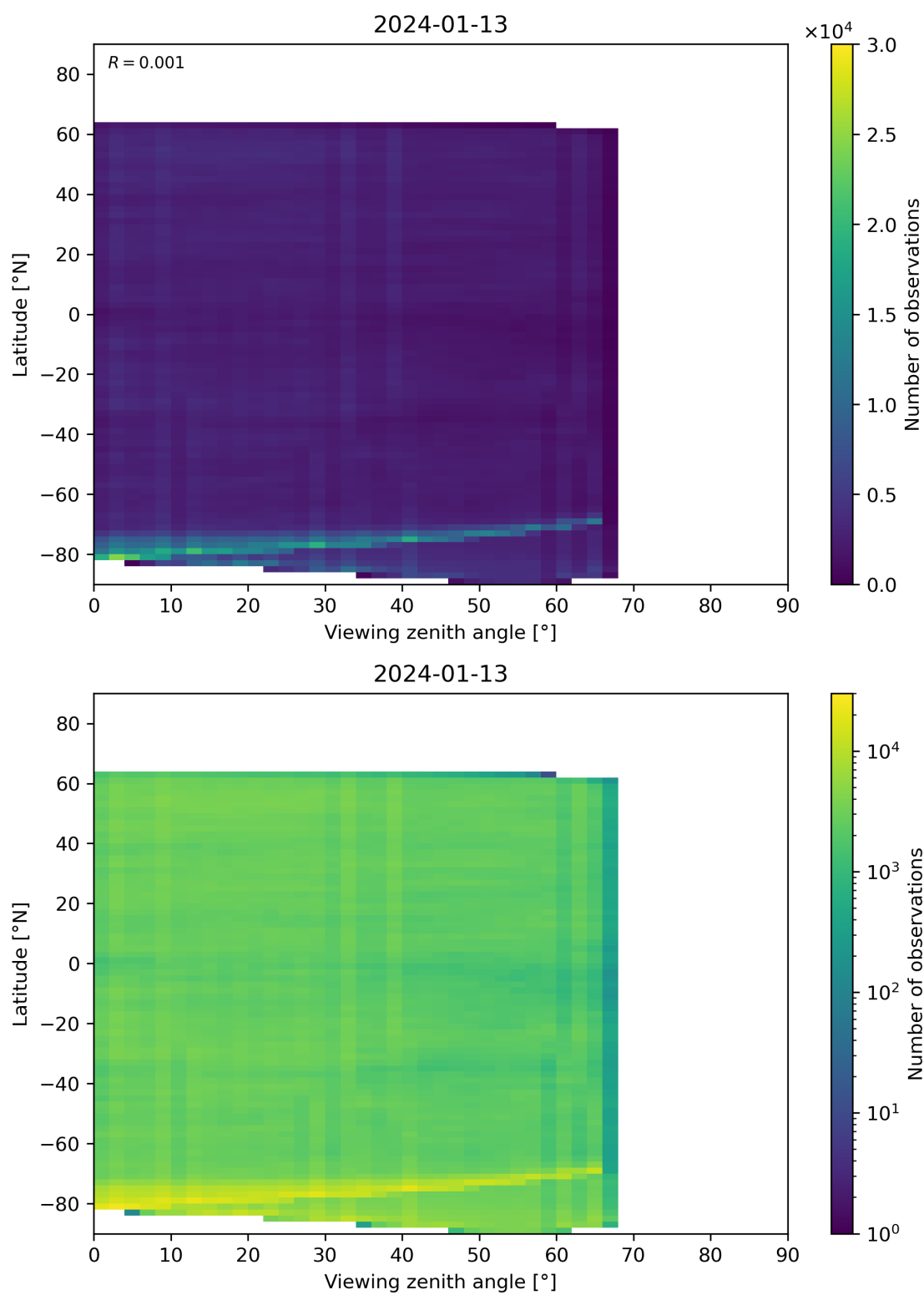
Figure 74: Scatter density plot of “Viewing zenith angle” against “Latitude” for 2024-01-12 to 2024-01-14.
