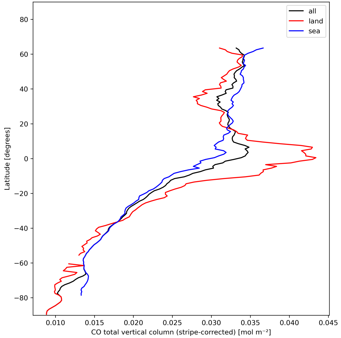
Figure 11: Zonal average of “CO total vertical column (stripe-corrected)” for 2024-01-12 to 2024-01-14.
