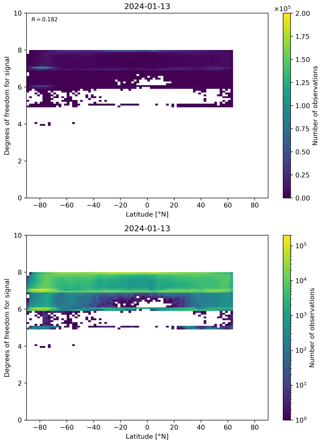
Figure 55: Scatter density plot of “Latitude” against “Degrees of freedom for signal” for 2024-01-12 to 2024-01-14.
