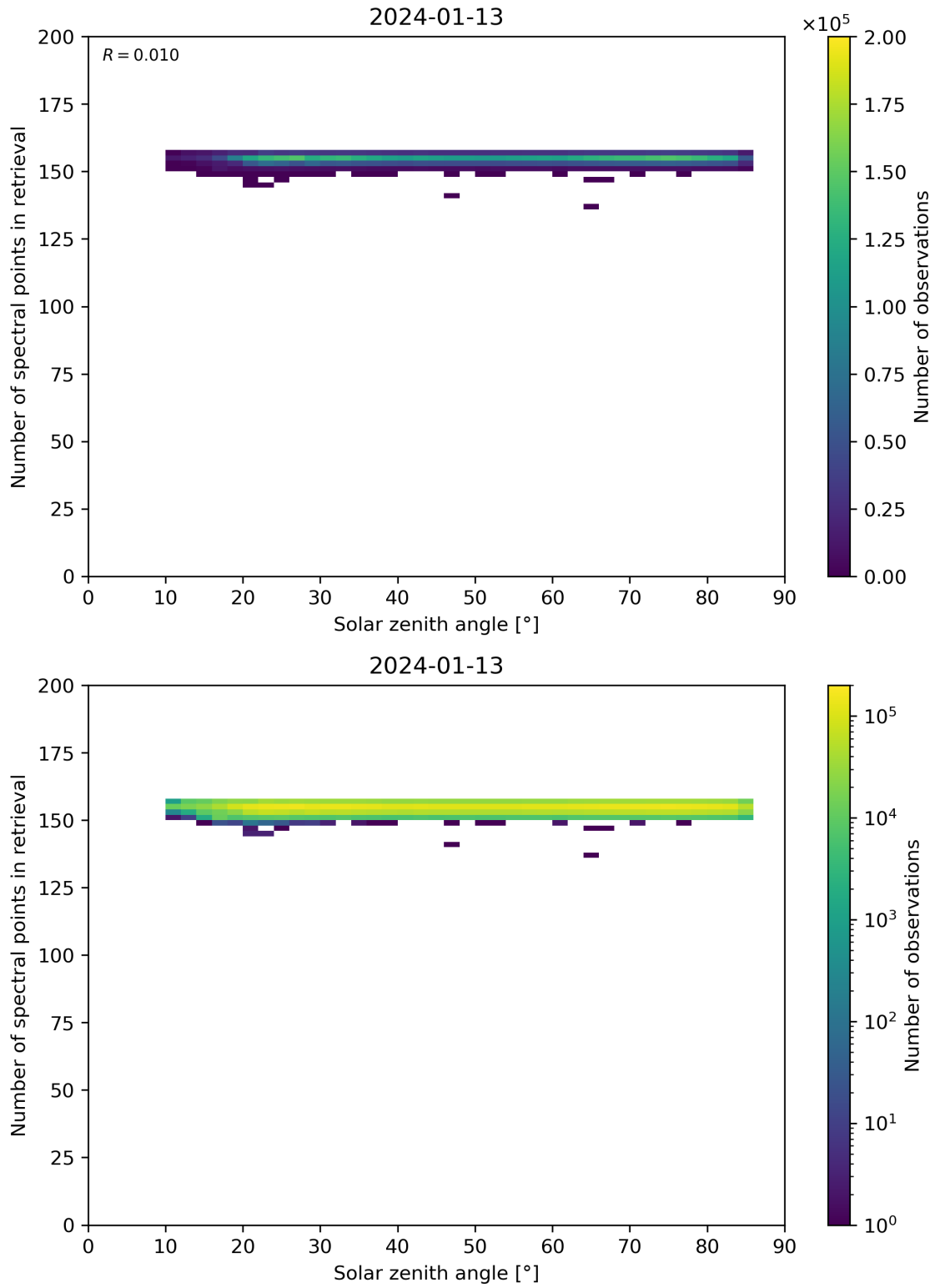
Figure 68: Scatter density plot of “Solar zenith angle” against “Number of spectral points in retrieval” for 2024-01-12 to 2024-01-14.
