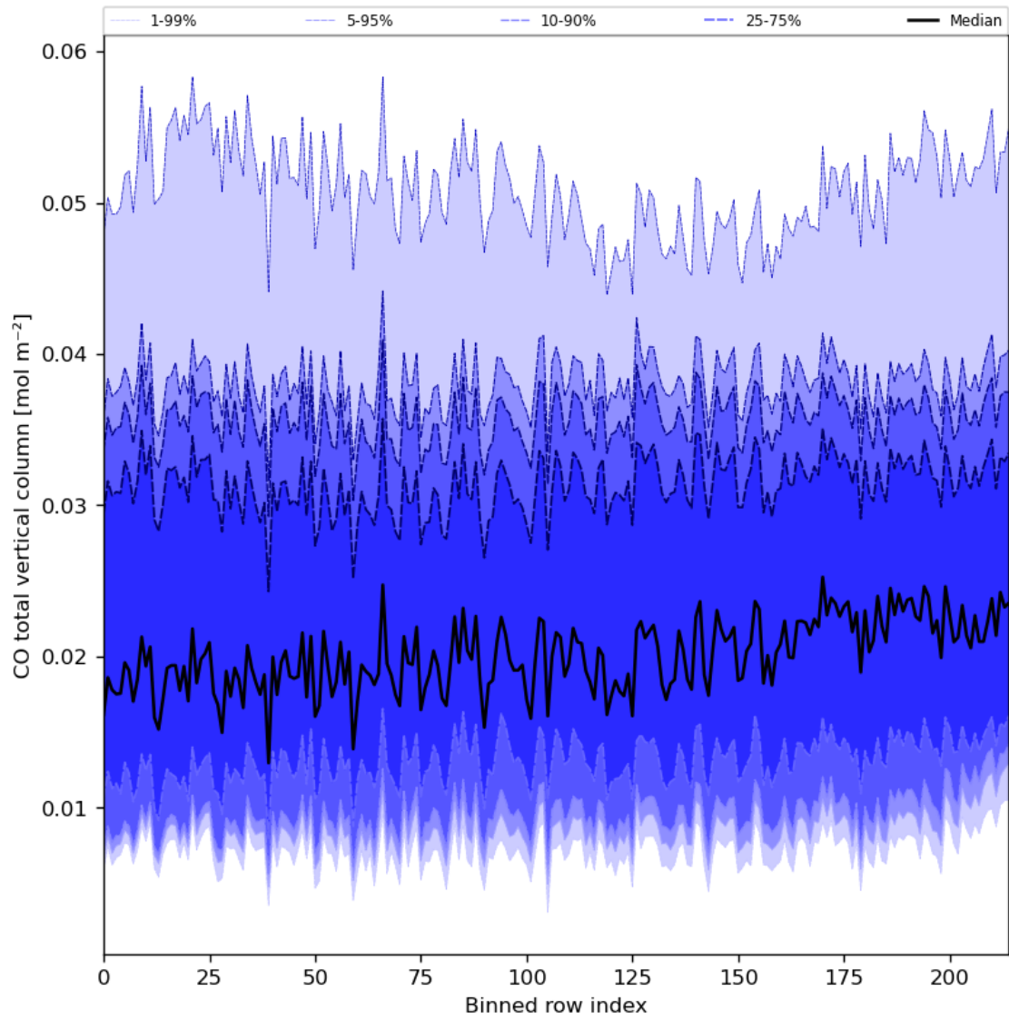
Figure 26: Along track statistics of “CO total vertical column” for 2024-01-12 to 2024-01-14
