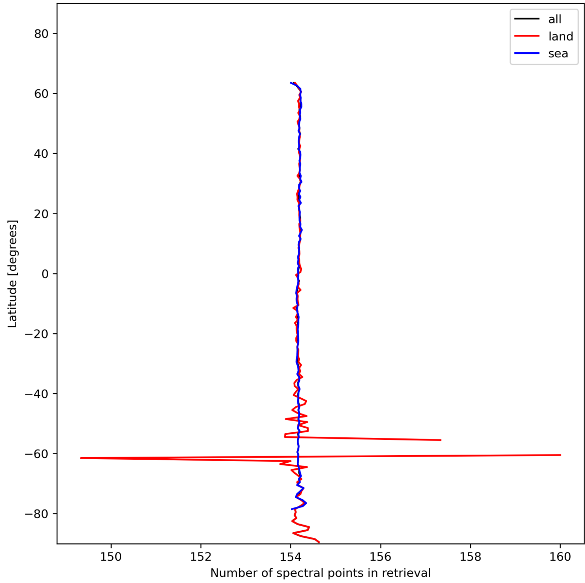
Figure 13: Zonal average of “Number of spectral points in retrieval” for 2024-01-12 to 2024-01-14.
