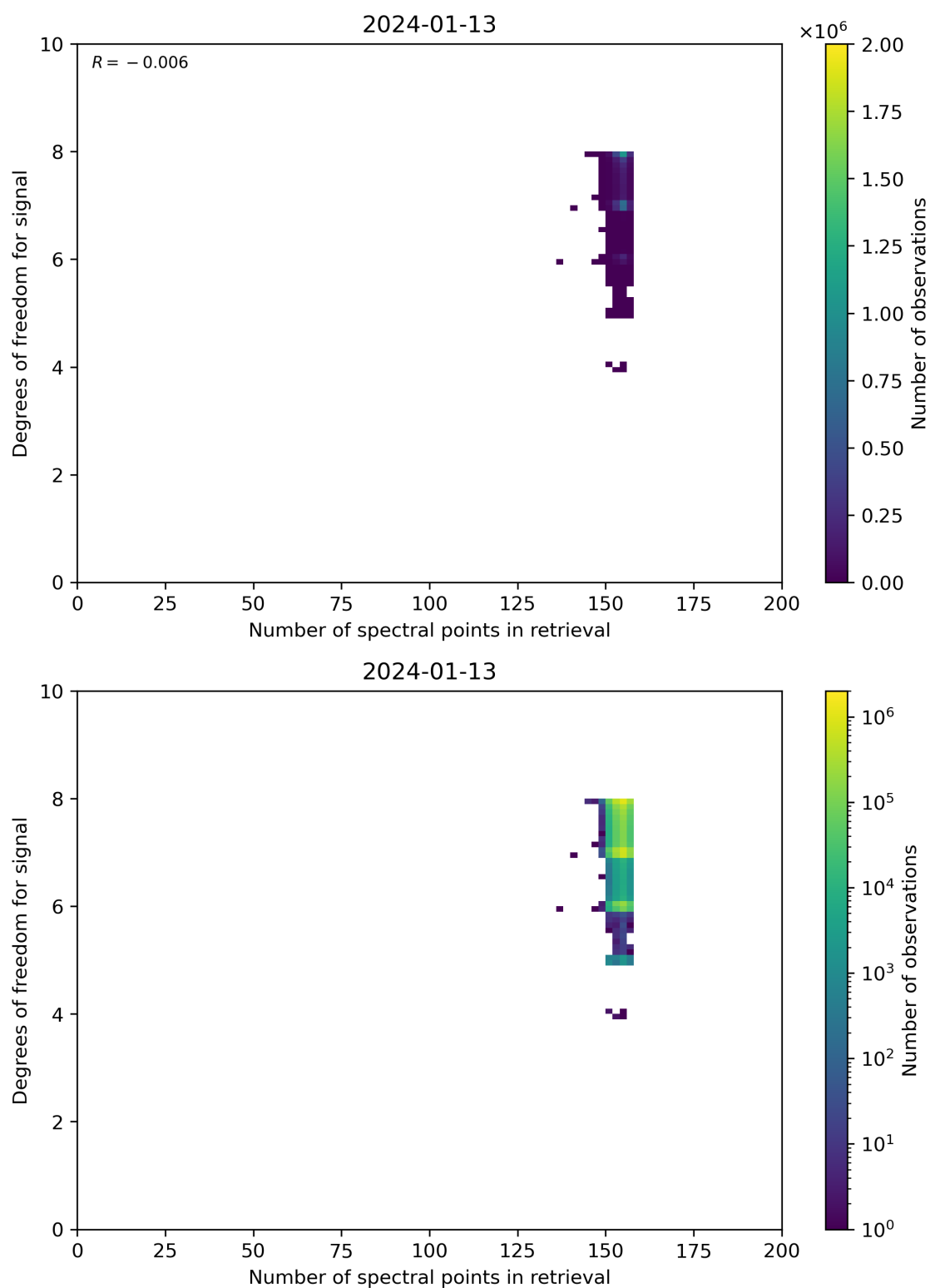
Figure 59: Scatter density plot of “Number of spectral points in retrieval” against “Degrees of freedom for signal” for 2024-01-12 to 2024-01-14.
