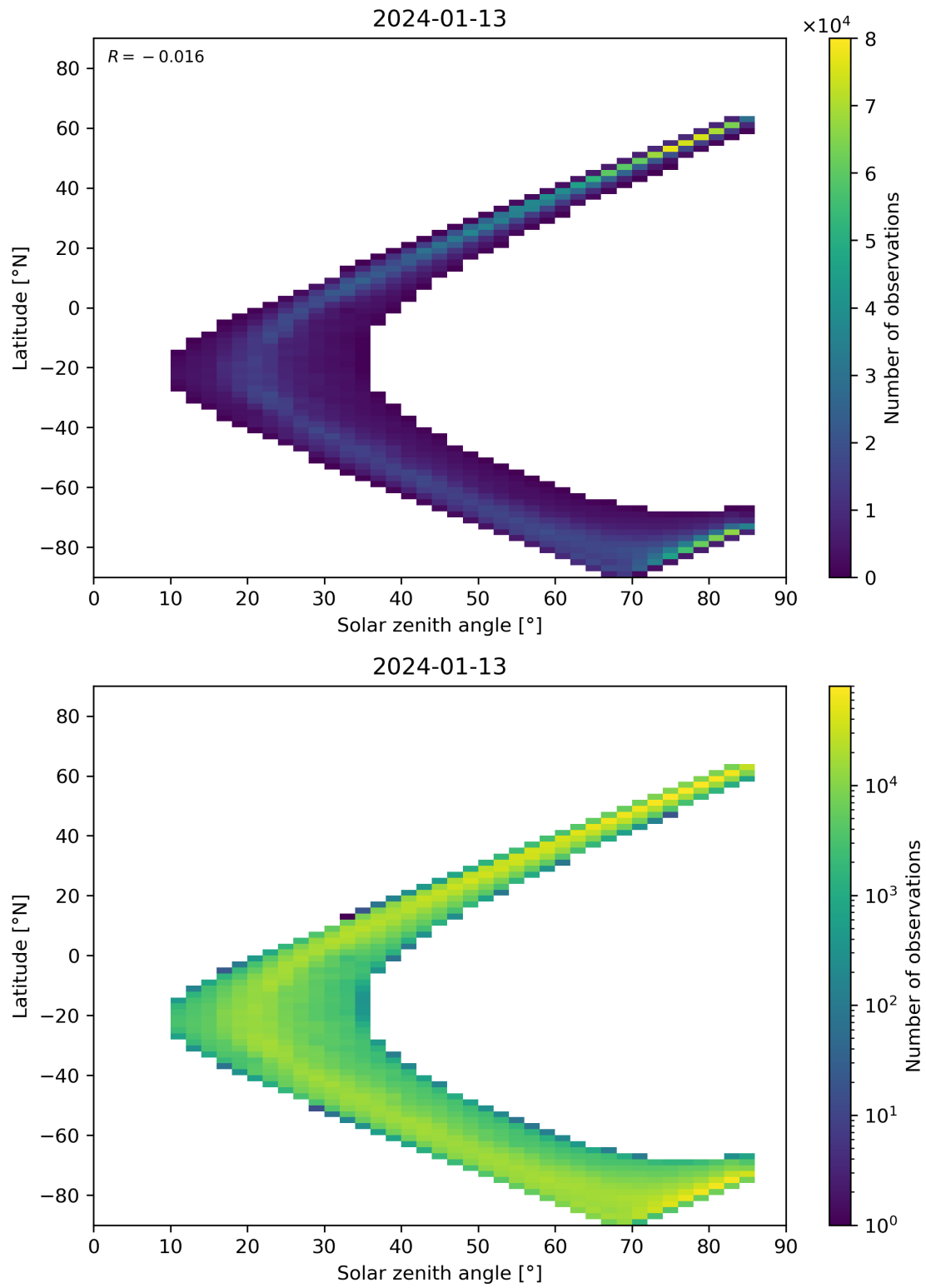
Figure 66: Scatter density plot of “Solar zenith angle” against “Latitude” for 2024-01-12 to 2024-01-14.
