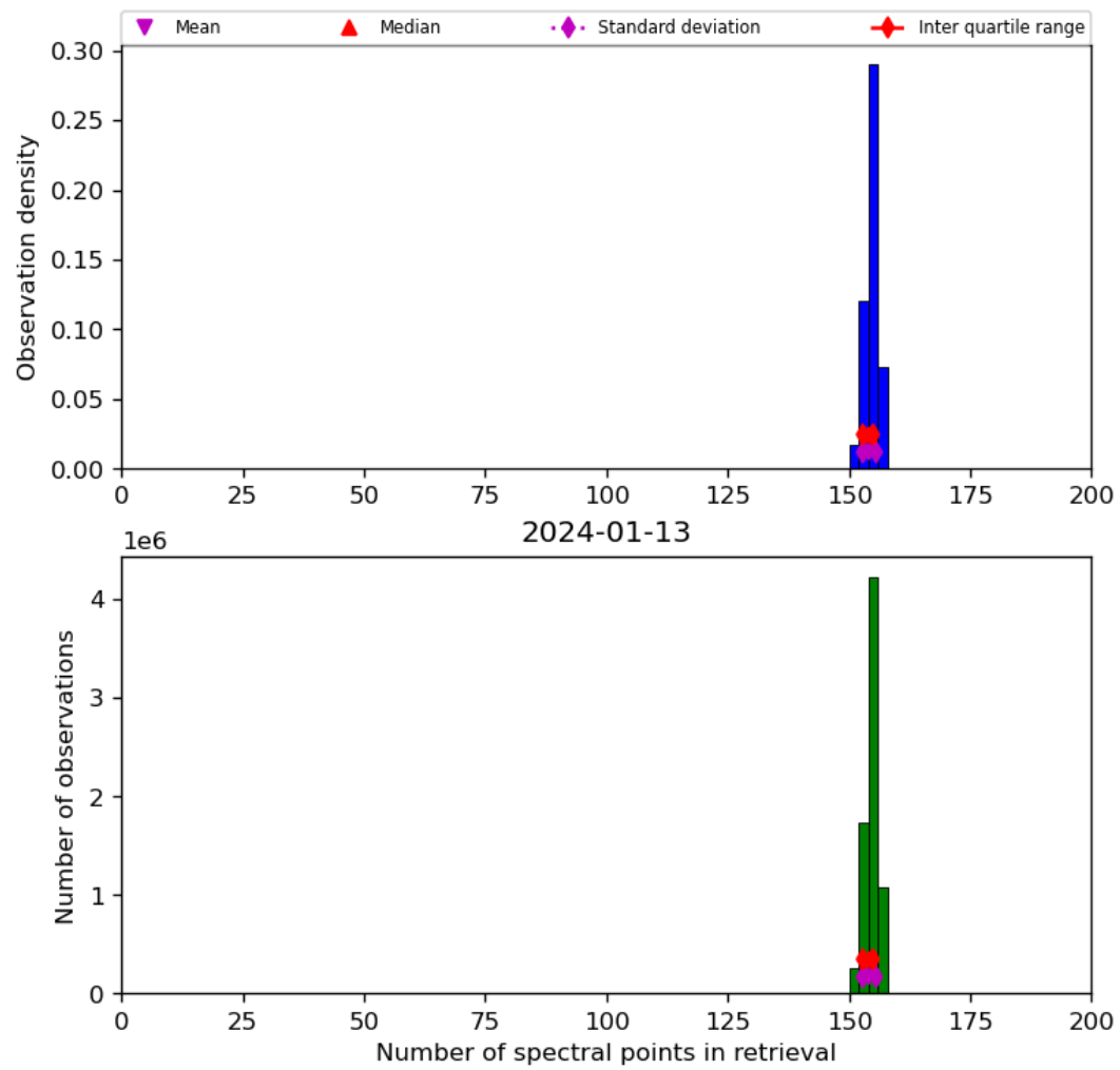
Figure 21: Histogram of “Number of spectral points in retrieval” for 2024-01-12 to 2024-01-14
