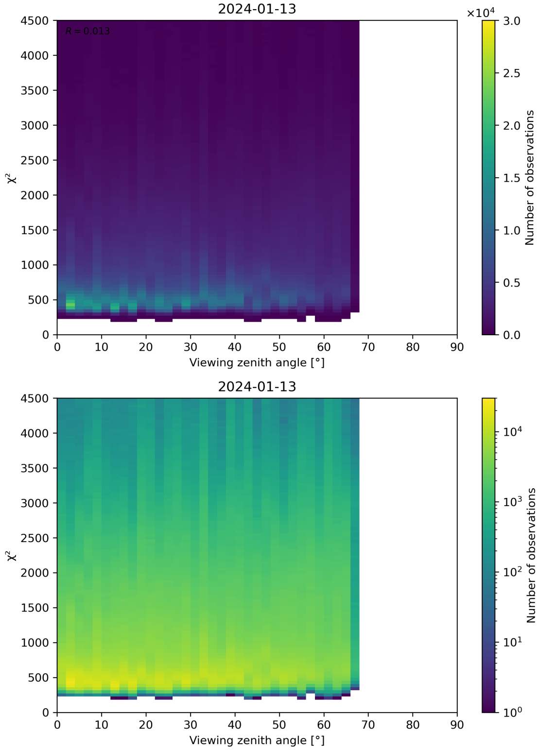
Figure 72: Scatter density plot of “Viewing zenith angle” against “ \chi^2 ” for 2024-01-12 to 2024-01-14.
