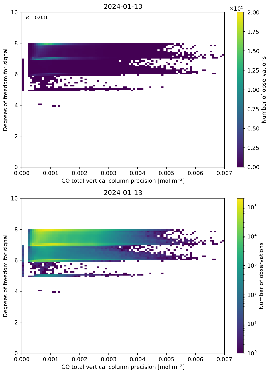
Figure 45: Scatter density plot of “CO total vertical column precision” against “Degrees of freedom for signal” for 2024-01-12 to 2024-01-14.
