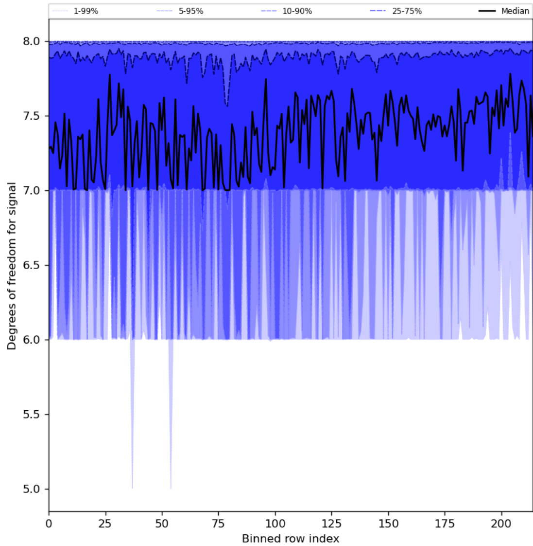
Figure 31: Along track statistics of “Degrees of freedom for signal” for 2024-01-12 to 2024-01-14
