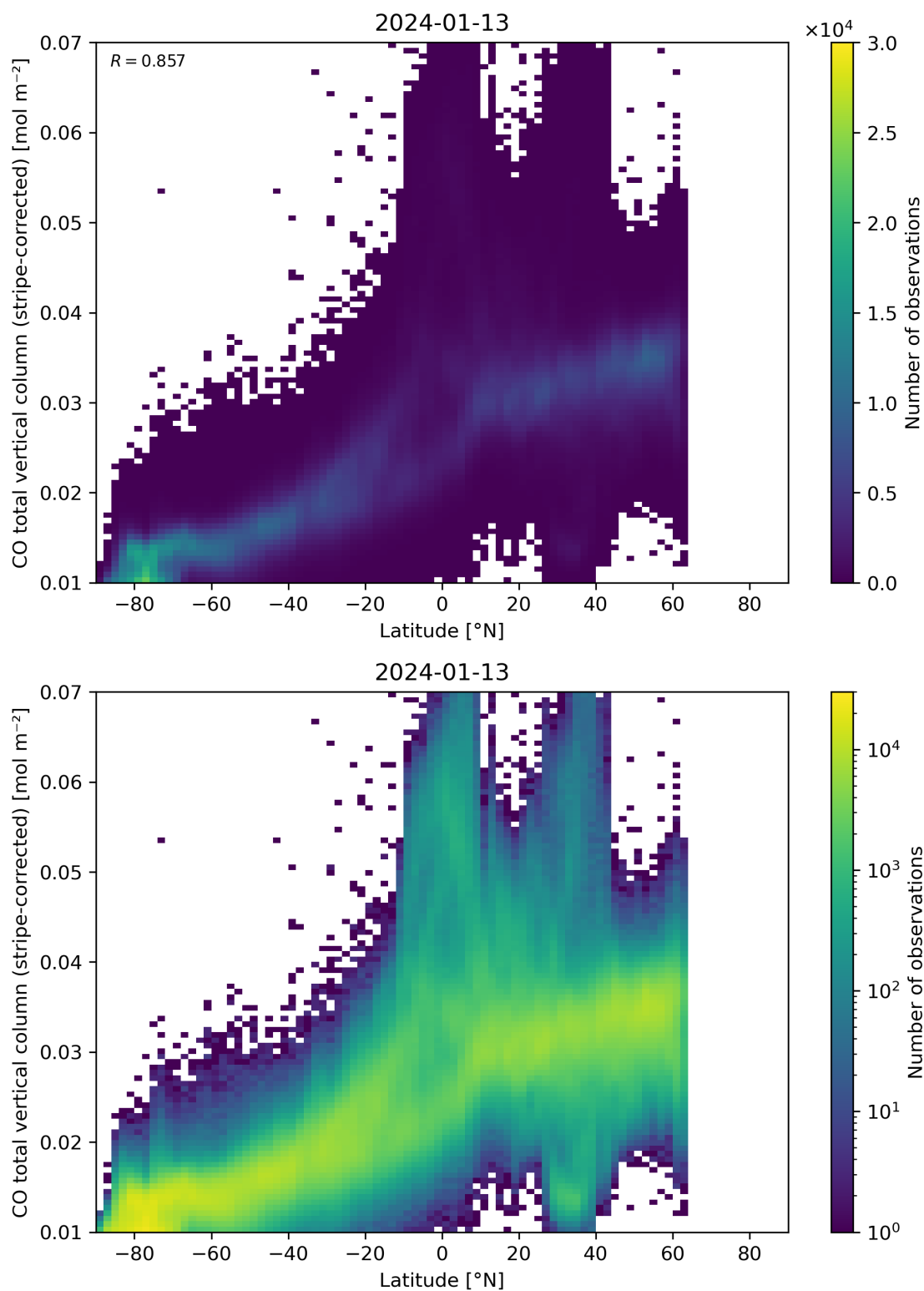
Figure 52: Scatter density plot of “Latitude” against “CO total vertical column (stripe-corrected)” for 2024-01-12 to 2024-01-14.
