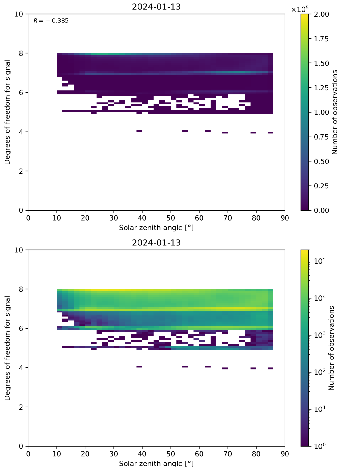
Figure 65: Scatter density plot of “Solar zenith angle” against “Degrees of freedom for signal” for 2024-01-12 to 2024-01-14.
