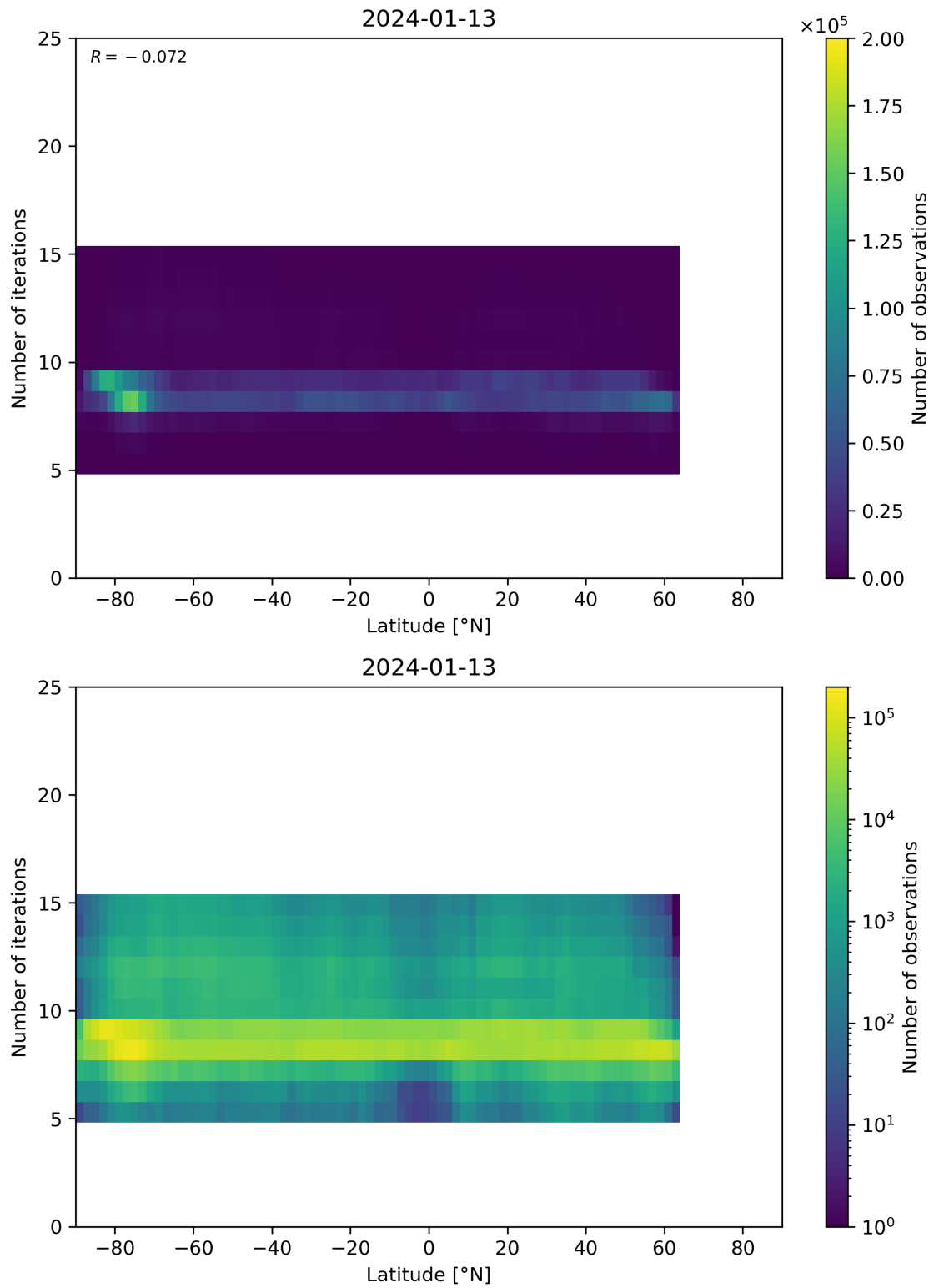
Figure 56: Scatter density plot of “Latitude” against “Number of iterations” for 2024-01-12 to 2024-01-14.
