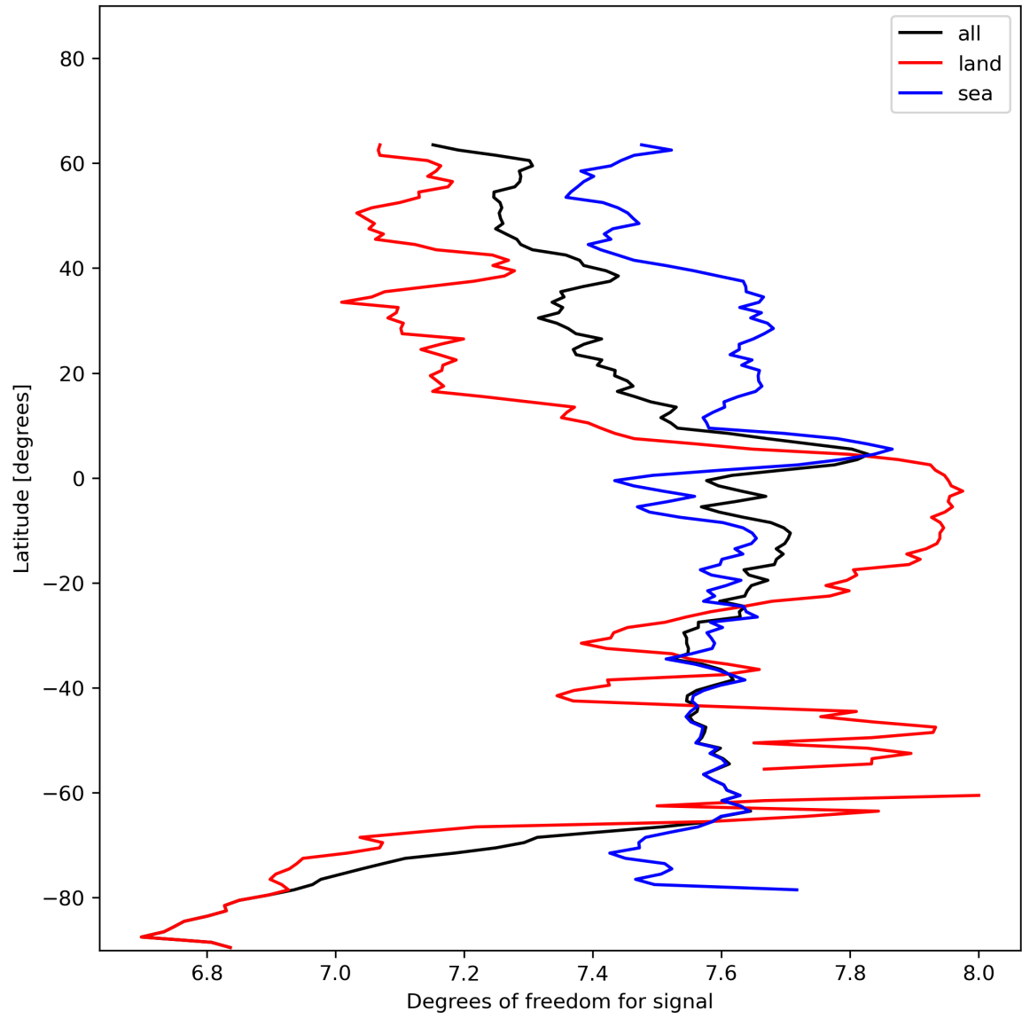
Figure 15: Zonal average of “Degrees of freedom for signal” for 2024-01-12 to 2024-01-14.
