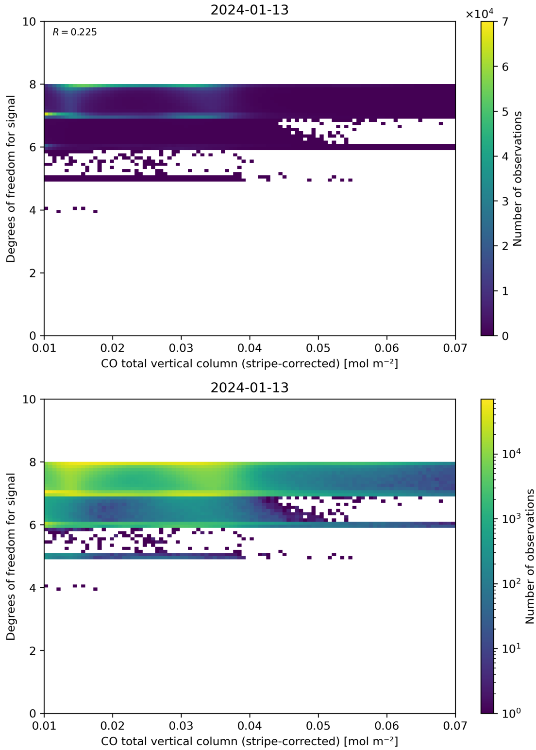
Figure 38: Scatter density plot of “CO total vertical column (stripe-corrected)” against “Degrees of freedom for signal” for 2024-01-12 to 2024-01-14.
