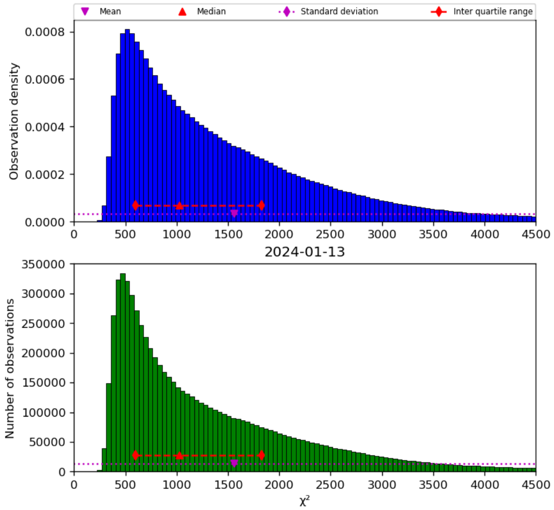
Figure 22: Histogram of “ \chi^2 ” for 2024-01-12 to 2024-01-14
