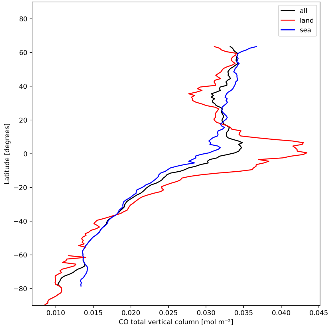
Figure 10: Zonal average of “CO total vertical column” for 2024-01-12 to 2024-01-14.
