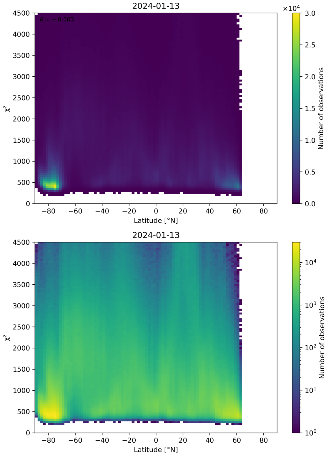
Figure 54: Scatter density plot of “Latitude” against “ \chi^2 ” for 2024-01-12 to 2024-01-14.
