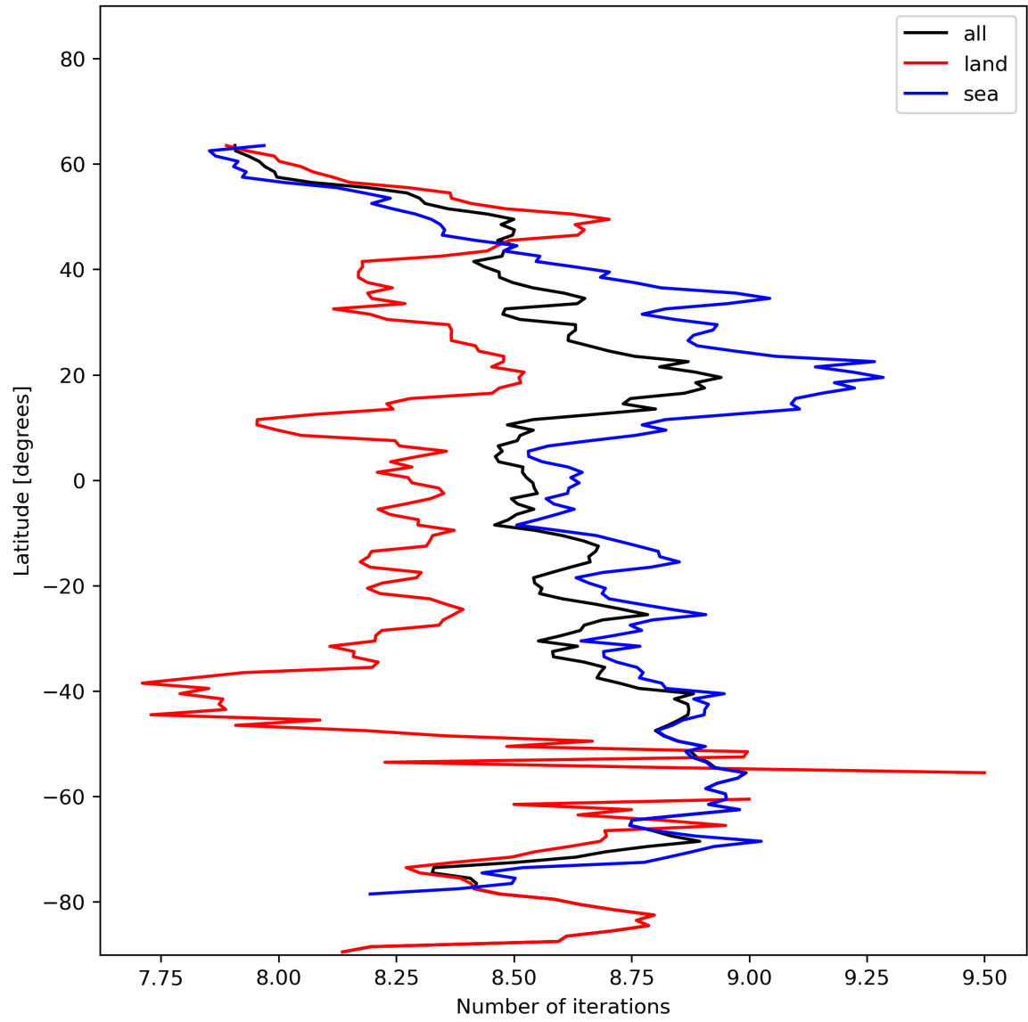
Figure 16: Zonal average of “Number of iterations” for 2024-01-12 to 2024-01-14.
