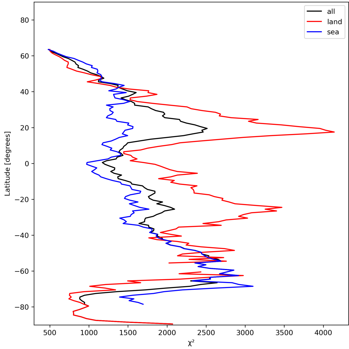
Figure 14: Zonal average of “ \chi^2 ” for 2024-01-12 to 2024-01-14.
