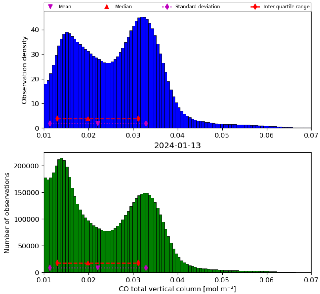
Figure 18: Histogram of “CO total vertical column” for 2024-01-12 to 2024-01-14
