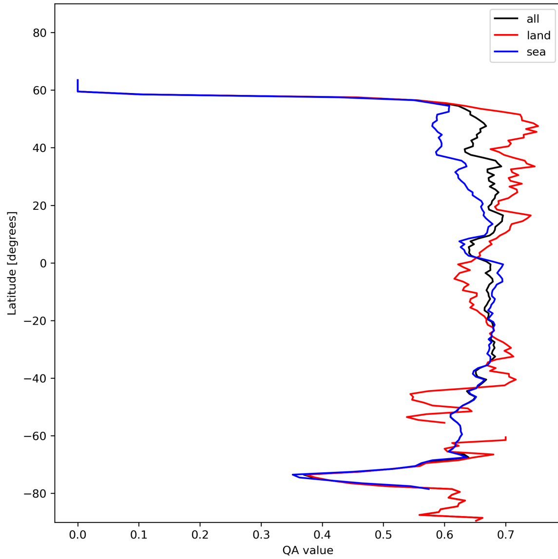
Figure 9: Zonal average of “QA value” for 2024-01-12 to 2024-01-14.
