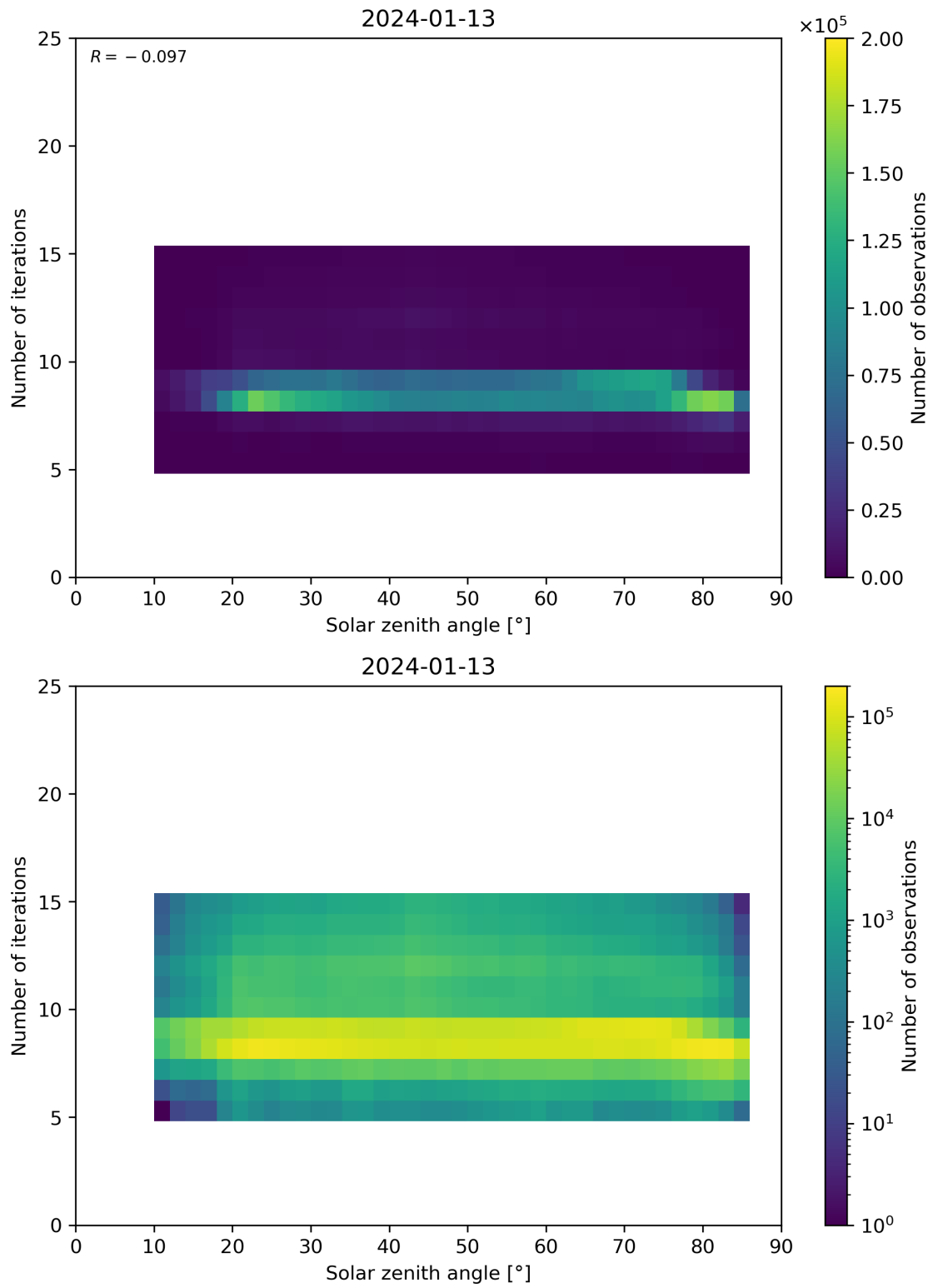
Figure 67: Scatter density plot of “Solar zenith angle” against “Number of iterations” for 2024-01-12 to 2024-01-14.
