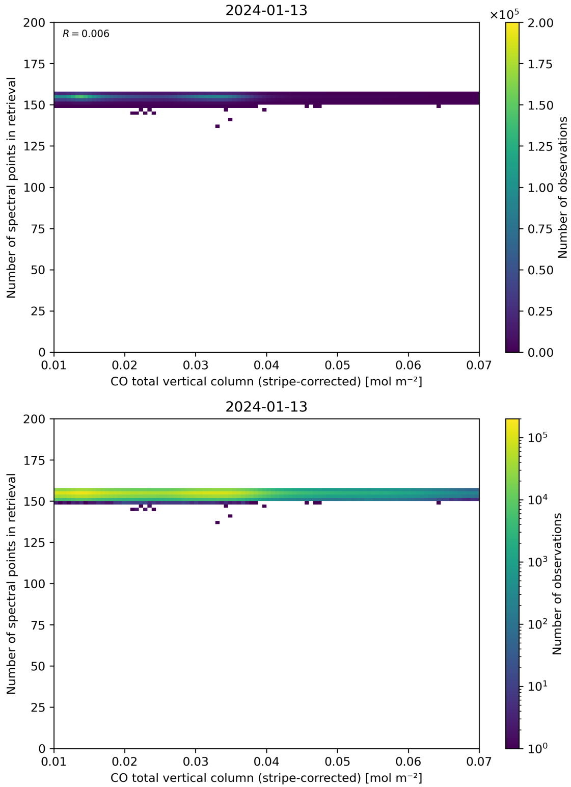
Figure 40: Scatter density plot of “CO total vertical column (stripe-corrected)” against “Number of spectral points in retrieval” for 2024-01-12 to 2024-01-14.
