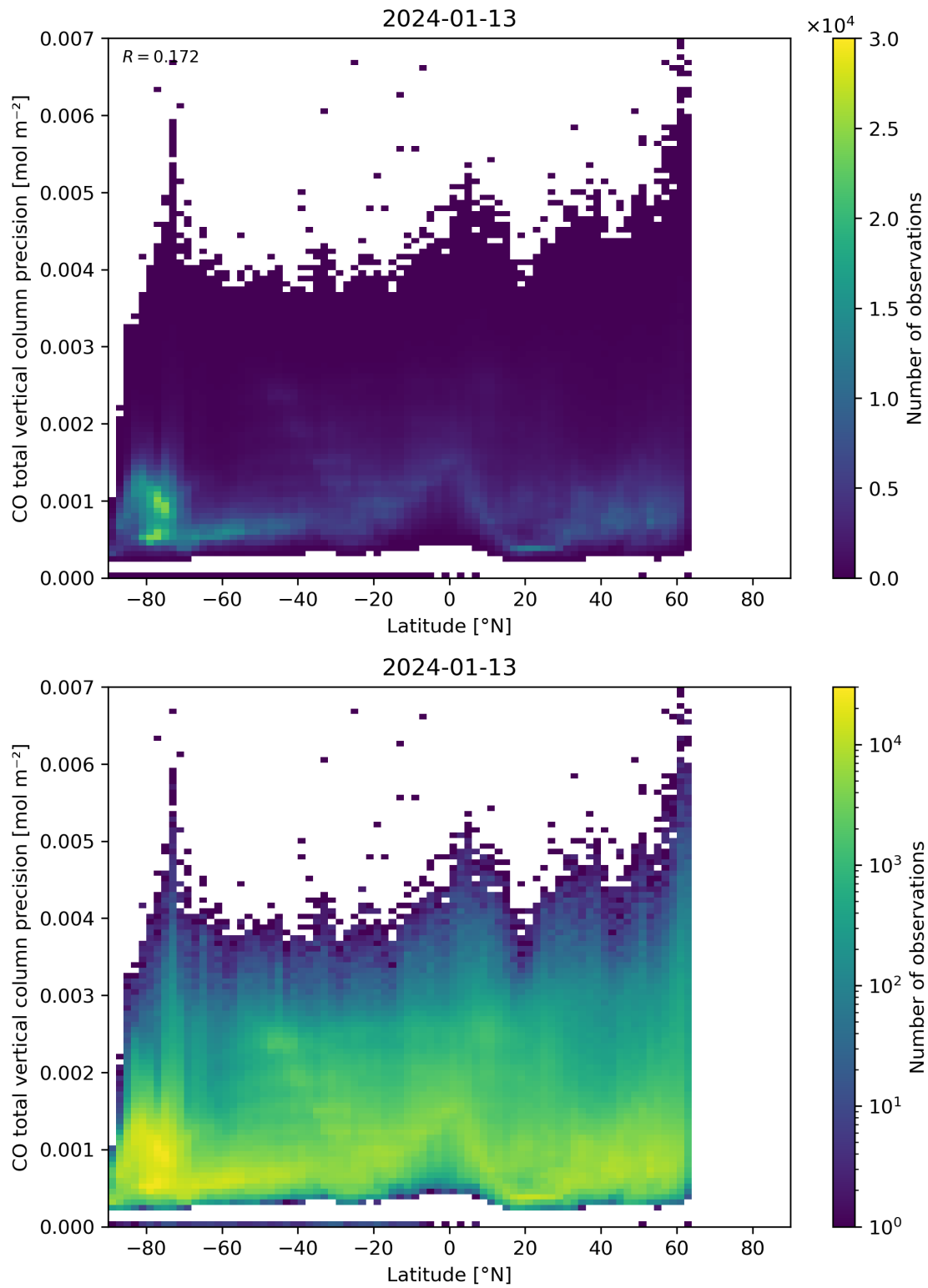
Figure 53: Scatter density plot of “Latitude” against “CO total vertical column precision” for 2024-01-12 to 2024-01-14.
