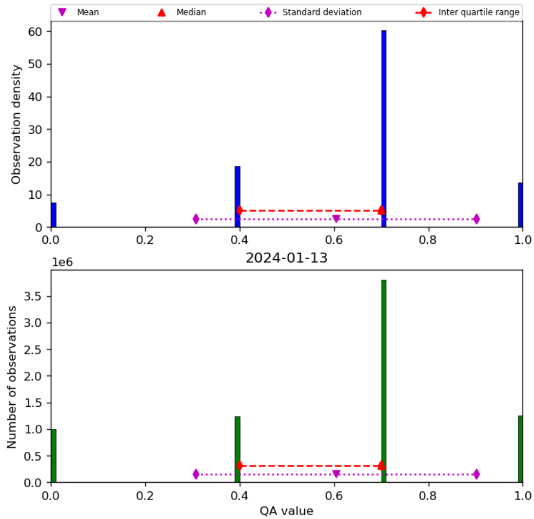
Figure 17: Histogram of “QA value” for 2024-01-12 to 2024-01-14
