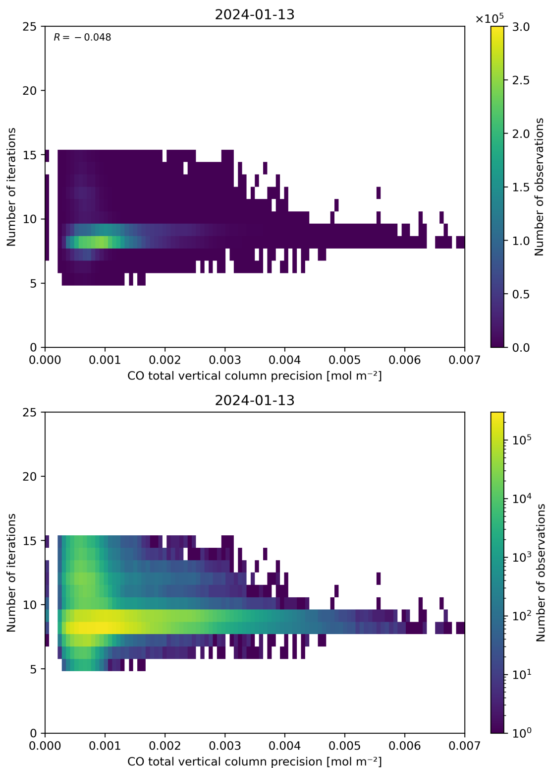
Figure 46: Scatter density plot of “CO total vertical column precision” against “Number of iterations” for 2024-01-12 to 2024-01-14.
