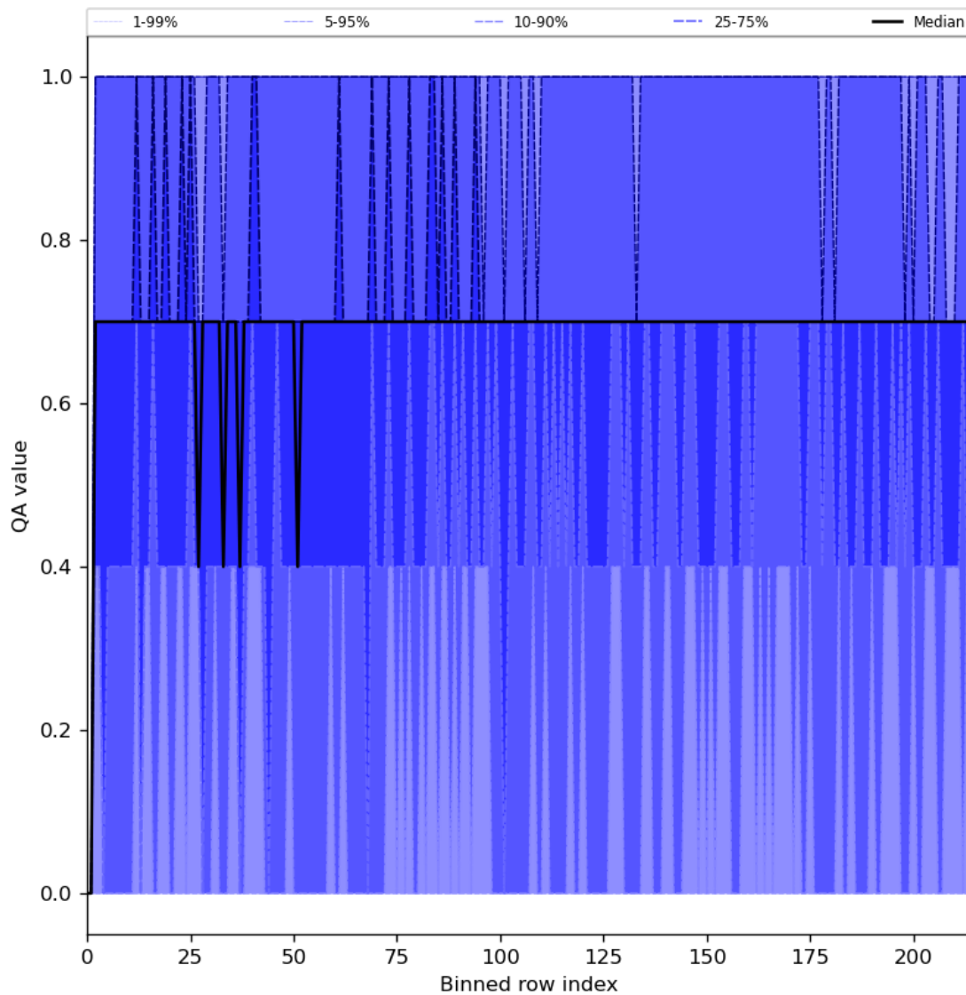
Figure 25: Along track statistics of “QA value” for 2024-01-12 to 2024-01-14
