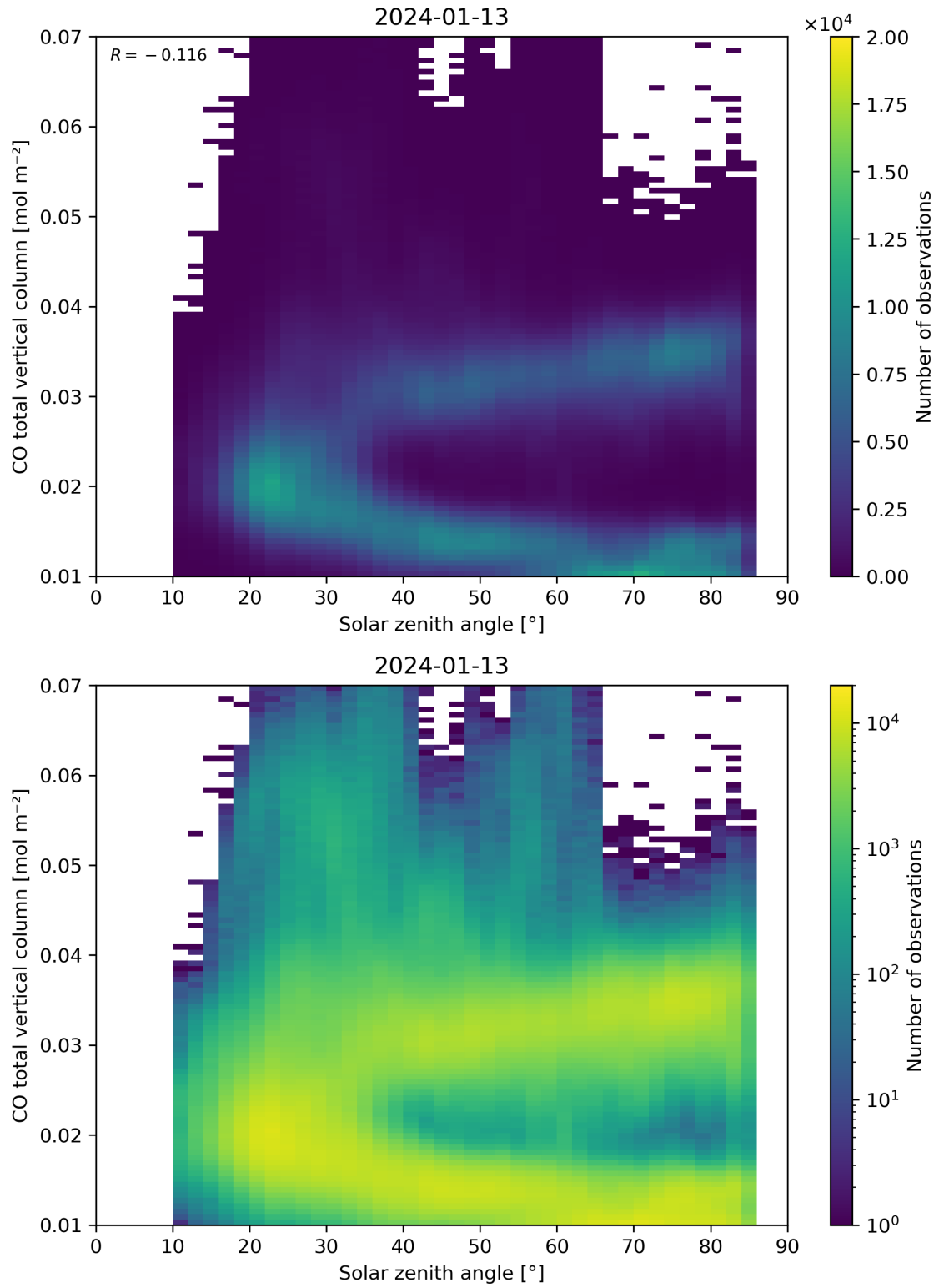
Figure 61: Scatter density plot of “Solar zenith angle” against “CO total vertical column” for 2024-01-12 to 2024-01-14.
