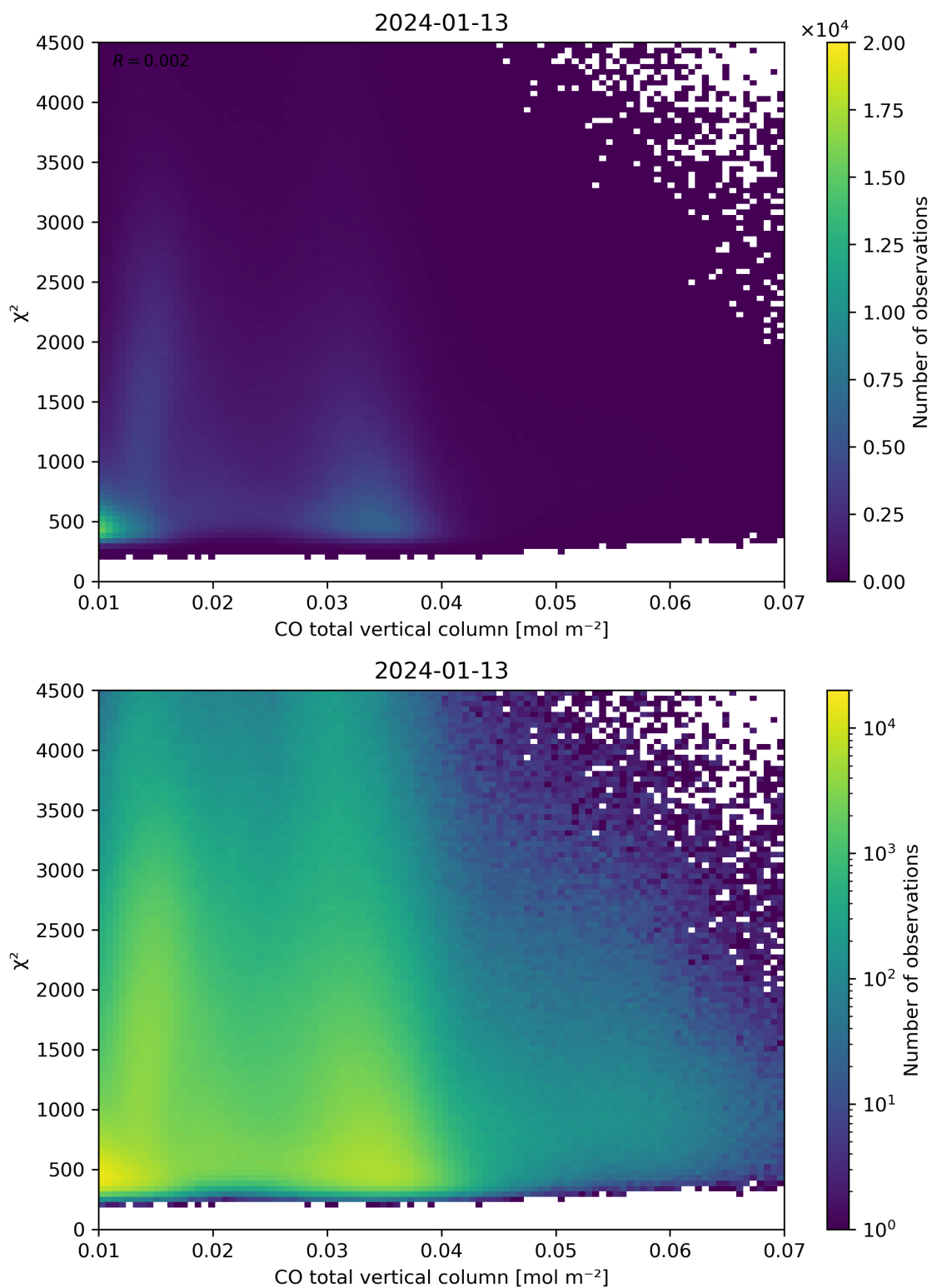
Figure 35: Scatter density plot of “CO total vertical column” against “ \chi^2 ” for 2024-01-12 to 2024-01-14.
