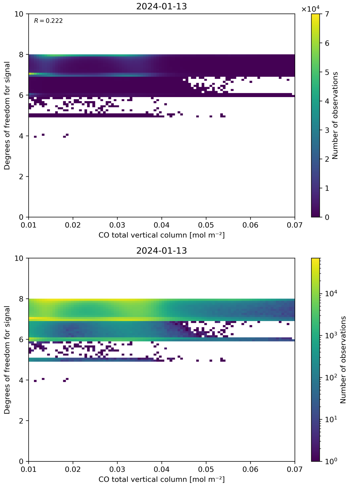
Figure 41: Scatter density plot of “CO total vertical column” against “Degrees of freedom for signal” for 2024-01-12 to 2024-01-14.
