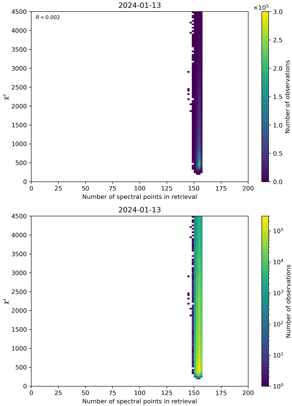
Figure 58: Scatter density plot of “Number of spectral points in retrieval” against “ \chi^2 ” for 2024-01-12 to 2024-01-14.
