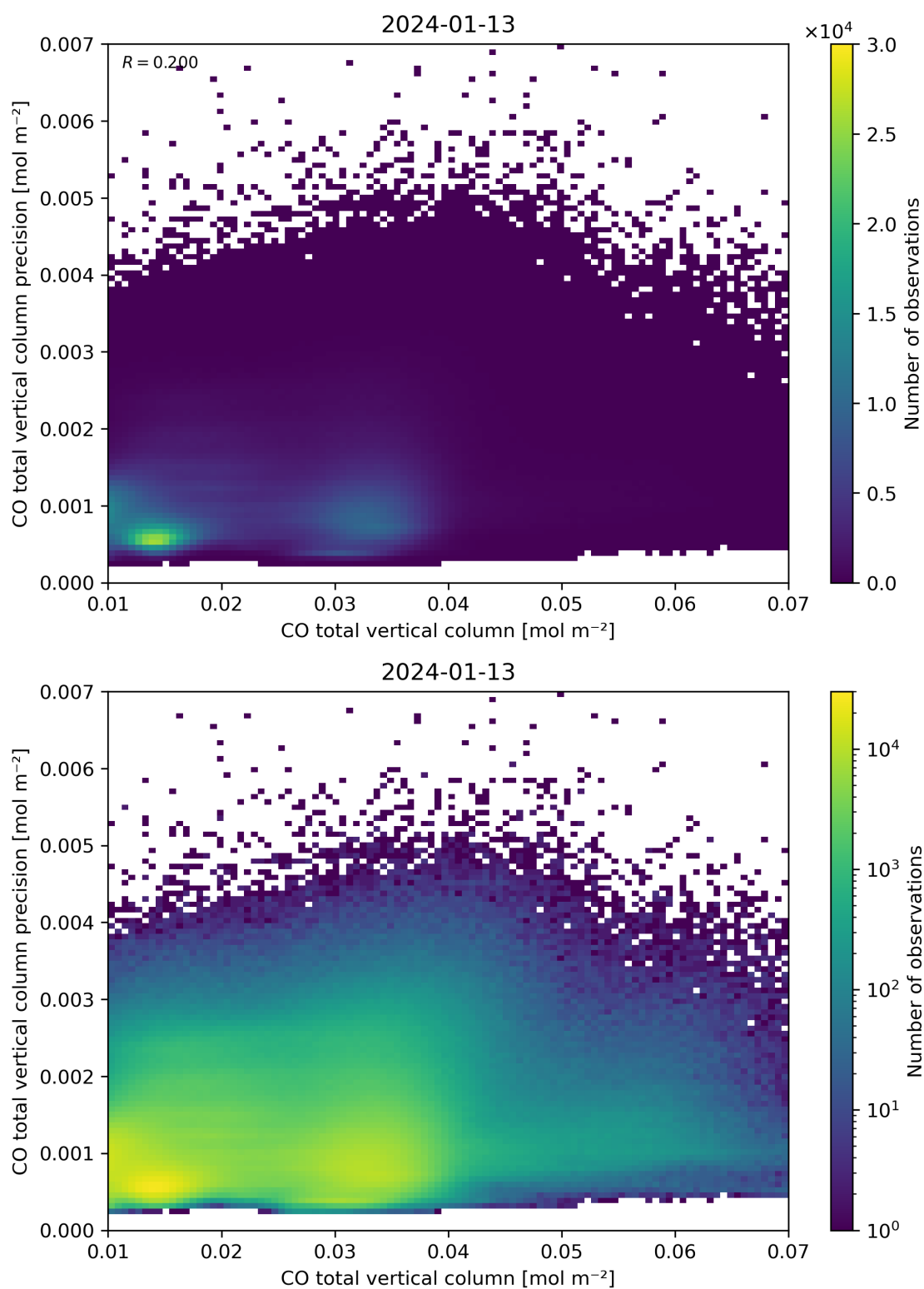
Figure 34: Scatter density plot of “CO total vertical column” against “CO total vertical column precision” for 2024-01-12 to 2024-01-14.
