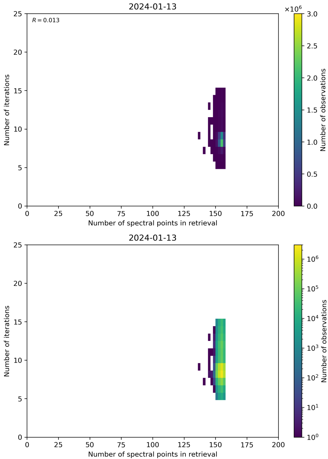
Figure 60: Scatter density plot of “Number of spectral points in retrieval” against “Number of iterations” for 2024-01-12 to 2024-01-14.
