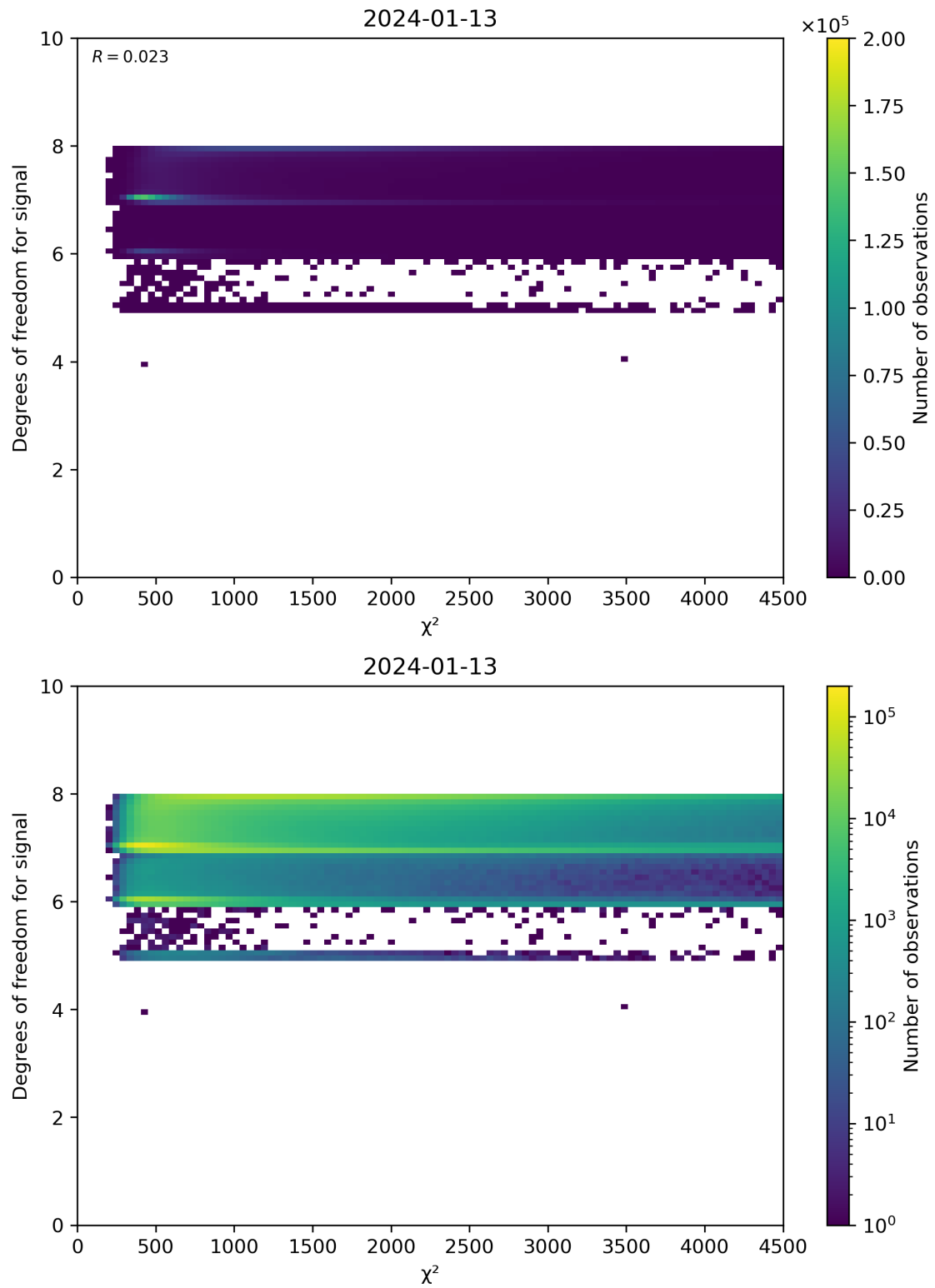
Figure 48: Scatter density plot of “ \chi^2 ” against “Degrees of freedom for signal” for 2024-01-12 to 2024-01-14.
