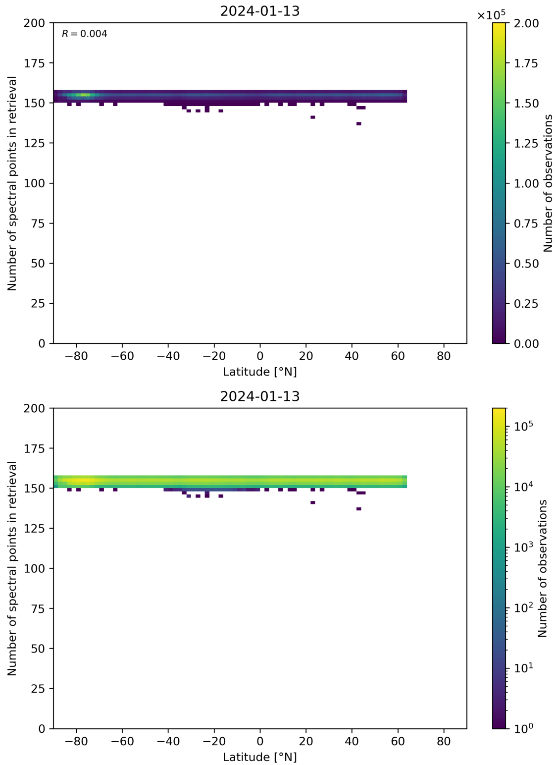
Figure 57: Scatter density plot of “Latitude” against “Number of spectral points in retrieval” for 2024-01-12 to 2024-01-14.
