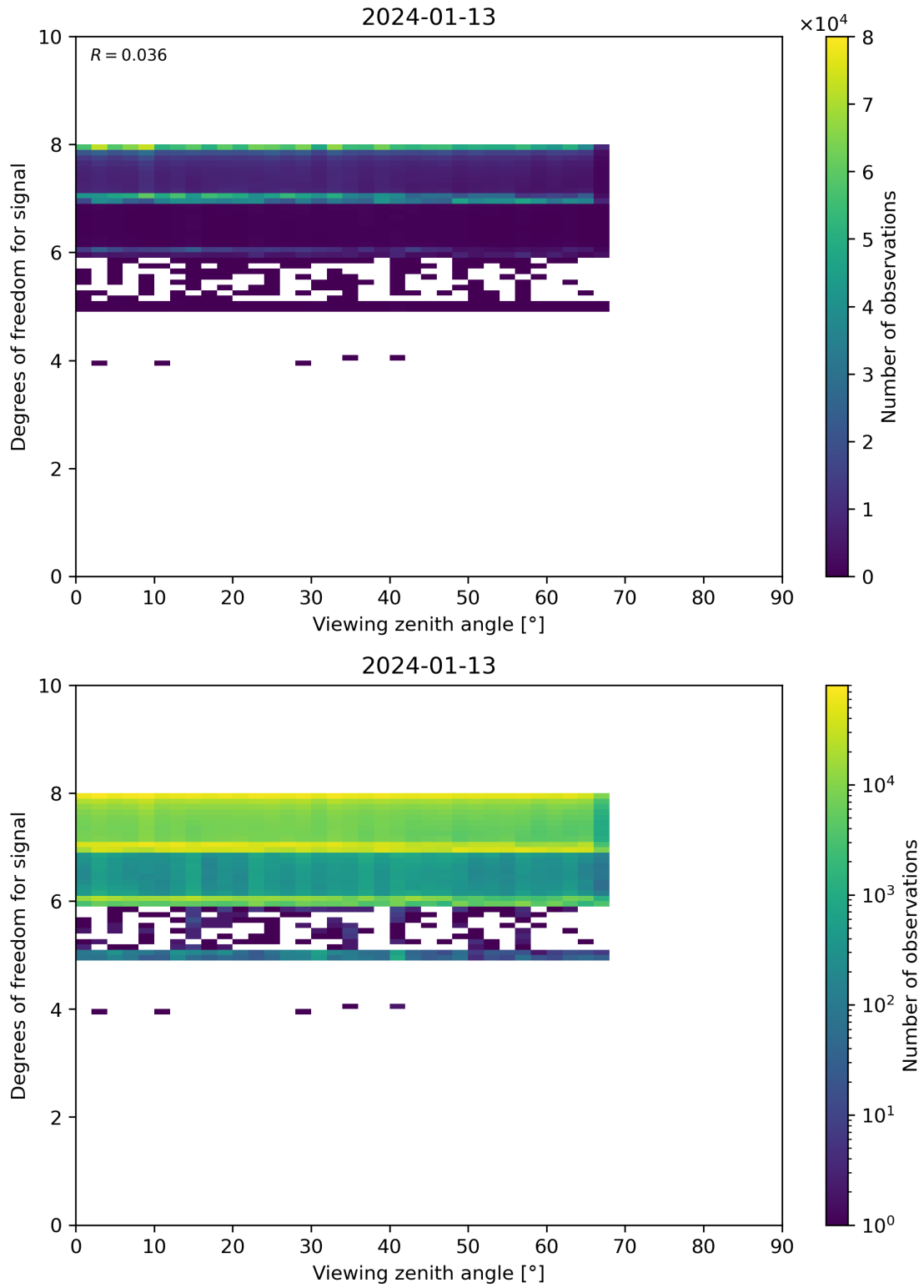
Figure 73: Scatter density plot of “Viewing zenith angle” against “Degrees of freedom for signal” for 2024-01-12 to 2024-01-14.
