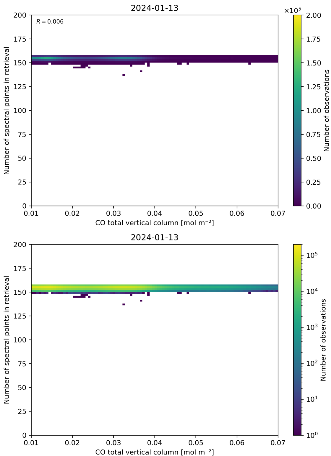
Figure 43: Scatter density plot of “CO total vertical column” against “Number of spectral points in retrieval” for 2024-01-12 to 2024-01-14.
