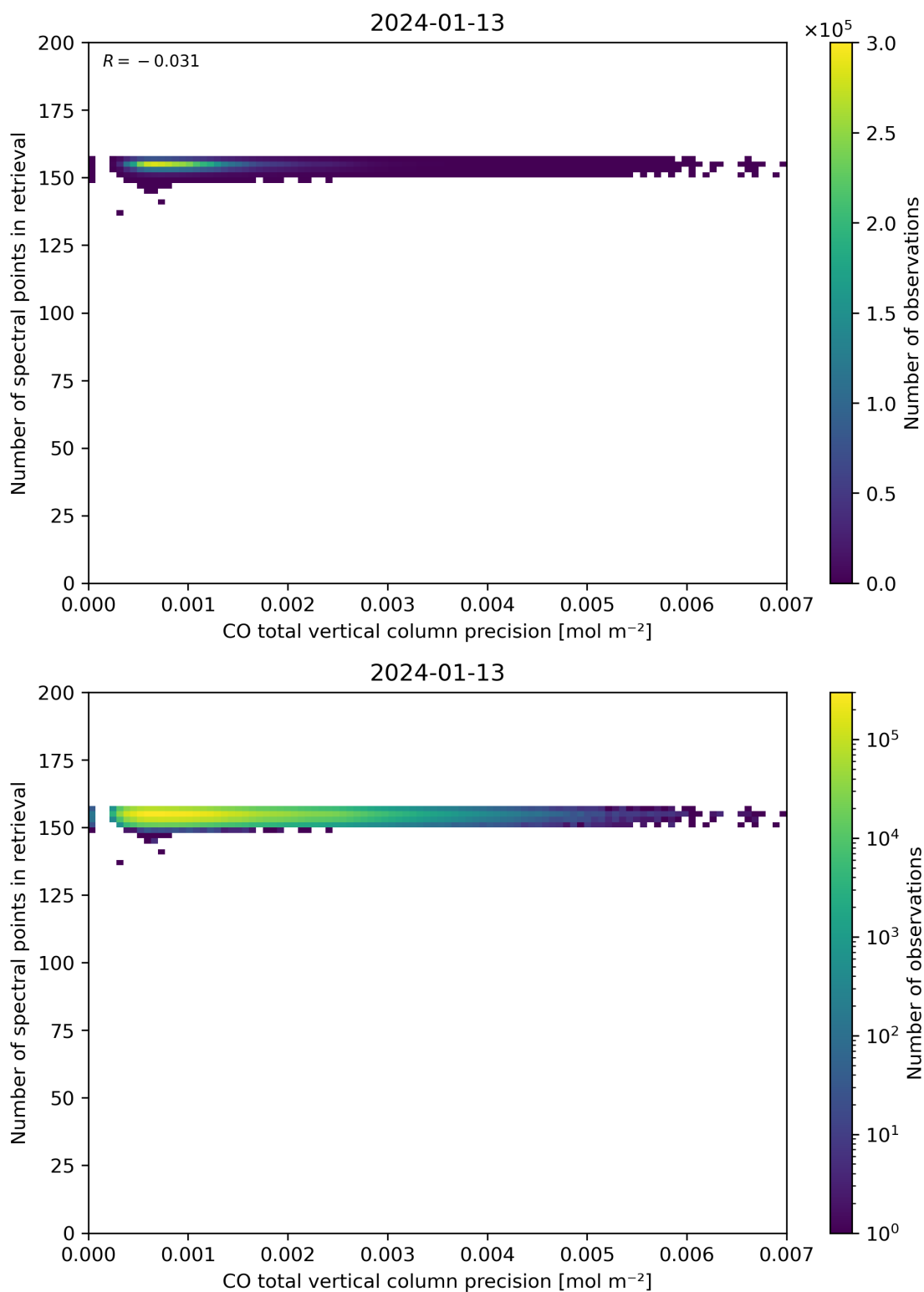
Figure 47: Scatter density plot of “CO total vertical column precision” against “Number of spectral points in retrieval” for 2024-01-12 to 2024-01-14.
