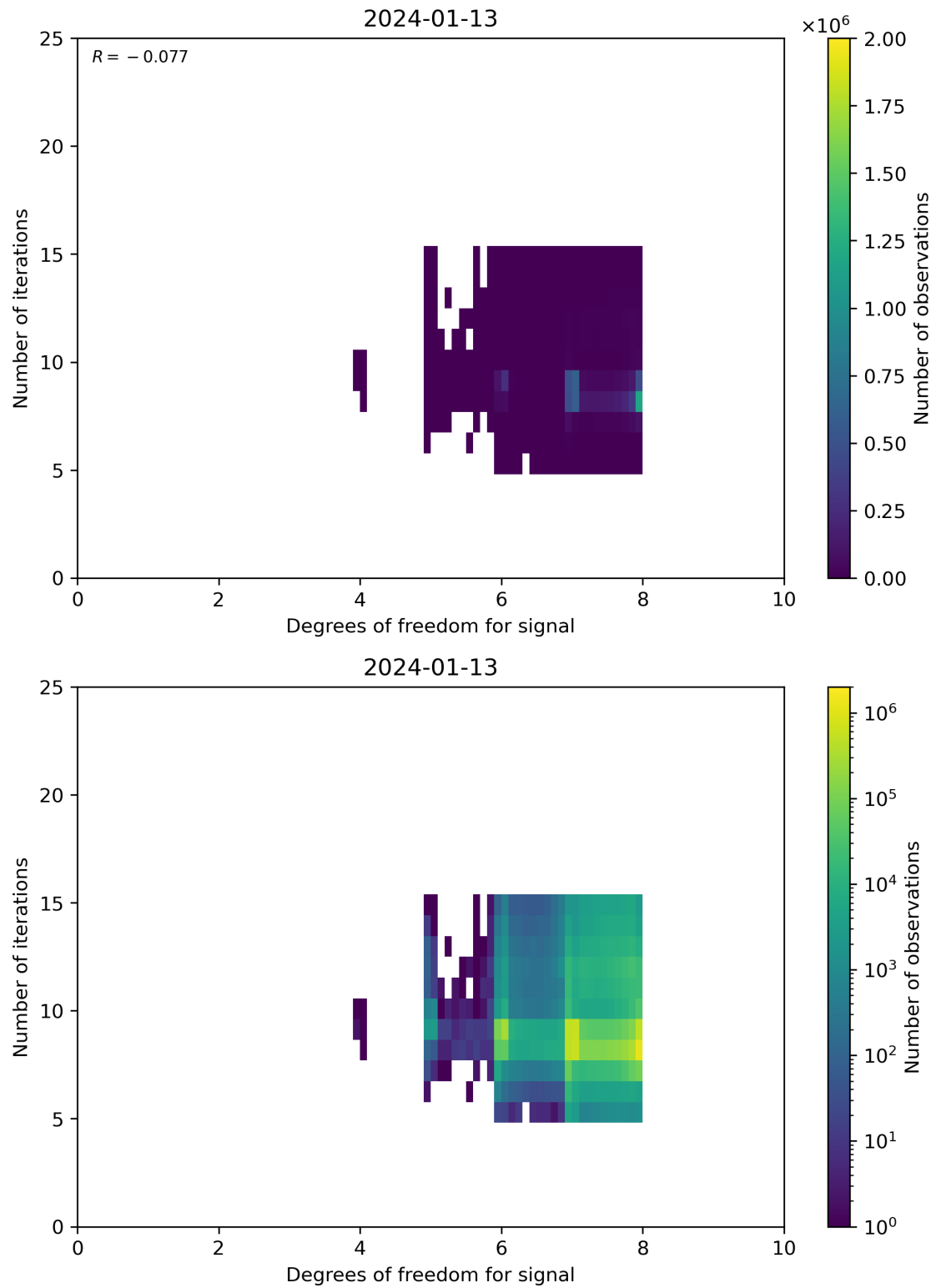
Figure 50: Scatter density plot of “Degrees of freedom for signal” against “Number of iterations” for 2024-01-12 to 2024-01-14.
