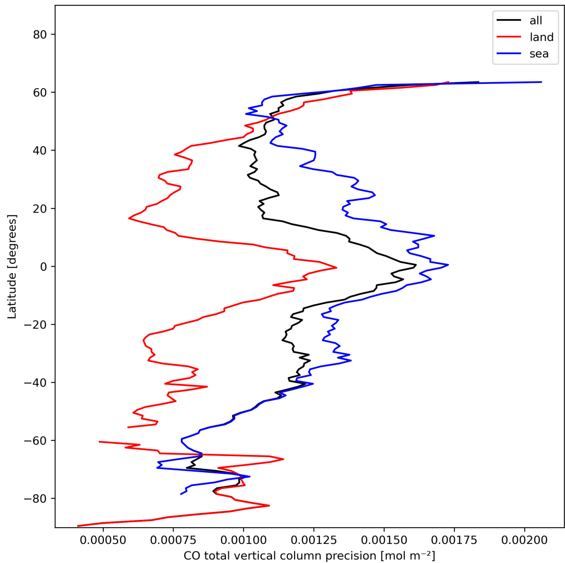
Figure 12: Zonal average of “CO total vertical column precision” for 2024-01-12 to 2024-01-14.
