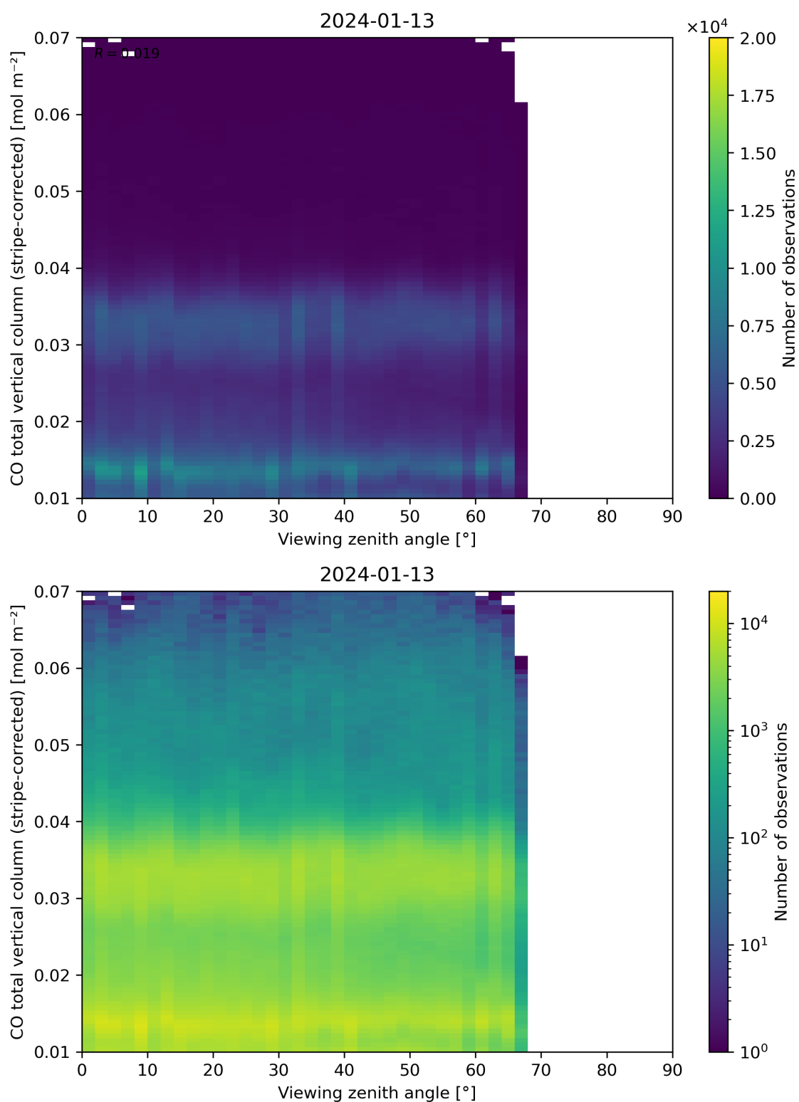
Figure 70: Scatter density plot of “Viewing zenith angle” against “CO total vertical column (stripe-corrected)” for 2024-01-12 to 2024-01-14.
