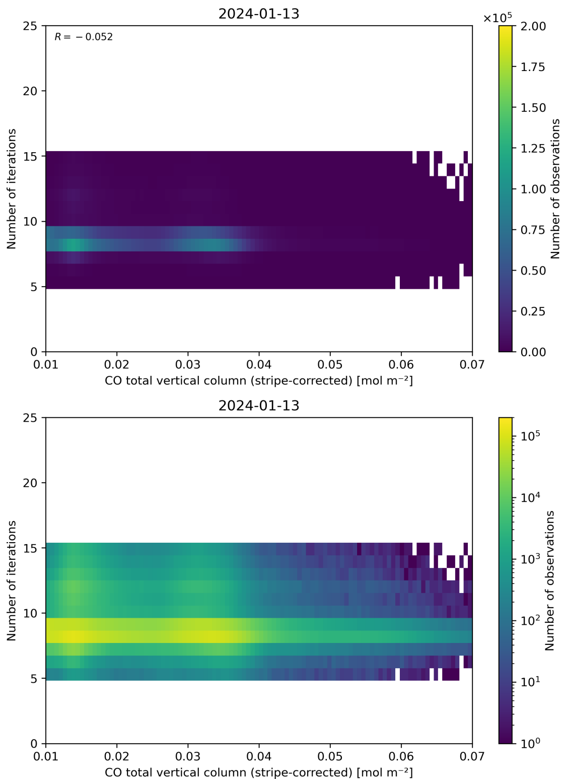
Figure 39: Scatter density plot of “CO total vertical column (stripe-corrected)” against “Number of iterations” for 2024-01-12 to 2024-01-14.
