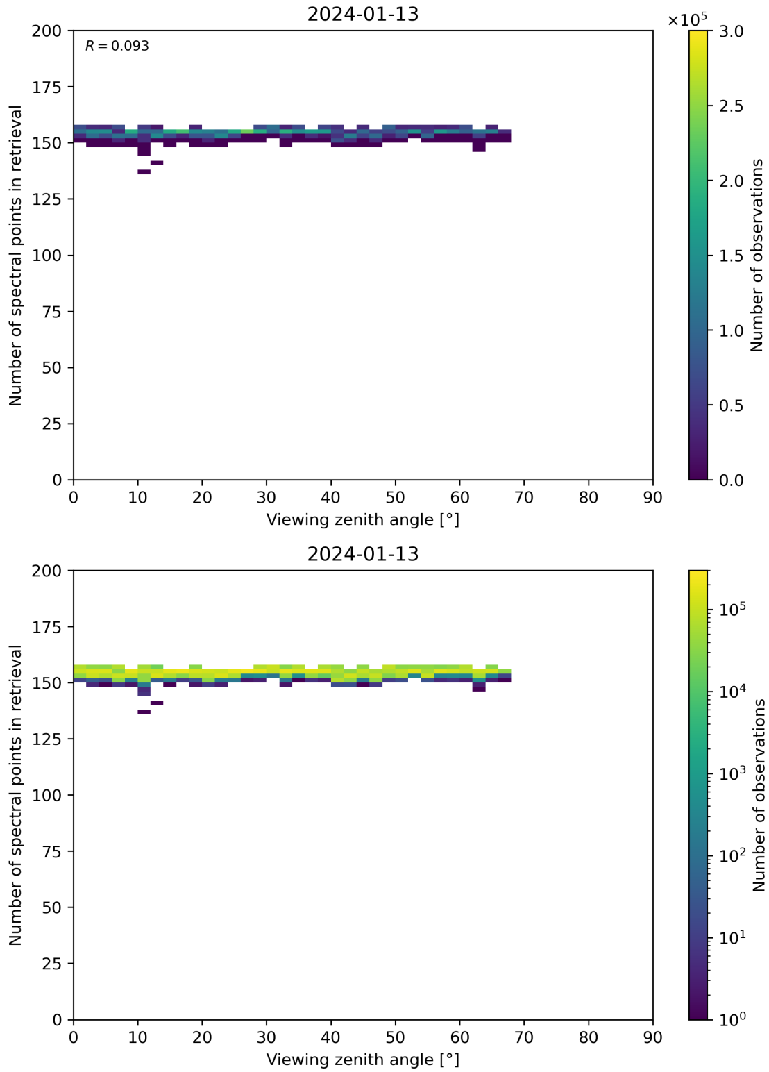
Figure 76: Scatter density plot of “Viewing zenith angle” against “Number of spectral points in retrieval” for 2024-01-12 to 2024-01-14.
