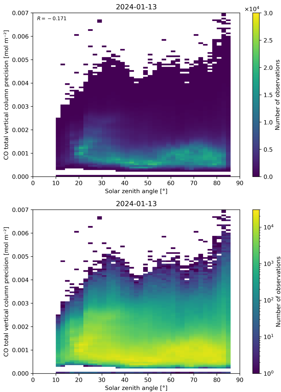
Figure 63: Scatter density plot of “Solar zenith angle” against “CO total vertical column precision” for 2024-01-12 to 2024-01-14.
