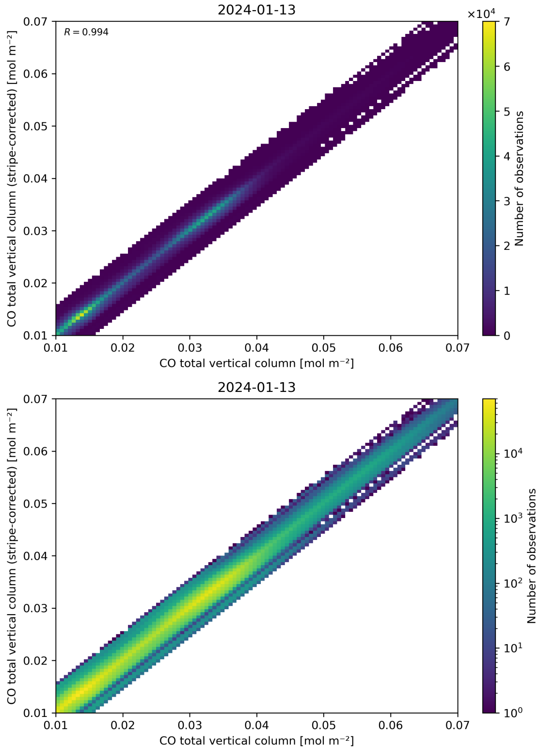
Figure 33: Scatter density plot of “CO total vertical column” against “CO total vertical column (stripe-corrected)” for 2024-01-12 to 2024-01-14.
