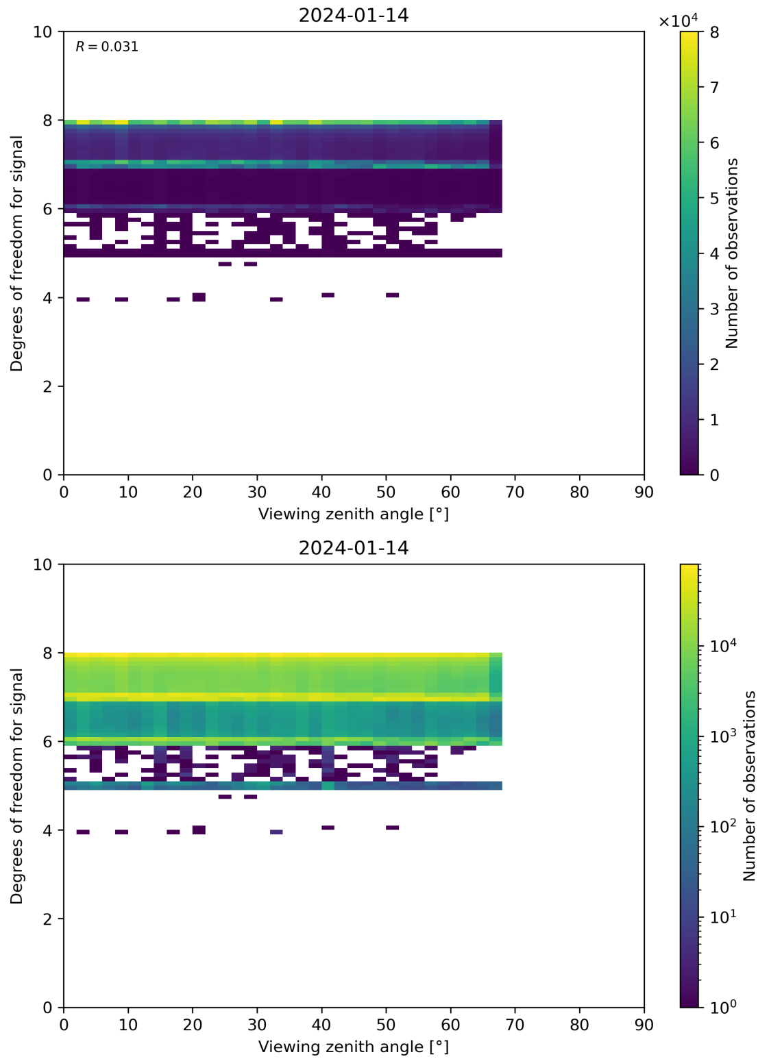
Figure 73: Scatter density plot of “Viewing zenith angle” against “Degrees of freedom for signal” for 2024-01-13 to 2024-01-15.
