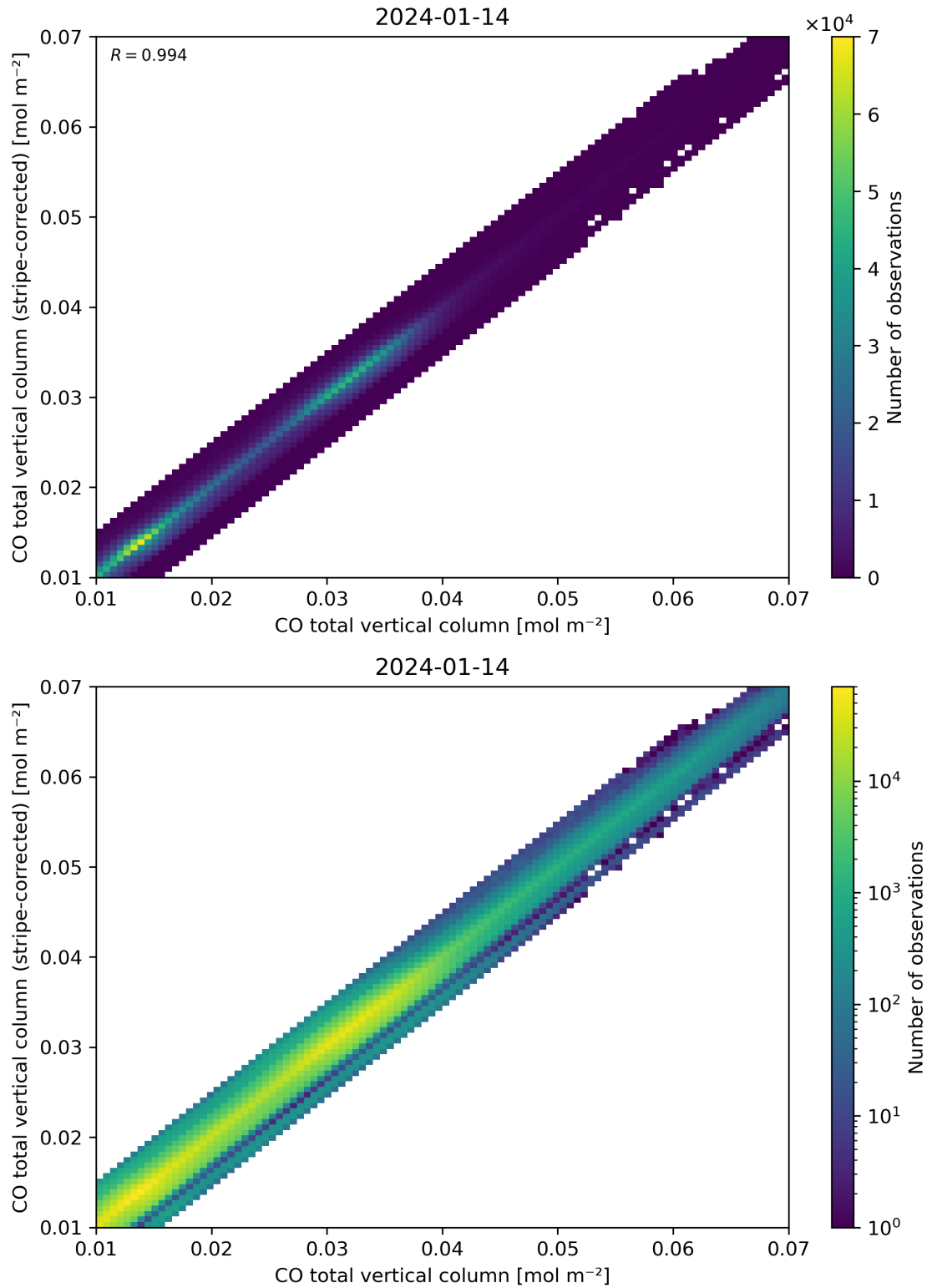
Figure 33: Scatter density plot of “CO total vertical column” against “CO total vertical column (stripe-corrected)” for 2024-01-13 to 2024-01-15.
