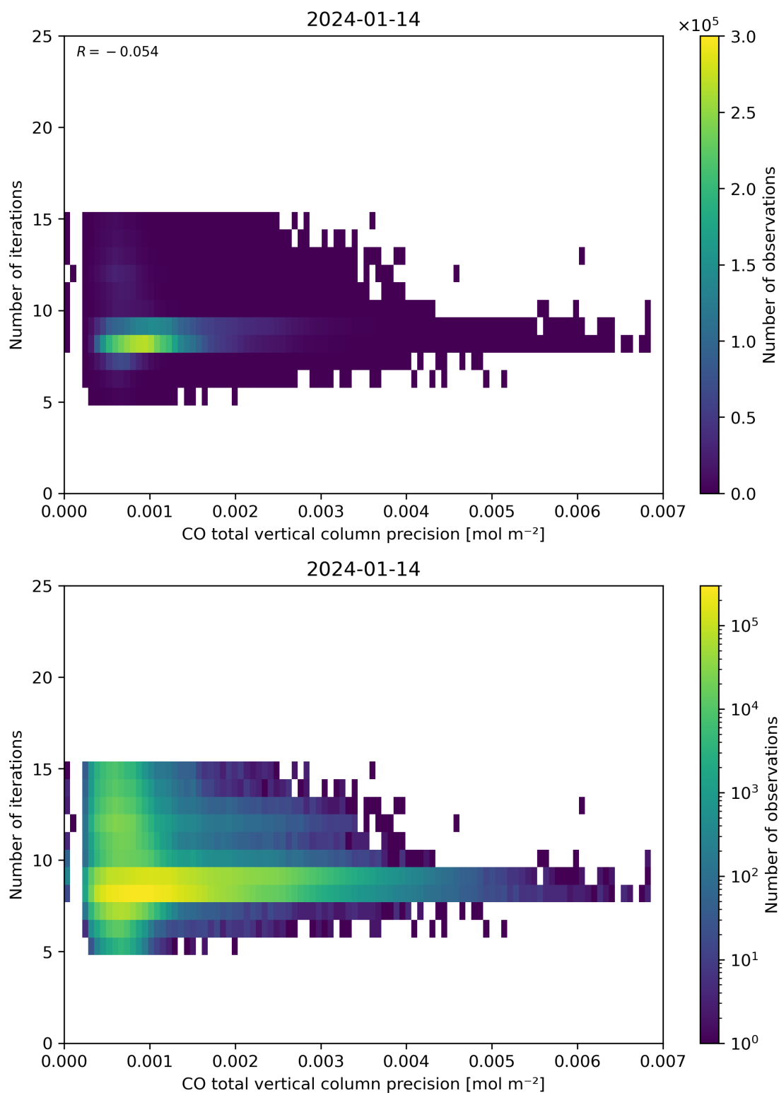
Figure 46: Scatter density plot of “CO total vertical column precision” against “Number of iterations” for 2024-01-13 to 2024-01-15.
