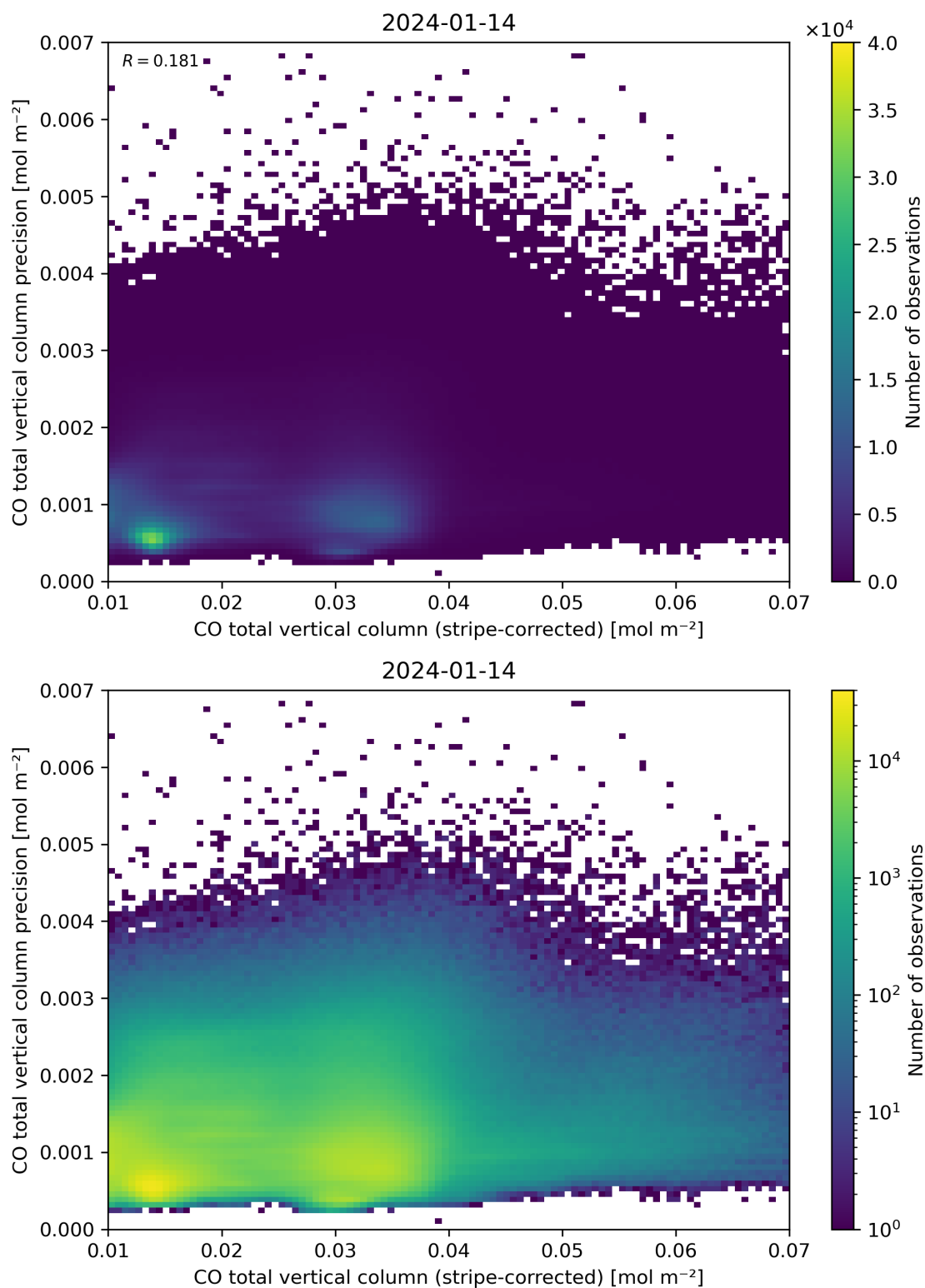
Figure 36: Scatter density plot of “CO total vertical column (stripe-corrected)” against “CO total vertical column precision” for 2024-01-13 to 2024-01-15.
