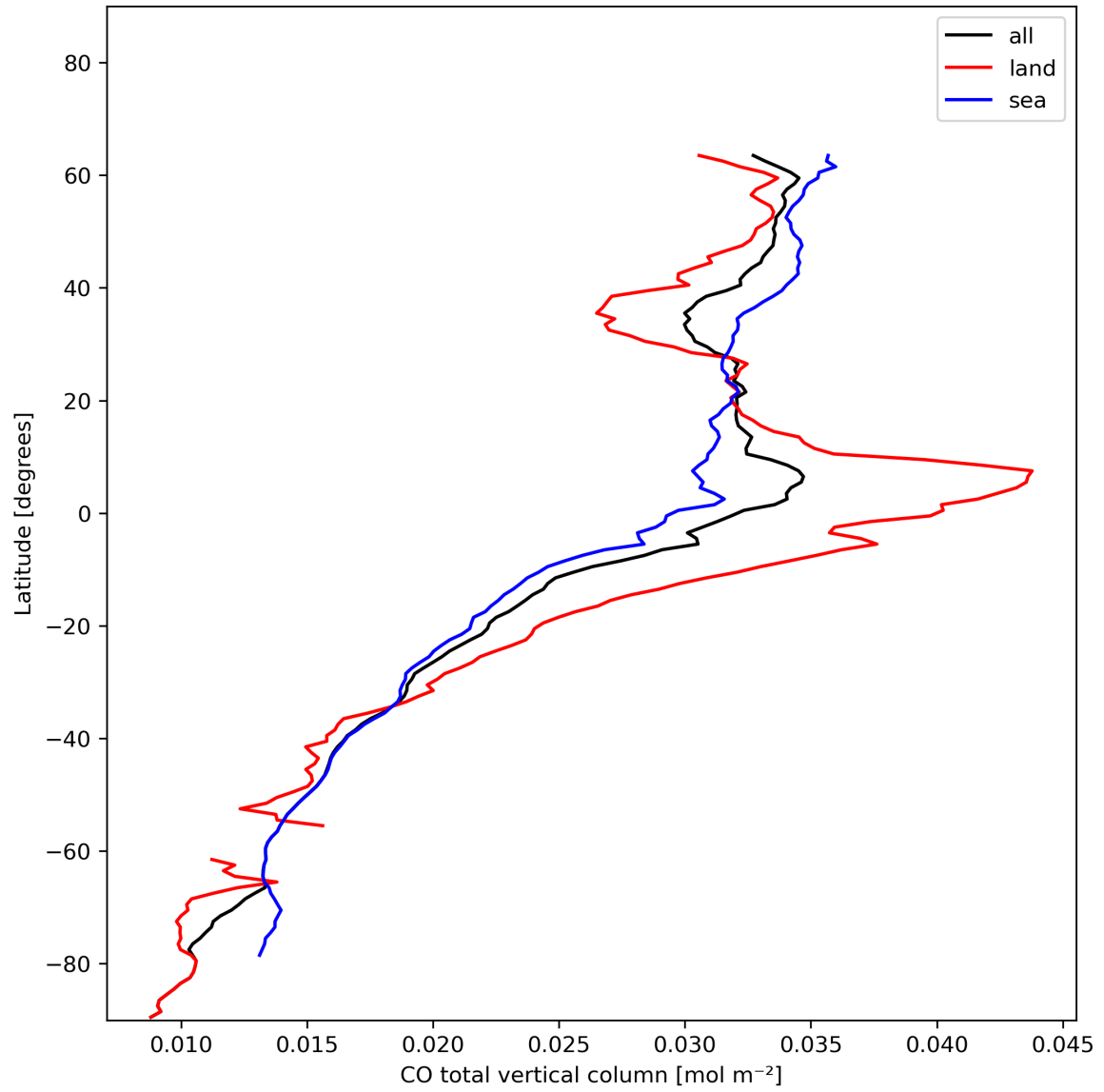
Figure 10: Zonal average of “CO total vertical column” for 2024-01-13 to 2024-01-15.
