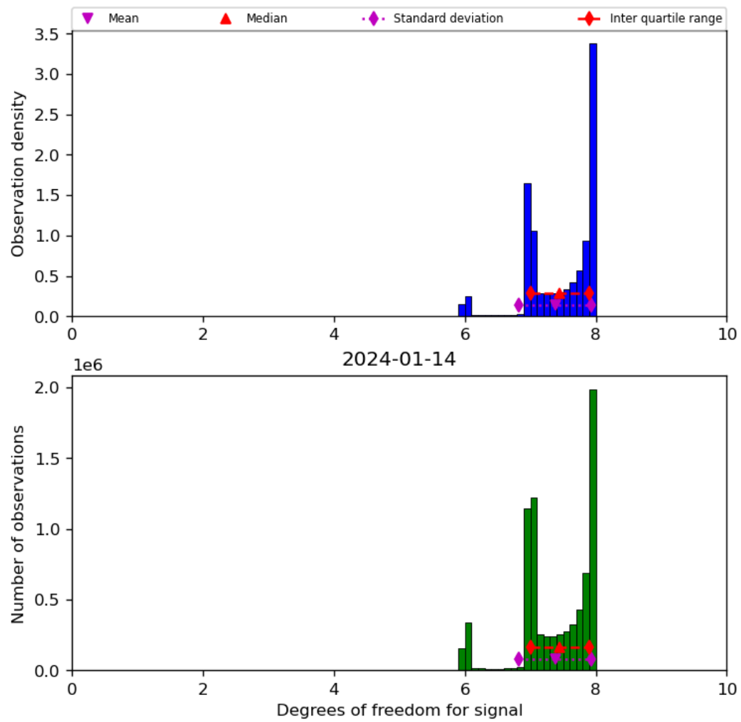
Figure 23: Histogram of “Degrees of freedom for signal” for 2024-01-13 to 2024-01-15
