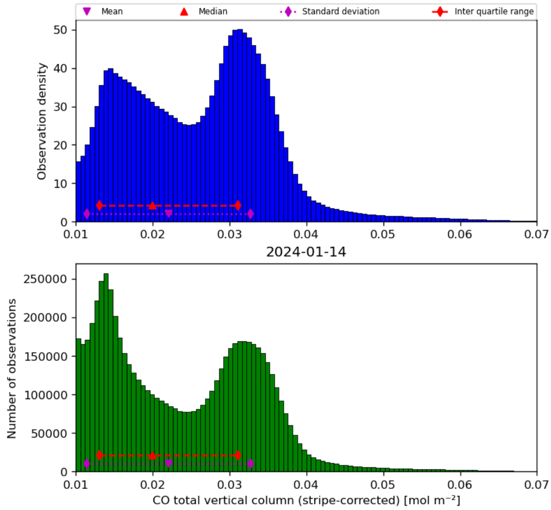
Figure 19: Histogram of “CO total vertical column (stripe-corrected)” for 2024-01-13 to 2024-01-15
