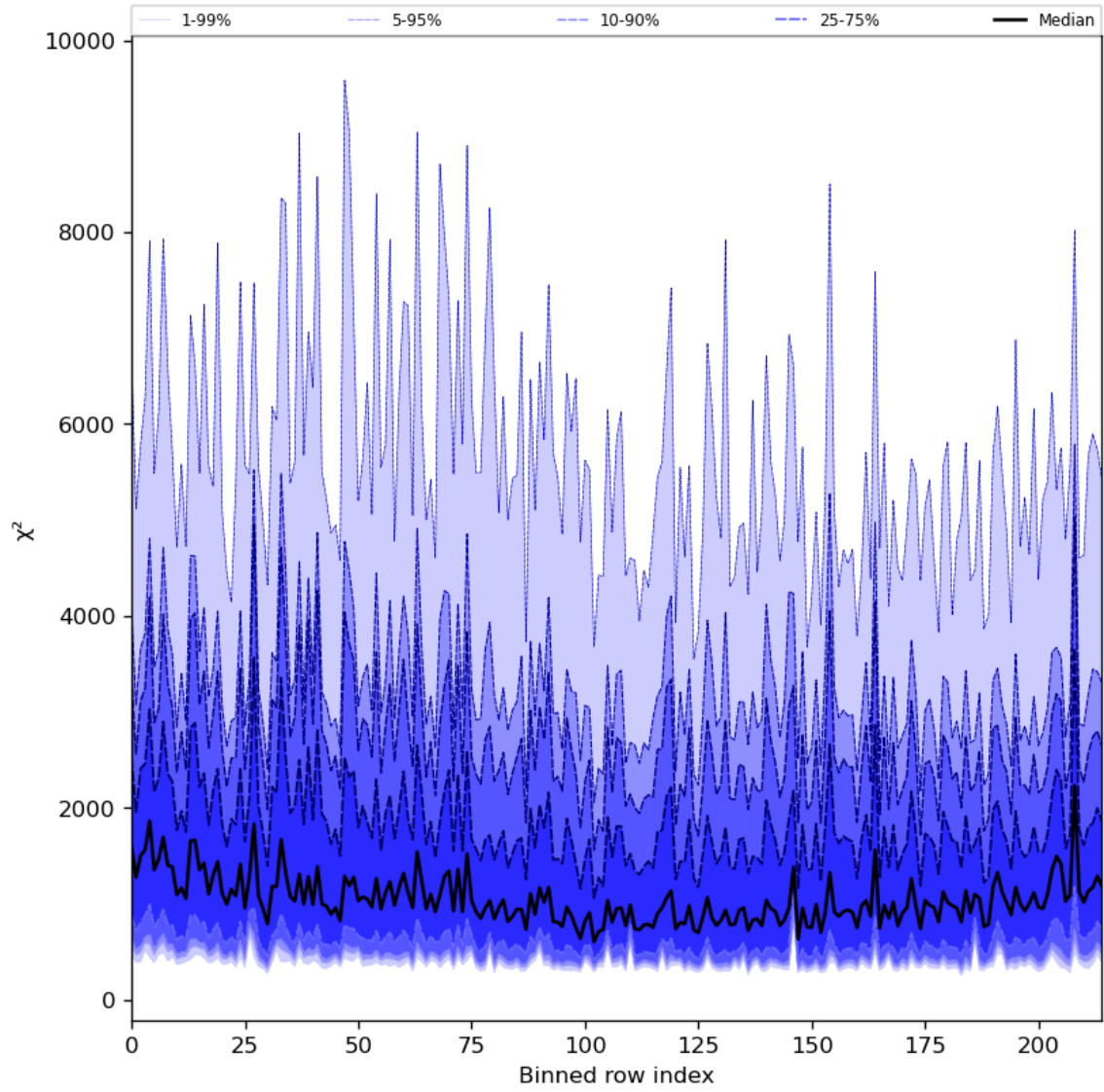
Figure 30: Along track statistics of “ \chi^2 ” for 2024-01-13 to 2024-01-15
