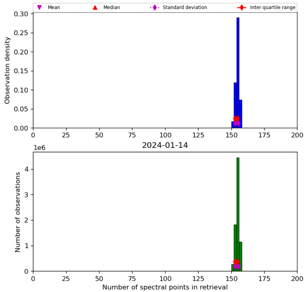
Figure 21: Histogram of “Number of spectral points in retrieval” for 2024-01-13 to 2024-01-15
