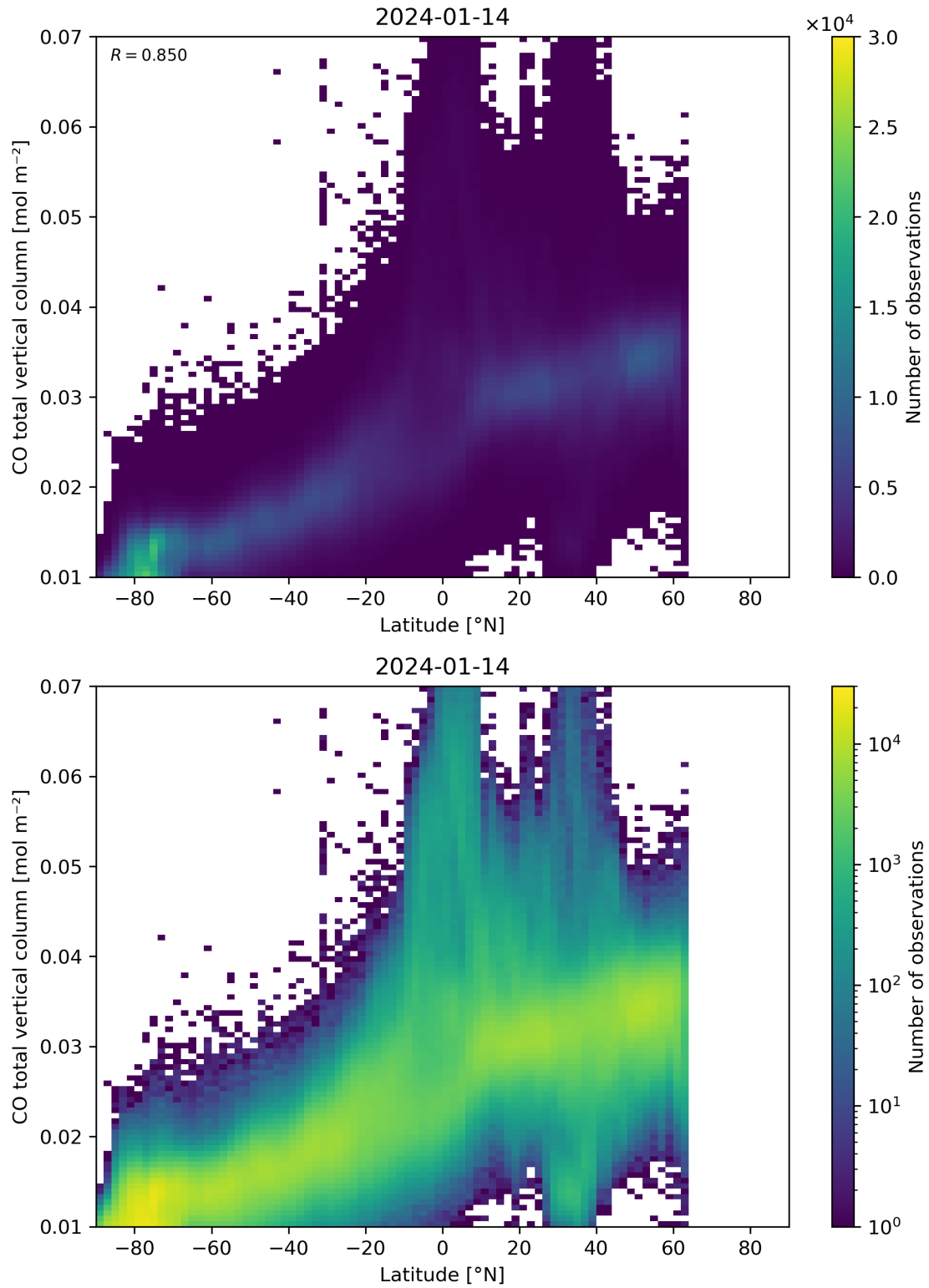
Figure 51: Scatter density plot of “Latitude” against “CO total vertical column” for 2024-01-13 to 2024-01-15.
