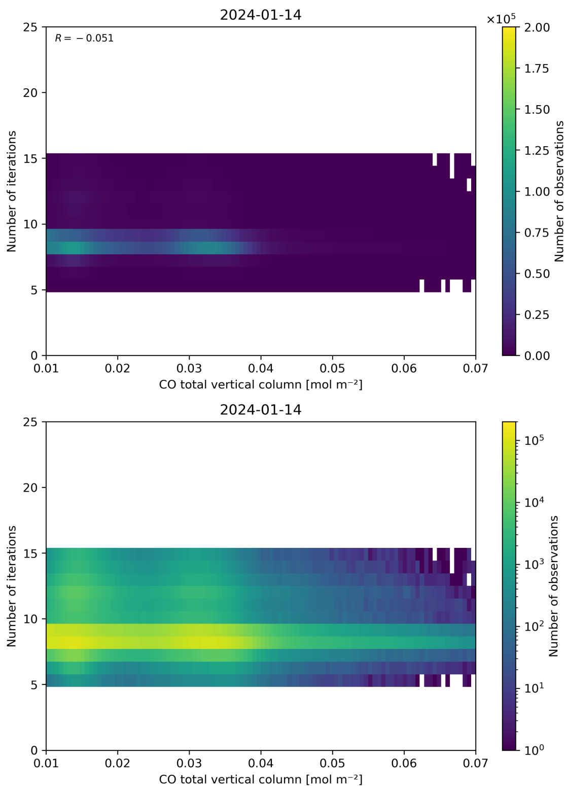
Figure 42: Scatter density plot of “CO total vertical column” against “Number of iterations” for 2024-01-13 to 2024-01-15.
