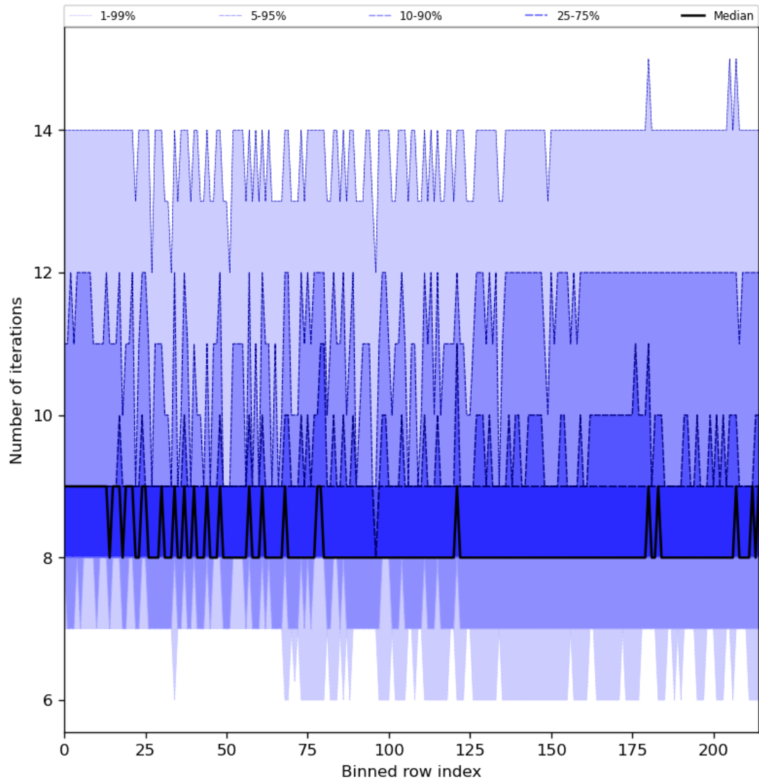
Figure 32: Along track statistics of “Number of iterations” for 2024-01-13 to 2024-01-15
