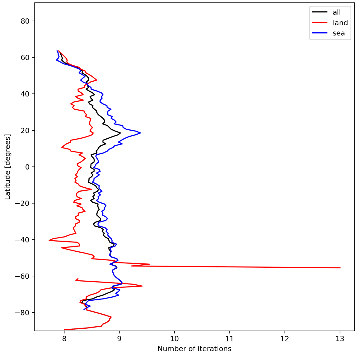
Figure 16: Zonal average of “Number of iterations” for 2024-01-13 to 2024-01-15.
