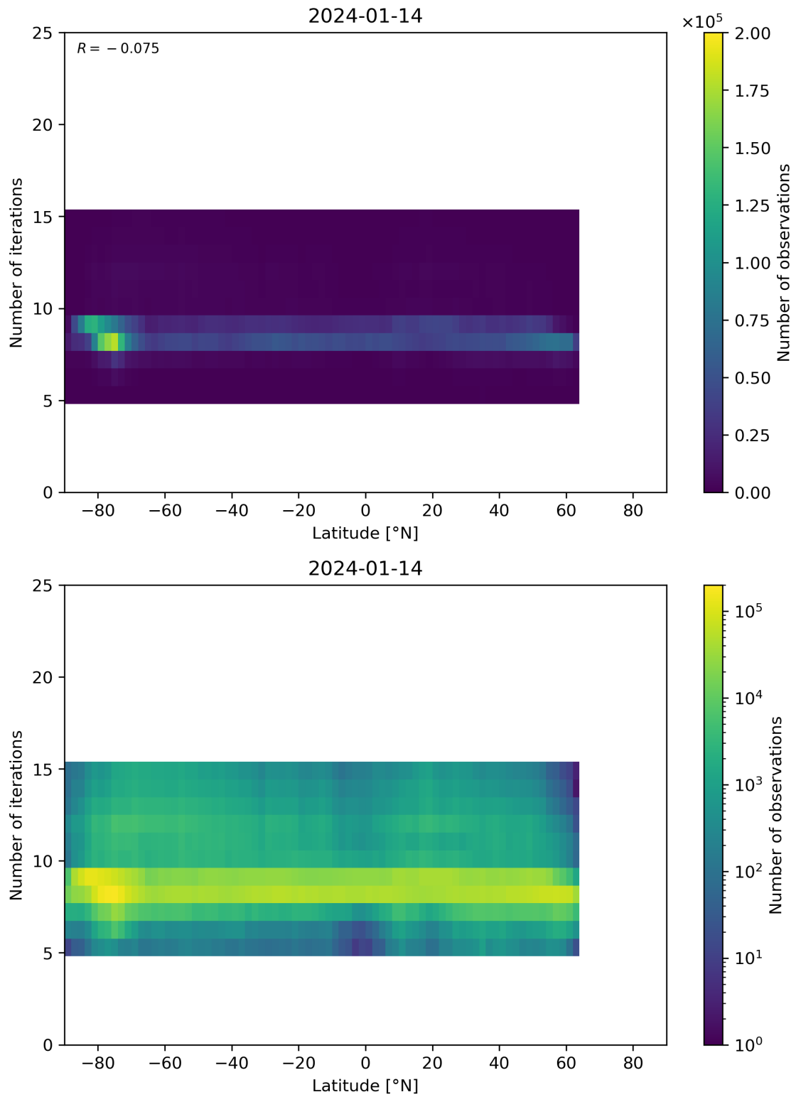
Figure 56: Scatter density plot of “Latitude” against “Number of iterations” for 2024-01-13 to 2024-01-15.
