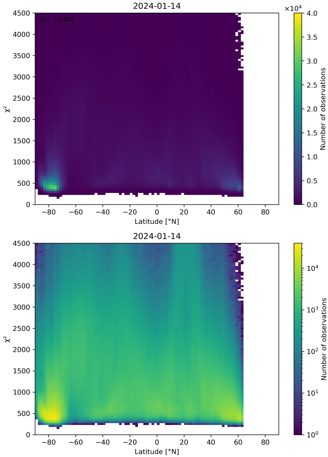
Figure 54: Scatter density plot of “Latitude” against “ \chi^2 ” for 2024-01-13 to 2024-01-15.
