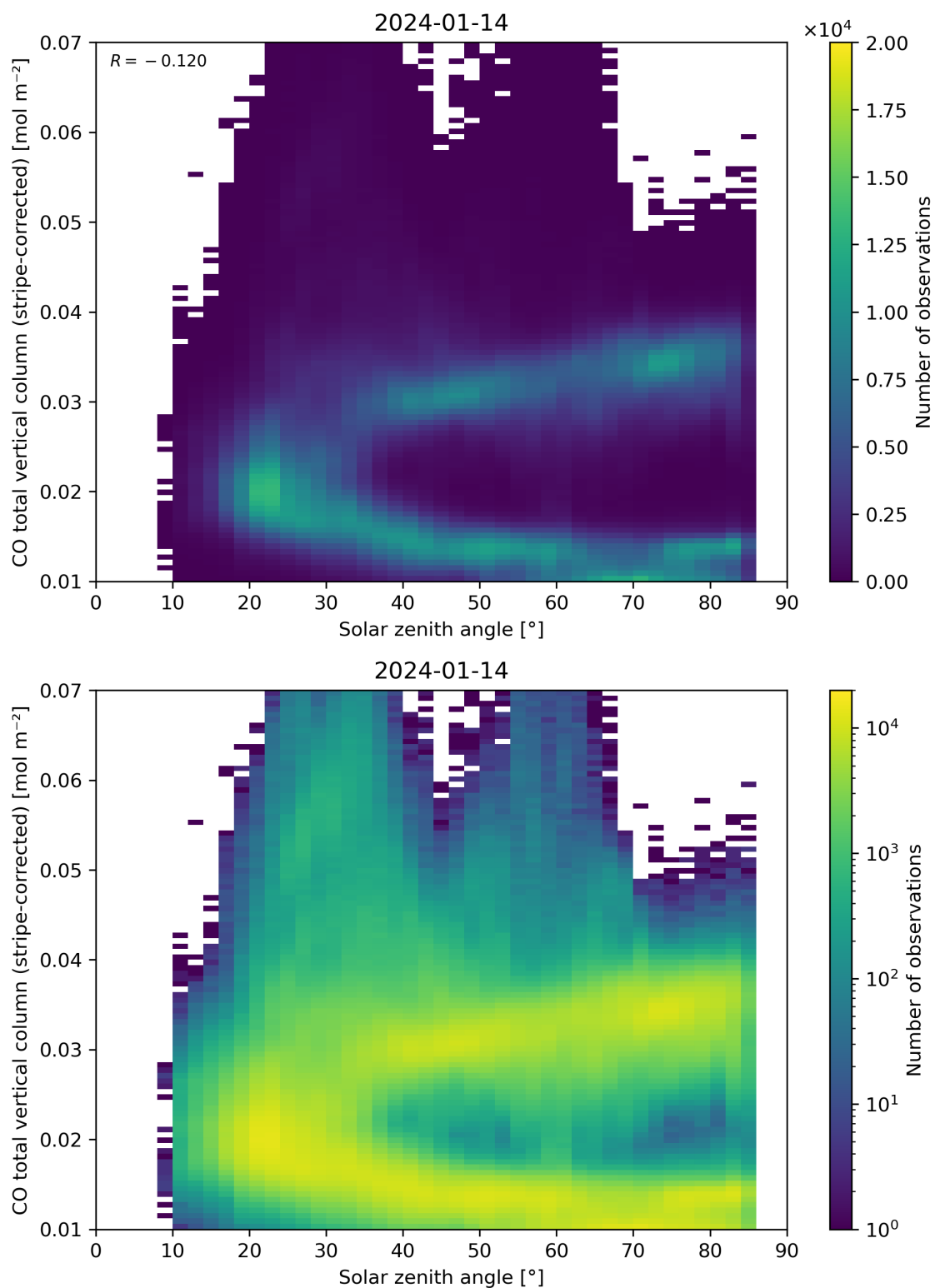
Figure 62: Scatter density plot of “Solar zenith angle” against “CO total vertical column (stripe-corrected)” for 2024-01-13 to 2024-01-15.
