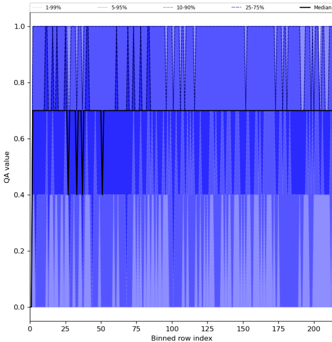
Figure 25: Along track statistics of “QA value” for 2024-01-13 to 2024-01-15
