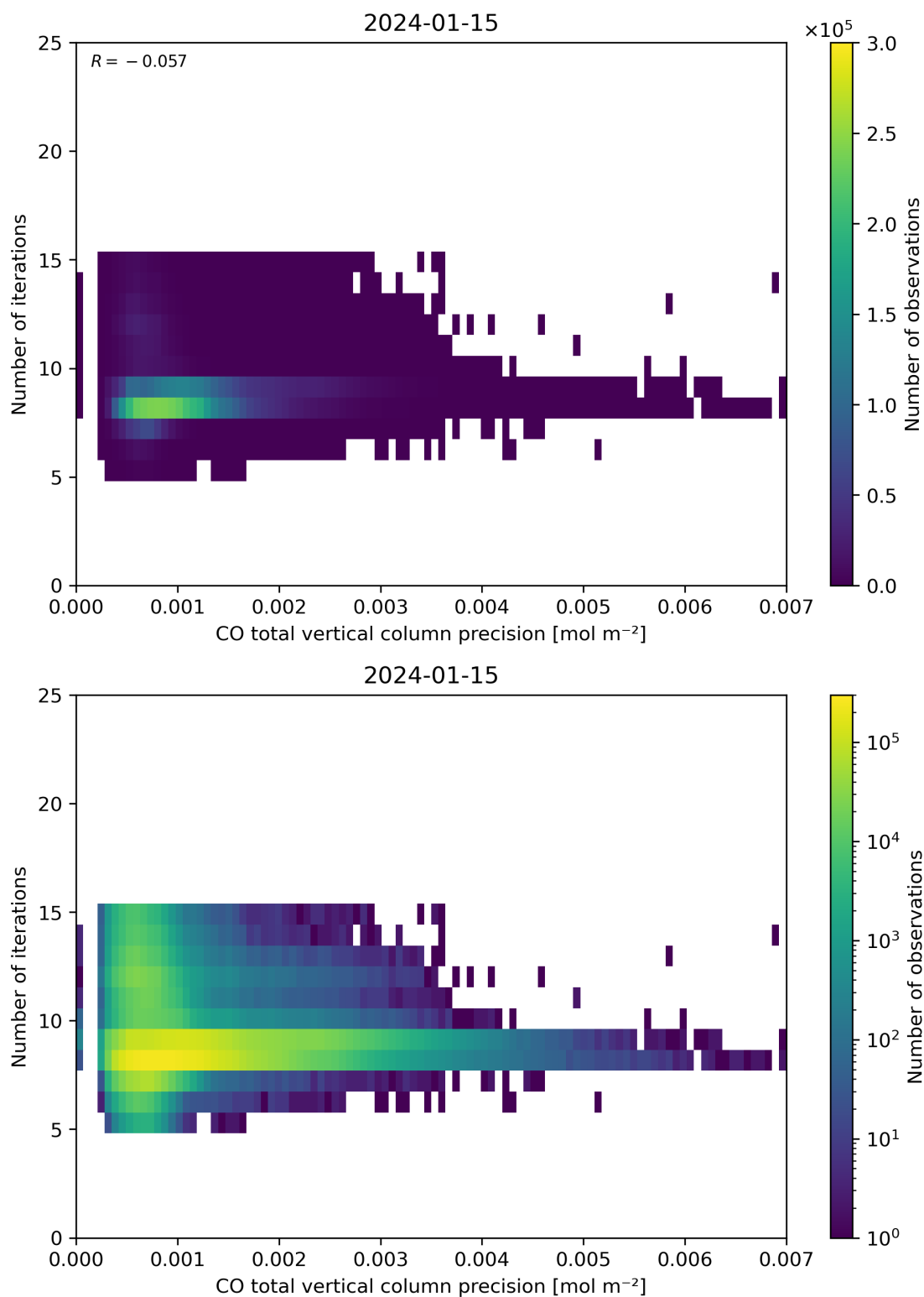
Figure 46: Scatter density plot of “CO total vertical column precision” against “Number of iterations” for 2024-01-15 to 2024-01-16.
