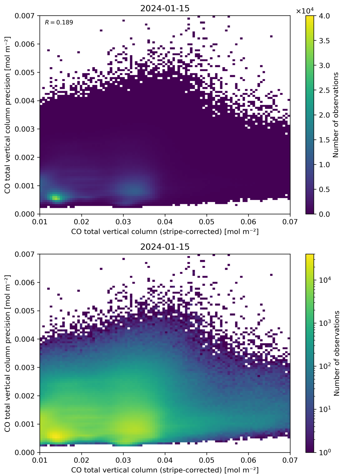
Figure 36: Scatter density plot of “CO total vertical column (stripe-corrected)” against “CO total vertical column precision” for 2024-01-15 to 2024-01-16.
