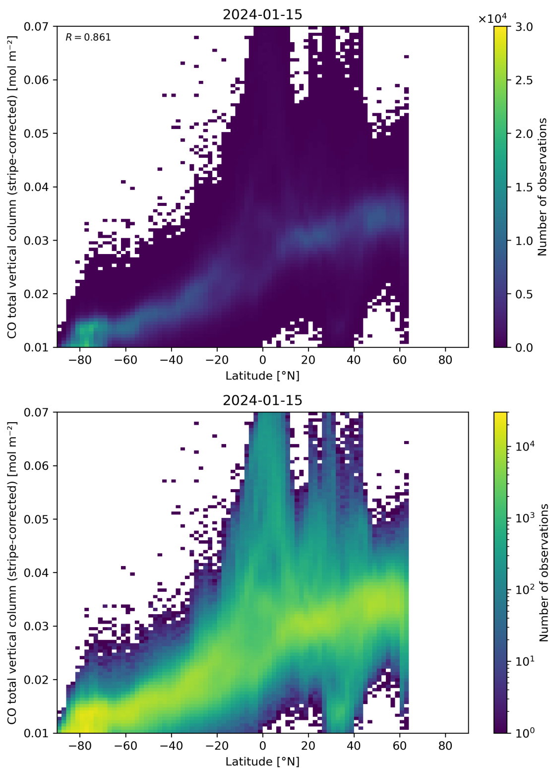
Figure 52: Scatter density plot of “Latitude” against “CO total vertical column (stripe-corrected)” for 2024-01-15 to 2024-01-16.
