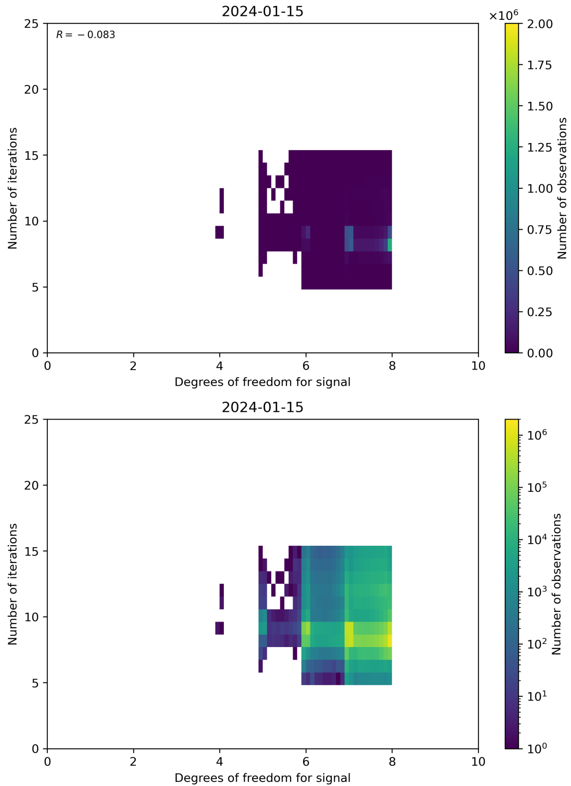
Figure 50: Scatter density plot of “Degrees of freedom for signal” against “Number of iterations” for 2024-01-15 to 2024-01-16.
