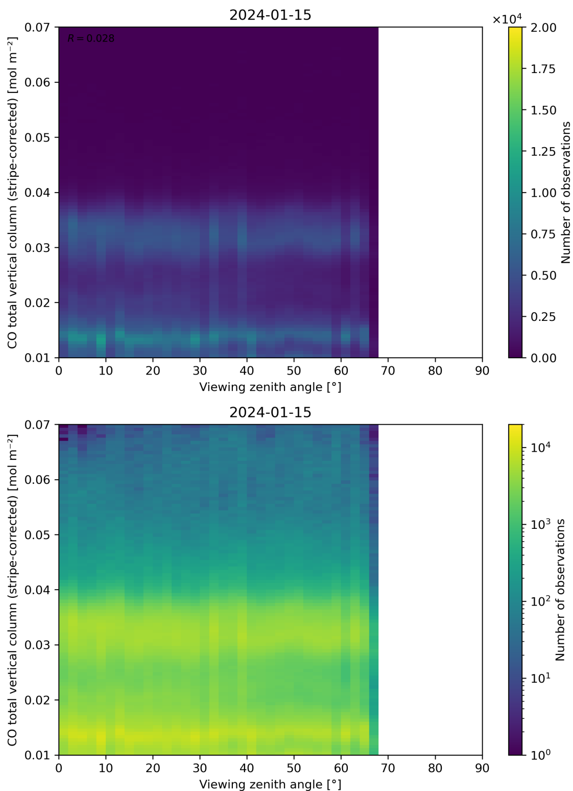
Figure 70: Scatter density plot of “Viewing zenith angle” against “CO total vertical column (stripe-corrected)” for 2024-01-15 to 2024-01-16.
