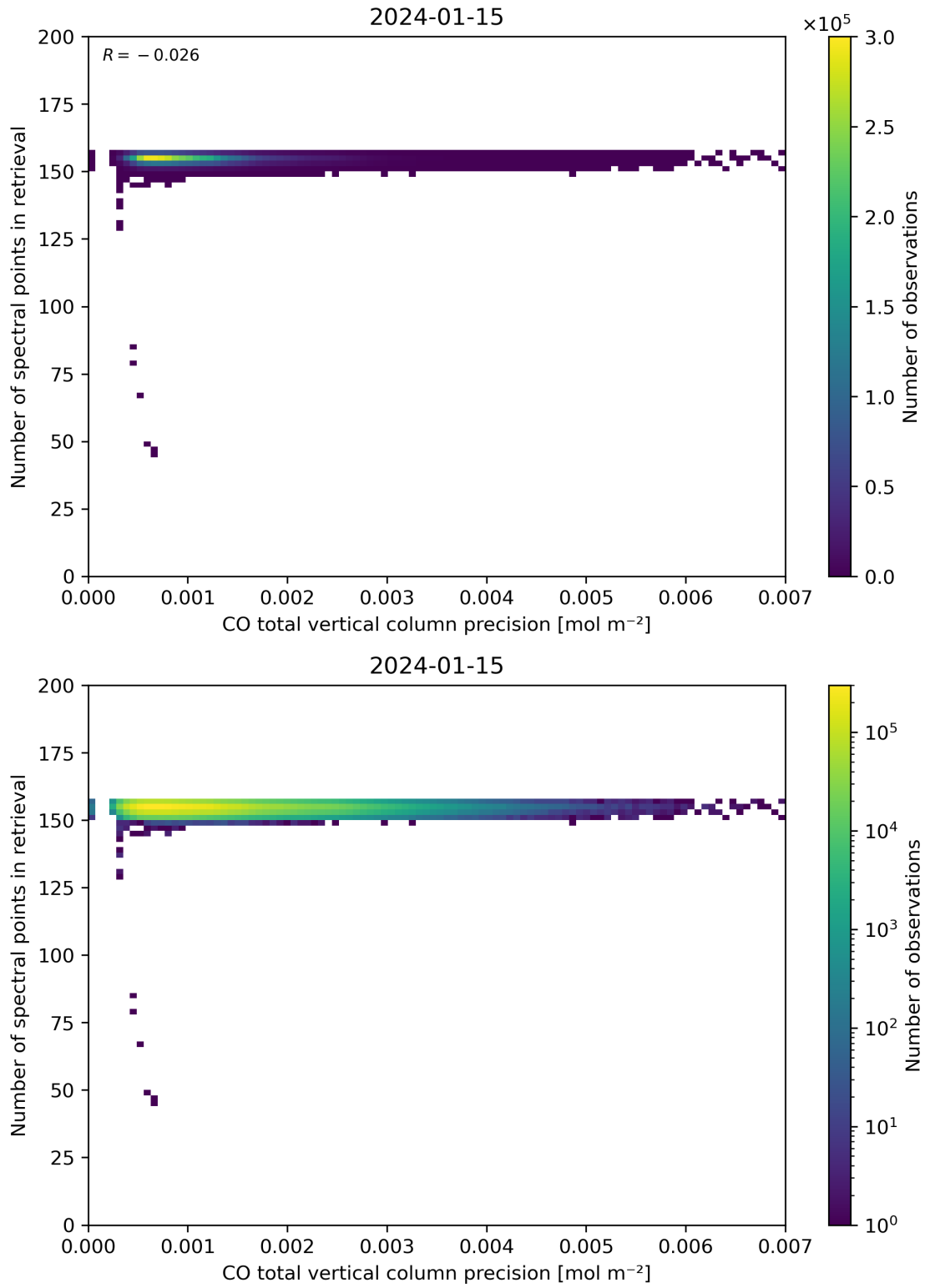
Figure 47: Scatter density plot of “CO total vertical column precision” against “Number of spectral points in retrieval” for 2024-01-15 to 2024-01-16.
