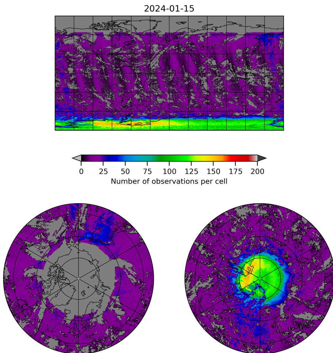
Figure 8: Map of the number of observations for 2024-01-15 to 2024-01-16
