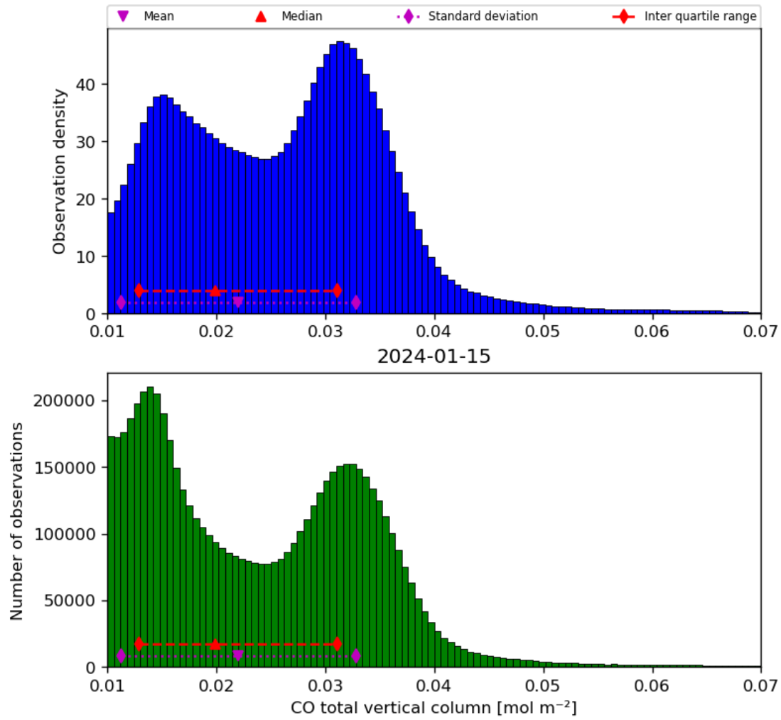
Figure 18: Histogram of “CO total vertical column” for 2024-01-15 to 2024-01-16
