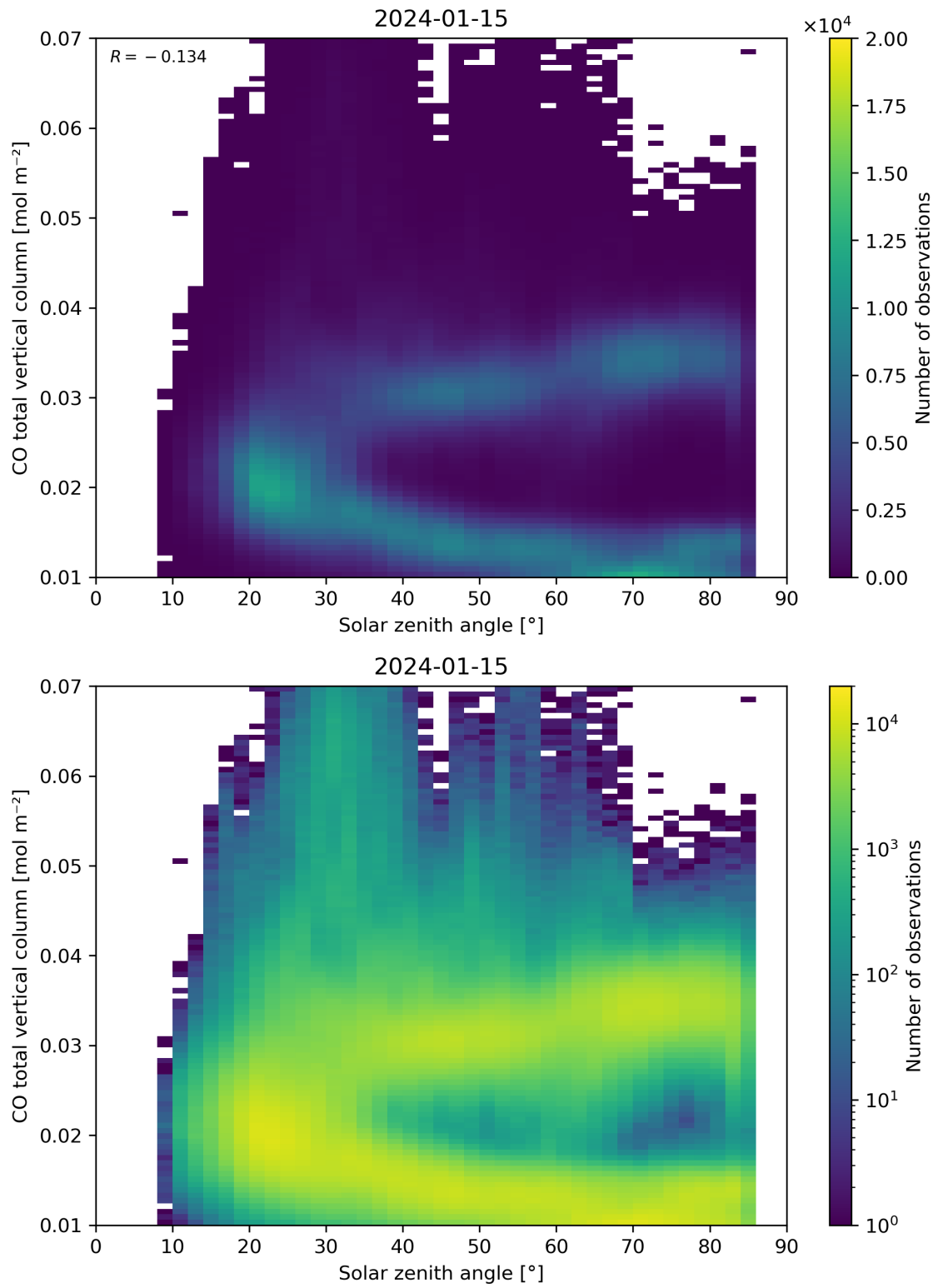
Figure 61: Scatter density plot of “Solar zenith angle” against “CO total vertical column” for 2024-01-15 to 2024-01-16.
