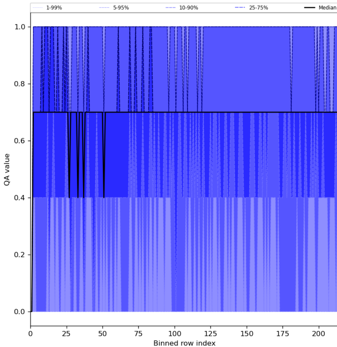
Figure 25: Along track statistics of “QA value” for 2024-01-15 to 2024-01-16
