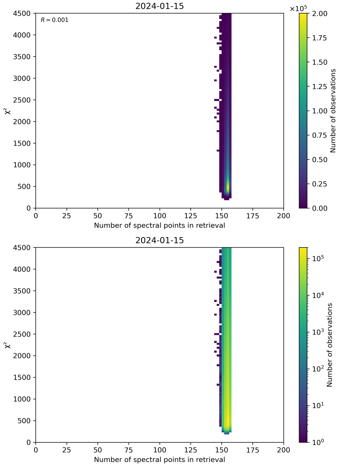
Figure 58: Scatter density plot of “Number of spectral points in retrieval” against “ \chi^2 ” for 2024-01-15 to 2024-01-16.
