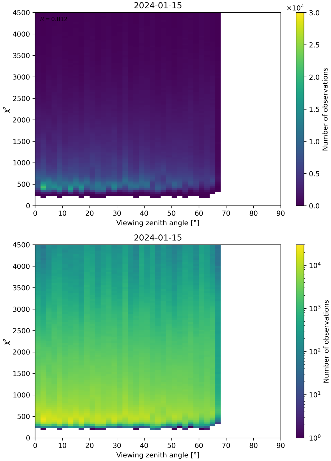
Figure 72: Scatter density plot of “Viewing zenith angle” against “ \chi^2 ” for 2024-01-15 to 2024-01-16.
