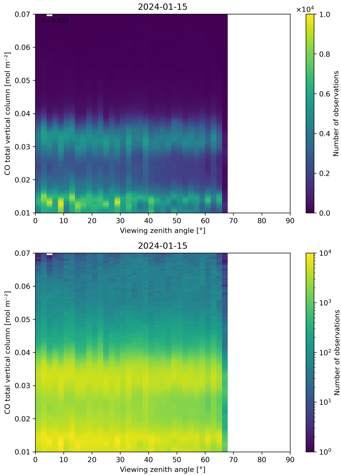
Figure 69: Scatter density plot of “Viewing zenith angle” against “CO total vertical column” for 2024-01-15 to 2024-01-16.
