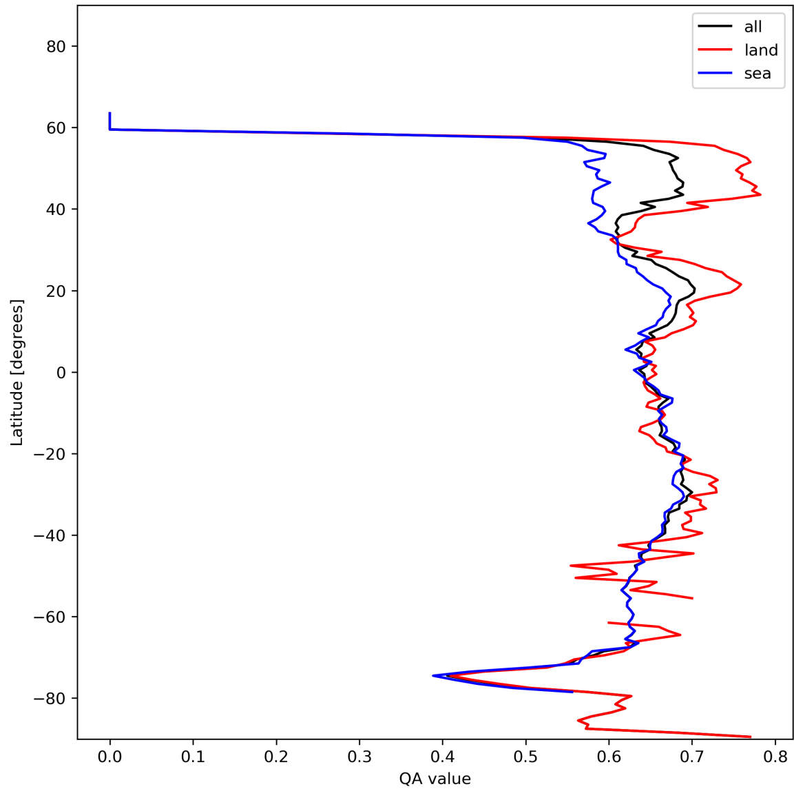
Figure 9: Zonal average of “QA value” for 2024-01-15 to 2024-01-16.
