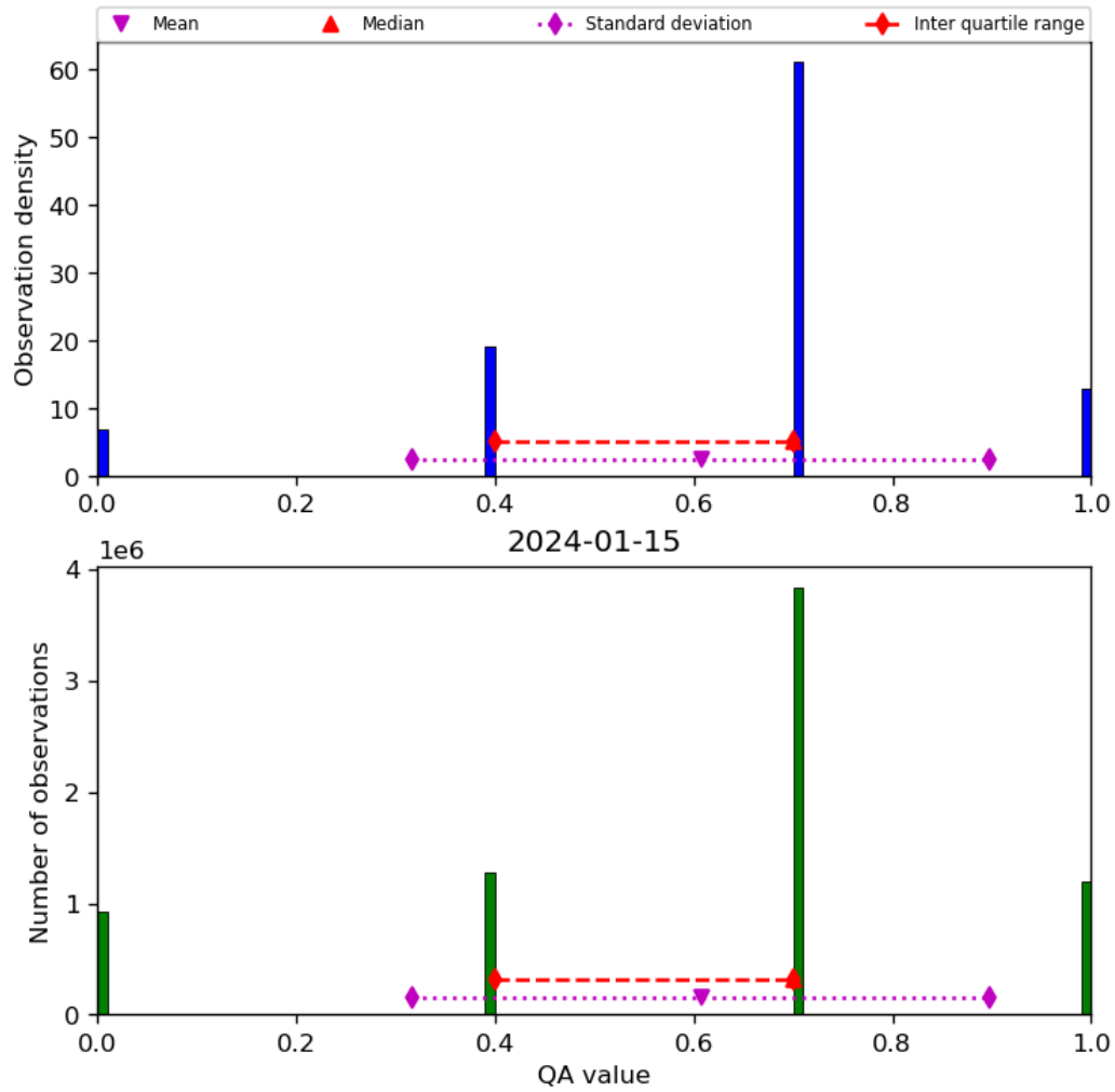
Figure 17: Histogram of “QA value” for 2024-01-15 to 2024-01-16
