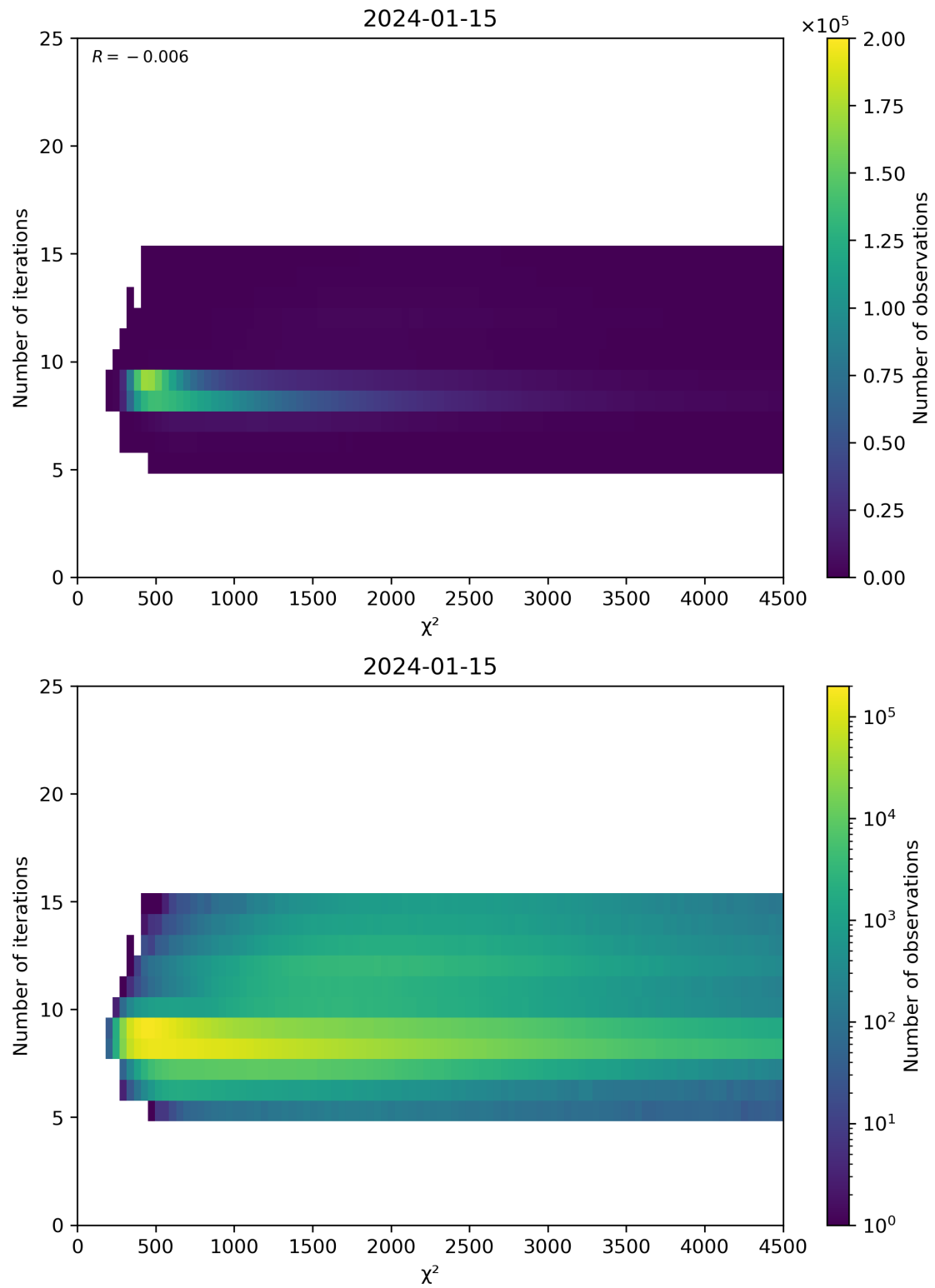
Figure 49: Scatter density plot of “ \chi^2 ” against “Number of iterations” for 2024-01-15 to 2024-01-16.
