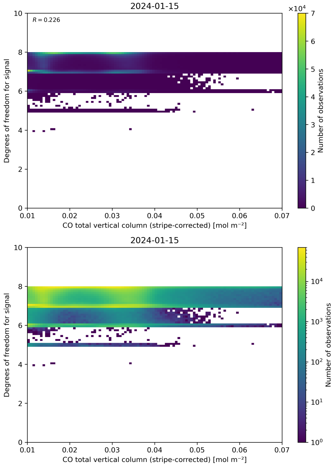
Figure 38: Scatter density plot of “CO total vertical column (stripe-corrected)” against “Degrees of freedom for signal” for 2024-01-15 to 2024-01-16.
