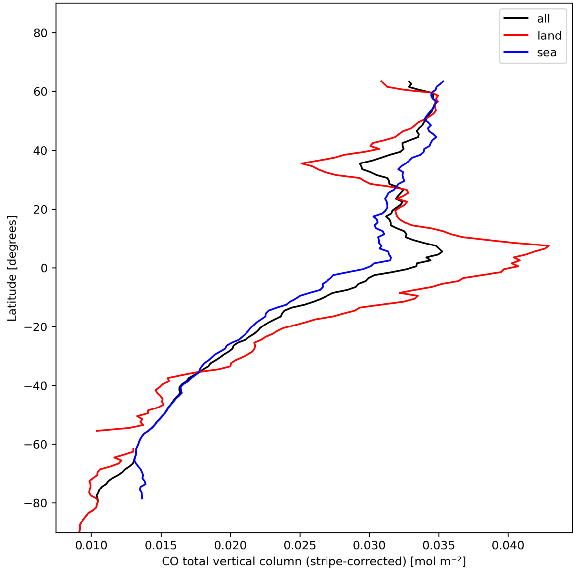
Figure 11: Zonal average of “CO total vertical column (stripe-corrected)” for 2024-01-15 to 2024-01-16.
