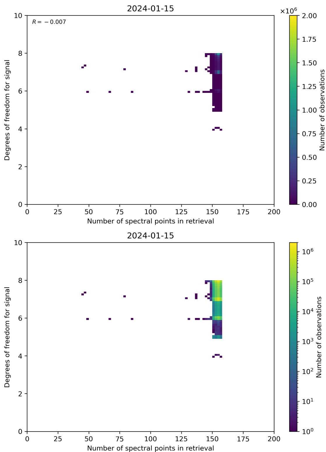
Figure 59: Scatter density plot of “Number of spectral points in retrieval” against “Degrees of freedom for signal” for 2024-01-15 to 2024-01-16.
