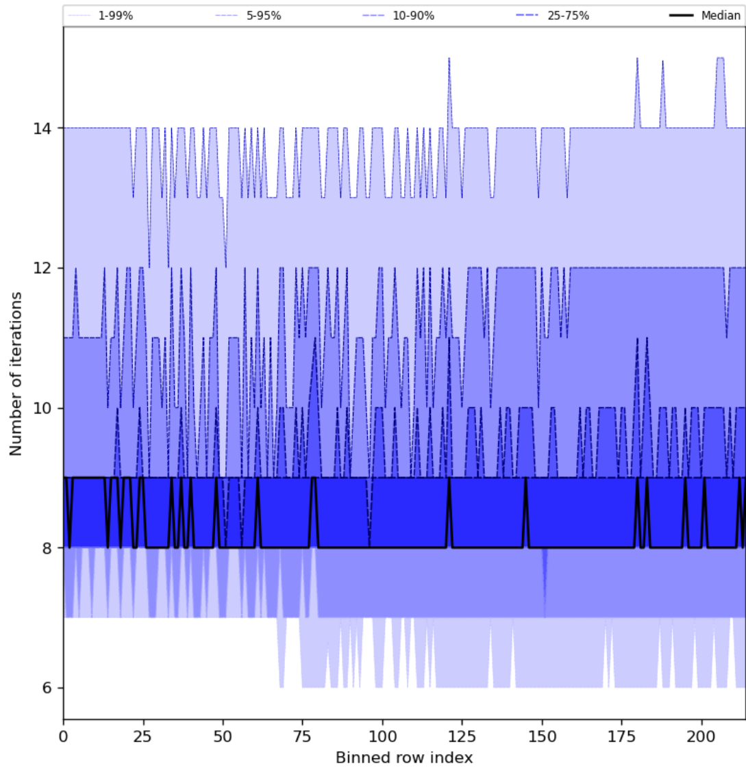
Figure 32: Along track statistics of “Number of iterations” for 2024-01-15 to 2024-01-16
