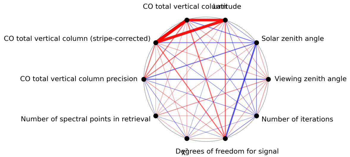
Figure 1: Map of correlation graph for 2024-01-15 to 2024-01-16.
