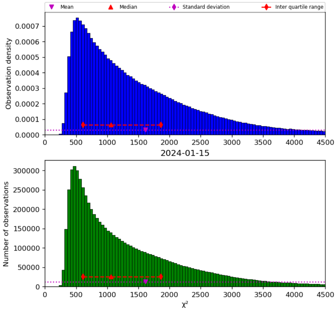
Figure 22: Histogram of “ \chi^2 ” for 2024-01-15 to 2024-01-16
