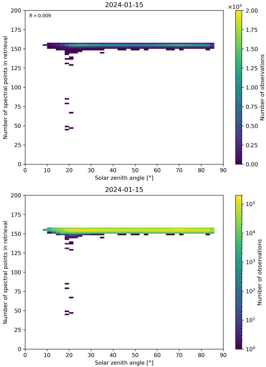
Figure 68: Scatter density plot of “Solar zenith angle” against “Number of spectral points in retrieval” for 2024-01-15 to 2024-01-16.
