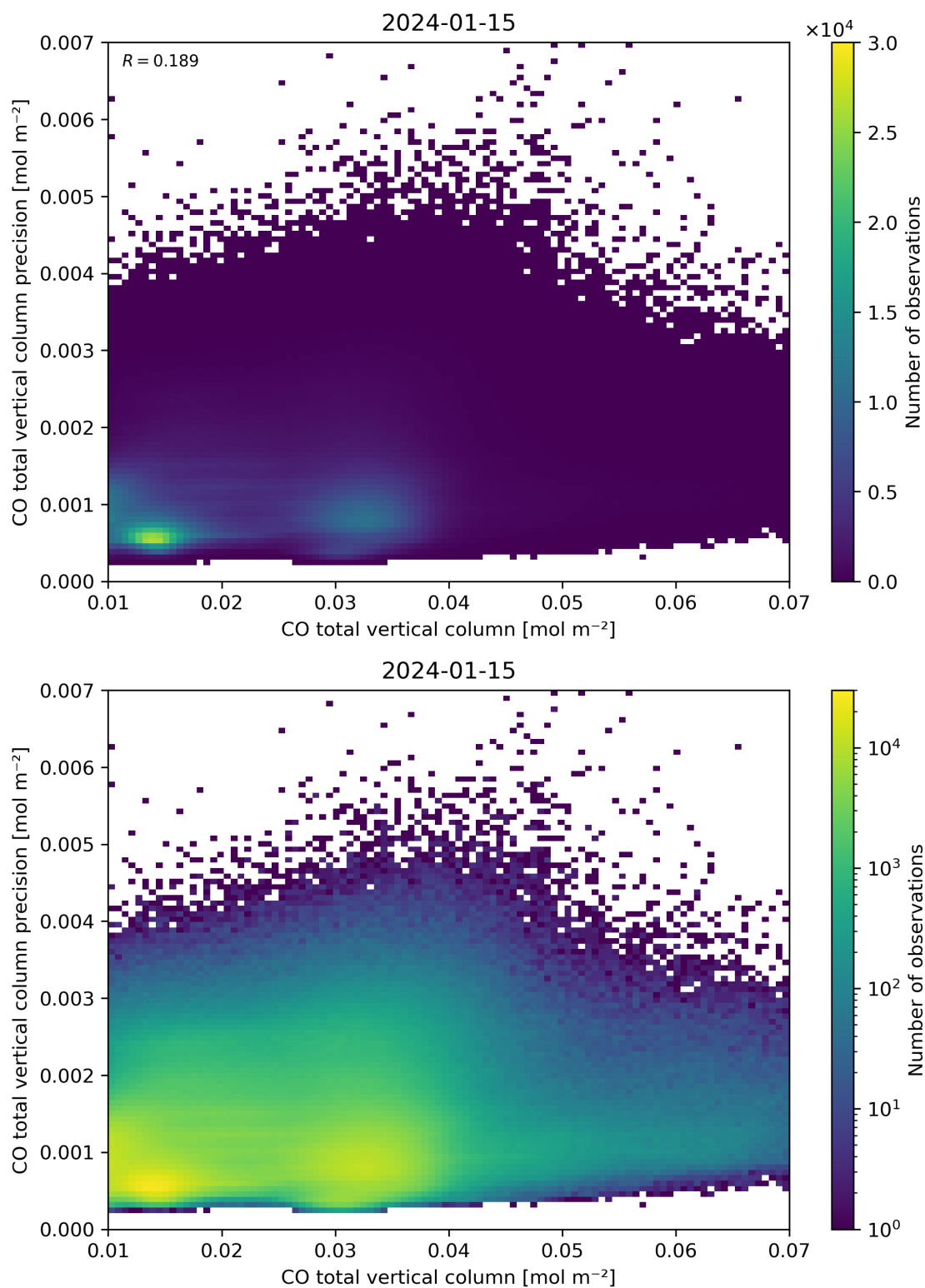
Figure 34: Scatter density plot of “CO total vertical column” against “CO total vertical column precision” for 2024-01-15 to 2024-01-16.
