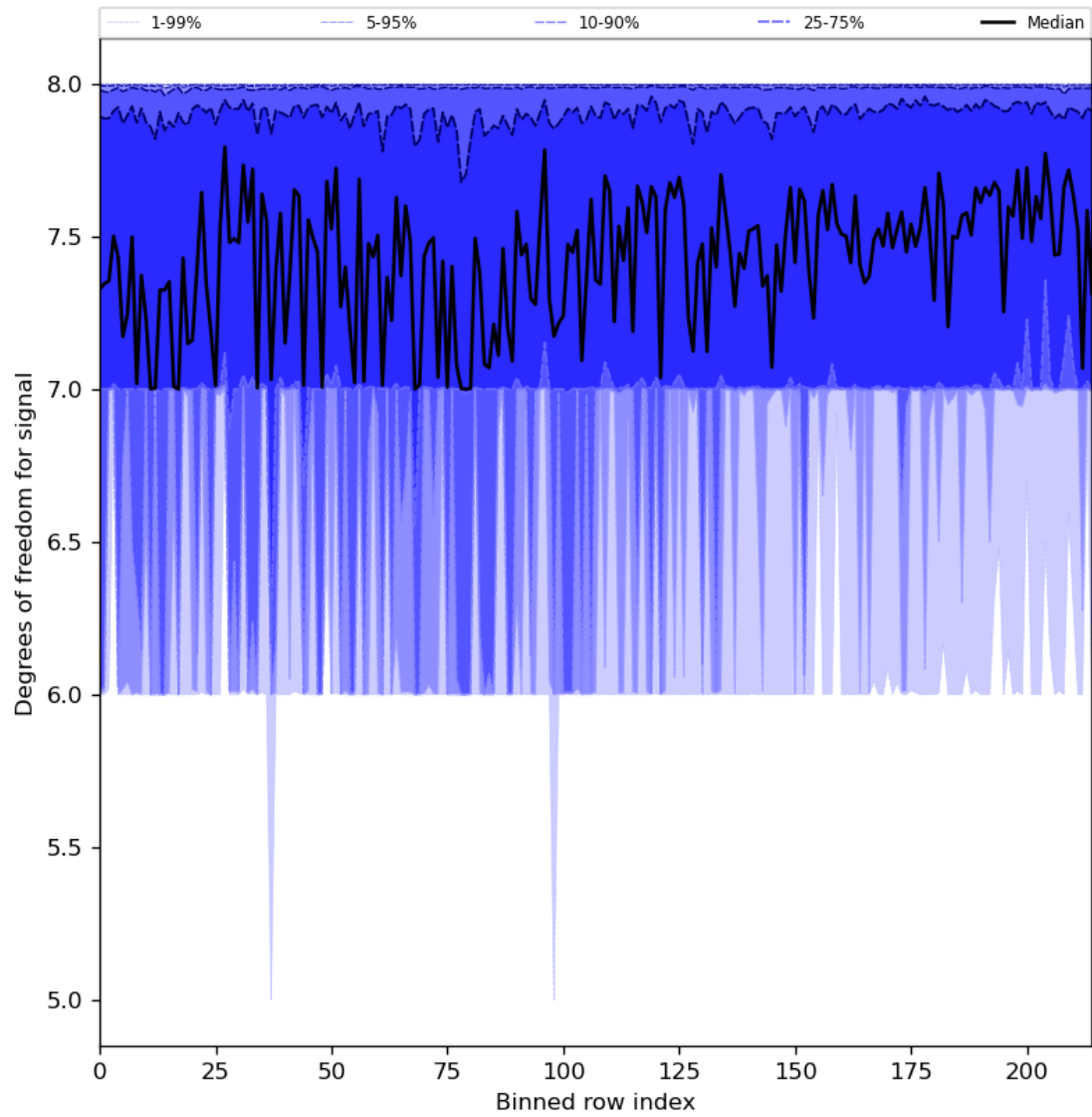
Figure 31: Along track statistics of “Degrees of freedom for signal” for 2024-01-15 to 2024-01-16
