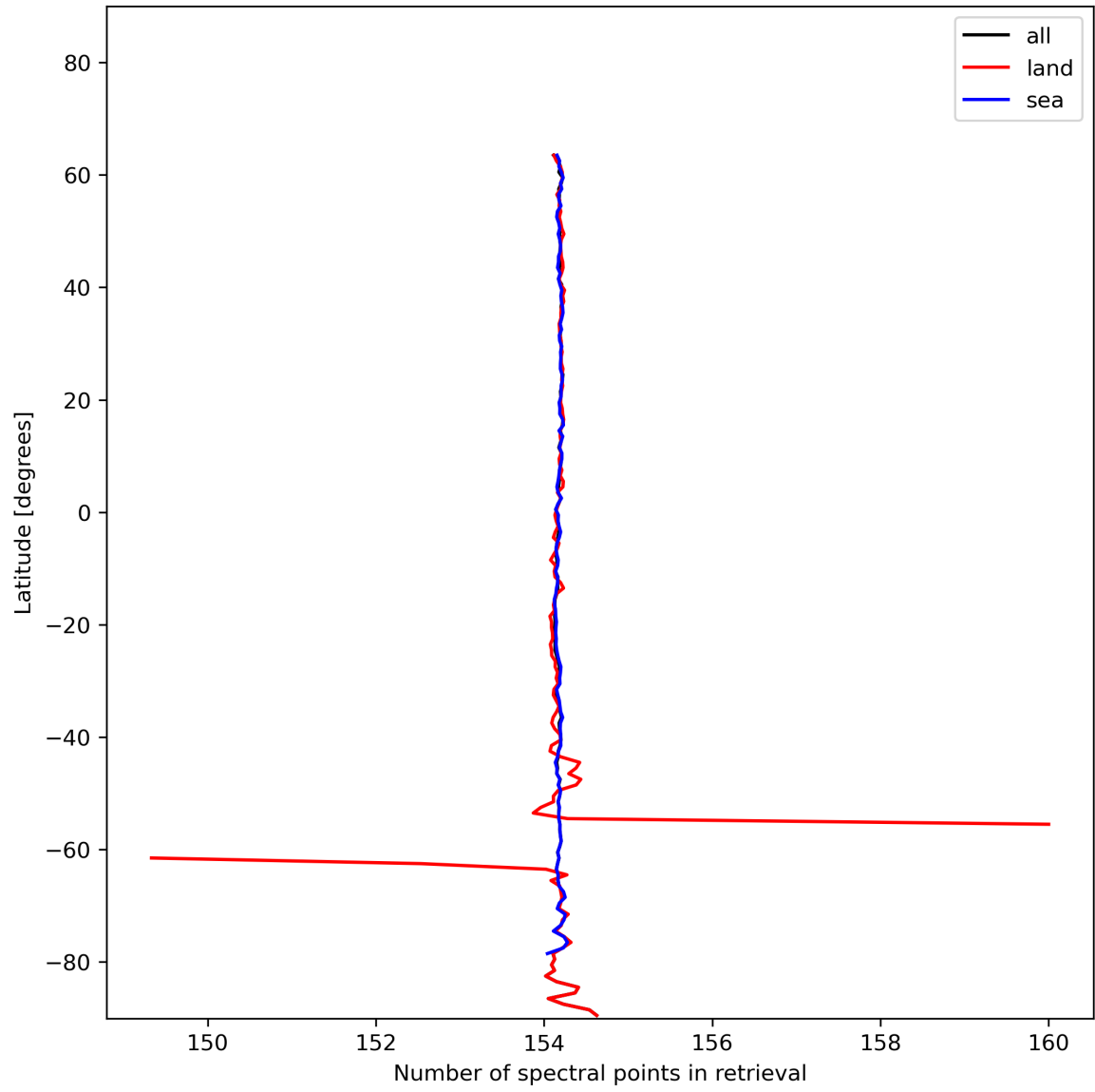
Figure 13: Zonal average of “Number of spectral points in retrieval” for 2024-01-15 to 2024-01-16.
