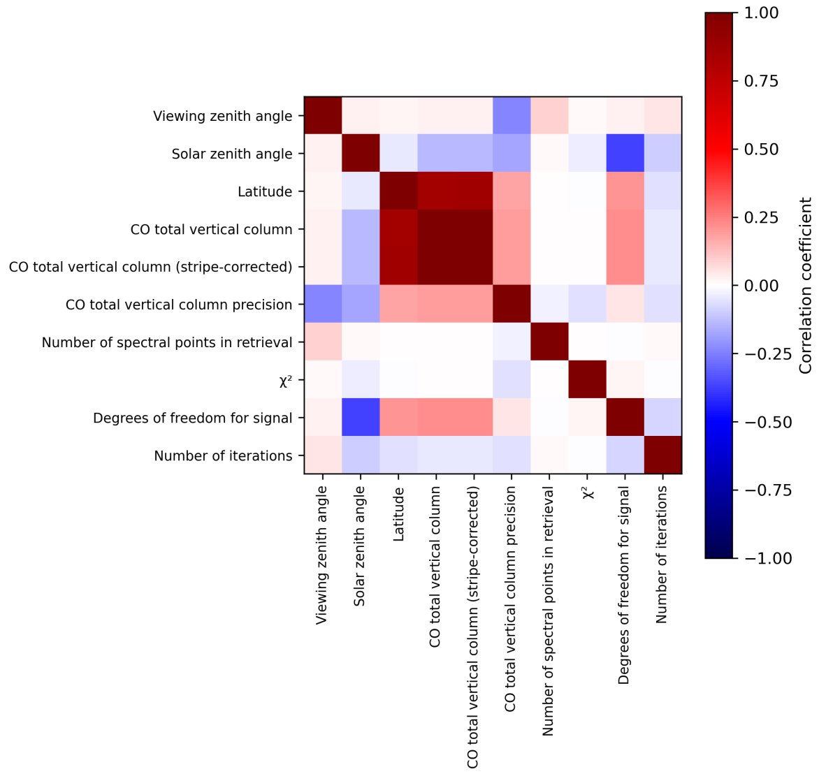
Figure 2: Map of correlation matrix for 2024-01-15 to 2024-01-16.
