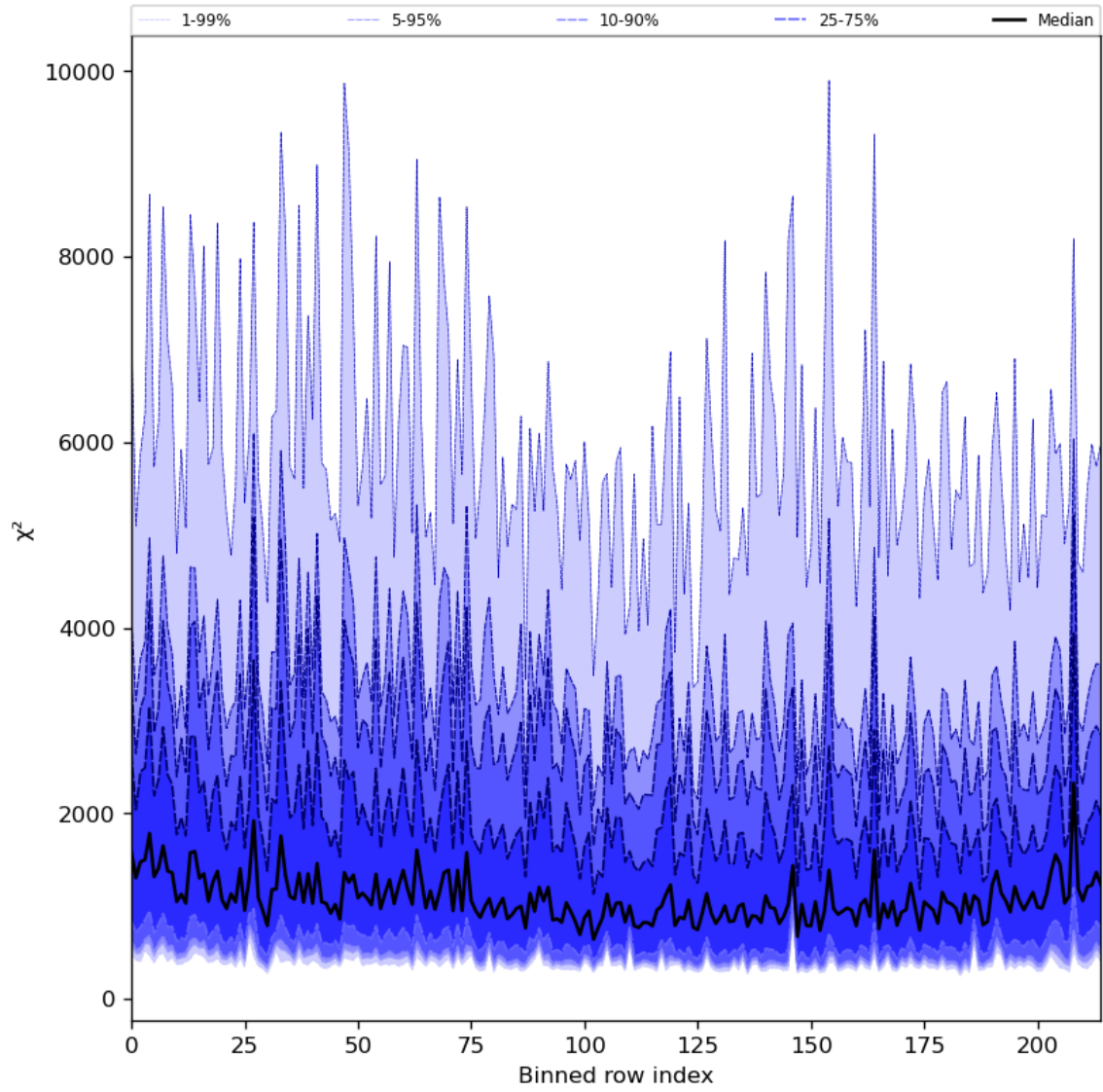
Figure 30: Along track statistics of “ \chi^2 ” for 2024-01-15 to 2024-01-16
