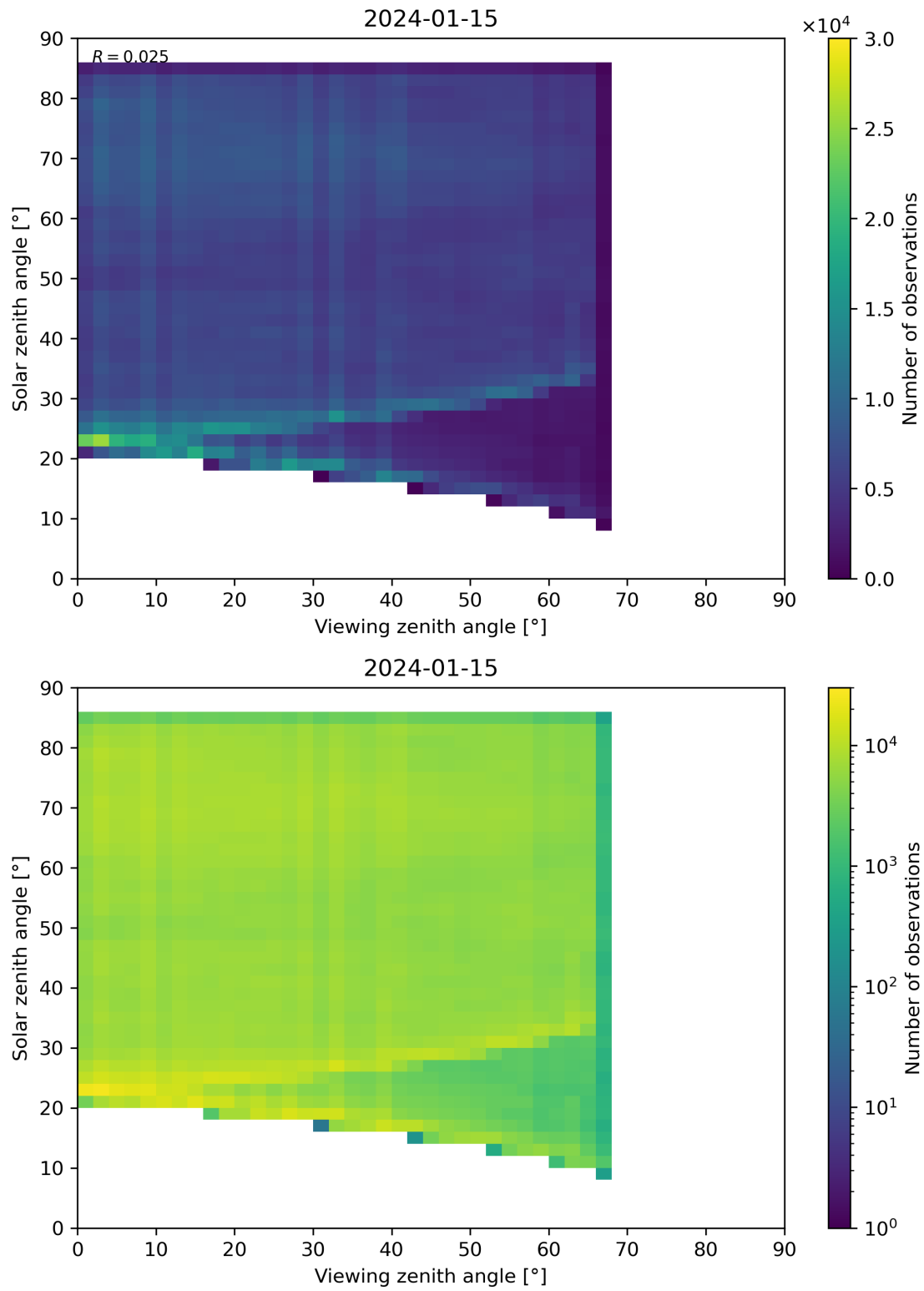
Figure 77: Scatter density plot of “Viewing zenith angle” against “Solar zenith angle” for 2024-01-15 to 2024-01-16.
