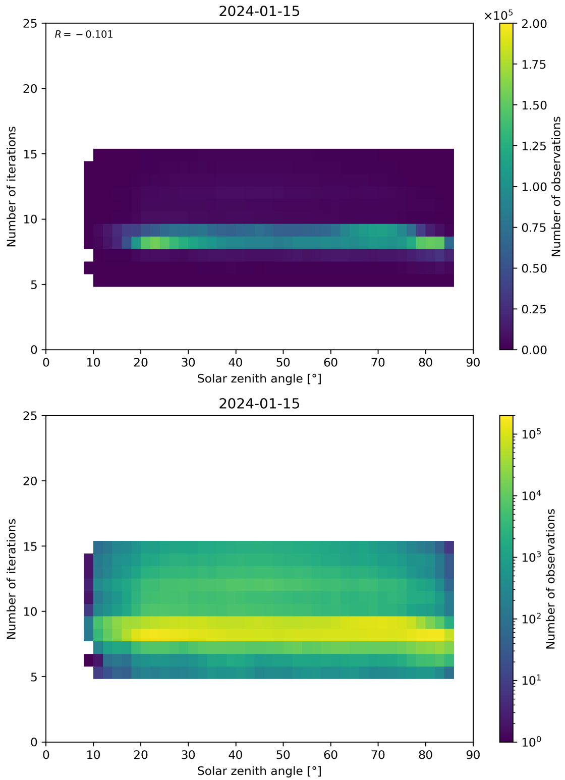
Figure 67: Scatter density plot of “Solar zenith angle” against “Number of iterations” for 2024-01-15 to 2024-01-16.
