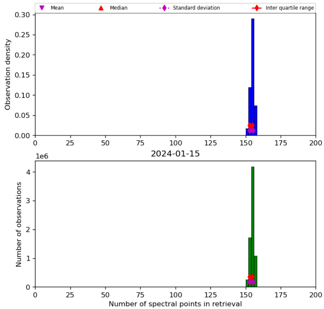
Figure 21: Histogram of “Number of spectral points in retrieval” for 2024-01-15 to 2024-01-16
