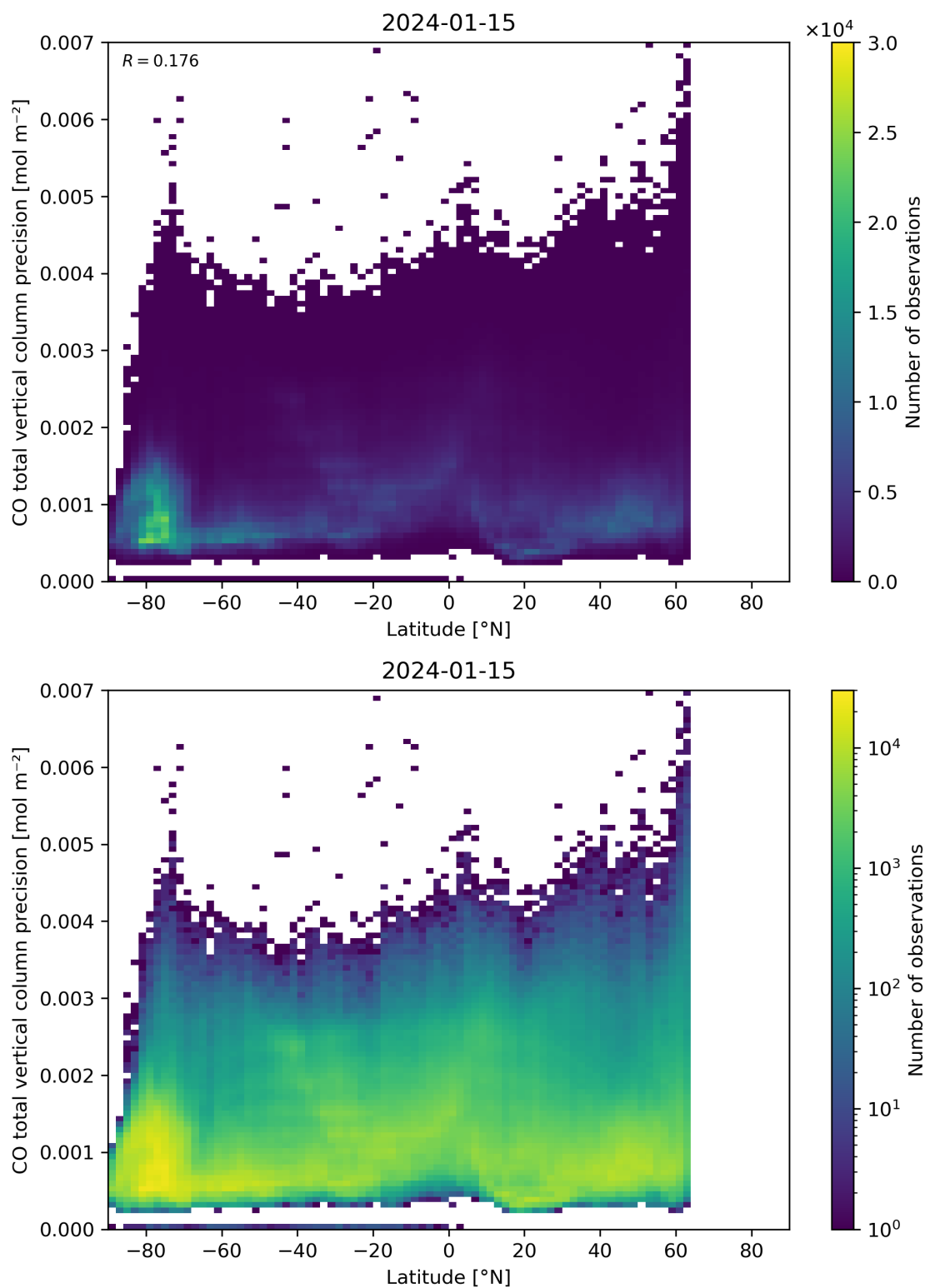
Figure 53: Scatter density plot of “Latitude” against “CO total vertical column precision” for 2024-01-15 to 2024-01-16.
