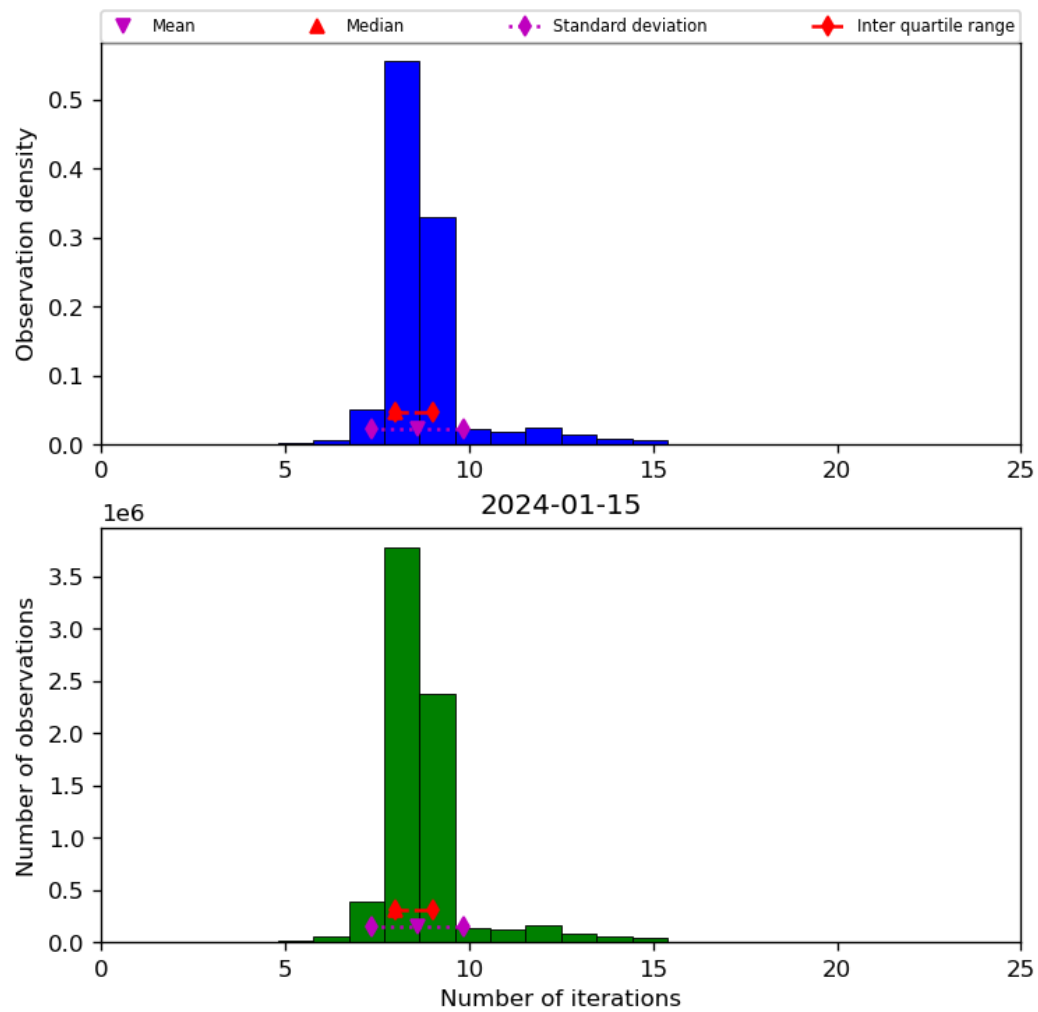
Figure 24: Histogram of “Number of iterations” for 2024-01-15 to 2024-01-16
