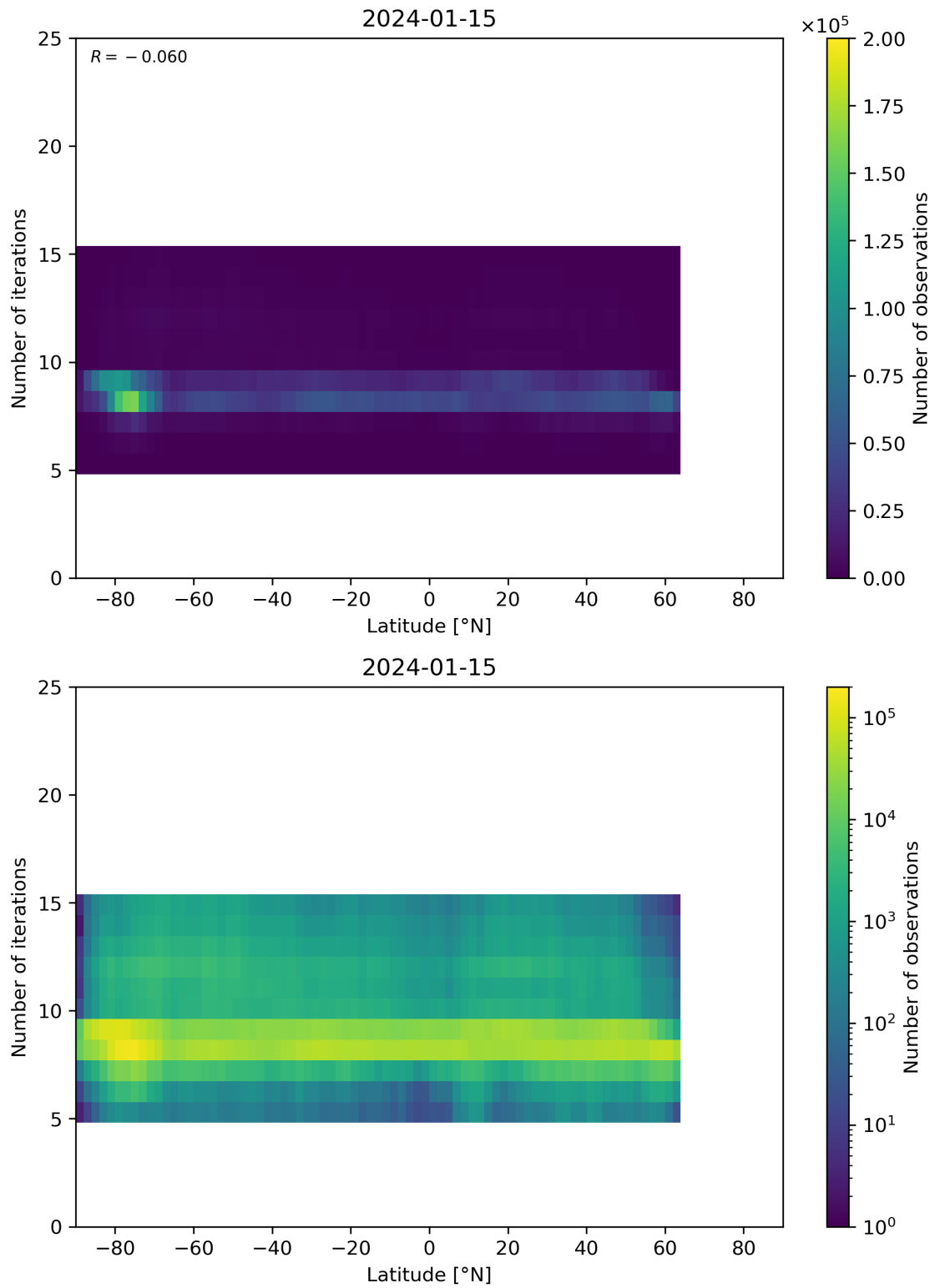
Figure 56: Scatter density plot of “Latitude” against “Number of iterations” for 2024-01-15 to 2024-01-16.
