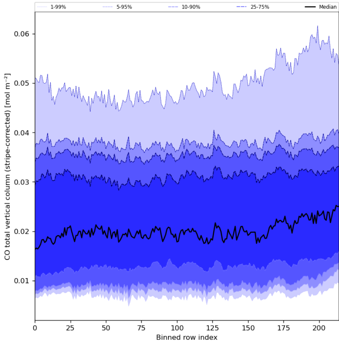
Figure 27: Along track statistics of “CO total vertical column (stripe-corrected)” for 2024-01-15 to 2024-01-16
