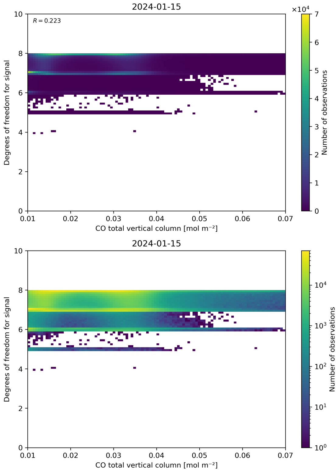
Figure 41: Scatter density plot of “CO total vertical column” against “Degrees of freedom for signal” for 2024-01-15 to 2024-01-16.
