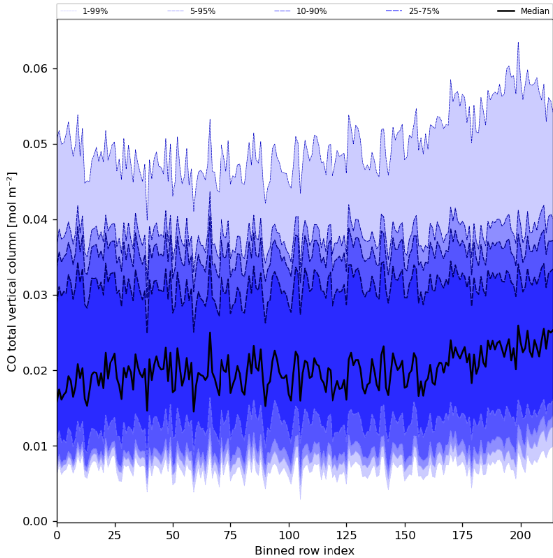
Figure 26: Along track statistics of “CO total vertical column” for 2024-01-15 to 2024-01-16
