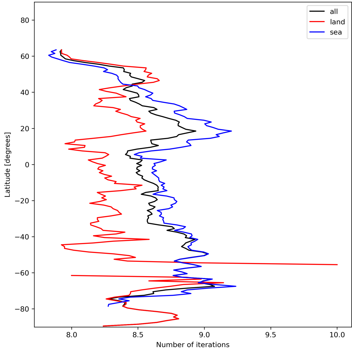
Figure 16: Zonal average of “Number of iterations” for 2024-01-15 to 2024-01-16.
