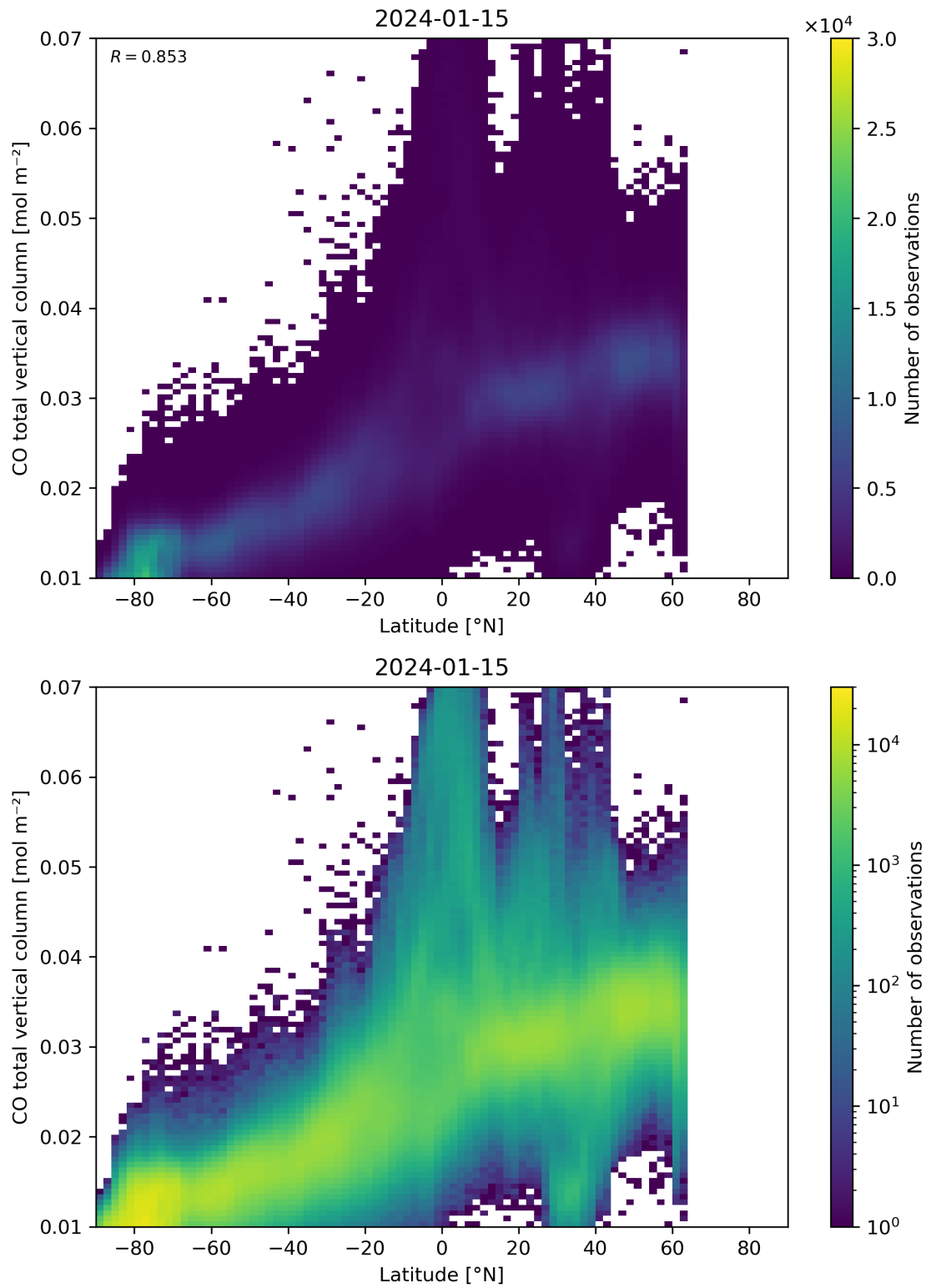
Figure 51: Scatter density plot of “Latitude” against “CO total vertical column” for 2024-01-15 to 2024-01-16.
