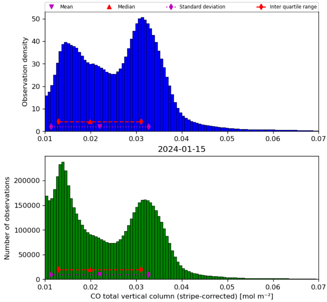
Figure 19: Histogram of “CO total vertical column (stripe-corrected)” for 2024-01-15 to 2024-01-16
