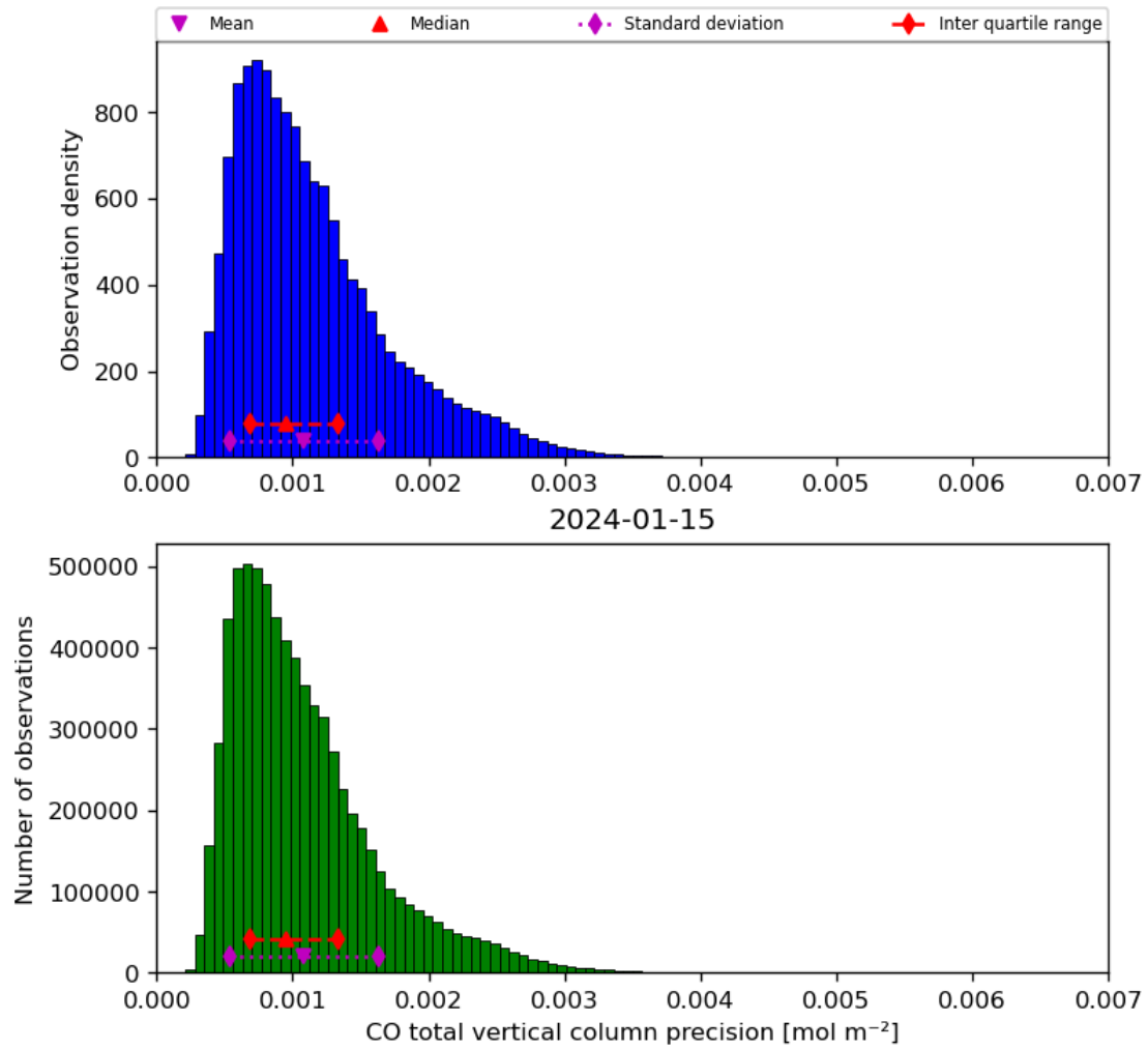
Figure 20: Histogram of “CO total vertical column precision” for 2024-01-15 to 2024-01-16
