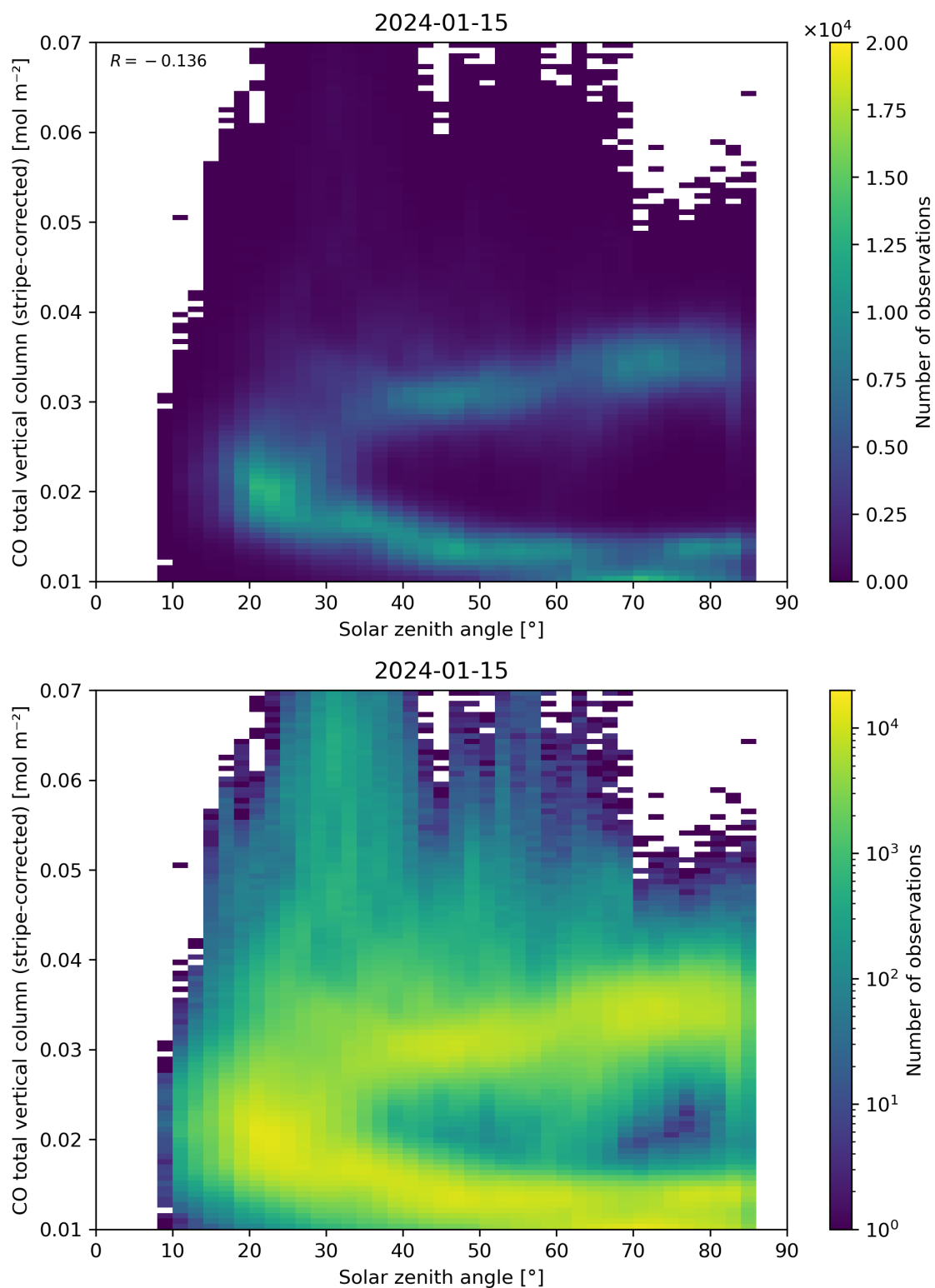
Figure 62: Scatter density plot of “Solar zenith angle” against “CO total vertical column (stripe-corrected)” for 2024-01-15 to 2024-01-16.
