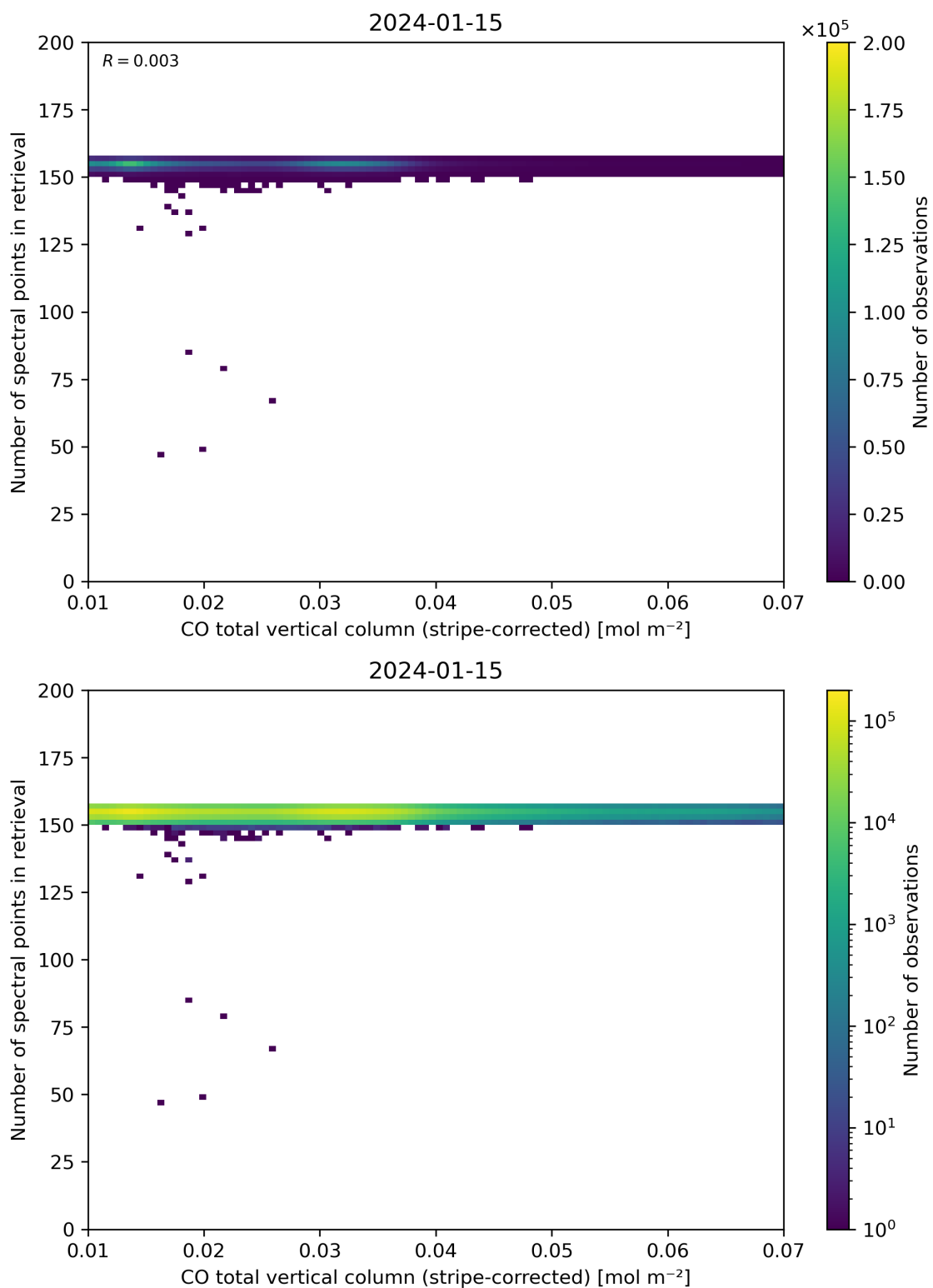
Figure 40: Scatter density plot of “CO total vertical column (stripe-corrected)” against “Number of spectral points in retrieval” for 2024-01-15 to 2024-01-16.
