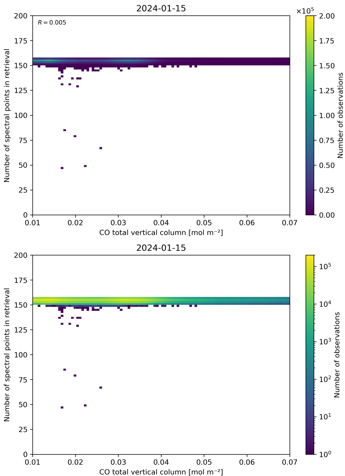
Figure 43: Scatter density plot of “CO total vertical column” against “Number of spectral points in retrieval” for 2024-01-15 to 2024-01-16.
