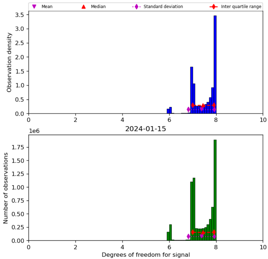
Figure 23: Histogram of “Degrees of freedom for signal” for 2024-01-15 to 2024-01-16
