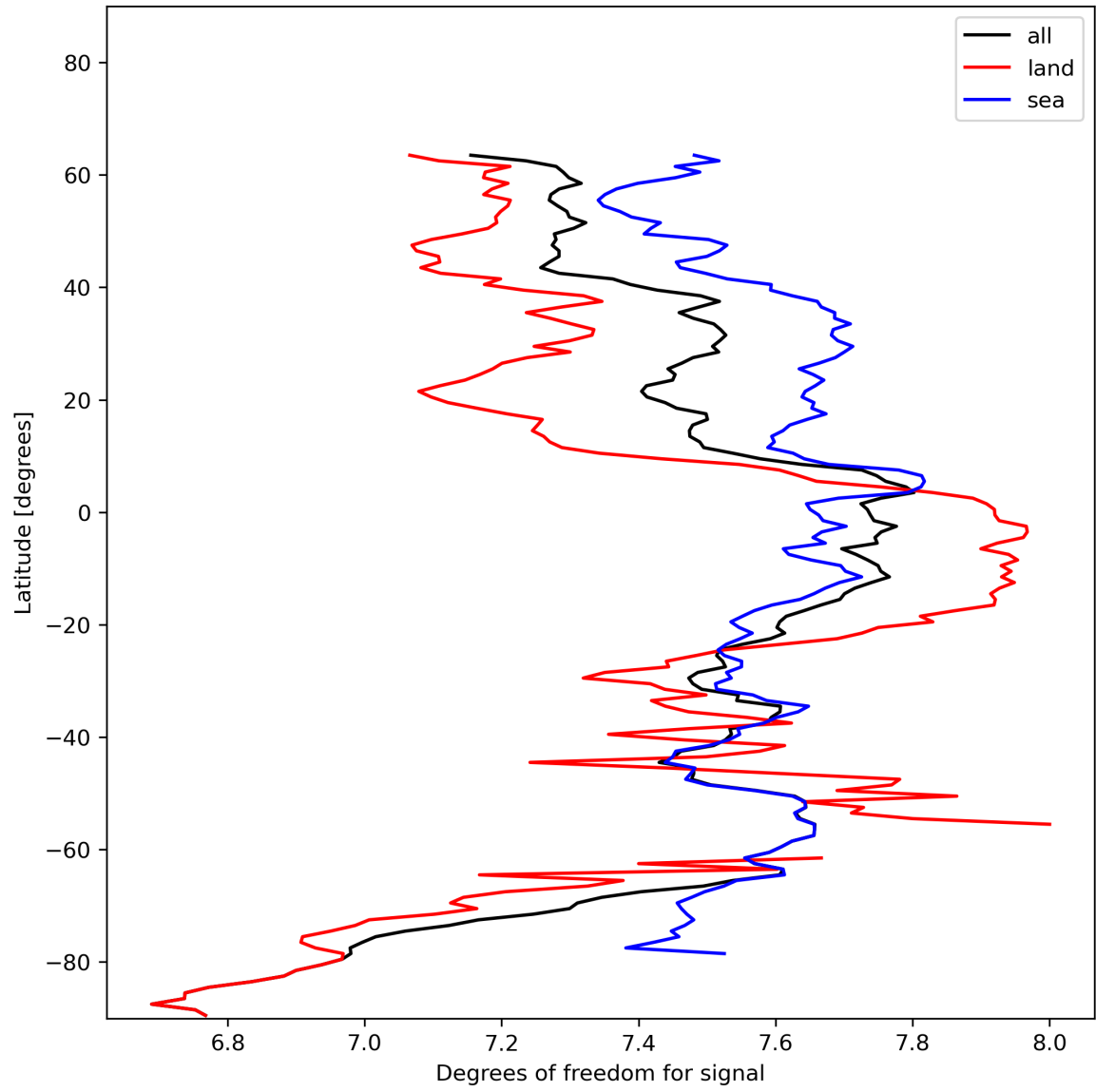
Figure 15: Zonal average of “Degrees of freedom for signal” for 2024-01-15 to 2024-01-16.
