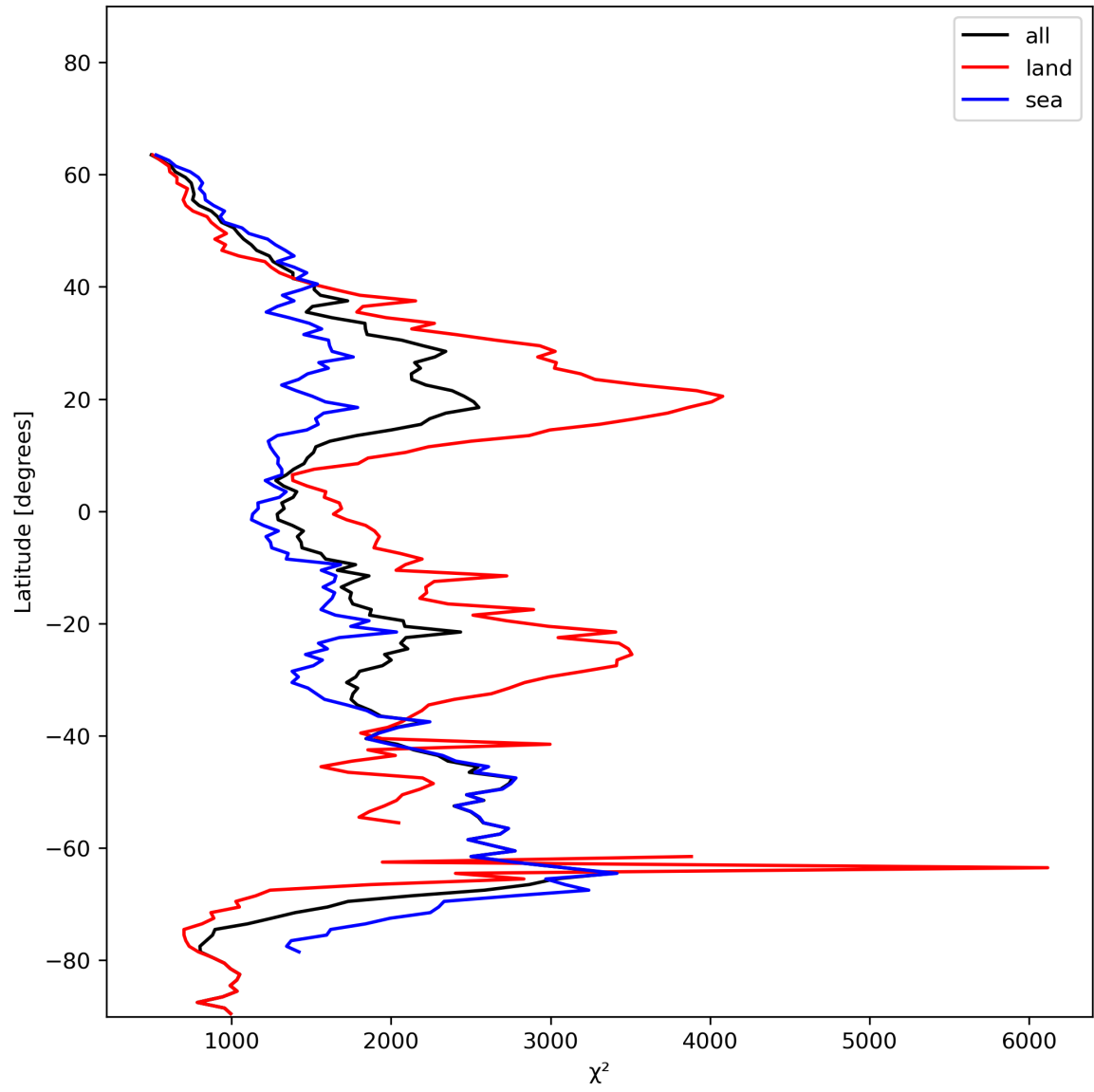
Figure 14: Zonal average of “ \chi^2 ” for 2024-01-15 to 2024-01-16.
