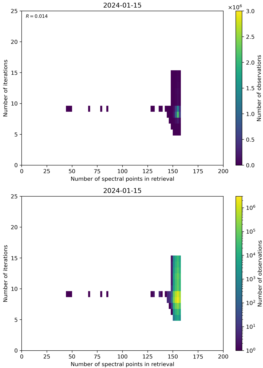
Figure 60: Scatter density plot of “Number of spectral points in retrieval” against “Number of iterations” for 2024-01-15 to 2024-01-16.
