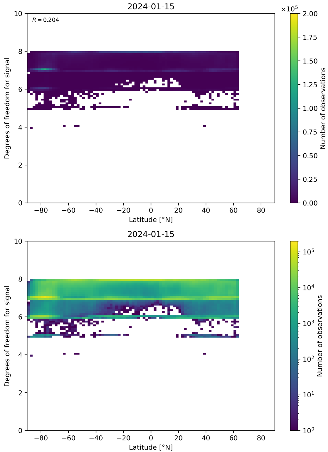
Figure 55: Scatter density plot of “Latitude” against “Degrees of freedom for signal” for 2024-01-15 to 2024-01-16.
