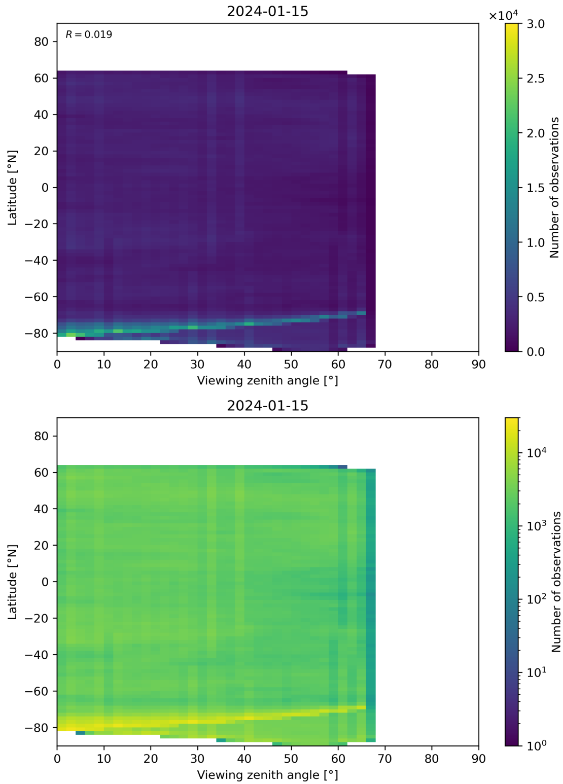
Figure 74: Scatter density plot of “Viewing zenith angle” against “Latitude” for 2024-01-15 to 2024-01-16.
