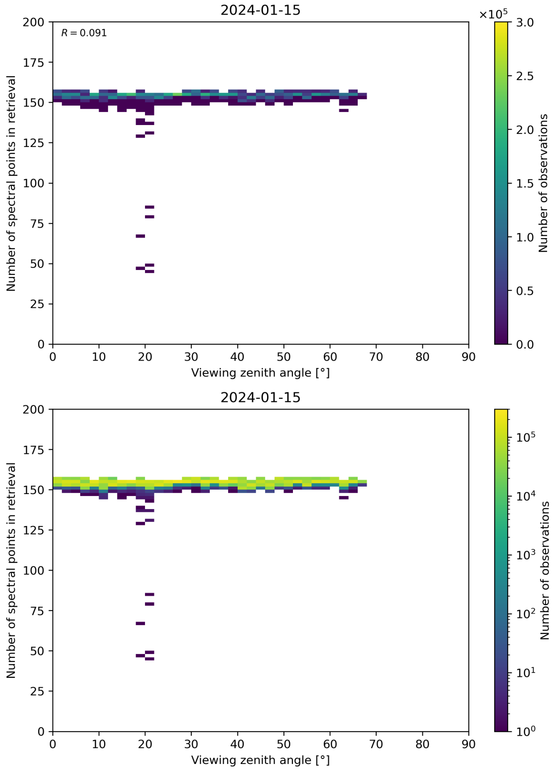
Figure 76: Scatter density plot of “Viewing zenith angle” against “Number of spectral points in retrieval” for 2024-01-15 to 2024-01-16.
