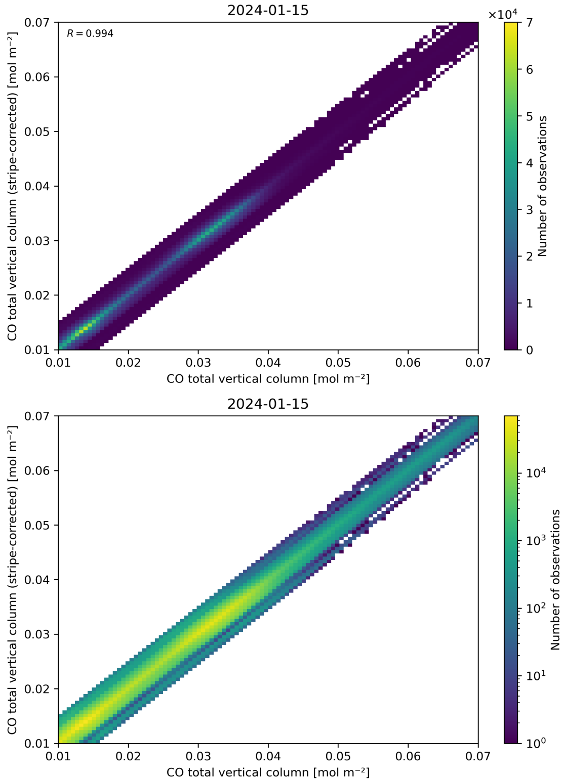
Figure 33: Scatter density plot of “CO total vertical column” against “CO total vertical column (stripe-corrected)” for 2024-01-15 to 2024-01-16.
