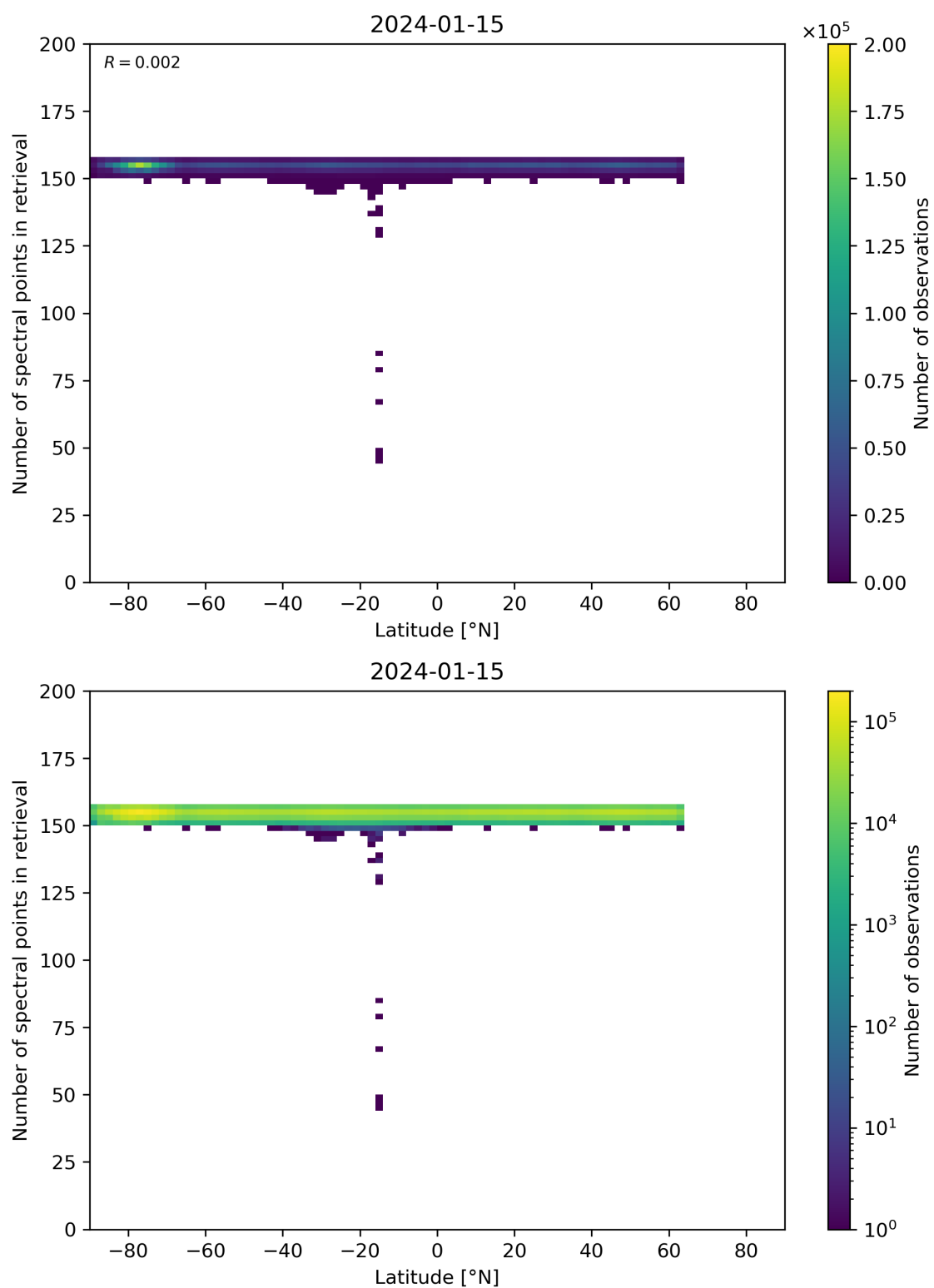
Figure 57: Scatter density plot of “Latitude” against “Number of spectral points in retrieval” for 2024-01-15 to 2024-01-16.
