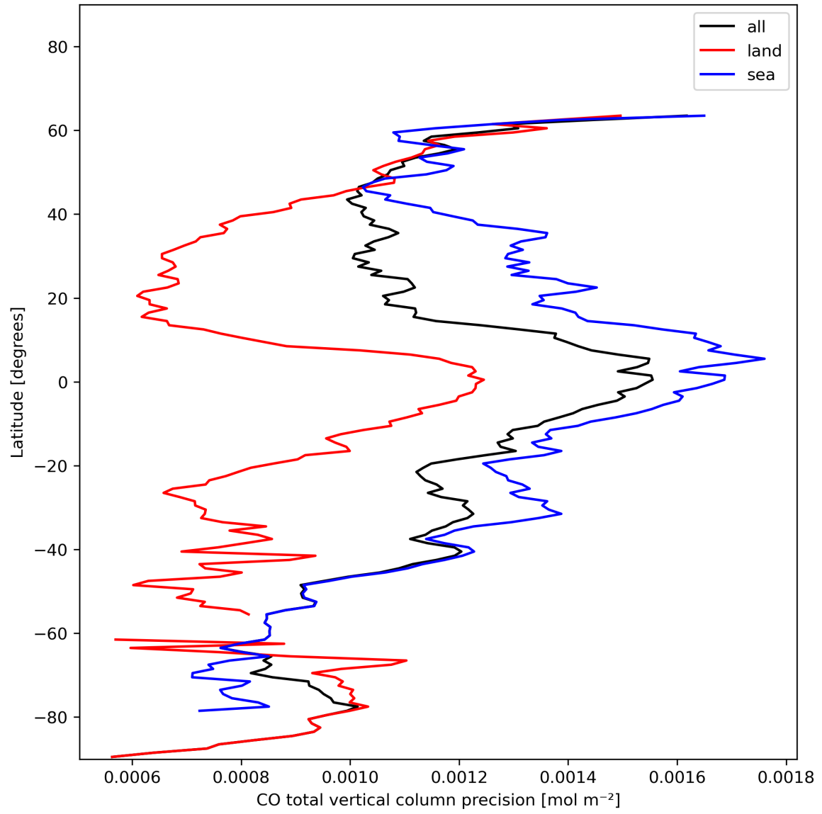
Figure 12: Zonal average of “CO total vertical column precision” for 2024-01-15 to 2024-01-16.
