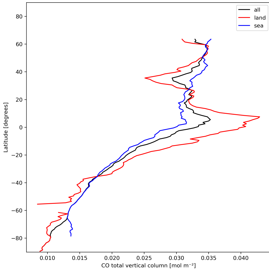
Figure 10: Zonal average of “CO total vertical column” for 2024-01-15 to 2024-01-16.
