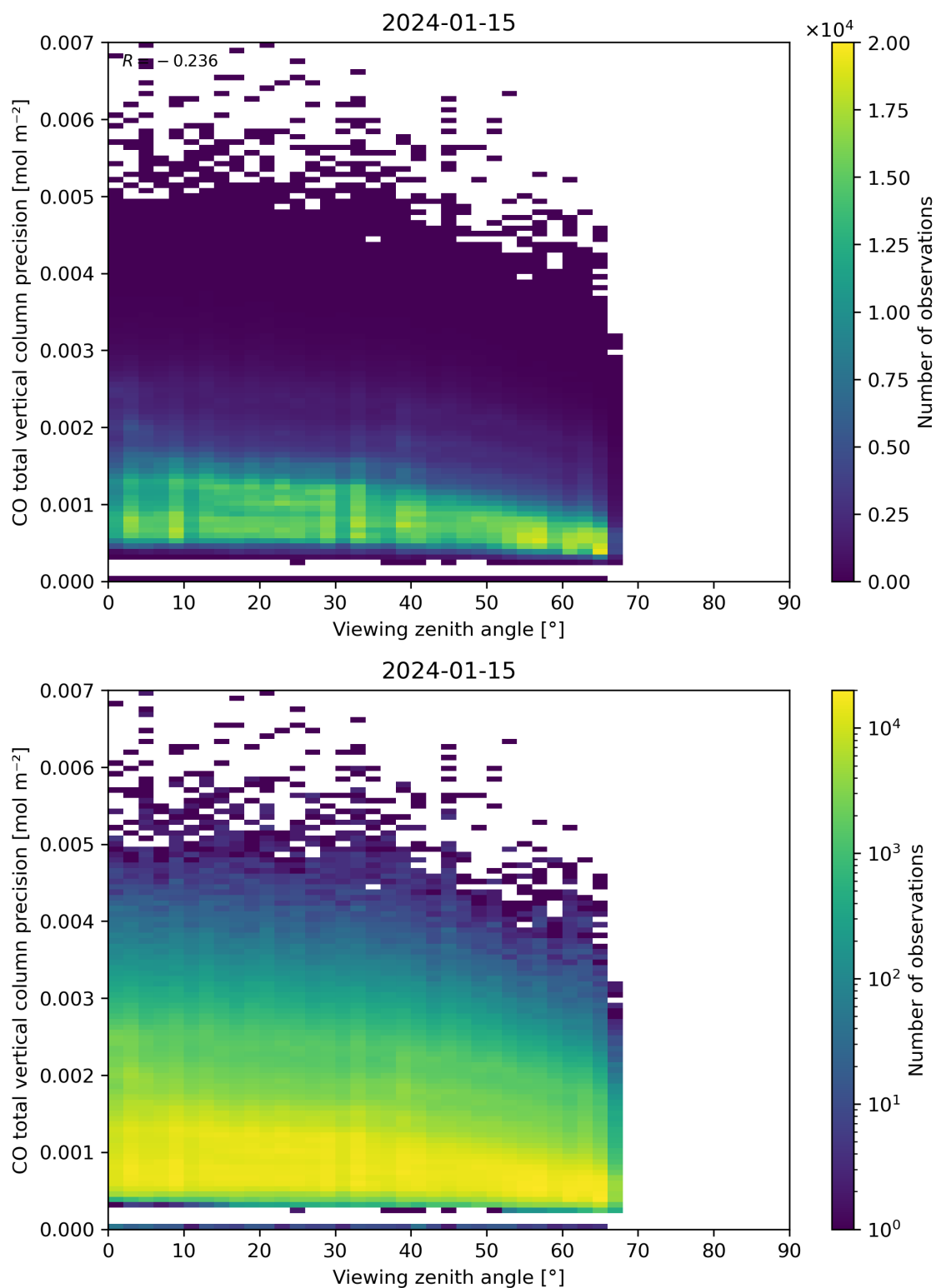
Figure 71: Scatter density plot of “Viewing zenith angle” against “CO total vertical column precision” for 2024-01-15 to 2024-01-16.
