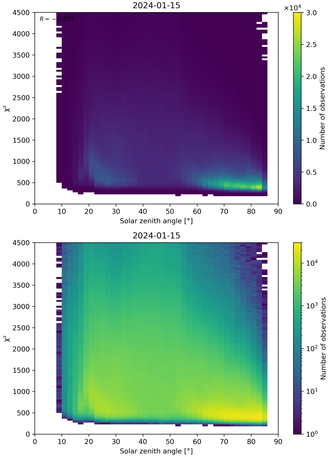
Figure 64: Scatter density plot of “Solar zenith angle” against “ \chi^2 ” for 2024-01-15 to 2024-01-16.
