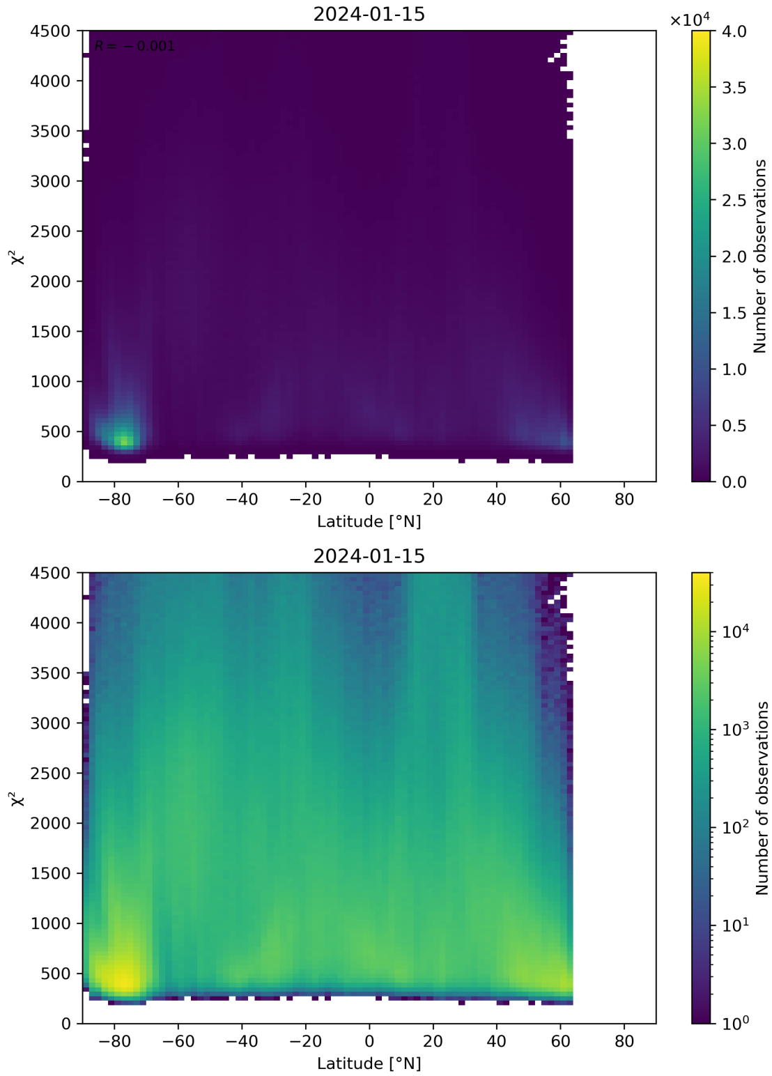
Figure 54: Scatter density plot of “Latitude” against “ \chi^2 ” for 2024-01-15 to 2024-01-16.
