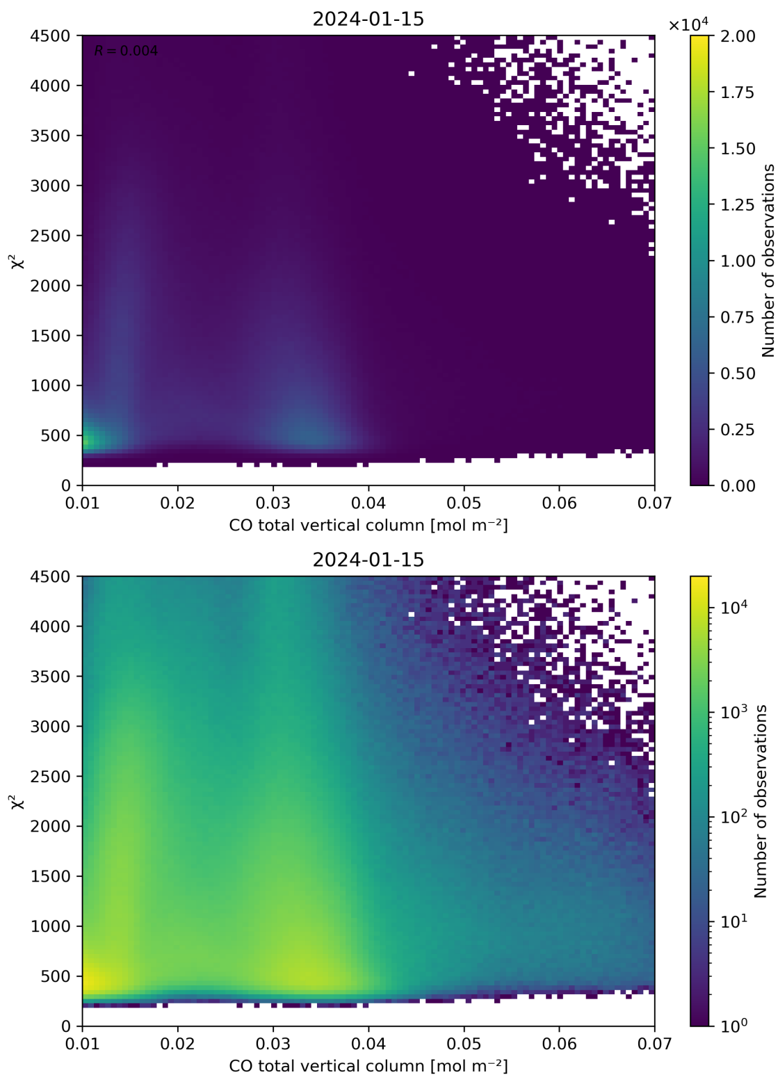
Figure 35: Scatter density plot of “CO total vertical column” against “ \chi^2 ” for 2024-01-15 to 2024-01-16.
