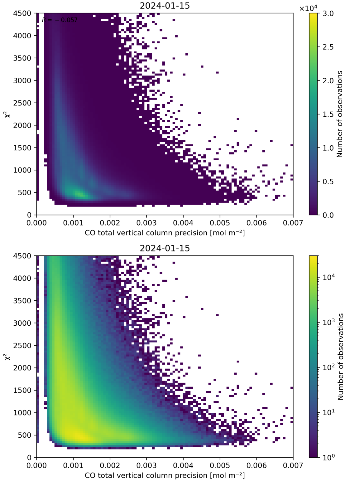
Figure 44: Scatter density plot of “CO total vertical column precision” against “ \chi^2 ” for 2024-01-15 to 2024-01-16.
