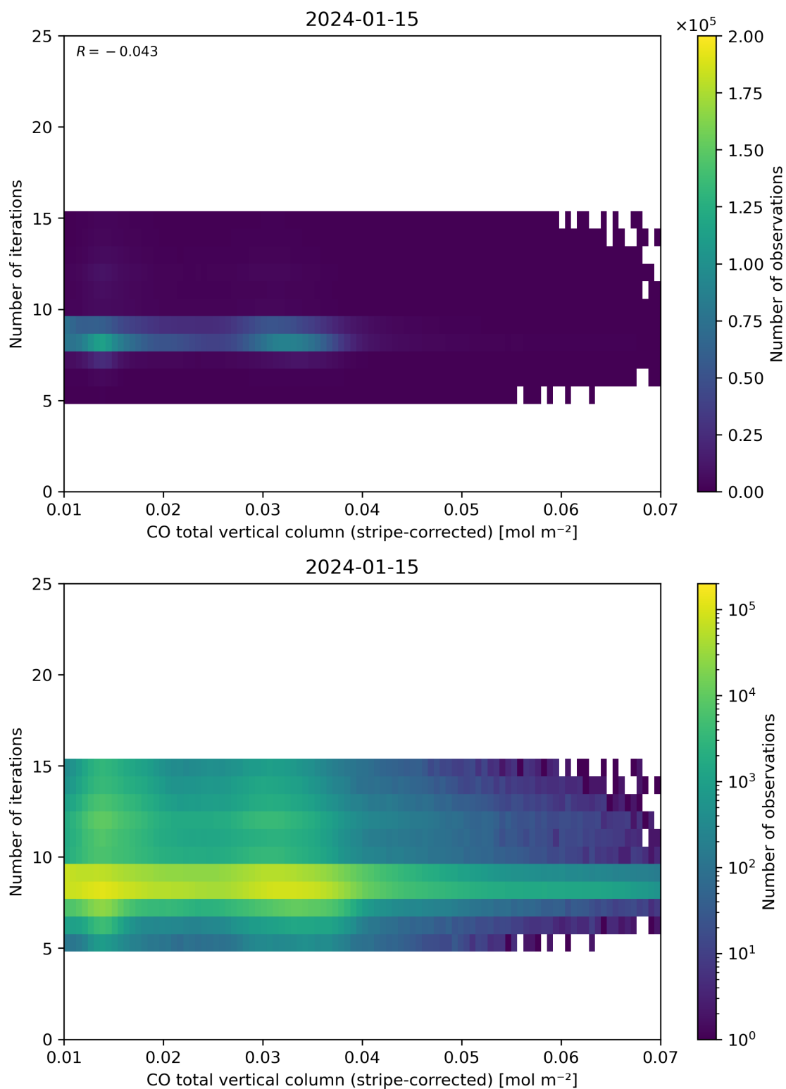
Figure 39: Scatter density plot of “CO total vertical column (stripe-corrected)” against “Number of iterations” for 2024-01-15 to 2024-01-16.
