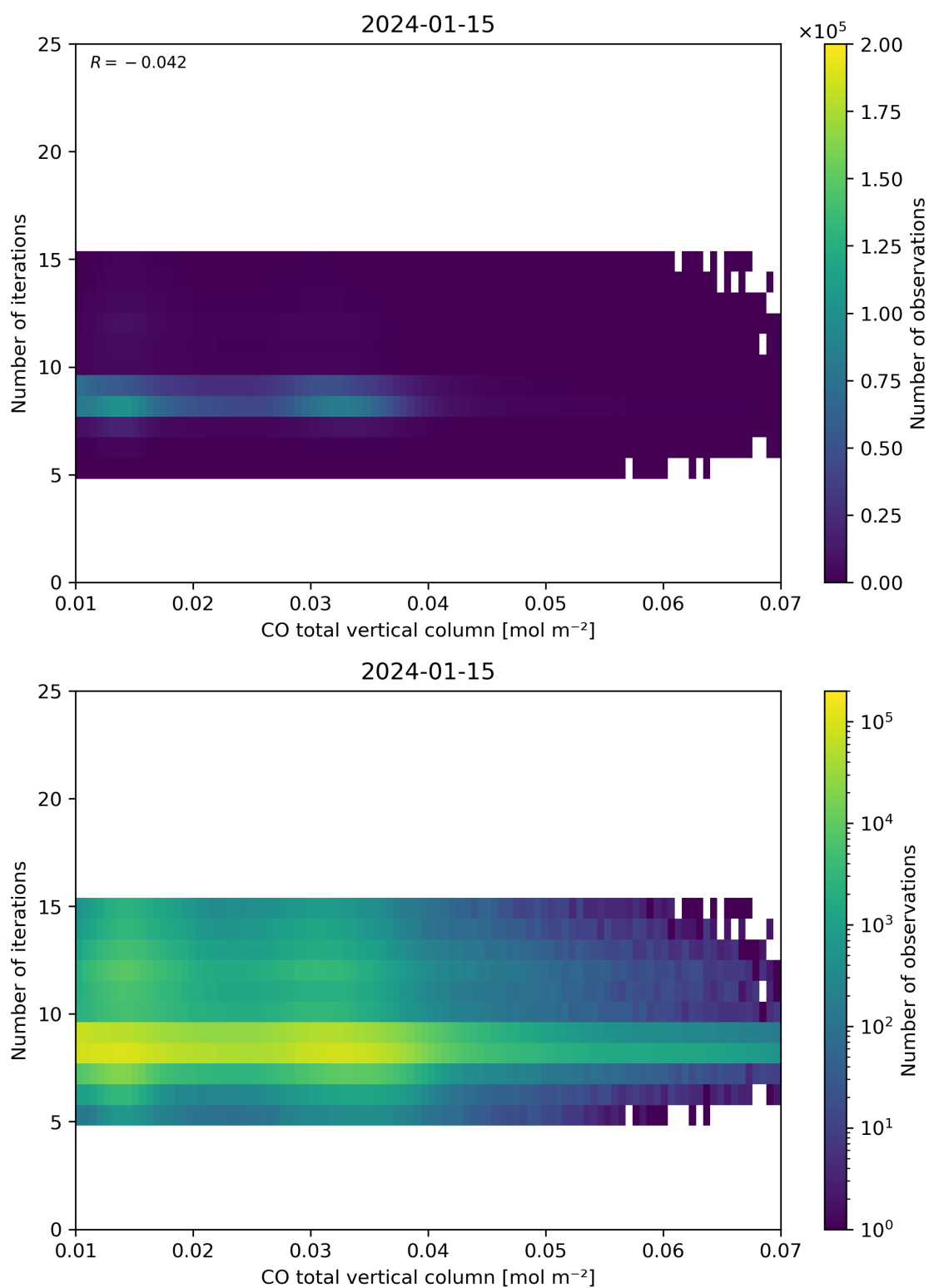
Figure 42: Scatter density plot of “CO total vertical column” against “Number of iterations” for 2024-01-15 to 2024-01-16.
