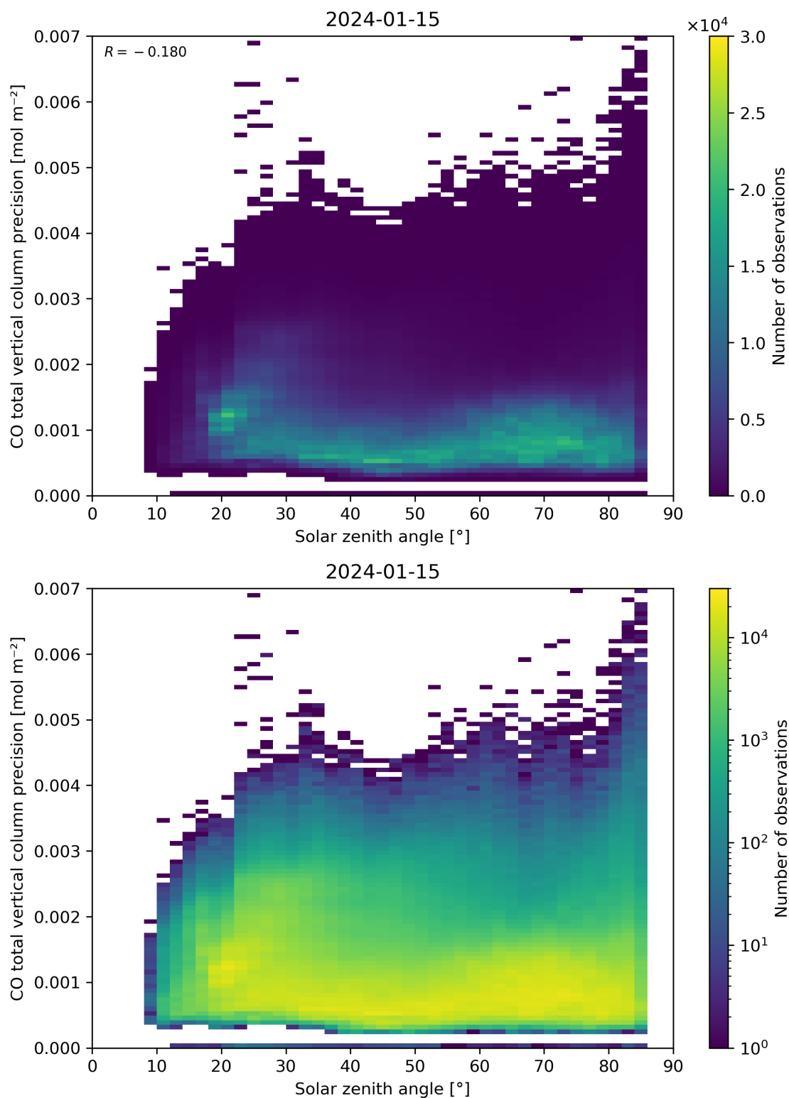
Figure 63: Scatter density plot of “Solar zenith angle” against “CO total vertical column precision” for 2024-01-15 to 2024-01-16.
