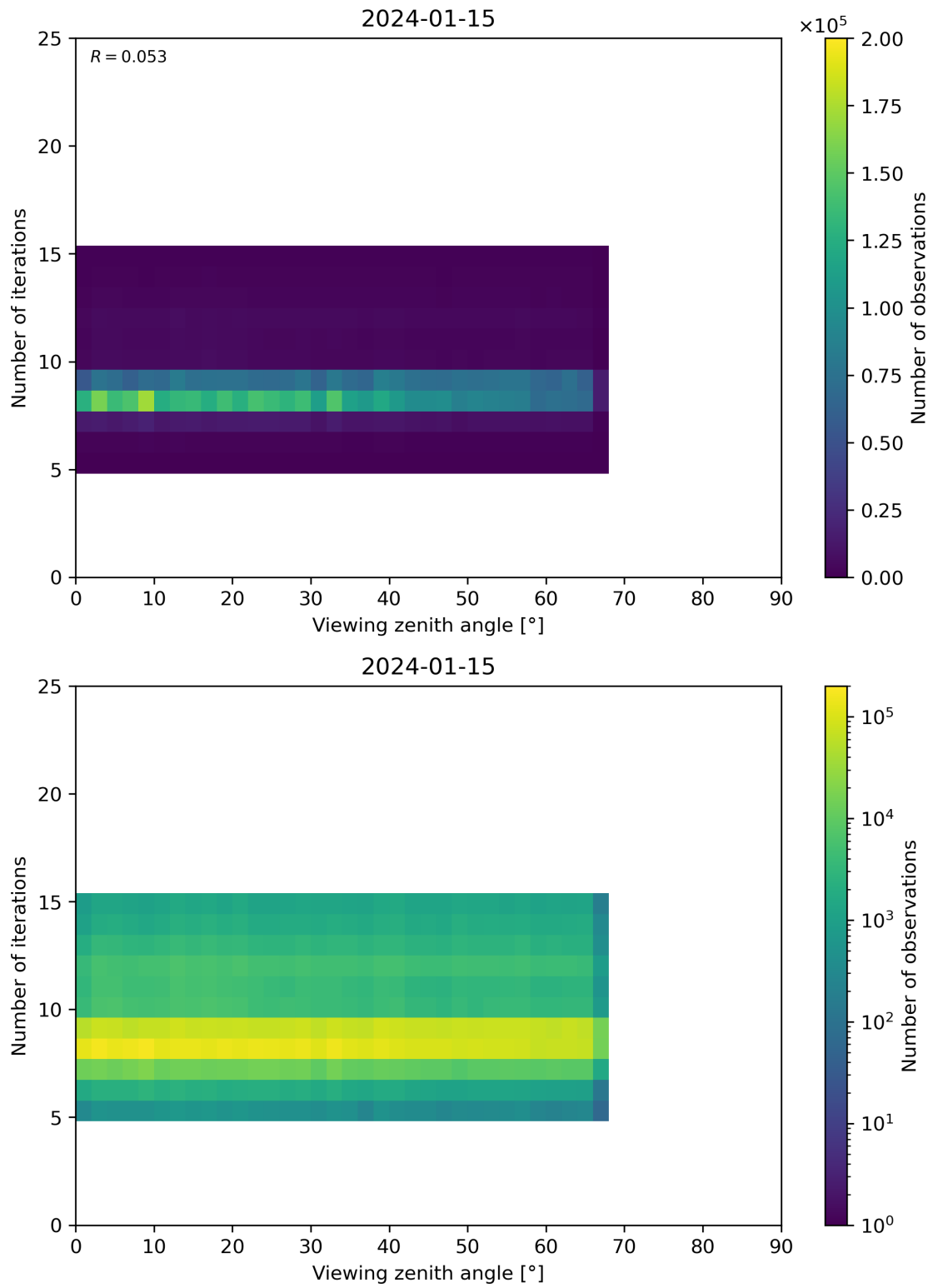
Figure 75: Scatter density plot of “Viewing zenith angle” against “Number of iterations” for 2024-01-15 to 2024-01-16.
