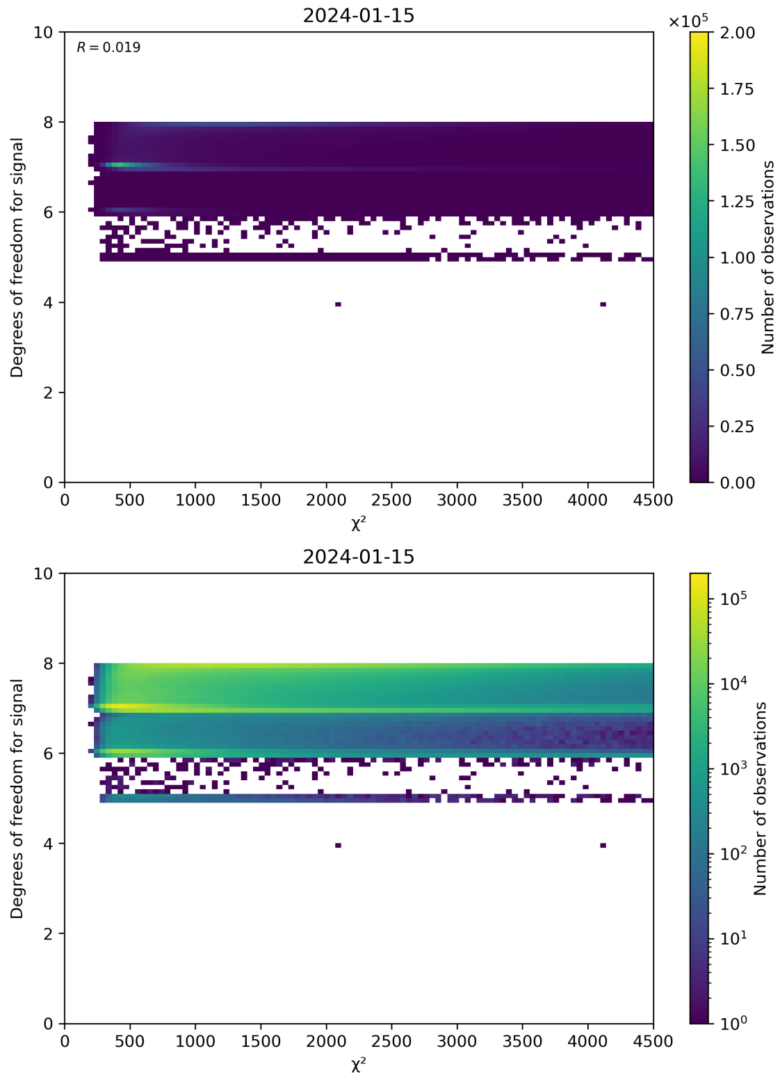
Figure 48: Scatter density plot of “ \chi^2 ” against “Degrees of freedom for signal” for 2024-01-15 to 2024-01-16.
