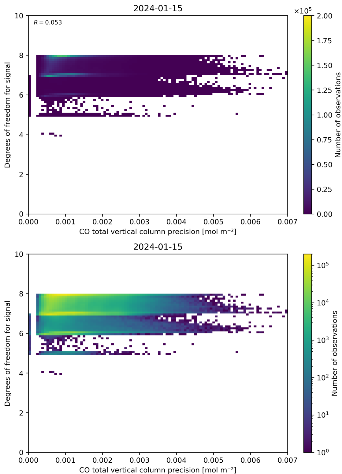
Figure 45: Scatter density plot of “CO total vertical column precision” against “Degrees of freedom for signal” for 2024-01-15 to 2024-01-16.
