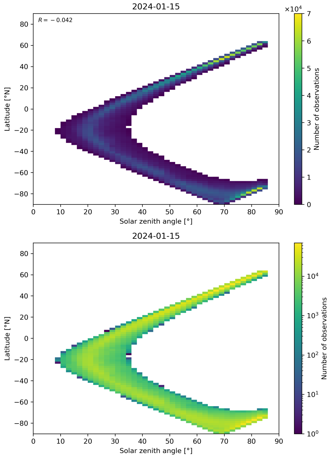
Figure 66: Scatter density plot of “Solar zenith angle” against “Latitude” for 2024-01-15 to 2024-01-16.
