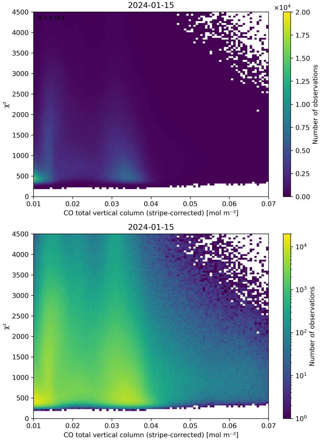
Figure 37: Scatter density plot of “CO total vertical column (stripe-corrected)” against “ \chi^2 ” for 2024-01-15 to 2024-01-16.
