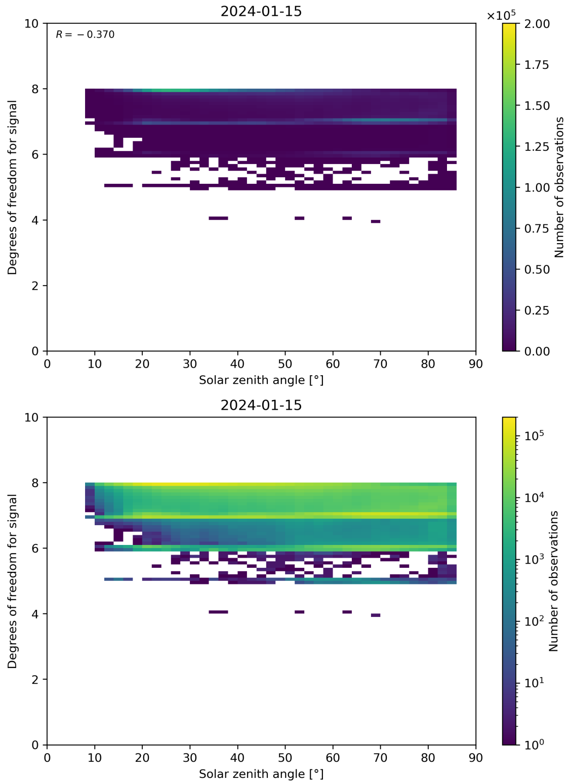
Figure 65: Scatter density plot of “Solar zenith angle” against “Degrees of freedom for signal” for 2024-01-15 to 2024-01-16.
