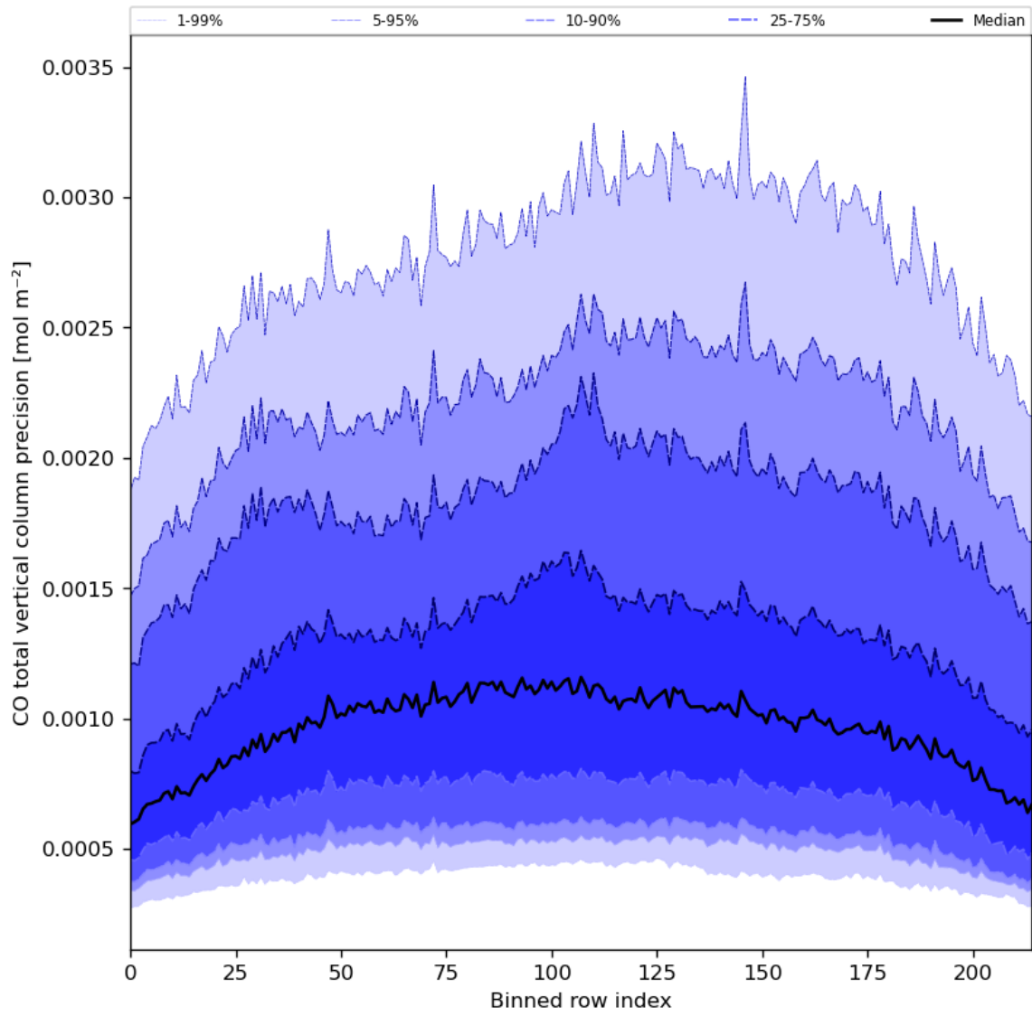
Figure 28: Along track statistics of “CO total vertical column precision” for 2024-01-15 to 2024-01-16
