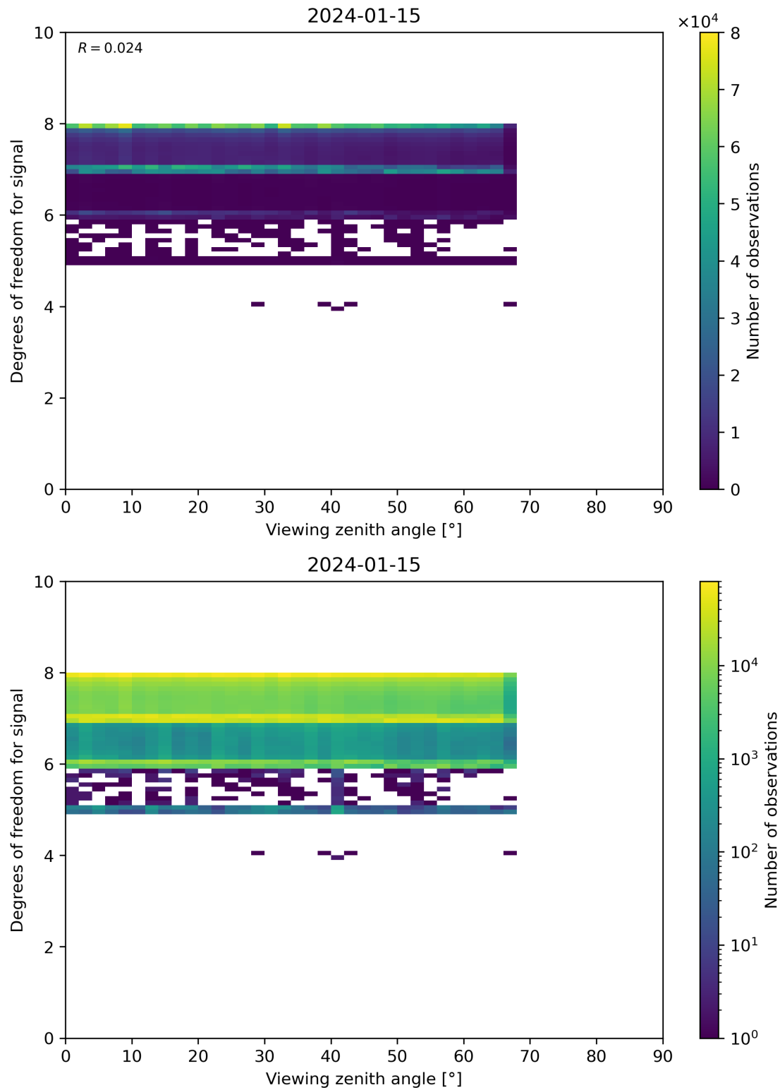
Figure 73: Scatter density plot of “Viewing zenith angle” against “Degrees of freedom for signal” for 2024-01-15 to 2024-01-16.
