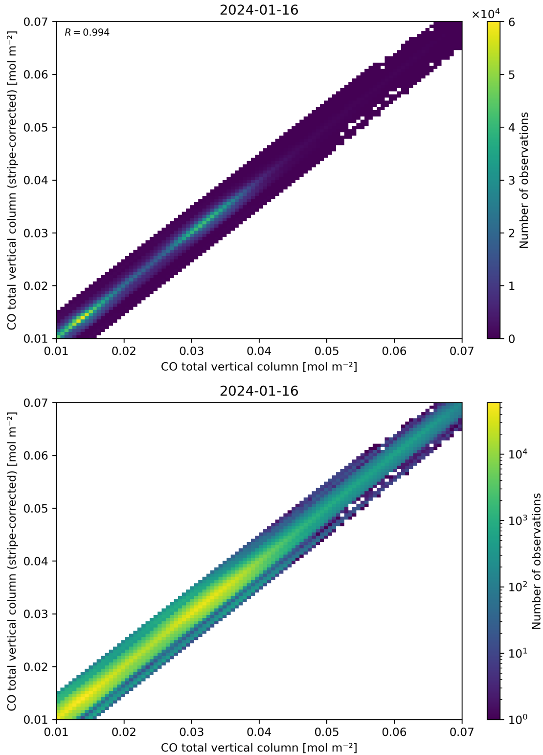
Figure 33: Scatter density plot of “CO total vertical column” against “CO total vertical column (stripe-corrected)” for 2024-01-15 to 2024-01-17.
