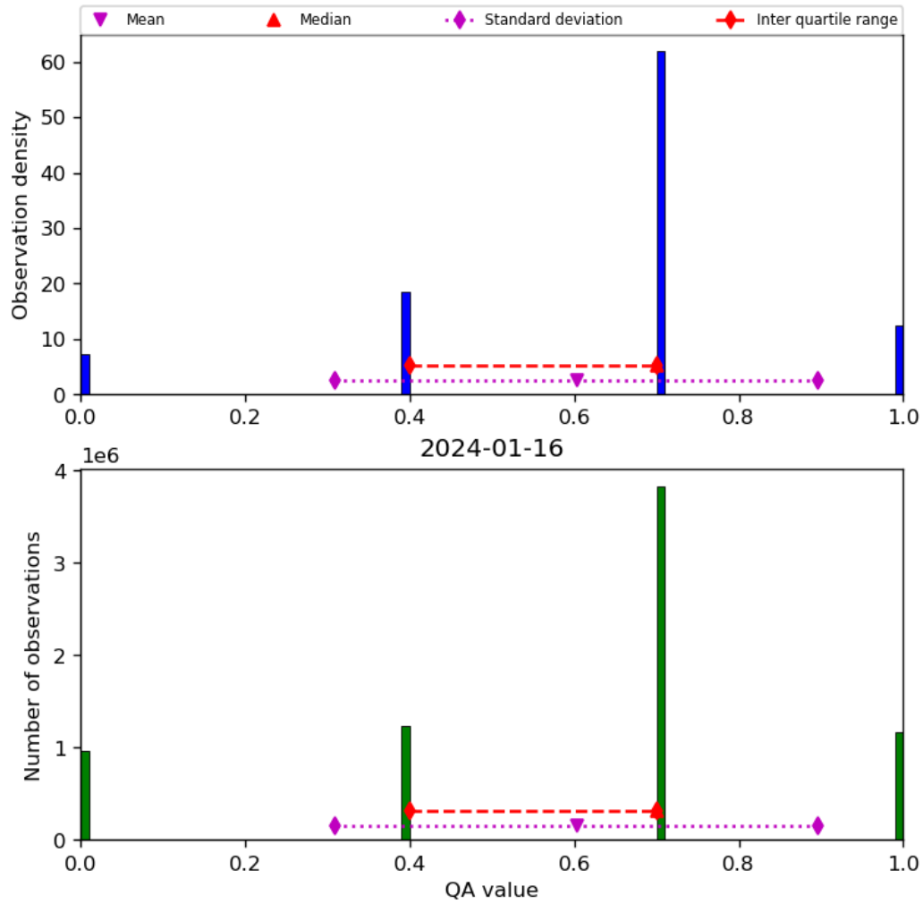
Figure 17: Histogram of “QA value” for 2024-01-15 to 2024-01-17
