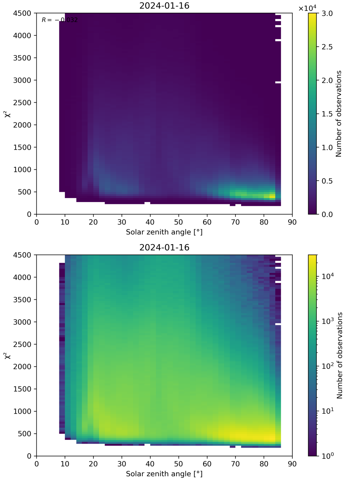
Figure 64: Scatter density plot of “Solar zenith angle” against “ \chi^2 ” for 2024-01-15 to 2024-01-17.
