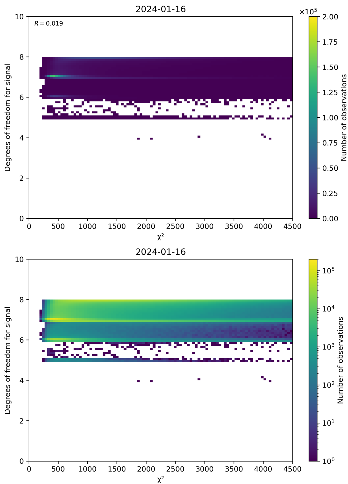
Figure 48: Scatter density plot of “ \chi^2 ” against “Degrees of freedom for signal” for 2024-01-15 to 2024-01-17.
