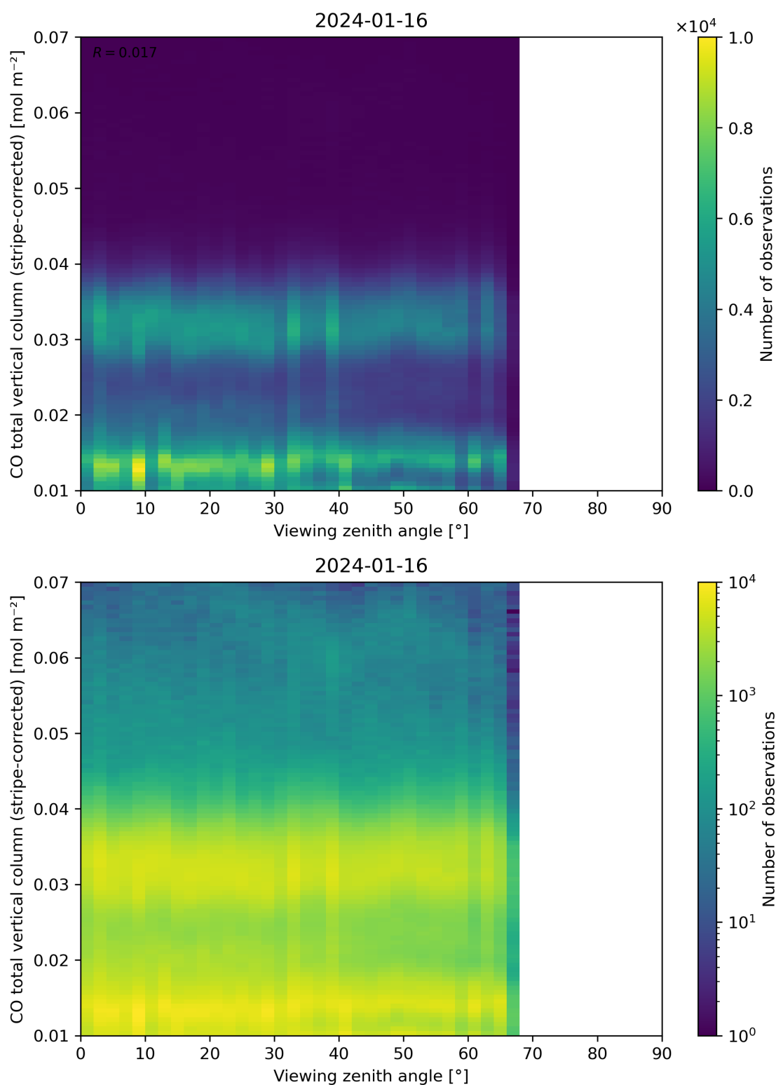
Figure 70: Scatter density plot of “Viewing zenith angle” against “CO total vertical column (stripe-corrected)” for 2024-01-15 to 2024-01-17.
