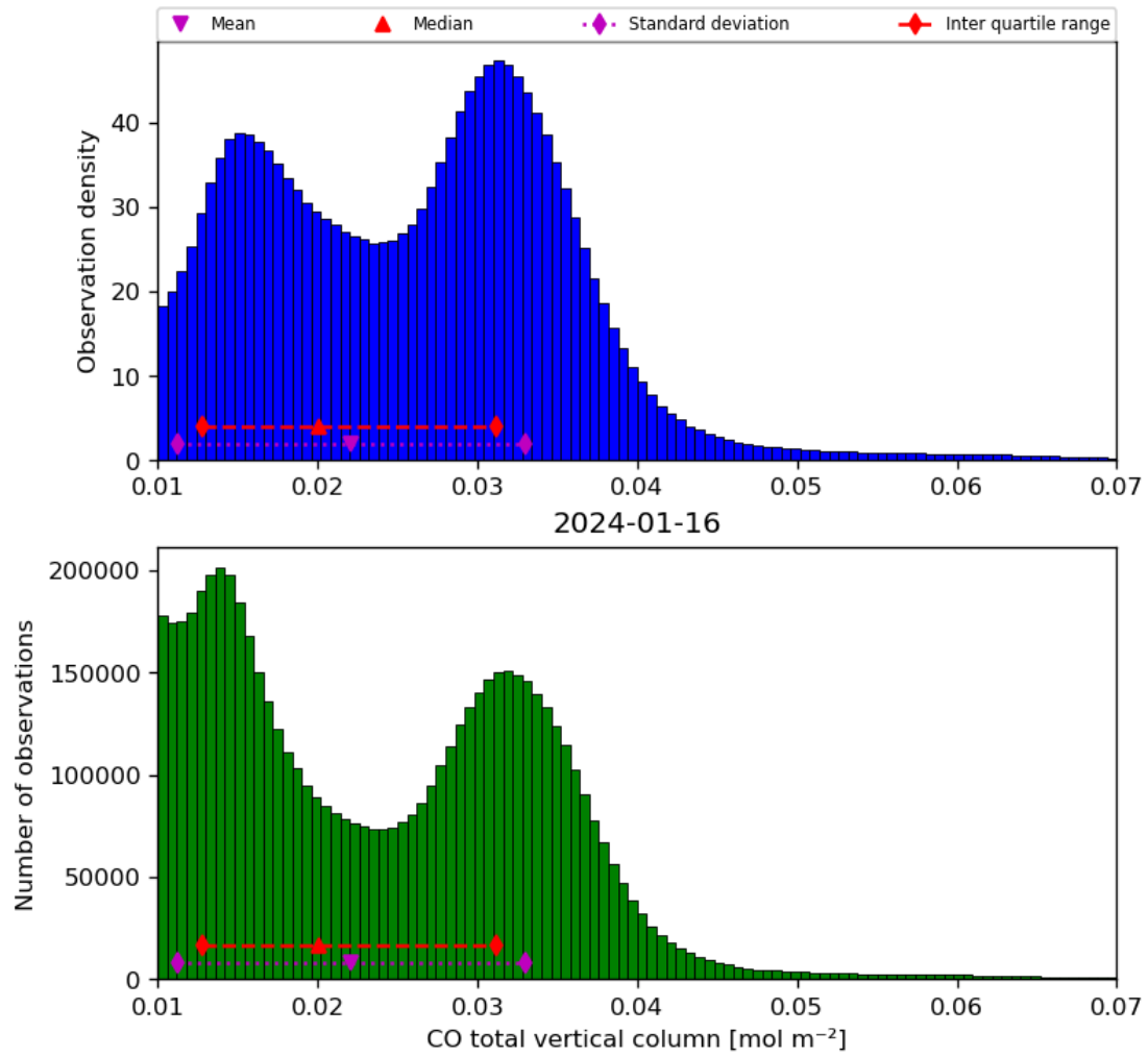
Figure 18: Histogram of “CO total vertical column” for 2024-01-15 to 2024-01-17
