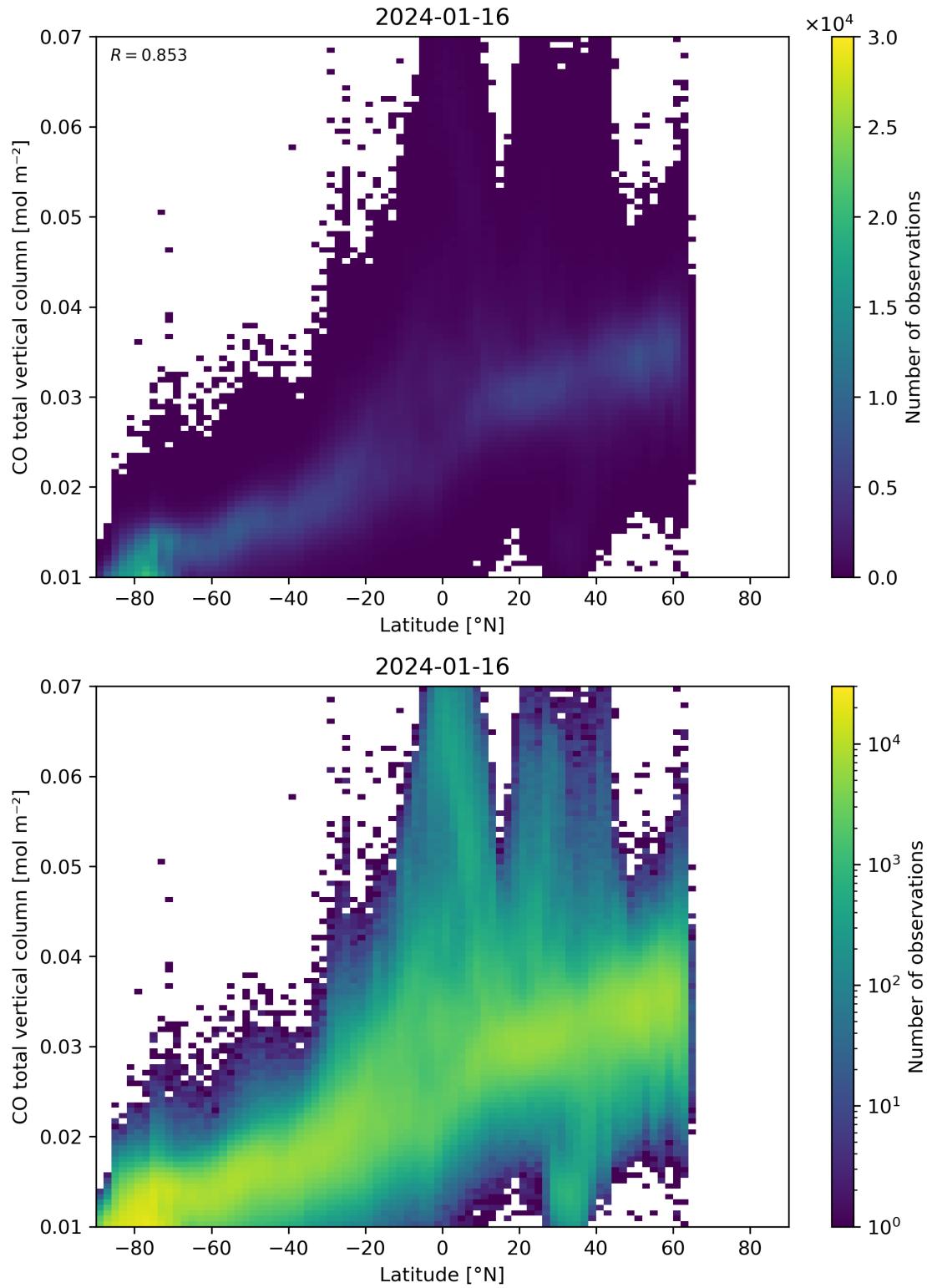
Figure 51: Scatter density plot of “Latitude” against “CO total vertical column” for 2024-01-15 to 2024-01-17.
