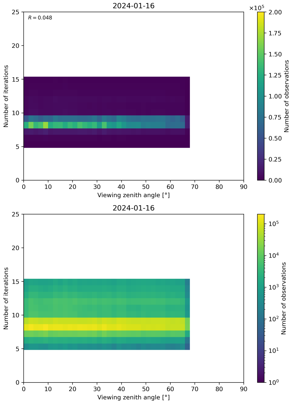
Figure 75: Scatter density plot of “Viewing zenith angle” against “Number of iterations” for 2024-01-15 to 2024-01-17.
