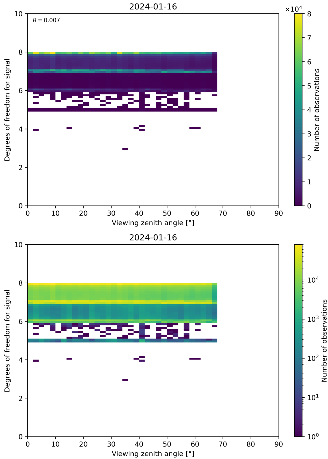
Figure 73: Scatter density plot of “Viewing zenith angle” against “Degrees of freedom for signal” for 2024-01-15 to 2024-01-17.
