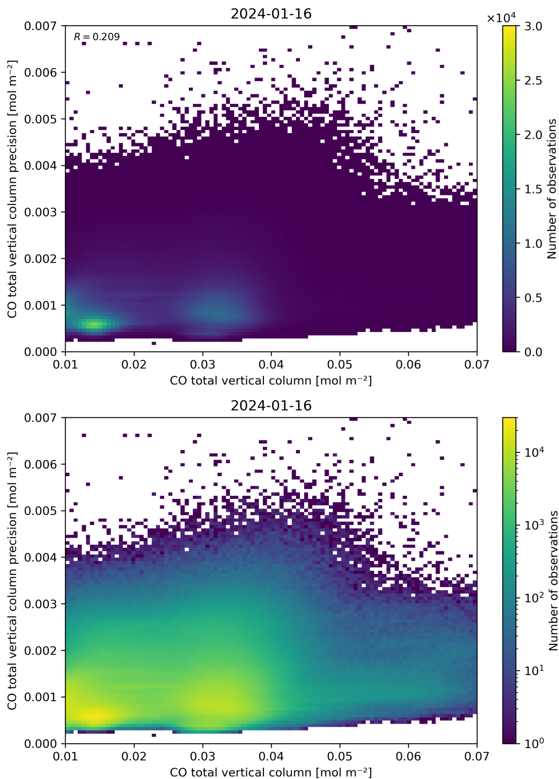
Figure 34: Scatter density plot of “CO total vertical column” against “CO total vertical column precision” for 2024-01-15 to 2024-01-17.
