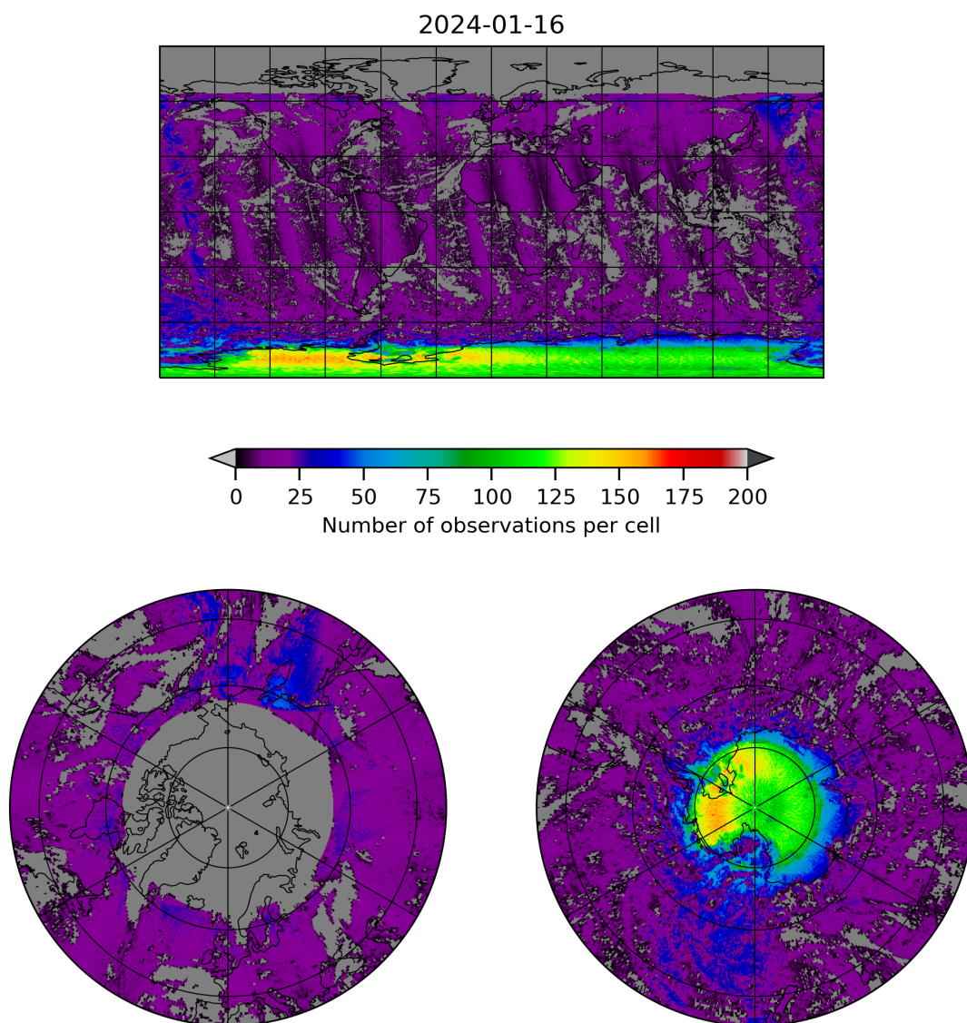
Figure 8: Map of the number of observations for 2024-01-15 to 2024-01-17
