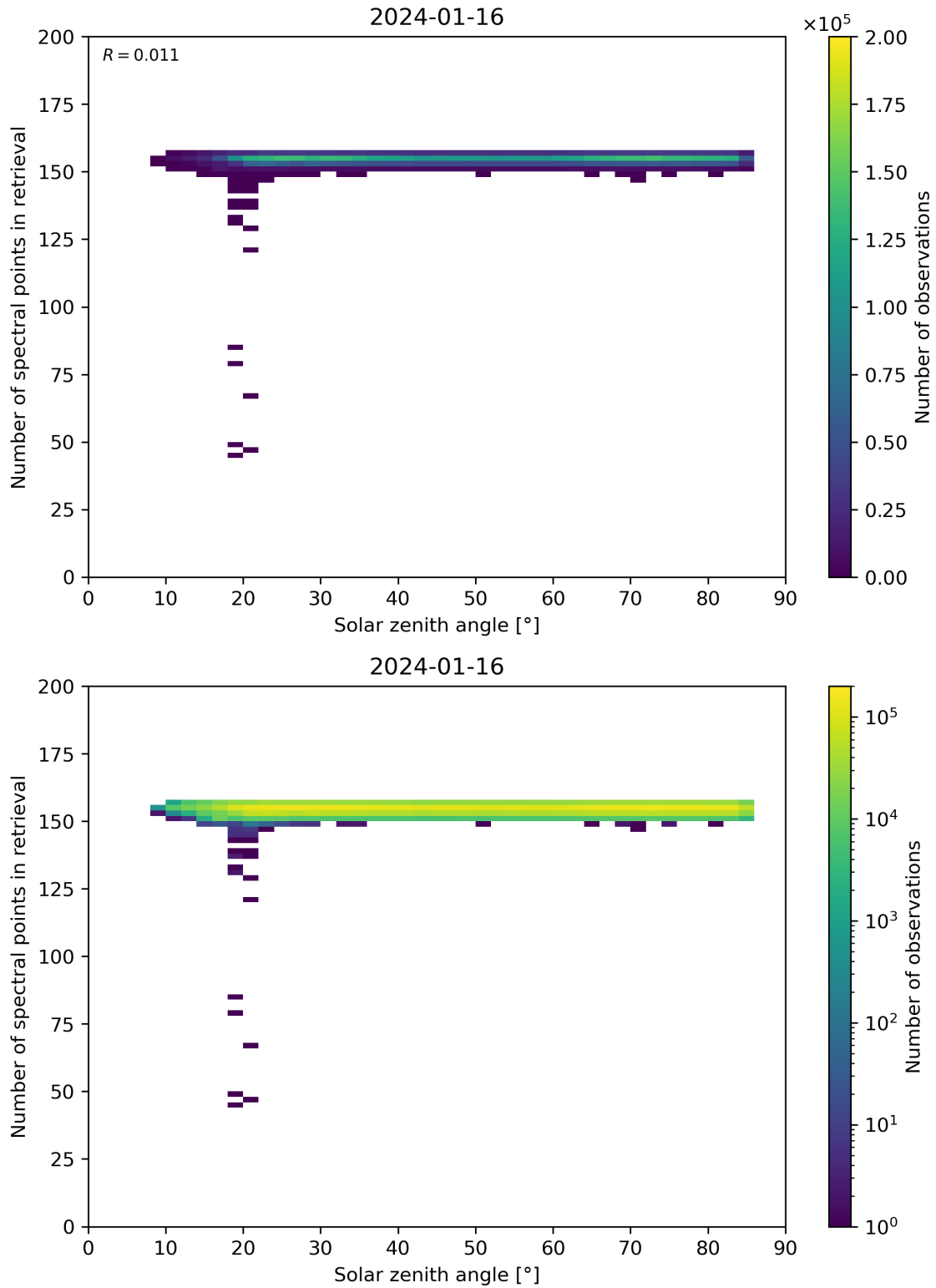
Figure 68: Scatter density plot of “Solar zenith angle” against “Number of spectral points in retrieval” for 2024-01-15 to 2024-01-17.
