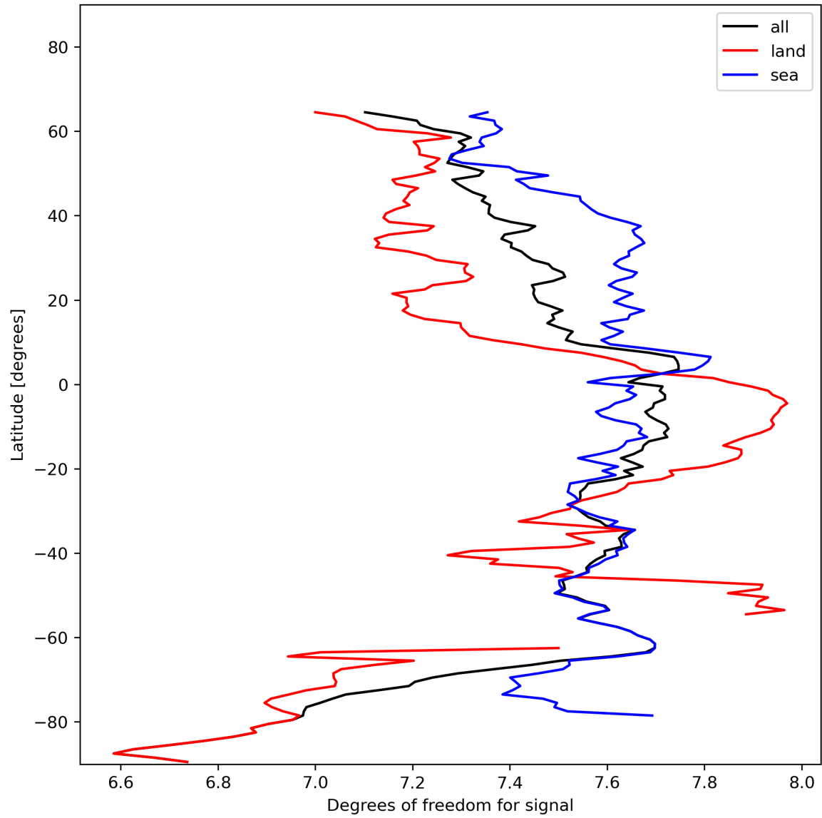
Figure 15: Zonal average of “Degrees of freedom for signal” for 2024-01-15 to 2024-01-17.
