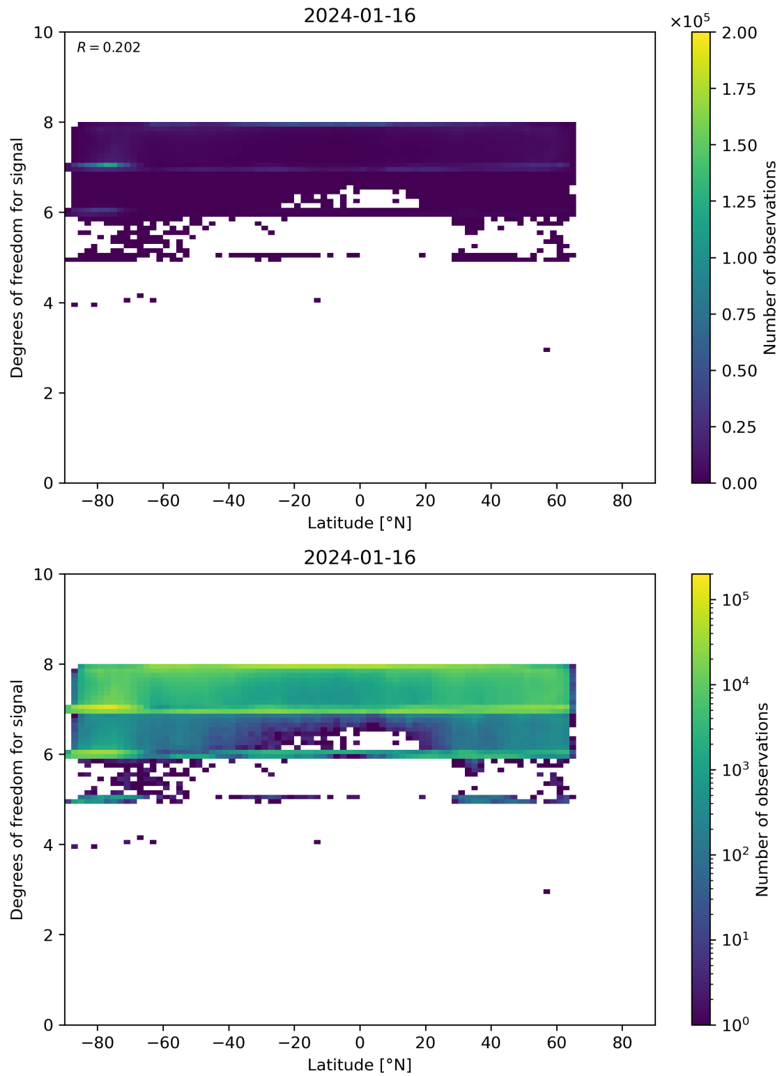
Figure 55: Scatter density plot of “Latitude” against “Degrees of freedom for signal” for 2024-01-15 to 2024-01-17.
