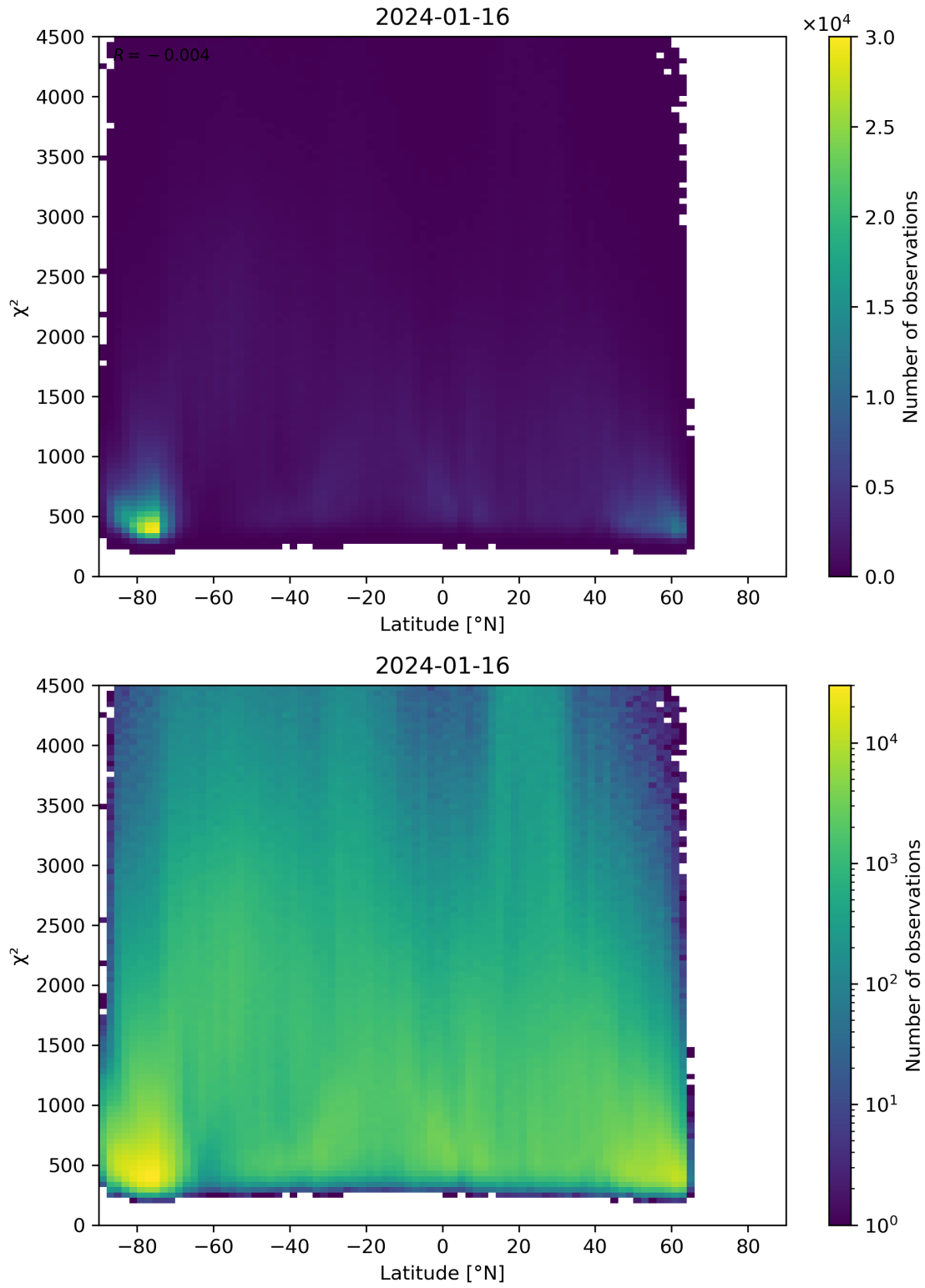
Figure 54: Scatter density plot of “Latitude” against “ \chi^2 ” for 2024-01-15 to 2024-01-17.
