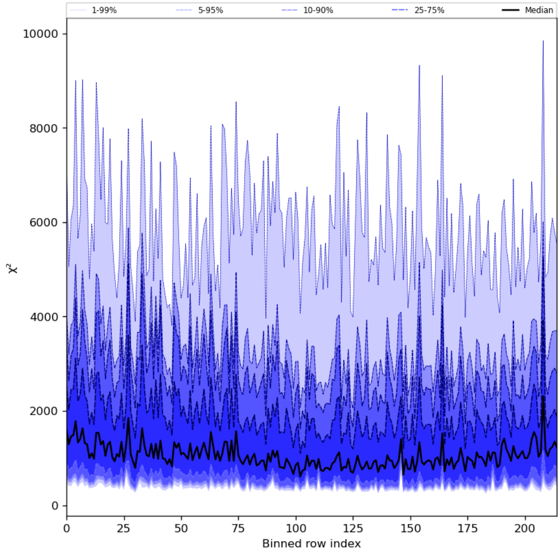
Figure 30: Along track statistics of “ \chi^2 ” for 2024-01-15 to 2024-01-17
