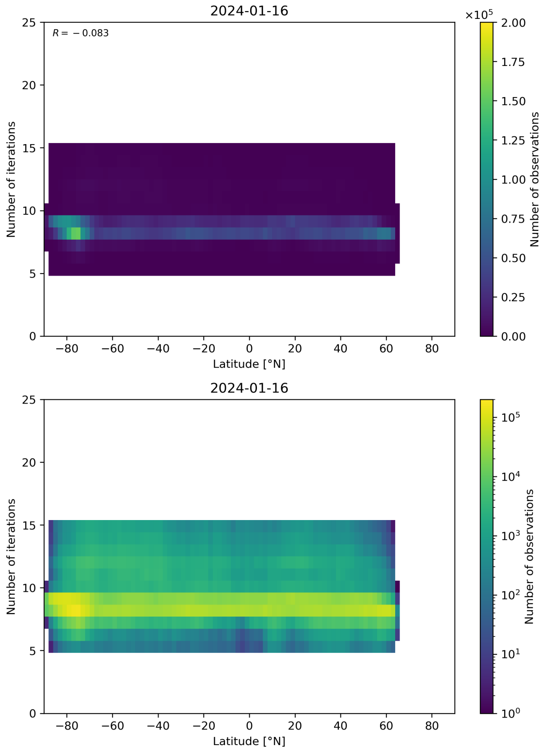
Figure 56: Scatter density plot of “Latitude” against “Number of iterations” for 2024-01-15 to 2024-01-17.
