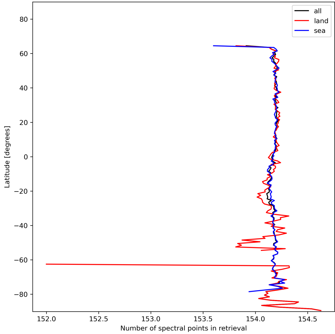
Figure 13: Zonal average of “Number of spectral points in retrieval” for 2024-01-15 to 2024-01-17.
