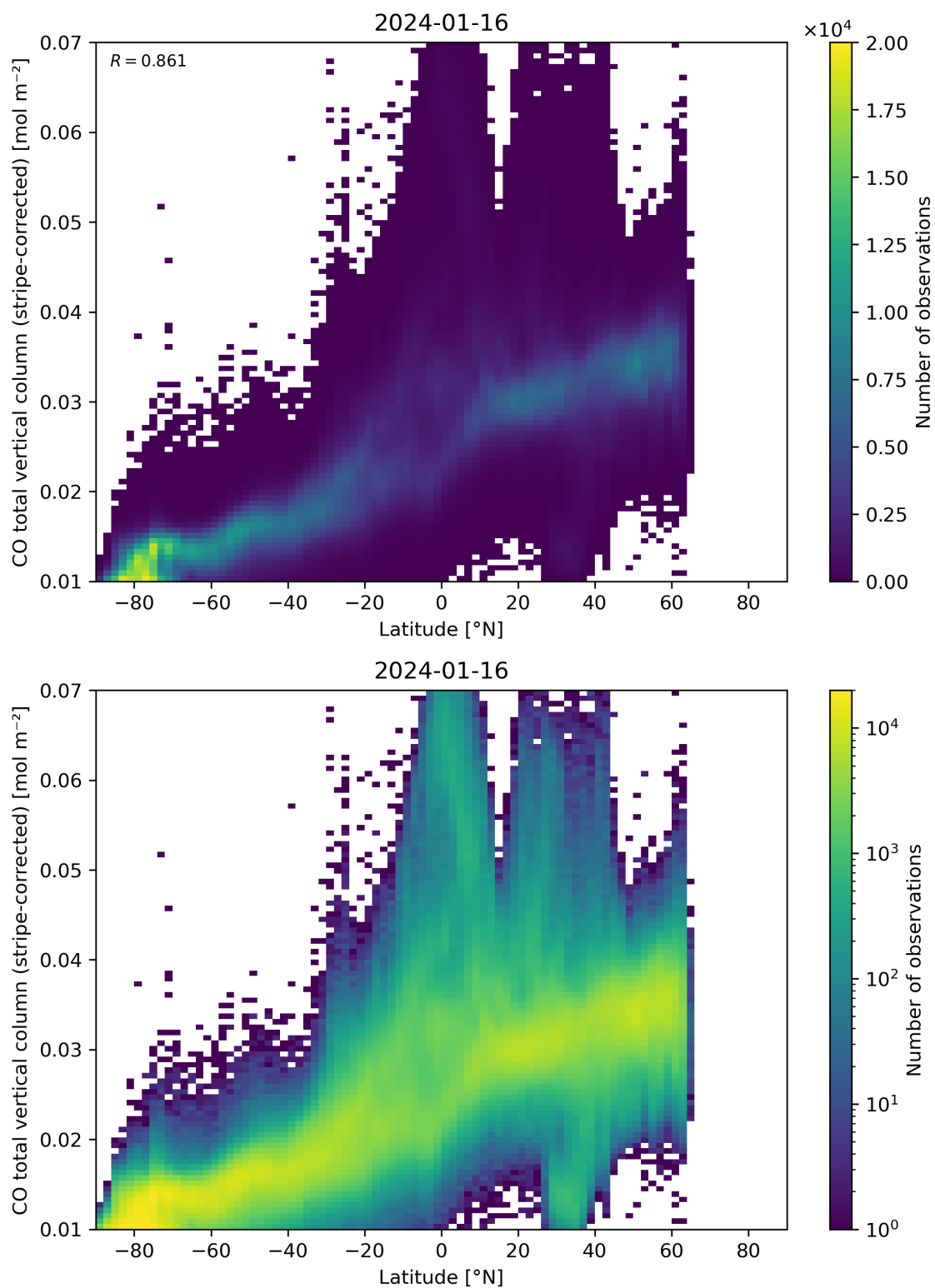
Figure 52: Scatter density plot of “Latitude” against “CO total vertical column (stripe-corrected)” for 2024-01-15 to 2024-01-17.
