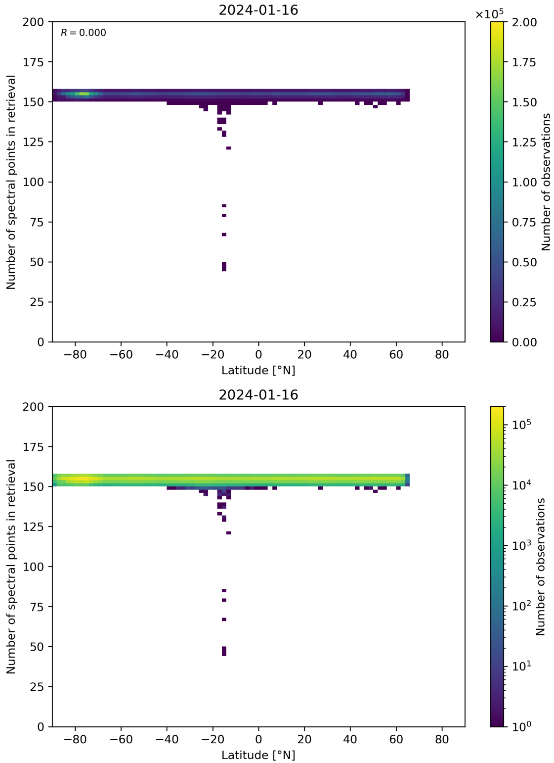
Figure 57: Scatter density plot of “Latitude” against “Number of spectral points in retrieval” for 2024-01-15 to 2024-01-17.
