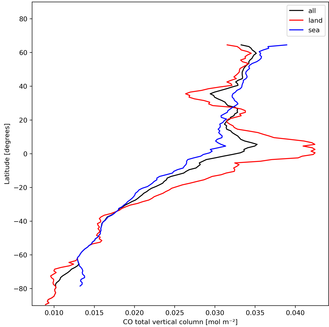
Figure 10: Zonal average of “CO total vertical column” for 2024-01-15 to 2024-01-17.
