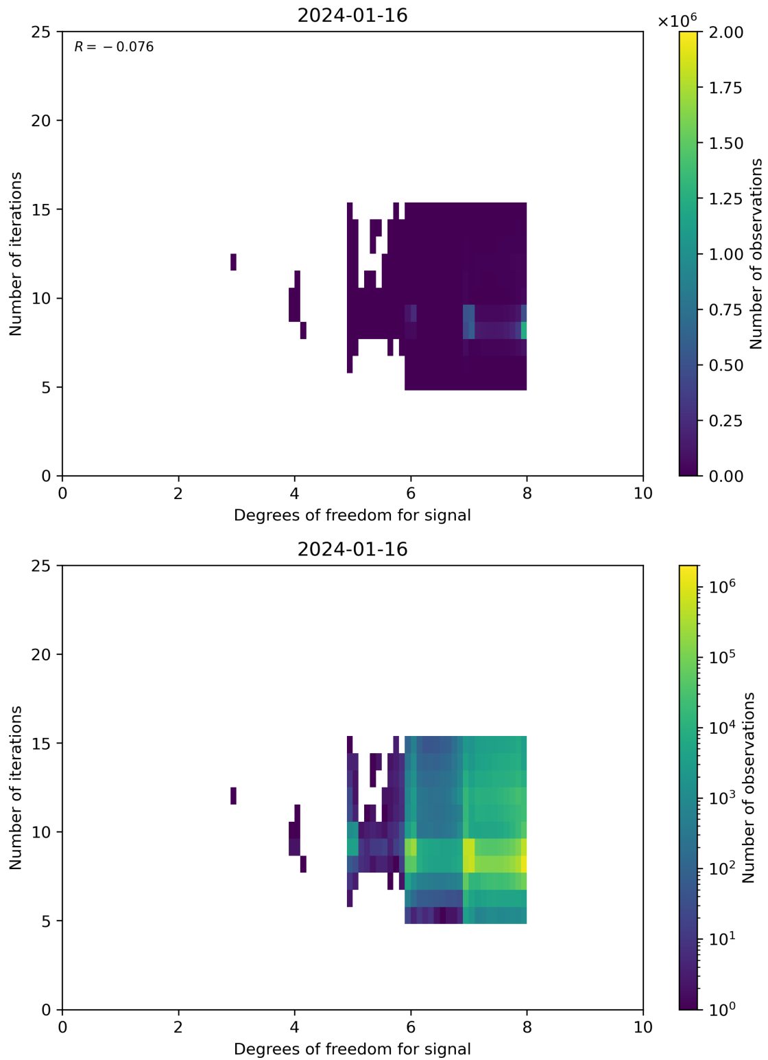
Figure 50: Scatter density plot of “Degrees of freedom for signal” against “Number of iterations” for 2024-01-15 to 2024-01-17.
