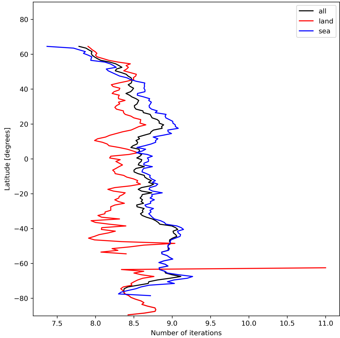
Figure 16: Zonal average of “Number of iterations” for 2024-01-15 to 2024-01-17.
