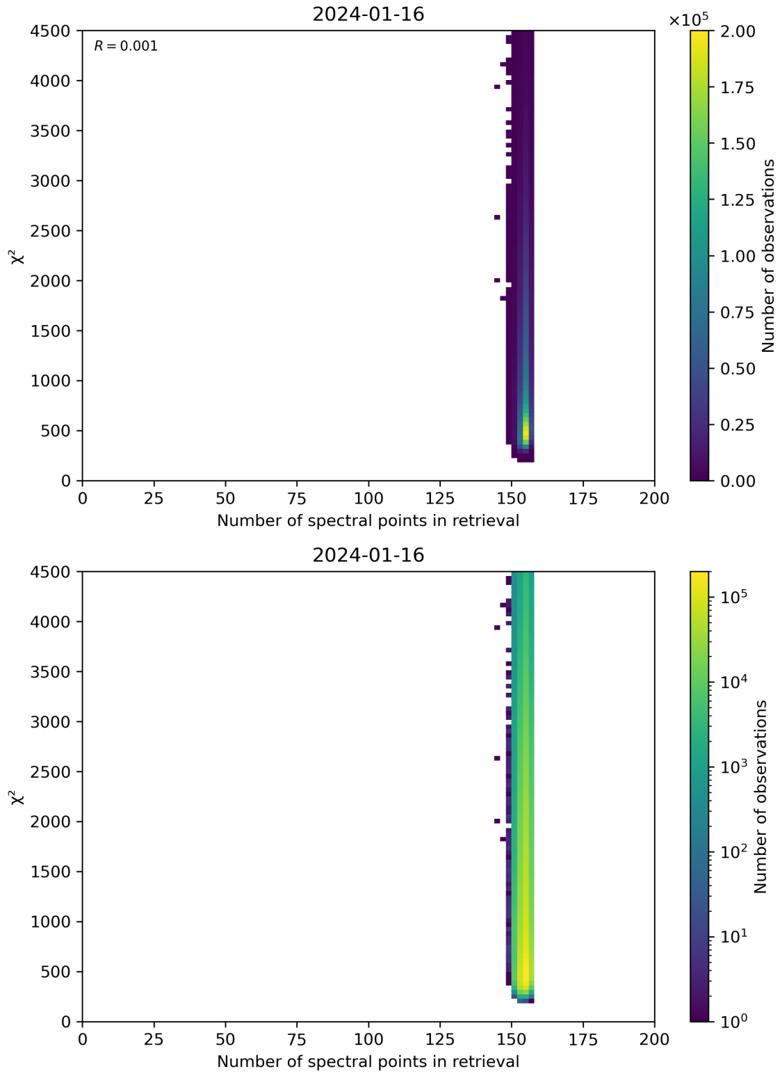
Figure 58: Scatter density plot of “Number of spectral points in retrieval” against “ \chi^2 ” for 2024-01-15 to 2024-01-17.
