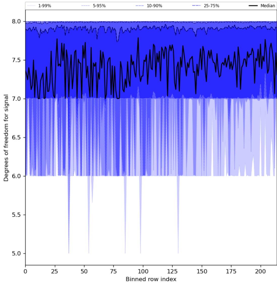
Figure 31: Along track statistics of “Degrees of freedom for signal” for 2024-01-15 to 2024-01-17
