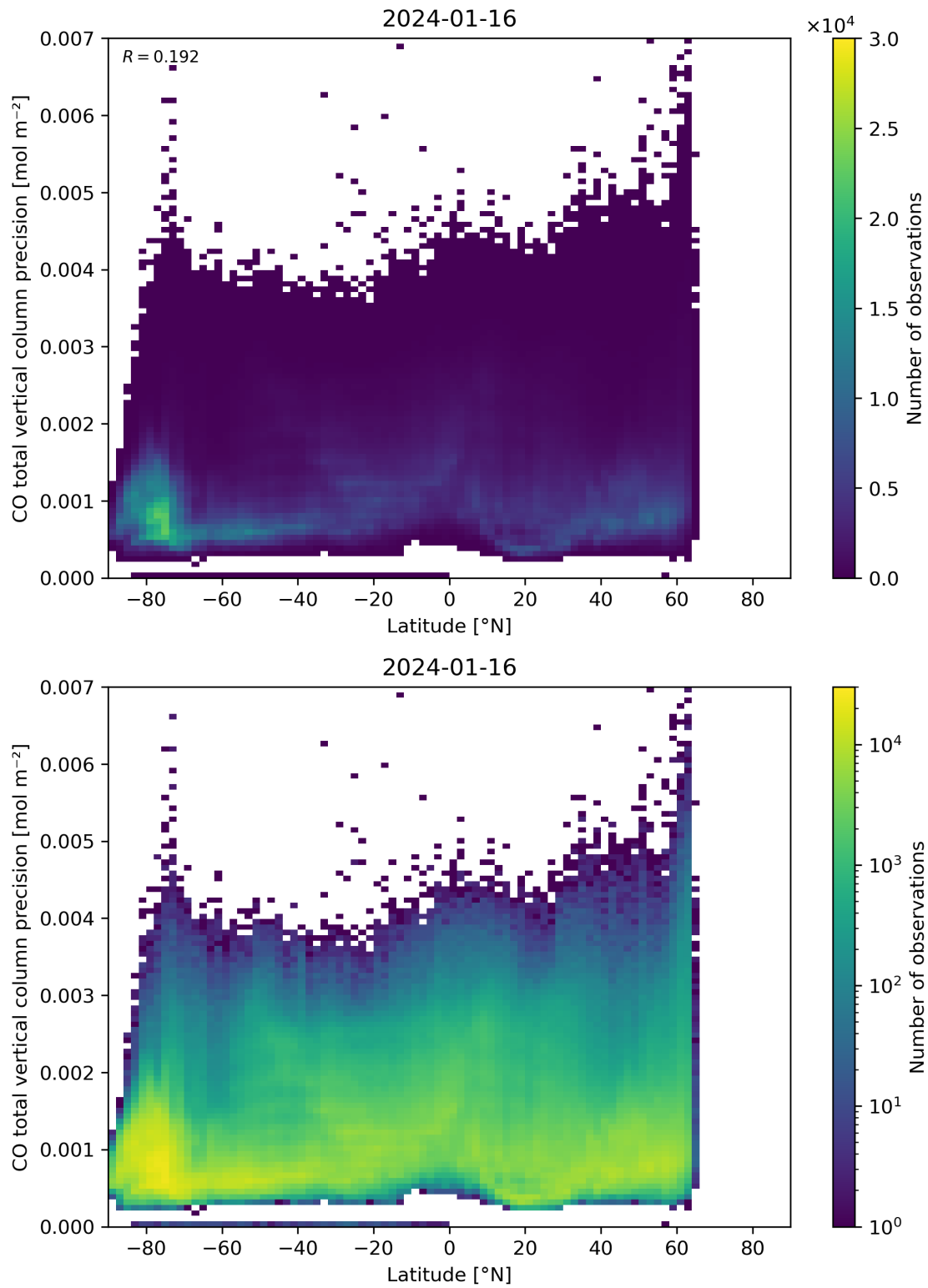
Figure 53: Scatter density plot of “Latitude” against “CO total vertical column precision” for 2024-01-15 to 2024-01-17.
