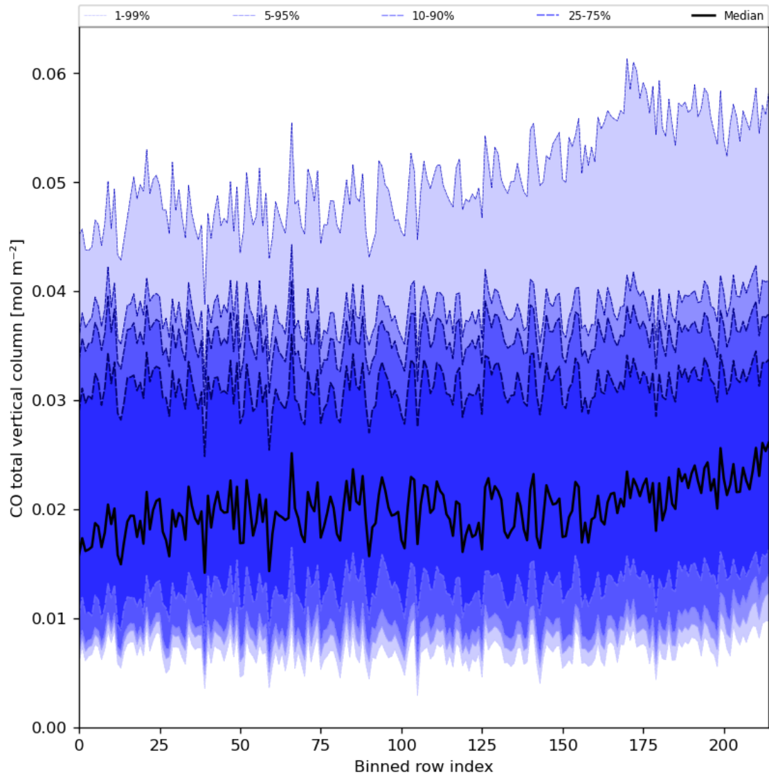
Figure 26: Along track statistics of “CO total vertical column” for 2024-01-15 to 2024-01-17
