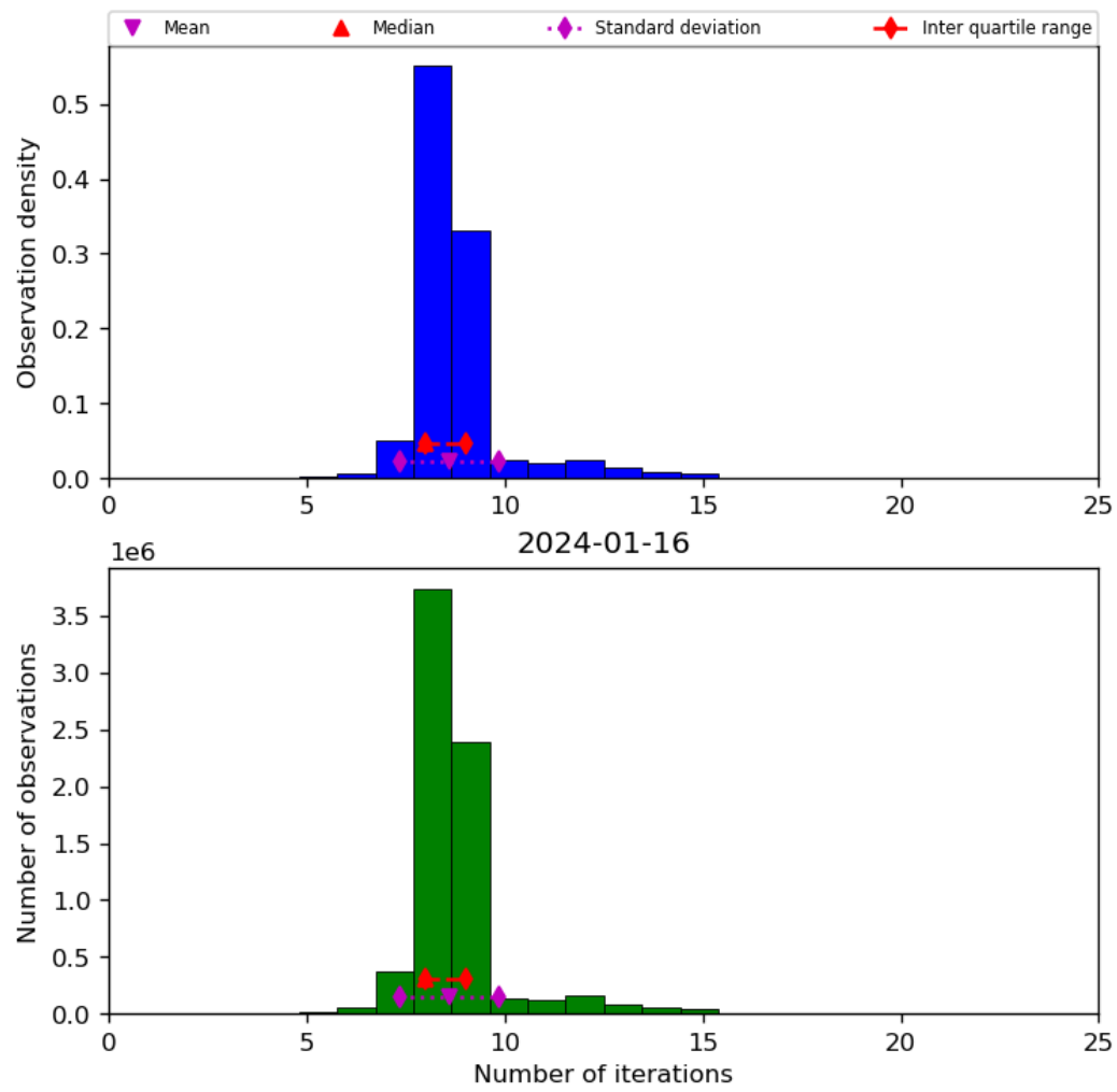
Figure 24: Histogram of “Number of iterations” for 2024-01-15 to 2024-01-17
