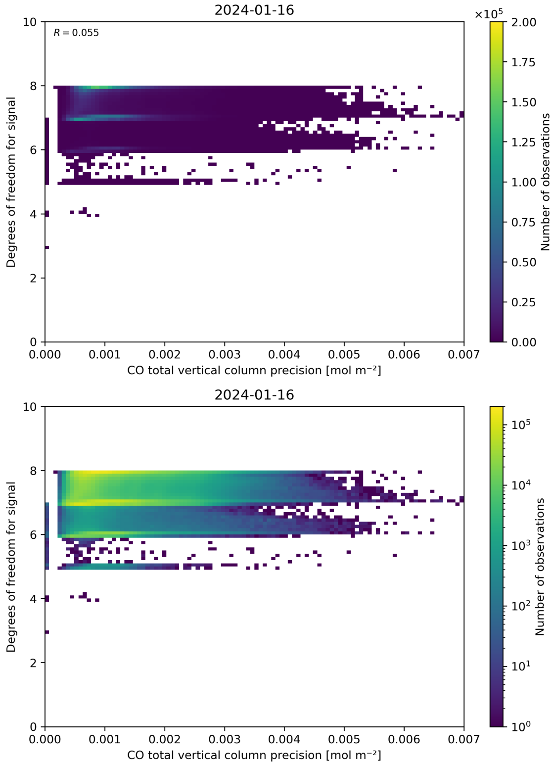
Figure 45: Scatter density plot of “CO total vertical column precision” against “Degrees of freedom for signal” for 2024-01-15 to 2024-01-17.
