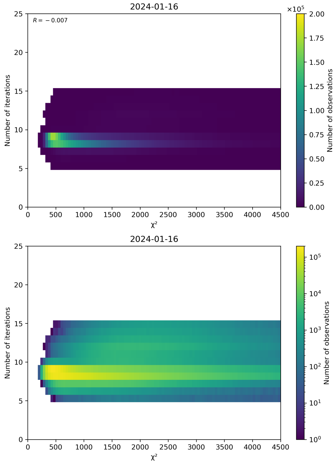
Figure 49: Scatter density plot of “ \chi^2 ” against “Number of iterations” for 2024-01-15 to 2024-01-17.
