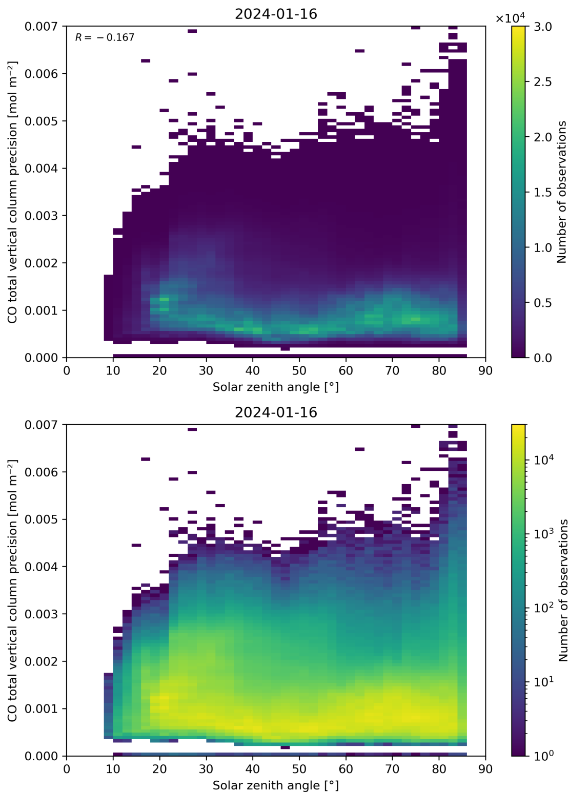
Figure 63: Scatter density plot of “Solar zenith angle” against “CO total vertical column precision” for 2024-01-15 to 2024-01-17.
