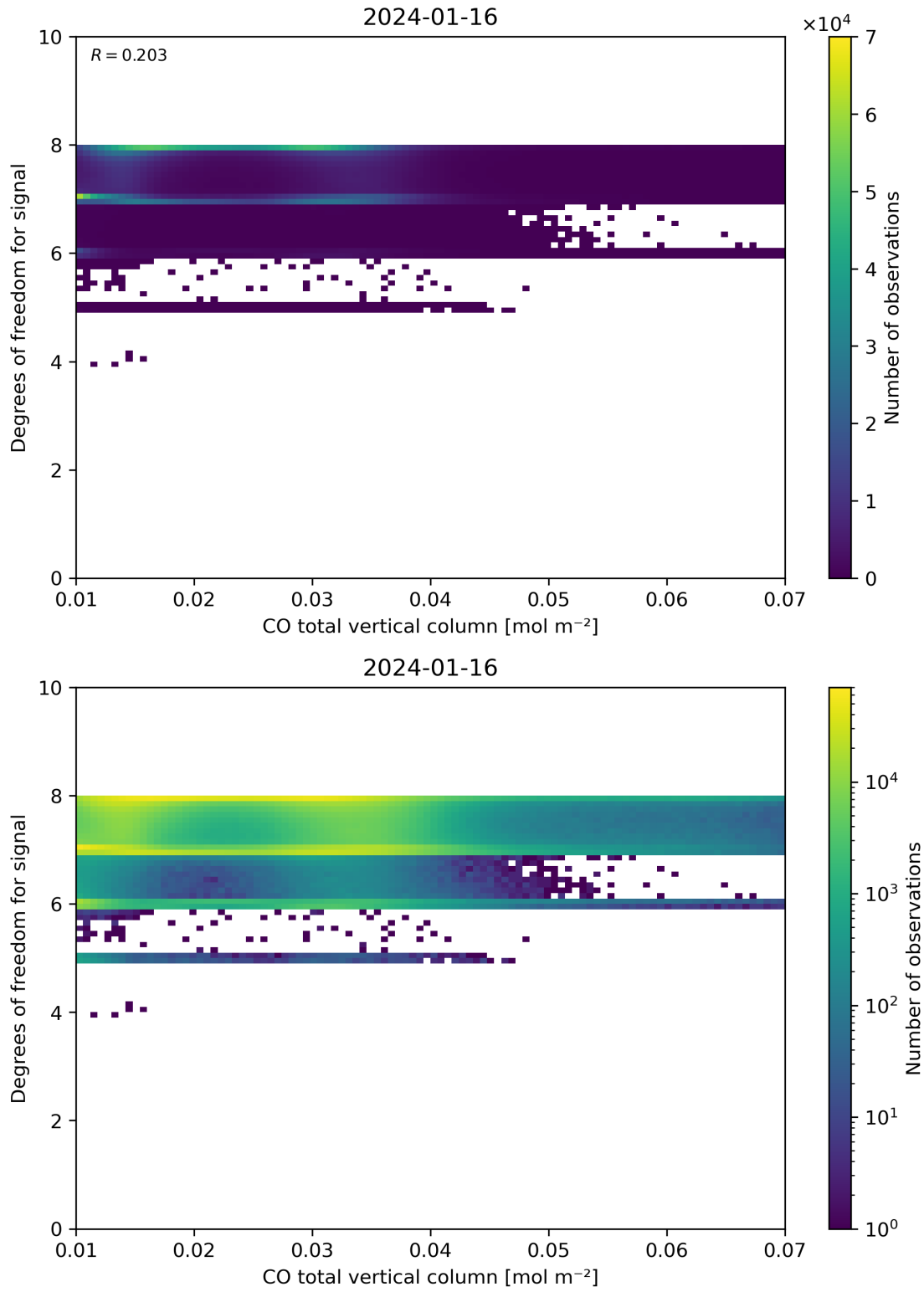
Figure 41: Scatter density plot of “CO total vertical column” against “Degrees of freedom for signal” for 2024-01-15 to 2024-01-17.
