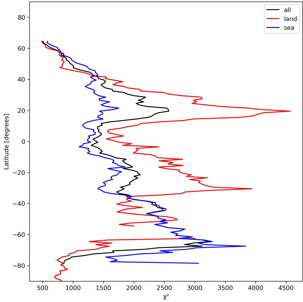
Figure 14: Zonal average of “ \chi^2 ” for 2024-01-15 to 2024-01-17.
