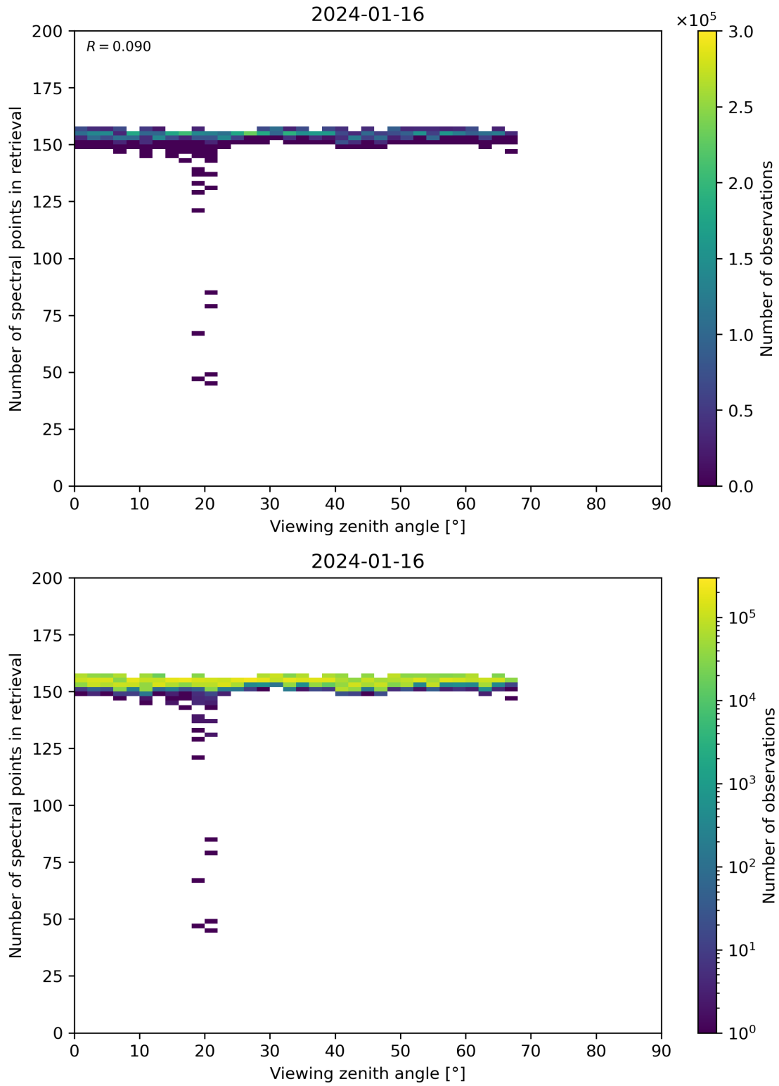
Figure 76: Scatter density plot of “Viewing zenith angle” against “Number of spectral points in retrieval” for 2024-01-15 to 2024-01-17.
