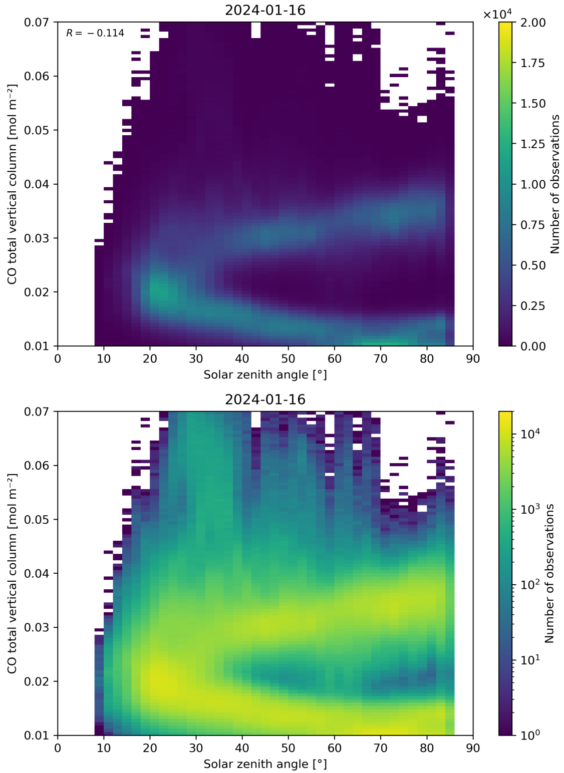
Figure 61: Scatter density plot of “Solar zenith angle” against “CO total vertical column” for 2024-01-15 to 2024-01-17.
