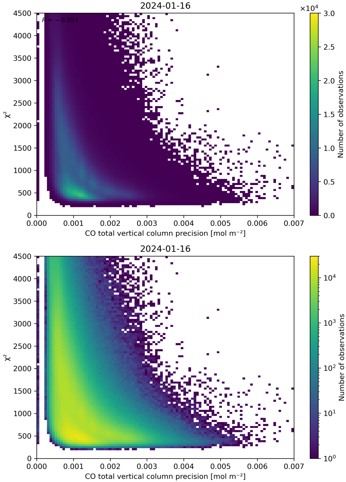
Figure 44: Scatter density plot of “CO total vertical column precision” against “ \chi^2 ” for 2024-01-15 to 2024-01-17.
