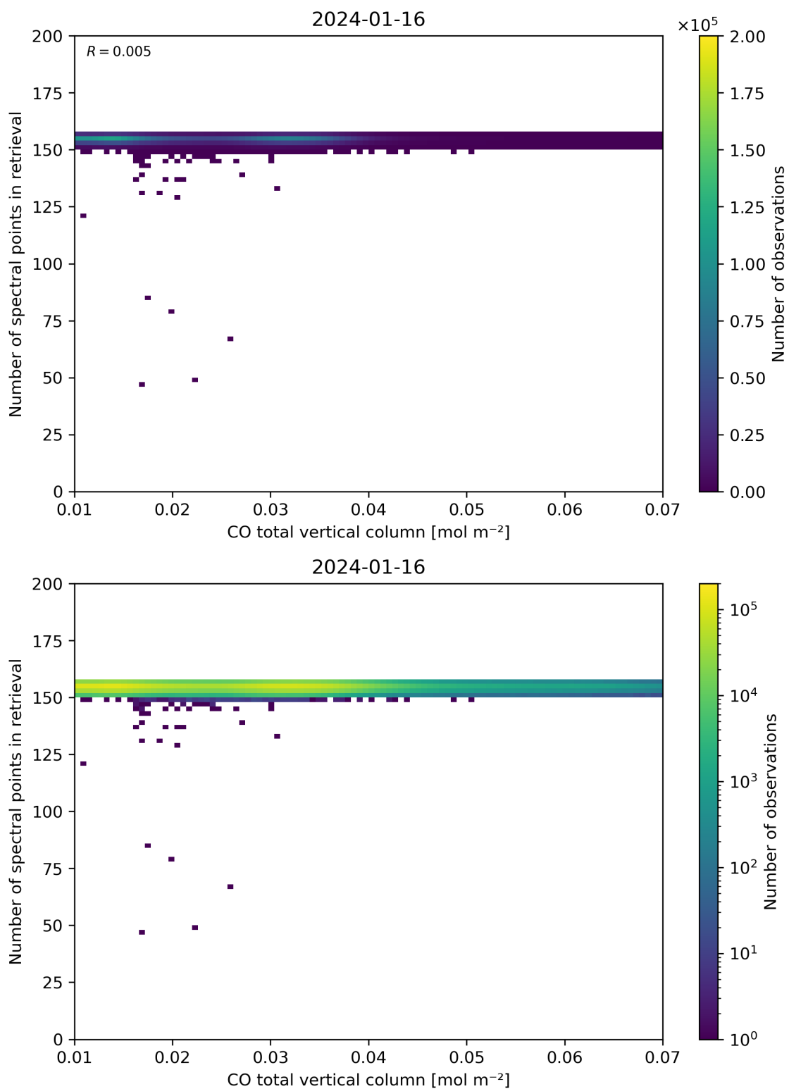
Figure 43: Scatter density plot of “CO total vertical column” against “Number of spectral points in retrieval” for 2024-01-15 to 2024-01-17.
