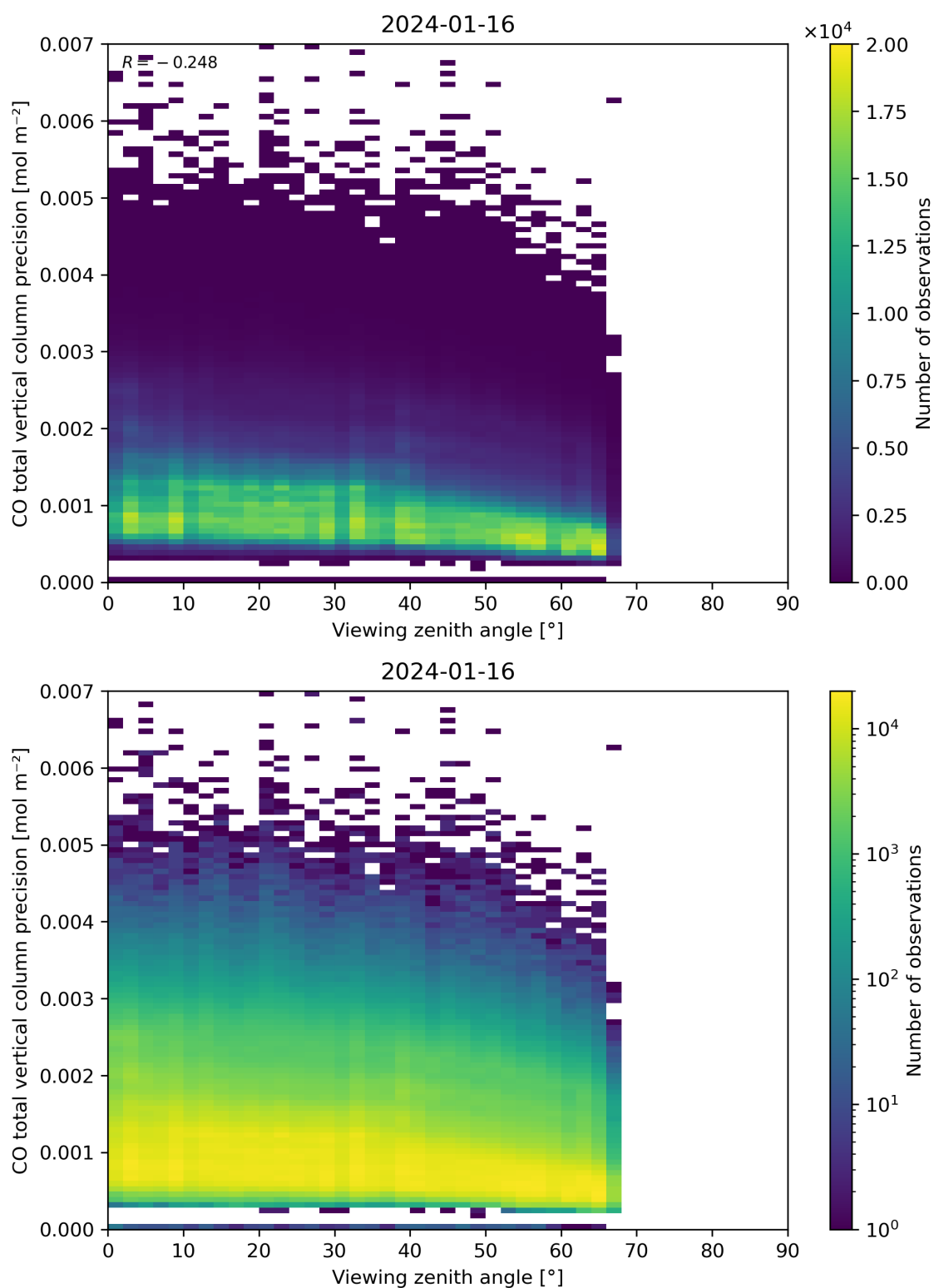
Figure 71: Scatter density plot of “Viewing zenith angle” against “CO total vertical column precision” for 2024-01-15 to 2024-01-17.
