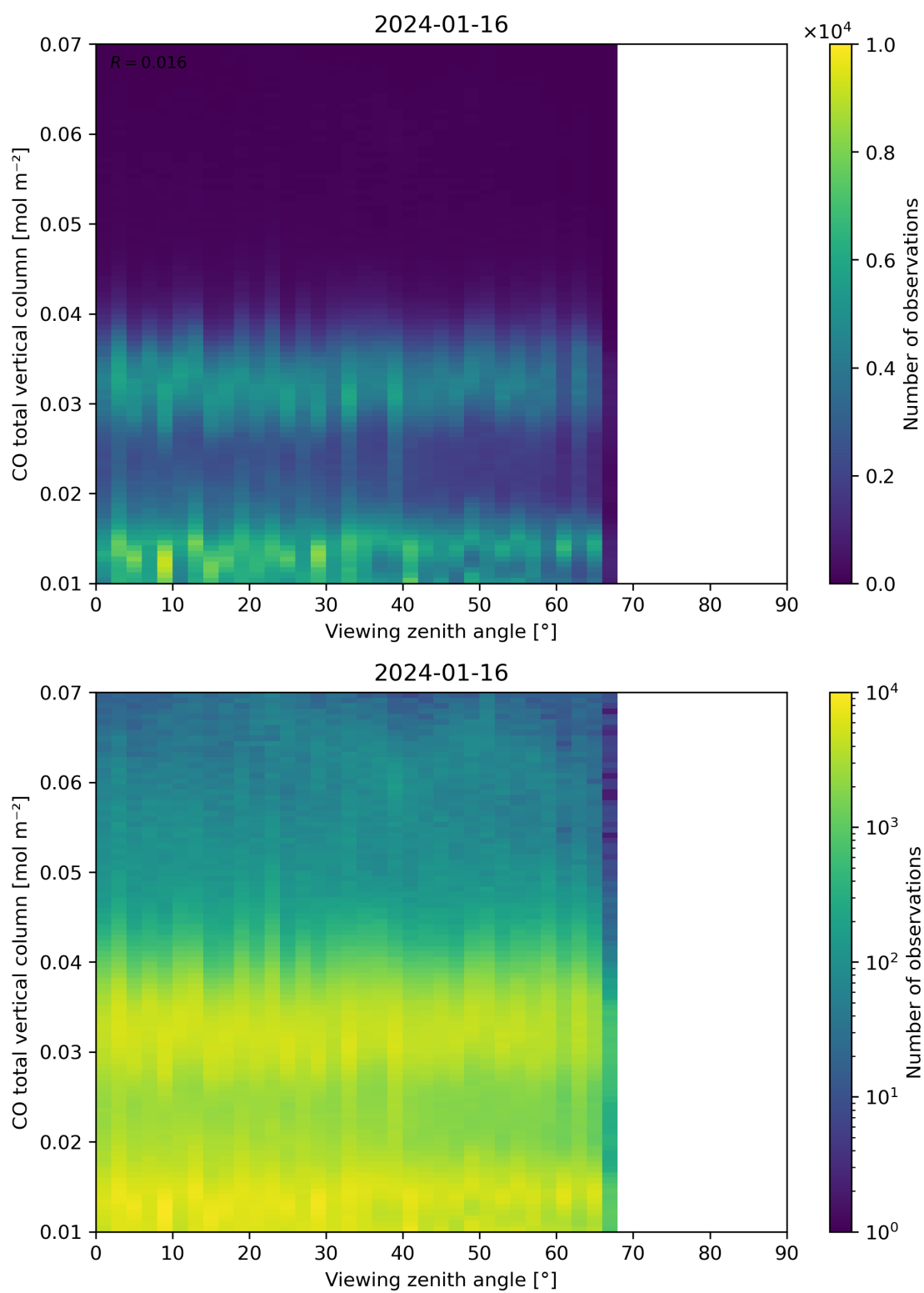
Figure 69: Scatter density plot of “Viewing zenith angle” against “CO total vertical column” for 2024-01-15 to 2024-01-17.
