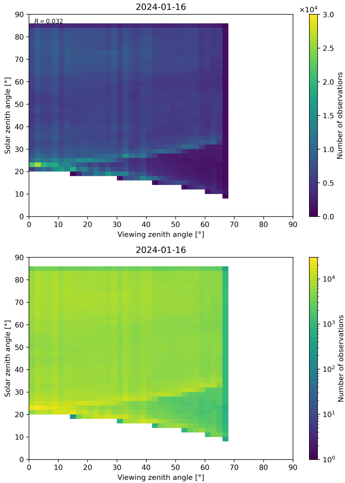
Figure 77: Scatter density plot of “Viewing zenith angle” against “Solar zenith angle” for 2024-01-15 to 2024-01-17.
