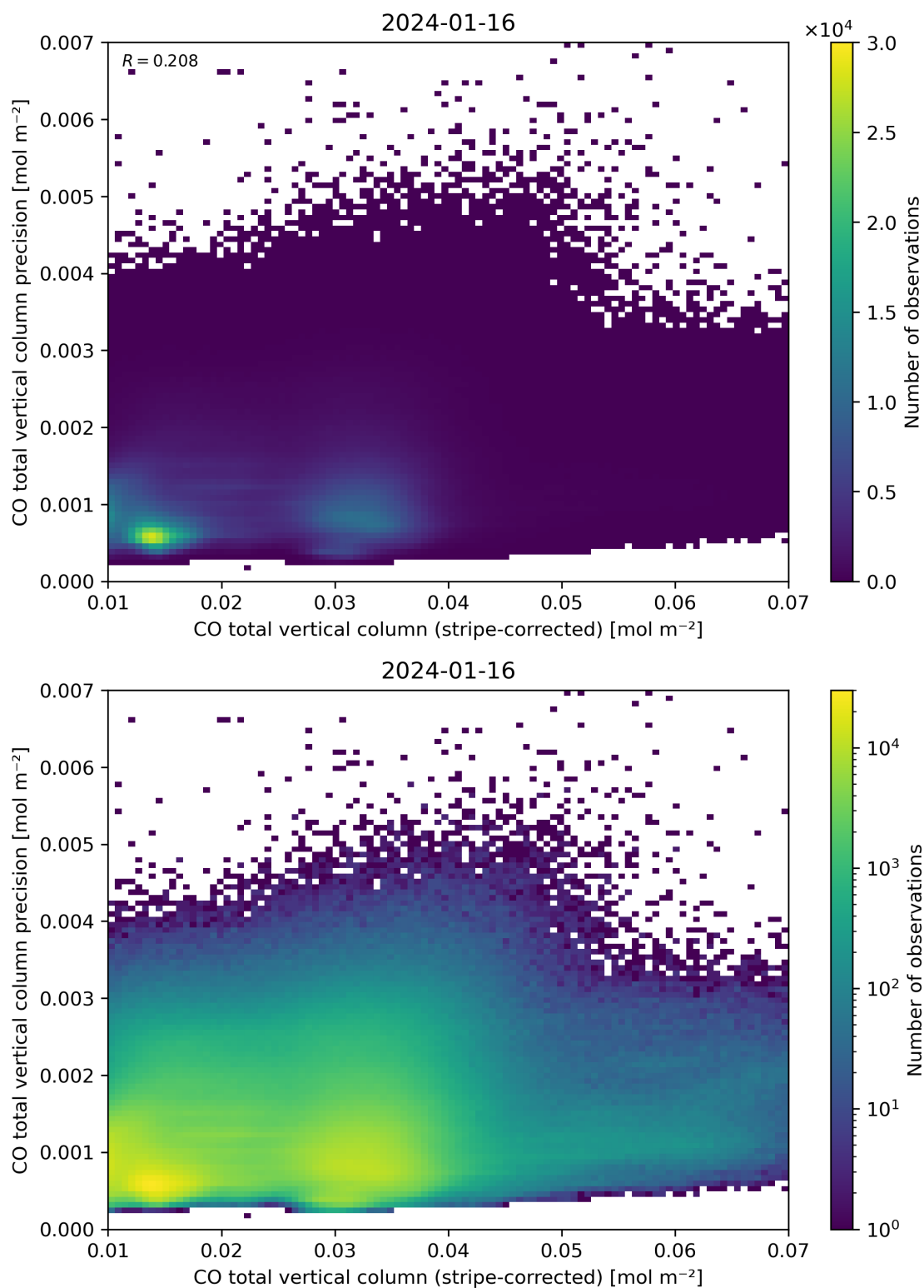
Figure 36: Scatter density plot of “CO total vertical column (stripe-corrected)” against “CO total vertical column precision” for 2024-01-15 to 2024-01-17.
