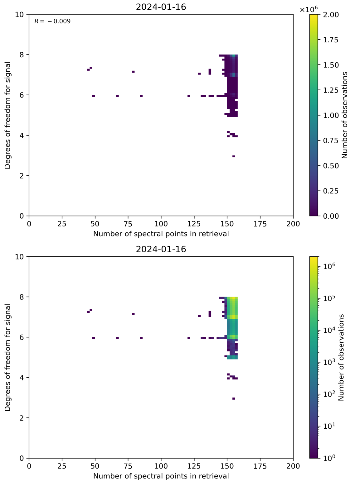
Figure 59: Scatter density plot of “Number of spectral points in retrieval” against “Degrees of freedom for signal” for 2024-01-15 to 2024-01-17.
