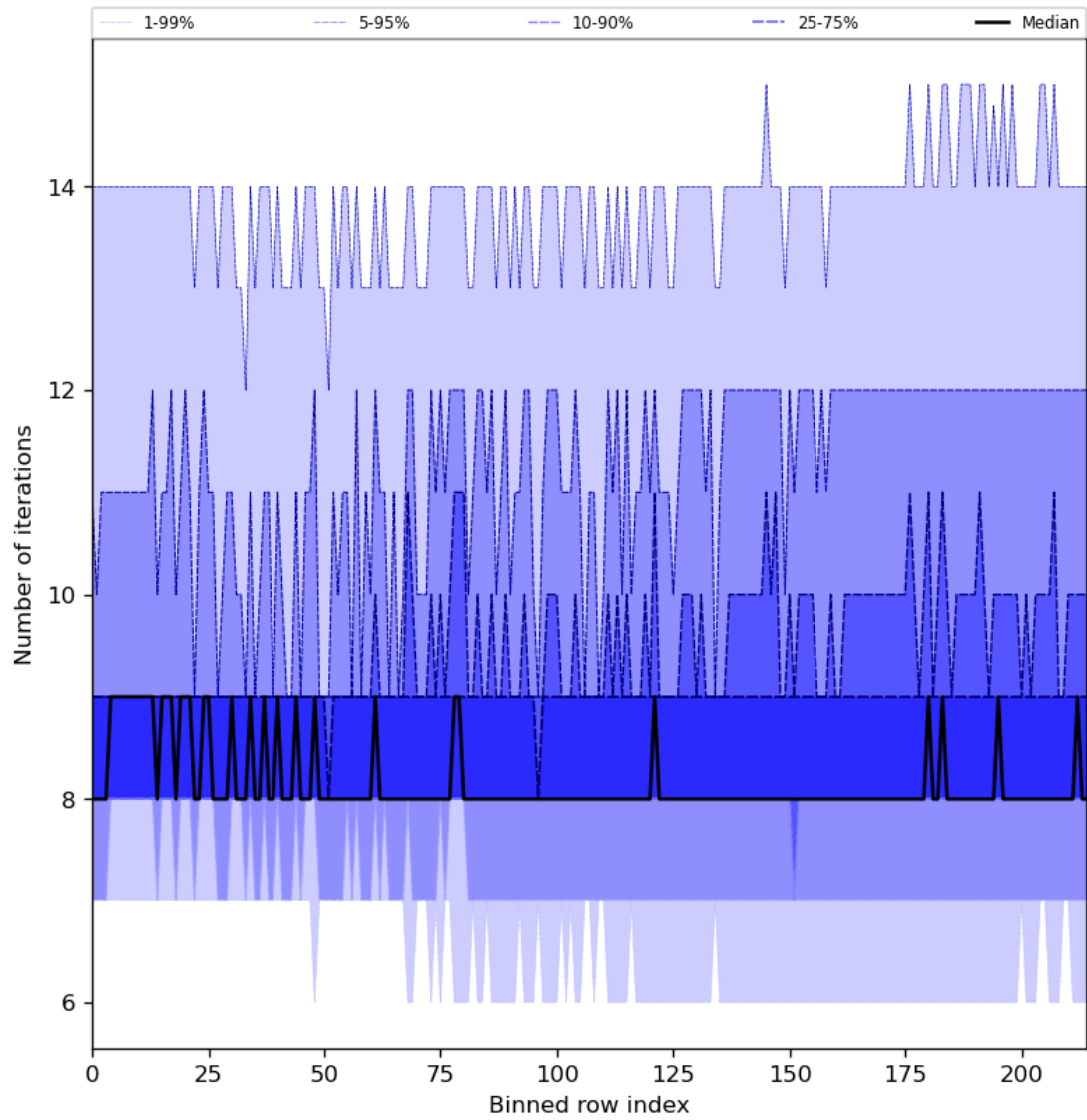
Figure 32: Along track statistics of “Number of iterations” for 2024-01-15 to 2024-01-17
