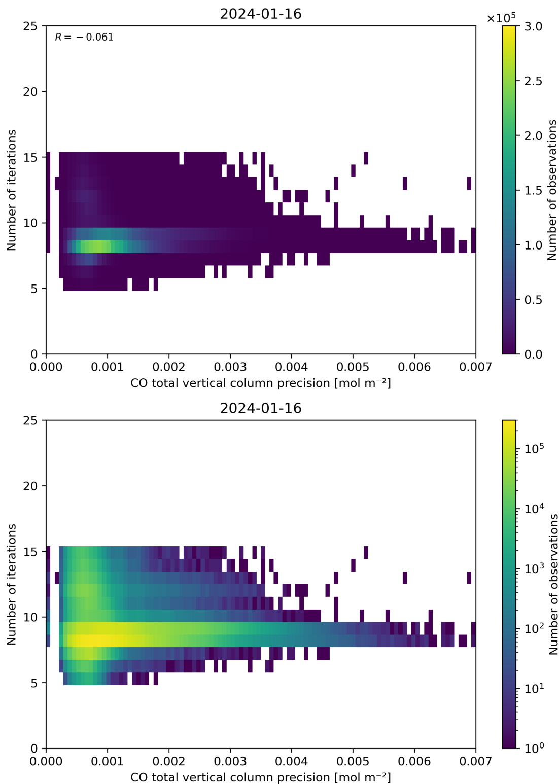
Figure 46: Scatter density plot of “CO total vertical column precision” against “Number of iterations” for 2024-01-15 to 2024-01-17.
