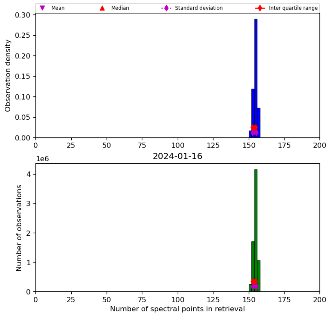
Figure 21: Histogram of “Number of spectral points in retrieval” for 2024-01-15 to 2024-01-17
