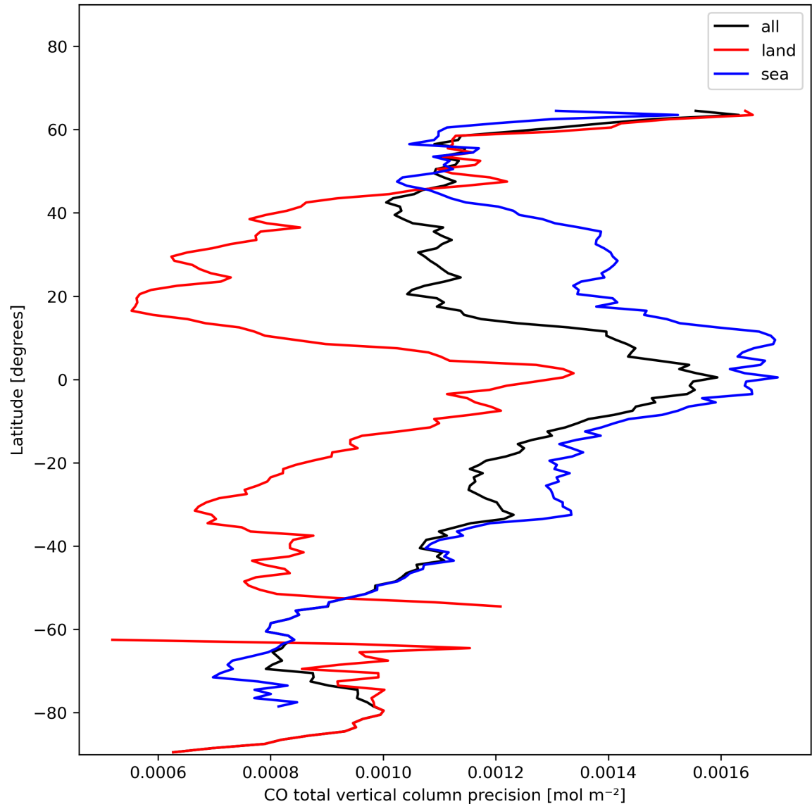
Figure 12: Zonal average of “CO total vertical column precision” for 2024-01-15 to 2024-01-17.
