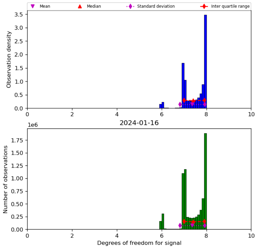
Figure 23: Histogram of “Degrees of freedom for signal” for 2024-01-15 to 2024-01-17
