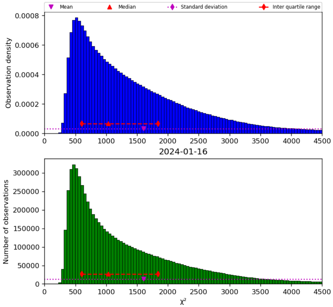
Figure 22: Histogram of “ \chi^2 ” for 2024-01-15 to 2024-01-17
