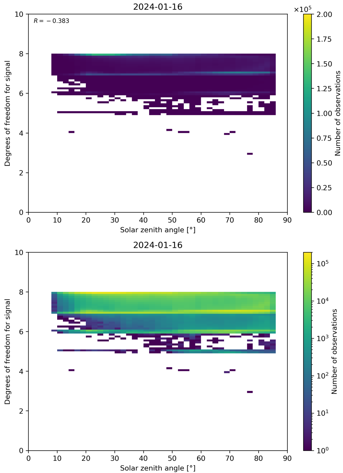
Figure 65: Scatter density plot of “Solar zenith angle” against “Degrees of freedom for signal” for 2024-01-15 to 2024-01-17.
