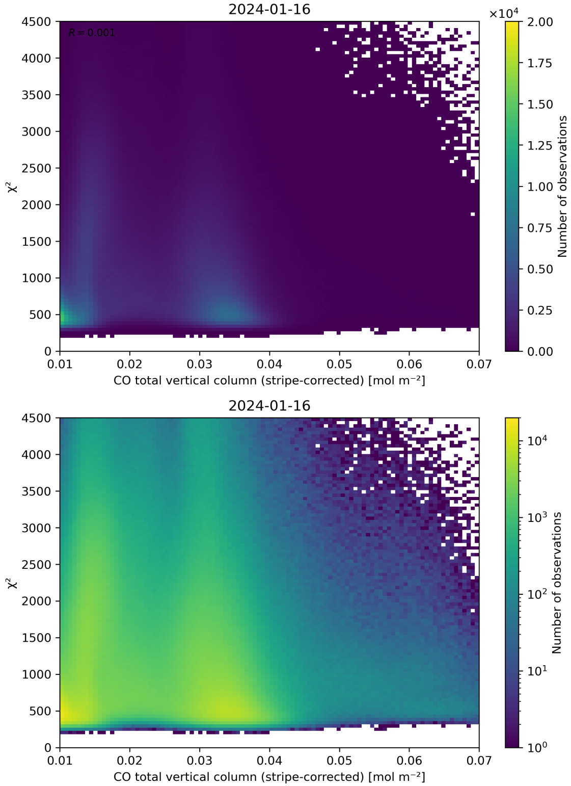
Figure 37: Scatter density plot of “CO total vertical column (stripe-corrected)” against “ \chi^2 ” for 2024-01-15 to 2024-01-17.
