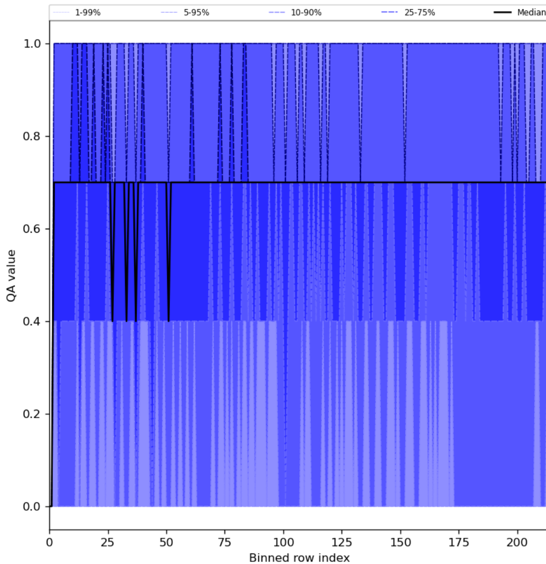
Figure 25: Along track statistics of “QA value” for 2024-01-15 to 2024-01-17
