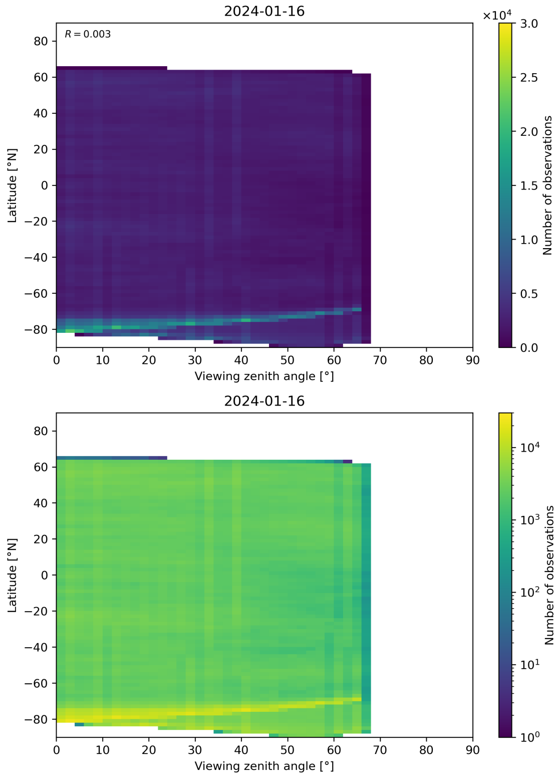
Figure 74: Scatter density plot of “Viewing zenith angle” against “Latitude” for 2024-01-15 to 2024-01-17.
