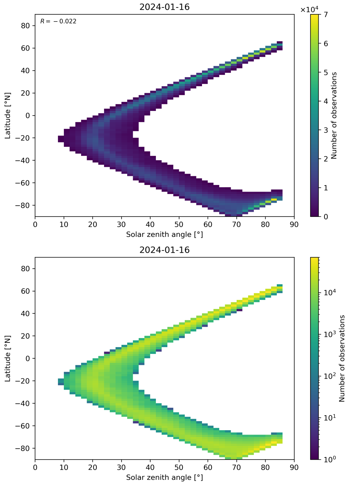
Figure 66: Scatter density plot of “Solar zenith angle” against “Latitude” for 2024-01-15 to 2024-01-17.
