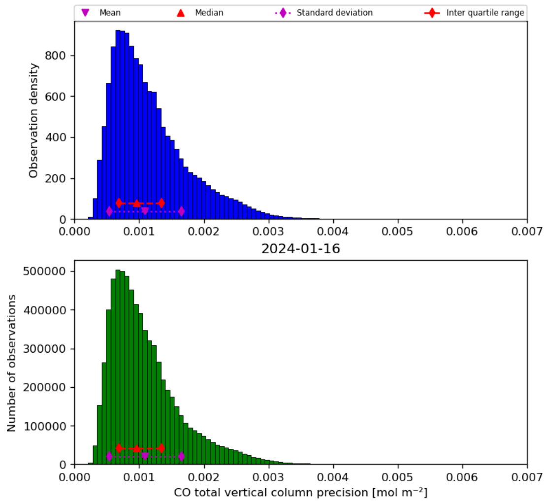
Figure 20: Histogram of “CO total vertical column precision” for 2024-01-15 to 2024-01-17
