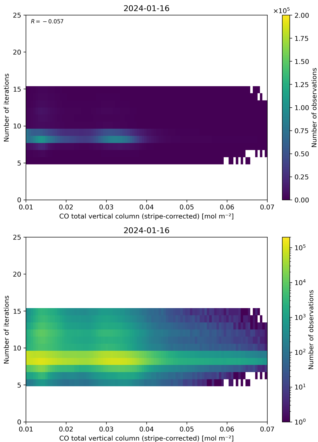
Figure 39: Scatter density plot of “CO total vertical column (stripe-corrected)” against “Number of iterations” for 2024-01-15 to 2024-01-17.
