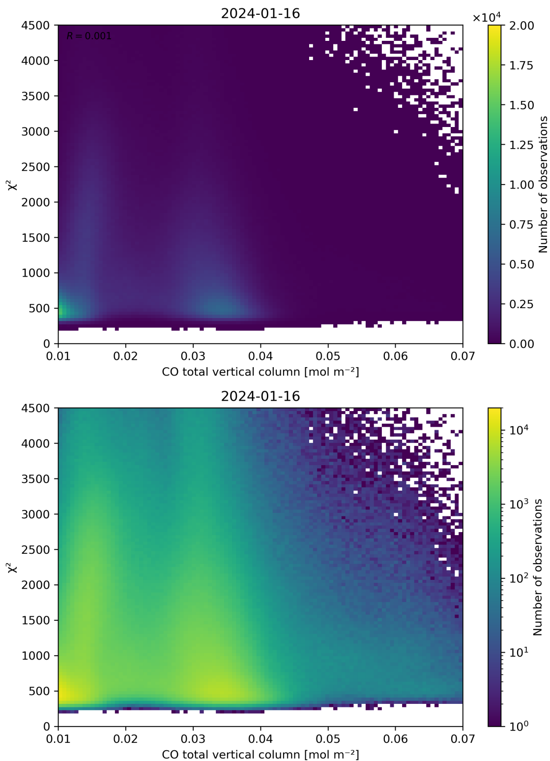
Figure 35: Scatter density plot of “CO total vertical column” against “ \chi^2 ” for 2024-01-15 to 2024-01-17.
