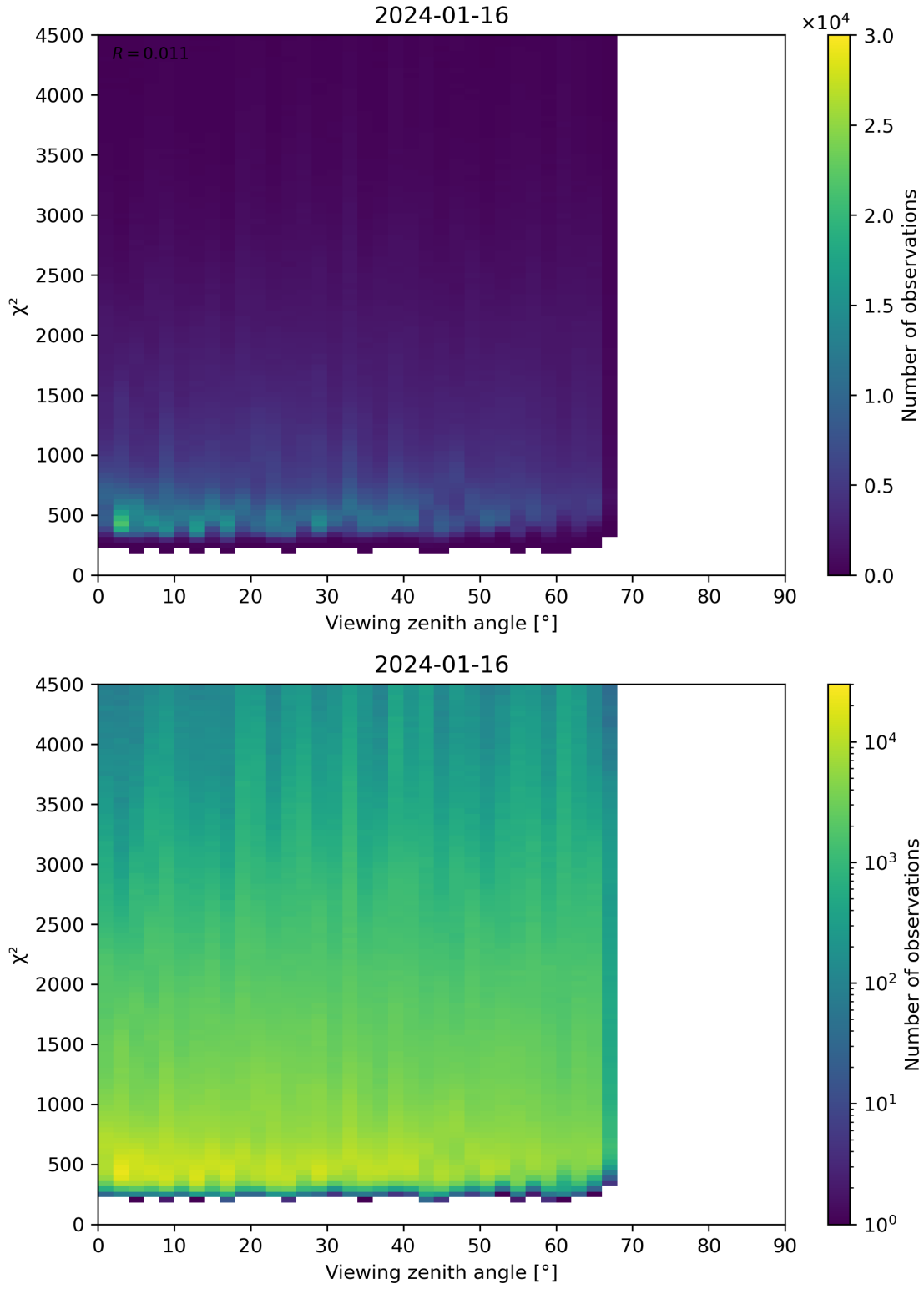
Figure 72: Scatter density plot of “Viewing zenith angle” against “ \chi^2 ” for 2024-01-15 to 2024-01-17.
