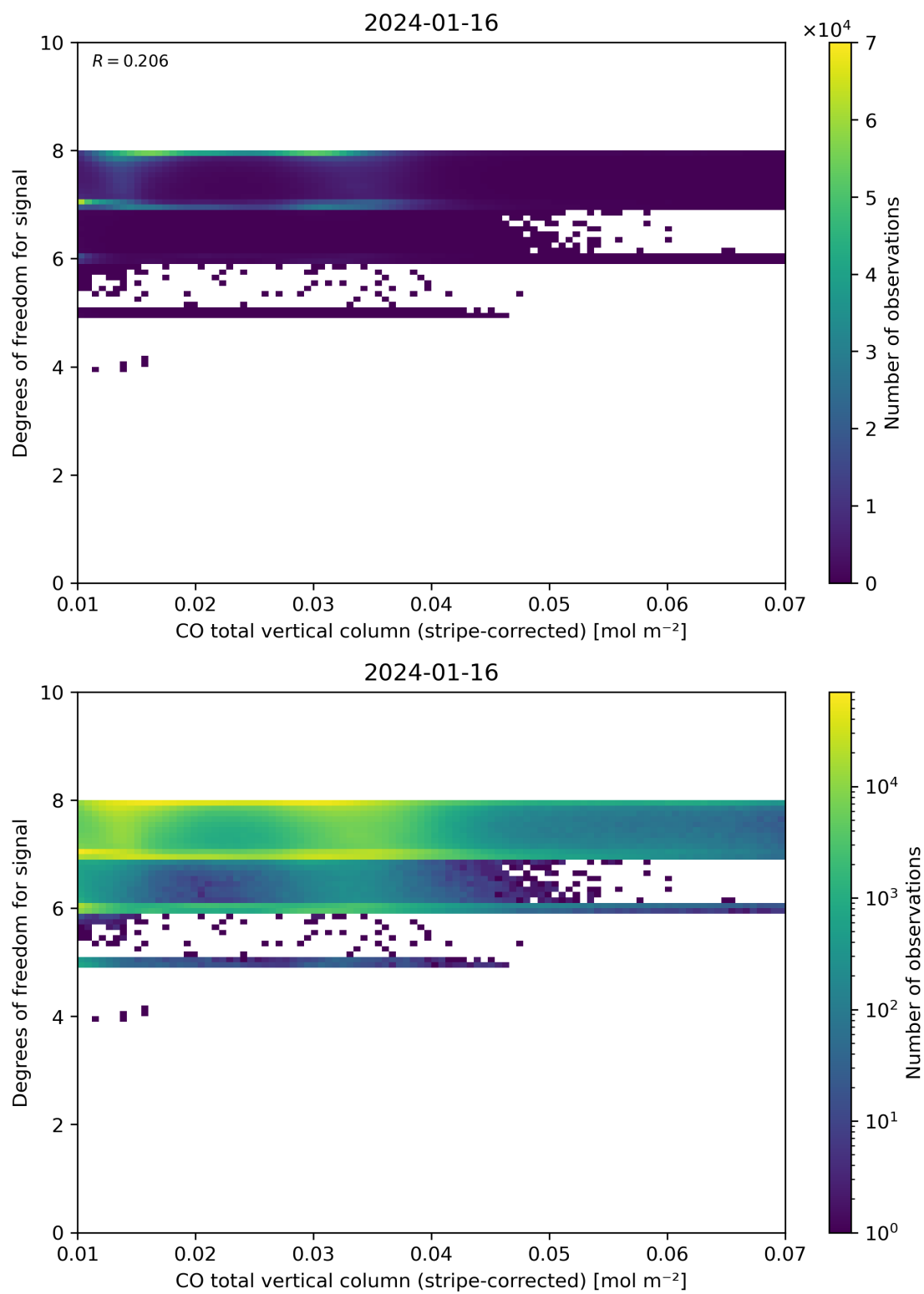
Figure 38: Scatter density plot of “CO total vertical column (stripe-corrected)” against “Degrees of freedom for signal” for 2024-01-15 to 2024-01-17.
