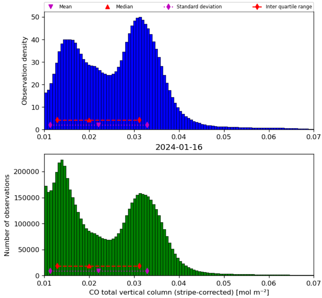
Figure 19: Histogram of “CO total vertical column (stripe-corrected)” for 2024-01-15 to 2024-01-17
