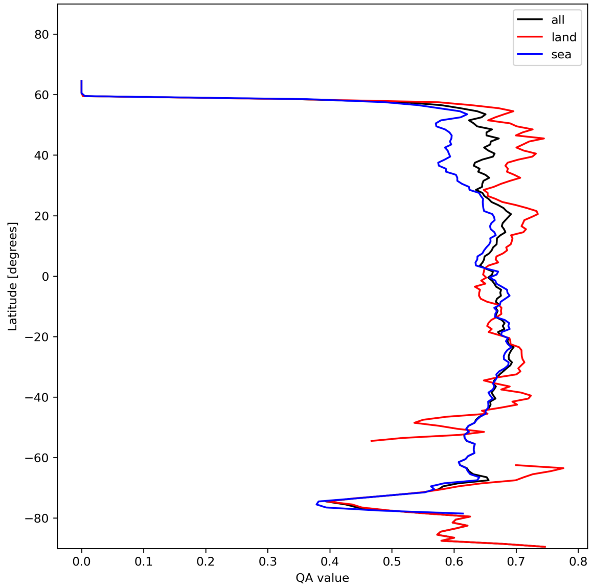
Figure 9: Zonal average of “QA value” for 2024-01-15 to 2024-01-17.
