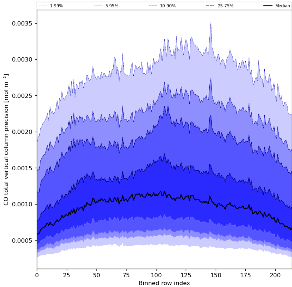
Figure 28: Along track statistics of “CO total vertical column precision” for 2024-01-15 to 2024-01-17
