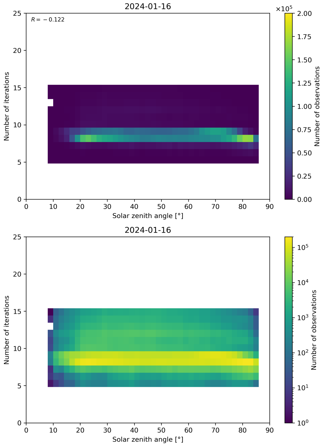
Figure 67: Scatter density plot of “Solar zenith angle” against “Number of iterations” for 2024-01-15 to 2024-01-17.
