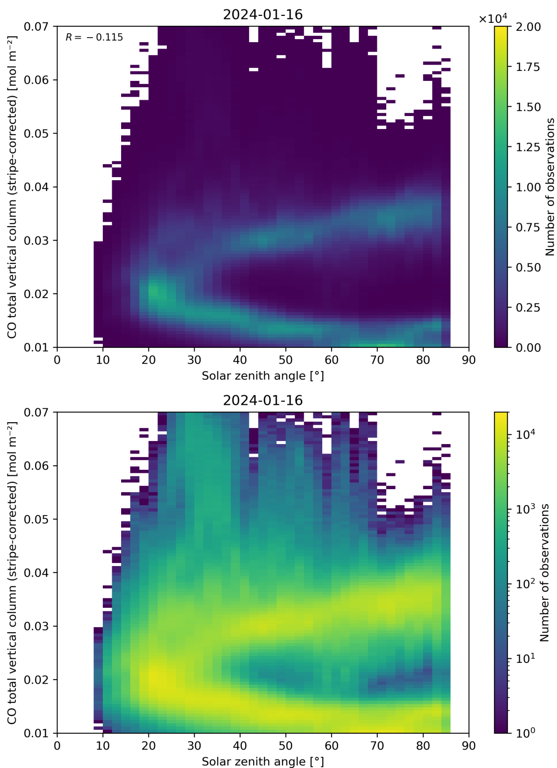
Figure 62: Scatter density plot of “Solar zenith angle” against “CO total vertical column (stripe-corrected)” for 2024-01-15 to 2024-01-17.
