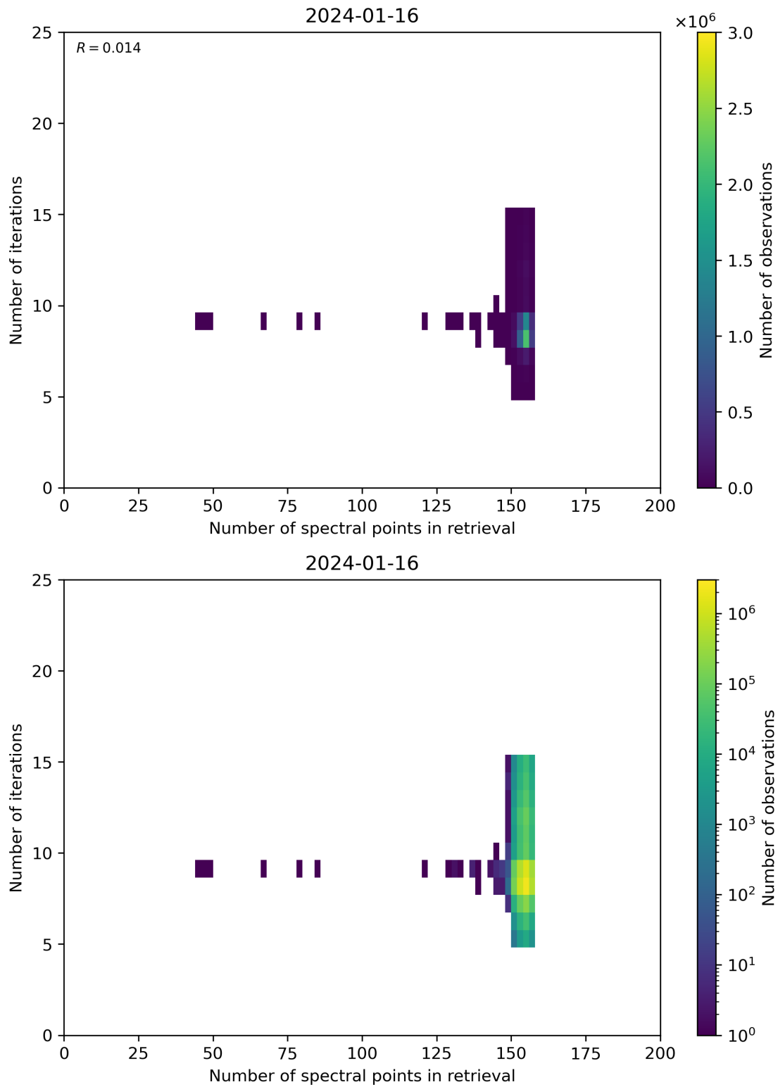
Figure 60: Scatter density plot of “Number of spectral points in retrieval” against “Number of iterations” for 2024-01-15 to 2024-01-17.
