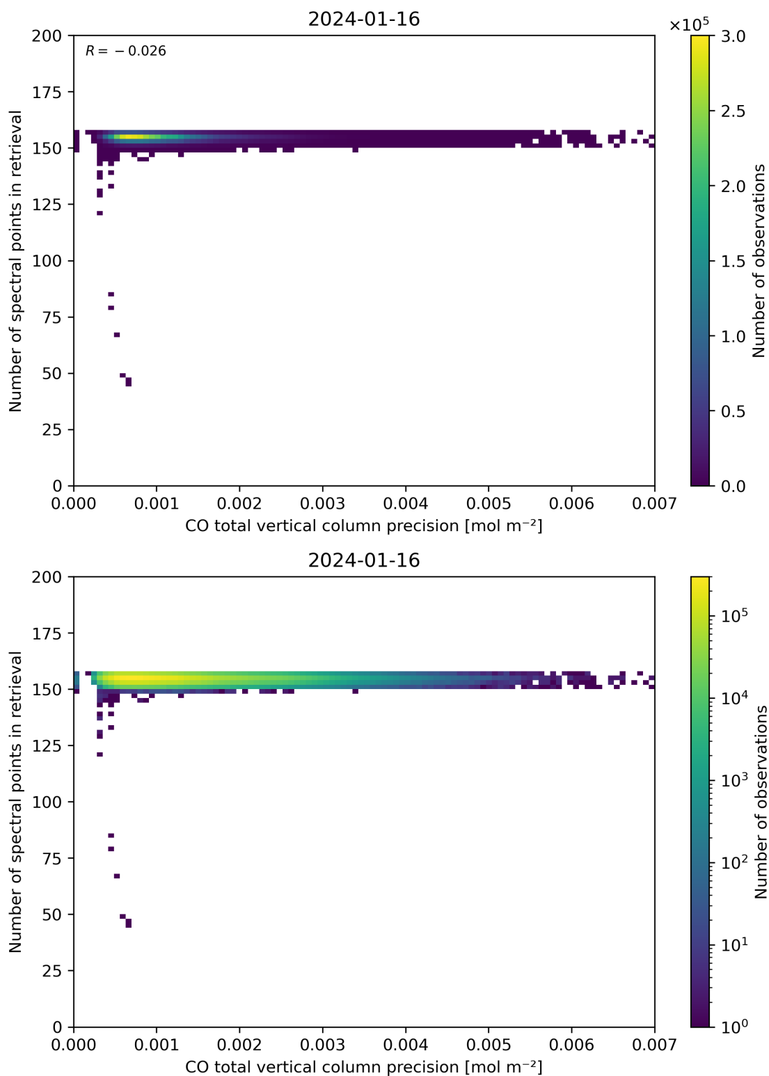
Figure 47: Scatter density plot of “CO total vertical column precision” against “Number of spectral points in retrieval” for 2024-01-15 to 2024-01-17.
