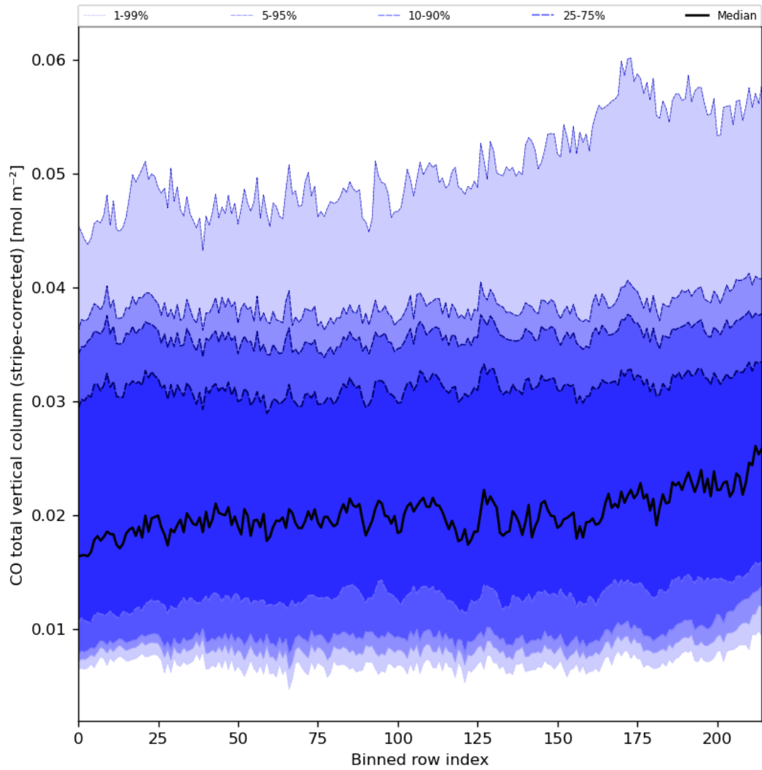
Figure 27: Along track statistics of “CO total vertical column (stripe-corrected)” for 2024-01-15 to 2024-01-17
