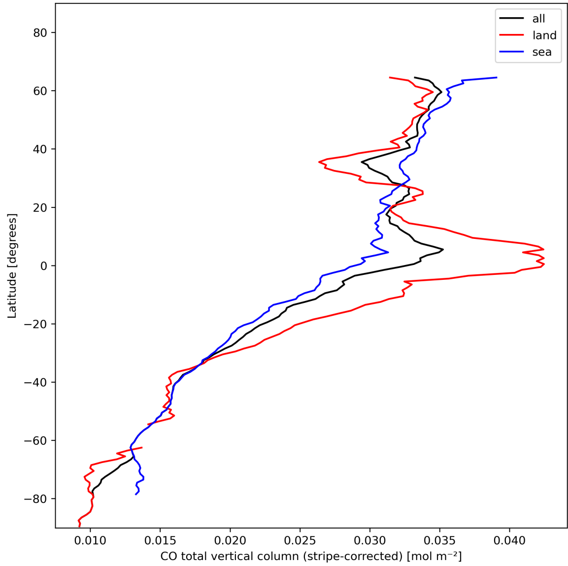
Figure 11: Zonal average of “CO total vertical column (stripe-corrected)” for 2024-01-15 to 2024-01-17.
