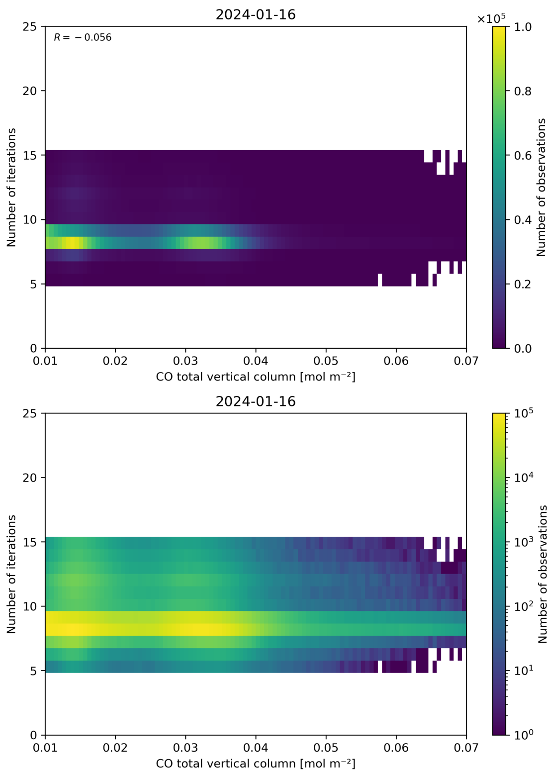
Figure 42: Scatter density plot of “CO total vertical column” against “Number of iterations” for 2024-01-15 to 2024-01-17.
