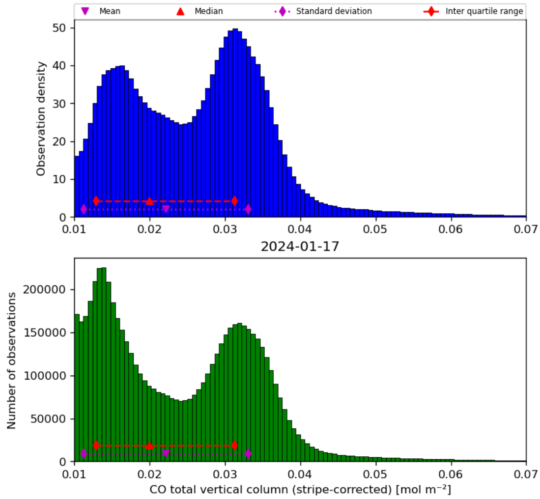
Figure 19: Histogram of “CO total vertical column (stripe-corrected)” for 2024-01-16 to 2024-01-18
