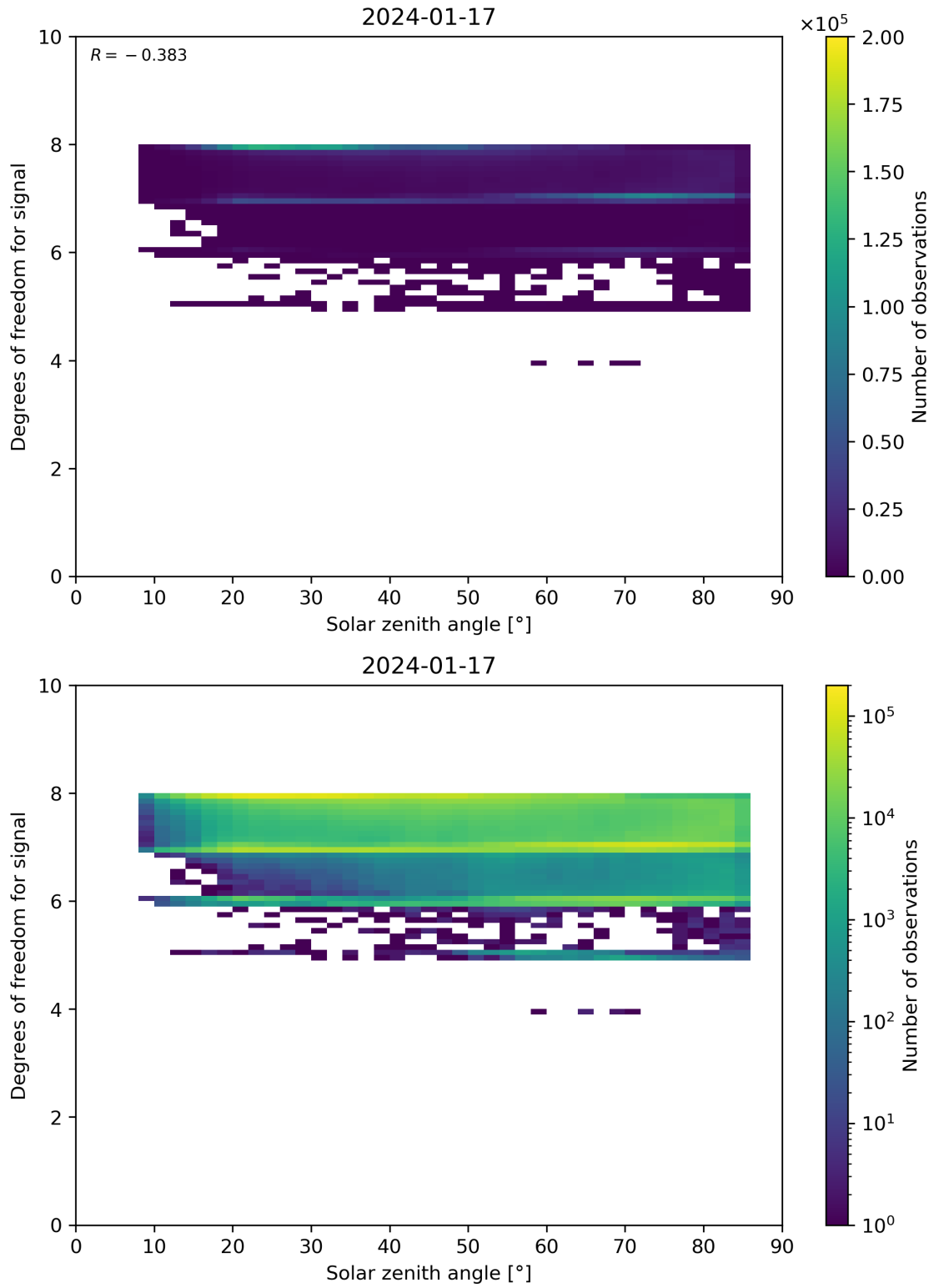
Figure 65: Scatter density plot of “Solar zenith angle” against “Degrees of freedom for signal” for 2024-01-16 to 2024-01-18.
