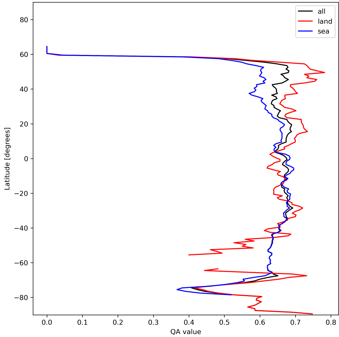
Figure 9: Zonal average of “QA value” for 2024-01-16 to 2024-01-18.
