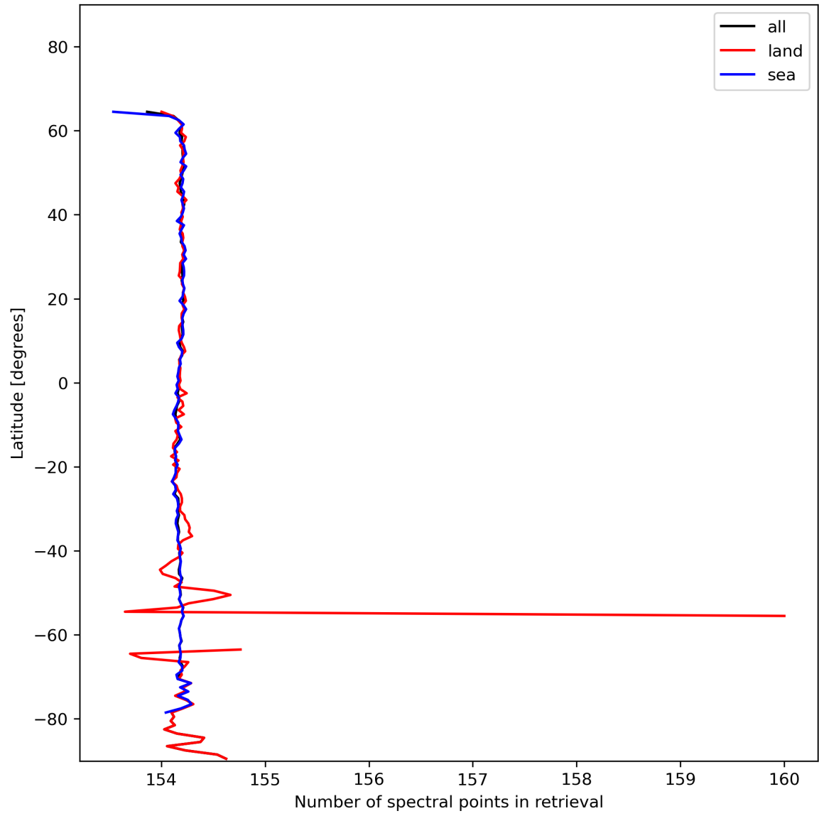
Figure 13: Zonal average of “Number of spectral points in retrieval” for 2024-01-16 to 2024-01-18.
