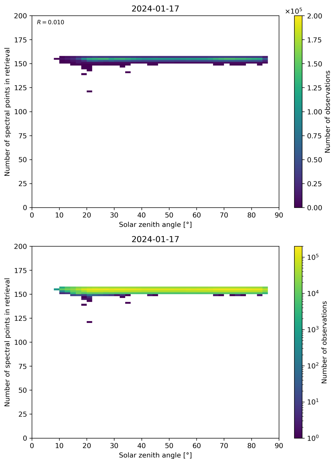
Figure 68: Scatter density plot of “Solar zenith angle” against “Number of spectral points in retrieval” for 2024-01-16 to 2024-01-18.
