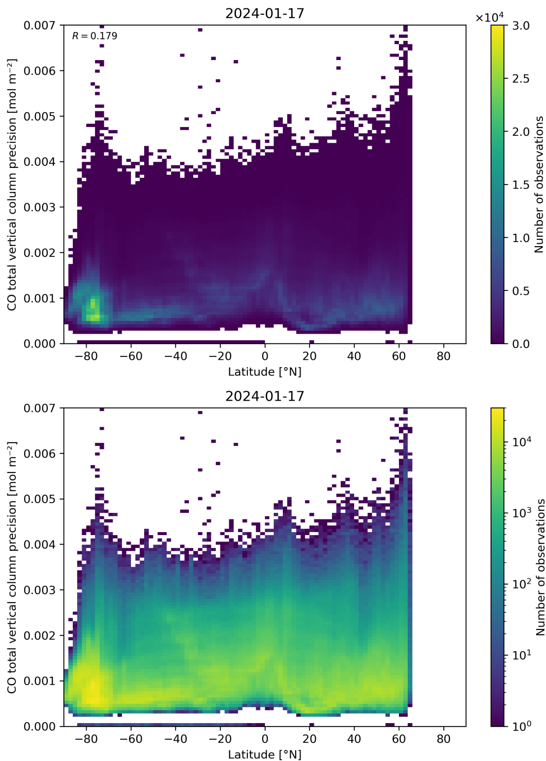
Figure 53: Scatter density plot of “Latitude” against “CO total vertical column precision” for 2024-01-16 to 2024-01-18.
