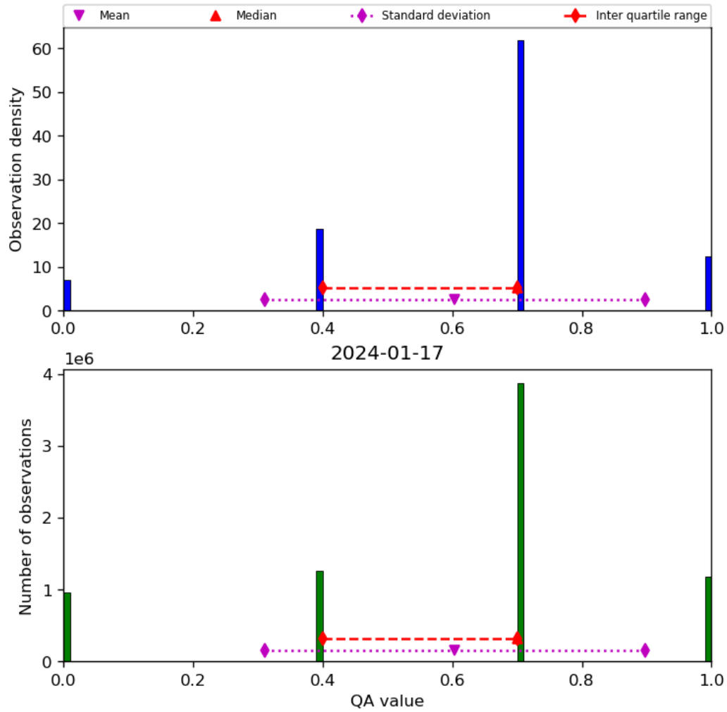
Figure 17: Histogram of “QA value” for 2024-01-16 to 2024-01-18
