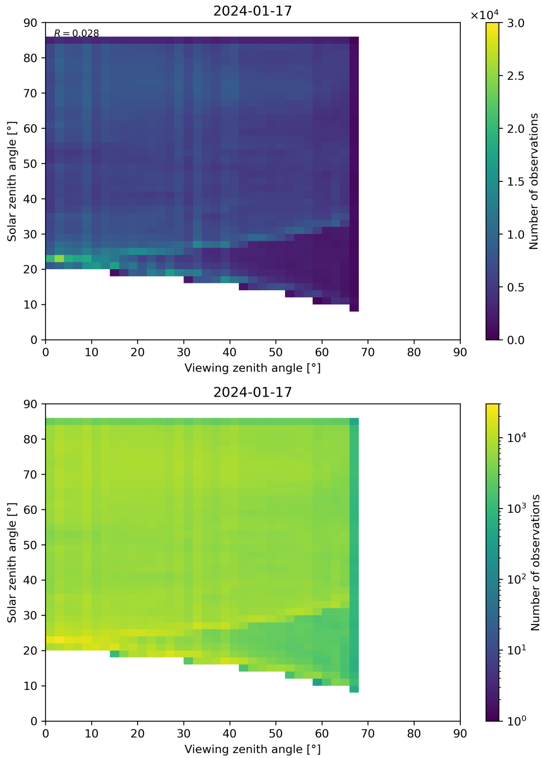
Figure 77: Scatter density plot of “Viewing zenith angle” against “Solar zenith angle” for 2024-01-16 to 2024-01-18.
