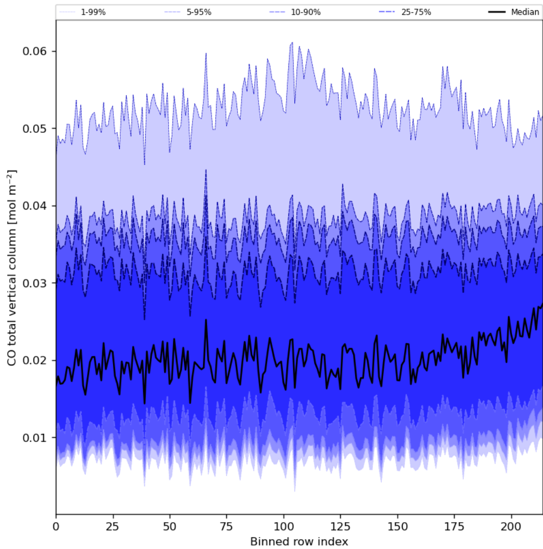
Figure 26: Along track statistics of “CO total vertical column” for 2024-01-16 to 2024-01-18
