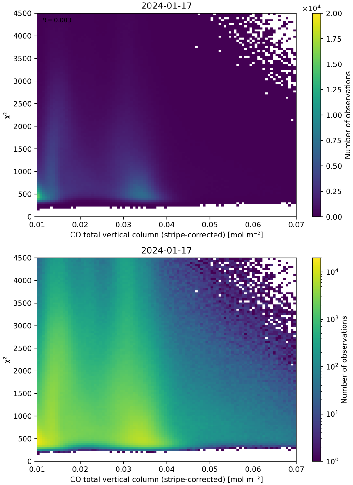
Figure 37: Scatter density plot of “CO total vertical column (stripe-corrected)” against “ \chi^2 ” for 2024-01-16 to 2024-01-18.
