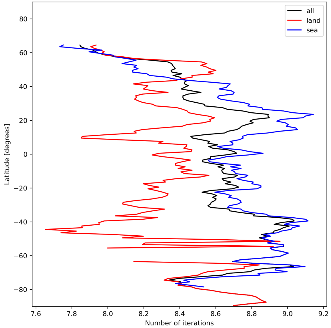
Figure 16: Zonal average of “Number of iterations” for 2024-01-16 to 2024-01-18.
