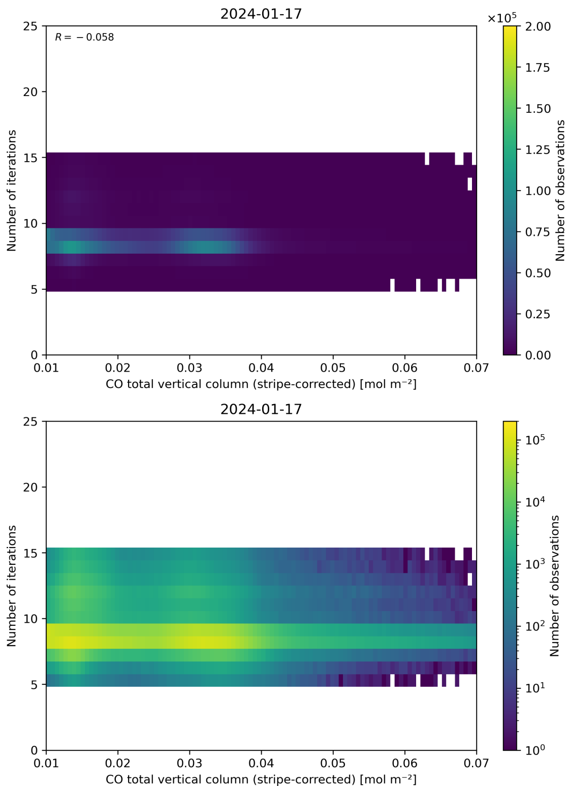
Figure 39: Scatter density plot of “CO total vertical column (stripe-corrected)” against “Number of iterations” for 2024-01-16 to 2024-01-18.
