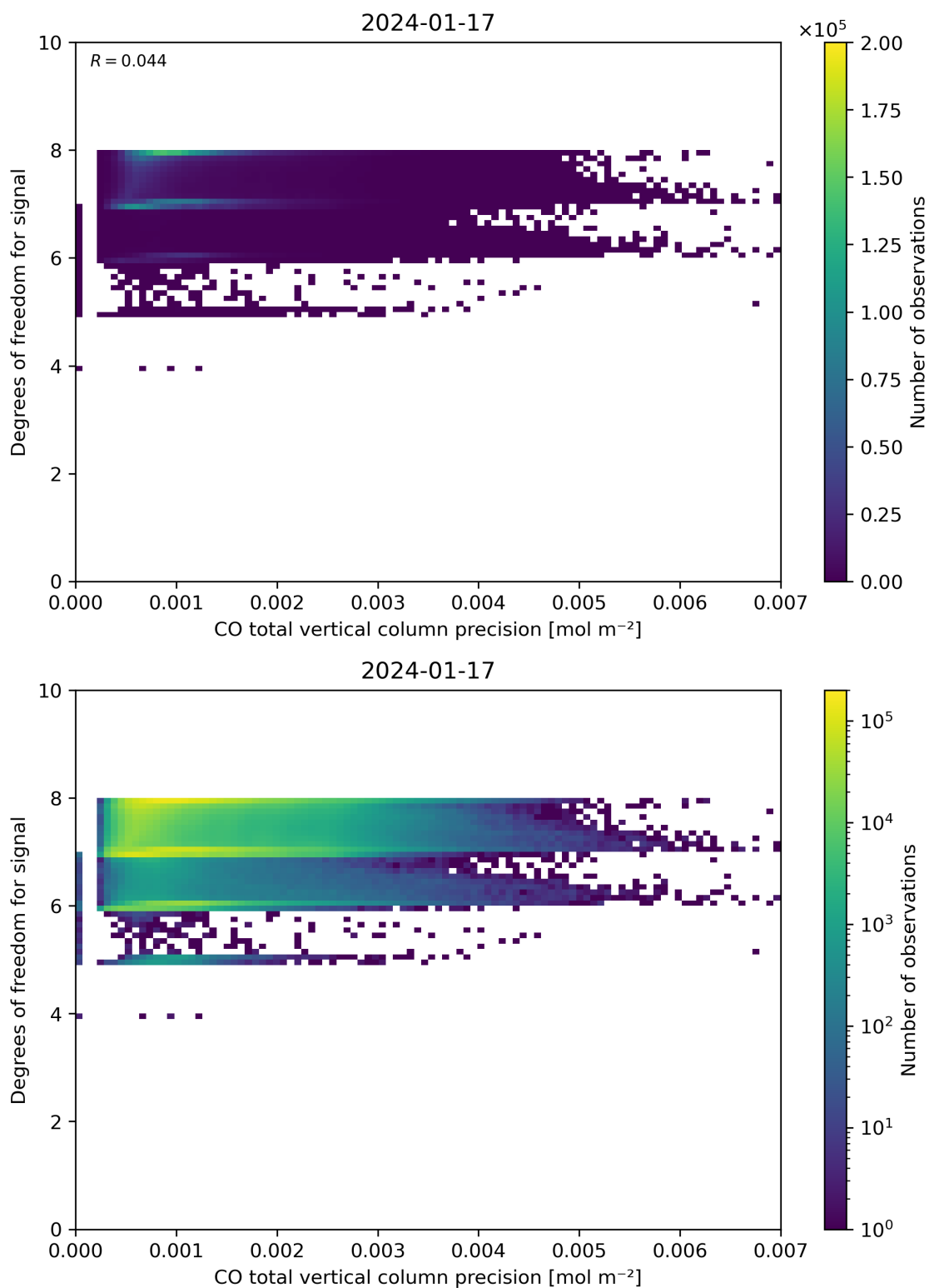
Figure 45: Scatter density plot of “CO total vertical column precision” against “Degrees of freedom for signal” for 2024-01-16 to 2024-01-18.
