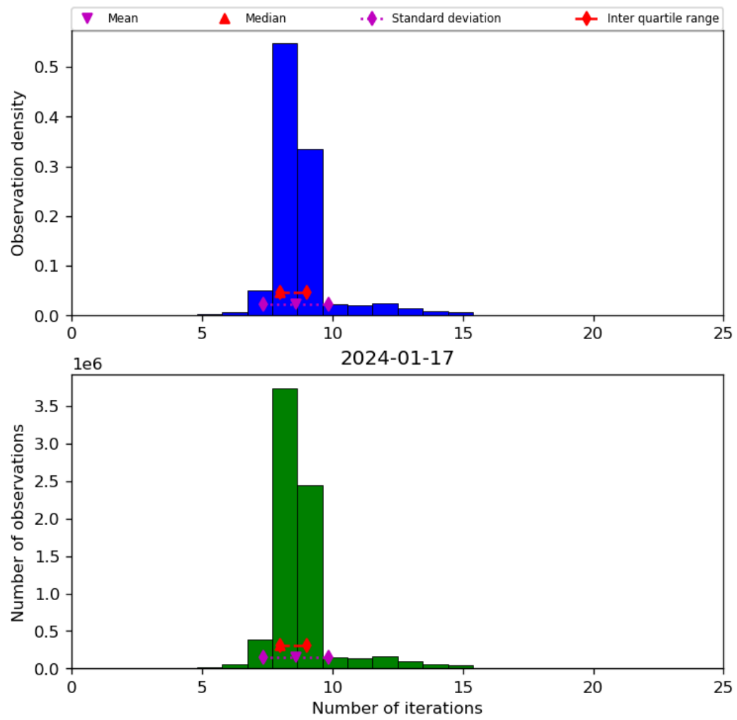
Figure 24: Histogram of “Number of iterations” for 2024-01-16 to 2024-01-18
