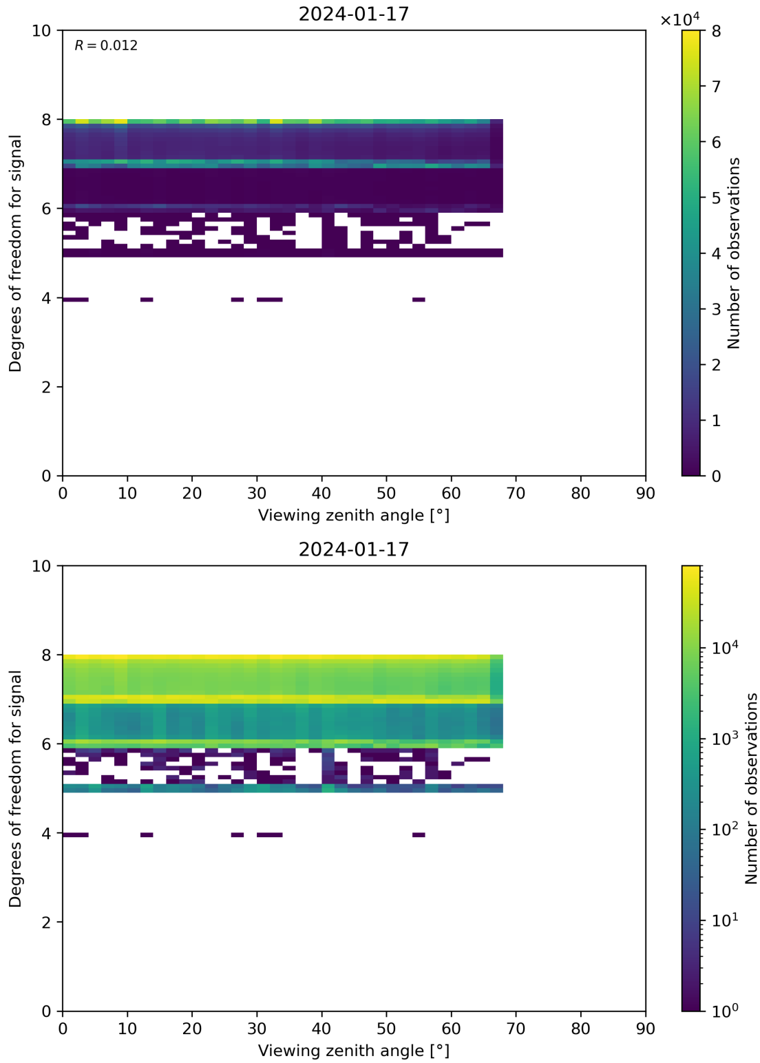
Figure 73: Scatter density plot of “Viewing zenith angle” against “Degrees of freedom for signal” for 2024-01-16 to 2024-01-18.
