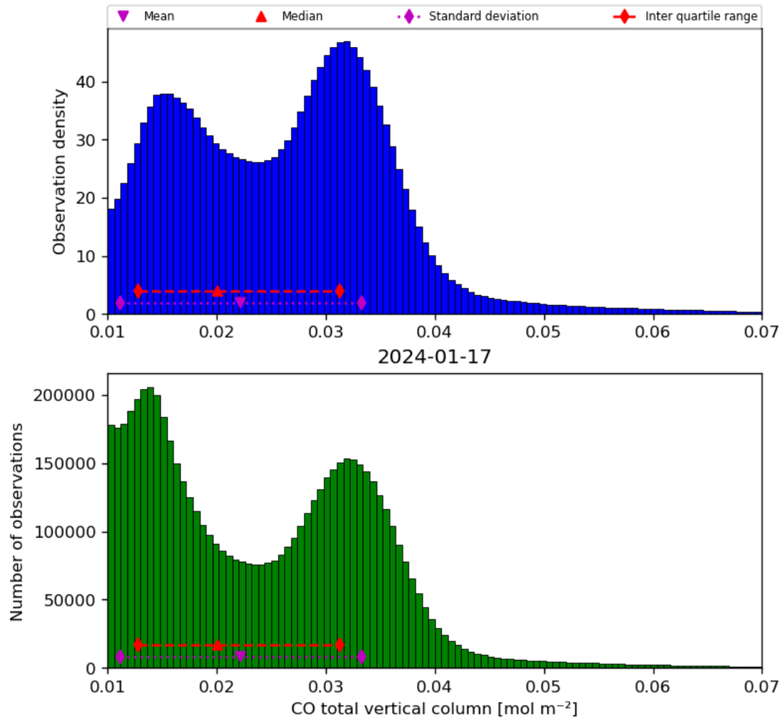
Figure 18: Histogram of “CO total vertical column” for 2024-01-16 to 2024-01-18
