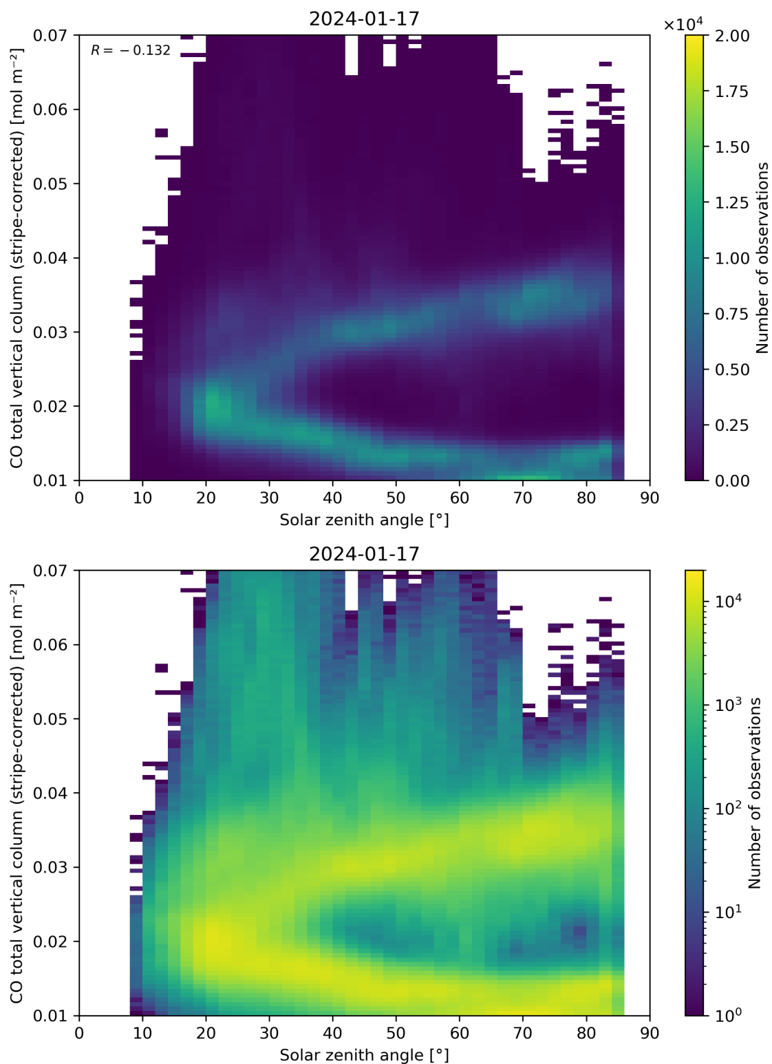
Figure 62: Scatter density plot of “Solar zenith angle” against “CO total vertical column (stripe-corrected)” for 2024-01-16 to 2024-01-18.
