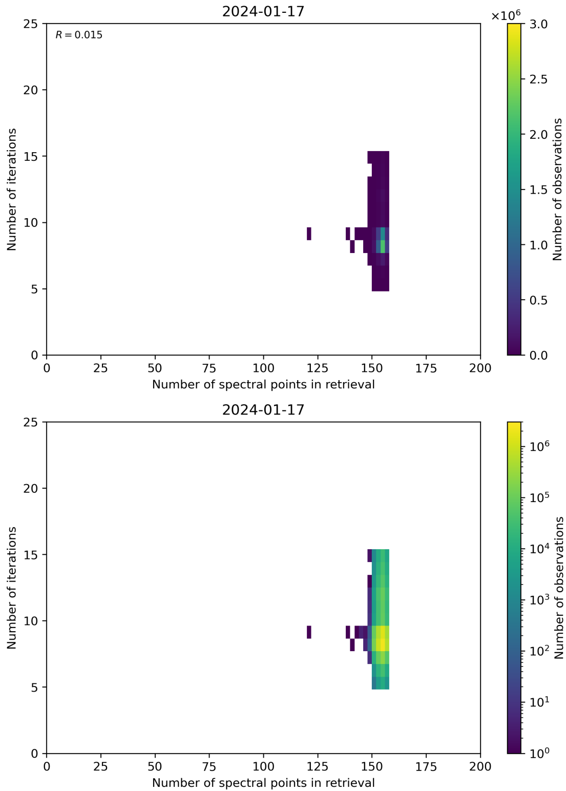
Figure 60: Scatter density plot of “Number of spectral points in retrieval” against “Number of iterations” for 2024-01-16 to 2024-01-18.
