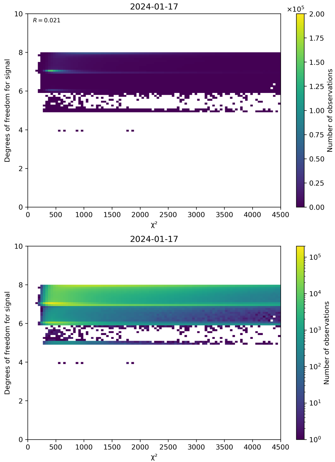
Figure 48: Scatter density plot of “ \chi^2 ” against “Degrees of freedom for signal” for 2024-01-16 to 2024-01-18.
