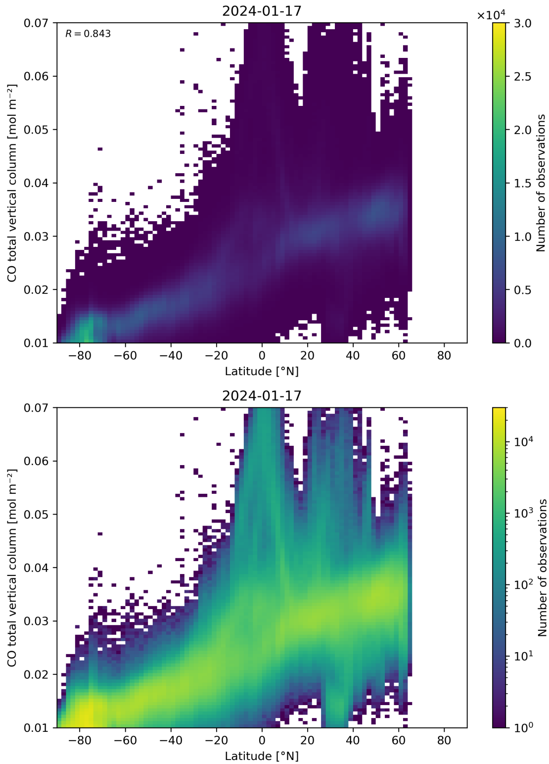
Figure 51: Scatter density plot of “Latitude” against “CO total vertical column” for 2024-01-16 to 2024-01-18.
