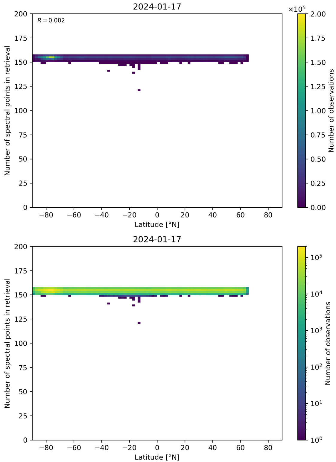
Figure 57: Scatter density plot of “Latitude” against “Number of spectral points in retrieval” for 2024-01-16 to 2024-01-18.
