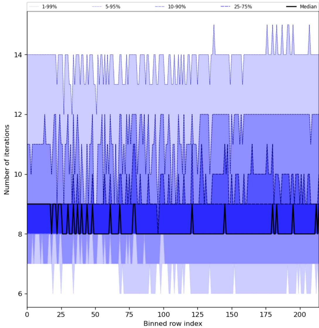
Figure 32: Along track statistics of “Number of iterations” for 2024-01-16 to 2024-01-18
