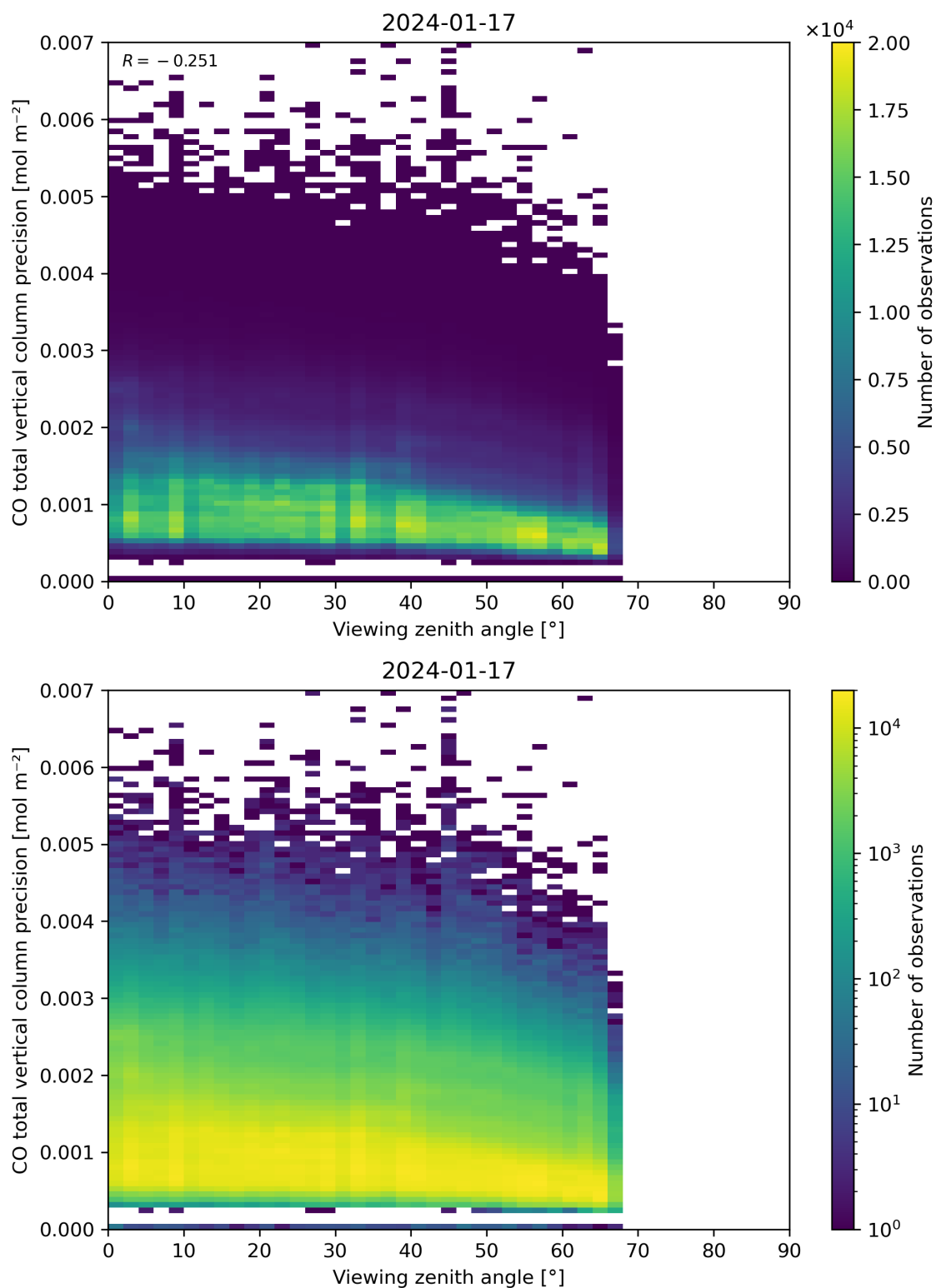
Figure 71: Scatter density plot of “Viewing zenith angle” against “CO total vertical column precision” for 2024-01-16 to 2024-01-18.
