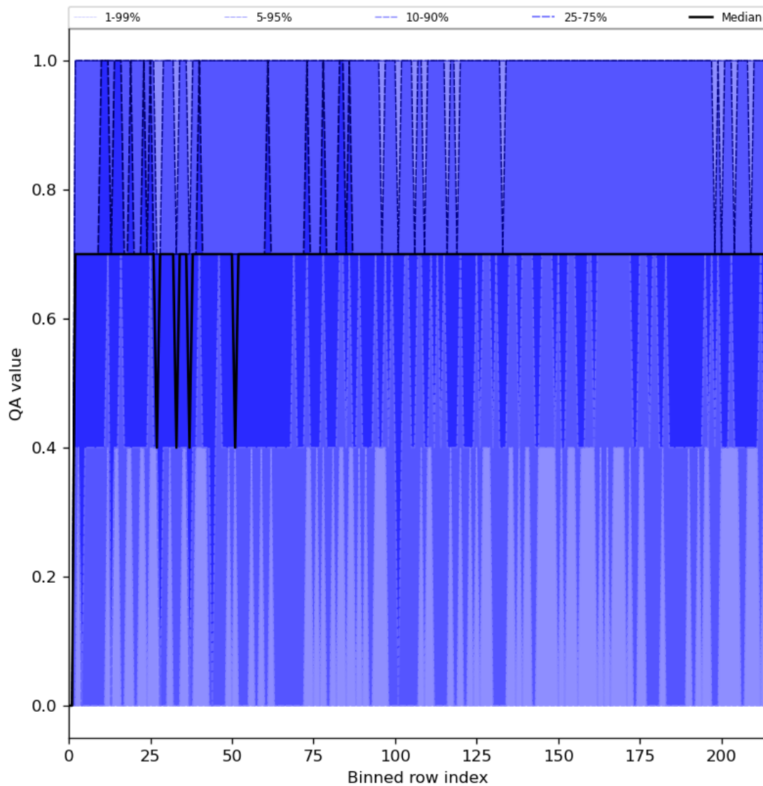
Figure 25: Along track statistics of “QA value” for 2024-01-16 to 2024-01-18
