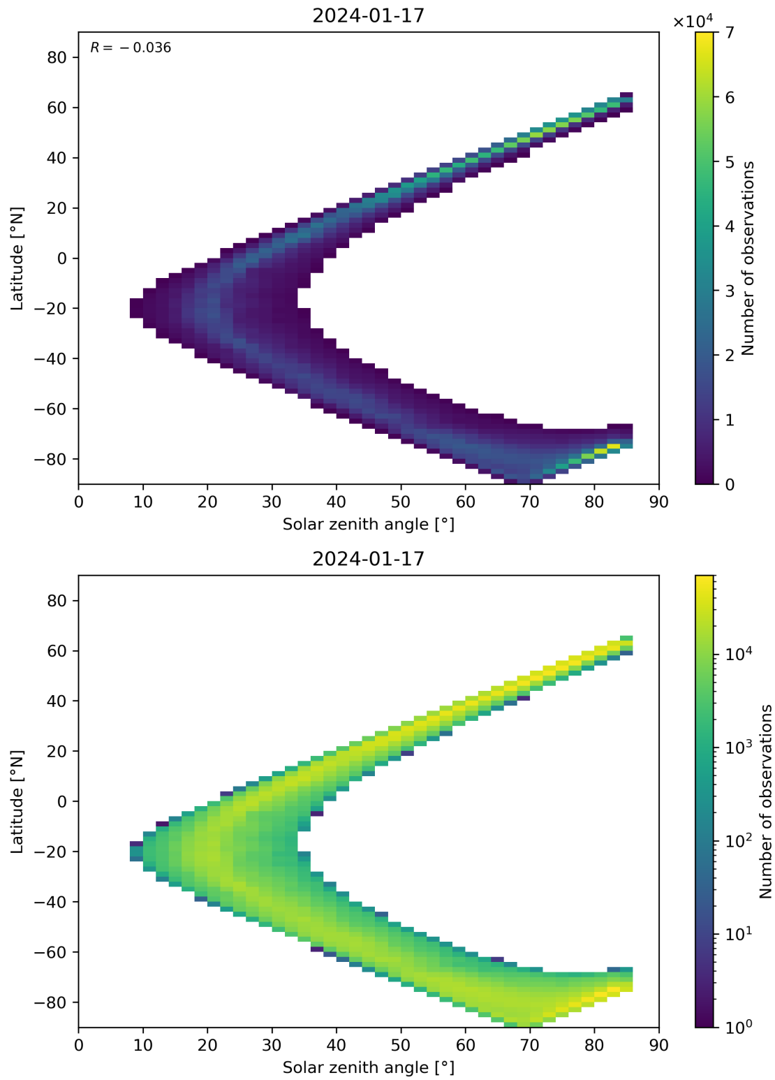
Figure 66: Scatter density plot of “Solar zenith angle” against “Latitude” for 2024-01-16 to 2024-01-18.
