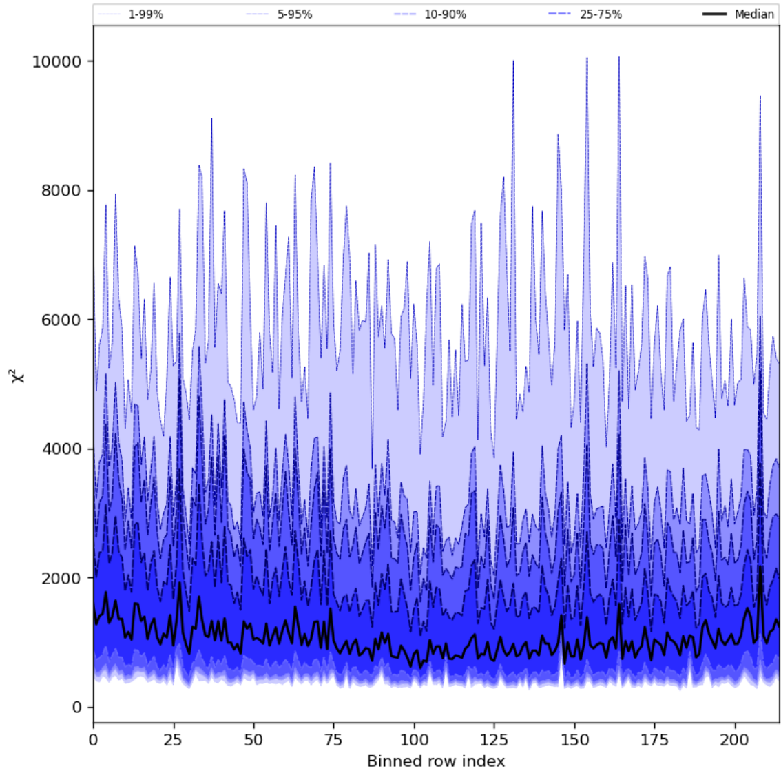
Figure 30: Along track statistics of “ \chi^2 ” for 2024-01-16 to 2024-01-18
