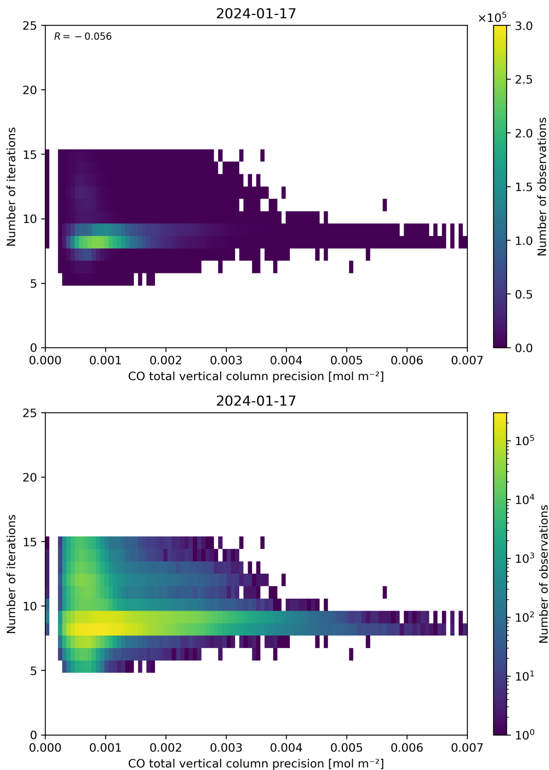
Figure 46: Scatter density plot of “CO total vertical column precision” against “Number of iterations” for 2024-01-16 to 2024-01-18.
