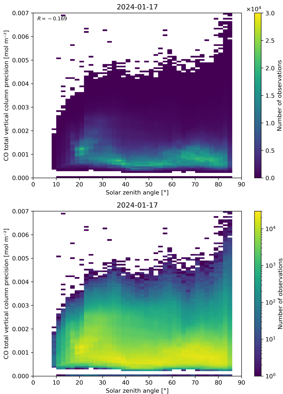
Figure 63: Scatter density plot of “Solar zenith angle” against “CO total vertical column precision” for 2024-01-16 to 2024-01-18.
