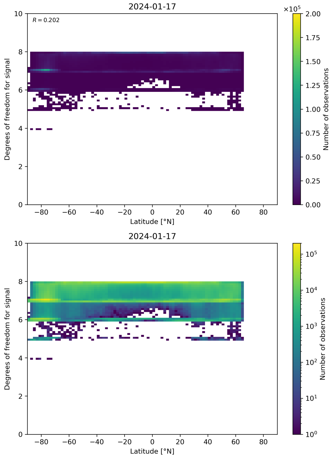
Figure 55: Scatter density plot of “Latitude” against “Degrees of freedom for signal” for 2024-01-16 to 2024-01-18.
