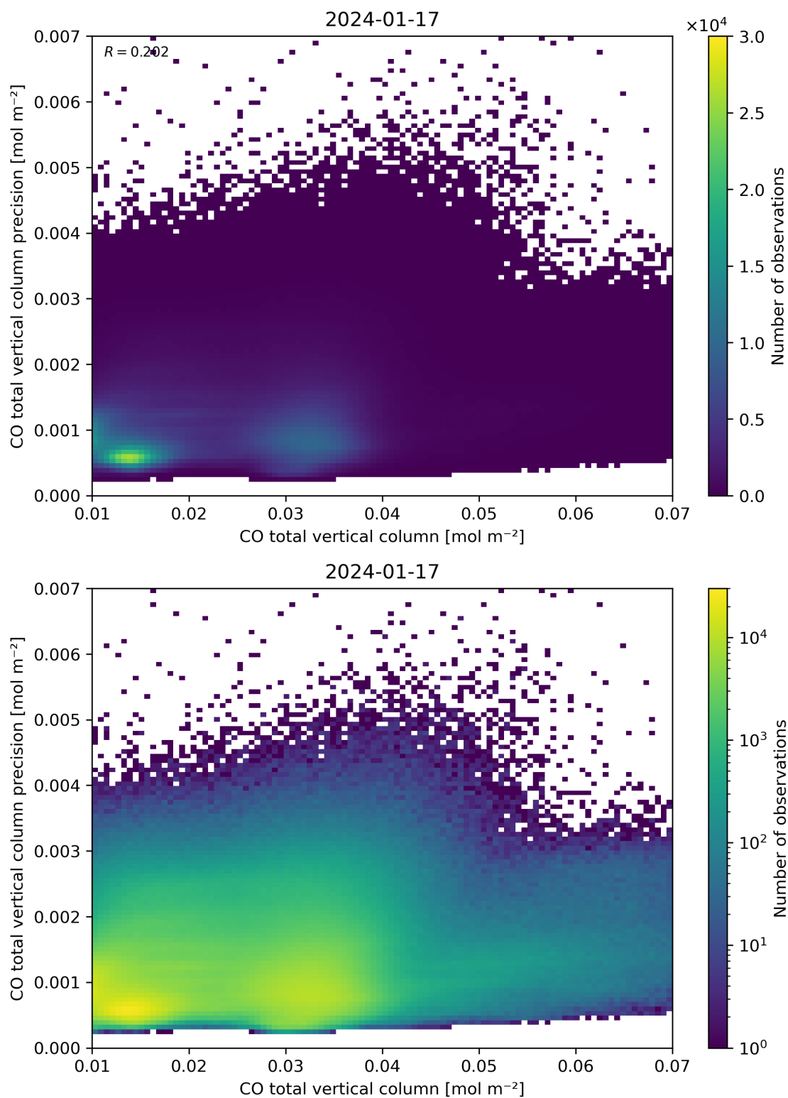
Figure 34: Scatter density plot of “CO total vertical column” against “CO total vertical column precision” for 2024-01-16 to 2024-01-18.
