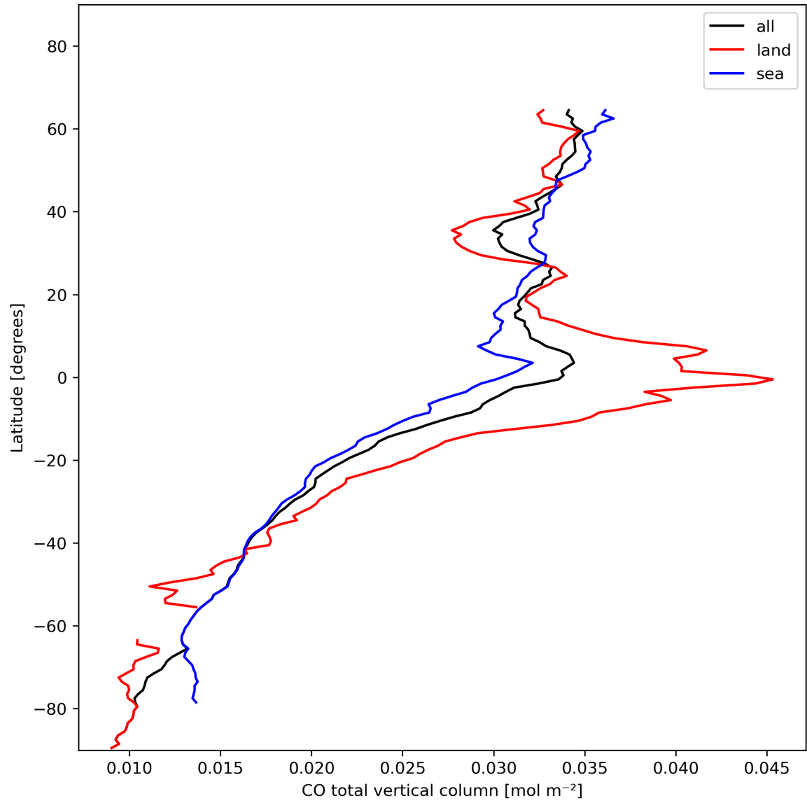
Figure 10: Zonal average of “CO total vertical column” for 2024-01-16 to 2024-01-18.
