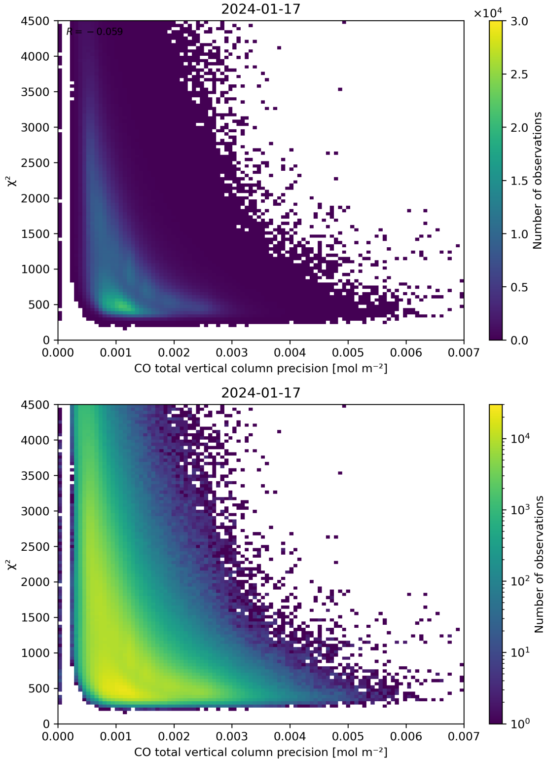
Figure 44: Scatter density plot of “CO total vertical column precision” against “ \chi^2 ” for 2024-01-16 to 2024-01-18.
