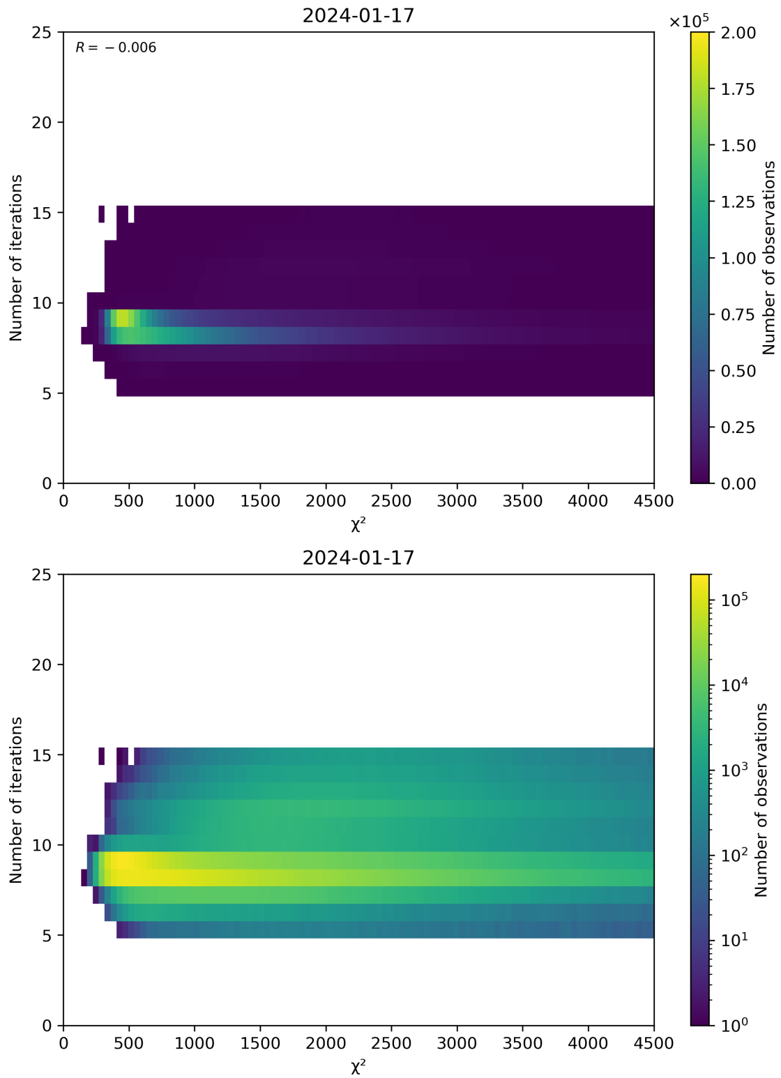
Figure 49: Scatter density plot of “ \chi^2 ” against “Number of iterations” for 2024-01-16 to 2024-01-18.
