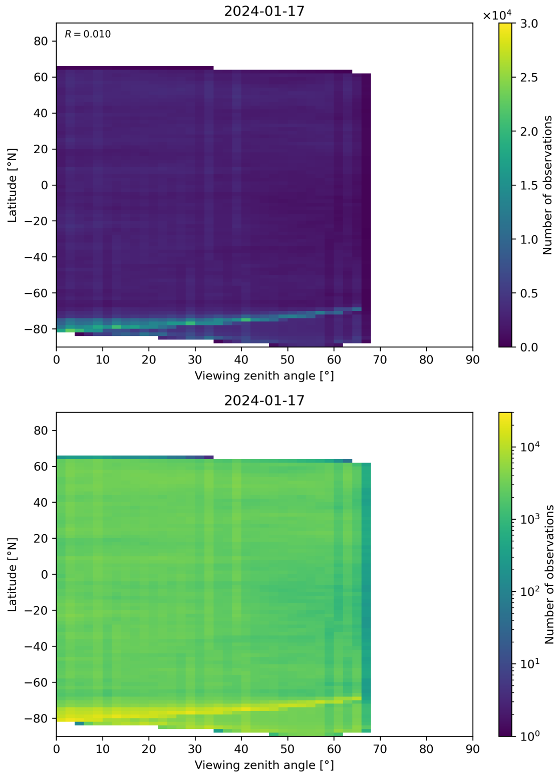
Figure 74: Scatter density plot of “Viewing zenith angle” against “Latitude” for 2024-01-16 to 2024-01-18.
