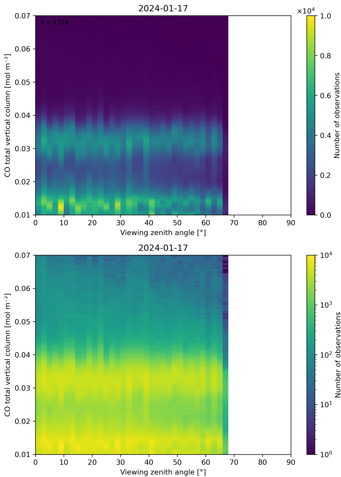
Figure 69: Scatter density plot of “Viewing zenith angle” against “CO total vertical column” for 2024-01-16 to 2024-01-18.
