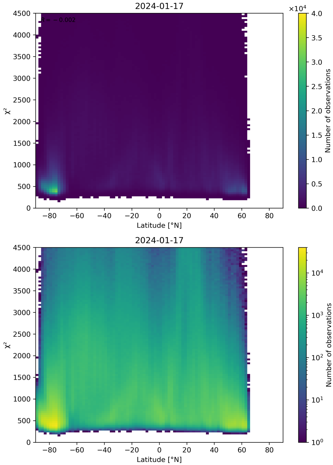
Figure 54: Scatter density plot of “Latitude” against “ \chi^2 ” for 2024-01-16 to 2024-01-18.
