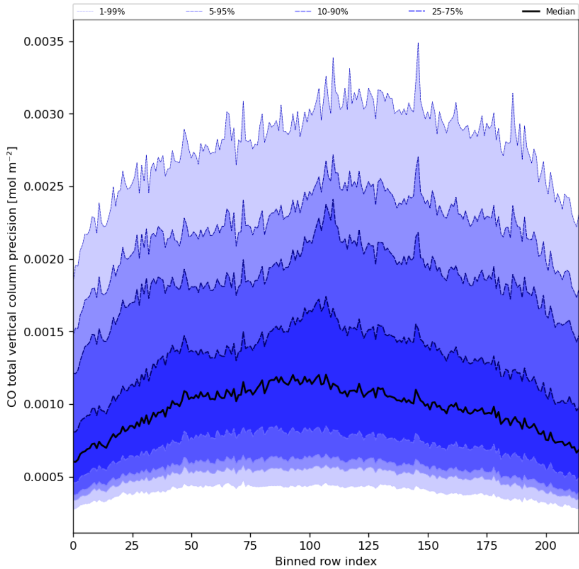
Figure 28: Along track statistics of “CO total vertical column precision” for 2024-01-16 to 2024-01-18
