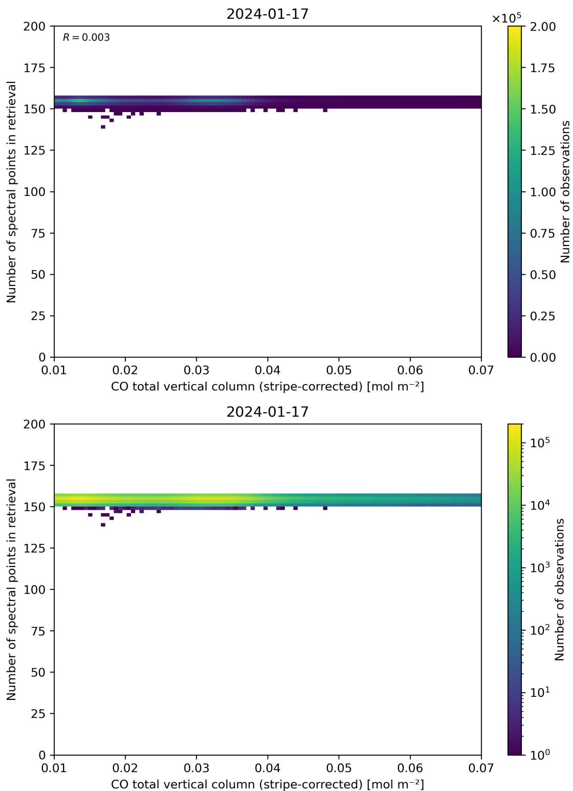
Figure 40: Scatter density plot of “CO total vertical column (stripe-corrected)” against “Number of spectral points in retrieval” for 2024-01-16 to 2024-01-18.
