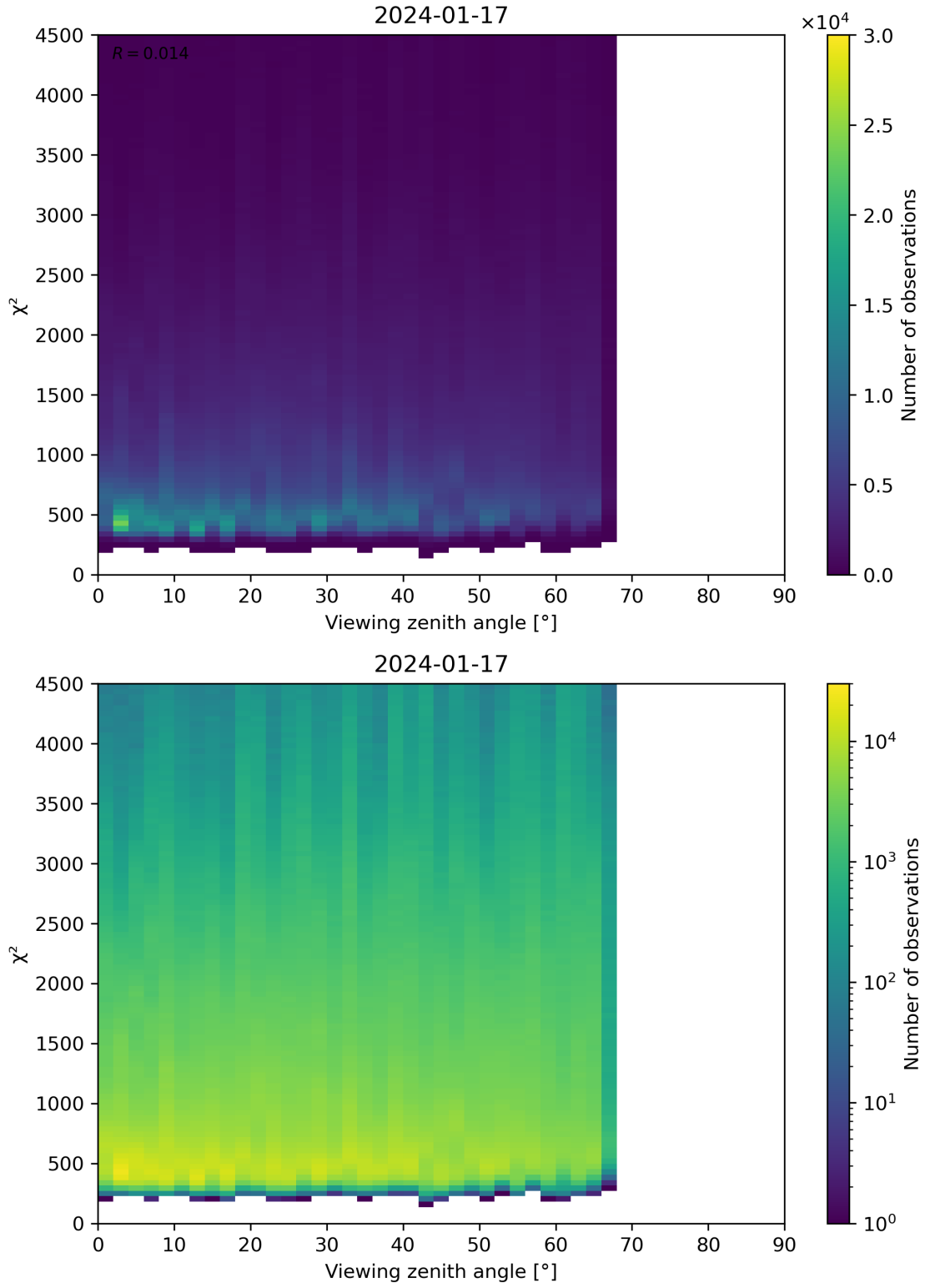
Figure 72: Scatter density plot of “Viewing zenith angle” against “ \chi^2 ” for 2024-01-16 to 2024-01-18.
