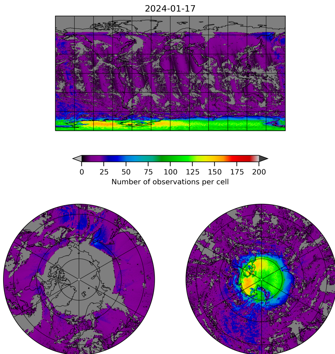
Figure 8: Map of the number of observations for 2024-01-16 to 2024-01-18
