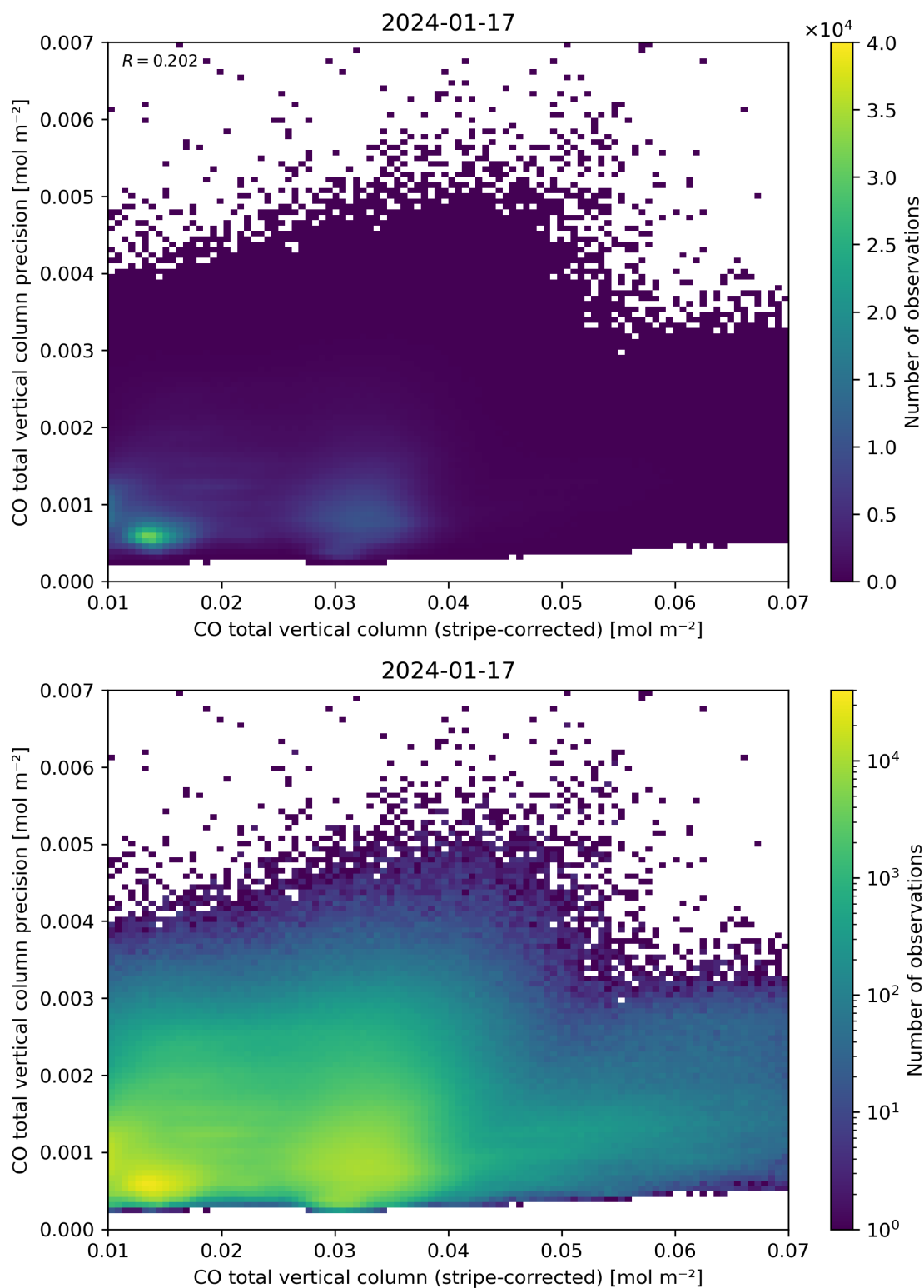
Figure 36: Scatter density plot of “CO total vertical column (stripe-corrected)” against “CO total vertical column precision” for 2024-01-16 to 2024-01-18.
