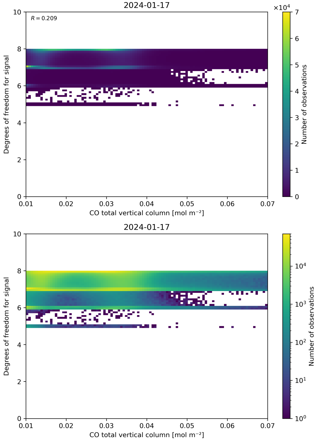
Figure 41: Scatter density plot of “CO total vertical column” against “Degrees of freedom for signal” for 2024-01-16 to 2024-01-18.
