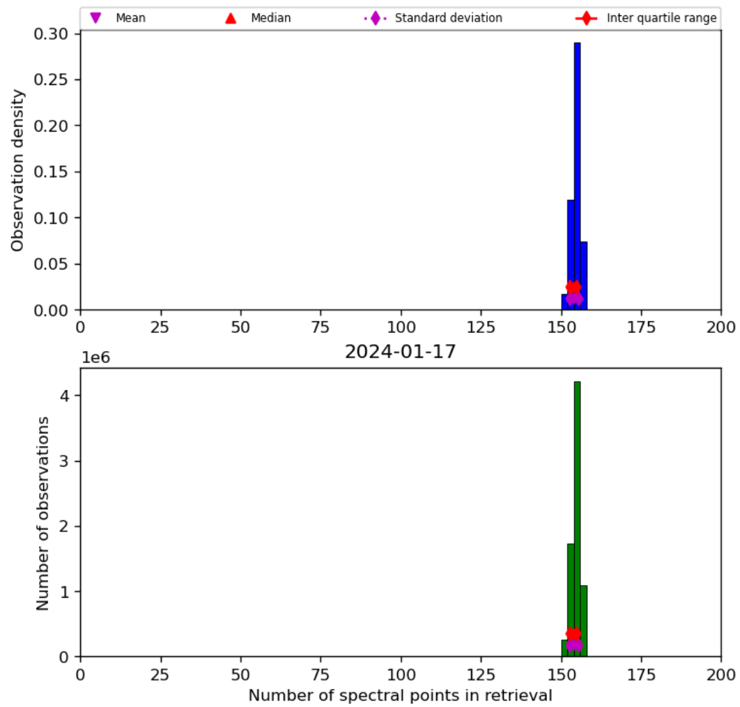
Figure 21: Histogram of “Number of spectral points in retrieval” for 2024-01-16 to 2024-01-18
