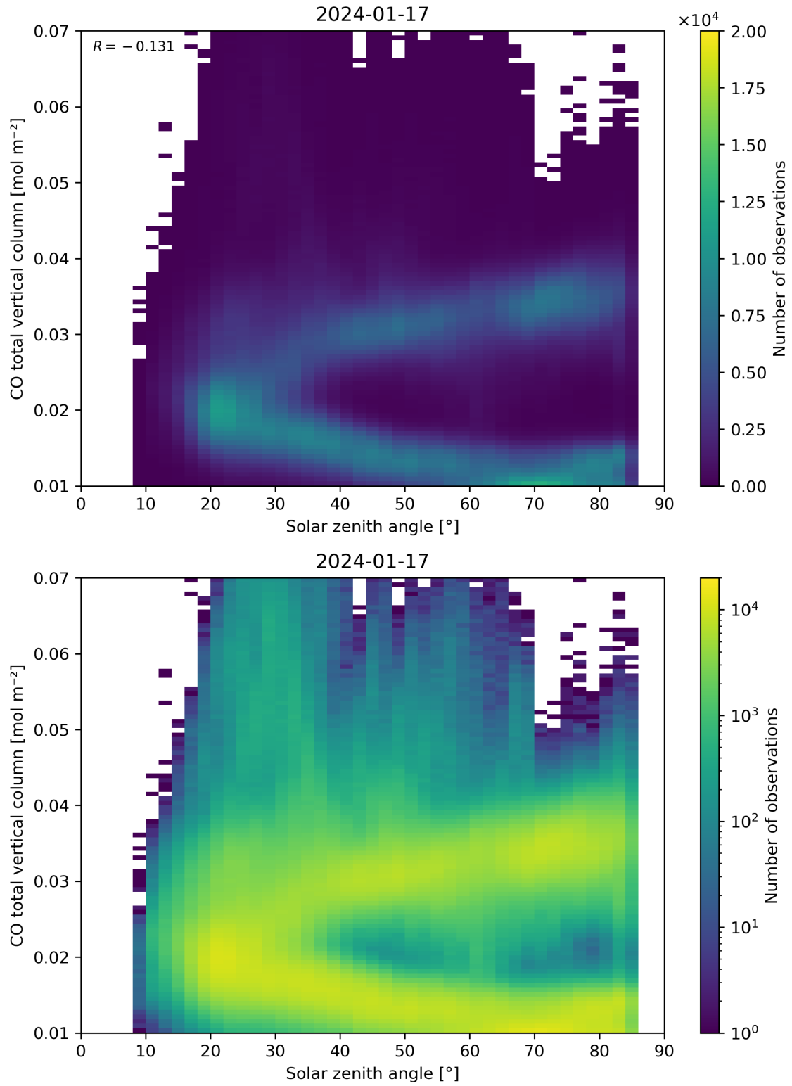
Figure 61: Scatter density plot of “Solar zenith angle” against “CO total vertical column” for 2024-01-16 to 2024-01-18.
