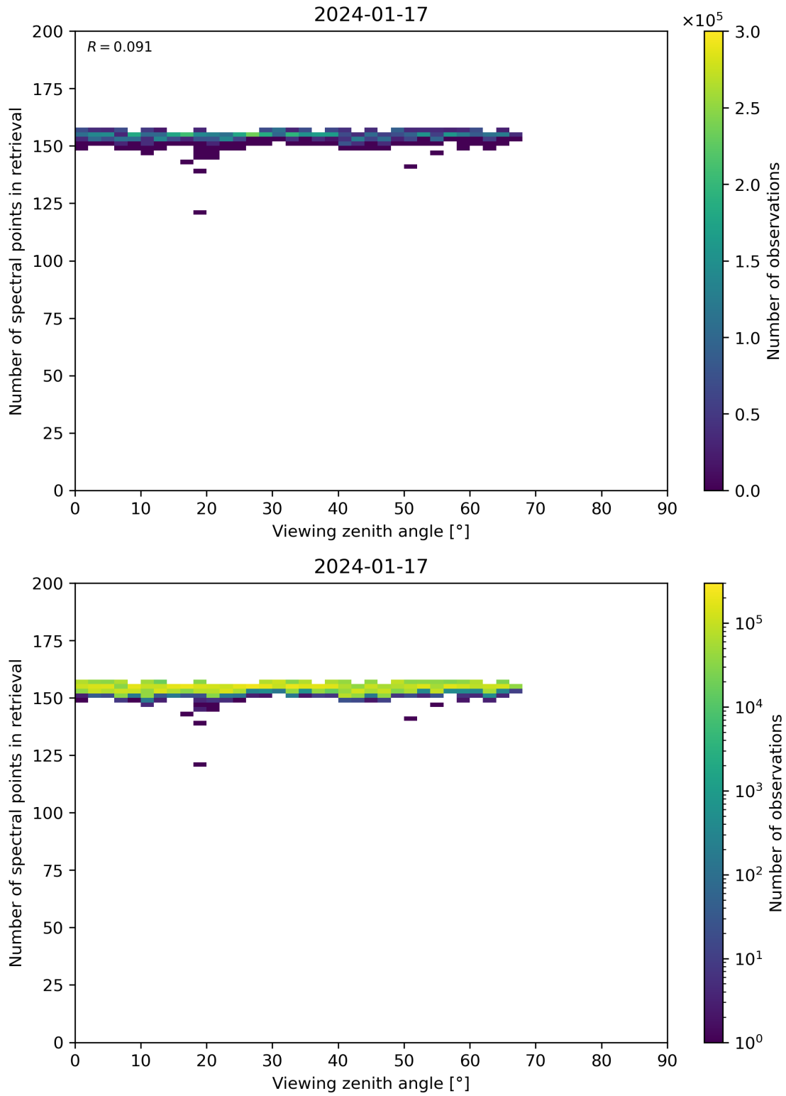
Figure 76: Scatter density plot of “Viewing zenith angle” against “Number of spectral points in retrieval” for 2024-01-16 to 2024-01-18.
