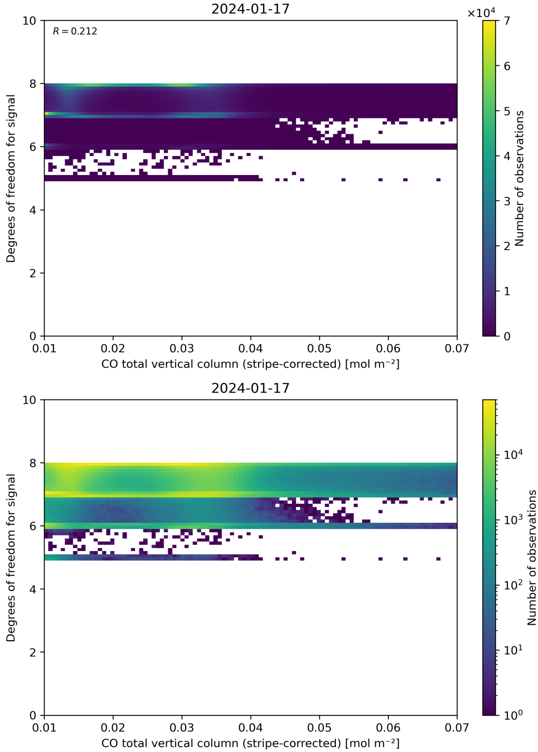
Figure 38: Scatter density plot of “CO total vertical column (stripe-corrected)” against “Degrees of freedom for signal” for 2024-01-16 to 2024-01-18.
