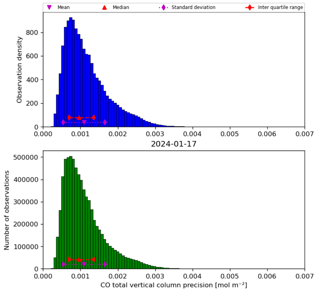
Figure 20: Histogram of “CO total vertical column precision” for 2024-01-16 to 2024-01-18
