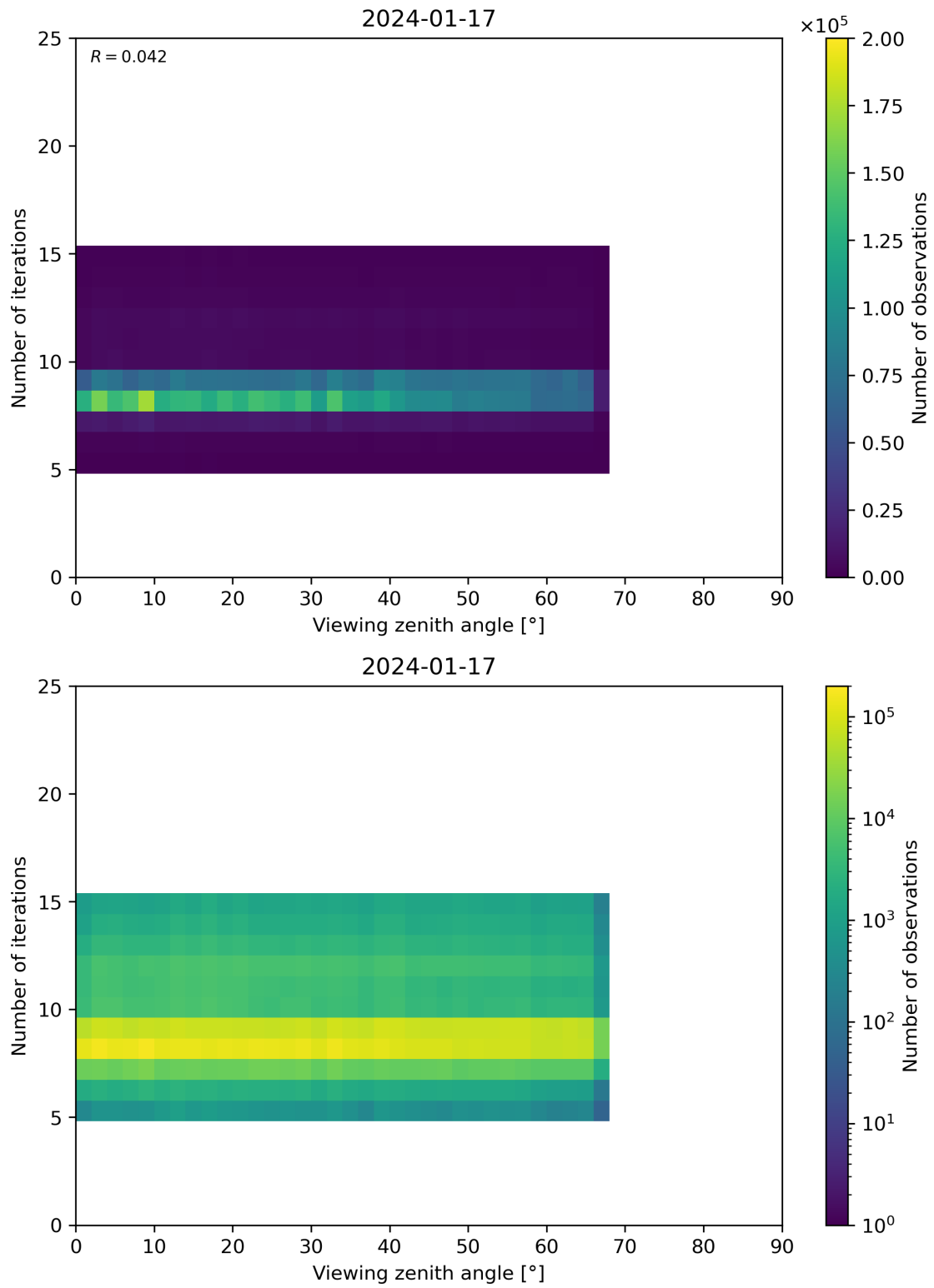
Figure 75: Scatter density plot of “Viewing zenith angle” against “Number of iterations” for 2024-01-16 to 2024-01-18.
