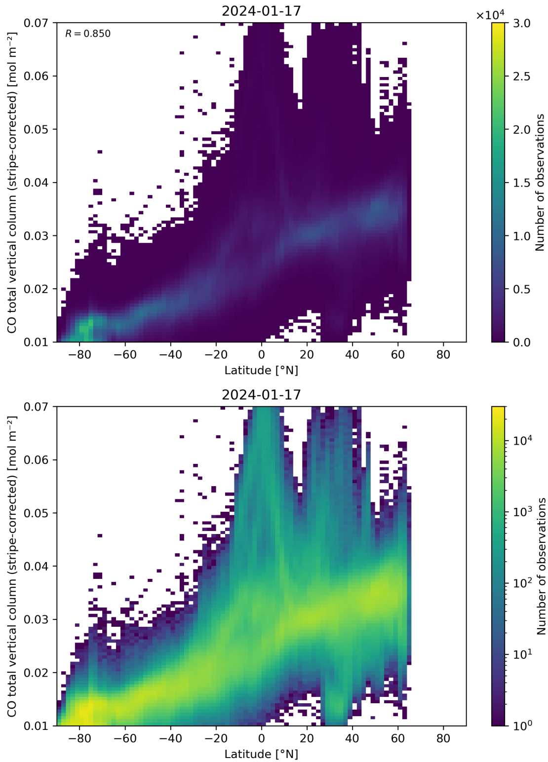
Figure 52: Scatter density plot of “Latitude” against “CO total vertical column (stripe-corrected)” for 2024-01-16 to 2024-01-18.
