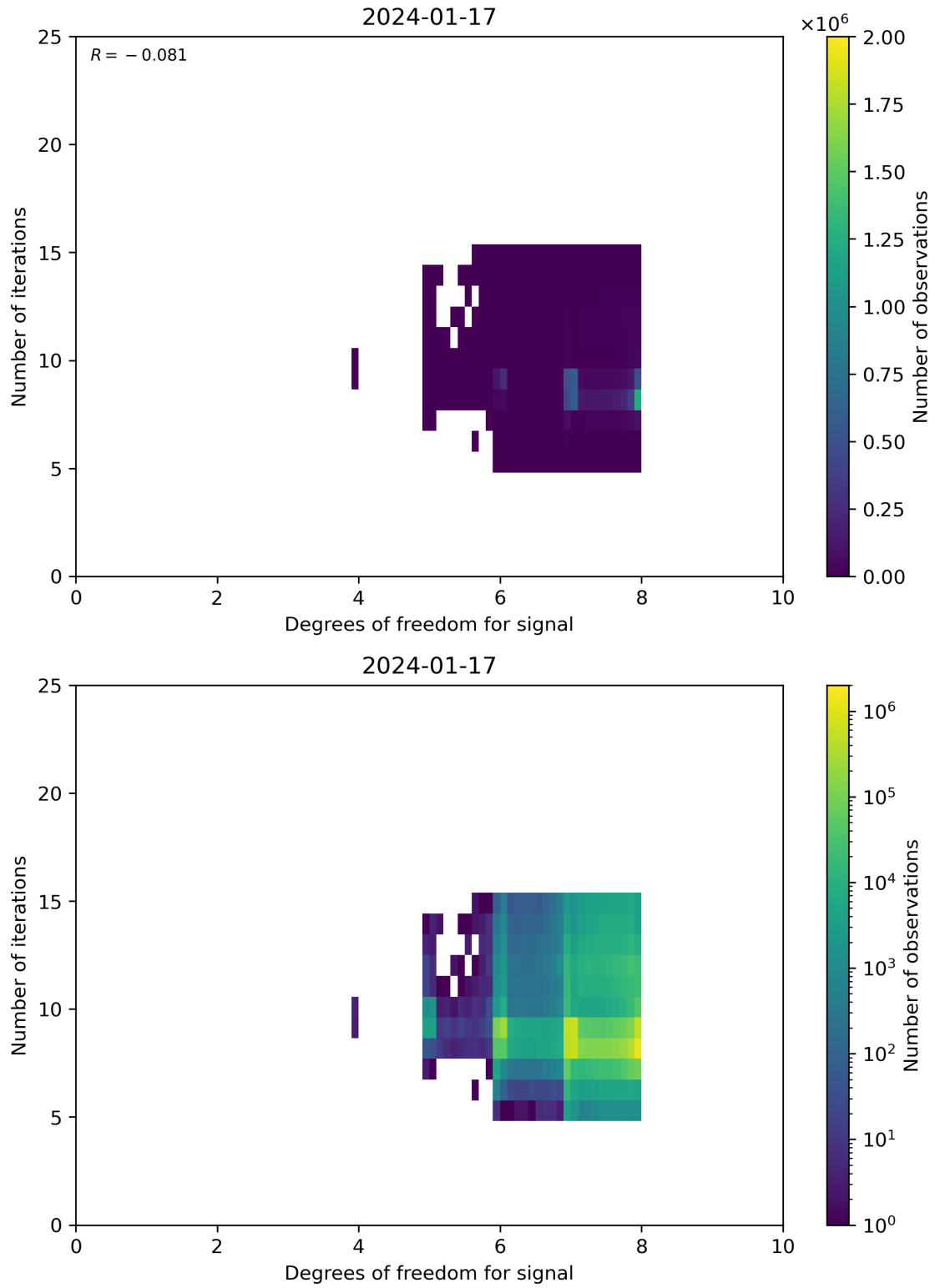
Figure 50: Scatter density plot of “Degrees of freedom for signal” against “Number of iterations” for 2024-01-16 to 2024-01-18.
