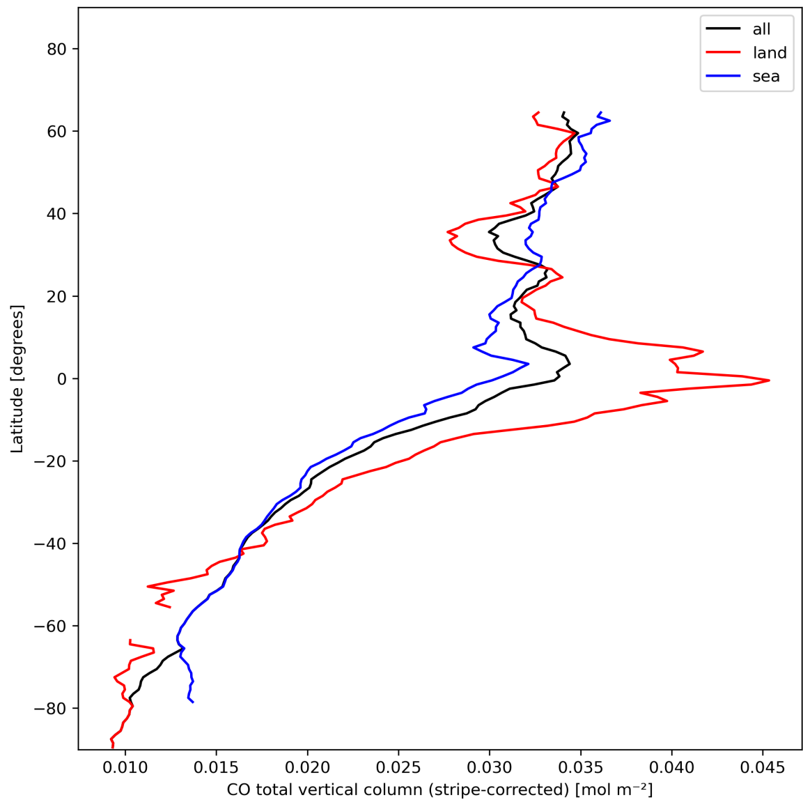
Figure 11: Zonal average of “CO total vertical column (stripe-corrected)” for 2024-01-16 to 2024-01-18.
