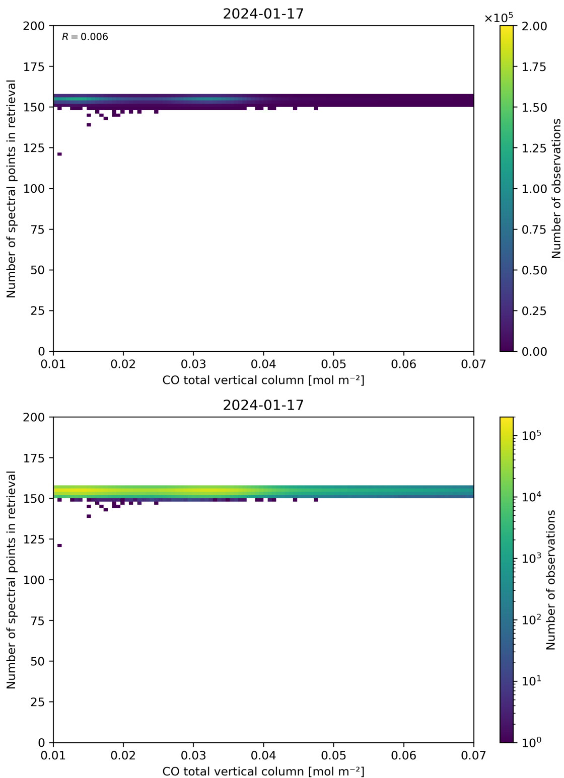
Figure 43: Scatter density plot of “CO total vertical column” against “Number of spectral points in retrieval” for 2024-01-16 to 2024-01-18.
