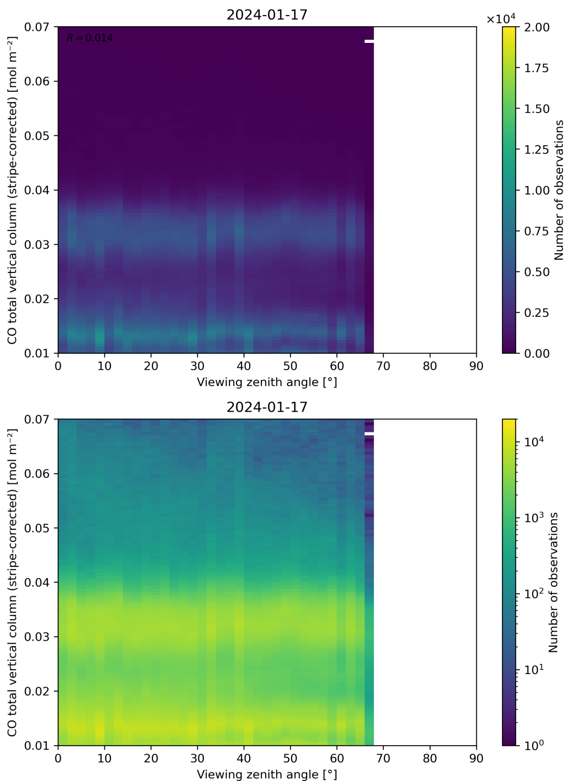
Figure 70: Scatter density plot of “Viewing zenith angle” against “CO total vertical column (stripe-corrected)” for 2024-01-16 to 2024-01-18.
