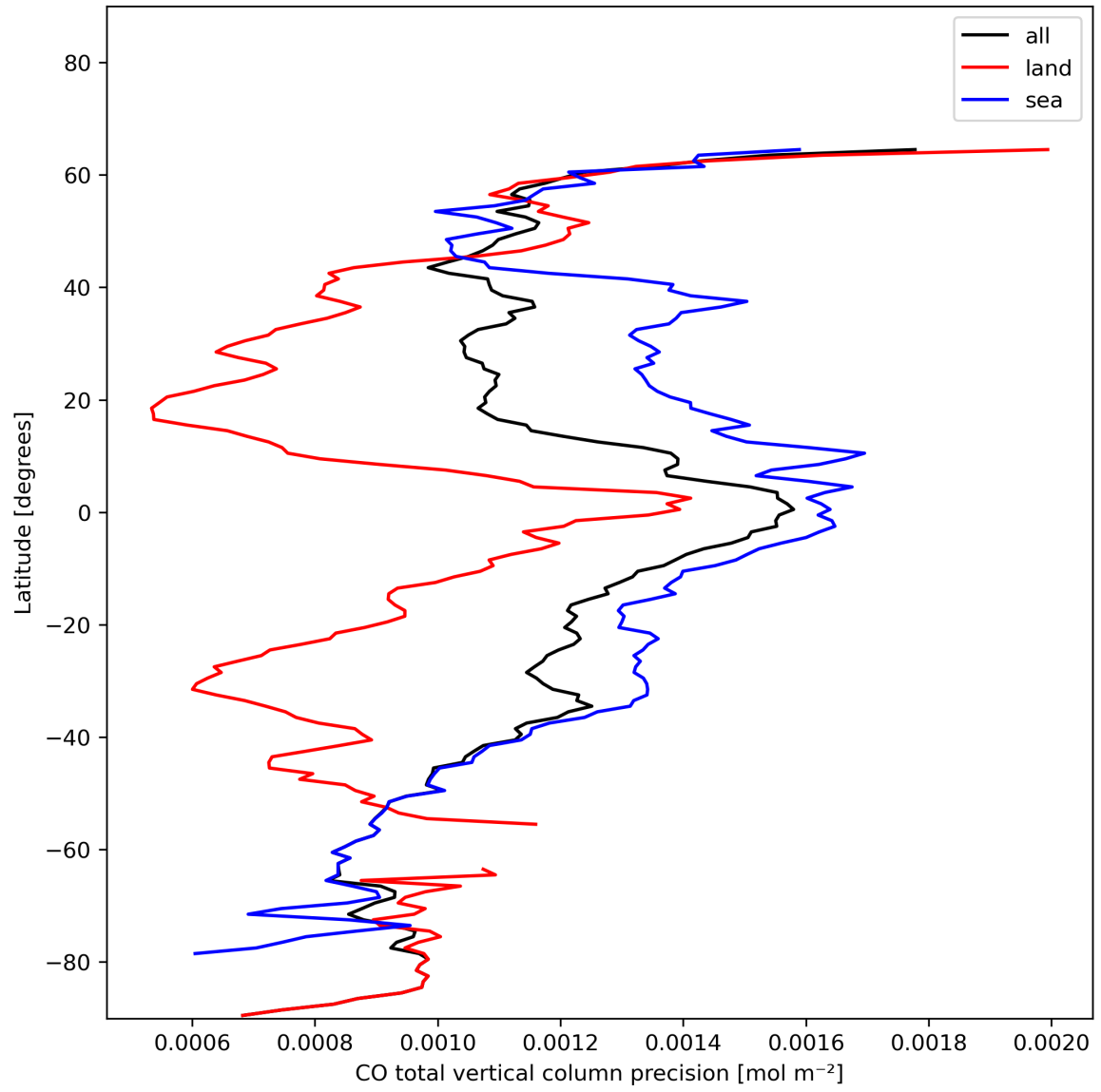
Figure 12: Zonal average of "CO total vertical column precision" for 2024-01-16 to 2024-01-18.
