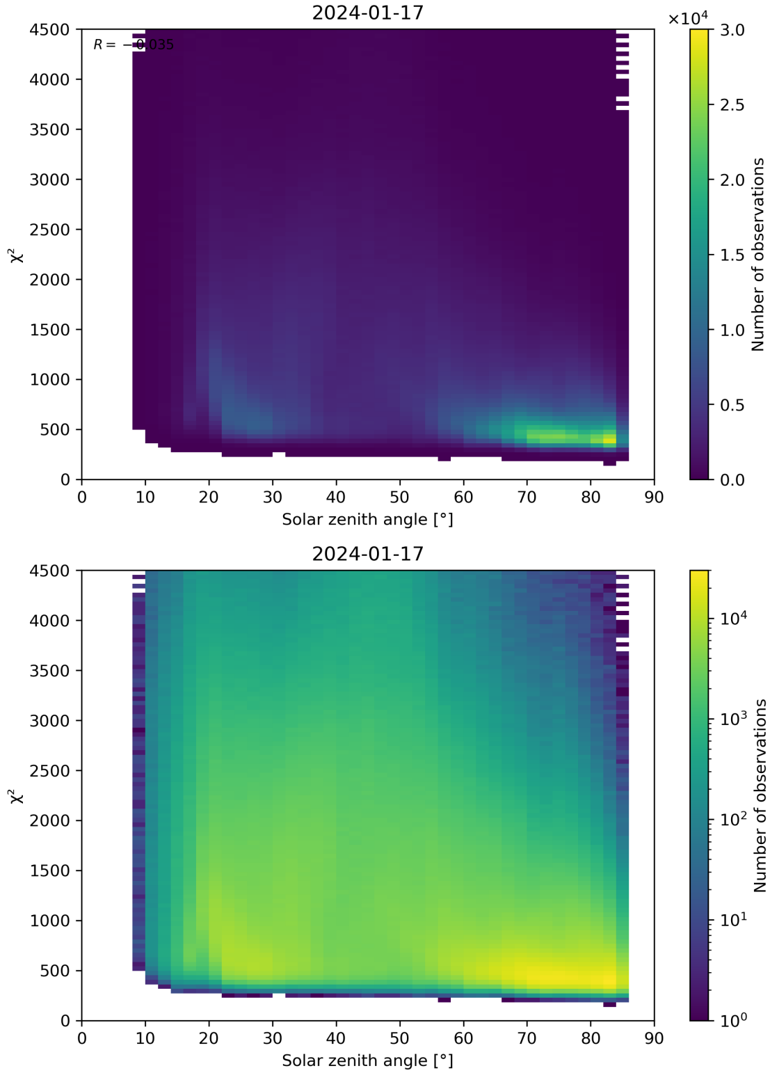
Figure 64: Scatter density plot of “Solar zenith angle” against “ \chi^2 ” for 2024-01-16 to 2024-01-18.
