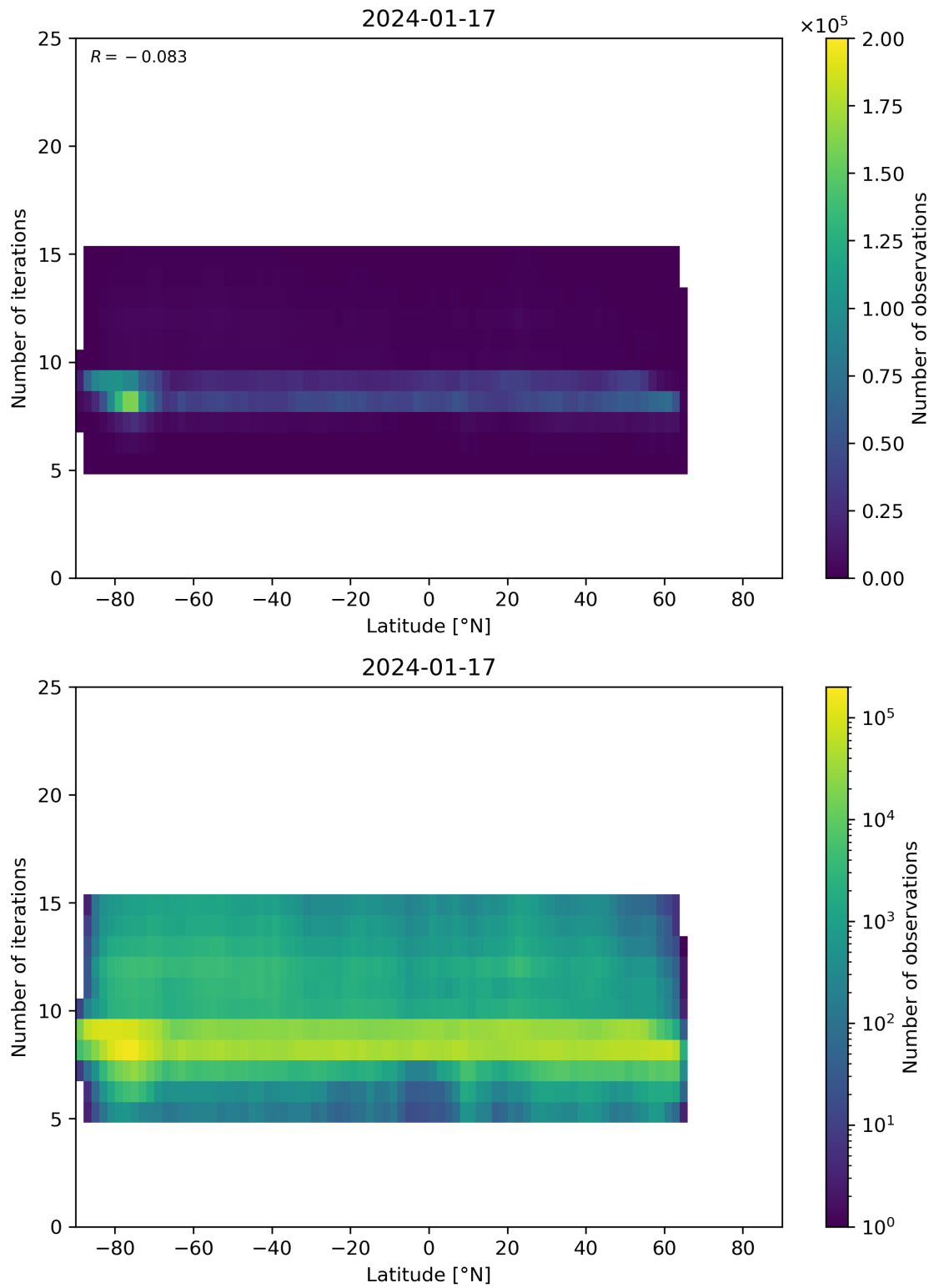
Figure 56: Scatter density plot of “Latitude” against “Number of iterations” for 2024-01-16 to 2024-01-18.
