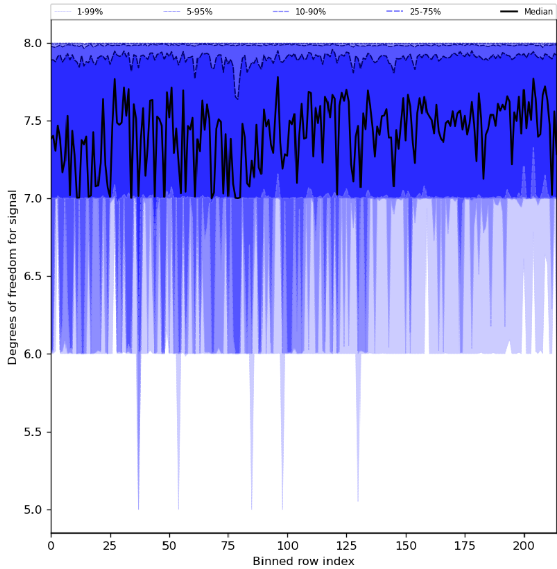
Figure 31: Along track statistics of “Degrees of freedom for signal” for 2024-01-16 to 2024-01-18
