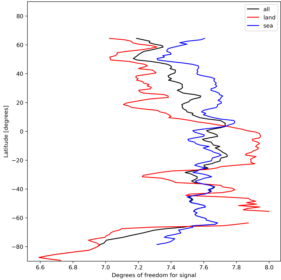
Figure 15: Zonal average of “Degrees of freedom for signal” for 2024-01-16 to 2024-01-18.
