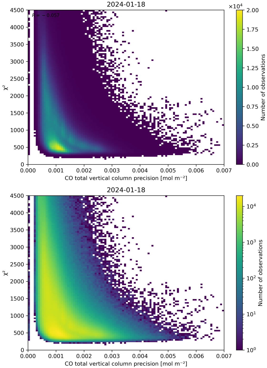
Figure 44: Scatter density plot of “CO total vertical column precision” against “ \chi^2 ” for 2024-01-17 to 2024-01-19.
