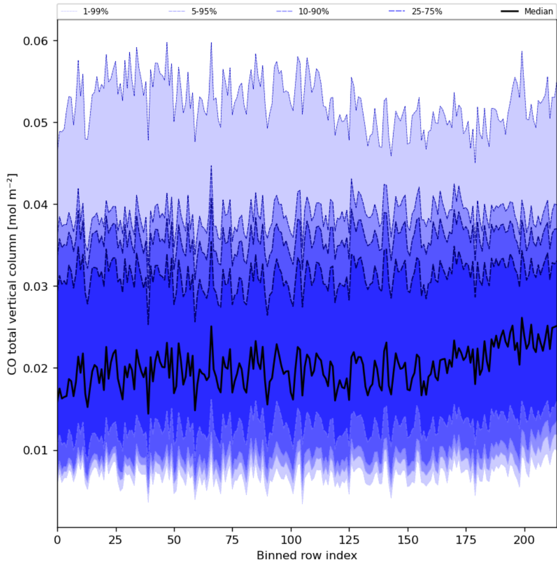
Figure 26: Along track statistics of “CO total vertical column” for 2024-01-17 to 2024-01-19
