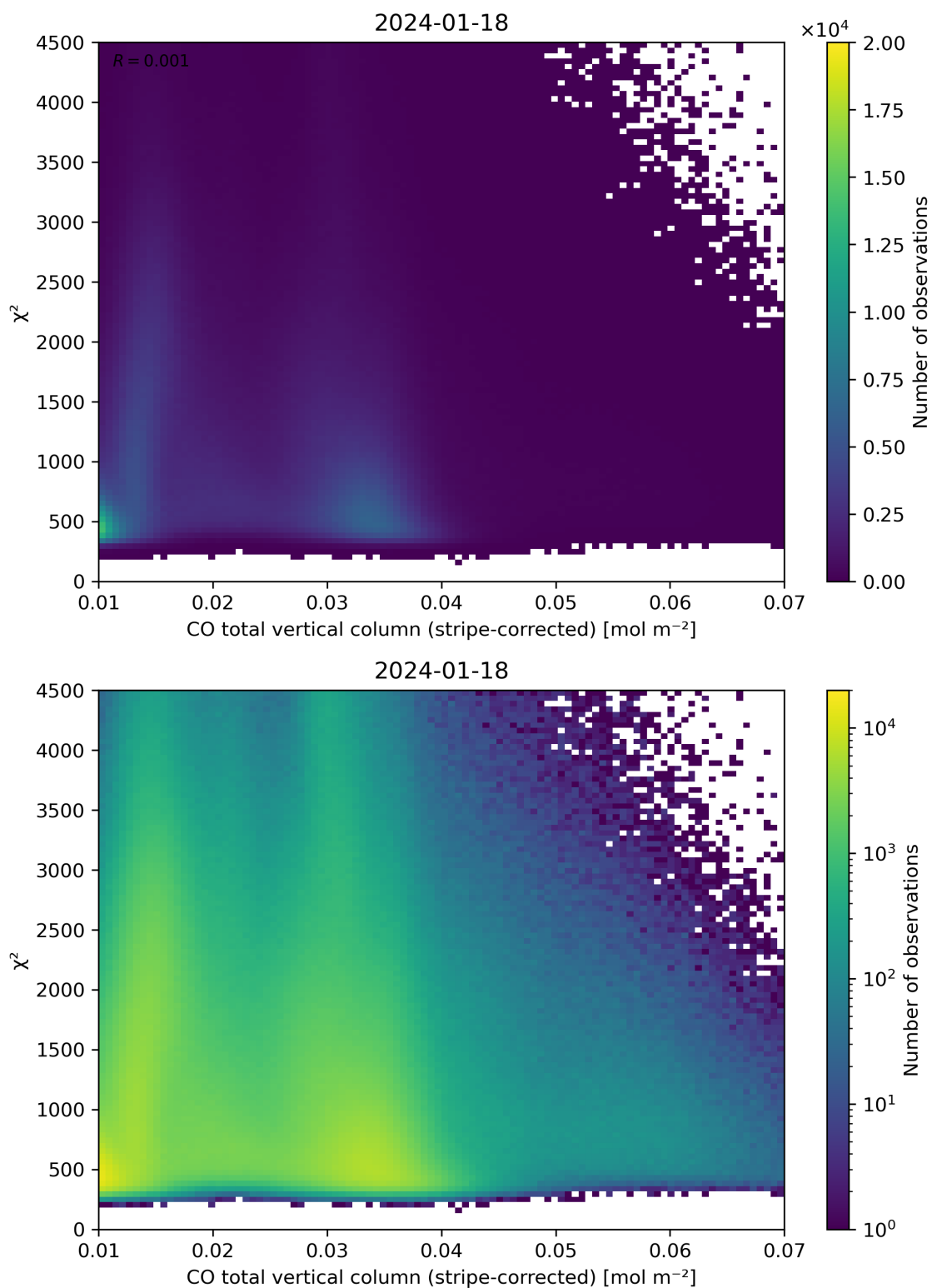
Figure 37: Scatter density plot of “CO total vertical column (stripe-corrected)” against “ \chi^2 ” for 2024-01-17 to 2024-01-19.
