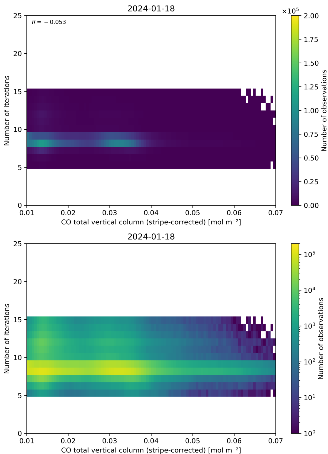
Figure 39: Scatter density plot of “CO total vertical column (stripe-corrected)” against “Number of iterations” for 2024-01-17 to 2024-01-19.
