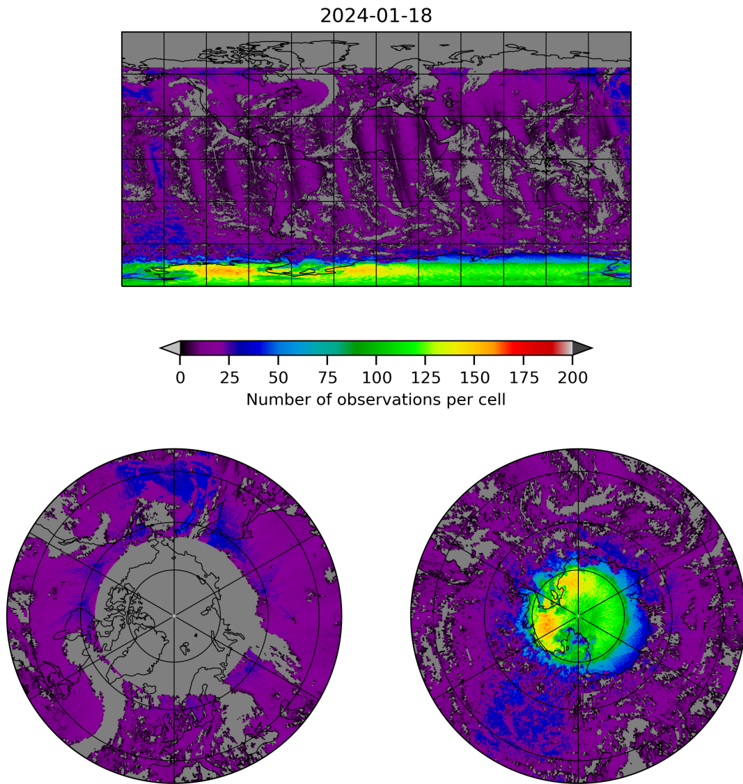
Figure 8: Map of the number of observations for 2024-01-17 to 2024-01-19
