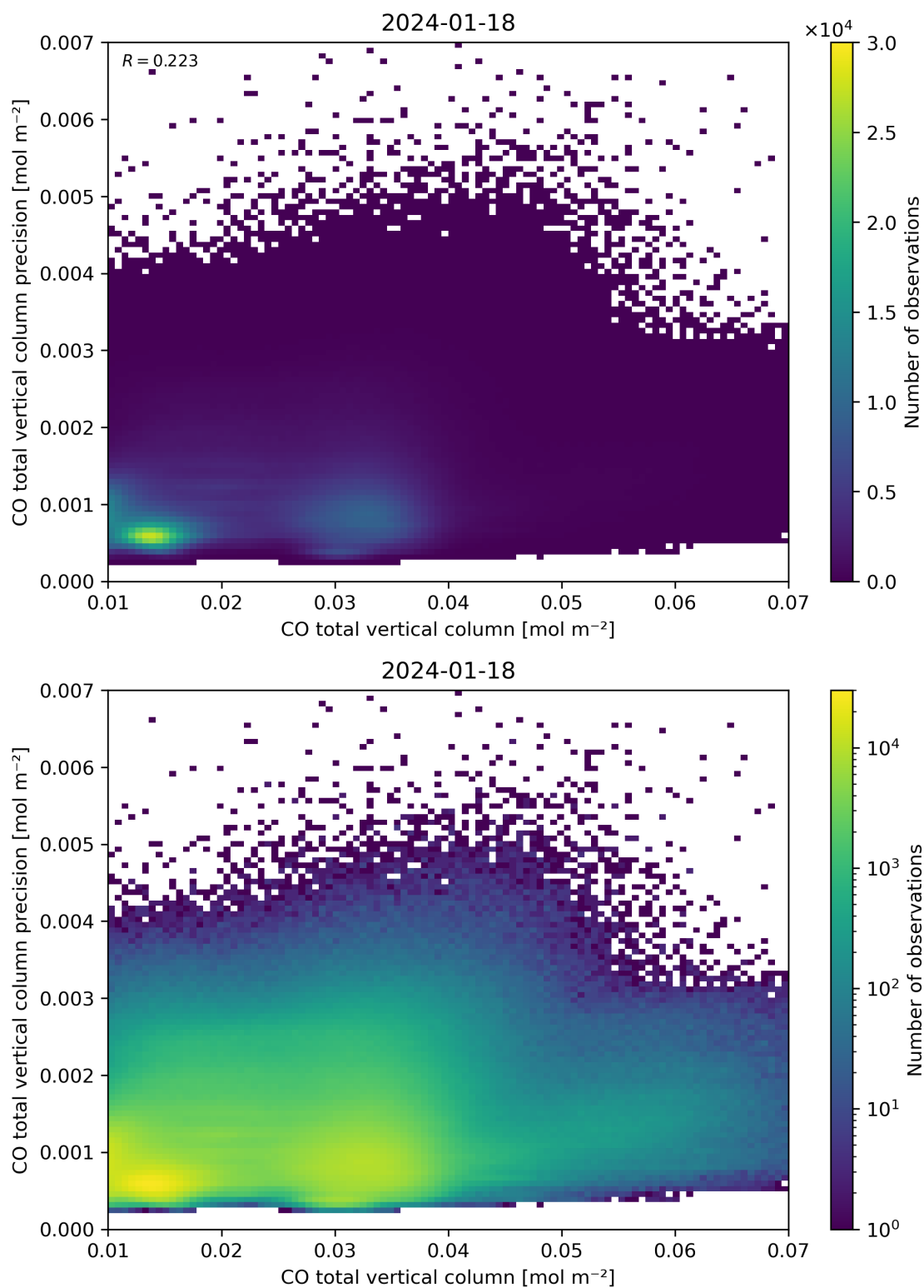
Figure 34: Scatter density plot of “CO total vertical column” against “CO total vertical column precision” for 2024-01-17 to 2024-01-19.
