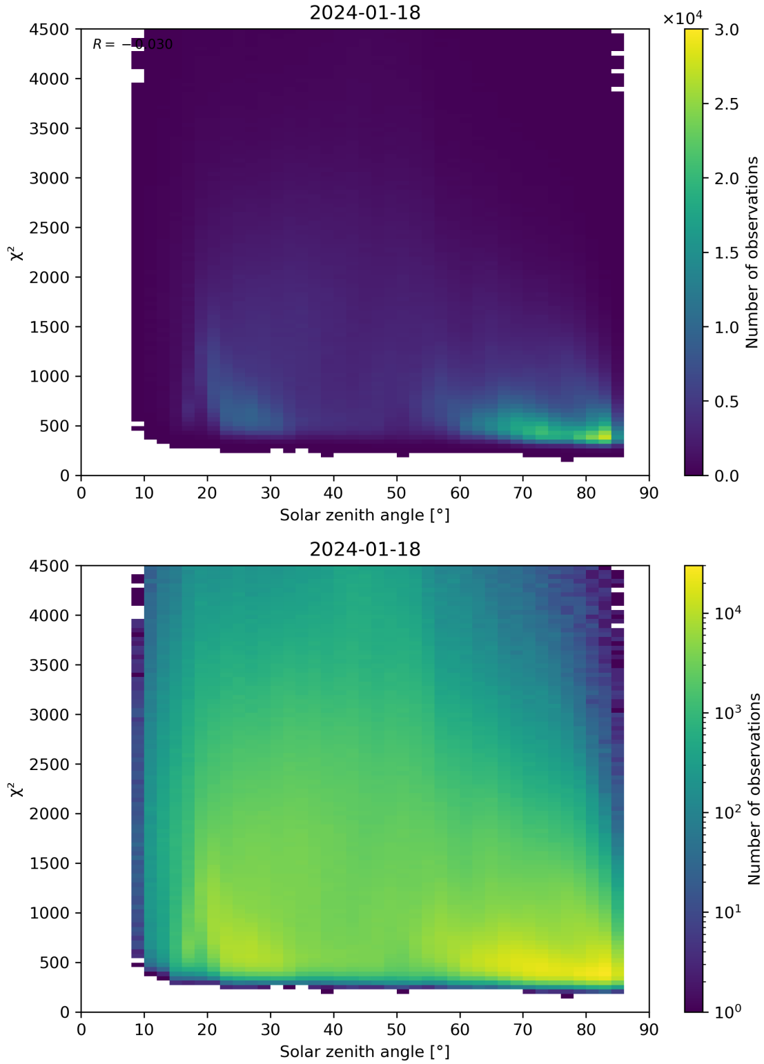
Figure 64: Scatter density plot of “Solar zenith angle” against “ \chi^2 ” for 2024-01-17 to 2024-01-19.
