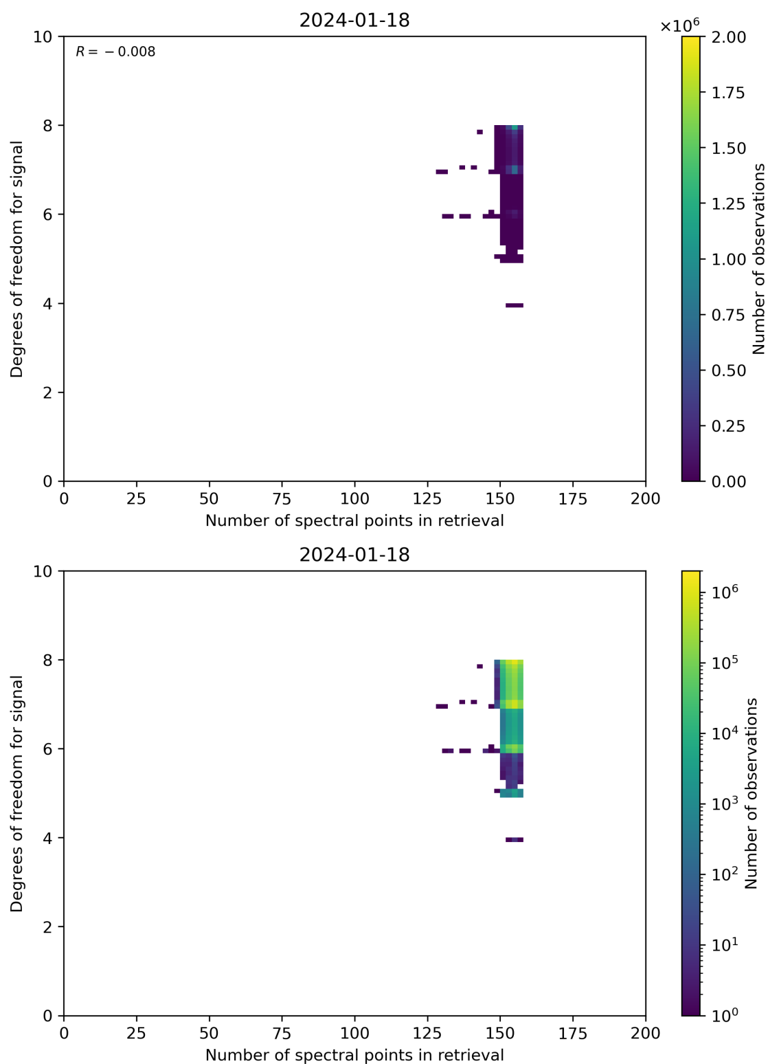
Figure 59: Scatter density plot of “Number of spectral points in retrieval” against “Degrees of freedom for signal” for 2024-01-17 to 2024-01-19.
