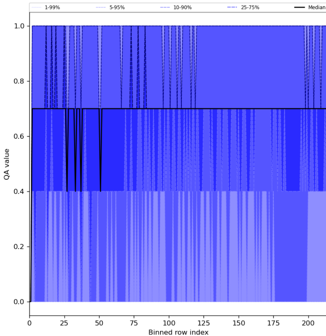
Figure 25: Along track statistics of “QA value” for 2024-01-17 to 2024-01-19
