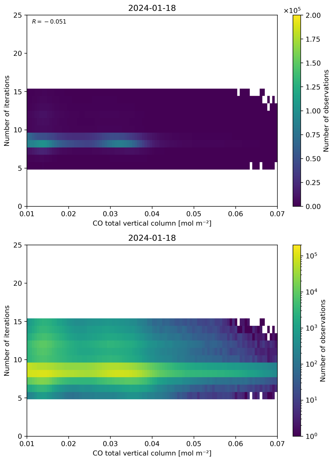
Figure 42: Scatter density plot of “CO total vertical column” against “Number of iterations” for 2024-01-17 to 2024-01-19.
