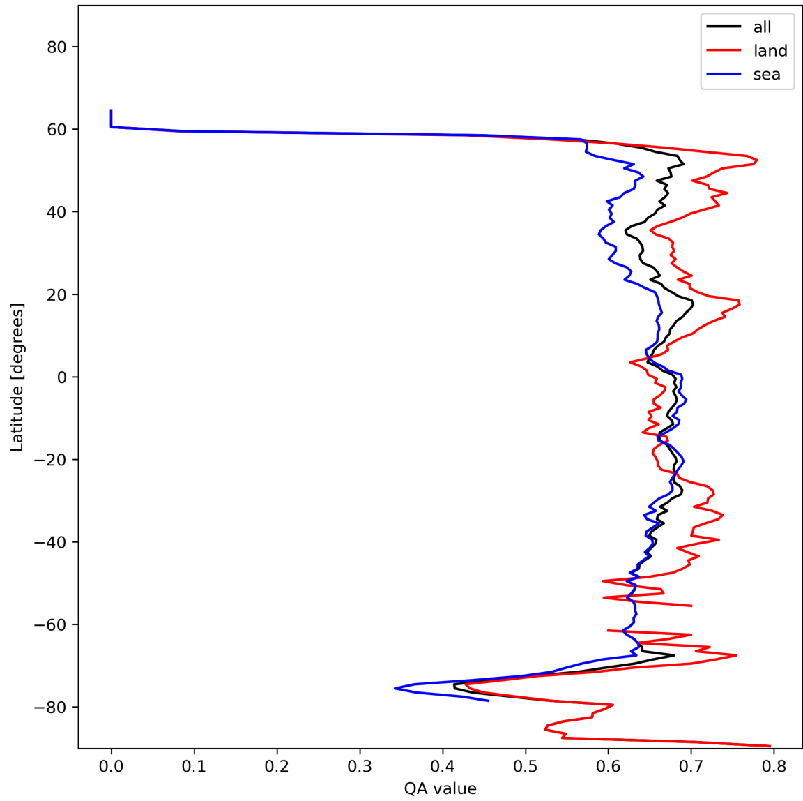
Figure 9: Zonal average of “QA value” for 2024-01-17 to 2024-01-19.
