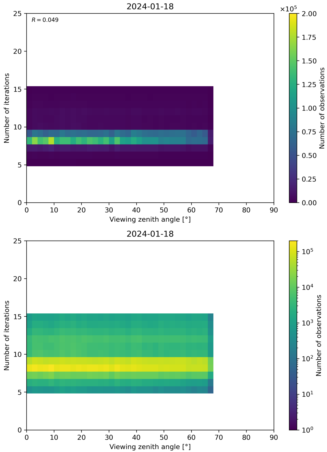
Figure 75: Scatter density plot of “Viewing zenith angle” against “Number of iterations” for 2024-01-17 to 2024-01-19.
