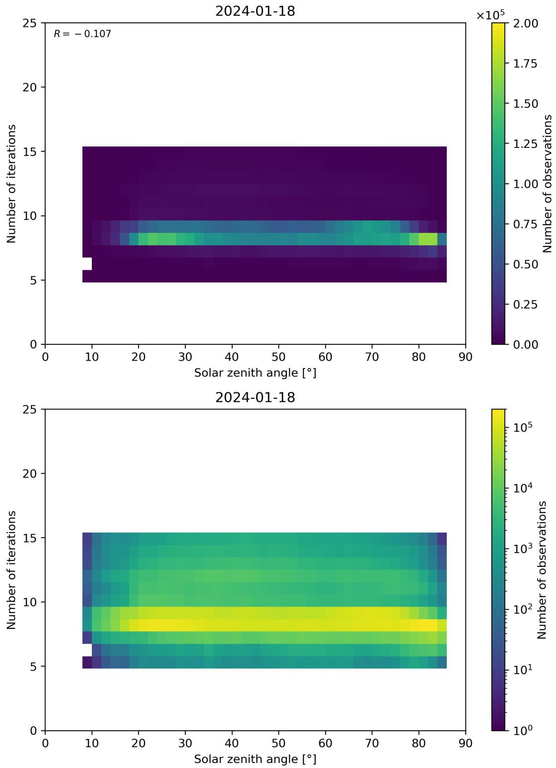
Figure 67: Scatter density plot of “Solar zenith angle” against “Number of iterations” for 2024-01-17 to 2024-01-19.
