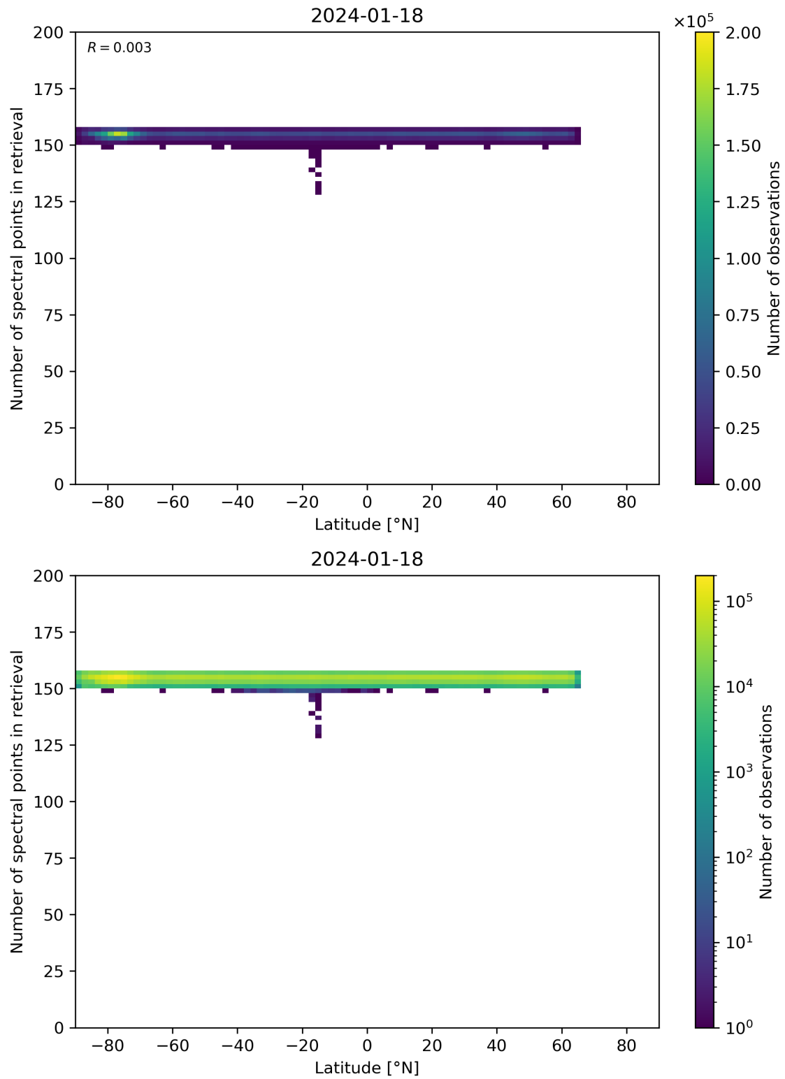
Figure 57: Scatter density plot of “Latitude” against “Number of spectral points in retrieval” for 2024-01-17 to 2024-01-19.
