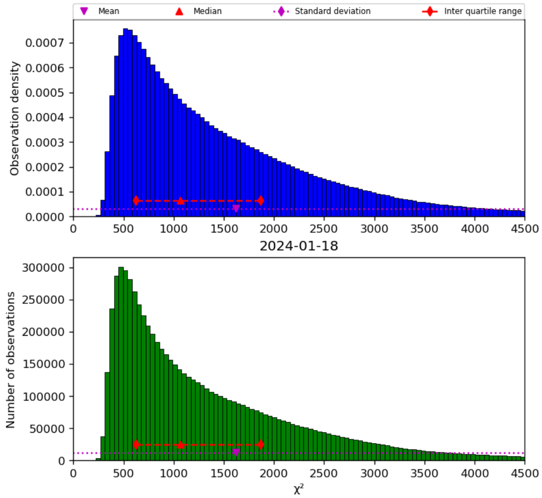
Figure 22: Histogram of “ \chi^2 ” for 2024-01-17 to 2024-01-19
