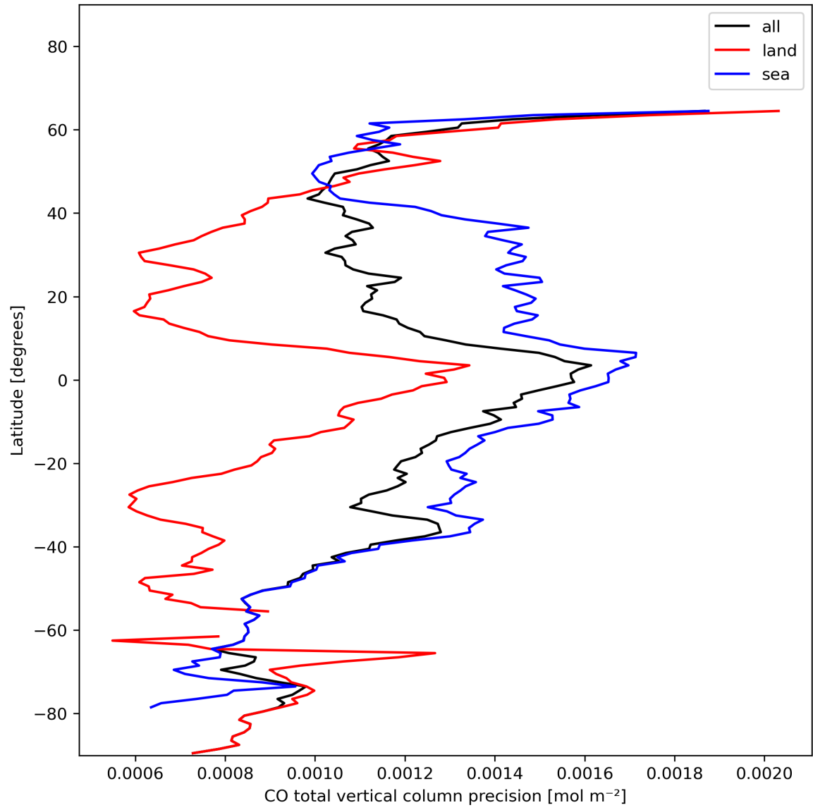
Figure 12: Zonal average of “CO total vertical column precision” for 2024-01-17 to 2024-01-19.
