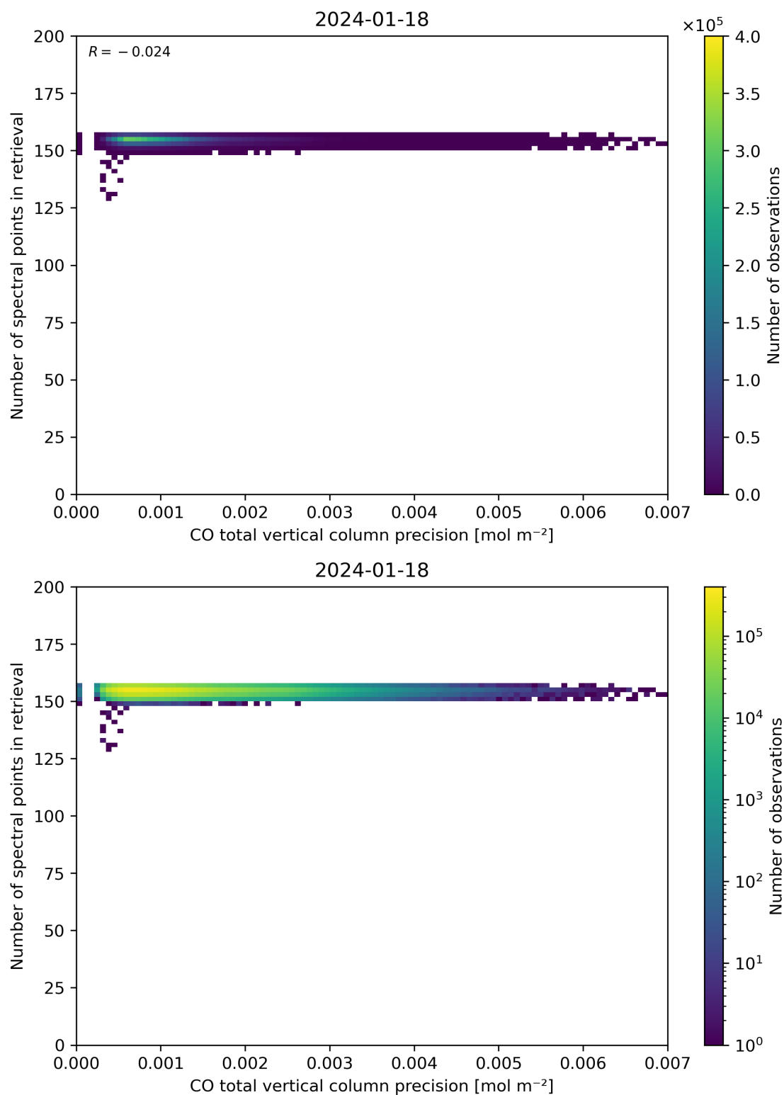
Figure 47: Scatter density plot of “CO total vertical column precision” against “Number of spectral points in retrieval” for 2024-01-17 to 2024-01-19.
