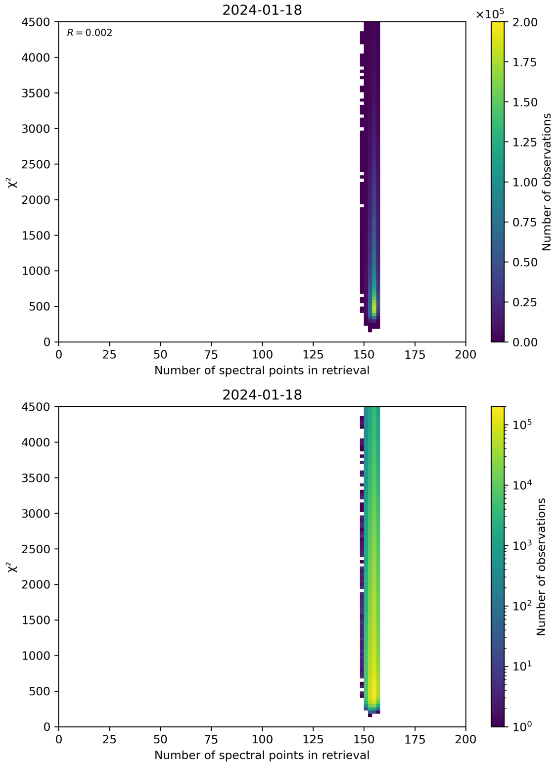
Figure 58: Scatter density plot of “Number of spectral points in retrieval” against “ \chi^2 ” for 2024-01-17 to 2024-01-19.
