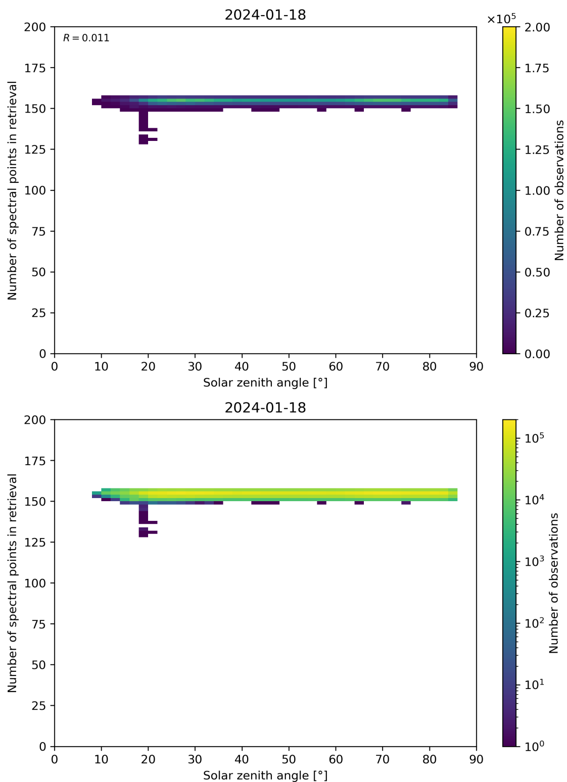
Figure 68: Scatter density plot of “Solar zenith angle” against “Number of spectral points in retrieval” for 2024-01-17 to 2024-01-19.
