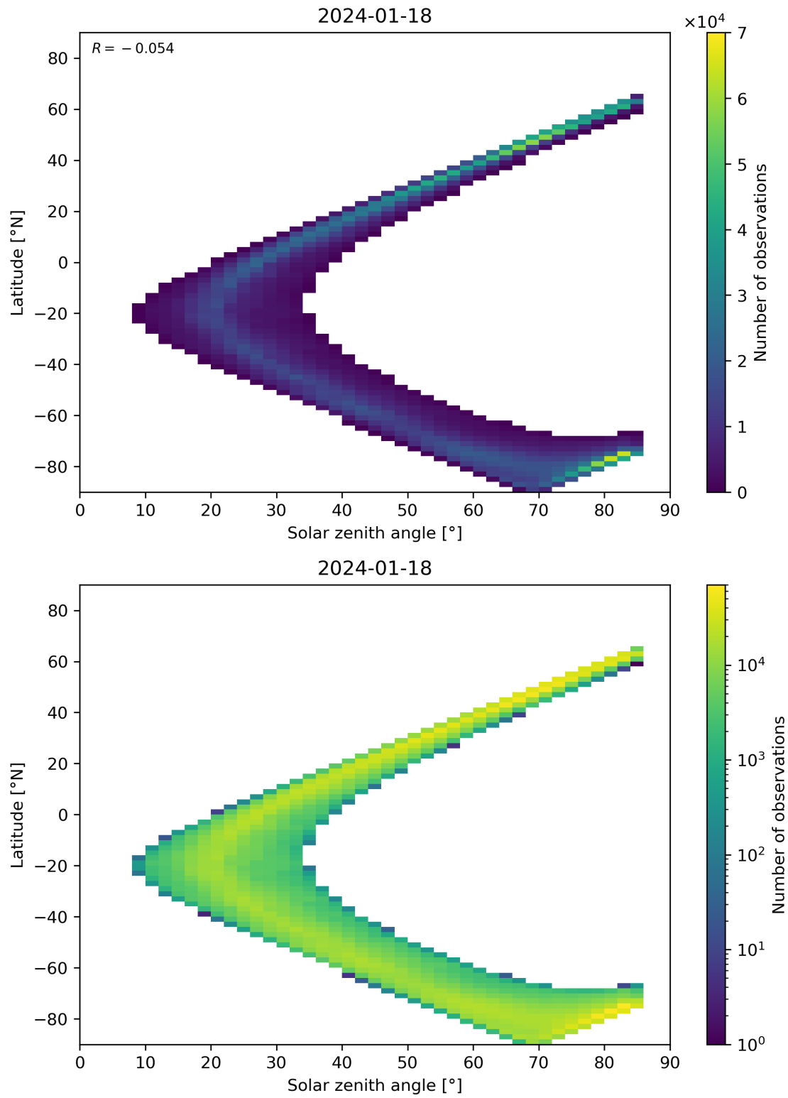
Figure 66: Scatter density plot of “Solar zenith angle” against “Latitude” for 2024-01-17 to 2024-01-19.
