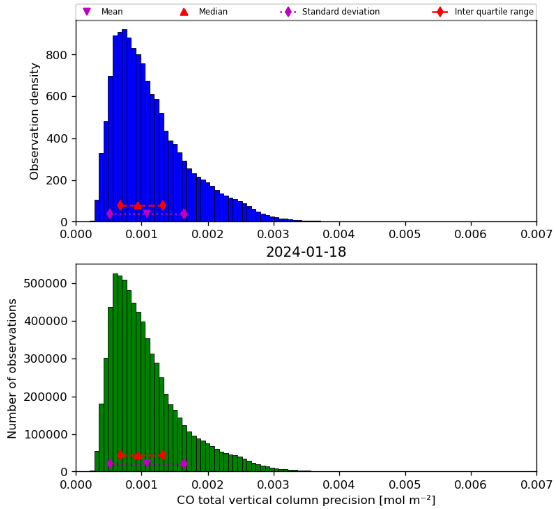
Figure 20: Histogram of “CO total vertical column precision” for 2024-01-17 to 2024-01-19
