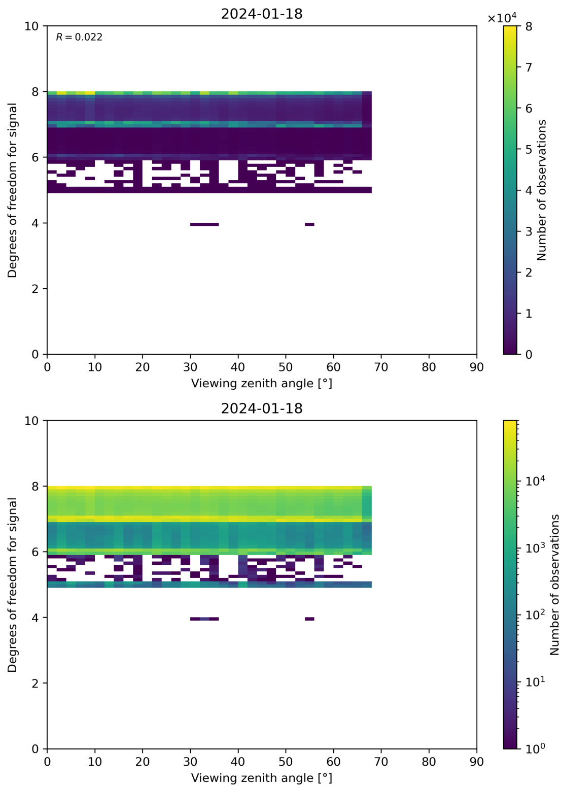
Figure 73: Scatter density plot of “Viewing zenith angle” against “Degrees of freedom for signal” for 2024-01-17 to 2024-01-19.
