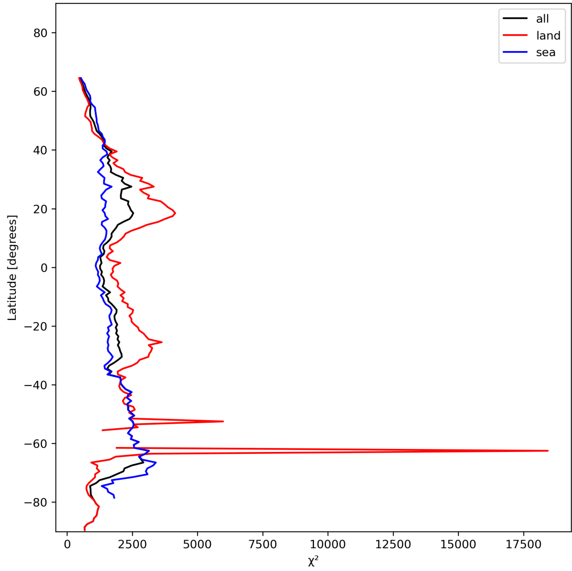
Figure 14: Zonal average of “ \chi^2 ” for 2024-01-17 to 2024-01-19.
