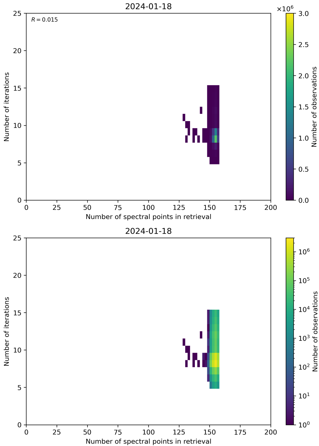
Figure 60: Scatter density plot of “Number of spectral points in retrieval” against “Number of iterations” for 2024-01-17 to 2024-01-19.
