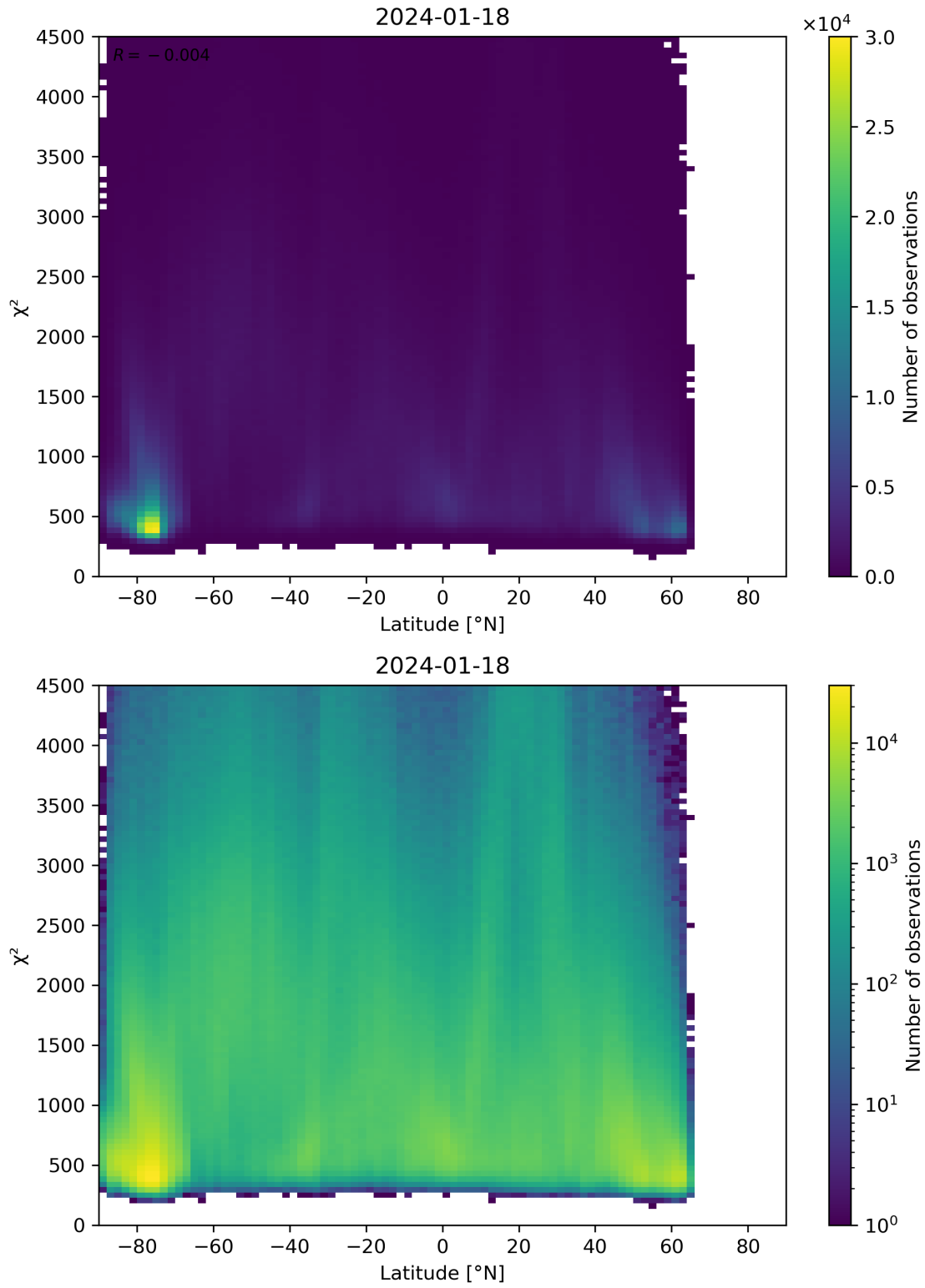
Figure 54: Scatter density plot of “Latitude” against “ \chi^2 ” for 2024-01-17 to 2024-01-19.
