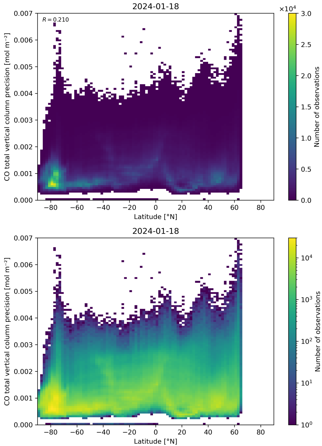
Figure 53: Scatter density plot of “Latitude” against “CO total vertical column precision” for 2024-01-17 to 2024-01-19.
