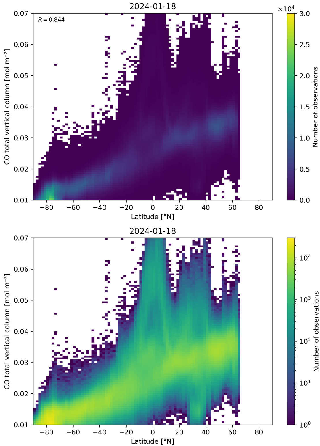
Figure 51: Scatter density plot of “Latitude” against “CO total vertical column” for 2024-01-17 to 2024-01-19.
