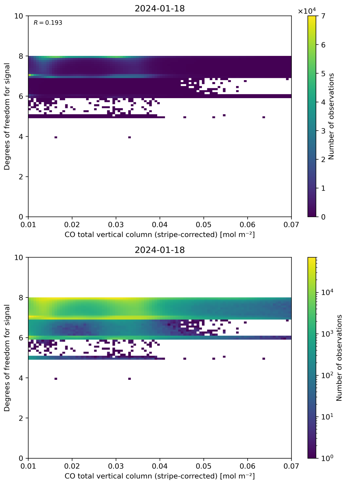
Figure 38: Scatter density plot of “CO total vertical column (stripe-corrected)” against “Degrees of freedom for signal” for 2024-01-17 to 2024-01-19.
