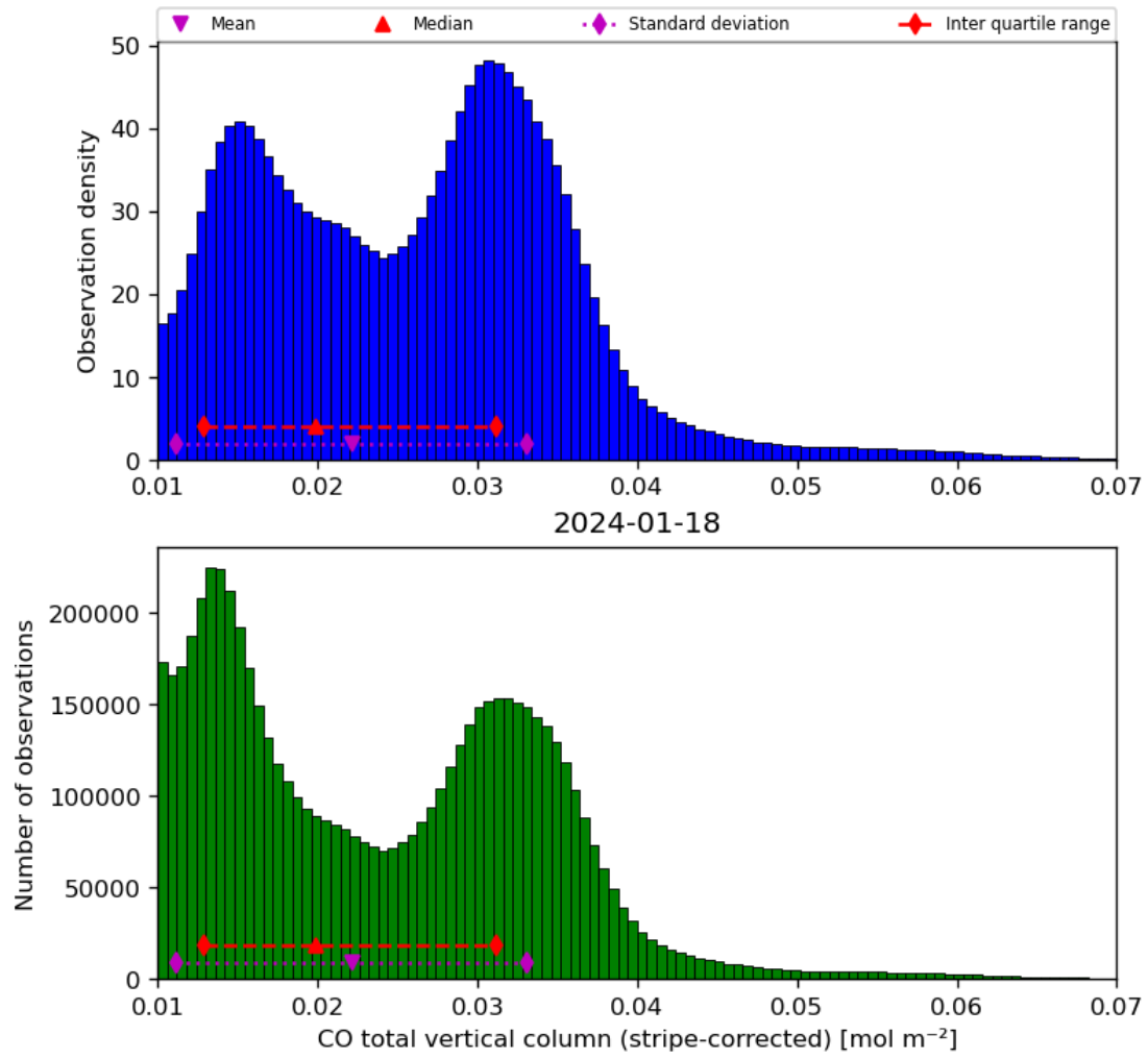
Figure 19: Histogram of “CO total vertical column (stripe-corrected)” for 2024-01-17 to 2024-01-19
