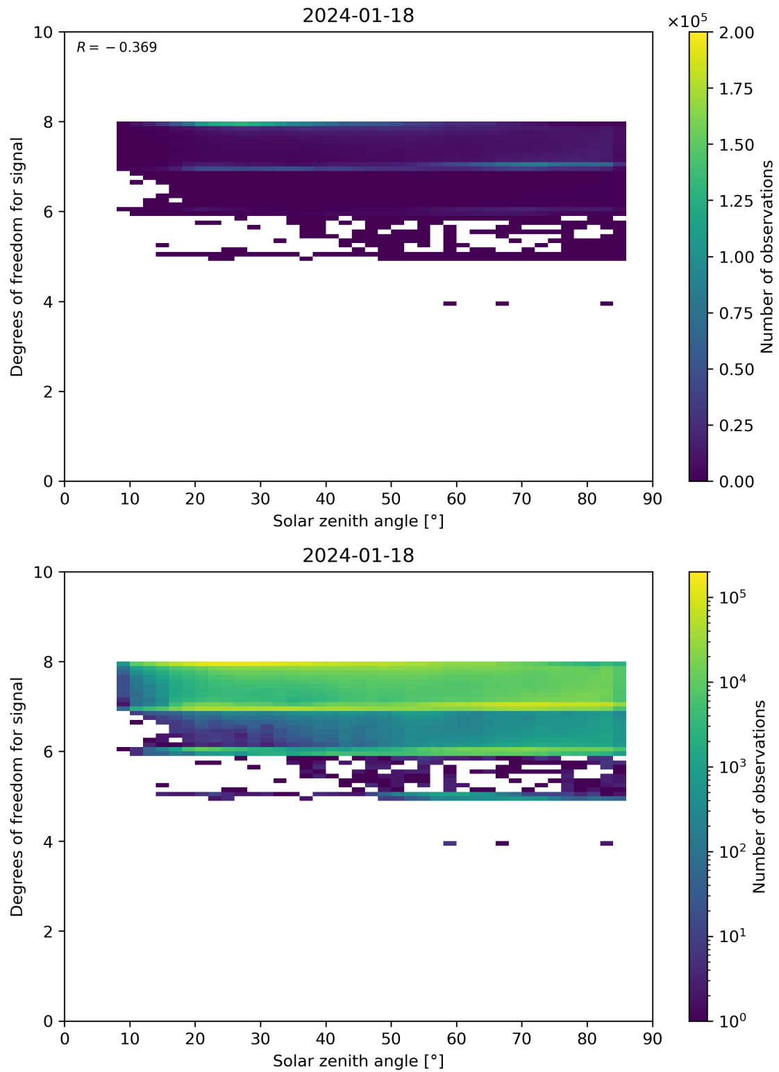
Figure 65: Scatter density plot of “Solar zenith angle” against “Degrees of freedom for signal” for 2024-01-17 to 2024-01-19.
