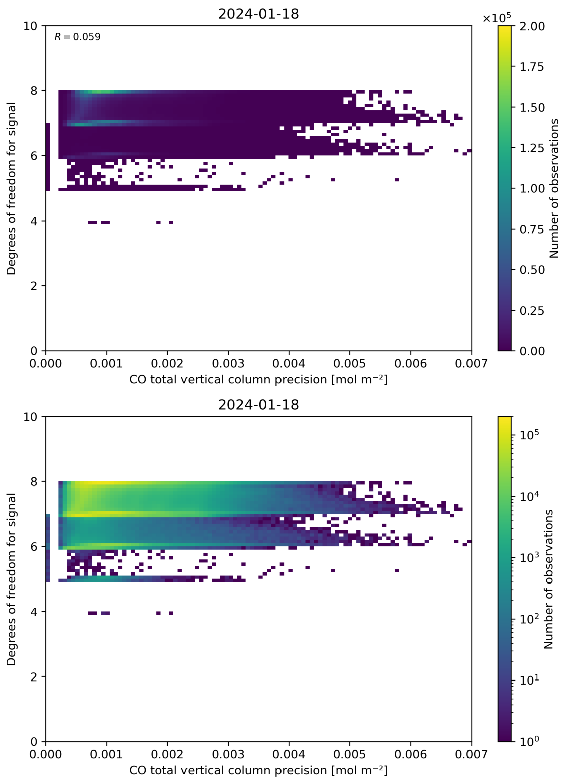
Figure 45: Scatter density plot of “CO total vertical column precision” against “Degrees of freedom for signal” for 2024-01-17 to 2024-01-19.
