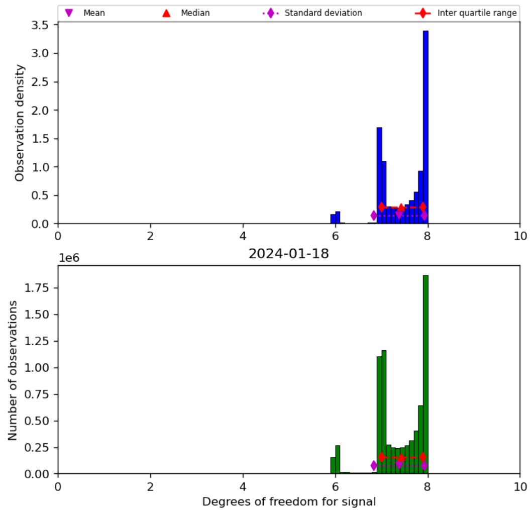
Figure 23: Histogram of “Degrees of freedom for signal” for 2024-01-17 to 2024-01-19
