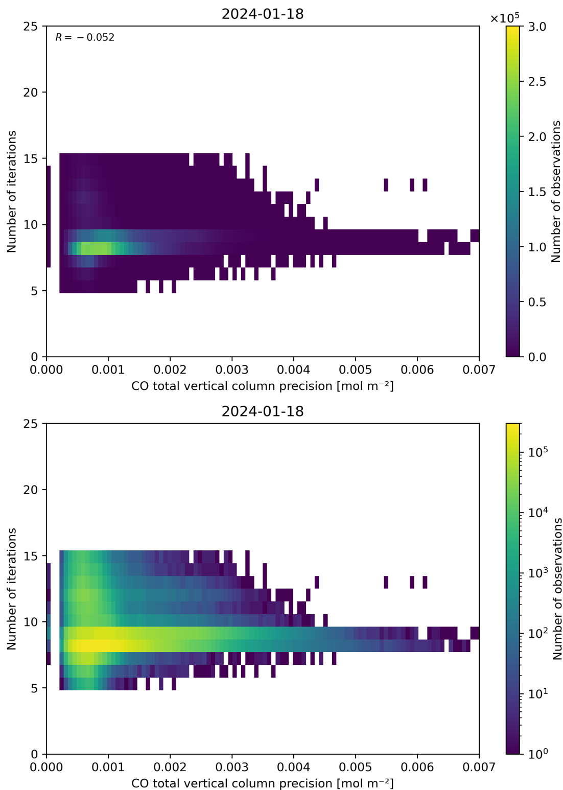
Figure 46: Scatter density plot of “CO total vertical column precision” against “Number of iterations” for 2024-01-17 to 2024-01-19.
