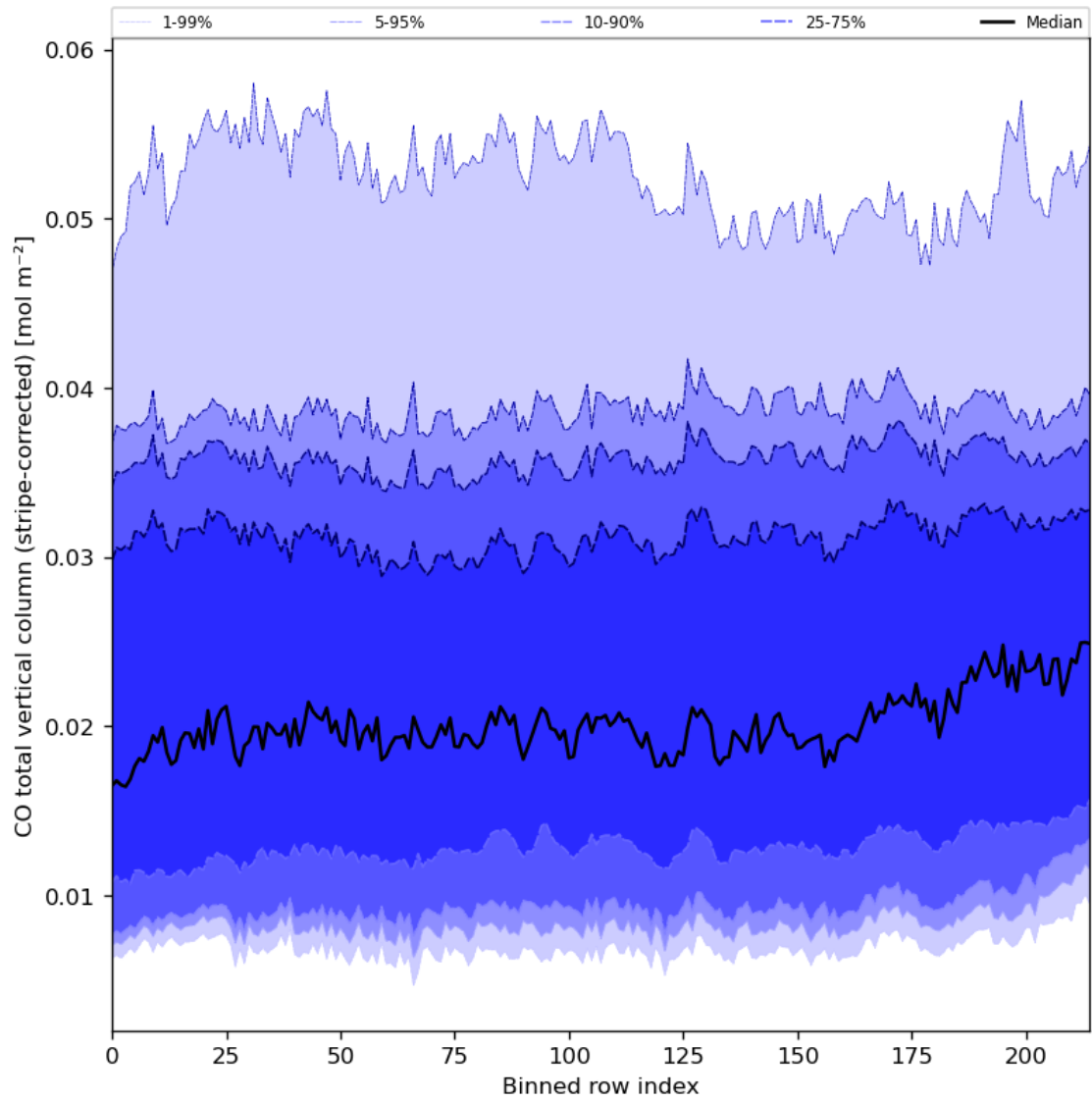
Figure 27: Along track statistics of “CO total vertical column (stripe-corrected)” for 2024-01-17 to 2024-01-19
