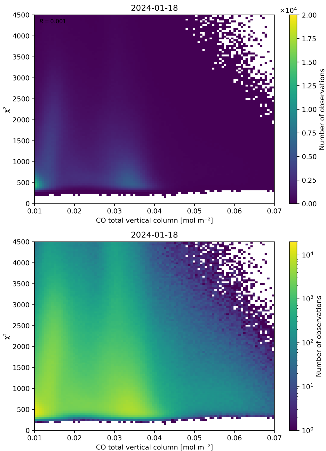
Figure 35: Scatter density plot of “CO total vertical column” against “ \chi^2 ” for 2024-01-17 to 2024-01-19.
