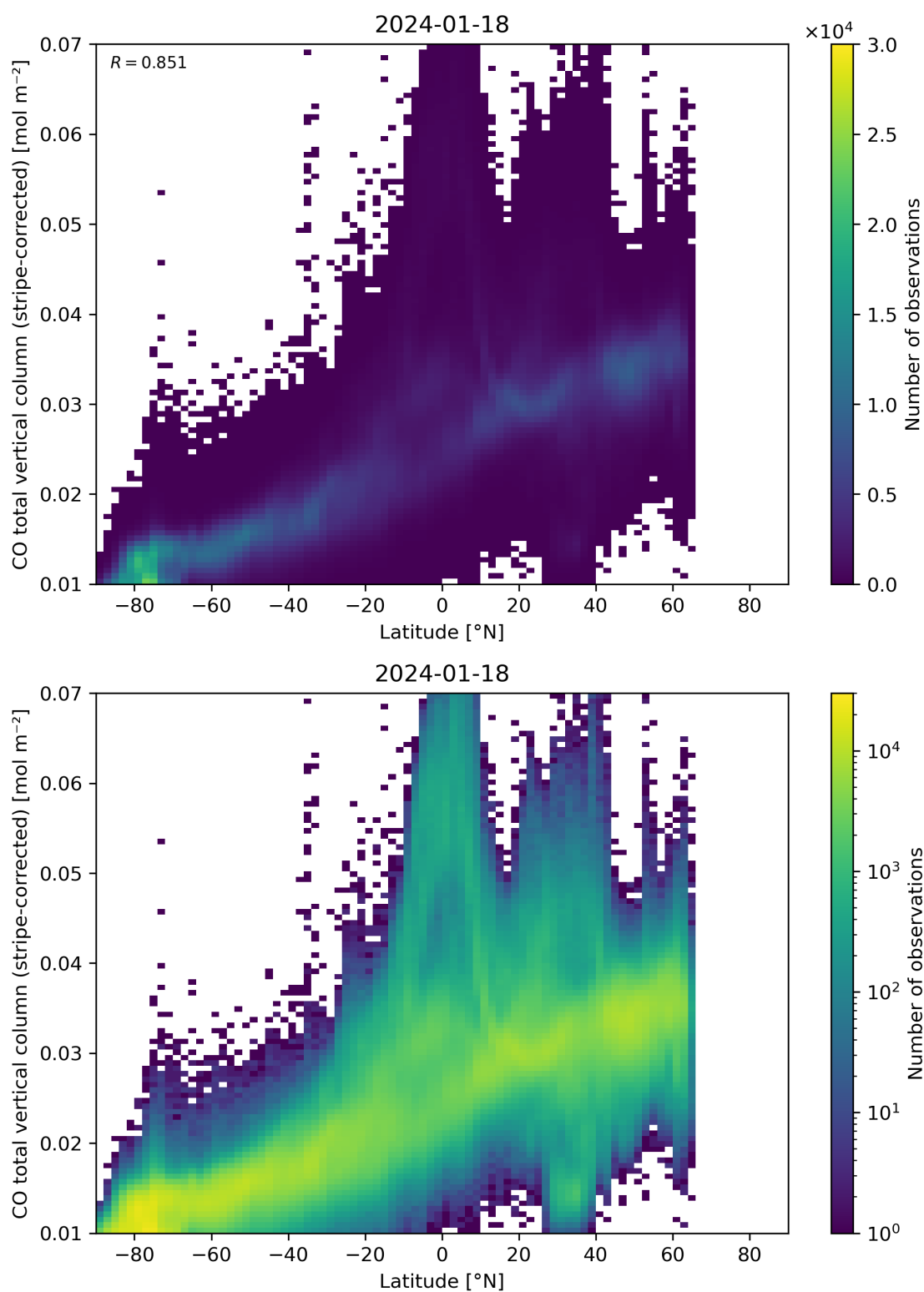
Figure 52: Scatter density plot of “Latitude” against “CO total vertical column (stripe-corrected)” for 2024-01-17 to 2024-01-19.
