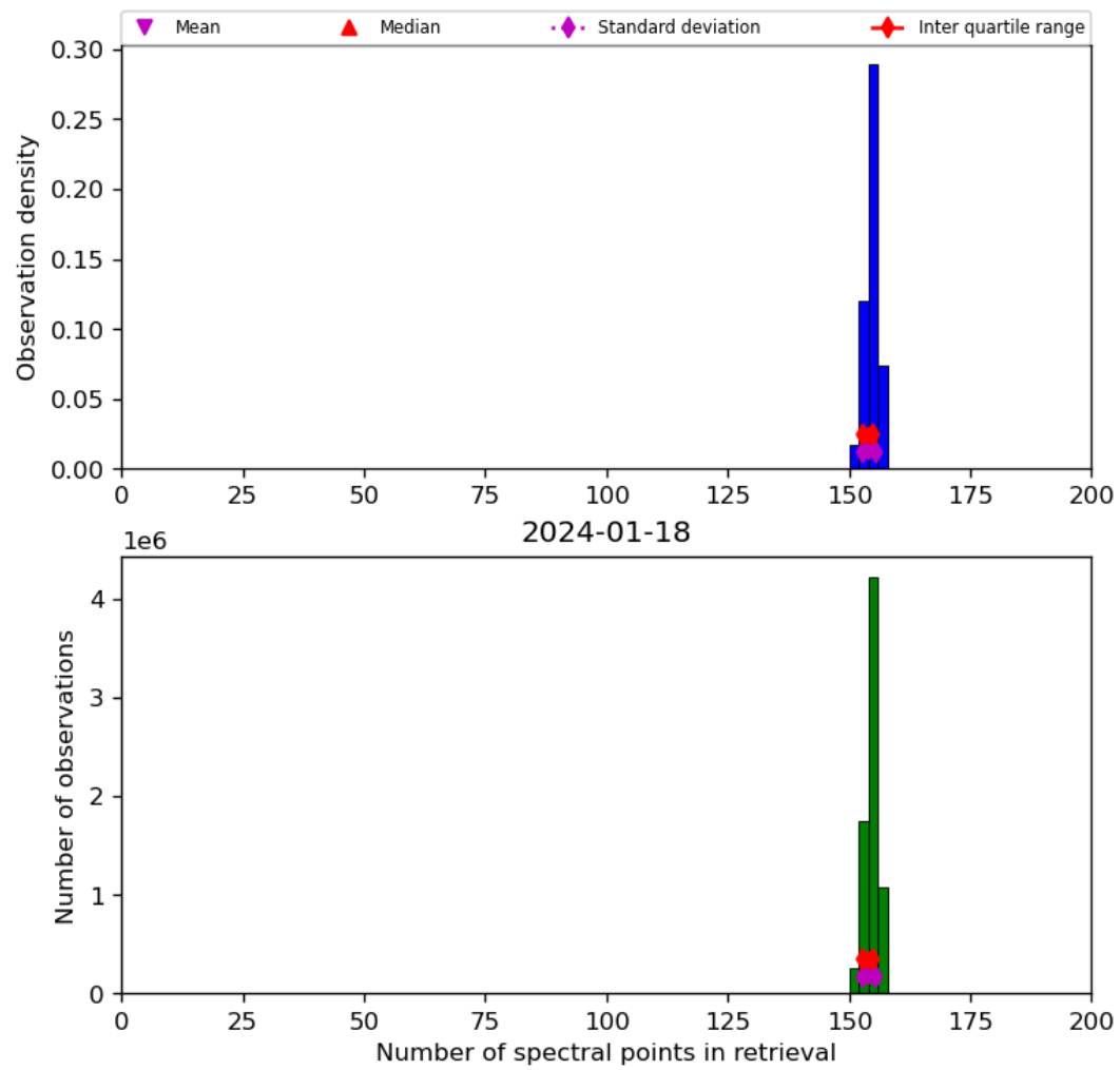
Figure 21: Histogram of “Number of spectral points in retrieval” for 2024-01-17 to 2024-01-19
