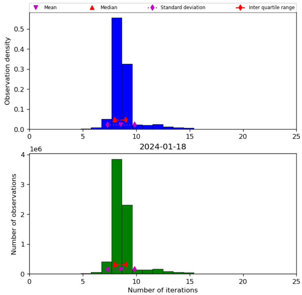
Figure 24: Histogram of “Number of iterations” for 2024-01-17 to 2024-01-19
