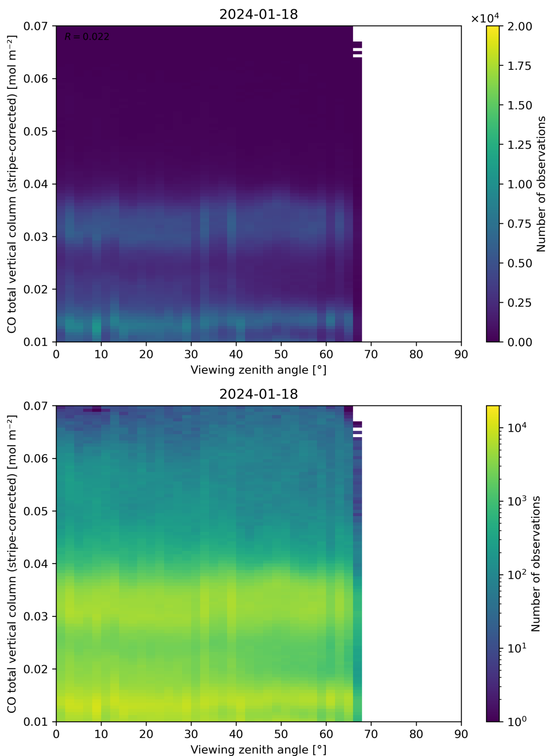
Figure 70: Scatter density plot of “Viewing zenith angle” against “CO total vertical column (stripe-corrected)” for 2024-01-17 to 2024-01-19.
