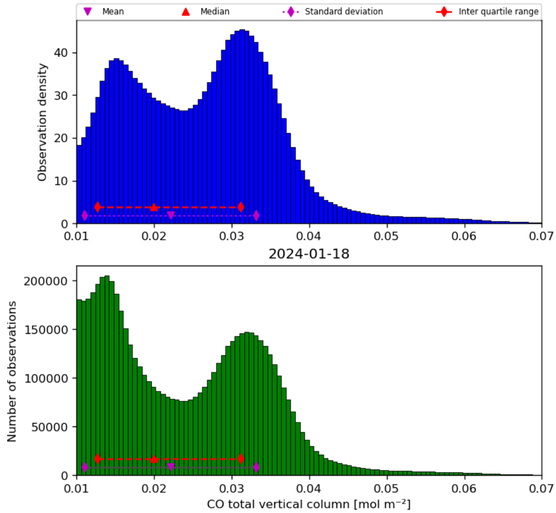
Figure 18: Histogram of “CO total vertical column” for 2024-01-17 to 2024-01-19
