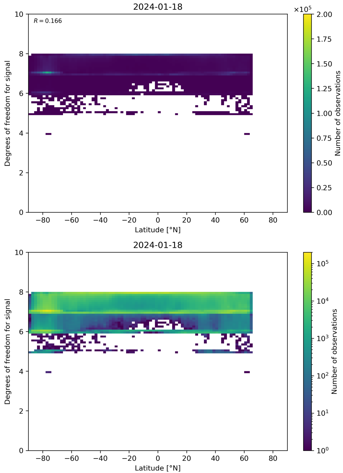
Figure 55: Scatter density plot of “Latitude” against “Degrees of freedom for signal” for 2024-01-17 to 2024-01-19.
