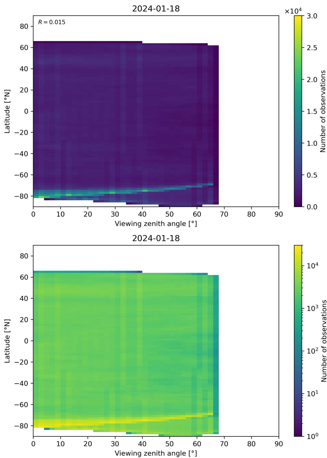
Figure 74: Scatter density plot of “Viewing zenith angle” against “Latitude” for 2024-01-17 to 2024-01-19.
