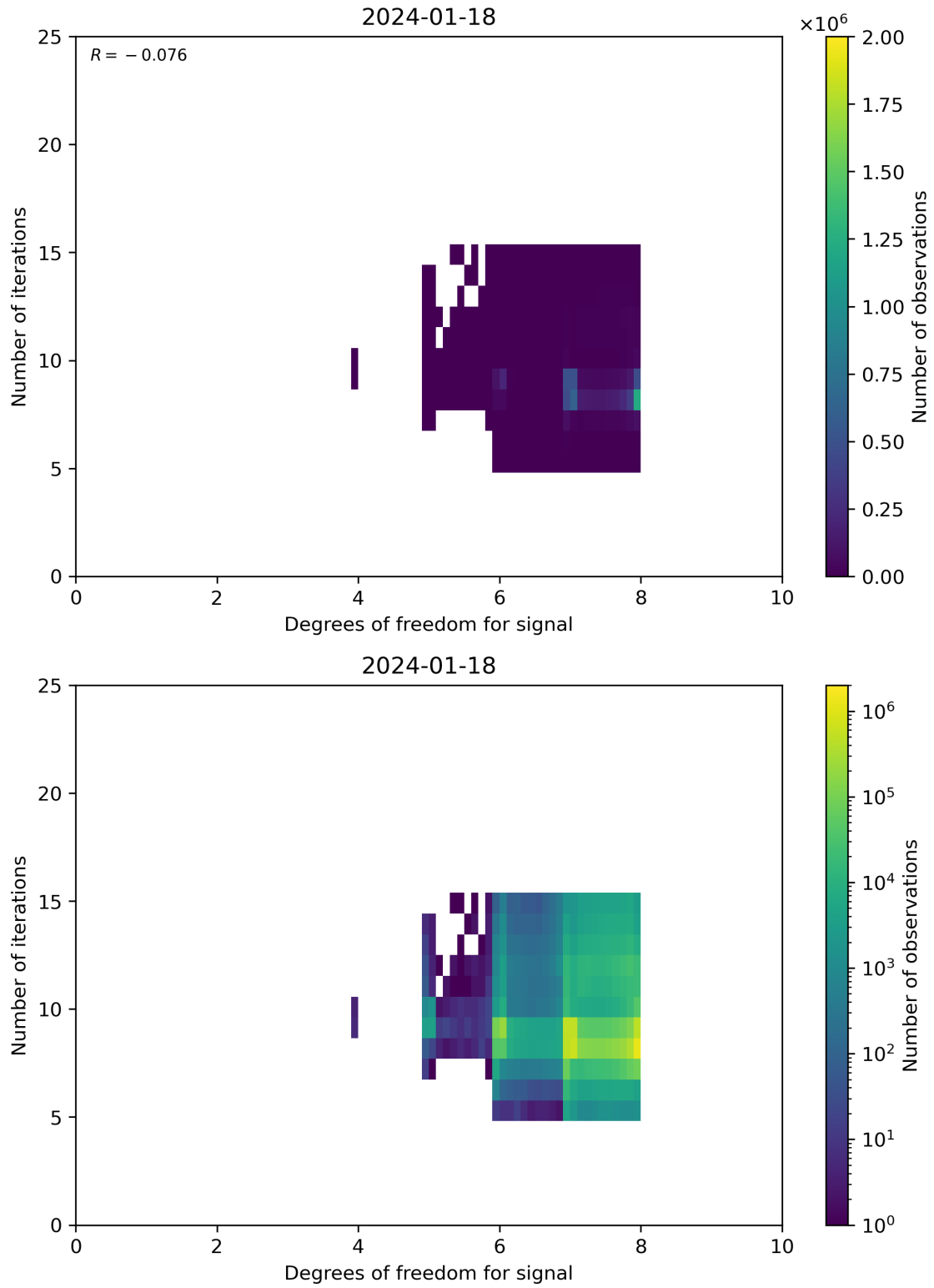
Figure 50: Scatter density plot of “Degrees of freedom for signal” against “Number of iterations” for 2024-01-17 to 2024-01-19.
