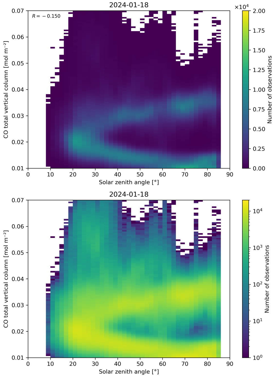
Figure 61: Scatter density plot of “Solar zenith angle” against “CO total vertical column” for 2024-01-17 to 2024-01-19.
