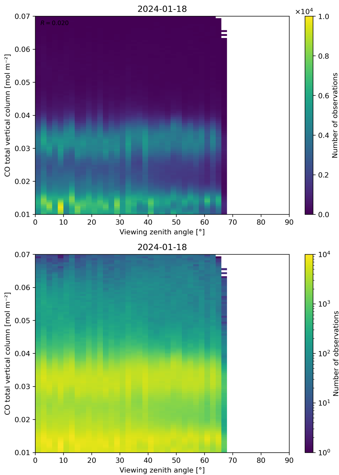
Figure 69: Scatter density plot of “Viewing zenith angle” against “CO total vertical column” for 2024-01-17 to 2024-01-19.
