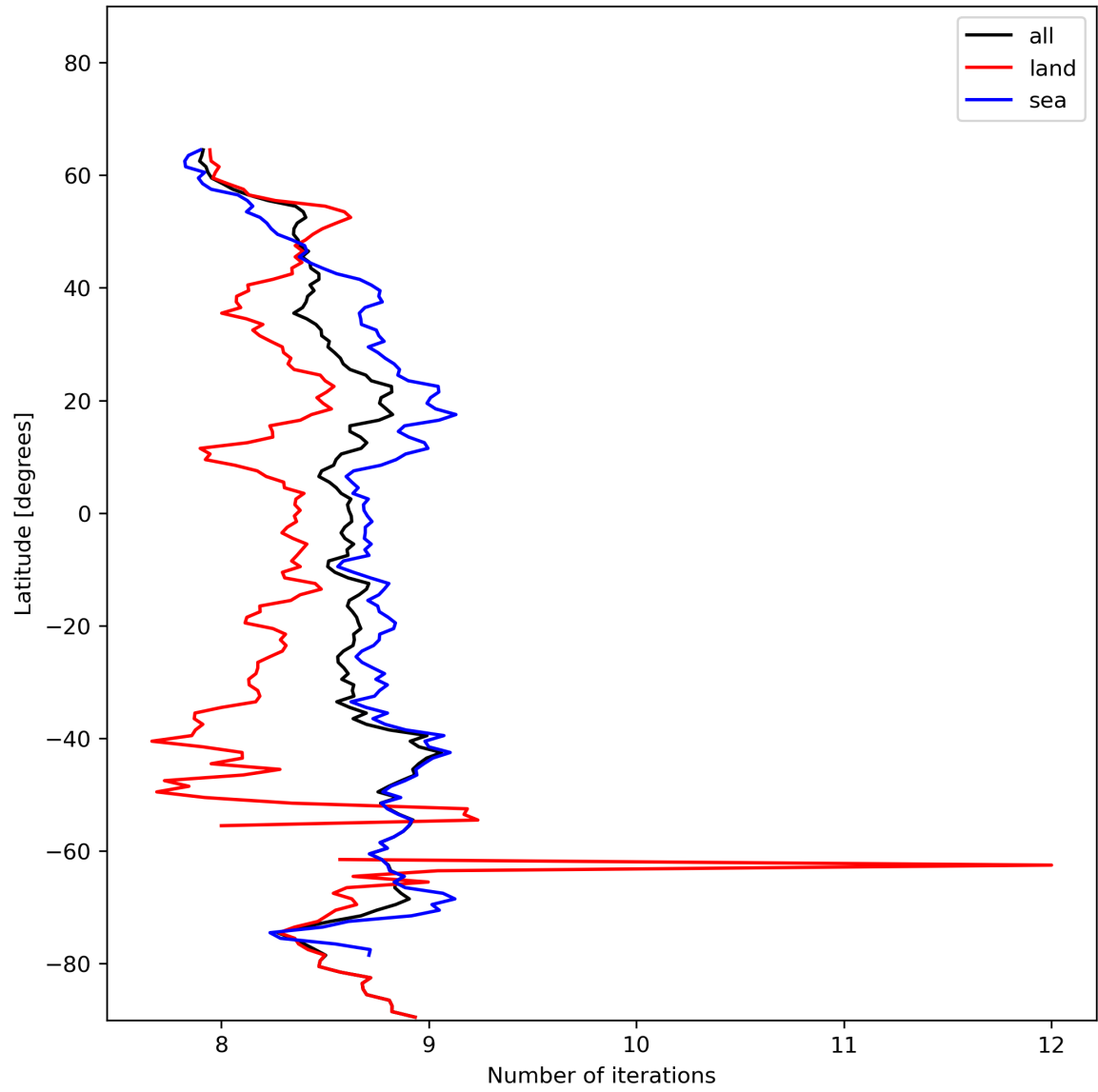
Figure 16: Zonal average of “Number of iterations” for 2024-01-17 to 2024-01-19.
