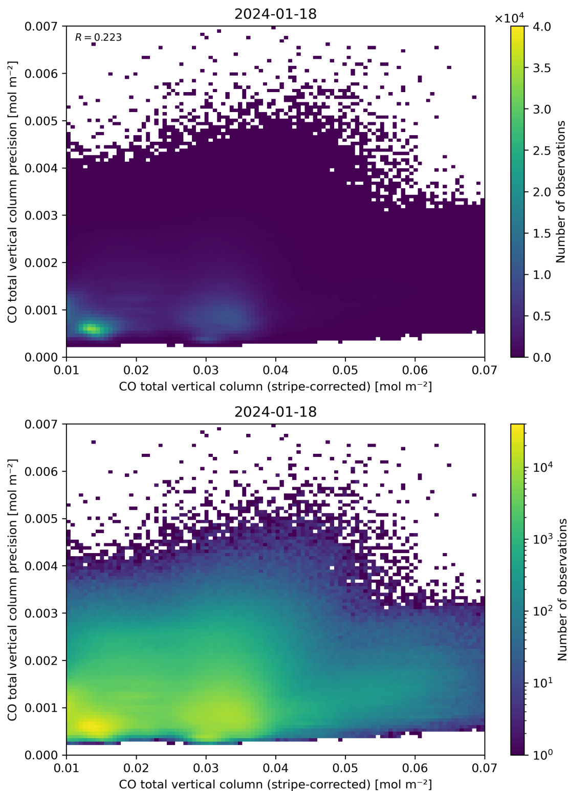
Figure 36: Scatter density plot of “CO total vertical column (stripe-corrected)” against “CO total vertical column precision” for 2024-01-17 to 2024-01-19.
