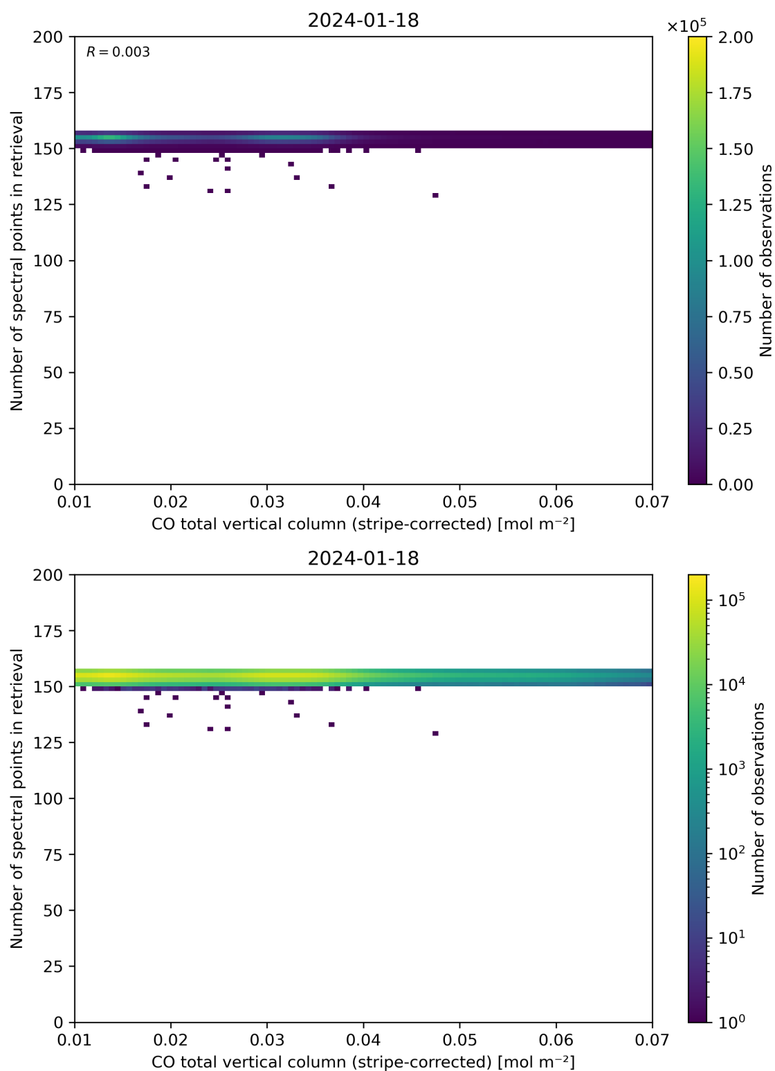
Figure 40: Scatter density plot of “CO total vertical column (stripe-corrected)” against “Number of spectral points in retrieval” for 2024-01-17 to 2024-01-19.
