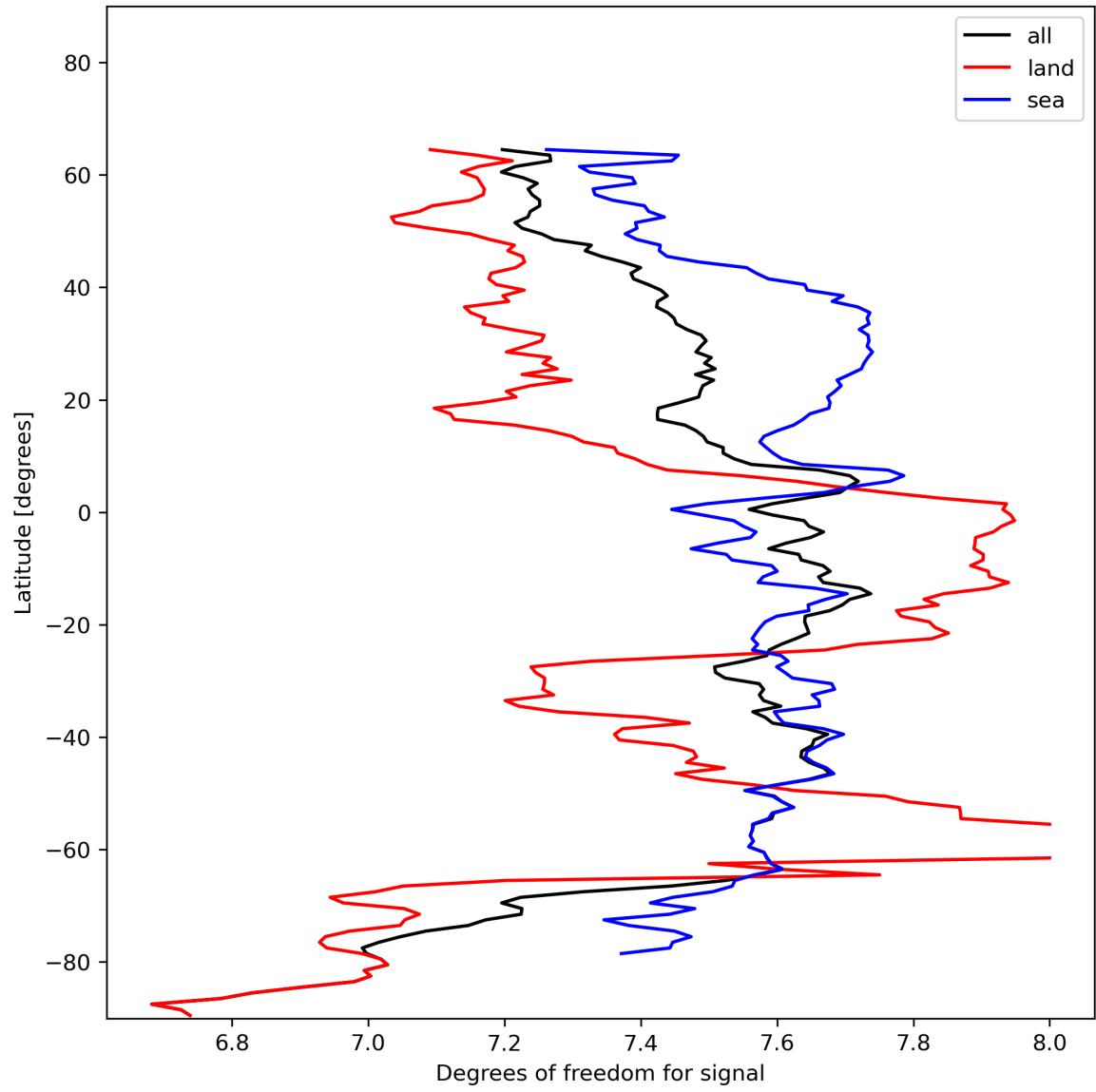
Figure 15: Zonal average of “Degrees of freedom for signal” for 2024-01-17 to 2024-01-19.
