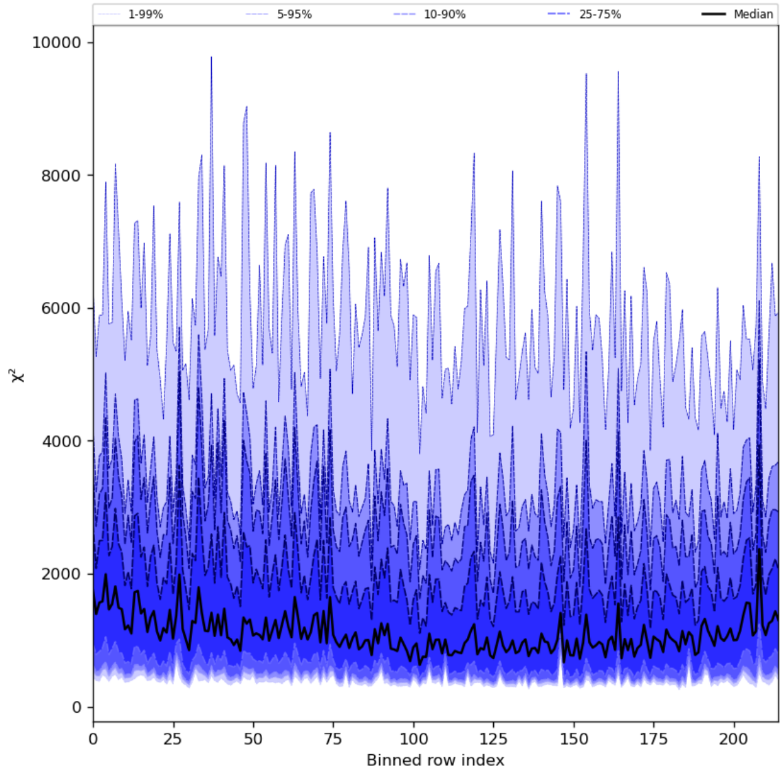
Figure 30: Along track statistics of “ \chi^2 ” for 2024-01-17 to 2024-01-19
