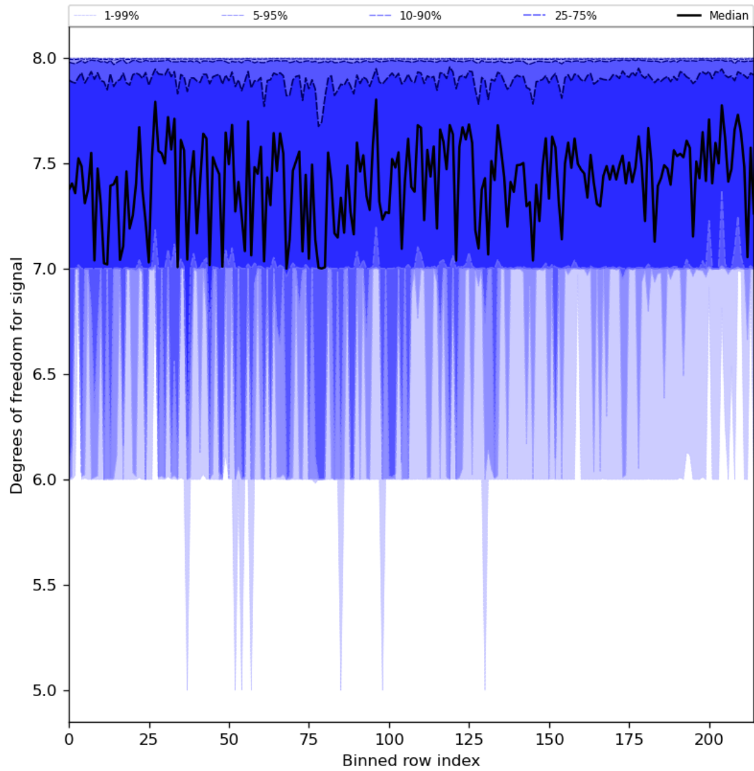
Figure 31: Along track statistics of “Degrees of freedom for signal” for 2024-01-17 to 2024-01-19
