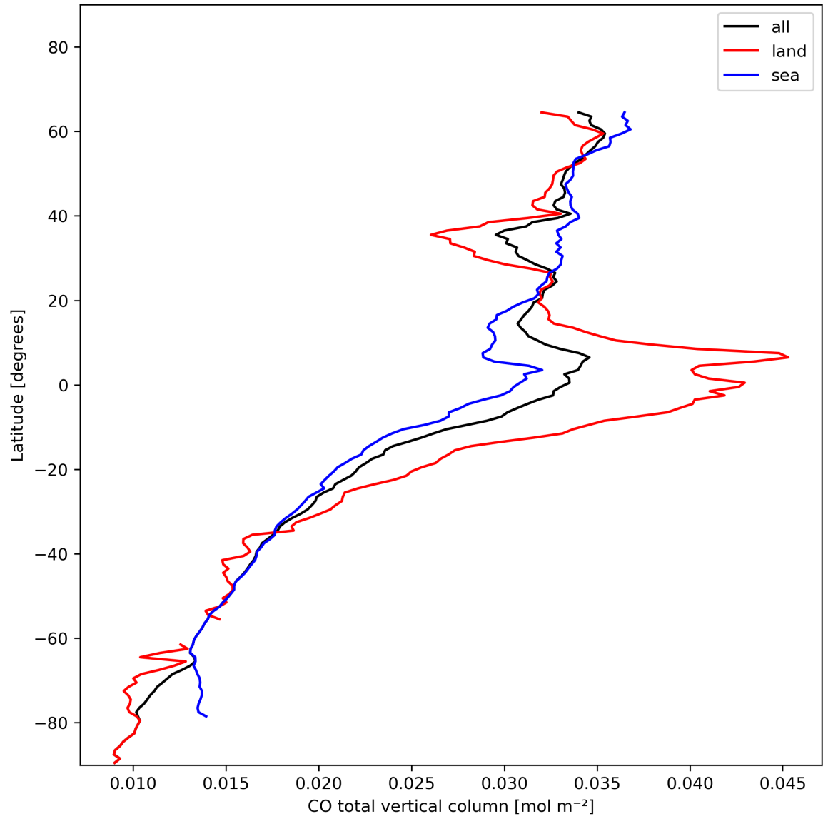
Figure 10: Zonal average of “CO total vertical column” for 2024-01-17 to 2024-01-19.
