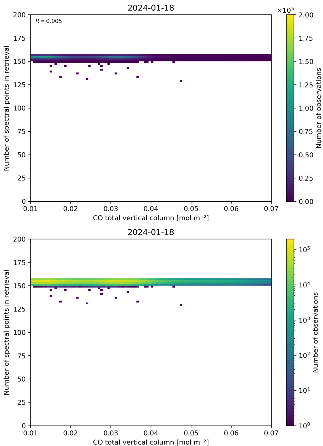
Figure 43: Scatter density plot of “CO total vertical column” against “Number of spectral points in retrieval” for 2024-01-17 to 2024-01-19.
