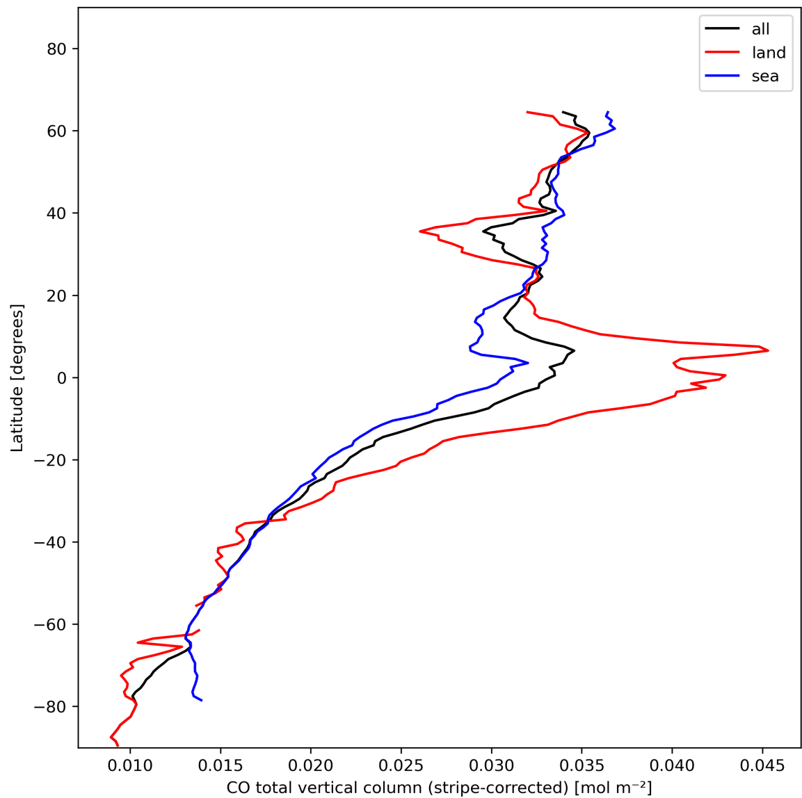
Figure 11: Zonal average of “CO total vertical column (stripe-corrected)” for 2024-01-17 to 2024-01-19.
