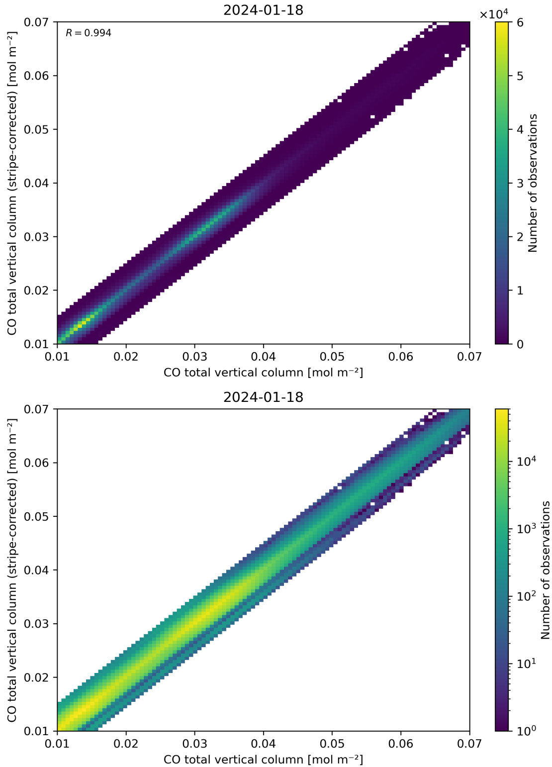
Figure 33: Scatter density plot of “CO total vertical column” against “CO total vertical column (stripe-corrected)” for 2024-01-17 to 2024-01-19.
