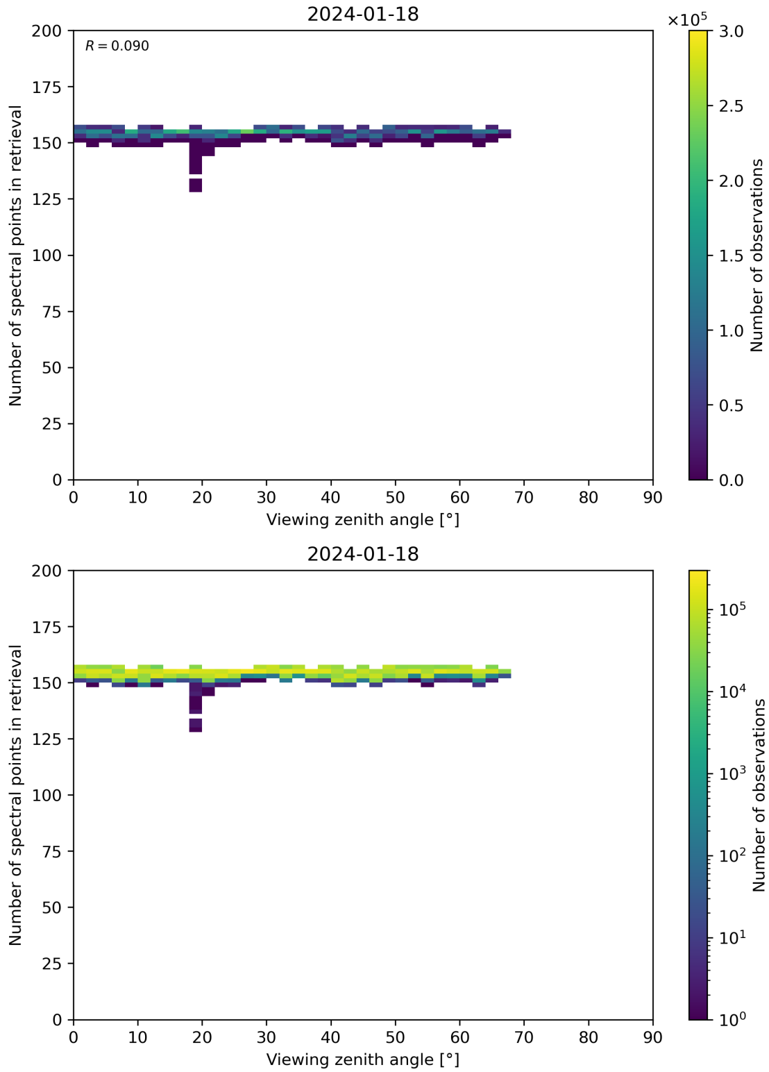
Figure 76: Scatter density plot of “Viewing zenith angle” against “Number of spectral points in retrieval” for 2024-01-17 to 2024-01-19.
