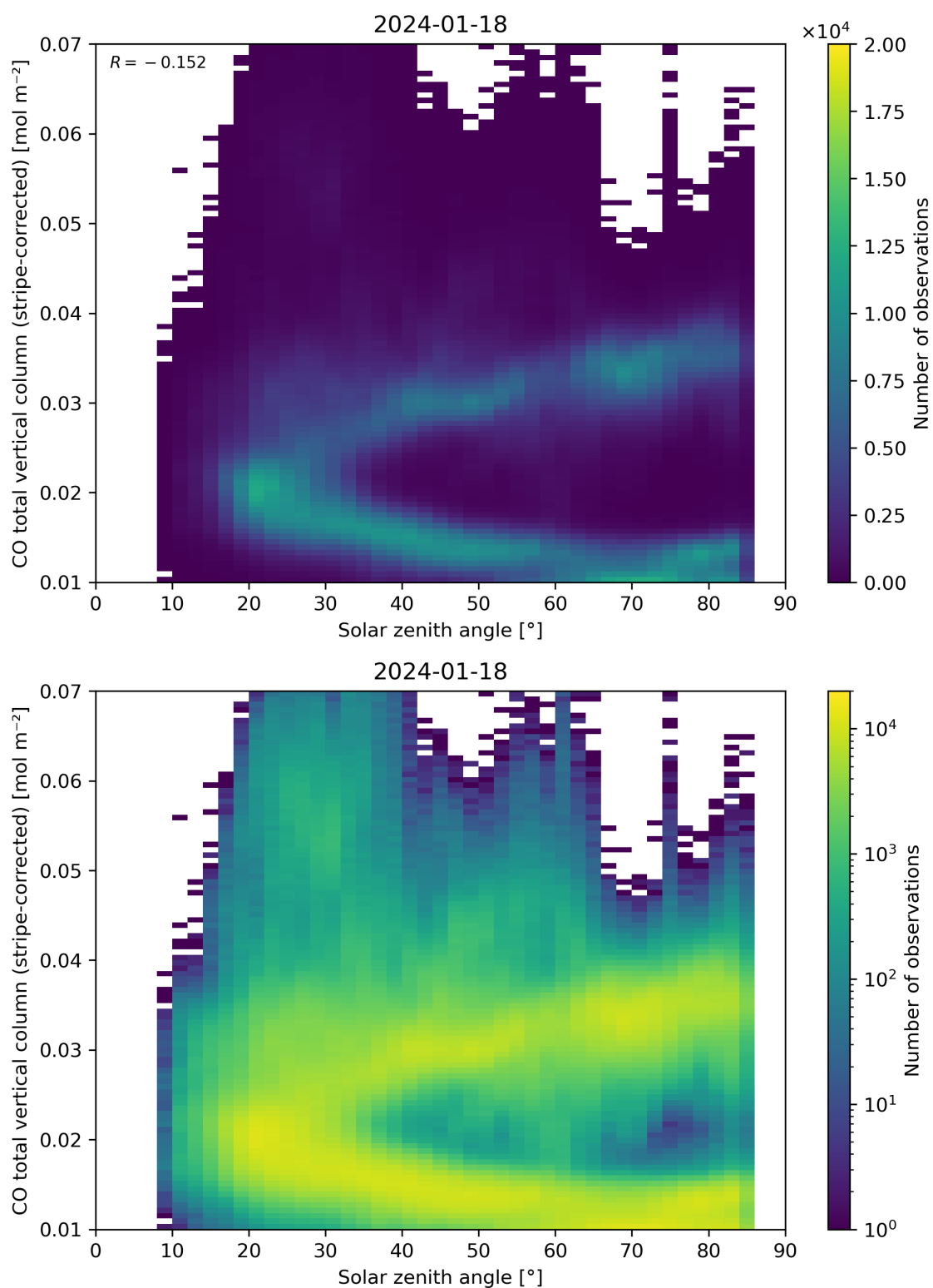
Figure 62: Scatter density plot of “Solar zenith angle” against “CO total vertical column (stripe-corrected)” for 2024-01-17 to 2024-01-19.
