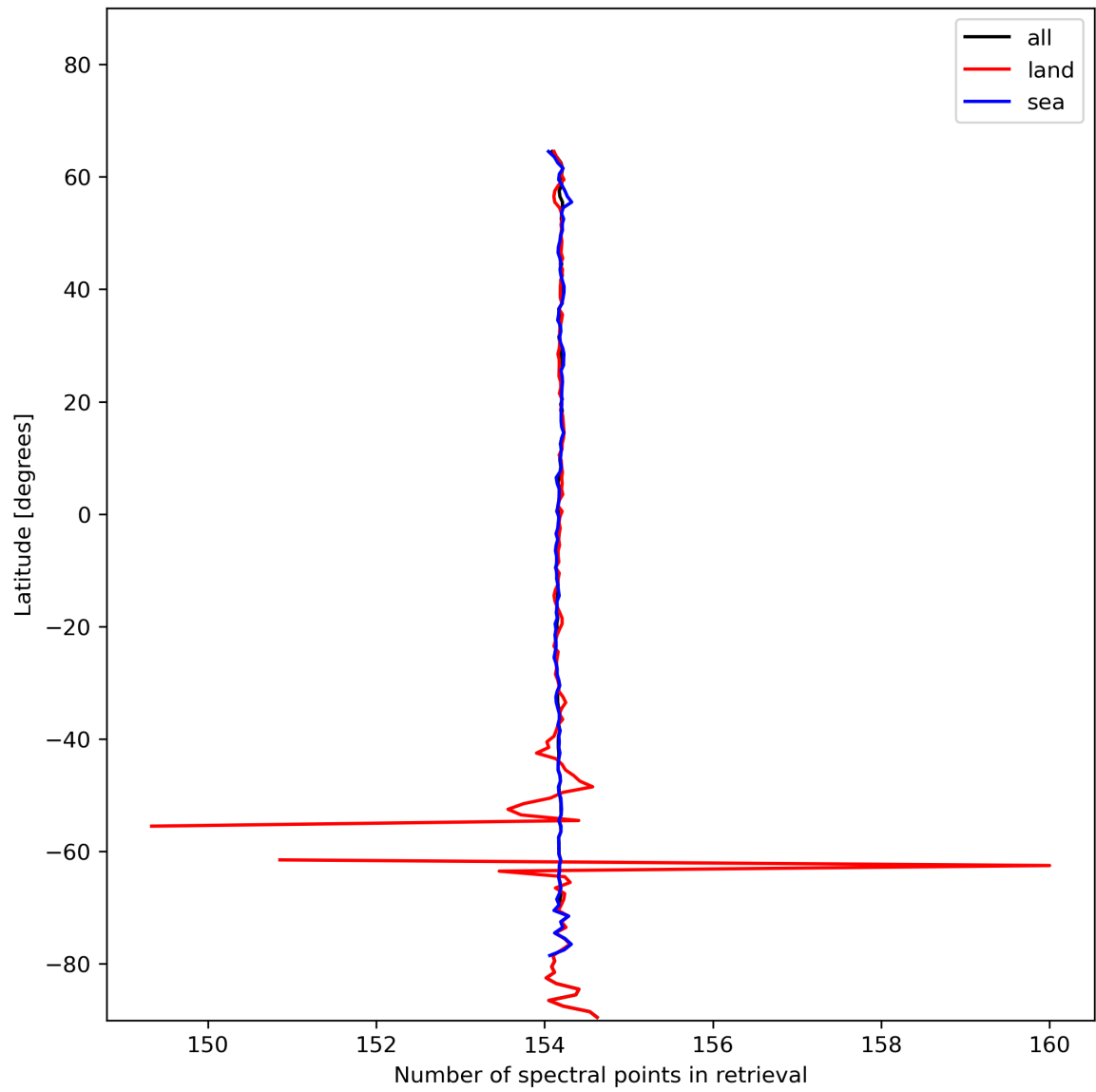
Figure 13: Zonal average of “Number of spectral points in retrieval” for 2024-01-17 to 2024-01-19.
