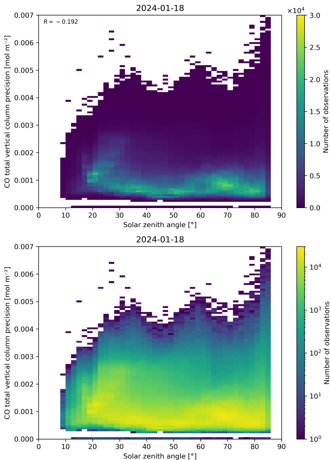
Figure 63: Scatter density plot of “Solar zenith angle” against “CO total vertical column precision” for 2024-01-17 to 2024-01-19.
