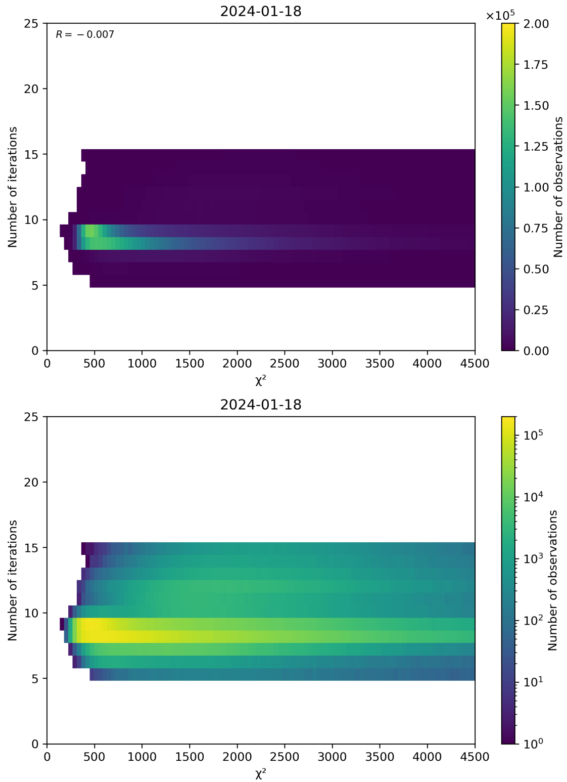
Figure 49: Scatter density plot of “ \chi^2 ” against “Number of iterations” for 2024-01-17 to 2024-01-19.
