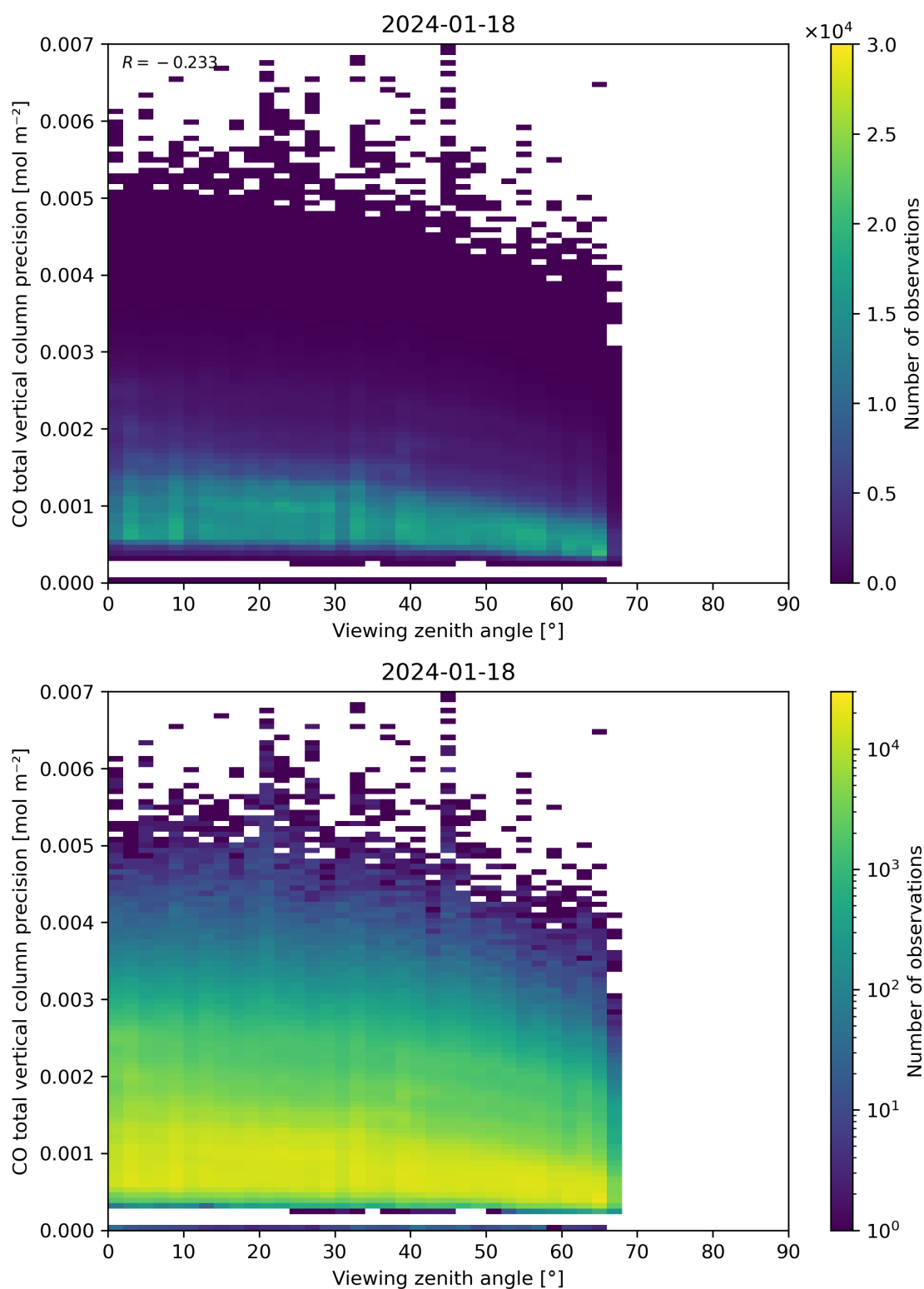
Figure 71: Scatter density plot of “Viewing zenith angle” against “CO total vertical column precision” for 2024-01-17 to 2024-01-19.
