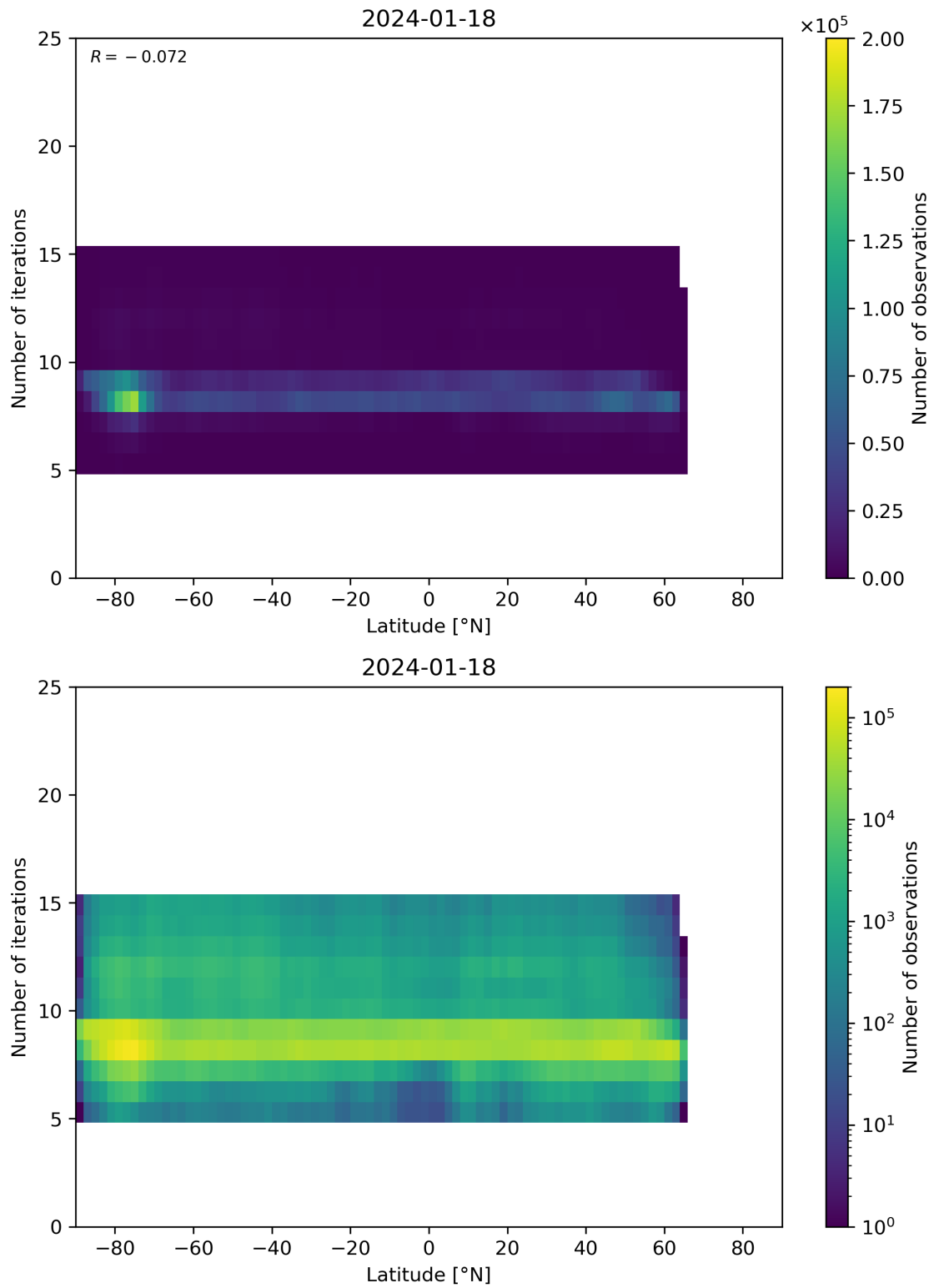
Figure 56: Scatter density plot of “Latitude” against “Number of iterations” for 2024-01-17 to 2024-01-19.
