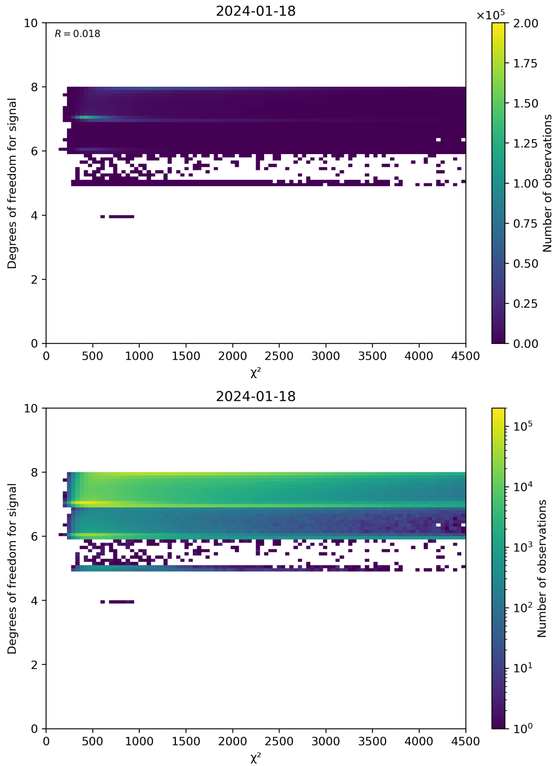
Figure 48: Scatter density plot of “ \chi^2 ” against “Degrees of freedom for signal” for 2024-01-17 to 2024-01-19.
