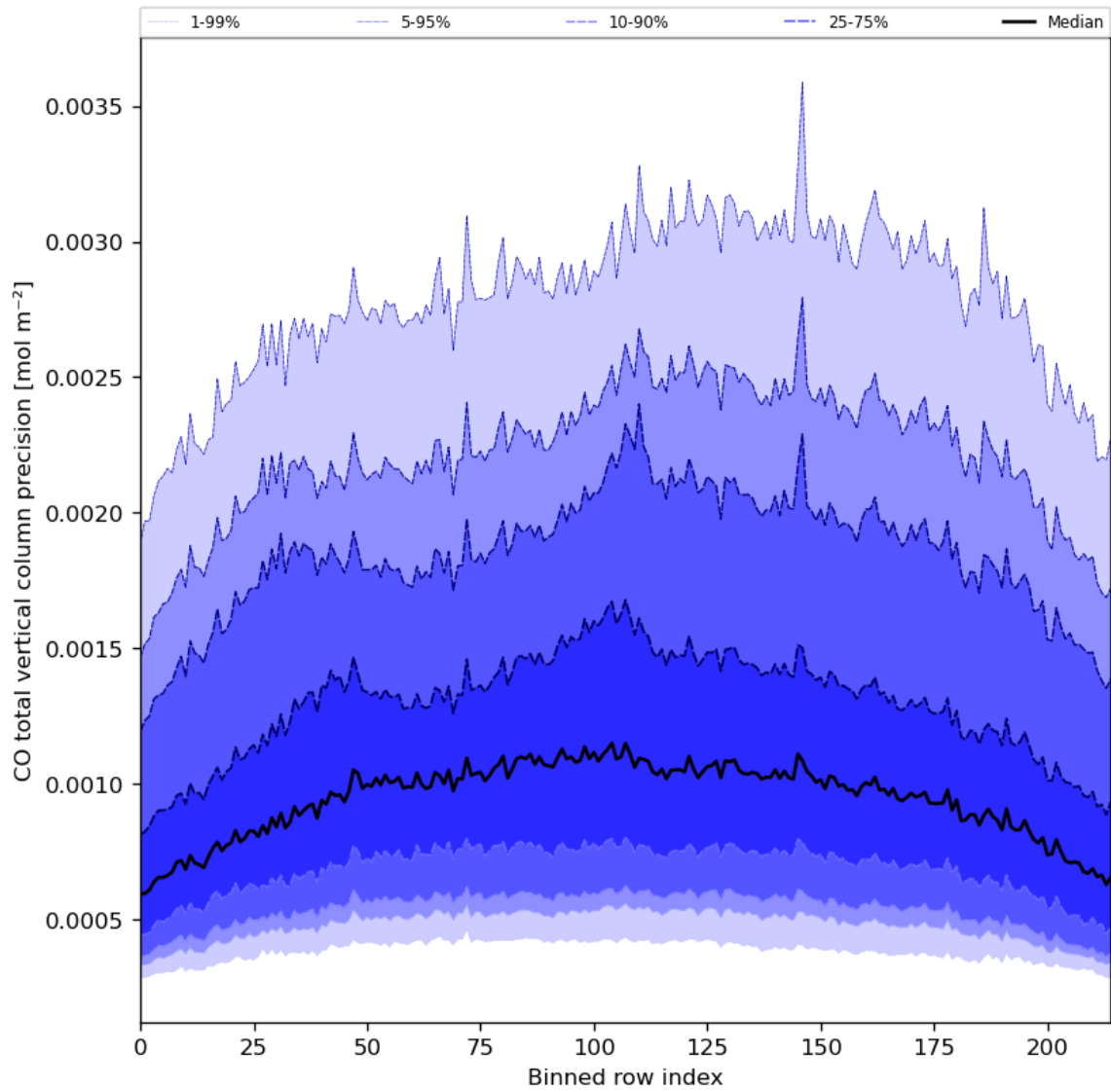
Figure 28: Along track statistics of “CO total vertical column precision” for 2024-01-17 to 2024-01-19
