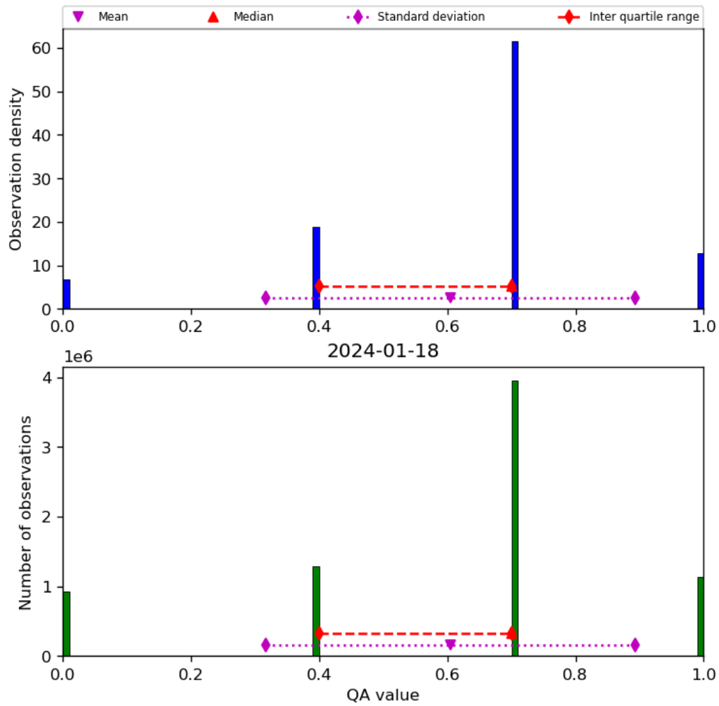
Figure 17: Histogram of “QA value” for 2024-01-17 to 2024-01-19
