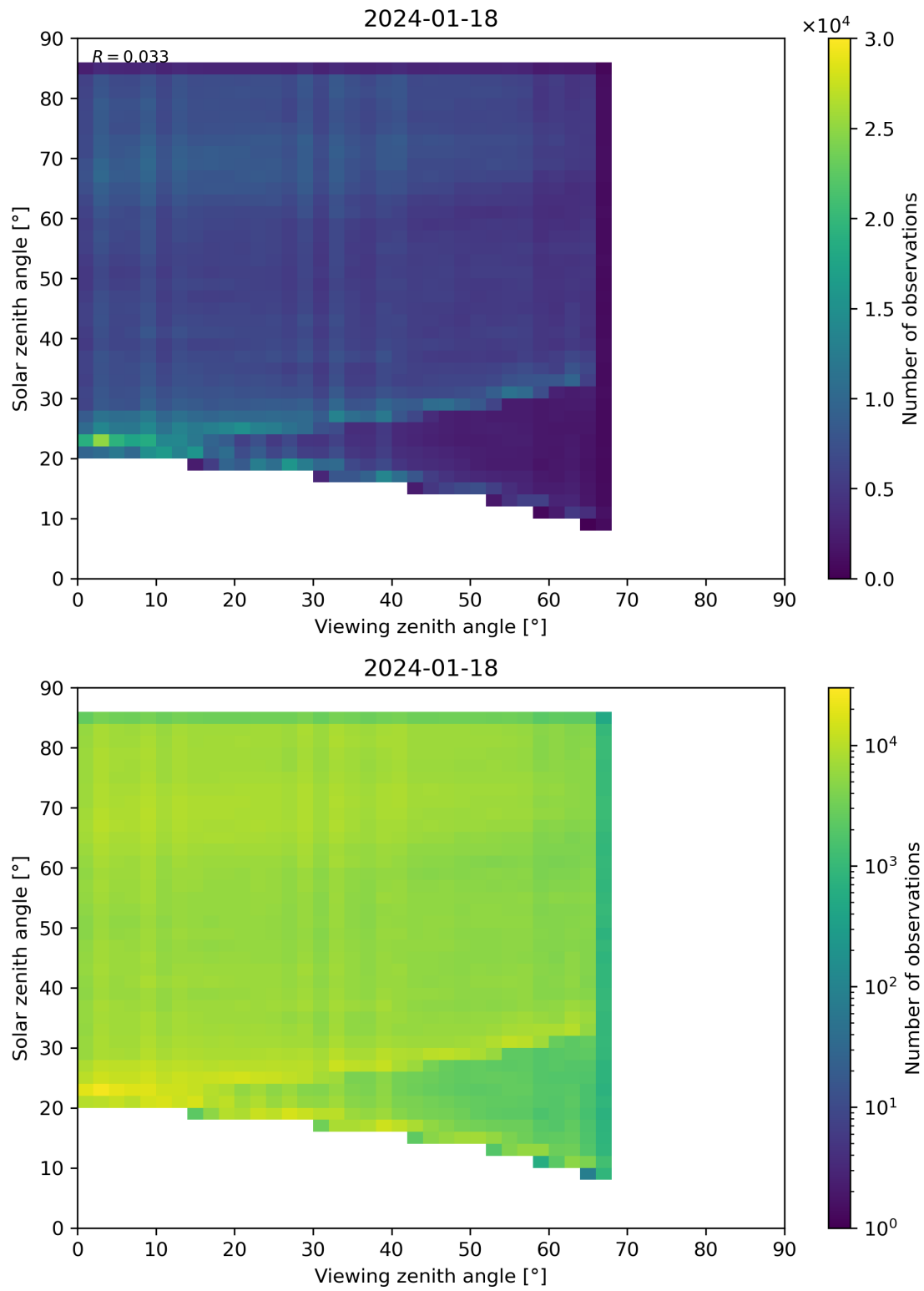
Figure 77: Scatter density plot of “Viewing zenith angle” against “Solar zenith angle” for 2024-01-17 to 2024-01-19.
