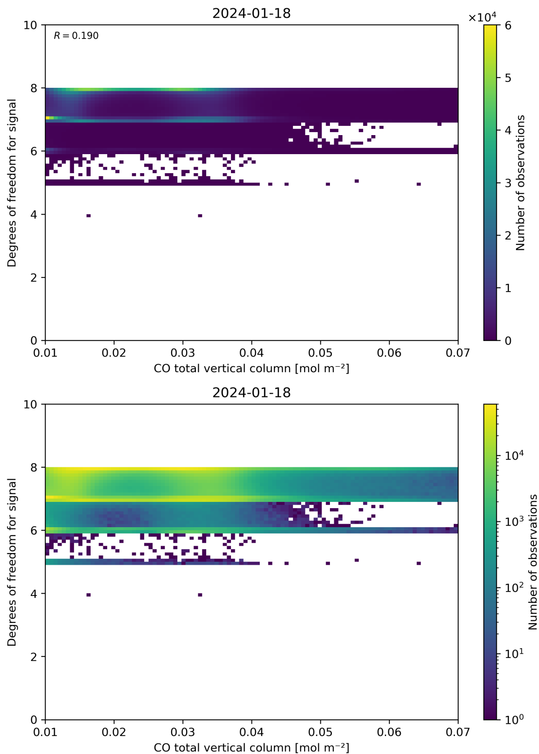
Figure 41: Scatter density plot of “CO total vertical column” against “Degrees of freedom for signal” for 2024-01-17 to 2024-01-19.
