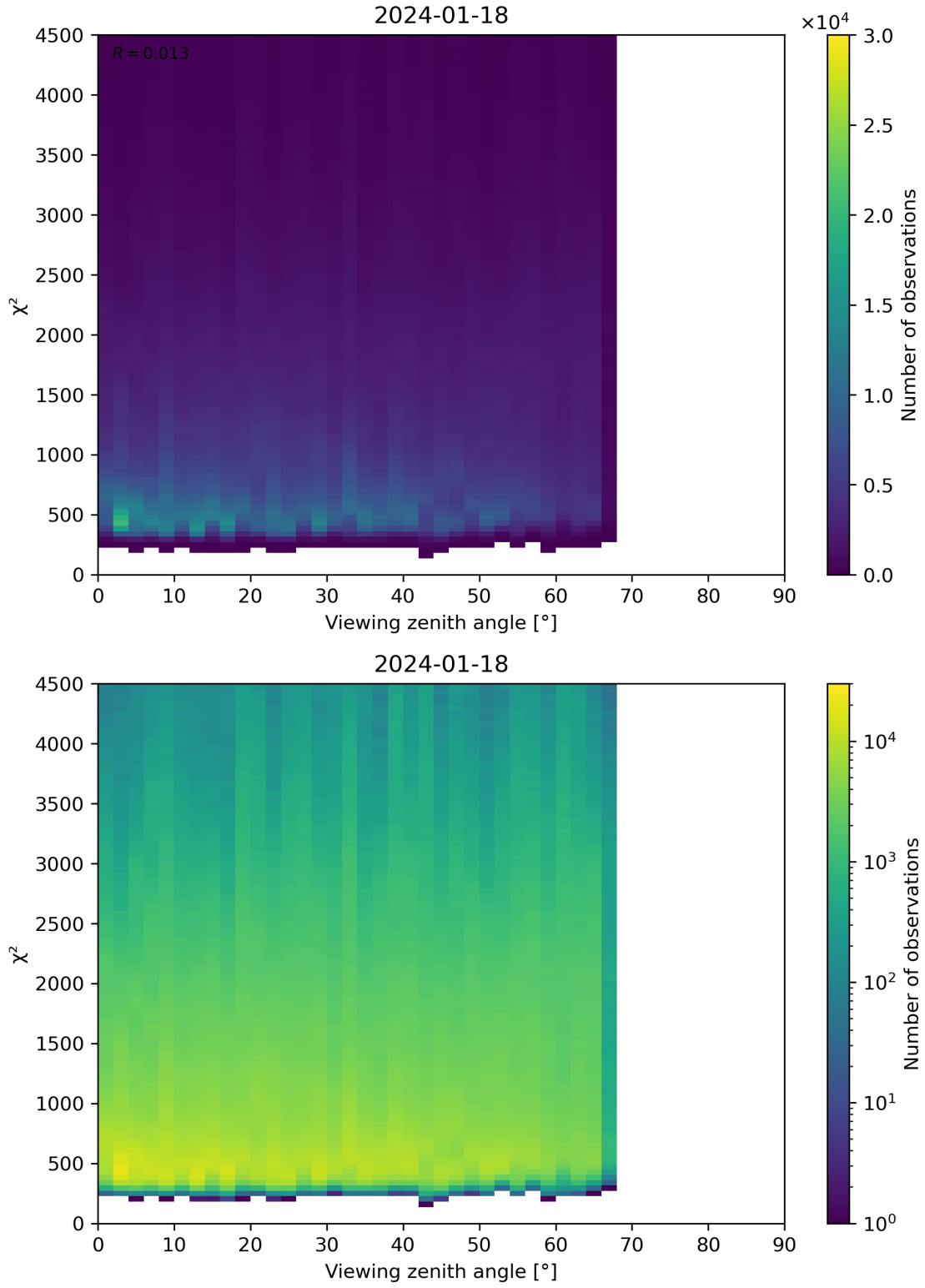
Figure 72: Scatter density plot of “Viewing zenith angle” against “ \chi^2 ” for 2024-01-17 to 2024-01-19.
