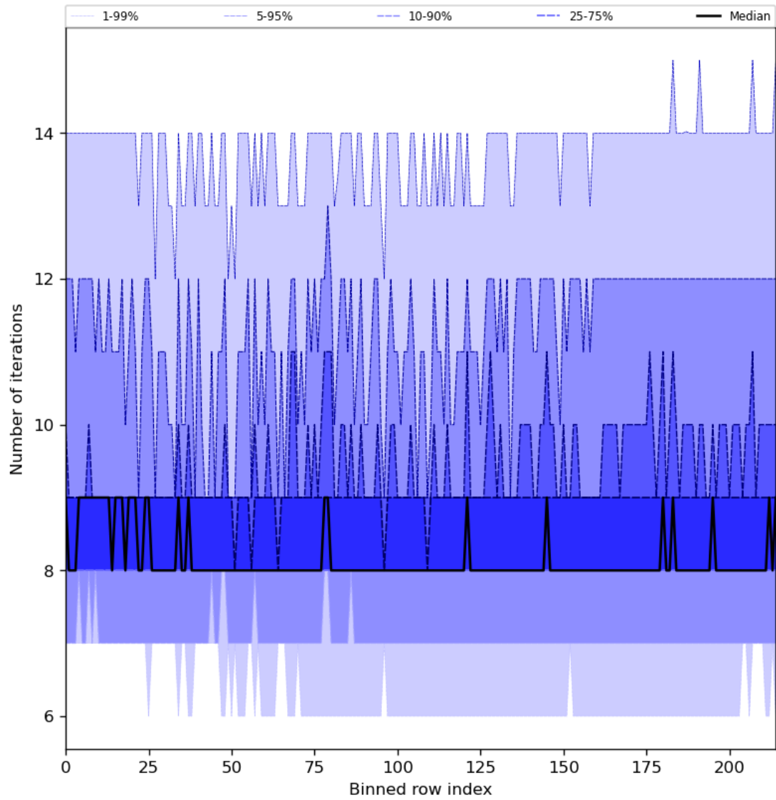
Figure 32: Along track statistics of “Number of iterations” for 2024-01-17 to 2024-01-19
