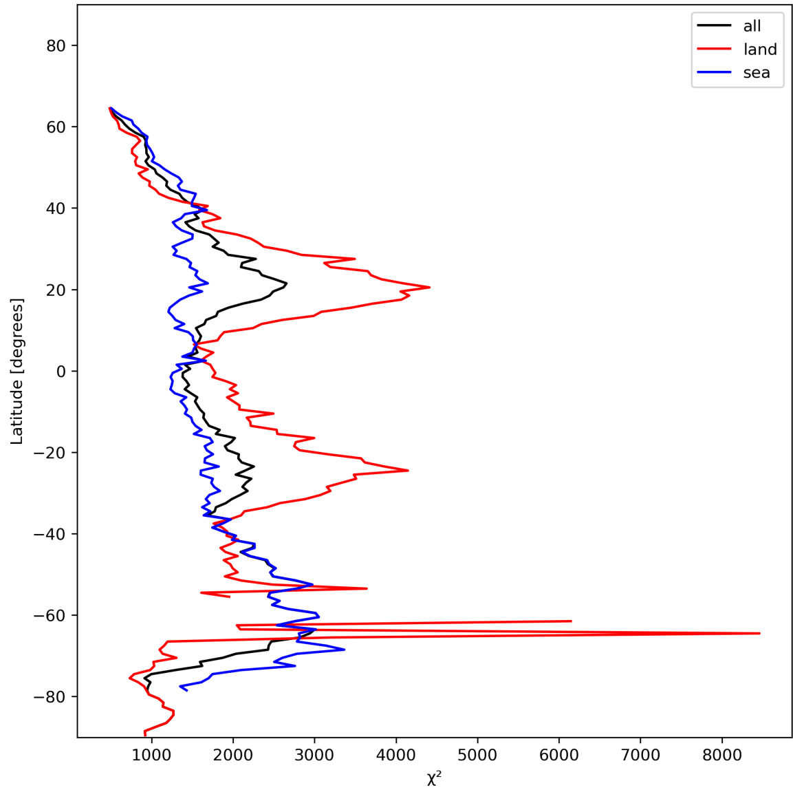
Figure 14: Zonal average of “ \chi^2 ” for 2024-01-19 to 2024-01-21.
