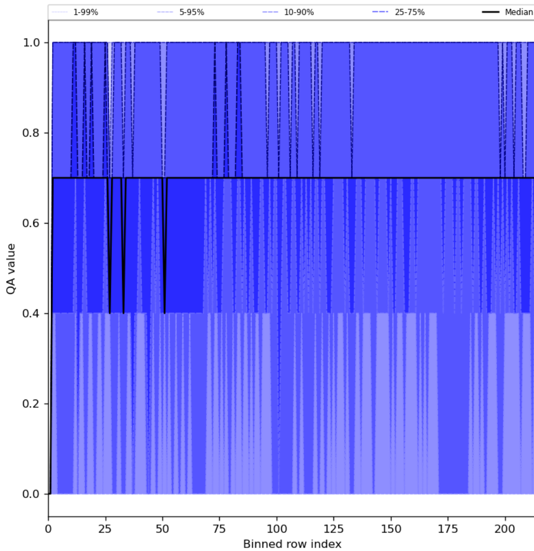
Figure 25: Along track statistics of “QA value” for 2024-01-19 to 2024-01-21
