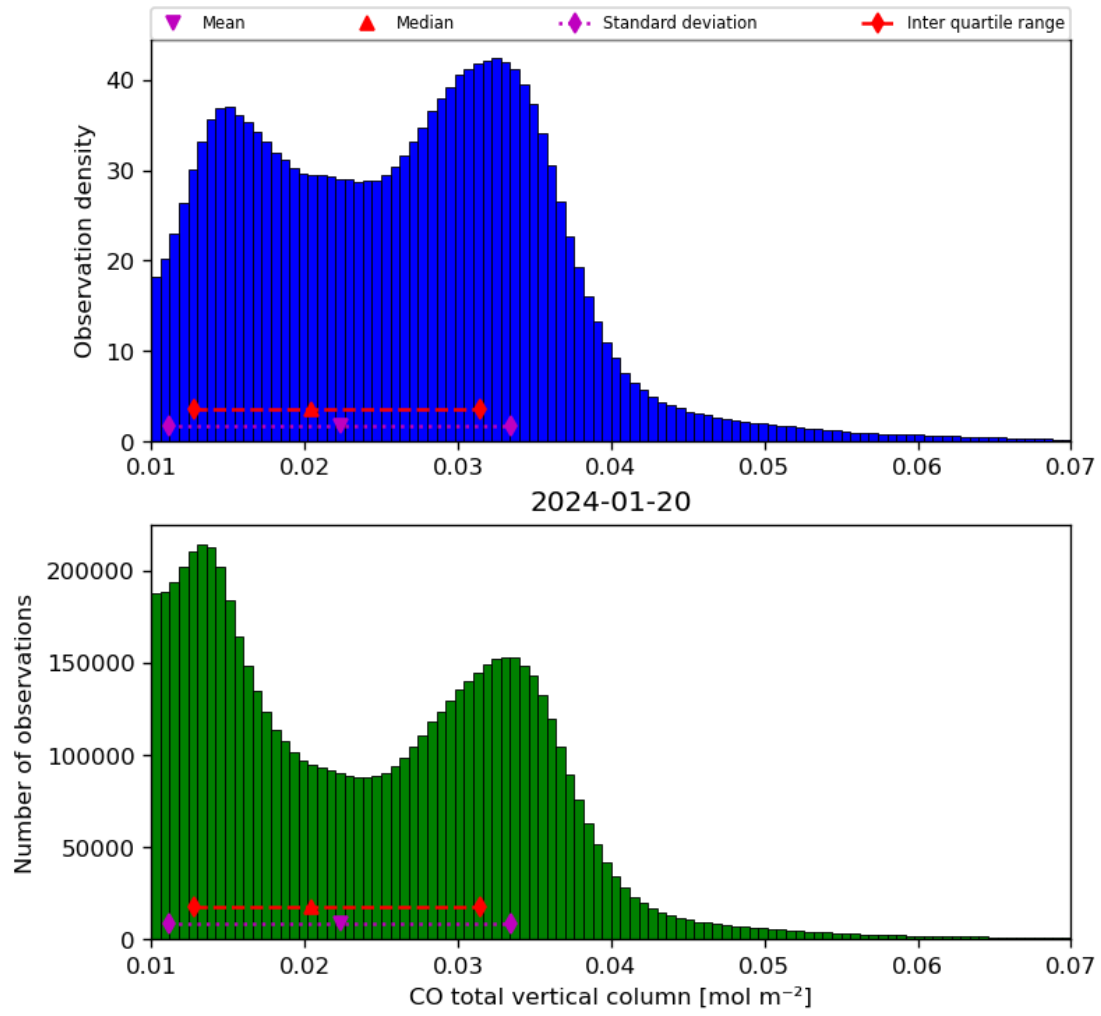
Figure 18: Histogram of “CO total vertical column” for 2024-01-19 to 2024-01-21
