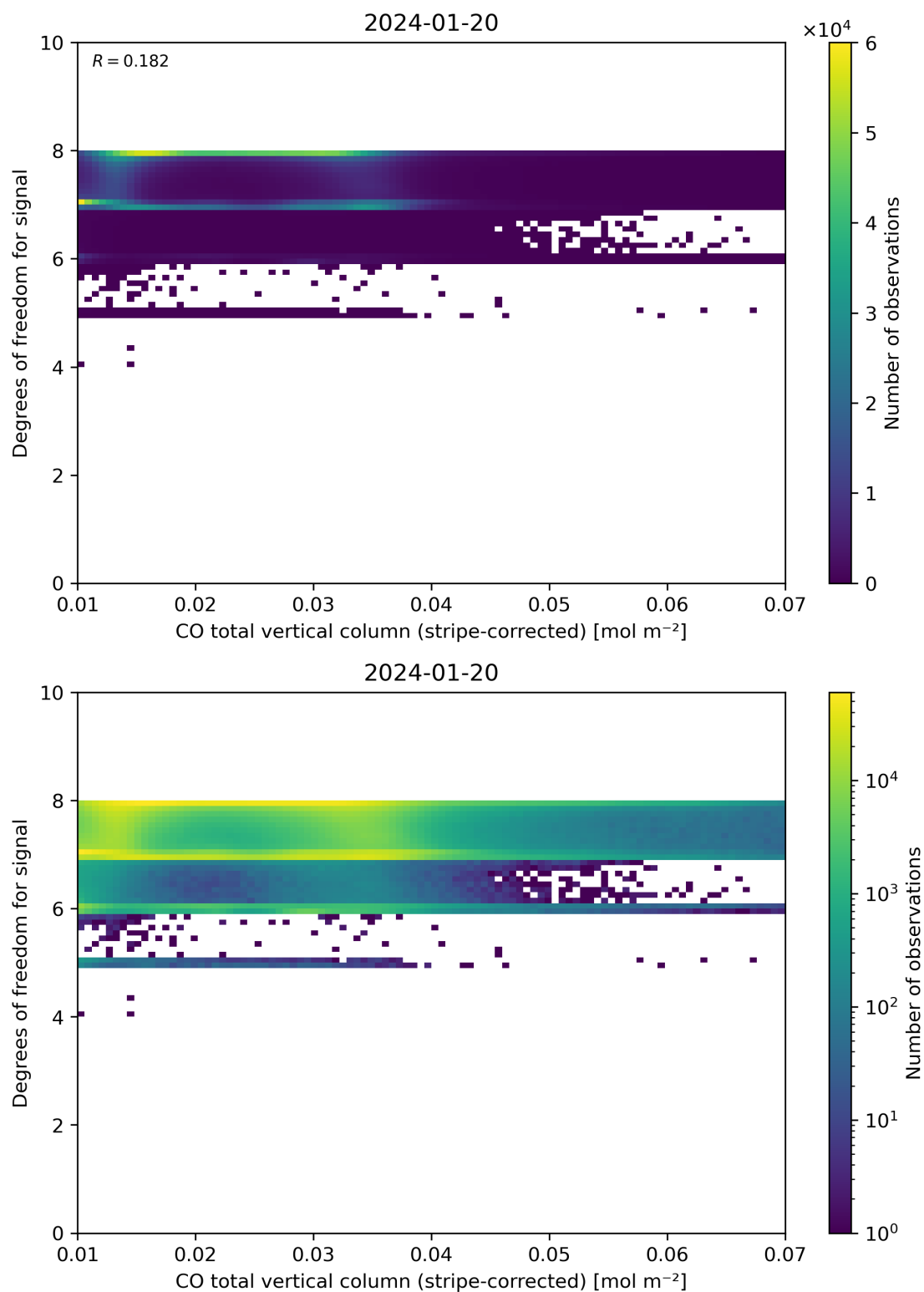
Figure 38: Scatter density plot of “CO total vertical column (stripe-corrected)” against “Degrees of freedom for signal” for 2024-01-19 to 2024-01-21.
