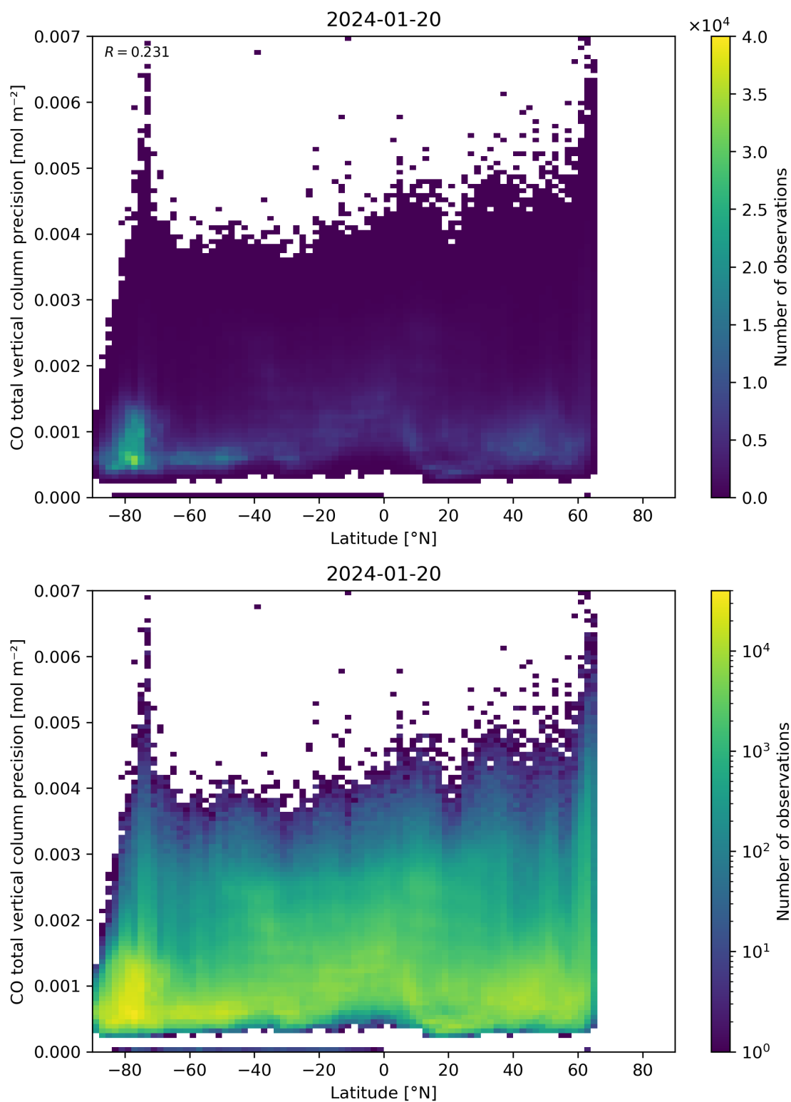
Figure 53: Scatter density plot of “Latitude” against “CO total vertical column precision” for 2024-01-19 to 2024-01-21.
