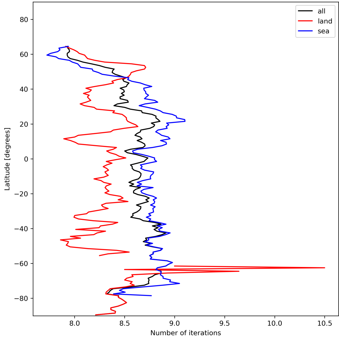
Figure 16: Zonal average of “Number of iterations” for 2024-01-19 to 2024-01-21.
