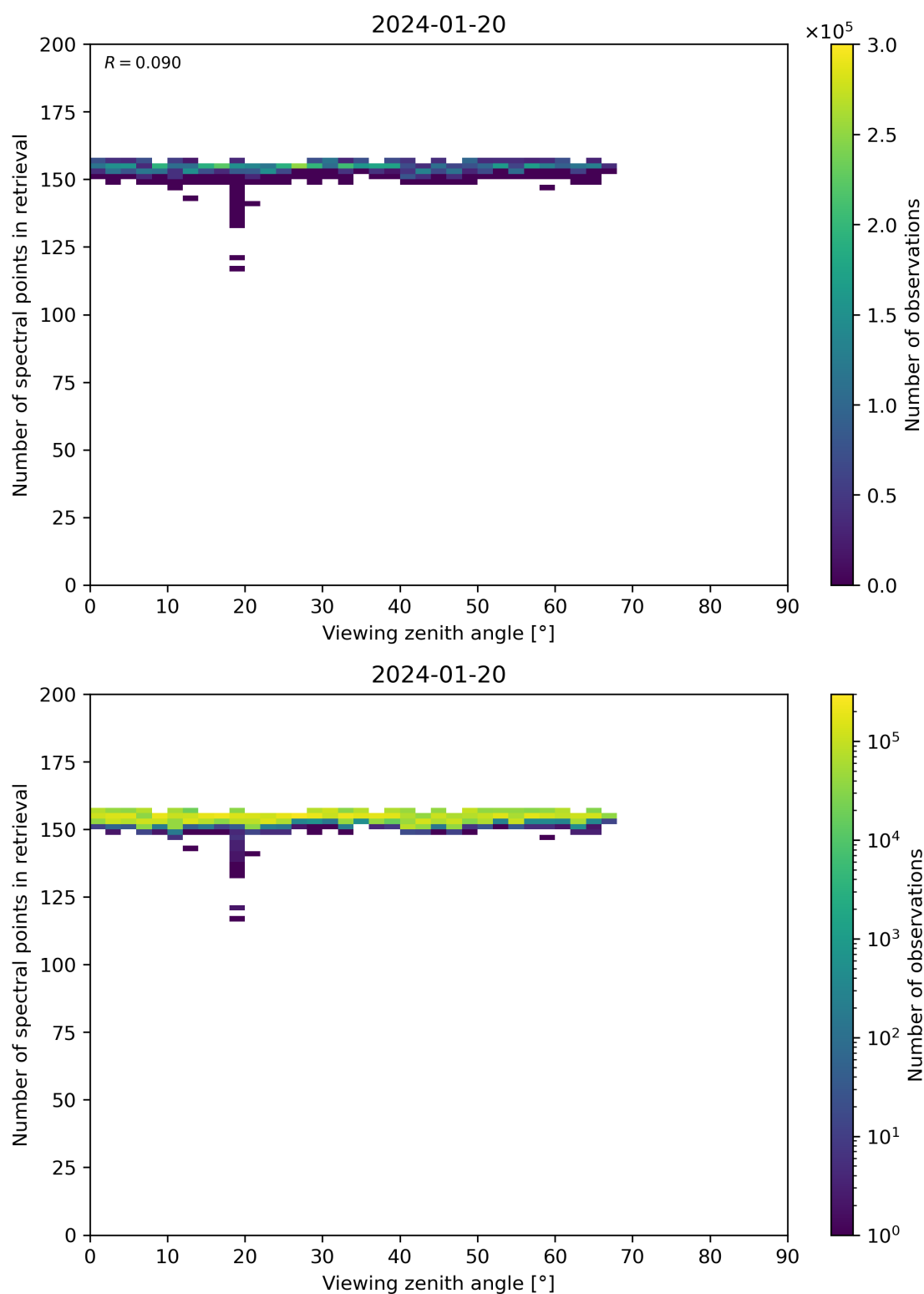
Figure 76: Scatter density plot of “Viewing zenith angle” against “Number of spectral points in retrieval” for 2024-01-19 to 2024-01-21.
