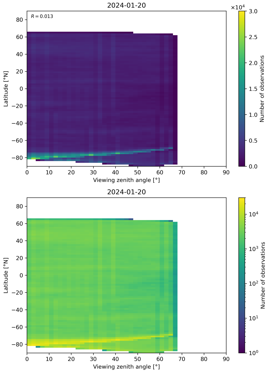
Figure 74: Scatter density plot of “Viewing zenith angle” against “Latitude” for 2024-01-19 to 2024-01-21.
