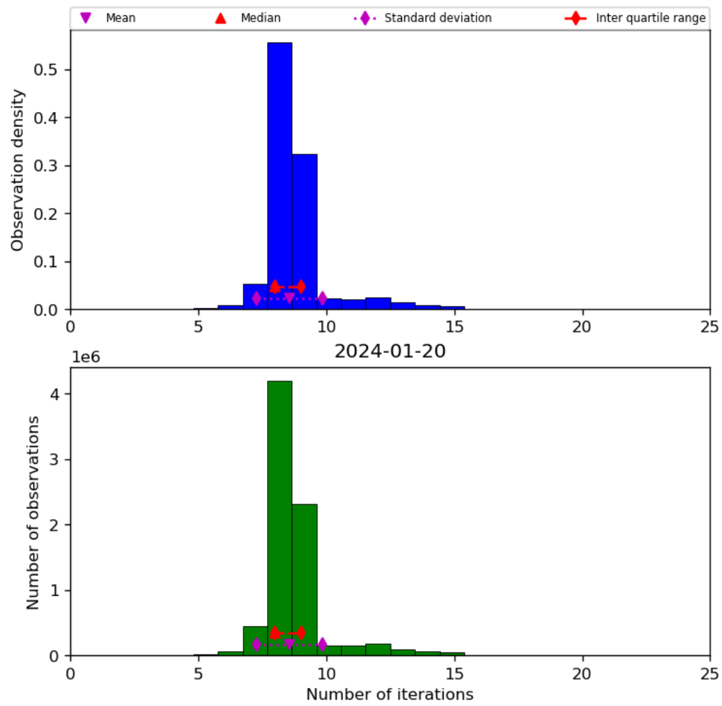
Figure 24: Histogram of “Number of iterations” for 2024-01-19 to 2024-01-21
