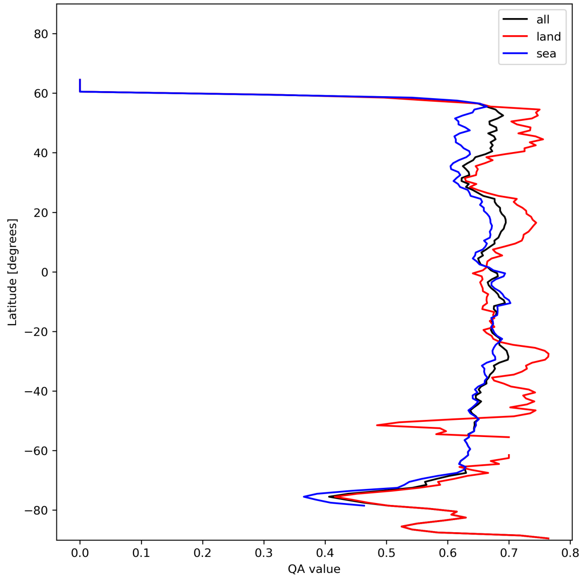
Figure 9: Zonal average of “QA value” for 2024-01-19 to 2024-01-21.
