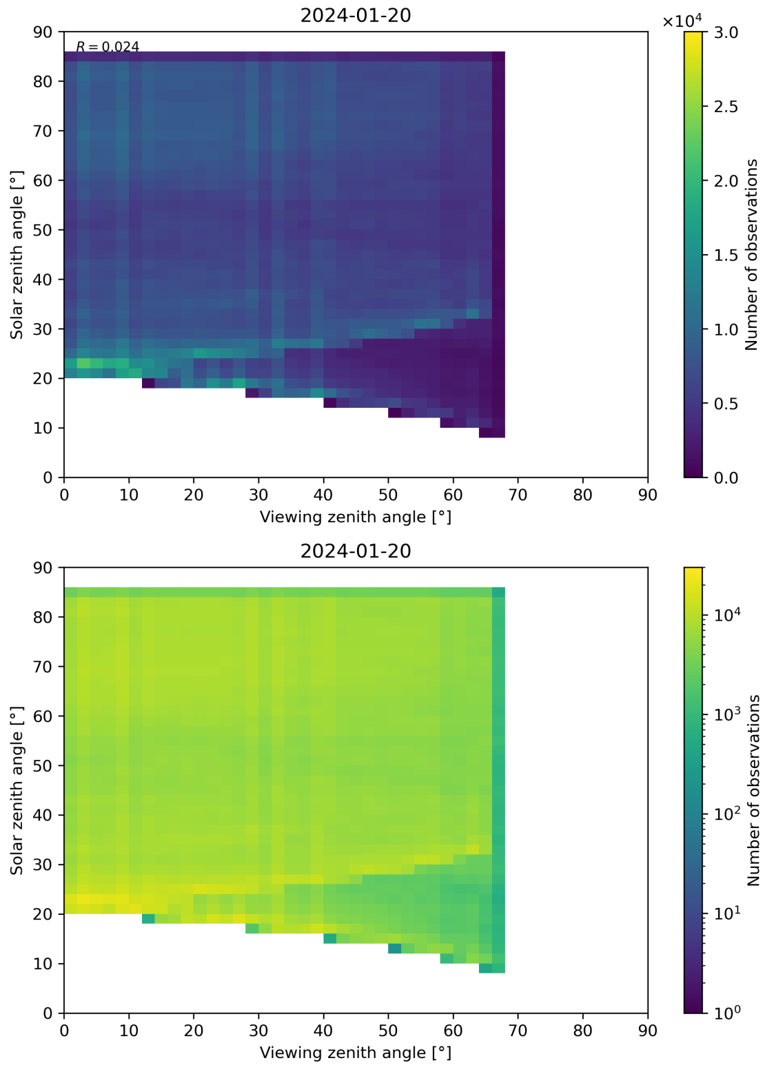
Figure 77: Scatter density plot of “Viewing zenith angle” against “Solar zenith angle” for 2024-01-19 to 2024-01-21.
