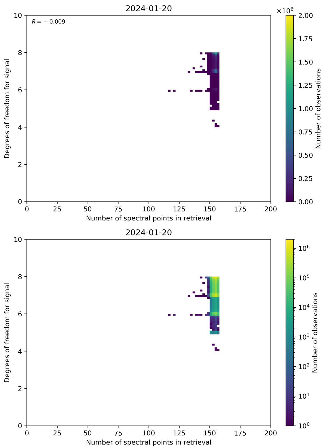
Figure 59: Scatter density plot of “Number of spectral points in retrieval” against “Degrees of freedom for signal” for 2024-01-19 to 2024-01-21.
