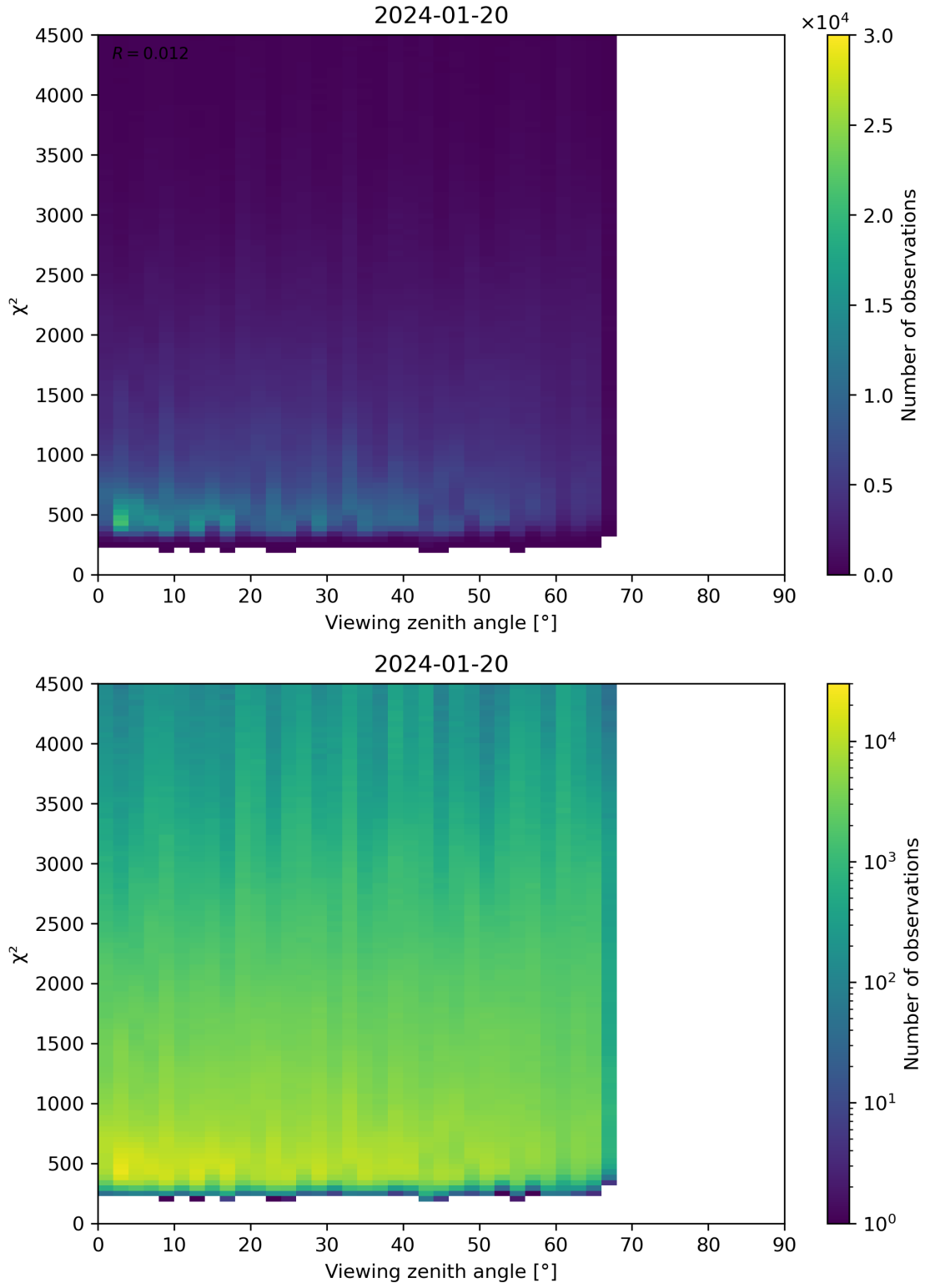
Figure 72: Scatter density plot of “Viewing zenith angle” against “ \chi^2 ” for 2024-01-19 to 2024-01-21.
