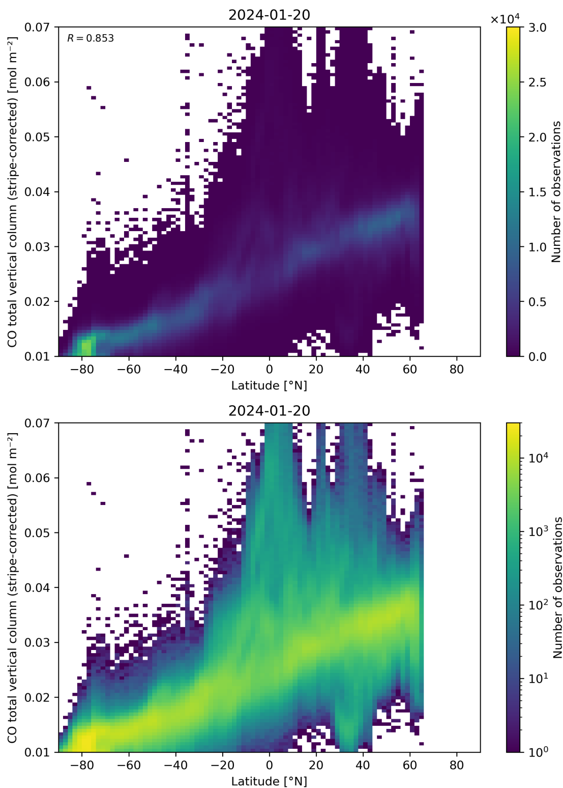
Figure 52: Scatter density plot of “Latitude” against “CO total vertical column (stripe-corrected)” for 2024-01-19 to 2024-01-21.
