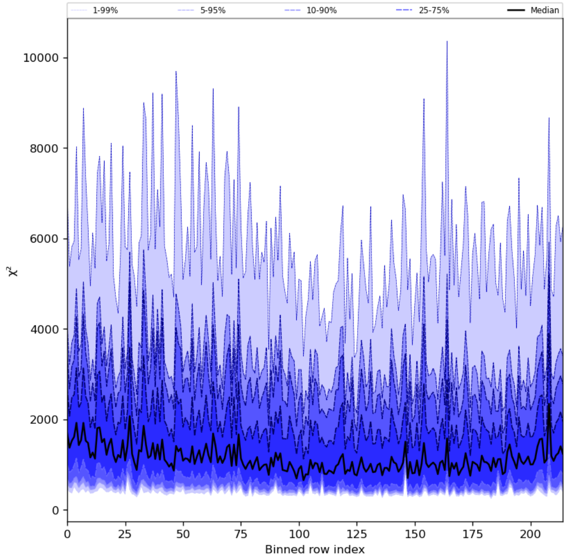
Figure 30: Along track statistics of “ \chi^2 ” for 2024-01-19 to 2024-01-21
