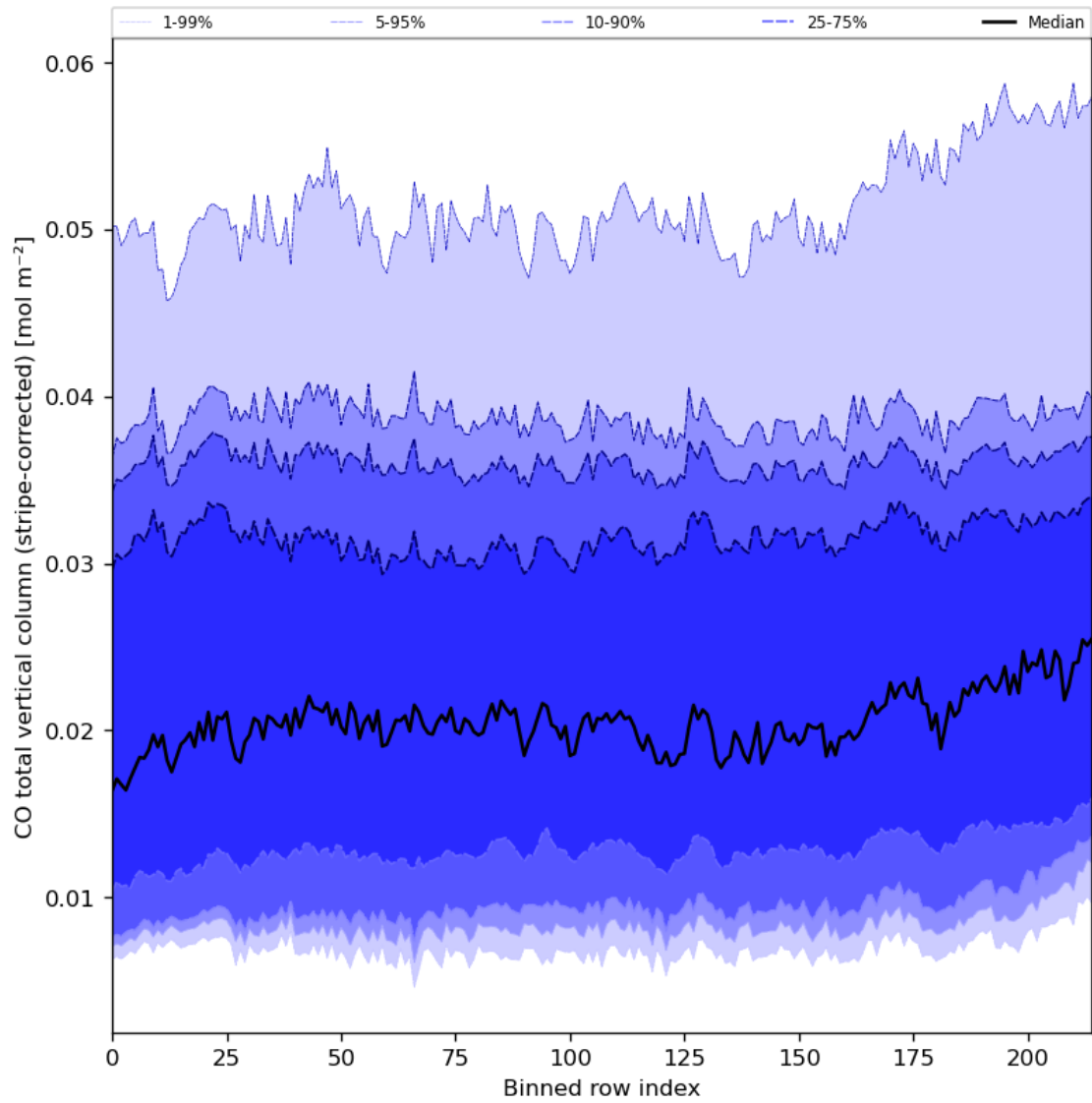
Figure 27: Along track statistics of “CO total vertical column (stripe-corrected)” for 2024-01-19 to 2024-01-21
