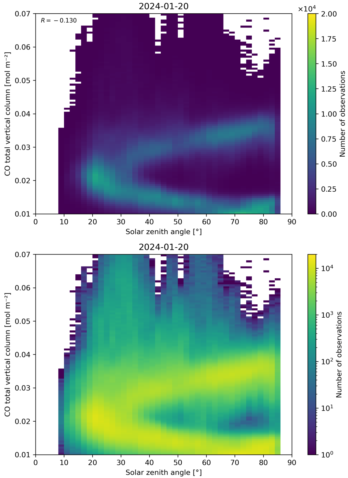
Figure 61: Scatter density plot of “Solar zenith angle” against “CO total vertical column” for 2024-01-19 to 2024-01-21.
