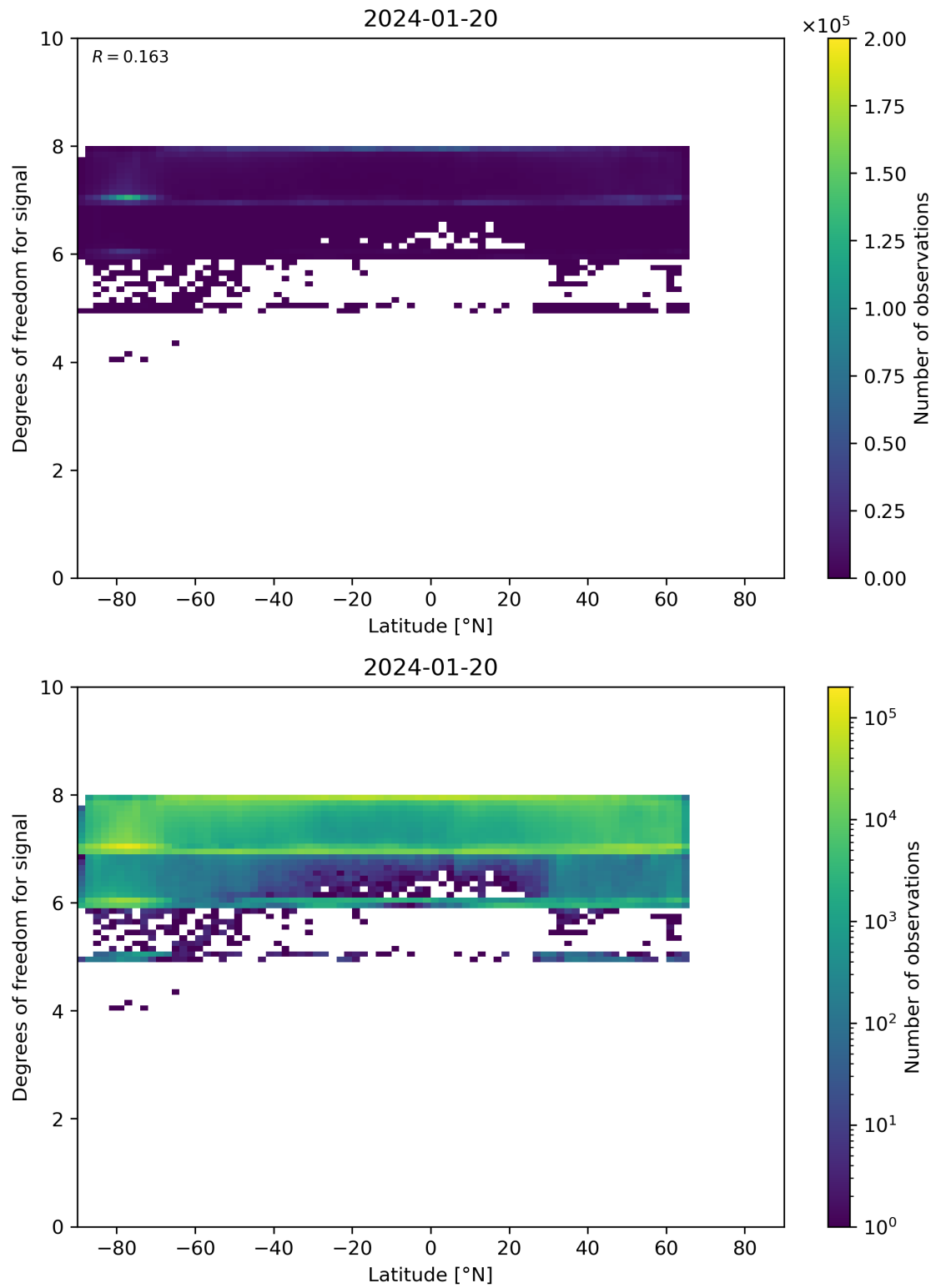
Figure 55: Scatter density plot of “Latitude” against “Degrees of freedom for signal” for 2024-01-19 to 2024-01-21.
