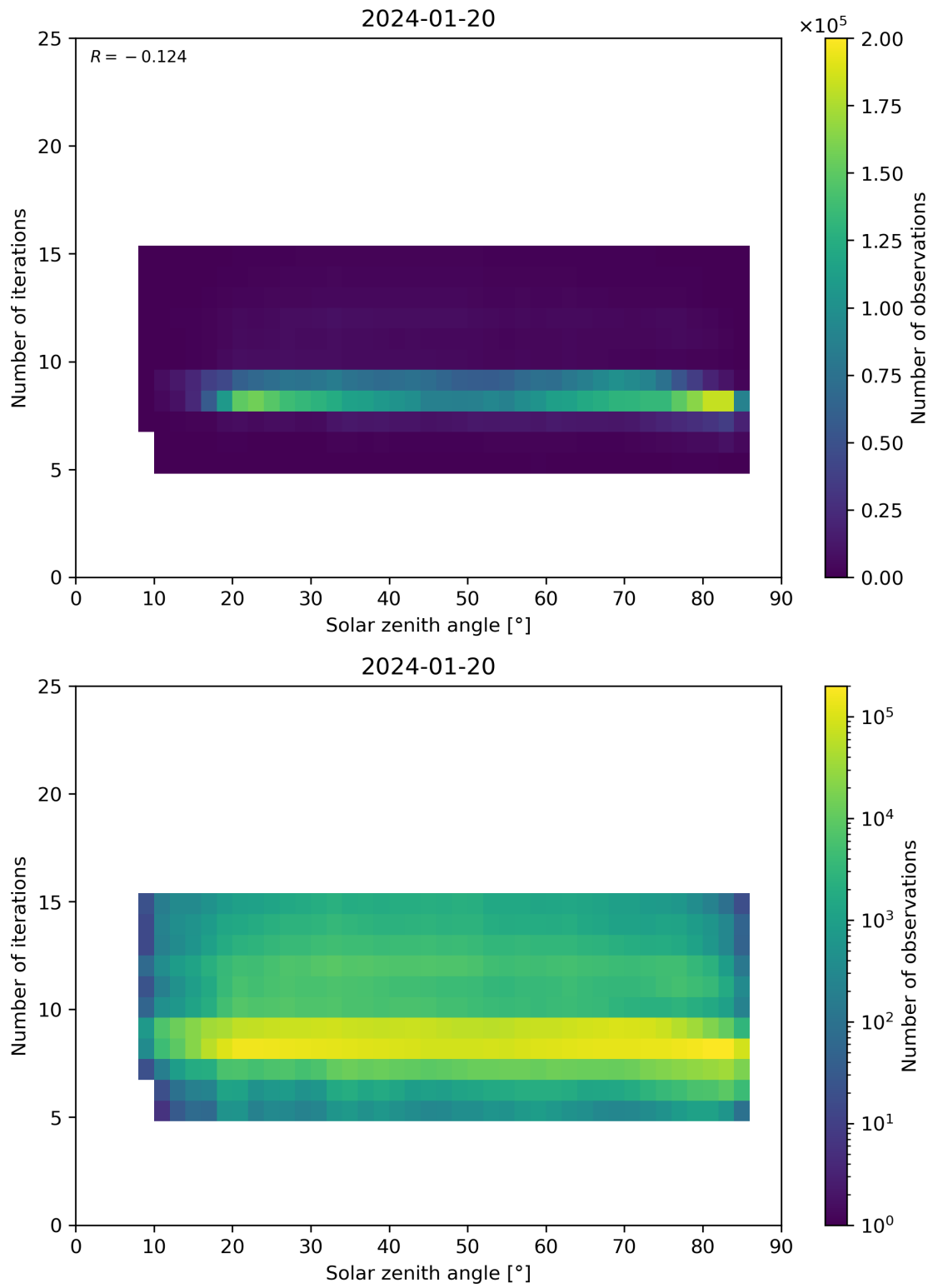
Figure 67: Scatter density plot of “Solar zenith angle” against “Number of iterations” for 2024-01-19 to 2024-01-21.
