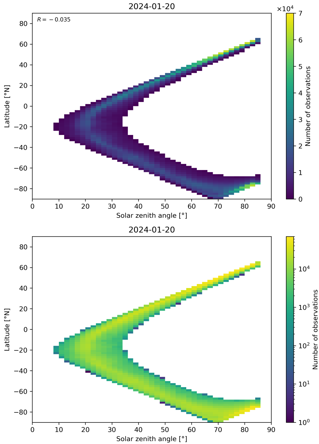
Figure 66: Scatter density plot of “Solar zenith angle” against “Latitude” for 2024-01-19 to 2024-01-21.
