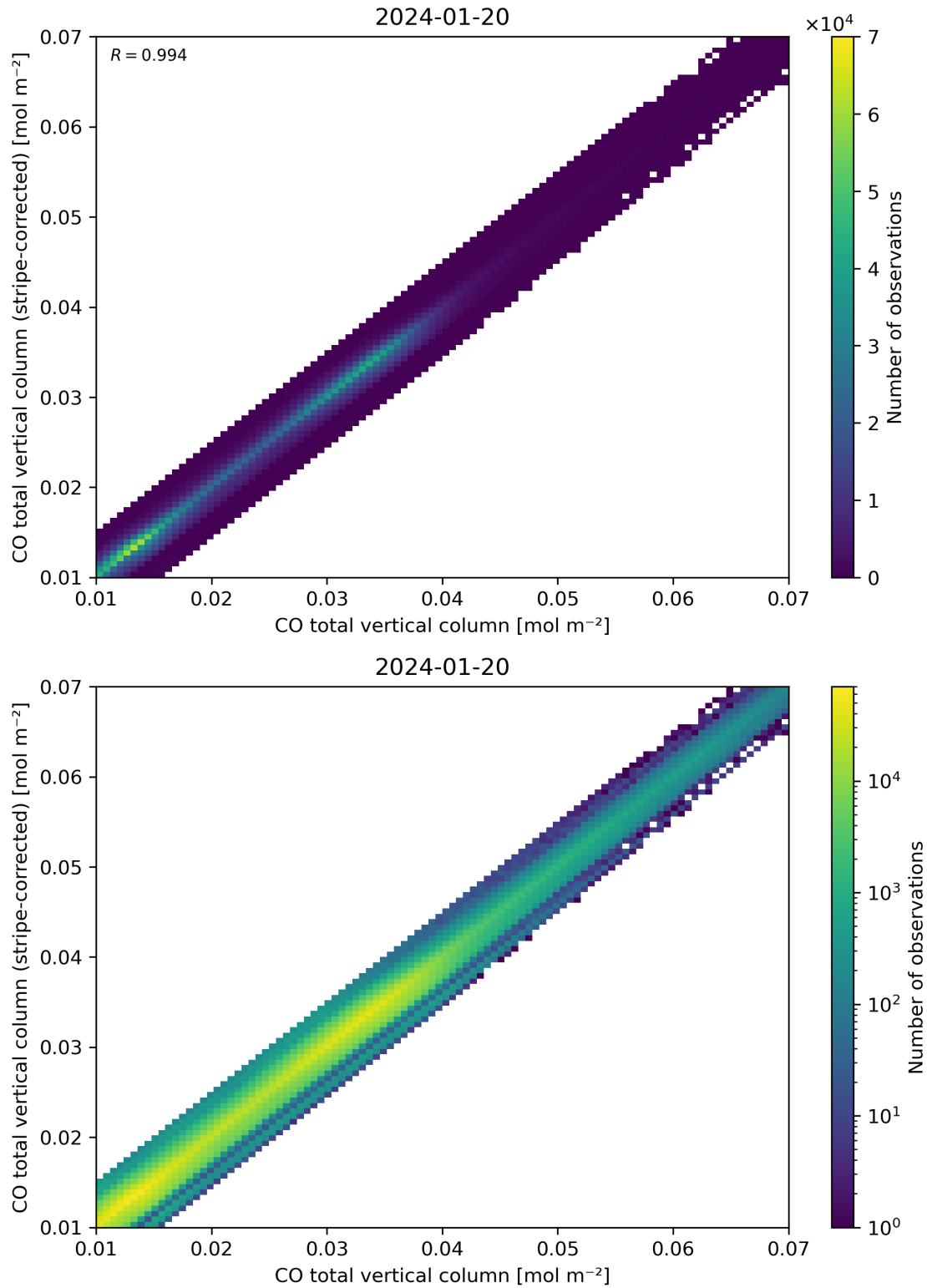
Figure 33: Scatter density plot of “CO total vertical column” against “CO total vertical column (stripe-corrected)” for 2024-01-19 to 2024-01-21.
