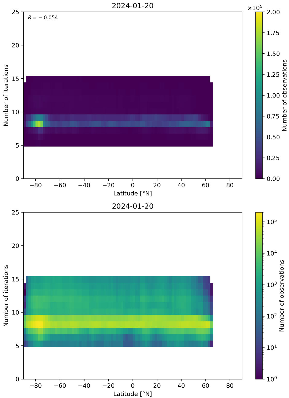
Figure 56: Scatter density plot of “Latitude” against “Number of iterations” for 2024-01-19 to 2024-01-21.
