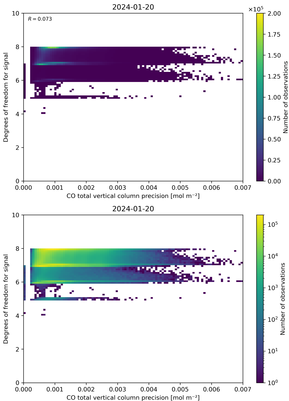
Figure 45: Scatter density plot of “CO total vertical column precision” against “Degrees of freedom for signal” for 2024-01-19 to 2024-01-21.
