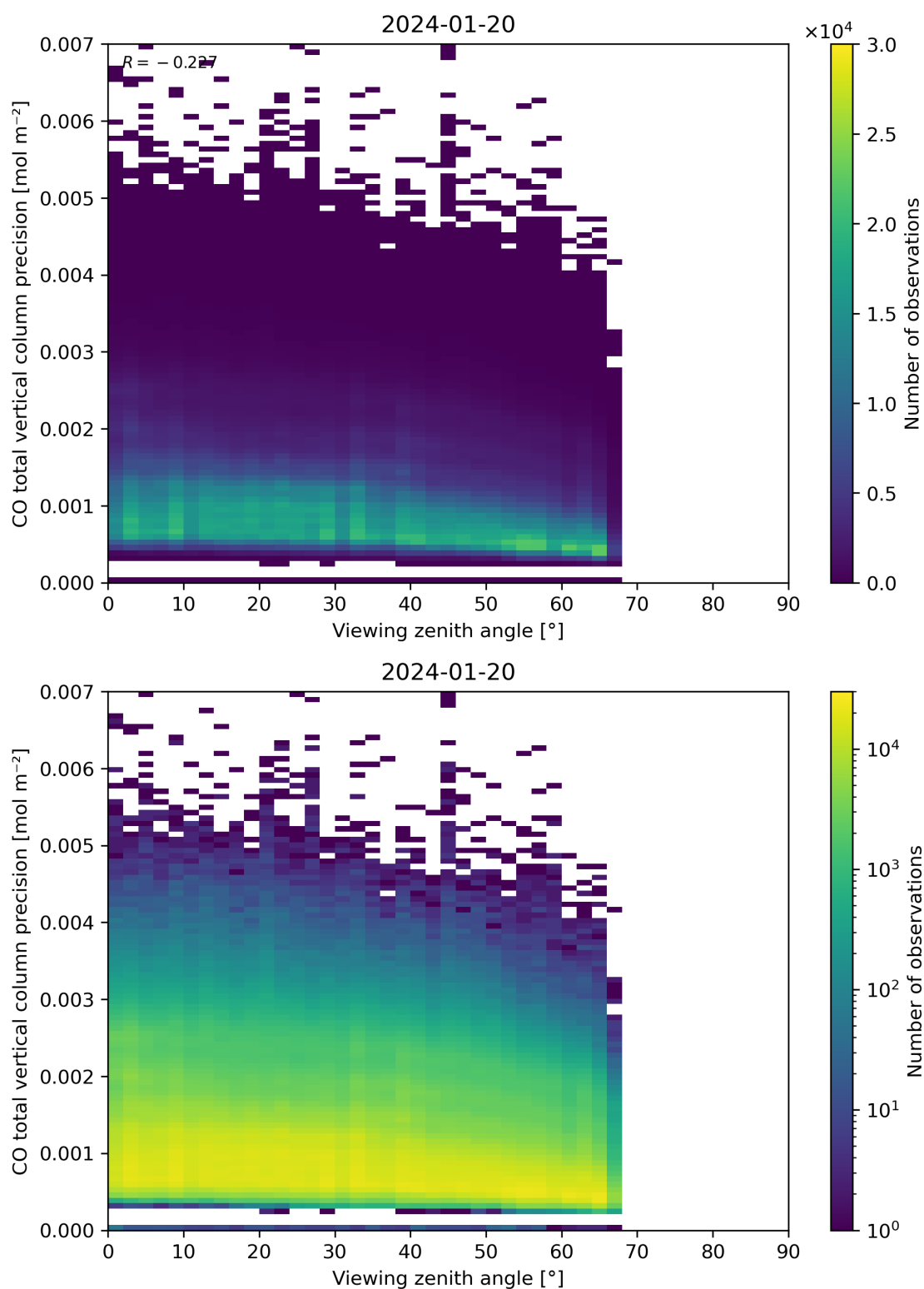
Figure 71: Scatter density plot of “Viewing zenith angle” against “CO total vertical column precision” for 2024-01-19 to 2024-01-21.
