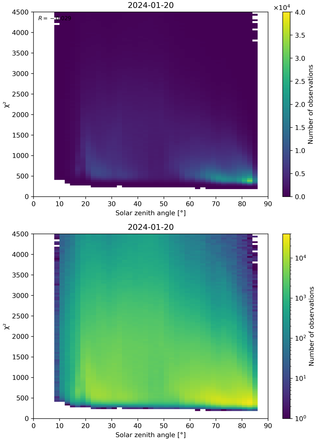
Figure 64: Scatter density plot of “Solar zenith angle” against “ \chi^2 ” for 2024-01-19 to 2024-01-21.
