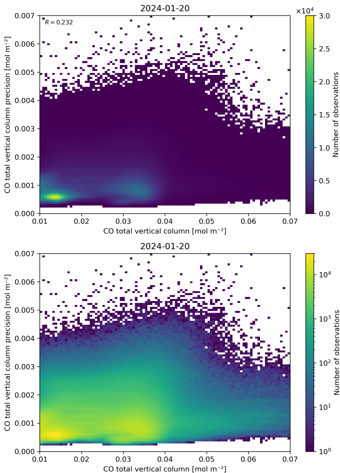
Figure 34: Scatter density plot of “CO total vertical column” against “CO total vertical column precision” for 2024-01-19 to 2024-01-21.
