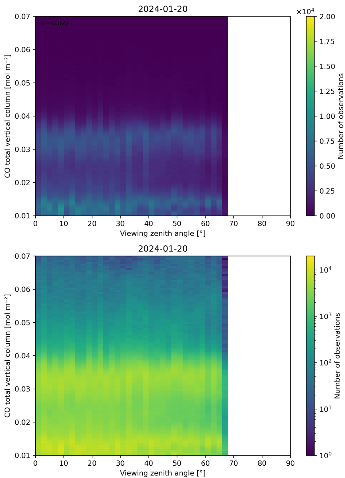
Figure 69: Scatter density plot of “Viewing zenith angle” against “CO total vertical column” for 2024-01-19 to 2024-01-21.
