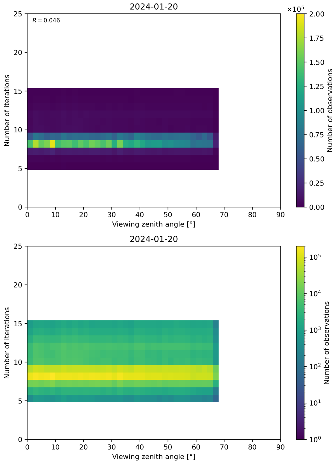
Figure 75: Scatter density plot of “Viewing zenith angle” against “Number of iterations” for 2024-01-19 to 2024-01-21.
