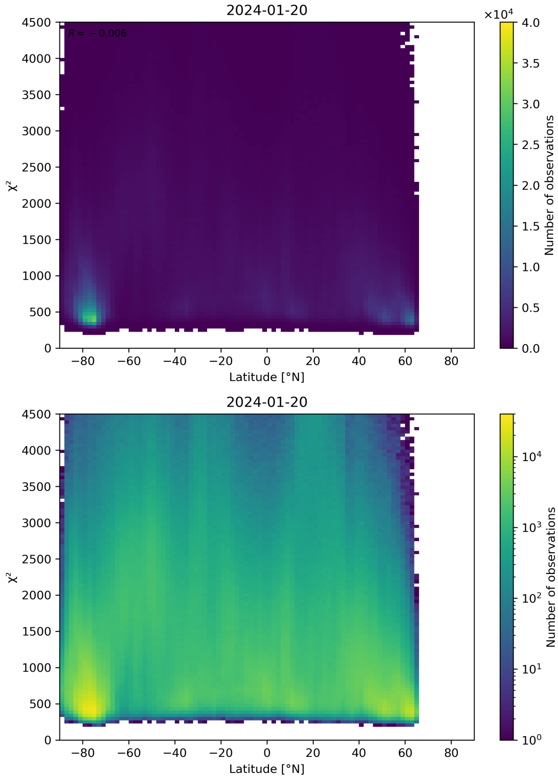
Figure 54: Scatter density plot of “Latitude” against “ \chi^2 ” for 2024-01-19 to 2024-01-21.
