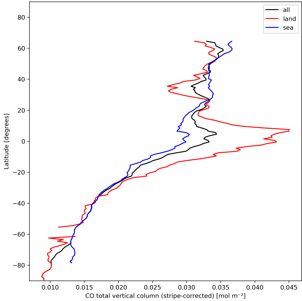
Figure 11: Zonal average of “CO total vertical column (stripe-corrected)” for 2024-01-19 to 2024-01-21.
