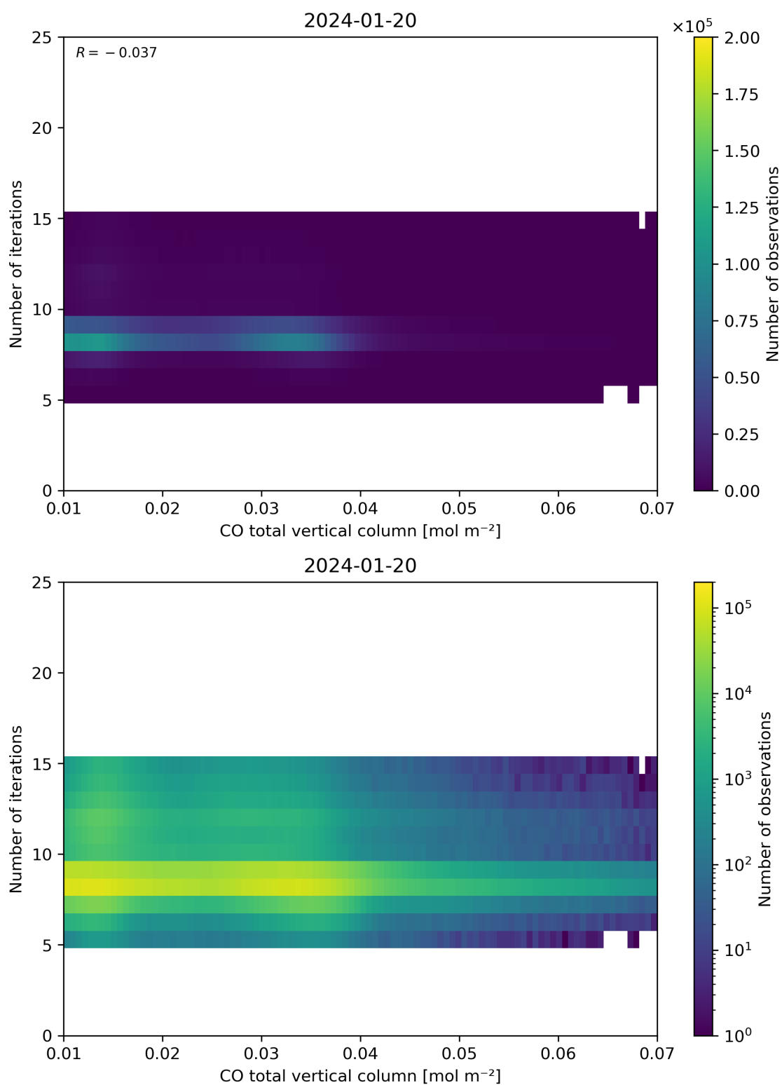
Figure 42: Scatter density plot of “CO total vertical column” against “Number of iterations” for 2024-01-19 to 2024-01-21.
