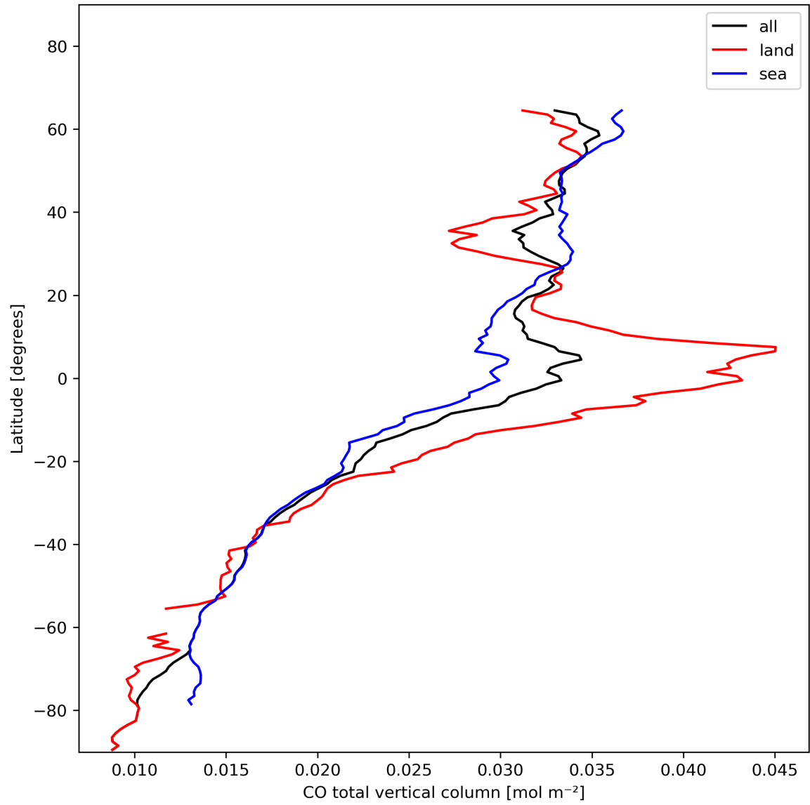
Figure 10: Zonal average of “CO total vertical column” for 2024-01-19 to 2024-01-21.
