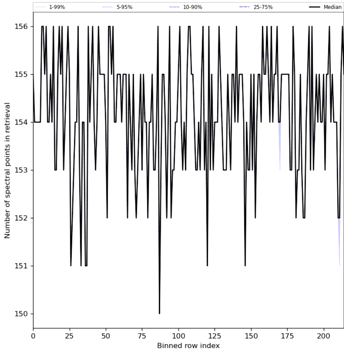
Figure 29: Along track statistics of “Number of spectral points in retrieval” for 2024-01-19 to 2024-01-21
