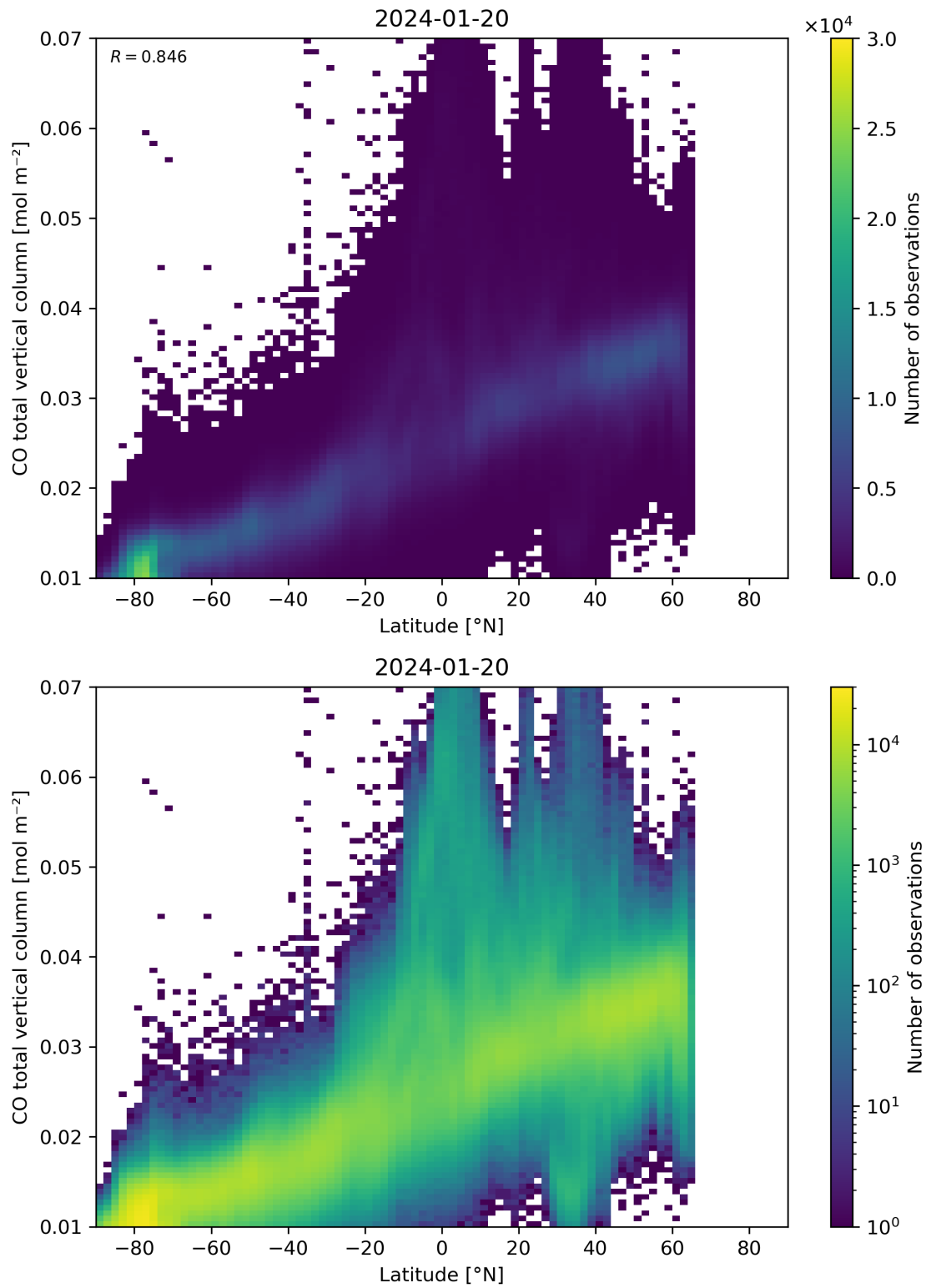
Figure 51: Scatter density plot of “Latitude” against “CO total vertical column” for 2024-01-19 to 2024-01-21.
