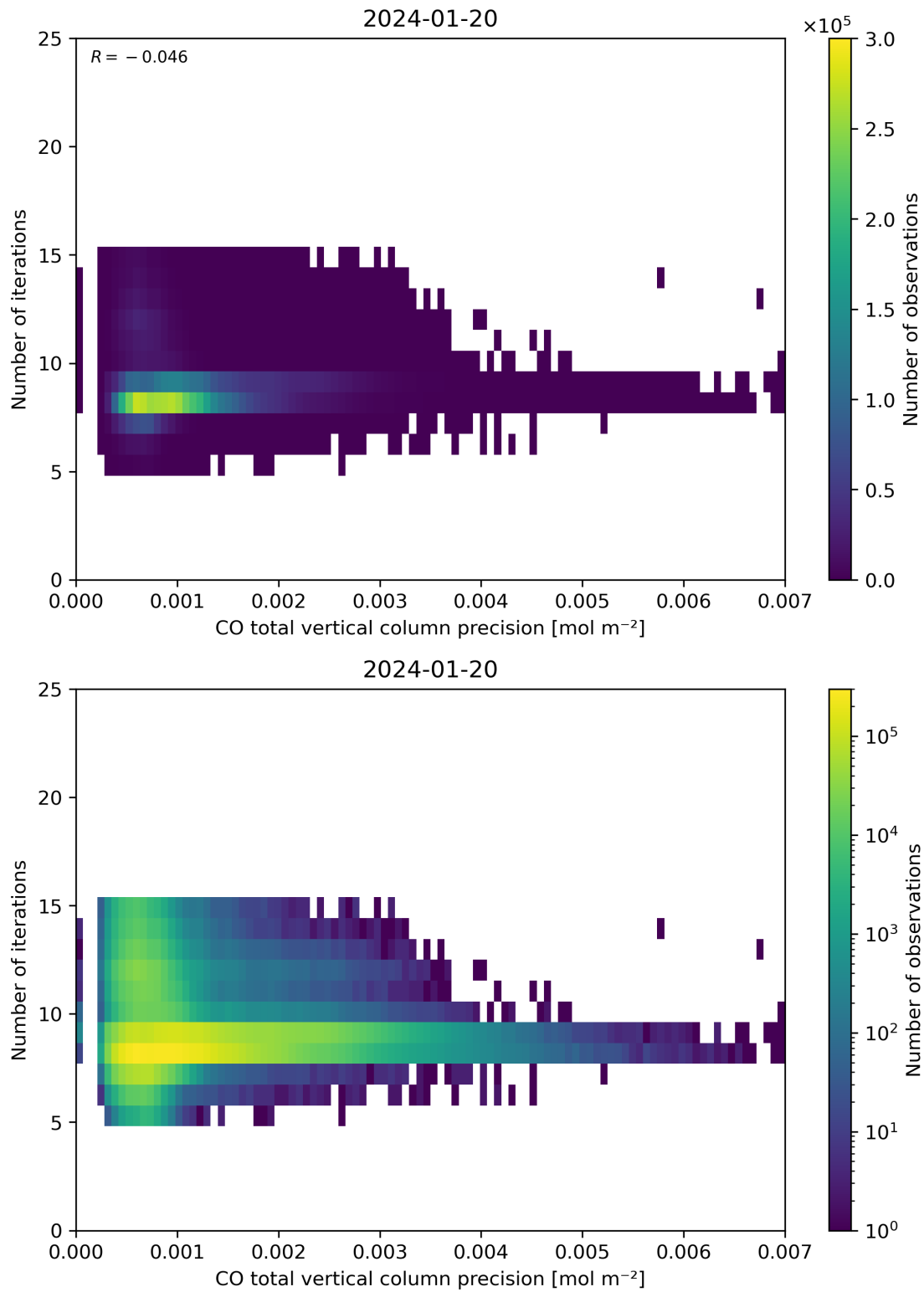
Figure 46: Scatter density plot of “CO total vertical column precision” against “Number of iterations” for 2024-01-19 to 2024-01-21.
