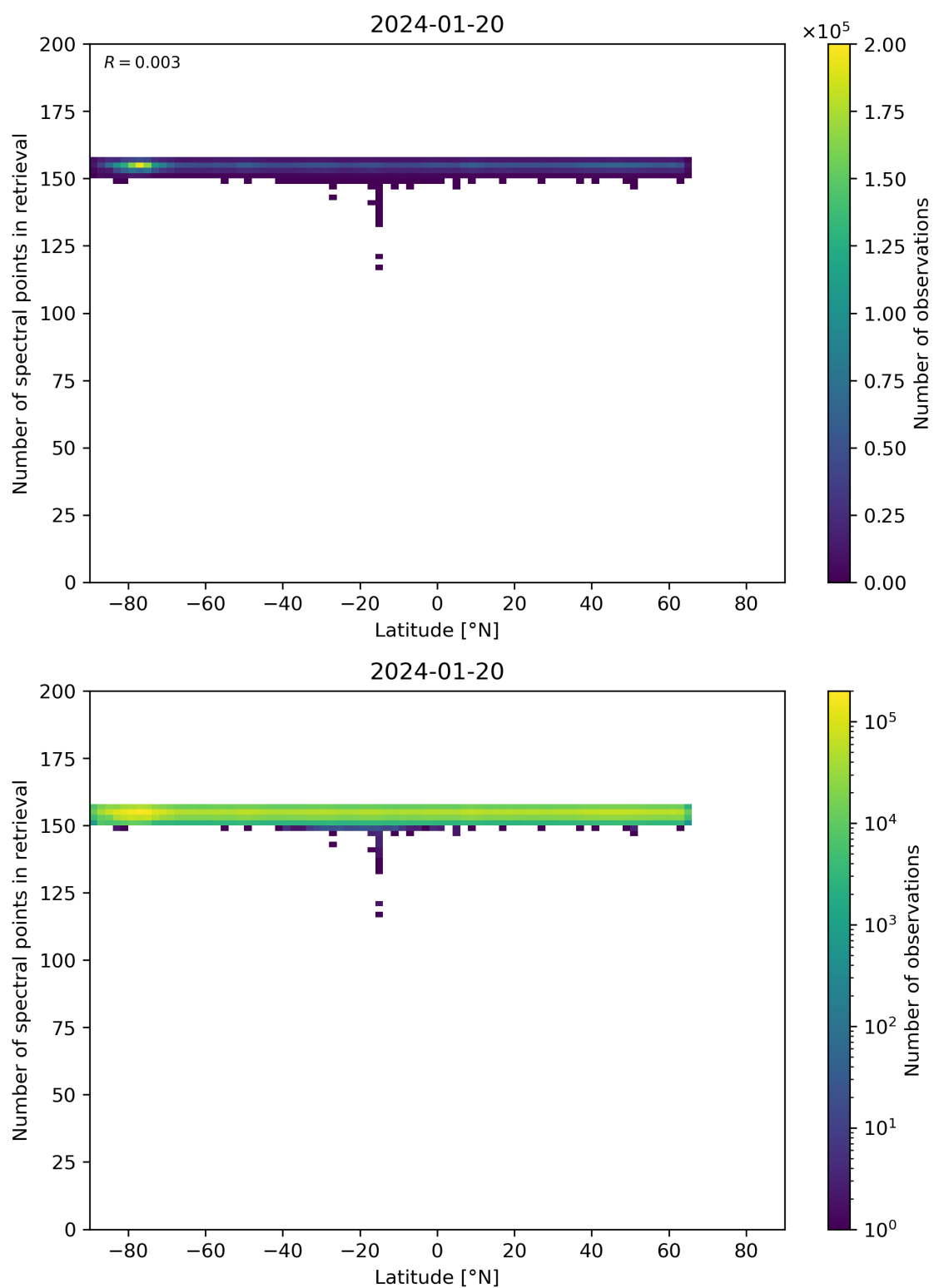
Figure 57: Scatter density plot of “Latitude” against “Number of spectral points in retrieval” for 2024-01-19 to 2024-01-21.
