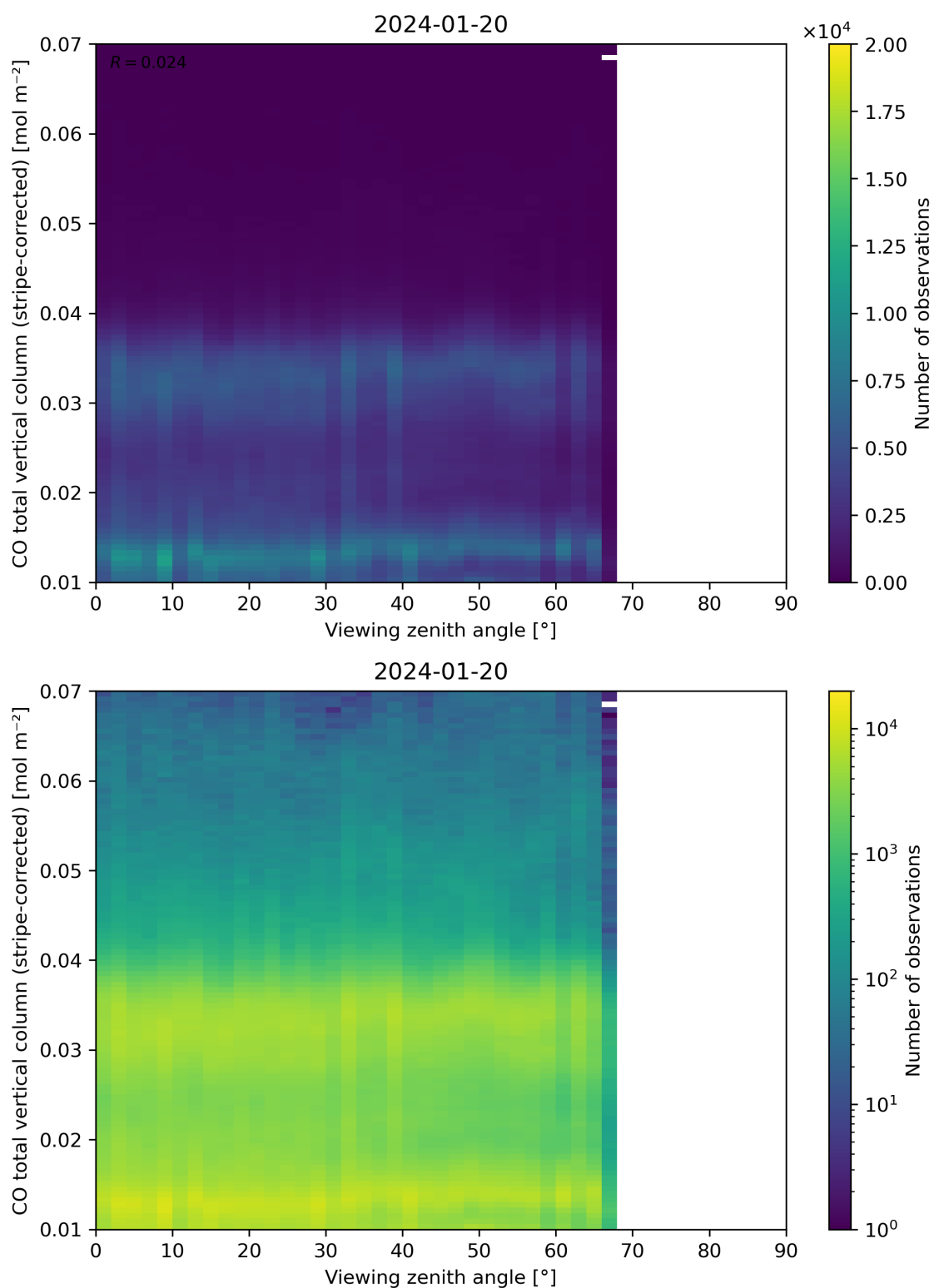
Figure 70: Scatter density plot of “Viewing zenith angle” against “CO total vertical column (stripe-corrected)” for 2024-01-19 to 2024-01-21.
