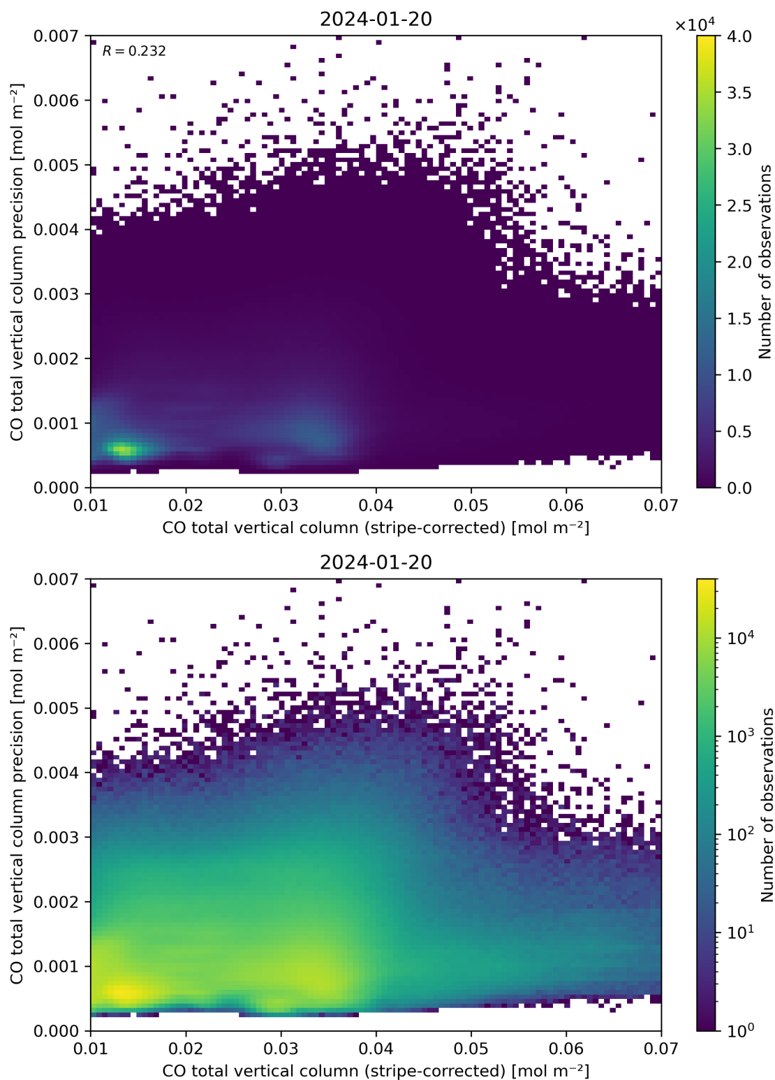
Figure 36: Scatter density plot of “CO total vertical column (stripe-corrected)” against “CO total vertical column precision” for 2024-01-19 to 2024-01-21.
