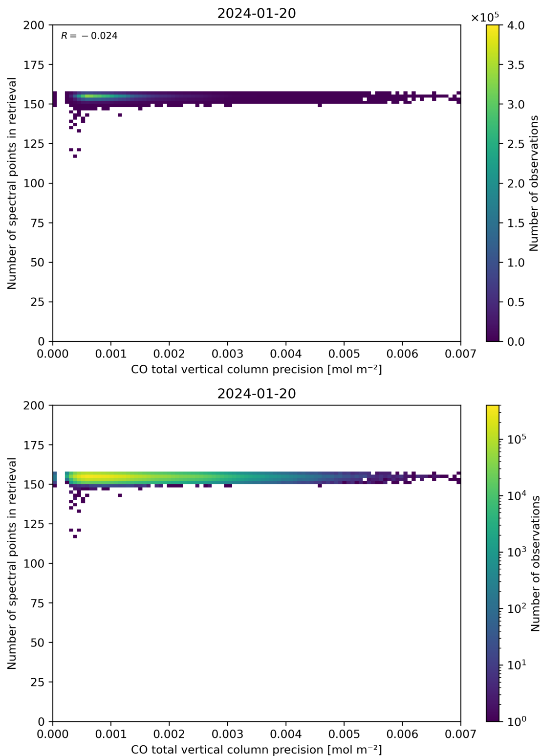
Figure 47: Scatter density plot of “CO total vertical column precision” against “Number of spectral points in retrieval” for 2024-01-19 to 2024-01-21.
