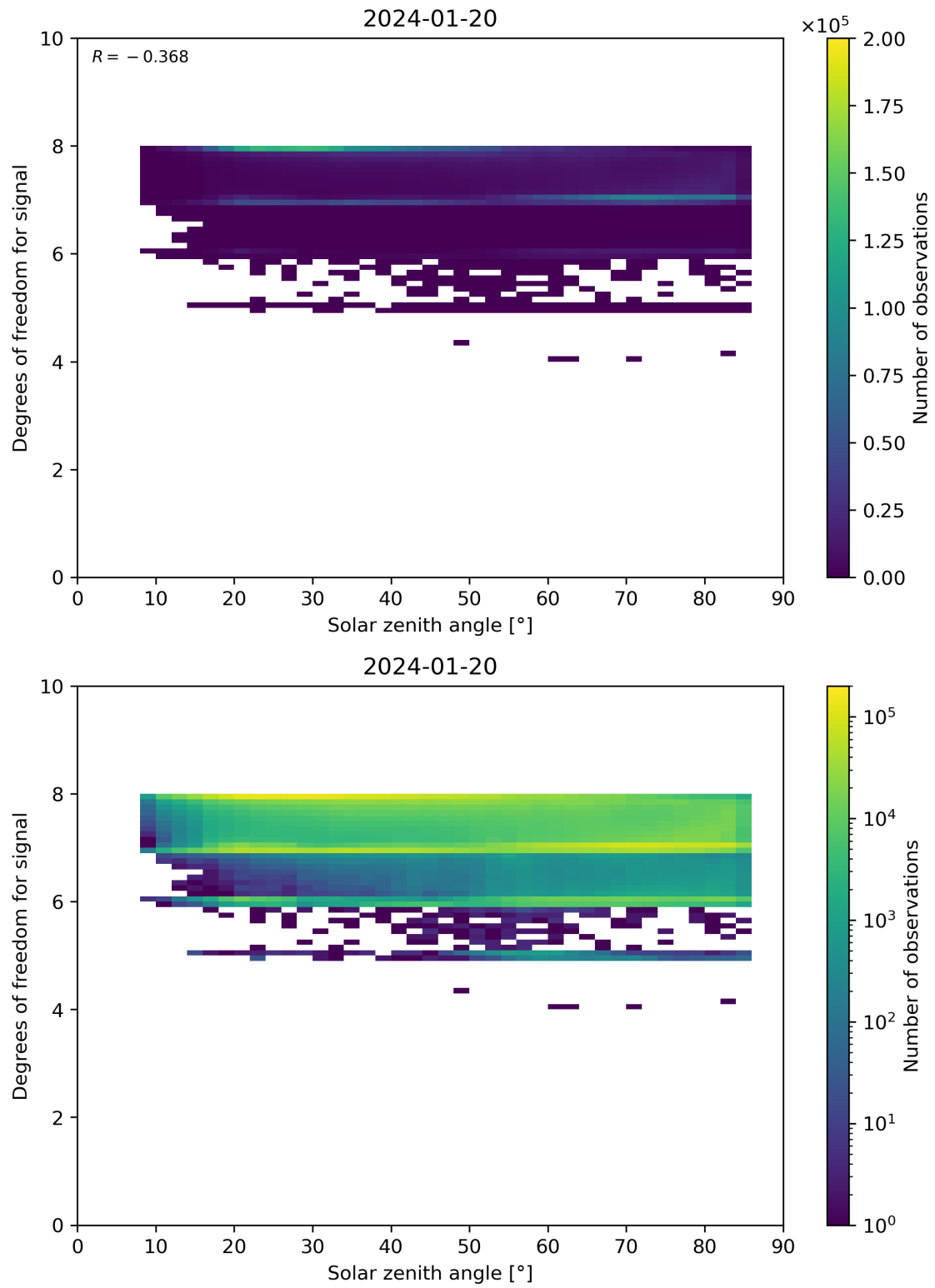
Figure 65: Scatter density plot of “Solar zenith angle” against “Degrees of freedom for signal” for 2024-01-19 to 2024-01-21.
