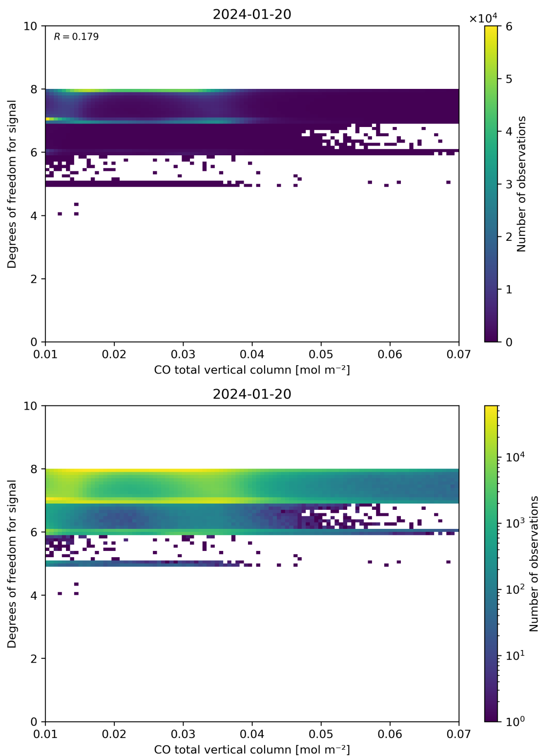
Figure 41: Scatter density plot of “CO total vertical column” against “Degrees of freedom for signal” for 2024-01-19 to 2024-01-21.
