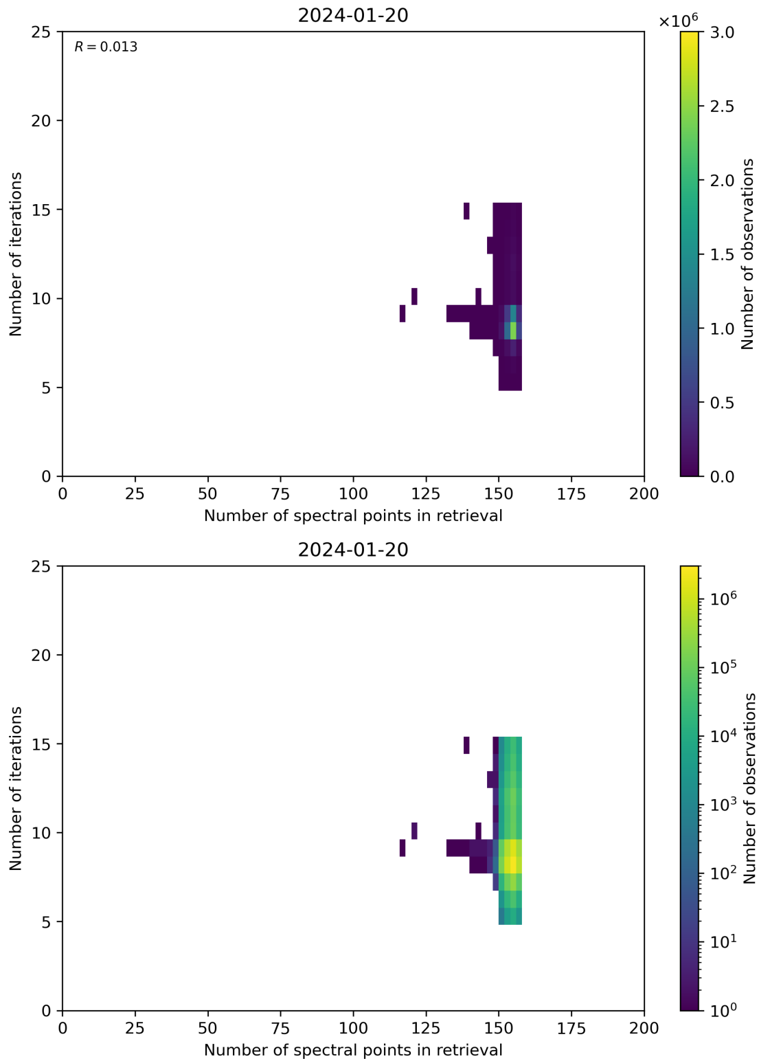
Figure 60: Scatter density plot of “Number of spectral points in retrieval” against “Number of iterations” for 2024-01-19 to 2024-01-21.
