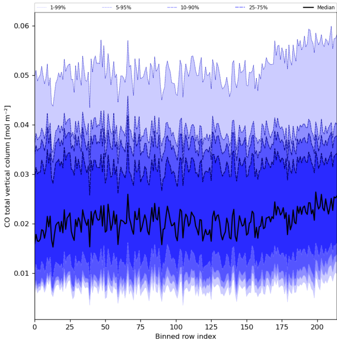
Figure 26: Along track statistics of “CO total vertical column” for 2024-01-19 to 2024-01-21
