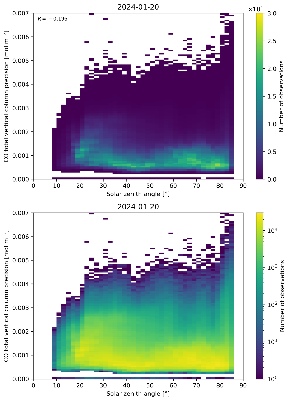
Figure 63: Scatter density plot of “Solar zenith angle” against “CO total vertical column precision” for 2024-01-19 to 2024-01-21.
