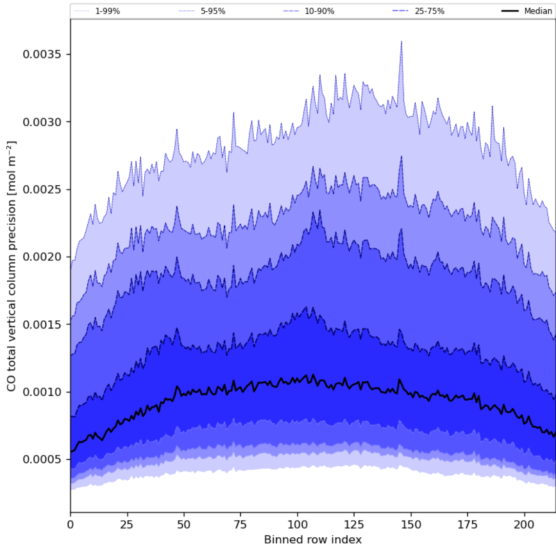
Figure 28: Along track statistics of “CO total vertical column precision” for 2024-01-19 to 2024-01-21
