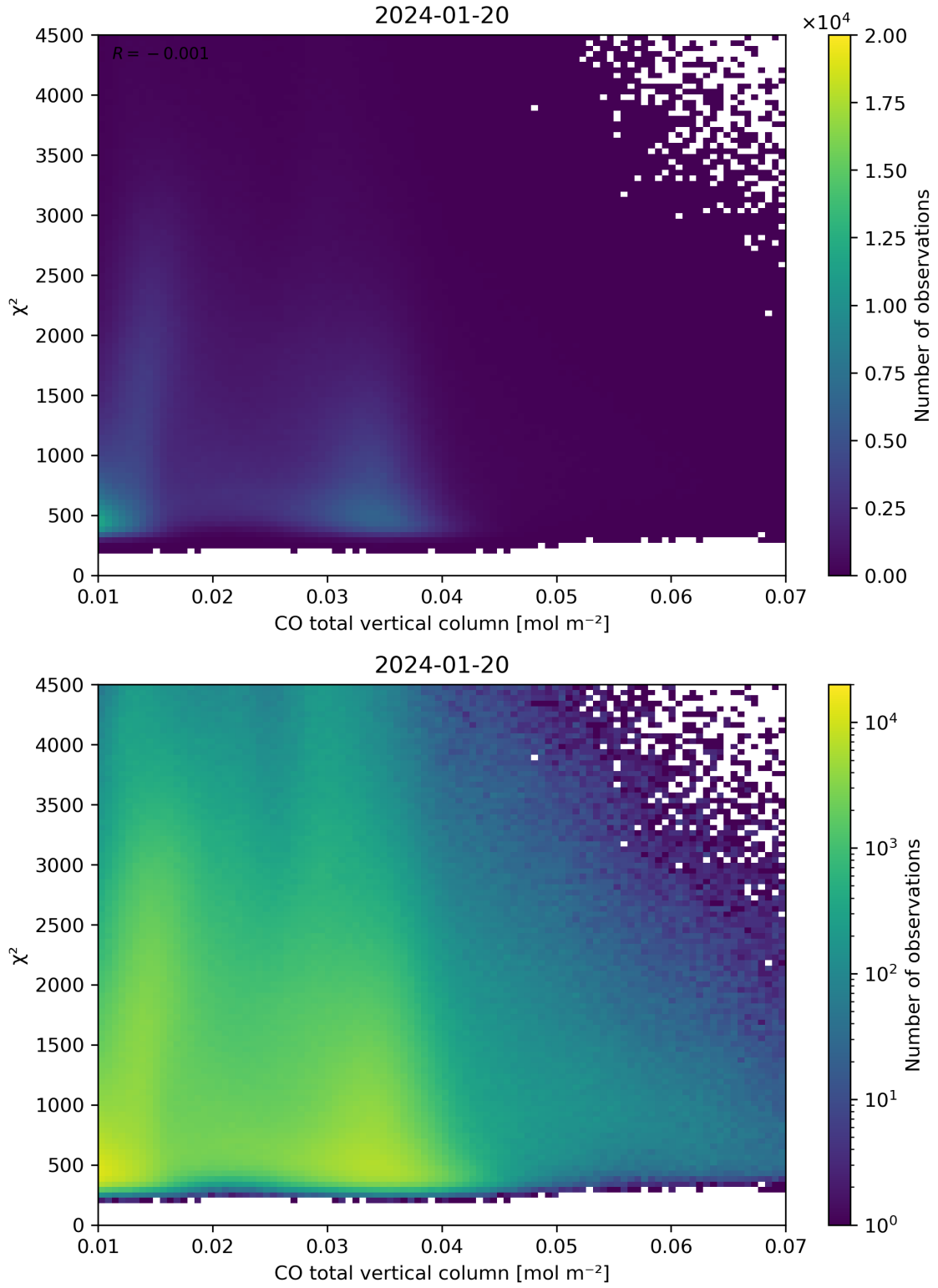
Figure 35: Scatter density plot of “CO total vertical column” against “ \chi^2 ” for 2024-01-19 to 2024-01-21.
