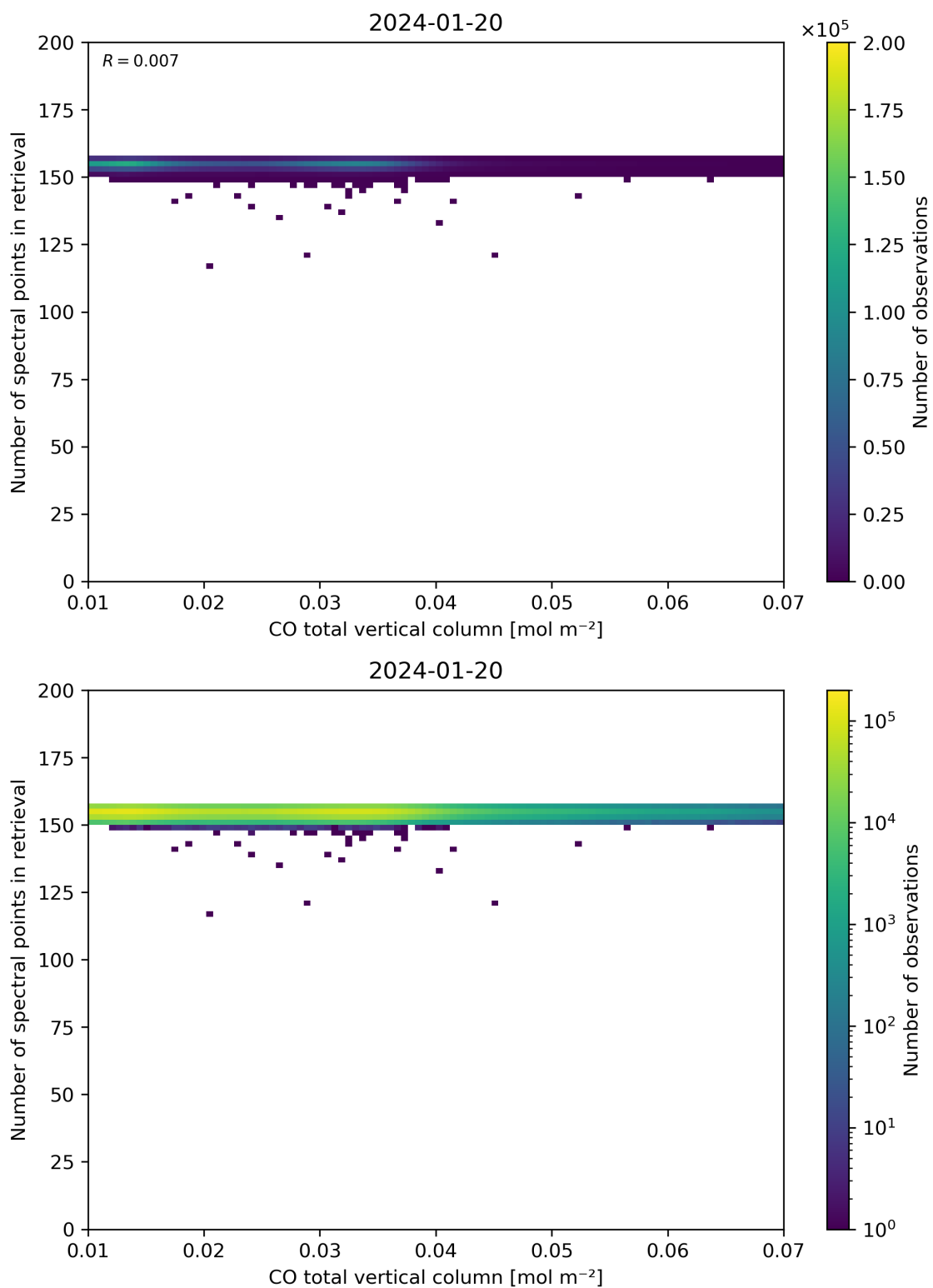
Figure 43: Scatter density plot of “CO total vertical column” against “Number of spectral points in retrieval” for 2024-01-19 to 2024-01-21.
