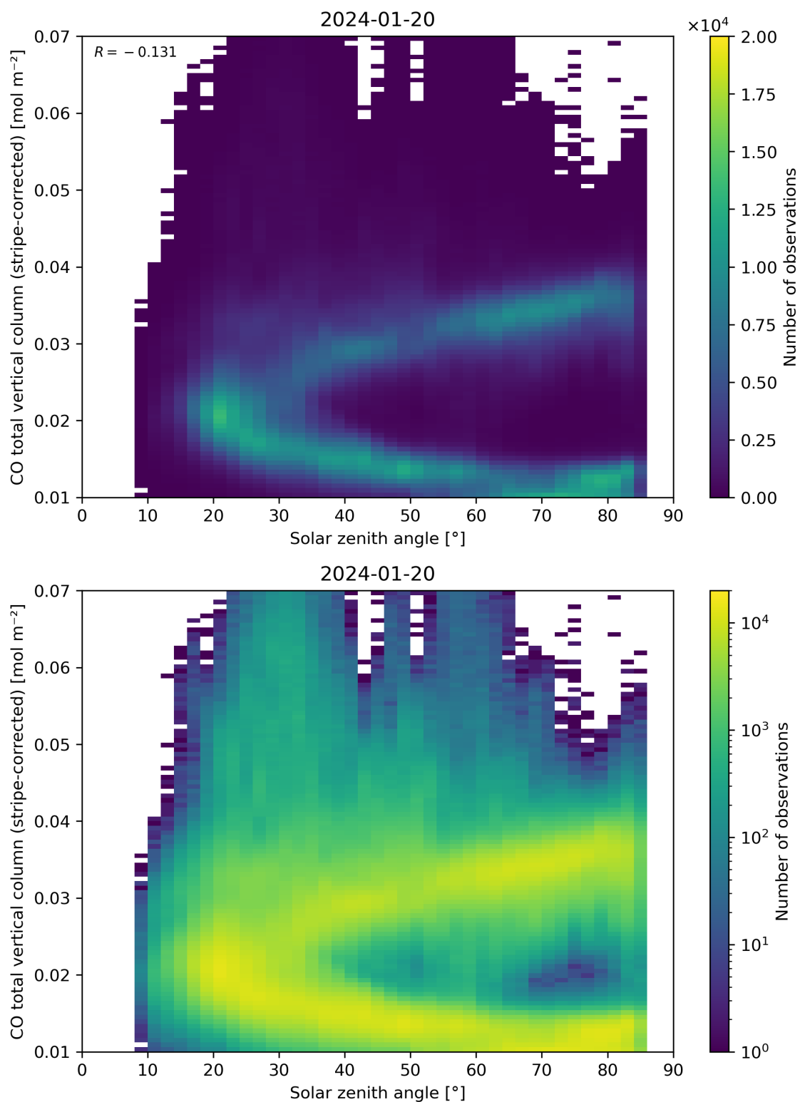
Figure 62: Scatter density plot of “Solar zenith angle” against “CO total vertical column (stripe-corrected)” for 2024-01-19 to 2024-01-21.
