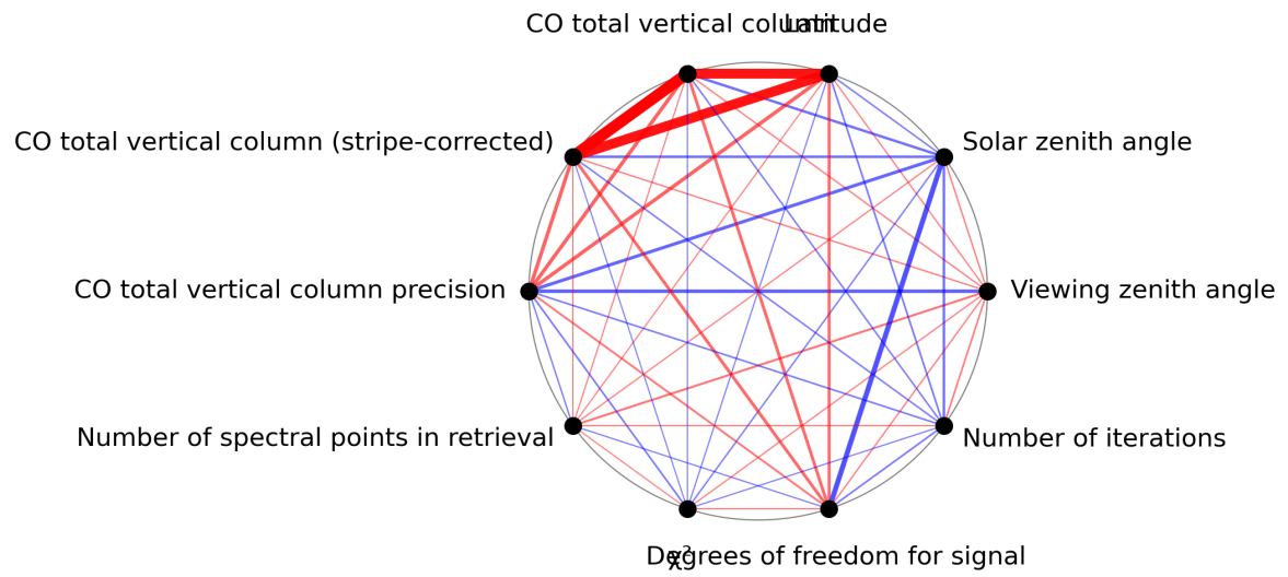
Figure 1: Map of correlation graph for 2024-01-19 to 2024-01-21.
