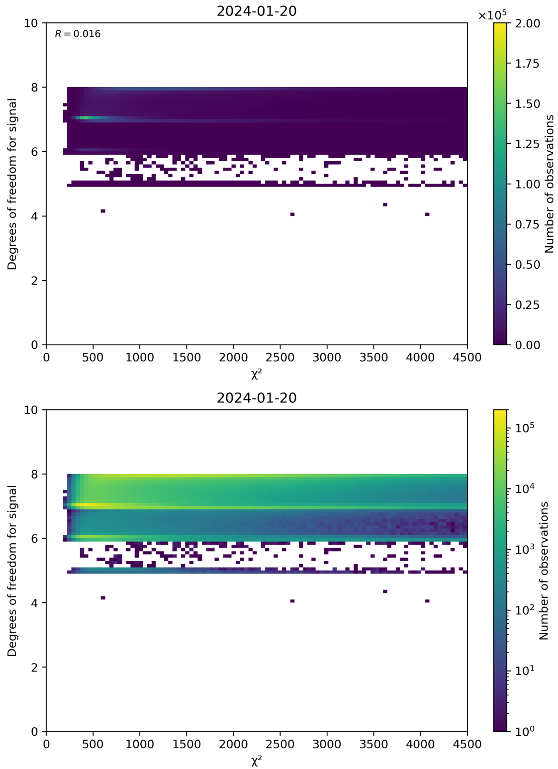
Figure 48: Scatter density plot of “ \chi^2 ” against “Degrees of freedom for signal” for 2024-01-19 to 2024-01-21.
