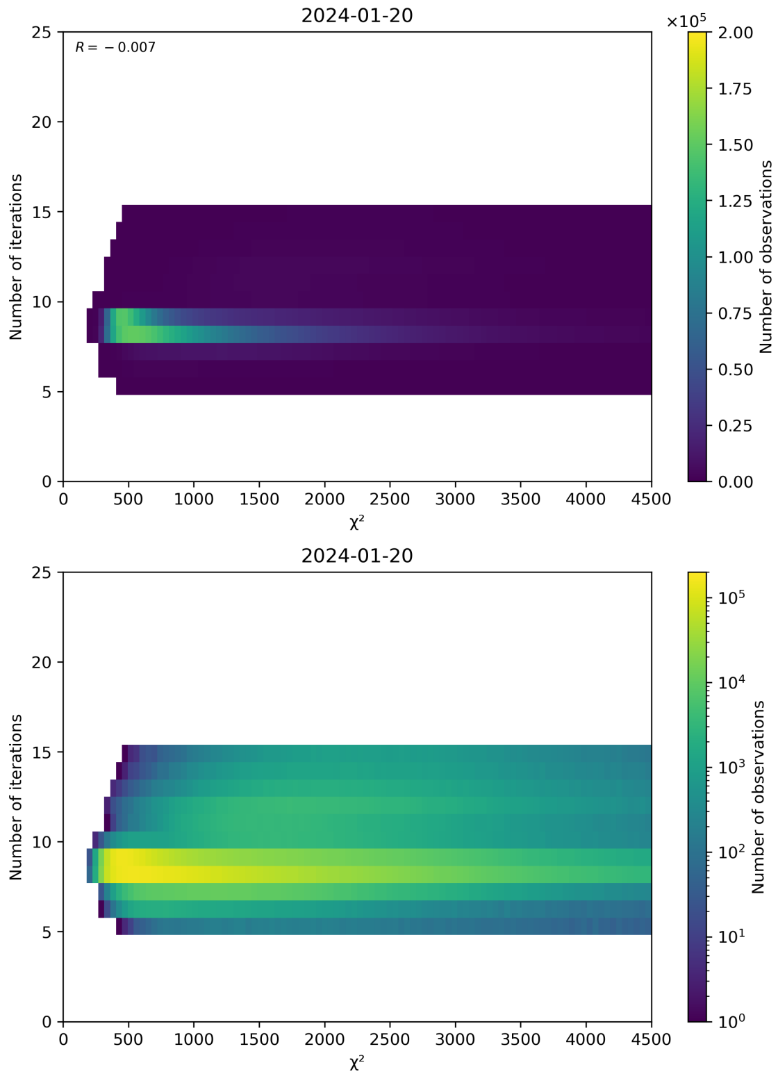
Figure 49: Scatter density plot of “ \chi^2 ” against “Number of iterations” for 2024-01-19 to 2024-01-21.
