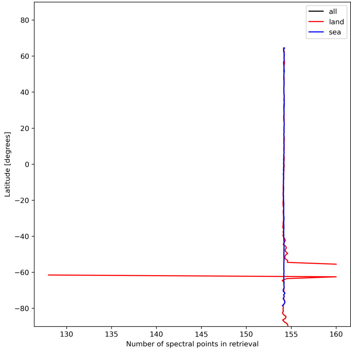
Figure 13: Zonal average of “Number of spectral points in retrieval” for 2024-01-19 to 2024-01-21.
