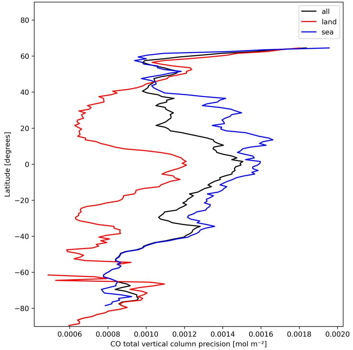
Figure 12: Zonal average of “CO total vertical column precision” for 2024-01-19 to 2024-01-21.
