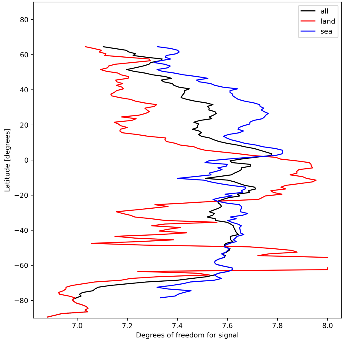
Figure 15: Zonal average of “Degrees of freedom for signal” for 2024-01-19 to 2024-01-21.
