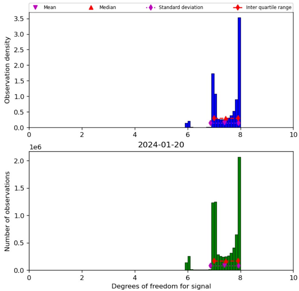
Figure 23: Histogram of “Degrees of freedom for signal” for 2024-01-19 to 2024-01-21
