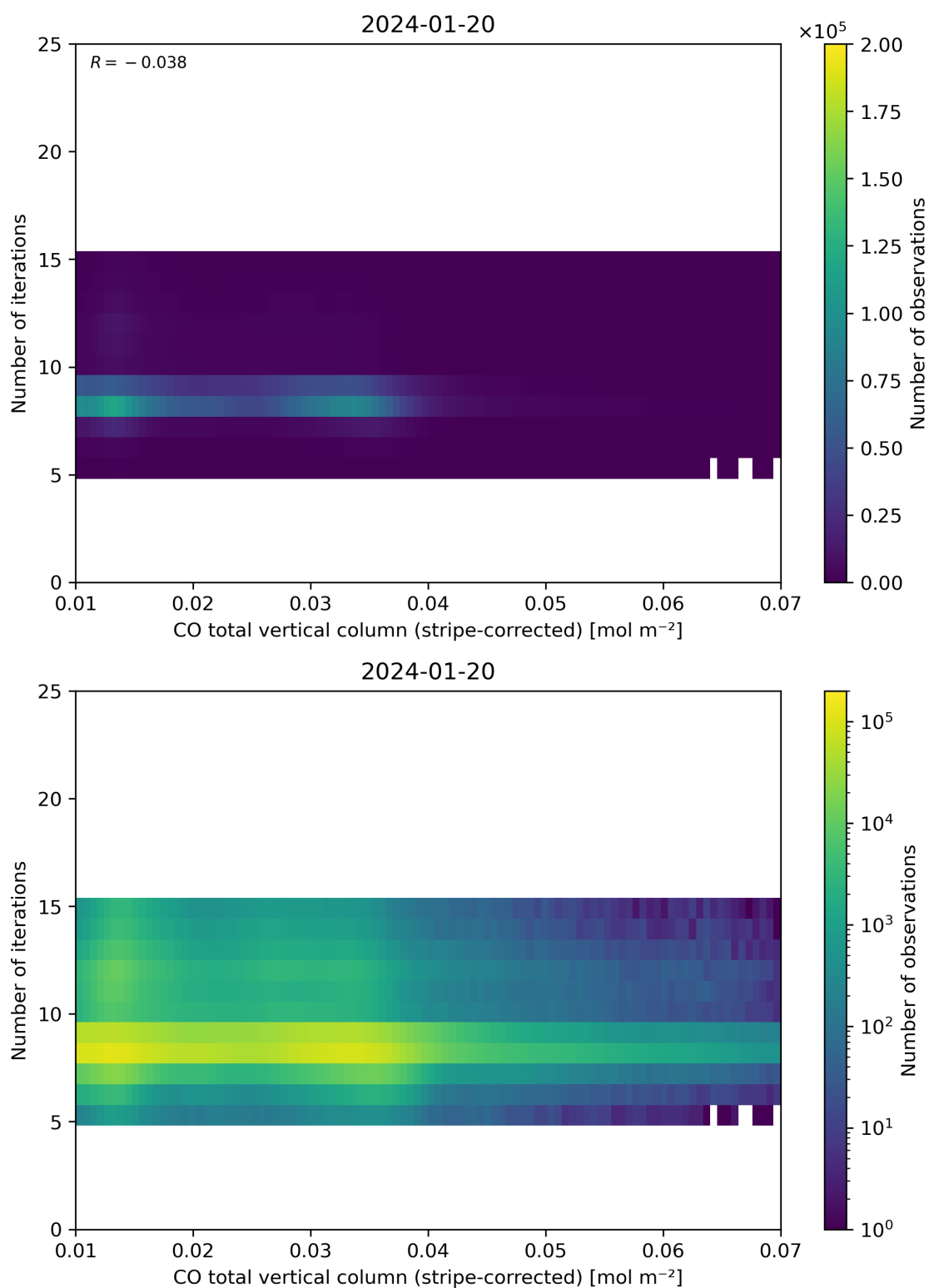
Figure 39: Scatter density plot of “CO total vertical column (stripe-corrected)” against “Number of iterations” for 2024-01-19 to 2024-01-21.
