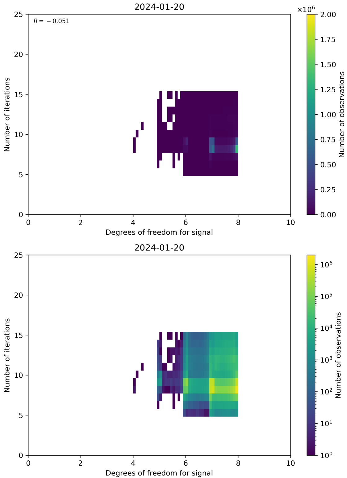
Figure 50: Scatter density plot of “Degrees of freedom for signal” against “Number of iterations” for 2024-01-19 to 2024-01-21.
