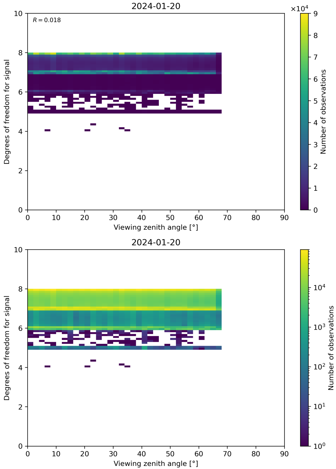
Figure 73: Scatter density plot of “Viewing zenith angle” against “Degrees of freedom for signal” for 2024-01-19 to 2024-01-21.
