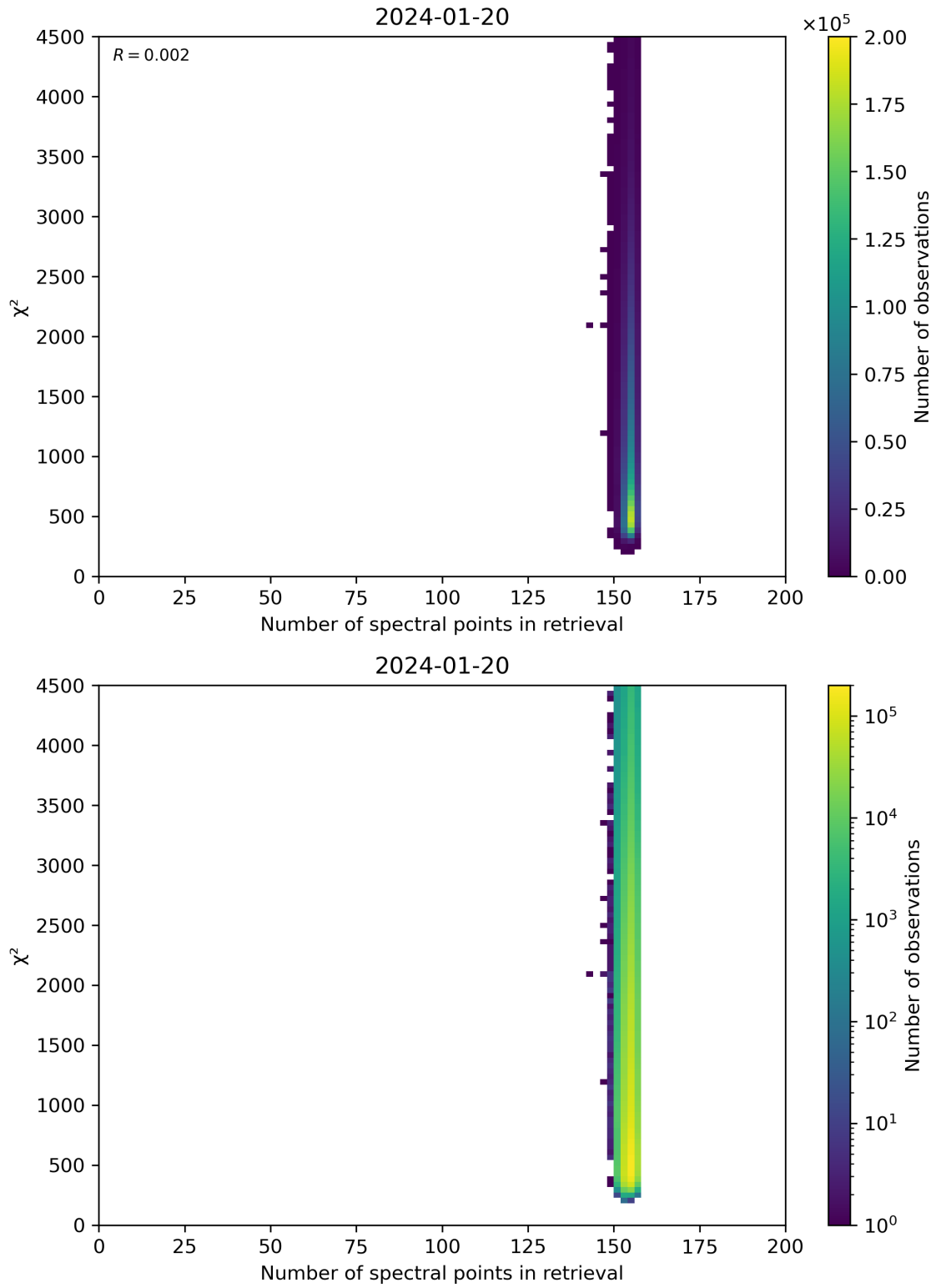
Figure 58: Scatter density plot of “Number of spectral points in retrieval” against “ \chi^2 ” for 2024-01-19 to 2024-01-21.
