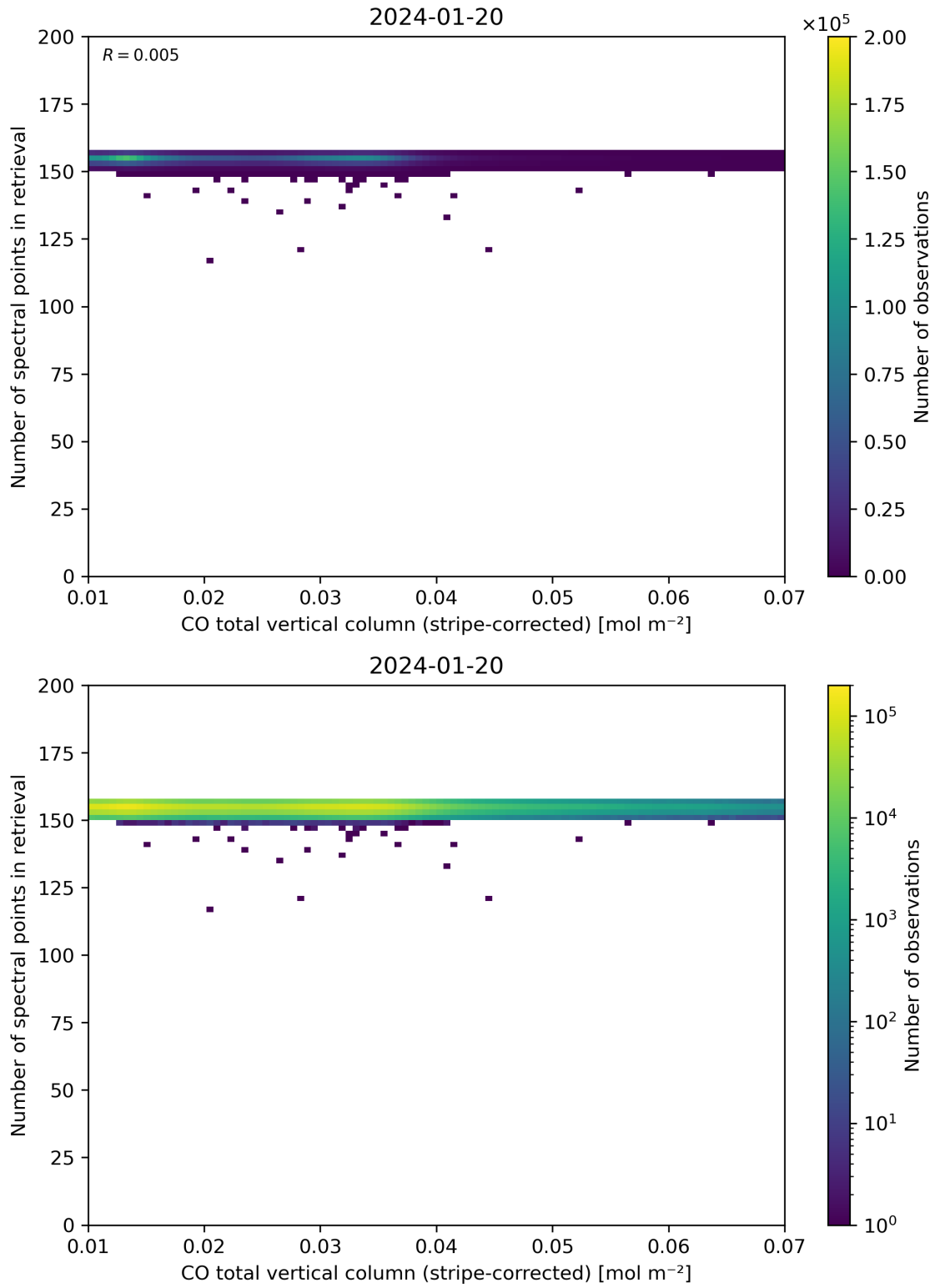
Figure 40: Scatter density plot of “CO total vertical column (stripe-corrected)” against “Number of spectral points in retrieval” for 2024-01-19 to 2024-01-21.
