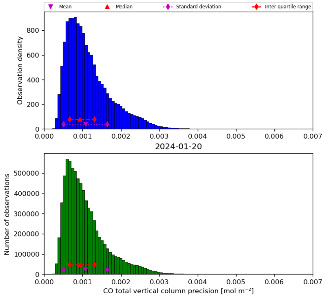
Figure 20: Histogram of “CO total vertical column precision” for 2024-01-19 to 2024-01-21
