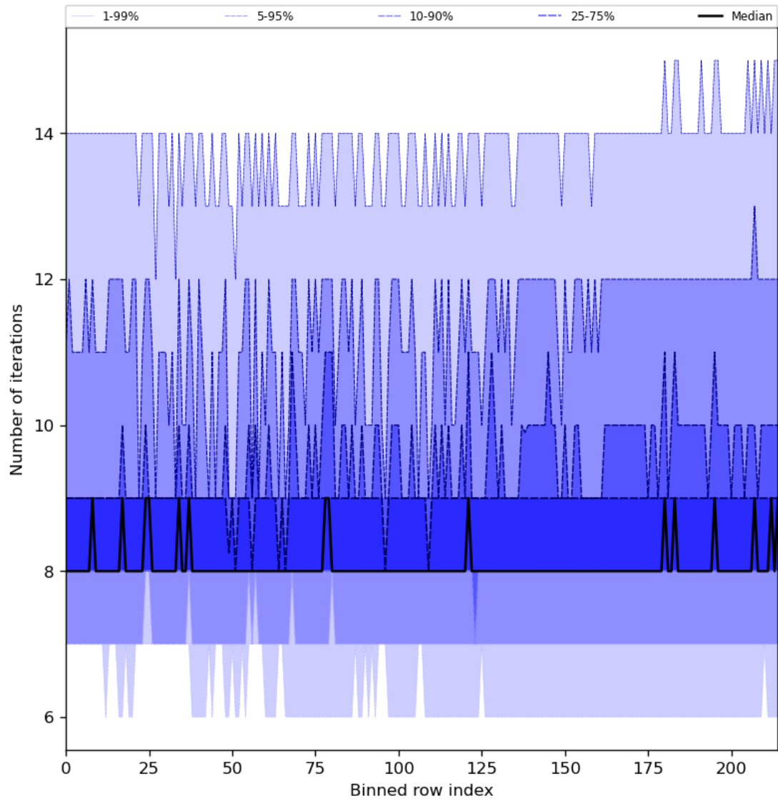
Figure 32: Along track statistics of “Number of iterations” for 2024-01-19 to 2024-01-21
