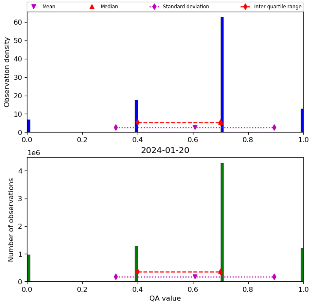
Figure 17: Histogram of “QA value” for 2024-01-19 to 2024-01-21
