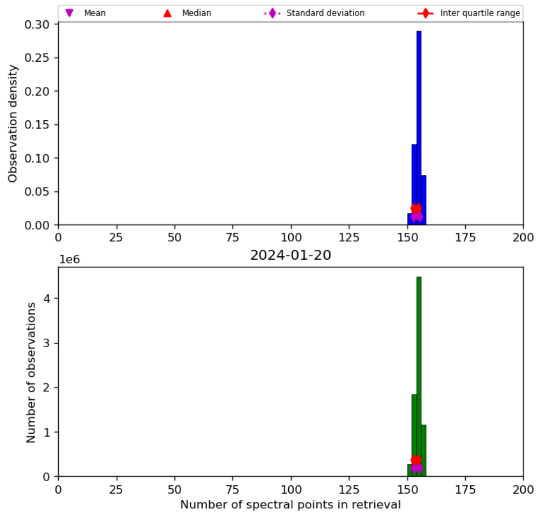
Figure 21: Histogram of “Number of spectral points in retrieval” for 2024-01-19 to 2024-01-21
