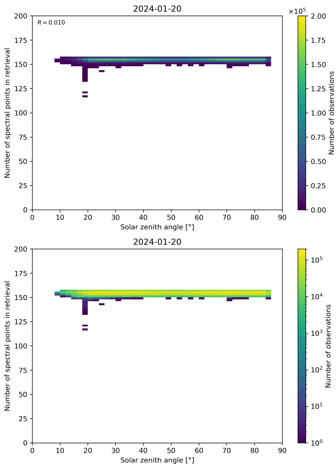
Figure 68: Scatter density plot of “Solar zenith angle” against “Number of spectral points in retrieval” for 2024-01-19 to 2024-01-21.
