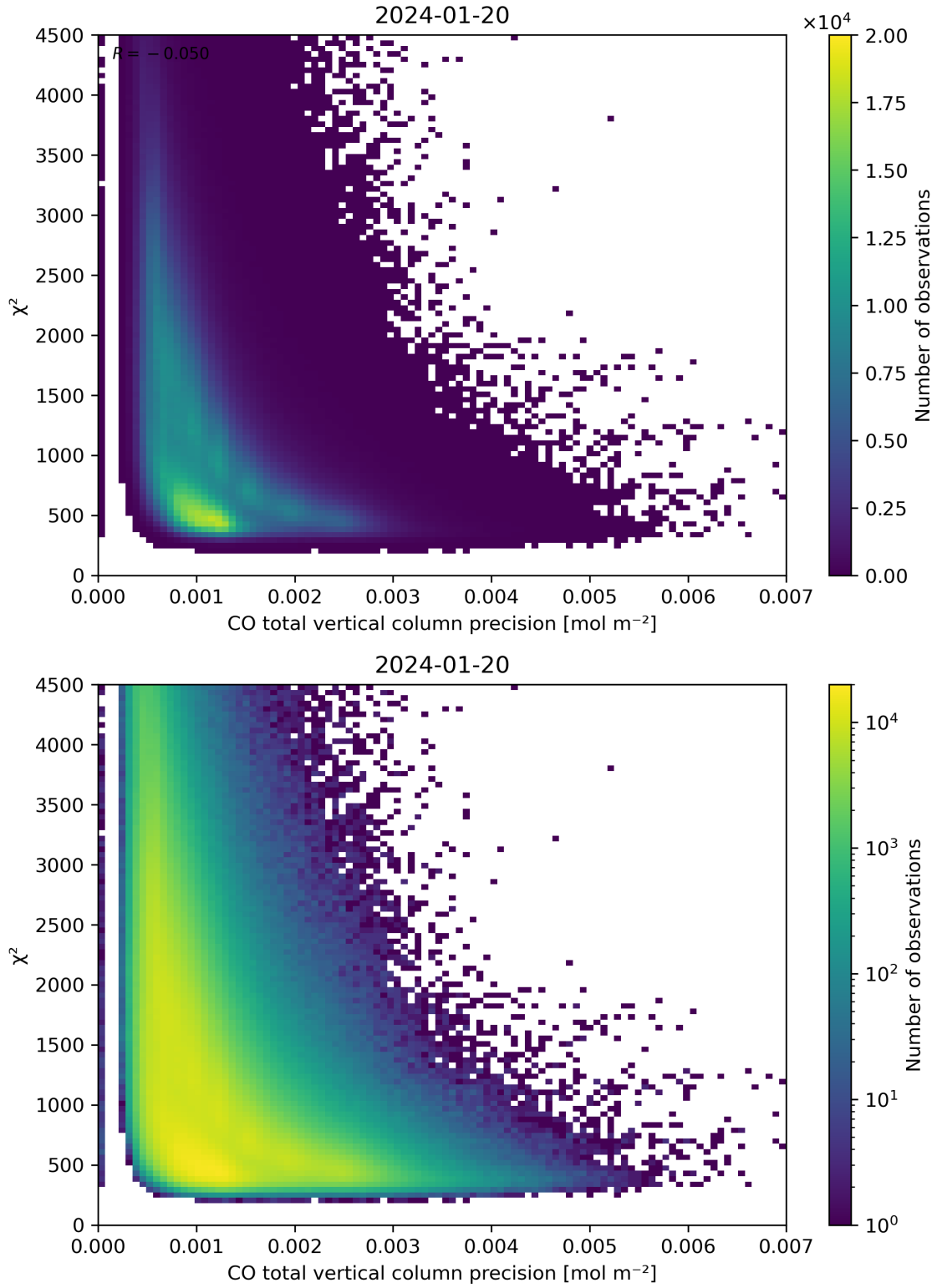
Figure 44: Scatter density plot of “CO total vertical column precision” against “ \chi^2 ” for 2024-01-19 to 2024-01-21.
