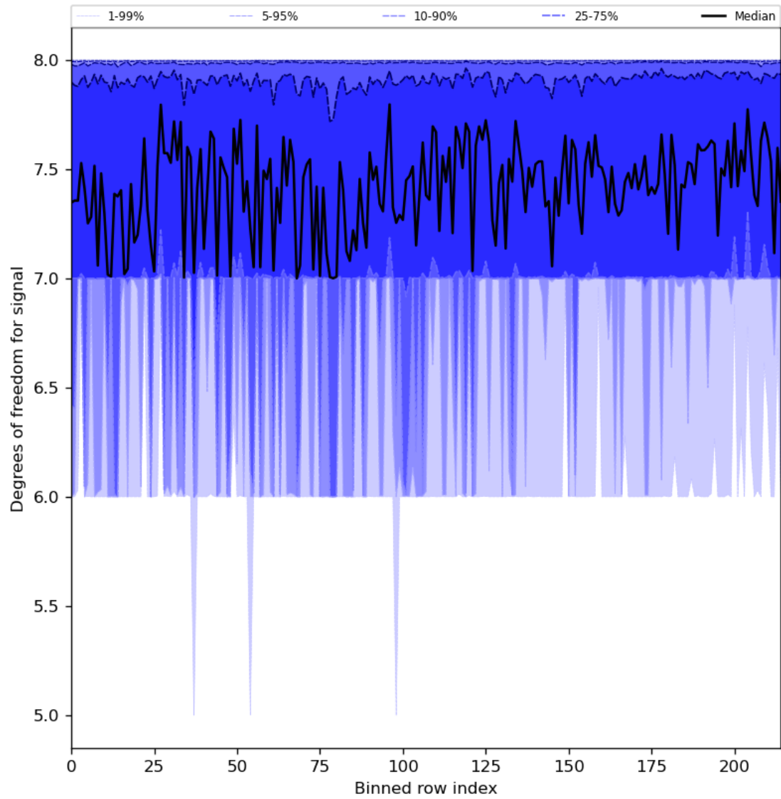
Figure 31: Along track statistics of “Degrees of freedom for signal” for 2024-01-19 to 2024-01-21
