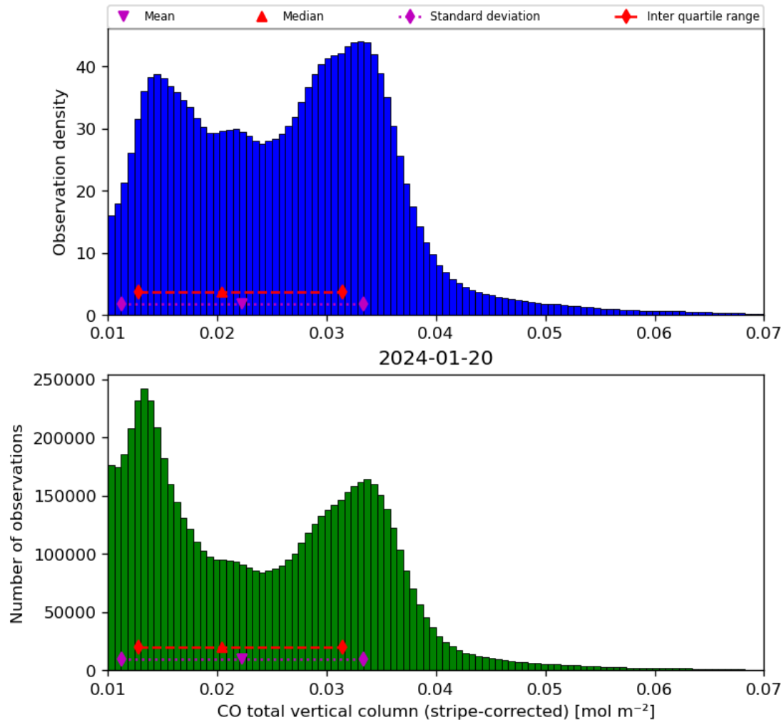
Figure 19: Histogram of “CO total vertical column (stripe-corrected)” for 2024-01-19 to 2024-01-21
