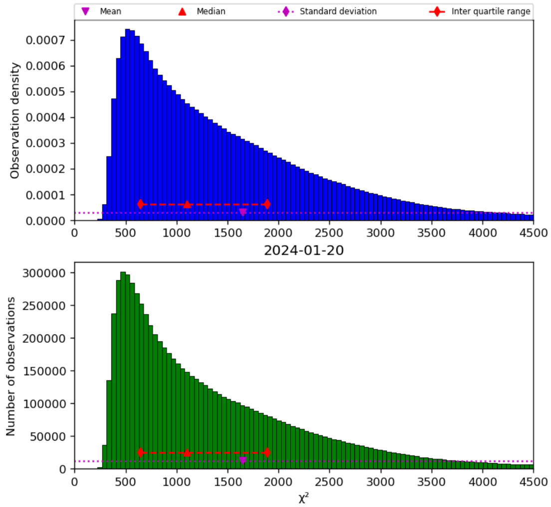
Figure 22: Histogram of “ \chi^2 ” for 2024-01-19 to 2024-01-21
