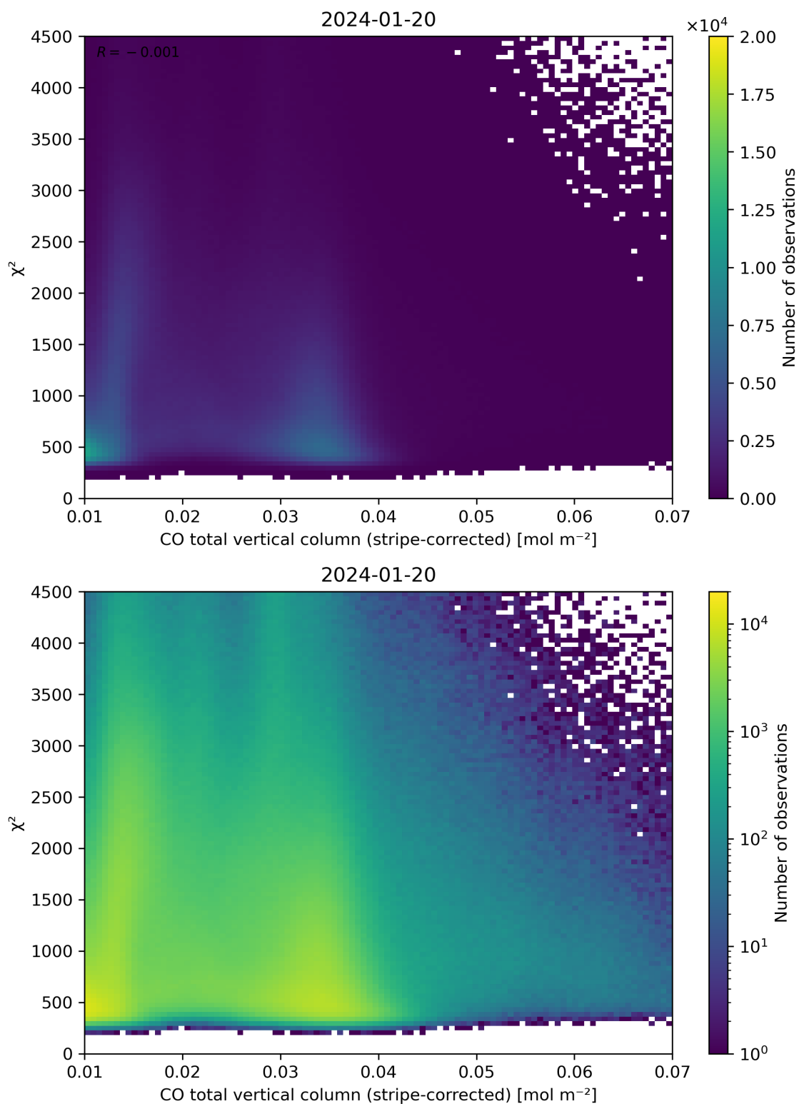
Figure 37: Scatter density plot of “CO total vertical column (stripe-corrected)” against “ \chi^2 ” for 2024-01-19 to 2024-01-21.
