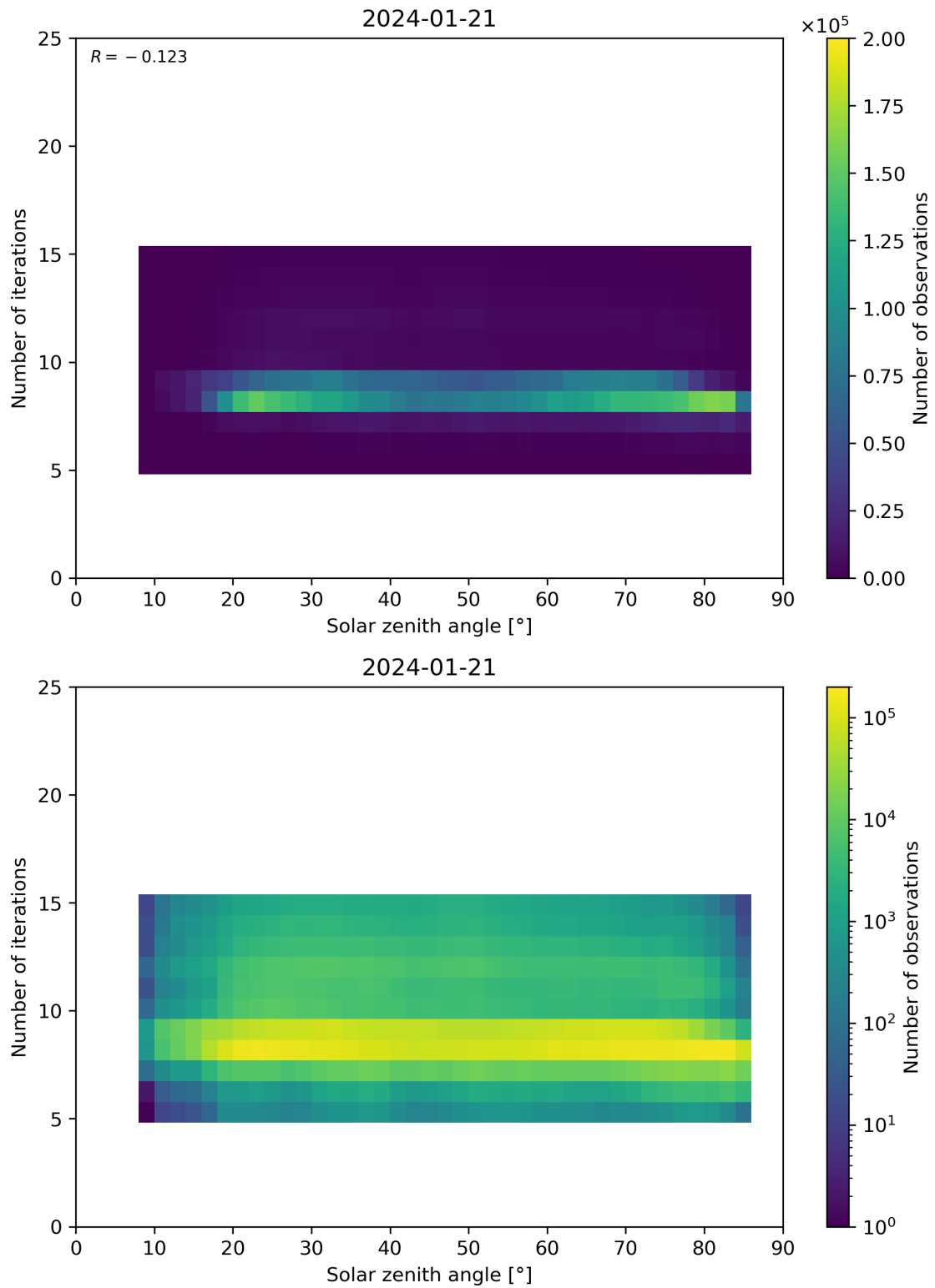
Figure 67: Scatter density plot of “Solar zenith angle” against “Number of iterations” for 2024-01-21 to 2024-01-22.
