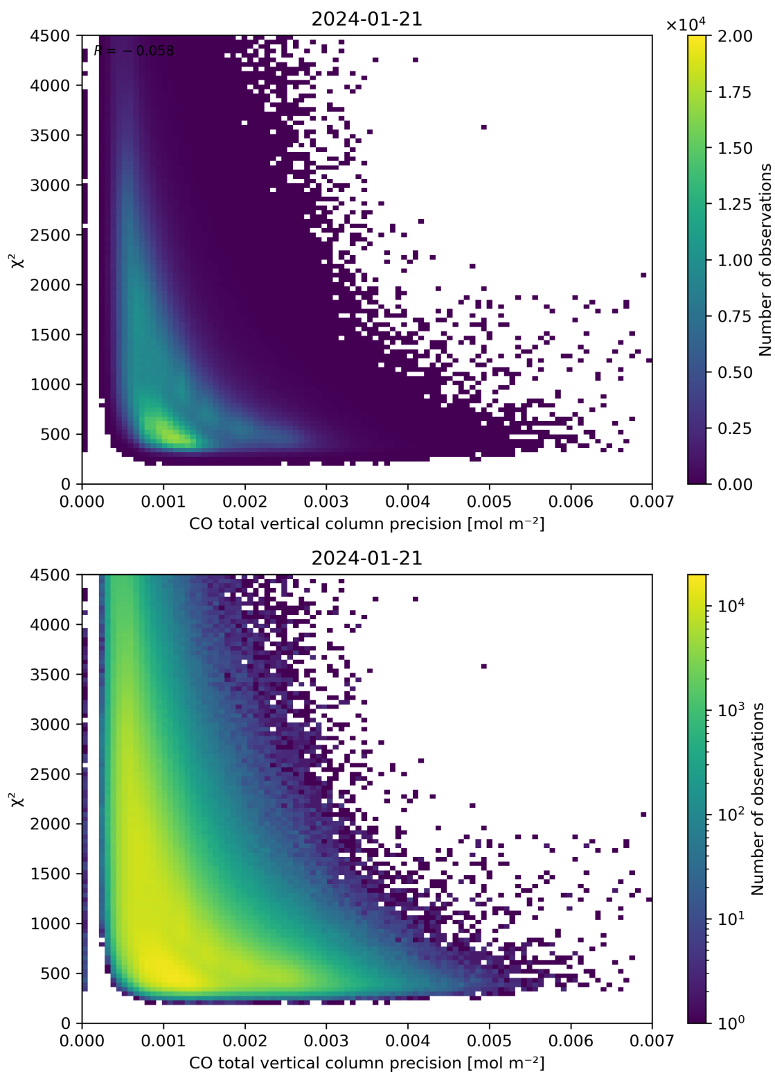
Figure 44: Scatter density plot of “CO total vertical column precision” against “ \chi^2 ” for 2024-01-21 to 2024-01-22.
