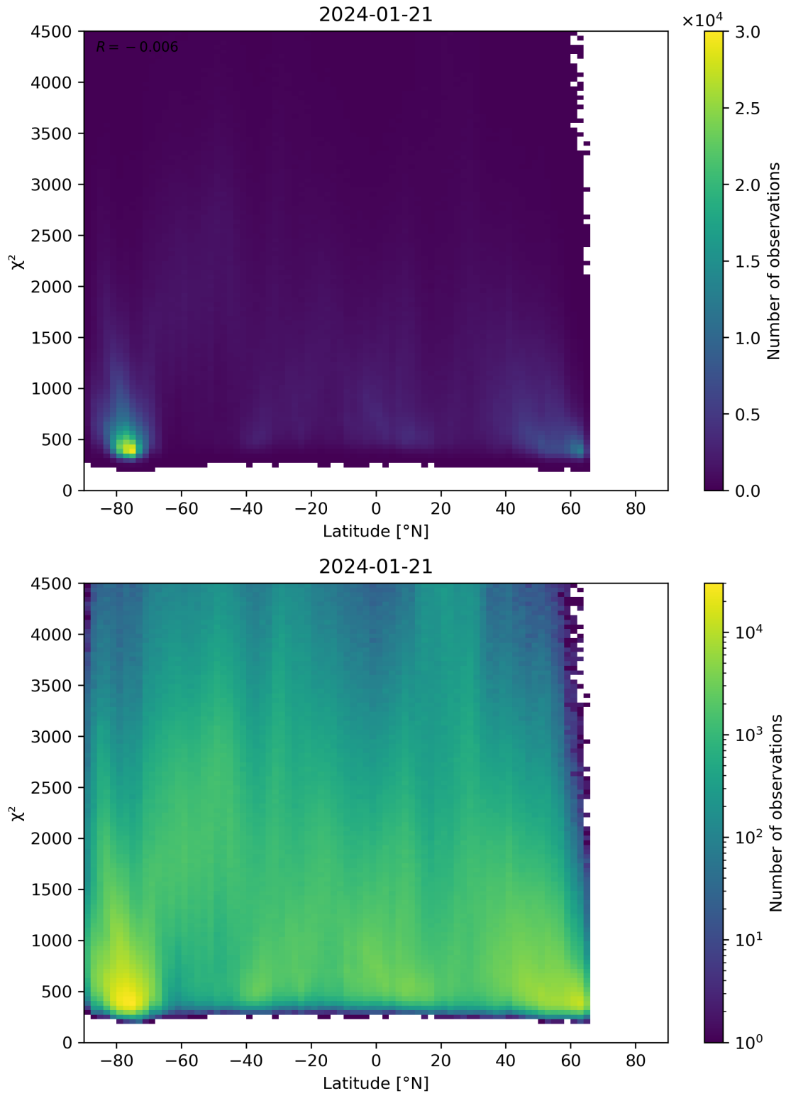
Figure 54: Scatter density plot of “Latitude” against “ \chi^2 ” for 2024-01-21 to 2024-01-22.
