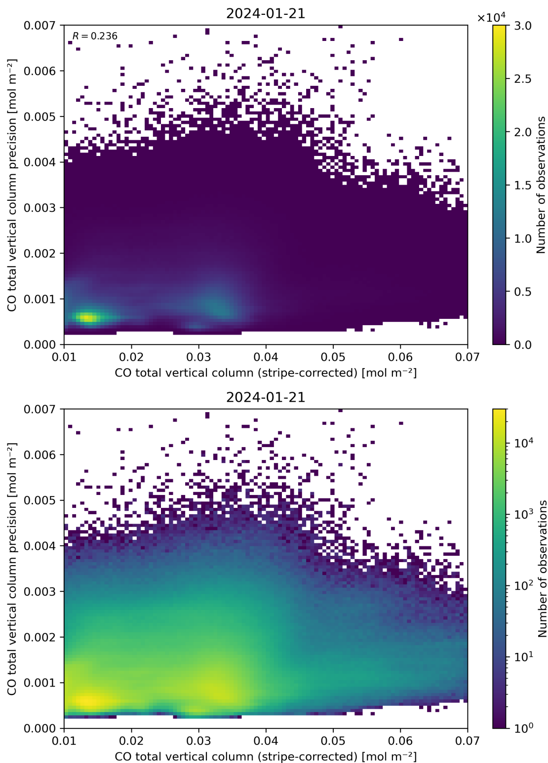
Figure 36: Scatter density plot of “CO total vertical column (stripe-corrected)” against “CO total vertical column precision” for 2024-01-21 to 2024-01-22.
