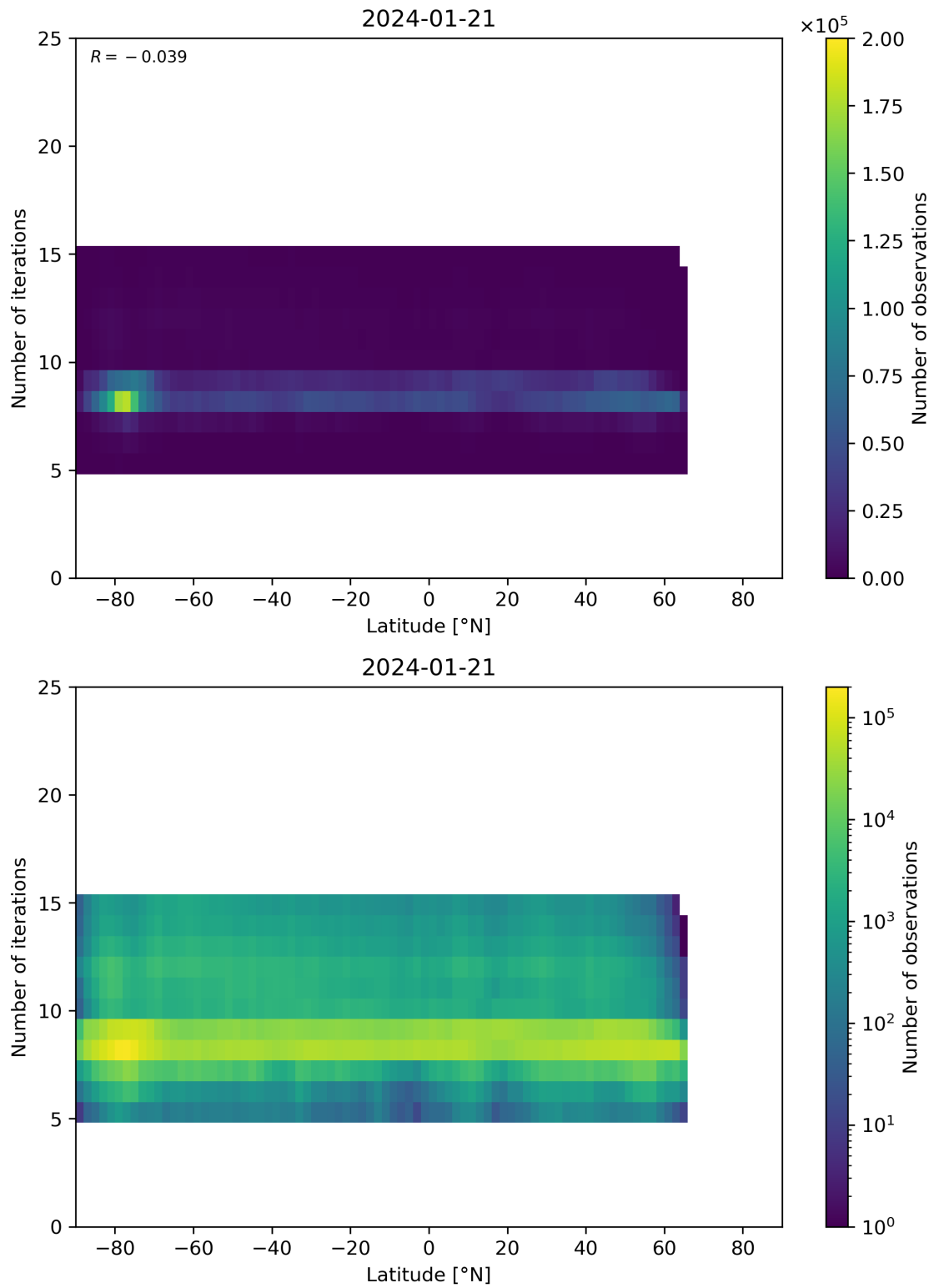
Figure 56: Scatter density plot of “Latitude” against “Number of iterations” for 2024-01-21 to 2024-01-22.
