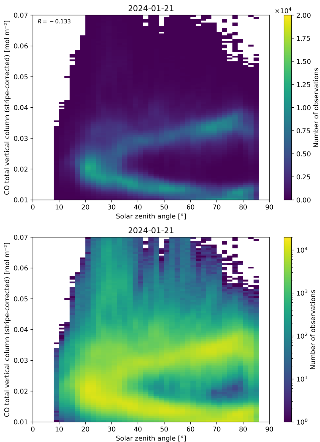
Figure 62: Scatter density plot of “Solar zenith angle” against “CO total vertical column (stripe-corrected)” for 2024-01-21 to 2024-01-22.
