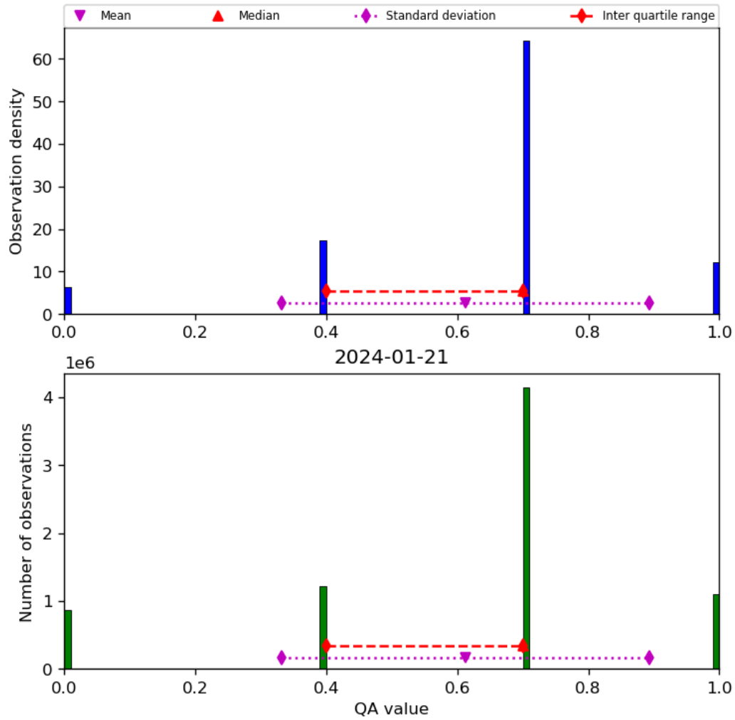
Figure 17: Histogram of “QA value” for 2024-01-21 to 2024-01-22
