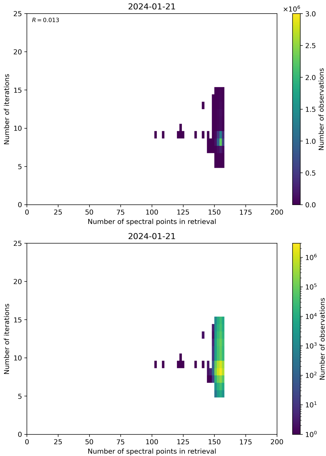
Figure 60: Scatter density plot of “Number of spectral points in retrieval” against “Number of iterations” for 2024-01-21 to 2024-01-22.
