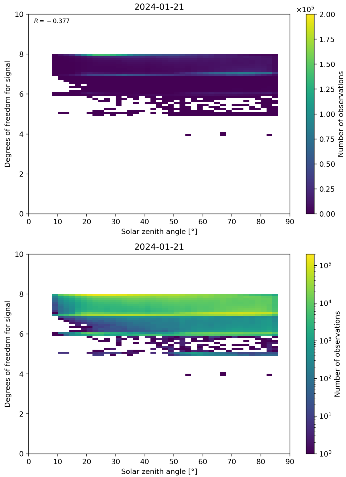
Figure 65: Scatter density plot of “Solar zenith angle” against “Degrees of freedom for signal” for 2024-01-21 to 2024-01-22.
