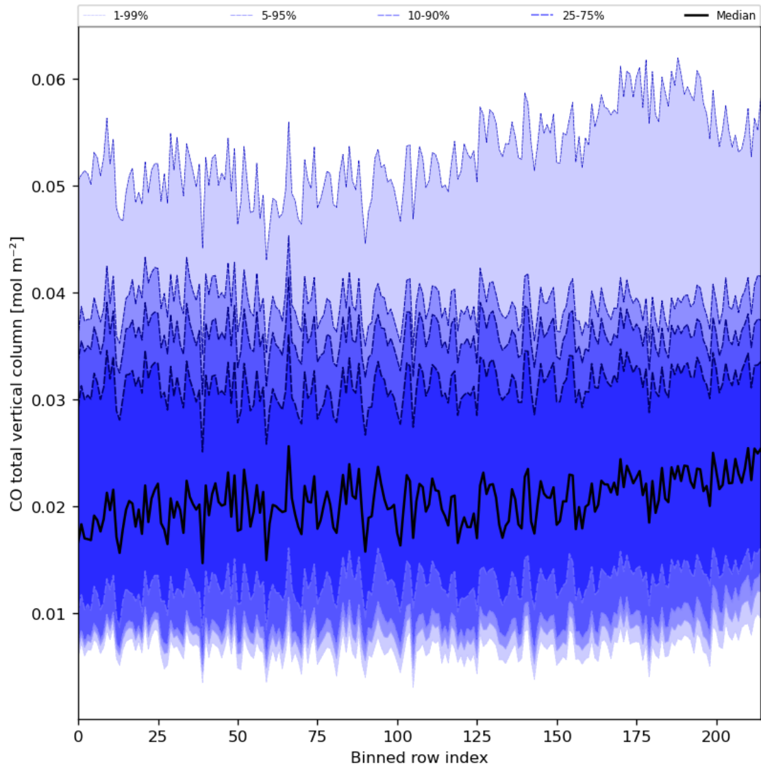
Figure 26: Along track statistics of “CO total vertical column” for 2024-01-21 to 2024-01-22
