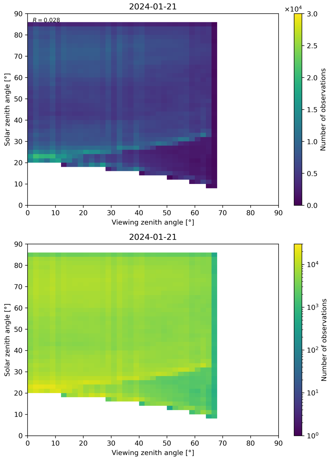
Figure 77: Scatter density plot of “Viewing zenith angle” against “Solar zenith angle” for 2024-01-21 to 2024-01-22.
