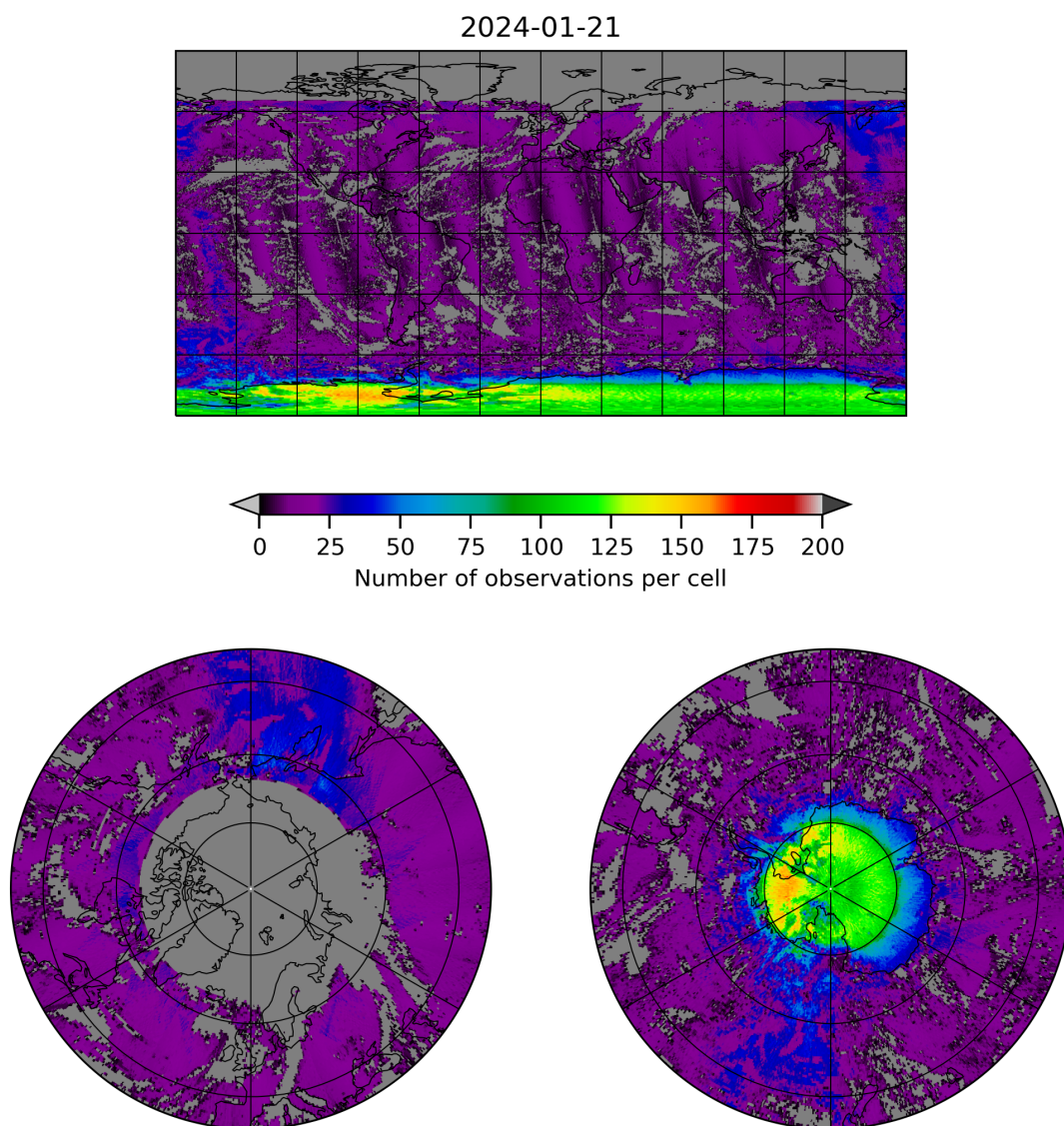
Figure 8: Map of the number of observations for 2024-01-21 to 2024-01-22
