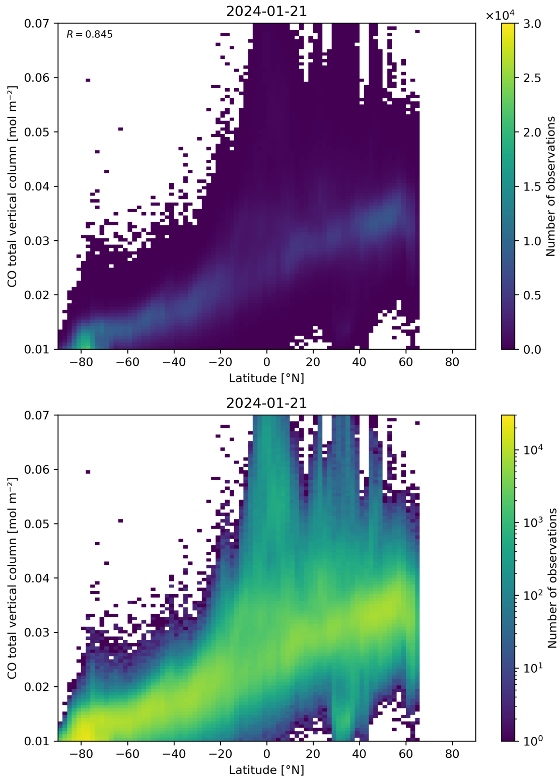
Figure 51: Scatter density plot of “Latitude” against “CO total vertical column” for 2024-01-21 to 2024-01-22.
