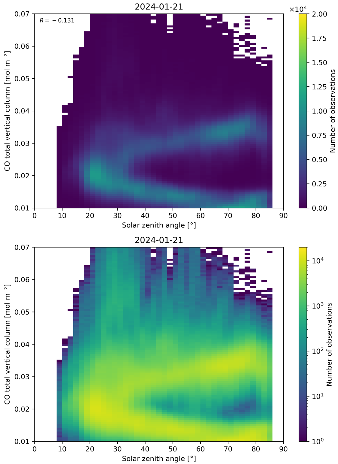
Figure 61: Scatter density plot of “Solar zenith angle” against “CO total vertical column” for 2024-01-21 to 2024-01-22.
