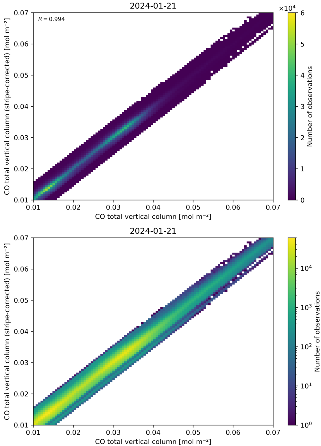
Figure 33: Scatter density plot of “CO total vertical column” against “CO total vertical column (stripe-corrected)” for 2024-01-21 to 2024-01-22.
