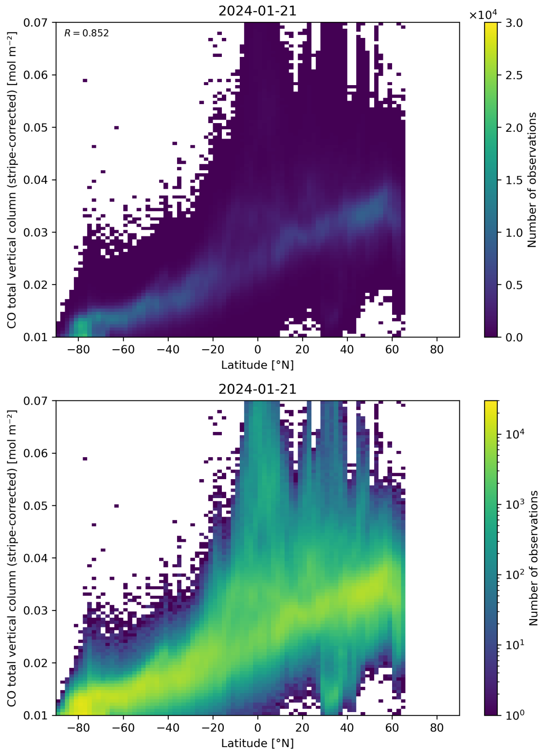
Figure 52: Scatter density plot of “Latitude” against “CO total vertical column (stripe-corrected)” for 2024-01-21 to 2024-01-22.
