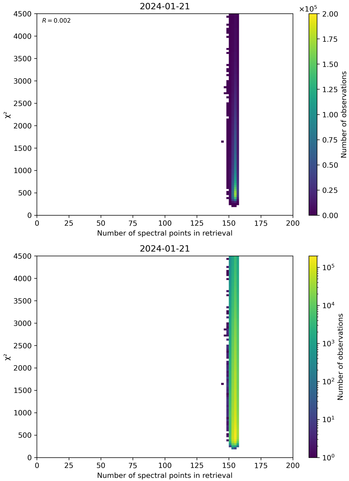
Figure 58: Scatter density plot of “Number of spectral points in retrieval” against “ \chi^2 ” for 2024-01-21 to 2024-01-22.
