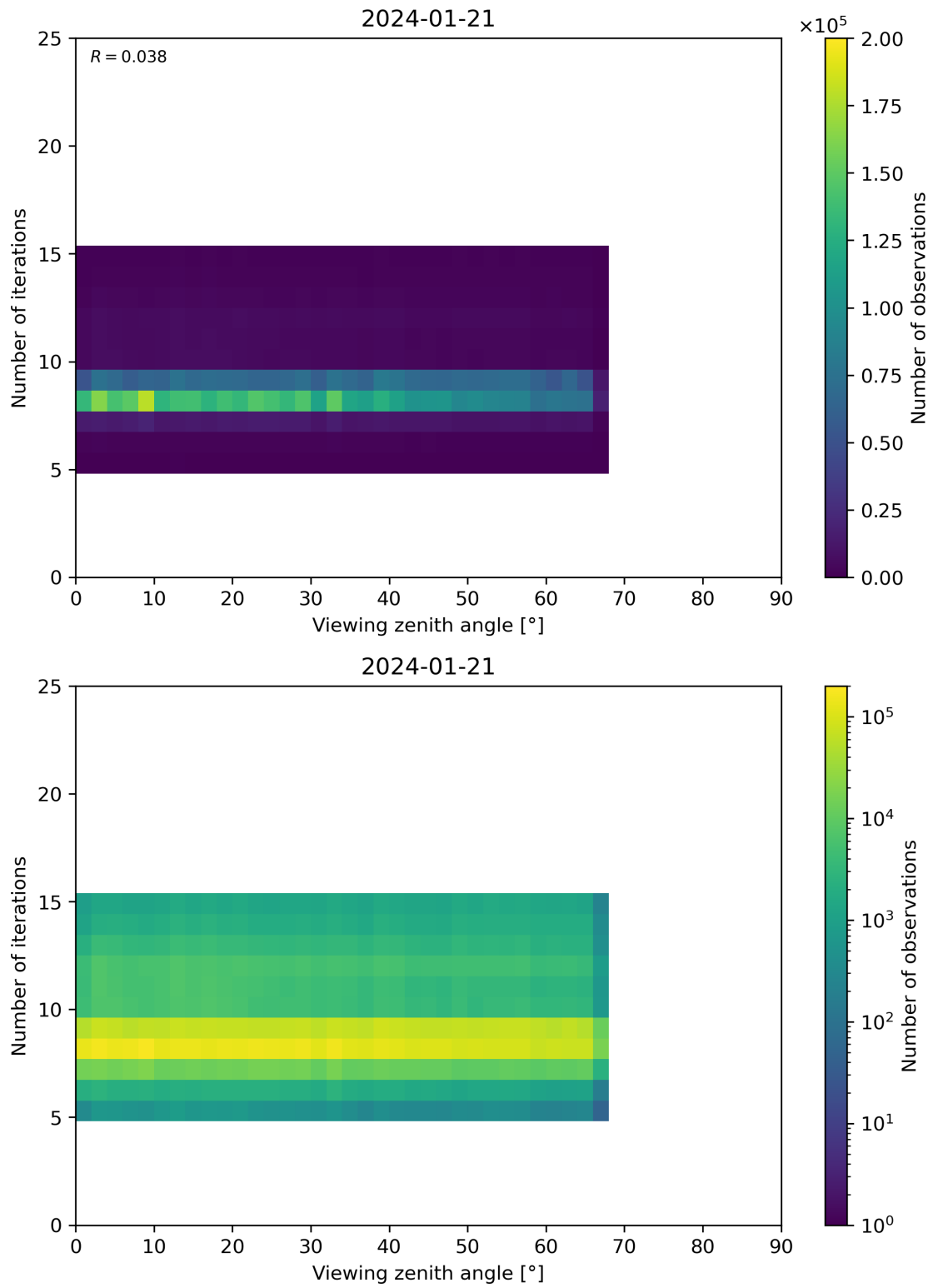
Figure 75: Scatter density plot of “Viewing zenith angle” against “Number of iterations” for 2024-01-21 to 2024-01-22.
