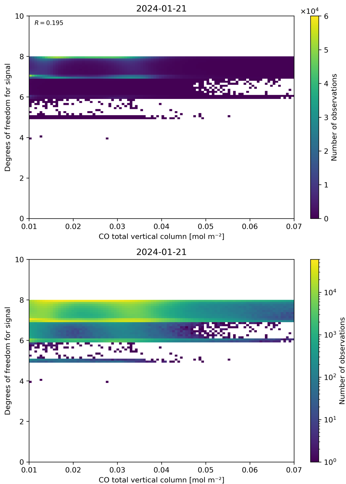
Figure 41: Scatter density plot of “CO total vertical column” against “Degrees of freedom for signal” for 2024-01-21 to 2024-01-22.
