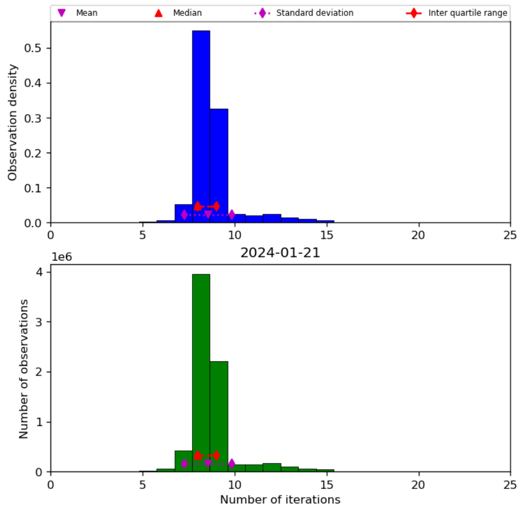
Figure 24: Histogram of “Number of iterations” for 2024-01-21 to 2024-01-22
