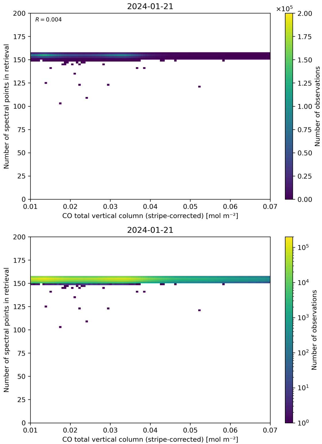
Figure 40: Scatter density plot of “CO total vertical column (stripe-corrected)” against “Number of spectral points in retrieval” for 2024-01-21 to 2024-01-22.
