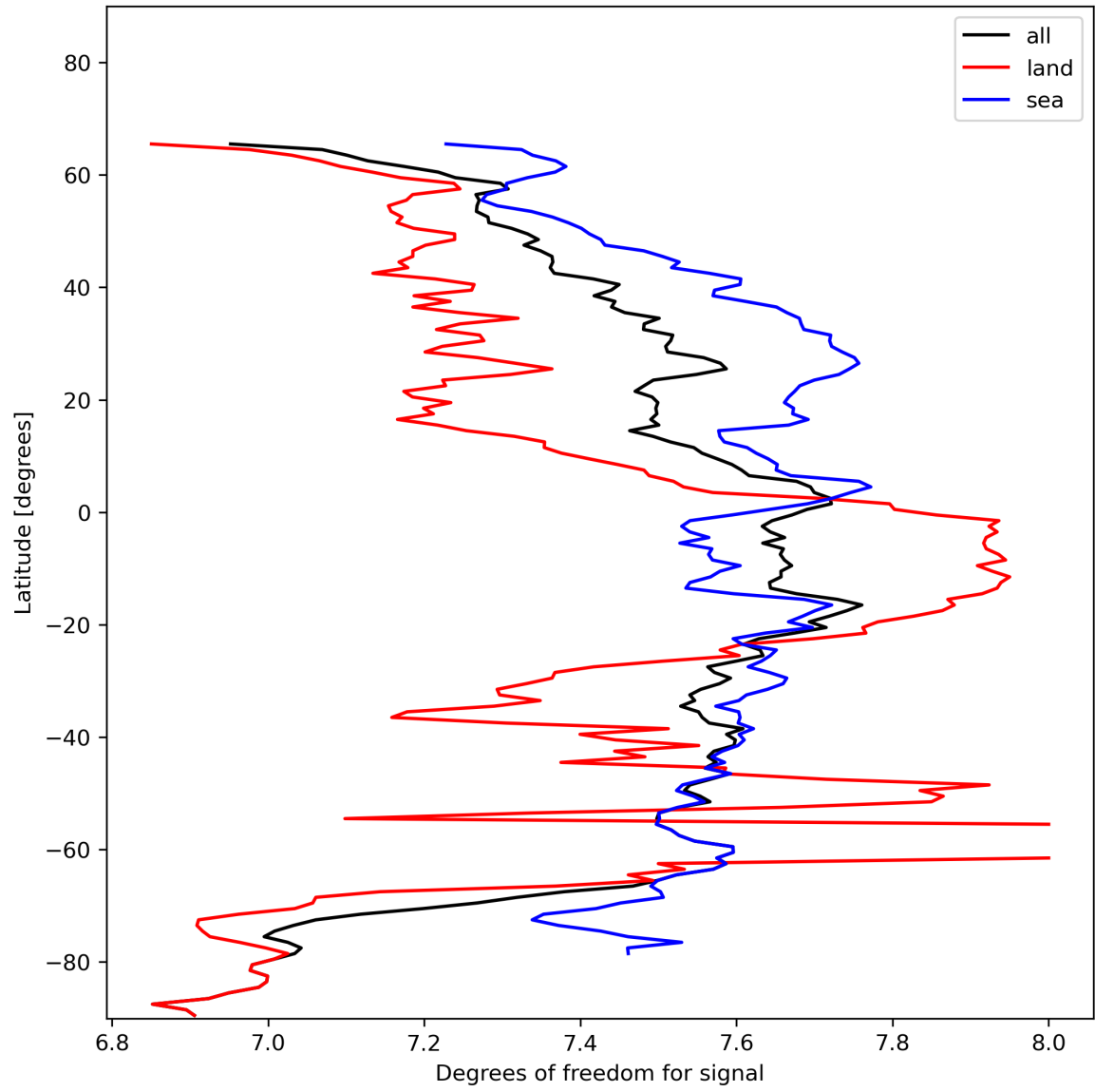
Figure 15: Zonal average of “Degrees of freedom for signal” for 2024-01-21 to 2024-01-22.
