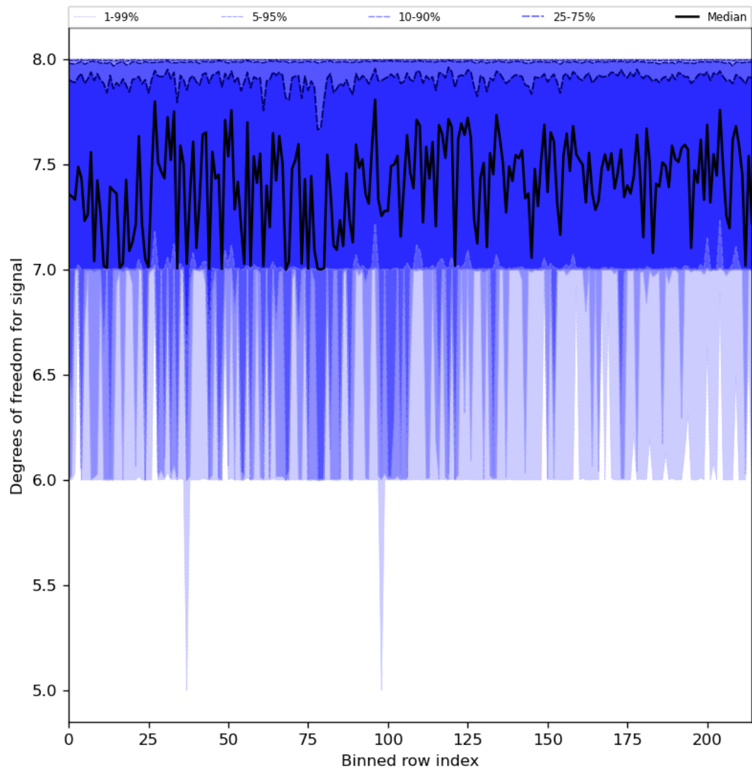
Figure 31: Along track statistics of “Degrees of freedom for signal” for 2024-01-21 to 2024-01-22
