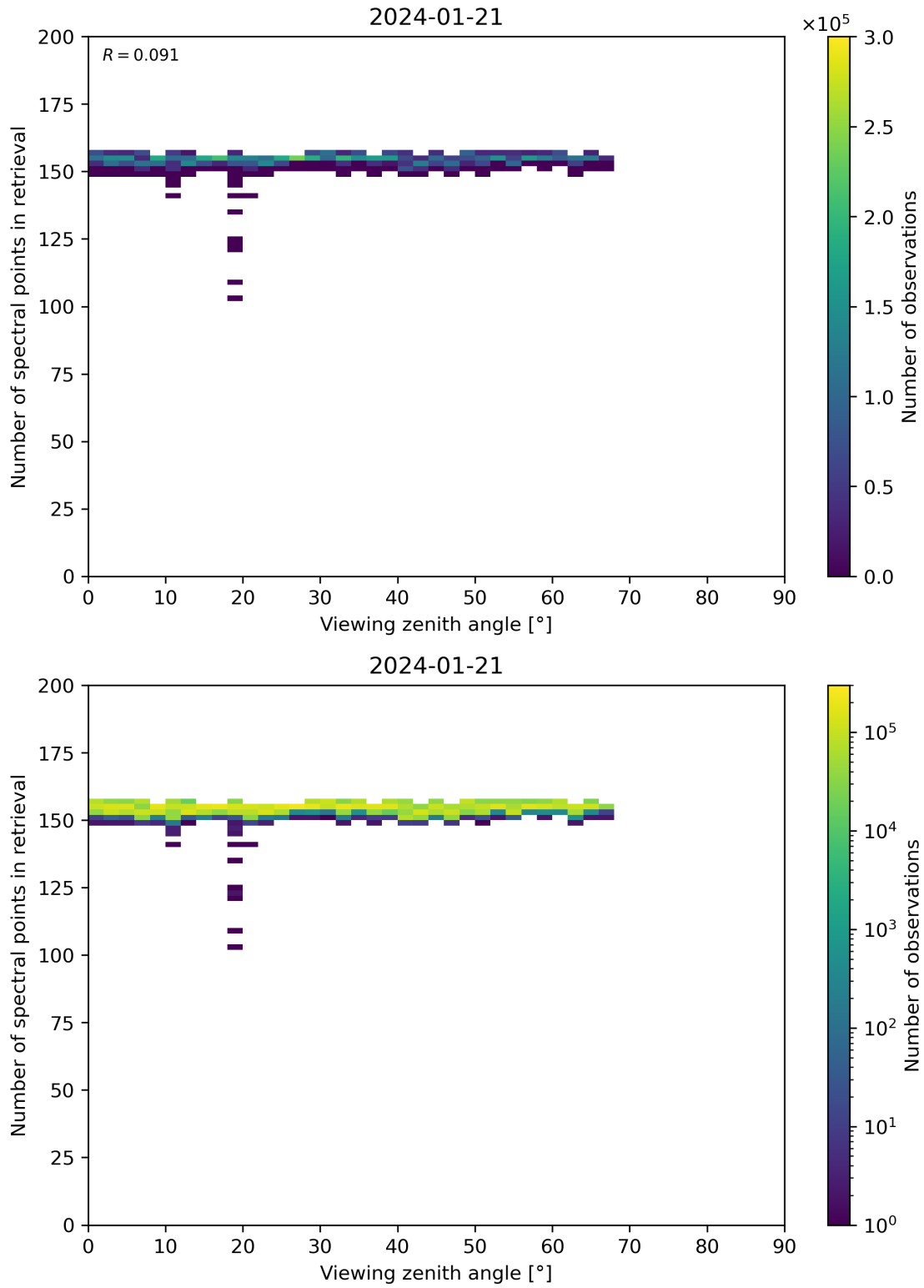
Figure 76: Scatter density plot of “Viewing zenith angle” against “Number of spectral points in retrieval” for 2024-01-21 to 2024-01-22.
