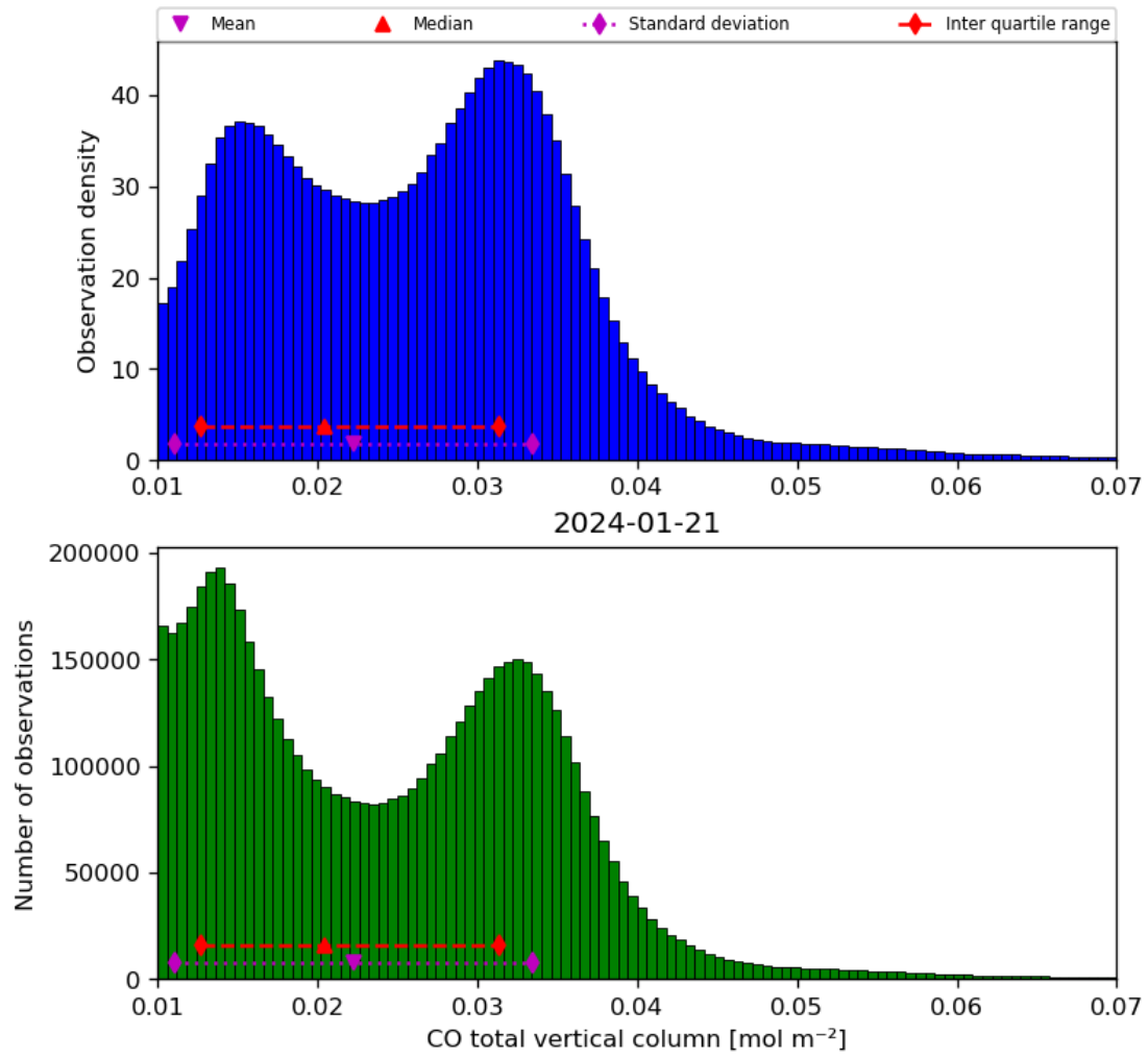
Figure 18: Histogram of “CO total vertical column” for 2024-01-21 to 2024-01-22
