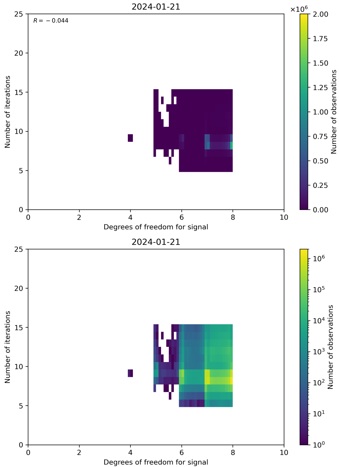
Figure 50: Scatter density plot of “Degrees of freedom for signal” against “Number of iterations” for 2024-01-21 to 2024-01-22.
