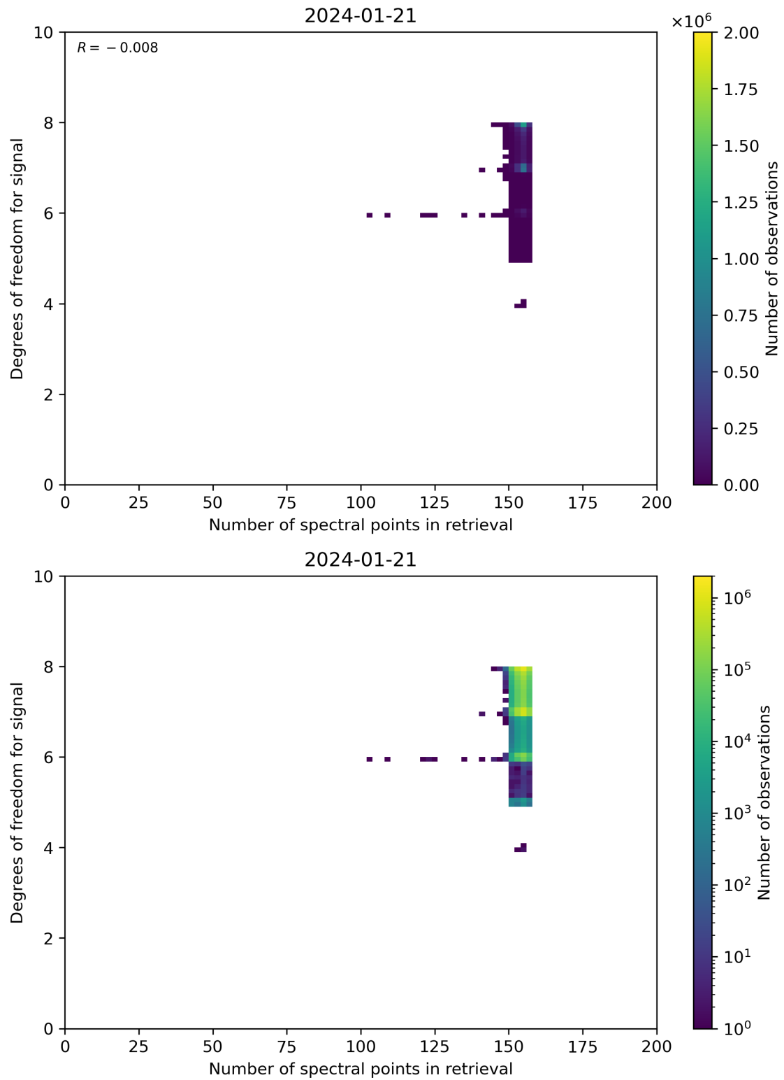
Figure 59: Scatter density plot of “Number of spectral points in retrieval” against “Degrees of freedom for signal” for 2024-01-21 to 2024-01-22.
