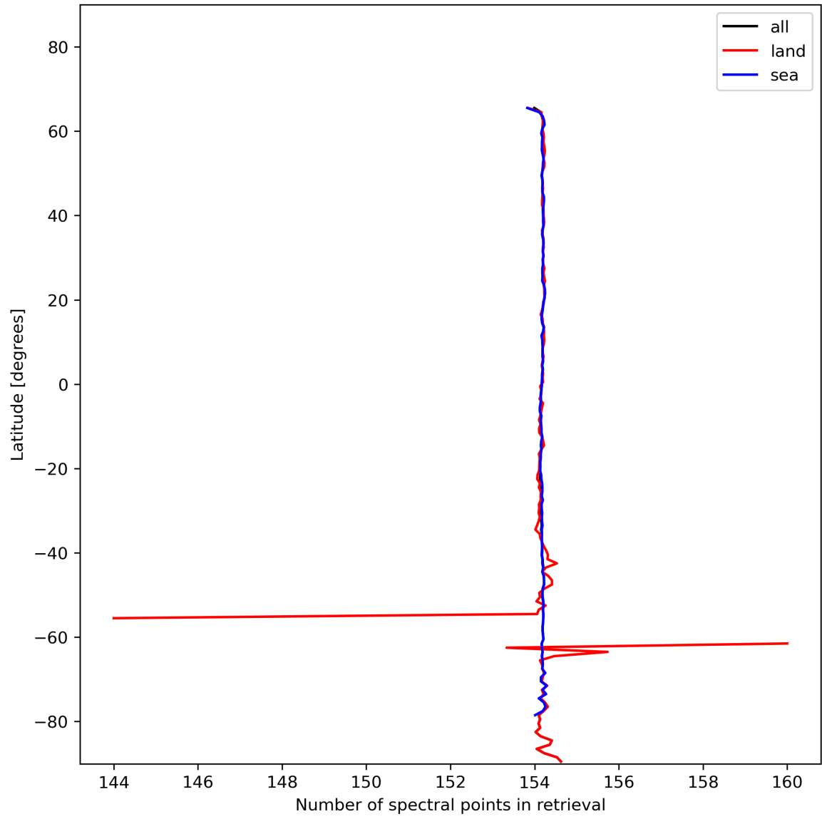
Figure 13: Zonal average of “Number of spectral points in retrieval” for 2024-01-21 to 2024-01-22.
