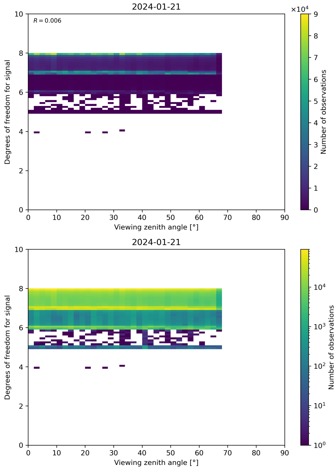
Figure 73: Scatter density plot of “Viewing zenith angle” against “Degrees of freedom for signal” for 2024-01-21 to 2024-01-22.
