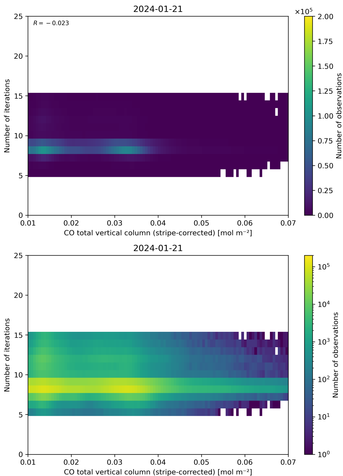
Figure 39: Scatter density plot of “CO total vertical column (stripe-corrected)” against “Number of iterations” for 2024-01-21 to 2024-01-22.
