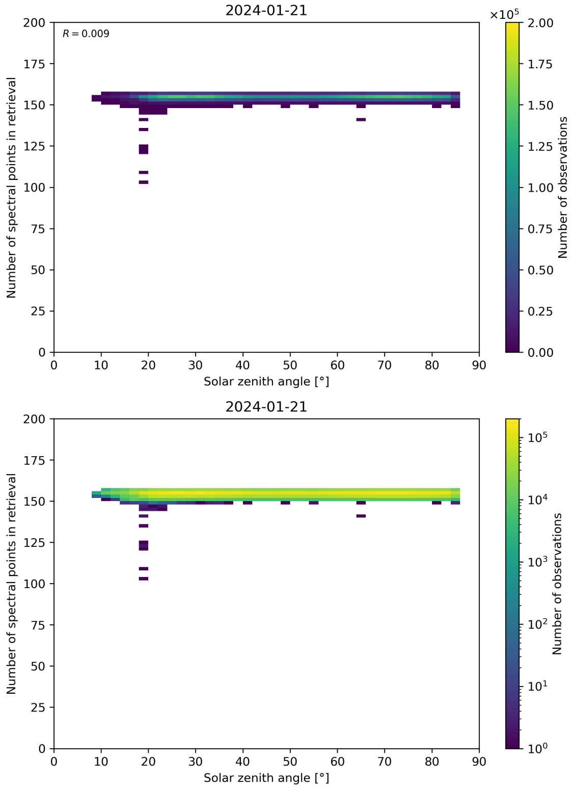
Figure 68: Scatter density plot of “Solar zenith angle” against “Number of spectral points in retrieval” for 2024-01-21 to 2024-01-22.
