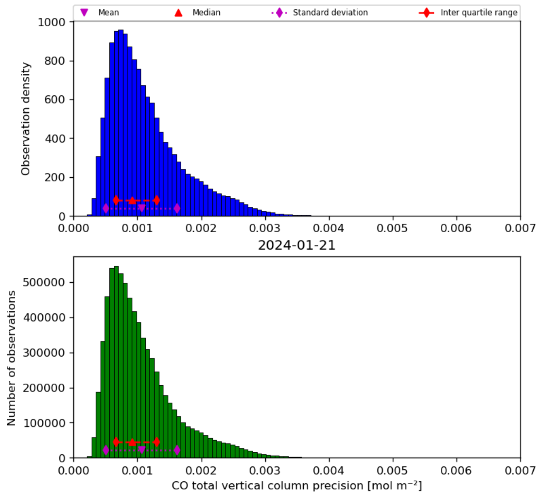
Figure 20: Histogram of “CO total vertical column precision” for 2024-01-21 to 2024-01-22
