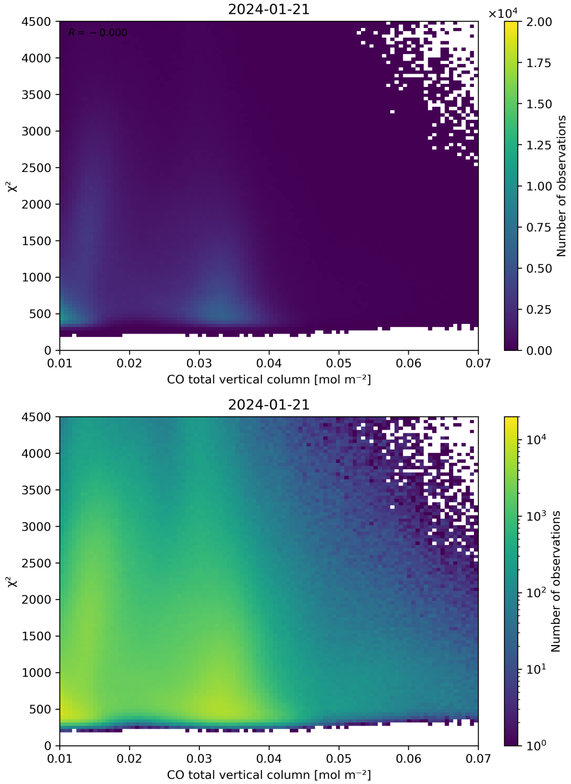
Figure 35: Scatter density plot of “CO total vertical column” against “ \chi^2 ” for 2024-01-21 to 2024-01-22.
