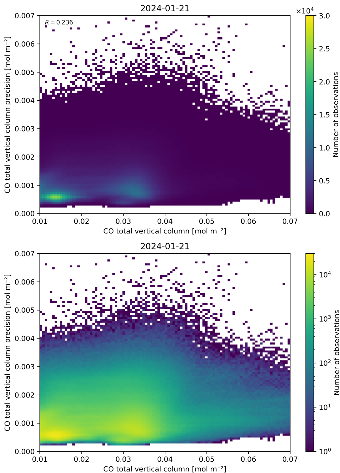
Figure 34: Scatter density plot of “CO total vertical column” against “CO total vertical column precision” for 2024-01-21 to 2024-01-22.
