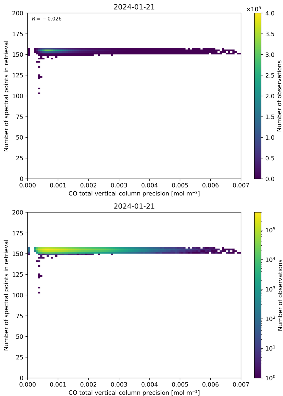
Figure 47: Scatter density plot of “CO total vertical column precision” against “Number of spectral points in retrieval” for 2024-01-21 to 2024-01-22.
