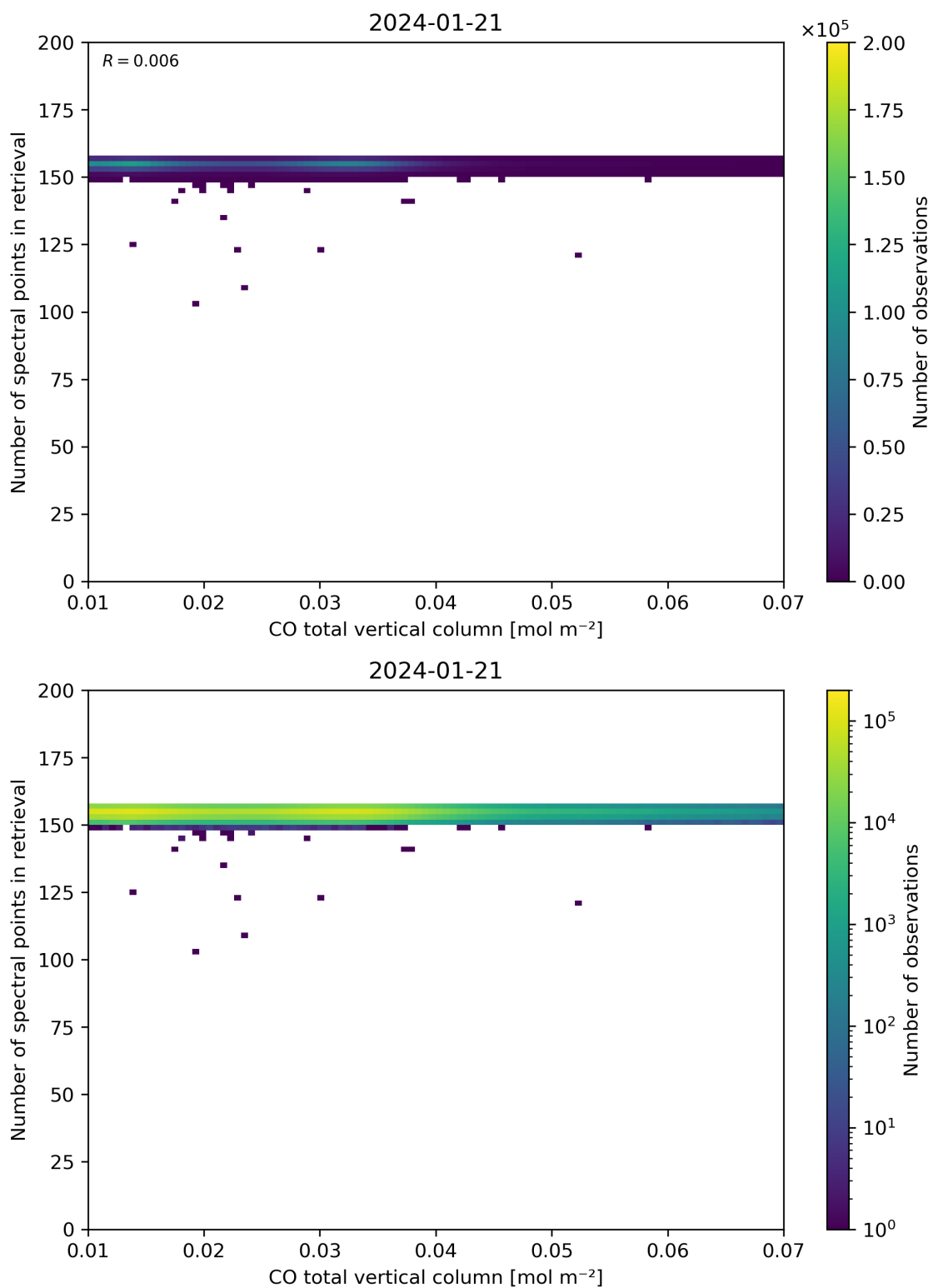
Figure 43: Scatter density plot of “CO total vertical column” against “Number of spectral points in retrieval” for 2024-01-21 to 2024-01-22.
