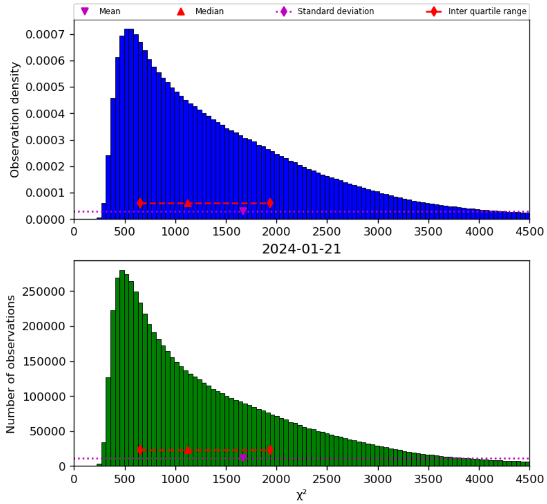
Figure 22: Histogram of “ \chi^2 ” for 2024-01-21 to 2024-01-22
