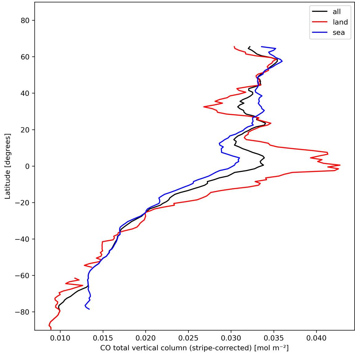
Figure 11: Zonal average of “CO total vertical column (stripe-corrected)” for 2024-01-21 to 2024-01-22.
