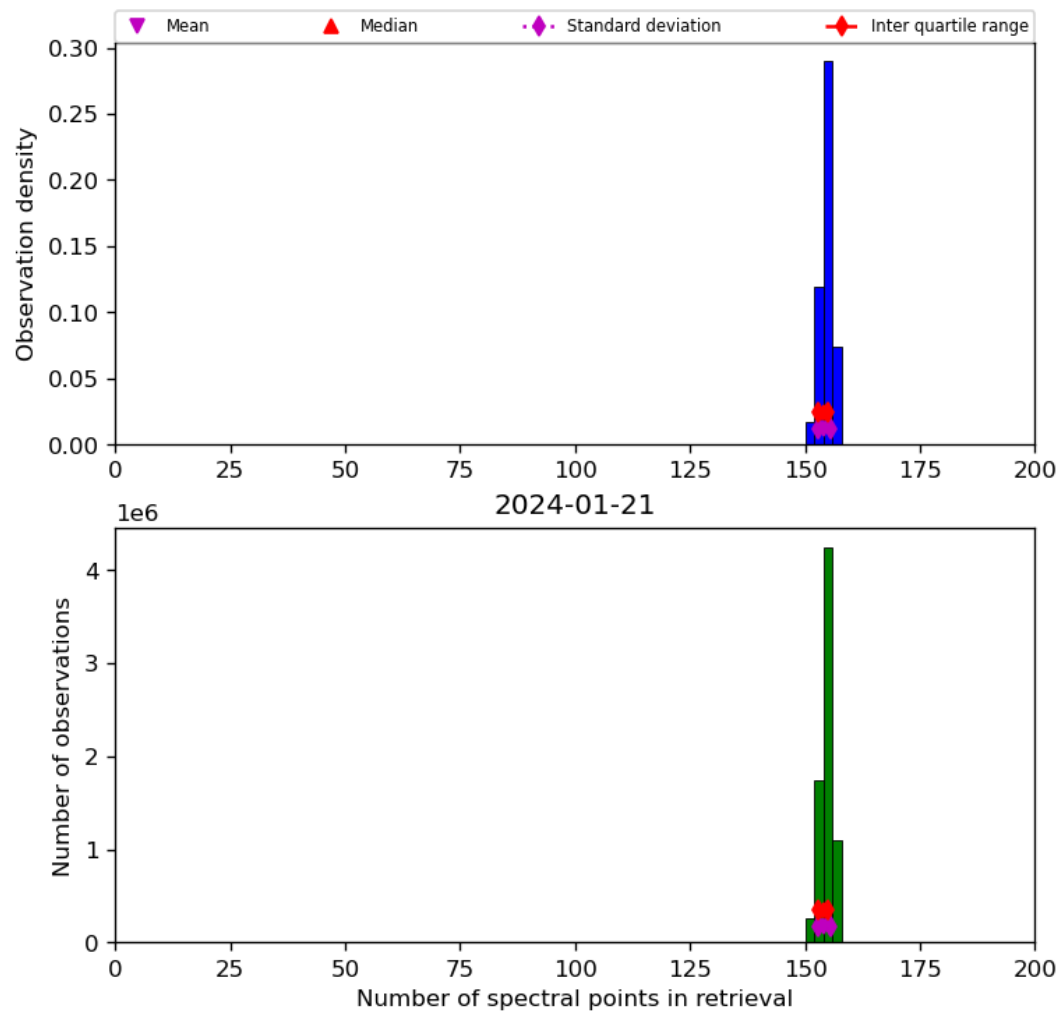
Figure 21: Histogram of “Number of spectral points in retrieval” for 2024-01-21 to 2024-01-22
