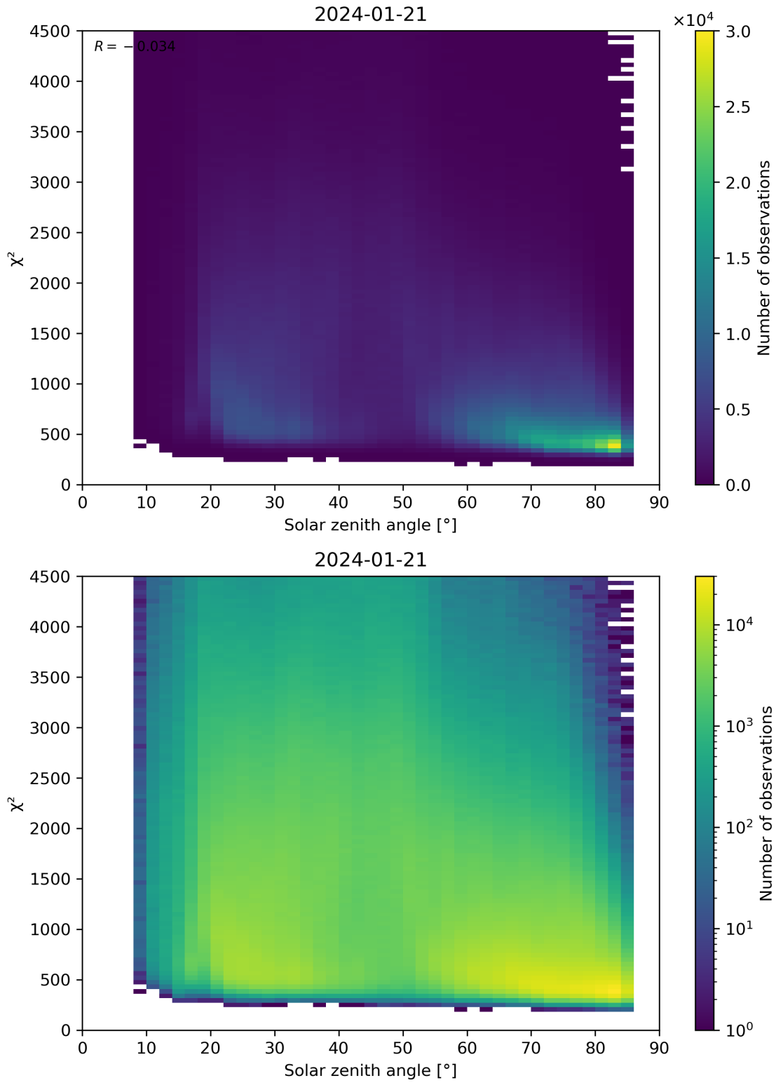
Figure 64: Scatter density plot of “Solar zenith angle” against “ \chi^2 ” for 2024-01-21 to 2024-01-22.
