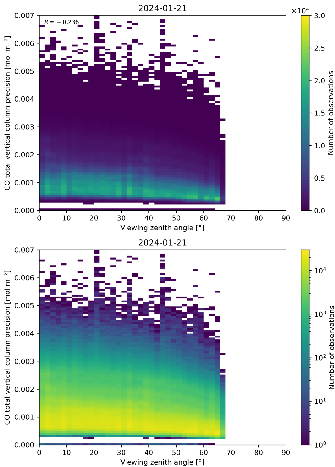
Figure 71: Scatter density plot of “Viewing zenith angle” against “CO total vertical column precision” for 2024-01-21 to 2024-01-22.
