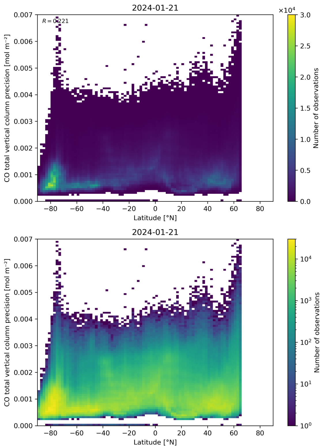
Figure 53: Scatter density plot of “Latitude” against “CO total vertical column precision” for 2024-01-21 to 2024-01-22.
