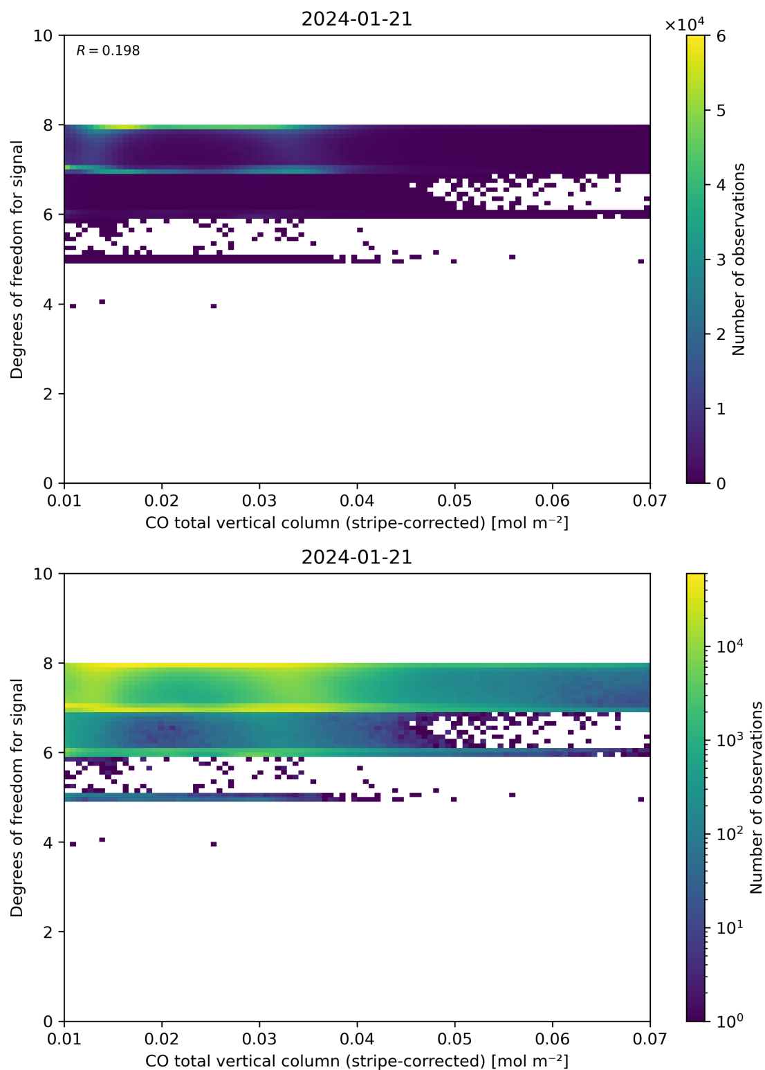
Figure 38: Scatter density plot of “CO total vertical column (stripe-corrected)” against “Degrees of freedom for signal” for 2024-01-21 to 2024-01-22.
