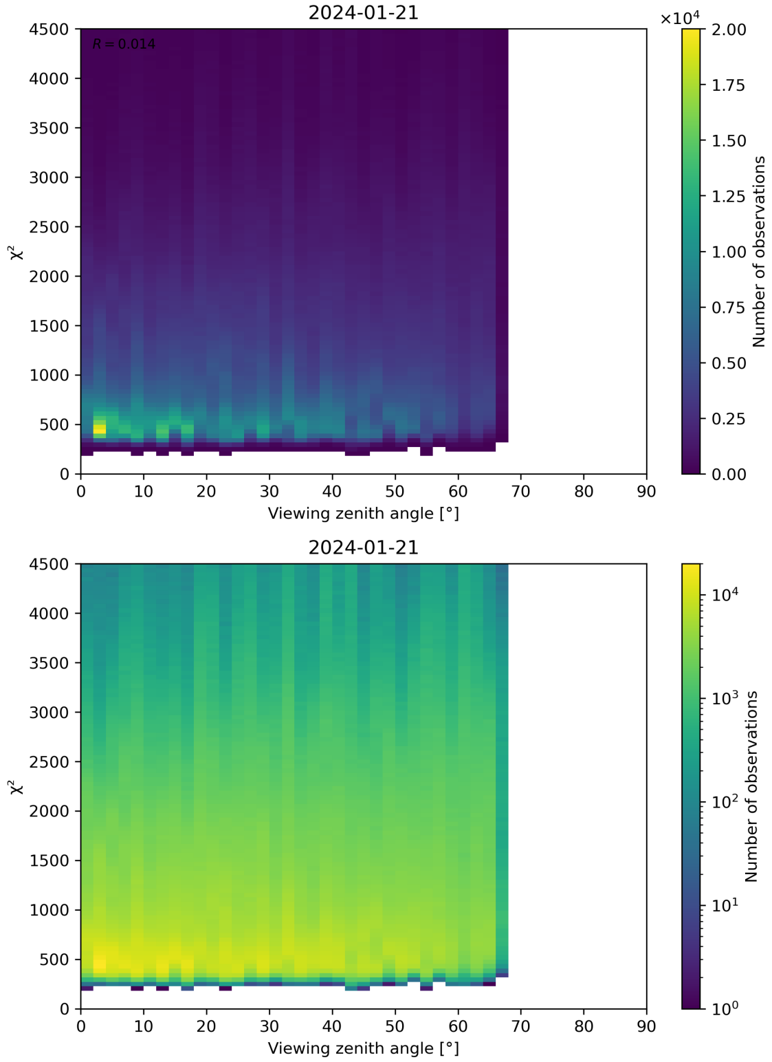
Figure 72: Scatter density plot of “Viewing zenith angle” against “ \chi^2 ” for 2024-01-21 to 2024-01-22.
