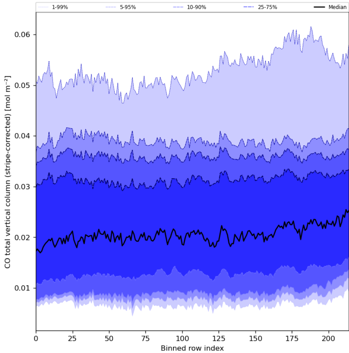
Figure 27: Along track statistics of “CO total vertical column (stripe-corrected)” for 2024-01-21 to 2024-01-22
