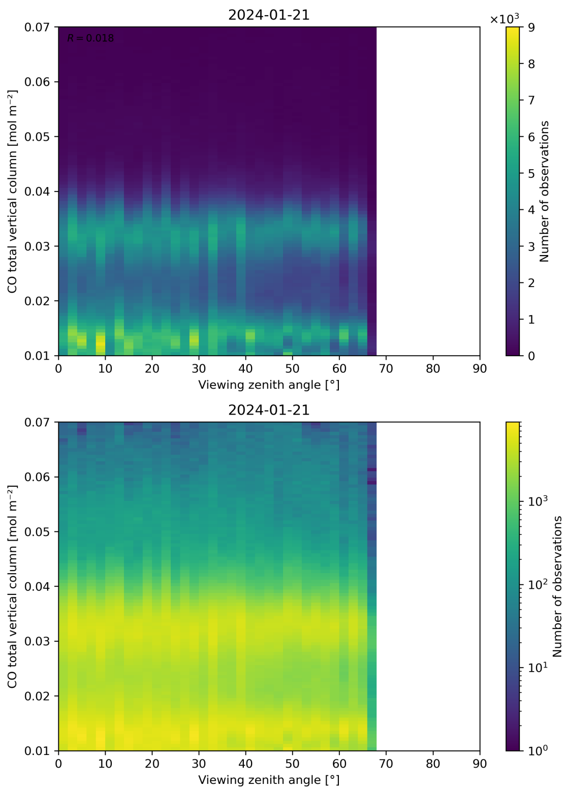
Figure 69: Scatter density plot of “Viewing zenith angle” against “CO total vertical column” for 2024-01-21 to 2024-01-22.
