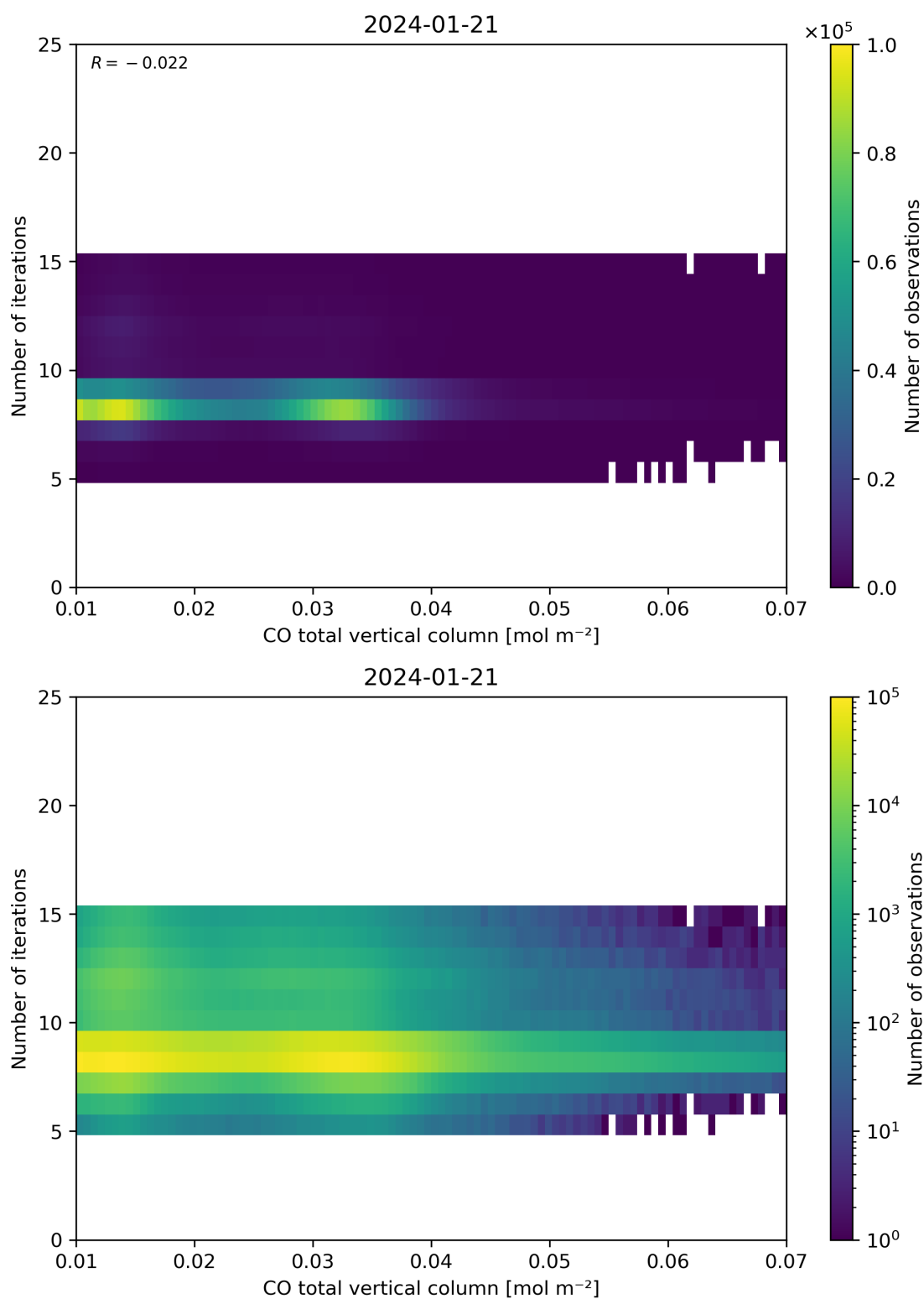
Figure 42: Scatter density plot of “CO total vertical column” against “Number of iterations” for 2024-01-21 to 2024-01-22.
