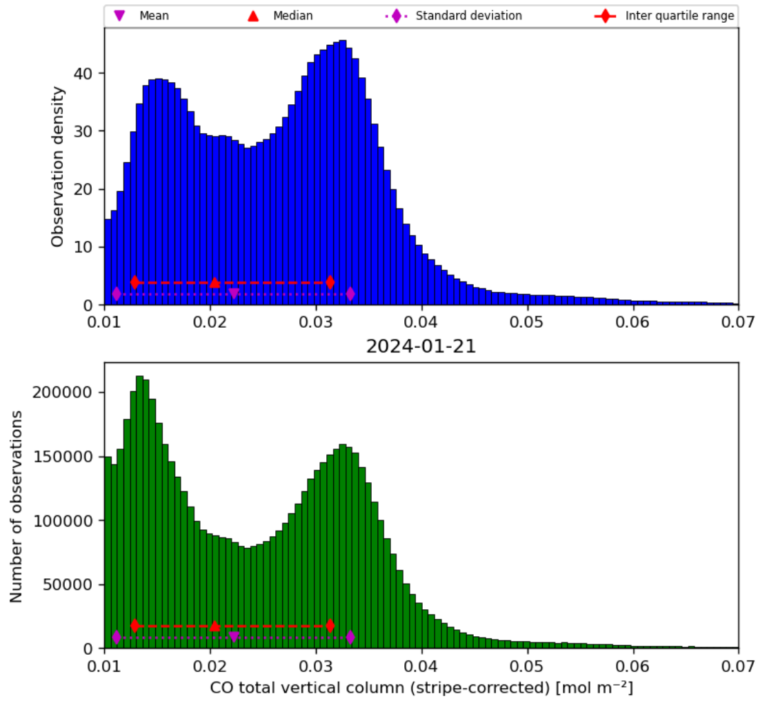
Figure 19: Histogram of “CO total vertical column (stripe-corrected)” for 2024-01-21 to 2024-01-22
