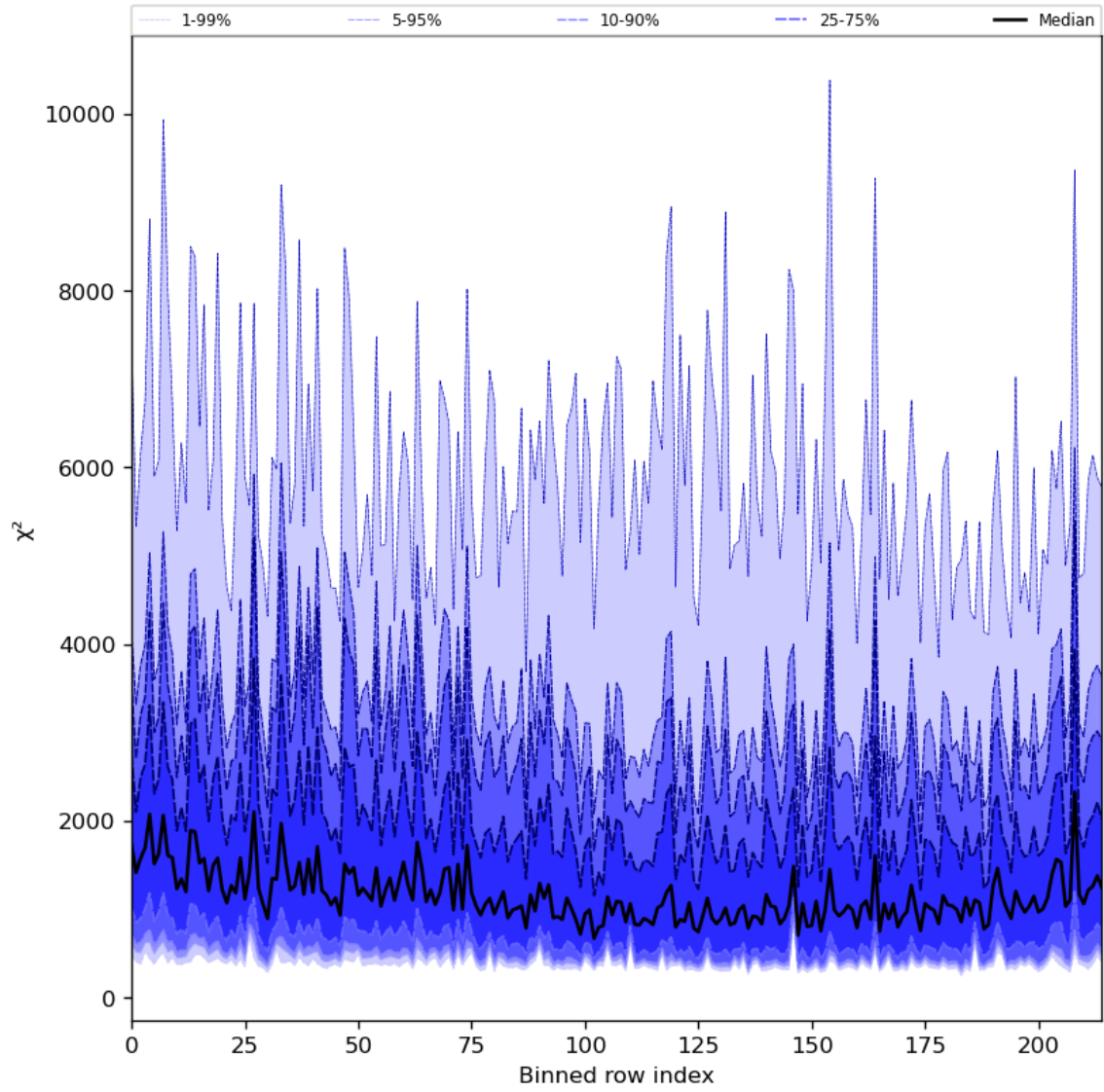
Figure 30: Along track statistics of “ \chi^2 ” for 2024-01-21 to 2024-01-22
