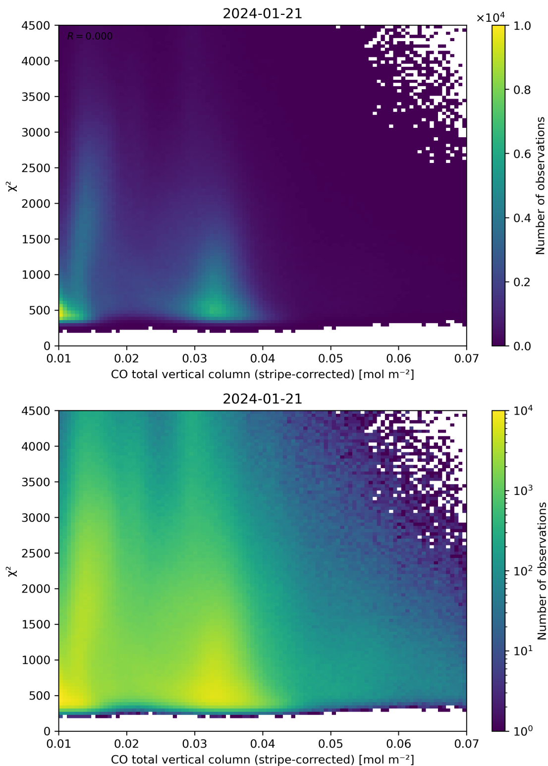
Figure 37: Scatter density plot of “CO total vertical column (stripe-corrected)” against “ \chi^2 ” for 2024-01-21 to 2024-01-22.
