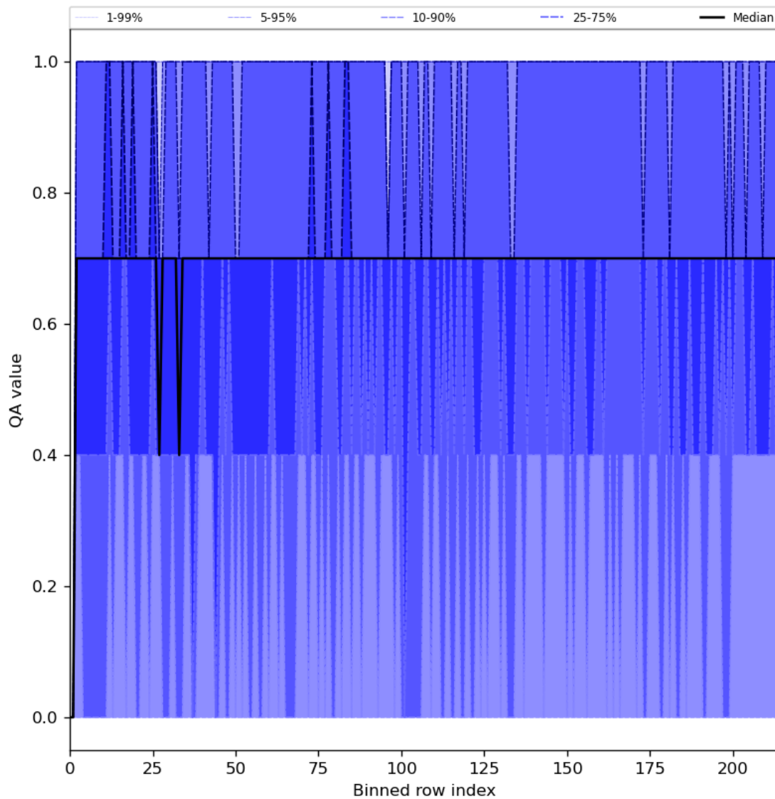
Figure 25: Along track statistics of “QA value” for 2024-01-21 to 2024-01-22
