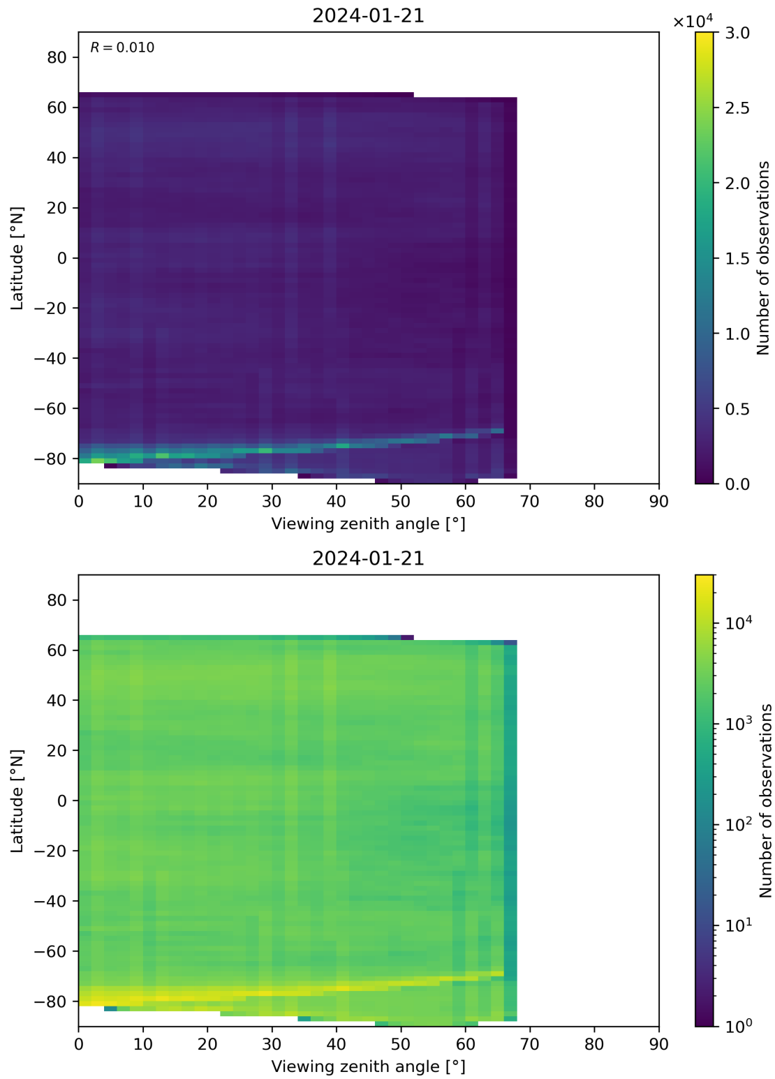
Figure 74: Scatter density plot of “Viewing zenith angle” against “Latitude” for 2024-01-21 to 2024-01-22.
