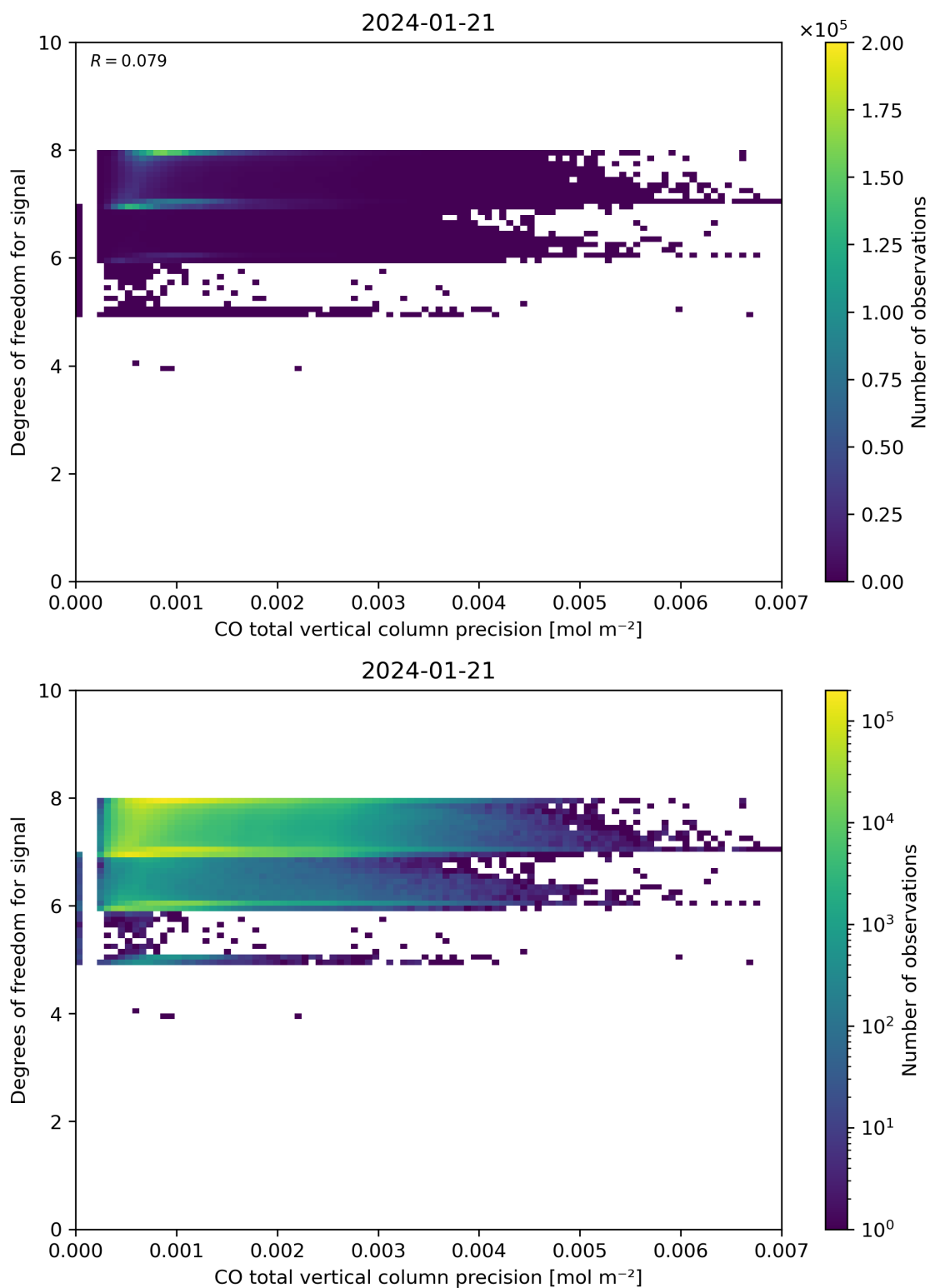
Figure 45: Scatter density plot of “CO total vertical column precision” against “Degrees of freedom for signal” for 2024-01-21 to 2024-01-22.
