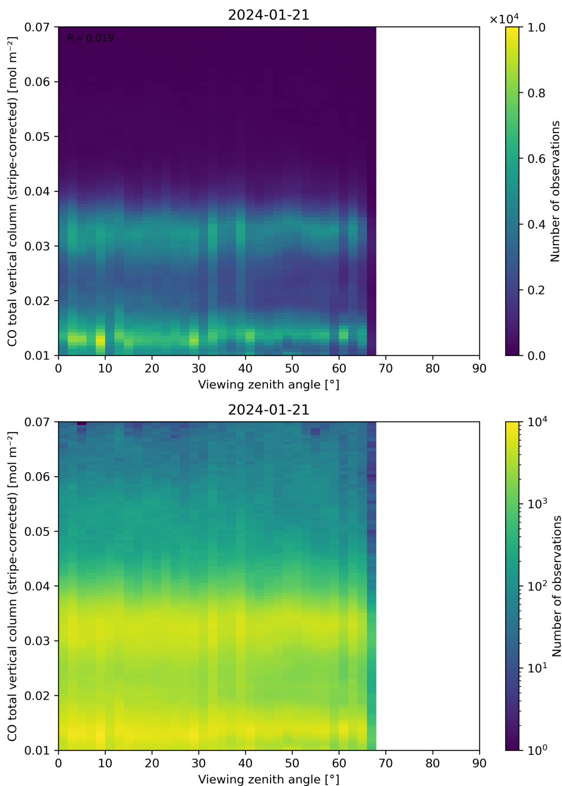
Figure 70: Scatter density plot of “Viewing zenith angle” against “CO total vertical column (stripe-corrected)” for 2024-01-21 to 2024-01-22.
