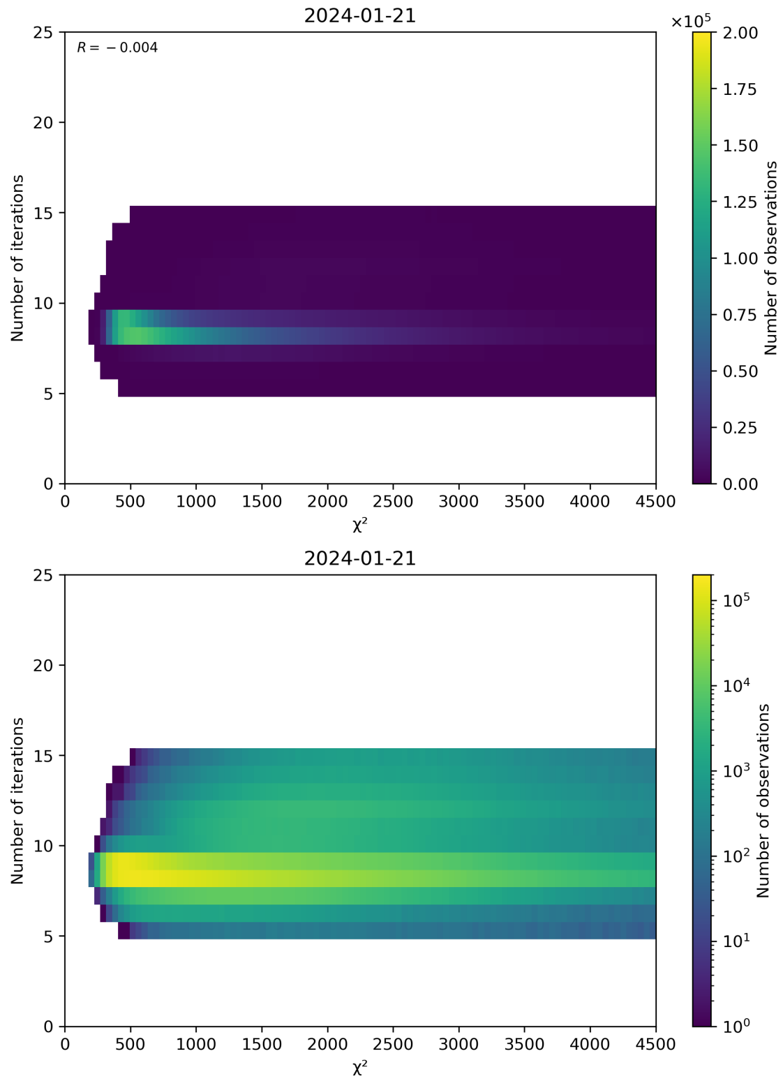
Figure 49: Scatter density plot of “ \chi^2 ” against “Number of iterations” for 2024-01-21 to 2024-01-22.
