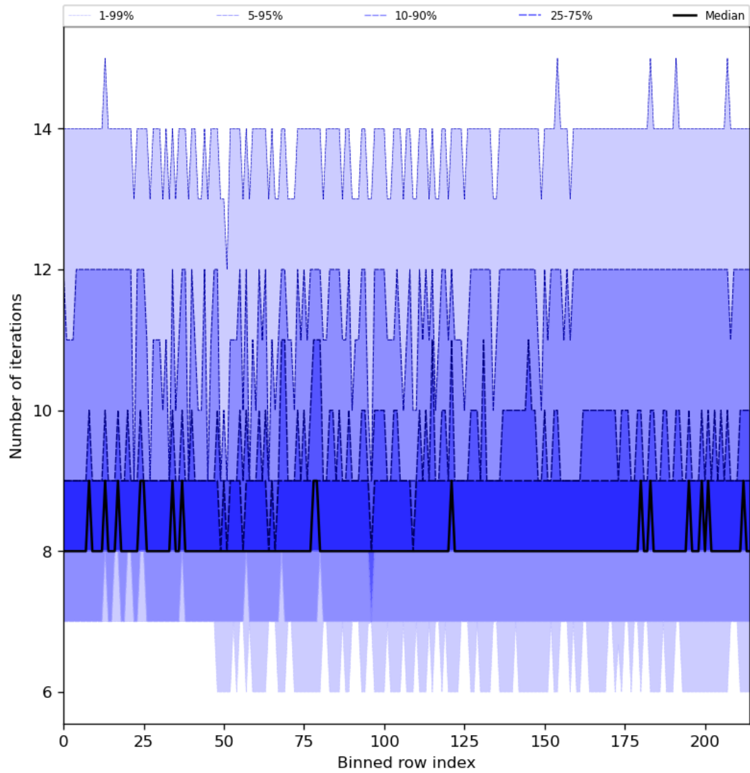
Figure 32: Along track statistics of “Number of iterations” for 2024-01-21 to 2024-01-22
