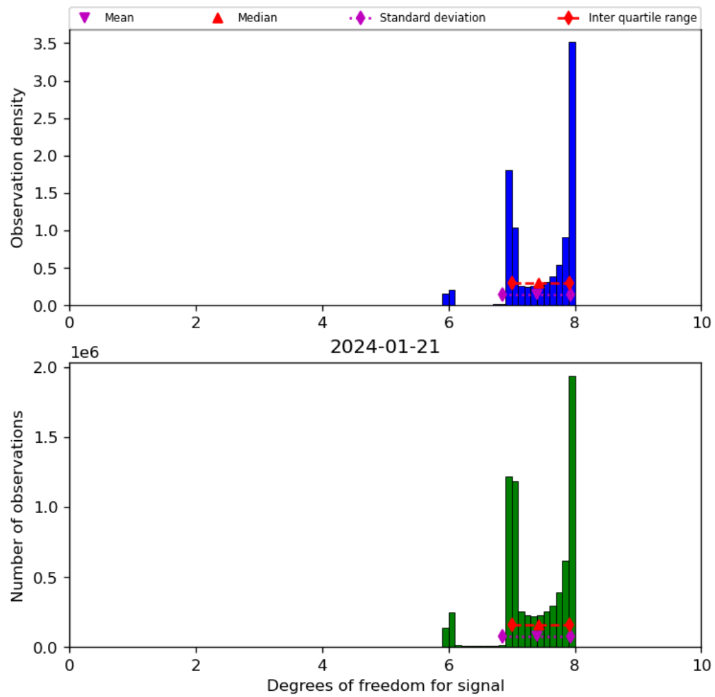
Figure 23: Histogram of “Degrees of freedom for signal” for 2024-01-21 to 2024-01-22
