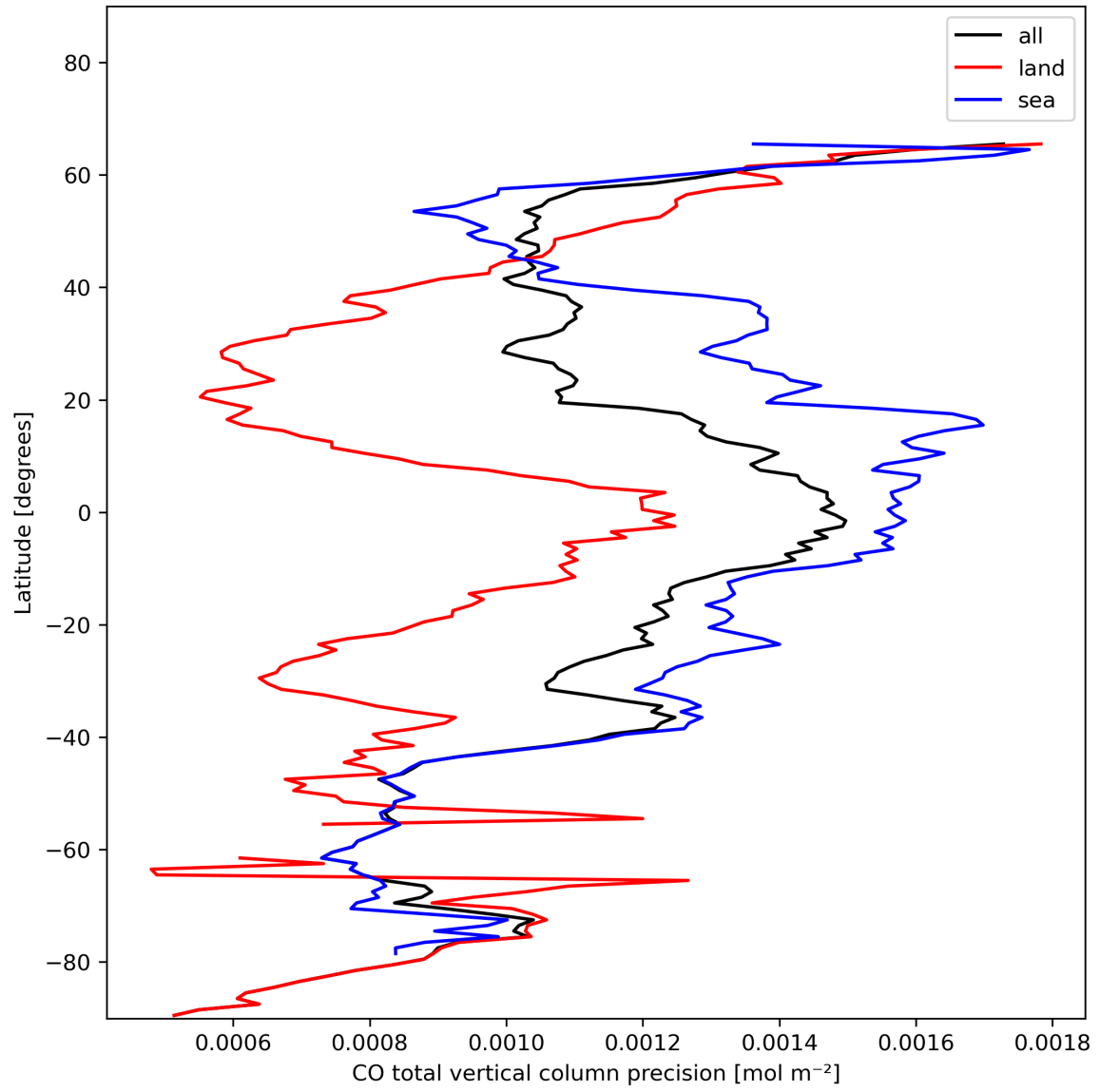
Figure 12: Zonal average of “CO total vertical column precision” for 2024-01-21 to 2024-01-22.
