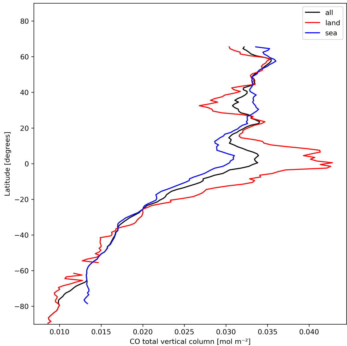
Figure 10: Zonal average of “CO total vertical column” for 2024-01-21 to 2024-01-22.
