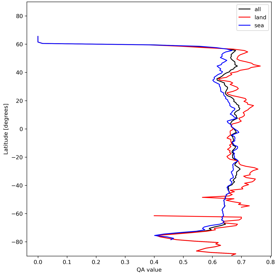
Figure 9: Zonal average of “QA value” for 2024-01-21 to 2024-01-22.
