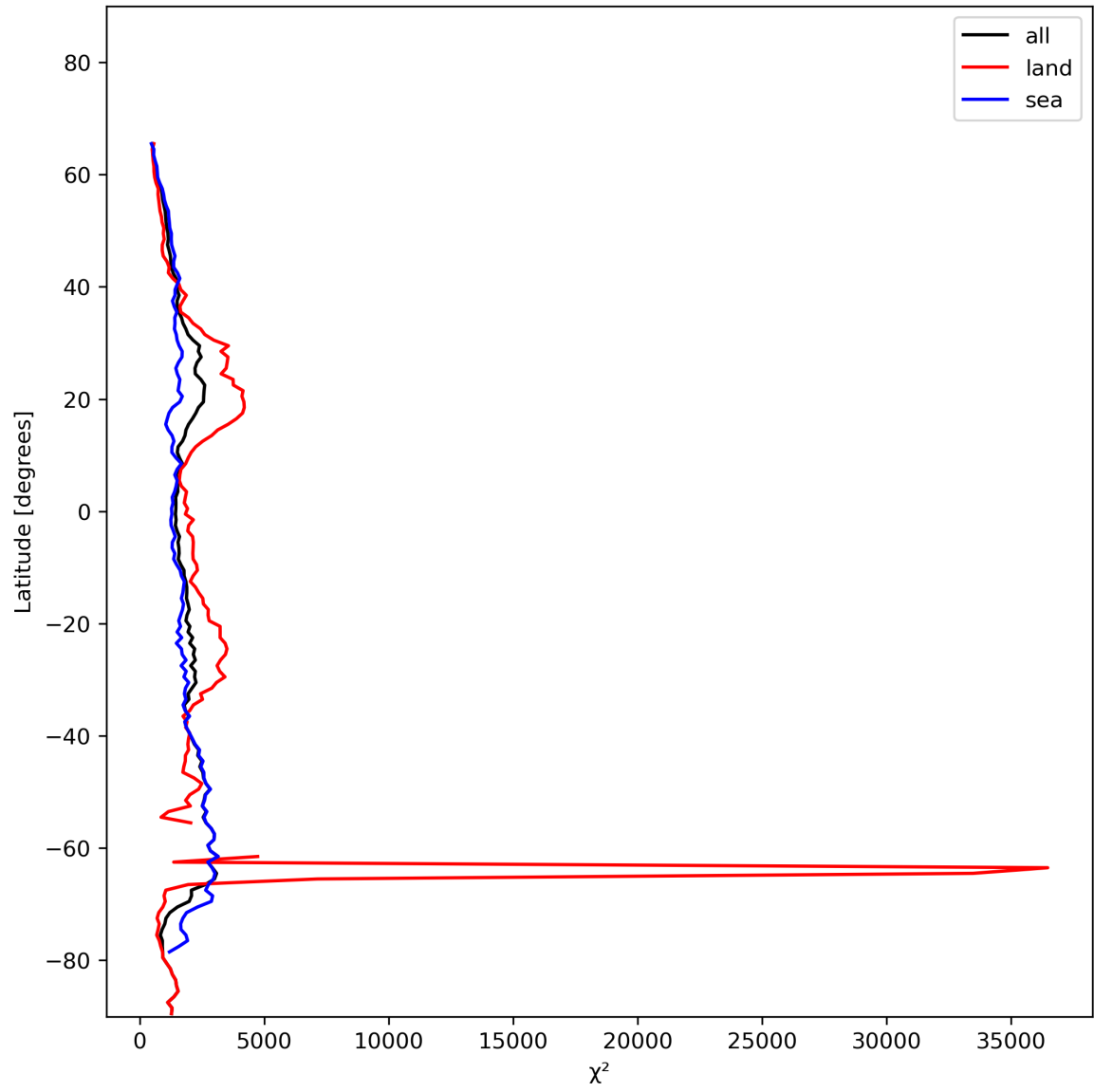
Figure 14: Zonal average of “ \chi^2 ” for 2024-01-21 to 2024-01-22.
