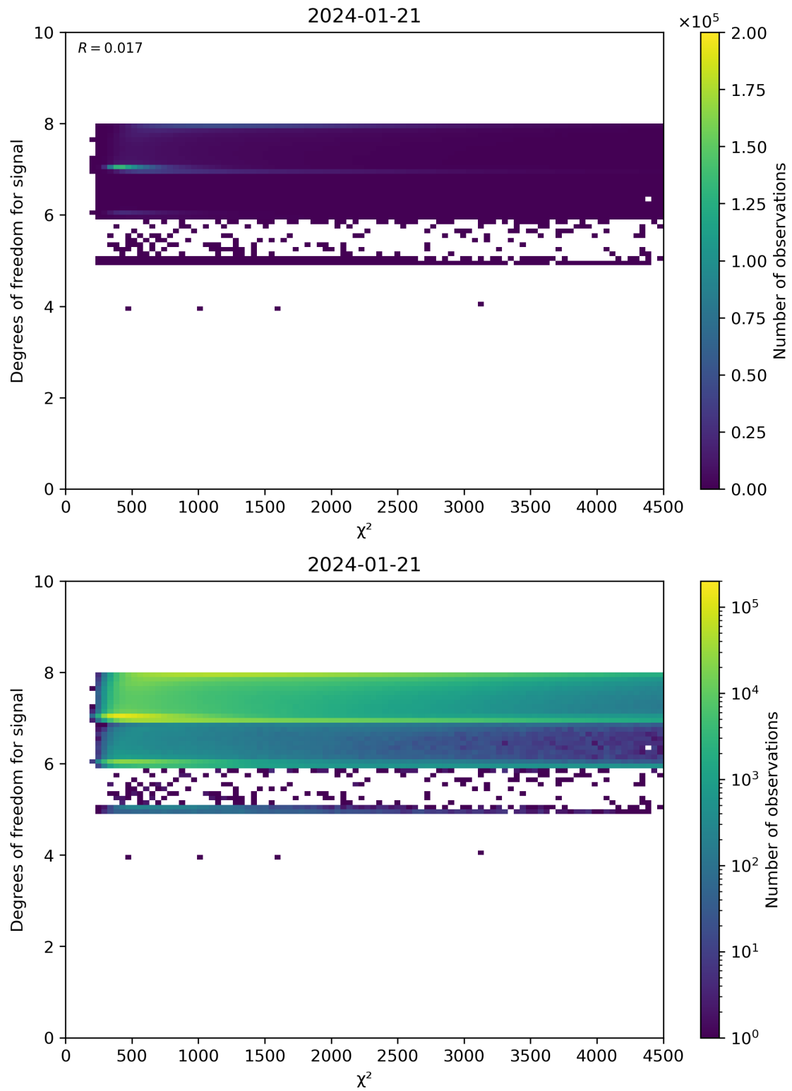
Figure 48: Scatter density plot of “ \chi^2 ” against “Degrees of freedom for signal” for 2024-01-21 to 2024-01-22.
