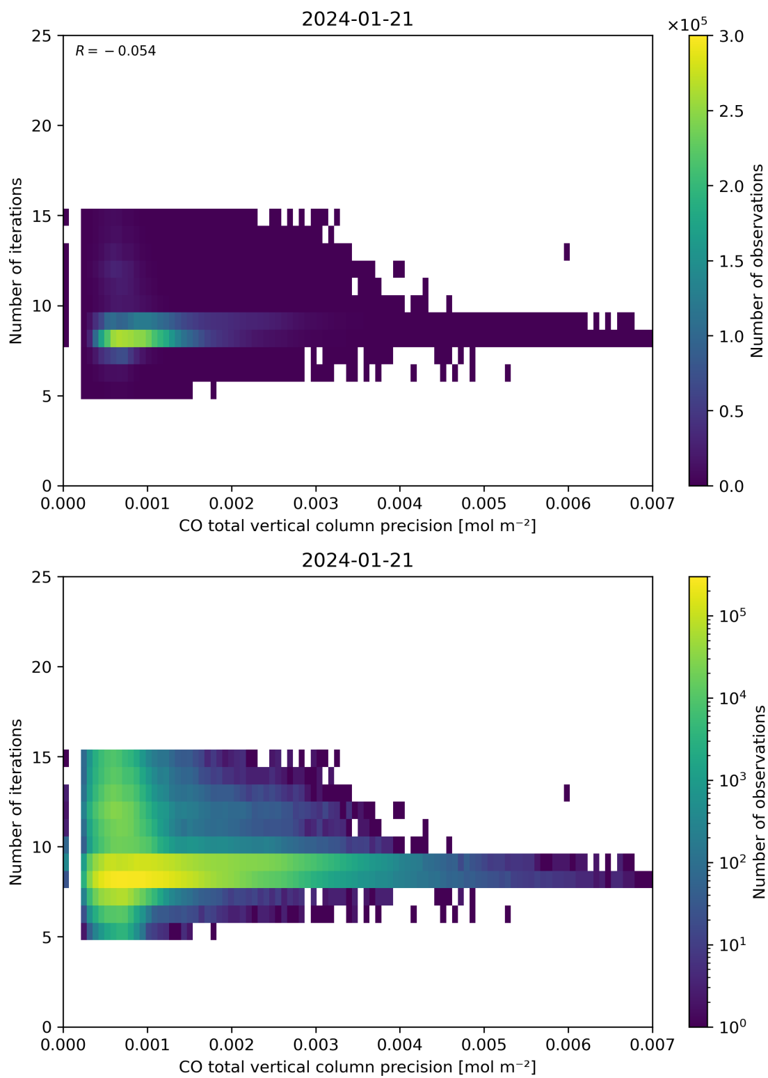
Figure 46: Scatter density plot of “CO total vertical column precision” against “Number of iterations” for 2024-01-21 to 2024-01-22.
