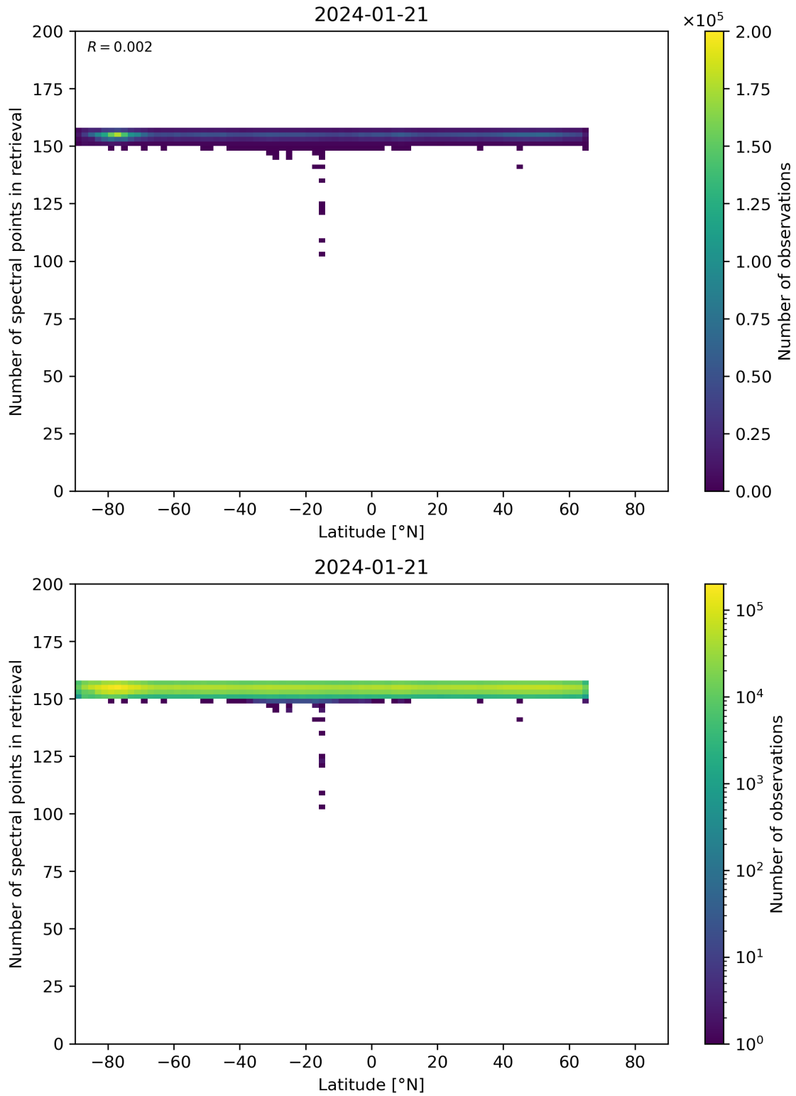
Figure 57: Scatter density plot of “Latitude” against “Number of spectral points in retrieval” for 2024-01-21 to 2024-01-22.
