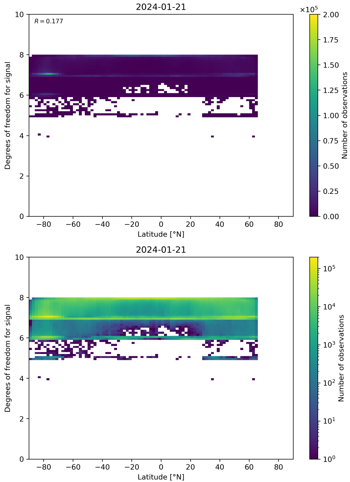
Figure 55: Scatter density plot of “Latitude” against “Degrees of freedom for signal” for 2024-01-21 to 2024-01-22.
