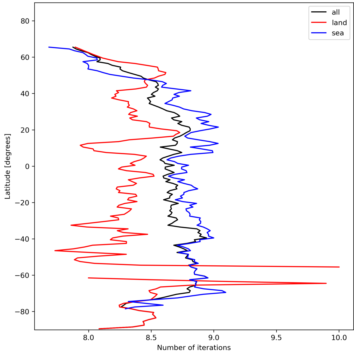
Figure 16: Zonal average of “Number of iterations” for 2024-01-21 to 2024-01-22.
