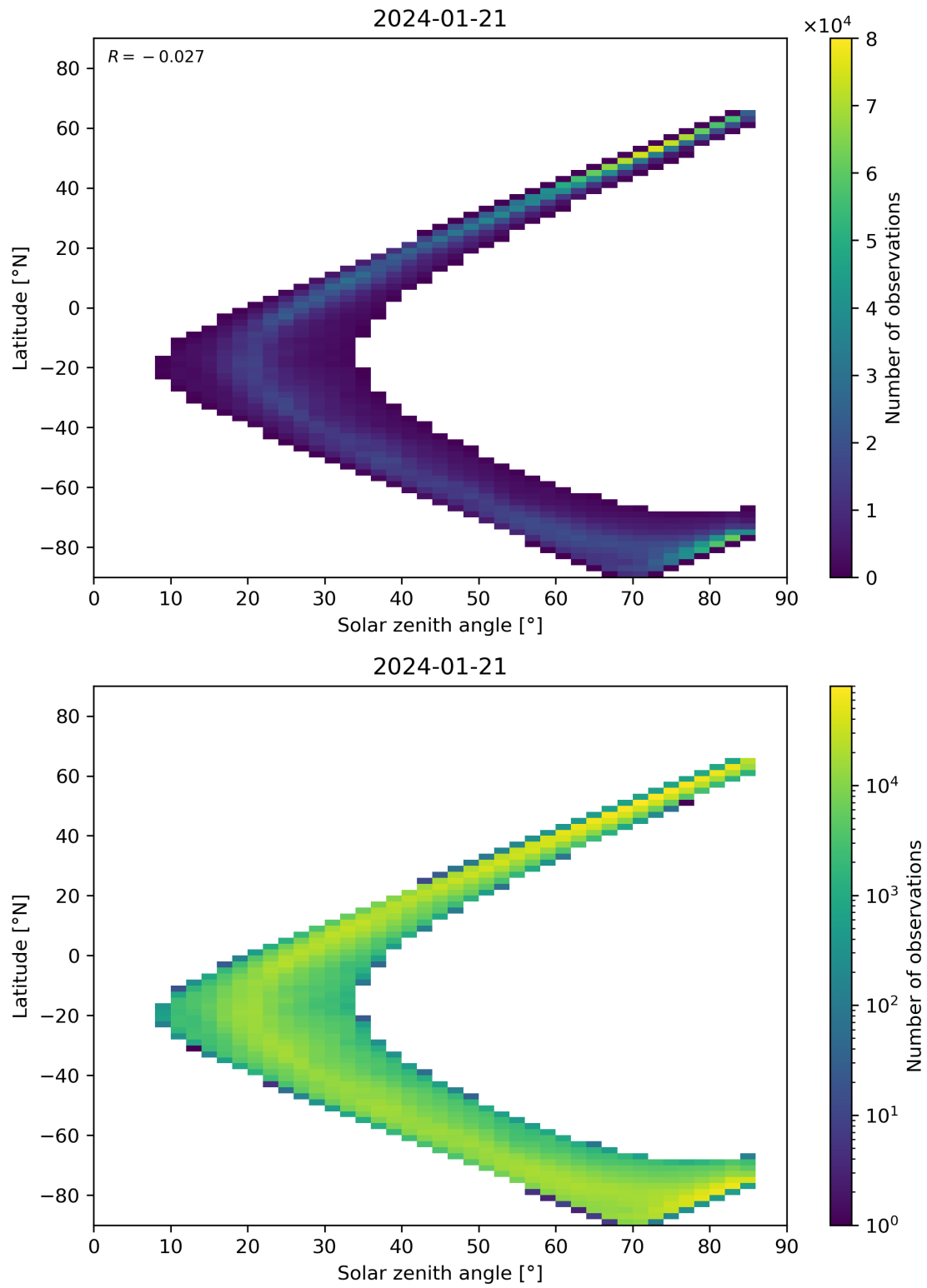
Figure 66: Scatter density plot of “Solar zenith angle” against “Latitude” for 2024-01-21 to 2024-01-22.
