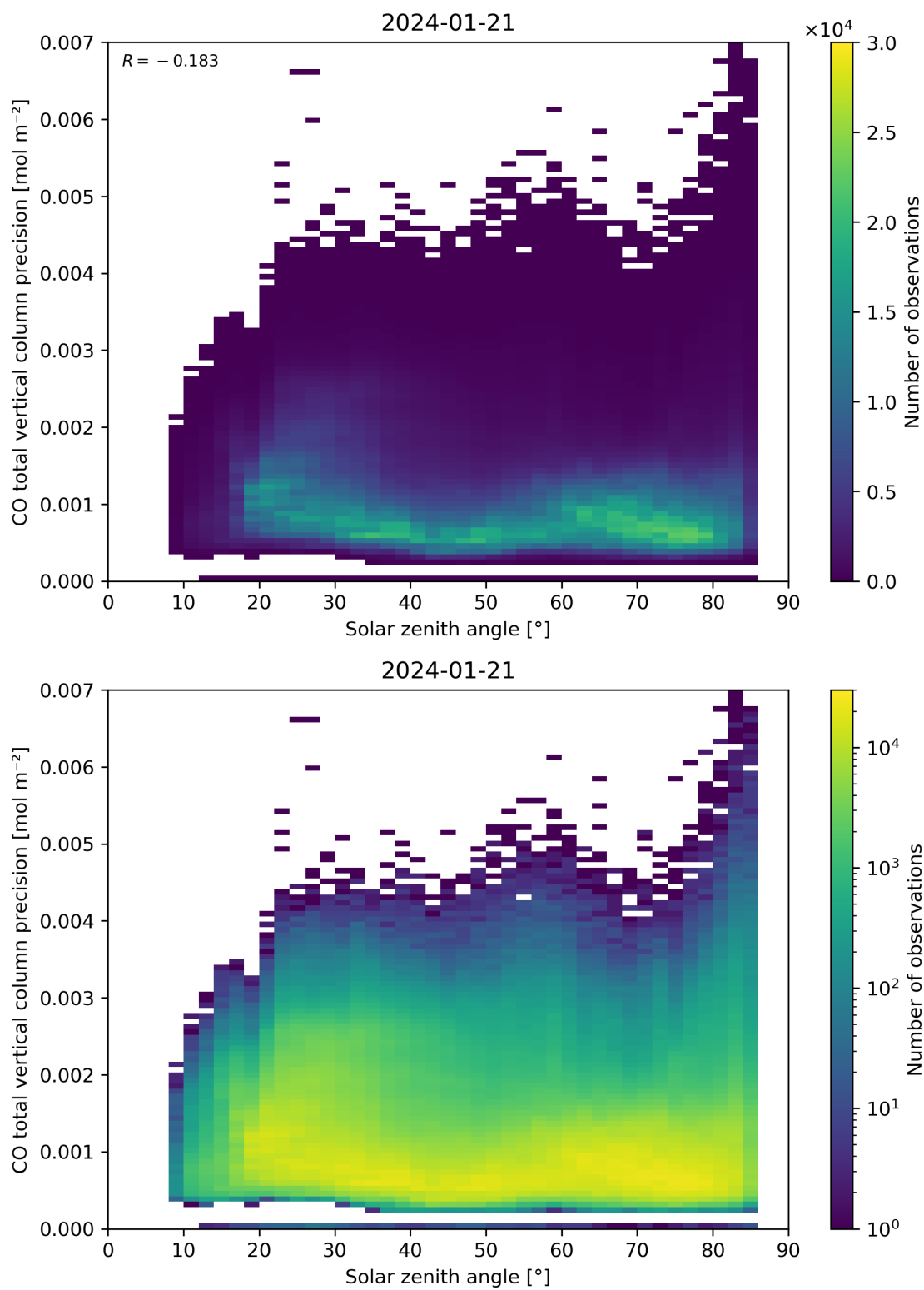
Figure 63: Scatter density plot of “Solar zenith angle” against “CO total vertical column precision” for 2024-01-21 to 2024-01-22.
