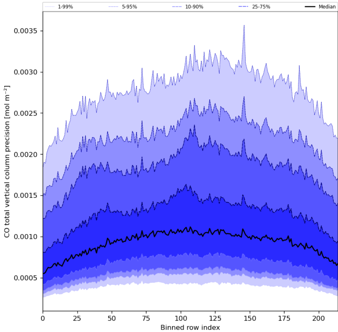
Figure 28: Along track statistics of “CO total vertical column precision” for 2024-01-21 to 2024-01-22
