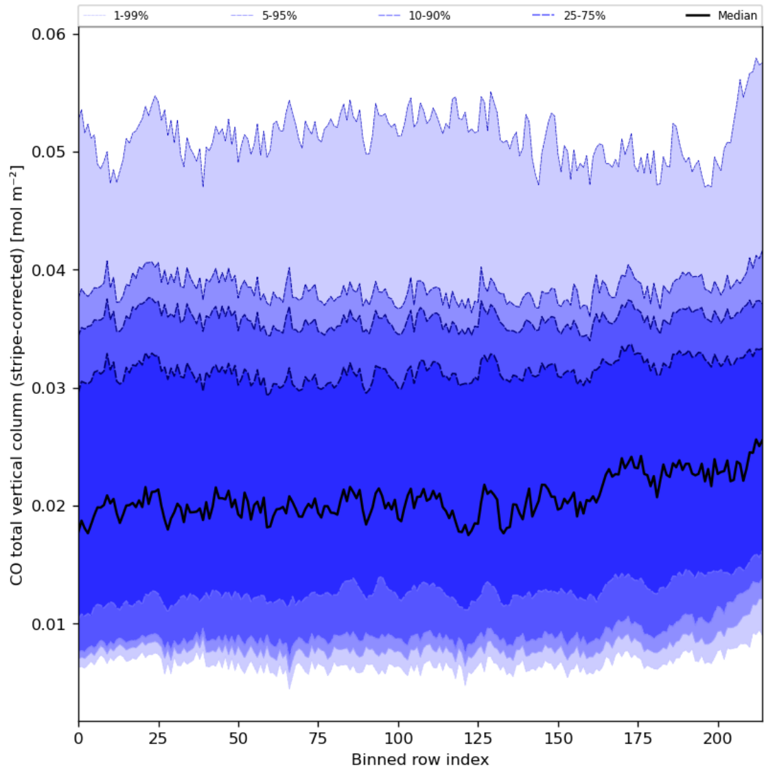
Figure 27: Along track statistics of “CO total vertical column (stripe-corrected)” for 2024-01-21 to 2024-01-23
