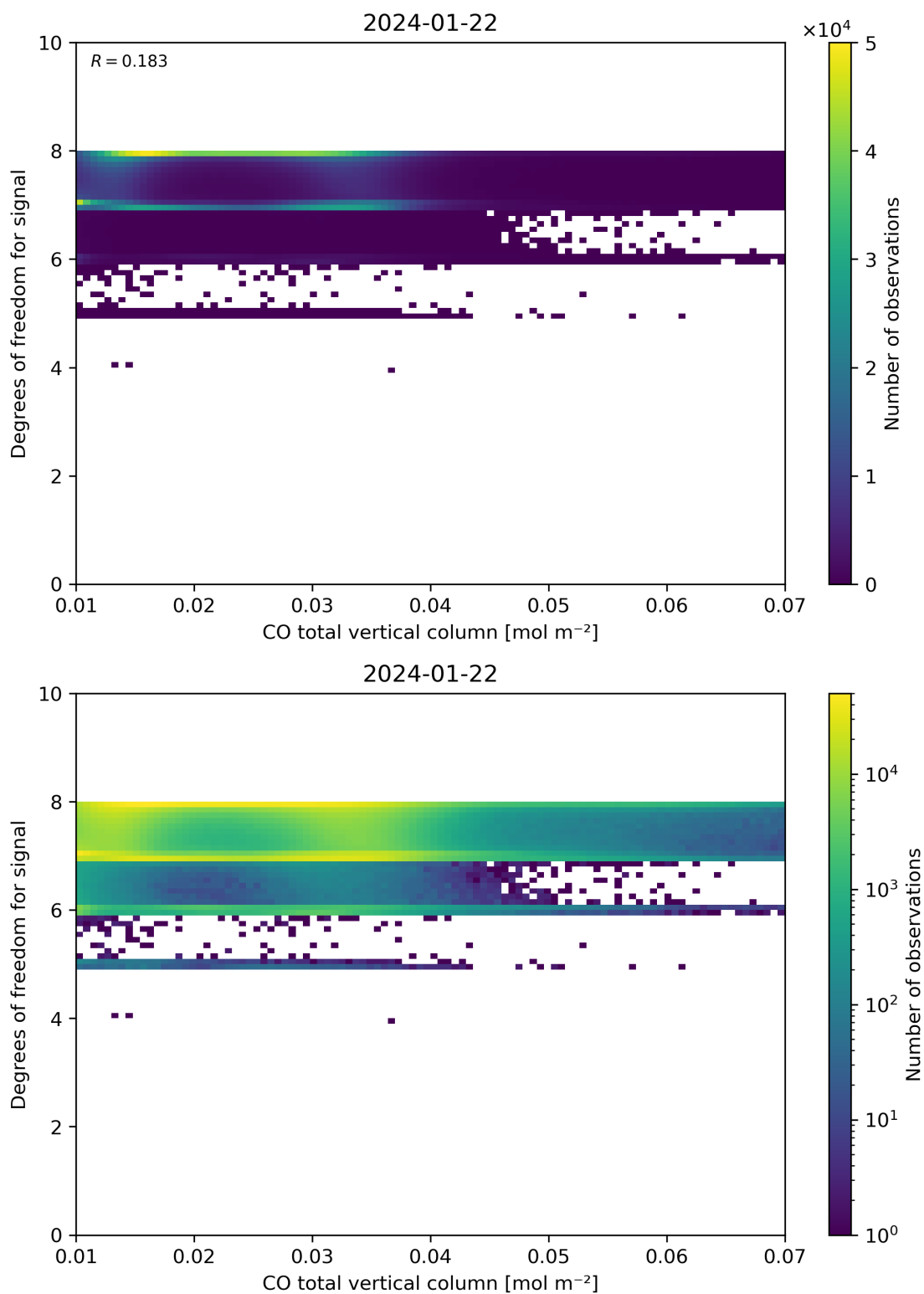
Figure 41: Scatter density plot of “CO total vertical column” against “Degrees of freedom for signal” for 2024-01-21 to 2024-01-23.
