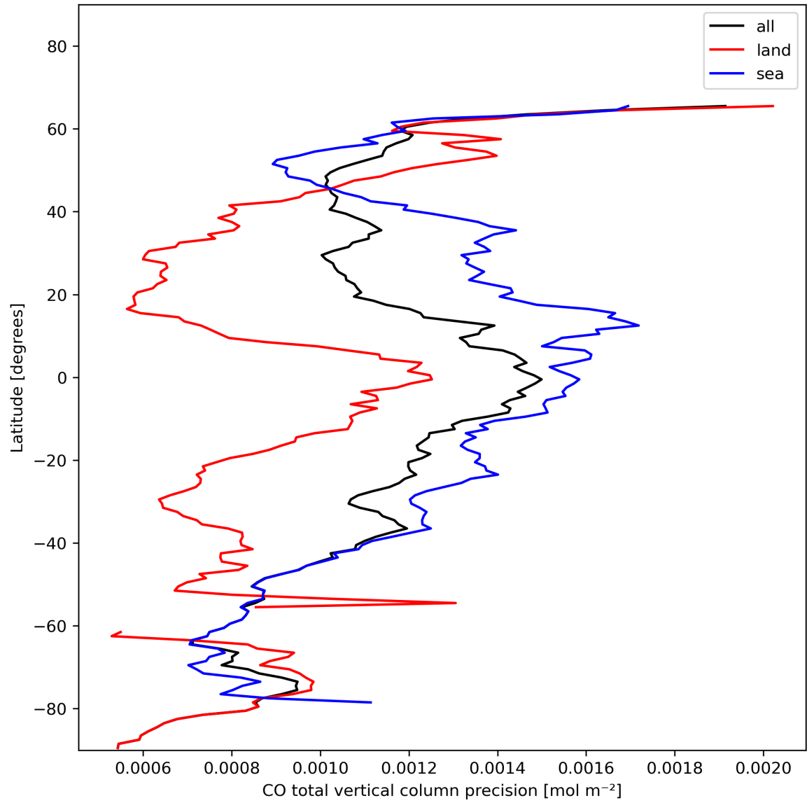
Figure 12: Zonal average of “CO total vertical column precision” for 2024-01-21 to 2024-01-23.
