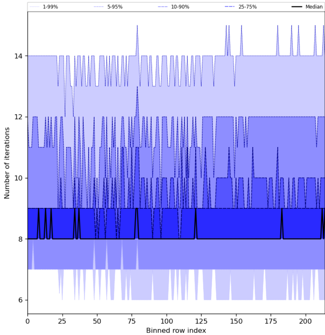
Figure 32: Along track statistics of “Number of iterations” for 2024-01-21 to 2024-01-23
