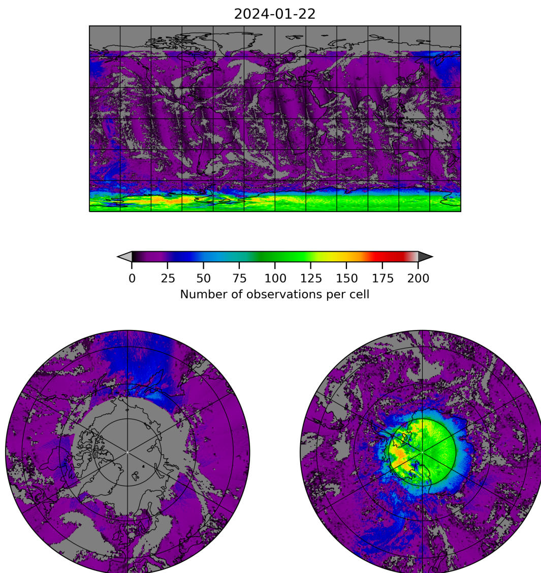
Figure 8: Map of the number of observations for 2024-01-21 to 2024-01-23
