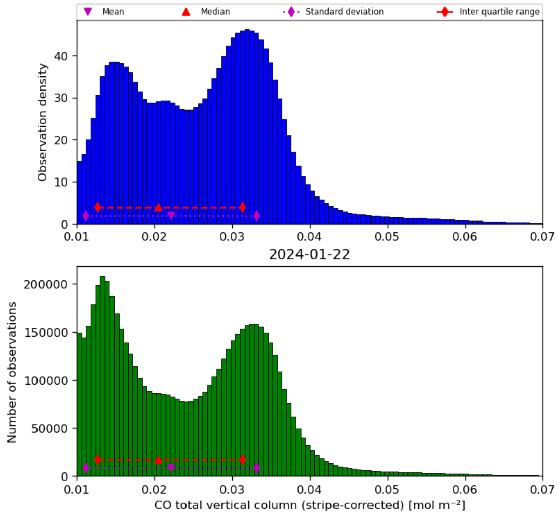
Figure 19: Histogram of “CO total vertical column (stripe-corrected)” for 2024-01-21 to 2024-01-23
