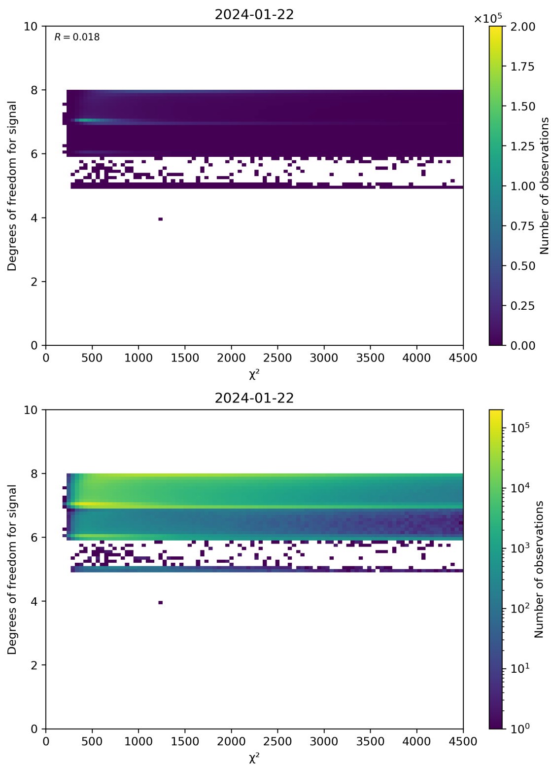
Figure 48: Scatter density plot of “ \chi^2 ” against “Degrees of freedom for signal” for 2024-01-21 to 2024-01-23.
