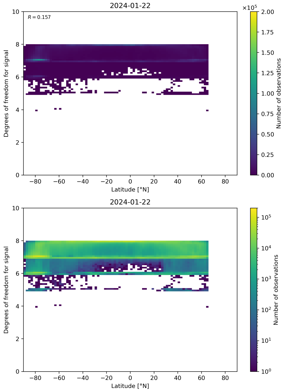
Figure 55: Scatter density plot of “Latitude” against “Degrees of freedom for signal” for 2024-01-21 to 2024-01-23.
