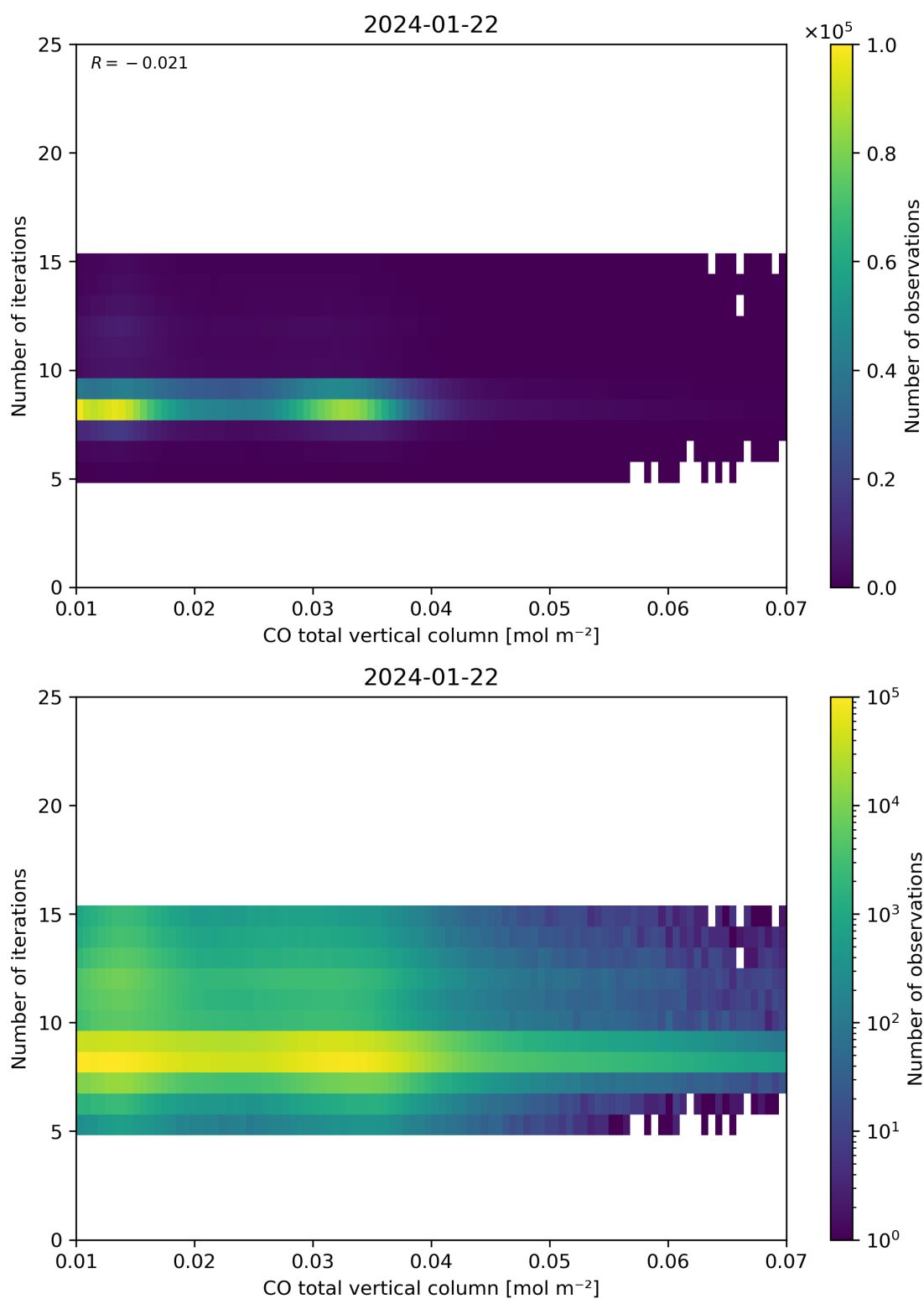
Figure 42: Scatter density plot of “CO total vertical column” against “Number of iterations” for 2024-01-21 to 2024-01-23.
