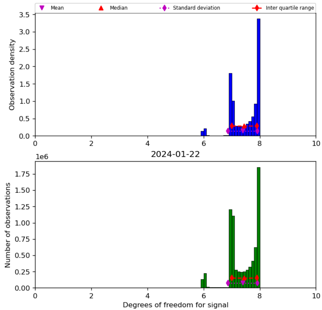
Figure 23: Histogram of “Degrees of freedom for signal” for 2024-01-21 to 2024-01-23
