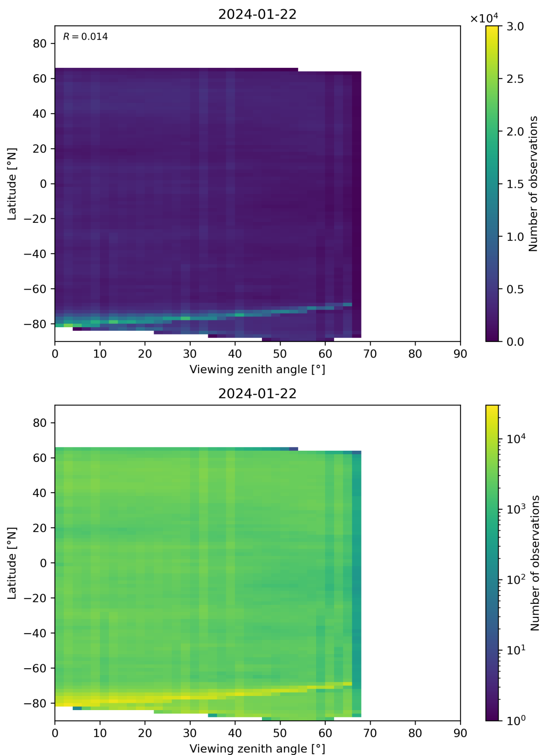
Figure 74: Scatter density plot of “Viewing zenith angle” against “Latitude” for 2024-01-21 to 2024-01-23.
