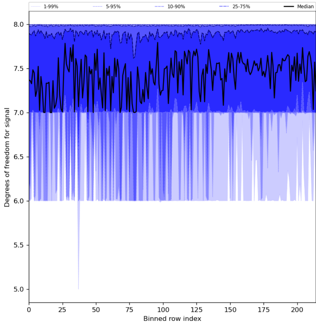
Figure 31: Along track statistics of “Degrees of freedom for signal” for 2024-01-21 to 2024-01-23
