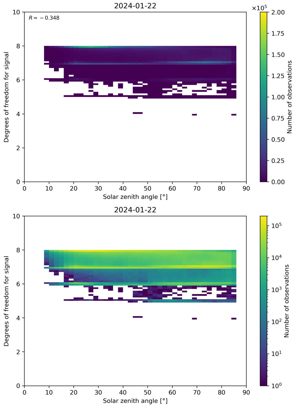
Figure 65: Scatter density plot of “Solar zenith angle” against “Degrees of freedom for signal” for 2024-01-21 to 2024-01-23.
