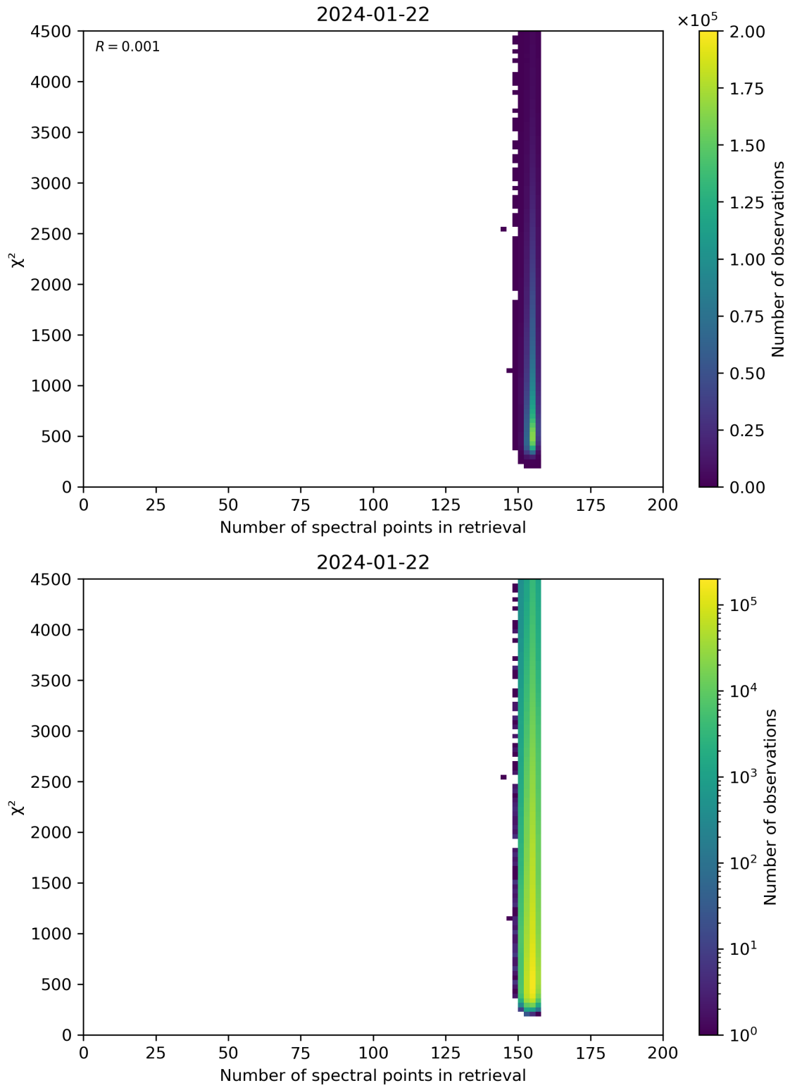
Figure 58: Scatter density plot of “Number of spectral points in retrieval” against “ \chi^2 ” for 2024-01-21 to 2024-01-23.
