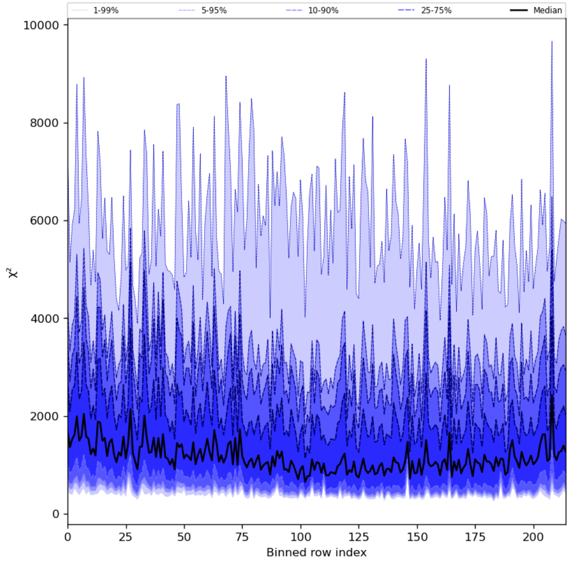
Figure 30: Along track statistics of “ \chi^2 ” for 2024-01-21 to 2024-01-23
