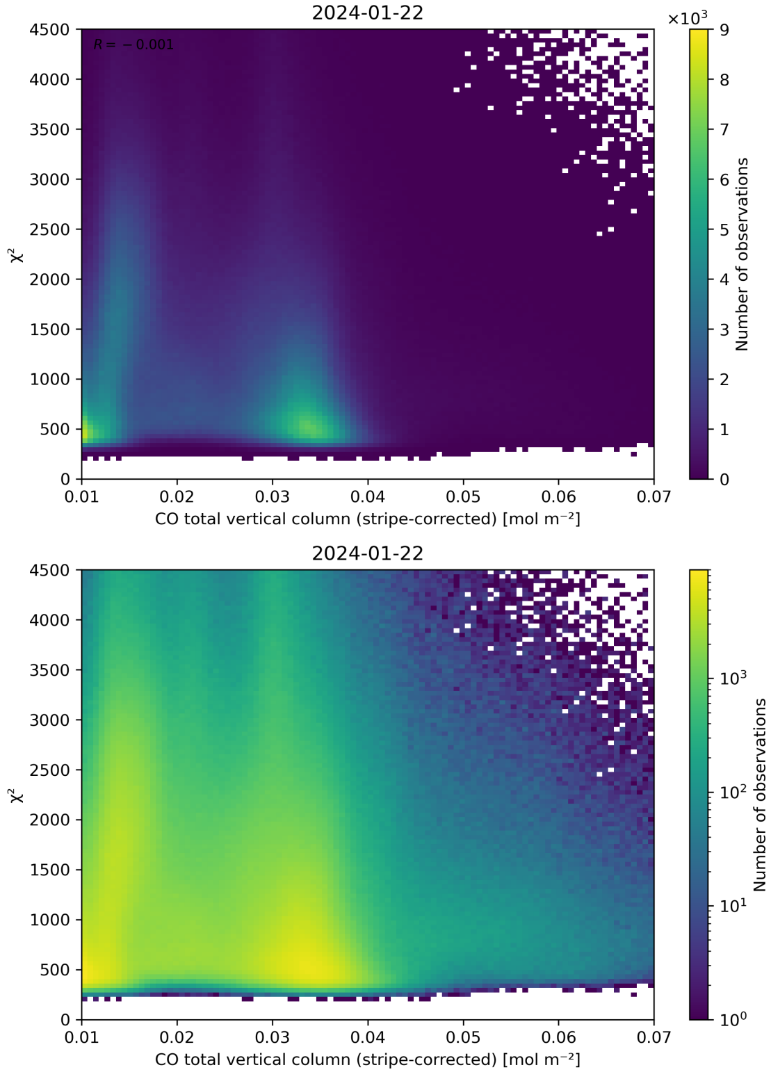
Figure 37: Scatter density plot of “CO total vertical column (stripe-corrected)” against “ \chi^2 ” for 2024-01-21 to 2024-01-23.
