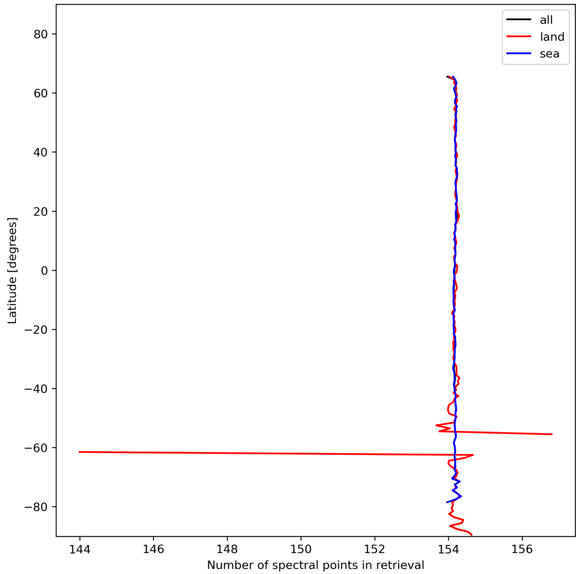
Figure 13: Zonal average of “Number of spectral points in retrieval” for 2024-01-21 to 2024-01-23.
