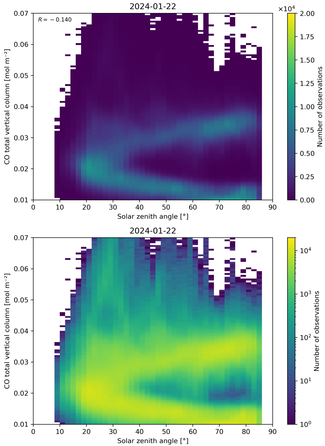
Figure 61: Scatter density plot of “Solar zenith angle” against “CO total vertical column” for 2024-01-21 to 2024-01-23.
