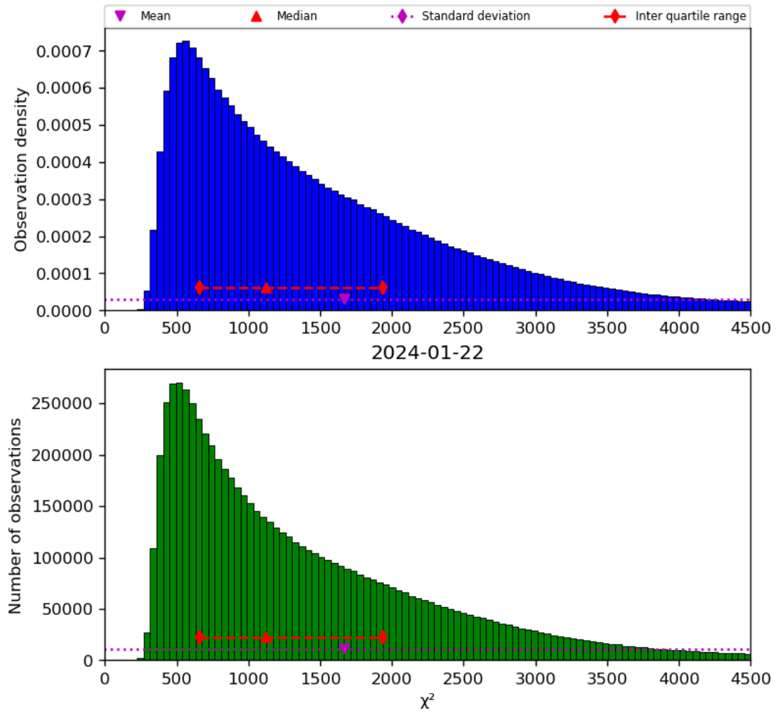
Figure 22: Histogram of “ \chi^2 ” for 2024-01-21 to 2024-01-23
