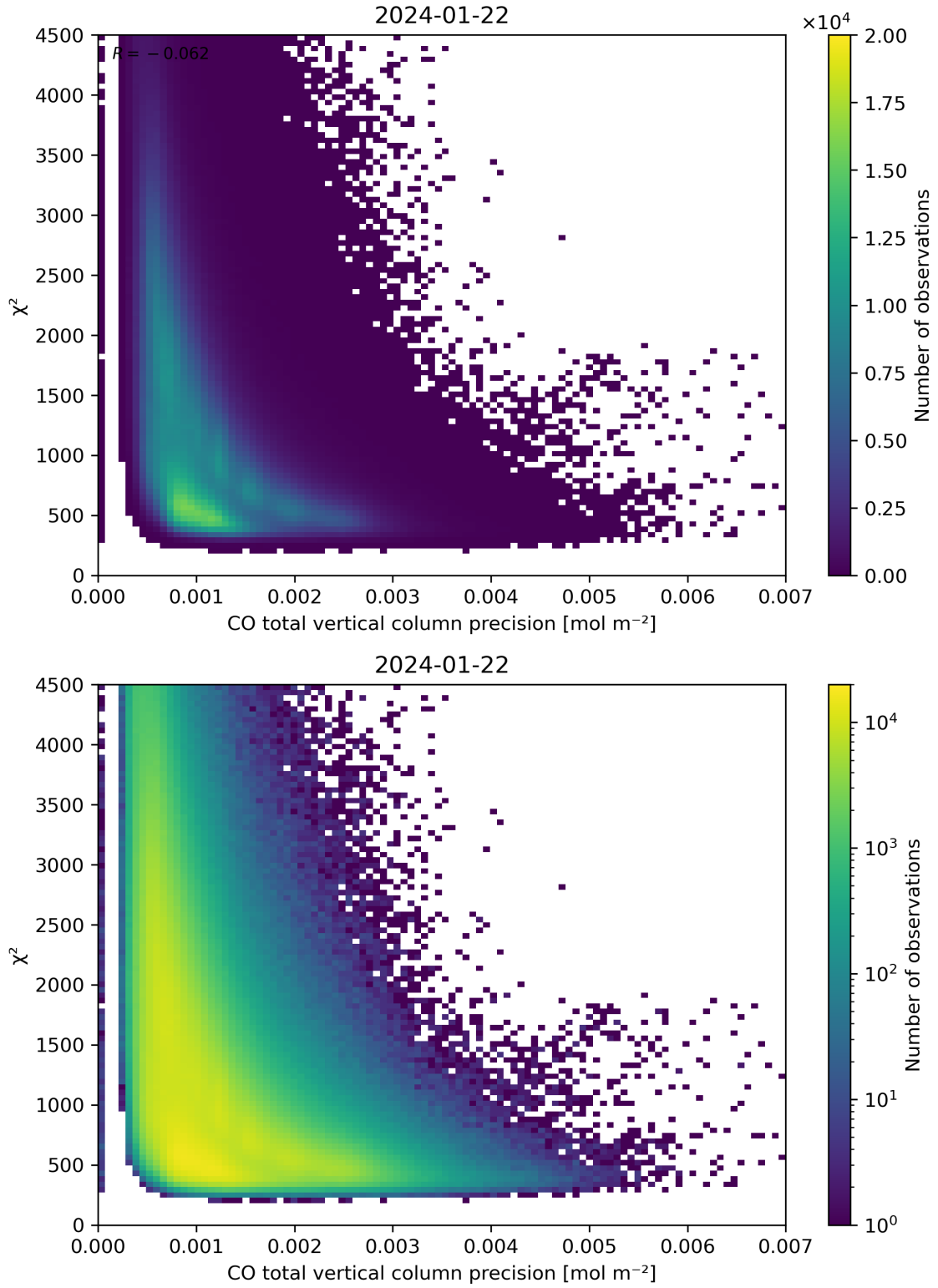
Figure 44: Scatter density plot of “CO total vertical column precision” against “ \chi^2 ” for 2024-01-21 to 2024-01-23.
