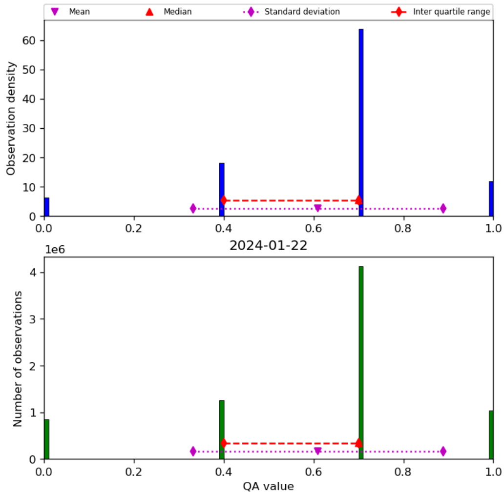
Figure 17: Histogram of “QA value” for 2024-01-21 to 2024-01-23
