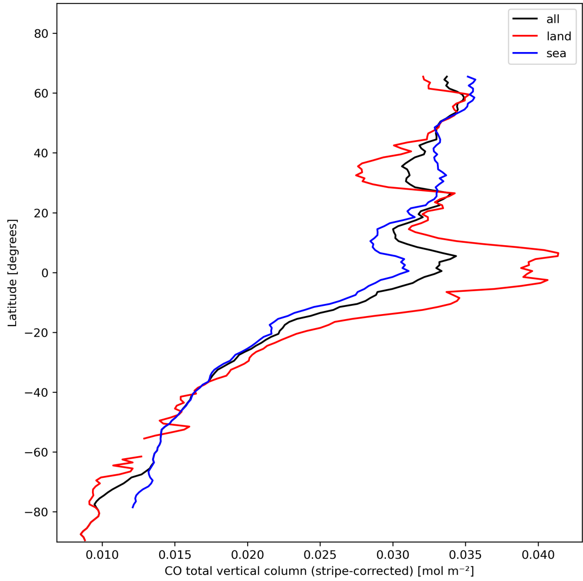
Figure 11: Zonal average of “CO total vertical column (stripe-corrected)” for 2024-01-21 to 2024-01-23.
