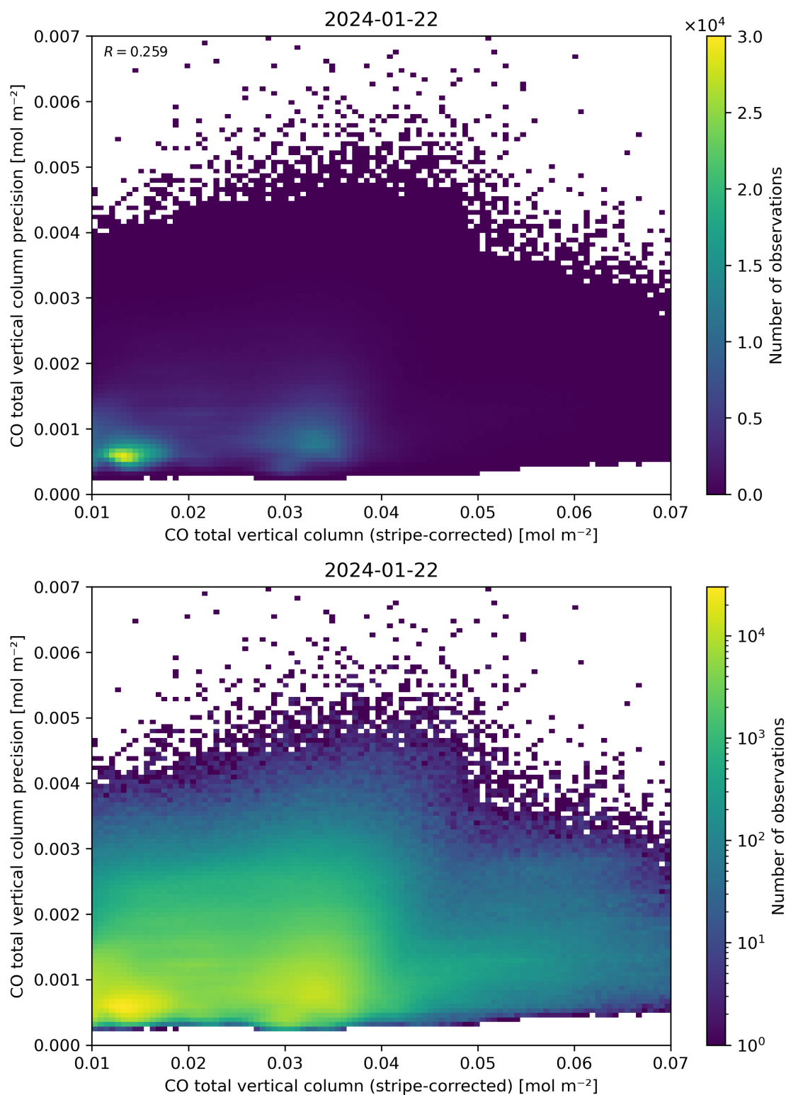
Figure 36: Scatter density plot of “CO total vertical column (stripe-corrected)” against “CO total vertical column precision” for 2024-01-21 to 2024-01-23.
