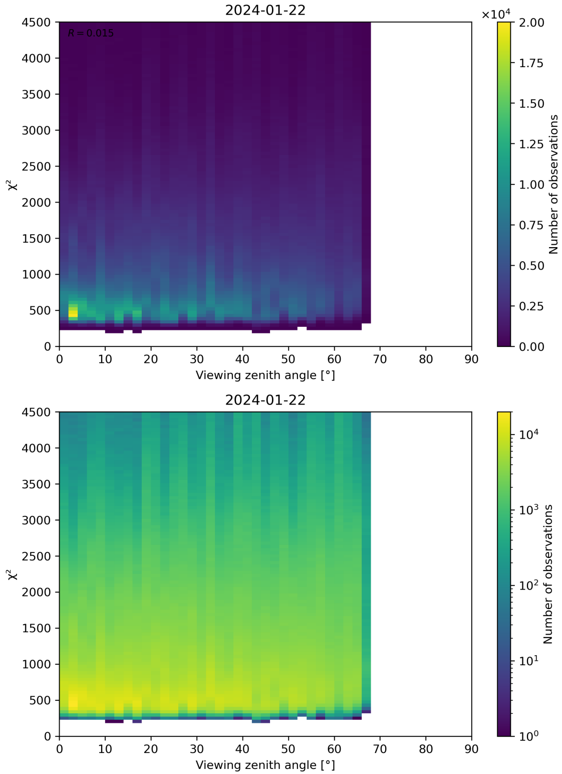
Figure 72: Scatter density plot of “Viewing zenith angle” against “ \chi^2 ” for 2024-01-21 to 2024-01-23.
