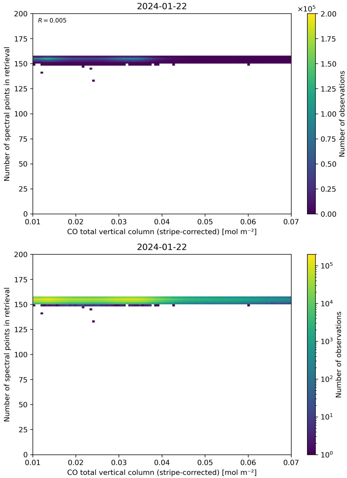
Figure 40: Scatter density plot of “CO total vertical column (stripe-corrected)” against “Number of spectral points in retrieval” for 2024-01-21 to 2024-01-23.
