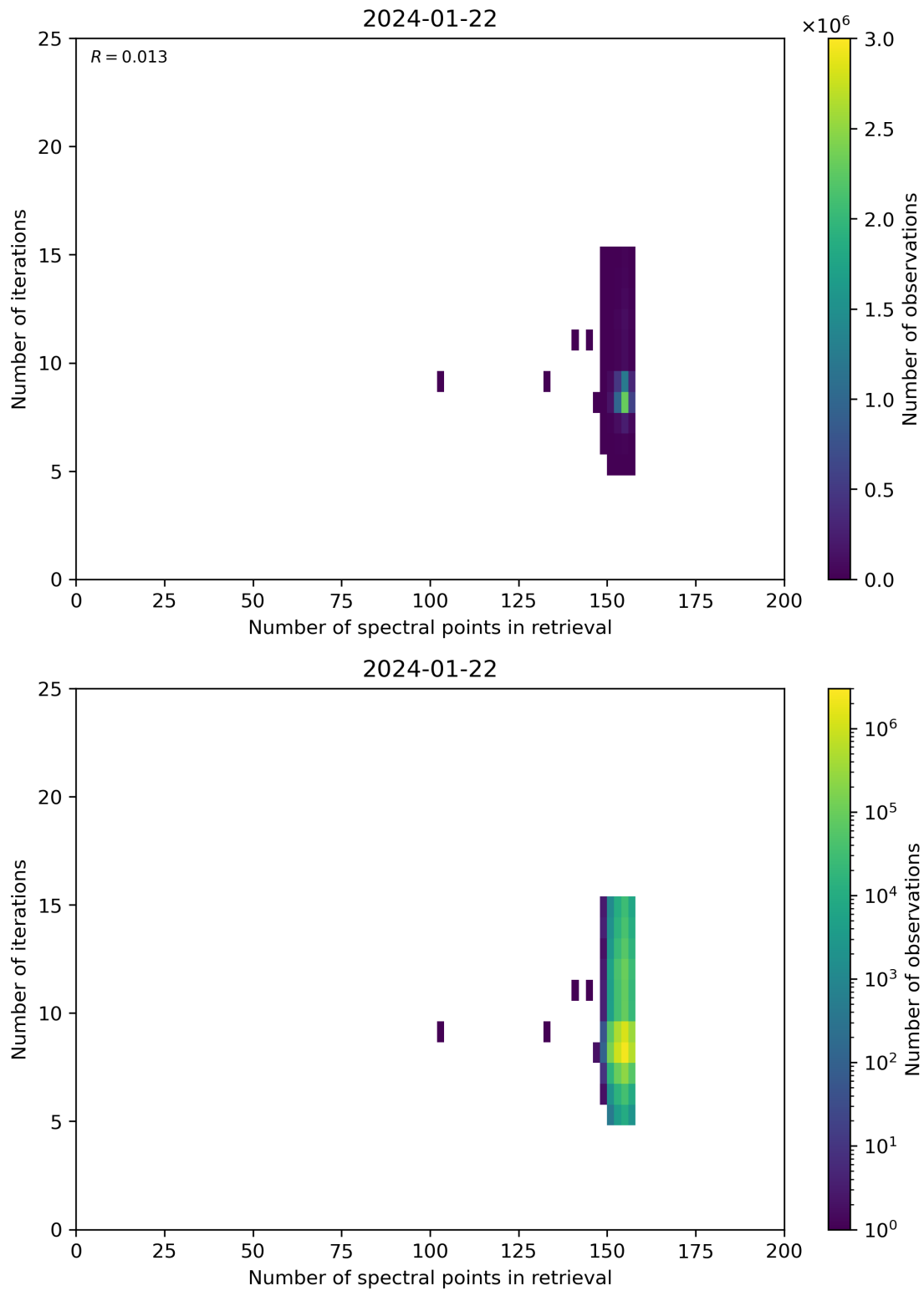
Figure 60: Scatter density plot of “Number of spectral points in retrieval” against “Number of iterations” for 2024-01-21 to 2024-01-23.
