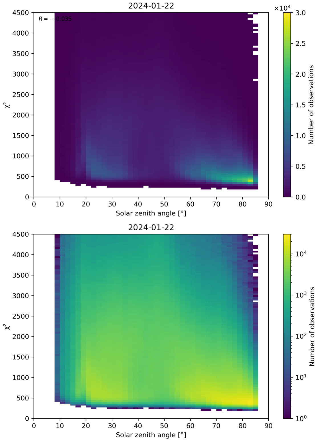
Figure 64: Scatter density plot of “Solar zenith angle” against “ \chi^2 ” for 2024-01-21 to 2024-01-23.
