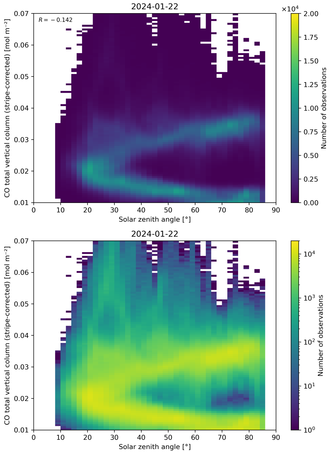
Figure 62: Scatter density plot of “Solar zenith angle” against “CO total vertical column (stripe-corrected)” for 2024-01-21 to 2024-01-23.
