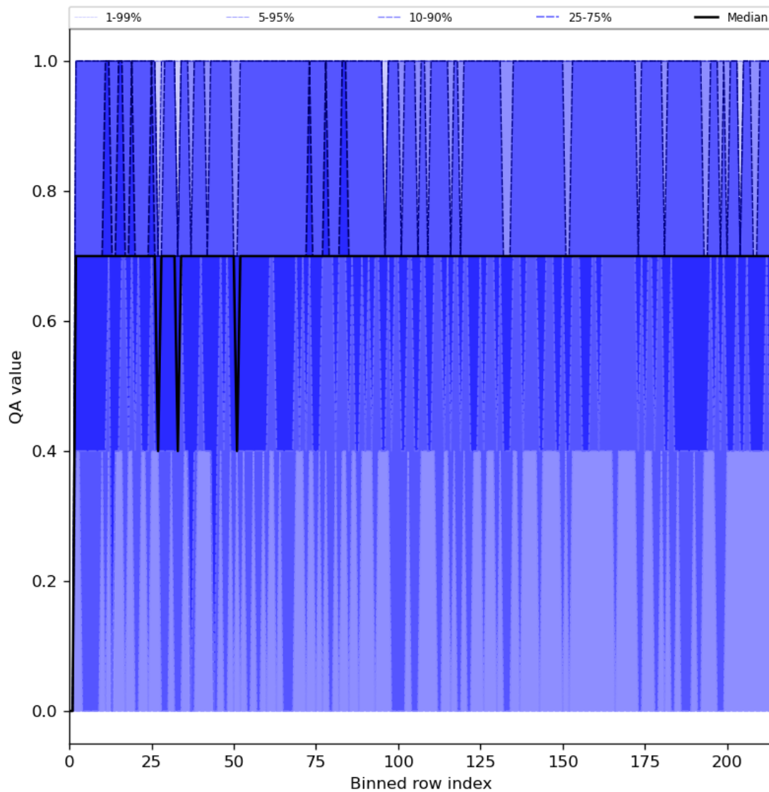
Figure 25: Along track statistics of “QA value” for 2024-01-21 to 2024-01-23
