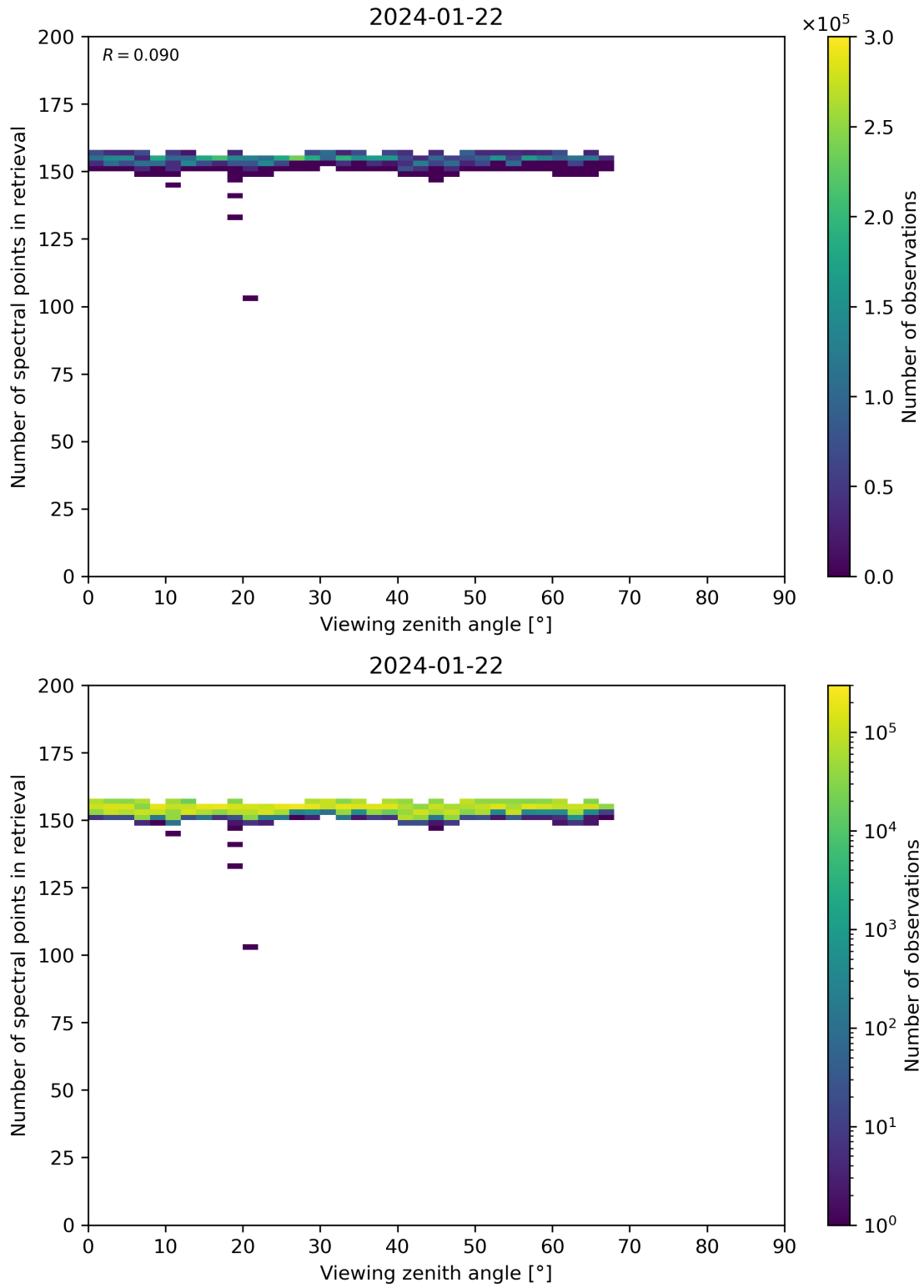
Figure 76: Scatter density plot of “Viewing zenith angle” against “Number of spectral points in retrieval” for 2024-01-21 to 2024-01-23.
