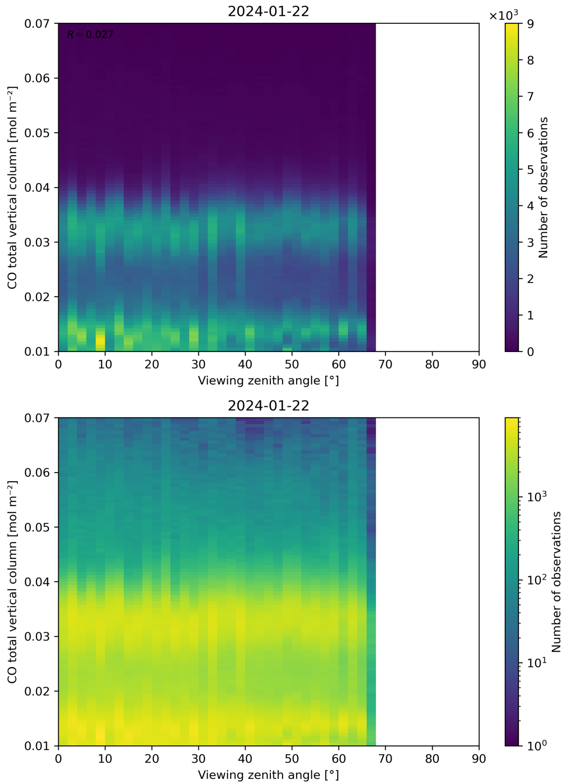
Figure 69: Scatter density plot of “Viewing zenith angle” against “CO total vertical column” for 2024-01-21 to 2024-01-23.
