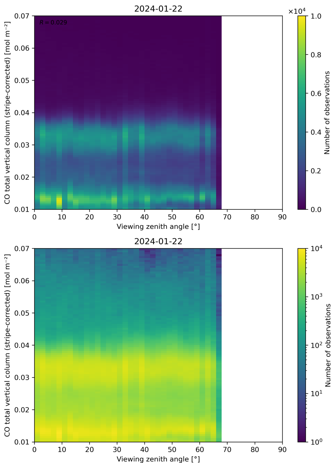
Figure 70: Scatter density plot of “Viewing zenith angle” against “CO total vertical column (stripe-corrected)” for 2024-01-21 to 2024-01-23.
