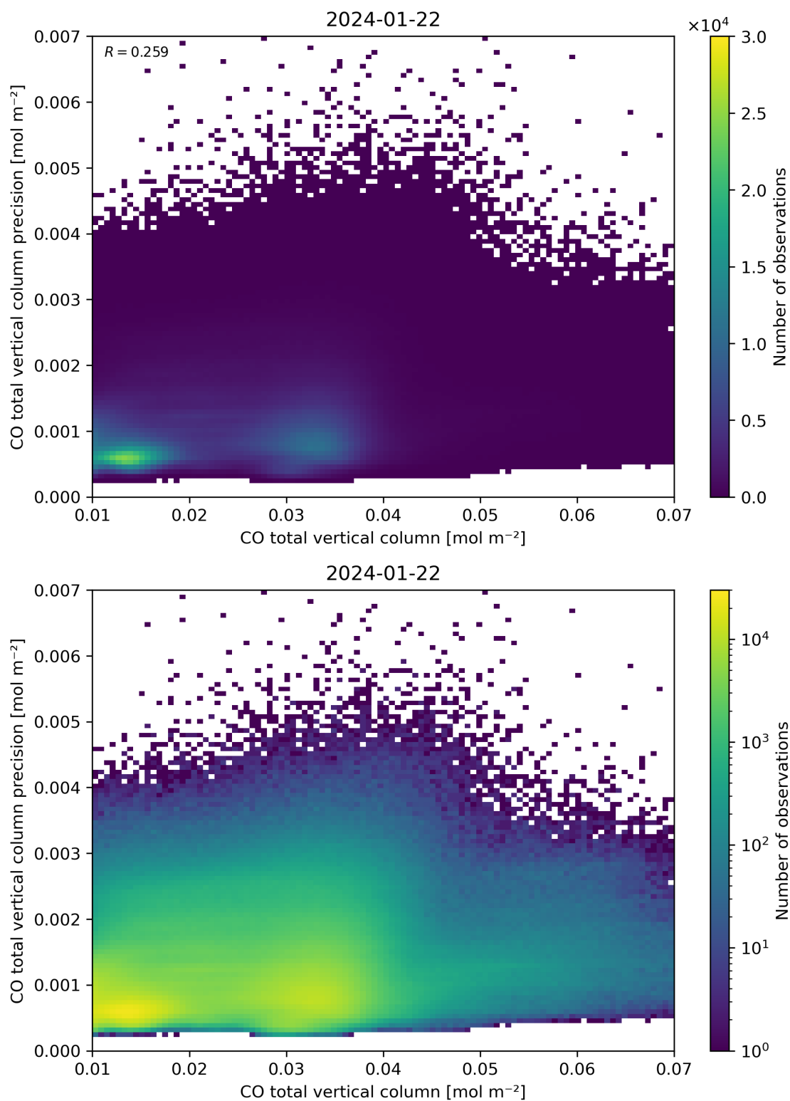
Figure 34: Scatter density plot of “CO total vertical column” against “CO total vertical column precision” for 2024-01-21 to 2024-01-23.
