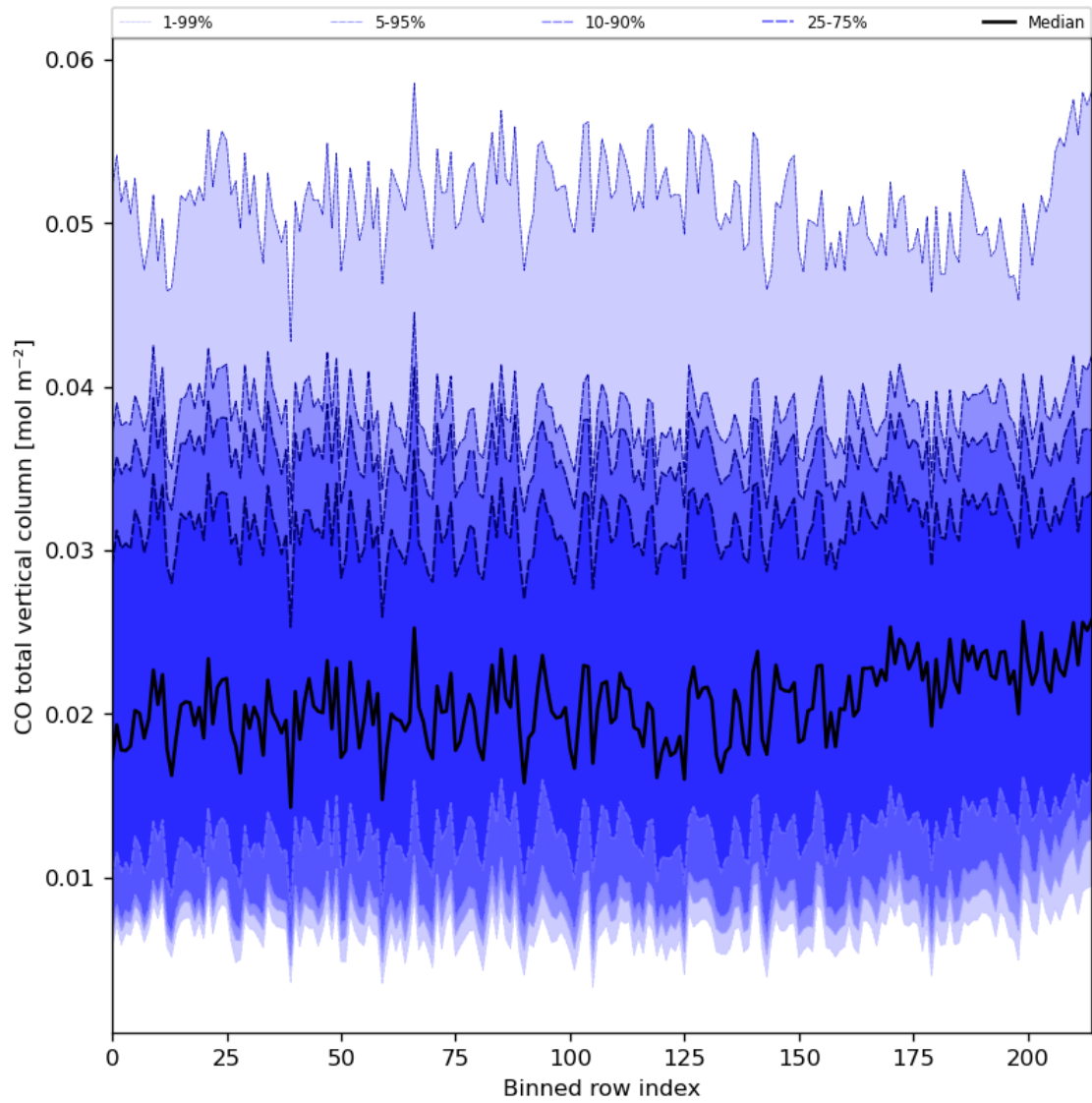
Figure 26: Along track statistics of “CO total vertical column” for 2024-01-21 to 2024-01-23
