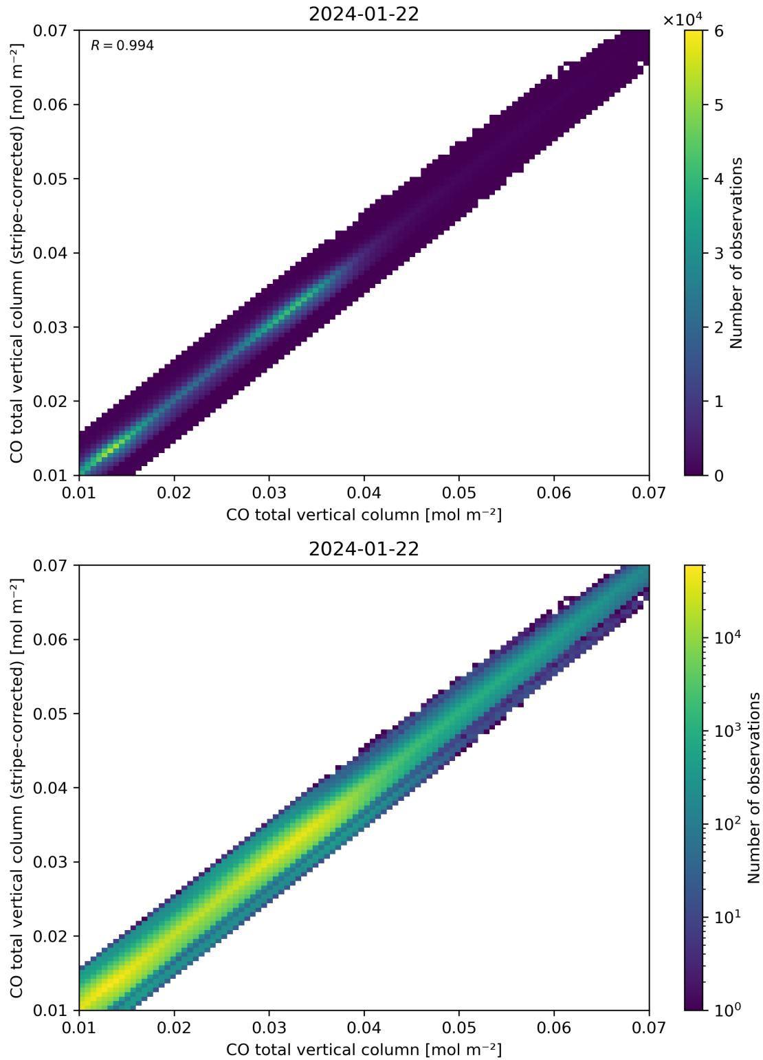
Figure 33: Scatter density plot of “CO total vertical column” against “CO total vertical column (stripe-corrected)” for 2024-01-21 to 2024-01-23.
