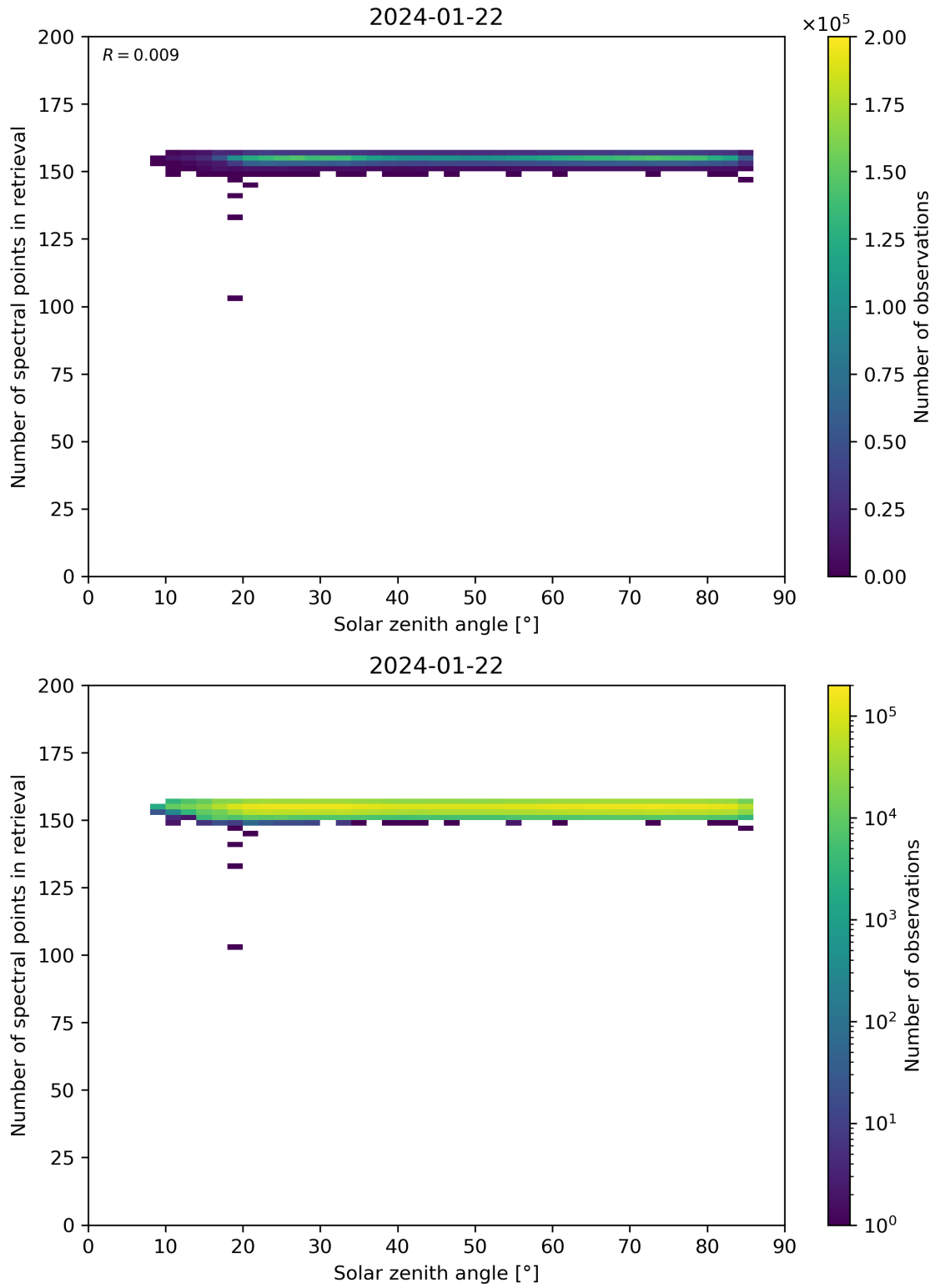
Figure 68: Scatter density plot of “Solar zenith angle” against “Number of spectral points in retrieval” for 2024-01-21 to 2024-01-23.
