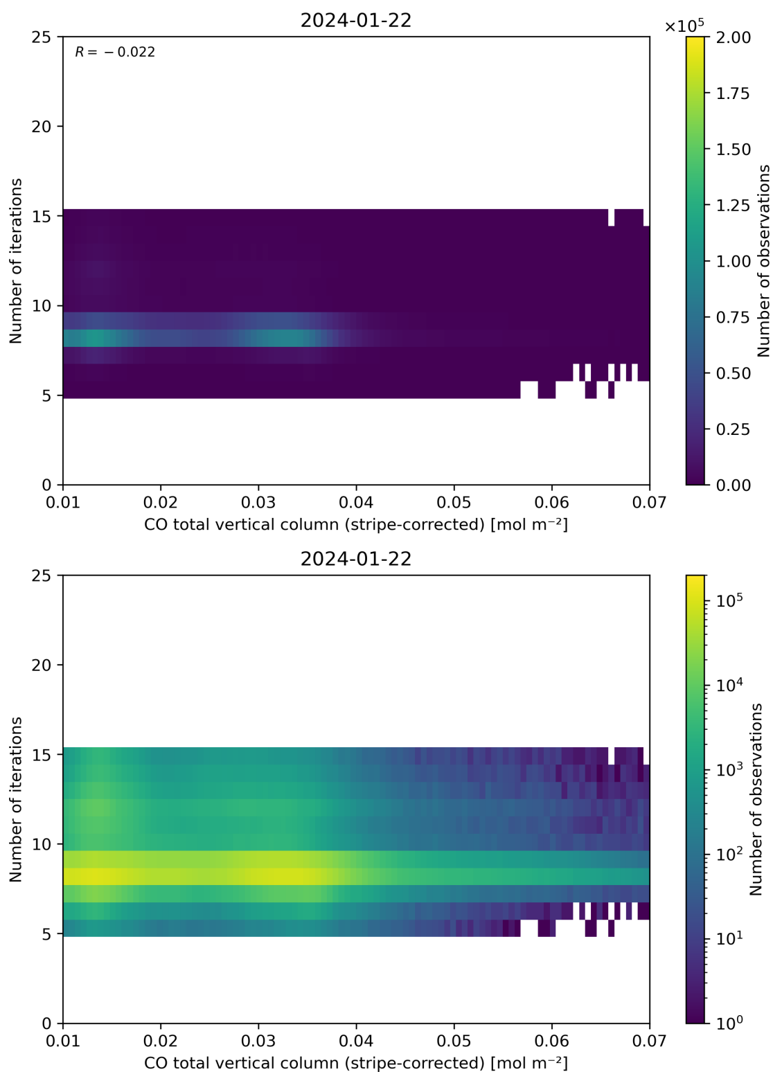
Figure 39: Scatter density plot of “CO total vertical column (stripe-corrected)” against “Number of iterations” for 2024-01-21 to 2024-01-23.
