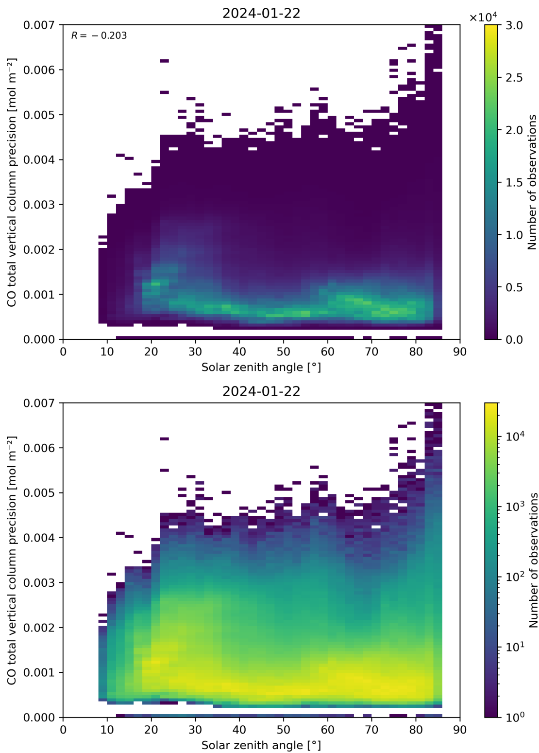
Figure 63: Scatter density plot of “Solar zenith angle” against “CO total vertical column precision” for 2024-01-21 to 2024-01-23.
