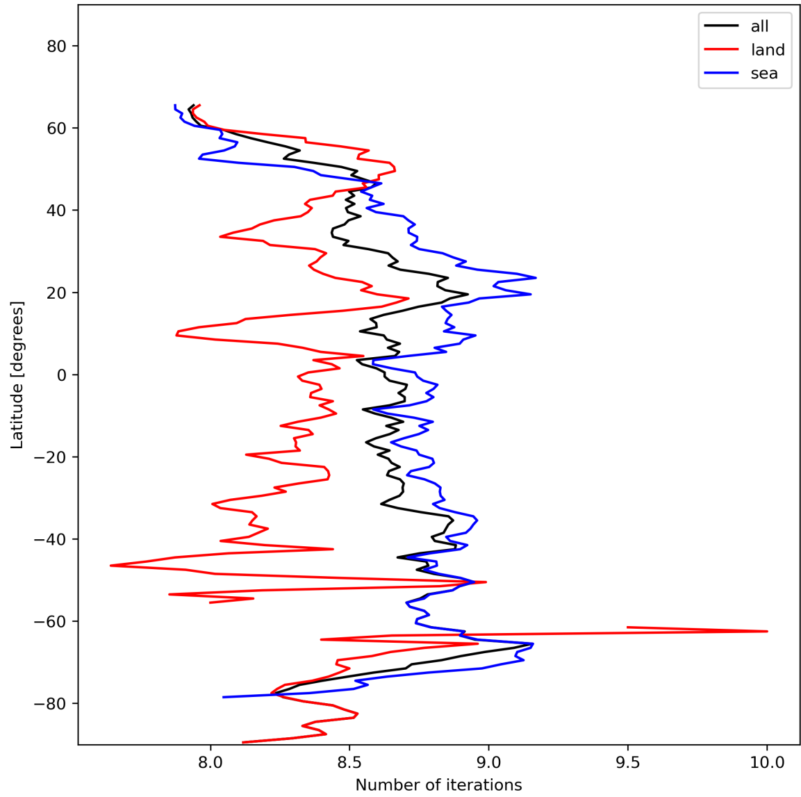
Figure 16: Zonal average of “Number of iterations” for 2024-01-21 to 2024-01-23.
