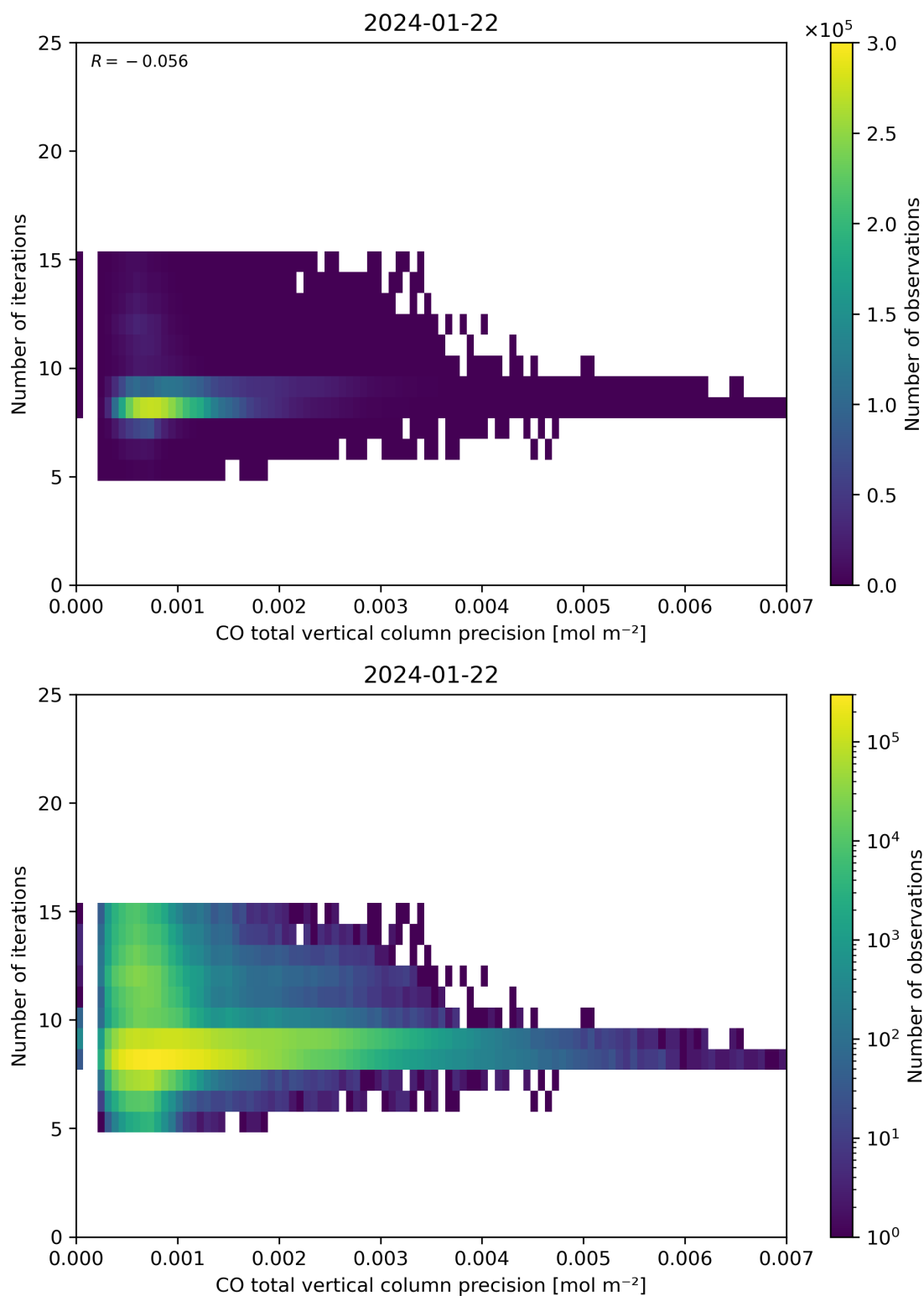
Figure 46: Scatter density plot of “CO total vertical column precision” against “Number of iterations” for 2024-01-21 to 2024-01-23.
