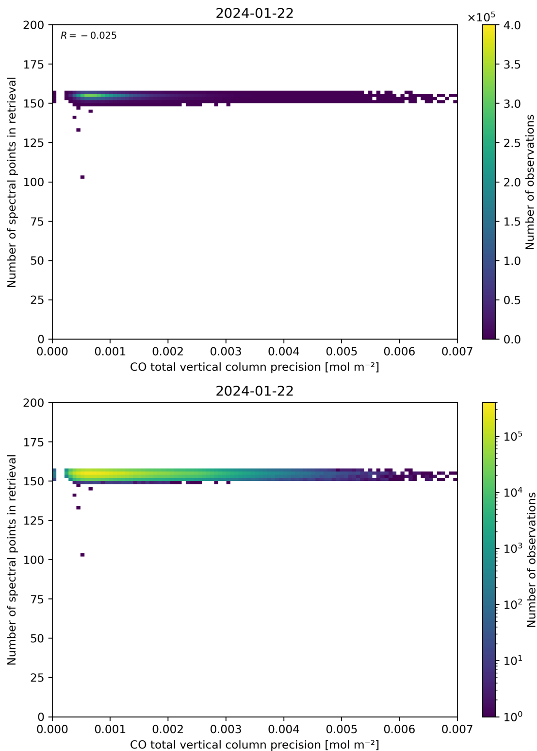
Figure 47: Scatter density plot of “CO total vertical column precision” against “Number of spectral points in retrieval” for 2024-01-21 to 2024-01-23.
