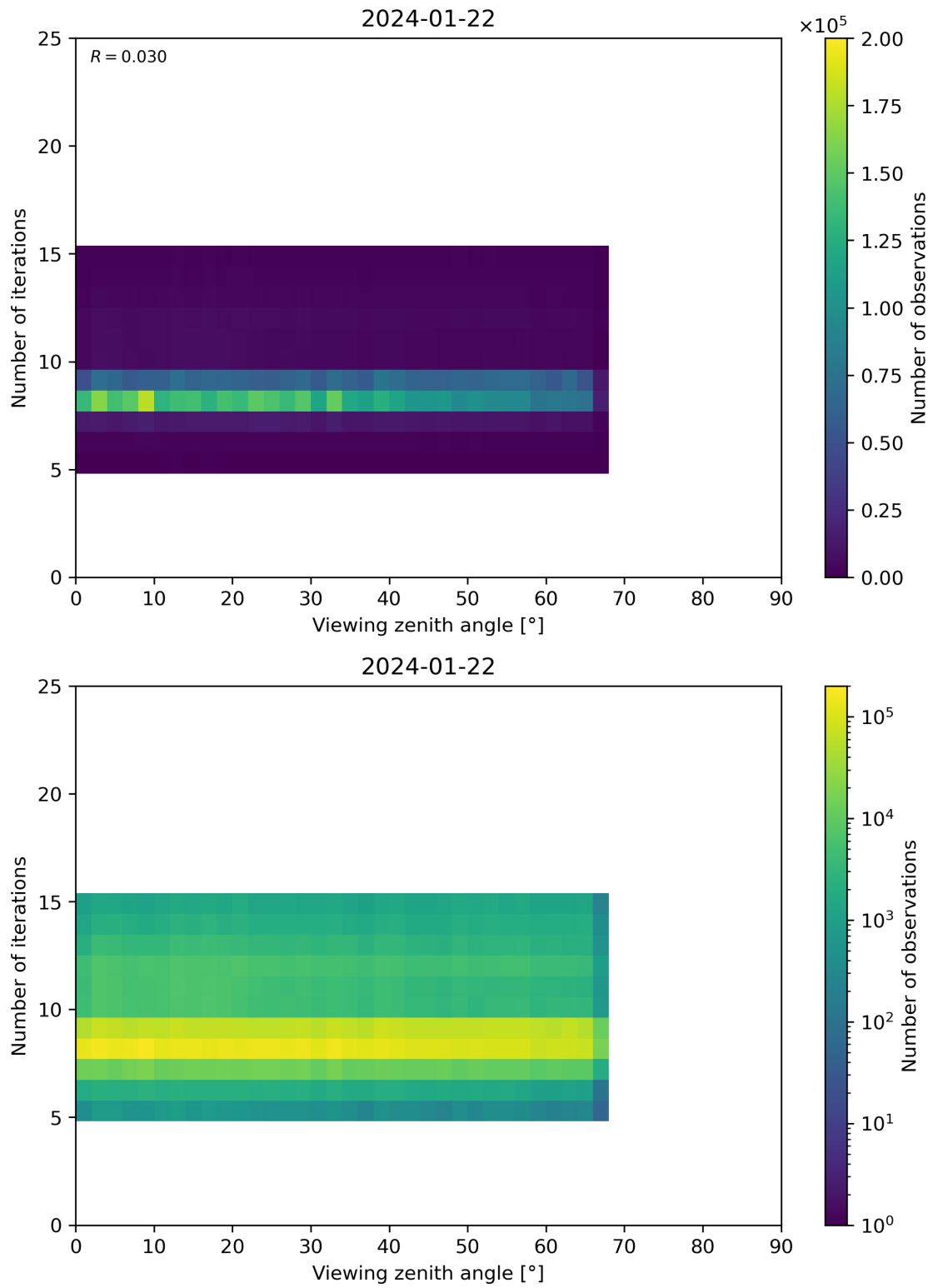
Figure 75: Scatter density plot of “Viewing zenith angle” against “Number of iterations” for 2024-01-21 to 2024-01-23.
