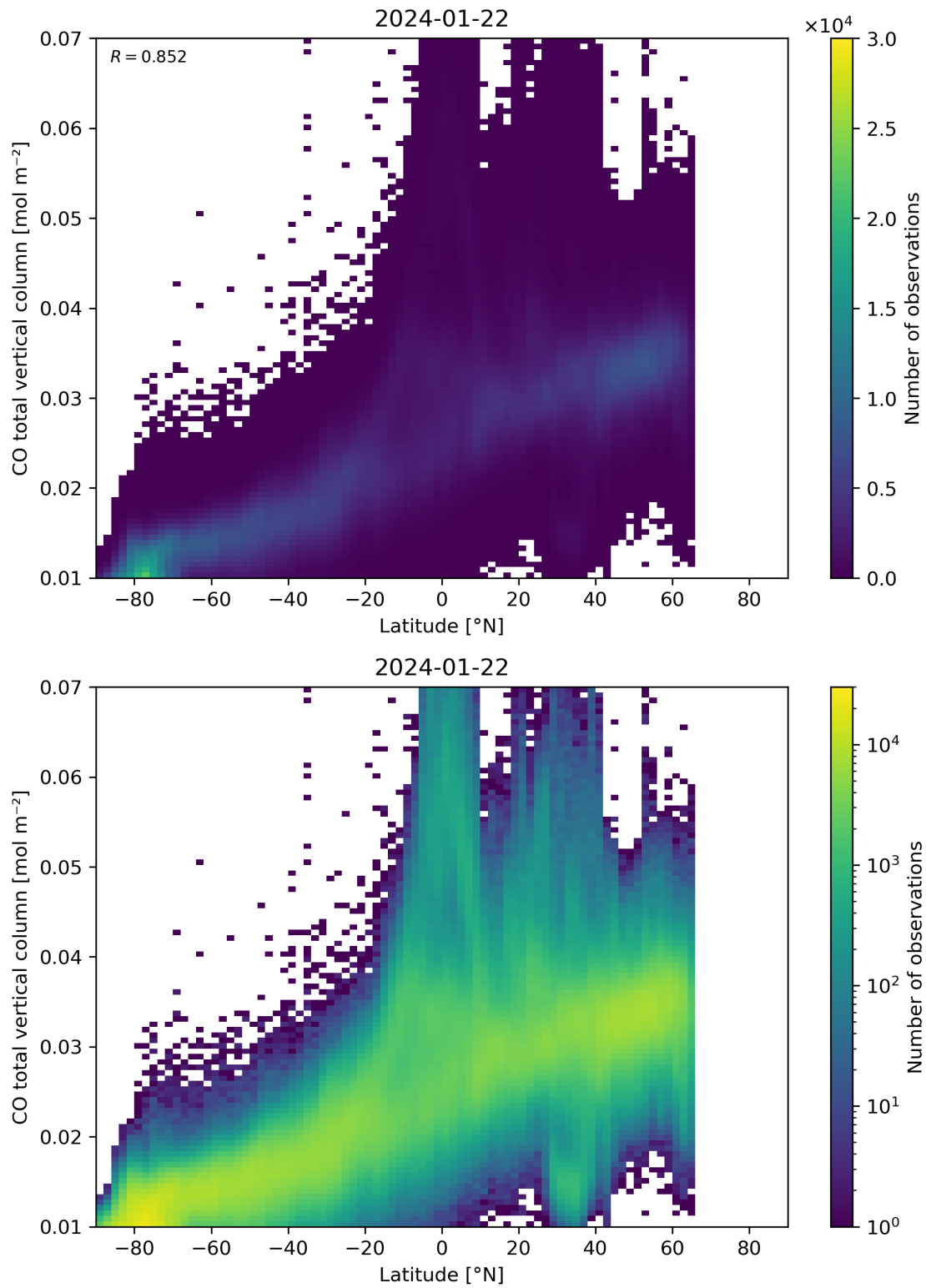
Figure 51: Scatter density plot of “Latitude” against “CO total vertical column” for 2024-01-21 to 2024-01-23.
