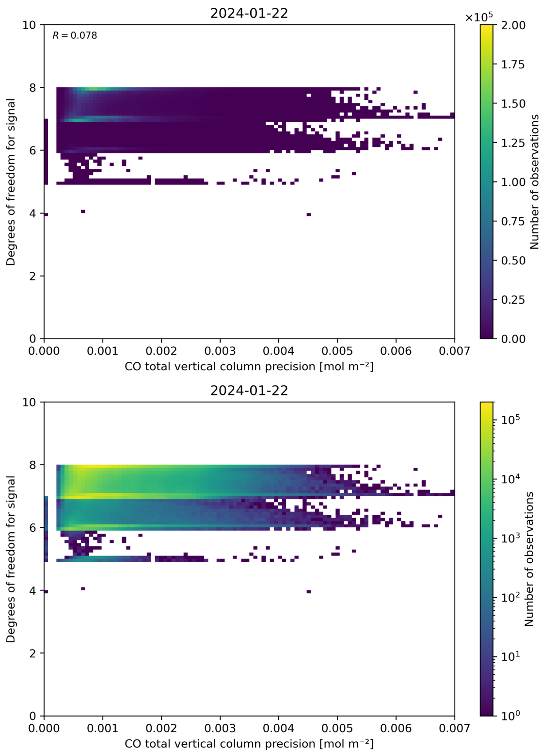
Figure 45: Scatter density plot of “CO total vertical column precision” against “Degrees of freedom for signal” for 2024-01-21 to 2024-01-23.
