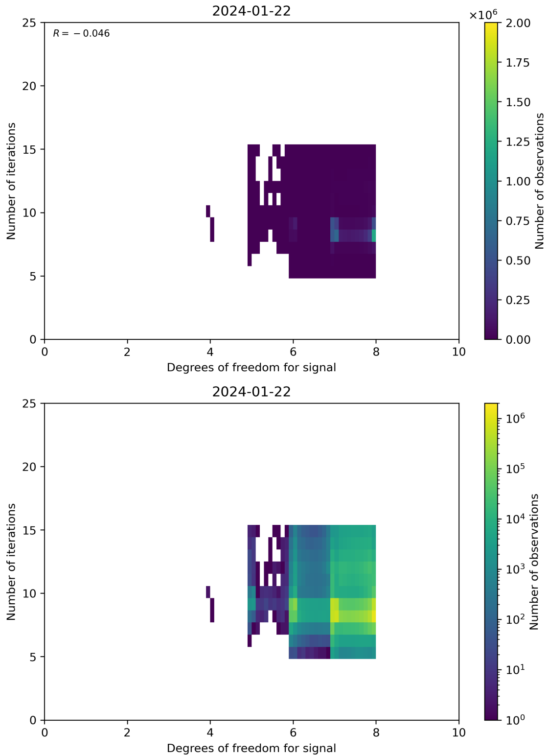
Figure 50: Scatter density plot of “Degrees of freedom for signal” against “Number of iterations” for 2024-01-21 to 2024-01-23.
