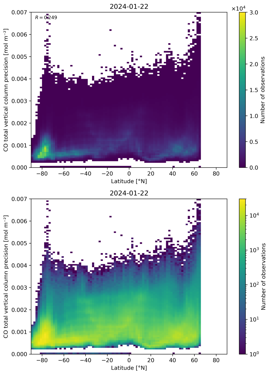
Figure 53: Scatter density plot of “Latitude” against “CO total vertical column precision” for 2024-01-21 to 2024-01-23.
