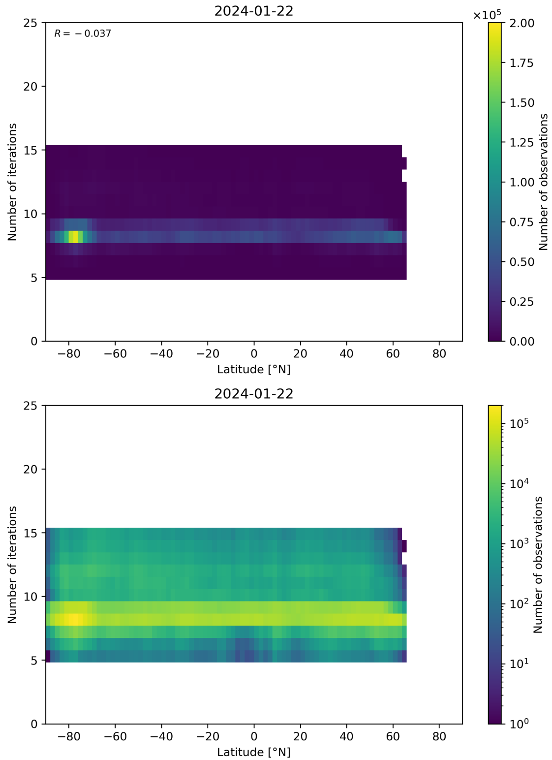
Figure 56: Scatter density plot of “Latitude” against “Number of iterations” for 2024-01-21 to 2024-01-23.
