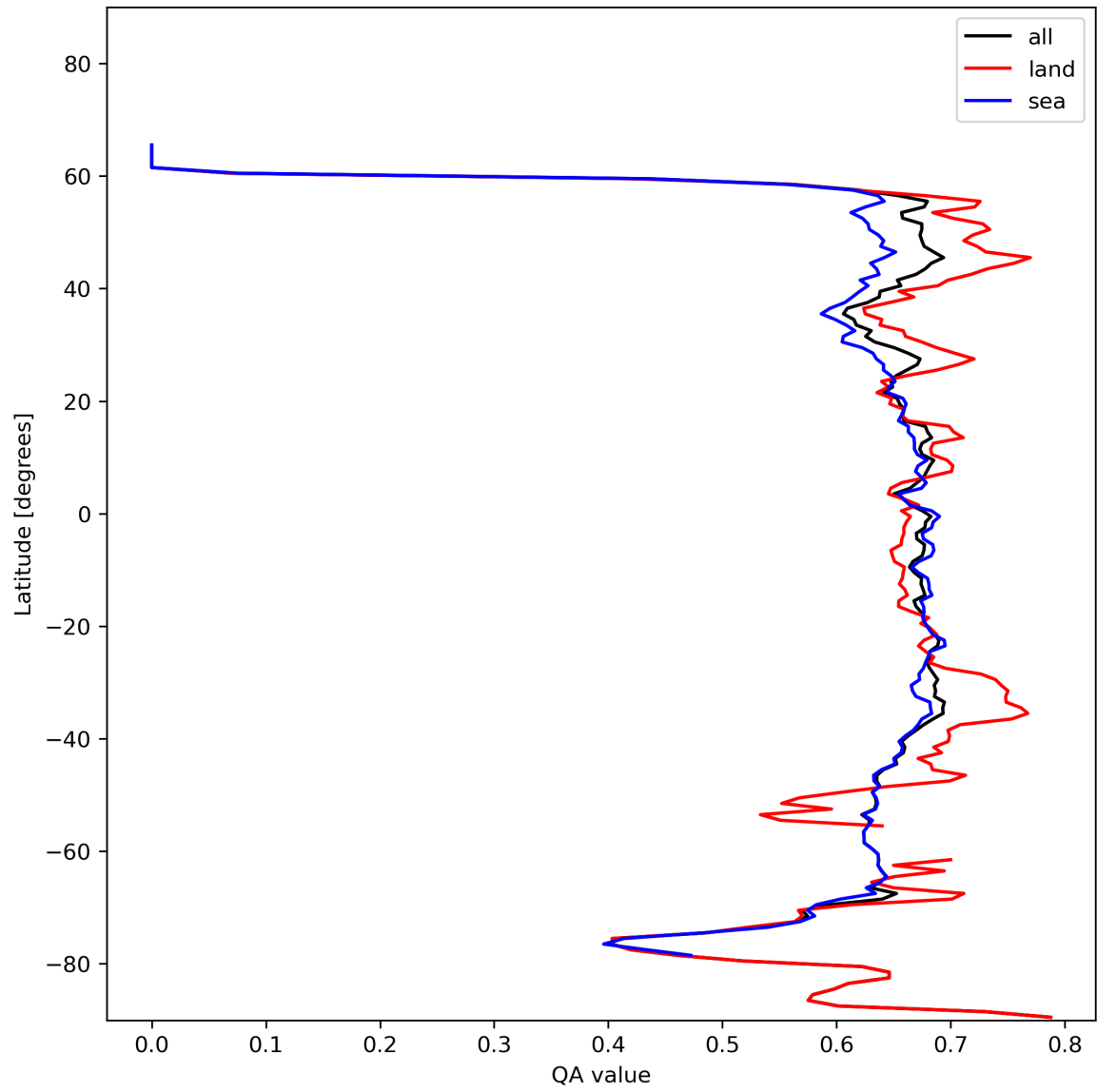
Figure 9: Zonal average of “QA value” for 2024-01-21 to 2024-01-23.
