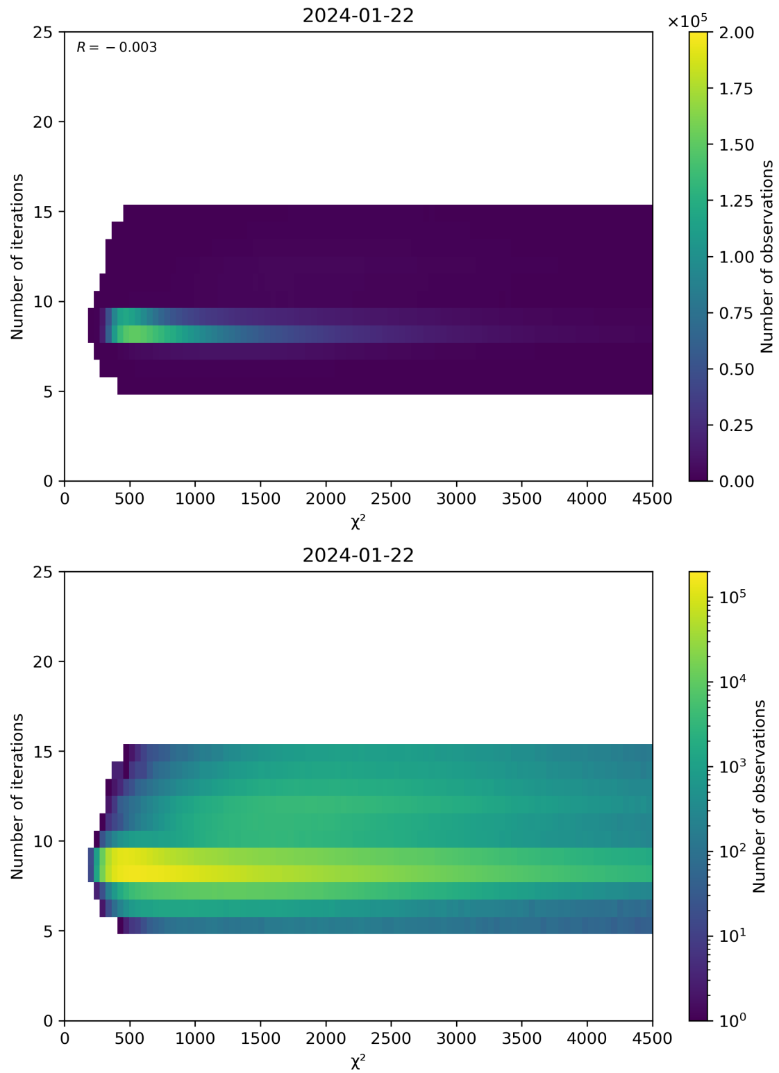
Figure 49: Scatter density plot of “ \chi^2 ” against “Number of iterations” for 2024-01-21 to 2024-01-23.
