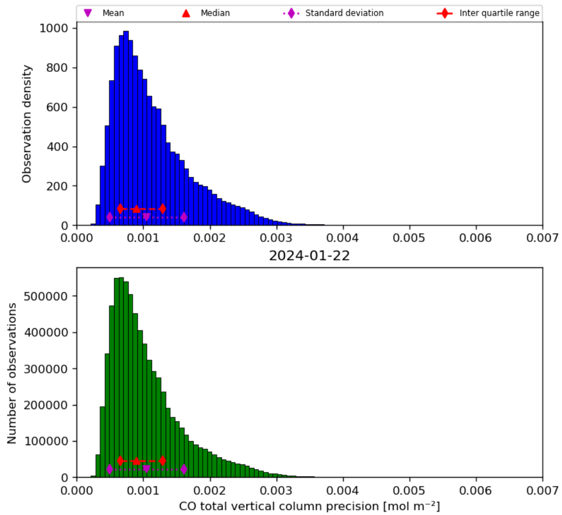
Figure 20: Histogram of “CO total vertical column precision” for 2024-01-21 to 2024-01-23
