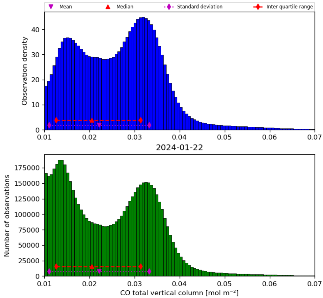
Figure 18: Histogram of “CO total vertical column” for 2024-01-21 to 2024-01-23
