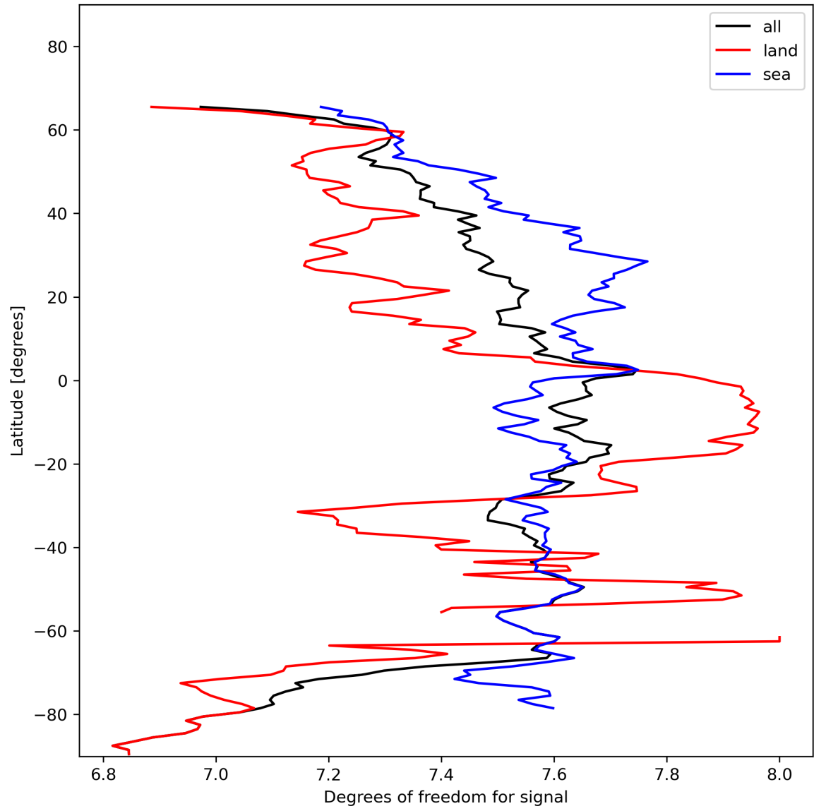
Figure 15: Zonal average of “Degrees of freedom for signal” for 2024-01-21 to 2024-01-23.
