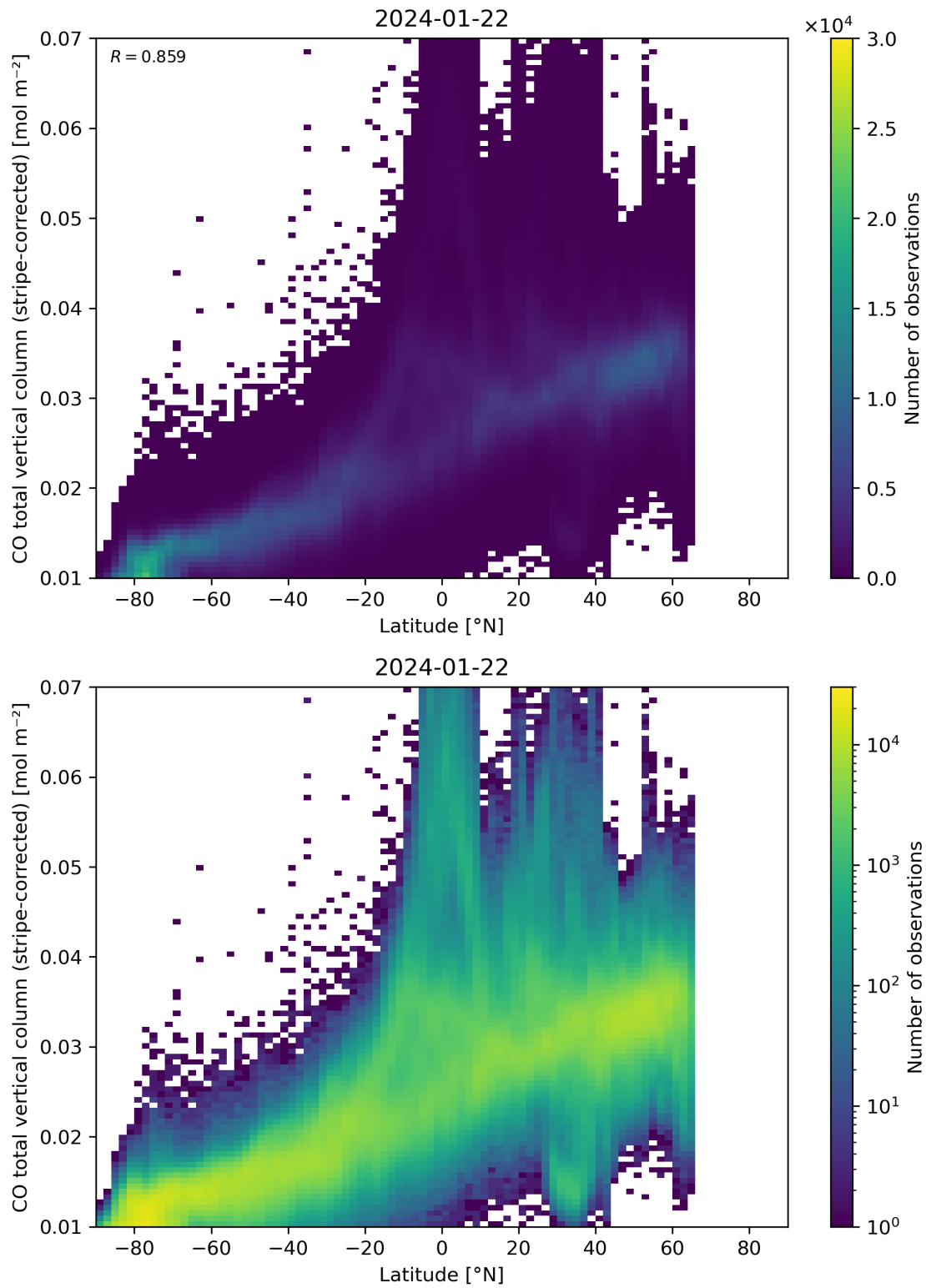
Figure 52: Scatter density plot of “Latitude” against “CO total vertical column (stripe-corrected)” for 2024-01-21 to 2024-01-23.
