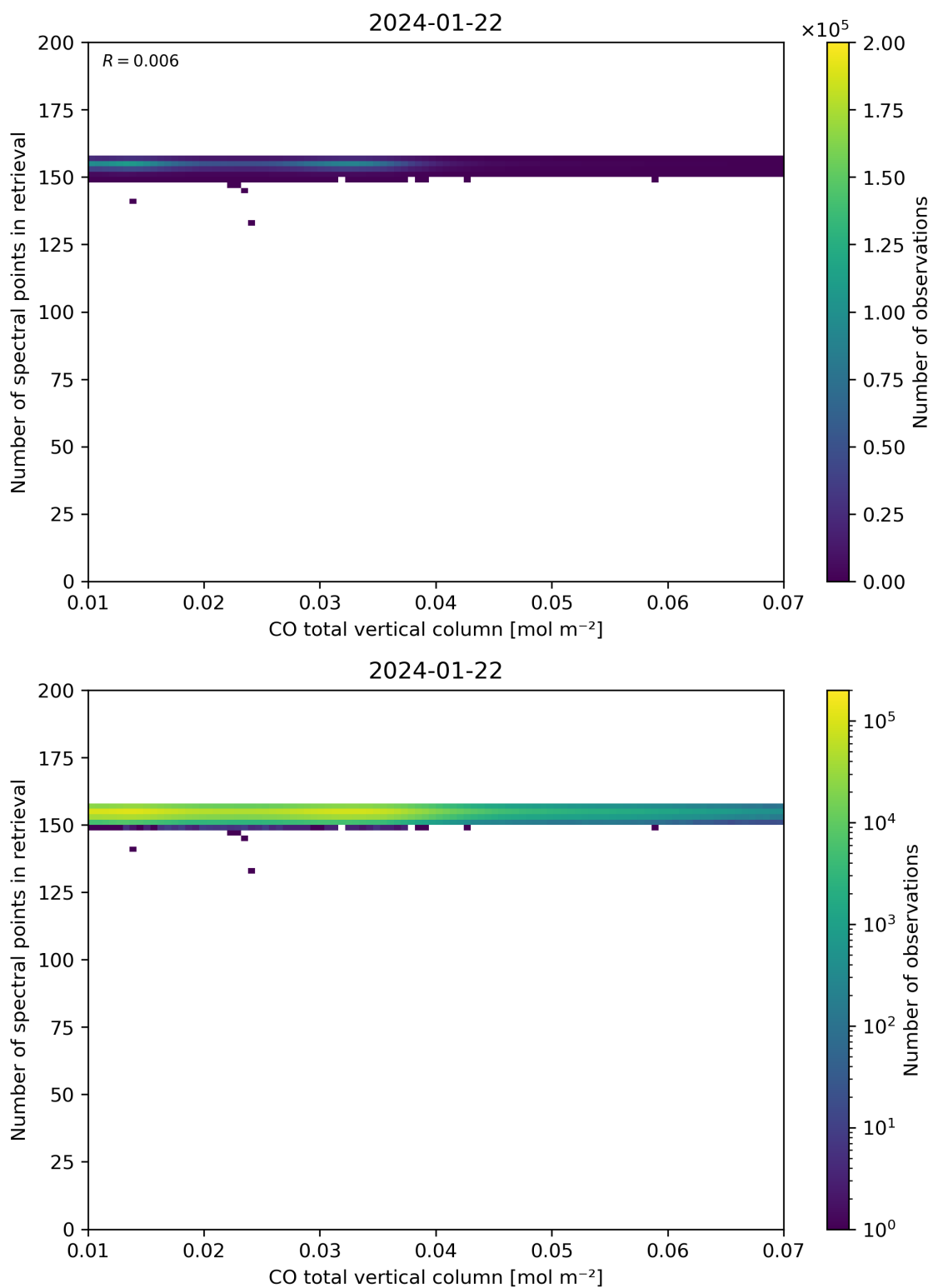
Figure 43: Scatter density plot of “CO total vertical column” against “Number of spectral points in retrieval” for 2024-01-21 to 2024-01-23.
