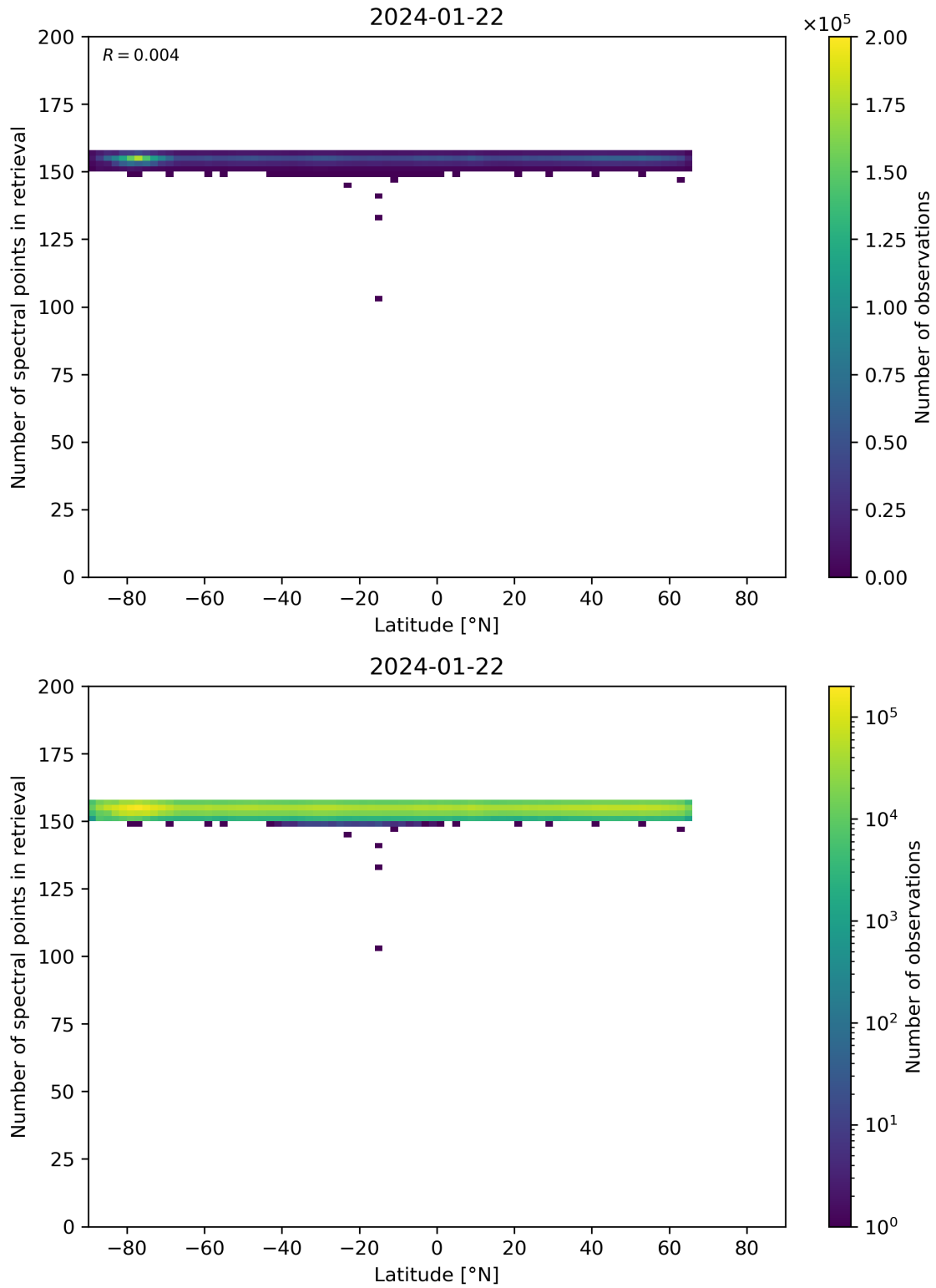
Figure 57: Scatter density plot of “Latitude” against “Number of spectral points in retrieval” for 2024-01-21 to 2024-01-23.
