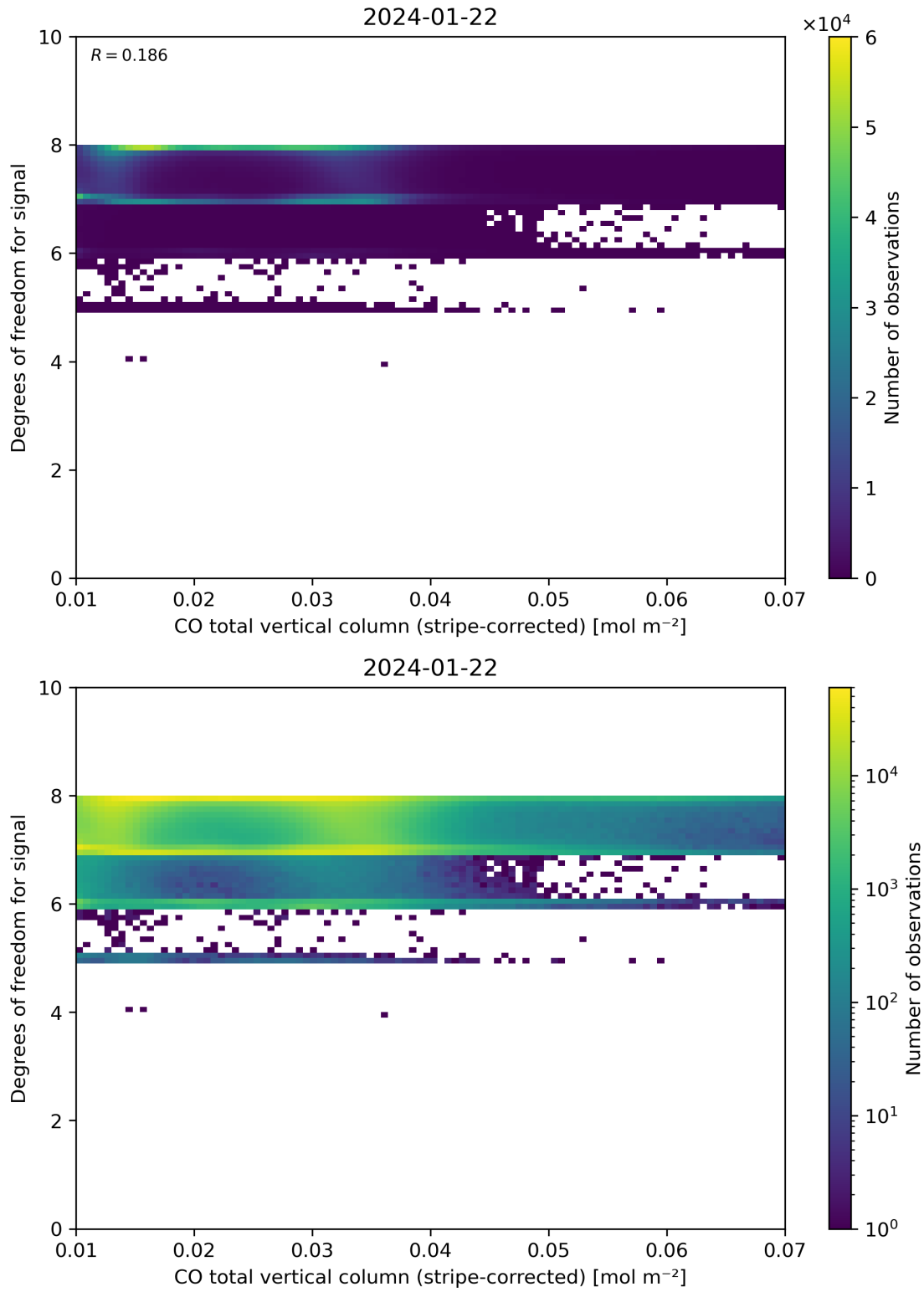
Figure 38: Scatter density plot of “CO total vertical column (stripe-corrected)” against “Degrees of freedom for signal” for 2024-01-21 to 2024-01-23.
