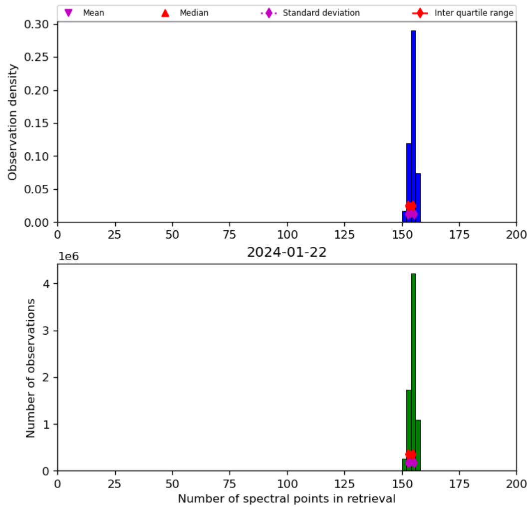
Figure 21: Histogram of “Number of spectral points in retrieval” for 2024-01-21 to 2024-01-23
