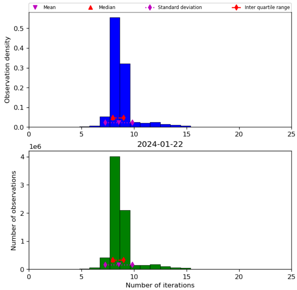
Figure 24: Histogram of “Number of iterations” for 2024-01-21 to 2024-01-23
