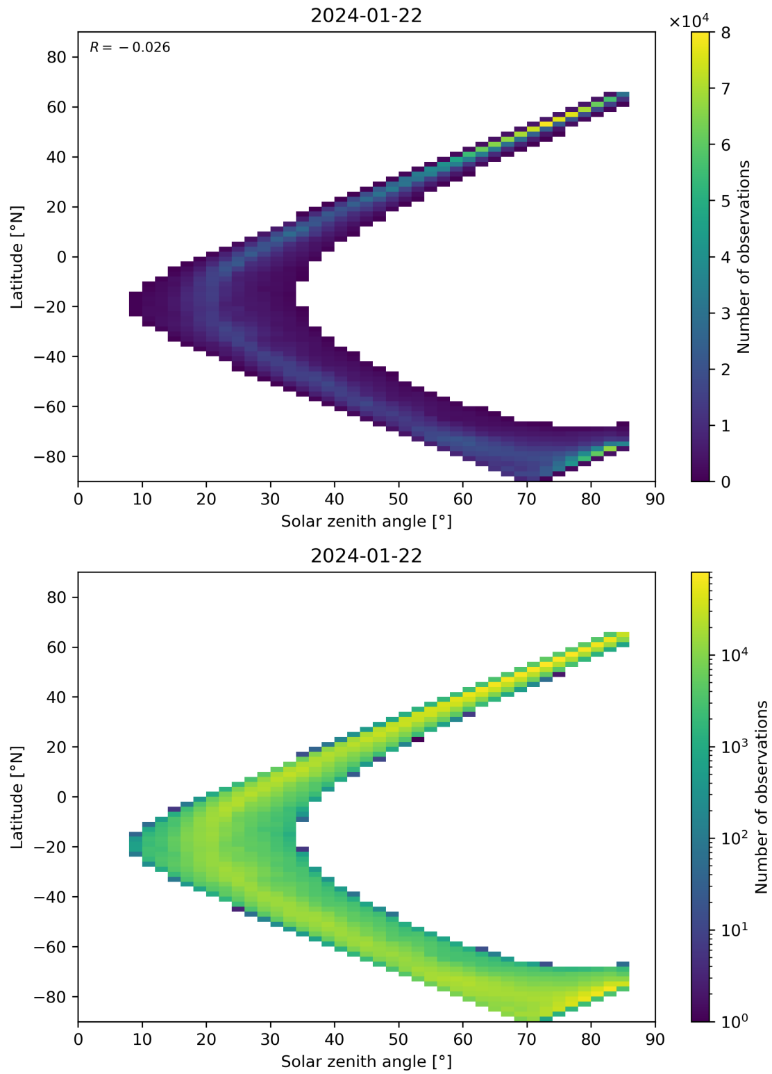
Figure 66: Scatter density plot of “Solar zenith angle” against “Latitude” for 2024-01-21 to 2024-01-23.
