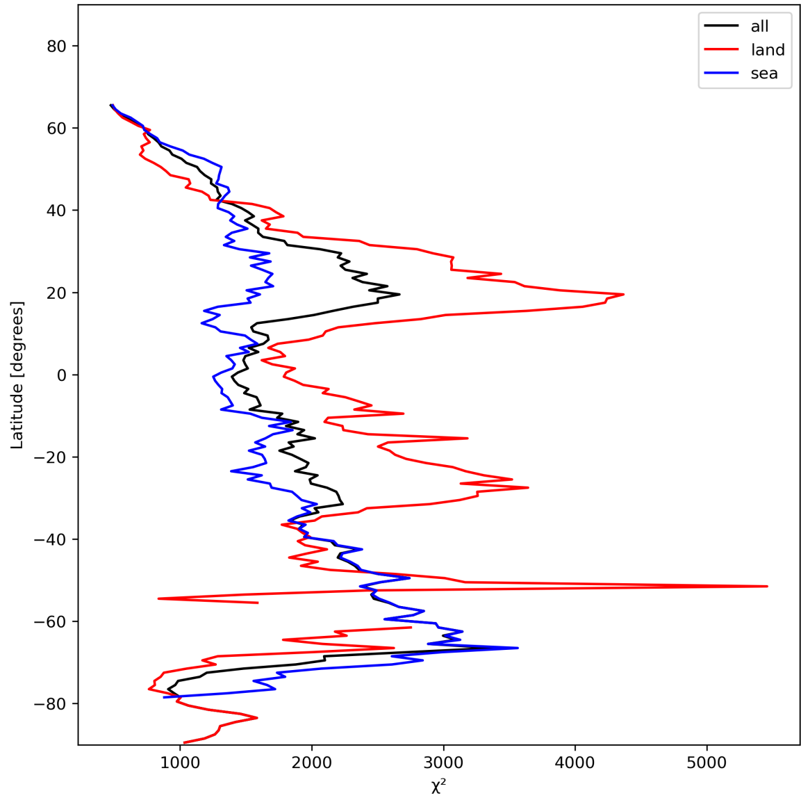
Figure 14: Zonal average of “ \chi^2 ” for 2024-01-21 to 2024-01-23.
