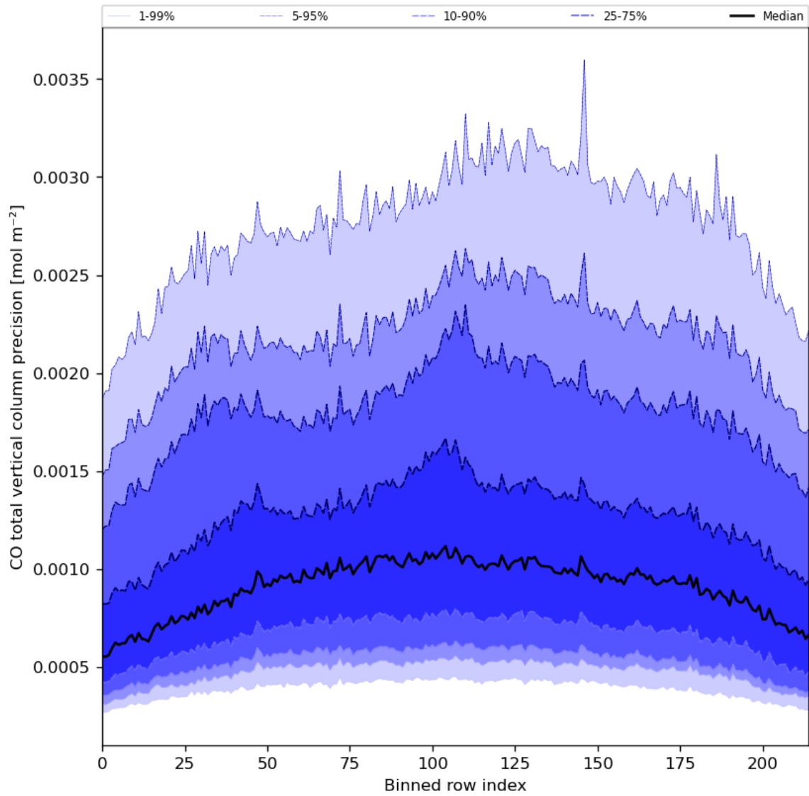
Figure 28: Along track statistics of “CO total vertical column precision” for 2024-01-21 to 2024-01-23
