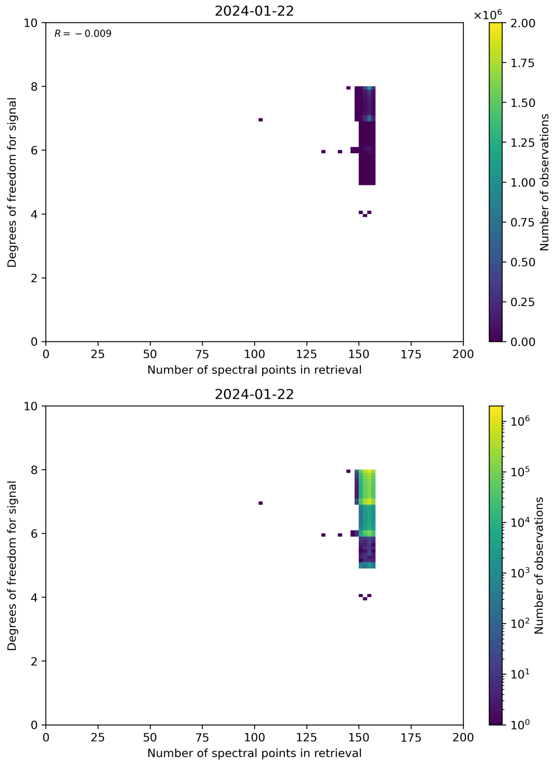
Figure 59: Scatter density plot of “Number of spectral points in retrieval” against “Degrees of freedom for signal” for 2024-01-21 to 2024-01-23.
