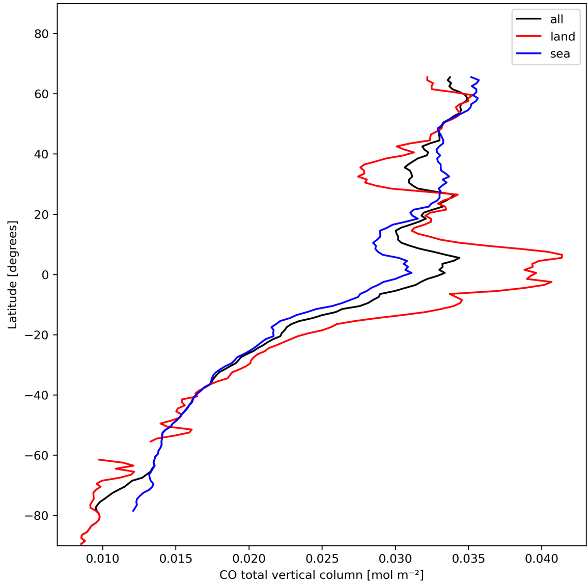
Figure 10: Zonal average of “CO total vertical column” for 2024-01-21 to 2024-01-23.
