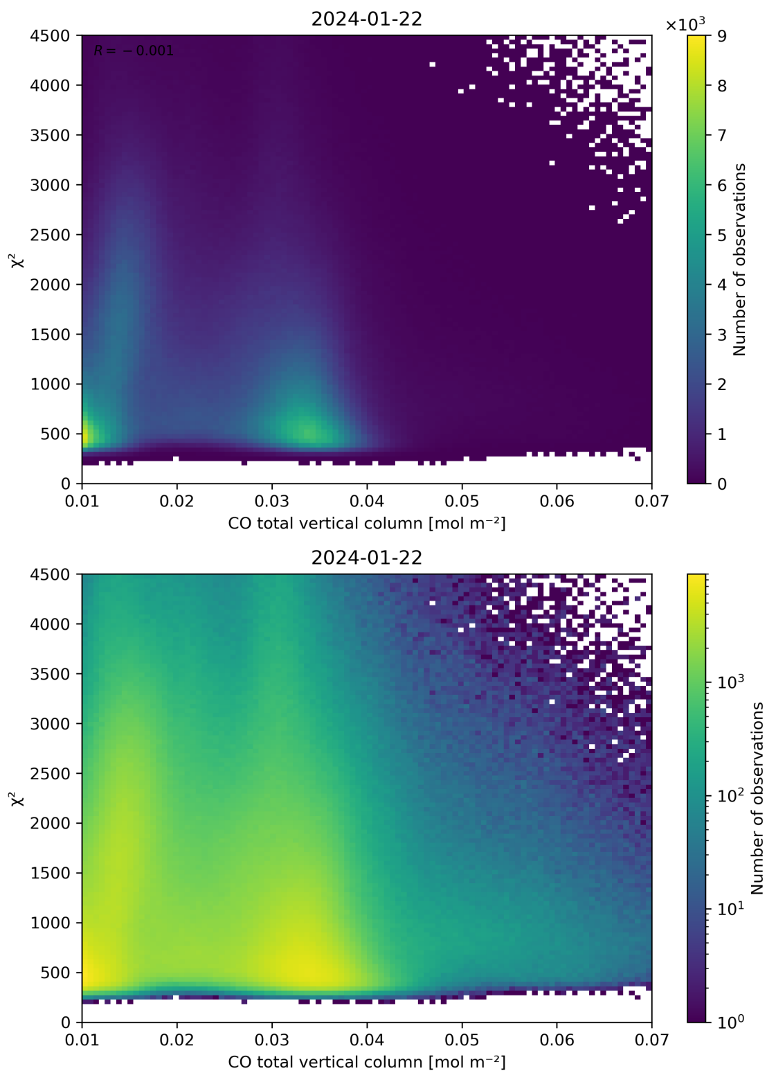
Figure 35: Scatter density plot of “CO total vertical column” against “ \chi^2 ” for 2024-01-21 to 2024-01-23.
