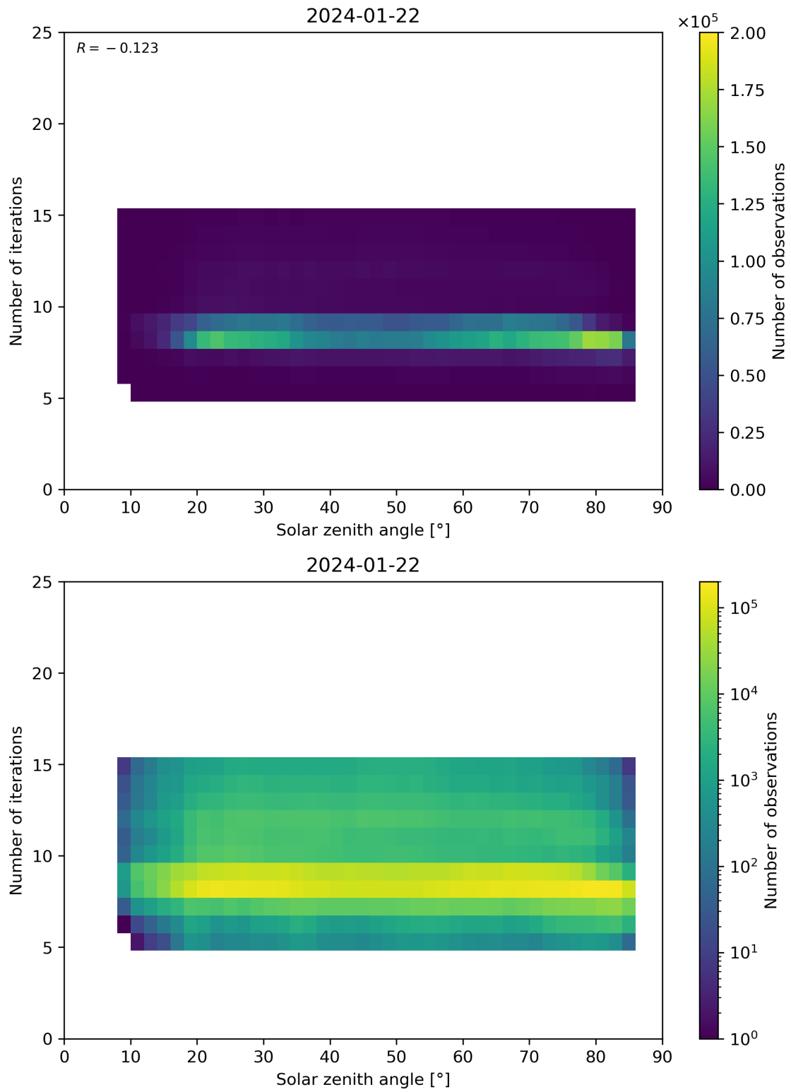
Figure 67: Scatter density plot of “Solar zenith angle” against “Number of iterations” for 2024-01-21 to 2024-01-23.
