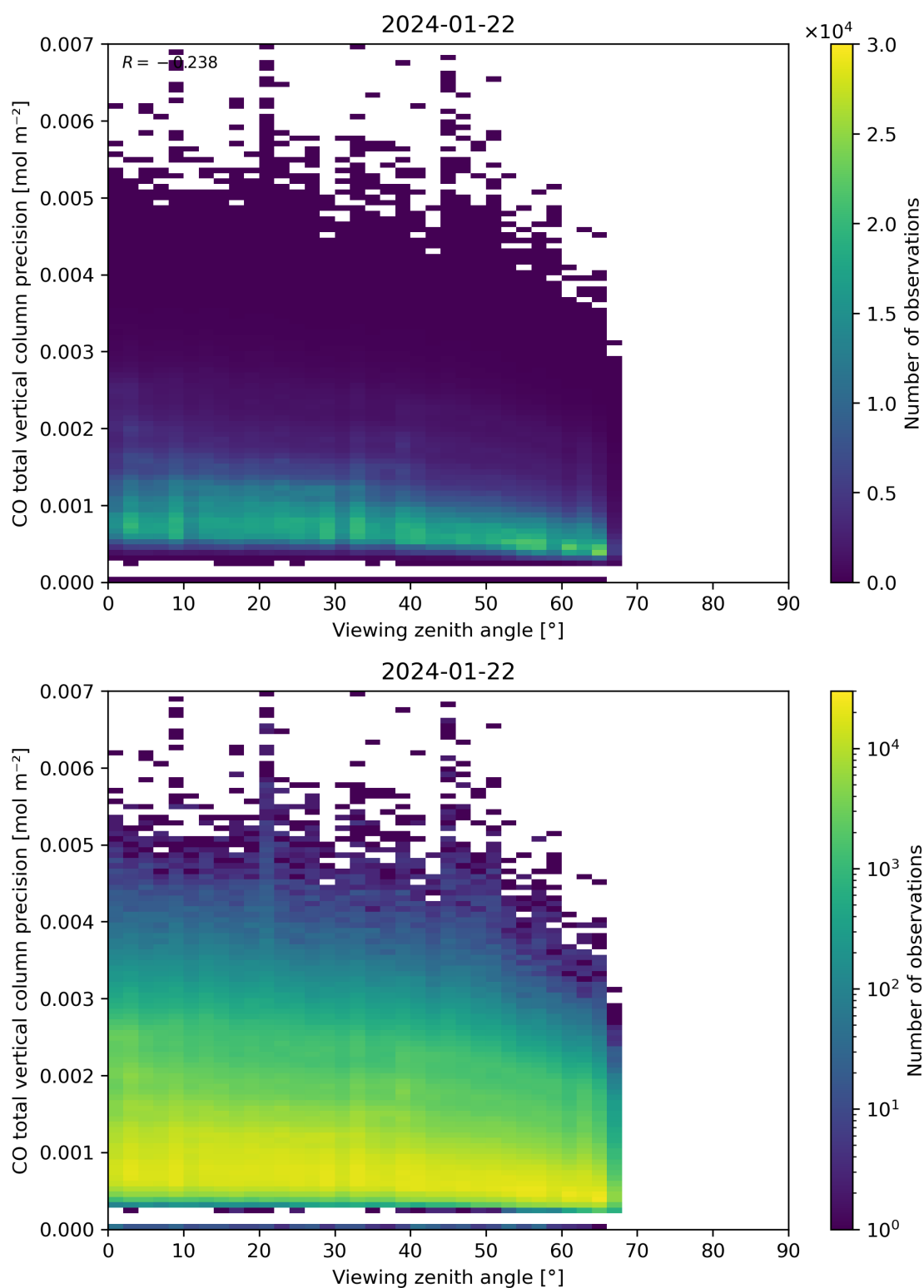
Figure 71: Scatter density plot of “Viewing zenith angle” against “CO total vertical column precision” for 2024-01-21 to 2024-01-23.
