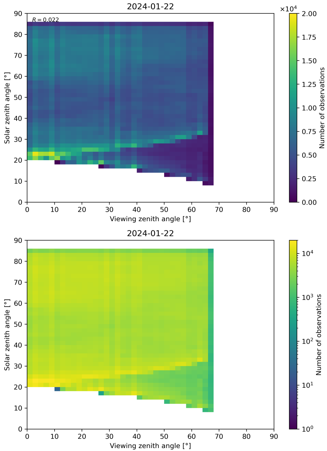
Figure 77: Scatter density plot of “Viewing zenith angle” against “Solar zenith angle” for 2024-01-21 to 2024-01-23.
