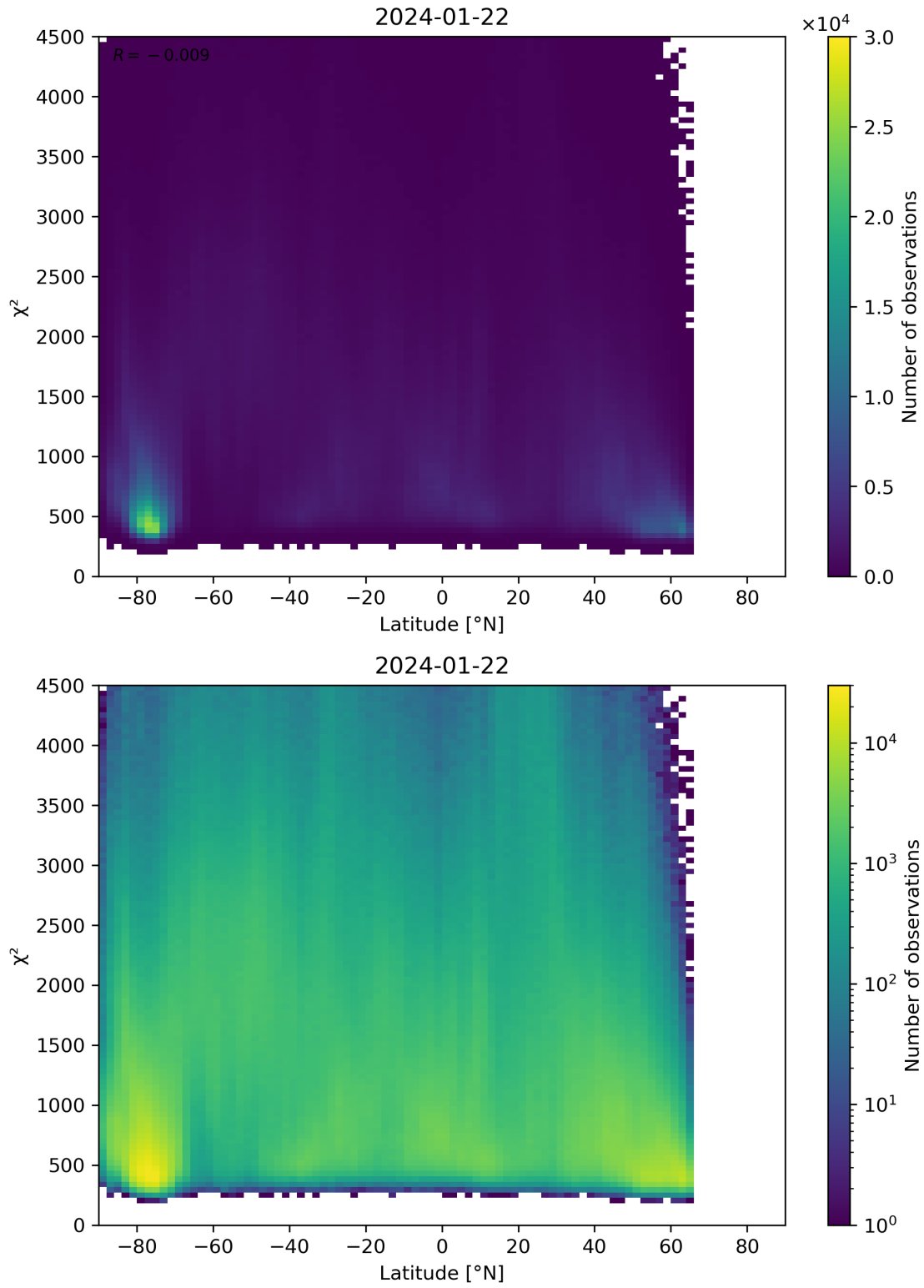
Figure 54: Scatter density plot of “Latitude” against “ \chi^2 ” for 2024-01-21 to 2024-01-23.
