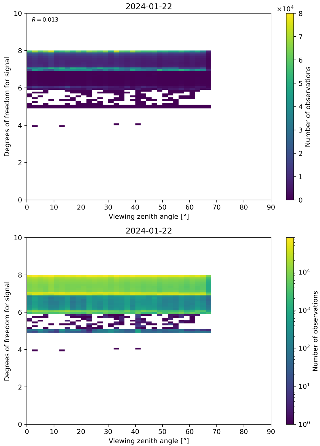
Figure 73: Scatter density plot of “Viewing zenith angle” against “Degrees of freedom for signal” for 2024-01-21 to 2024-01-23.
