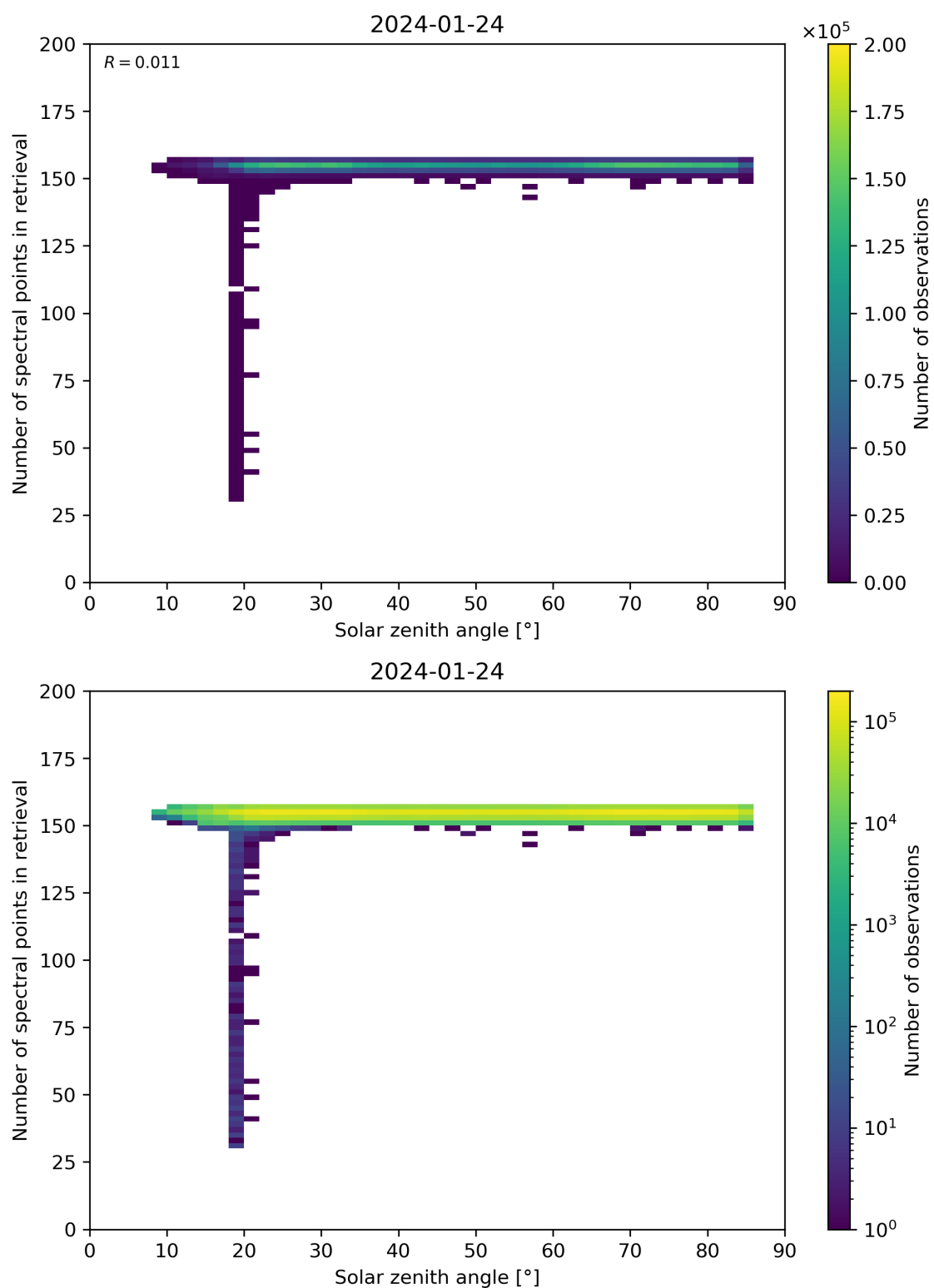
Figure 68: Scatter density plot of “Solar zenith angle” against “Number of spectral points in retrieval” for 2024-01-23 to 2024-01-25.
