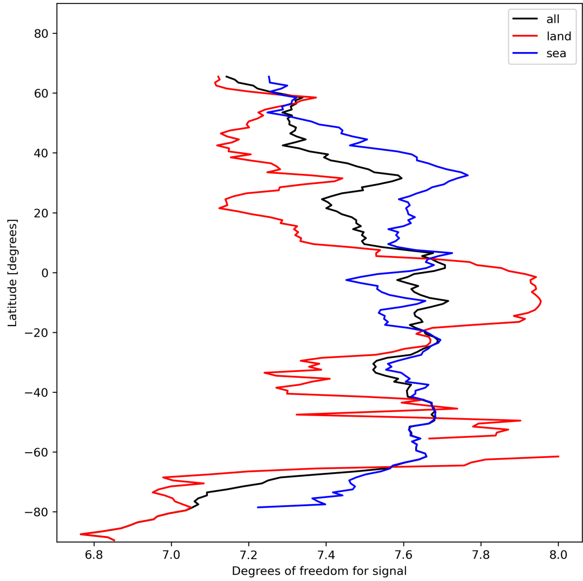
Figure 15: Zonal average of “Degrees of freedom for signal” for 2024-01-23 to 2024-01-25.
