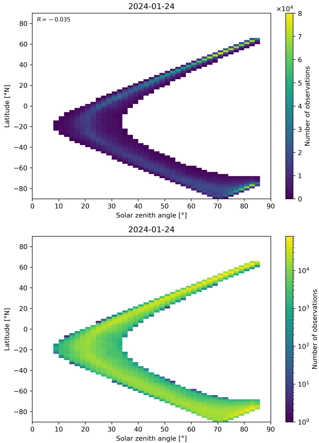
Figure 66: Scatter density plot of “Solar zenith angle” against “Latitude” for 2024-01-23 to 2024-01-25.
