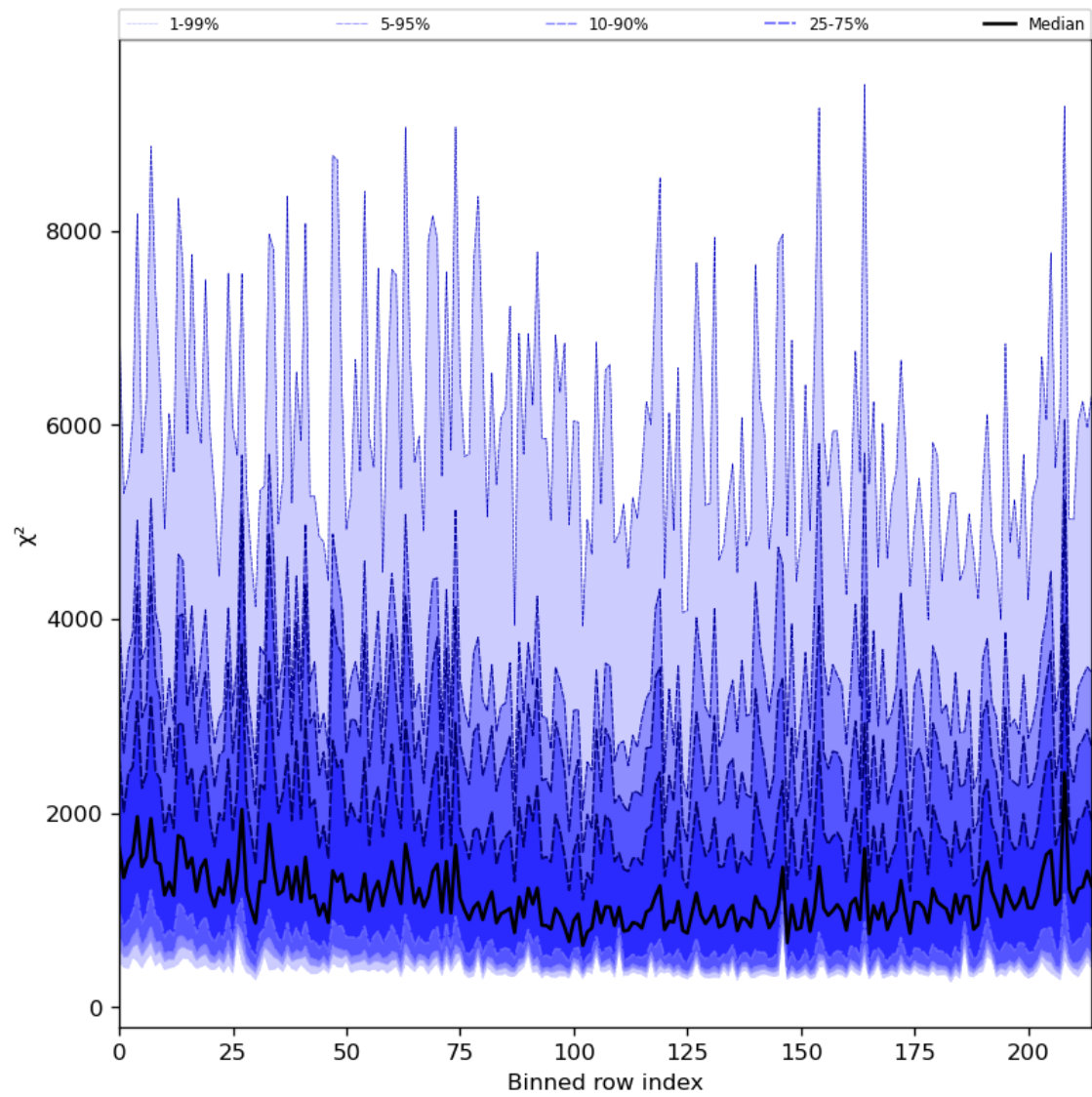
Figure 30: Along track statistics of “ \chi^2 ” for 2024-01-23 to 2024-01-25
