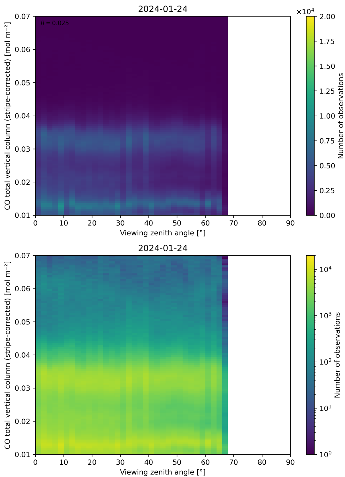
Figure 70: Scatter density plot of “Viewing zenith angle” against “CO total vertical column (stripe-corrected)” for 2024-01-23 to 2024-01-25.
