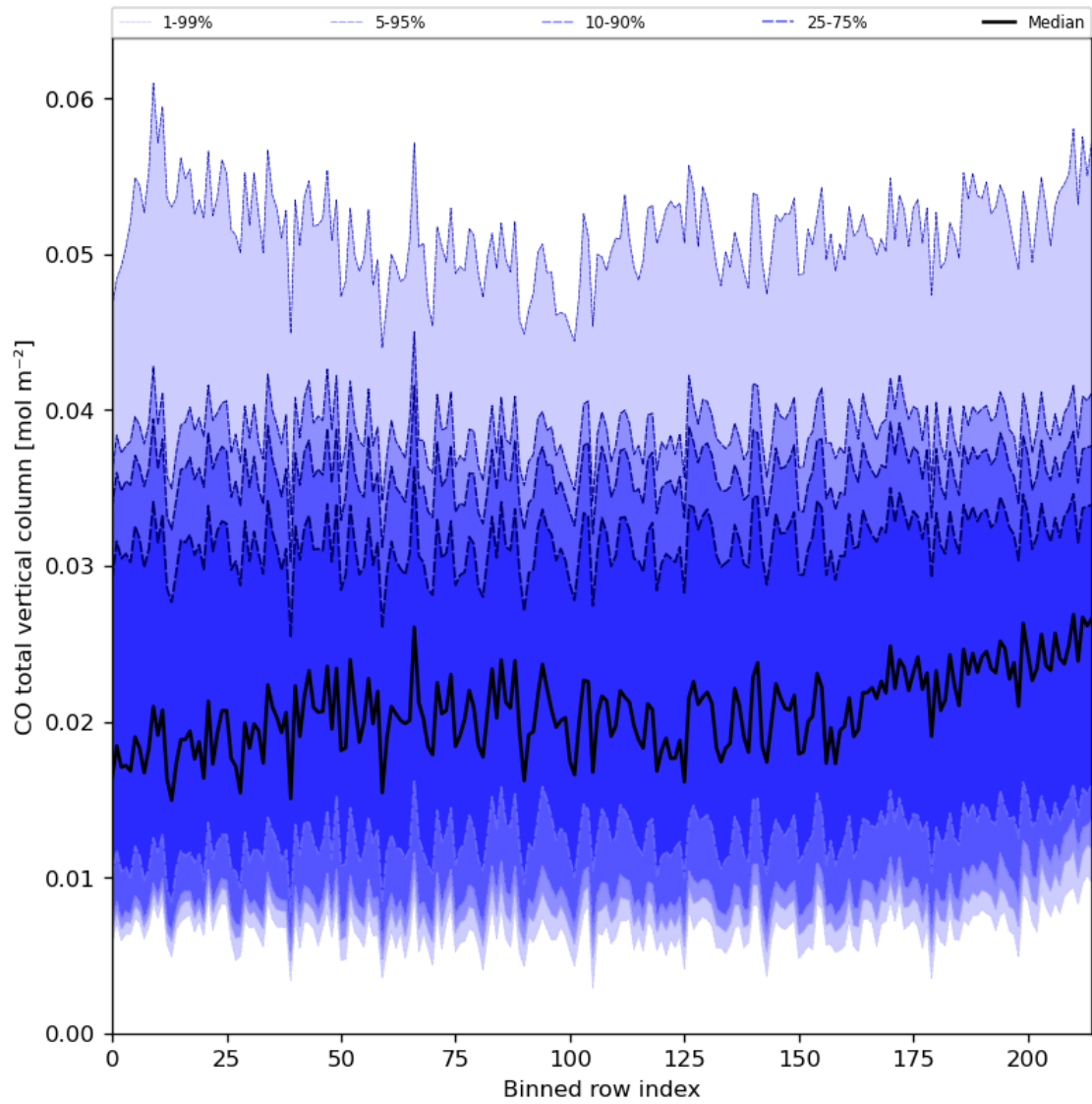
Figure 26: Along track statistics of “CO total vertical column” for 2024-01-23 to 2024-01-25
