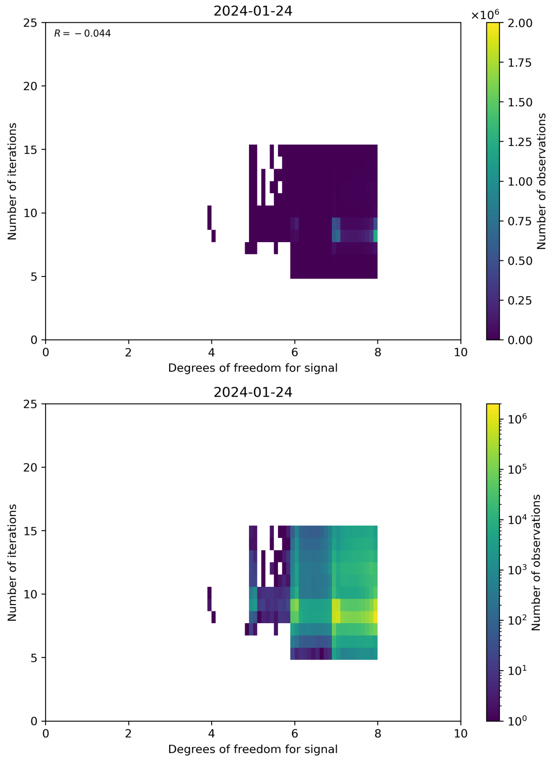
Figure 50: Scatter density plot of “Degrees of freedom for signal” against “Number of iterations” for 2024-01-23 to 2024-01-25.
