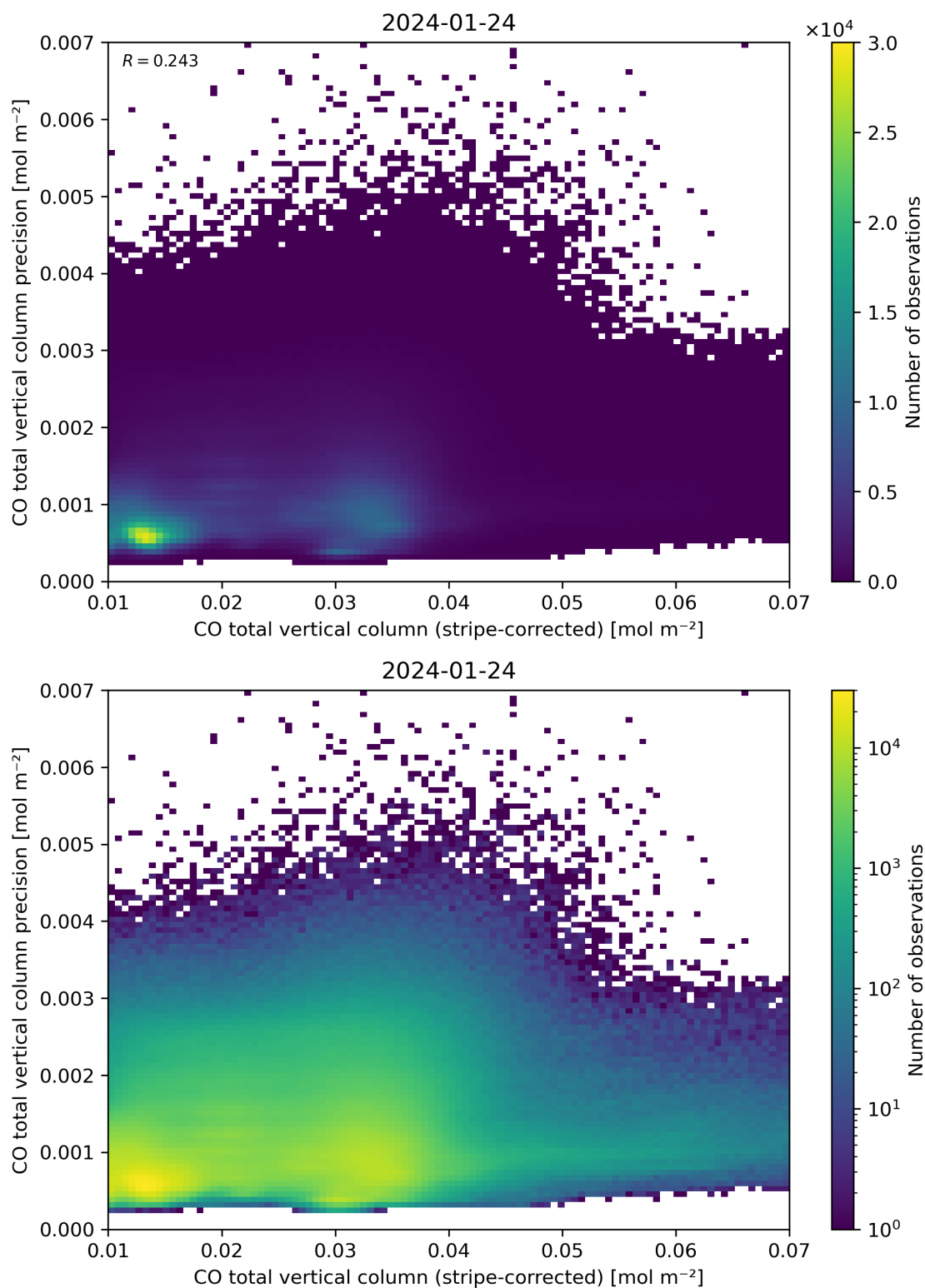
Figure 36: Scatter density plot of “CO total vertical column (stripe-corrected)” against “CO total vertical column precision” for 2024-01-23 to 2024-01-25.
