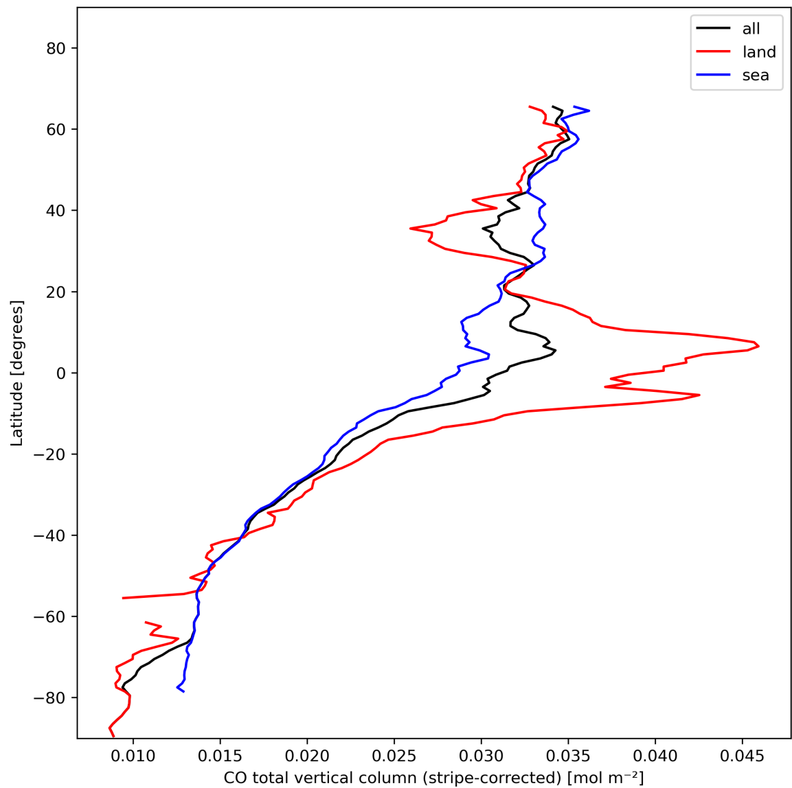
Figure 11: Zonal average of “CO total vertical column (stripe-corrected)” for 2024-01-23 to 2024-01-25.
