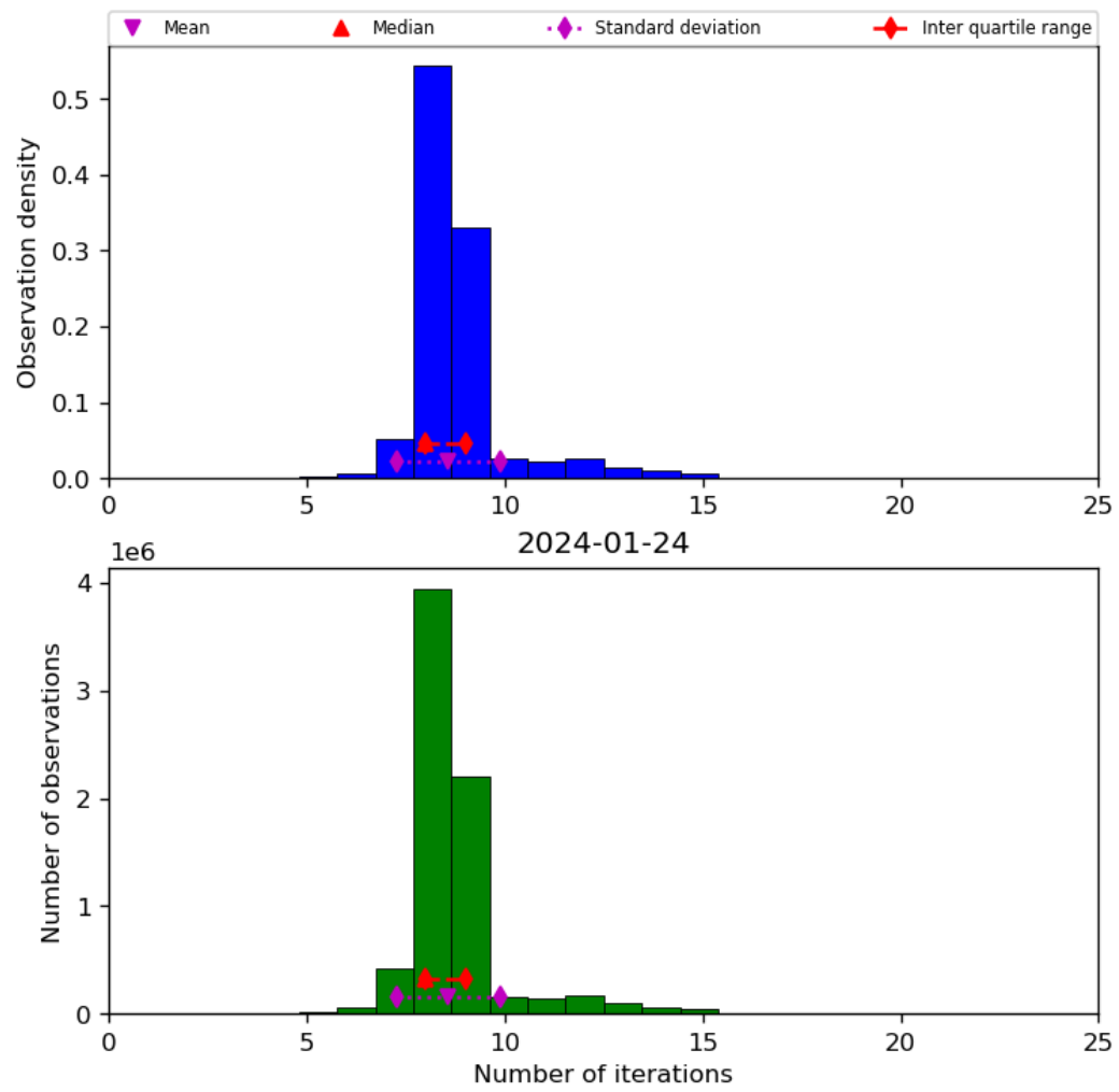
Figure 24: Histogram of “Number of iterations” for 2024-01-23 to 2024-01-25
