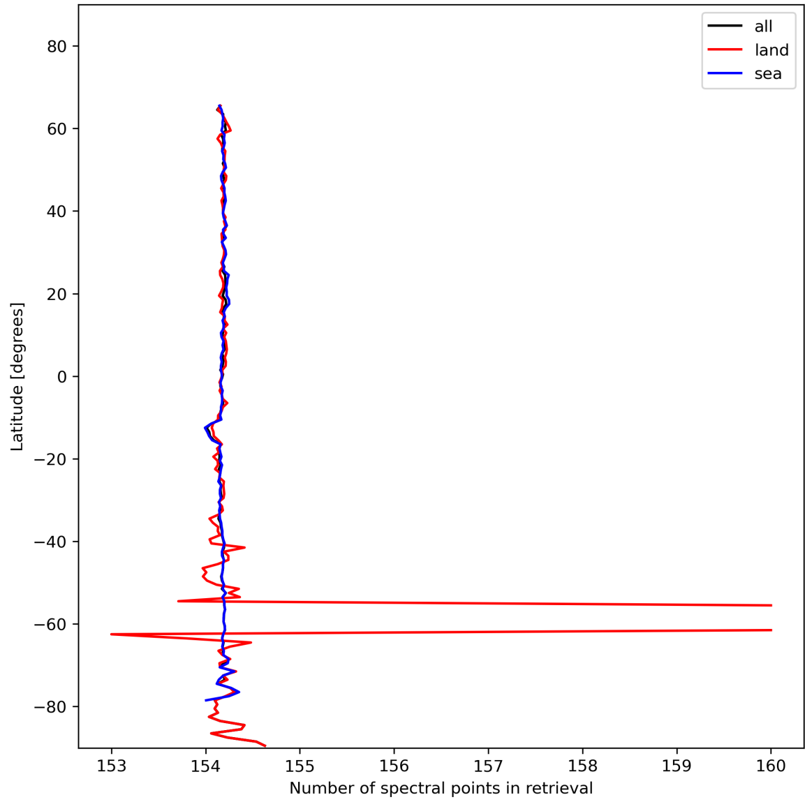
Figure 13: Zonal average of “Number of spectral points in retrieval” for 2024-01-23 to 2024-01-25.
