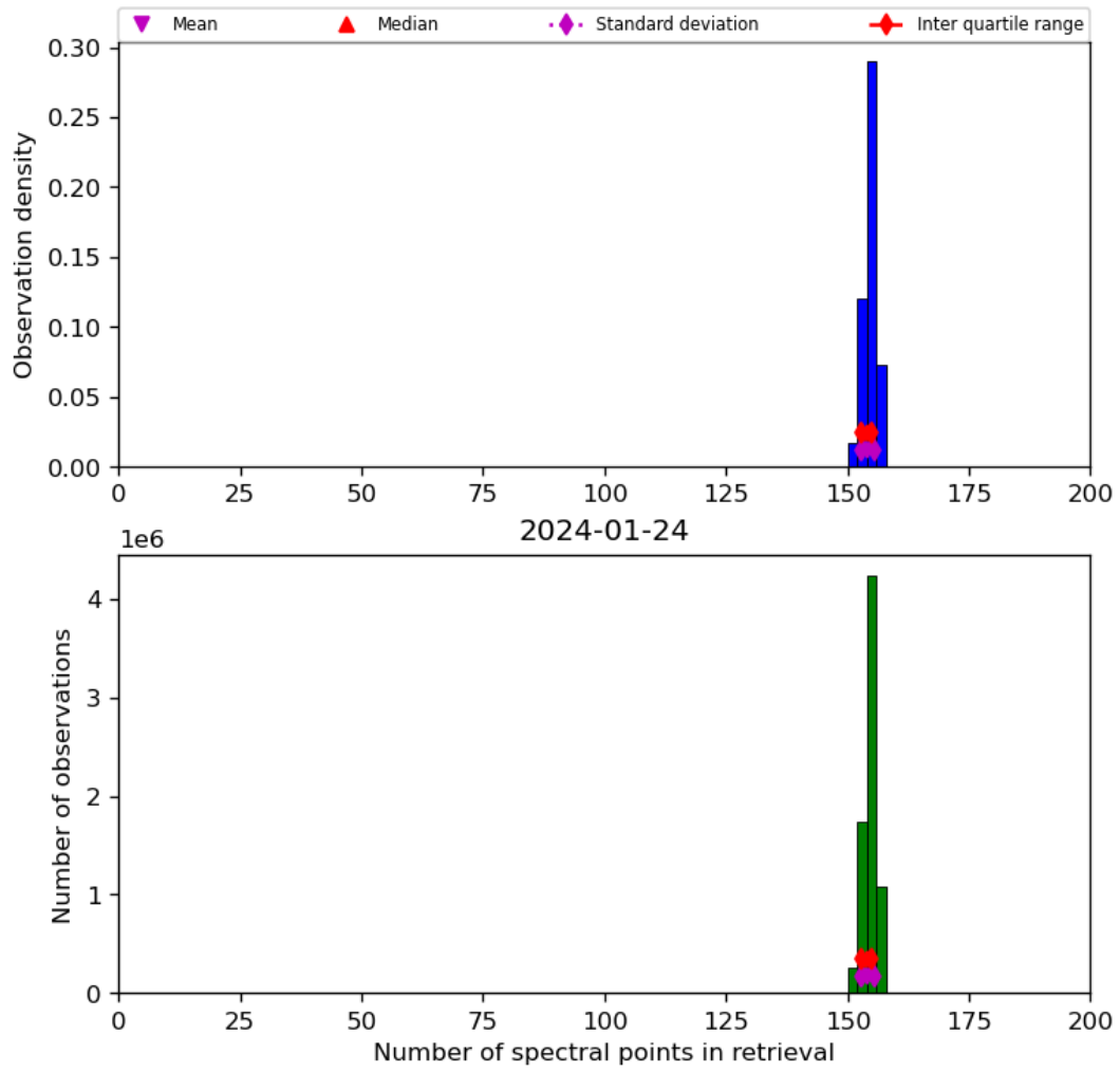
Figure 21: Histogram of “Number of spectral points in retrieval” for 2024-01-23 to 2024-01-25
