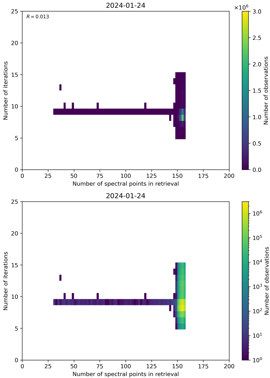
Figure 60: Scatter density plot of “Number of spectral points in retrieval” against “Number of iterations” for 2024-01-23 to 2024-01-25.
