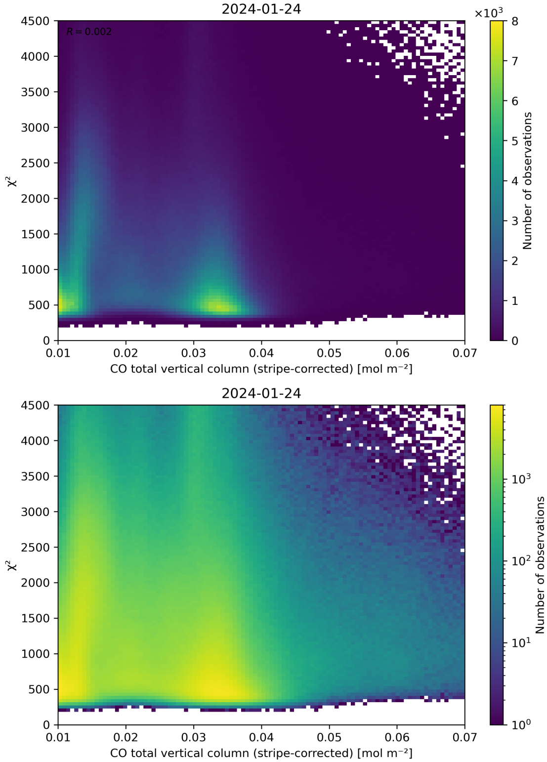
Figure 37: Scatter density plot of “CO total vertical column (stripe-corrected)” against “ \chi^2 ” for 2024-01-23 to 2024-01-25.
