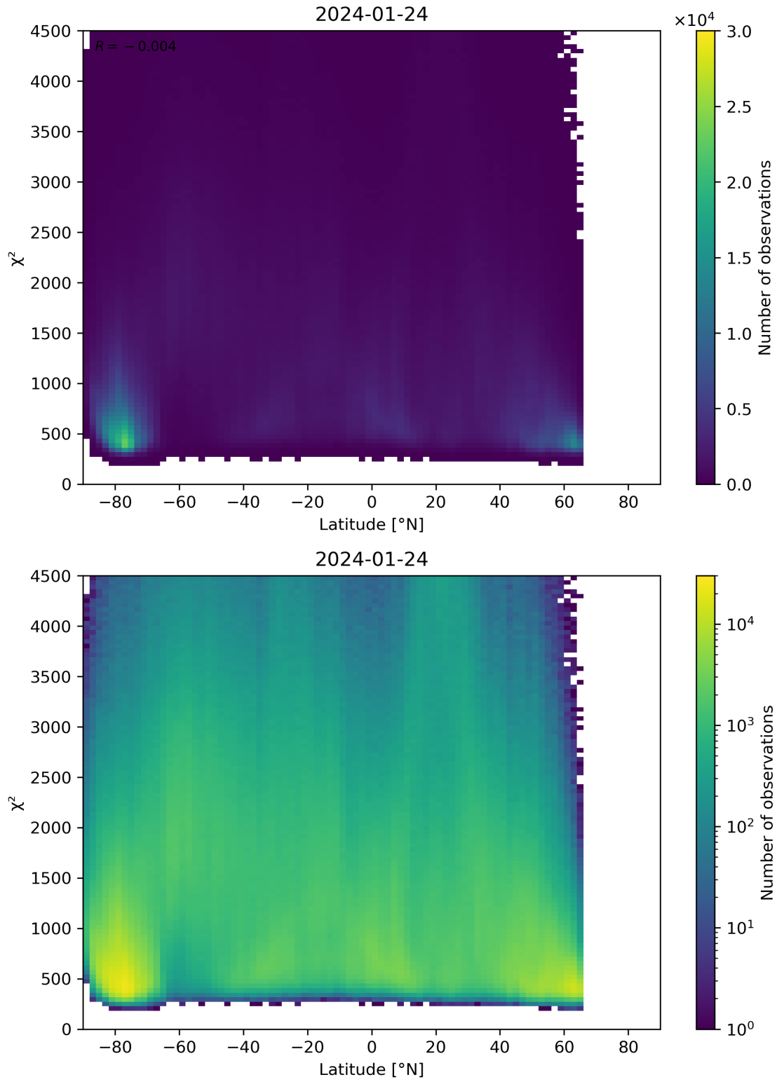
Figure 54: Scatter density plot of “Latitude” against “ \chi^2 ” for 2024-01-23 to 2024-01-25.
