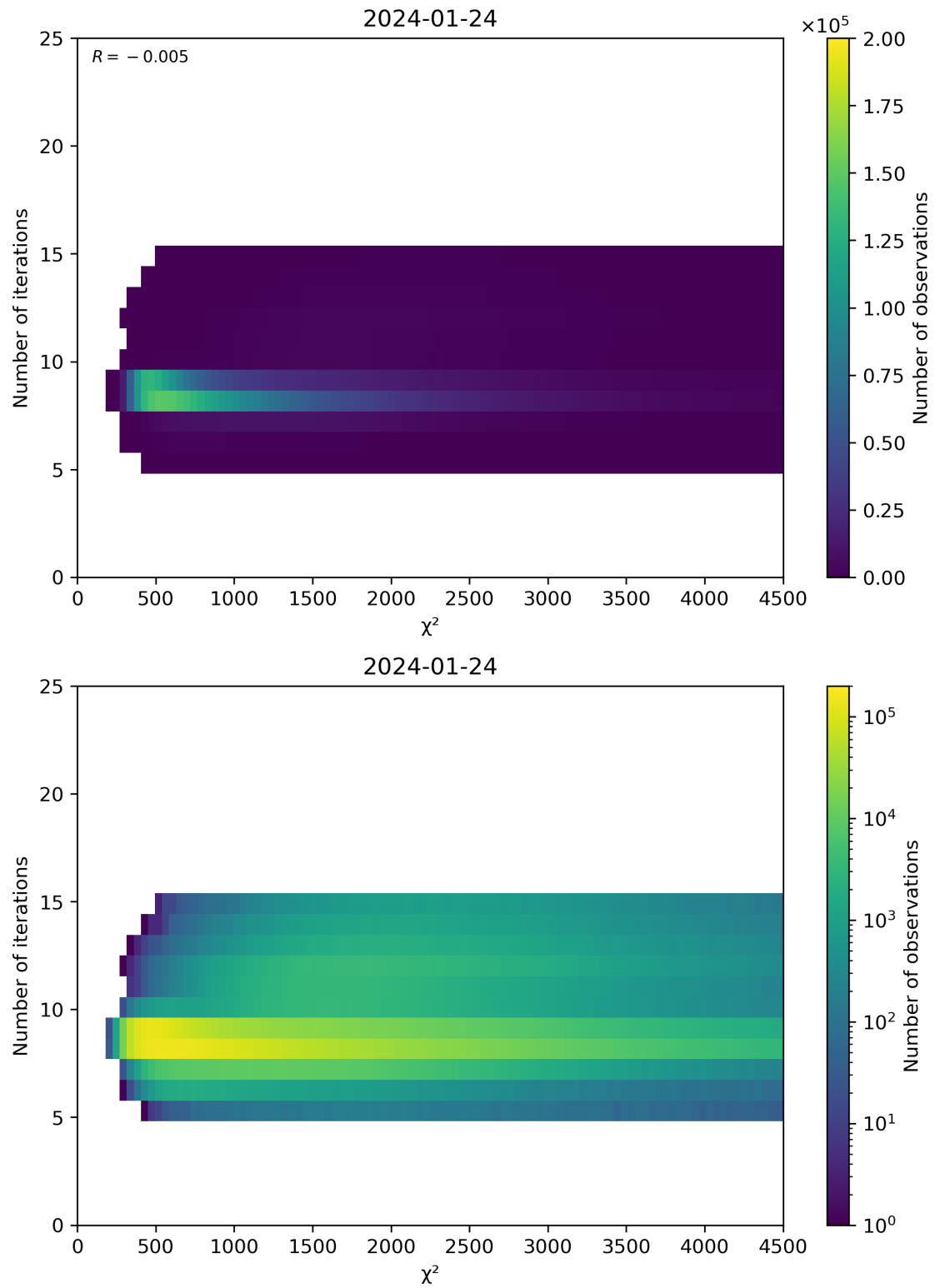
Figure 49: Scatter density plot of “ \chi^2 ” against “Number of iterations” for 2024-01-23 to 2024-01-25.
