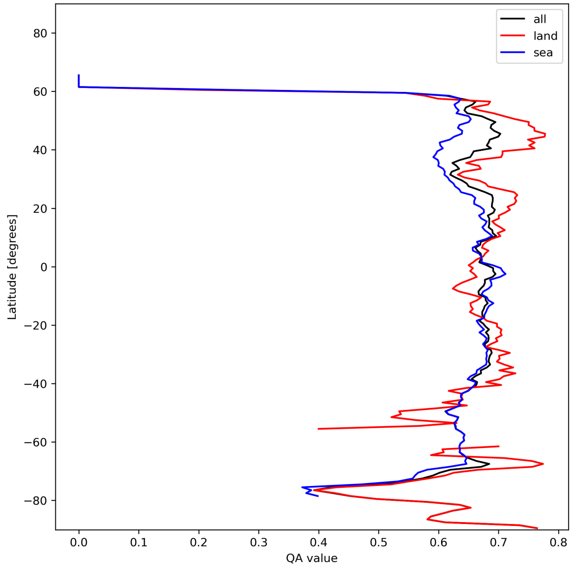
Figure 9: Zonal average of “QA value” for 2024-01-23 to 2024-01-25.
