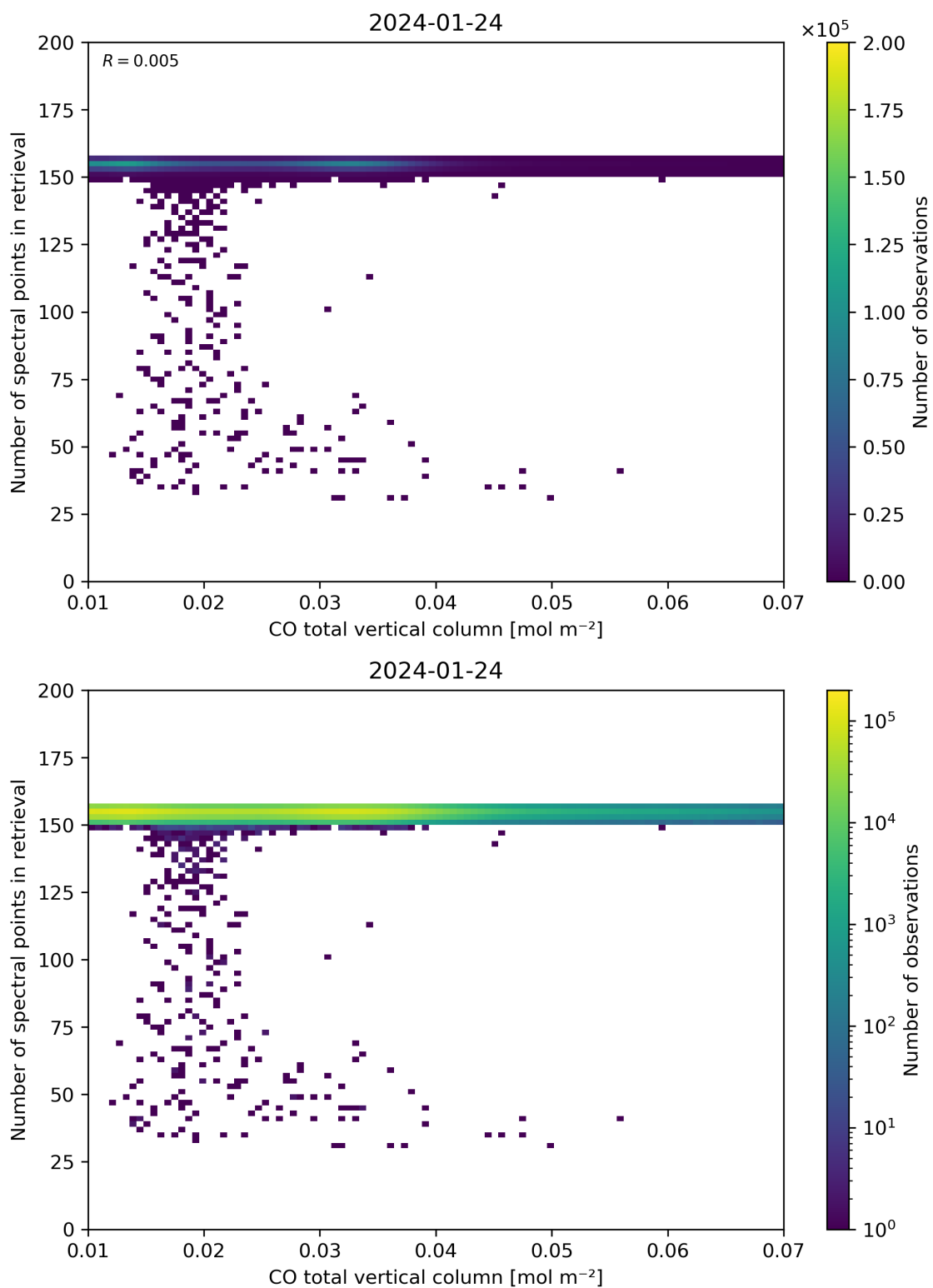
Figure 43: Scatter density plot of “CO total vertical column” against “Number of spectral points in retrieval” for 2024-01-23 to 2024-01-25.
