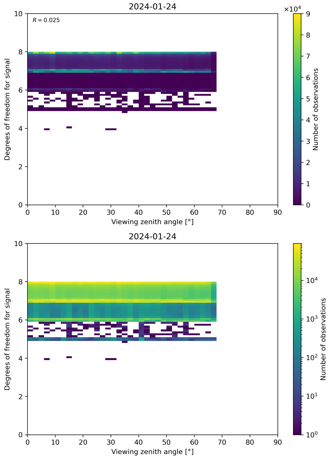
Figure 73: Scatter density plot of “Viewing zenith angle” against “Degrees of freedom for signal” for 2024-01-23 to 2024-01-25.
