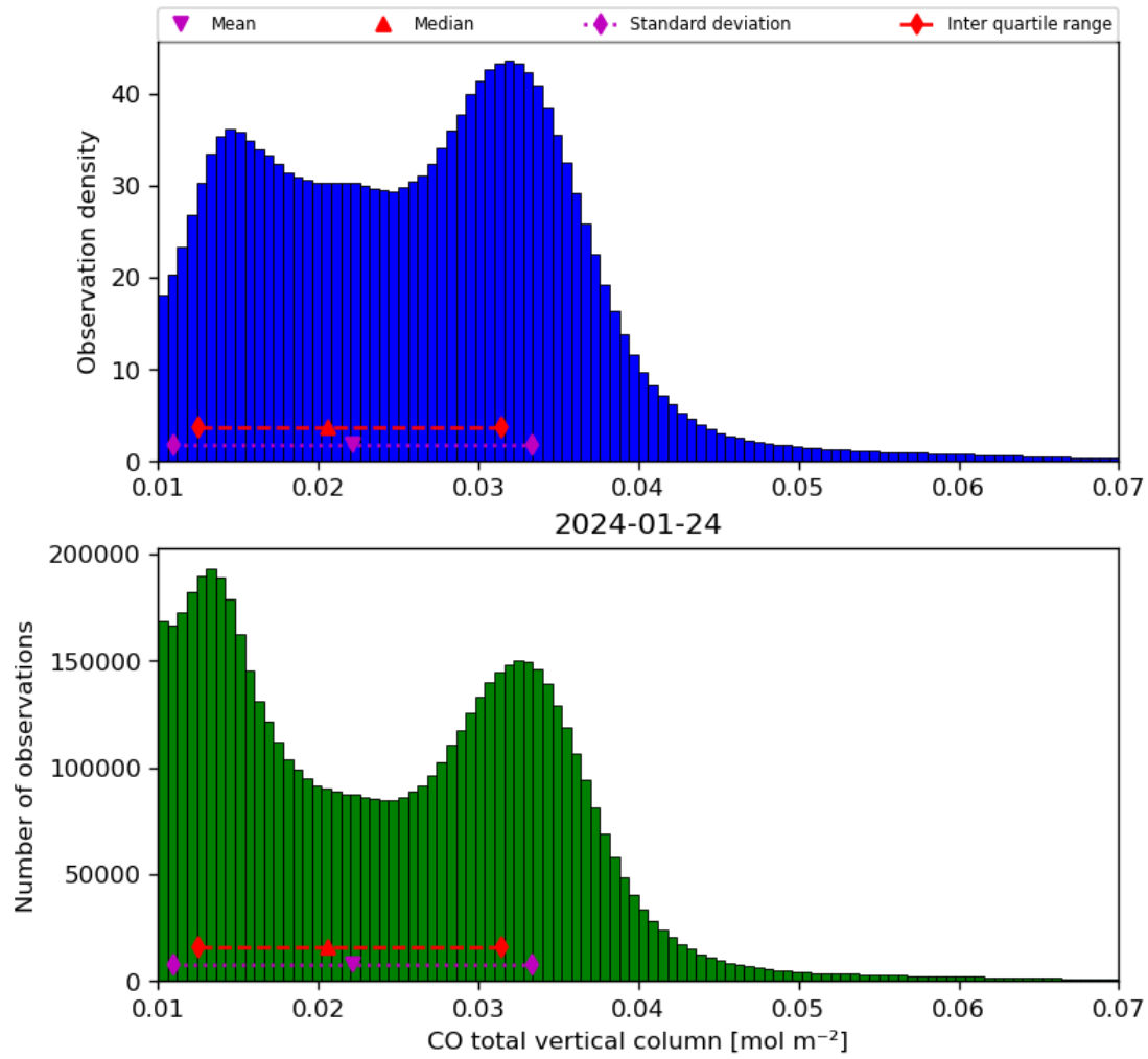
Figure 18: Histogram of “CO total vertical column” for 2024-01-23 to 2024-01-25
