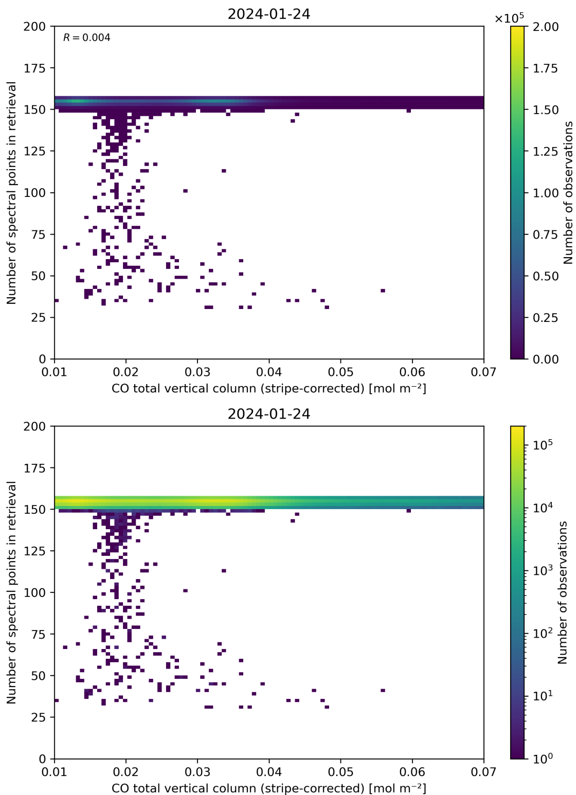
Figure 40: Scatter density plot of “CO total vertical column (stripe-corrected)” against “Number of spectral points in retrieval” for 2024-01-23 to 2024-01-25.
