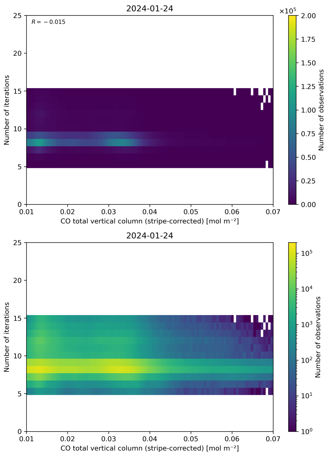
Figure 39: Scatter density plot of “CO total vertical column (stripe-corrected)” against “Number of iterations” for 2024-01-23 to 2024-01-25.
