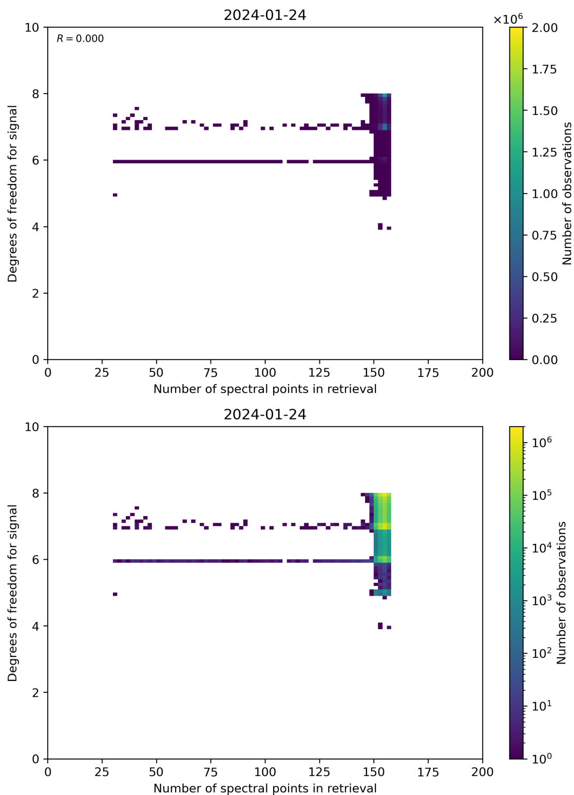
Figure 59: Scatter density plot of “Number of spectral points in retrieval” against “Degrees of freedom for signal” for 2024-01-23 to 2024-01-25.
