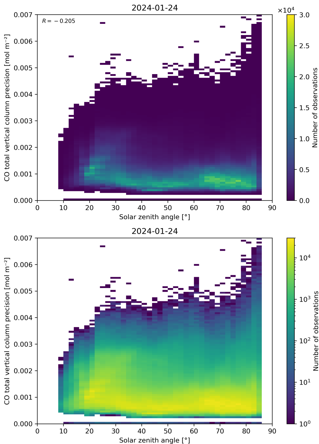
Figure 63: Scatter density plot of “Solar zenith angle” against “CO total vertical column precision” for 2024-01-23 to 2024-01-25.
