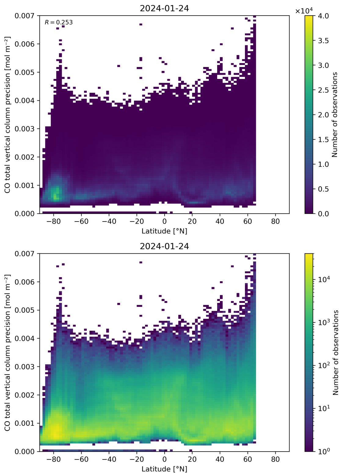
Figure 53: Scatter density plot of “Latitude” against “CO total vertical column precision” for 2024-01-23 to 2024-01-25.
