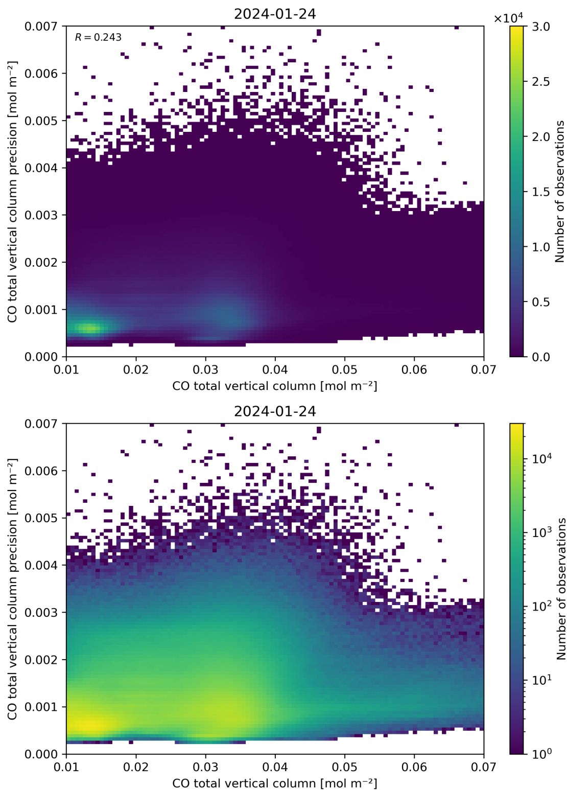
Figure 34: Scatter density plot of “CO total vertical column” against “CO total vertical column precision” for 2024-01-23 to 2024-01-25.
