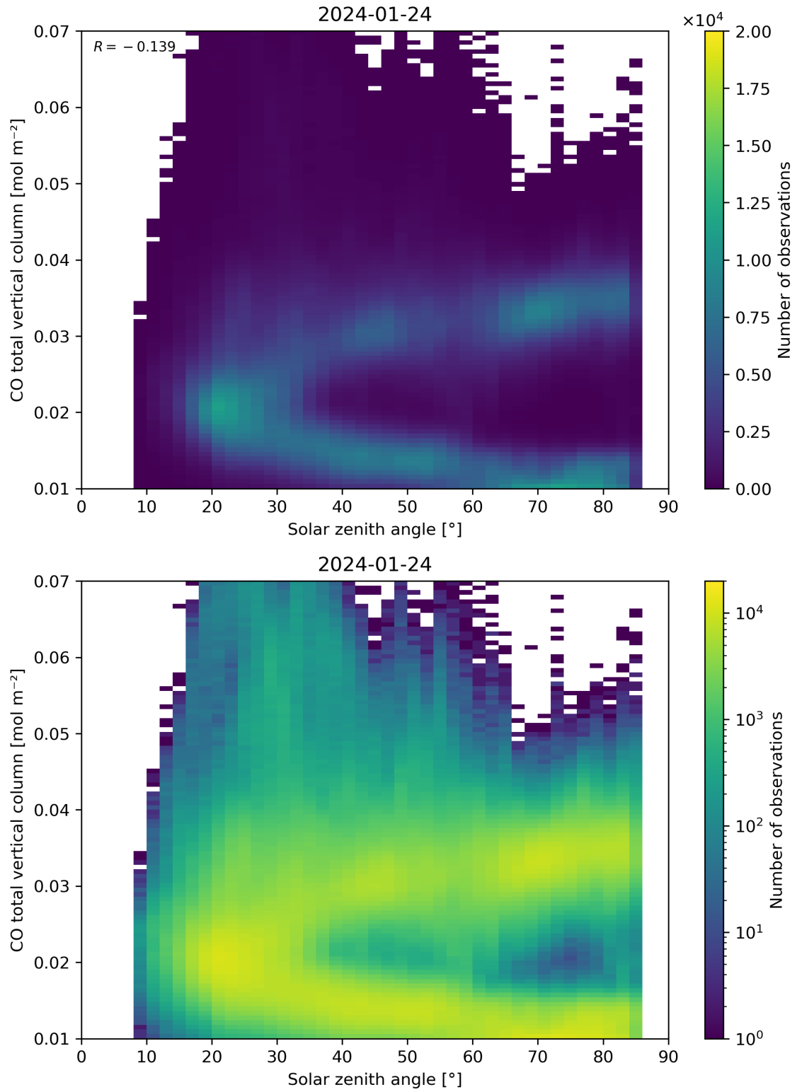
Figure 61: Scatter density plot of “Solar zenith angle” against “CO total vertical column” for 2024-01-23 to 2024-01-25.
