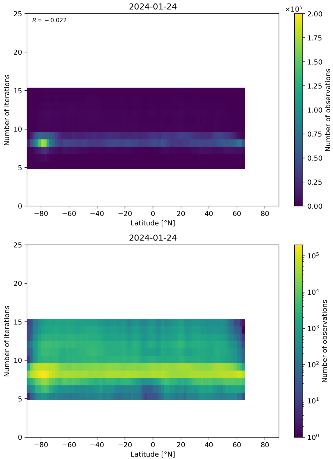
Figure 56: Scatter density plot of “Latitude” against “Number of iterations” for 2024-01-23 to 2024-01-25.
