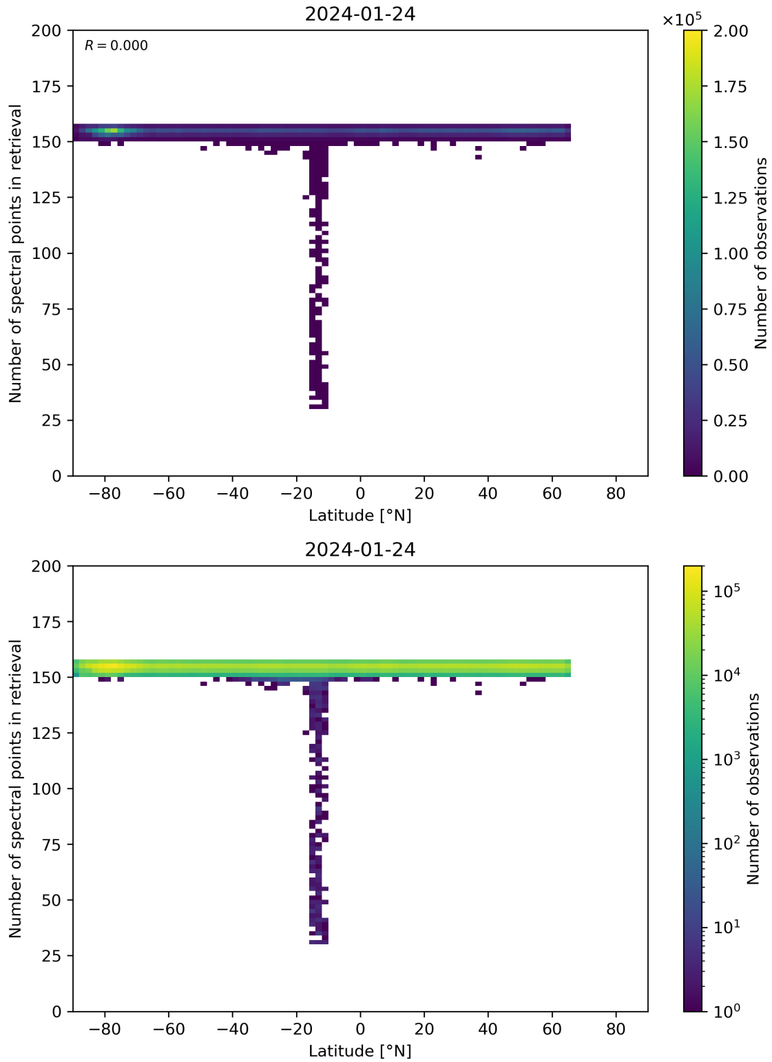
Figure 57: Scatter density plot of “Latitude” against “Number of spectral points in retrieval” for 2024-01-23 to 2024-01-25.
