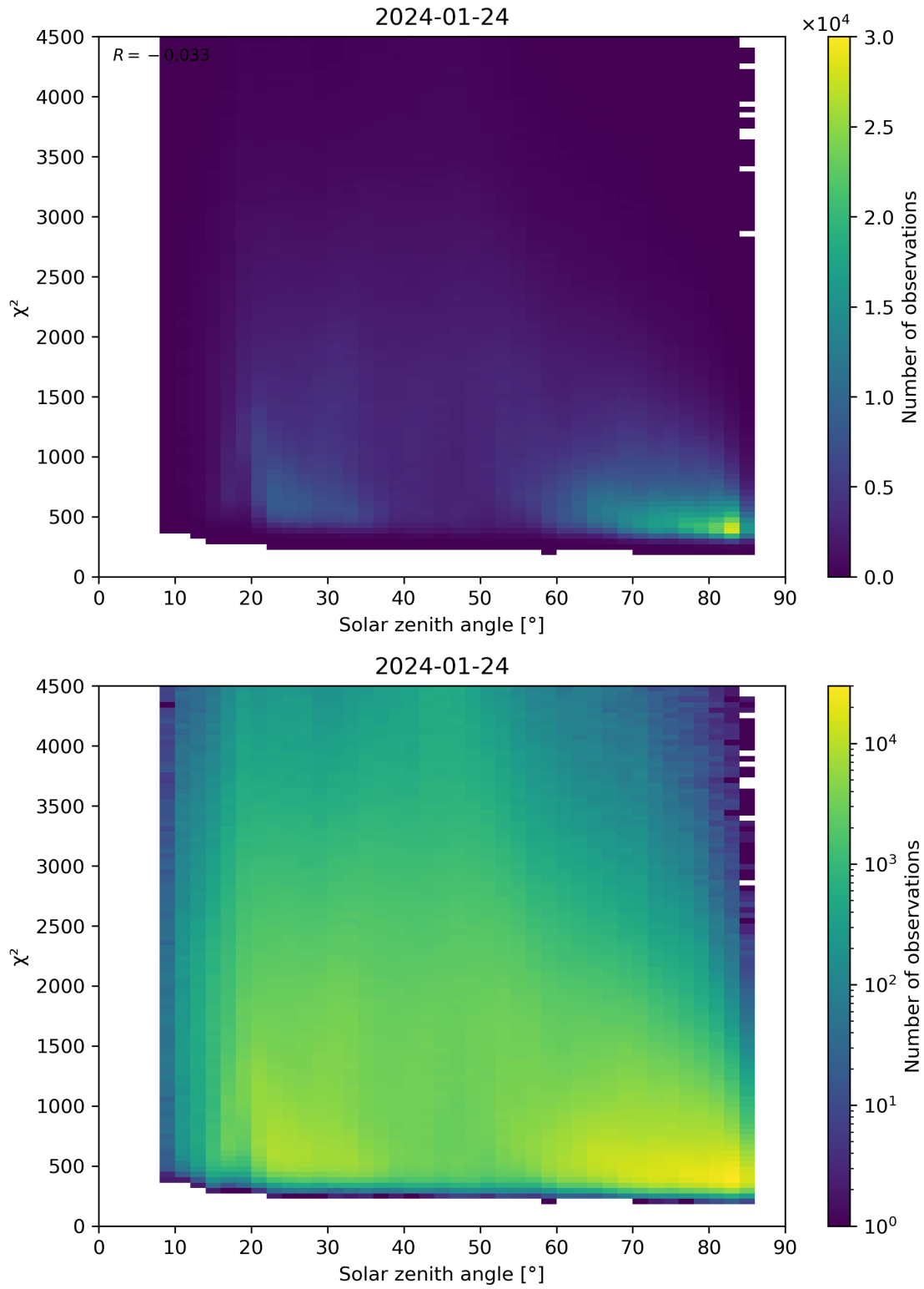
Figure 64: Scatter density plot of “Solar zenith angle” against “ \chi^2 ” for 2024-01-23 to 2024-01-25.
