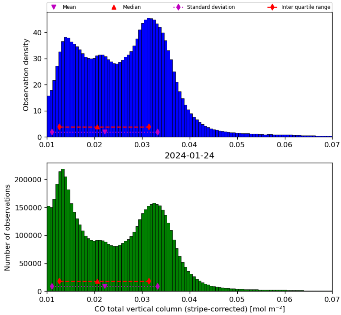
Figure 19: Histogram of “CO total vertical column (stripe-corrected)” for 2024-01-23 to 2024-01-25
