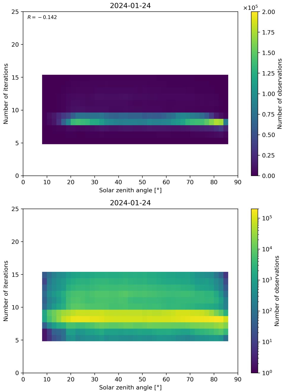
Figure 67: Scatter density plot of “Solar zenith angle” against “Number of iterations” for 2024-01-23 to 2024-01-25.
