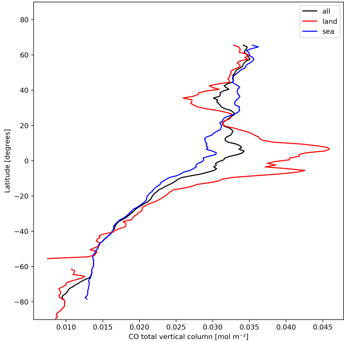
Figure 10: Zonal average of “CO total vertical column” for 2024-01-23 to 2024-01-25.
