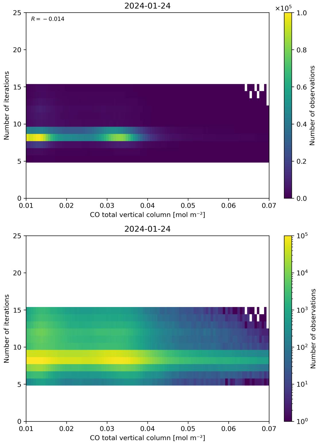
Figure 42: Scatter density plot of “CO total vertical column” against “Number of iterations” for 2024-01-23 to 2024-01-25.
