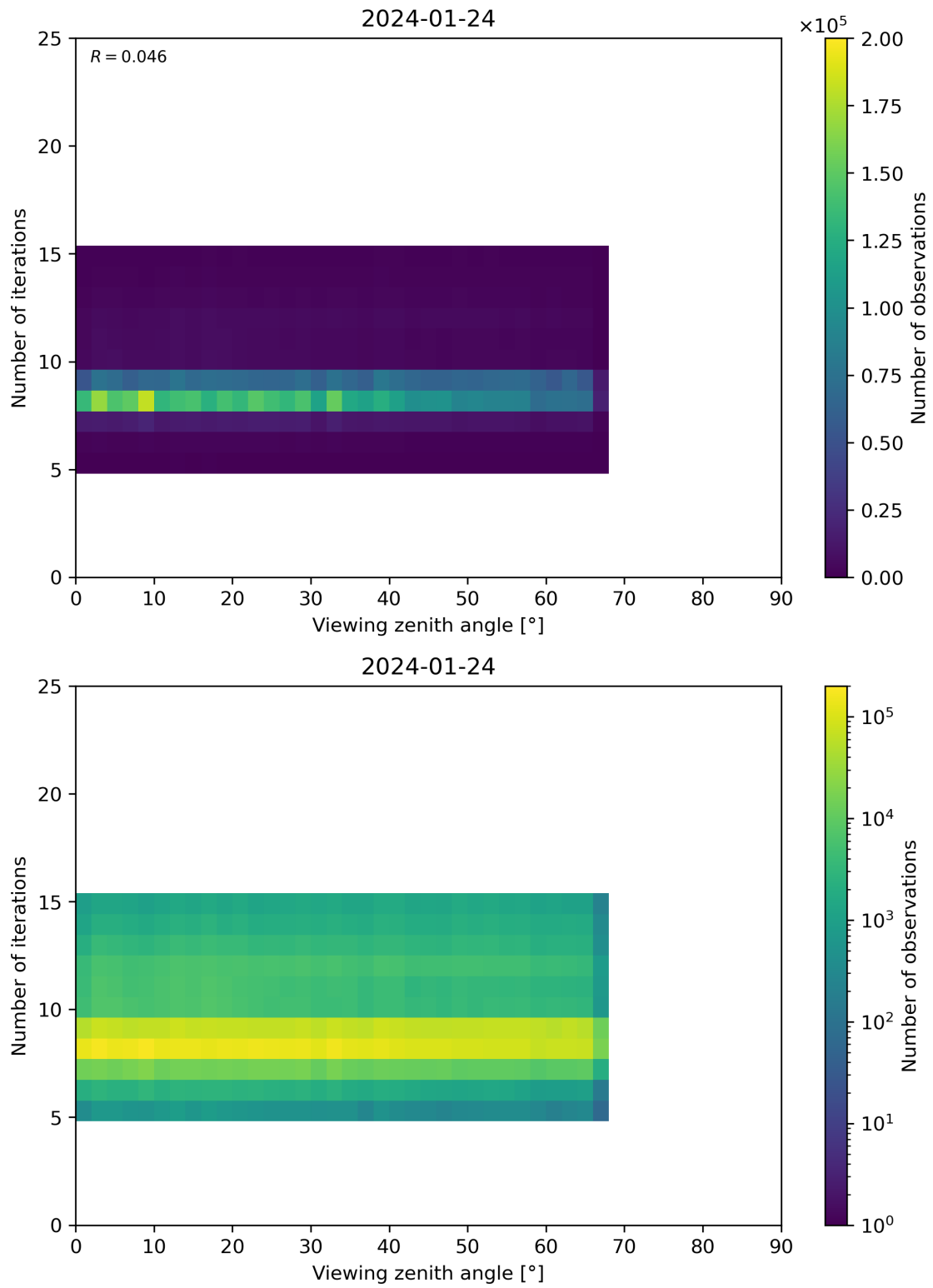
Figure 75: Scatter density plot of “Viewing zenith angle” against “Number of iterations” for 2024-01-23 to 2024-01-25.
