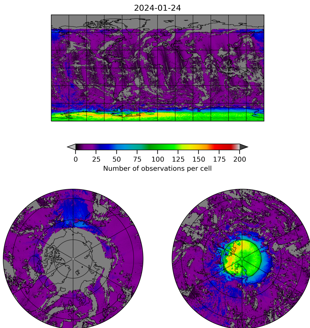
Figure 8: Map of the number of observations for 2024-01-23 to 2024-01-25
