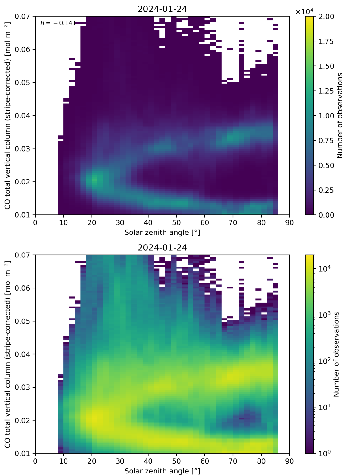
Figure 62: Scatter density plot of “Solar zenith angle” against “CO total vertical column (stripe-corrected)” for 2024-01-23 to 2024-01-25.
