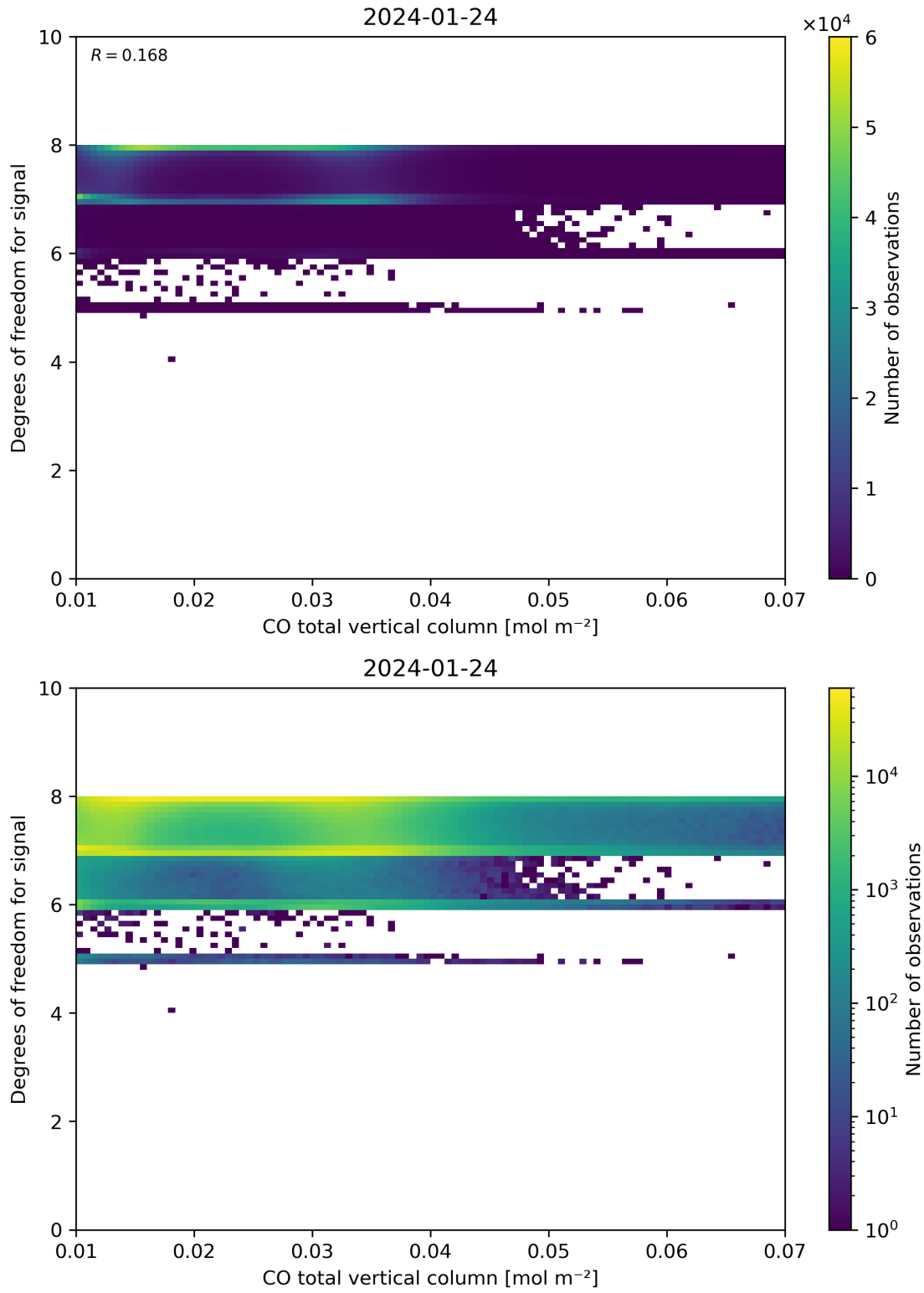
Figure 41: Scatter density plot of “CO total vertical column” against “Degrees of freedom for signal” for 2024-01-23 to 2024-01-25.
