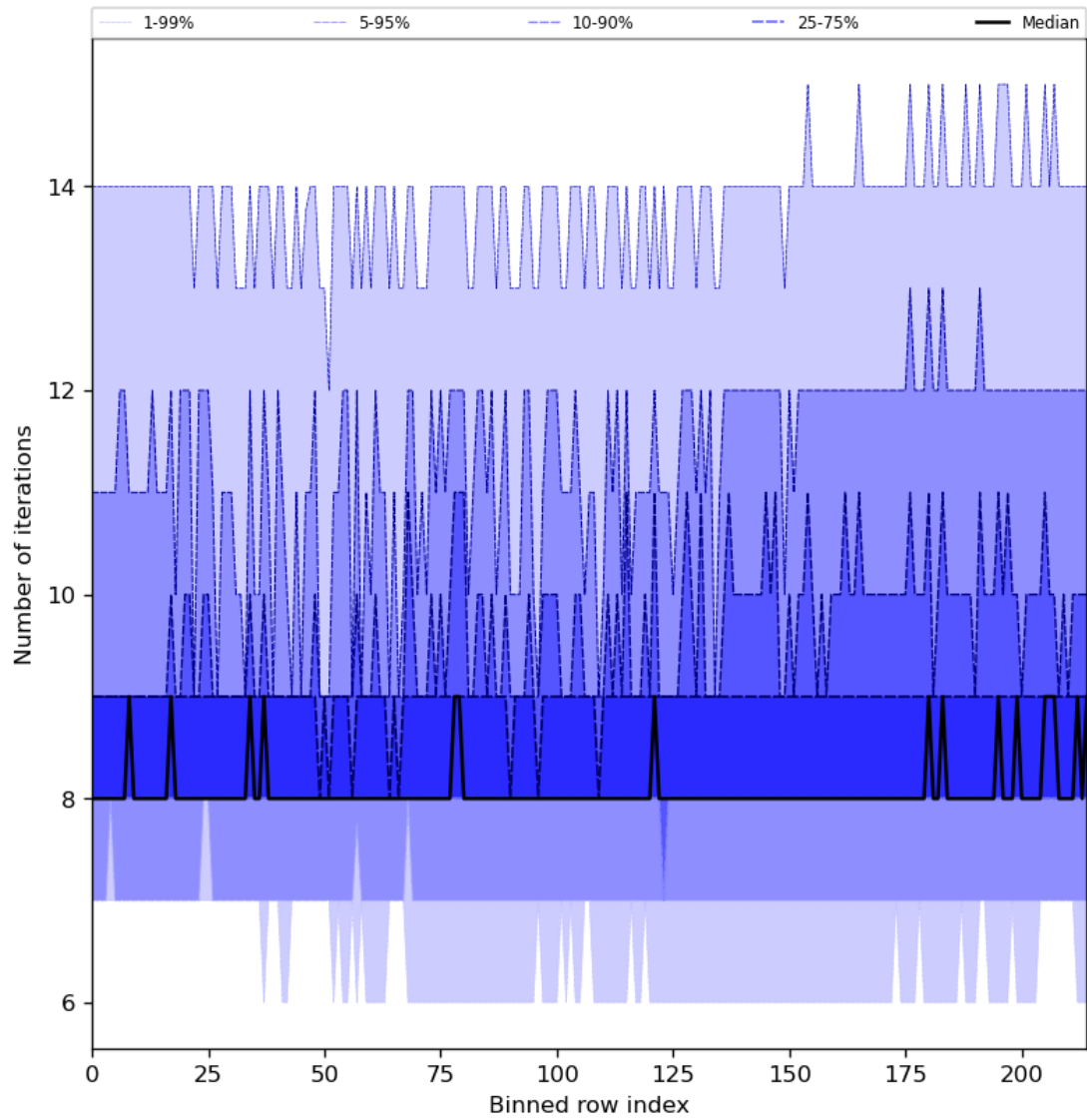
Figure 32: Along track statistics of “Number of iterations” for 2024-01-23 to 2024-01-25
