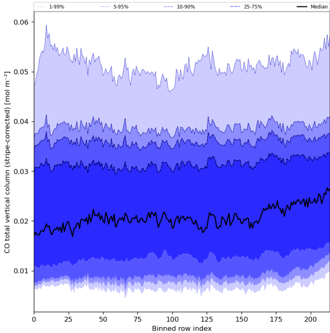
Figure 27: Along track statistics of “CO total vertical column (stripe-corrected)” for 2024-01-23 to 2024-01-25
