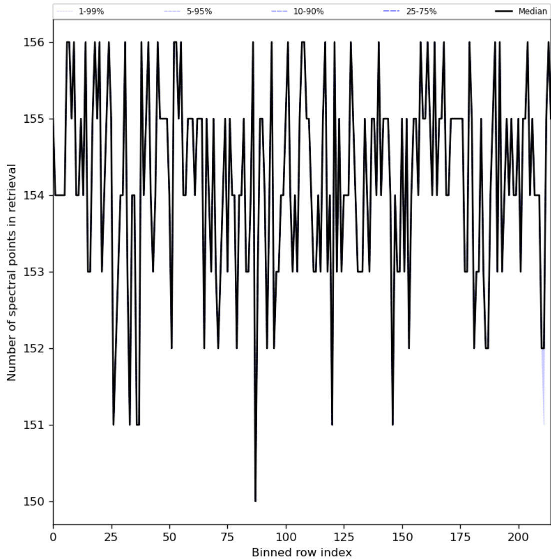
Figure 29: Along track statistics of “Number of spectral points in retrieval” for 2024-01-23 to 2024-01-25
