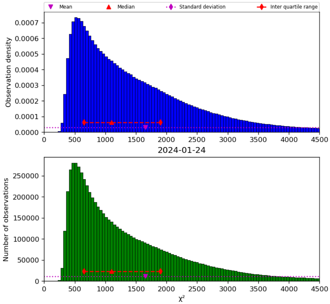
Figure 22: Histogram of “ \chi^2 ” for 2024-01-23 to 2024-01-25
