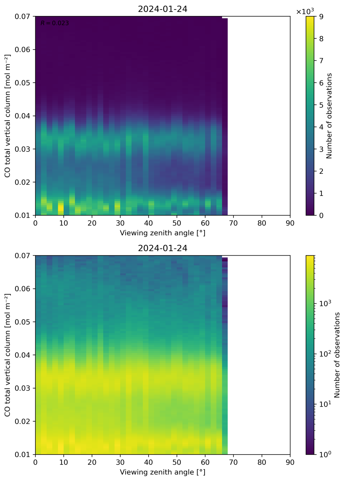
Figure 69: Scatter density plot of “Viewing zenith angle” against “CO total vertical column” for 2024-01-23 to 2024-01-25.
