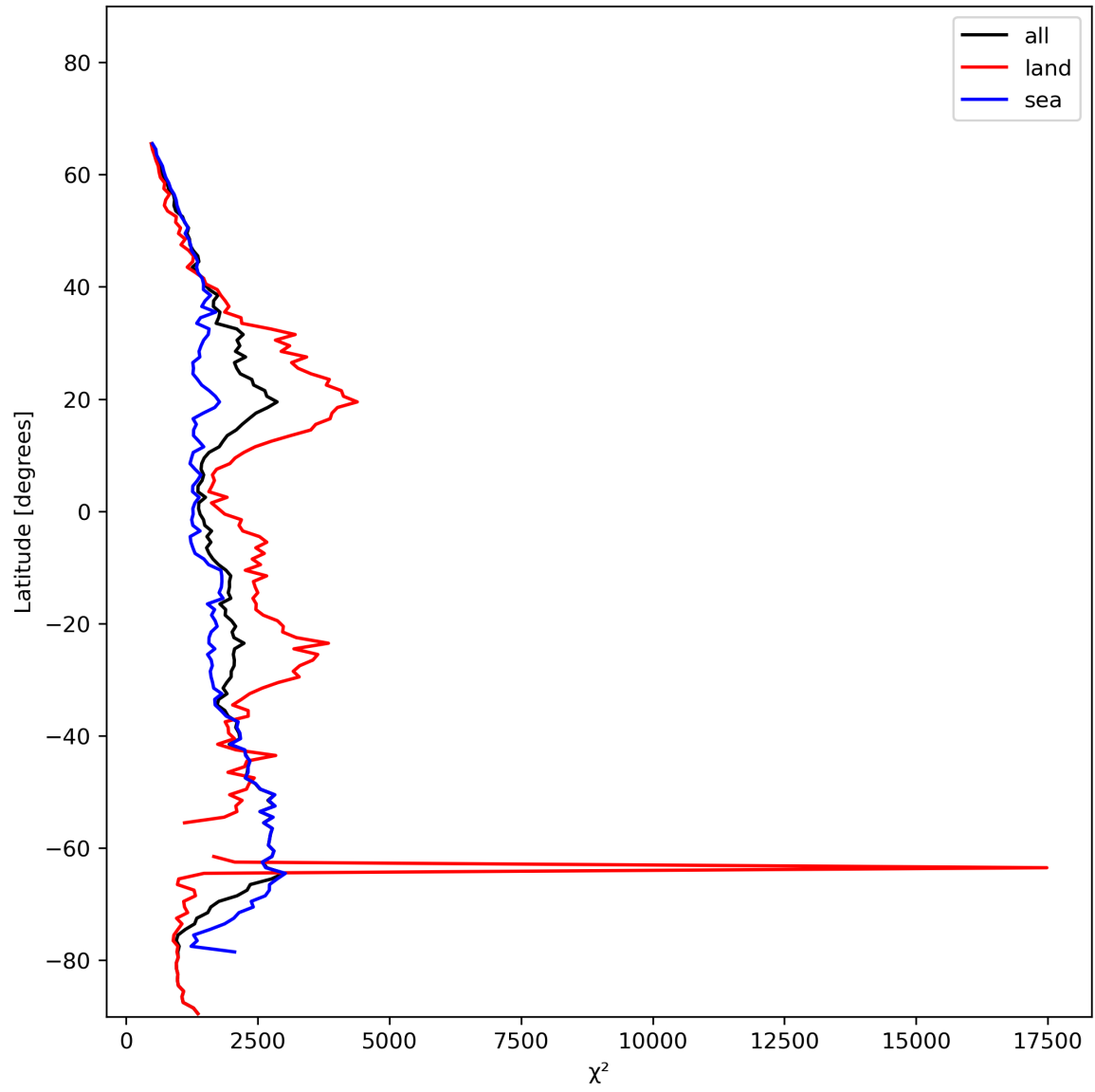
Figure 14: Zonal average of “ \chi^2 ” for 2024-01-23 to 2024-01-25.
