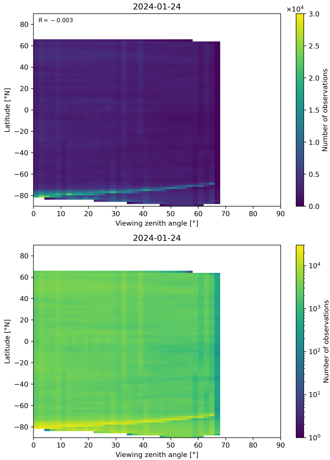
Figure 74: Scatter density plot of “Viewing zenith angle” against “Latitude” for 2024-01-23 to 2024-01-25.
