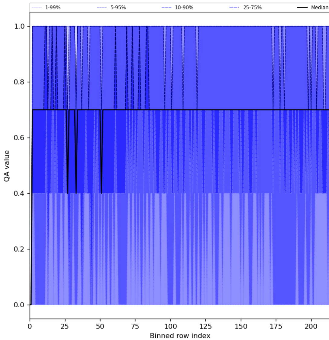
Figure 25: Along track statistics of “QA value” for 2024-01-23 to 2024-01-25
