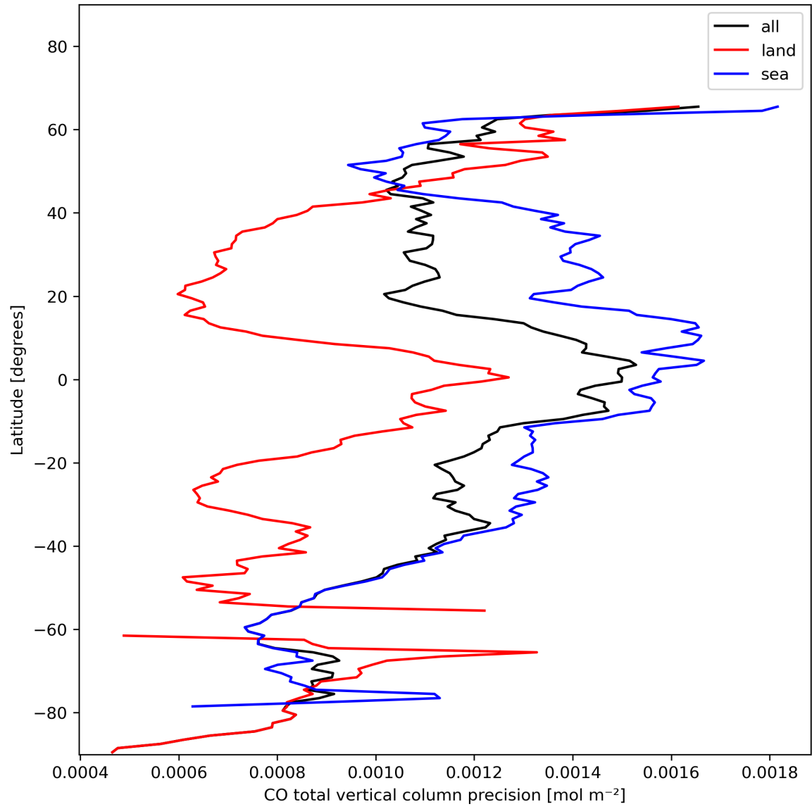
Figure 12: Zonal average of “CO total vertical column precision” for 2024-01-23 to 2024-01-25.
