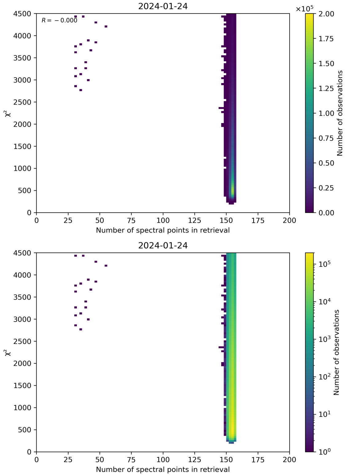
Figure 58: Scatter density plot of “Number of spectral points in retrieval” against “ \chi^2 ” for 2024-01-23 to 2024-01-25.
