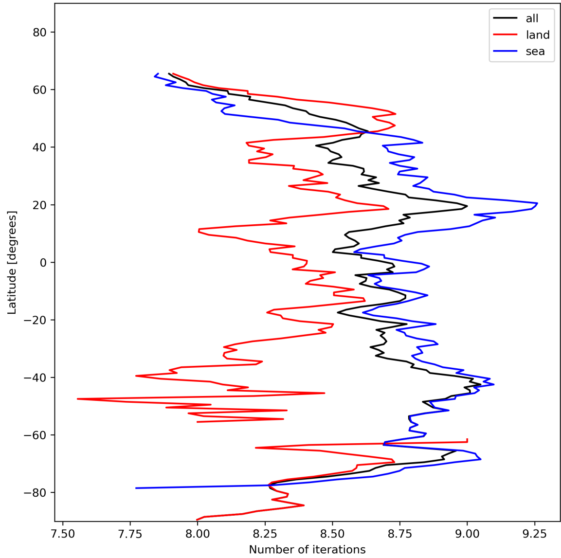
Figure 16: Zonal average of “Number of iterations” for 2024-01-23 to 2024-01-25.
