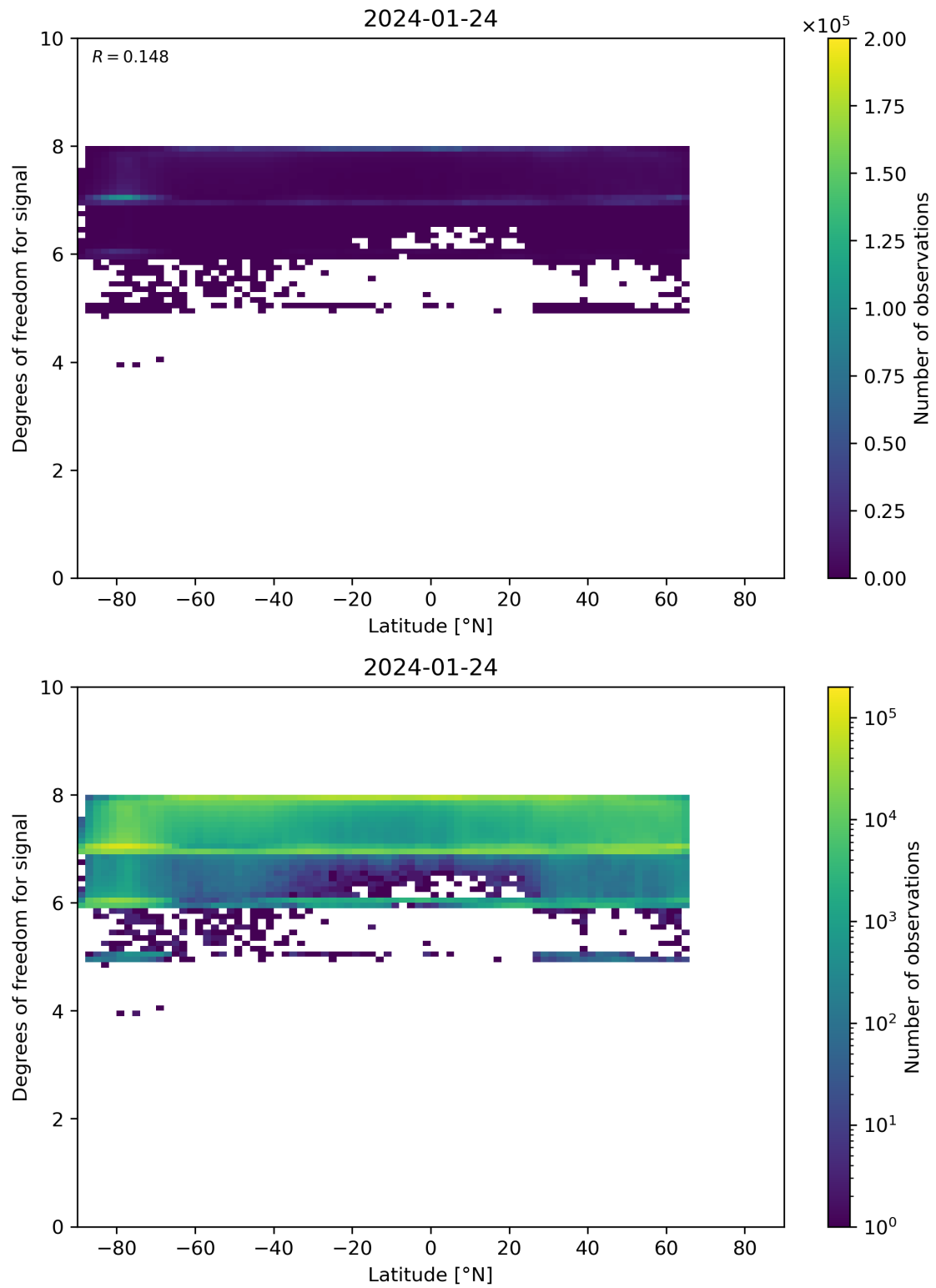
Figure 55: Scatter density plot of “Latitude” against “Degrees of freedom for signal” for 2024-01-23 to 2024-01-25.
