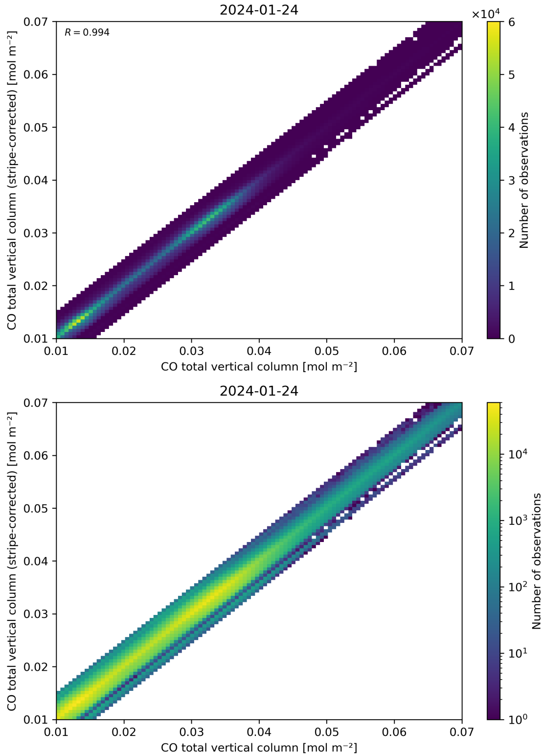
Figure 33: Scatter density plot of “CO total vertical column” against “CO total vertical column (stripe-corrected)” for 2024-01-23 to 2024-01-25.
