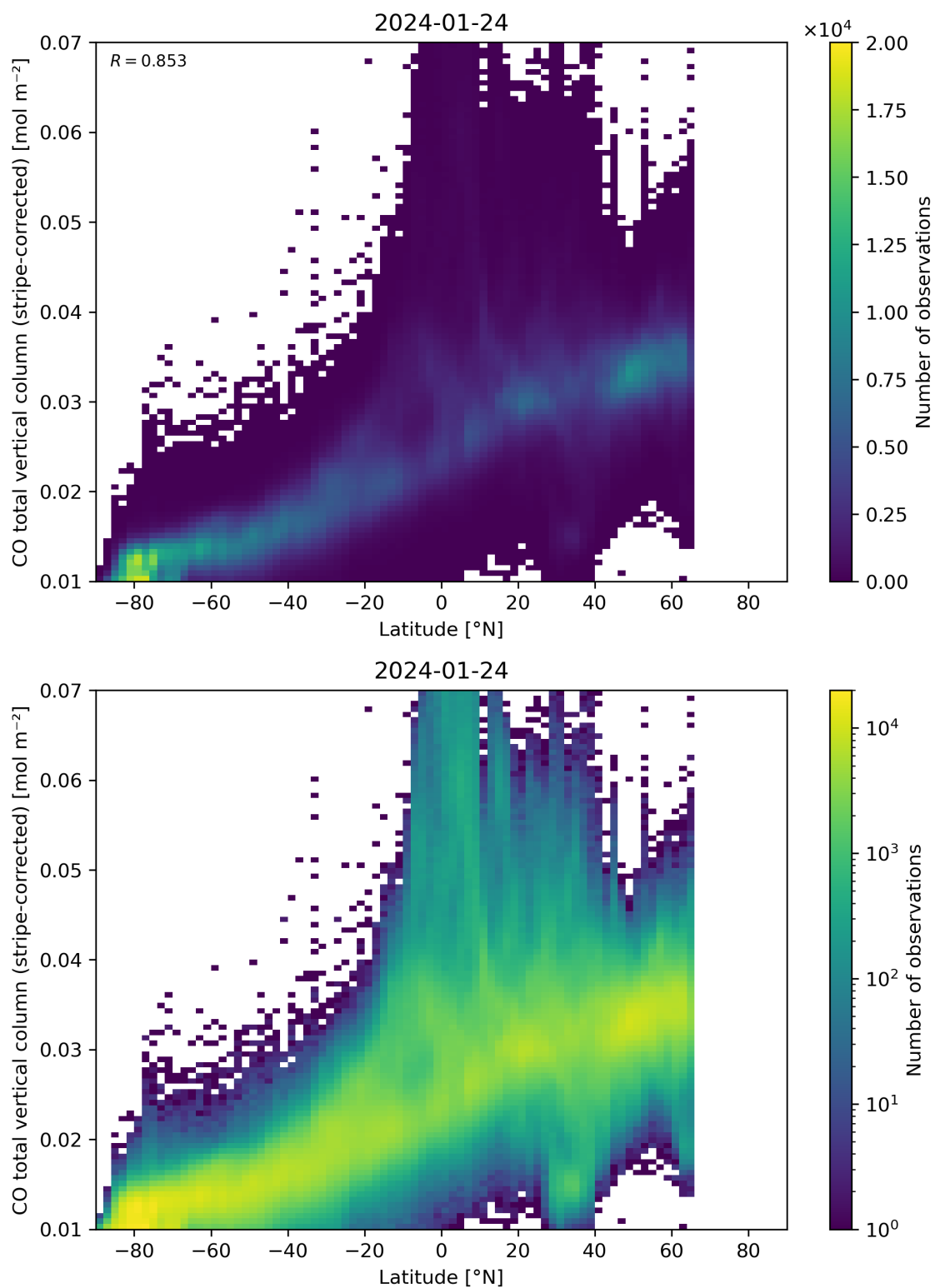
Figure 52: Scatter density plot of “Latitude” against “CO total vertical column (stripe-corrected)” for 2024-01-23 to 2024-01-25.
