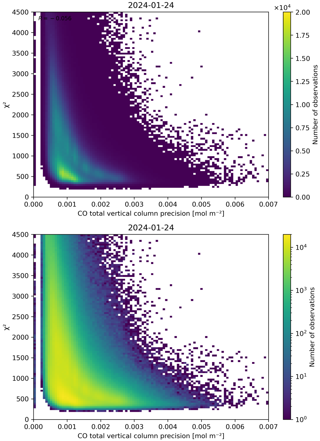
Figure 44: Scatter density plot of “CO total vertical column precision” against “ \chi^2 ” for 2024-01-23 to 2024-01-25.
