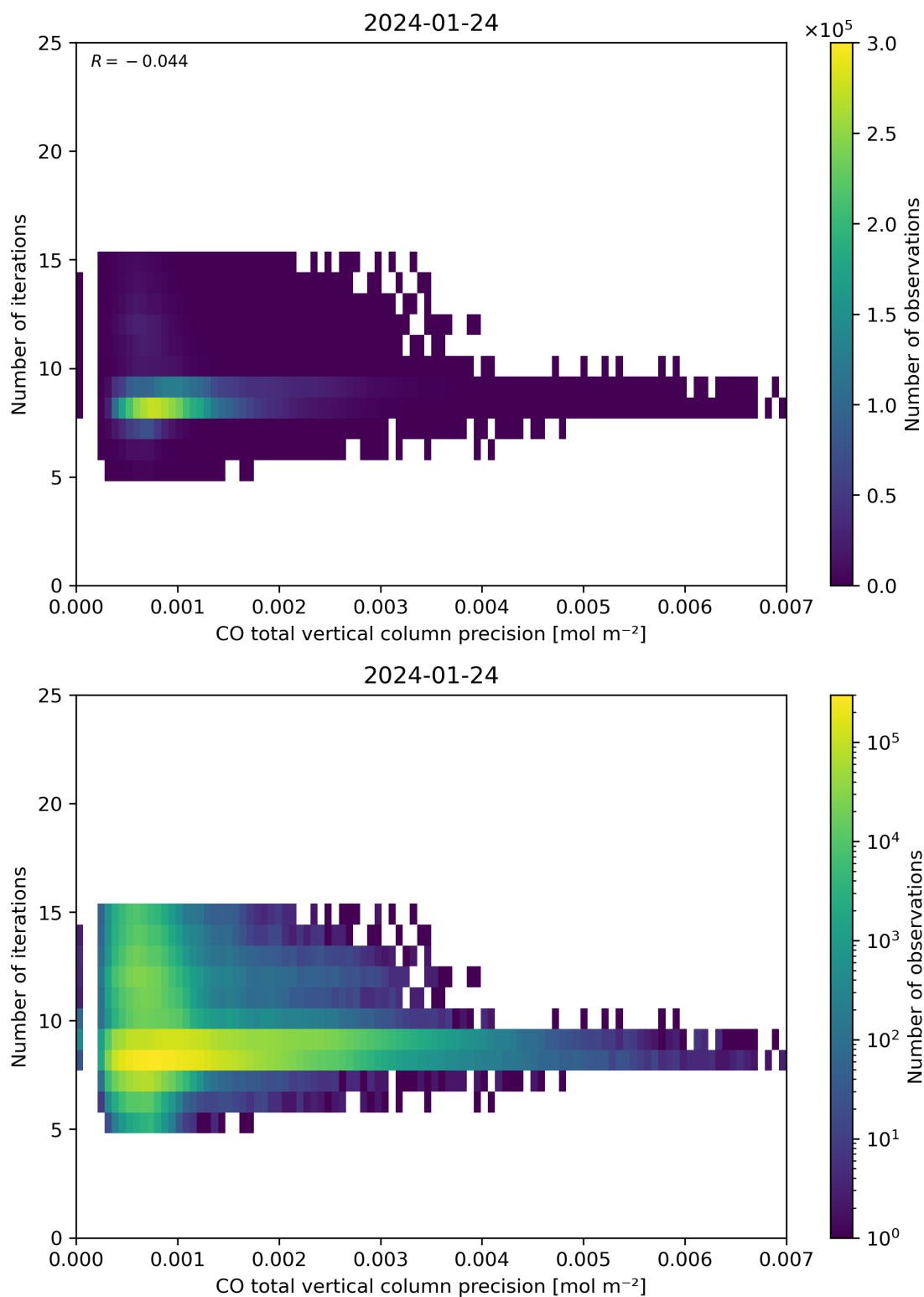
Figure 46: Scatter density plot of “CO total vertical column precision” against “Number of iterations” for 2024-01-23 to 2024-01-25.
