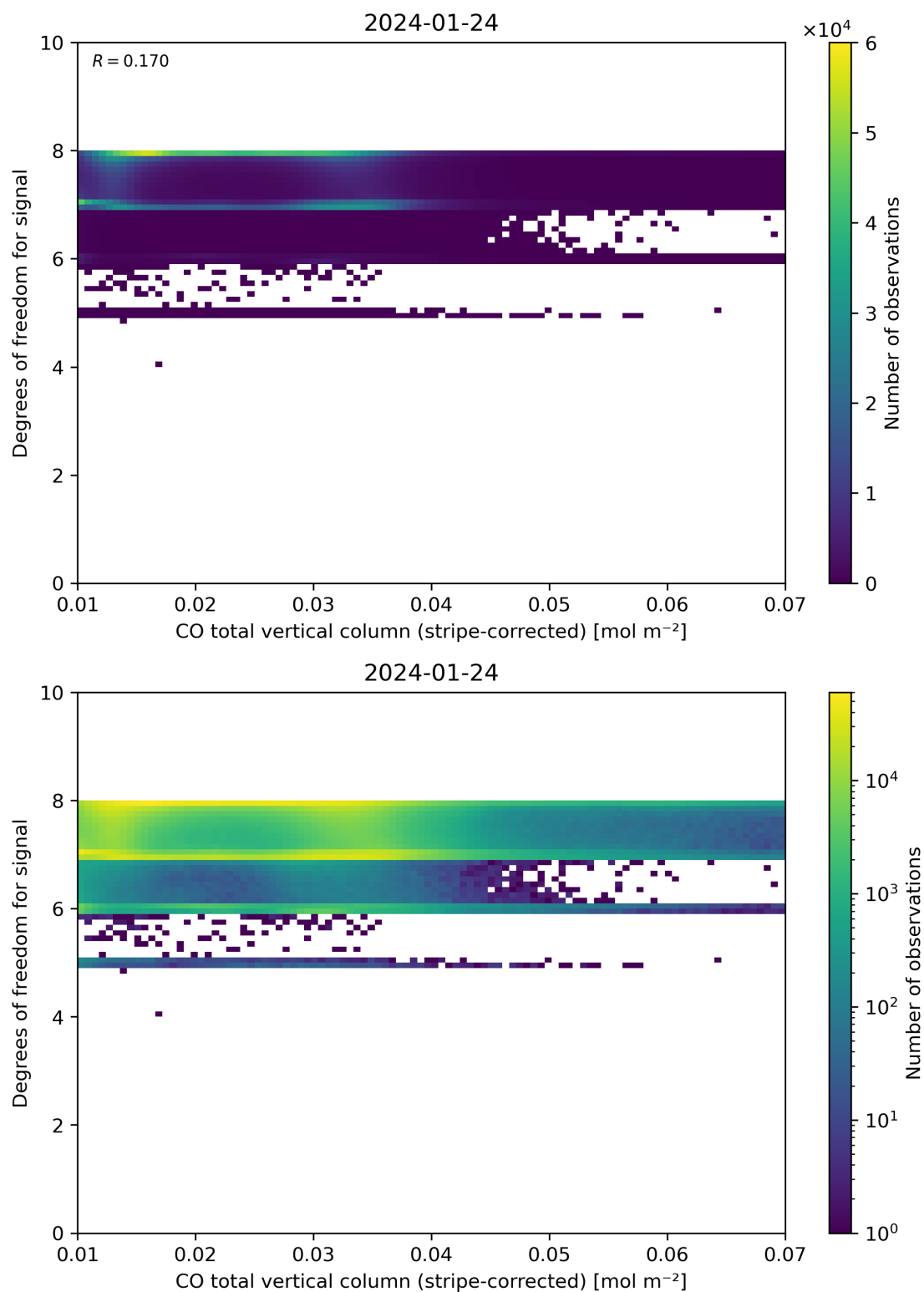
Figure 38: Scatter density plot of “CO total vertical column (stripe-corrected)” against “Degrees of freedom for signal” for 2024-01-23 to 2024-01-25.
