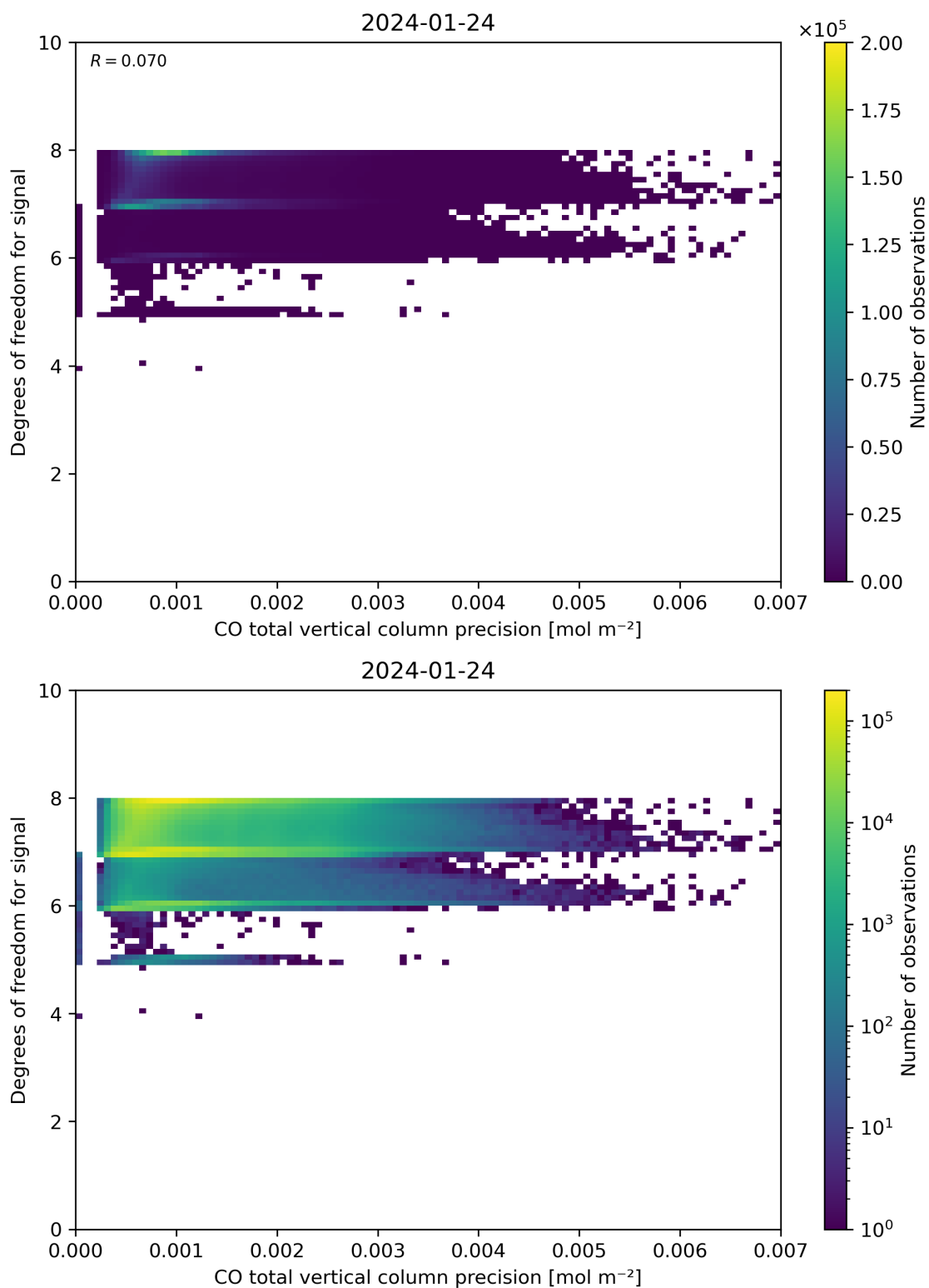
Figure 45: Scatter density plot of “CO total vertical column precision” against “Degrees of freedom for signal” for 2024-01-23 to 2024-01-25.
