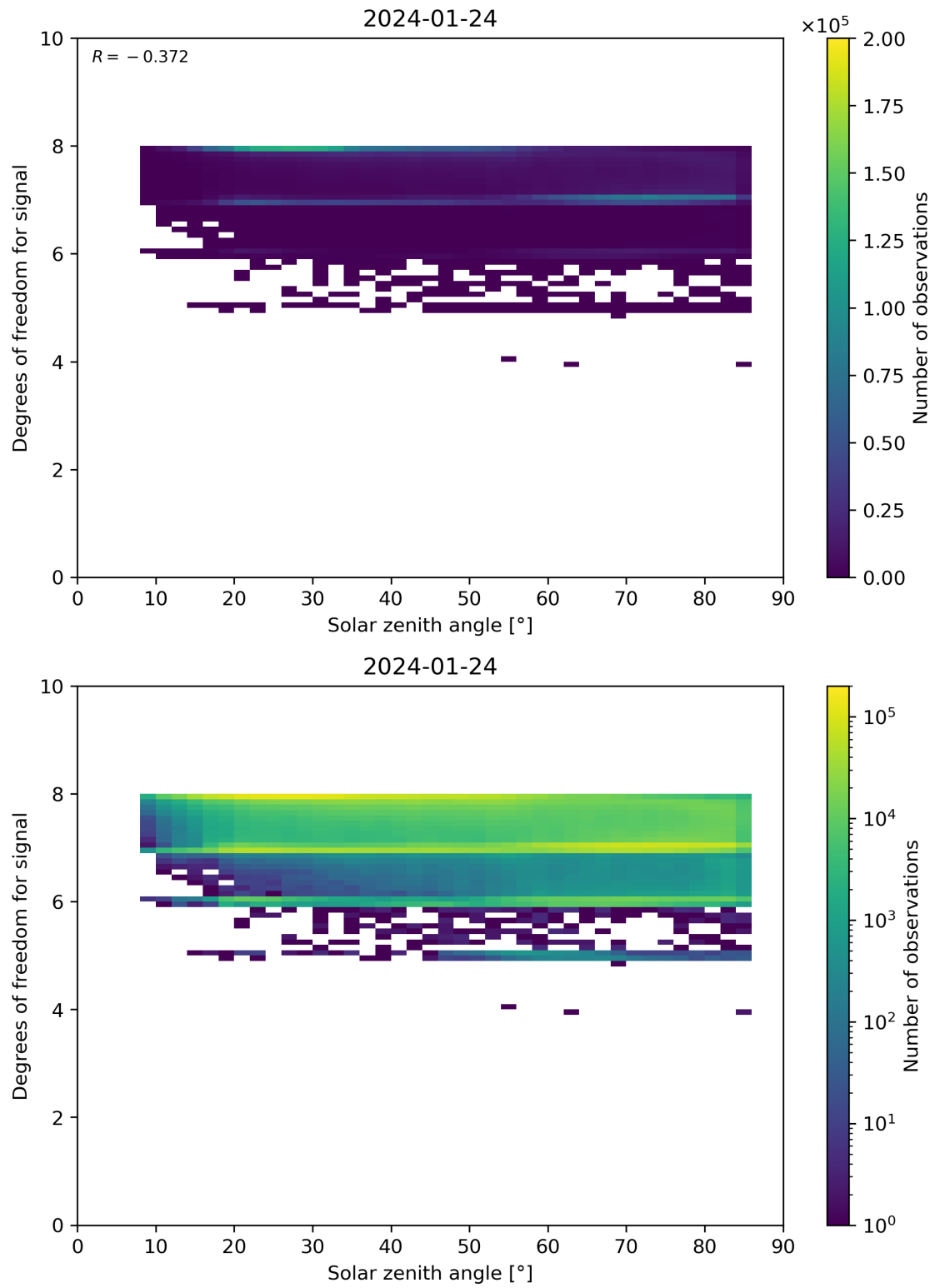
Figure 65: Scatter density plot of “Solar zenith angle” against “Degrees of freedom for signal” for 2024-01-23 to 2024-01-25.
