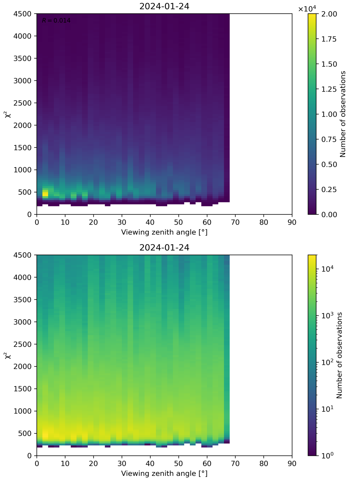
Figure 72: Scatter density plot of “Viewing zenith angle” against “ \chi^2 ” for 2024-01-23 to 2024-01-25.
