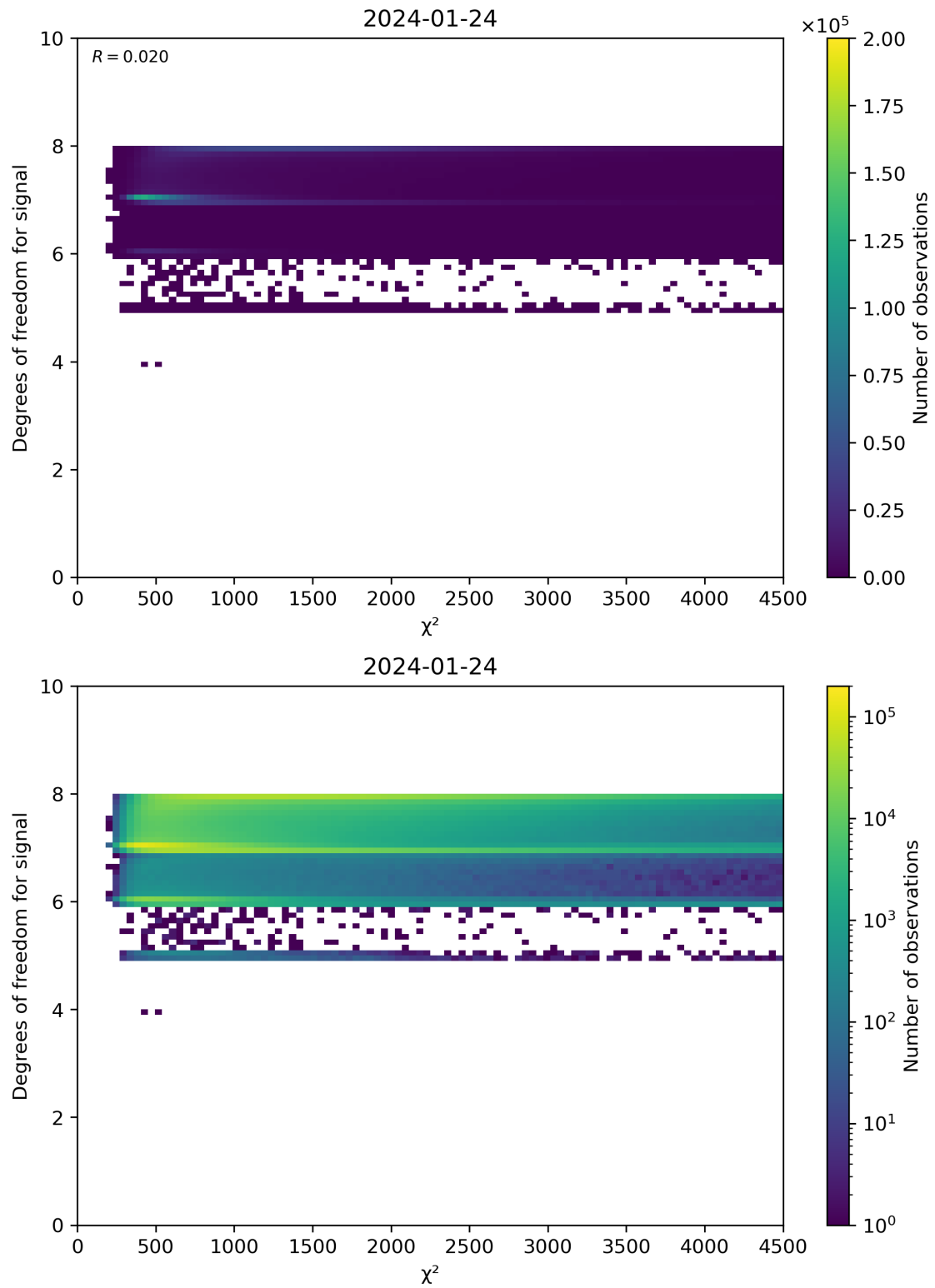
Figure 48: Scatter density plot of “ \chi^2 ” against “Degrees of freedom for signal” for 2024-01-23 to 2024-01-25.
