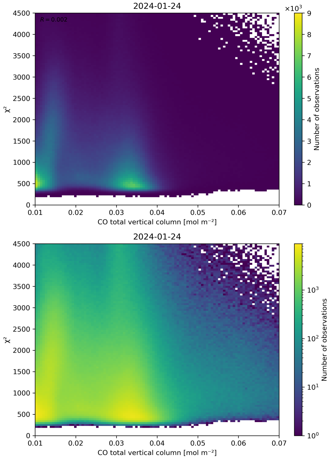
Figure 35: Scatter density plot of “CO total vertical column” against “ \chi^2 ” for 2024-01-23 to 2024-01-25.
