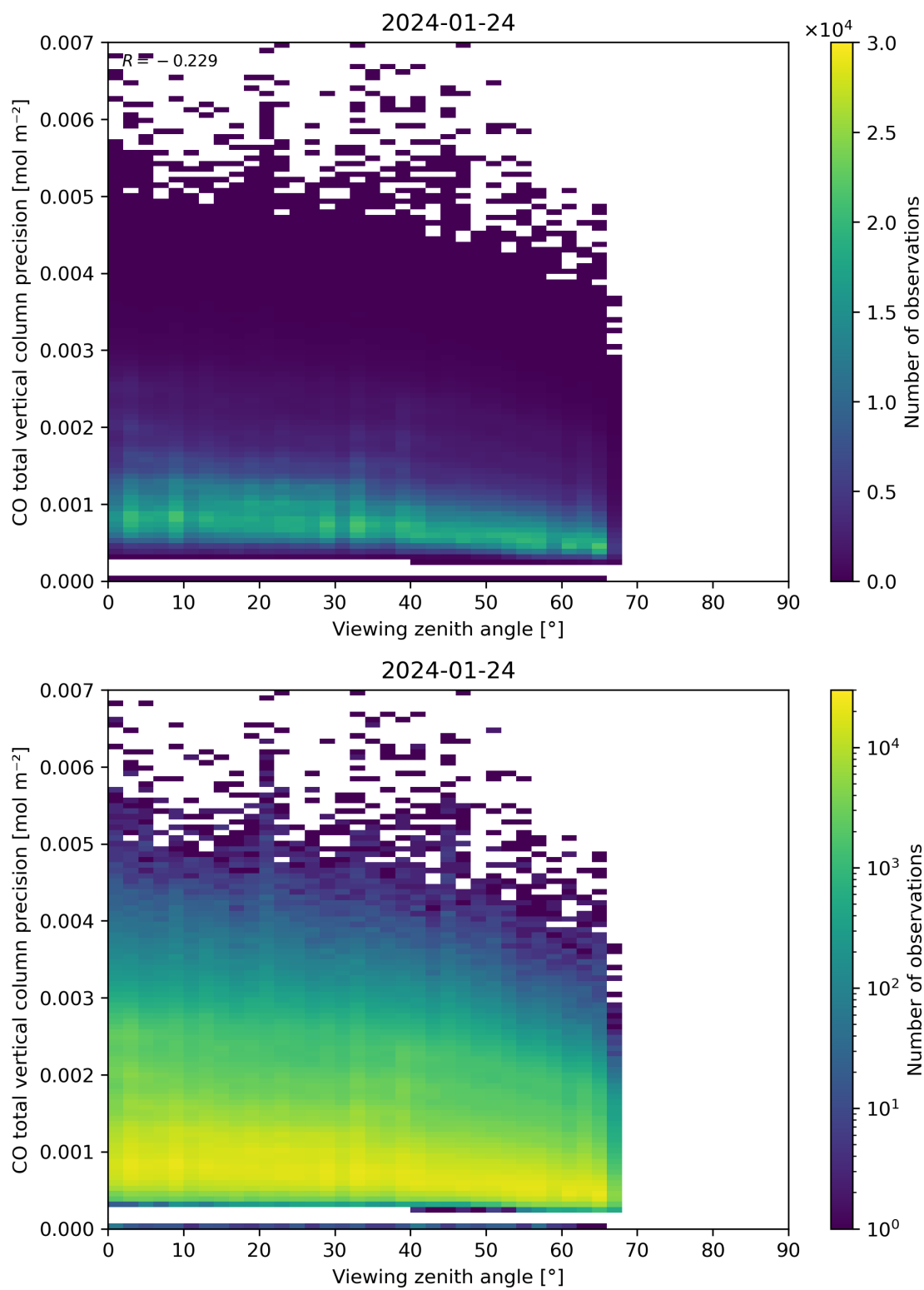
Figure 71: Scatter density plot of “Viewing zenith angle” against “CO total vertical column precision” for 2024-01-23 to 2024-01-25.
