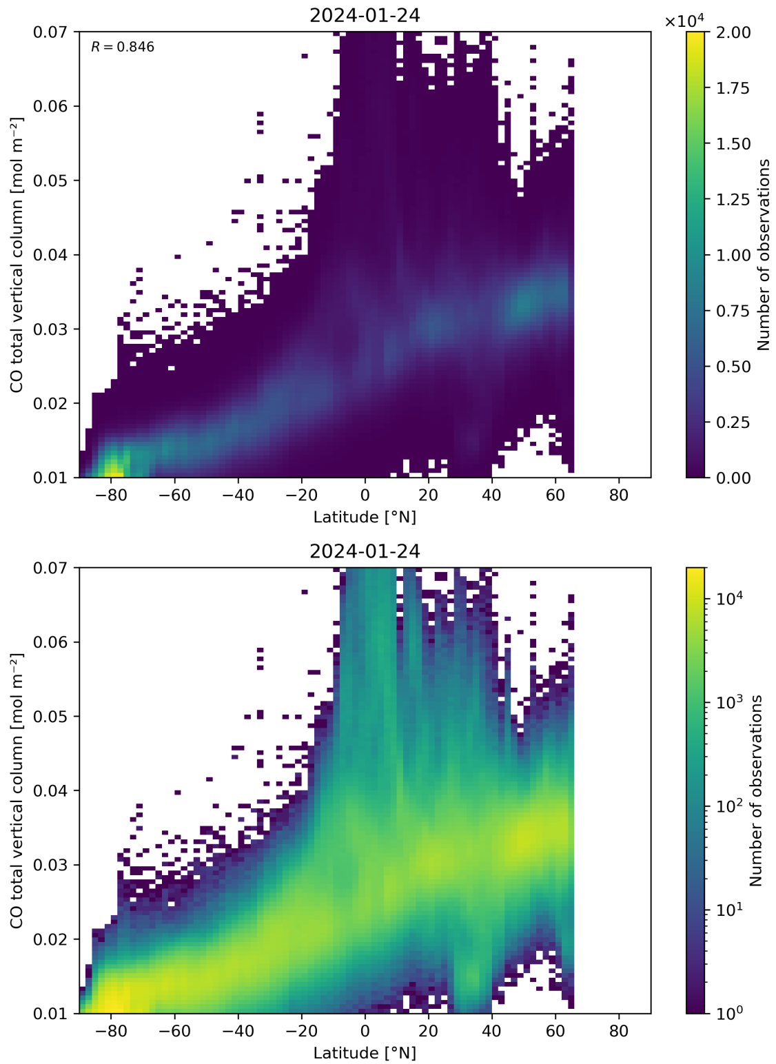
Figure 51: Scatter density plot of “Latitude” against “CO total vertical column” for 2024-01-23 to 2024-01-25.
