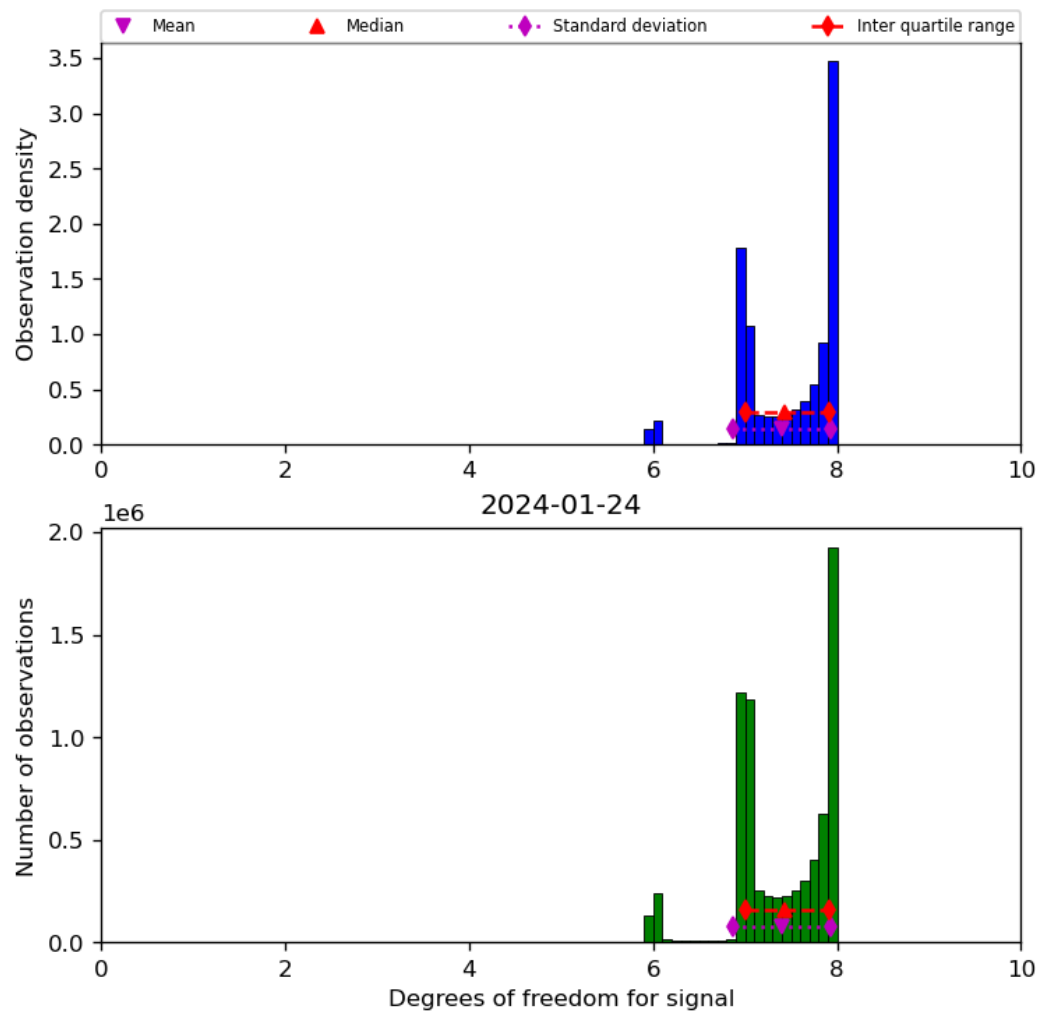
Figure 23: Histogram of “Degrees of freedom for signal” for 2024-01-23 to 2024-01-25
