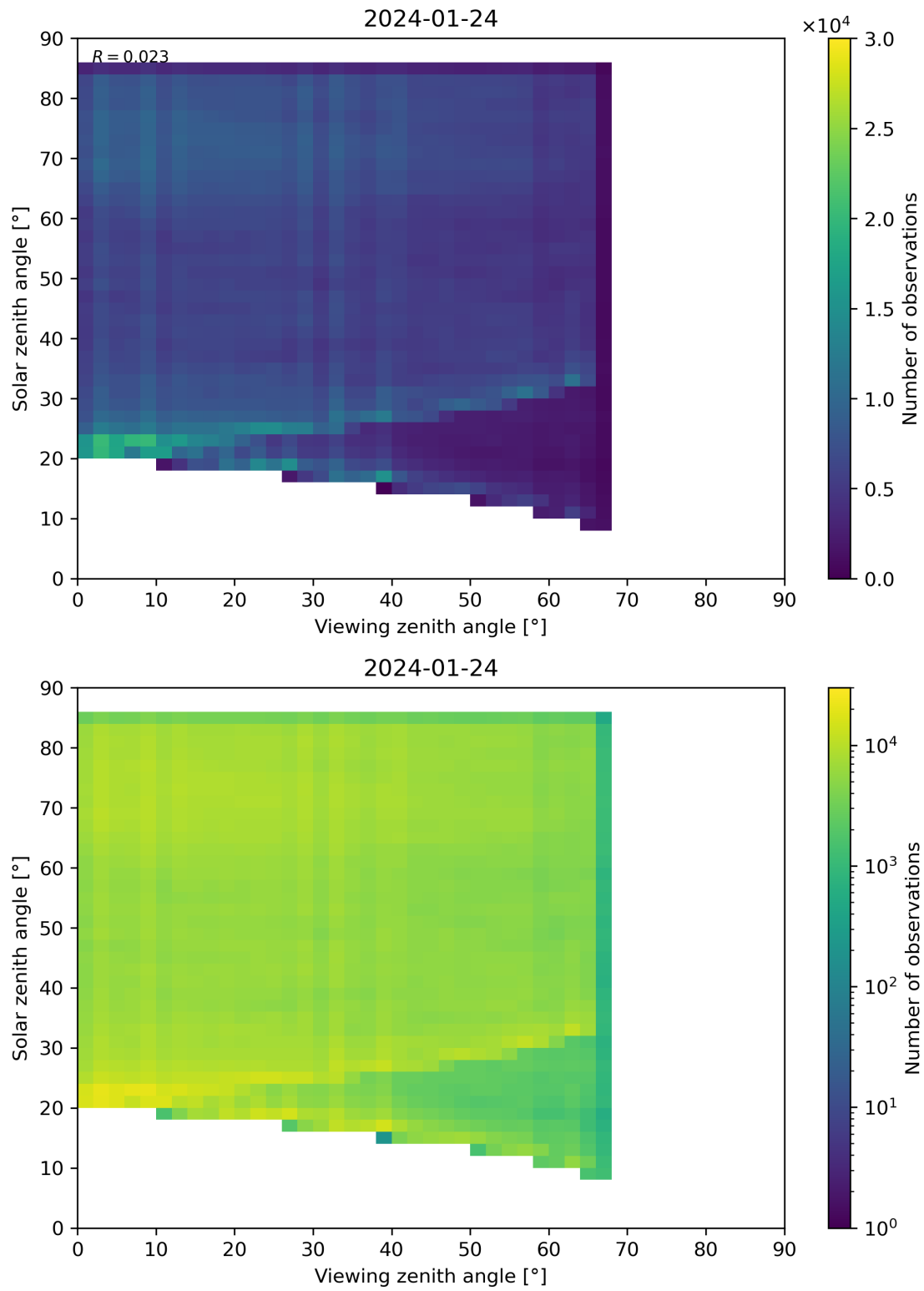
Figure 77: Scatter density plot of “Viewing zenith angle” against “Solar zenith angle” for 2024-01-23 to 2024-01-25.
