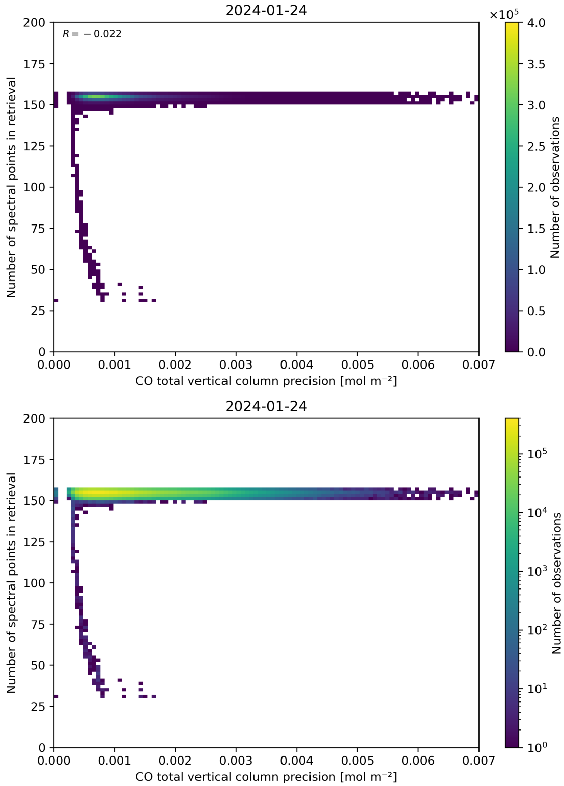
Figure 47: Scatter density plot of “CO total vertical column precision” against “Number of spectral points in retrieval” for 2024-01-23 to 2024-01-25.
