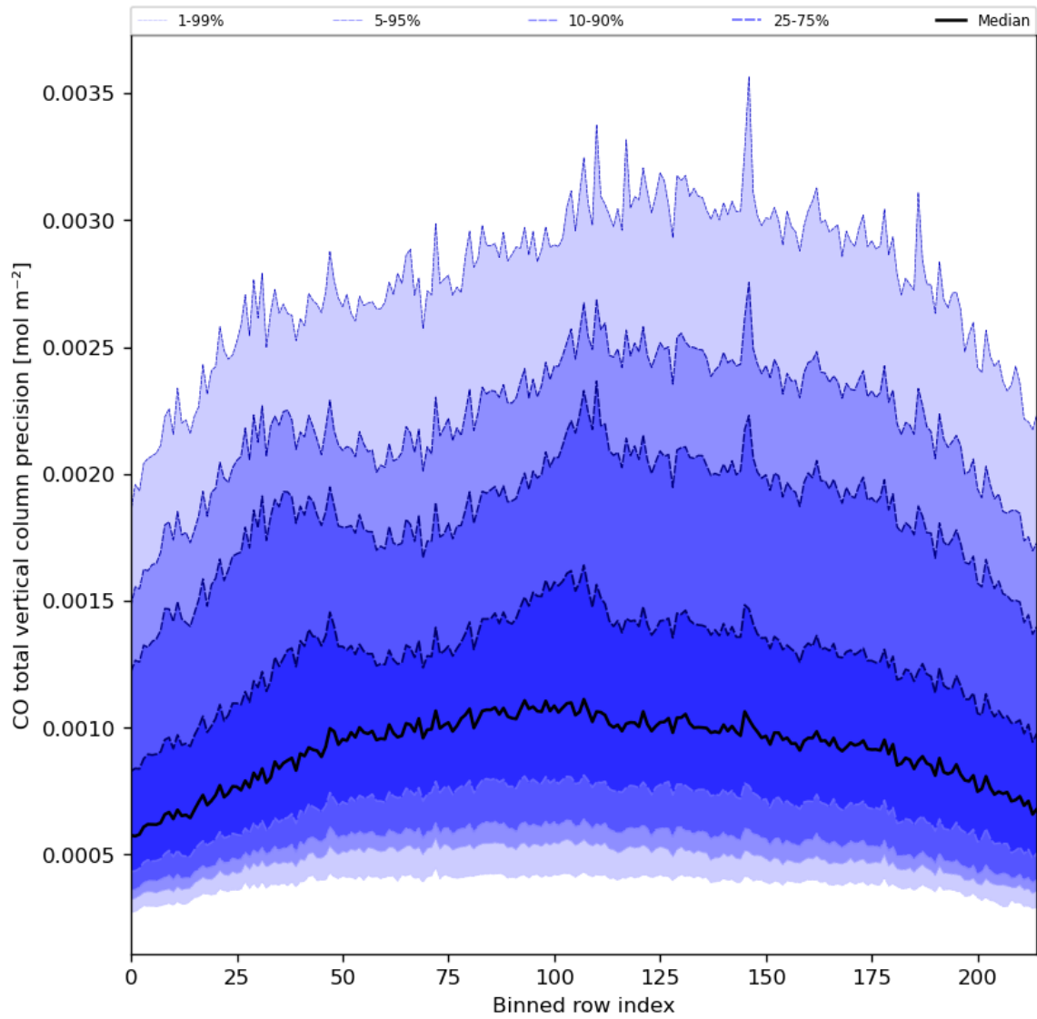
Figure 28: Along track statistics of “CO total vertical column precision” for 2024-01-23 to 2024-01-25
