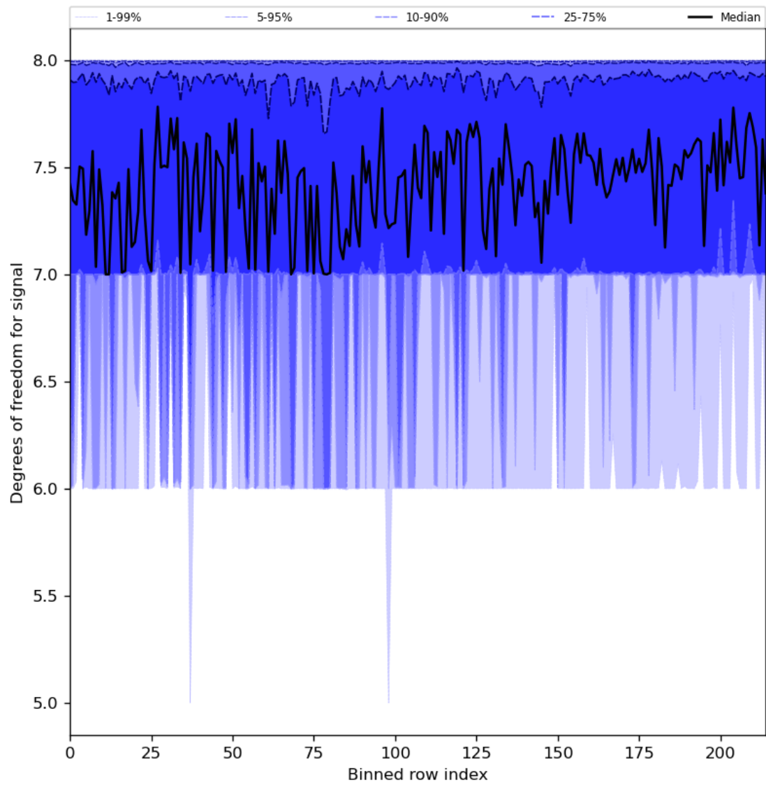
Figure 31: Along track statistics of “Degrees of freedom for signal” for 2024-01-23 to 2024-01-25
