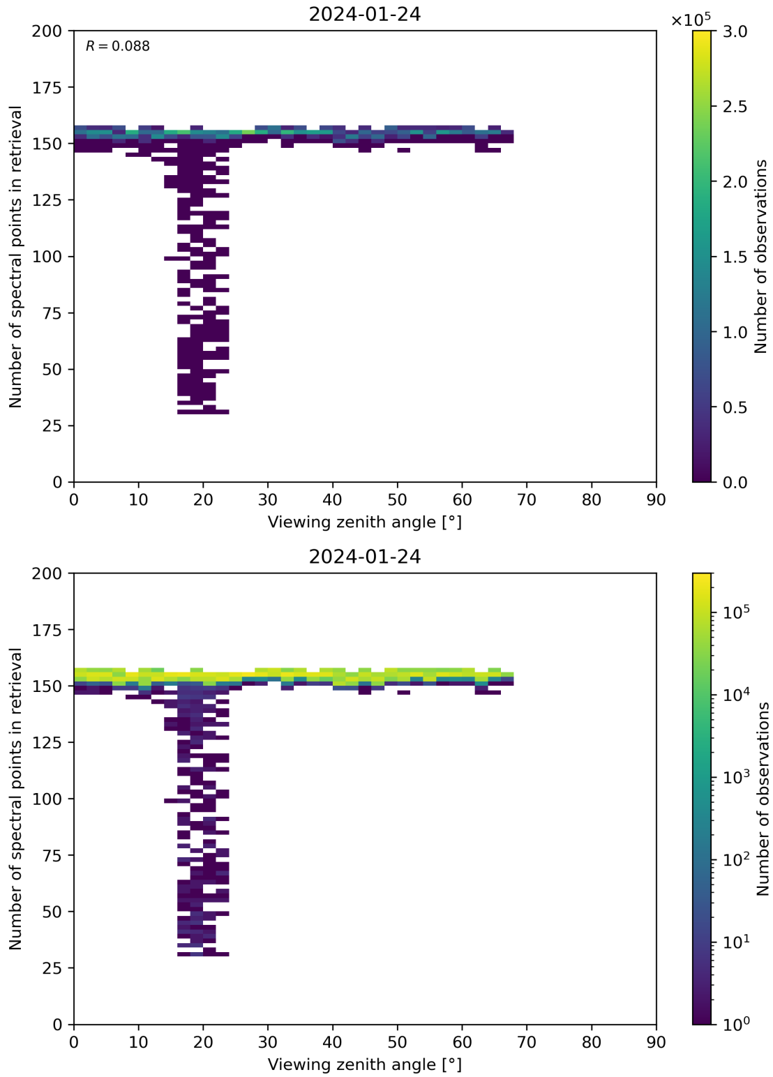
Figure 76: Scatter density plot of “Viewing zenith angle” against “Number of spectral points in retrieval” for 2024-01-23 to 2024-01-25.
