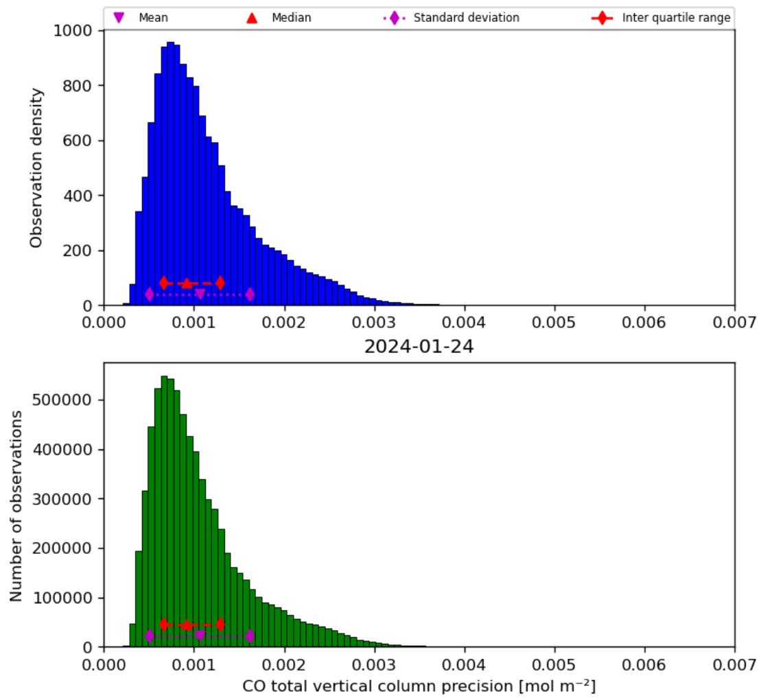
Figure 20: Histogram of “CO total vertical column precision” for 2024-01-23 to 2024-01-25
