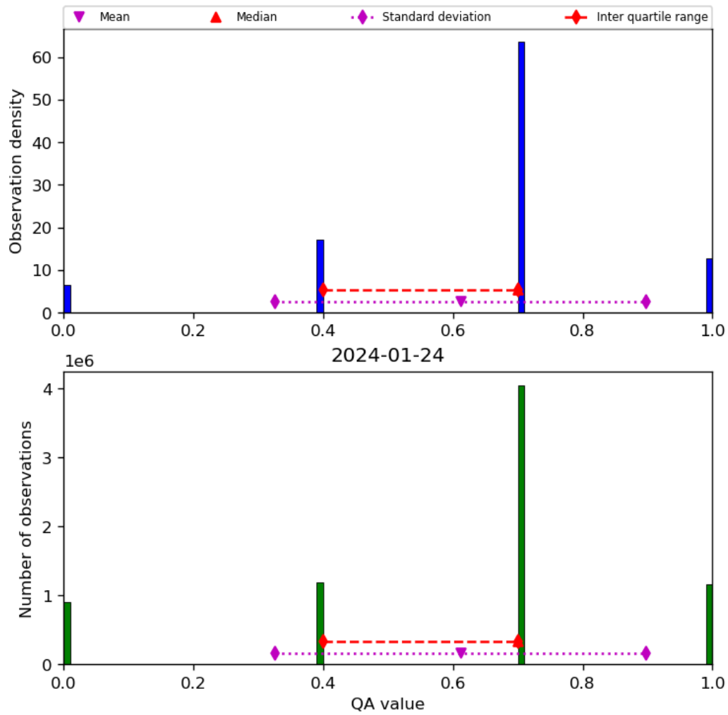
Figure 17: Histogram of “QA value” for 2024-01-23 to 2024-01-25
