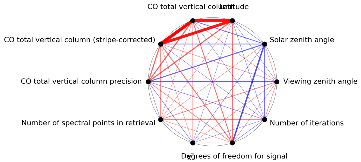
Figure 1: Map of correlation graph for 2024-01-23 to 2024-01-25.
