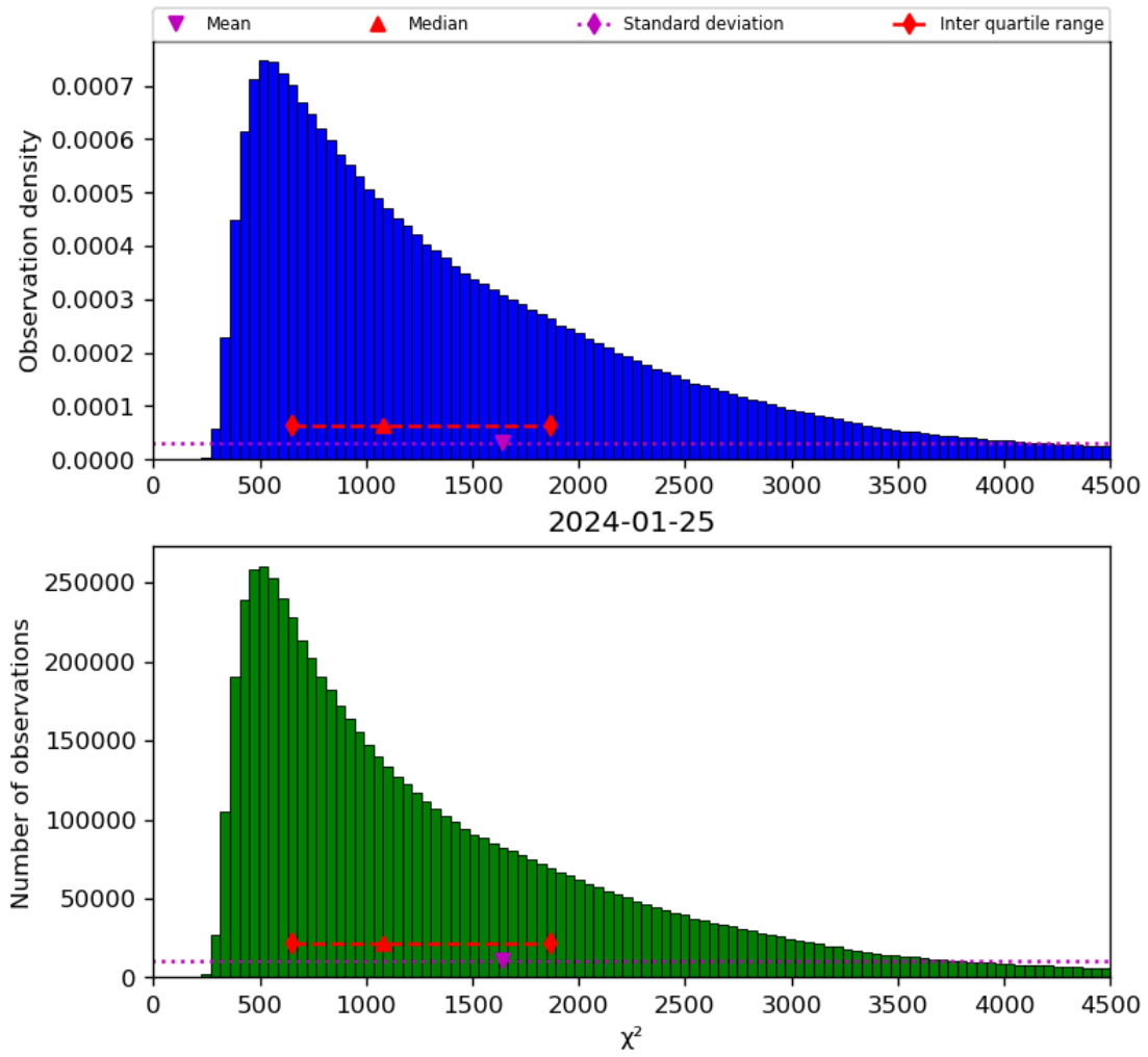
Figure 22: Histogram of “ \chi^2 ” for 2024-01-24 to 2024-01-26
