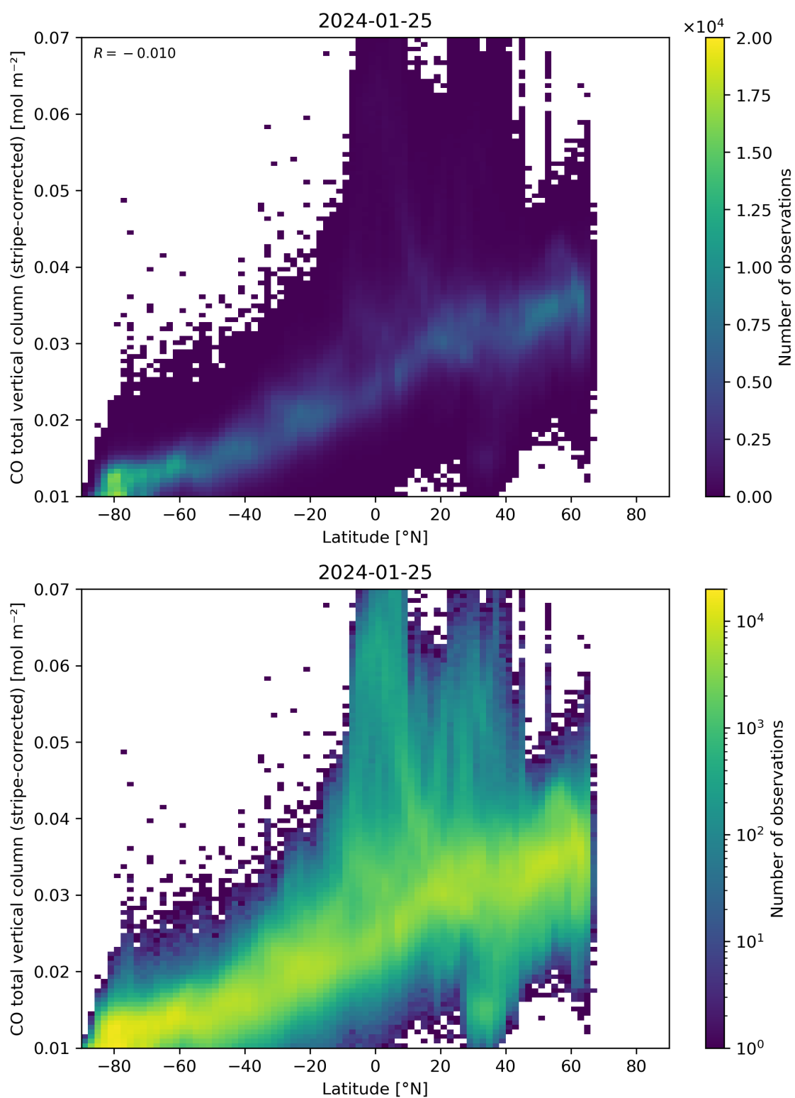
Figure 52: Scatter density plot of “Latitude” against “CO total vertical column (stripe-corrected)” for 2024-01-24 to 2024-01-26.
