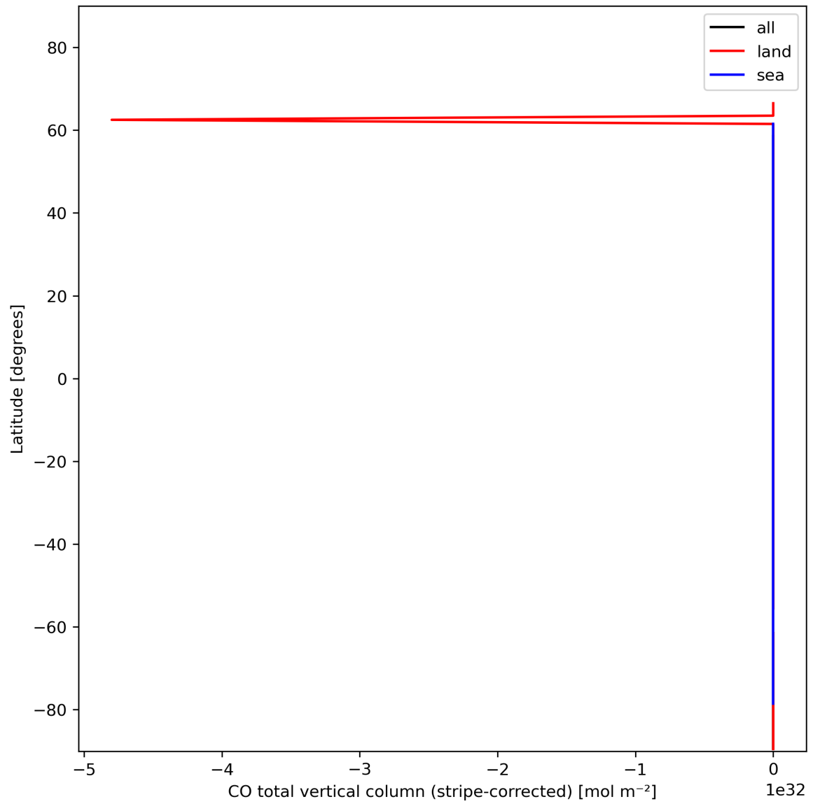
Figure 11: Zonal average of “CO total vertical column (stripe-corrected)” for 2024-01-24 to 2024-01-26.
