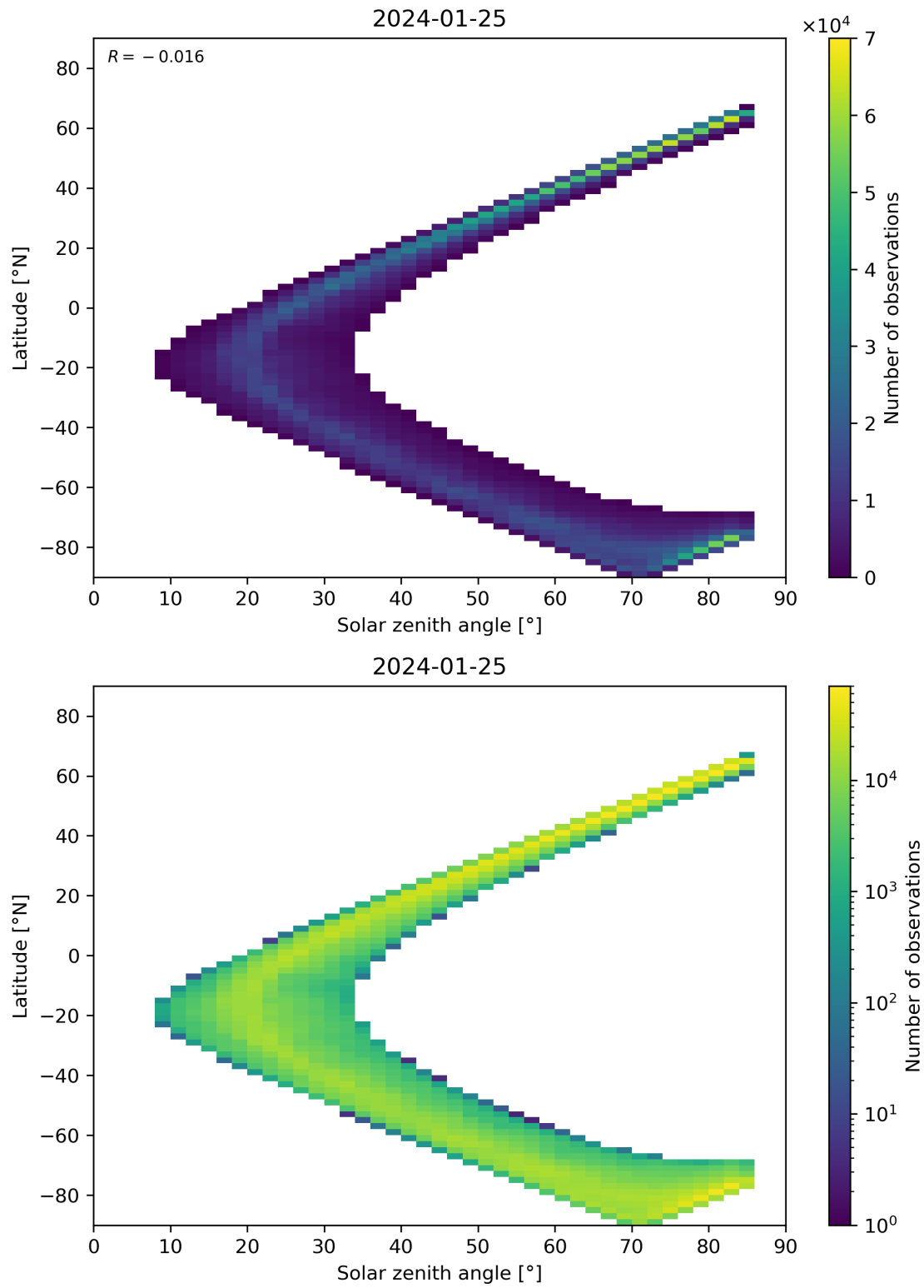
Figure 66: Scatter density plot of “Solar zenith angle” against “Latitude” for 2024-01-24 to 2024-01-26.
