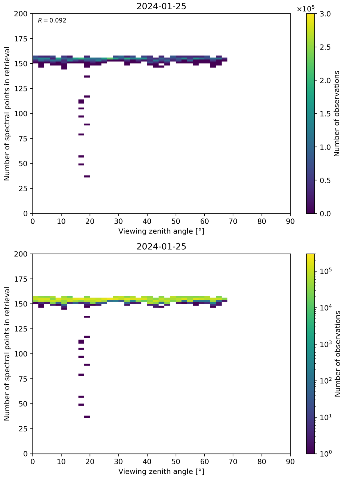
Figure 76: Scatter density plot of “Viewing zenith angle” against “Number of spectral points in retrieval” for 2024-01-24 to 2024-01-26.
