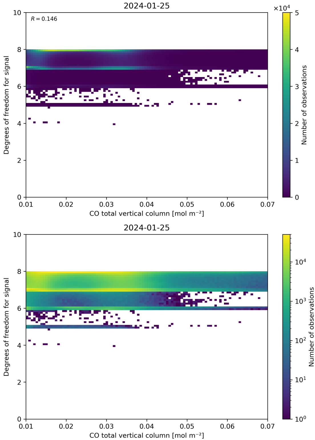
Figure 41: Scatter density plot of “CO total vertical column” against “Degrees of freedom for signal” for 2024-01-24 to 2024-01-26.
