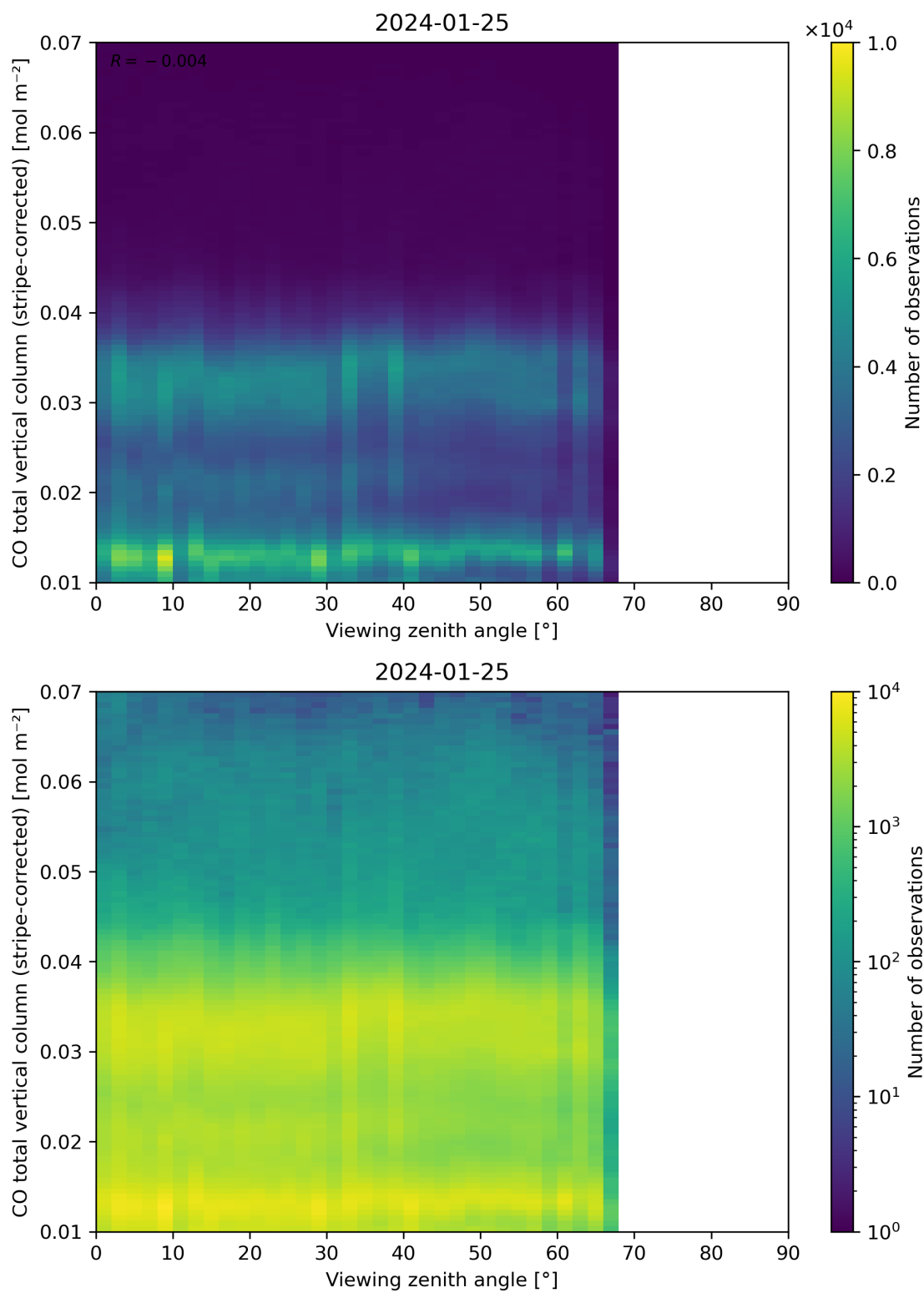
Figure 70: Scatter density plot of “Viewing zenith angle” against “CO total vertical column (stripe-corrected)” for 2024-01-24 to 2024-01-26.
