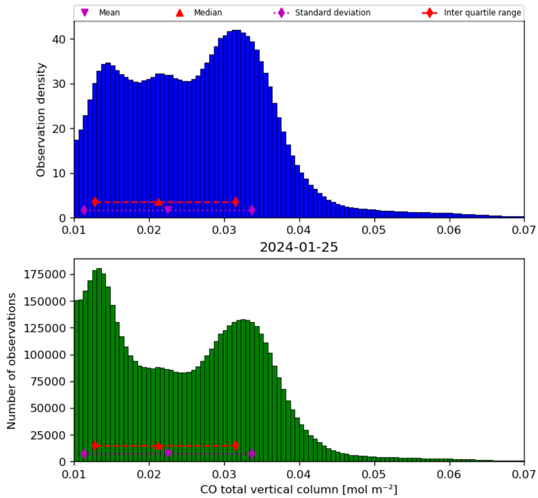
Figure 18: Histogram of “CO total vertical column” for 2024-01-24 to 2024-01-26
