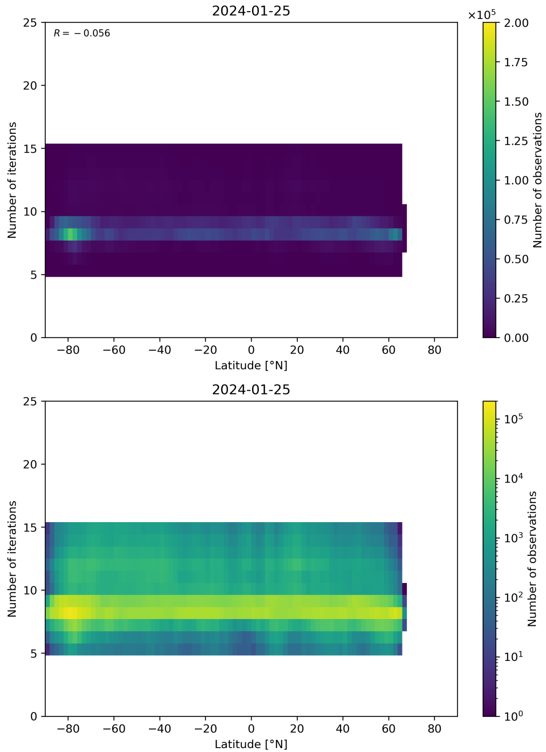
Figure 56: Scatter density plot of “Latitude” against “Number of iterations” for 2024-01-24 to 2024-01-26.
