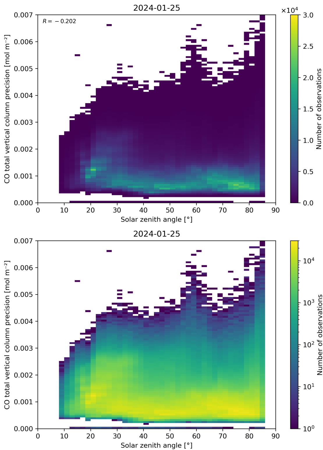
Figure 63: Scatter density plot of “Solar zenith angle” against “CO total vertical column precision” for 2024-01-24 to 2024-01-26.
