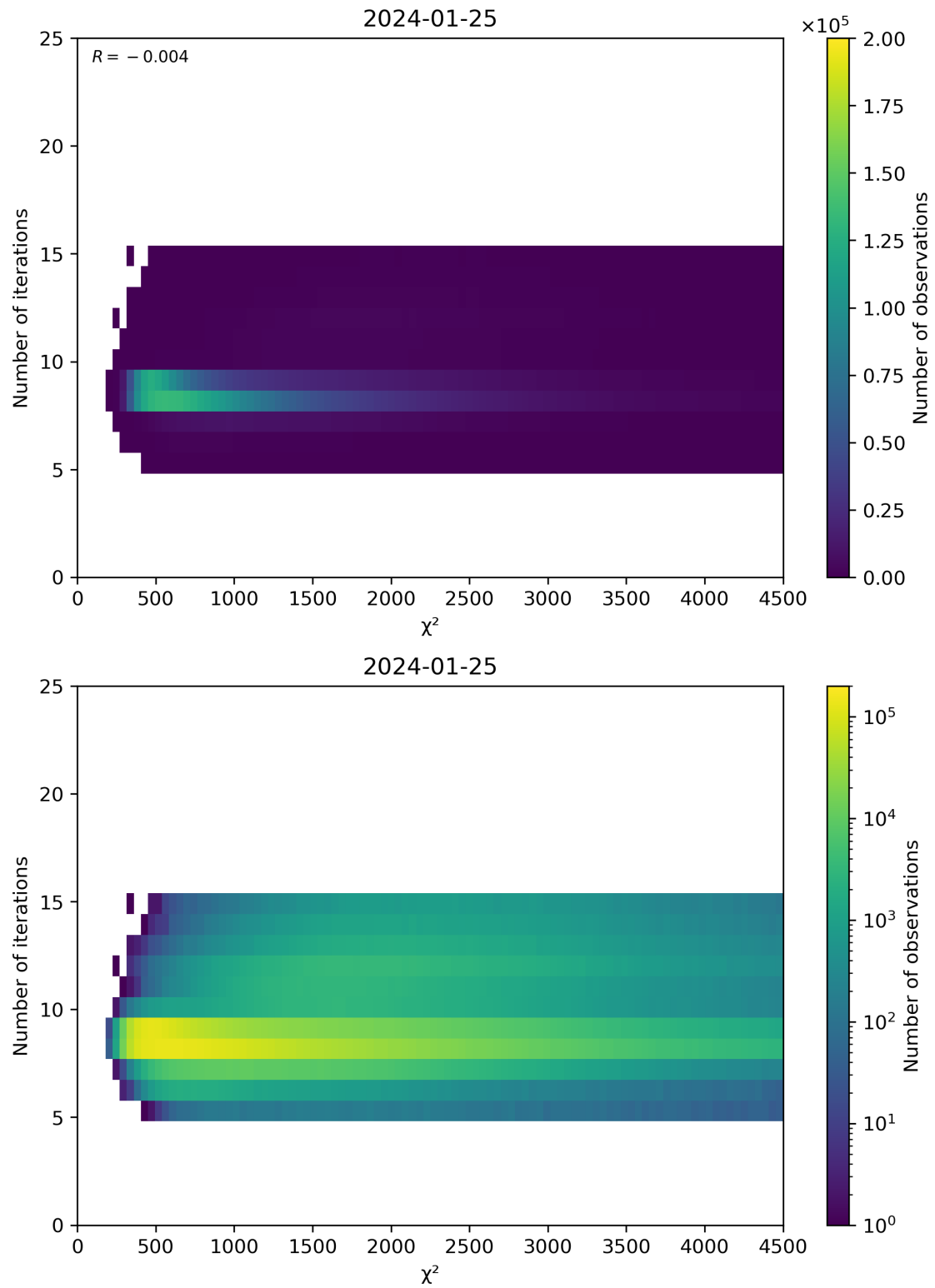
Figure 49: Scatter density plot of “ \chi^2 ” against “Number of iterations” for 2024-01-24 to 2024-01-26.
