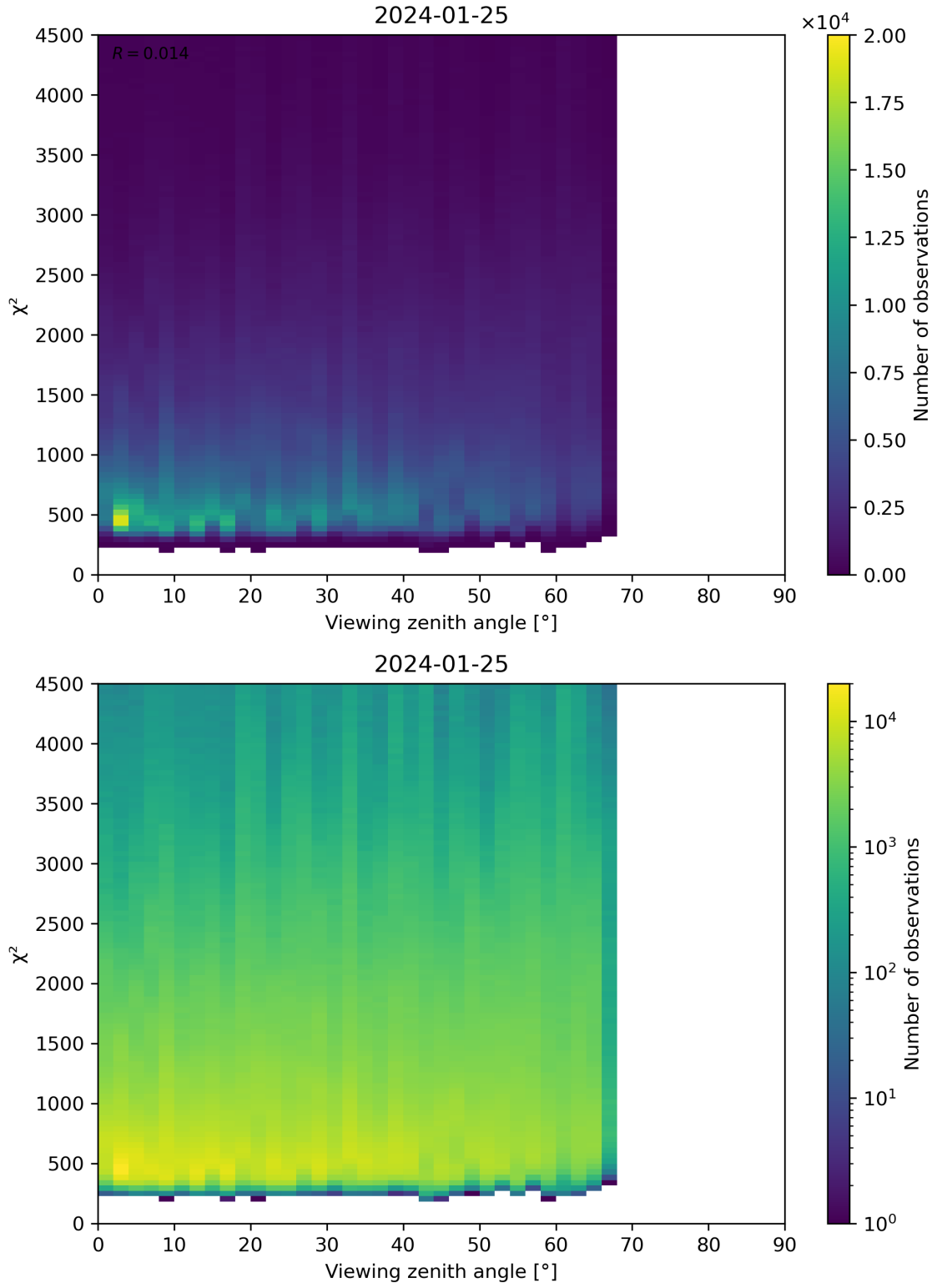
Figure 72: Scatter density plot of “Viewing zenith angle” against “ \chi^2 ” for 2024-01-24 to 2024-01-26.
