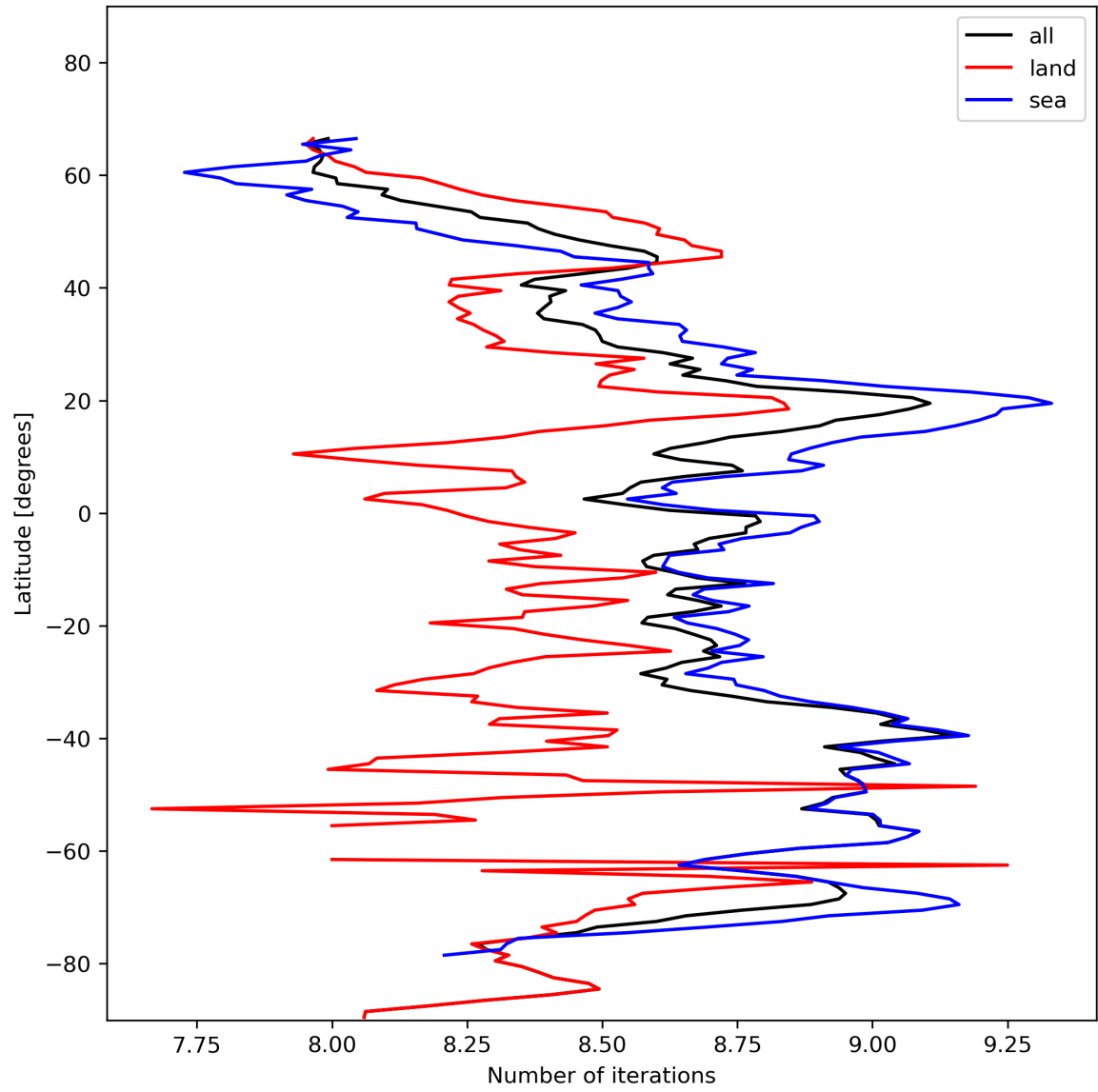
Figure 16: Zonal average of “Number of iterations” for 2024-01-24 to 2024-01-26.
