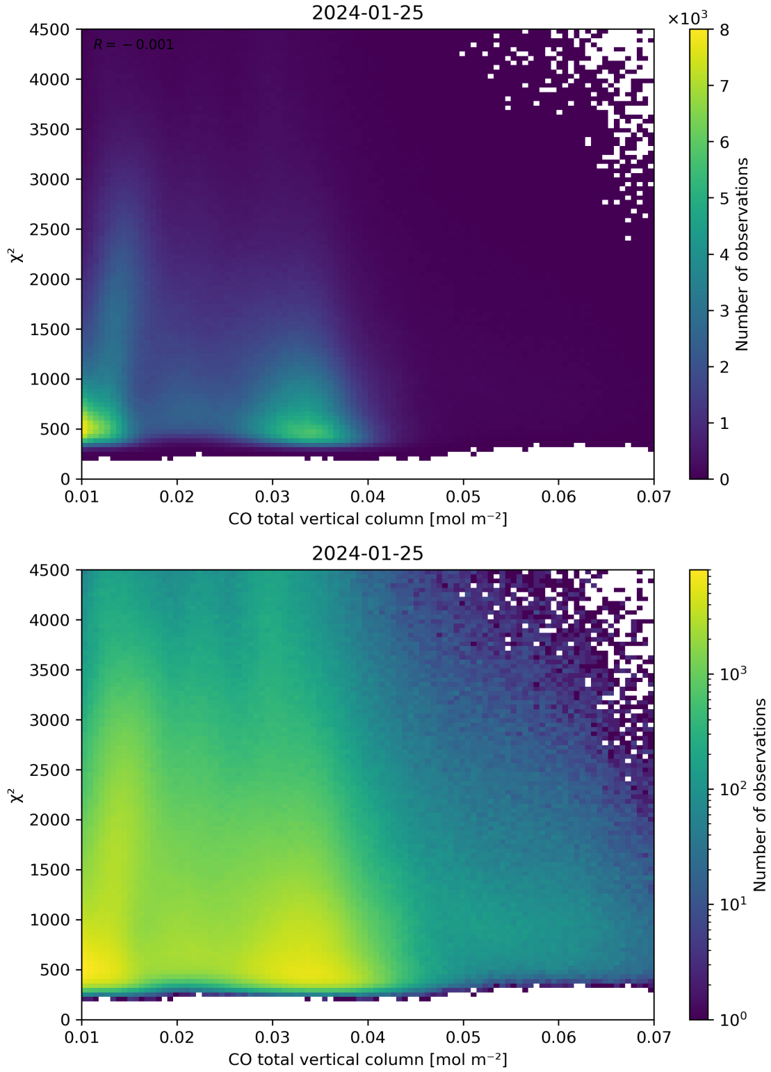
Figure 35: Scatter density plot of “CO total vertical column” against “ \chi^2 ” for 2024-01-24 to 2024-01-26.
