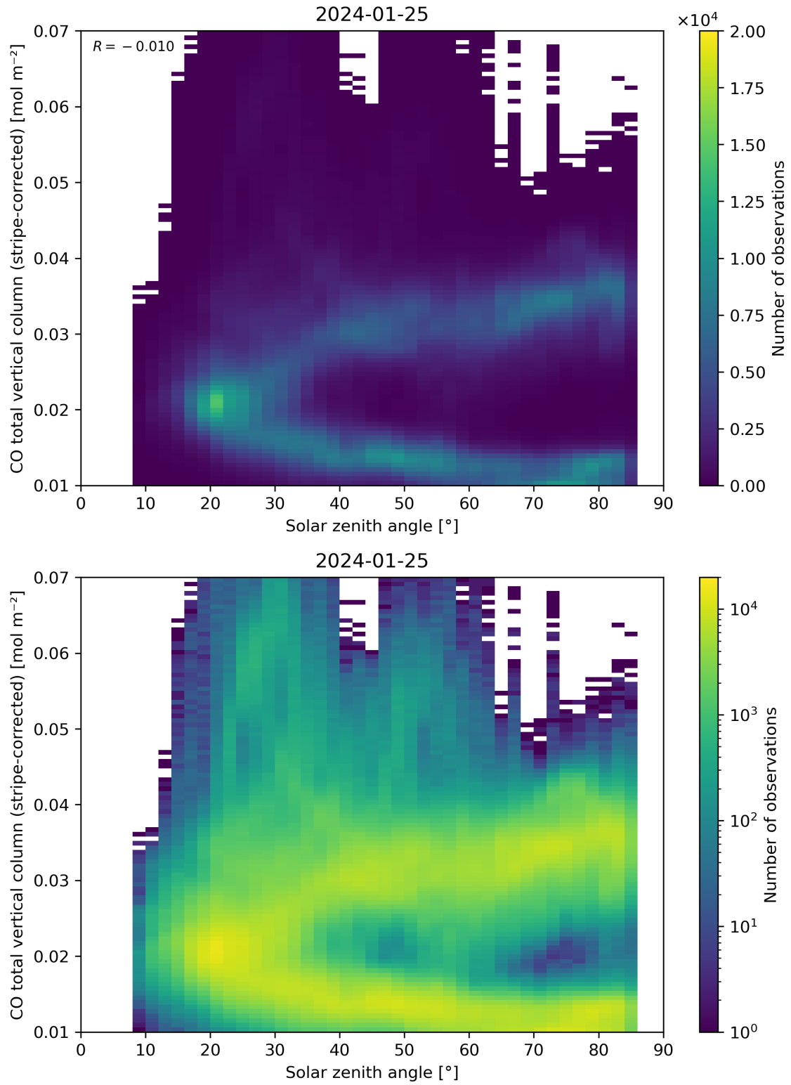
Figure 62: Scatter density plot of “Solar zenith angle” against “CO total vertical column (stripe-corrected)” for 2024-01-24 to 2024-01-26.
