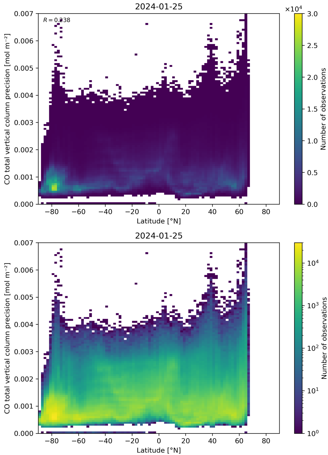
Figure 53: Scatter density plot of “Latitude” against “CO total vertical column precision” for 2024-01-24 to 2024-01-26.
