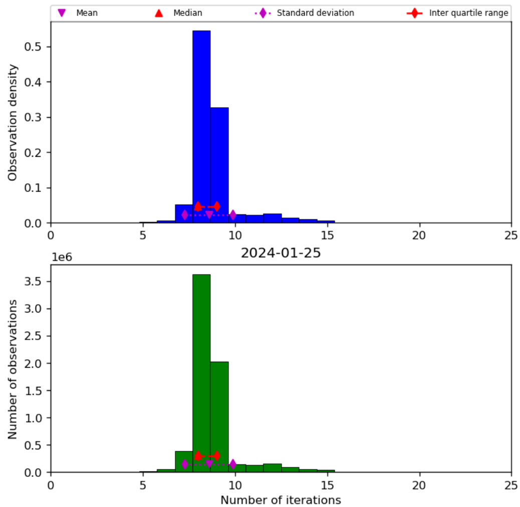
Figure 24: Histogram of “Number of iterations” for 2024-01-24 to 2024-01-26
