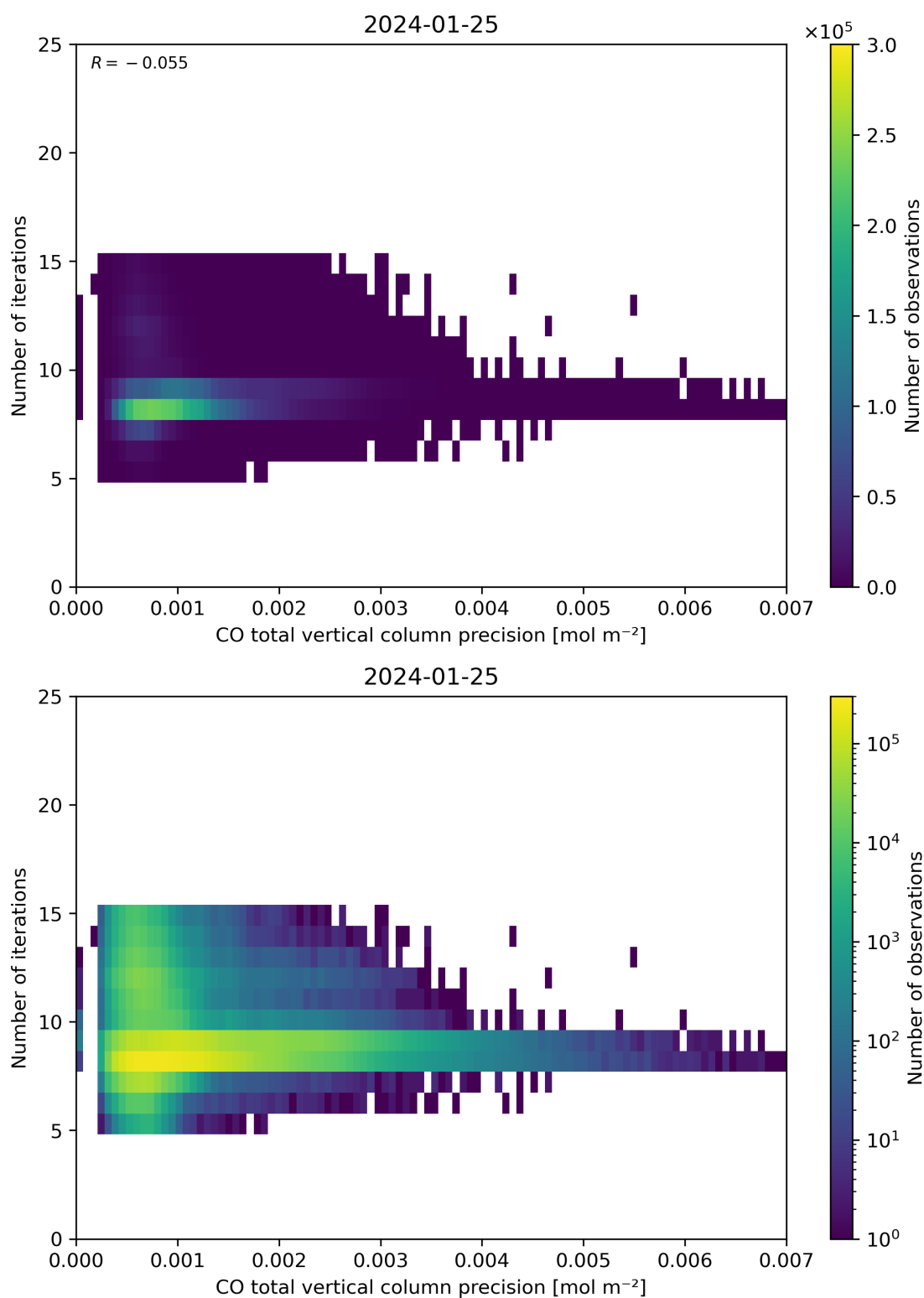
Figure 46: Scatter density plot of “CO total vertical column precision” against “Number of iterations” for 2024-01-24 to 2024-01-26.
