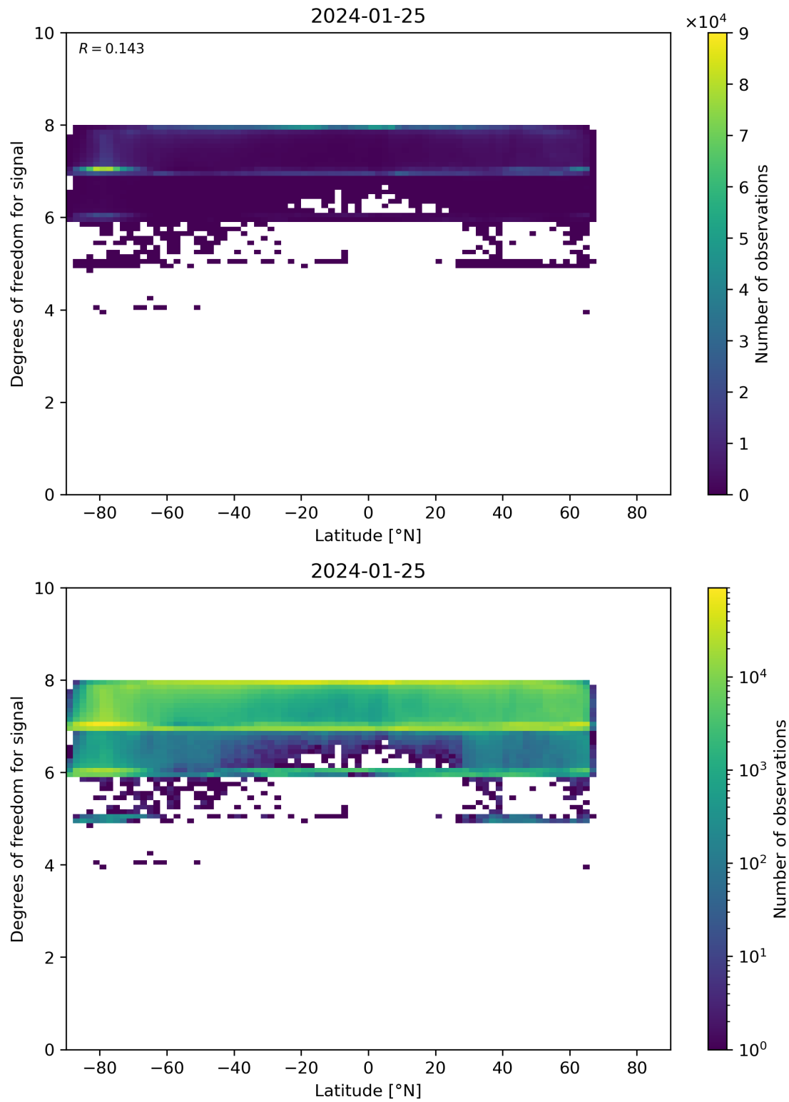
Figure 55: Scatter density plot of “Latitude” against “Degrees of freedom for signal” for 2024-01-24 to 2024-01-26.
