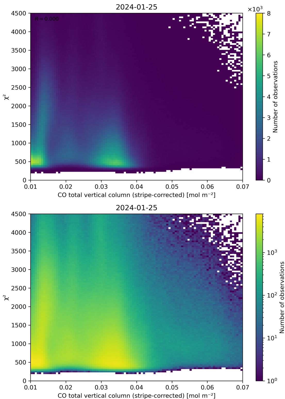
Figure 37: Scatter density plot of “CO total vertical column (stripe-corrected)” against “ \chi^2 ” for 2024-01-24 to 2024-01-26.
