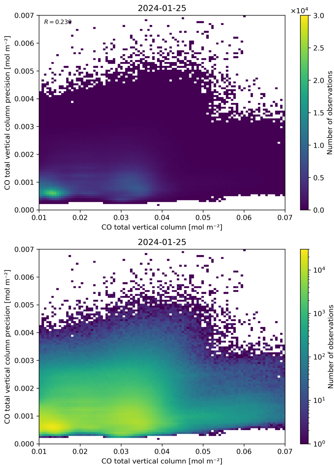
Figure 34: Scatter density plot of “CO total vertical column” against “CO total vertical column precision” for 2024-01-24 to 2024-01-26.
