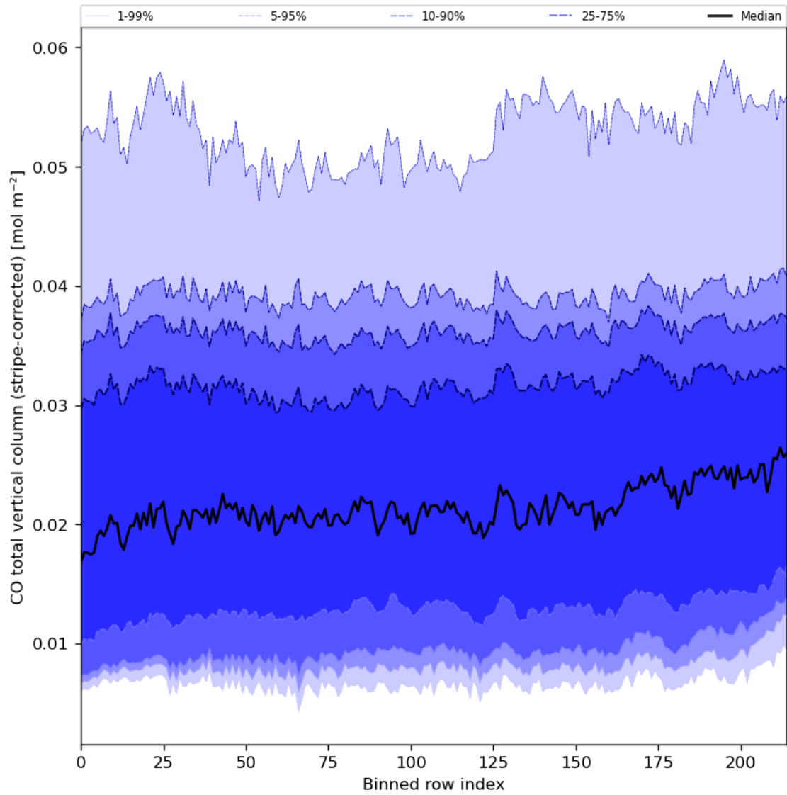
Figure 27: Along track statistics of “CO total vertical column (stripe-corrected)” for 2024-01-24 to 2024-01-26
