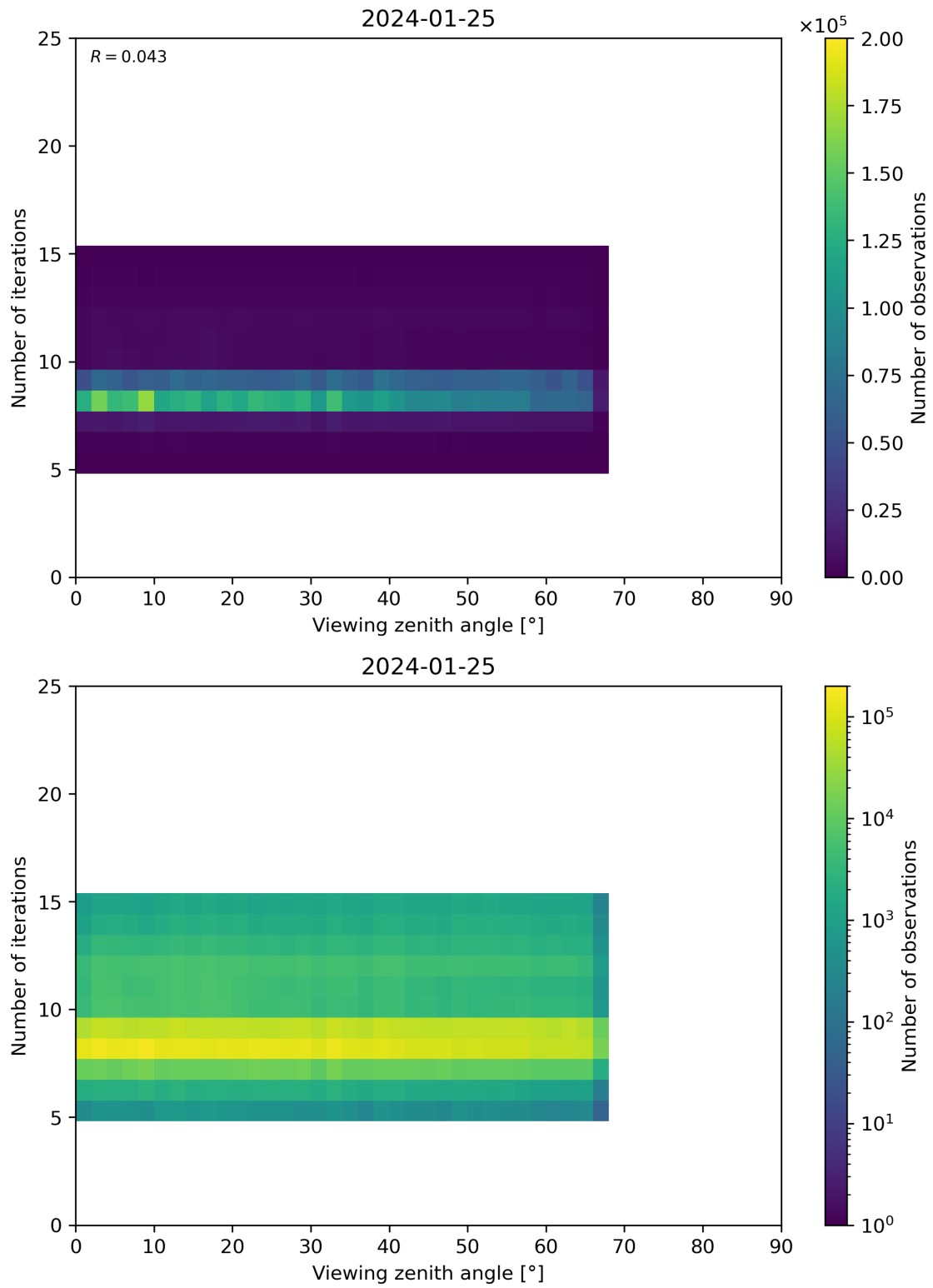
Figure 75: Scatter density plot of “Viewing zenith angle” against “Number of iterations” for 2024-01-24 to 2024-01-26.
