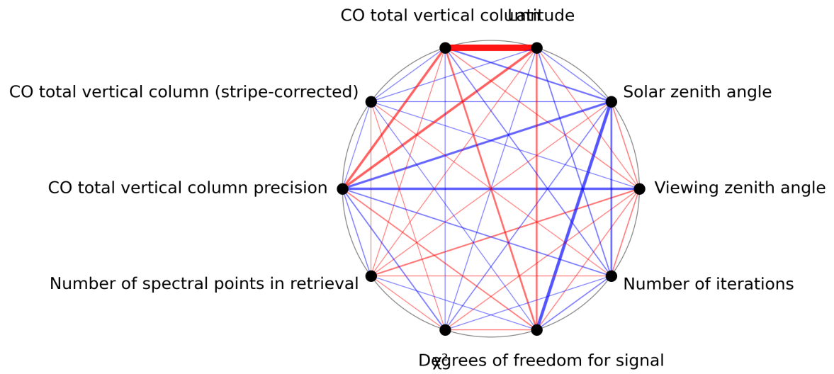
Figure 1: Map of correlation graph for 2024-01-24 to 2024-01-26.
