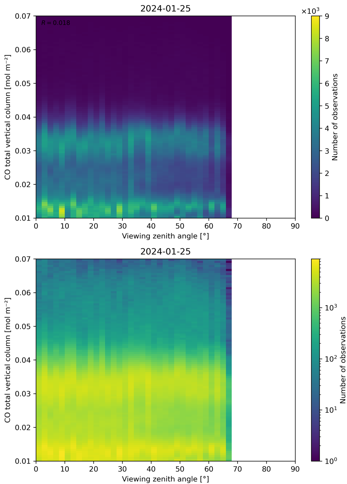
Figure 69: Scatter density plot of “Viewing zenith angle” against “CO total vertical column” for 2024-01-24 to 2024-01-26.
