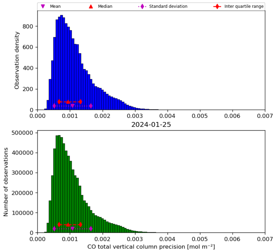
Figure 20: Histogram of “CO total vertical column precision” for 2024-01-24 to 2024-01-26
