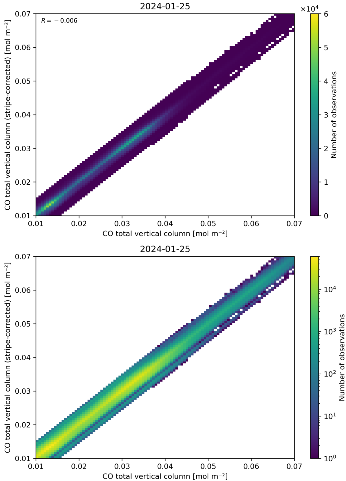
Figure 33: Scatter density plot of “CO total vertical column” against “CO total vertical column (stripe-corrected)” for 2024-01-24 to 2024-01-26.
