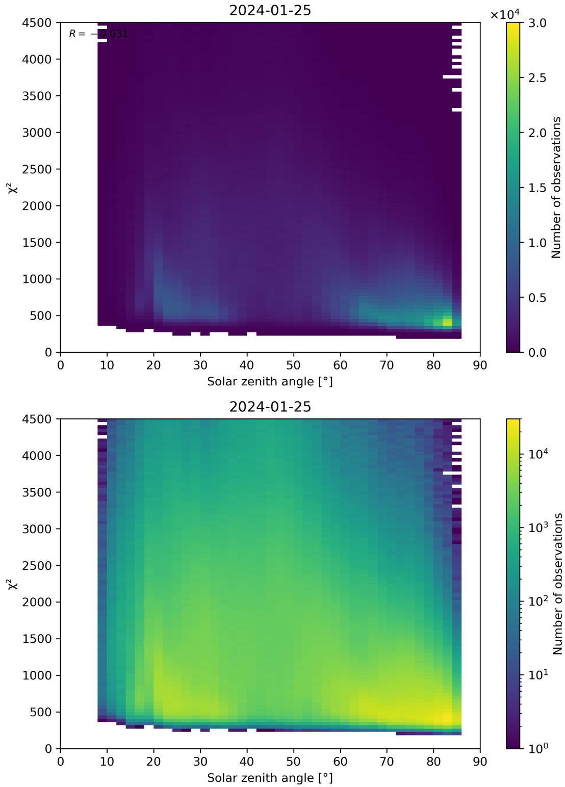
Figure 64: Scatter density plot of “Solar zenith angle” against “ \chi^2 ” for 2024-01-24 to 2024-01-26.
