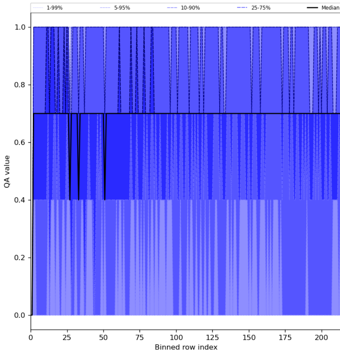
Figure 25: Along track statistics of “QA value” for 2024-01-24 to 2024-01-26
