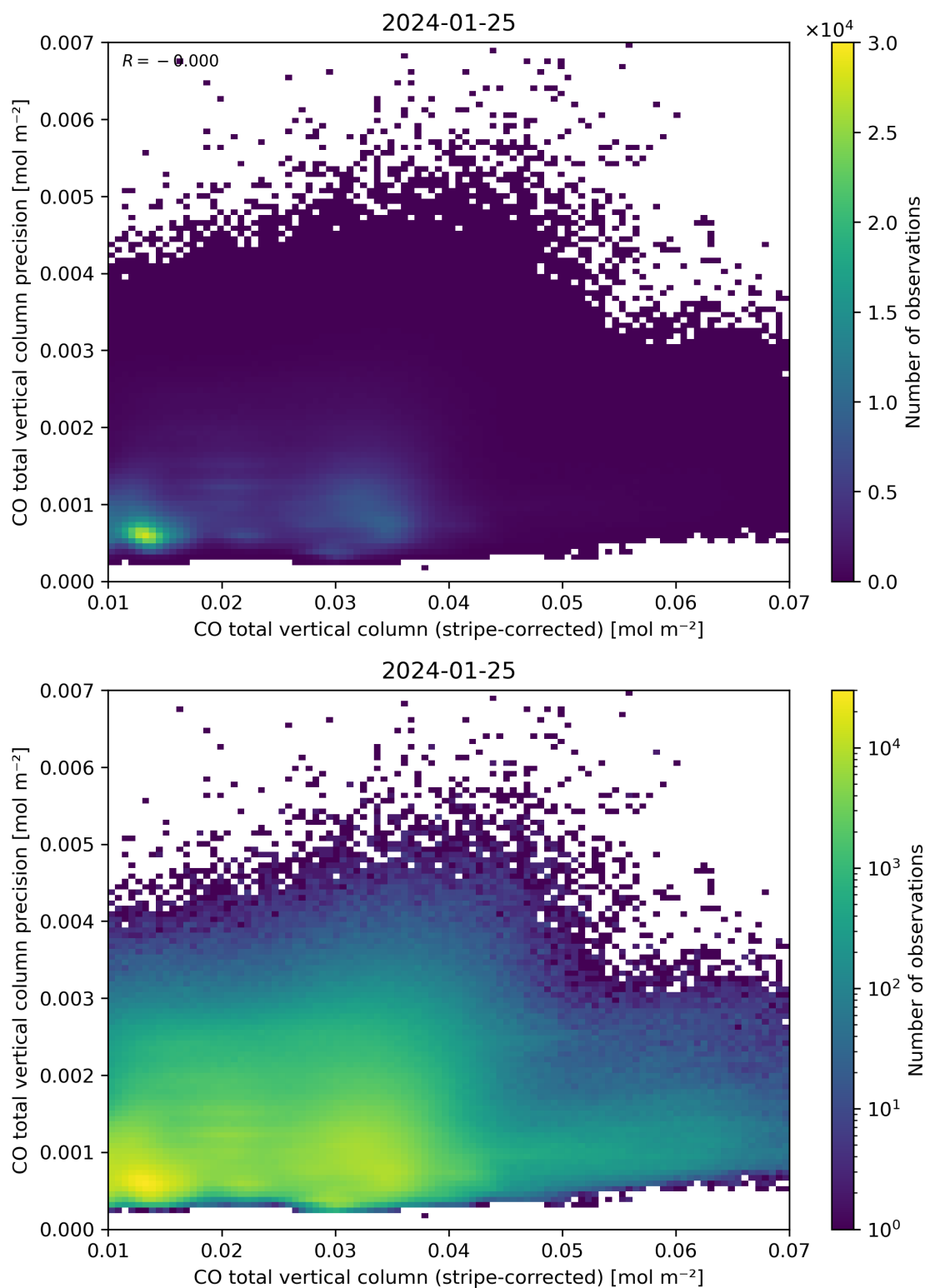
Figure 36: Scatter density plot of “CO total vertical column (stripe-corrected)” against “CO total vertical column precision” for 2024-01-24 to 2024-01-26.
