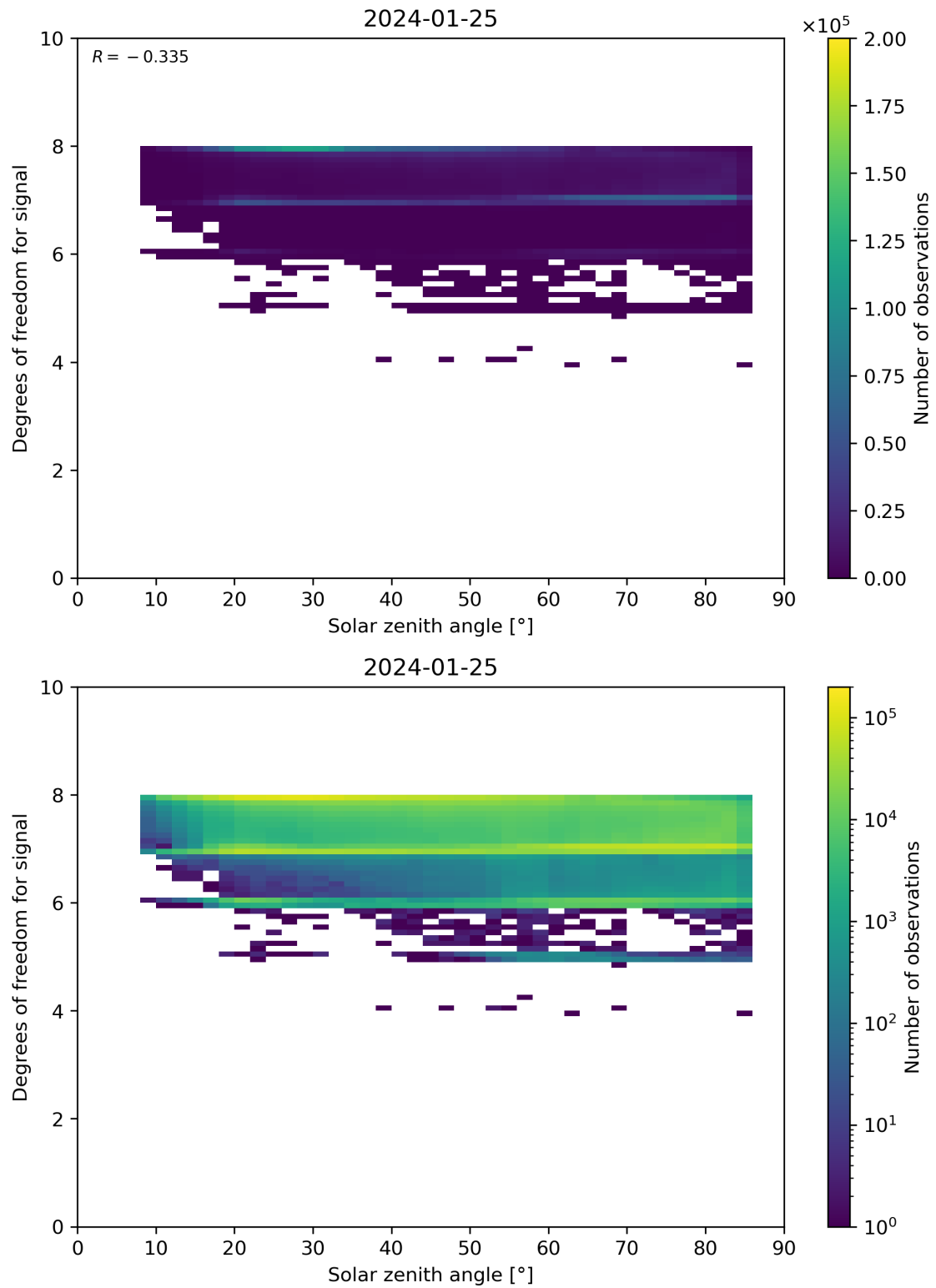
Figure 65: Scatter density plot of “Solar zenith angle” against “Degrees of freedom for signal” for 2024-01-24 to 2024-01-26.
