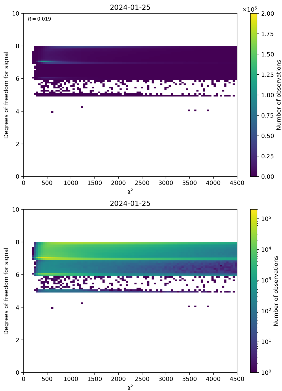
Figure 48: Scatter density plot of “ \chi^2 ” against “Degrees of freedom for signal” for 2024-01-24 to 2024-01-26.
