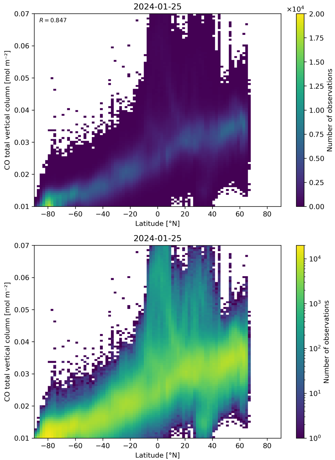
Figure 51: Scatter density plot of “Latitude” against “CO total vertical column” for 2024-01-24 to 2024-01-26.
