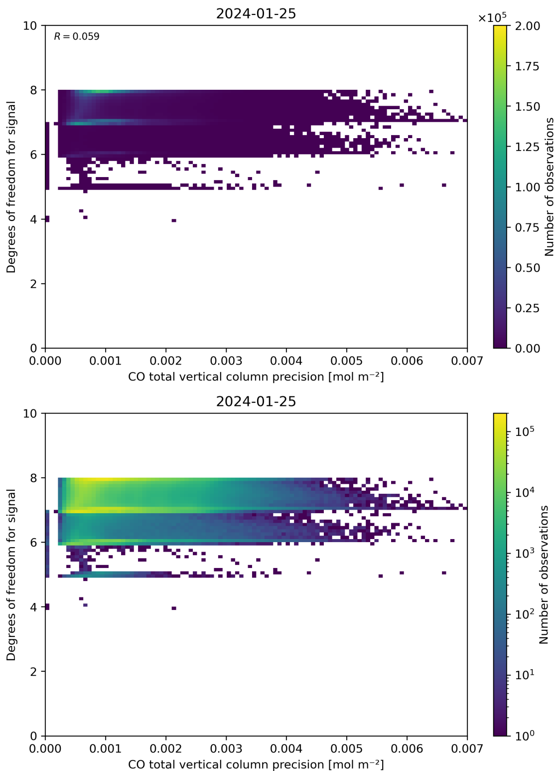
Figure 45: Scatter density plot of “CO total vertical column precision” against “Degrees of freedom for signal” for 2024-01-24 to 2024-01-26.
