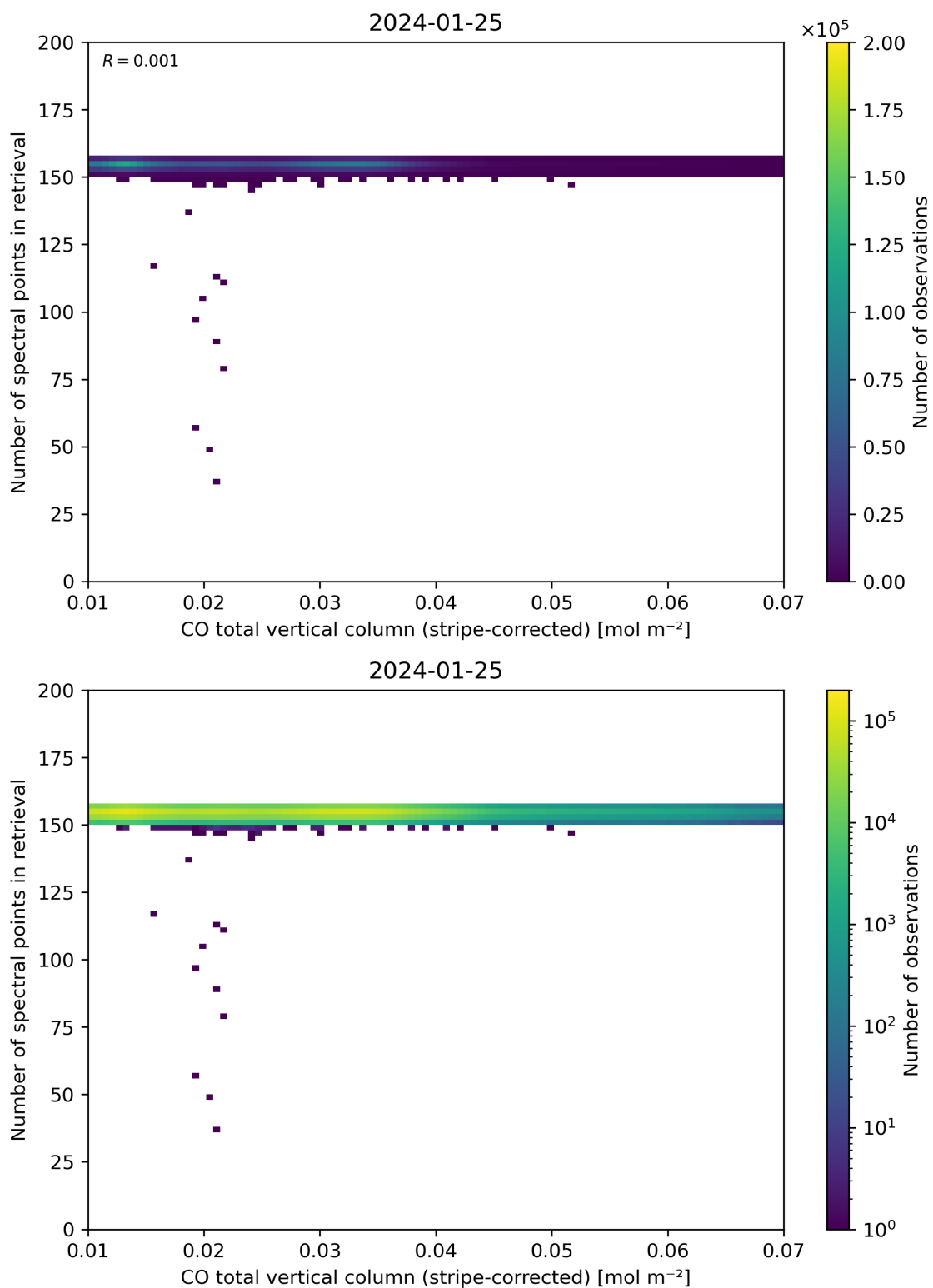
Figure 40: Scatter density plot of “CO total vertical column (stripe-corrected)” against “Number of spectral points in retrieval” for 2024-01-24 to 2024-01-26.
