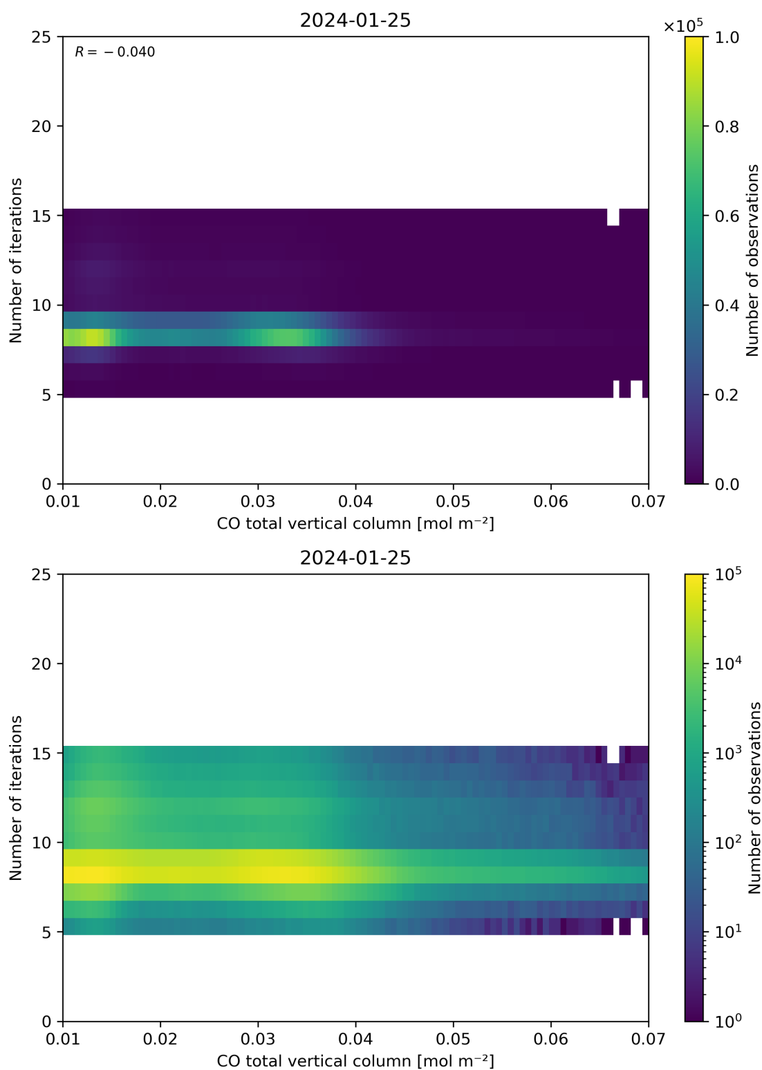
Figure 42: Scatter density plot of “CO total vertical column” against “Number of iterations” for 2024-01-24 to 2024-01-26.
