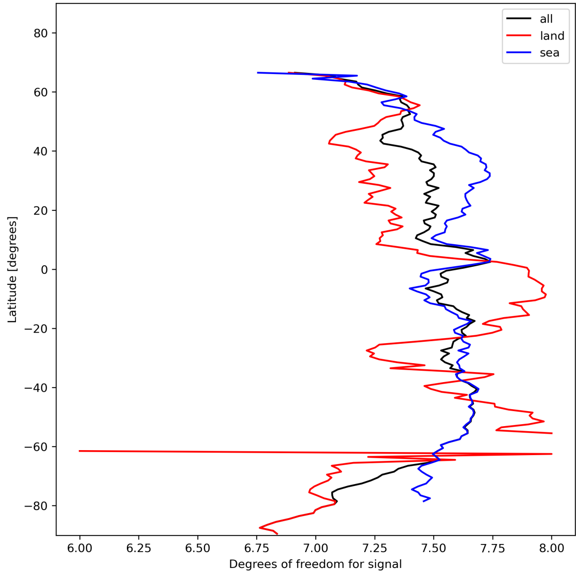
Figure 15: Zonal average of “Degrees of freedom for signal” for 2024-01-24 to 2024-01-26.
