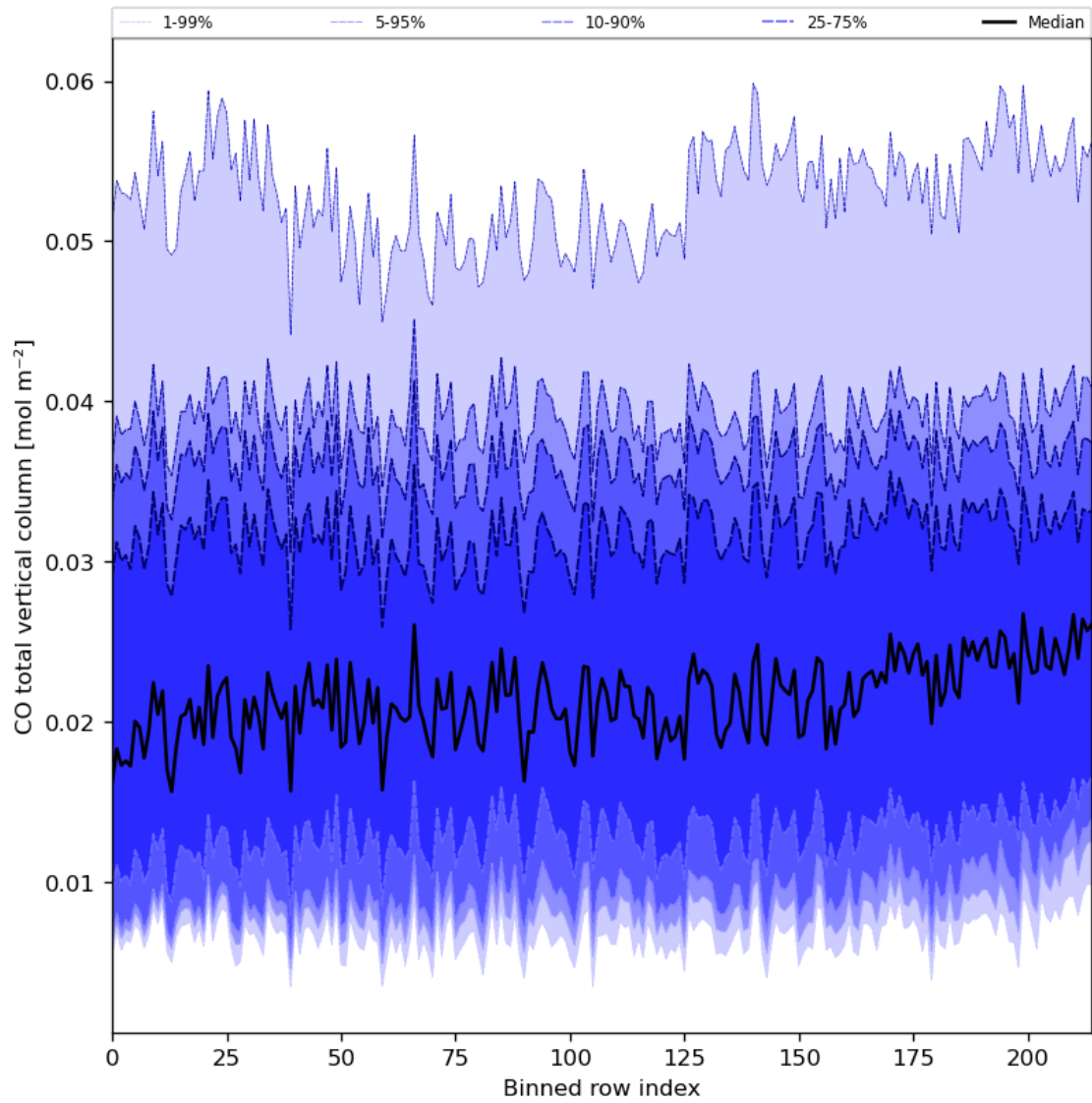
Figure 26: Along track statistics of “CO total vertical column” for 2024-01-24 to 2024-01-26
