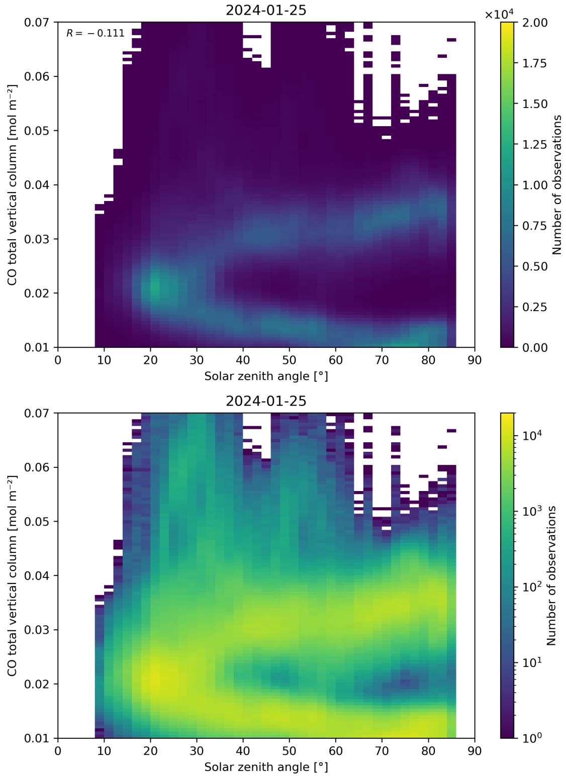
Figure 61: Scatter density plot of “Solar zenith angle” against “CO total vertical column” for 2024-01-24 to 2024-01-26.
