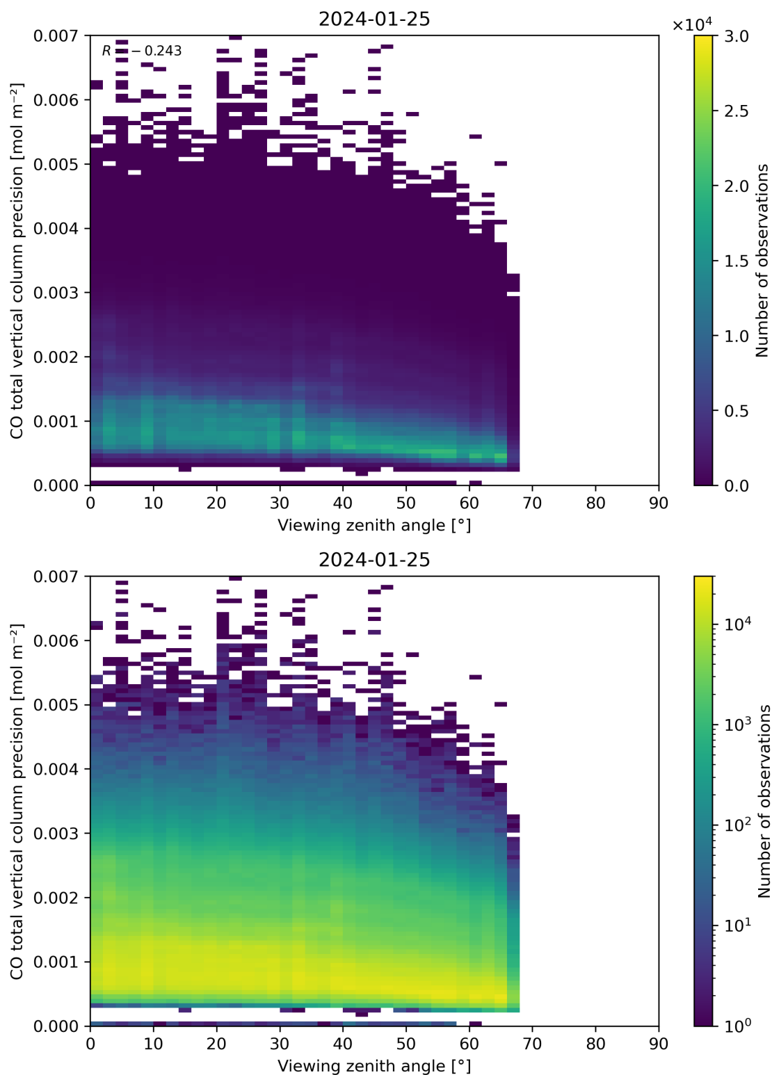
Figure 71: Scatter density plot of “Viewing zenith angle” against “CO total vertical column precision” for 2024-01-24 to 2024-01-26.
