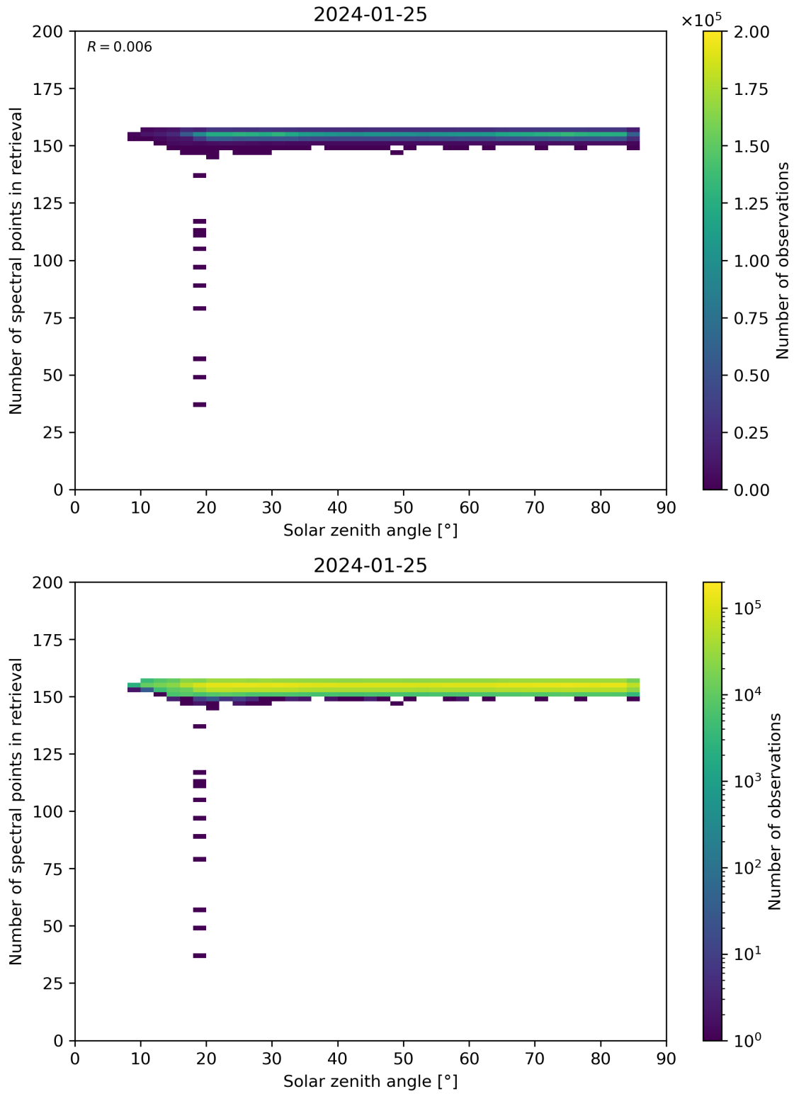
Figure 68: Scatter density plot of “Solar zenith angle” against “Number of spectral points in retrieval” for 2024-01-24 to 2024-01-26.
