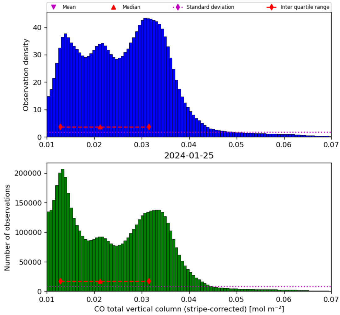
Figure 19: Histogram of “CO total vertical column (stripe-corrected)” for 2024-01-24 to 2024-01-26
