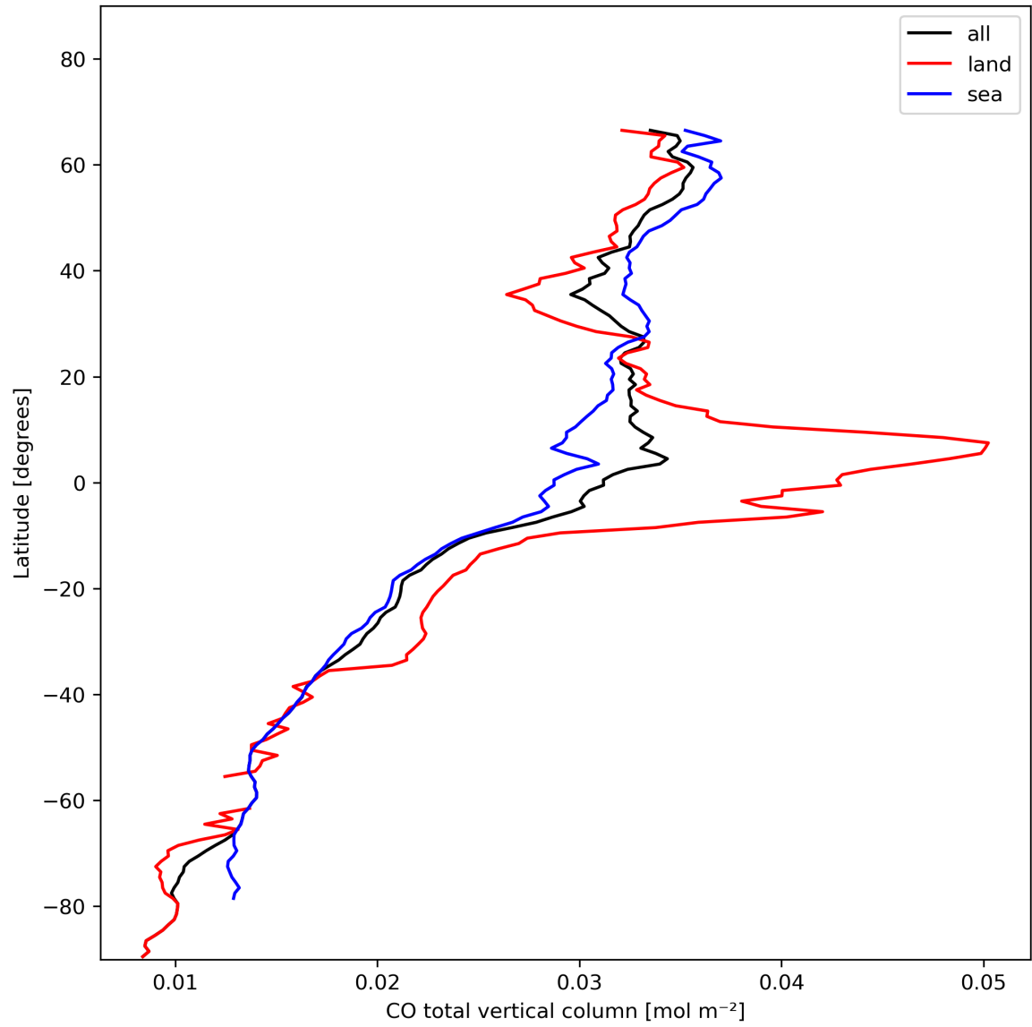
Figure 10: Zonal average of “CO total vertical column” for 2024-01-24 to 2024-01-26.
