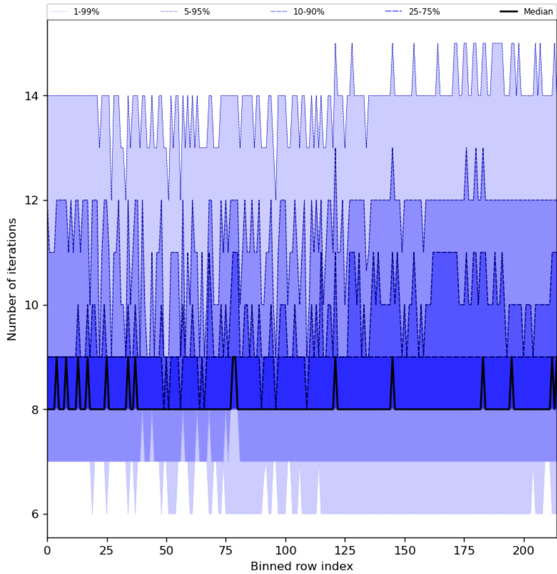
Figure 32: Along track statistics of “Number of iterations” for 2024-01-24 to 2024-01-26
