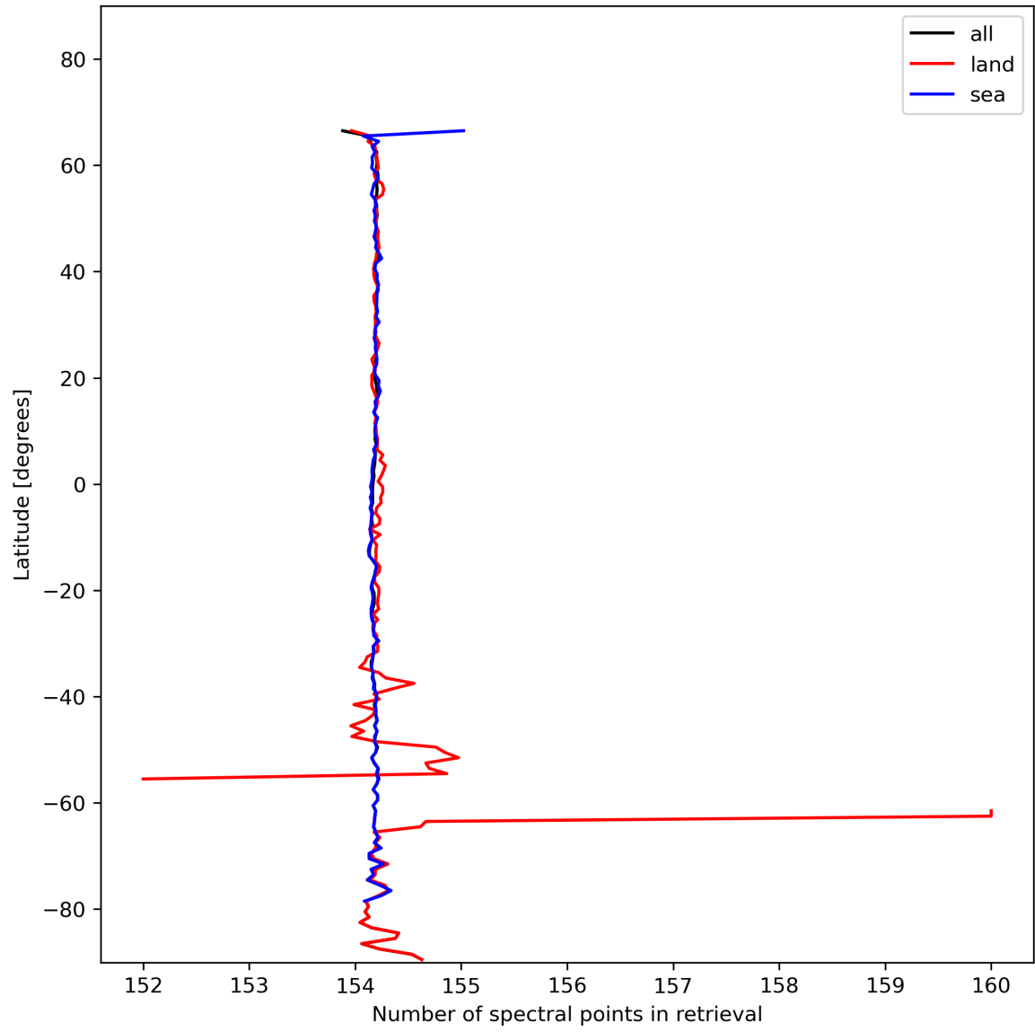
Figure 13: Zonal average of “Number of spectral points in retrieval” for 2024-01-24 to 2024-01-26.
