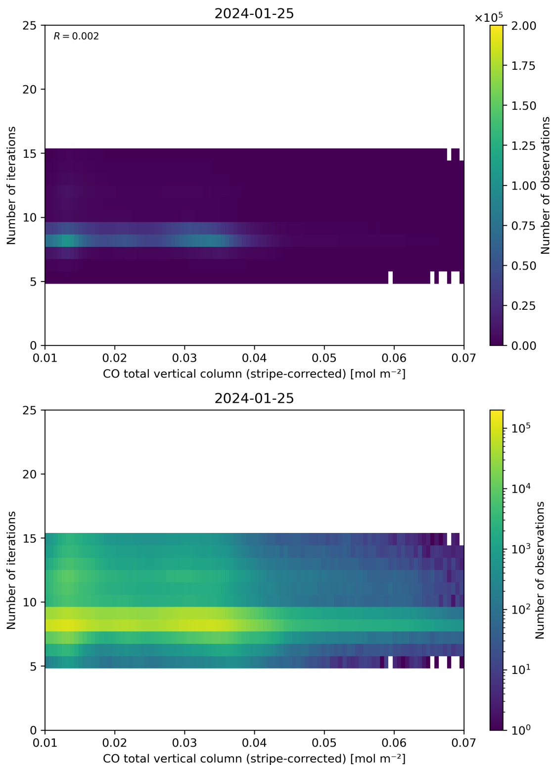
Figure 39: Scatter density plot of “CO total vertical column (stripe-corrected)” against “Number of iterations” for 2024-01-24 to 2024-01-26.
