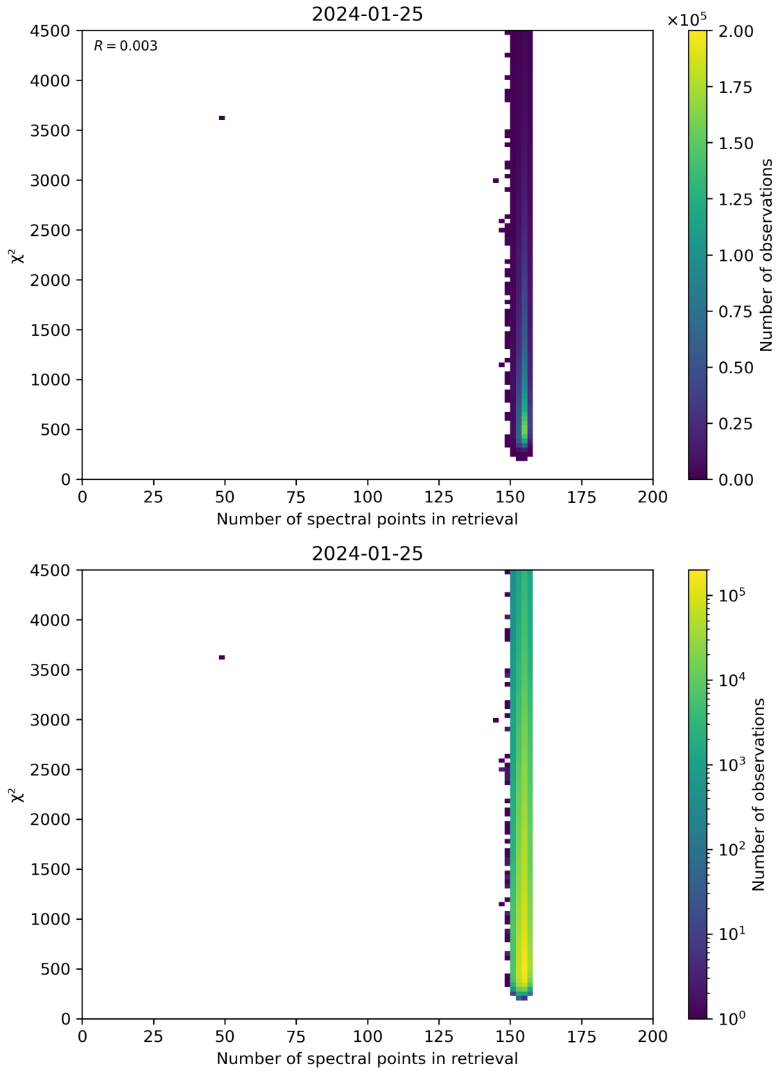
Figure 58: Scatter density plot of “Number of spectral points in retrieval” against “ \chi^2 ” for 2024-01-24 to 2024-01-26.
