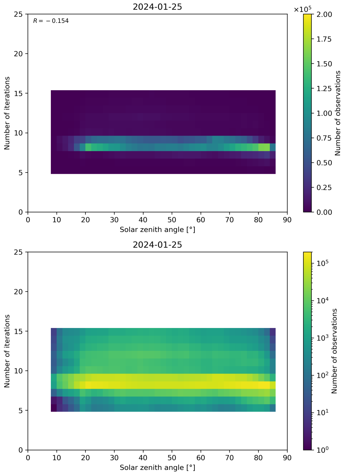
Figure 67: Scatter density plot of “Solar zenith angle” against “Number of iterations” for 2024-01-24 to 2024-01-26.
