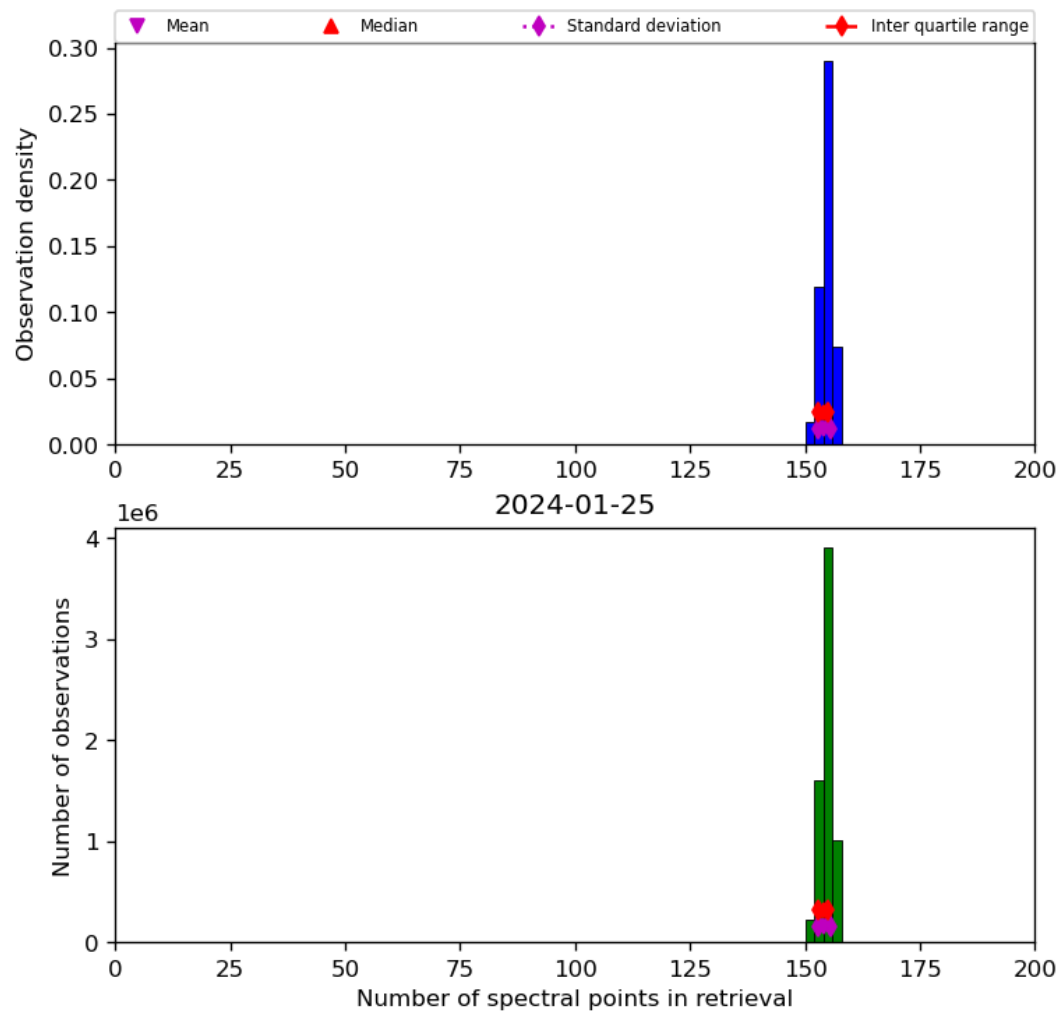
Figure 21: Histogram of “Number of spectral points in retrieval” for 2024-01-24 to 2024-01-26
