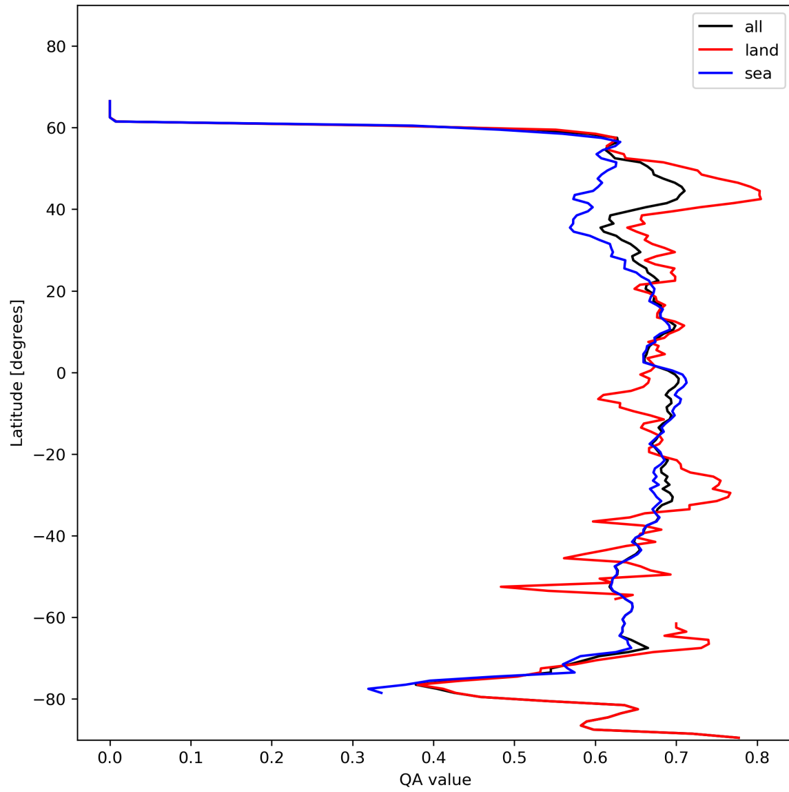
Figure 9: Zonal average of “QA value” for 2024-01-24 to 2024-01-26.
