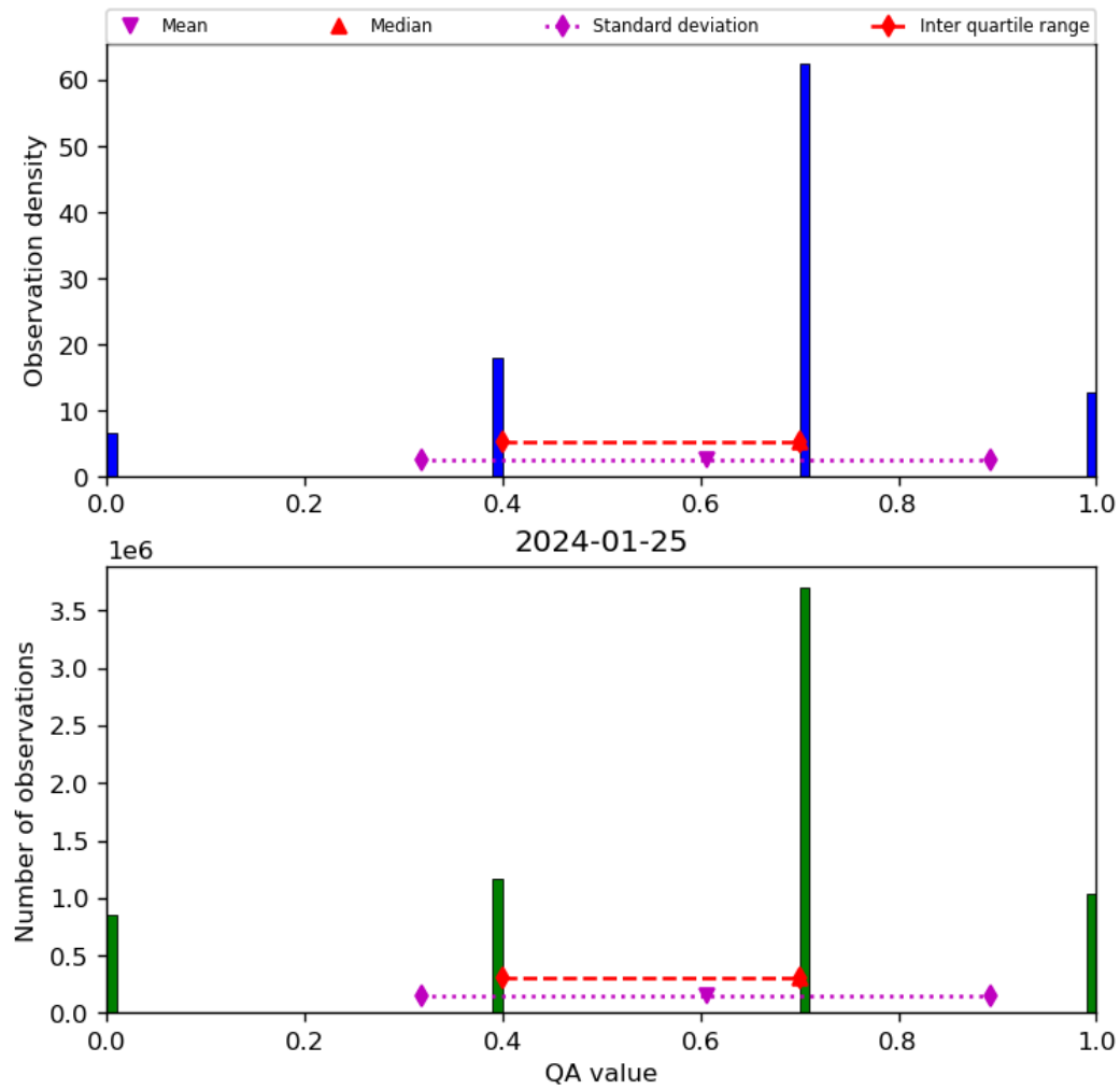
Figure 17: Histogram of “QA value” for 2024-01-24 to 2024-01-26
