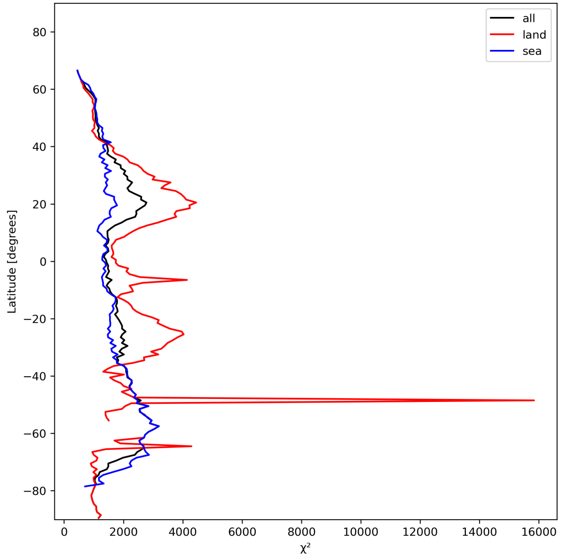
Figure 14: Zonal average of “ \chi^2 ” for 2024-01-24 to 2024-01-26.
