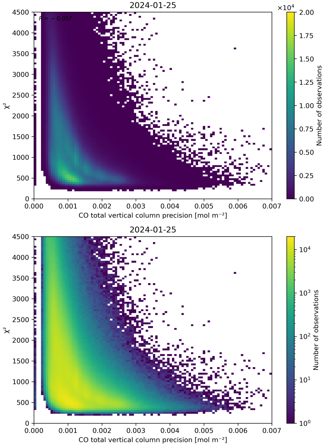
Figure 44: Scatter density plot of “CO total vertical column precision” against “ \chi^2 ” for 2024-01-24 to 2024-01-26.
