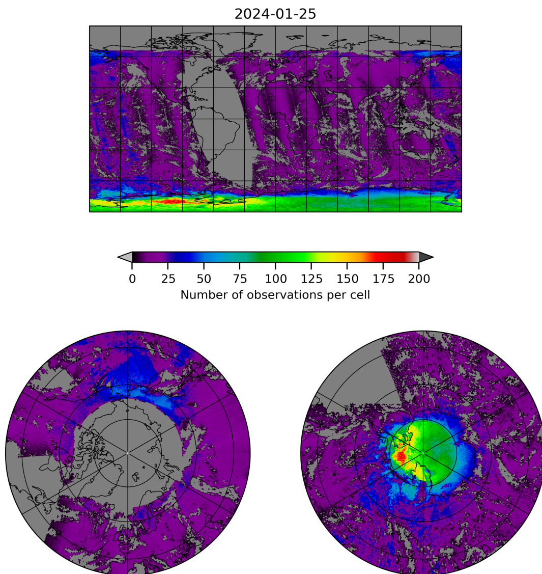
Figure 8: Map of the number of observations for 2024-01-24 to 2024-01-26
