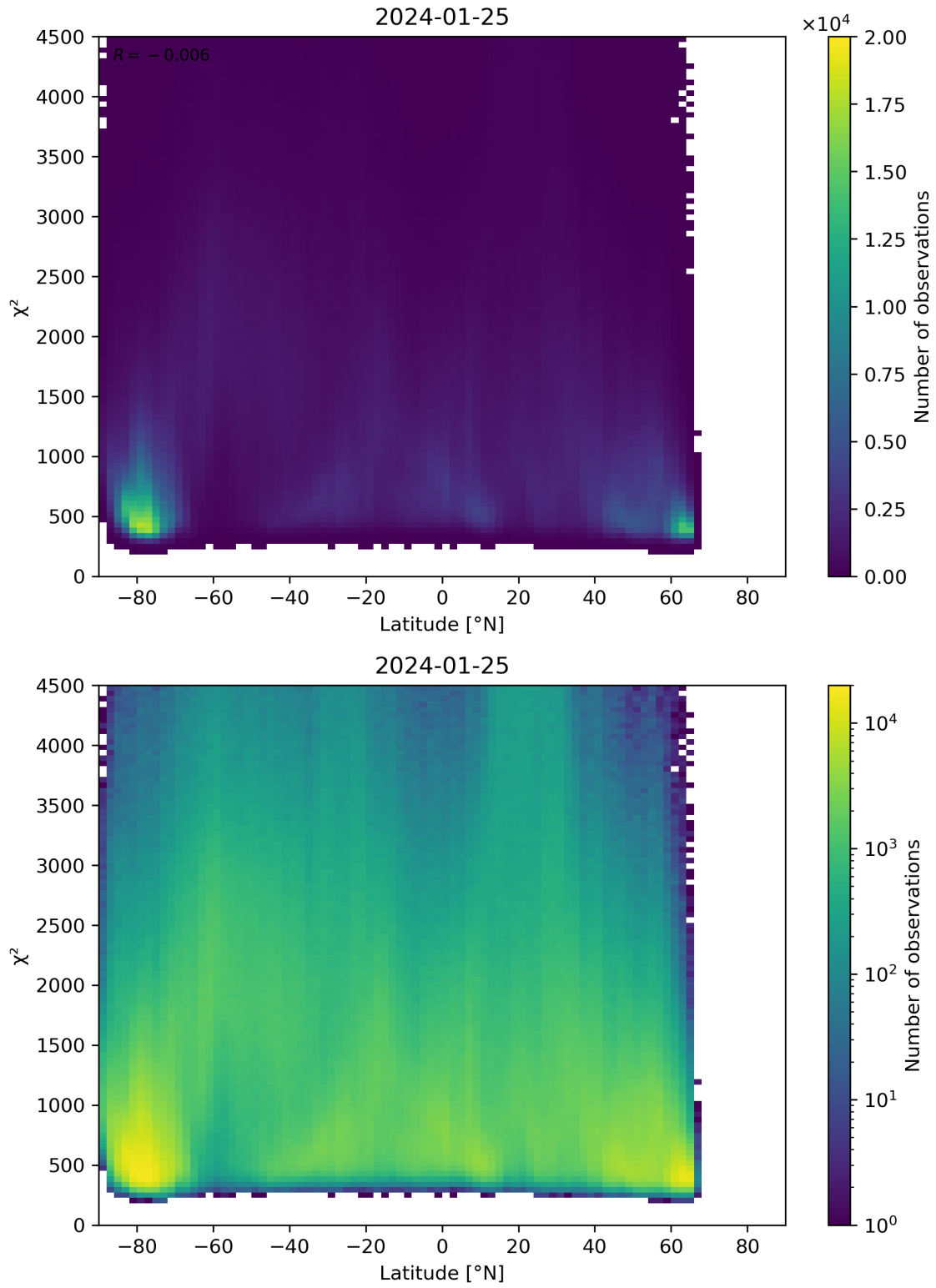
Figure 54: Scatter density plot of “Latitude” against “ \chi^2 ” for 2024-01-24 to 2024-01-26.
