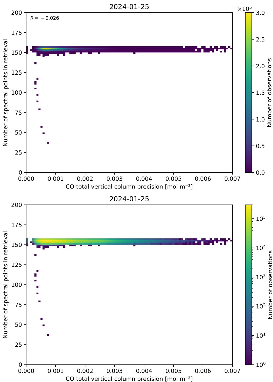
Figure 47: Scatter density plot of “CO total vertical column precision” against “Number of spectral points in retrieval” for 2024-01-24 to 2024-01-26.
