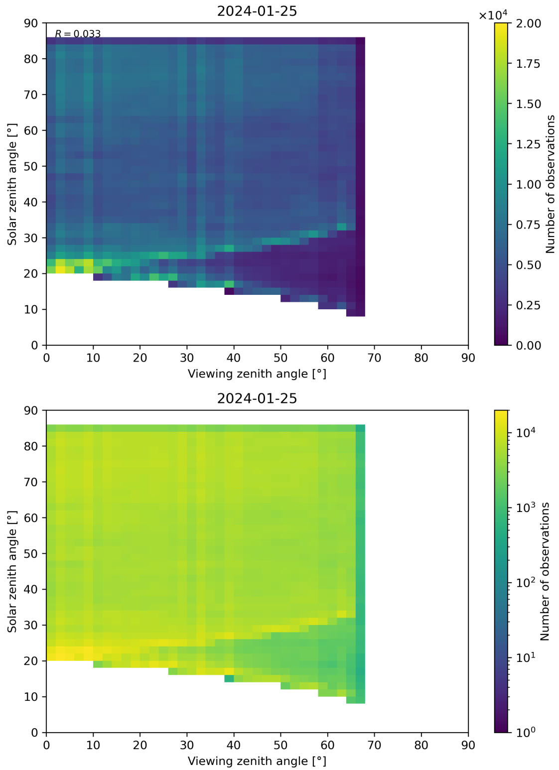
Figure 77: Scatter density plot of “Viewing zenith angle” against “Solar zenith angle” for 2024-01-24 to 2024-01-26.
