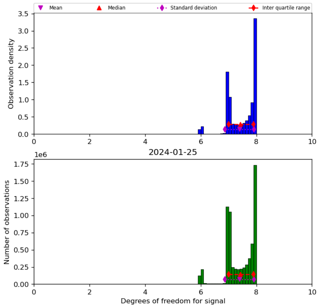
Figure 23: Histogram of “Degrees of freedom for signal” for 2024-01-24 to 2024-01-26
