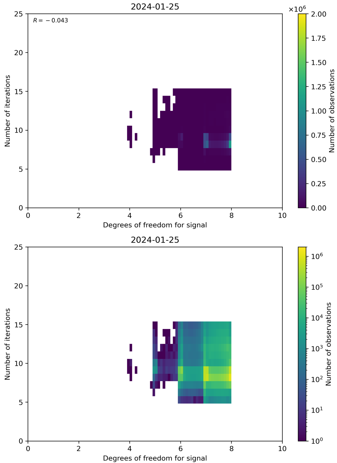
Figure 50: Scatter density plot of “Degrees of freedom for signal” against “Number of iterations” for 2024-01-24 to 2024-01-26.
