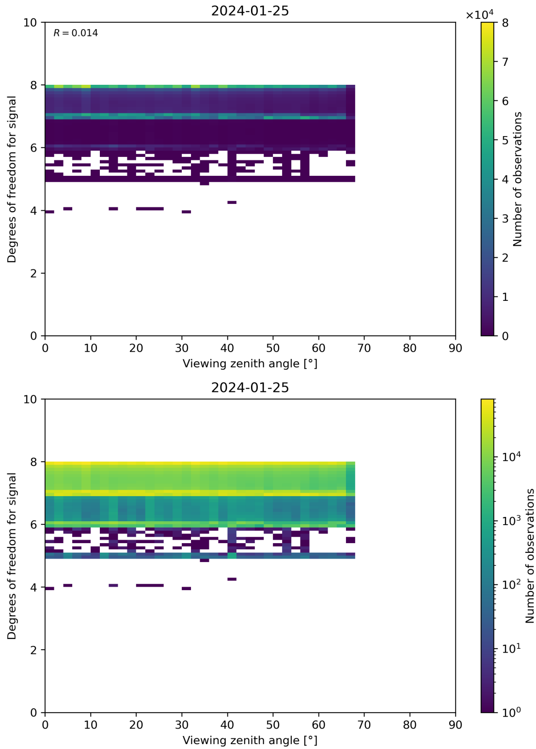
Figure 73: Scatter density plot of “Viewing zenith angle” against “Degrees of freedom for signal” for 2024-01-24 to 2024-01-26.
