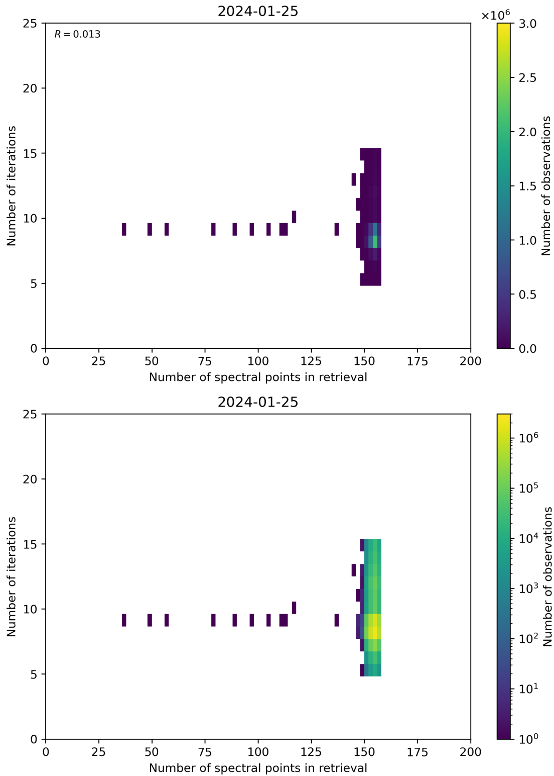
Figure 60: Scatter density plot of “Number of spectral points in retrieval” against “Number of iterations” for 2024-01-24 to 2024-01-26.
