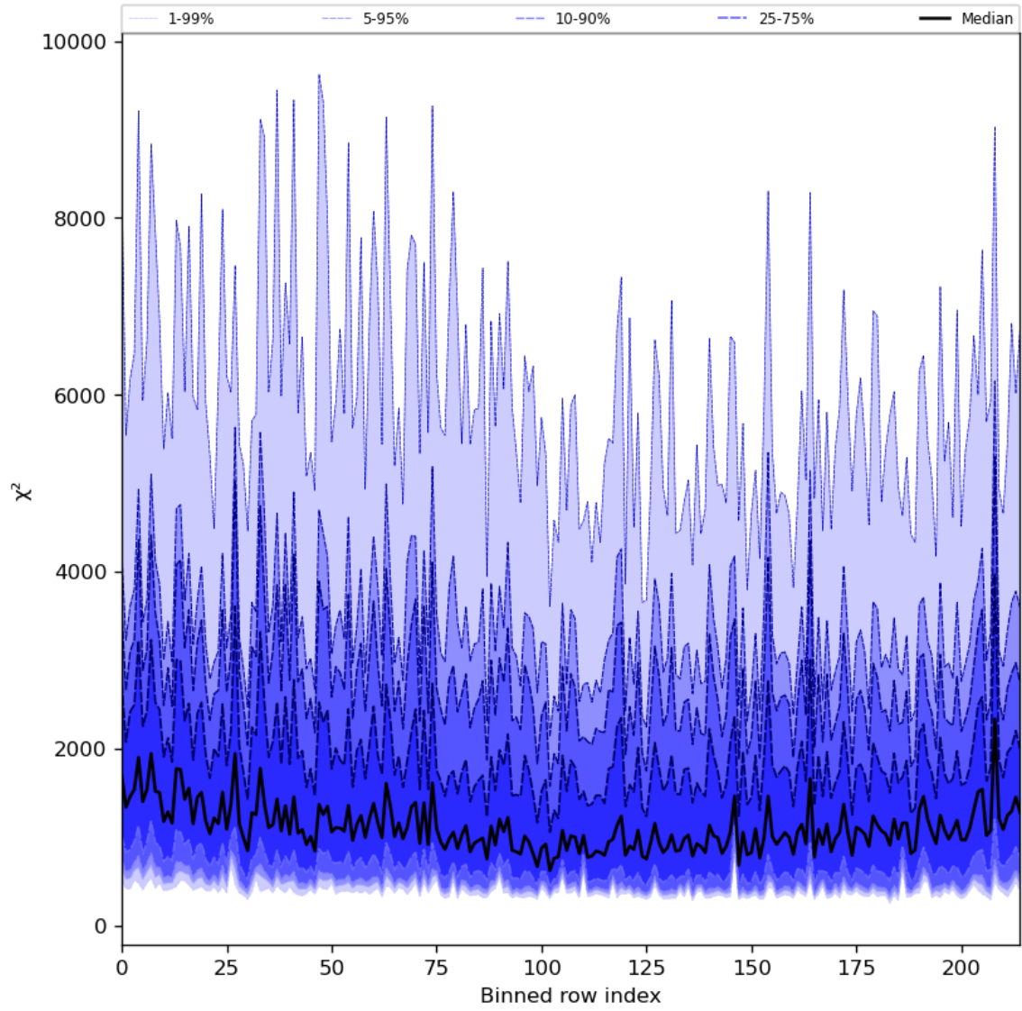
Figure 30: Along track statistics of “ \chi^2 ” for 2024-01-24 to 2024-01-26
