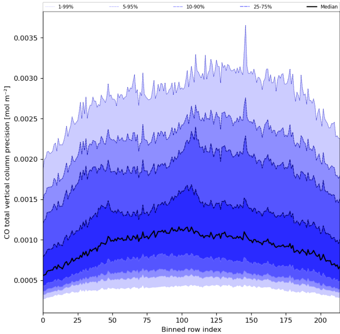
Figure 28: Along track statistics of “CO total vertical column precision” for 2024-01-24 to 2024-01-26
