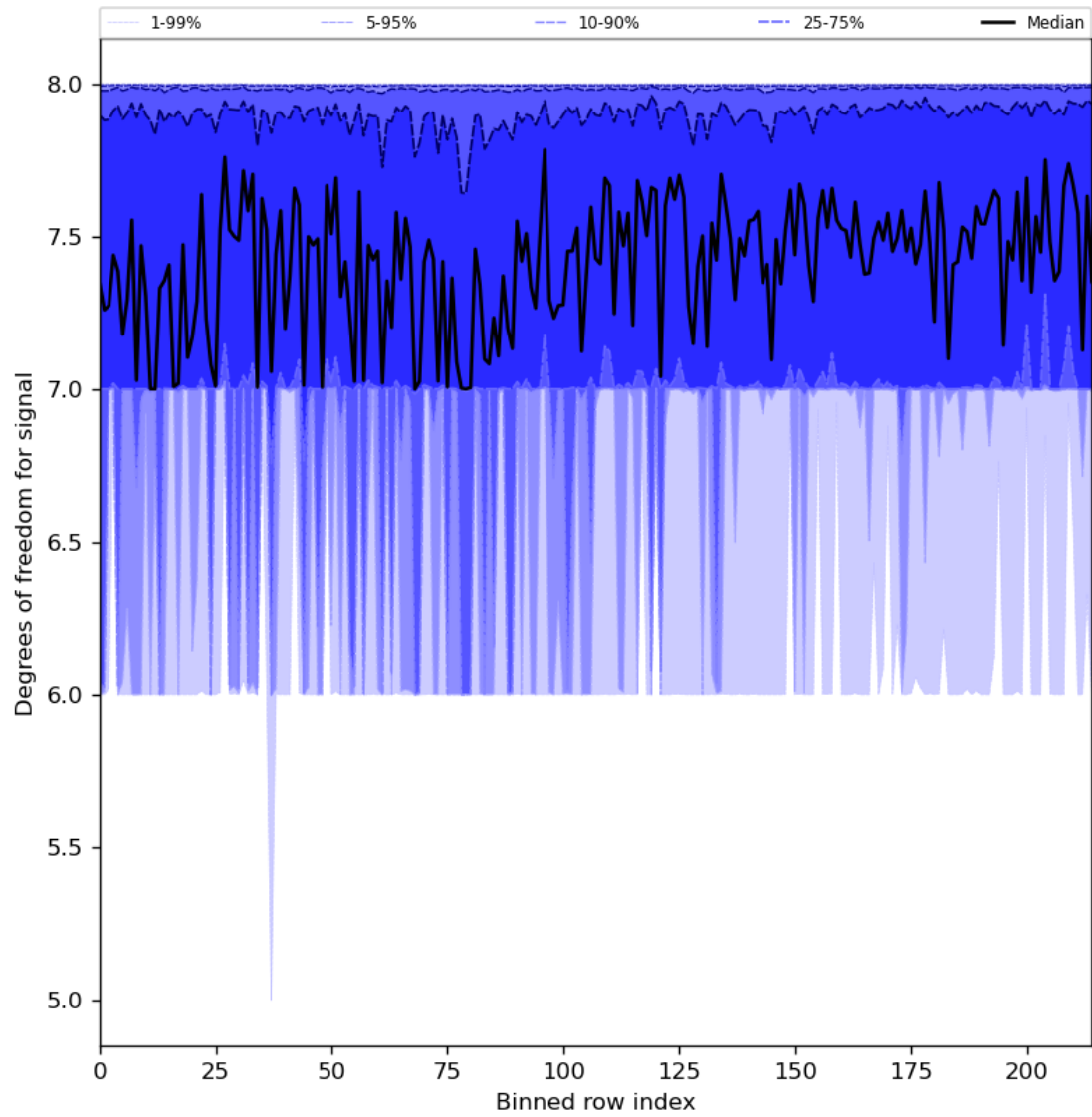
Figure 31: Along track statistics of “Degrees of freedom for signal” for 2024-01-24 to 2024-01-26
