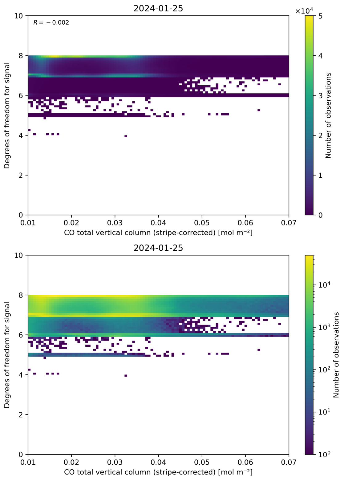
Figure 38: Scatter density plot of “CO total vertical column (stripe-corrected)” against “Degrees of freedom for signal” for 2024-01-24 to 2024-01-26.
