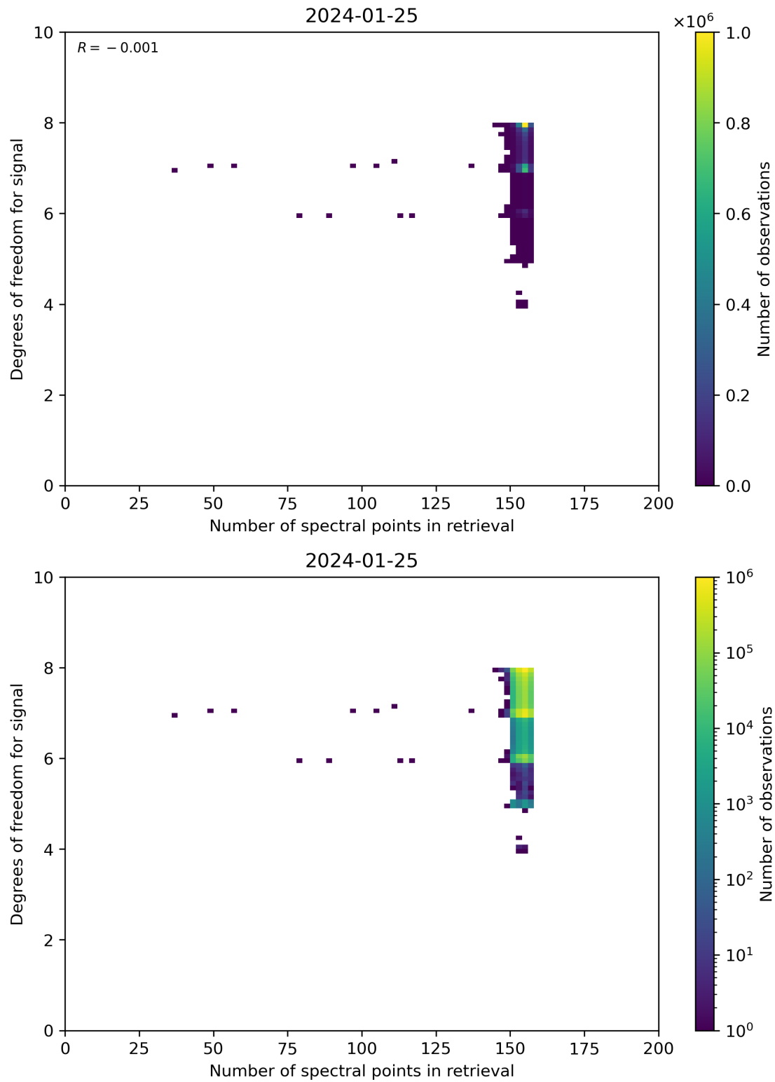
Figure 59: Scatter density plot of “Number of spectral points in retrieval” against “Degrees of freedom for signal” for 2024-01-24 to 2024-01-26.
