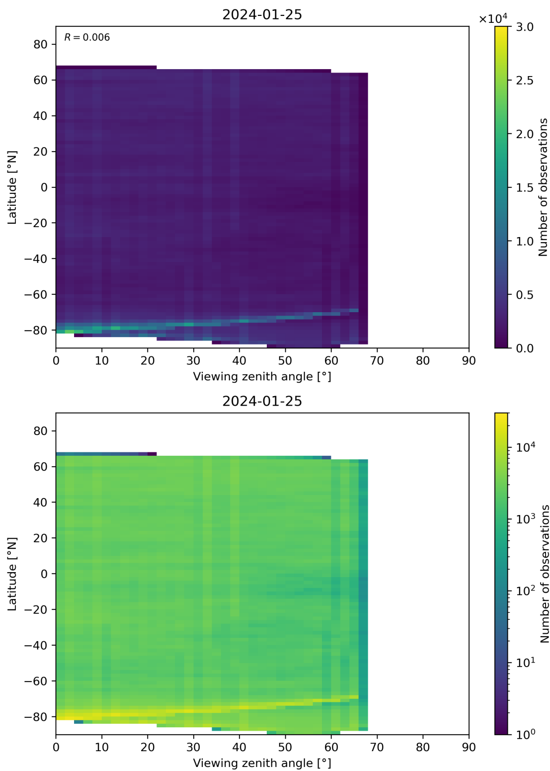
Figure 74: Scatter density plot of “Viewing zenith angle” against “Latitude” for 2024-01-24 to 2024-01-26.
