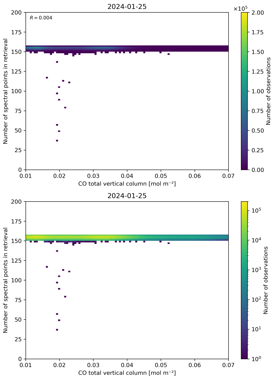
Figure 43: Scatter density plot of “CO total vertical column” against “Number of spectral points in retrieval” for 2024-01-24 to 2024-01-26.
