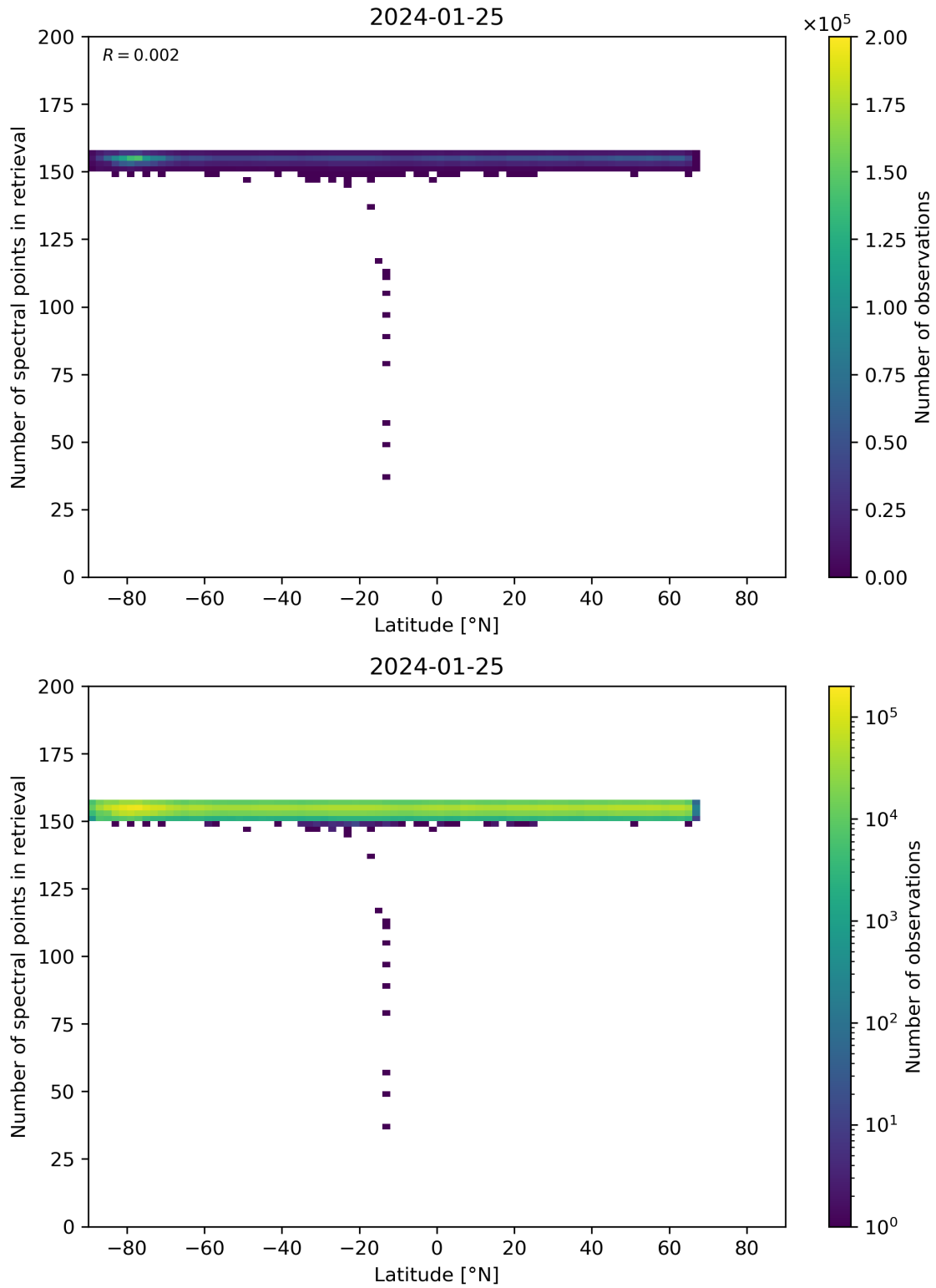
Figure 57: Scatter density plot of “Latitude” against “Number of spectral points in retrieval” for 2024-01-24 to 2024-01-26.
