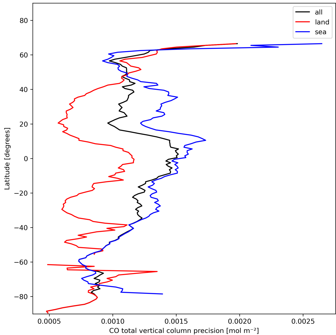
Figure 12: Zonal average of “CO total vertical column precision” for 2024-01-24 to 2024-01-26.
