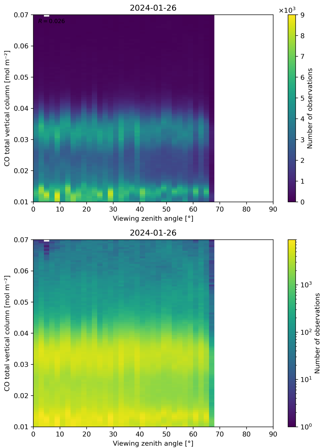
Figure 69: Scatter density plot of “Viewing zenith angle” against “CO total vertical column” for 2024-01-26 to 2024-01-27.
