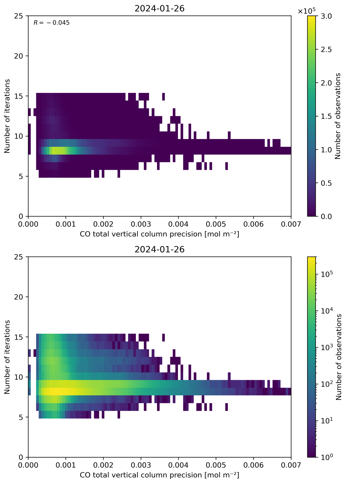
Figure 46: Scatter density plot of “CO total vertical column precision” against “Number of iterations” for 2024-01-26 to 2024-01-27.
