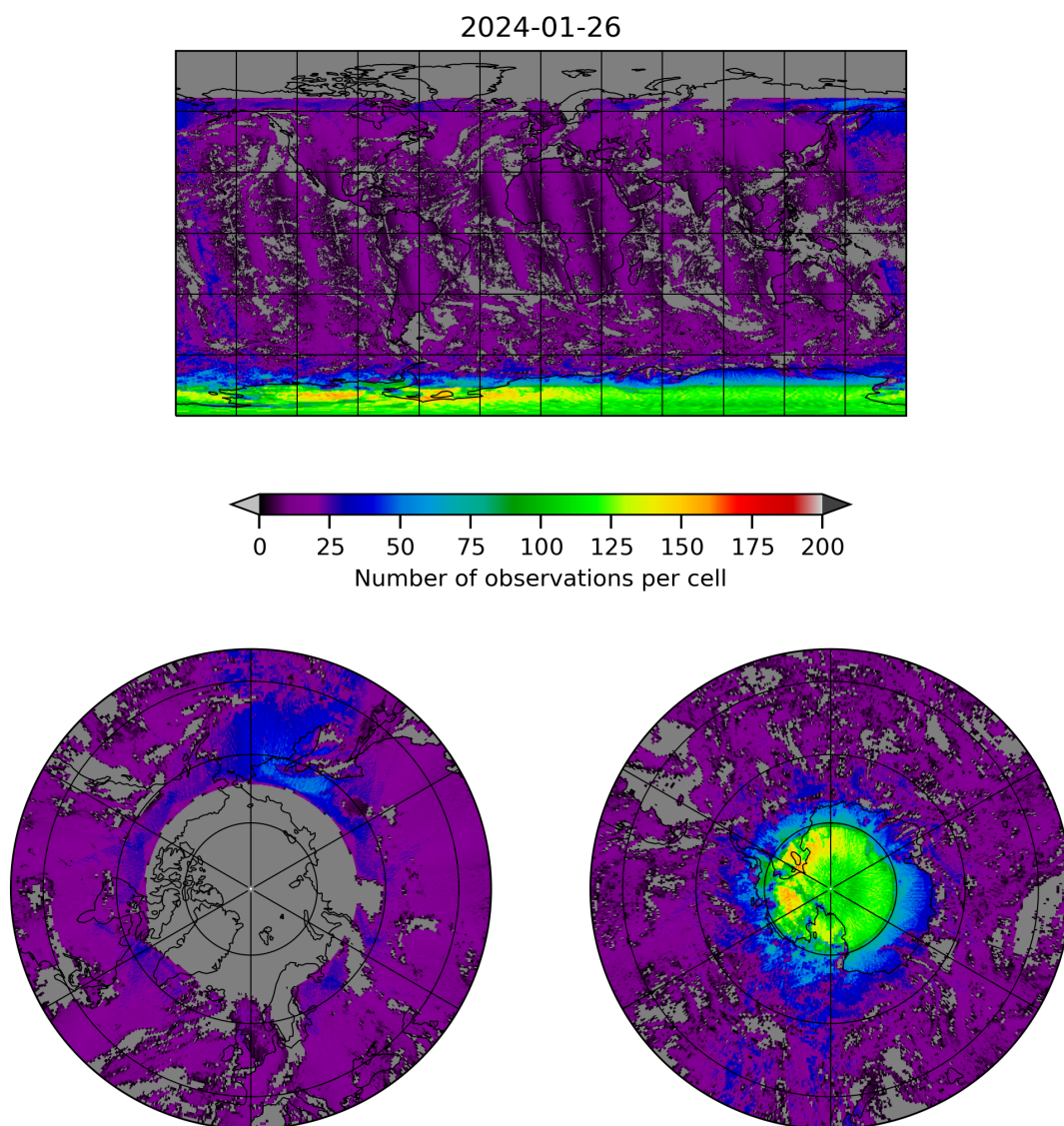
Figure 8: Map of the number of observations for 2024-01-26 to 2024-01-27
