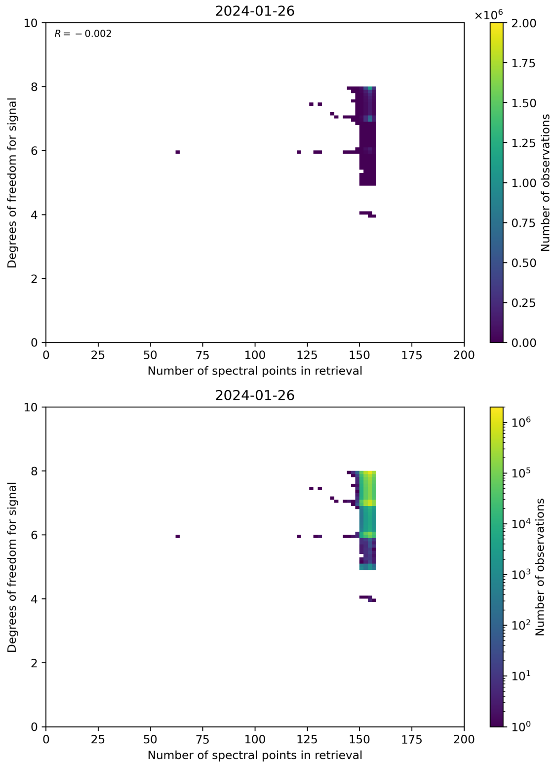
Figure 59: Scatter density plot of “Number of spectral points in retrieval” against “Degrees of freedom for signal” for 2024-01-26 to 2024-01-27.
