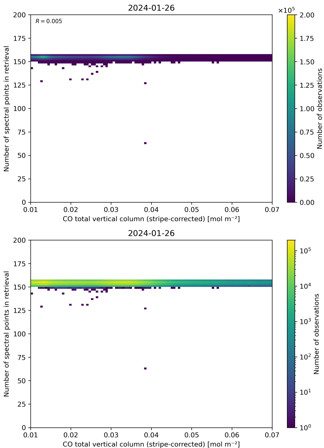
Figure 40: Scatter density plot of “CO total vertical column (stripe-corrected)” against “Number of spectral points in retrieval” for 2024-01-26 to 2024-01-27.
