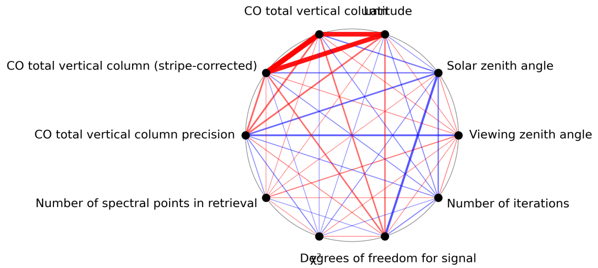
Figure 1: Map of correlation graph for 2024-01-26 to 2024-01-27.
