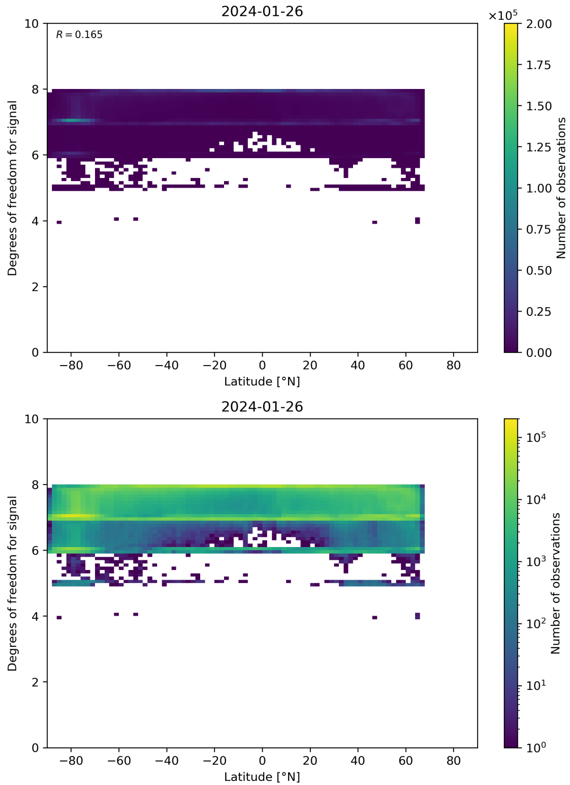
Figure 55: Scatter density plot of “Latitude” against “Degrees of freedom for signal” for 2024-01-26 to 2024-01-27.
