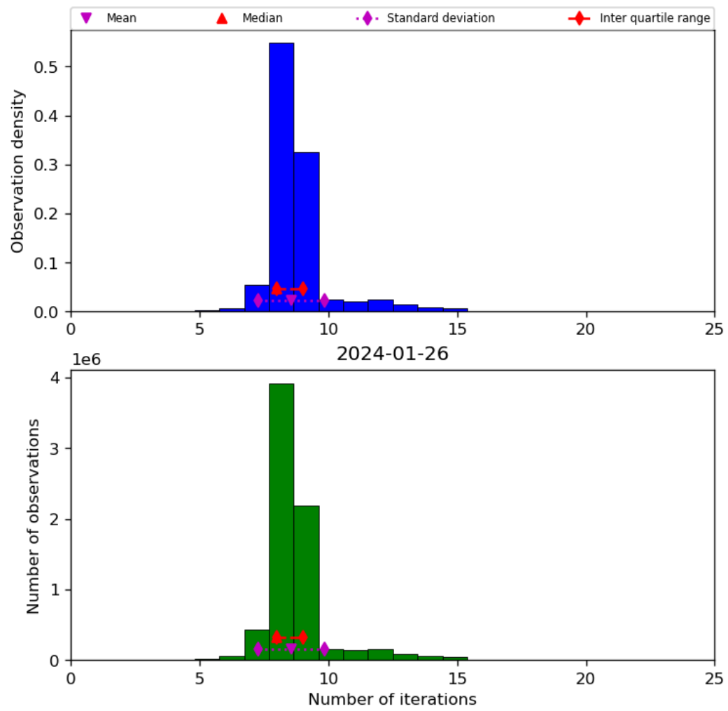
Figure 24: Histogram of “Number of iterations” for 2024-01-26 to 2024-01-27
