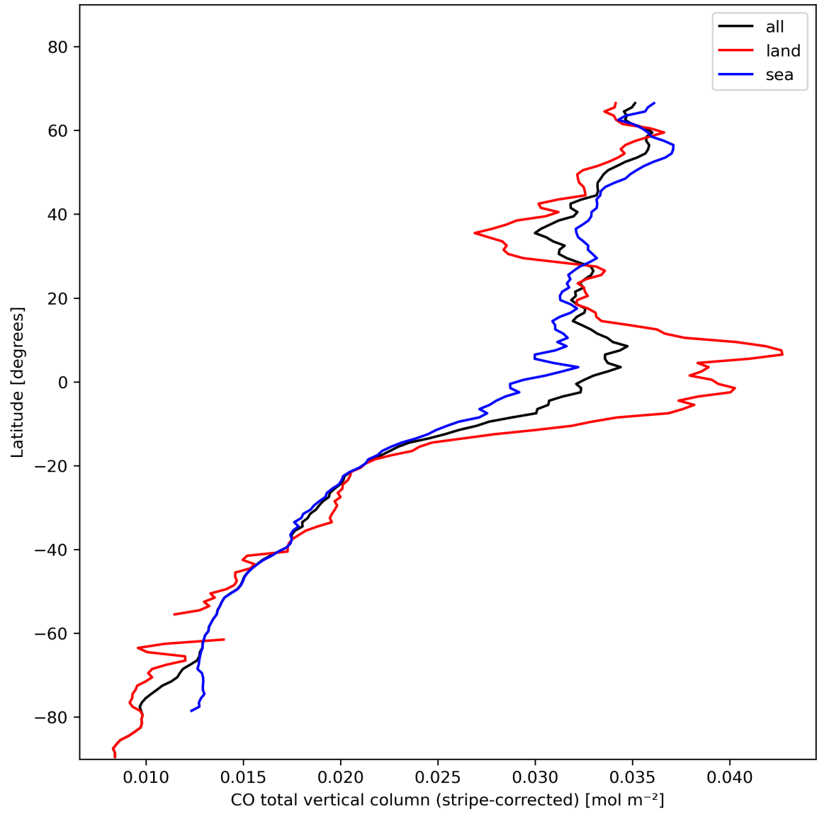
Figure 11: Zonal average of “CO total vertical column (stripe-corrected)” for 2024-01-26 to 2024-01-27.
