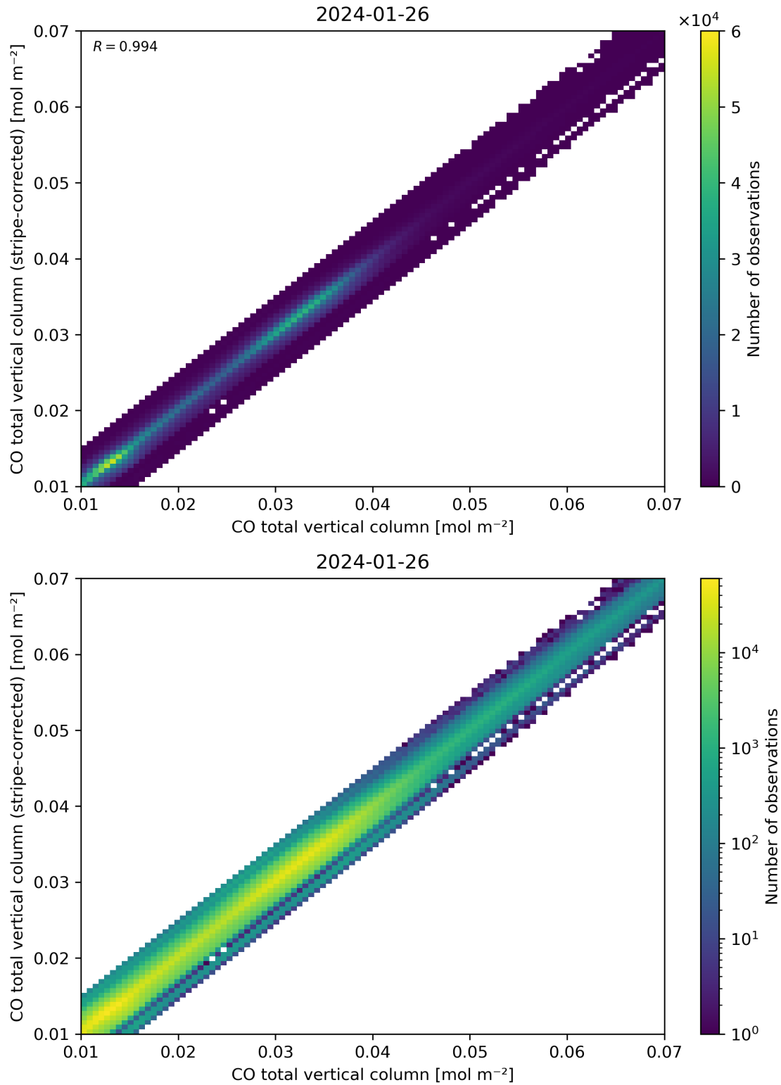
Figure 33: Scatter density plot of “CO total vertical column” against “CO total vertical column (stripe-corrected)” for 2024-01-26 to 2024-01-27.
