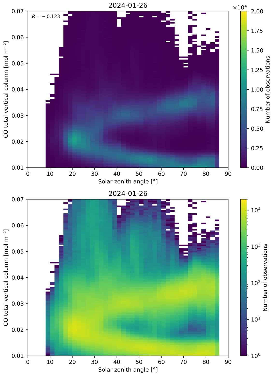
Figure 61: Scatter density plot of “Solar zenith angle” against “CO total vertical column” for 2024-01-26 to 2024-01-27.
