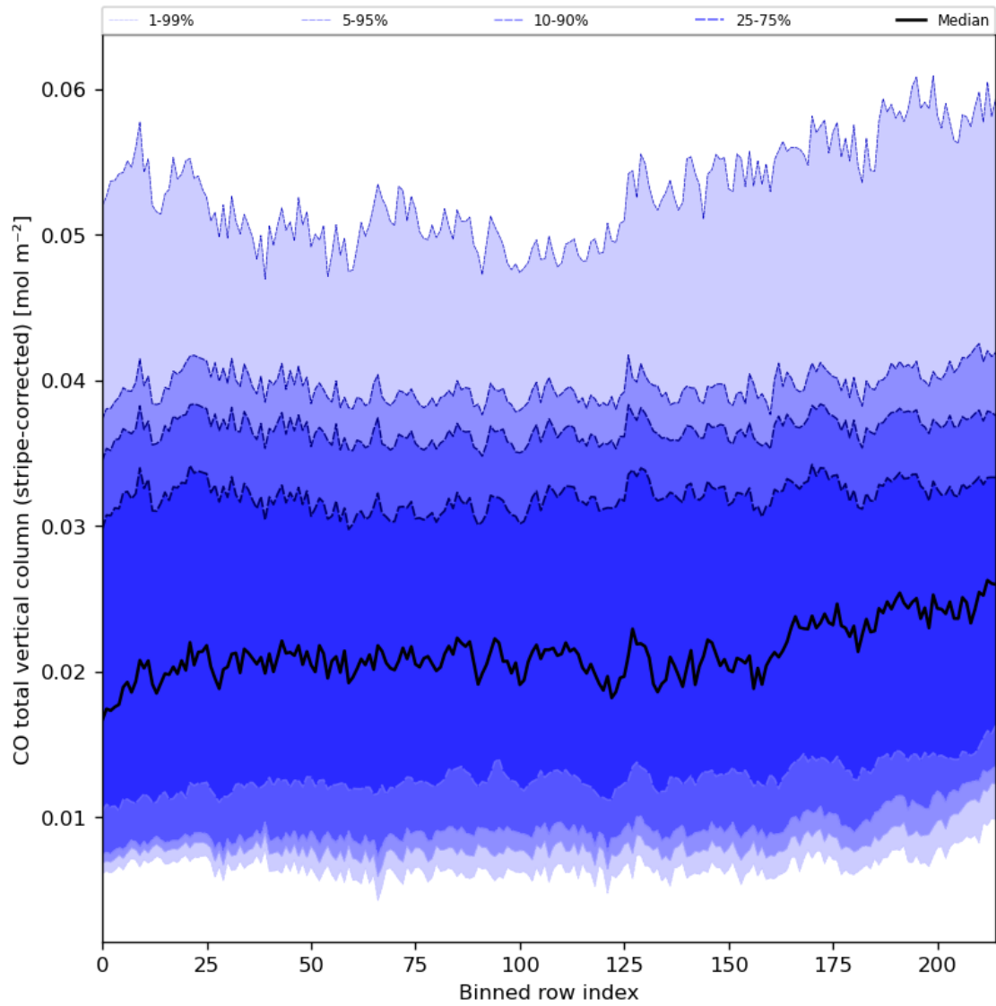
Figure 27: Along track statistics of “CO total vertical column (stripe-corrected)” for 2024-01-26 to 2024-01-27
