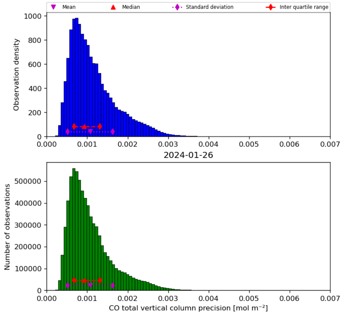
Figure 20: Histogram of “CO total vertical column precision” for 2024-01-26 to 2024-01-27
