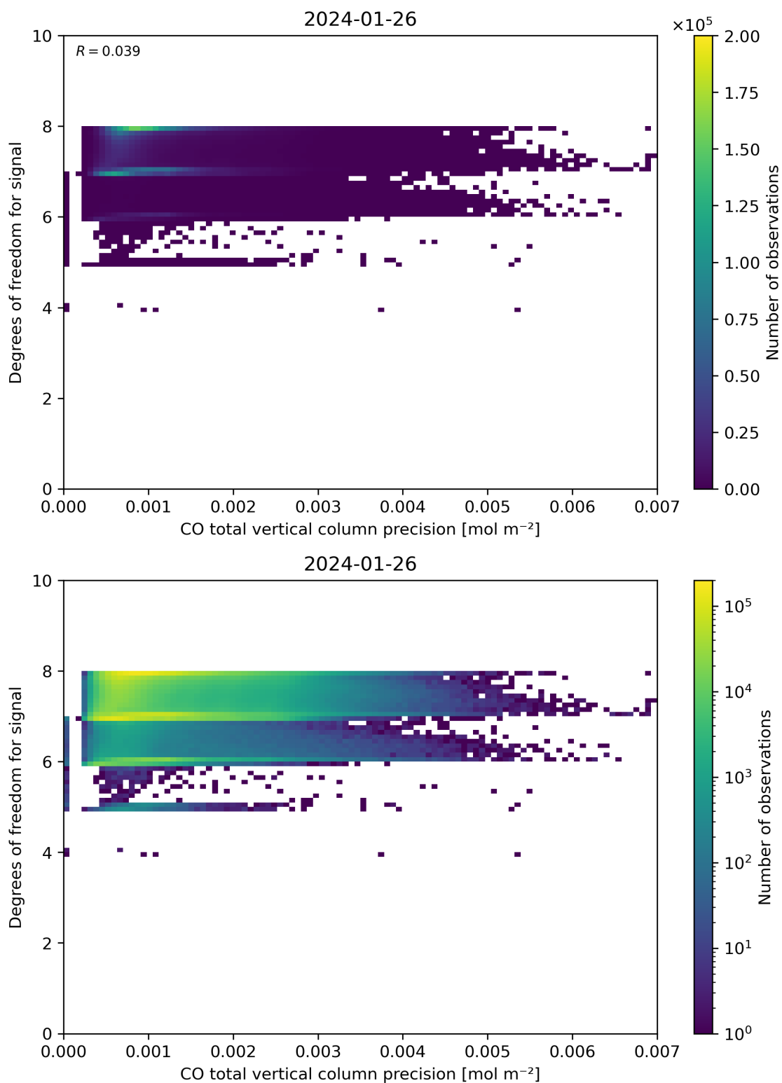
Figure 45: Scatter density plot of “CO total vertical column precision” against “Degrees of freedom for signal” for 2024-01-26 to 2024-01-27.
