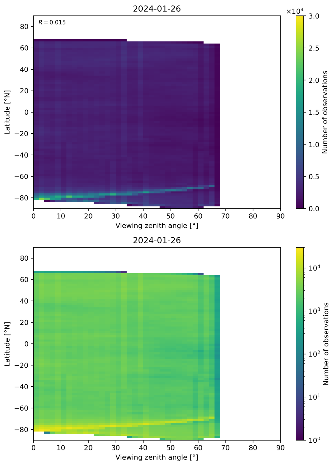
Figure 74: Scatter density plot of “Viewing zenith angle” against “Latitude” for 2024-01-26 to 2024-01-27.
