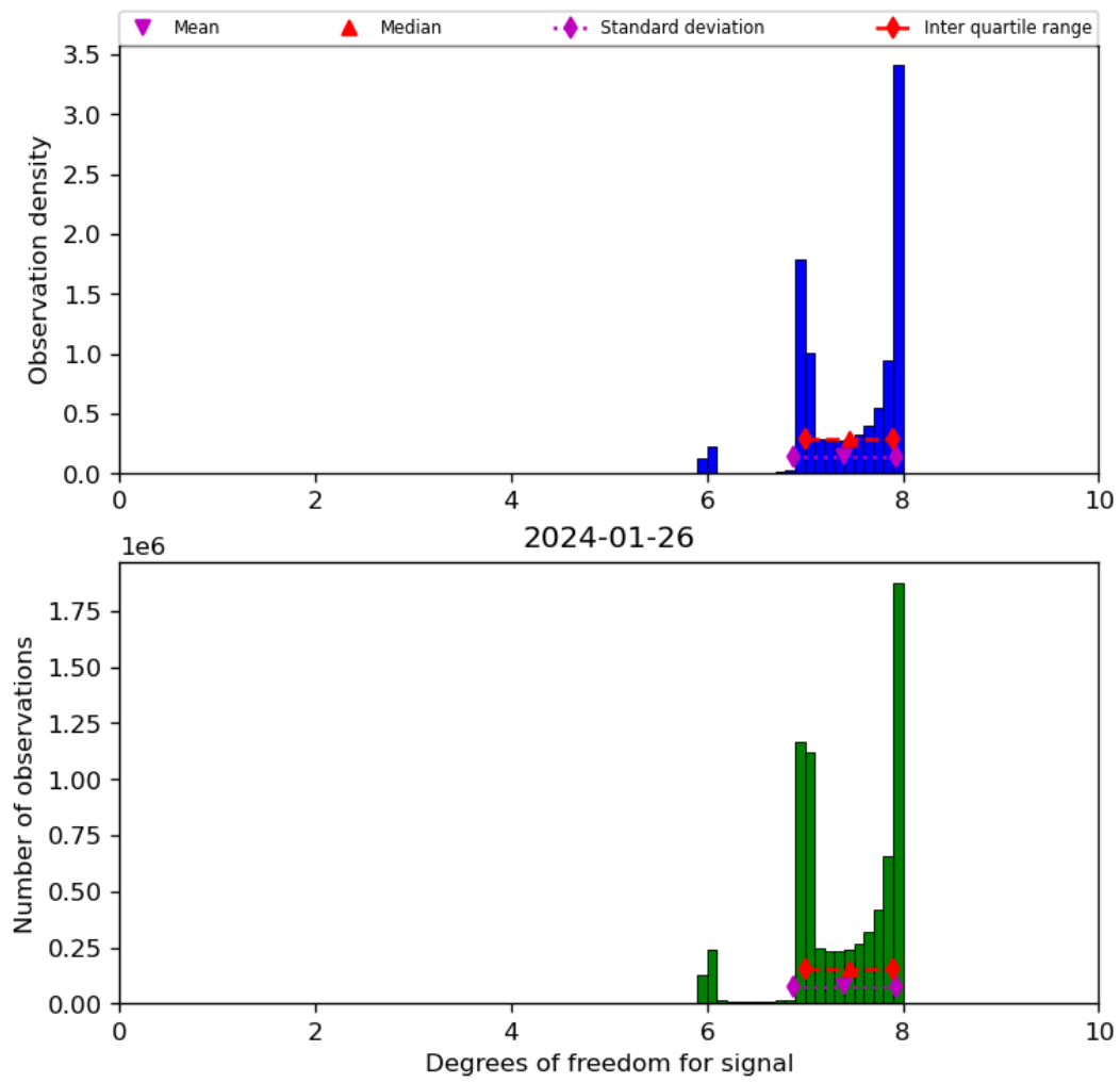
Figure 23: Histogram of “Degrees of freedom for signal” for 2024-01-26 to 2024-01-27
