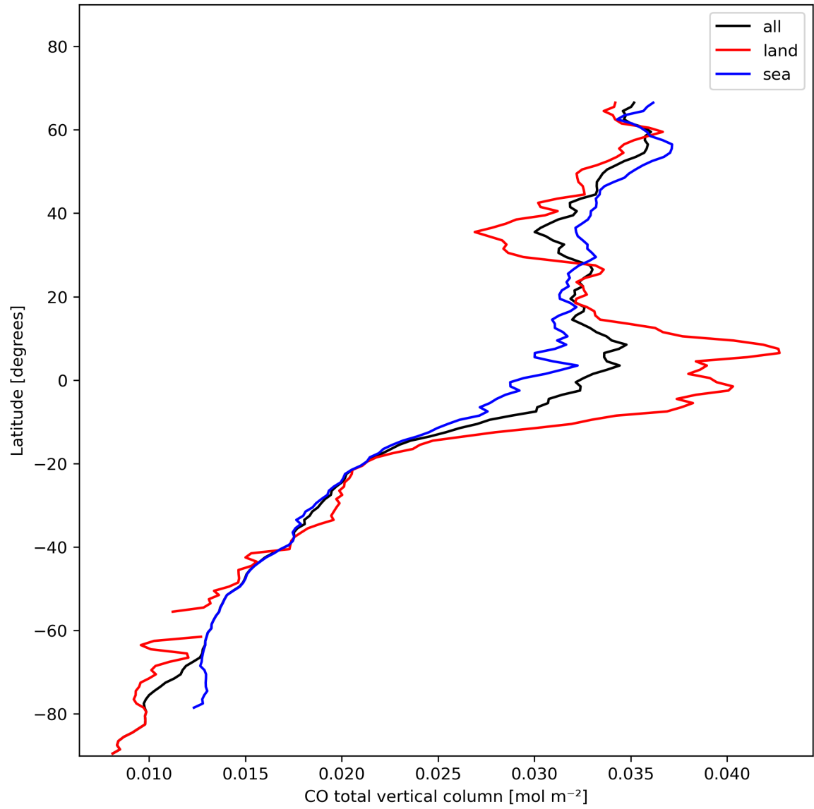
Figure 10: Zonal average of “CO total vertical column” for 2024-01-26 to 2024-01-27.
