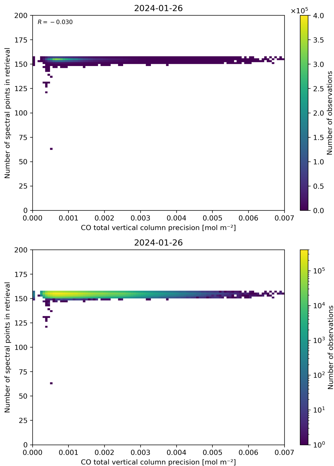
Figure 47: Scatter density plot of “CO total vertical column precision” against “Number of spectral points in retrieval” for 2024-01-26 to 2024-01-27.
