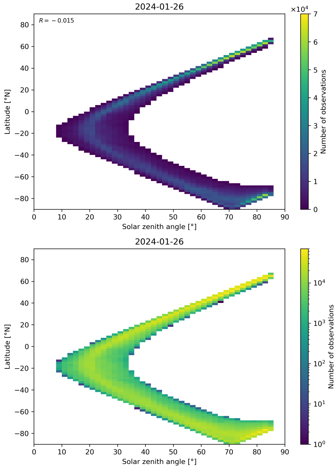
Figure 66: Scatter density plot of “Solar zenith angle” against “Latitude” for 2024-01-26 to 2024-01-27.
