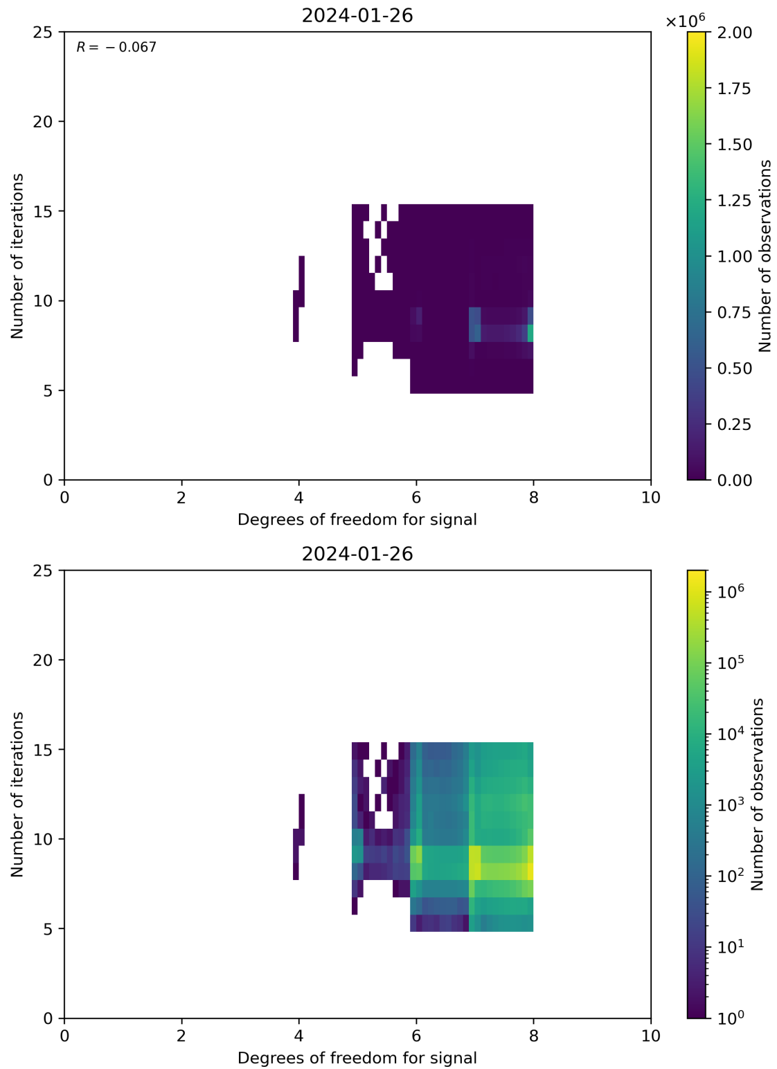
Figure 50: Scatter density plot of “Degrees of freedom for signal” against “Number of iterations” for 2024-01-26 to 2024-01-27.
