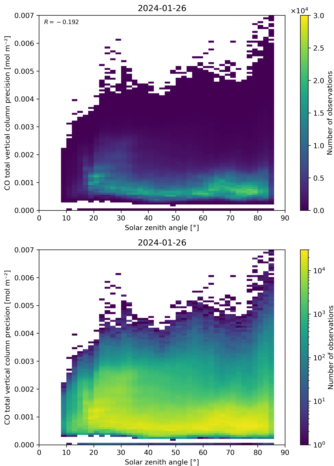
Figure 63: Scatter density plot of “Solar zenith angle” against “CO total vertical column precision” for 2024-01-26 to 2024-01-27.
