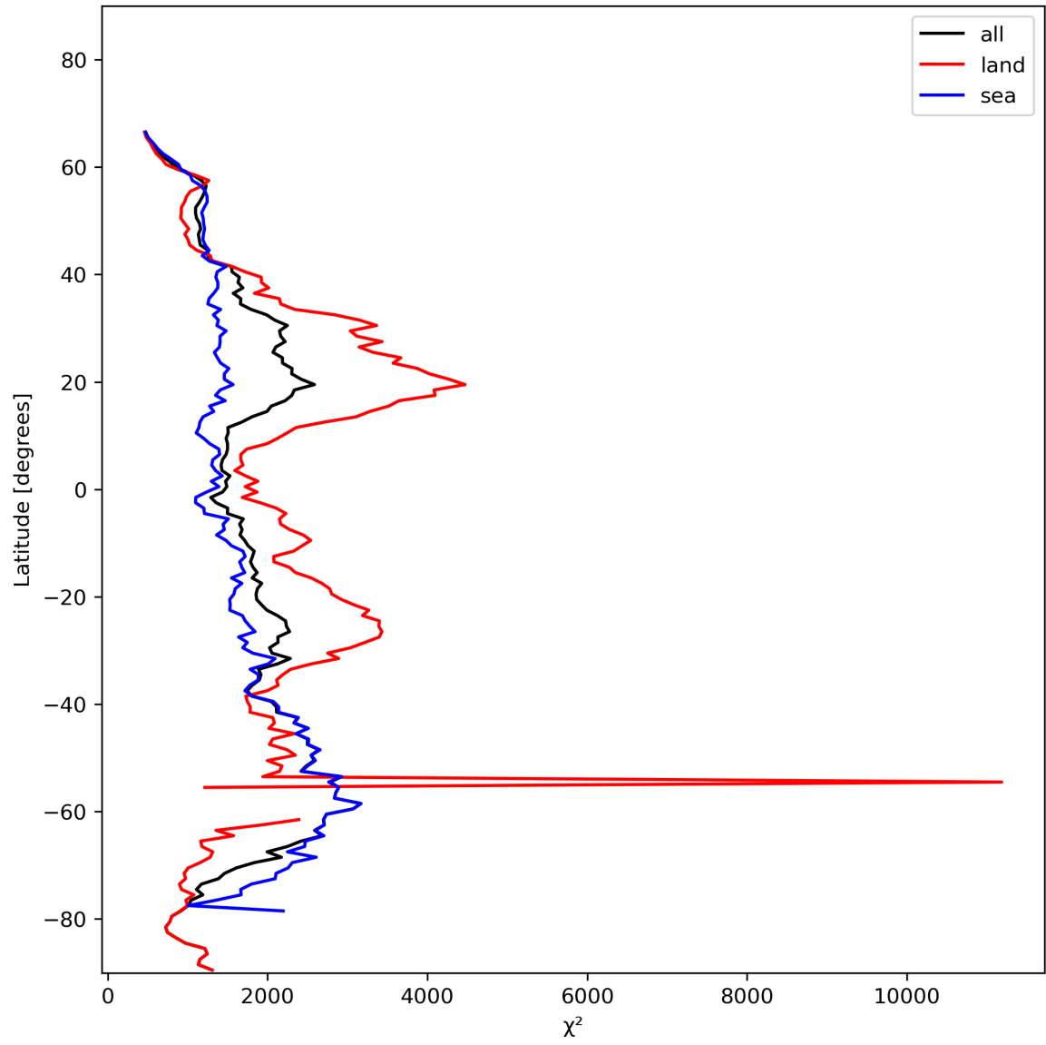
Figure 14: Zonal average of “ \chi^2 ” for 2024-01-26 to 2024-01-27.
