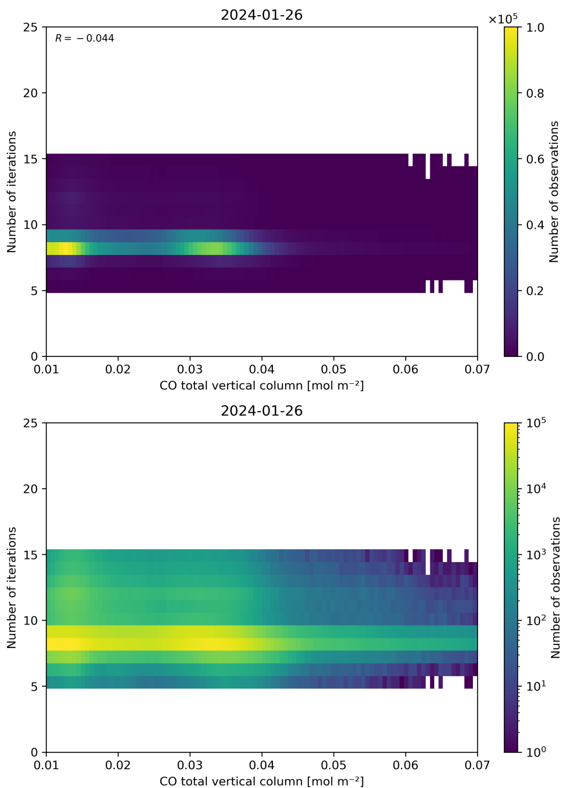
Figure 42: Scatter density plot of “CO total vertical column” against “Number of iterations” for 2024-01-26 to 2024-01-27.
