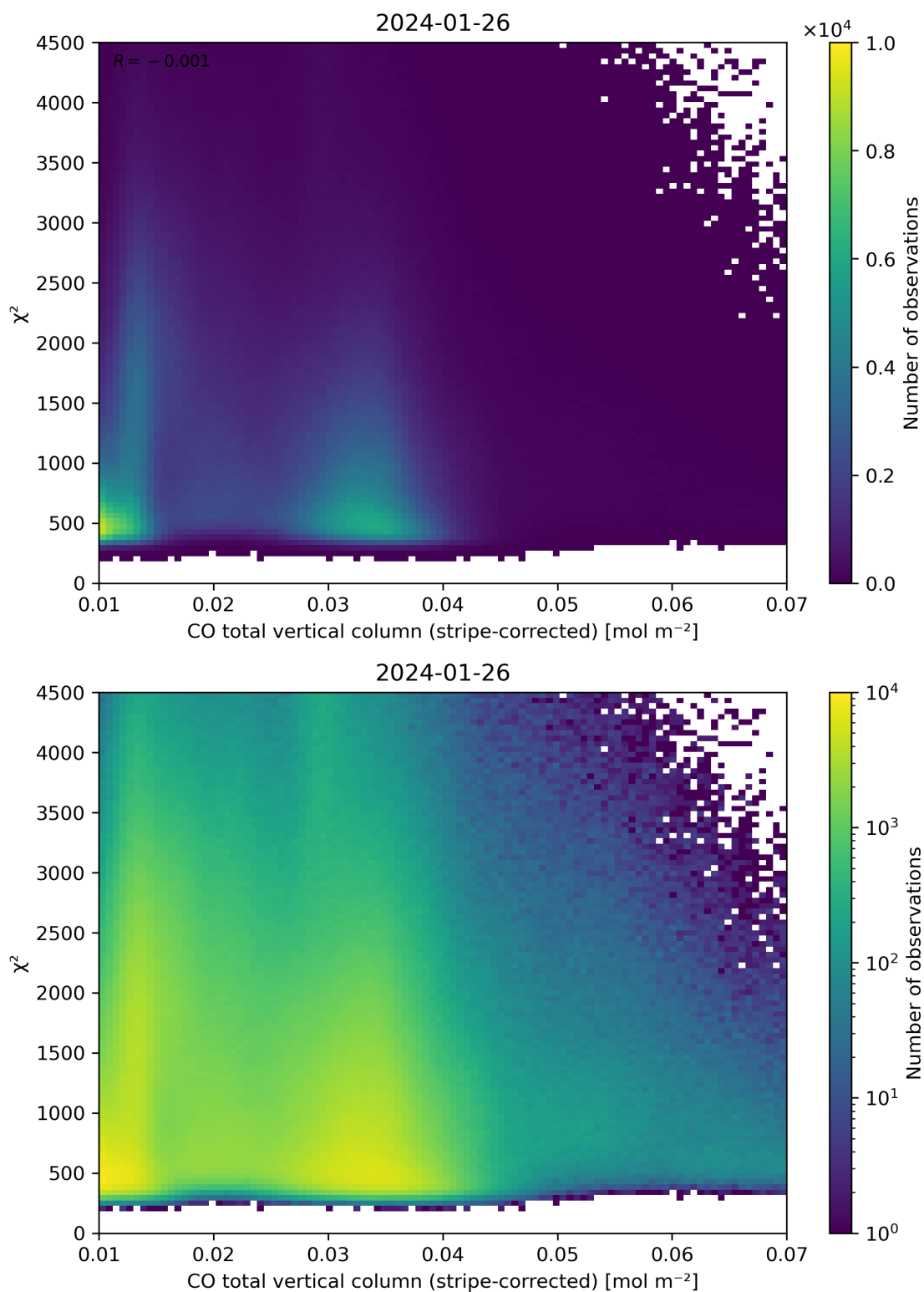
Figure 37: Scatter density plot of “CO total vertical column (stripe-corrected)” against “ \chi^2 ” for 2024-01-26 to 2024-01-27.
