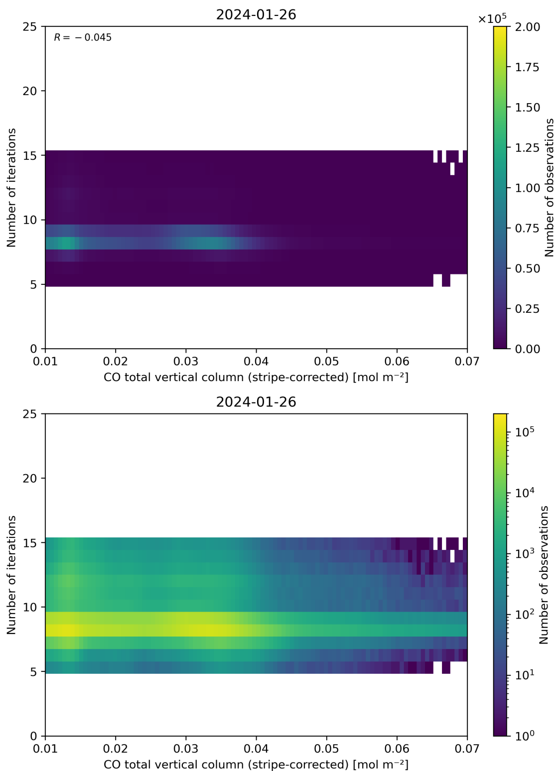
Figure 39: Scatter density plot of “CO total vertical column (stripe-corrected)” against “Number of iterations” for 2024-01-26 to 2024-01-27.
