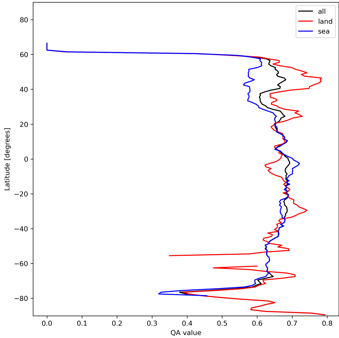
Figure 9: Zonal average of “QA value” for 2024-01-26 to 2024-01-27.
