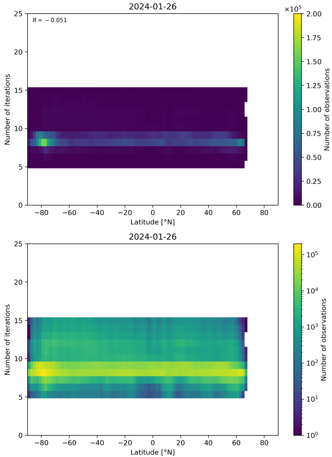
Figure 56: Scatter density plot of “Latitude” against “Number of iterations” for 2024-01-26 to 2024-01-27.
