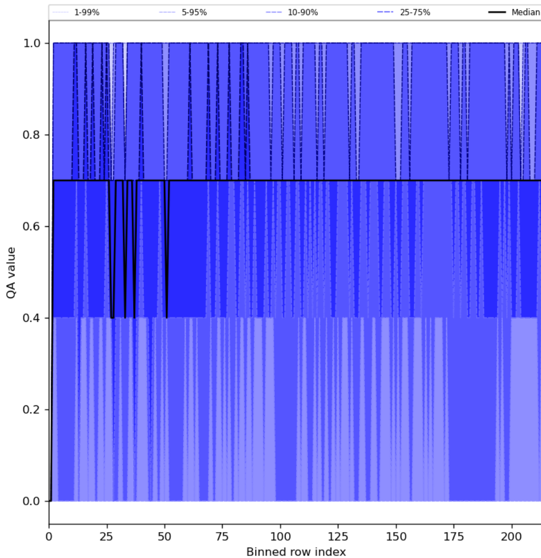
Figure 25: Along track statistics of “QA value” for 2024-01-26 to 2024-01-27
