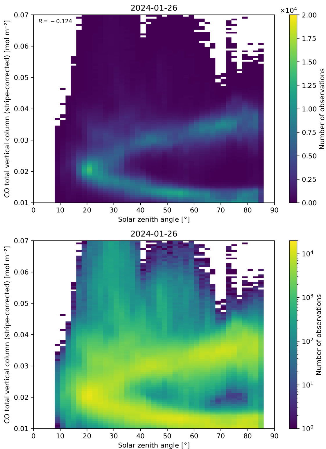
Figure 62: Scatter density plot of “Solar zenith angle” against “CO total vertical column (stripe-corrected)” for 2024-01-26 to 2024-01-27.
