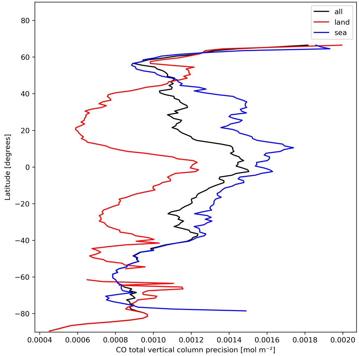
Figure 12: Zonal average of “CO total vertical column precision” for 2024-01-26 to 2024-01-27.
