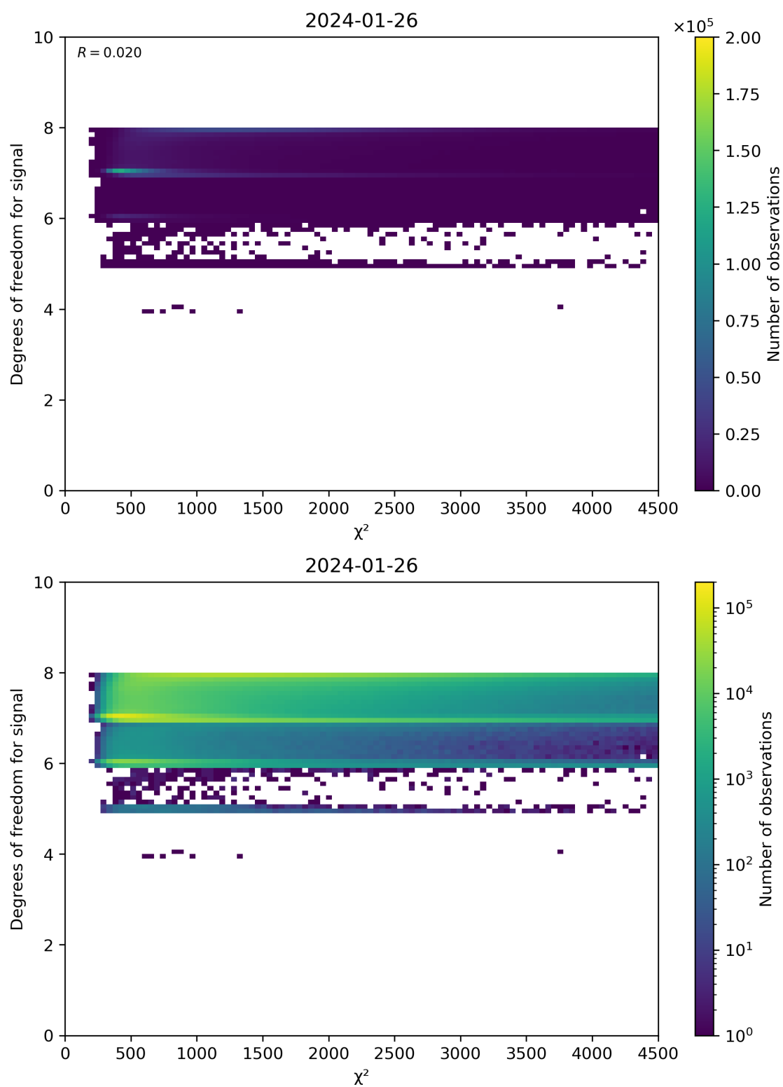
Figure 48: Scatter density plot of “ \chi^2 ” against “Degrees of freedom for signal” for 2024-01-26 to 2024-01-27.
