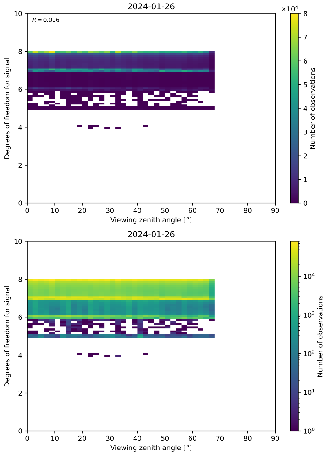
Figure 73: Scatter density plot of “Viewing zenith angle” against “Degrees of freedom for signal” for 2024-01-26 to 2024-01-27.
