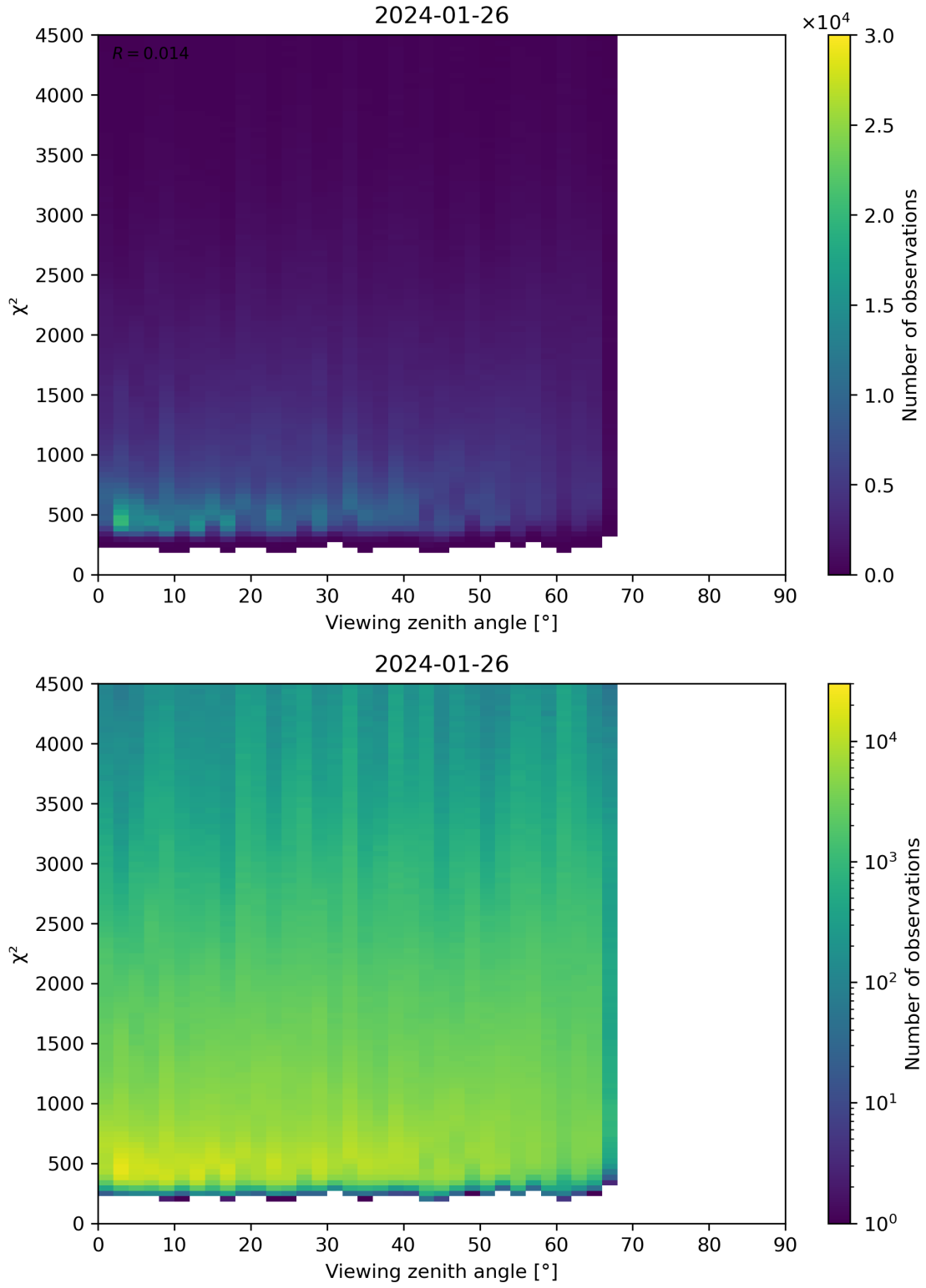
Figure 72: Scatter density plot of “Viewing zenith angle” against “ \chi^2 ” for 2024-01-26 to 2024-01-27.
