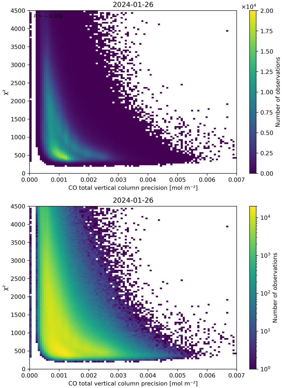
Figure 44: Scatter density plot of “CO total vertical column precision” against “ \chi^2 ” for 2024-01-26 to 2024-01-27.
