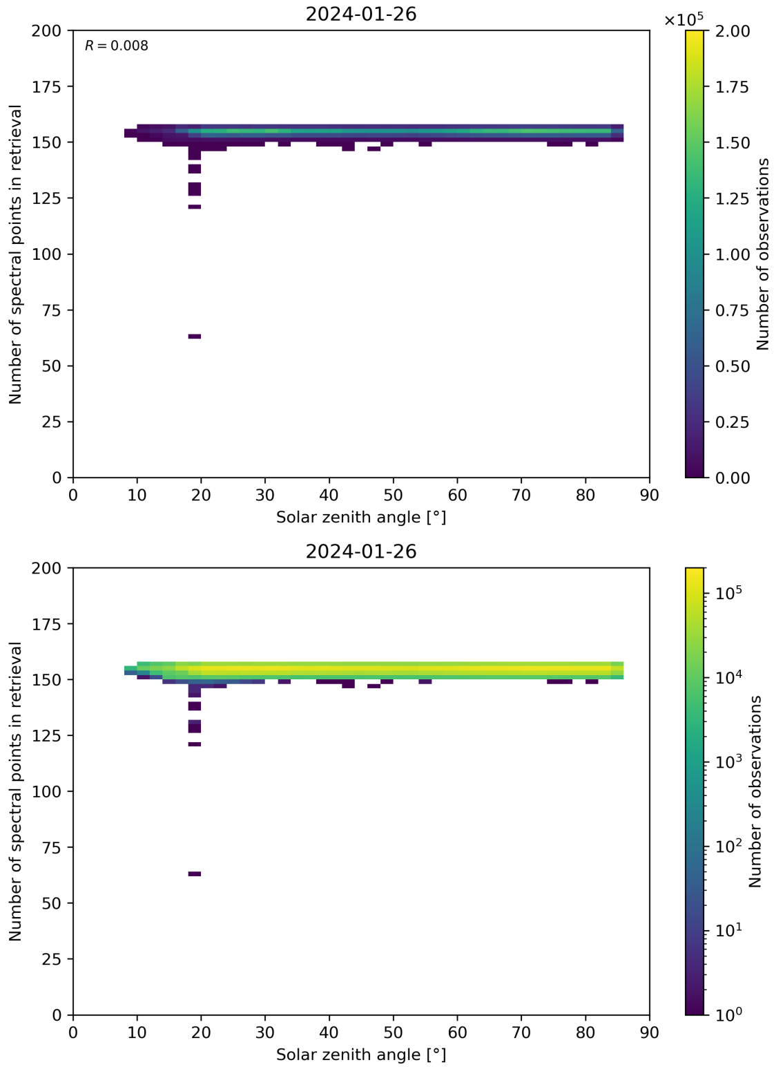
Figure 68: Scatter density plot of “Solar zenith angle” against “Number of spectral points in retrieval” for 2024-01-26 to 2024-01-27.
