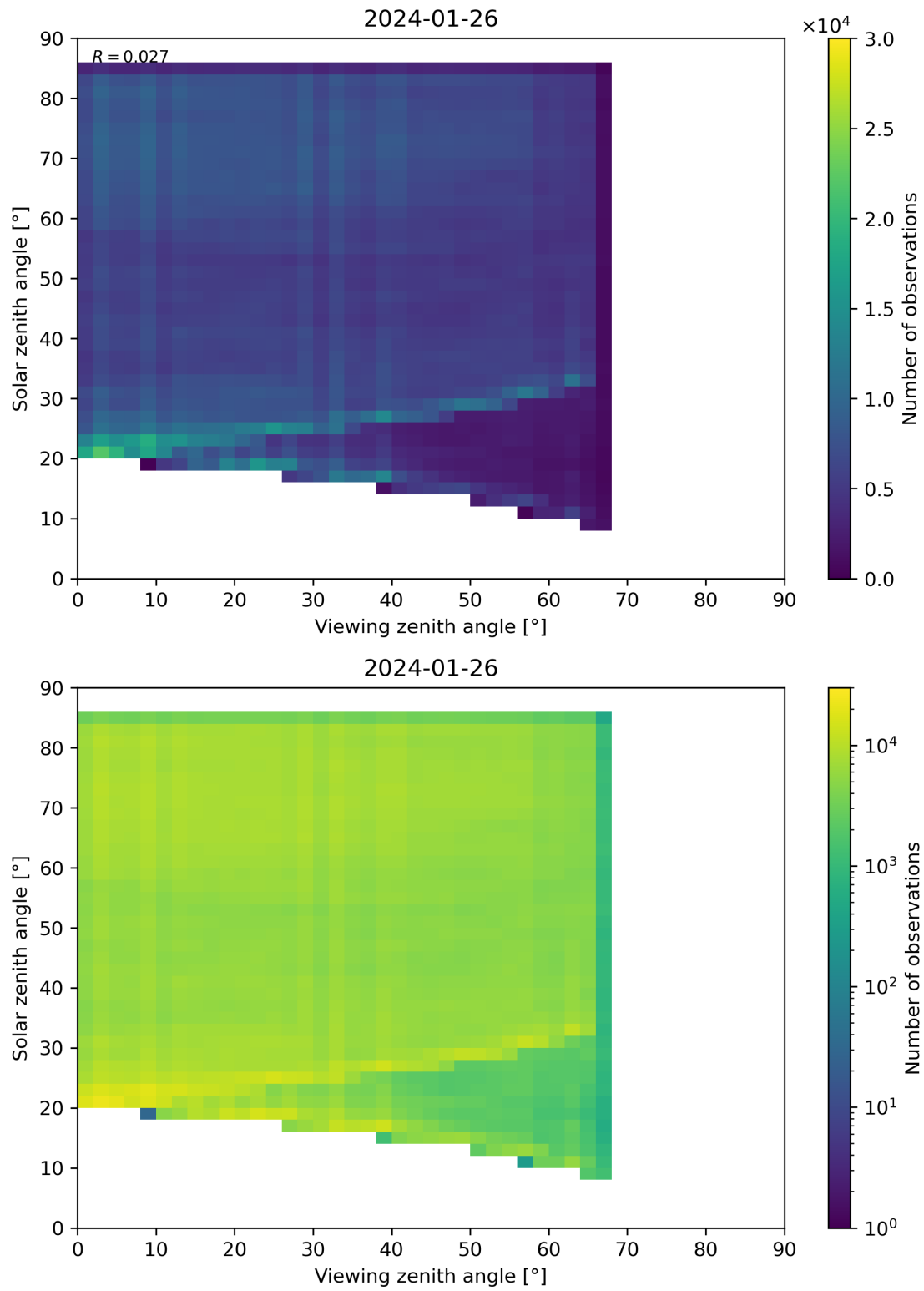
Figure 77: Scatter density plot of “Viewing zenith angle” against “Solar zenith angle” for 2024-01-26 to 2024-01-27.
