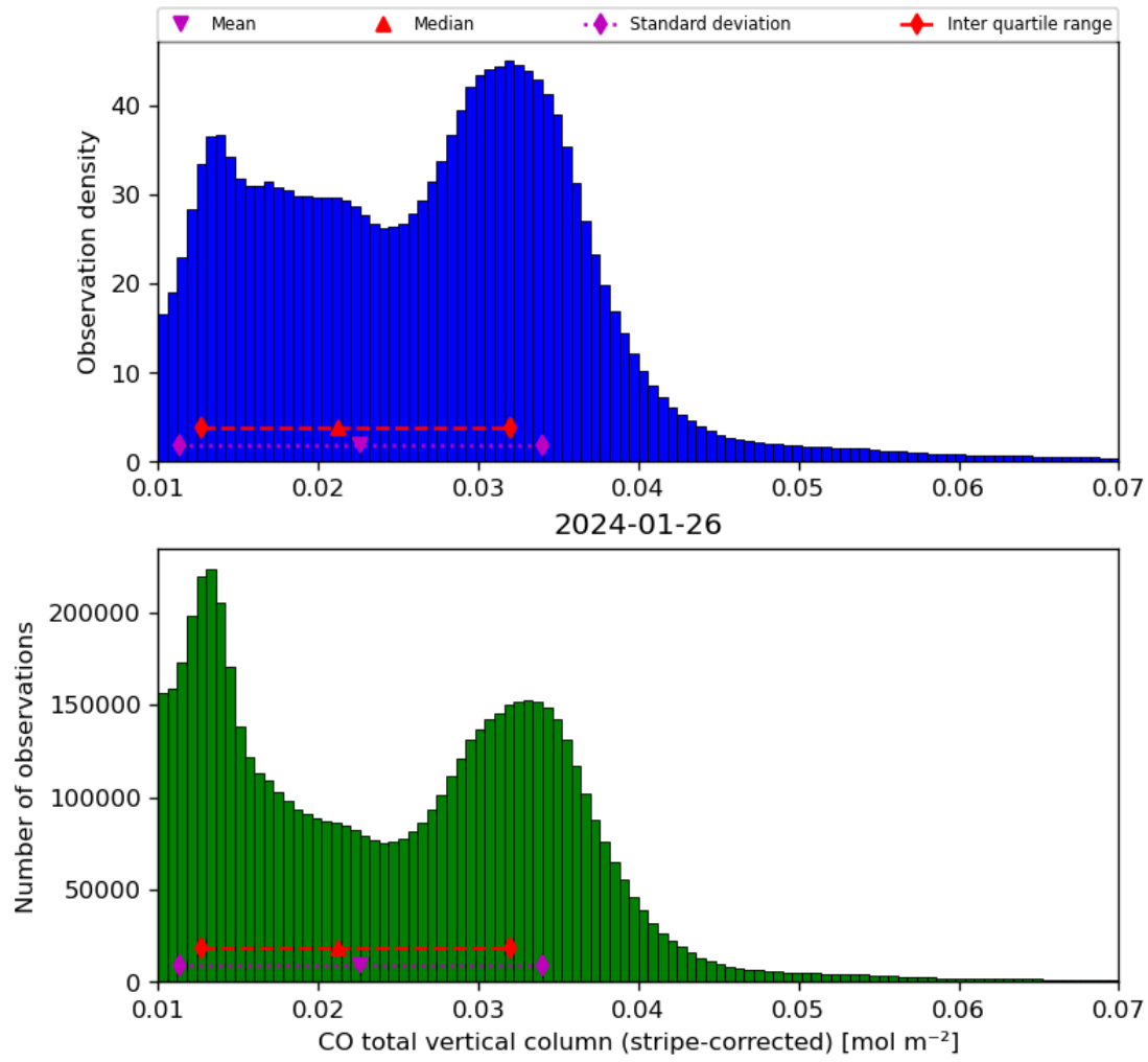
Figure 19: Histogram of “CO total vertical column (stripe-corrected)” for 2024-01-26 to 2024-01-27
