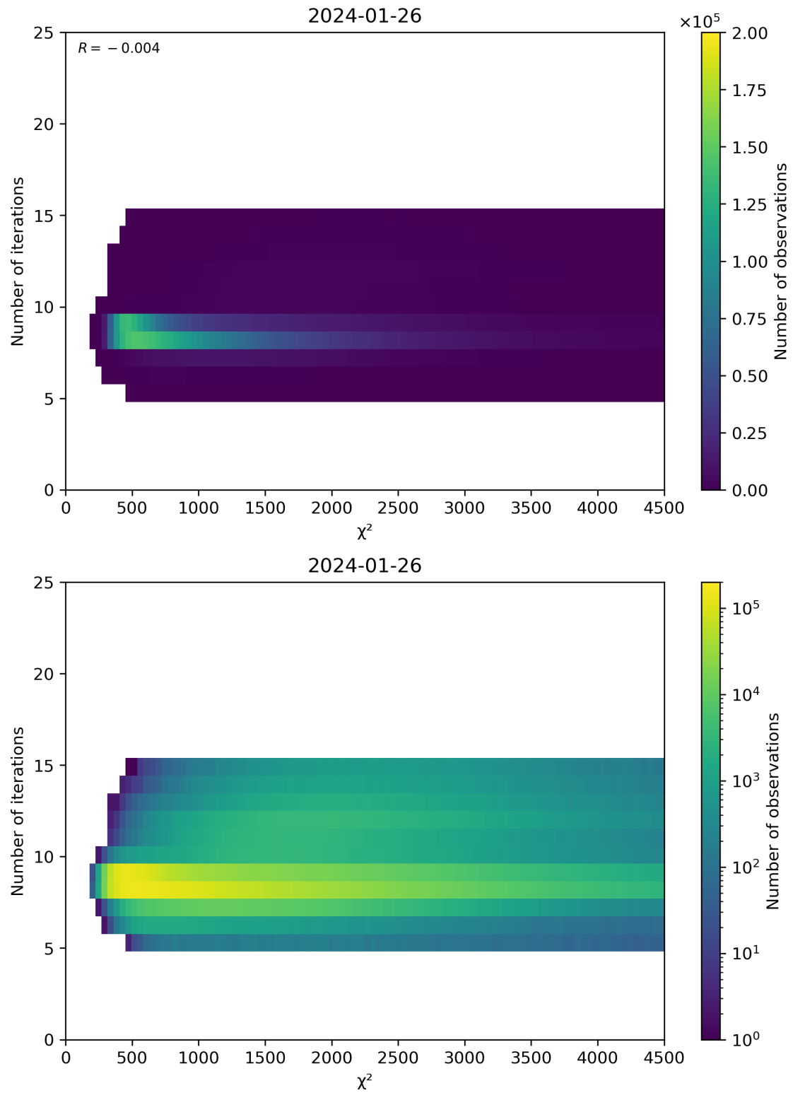
Figure 49: Scatter density plot of “ \chi^2 ” against “Number of iterations” for 2024-01-26 to 2024-01-27.
