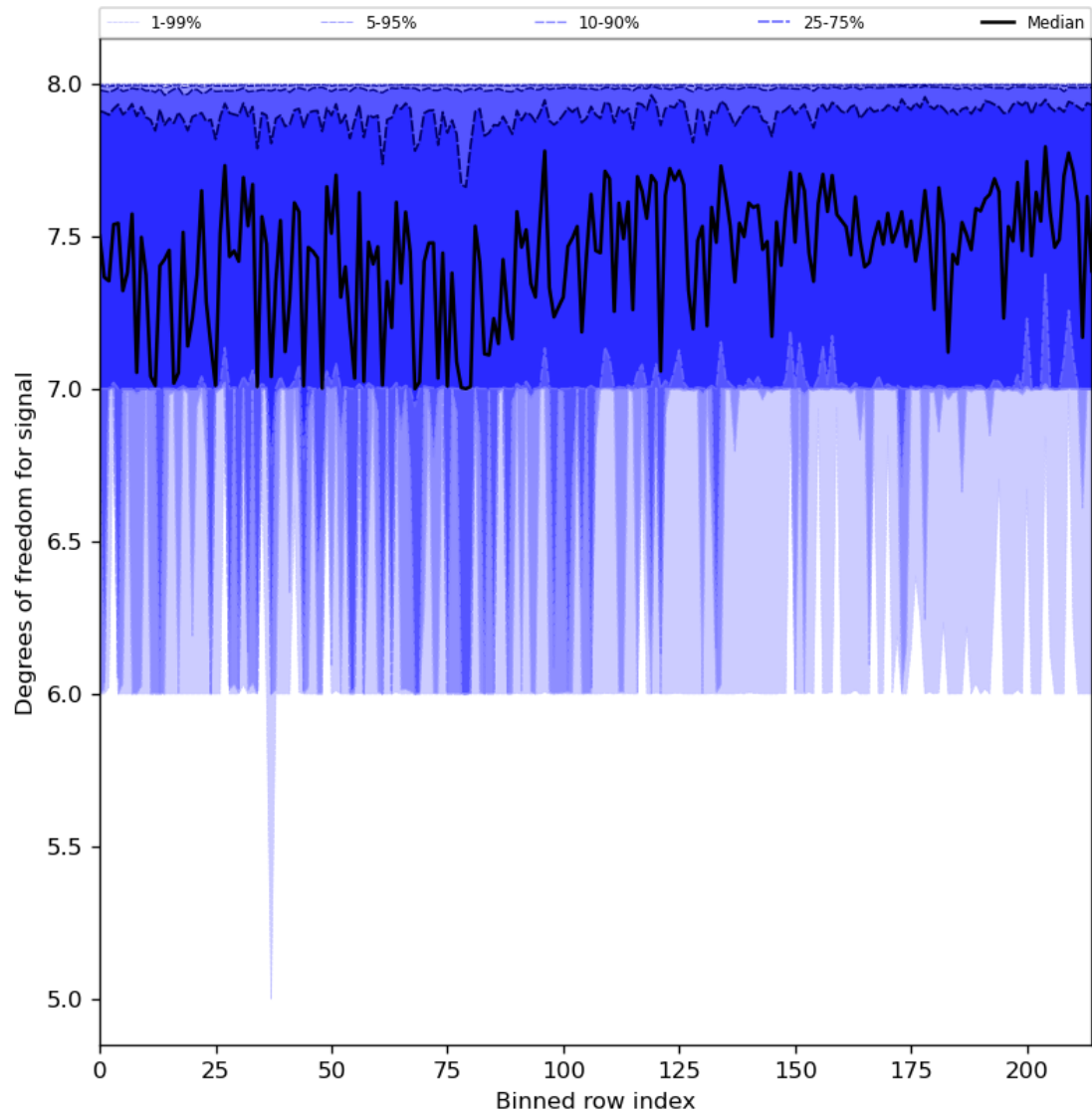
Figure 31: Along track statistics of “Degrees of freedom for signal” for 2024-01-26 to 2024-01-27
