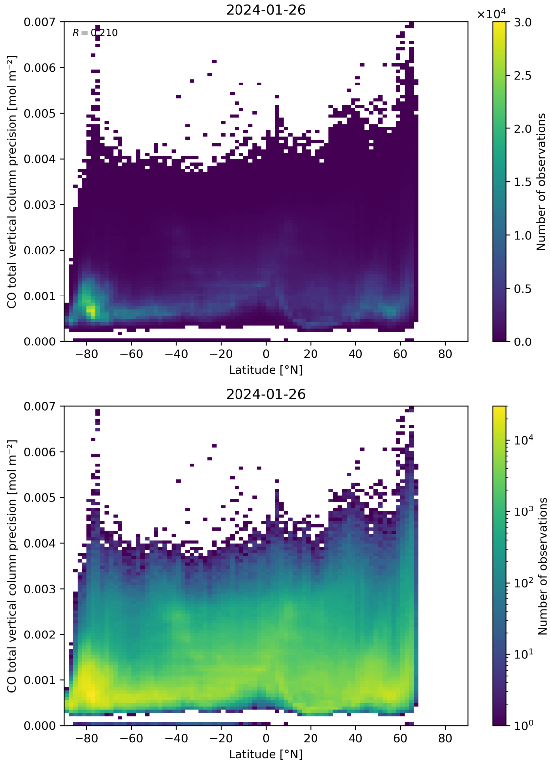
Figure 53: Scatter density plot of “Latitude” against “CO total vertical column precision” for 2024-01-26 to 2024-01-27.
