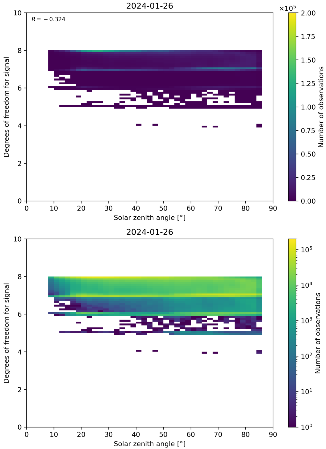
Figure 65: Scatter density plot of “Solar zenith angle” against “Degrees of freedom for signal” for 2024-01-26 to 2024-01-27.
