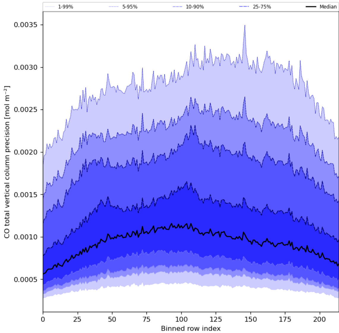
Figure 28: Along track statistics of “CO total vertical column precision” for 2024-01-26 to 2024-01-27
