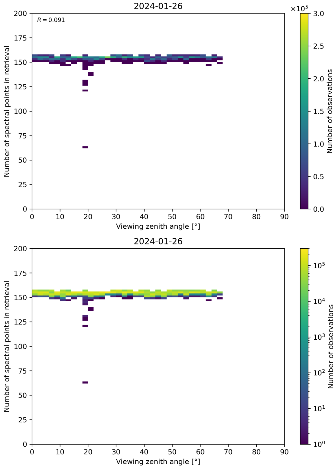
Figure 76: Scatter density plot of “Viewing zenith angle” against “Number of spectral points in retrieval” for 2024-01-26 to 2024-01-27.
