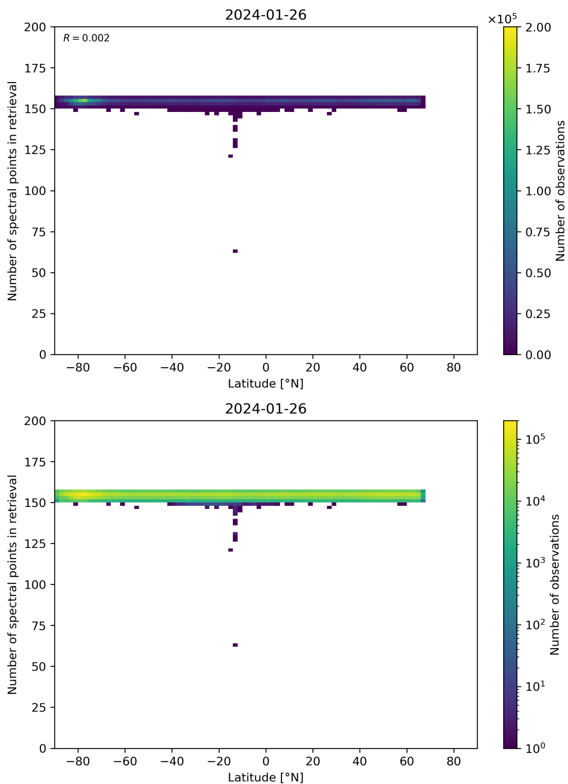
Figure 57: Scatter density plot of “Latitude” against “Number of spectral points in retrieval” for 2024-01-26 to 2024-01-27.
