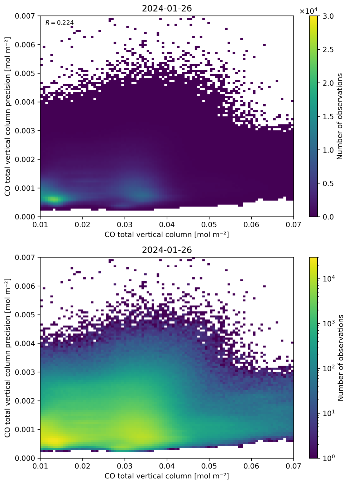
Figure 34: Scatter density plot of “CO total vertical column” against “CO total vertical column precision” for 2024-01-26 to 2024-01-27.
