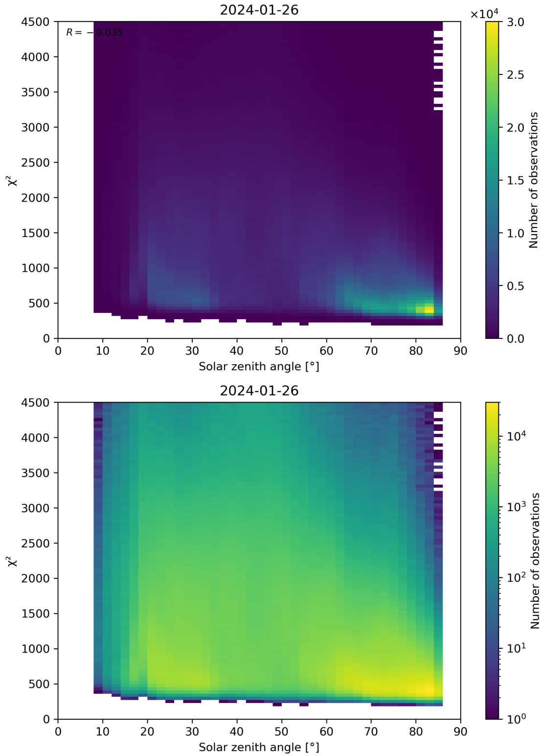
Figure 64: Scatter density plot of “Solar zenith angle” against “ \chi^2 ” for 2024-01-26 to 2024-01-27.
