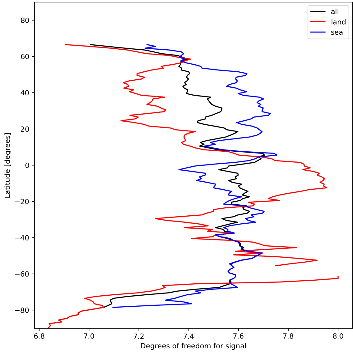
Figure 15: Zonal average of “Degrees of freedom for signal” for 2024-01-26 to 2024-01-27.
