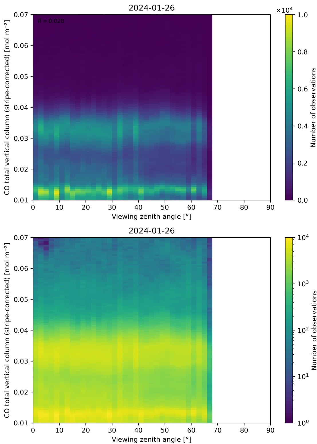
Figure 70: Scatter density plot of “Viewing zenith angle” against “CO total vertical column (stripe-corrected)” for 2024-01-26 to 2024-01-27.
