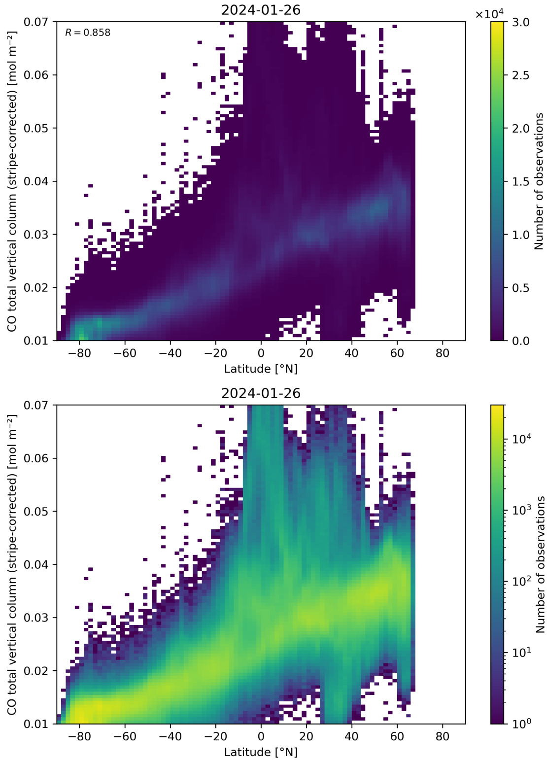
Figure 52: Scatter density plot of “Latitude” against “CO total vertical column (stripe-corrected)” for 2024-01-26 to 2024-01-27.
