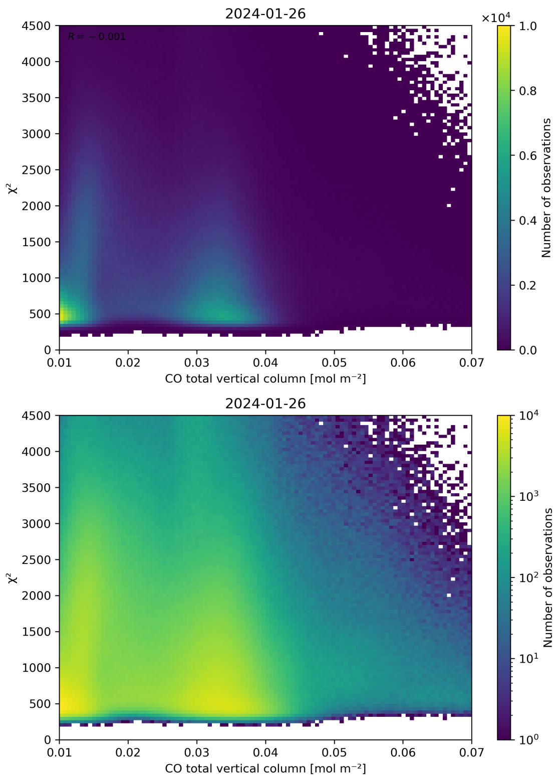
Figure 35: Scatter density plot of “CO total vertical column” against “ \chi^2 ” for 2024-01-26 to 2024-01-27.
