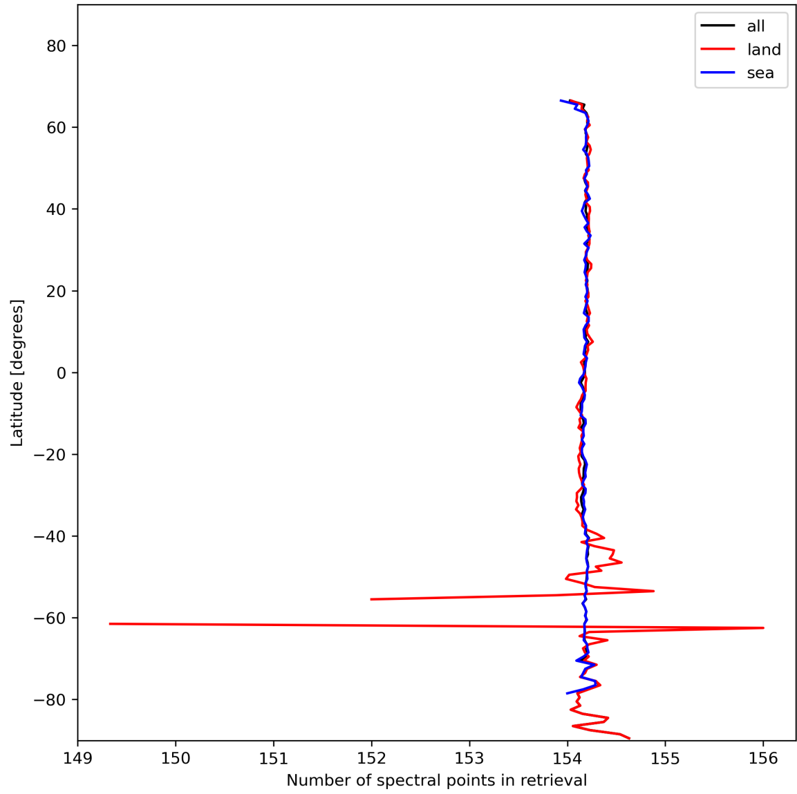
Figure 13: Zonal average of “Number of spectral points in retrieval” for 2024-01-26 to 2024-01-27.
