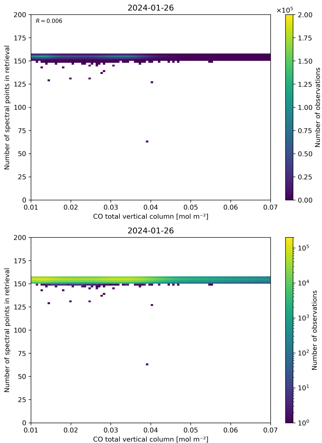
Figure 43: Scatter density plot of “CO total vertical column” against “Number of spectral points in retrieval” for 2024-01-26 to 2024-01-27.
