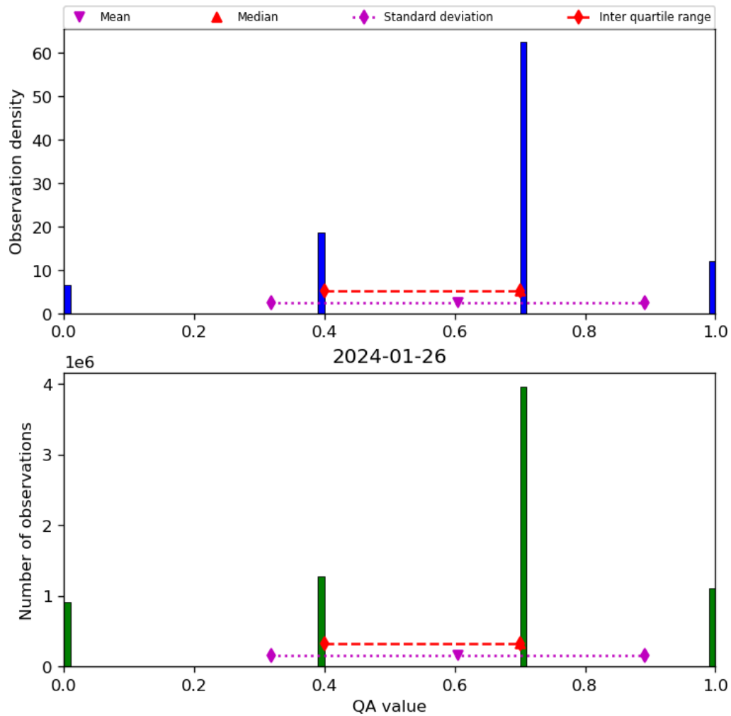
Figure 17: Histogram of “QA value” for 2024-01-26 to 2024-01-27
