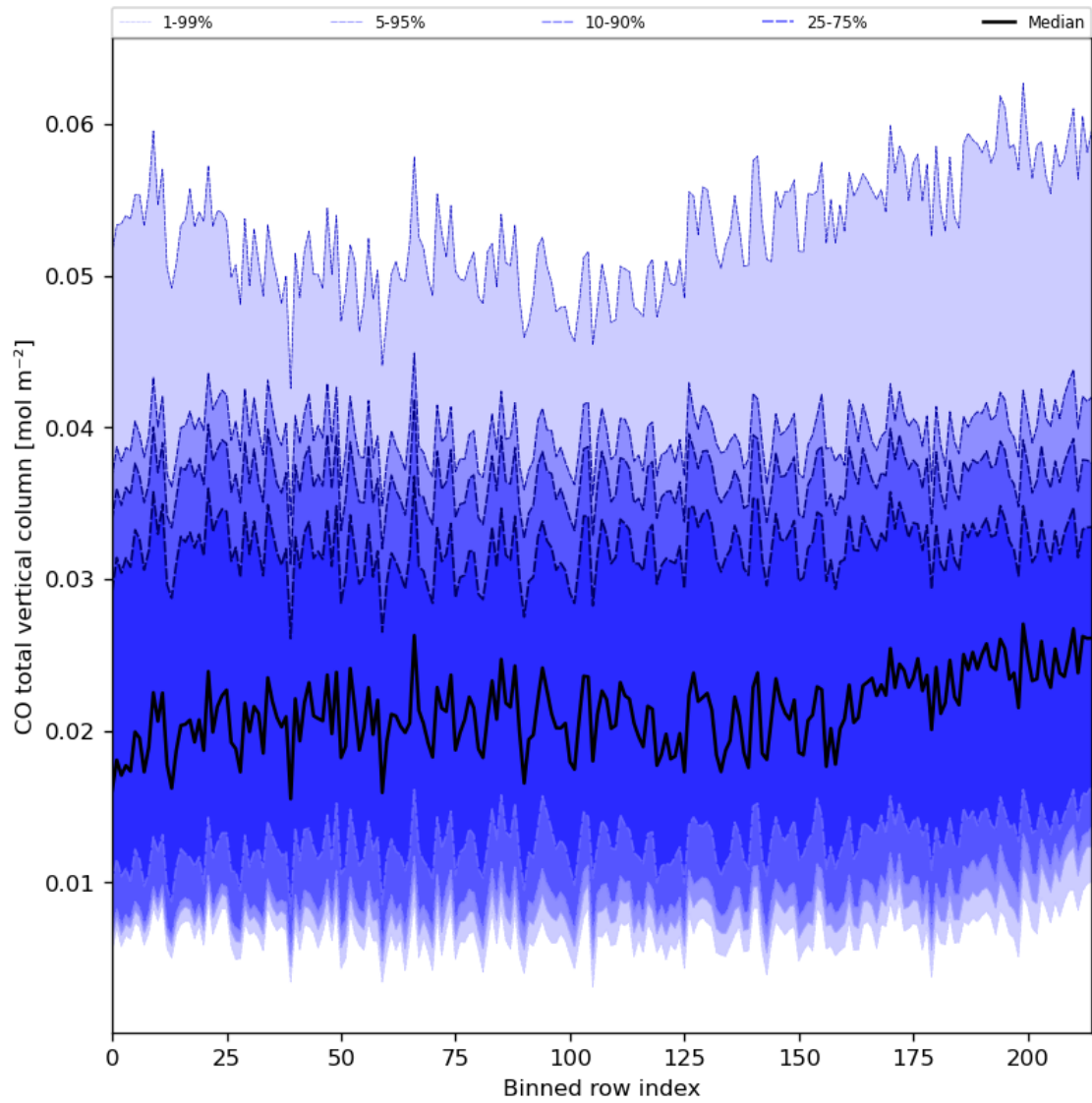
Figure 26: Along track statistics of “CO total vertical column” for 2024-01-26 to 2024-01-27
