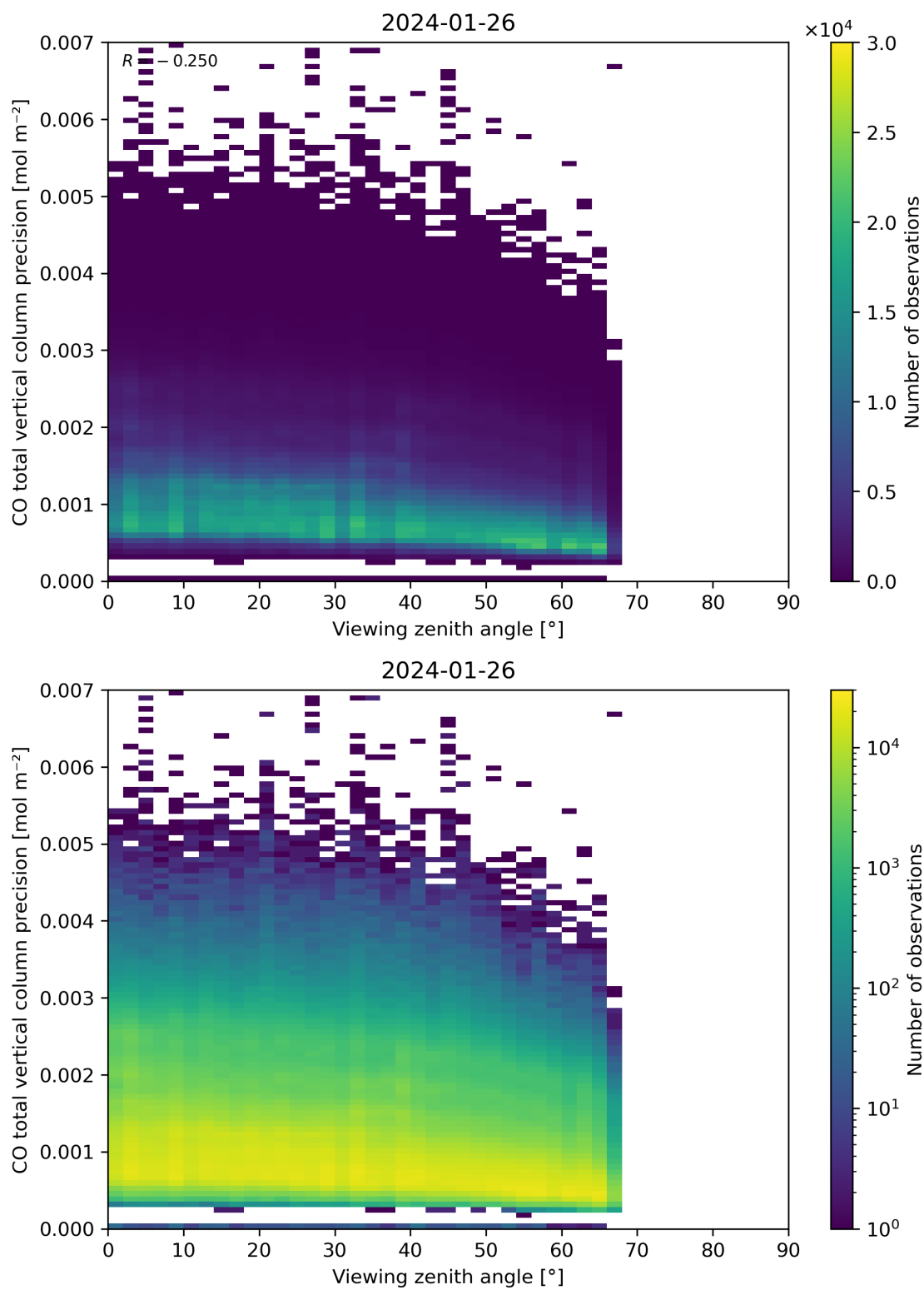
Figure 71: Scatter density plot of “Viewing zenith angle” against “CO total vertical column precision” for 2024-01-26 to 2024-01-27.
