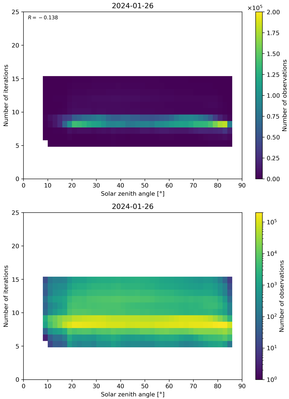
Figure 67: Scatter density plot of “Solar zenith angle” against “Number of iterations” for 2024-01-26 to 2024-01-27.
