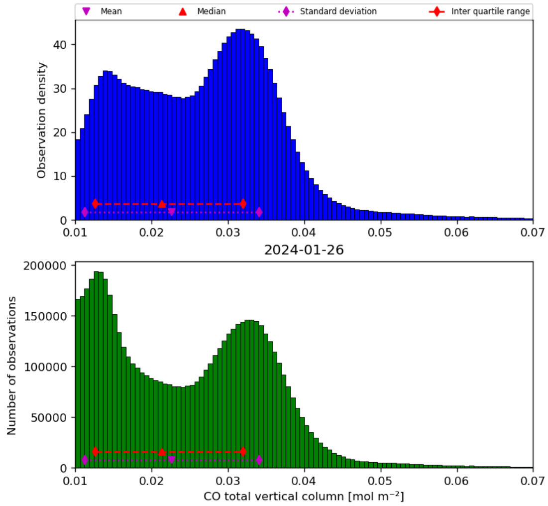
Figure 18: Histogram of “CO total vertical column” for 2024-01-26 to 2024-01-27
