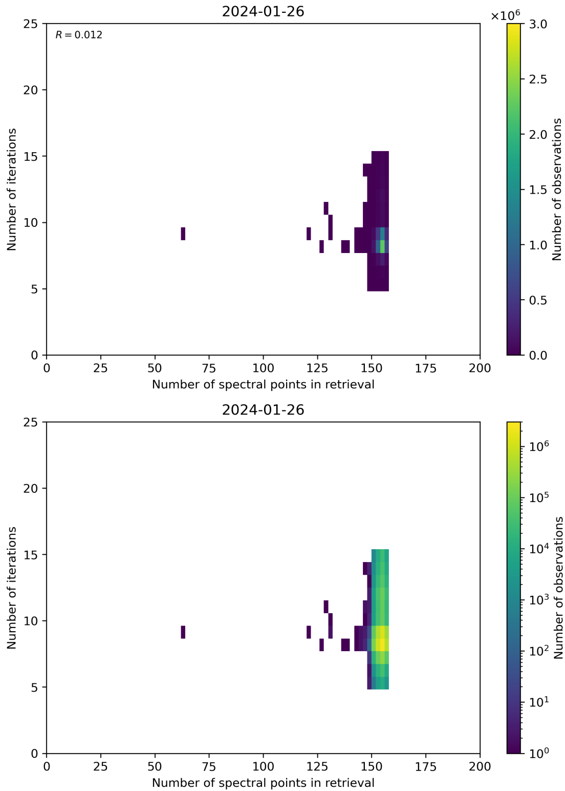
Figure 60: Scatter density plot of “Number of spectral points in retrieval” against “Number of iterations” for 2024-01-26 to 2024-01-27.
