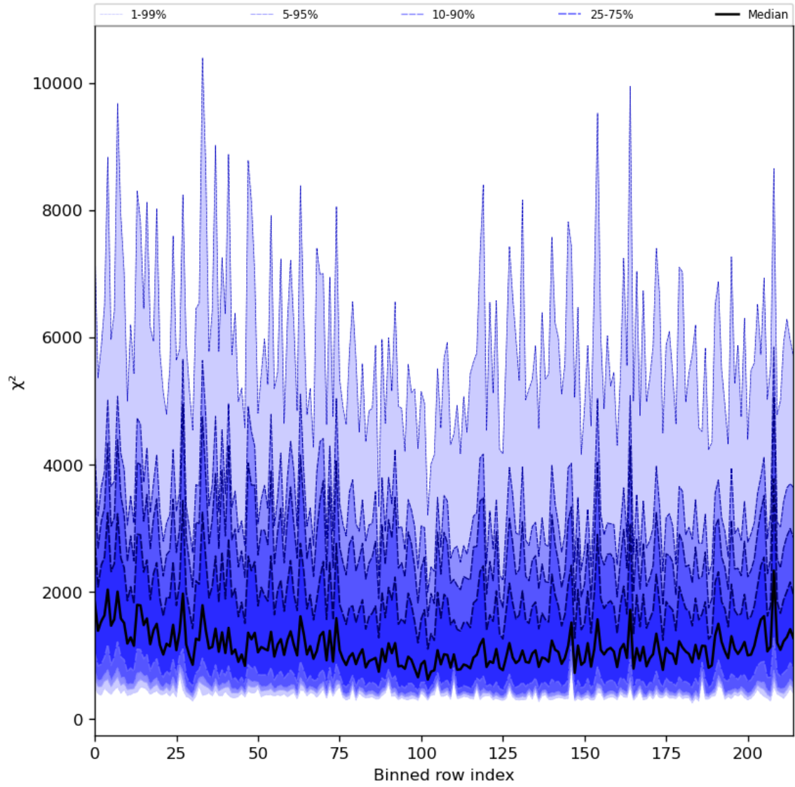
Figure 30: Along track statistics of “ \chi^2 ” for 2024-01-26 to 2024-01-27
