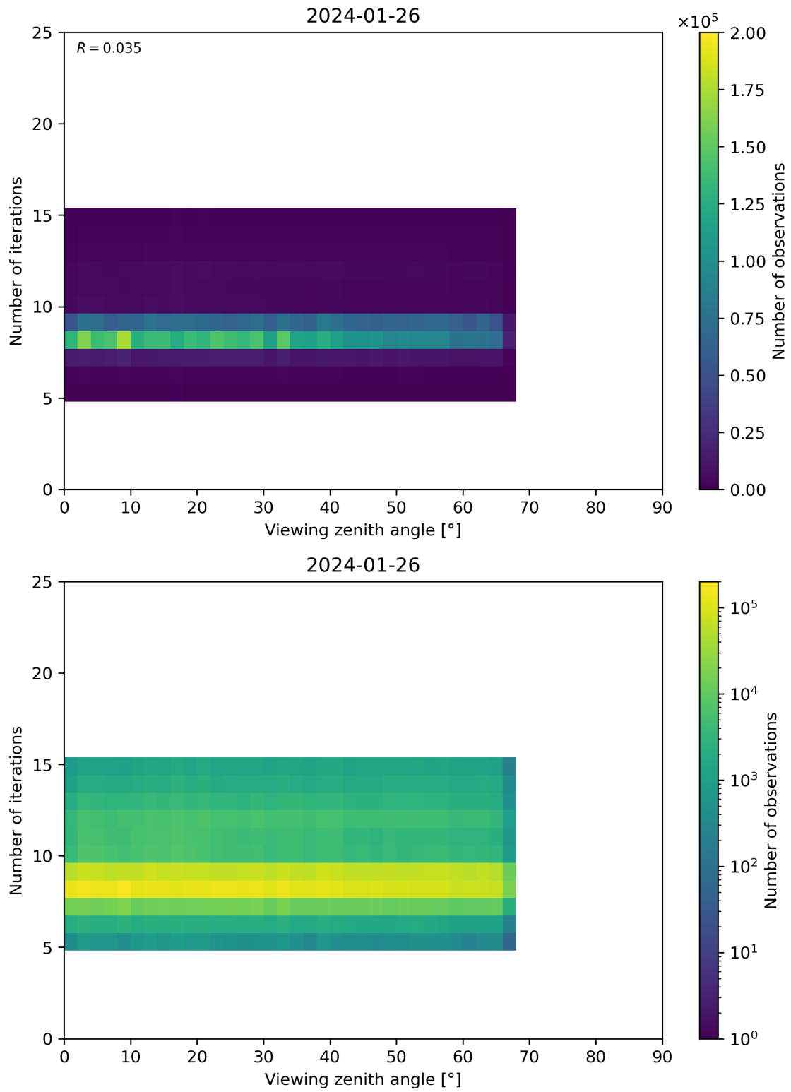
Figure 75: Scatter density plot of “Viewing zenith angle” against “Number of iterations” for 2024-01-26 to 2024-01-27.
