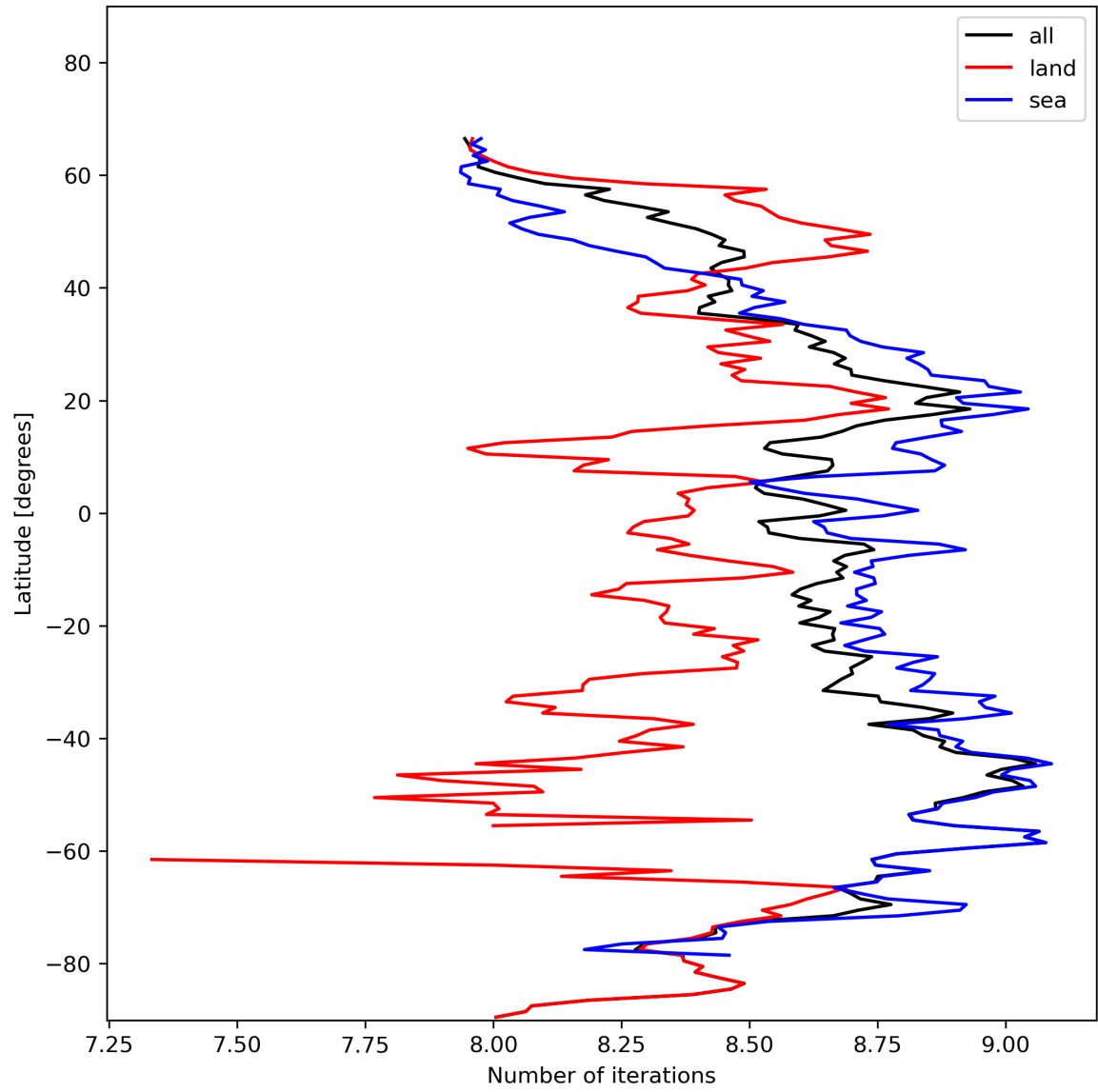
Figure 16: Zonal average of “Number of iterations” for 2024-01-26 to 2024-01-27.
