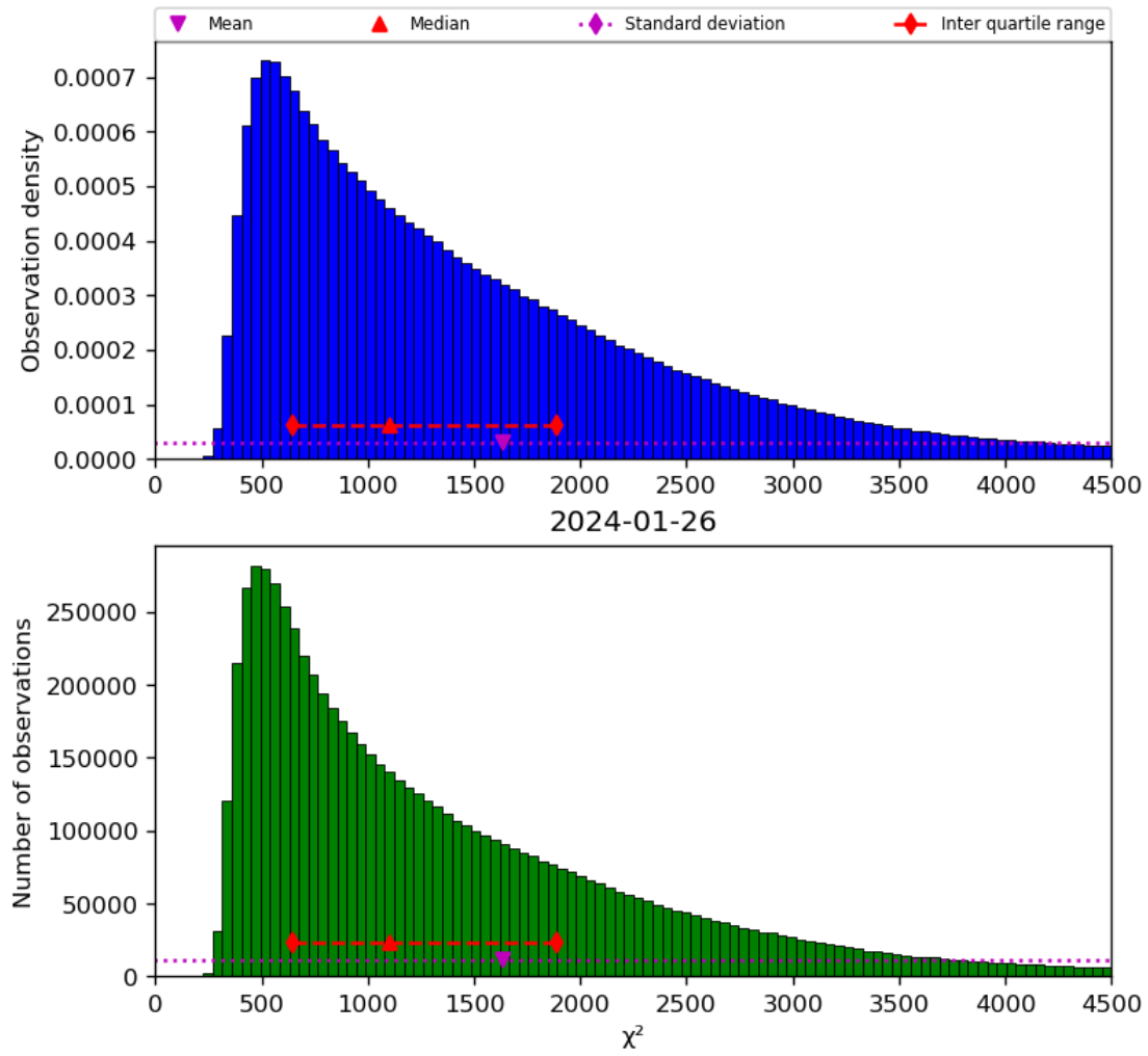
Figure 22: Histogram of “ \chi^2 ” for 2024-01-26 to 2024-01-27
