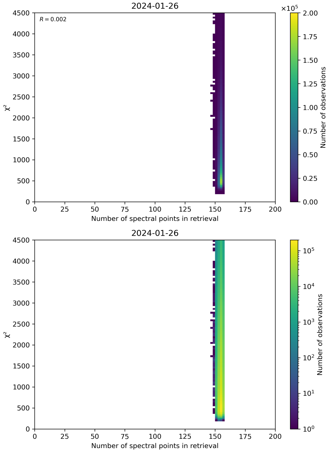
Figure 58: Scatter density plot of “Number of spectral points in retrieval” against “ \chi^2 ” for 2024-01-26 to 2024-01-27.
