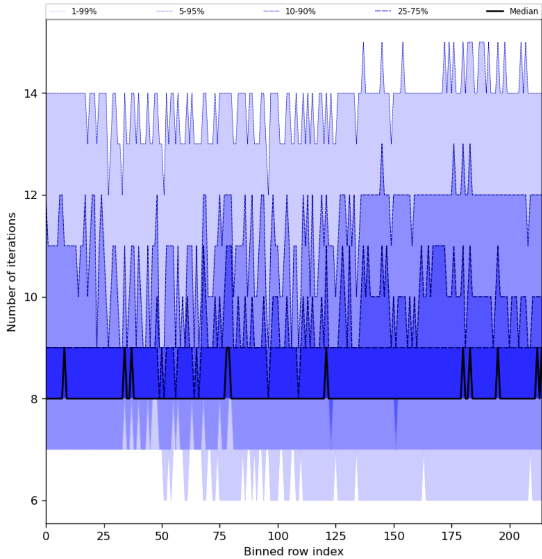
Figure 32: Along track statistics of “Number of iterations” for 2024-01-26 to 2024-01-27
