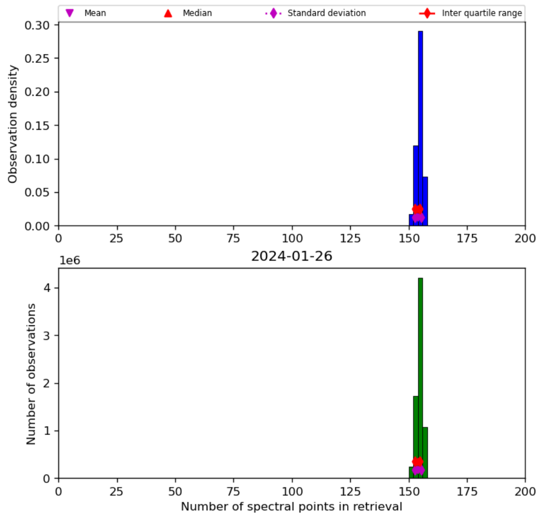
Figure 21: Histogram of “Number of spectral points in retrieval” for 2024-01-26 to 2024-01-27
