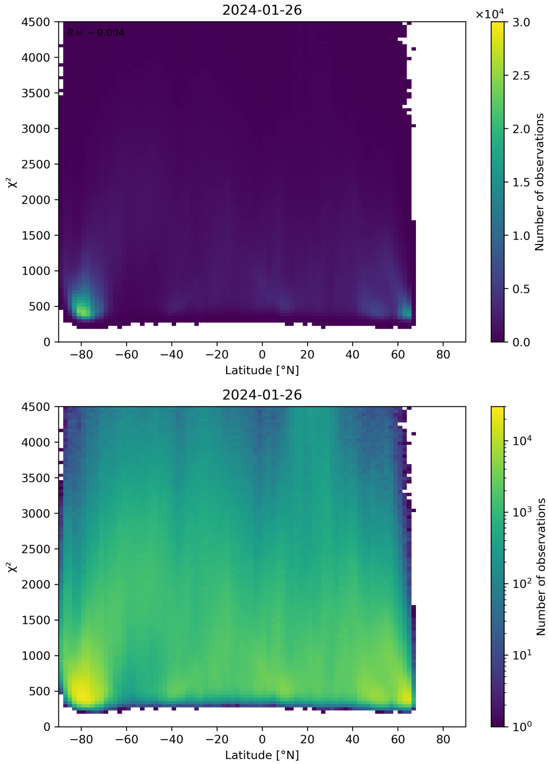
Figure 54: Scatter density plot of “Latitude” against “ \chi^2 ” for 2024-01-26 to 2024-01-27.
