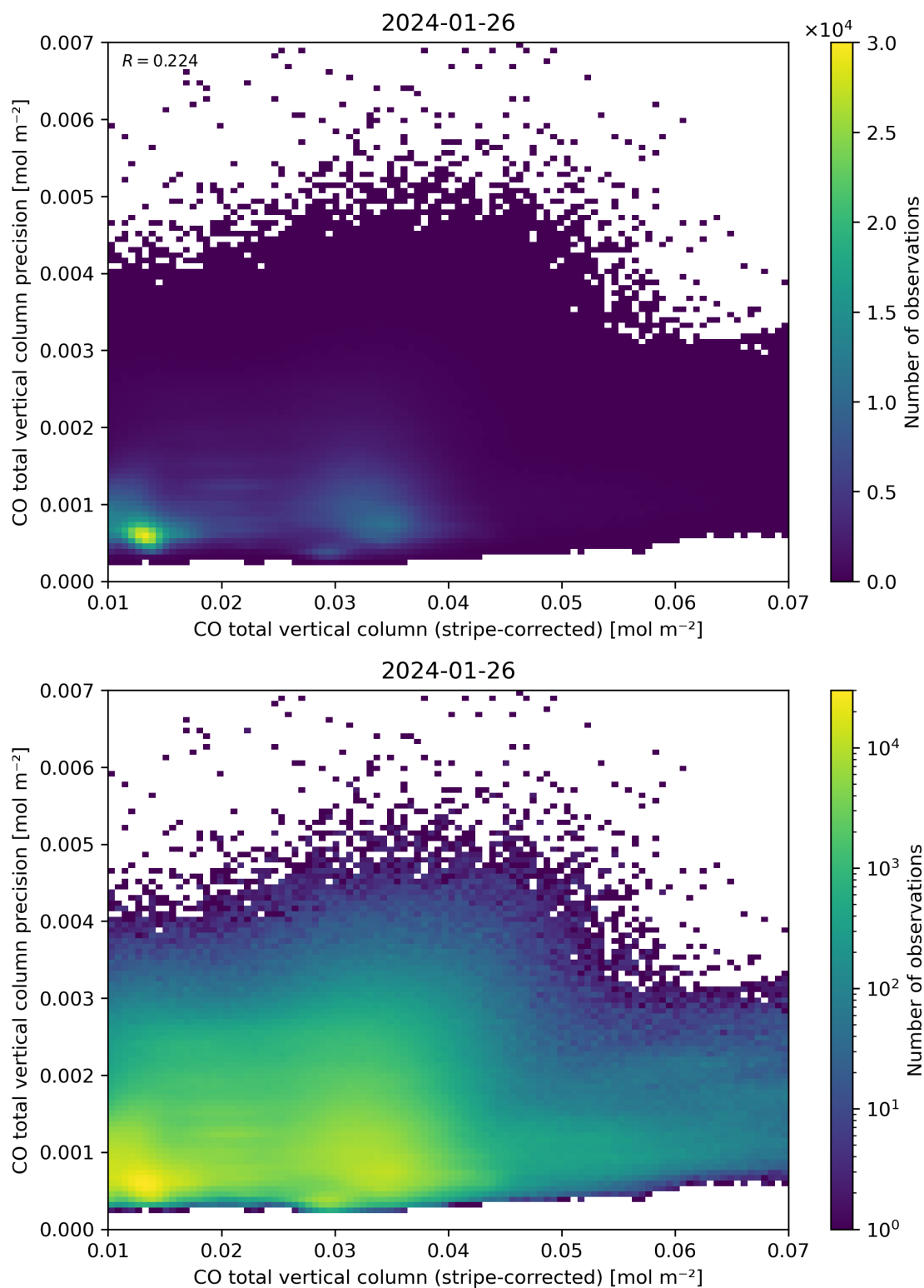
Figure 36: Scatter density plot of “CO total vertical column (stripe-corrected)” against “CO total vertical column precision” for 2024-01-26 to 2024-01-27.
