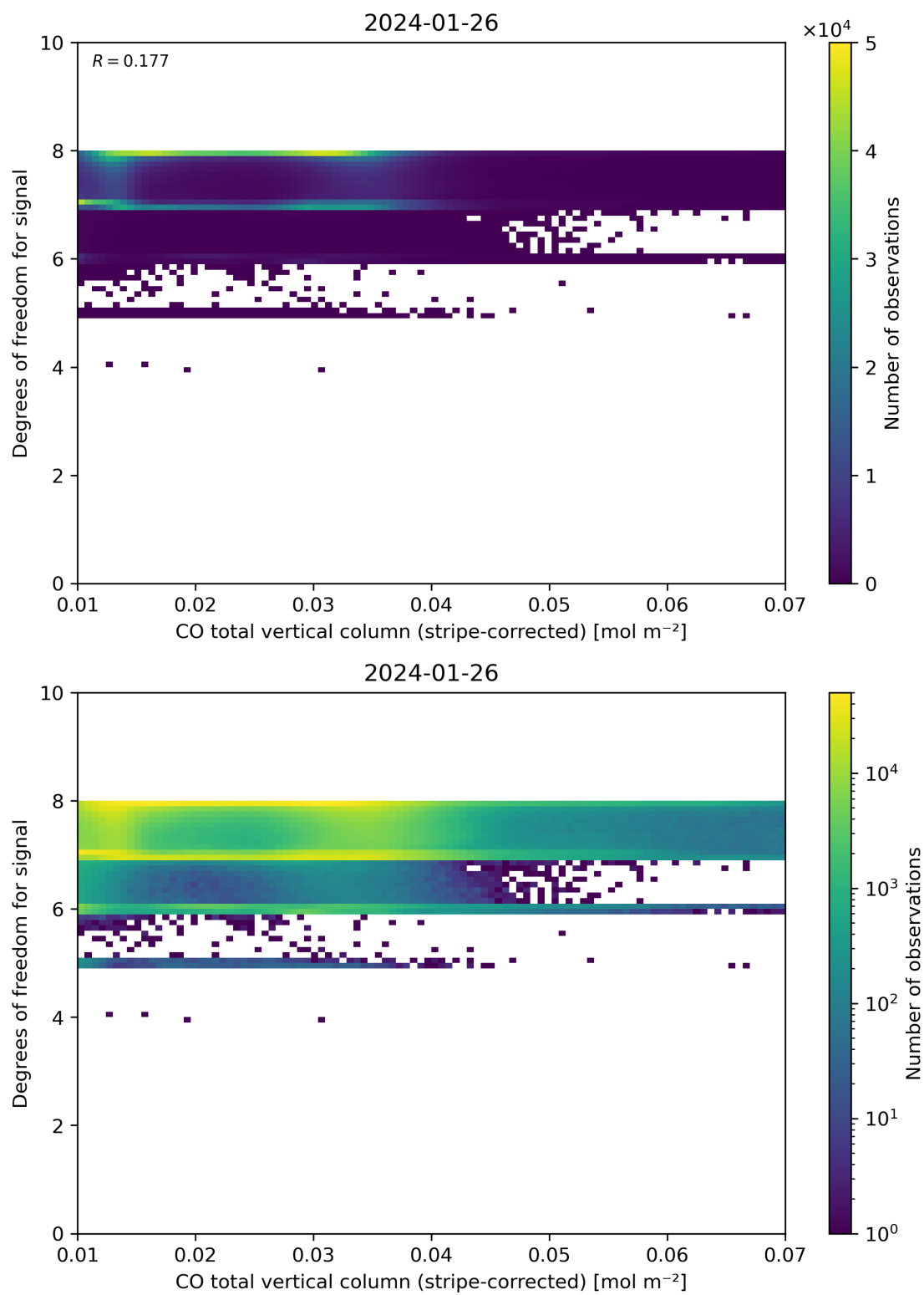
Figure 38: Scatter density plot of “CO total vertical column (stripe-corrected)” against “Degrees of freedom for signal” for 2024-01-26 to 2024-01-27.
