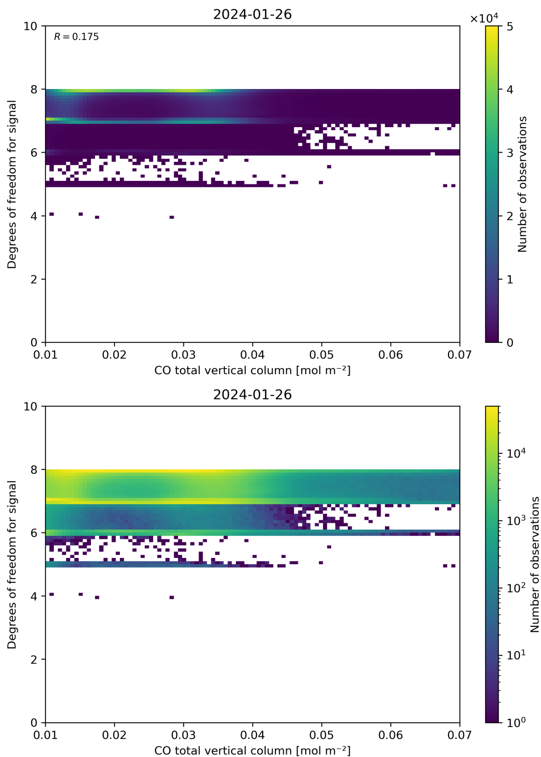
Figure 41: Scatter density plot of “CO total vertical column” against “Degrees of freedom for signal” for 2024-01-26 to 2024-01-27.
