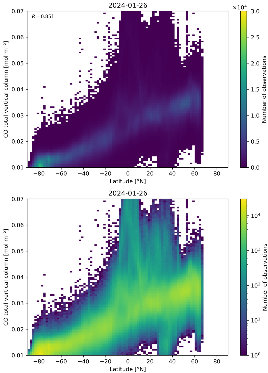
Figure 51: Scatter density plot of “Latitude” against “CO total vertical column” for 2024-01-26 to 2024-01-27.
