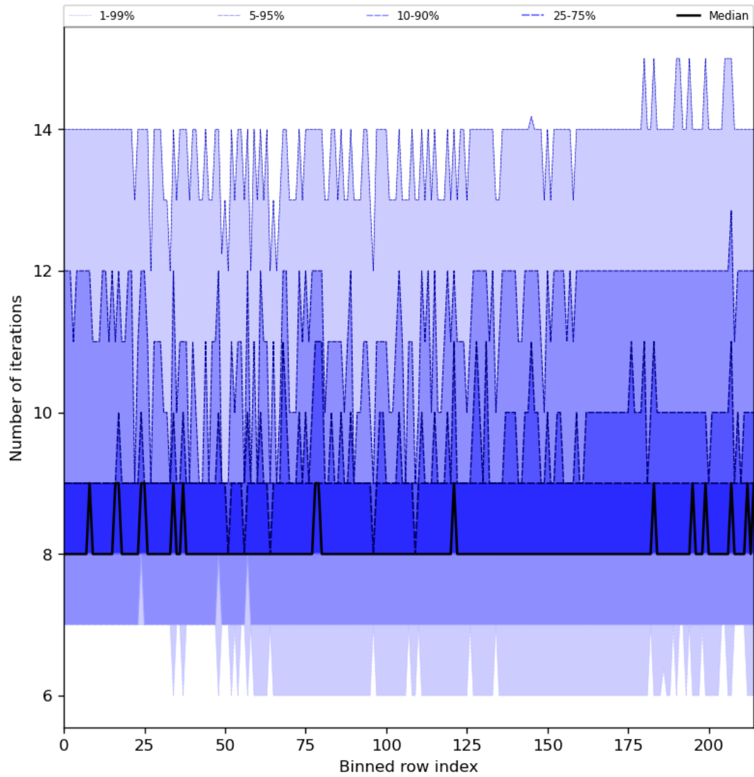
Figure 32: Along track statistics of “Number of iterations” for 2024-01-28 to 2024-01-30
