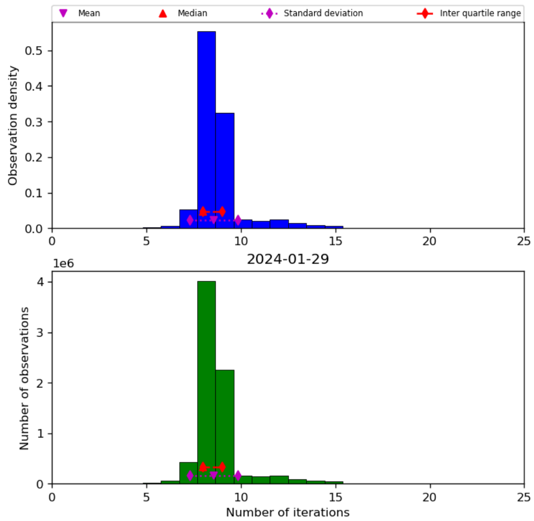
Figure 24: Histogram of “Number of iterations” for 2024-01-28 to 2024-01-30
