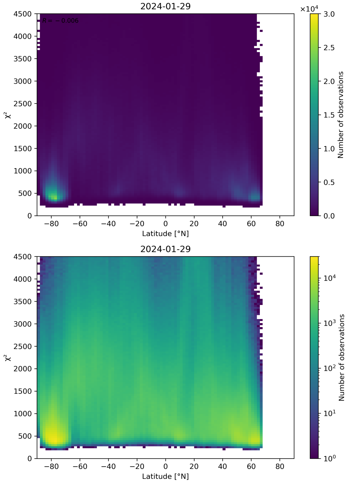
Figure 54: Scatter density plot of “Latitude” against “ \chi^2 ” for 2024-01-28 to 2024-01-30.
