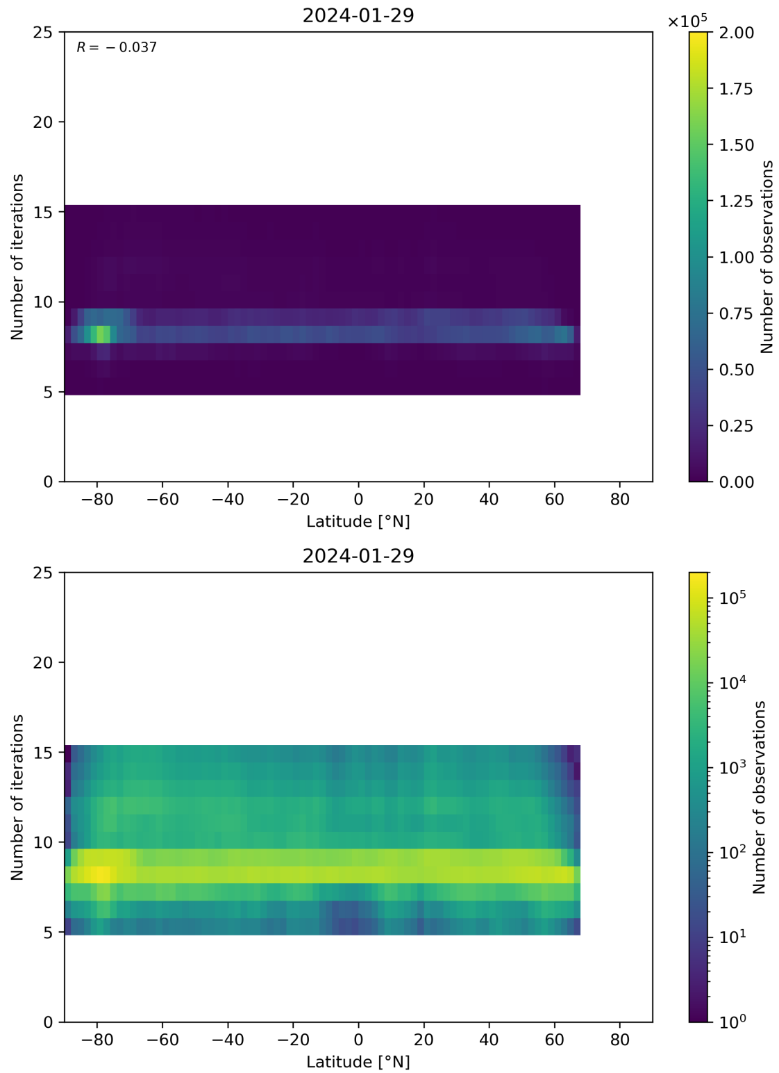
Figure 56: Scatter density plot of “Latitude” against “Number of iterations” for 2024-01-28 to 2024-01-30.
