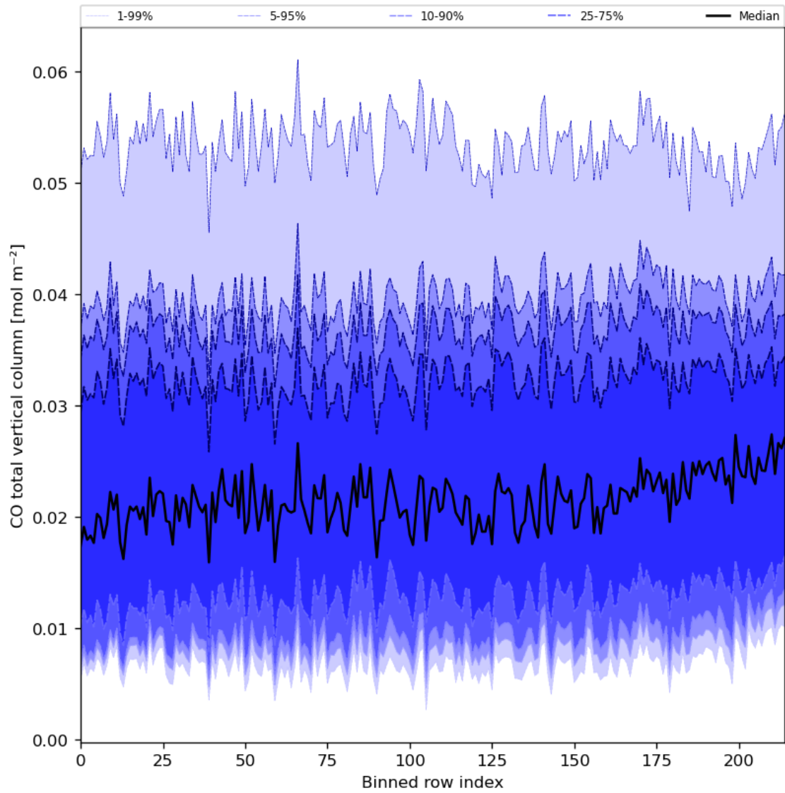
Figure 26: Along track statistics of “CO total vertical column” for 2024-01-28 to 2024-01-30
