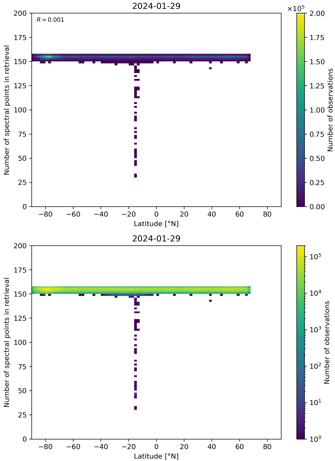
Figure 57: Scatter density plot of “Latitude” against “Number of spectral points in retrieval” for 2024-01-28 to 2024-01-30.
