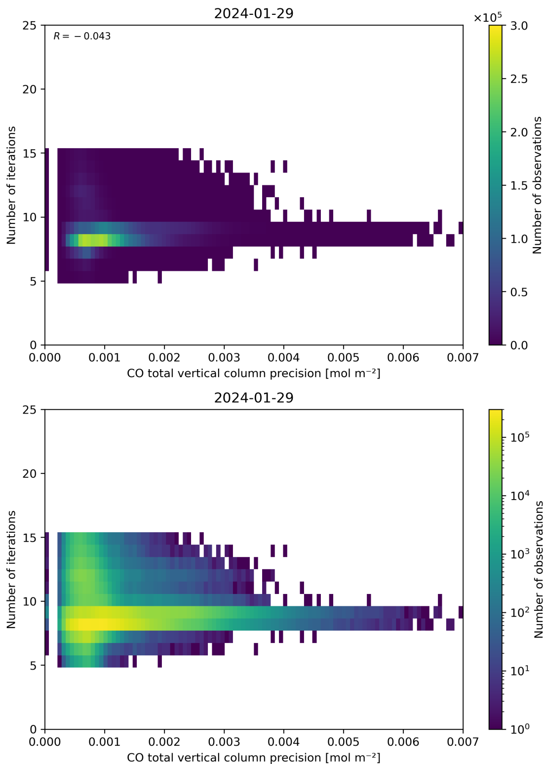
Figure 46: Scatter density plot of “CO total vertical column precision” against “Number of iterations” for 2024-01-28 to 2024-01-30.
