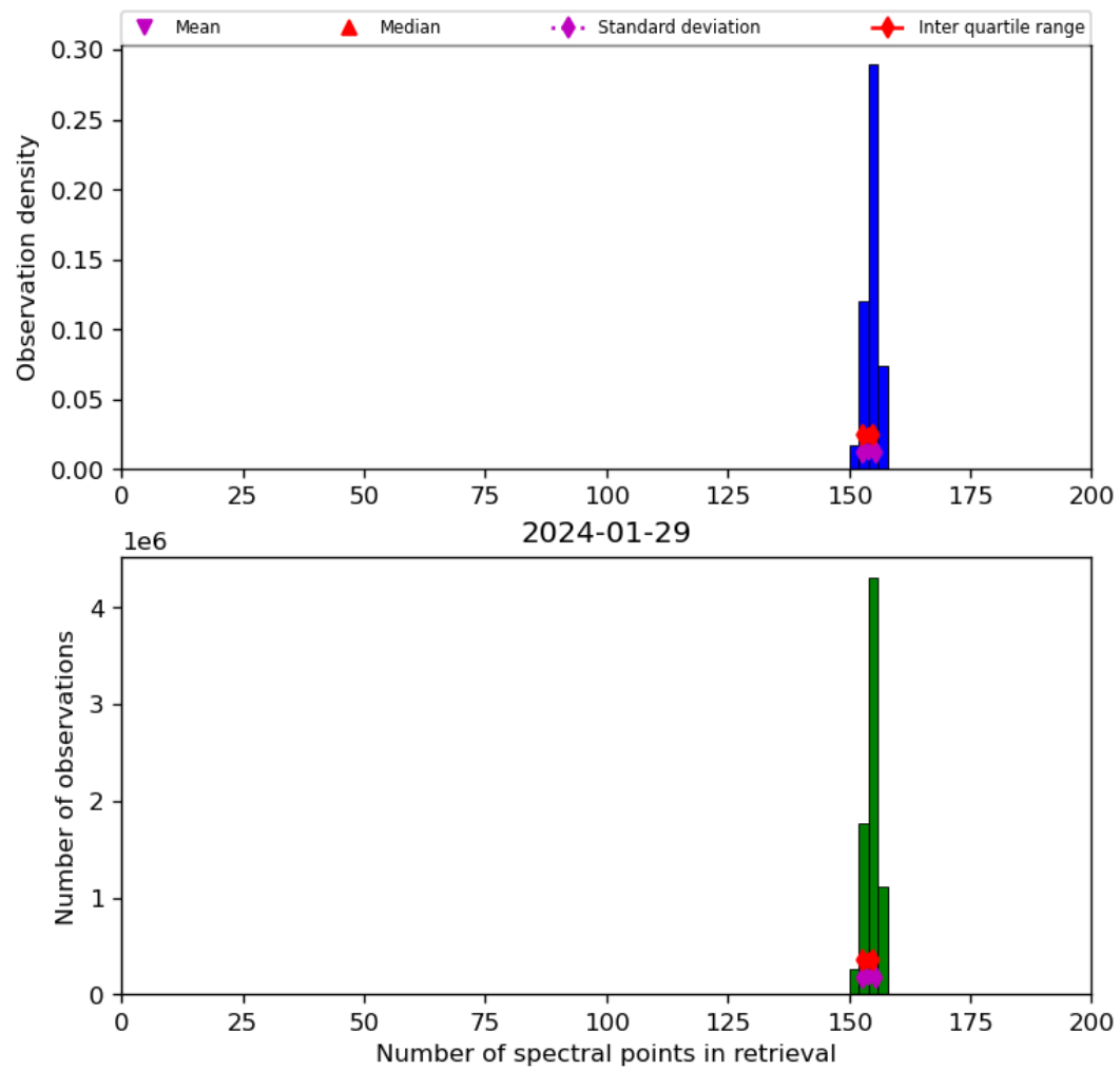
Figure 21: Histogram of “Number of spectral points in retrieval” for 2024-01-28 to 2024-01-30
