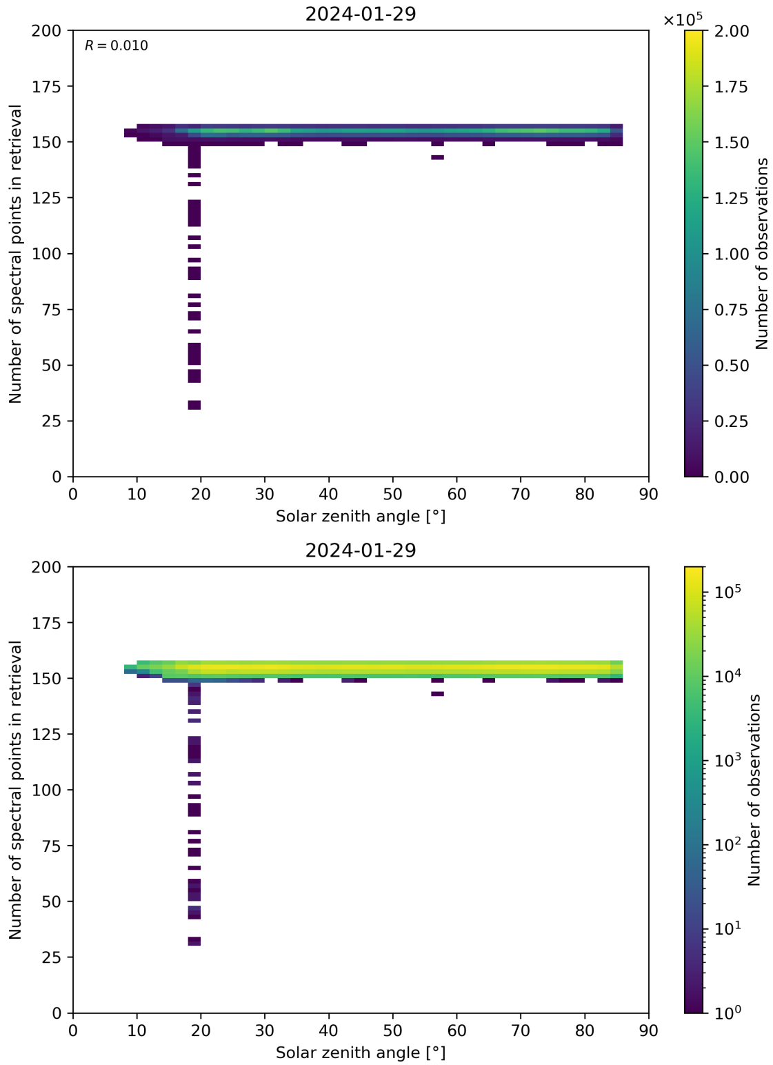
Figure 68: Scatter density plot of “Solar zenith angle” against “Number of spectral points in retrieval” for 2024-01-28 to 2024-01-30.
