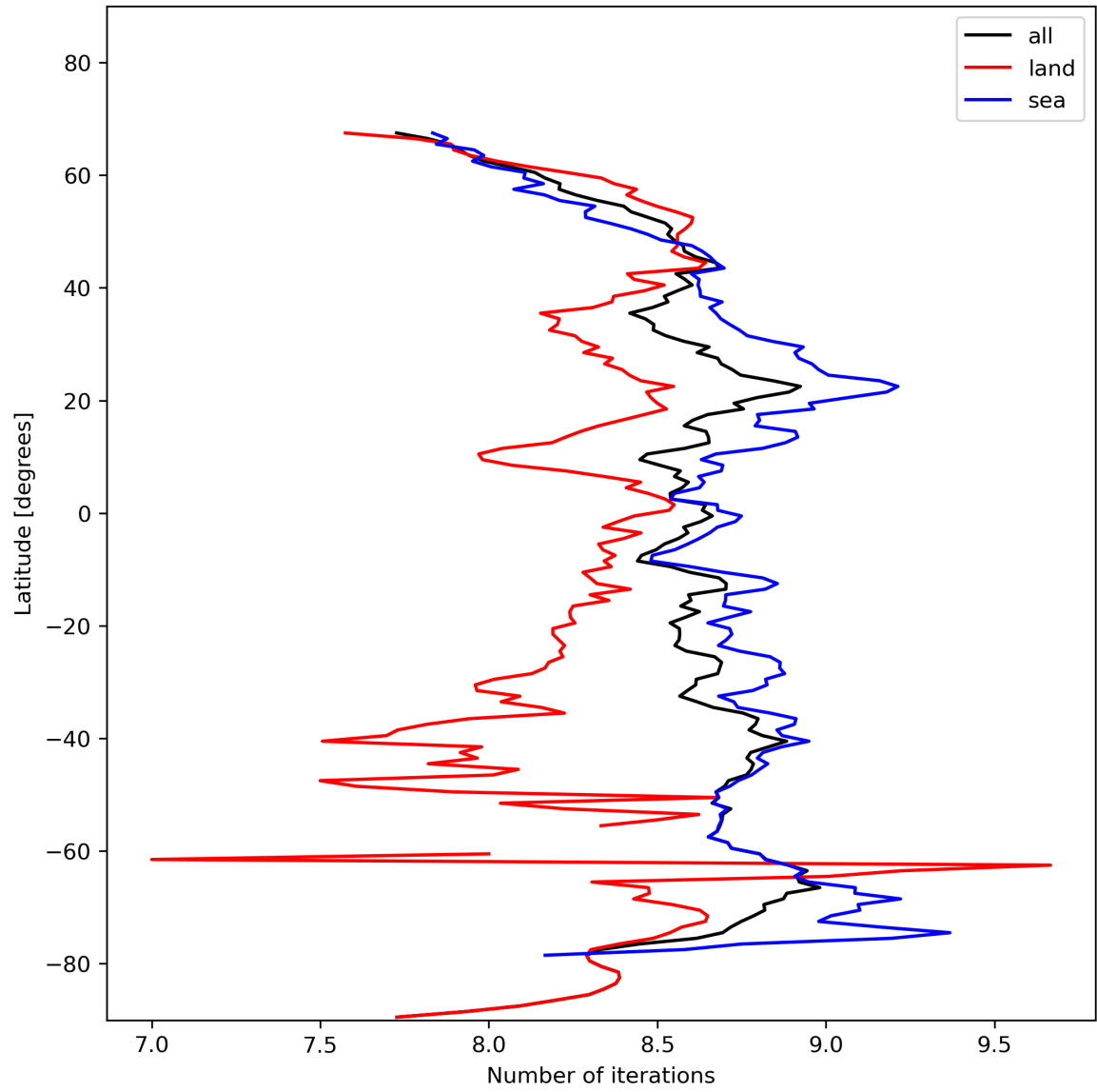
Figure 16: Zonal average of “Number of iterations” for 2024-01-28 to 2024-01-30.
