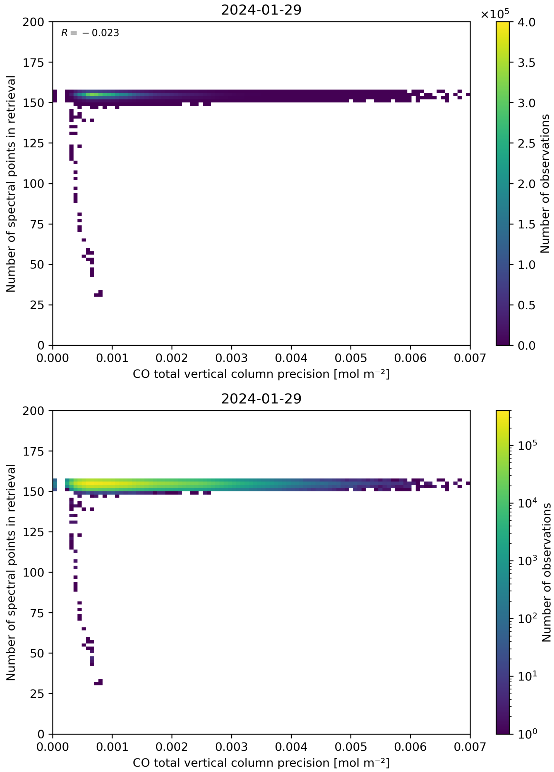
Figure 47: Scatter density plot of “CO total vertical column precision” against “Number of spectral points in retrieval” for 2024-01-28 to 2024-01-30.
