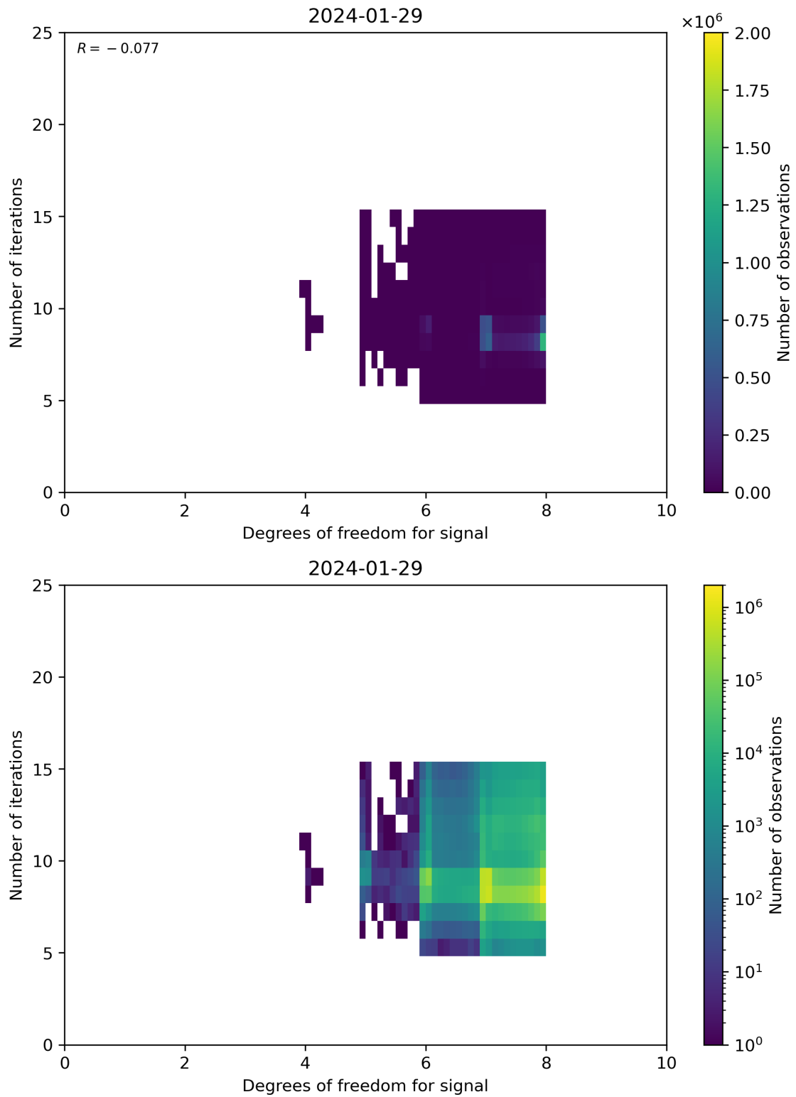
Figure 50: Scatter density plot of “Degrees of freedom for signal” against “Number of iterations” for 2024-01-28 to 2024-01-30.
