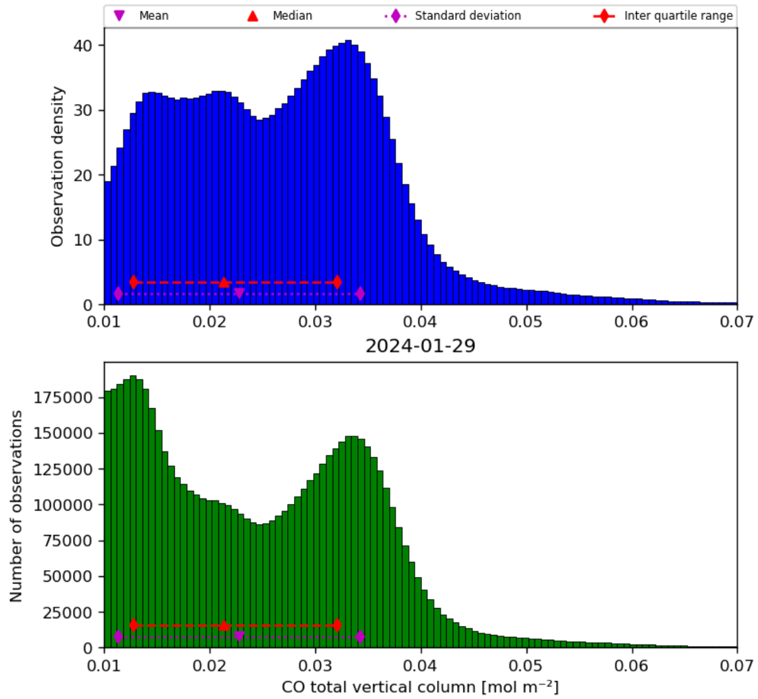
Figure 18: Histogram of “CO total vertical column” for 2024-01-28 to 2024-01-30
