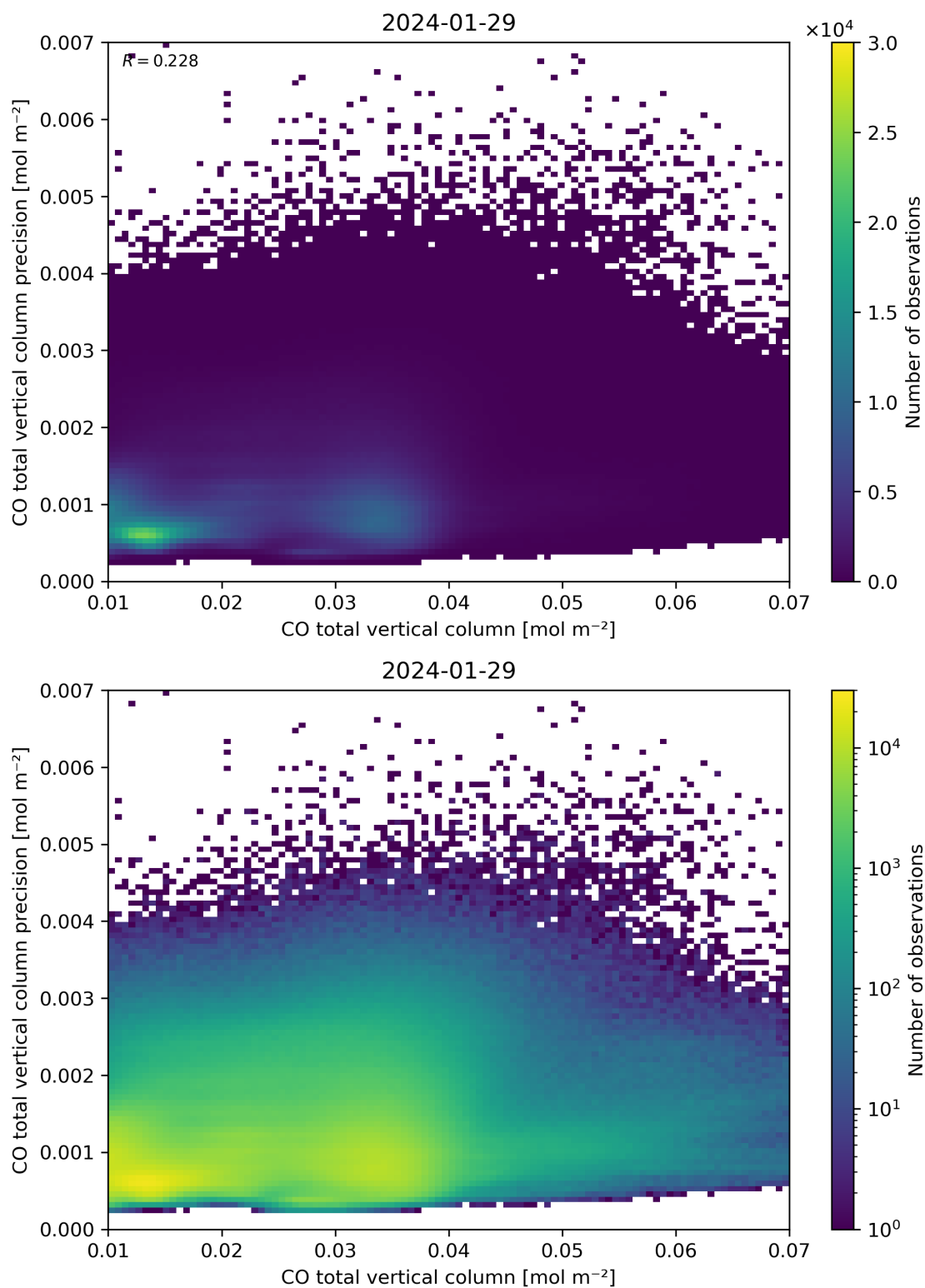
Figure 34: Scatter density plot of “CO total vertical column” against “CO total vertical column precision” for 2024-01-28 to 2024-01-30.
