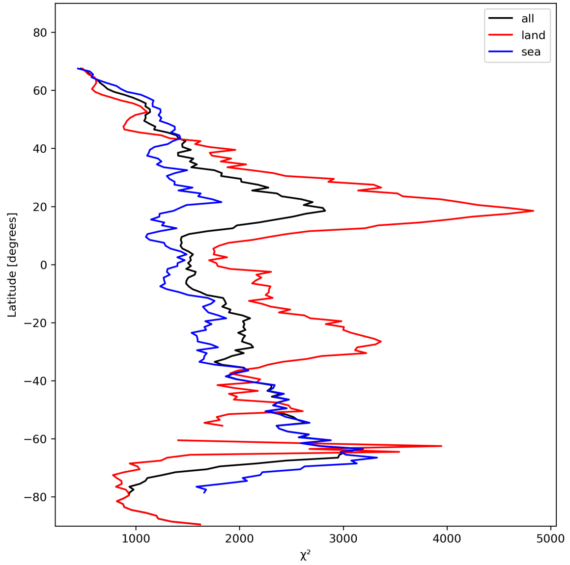
Figure 14: Zonal average of “ \chi^2 ” for 2024-01-28 to 2024-01-30.
