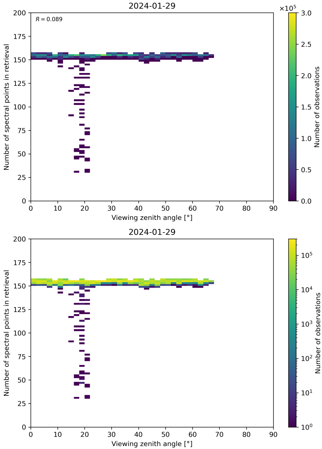
Figure 76: Scatter density plot of “Viewing zenith angle” against “Number of spectral points in retrieval” for 2024-01-28 to 2024-01-30.
