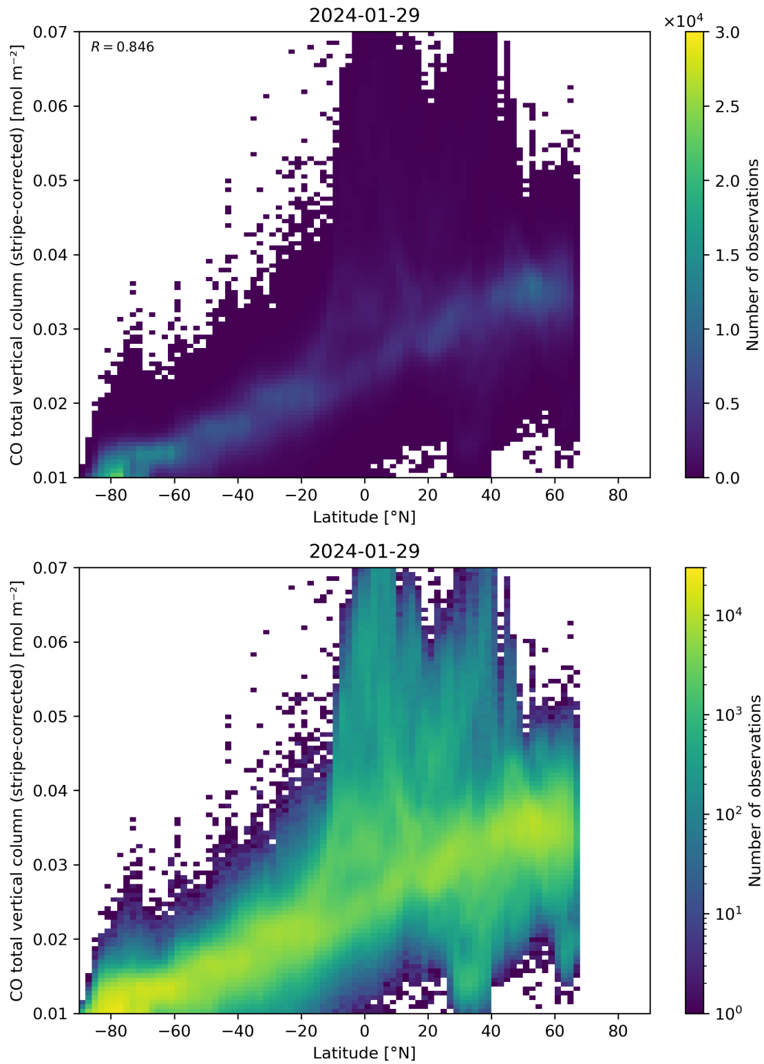
Figure 52: Scatter density plot of “Latitude” against “CO total vertical column (stripe-corrected)” for 2024-01-28 to 2024-01-30.
