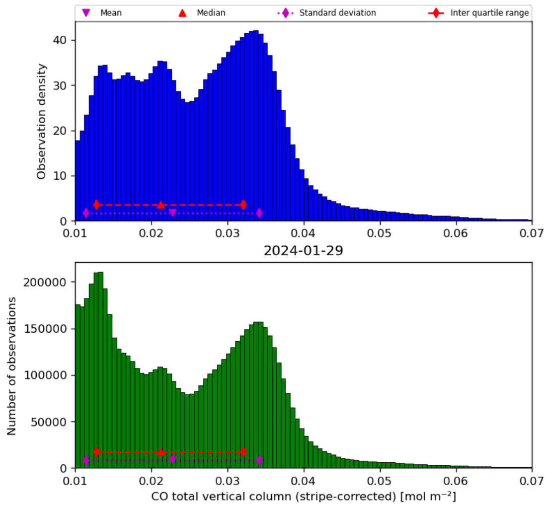
Figure 19: Histogram of “CO total vertical column (stripe-corrected)” for 2024-01-28 to 2024-01-30
