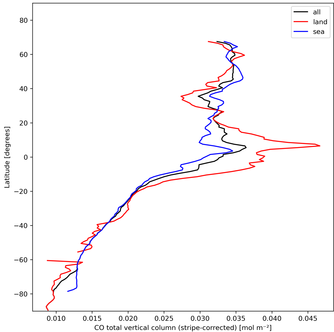
Figure 11: Zonal average of “CO total vertical column (stripe-corrected)” for 2024-01-28 to 2024-01-30.
