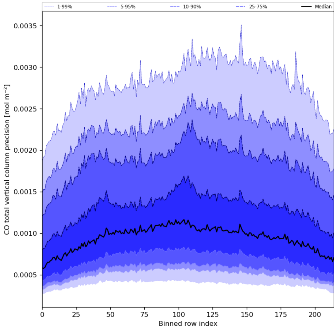
Figure 28: Along track statistics of “CO total vertical column precision” for 2024-01-28 to 2024-01-30
