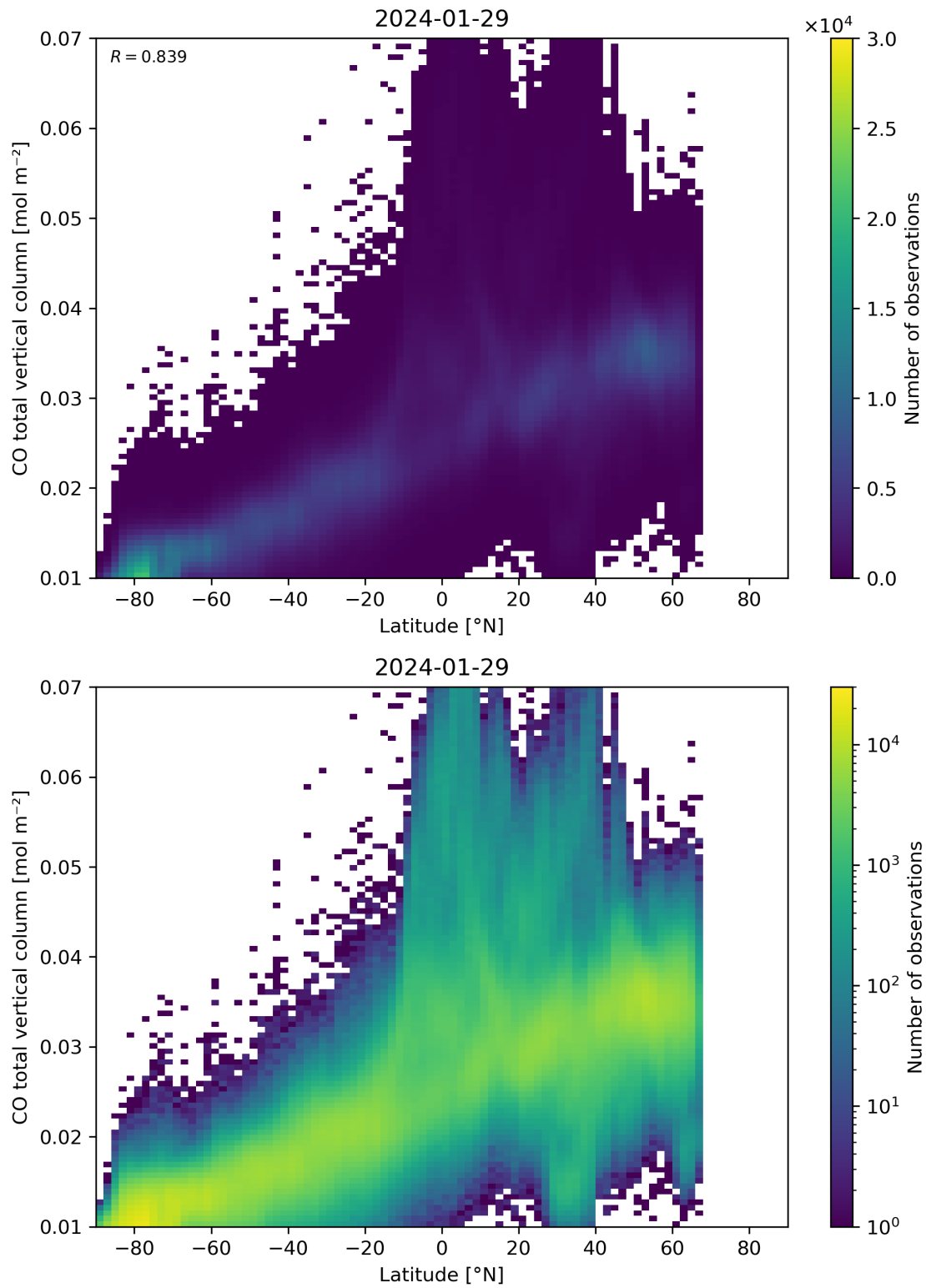
Figure 51: Scatter density plot of “Latitude” against “CO total vertical column” for 2024-01-28 to 2024-01-30.
