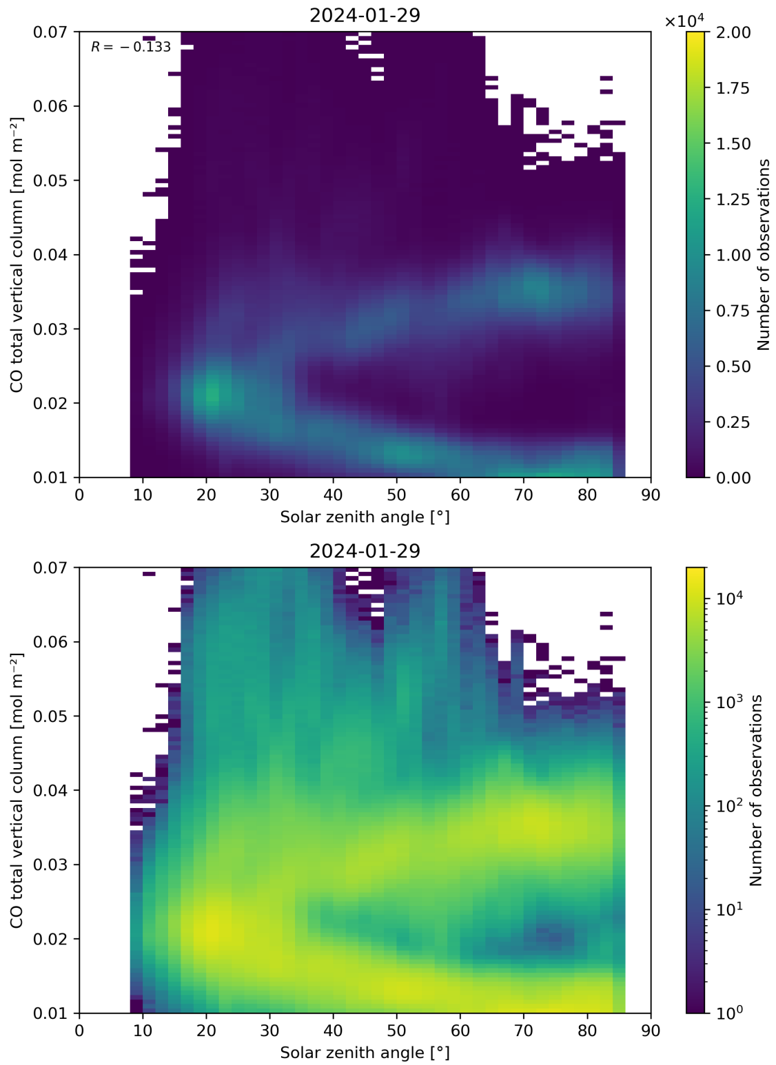
Figure 61: Scatter density plot of “Solar zenith angle” against “CO total vertical column” for 2024-01-28 to 2024-01-30.
