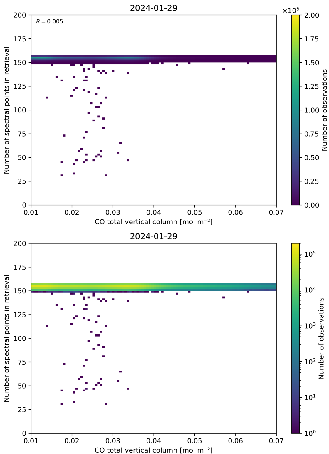
Figure 43: Scatter density plot of “CO total vertical column” against “Number of spectral points in retrieval” for 2024-01-28 to 2024-01-30.
