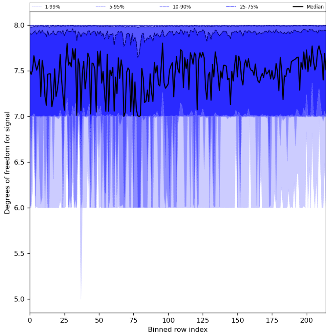
Figure 31: Along track statistics of “Degrees of freedom for signal” for 2024-01-28 to 2024-01-30
