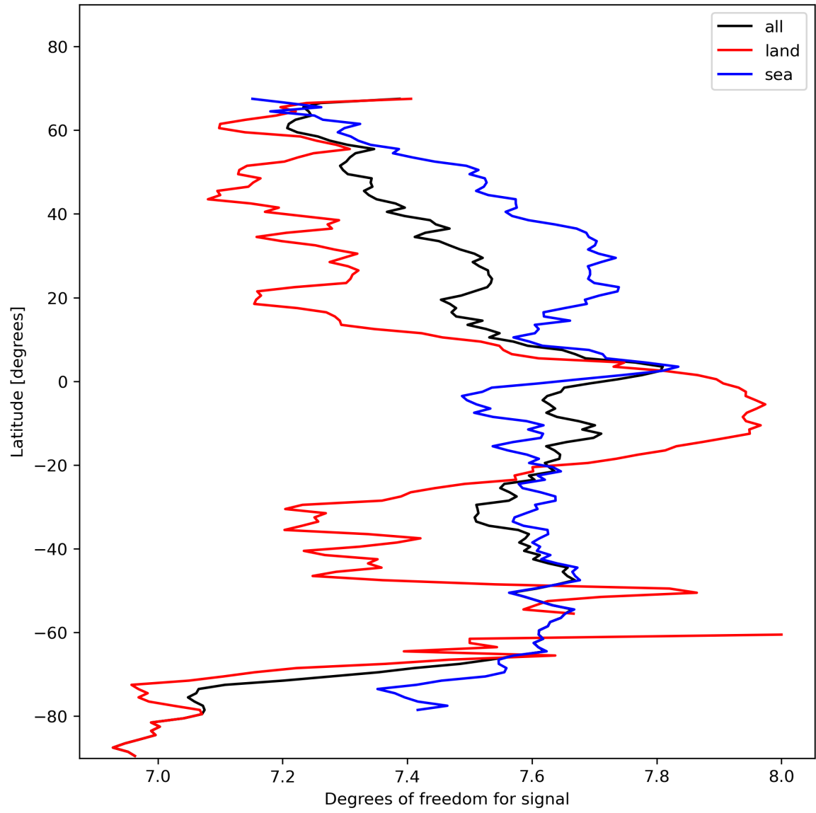
Figure 15: Zonal average of “Degrees of freedom for signal” for 2024-01-28 to 2024-01-30.
