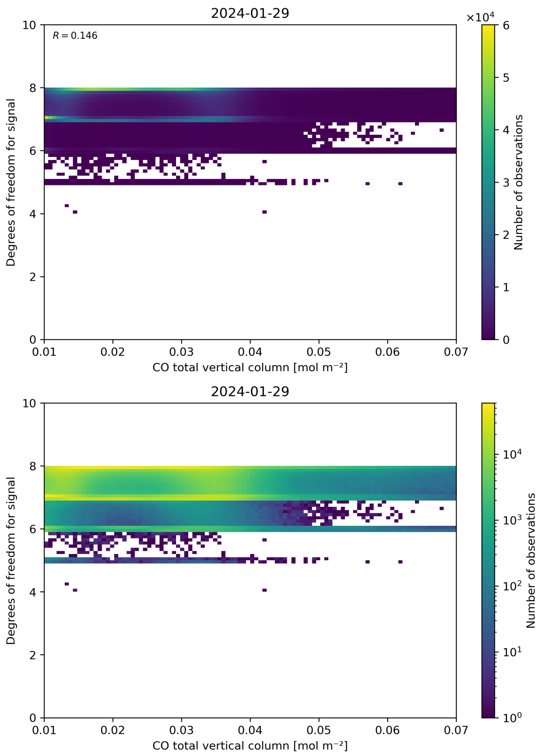
Figure 41: Scatter density plot of “CO total vertical column” against “Degrees of freedom for signal” for 2024-01-28 to 2024-01-30.
