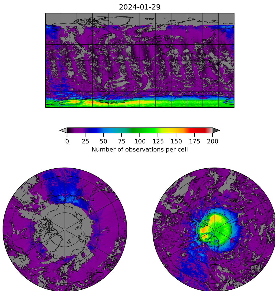
Figure 8: Map of the number of observations for 2024-01-28 to 2024-01-30
