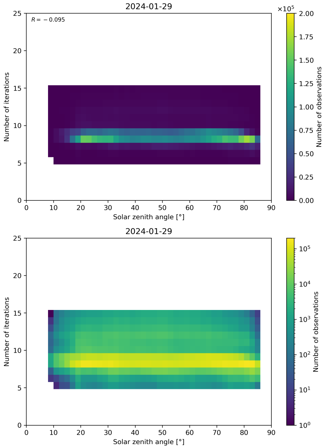
Figure 67: Scatter density plot of “Solar zenith angle” against “Number of iterations” for 2024-01-28 to 2024-01-30.
