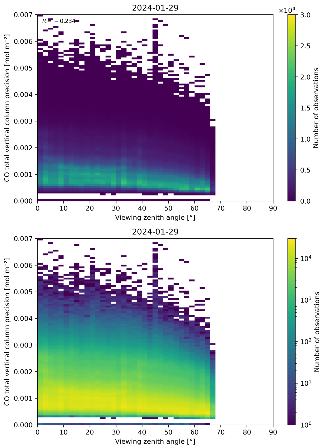
Figure 71: Scatter density plot of “Viewing zenith angle” against “CO total vertical column precision” for 2024-01-28 to 2024-01-30.
