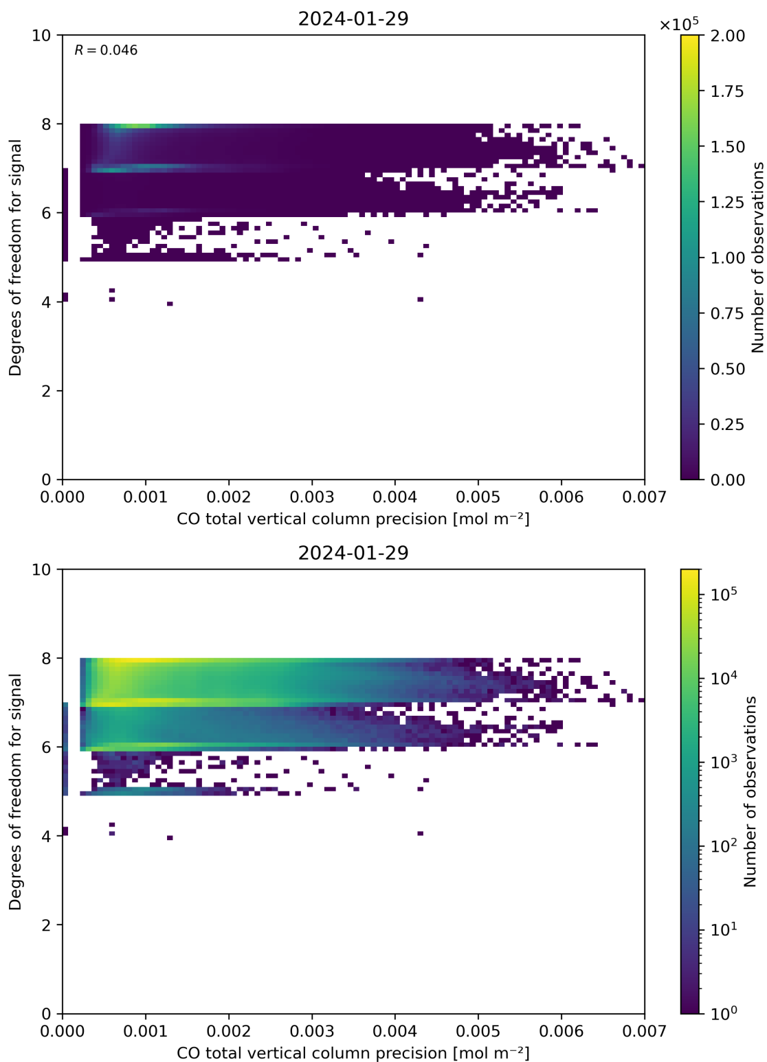
Figure 45: Scatter density plot of “CO total vertical column precision” against “Degrees of freedom for signal” for 2024-01-28 to 2024-01-30.
