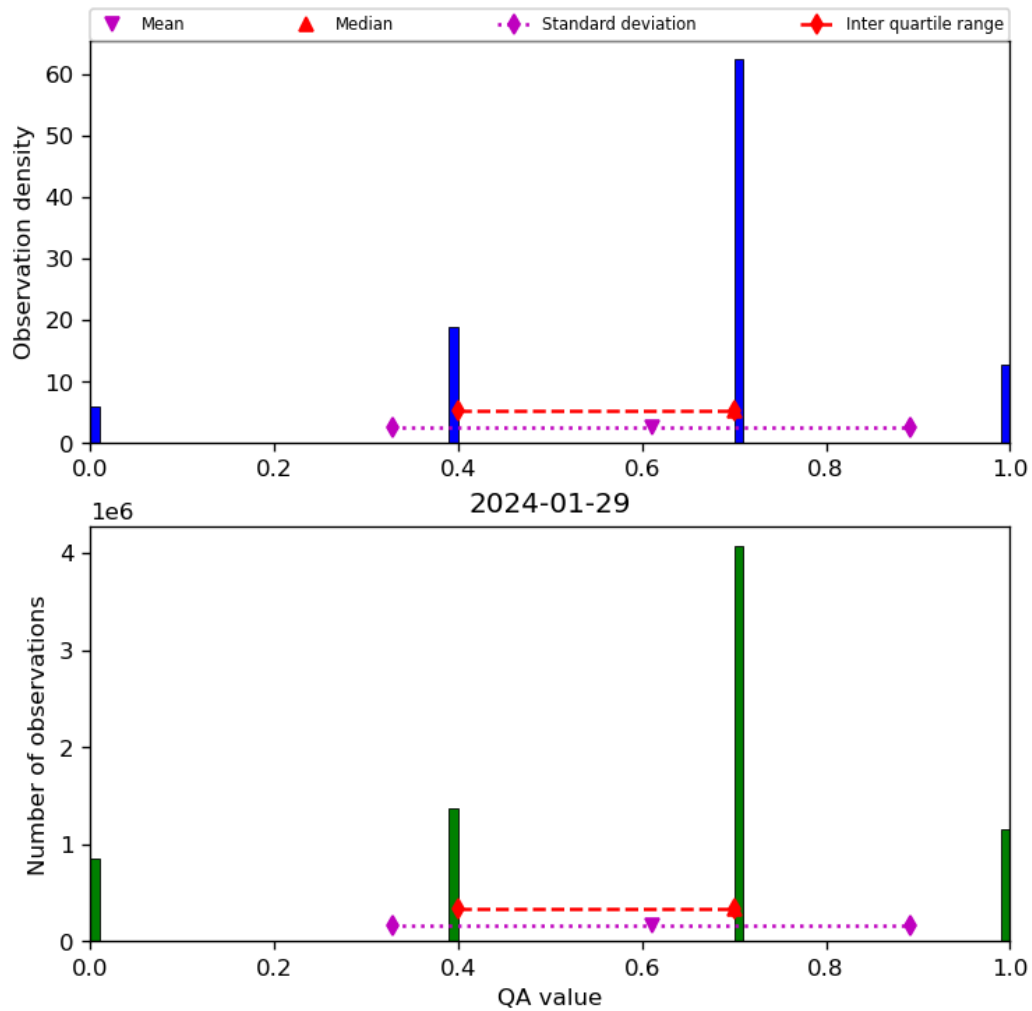
Figure 17: Histogram of “QA value” for 2024-01-28 to 2024-01-30
