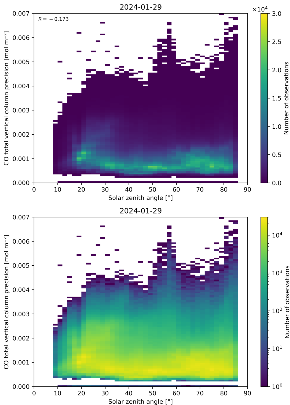
Figure 63: Scatter density plot of “Solar zenith angle” against “CO total vertical column precision” for 2024-01-28 to 2024-01-30.
