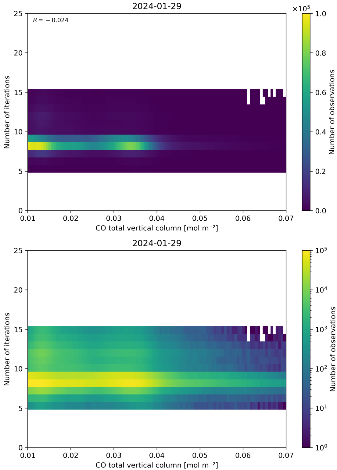
Figure 42: Scatter density plot of “CO total vertical column” against “Number of iterations” for 2024-01-28 to 2024-01-30.
