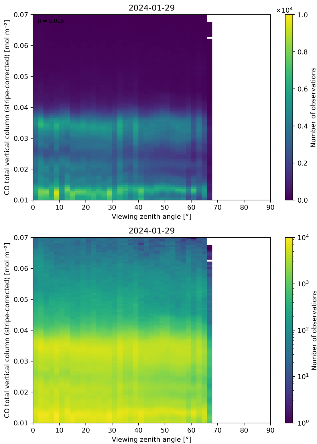
Figure 70: Scatter density plot of “Viewing zenith angle” against “CO total vertical column (stripe-corrected)” for 2024-01-28 to 2024-01-30.
