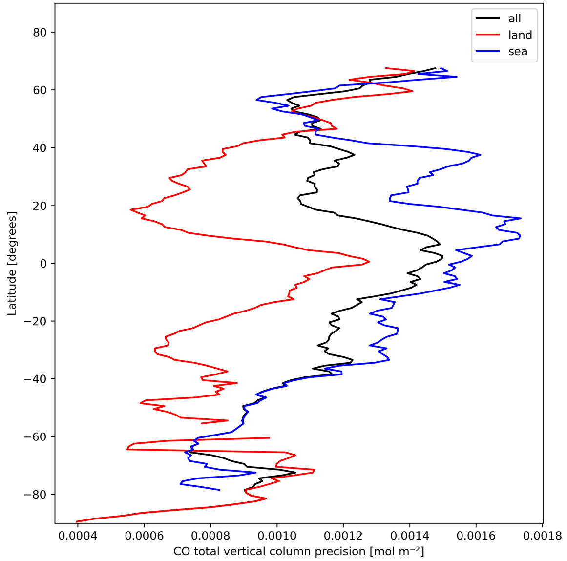
Figure 12: Zonal average of “CO total vertical column precision” for 2024-01-28 to 2024-01-30.
