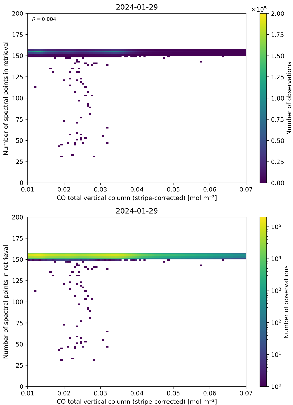
Figure 40: Scatter density plot of “CO total vertical column (stripe-corrected)” against “Number of spectral points in retrieval” for 2024-01-28 to 2024-01-30.
