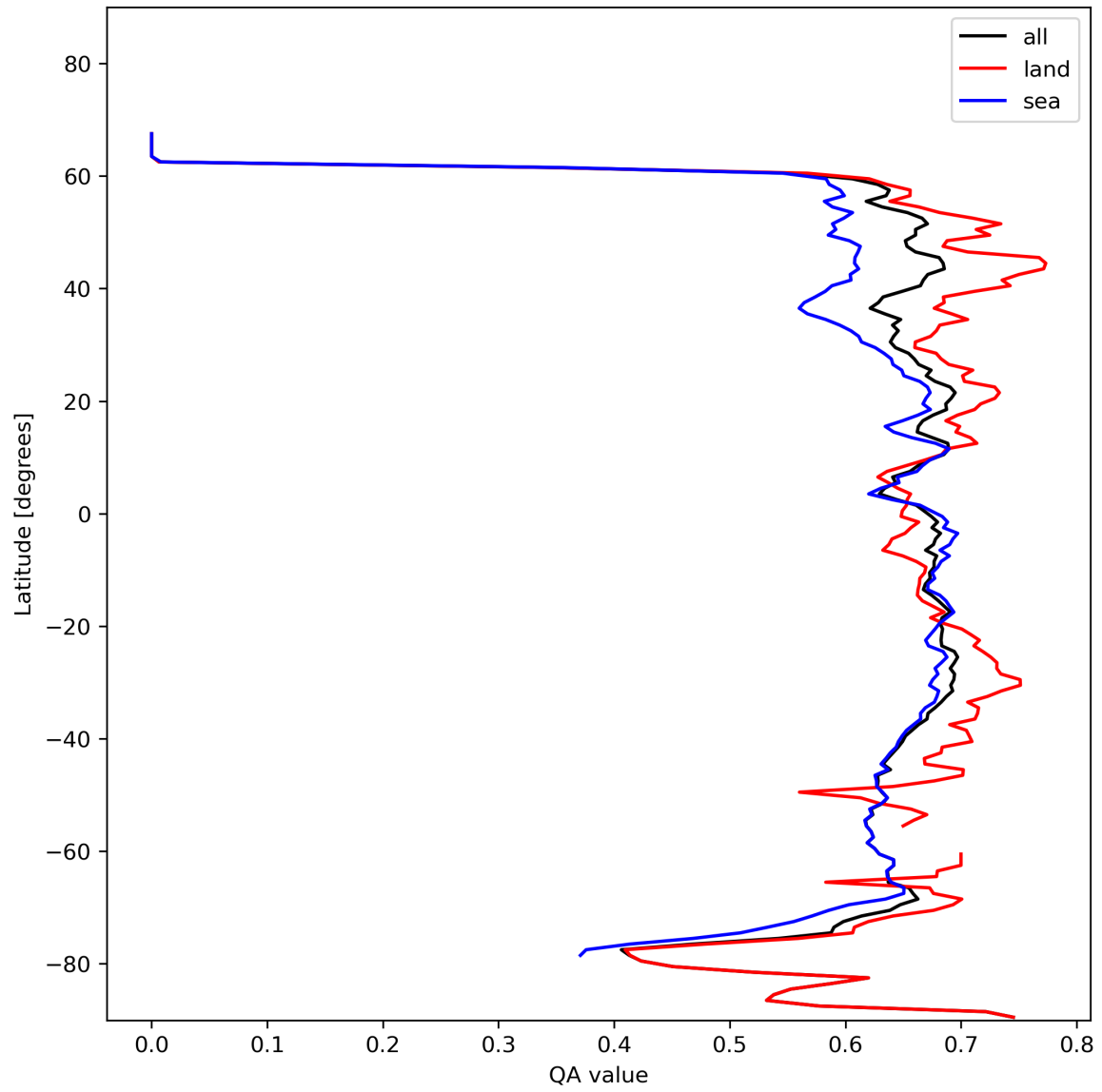
Figure 9: Zonal average of “QA value” for 2024-01-28 to 2024-01-30.
