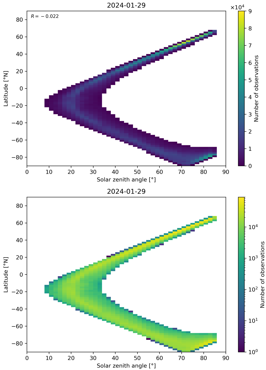
Figure 66: Scatter density plot of “Solar zenith angle” against “Latitude” for 2024-01-28 to 2024-01-30.
