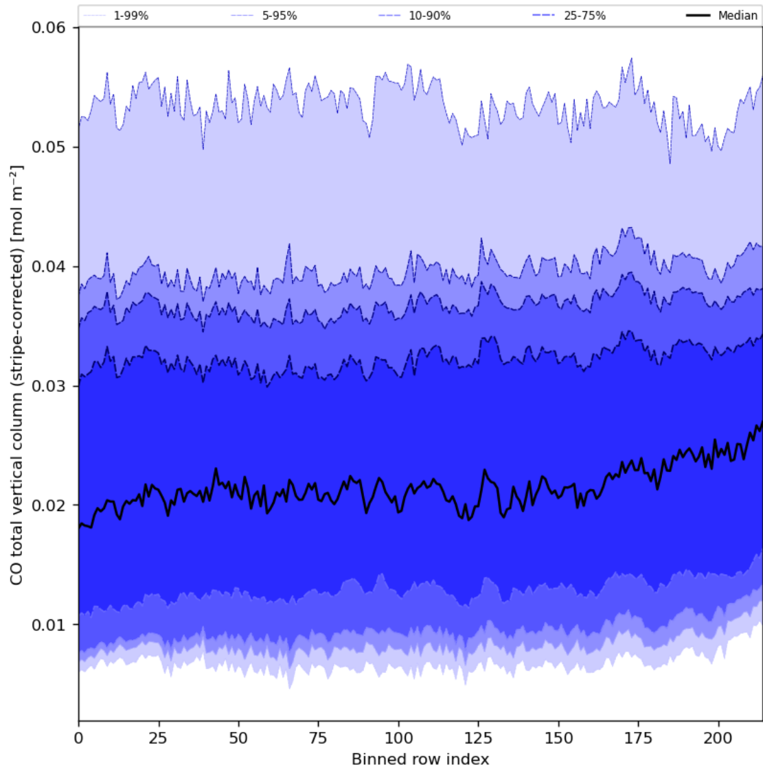
Figure 27: Along track statistics of “CO total vertical column (stripe-corrected)” for 2024-01-28 to 2024-01-30
