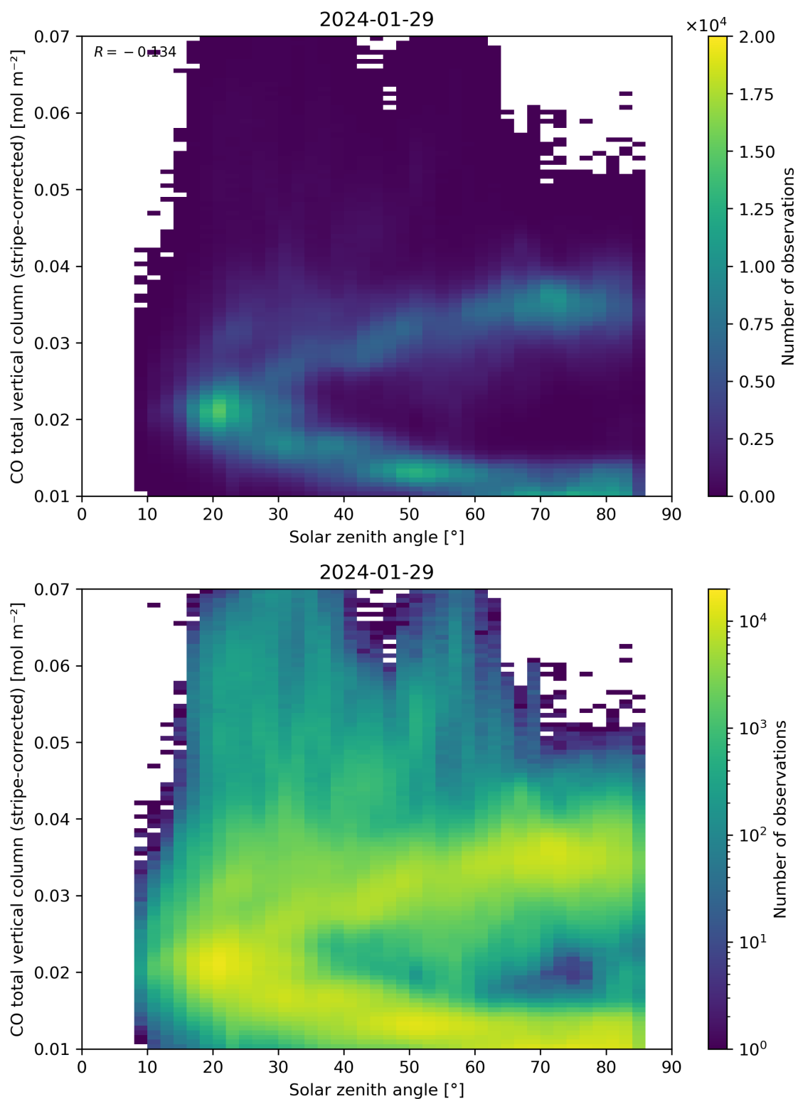
Figure 62: Scatter density plot of “Solar zenith angle” against “CO total vertical column (stripe-corrected)” for 2024-01-28 to 2024-01-30.
