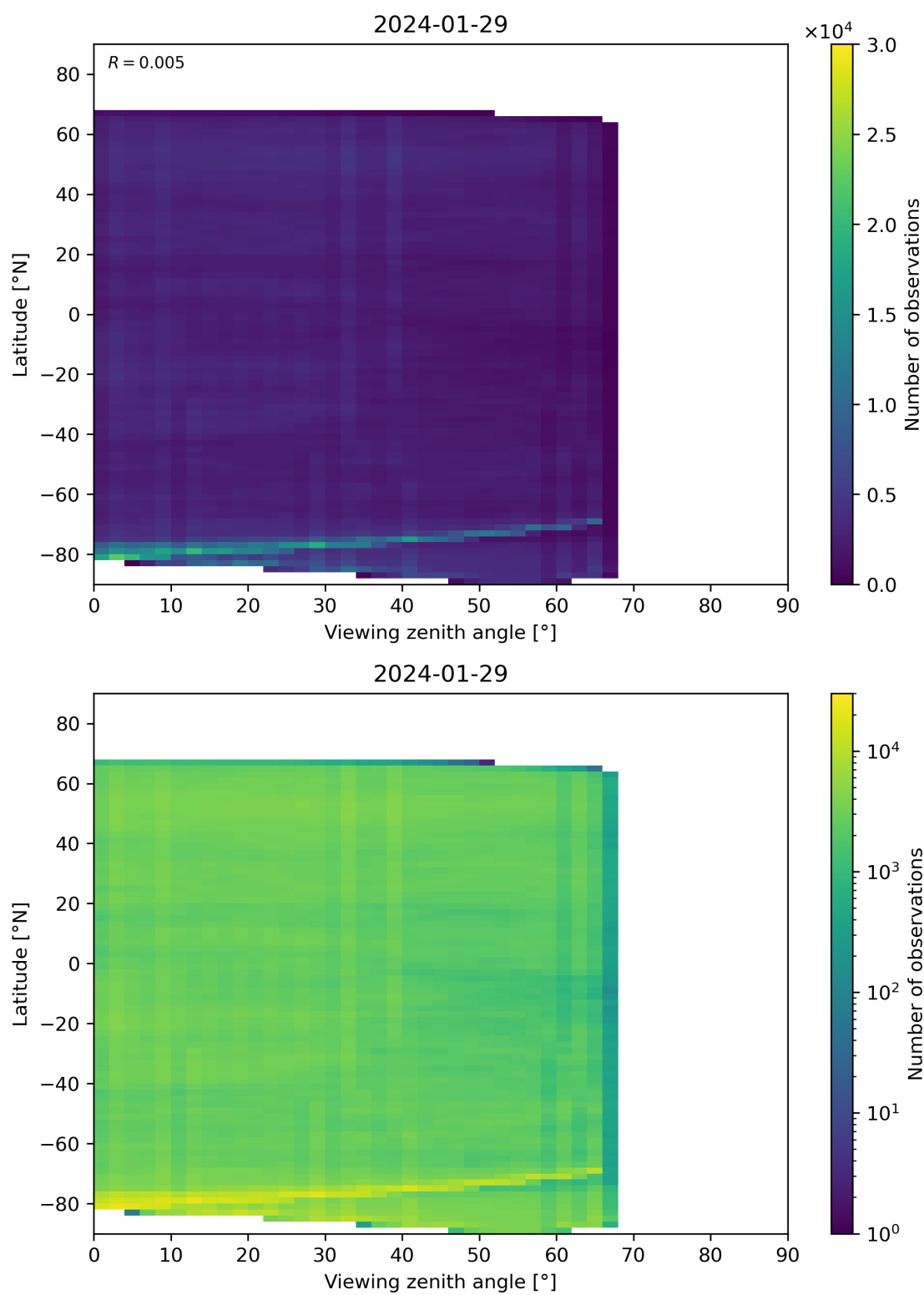
Figure 74: Scatter density plot of “Viewing zenith angle” against “Latitude” for 2024-01-28 to 2024-01-30.
