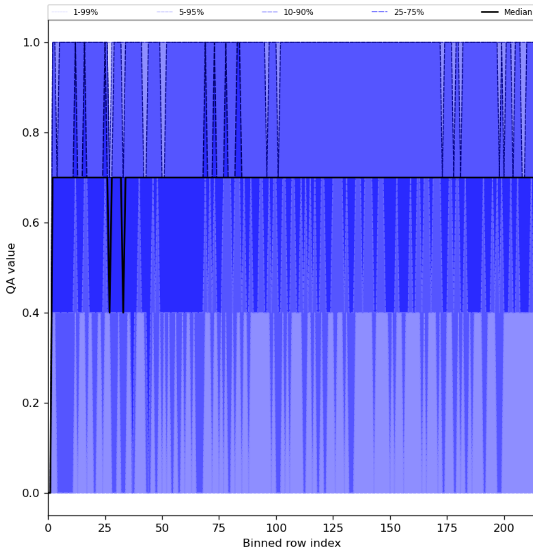
Figure 25: Along track statistics of “QA value” for 2024-01-28 to 2024-01-30
