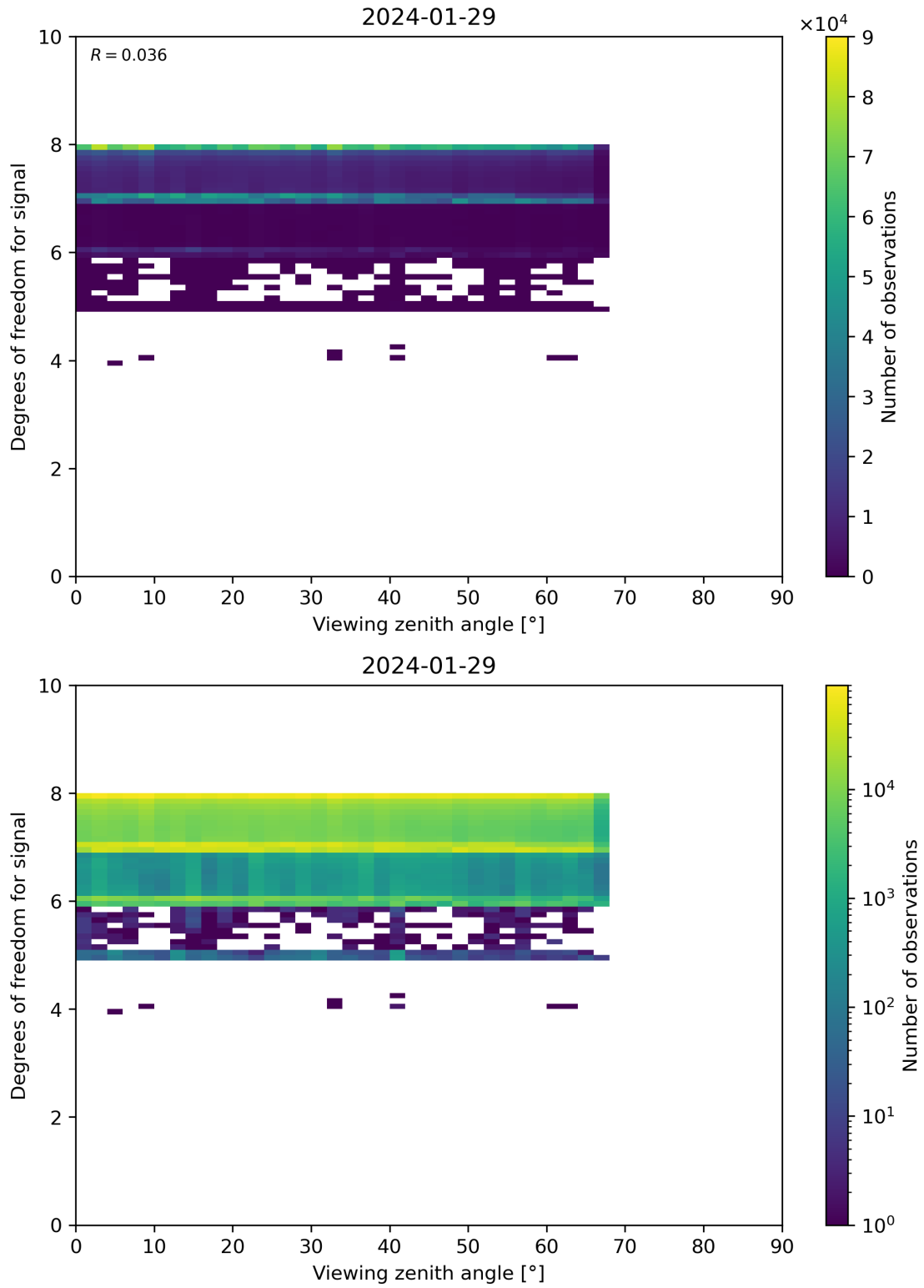
Figure 73: Scatter density plot of “Viewing zenith angle” against “Degrees of freedom for signal” for 2024-01-28 to 2024-01-30.
