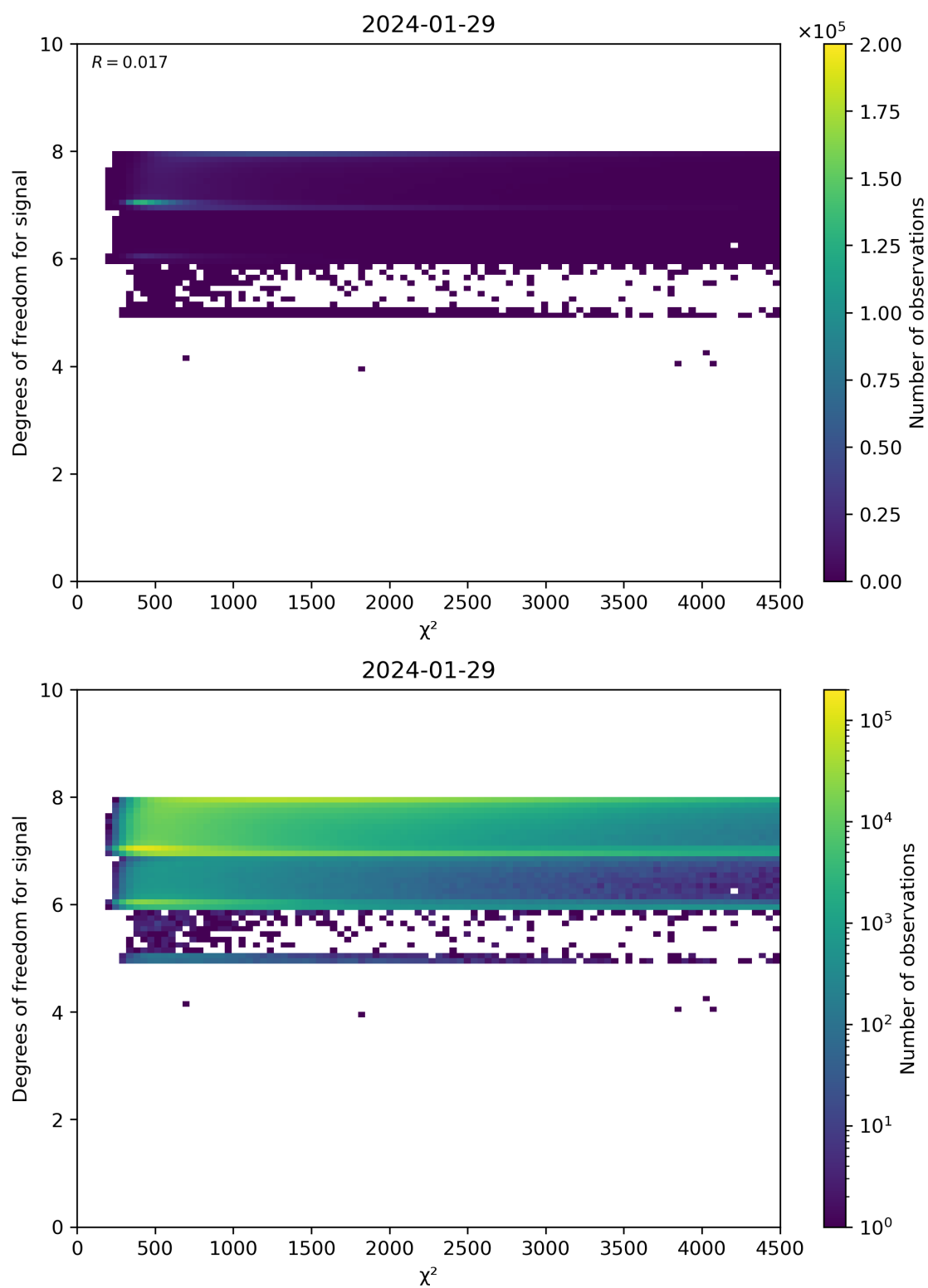
Figure 48: Scatter density plot of “ \chi^2 ” against “Degrees of freedom for signal” for 2024-01-28 to 2024-01-30.
