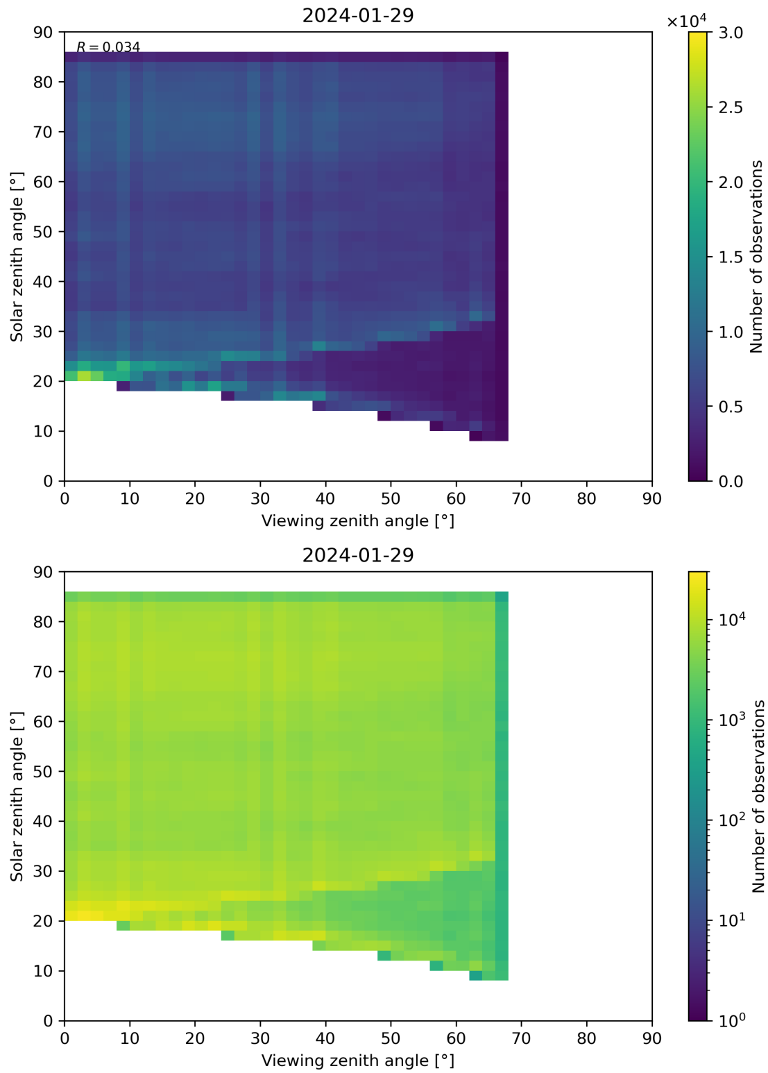
Figure 77: Scatter density plot of “Viewing zenith angle” against “Solar zenith angle” for 2024-01-28 to 2024-01-30.
