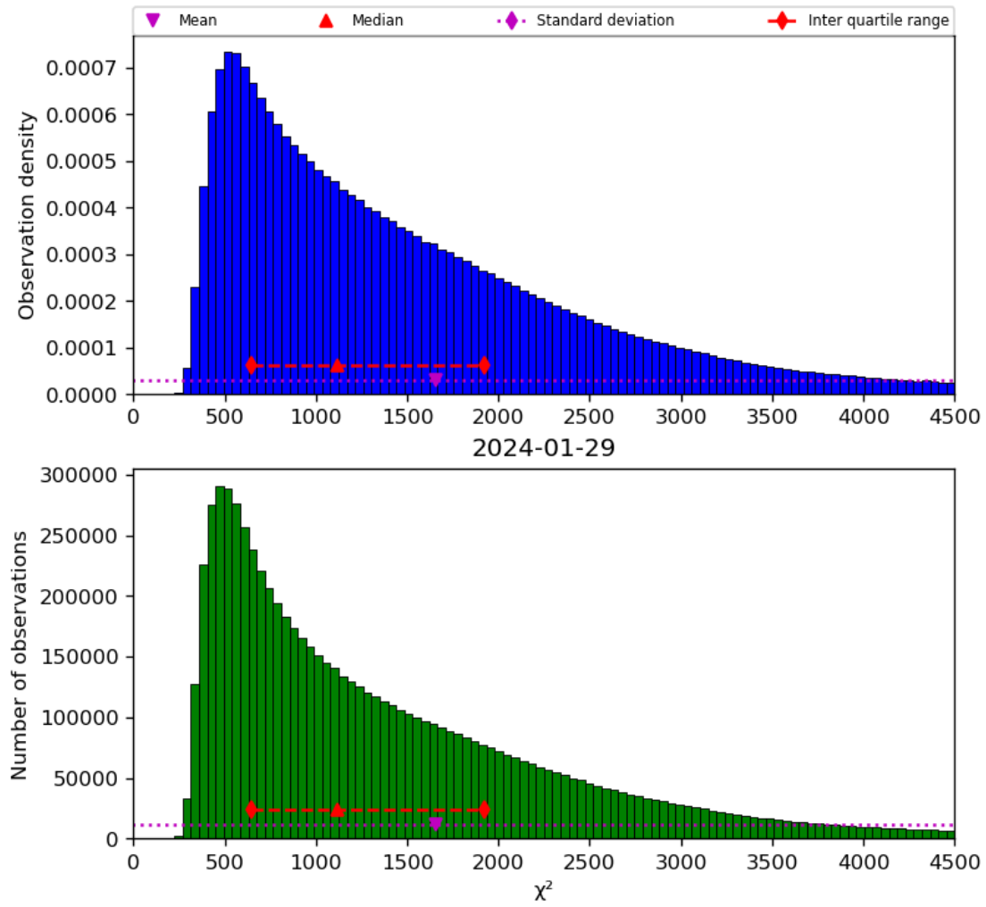
Figure 22: Histogram of “ \chi^2 ” for 2024-01-28 to 2024-01-30
