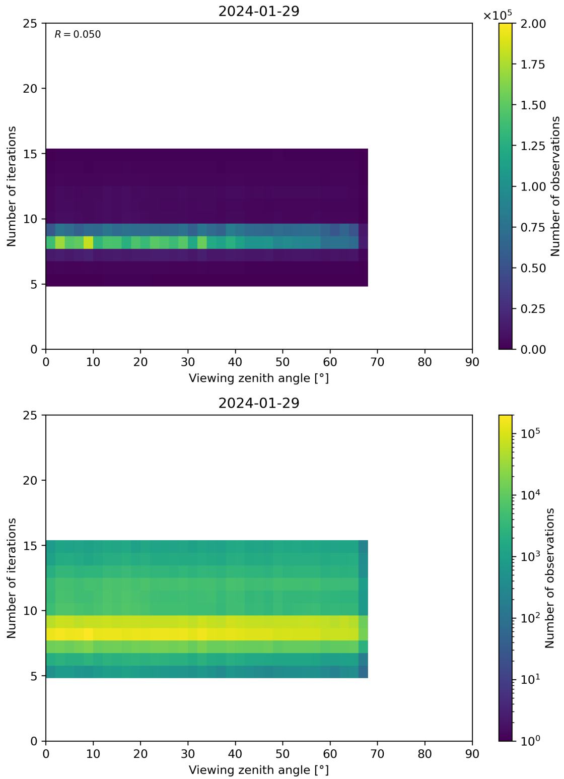
Figure 75: Scatter density plot of “Viewing zenith angle” against “Number of iterations” for 2024-01-28 to 2024-01-30.
