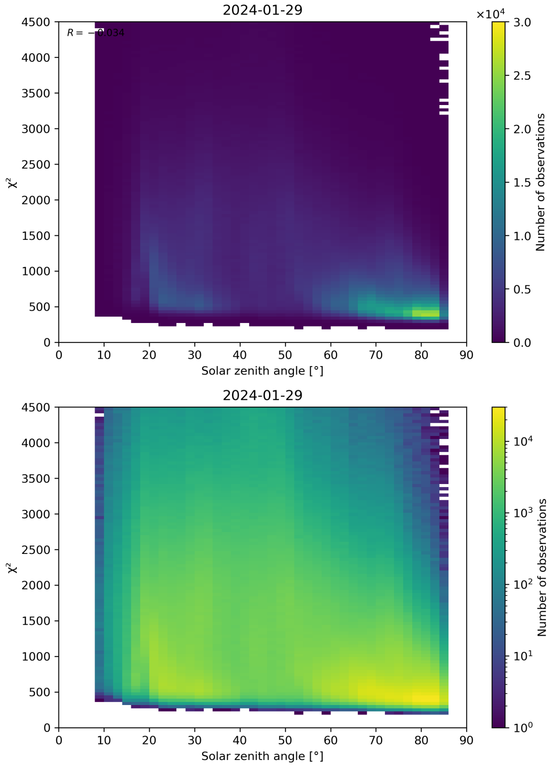
Figure 64: Scatter density plot of “Solar zenith angle” against “ \chi^2 ” for 2024-01-28 to 2024-01-30.
