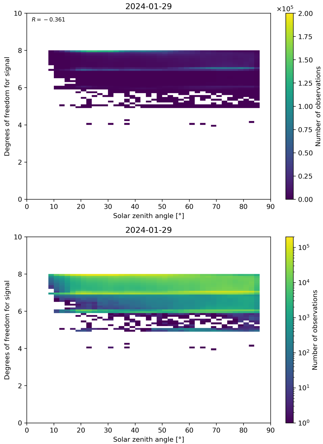
Figure 65: Scatter density plot of “Solar zenith angle” against “Degrees of freedom for signal” for 2024-01-28 to 2024-01-30.
