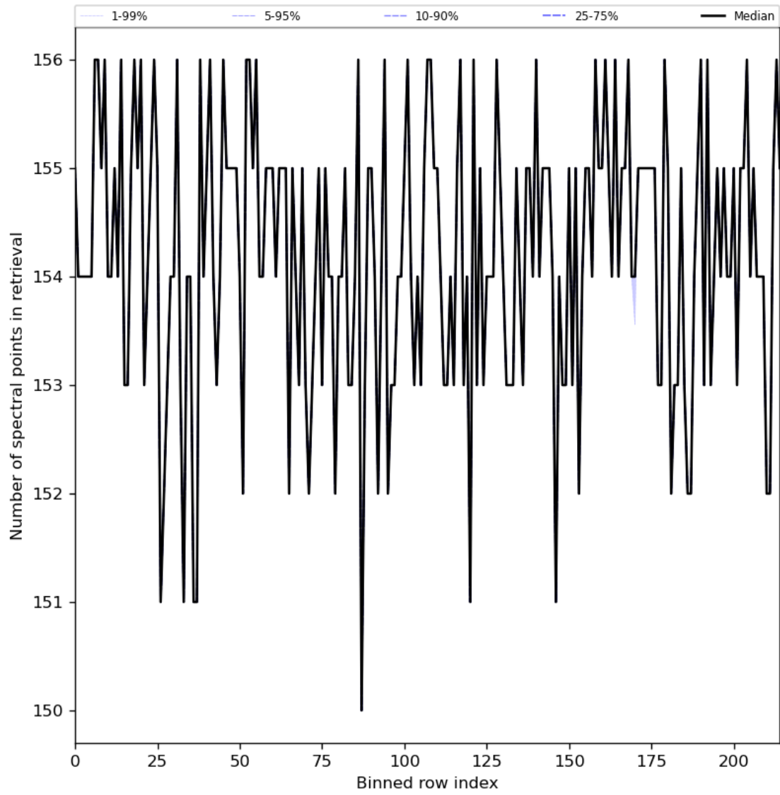
Figure 29: Along track statistics of “Number of spectral points in retrieval” for 2024-01-28 to 2024-01-30
