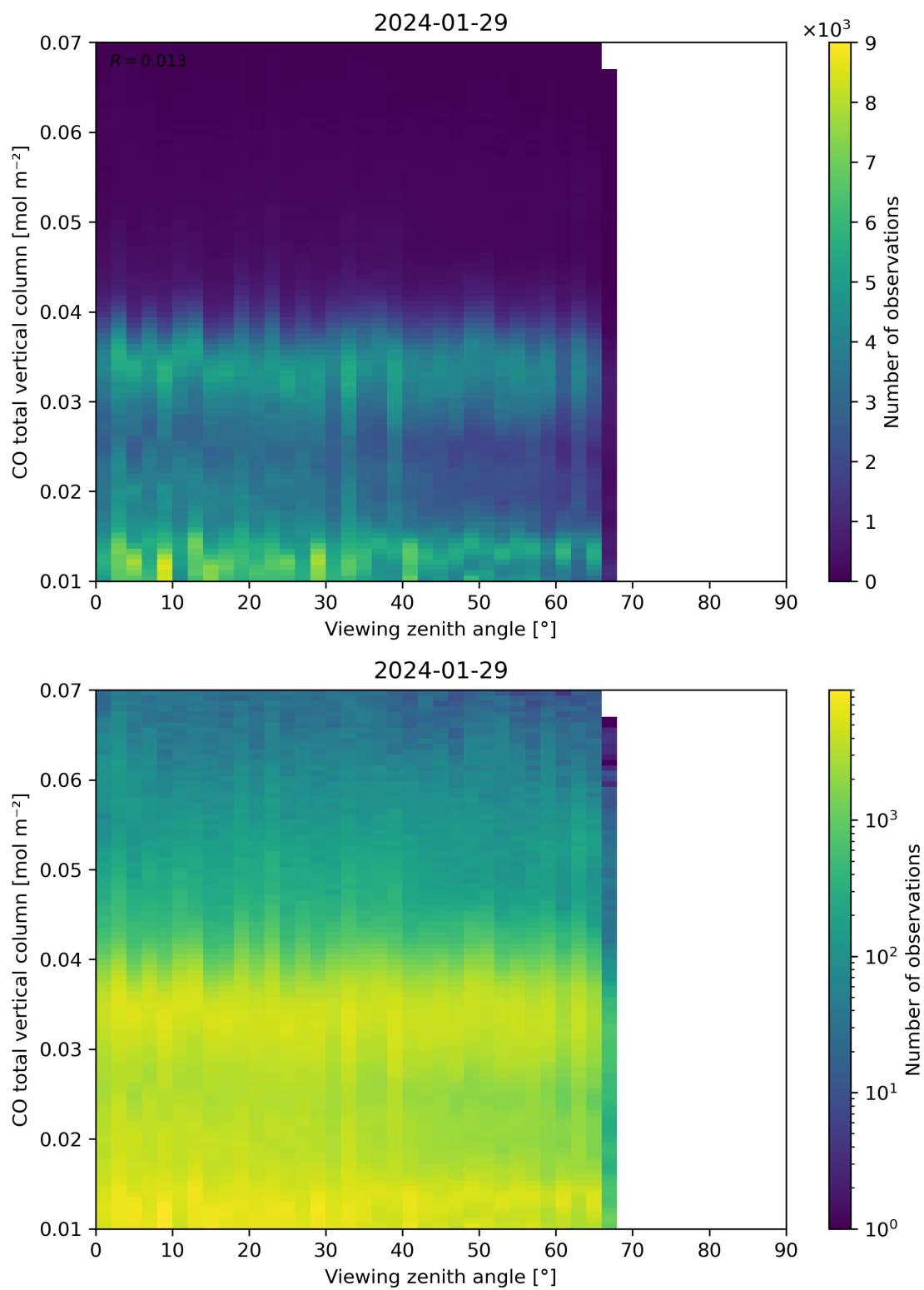
Figure 69: Scatter density plot of “Viewing zenith angle” against “CO total vertical column” for 2024-01-28 to 2024-01-30.
