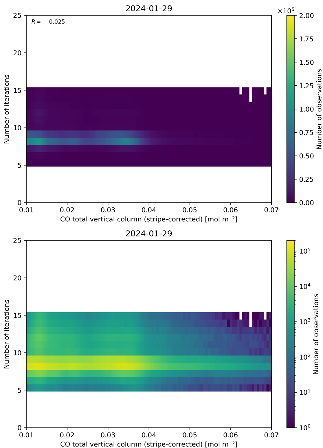
Figure 39: Scatter density plot of “CO total vertical column (stripe-corrected)” against “Number of iterations” for 2024-01-28 to 2024-01-30.
