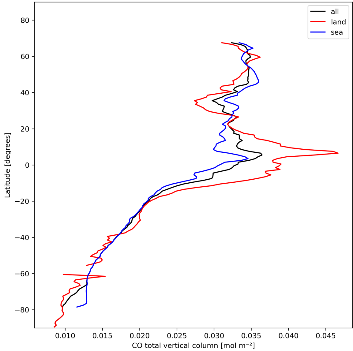
Figure 10: Zonal average of “CO total vertical column” for 2024-01-28 to 2024-01-30.
