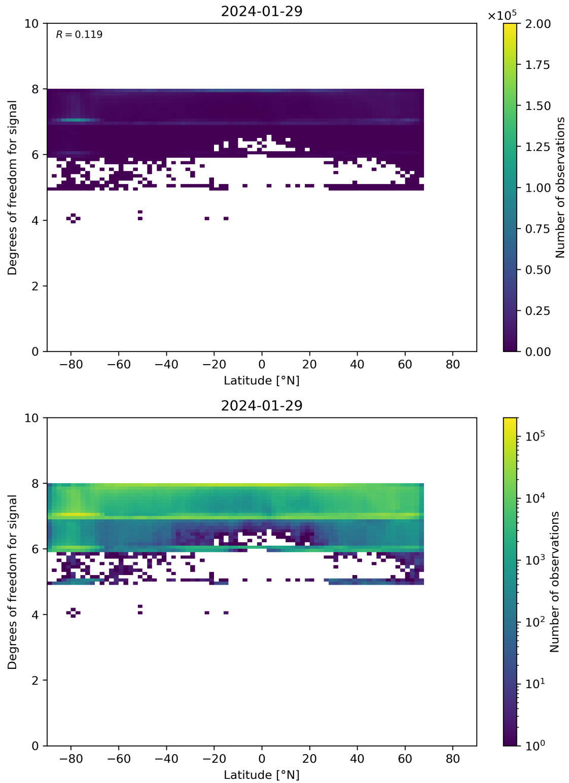
Figure 55: Scatter density plot of “Latitude” against “Degrees of freedom for signal” for 2024-01-28 to 2024-01-30.
