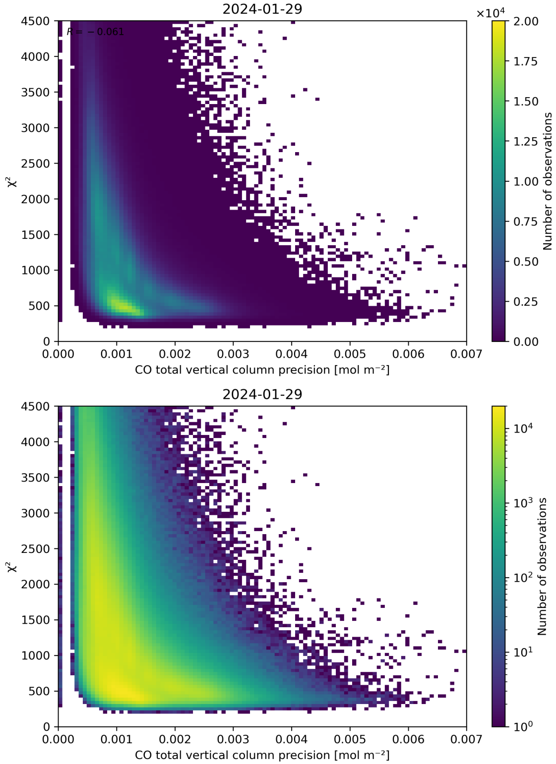
Figure 44: Scatter density plot of “CO total vertical column precision” against “ \chi^2 ” for 2024-01-28 to 2024-01-30.
