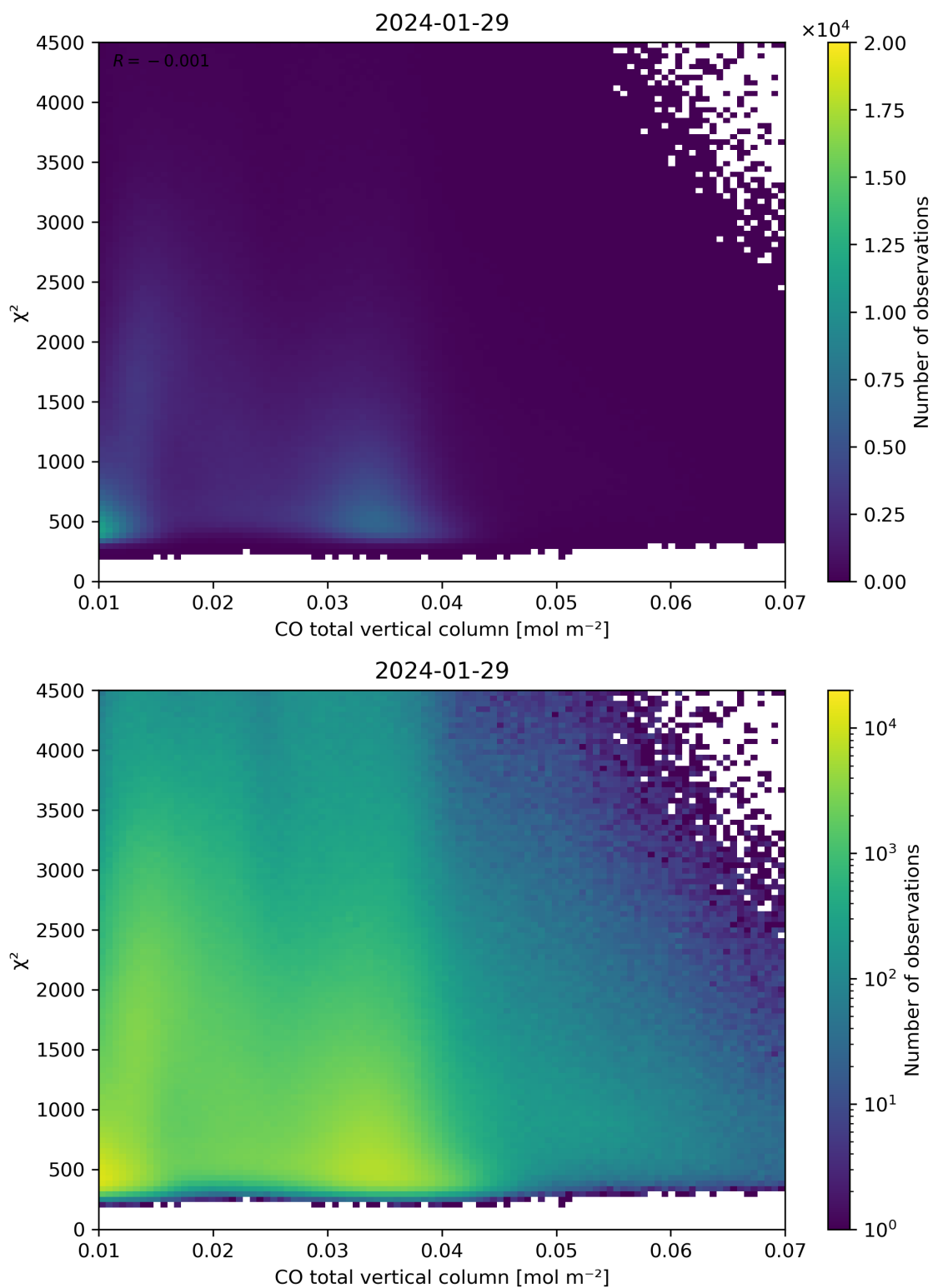
Figure 35: Scatter density plot of “CO total vertical column” against “ \chi^2 ” for 2024-01-28 to 2024-01-30.
