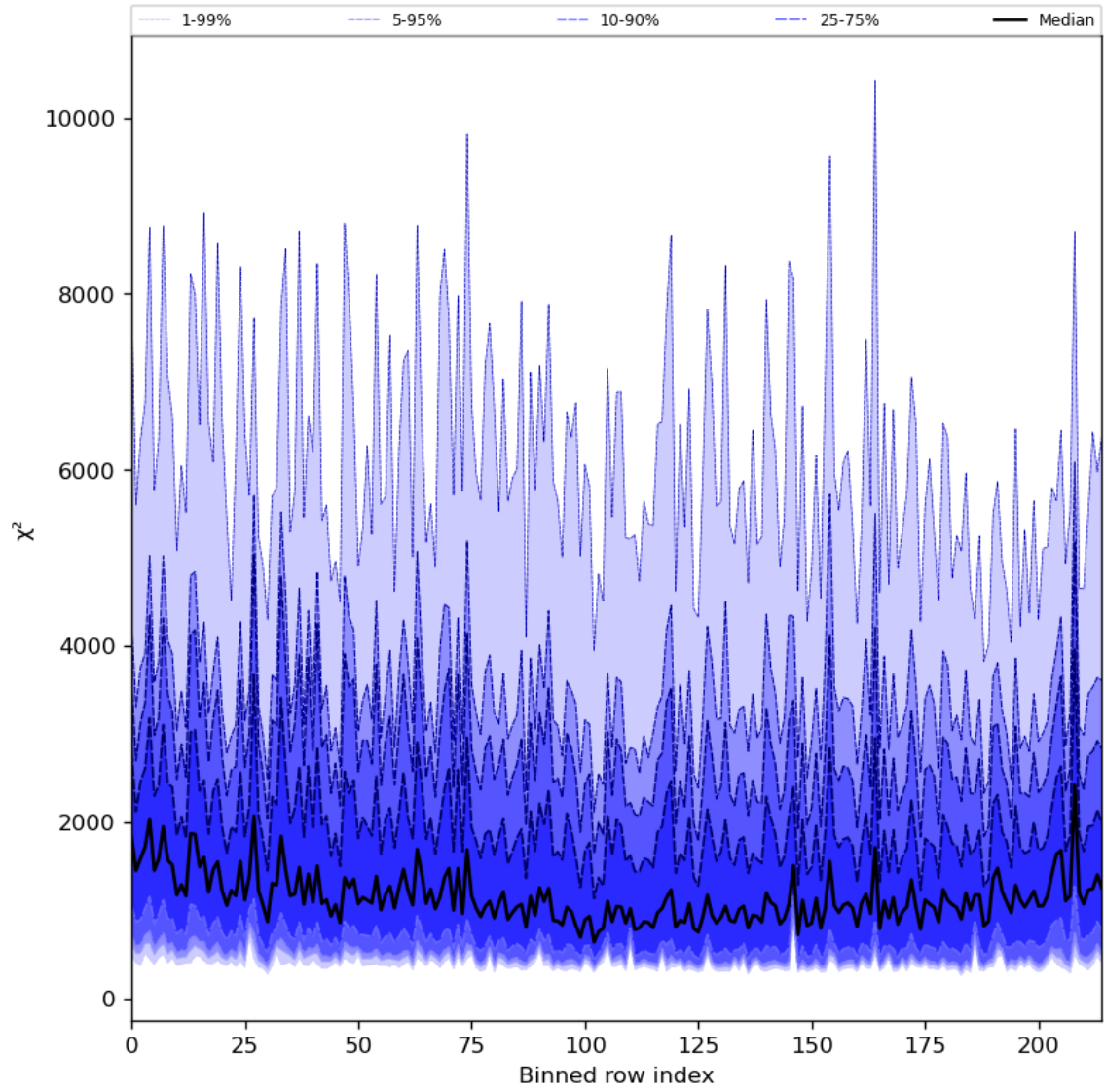
Figure 30: Along track statistics of “ \chi^2 ” for 2024-01-28 to 2024-01-30
