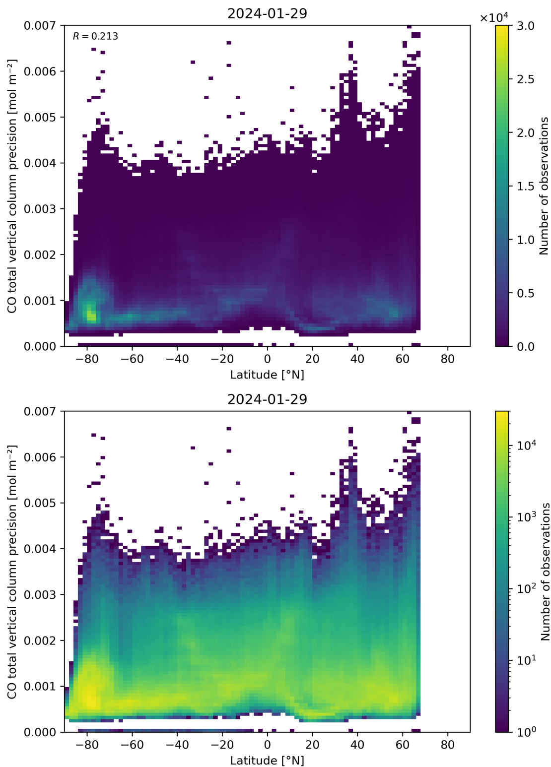
Figure 53: Scatter density plot of “Latitude” against “CO total vertical column precision” for 2024-01-28 to 2024-01-30.
