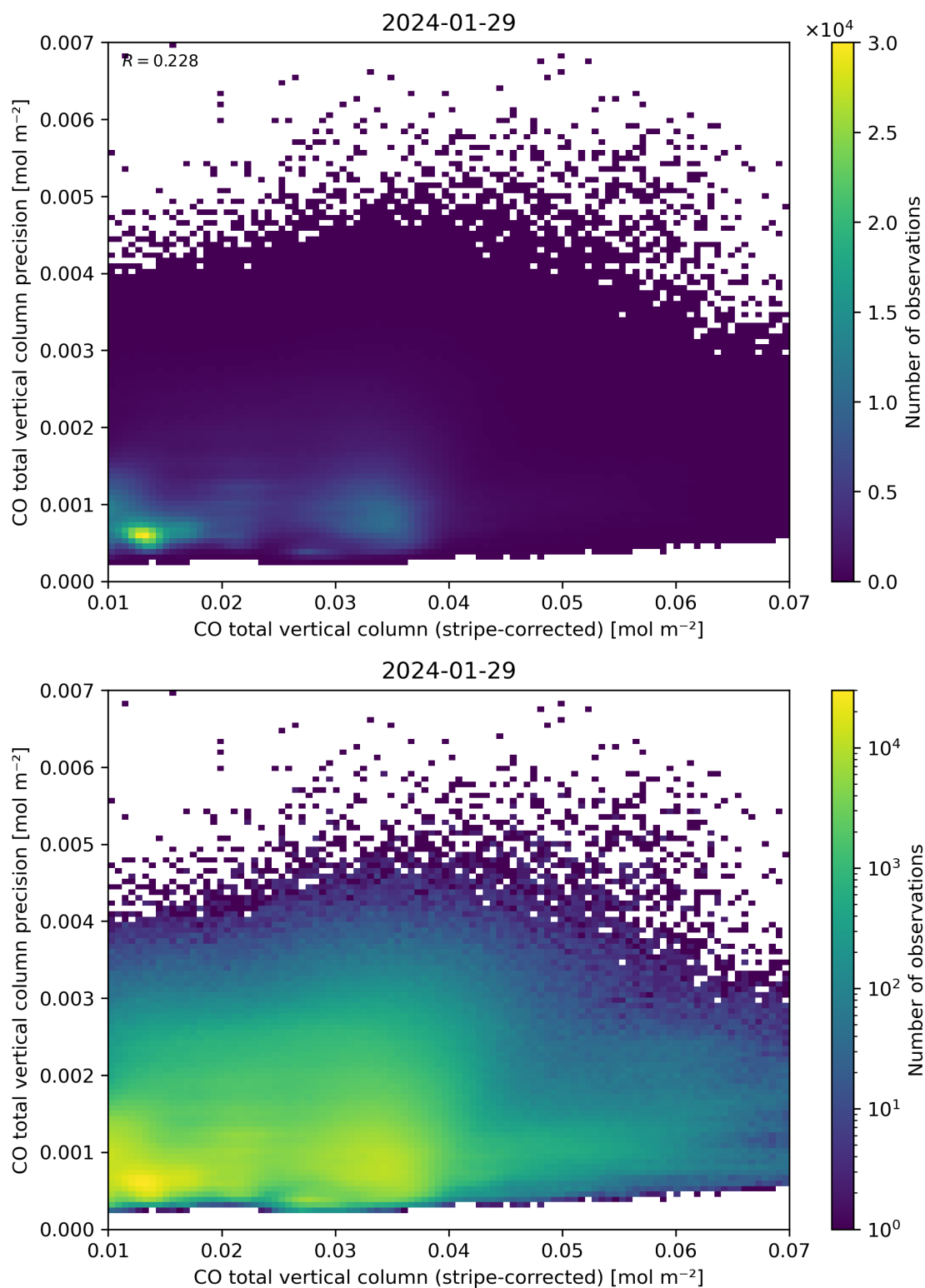
Figure 36: Scatter density plot of “CO total vertical column (stripe-corrected)” against “CO total vertical column precision” for 2024-01-28 to 2024-01-30.
