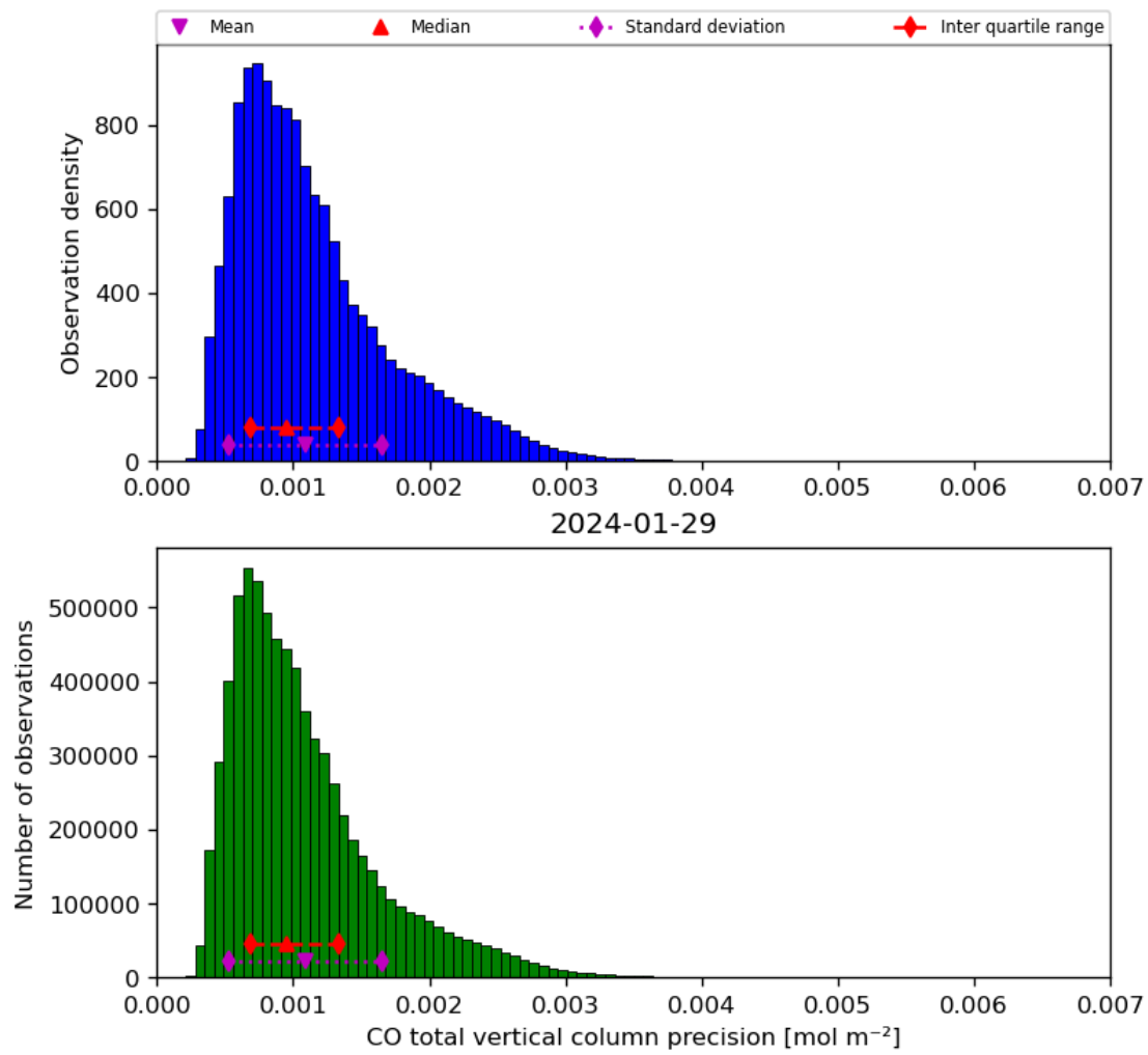
Figure 20: Histogram of “CO total vertical column precision” for 2024-01-28 to 2024-01-30
