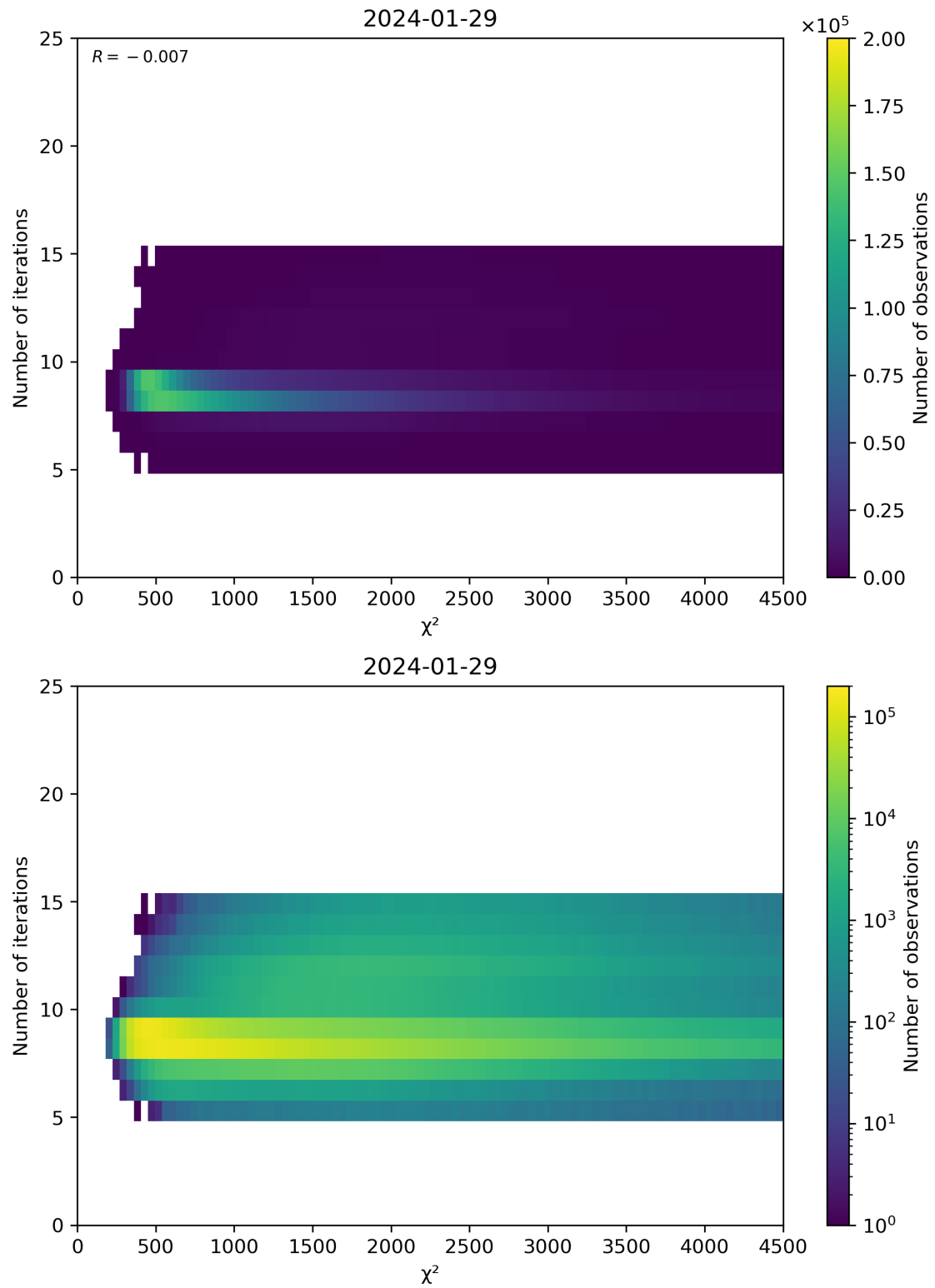
Figure 49: Scatter density plot of “ \chi^2 ” against “Number of iterations” for 2024-01-28 to 2024-01-30.
