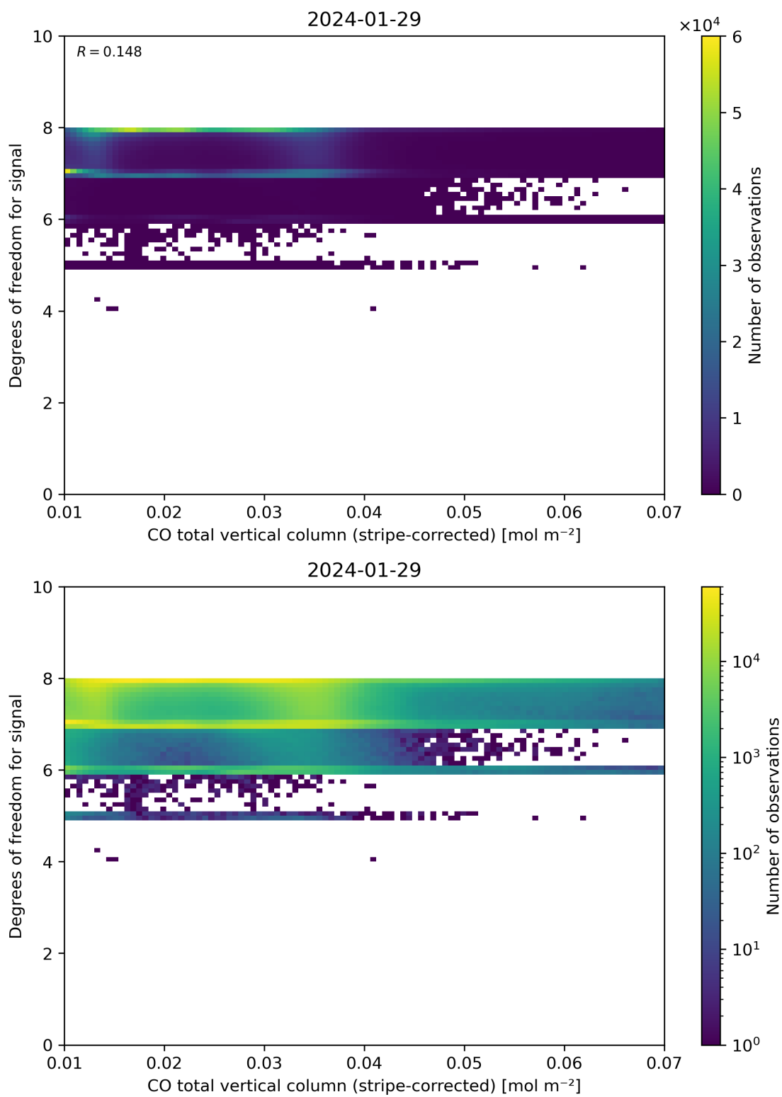
Figure 38: Scatter density plot of “CO total vertical column (stripe-corrected)” against “Degrees of freedom for signal” for 2024-01-28 to 2024-01-30.
