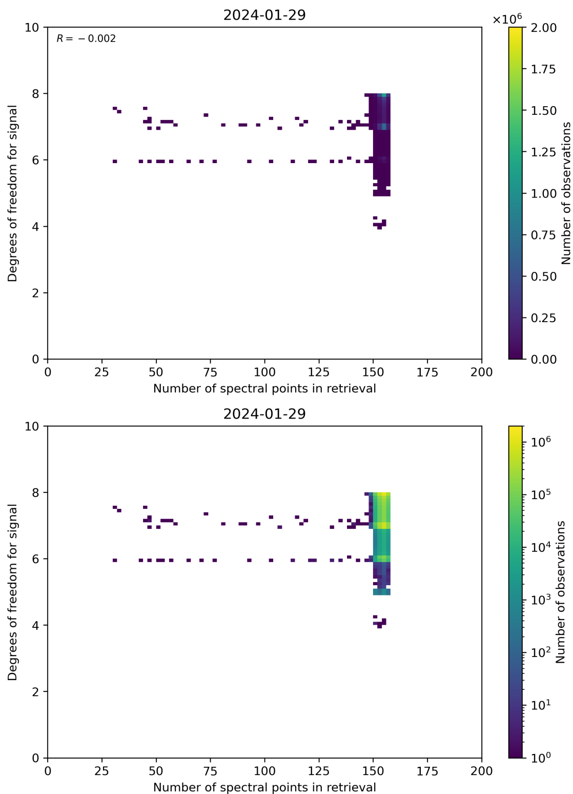
Figure 59: Scatter density plot of “Number of spectral points in retrieval” against “Degrees of freedom for signal” for 2024-01-28 to 2024-01-30.
