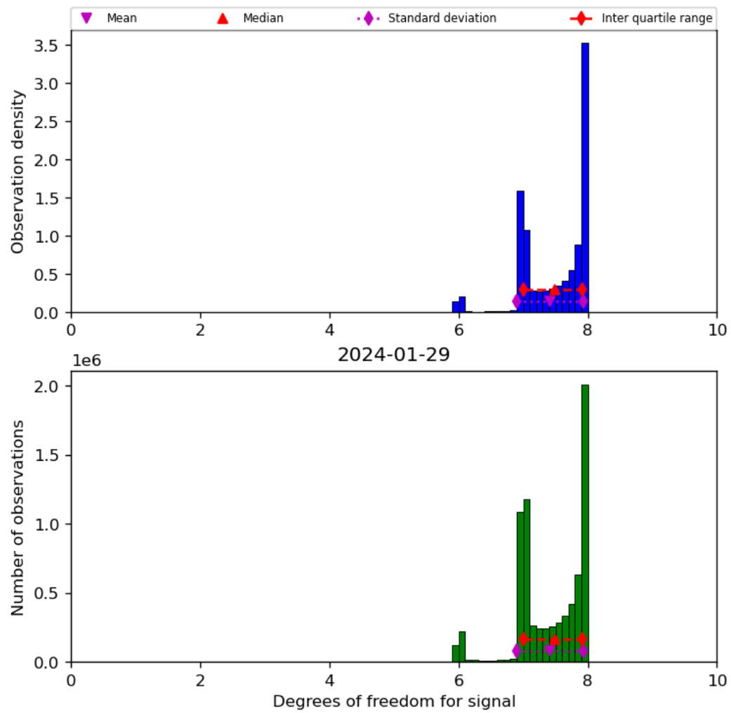
Figure 23: Histogram of “Degrees of freedom for signal” for 2024-01-28 to 2024-01-30
