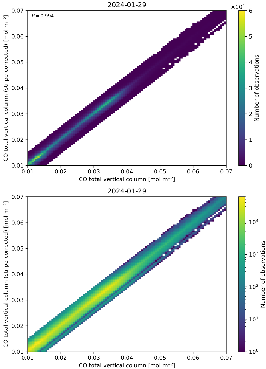
Figure 33: Scatter density plot of “CO total vertical column” against “CO total vertical column (stripe-corrected)” for 2024-01-28 to 2024-01-30.
