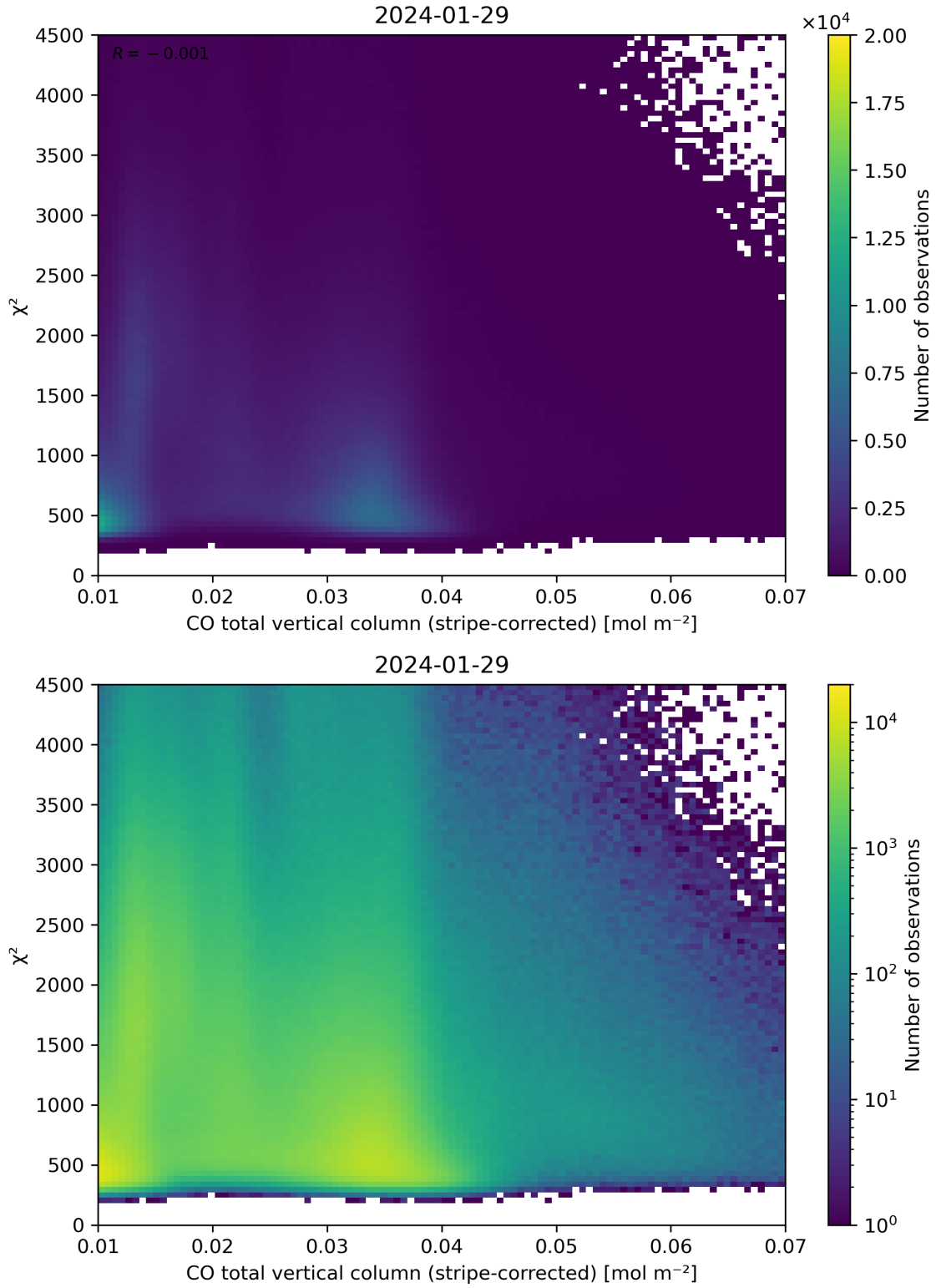
Figure 37: Scatter density plot of “CO total vertical column (stripe-corrected)” against “ \chi^2 ” for 2024-01-28 to 2024-01-30.
