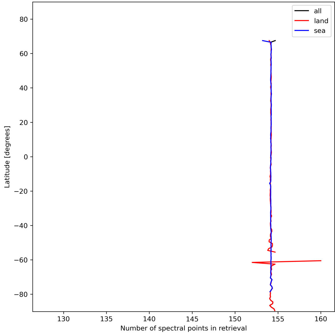
Figure 13: Zonal average of “Number of spectral points in retrieval” for 2024-01-28 to 2024-01-30.
