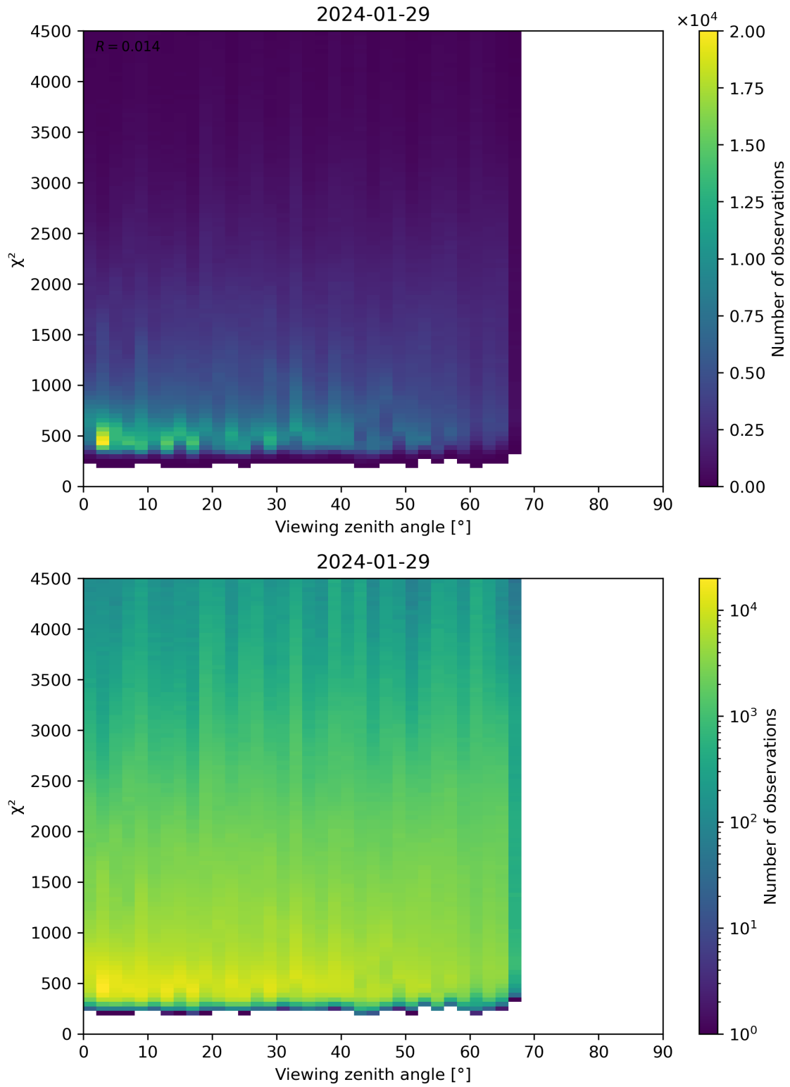
Figure 72: Scatter density plot of “Viewing zenith angle” against “ \chi^2 ” for 2024-01-28 to 2024-01-30.
