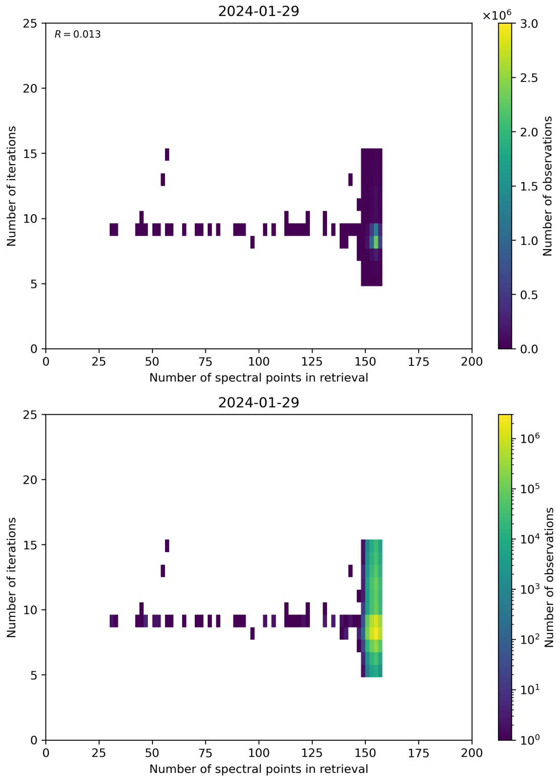
Figure 60: Scatter density plot of “Number of spectral points in retrieval” against “Number of iterations” for 2024-01-28 to 2024-01-30.
