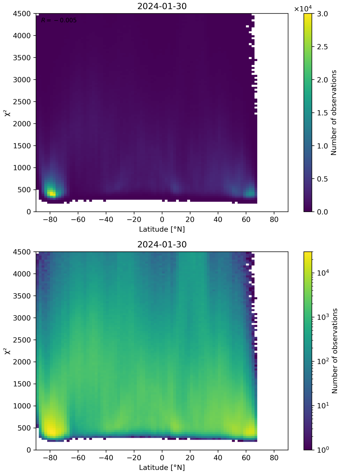
Figure 54: Scatter density plot of “Latitude” against “ \chi^2 ” for 2024-01-29 to 2024-01-31.
