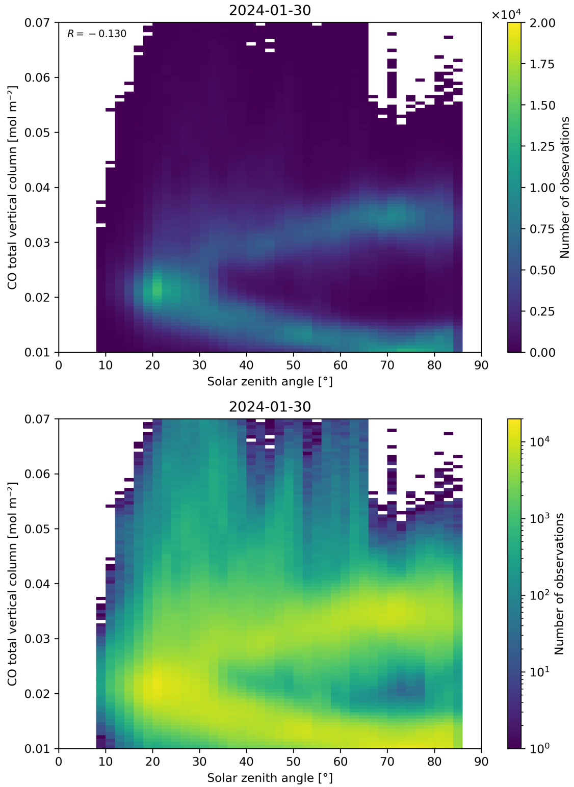
Figure 61: Scatter density plot of “Solar zenith angle” against “CO total vertical column” for 2024-01-29 to 2024-01-31.
