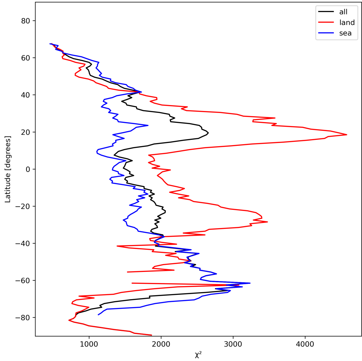
Figure 14: Zonal average of “ \chi^2 ” for 2024-01-29 to 2024-01-31.
