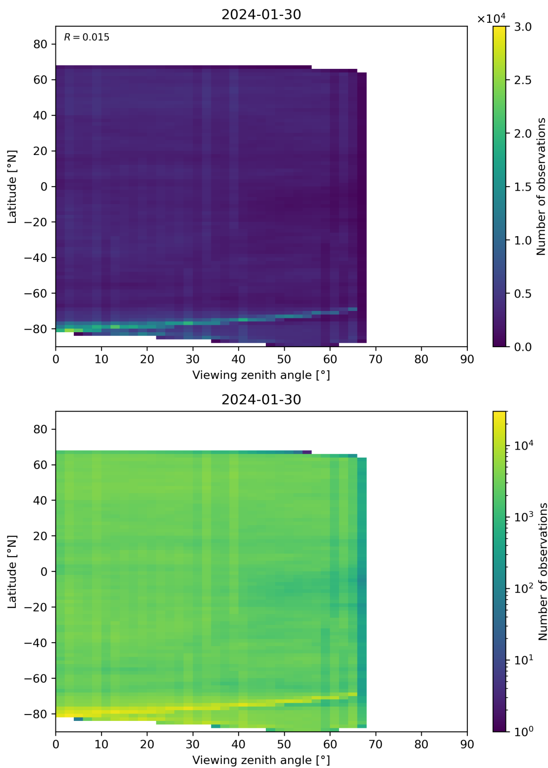
Figure 74: Scatter density plot of “Viewing zenith angle” against “Latitude” for 2024-01-29 to 2024-01-31.
