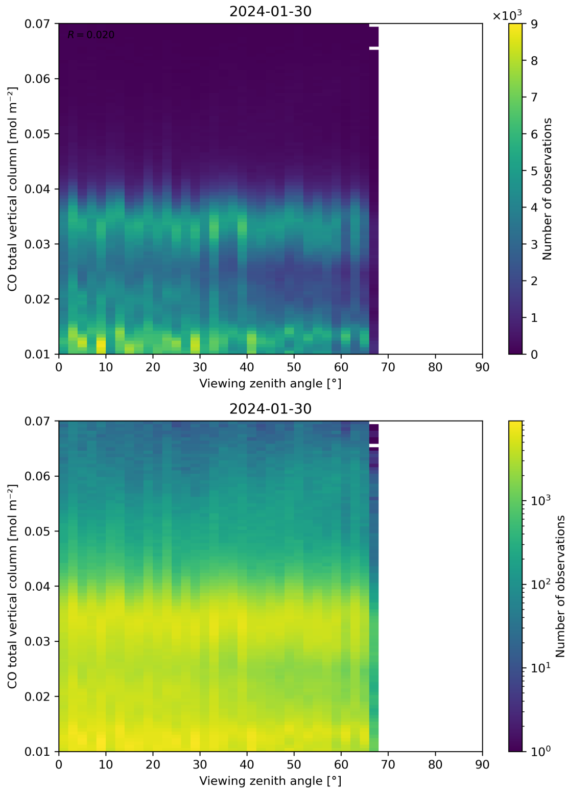
Figure 69: Scatter density plot of “Viewing zenith angle” against “CO total vertical column” for 2024-01-29 to 2024-01-31.
