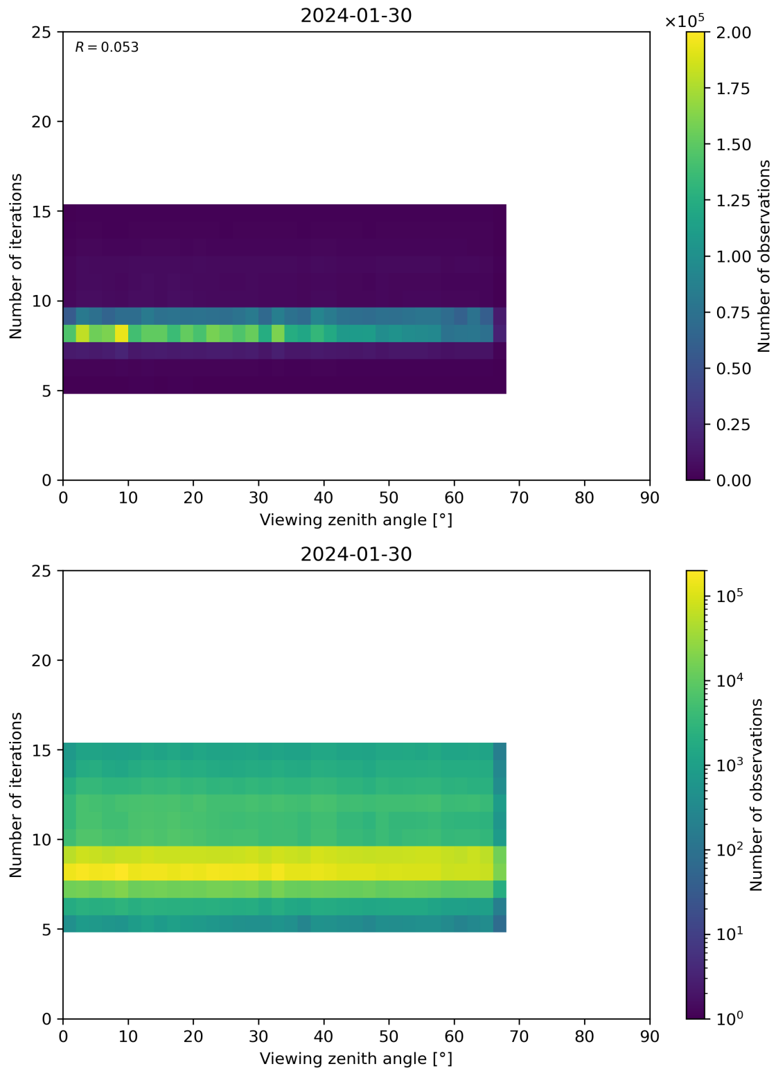
Figure 75: Scatter density plot of “Viewing zenith angle” against “Number of iterations” for 2024-01-29 to 2024-01-31.
