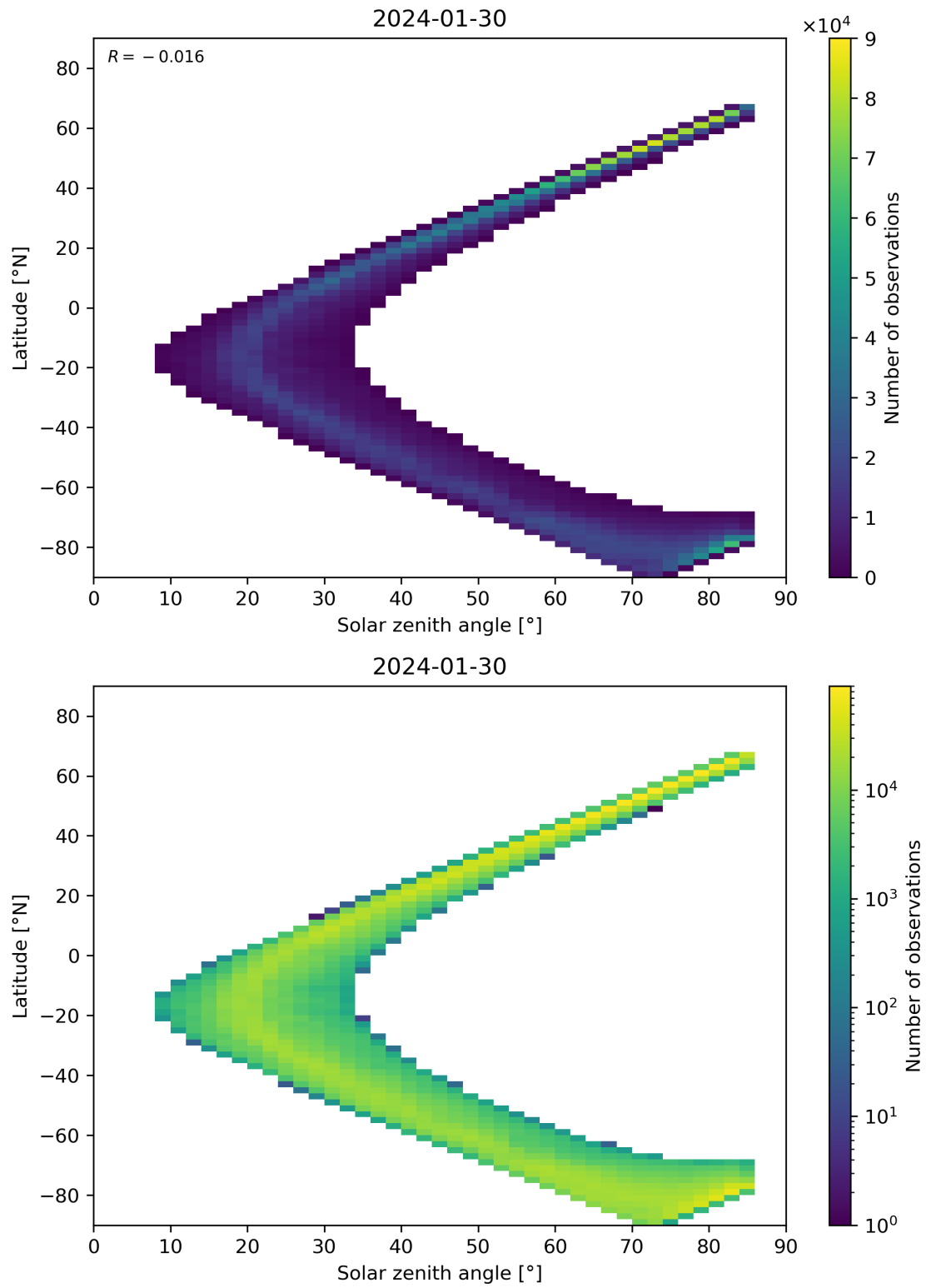
Figure 66: Scatter density plot of “Solar zenith angle” against “Latitude” for 2024-01-29 to 2024-01-31.
