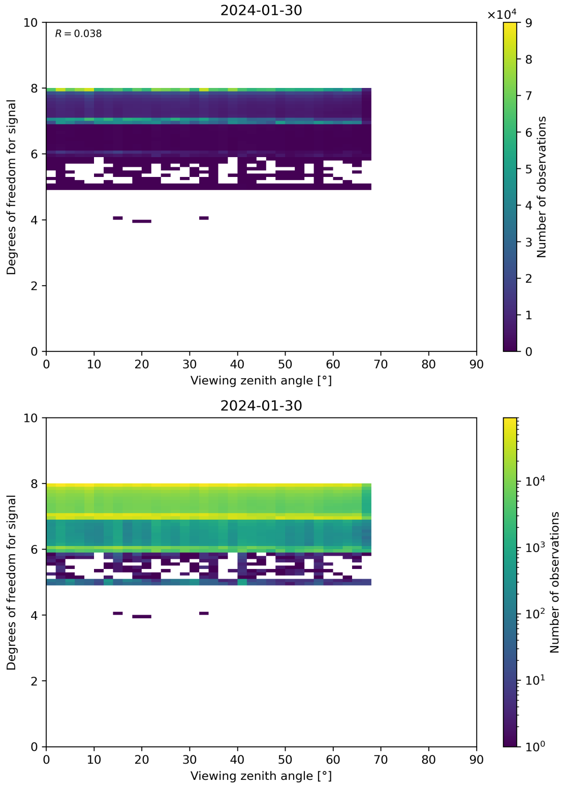
Figure 73: Scatter density plot of “Viewing zenith angle” against “Degrees of freedom for signal” for 2024-01-29 to 2024-01-31.
