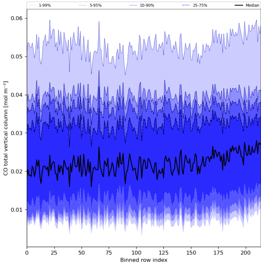
Figure 26: Along track statistics of “CO total vertical column” for 2024-01-29 to 2024-01-31
