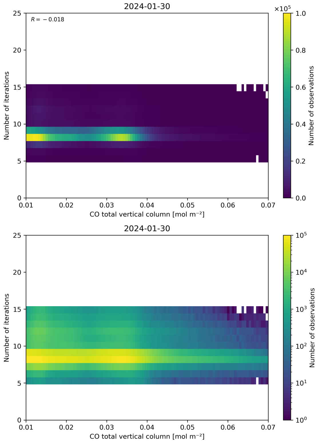
Figure 42: Scatter density plot of “CO total vertical column” against “Number of iterations” for 2024-01-29 to 2024-01-31.
