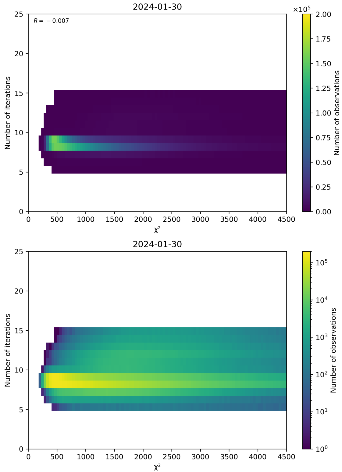
Figure 49: Scatter density plot of “ \chi^2 ” against “Number of iterations” for 2024-01-29 to 2024-01-31.
