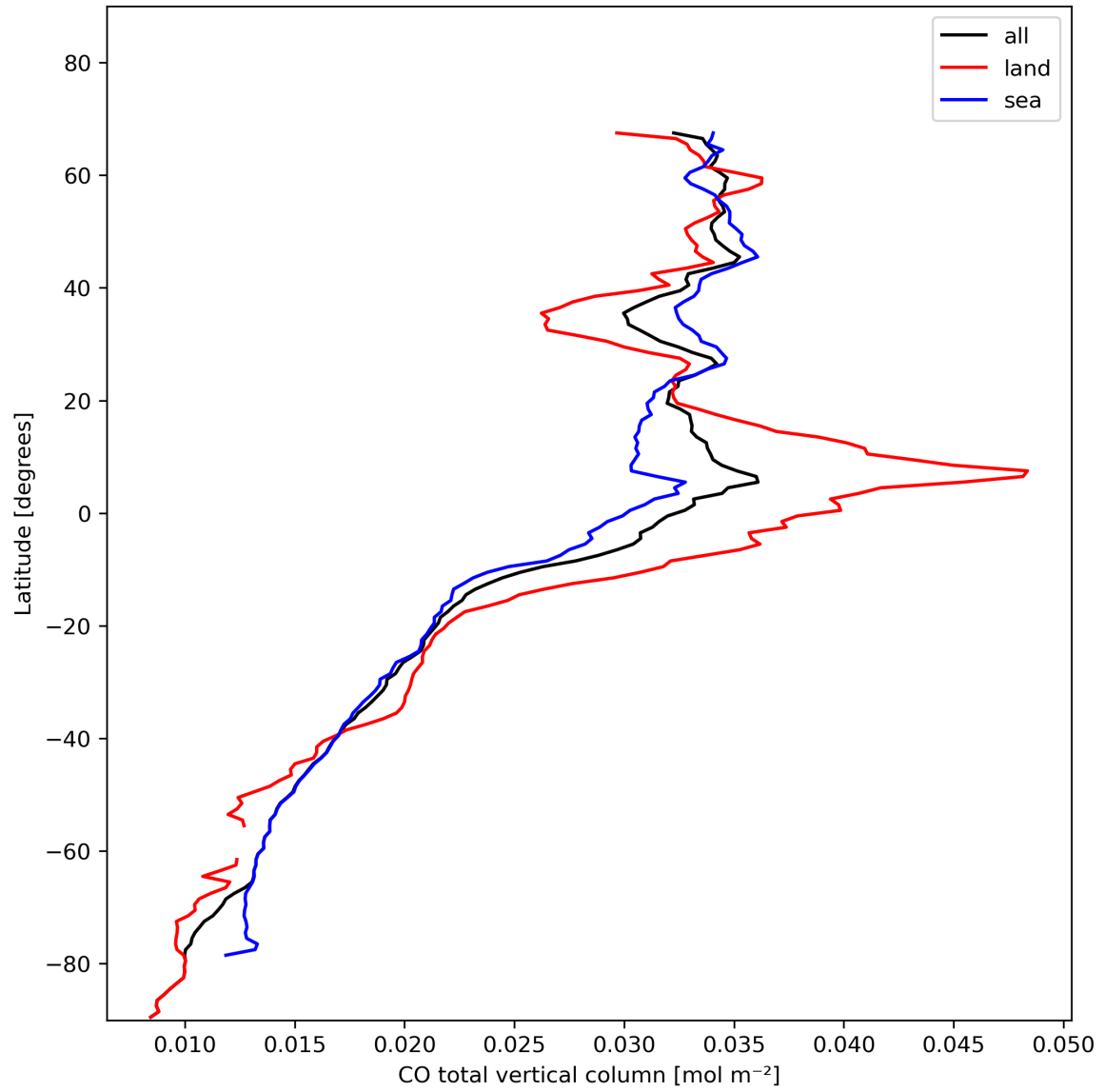
Figure 10: Zonal average of “CO total vertical column” for 2024-01-29 to 2024-01-31.
