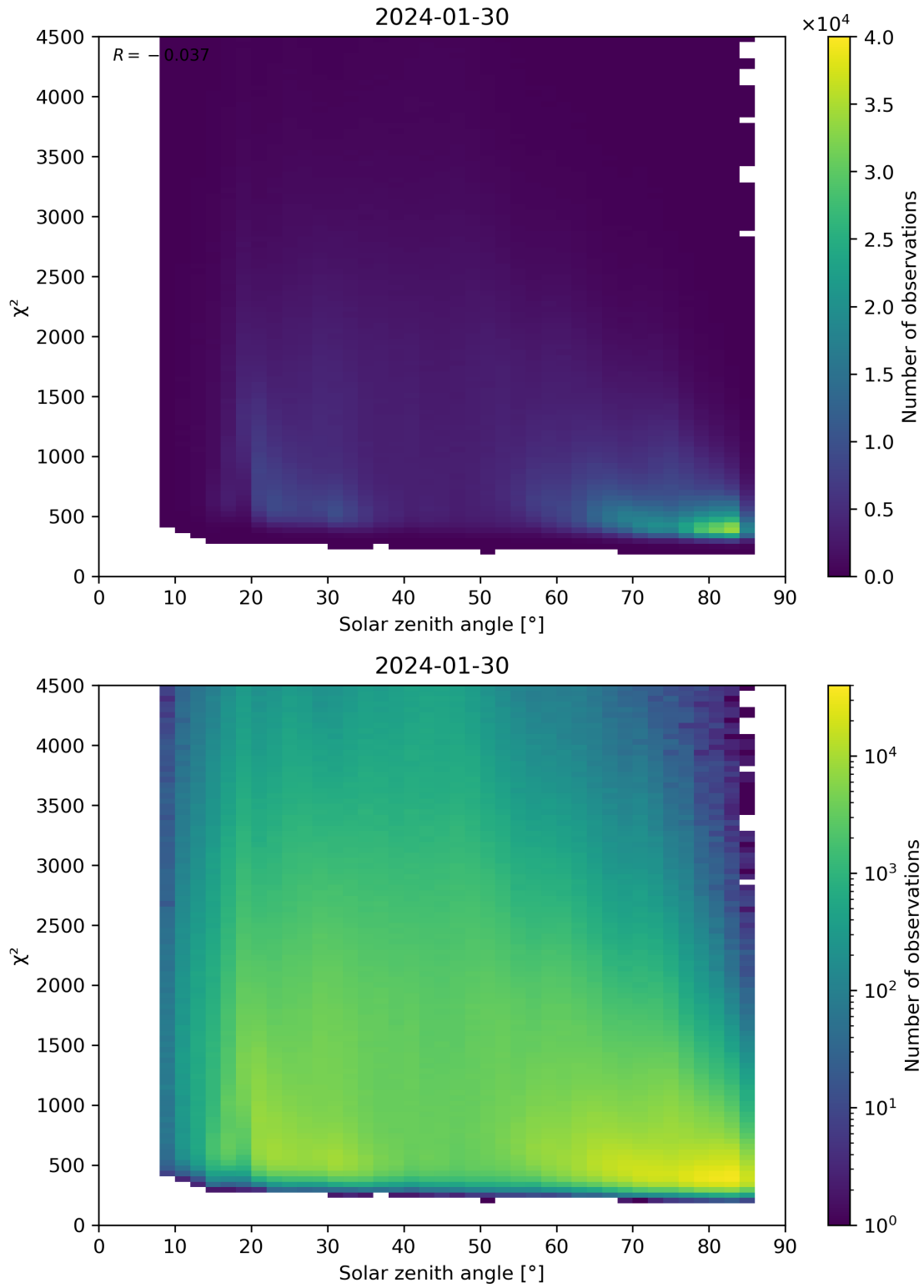
Figure 64: Scatter density plot of “Solar zenith angle” against “ \chi^2 ” for 2024-01-29 to 2024-01-31.
