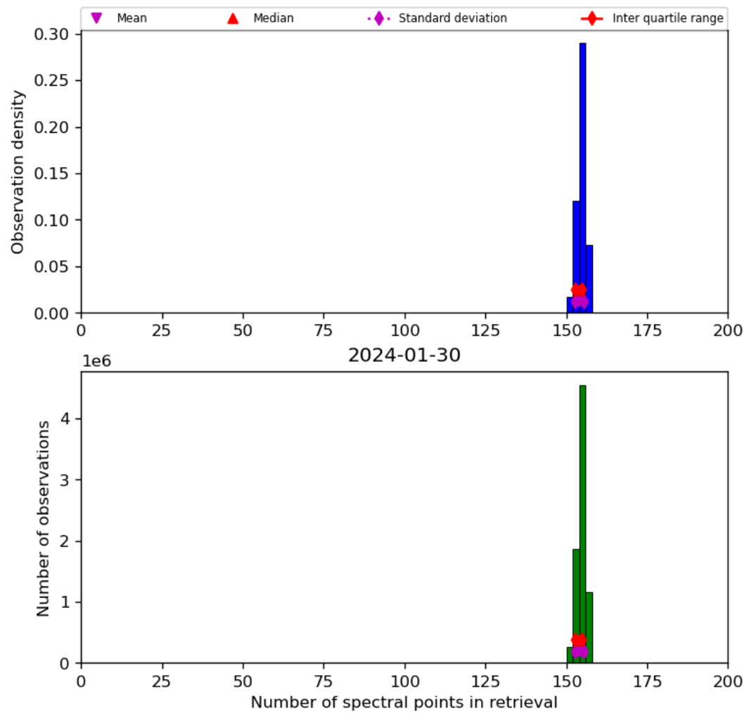
Figure 21: Histogram of “Number of spectral points in retrieval” for 2024-01-29 to 2024-01-31
