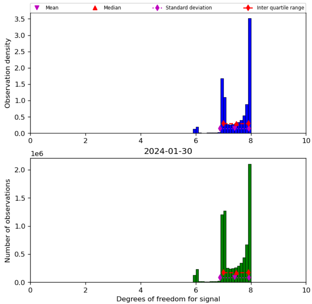
Figure 23: Histogram of “Degrees of freedom for signal” for 2024-01-29 to 2024-01-31
