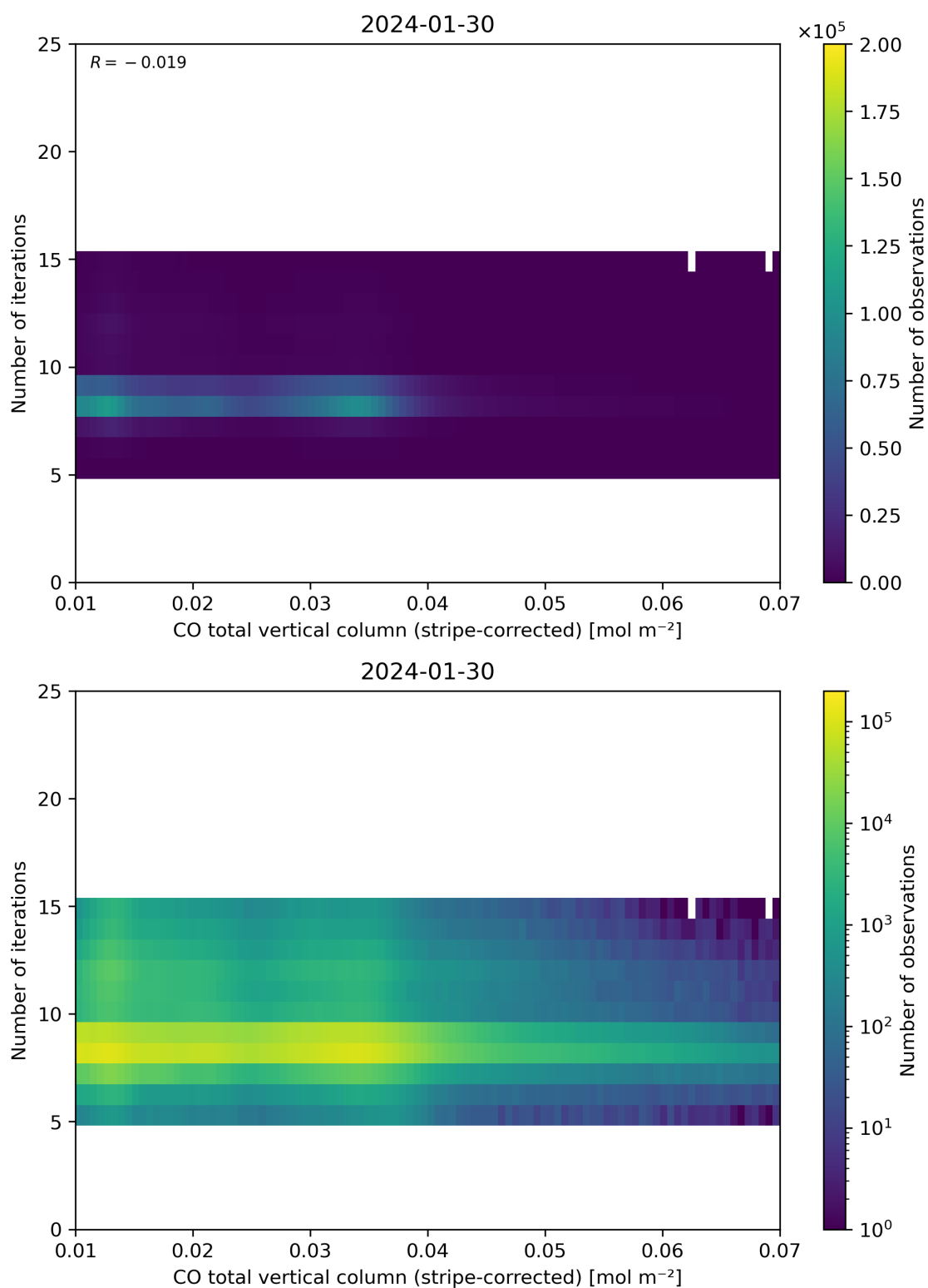
Figure 39: Scatter density plot of “CO total vertical column (stripe-corrected)” against “Number of iterations” for 2024-01-29 to 2024-01-31.
