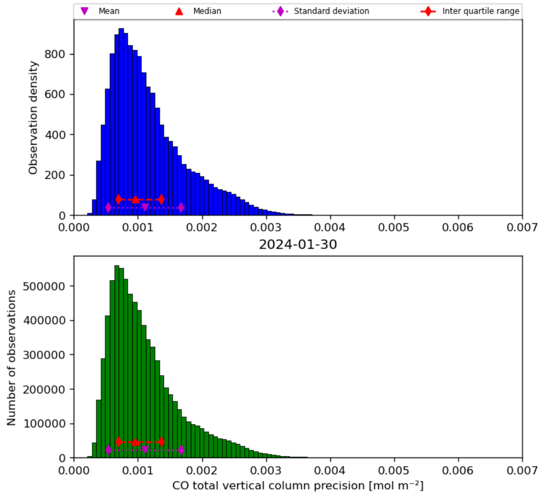
Figure 20: Histogram of “CO total vertical column precision” for 2024-01-29 to 2024-01-31
