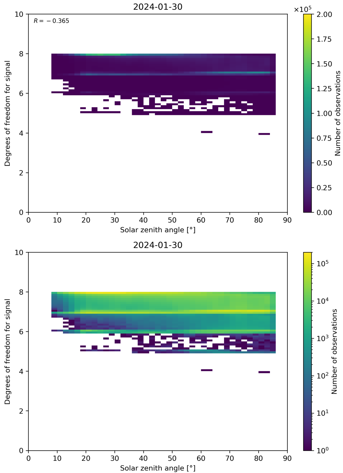
Figure 65: Scatter density plot of “Solar zenith angle” against “Degrees of freedom for signal” for 2024-01-29 to 2024-01-31.
