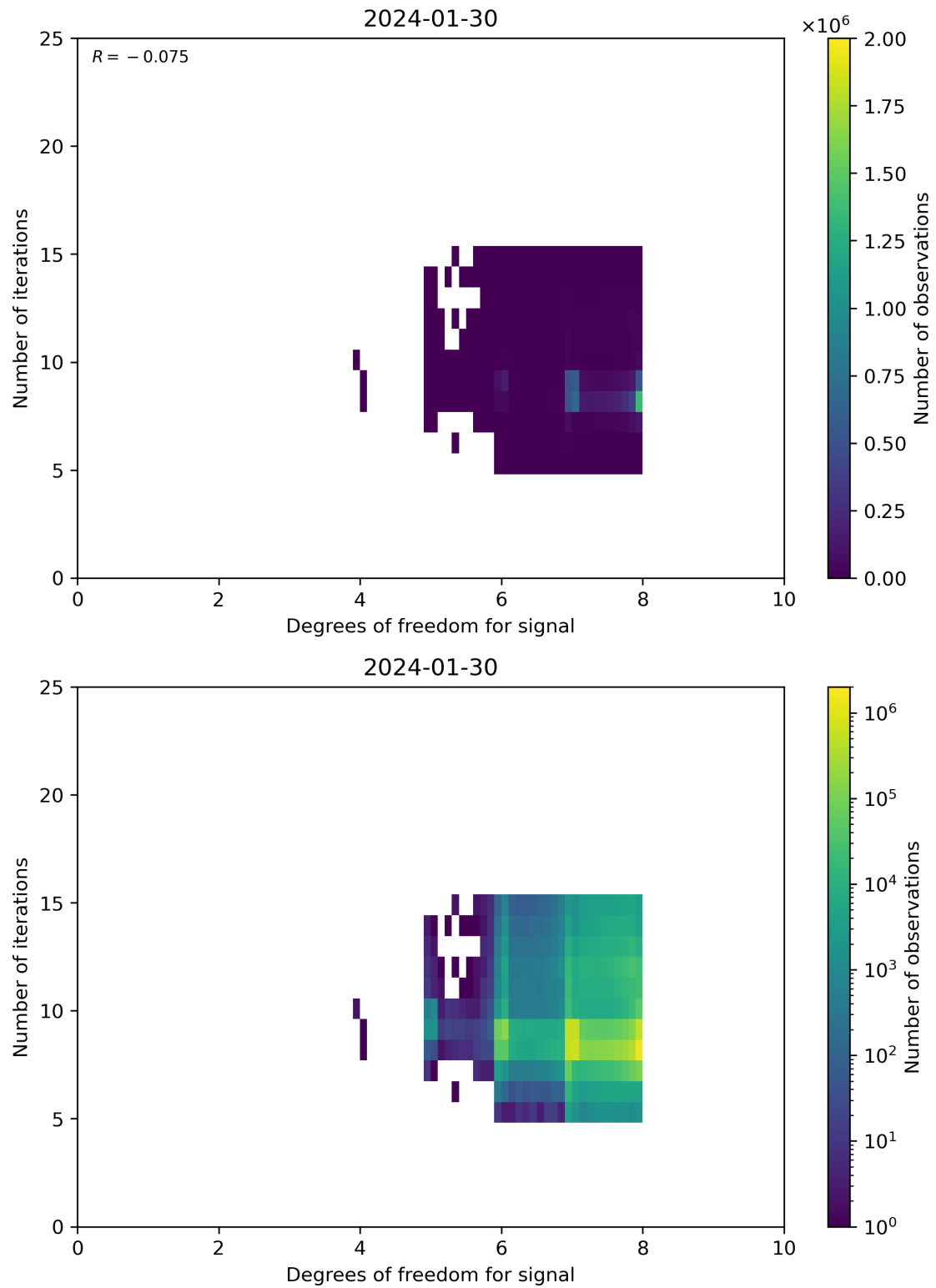
Figure 50: Scatter density plot of “Degrees of freedom for signal” against “Number of iterations” for 2024-01-29 to 2024-01-31.
