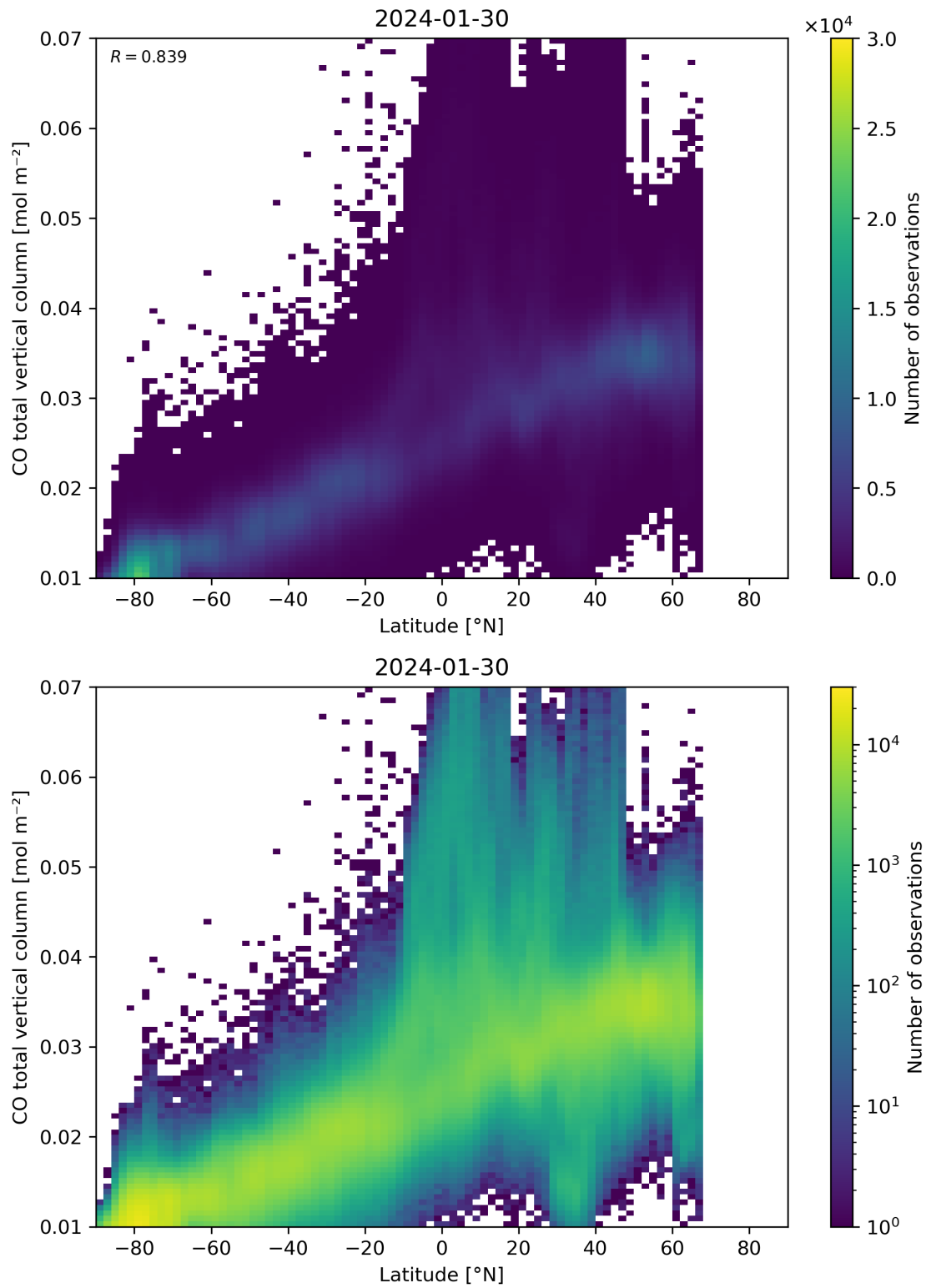
Figure 51: Scatter density plot of “Latitude” against “CO total vertical column” for 2024-01-29 to 2024-01-31.
