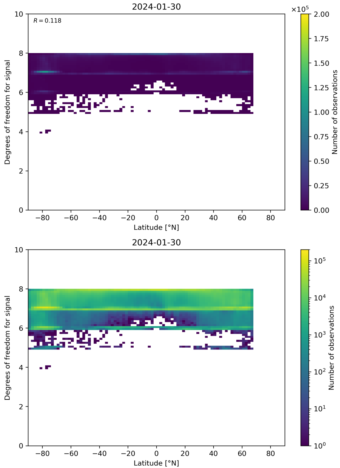
Figure 55: Scatter density plot of “Latitude” against “Degrees of freedom for signal” for 2024-01-29 to 2024-01-31.
