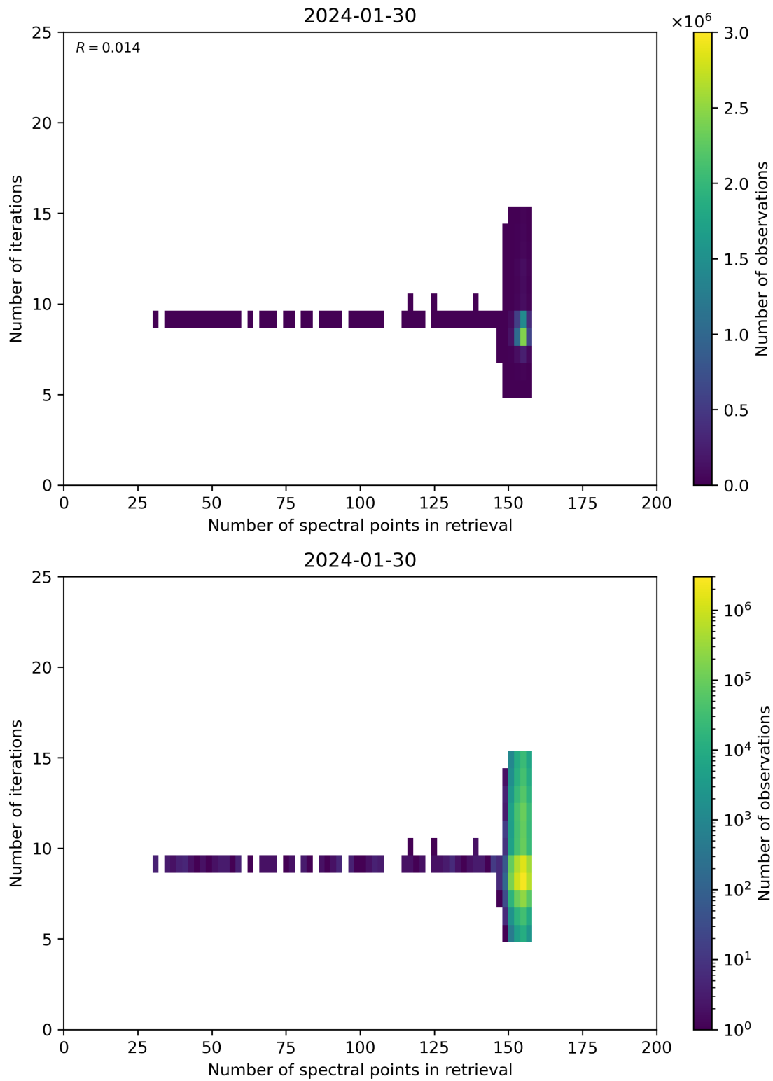
Figure 60: Scatter density plot of “Number of spectral points in retrieval” against “Number of iterations” for 2024-01-29 to 2024-01-31.
