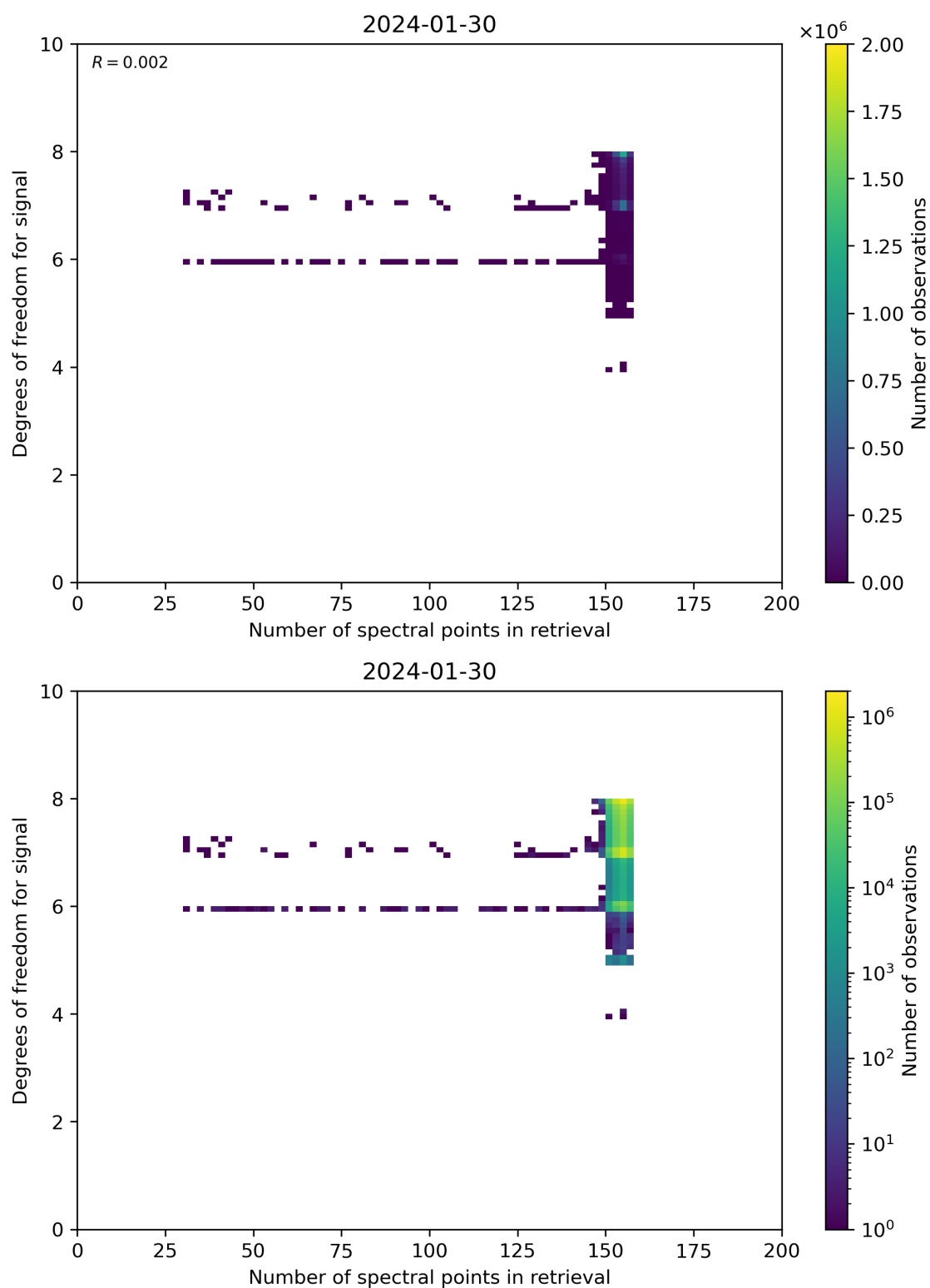
Figure 59: Scatter density plot of “Number of spectral points in retrieval” against “Degrees of freedom for signal” for 2024-01-29 to 2024-01-31.
