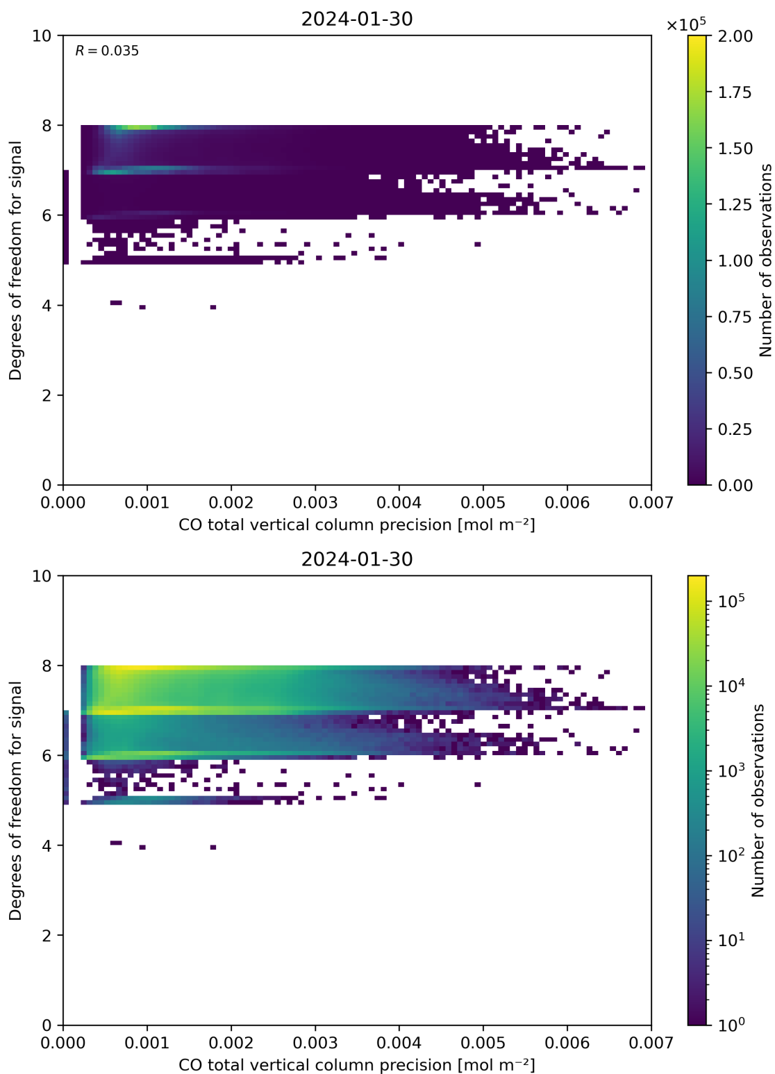
Figure 45: Scatter density plot of “CO total vertical column precision” against “Degrees of freedom for signal” for 2024-01-29 to 2024-01-31.
