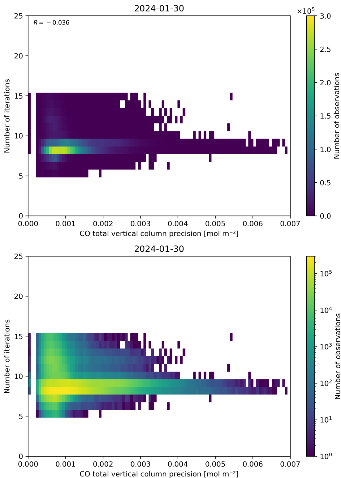
Figure 46: Scatter density plot of “CO total vertical column precision” against “Number of iterations” for 2024-01-29 to 2024-01-31.
