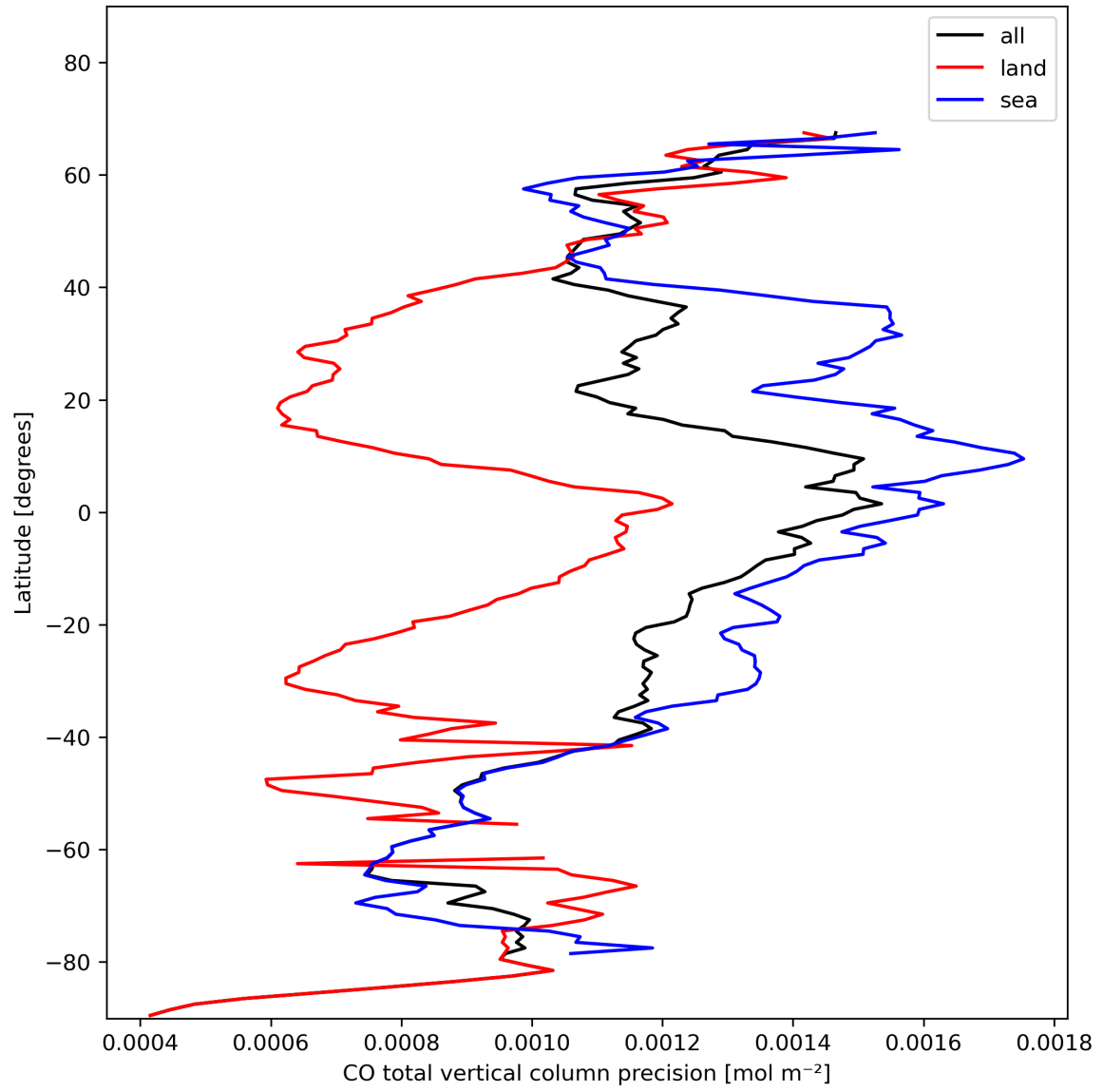
Figure 12: Zonal average of “CO total vertical column precision” for 2024-01-29 to 2024-01-31.
