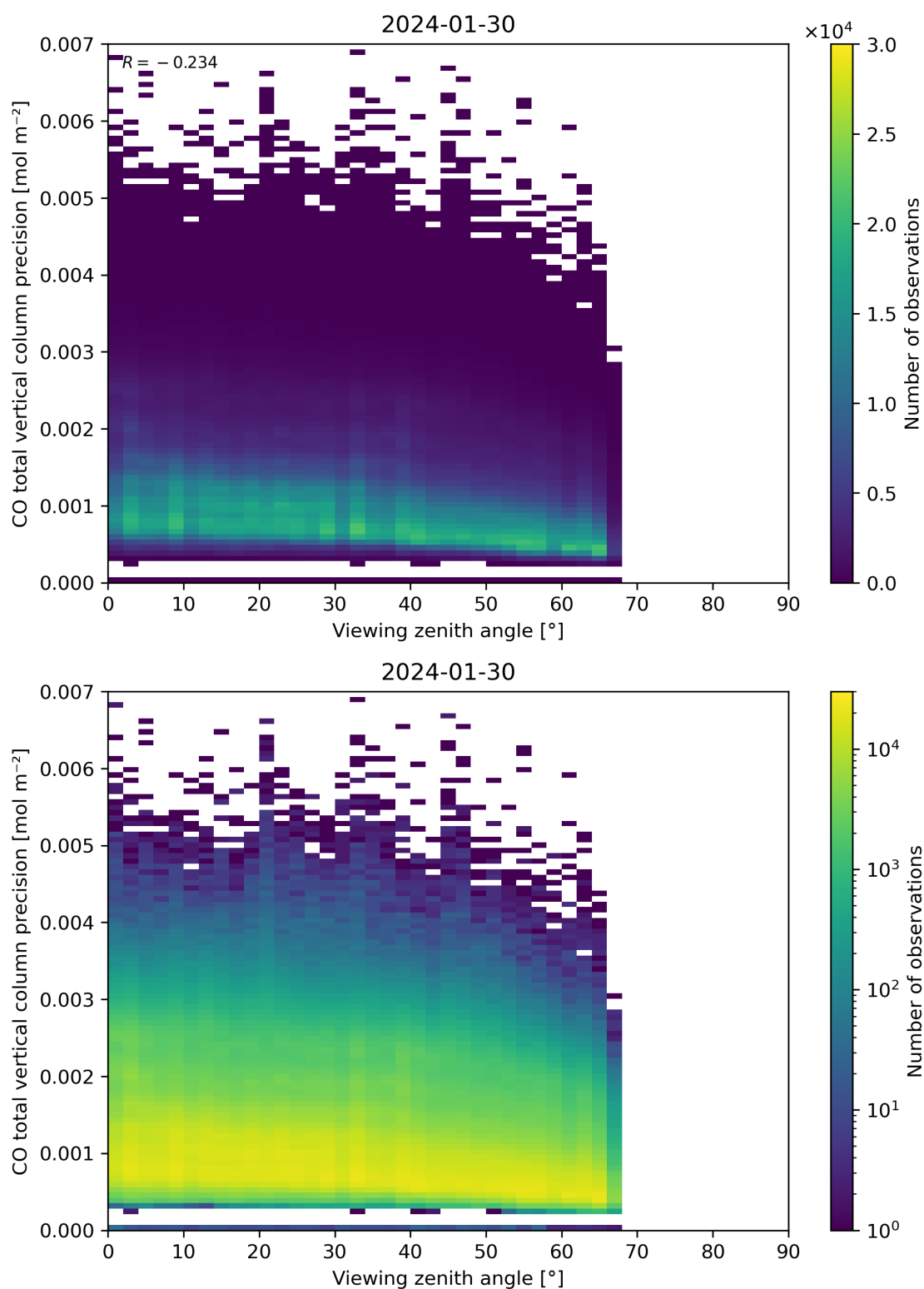
Figure 71: Scatter density plot of “Viewing zenith angle” against “CO total vertical column precision” for 2024-01-29 to 2024-01-31.
