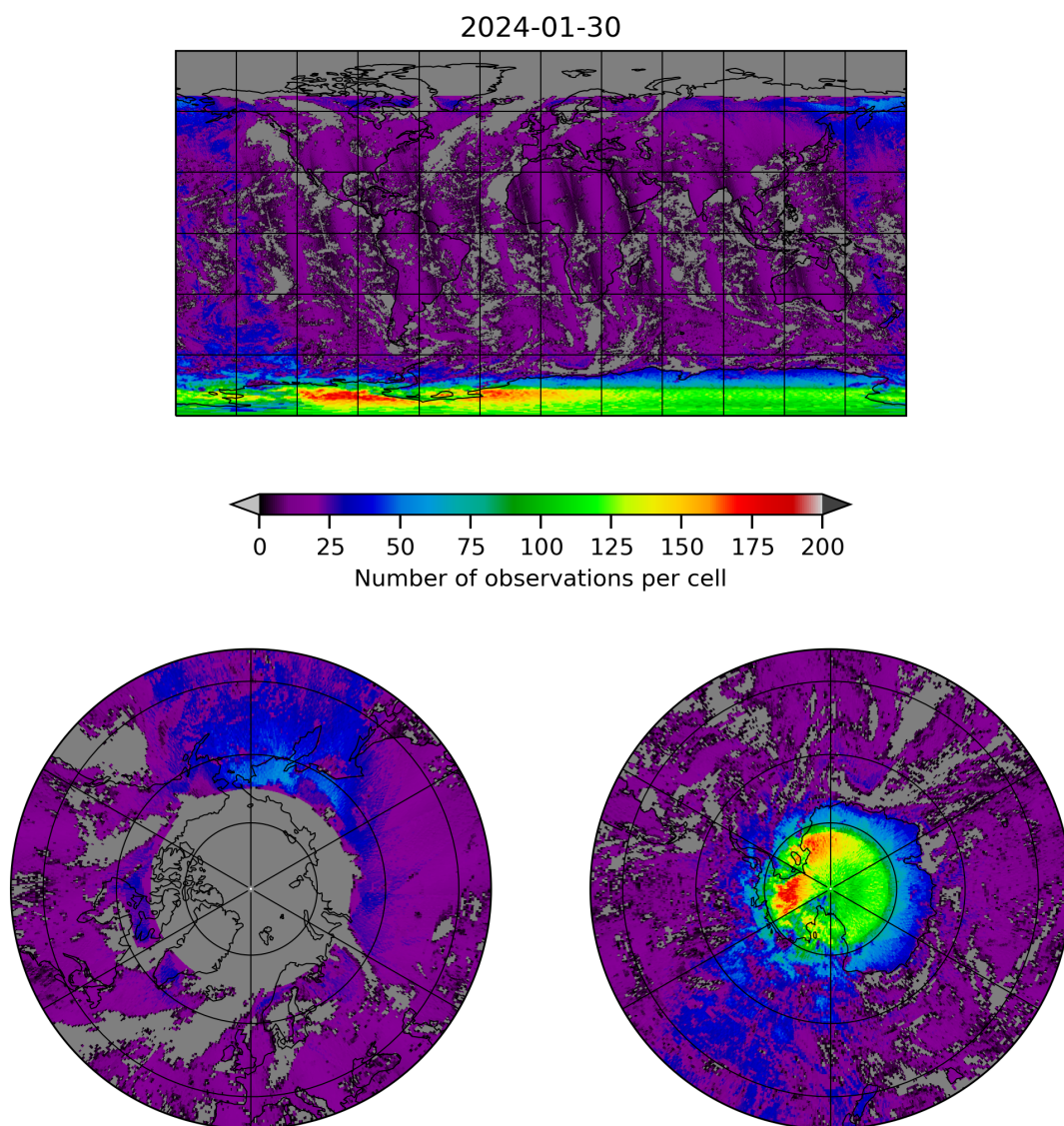
Figure 8: Map of the number of observations for 2024-01-29 to 2024-01-31
