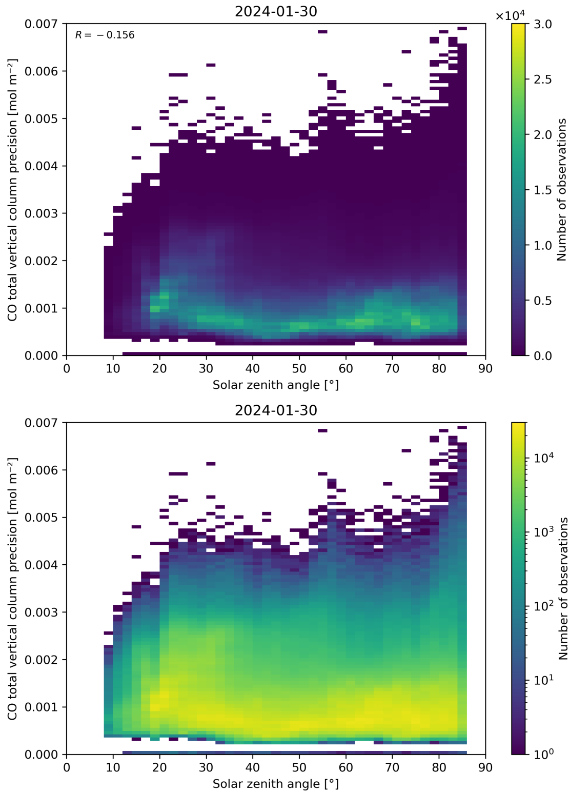
Figure 63: Scatter density plot of “Solar zenith angle” against “CO total vertical column precision” for 2024-01-29 to 2024-01-31.
