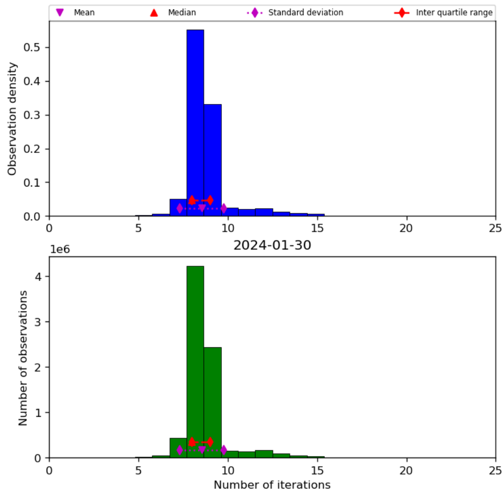
Figure 24: Histogram of “Number of iterations” for 2024-01-29 to 2024-01-31
