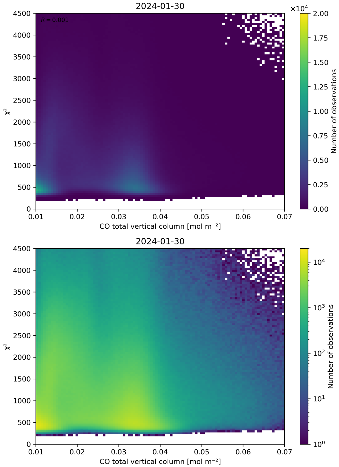
Figure 35: Scatter density plot of “CO total vertical column” against “ \chi^2 ” for 2024-01-29 to 2024-01-31.
