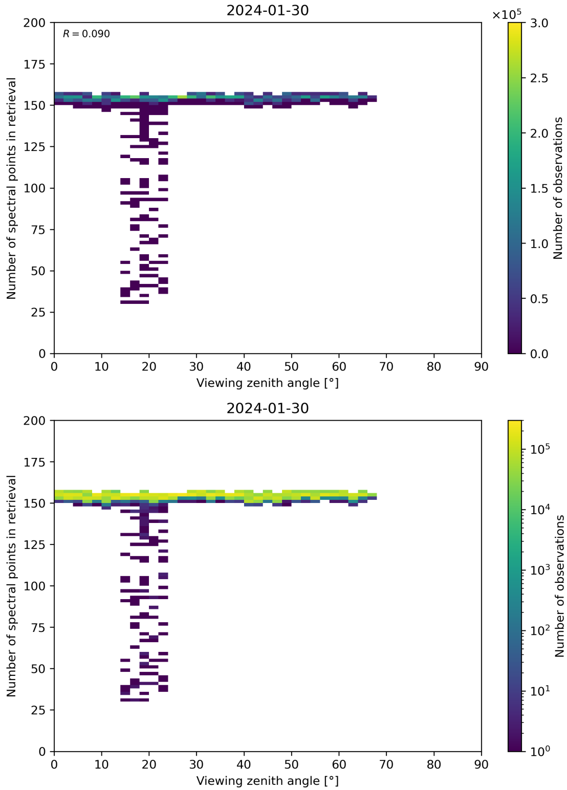
Figure 76: Scatter density plot of “Viewing zenith angle” against “Number of spectral points in retrieval” for 2024-01-29 to 2024-01-31.
