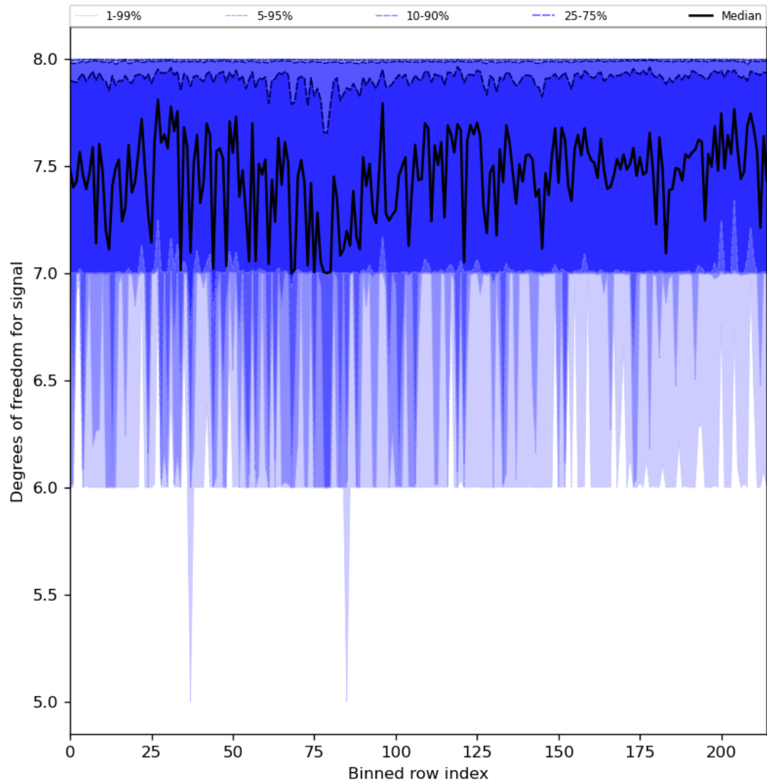
Figure 31: Along track statistics of “Degrees of freedom for signal” for 2024-01-29 to 2024-01-31
