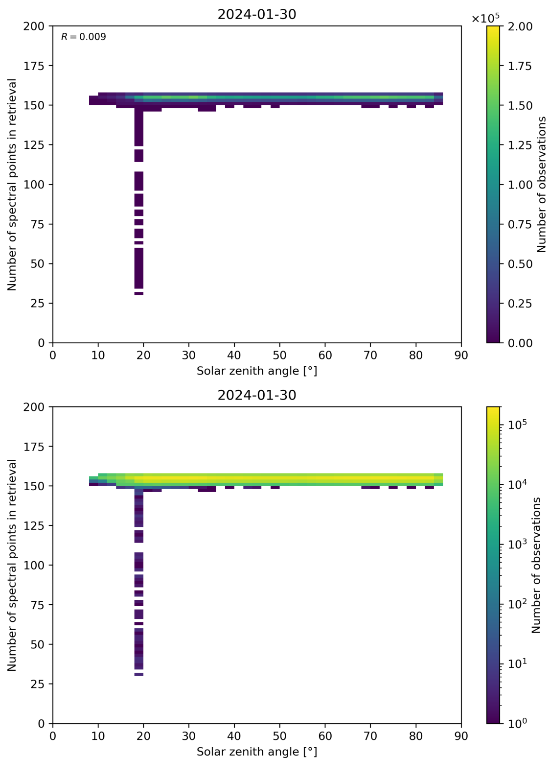
Figure 68: Scatter density plot of “Solar zenith angle” against “Number of spectral points in retrieval” for 2024-01-29 to 2024-01-31.
