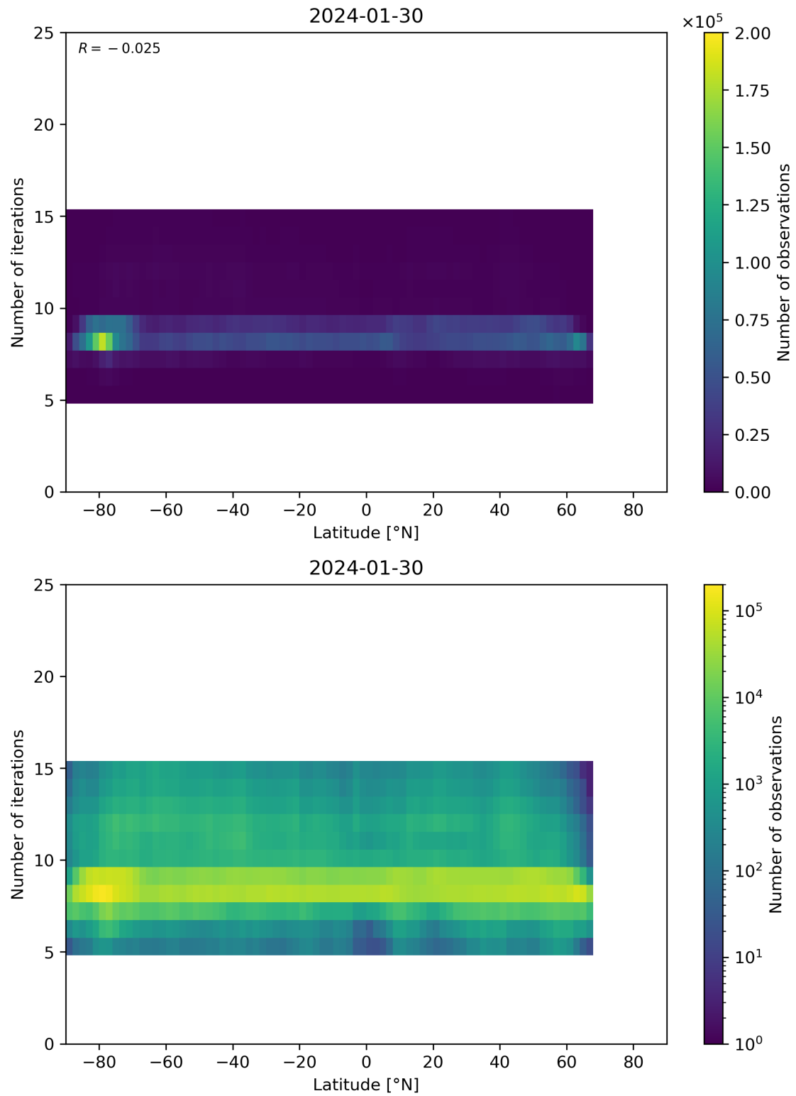
Figure 56: Scatter density plot of “Latitude” against “Number of iterations” for 2024-01-29 to 2024-01-31.
