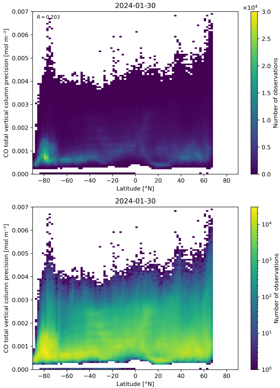
Figure 53: Scatter density plot of “Latitude” against “CO total vertical column precision” for 2024-01-29 to 2024-01-31.
