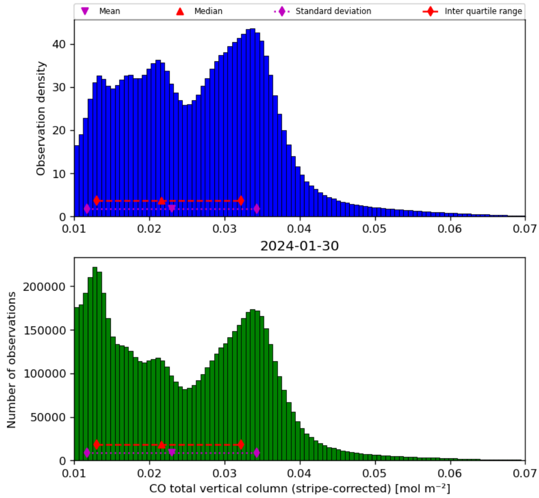
Figure 19: Histogram of “CO total vertical column (stripe-corrected)” for 2024-01-29 to 2024-01-31
