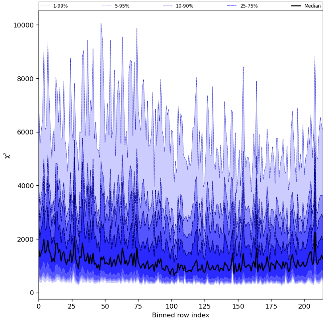
Figure 30: Along track statistics of “ \chi^2 ” for 2024-01-29 to 2024-01-31
