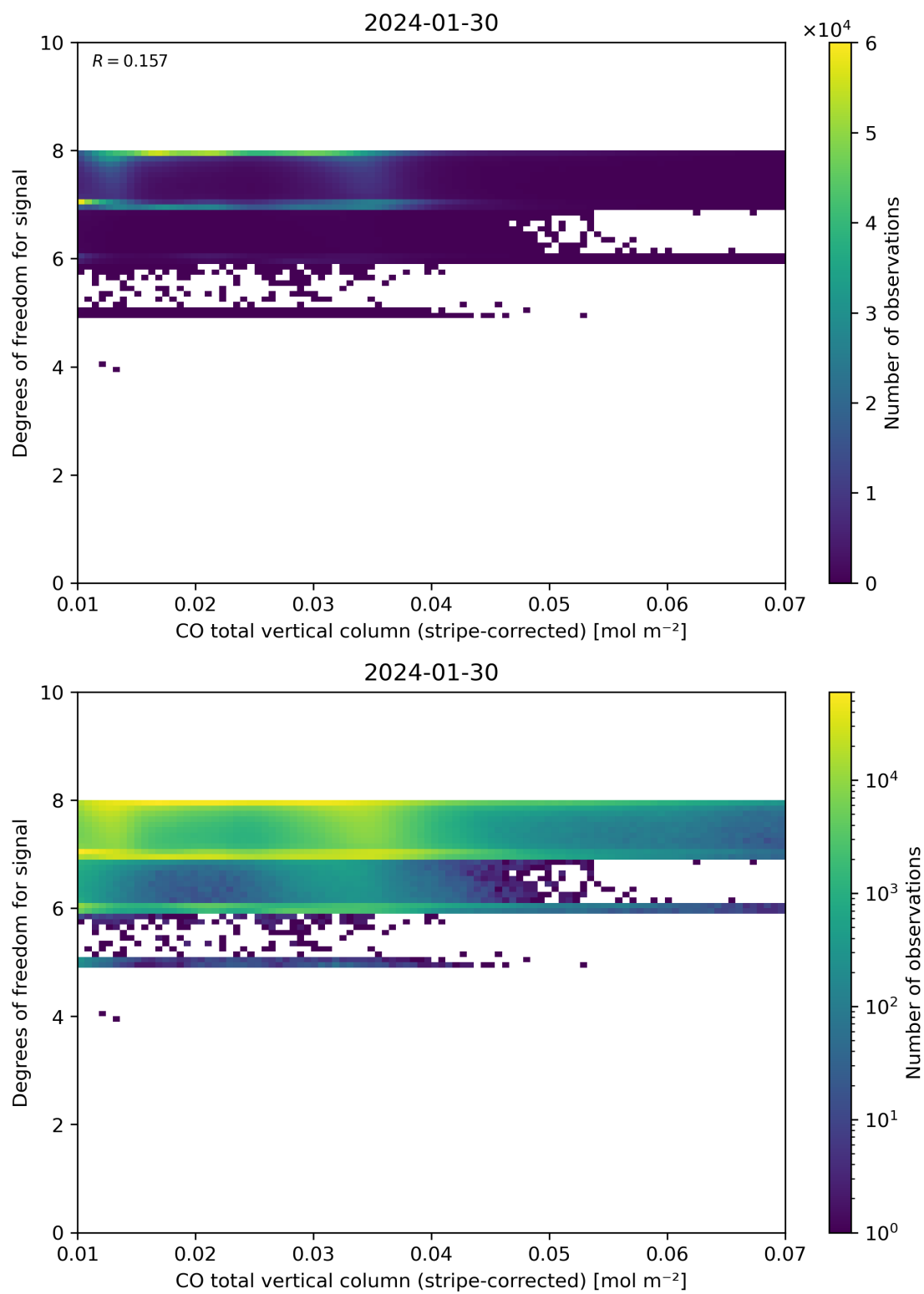
Figure 38: Scatter density plot of “CO total vertical column (stripe-corrected)” against “Degrees of freedom for signal” for 2024-01-29 to 2024-01-31.
