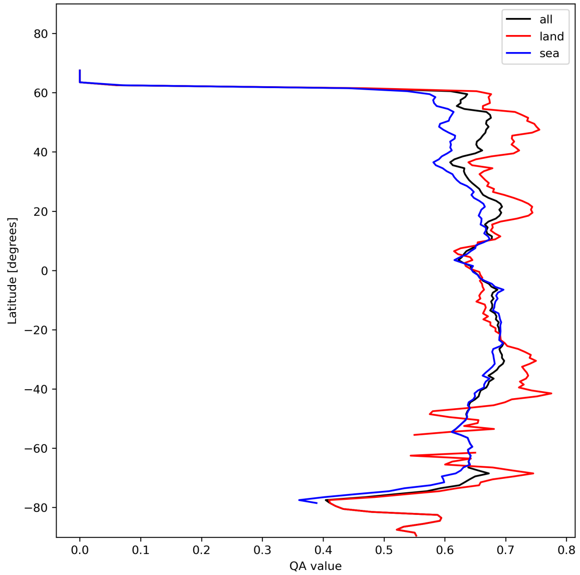
Figure 9: Zonal average of “QA value” for 2024-01-29 to 2024-01-31.
