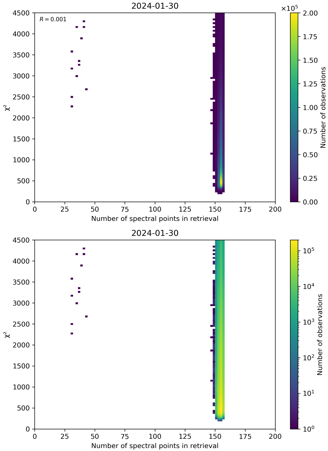
Figure 58: Scatter density plot of “Number of spectral points in retrieval” against “ \chi^2 ” for 2024-01-29 to 2024-01-31.
