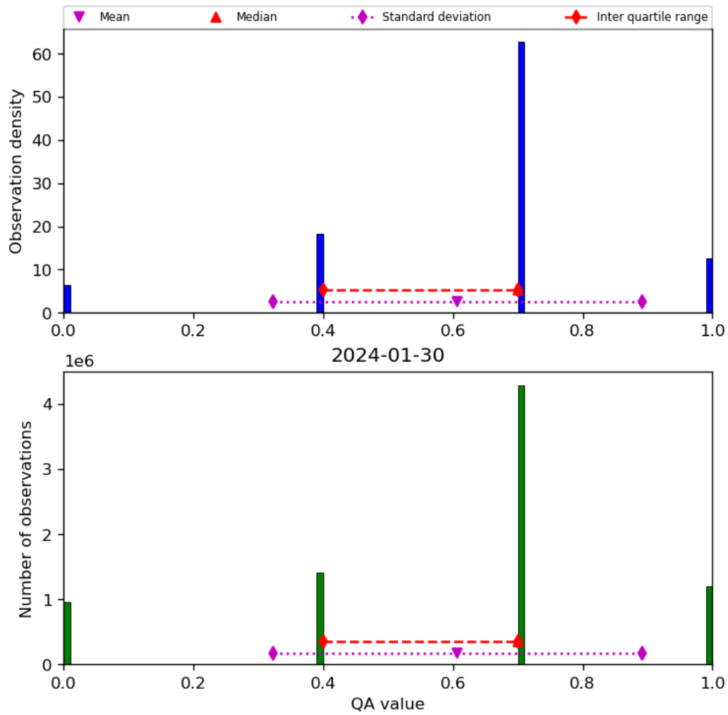
Figure 17: Histogram of “QA value” for 2024-01-29 to 2024-01-31
