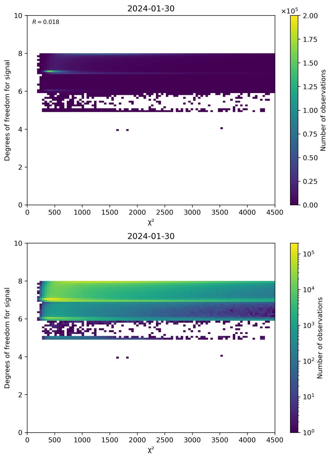
Figure 48: Scatter density plot of “ \chi^2 ” against “Degrees of freedom for signal” for 2024-01-29 to 2024-01-31.
