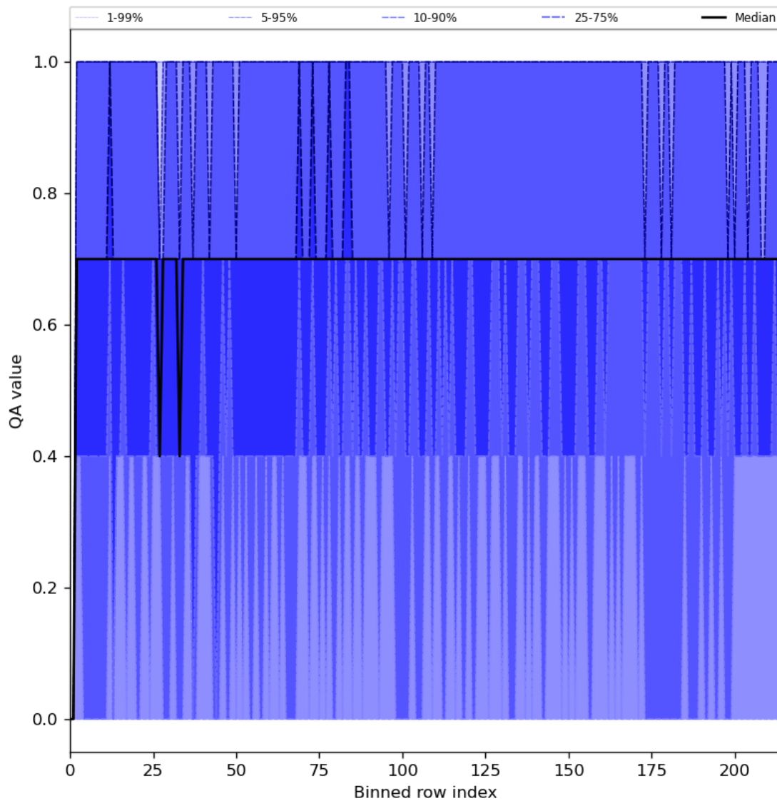
Figure 25: Along track statistics of “QA value” for 2024-01-29 to 2024-01-31
