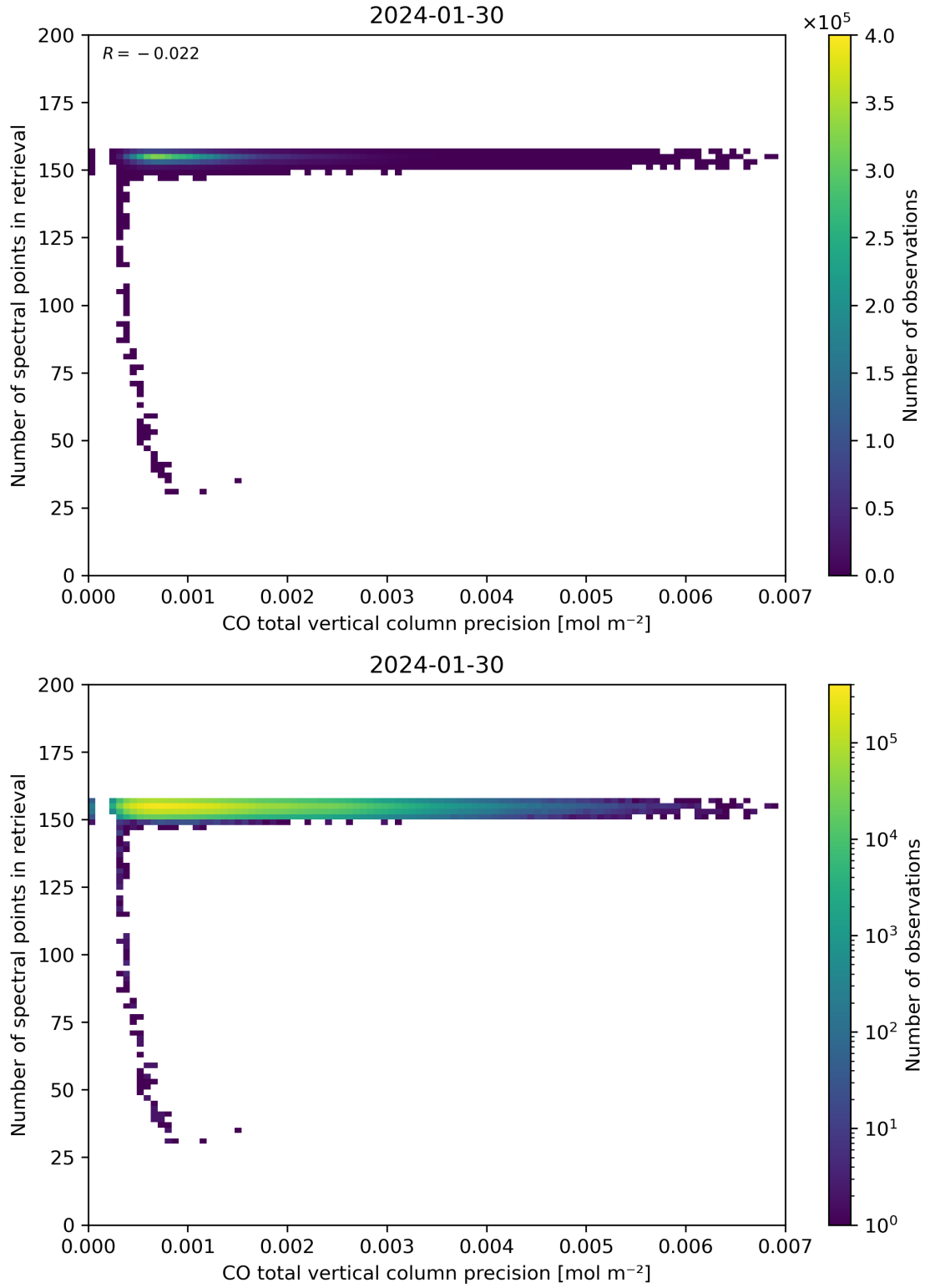
Figure 47: Scatter density plot of “CO total vertical column precision” against “Number of spectral points in retrieval” for 2024-01-29 to 2024-01-31.
