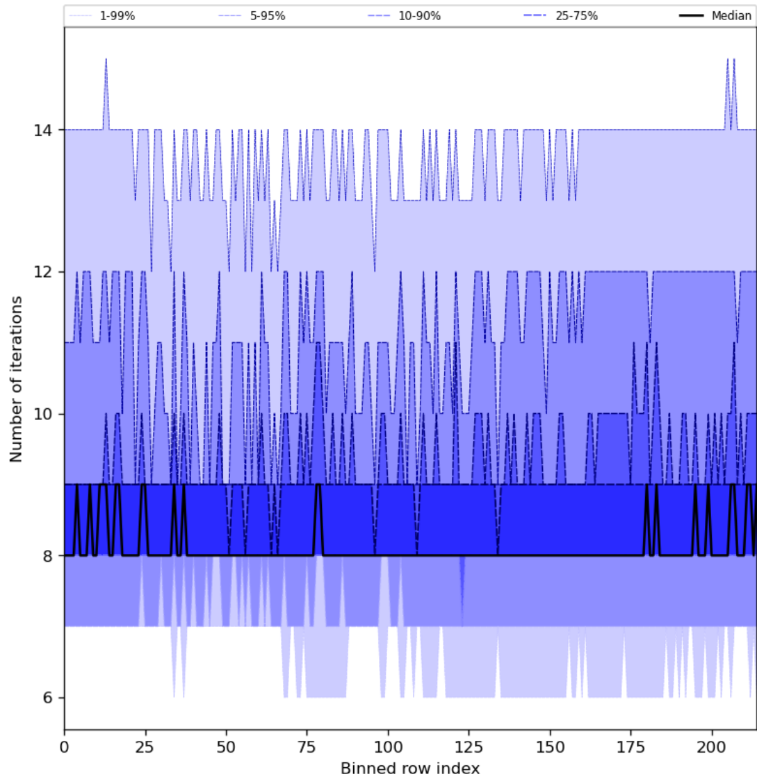
Figure 32: Along track statistics of “Number of iterations” for 2024-01-29 to 2024-01-31
