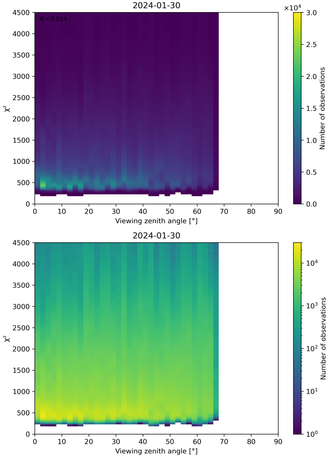
Figure 72: Scatter density plot of “Viewing zenith angle” against “ \chi^2 ” for 2024-01-29 to 2024-01-31.
