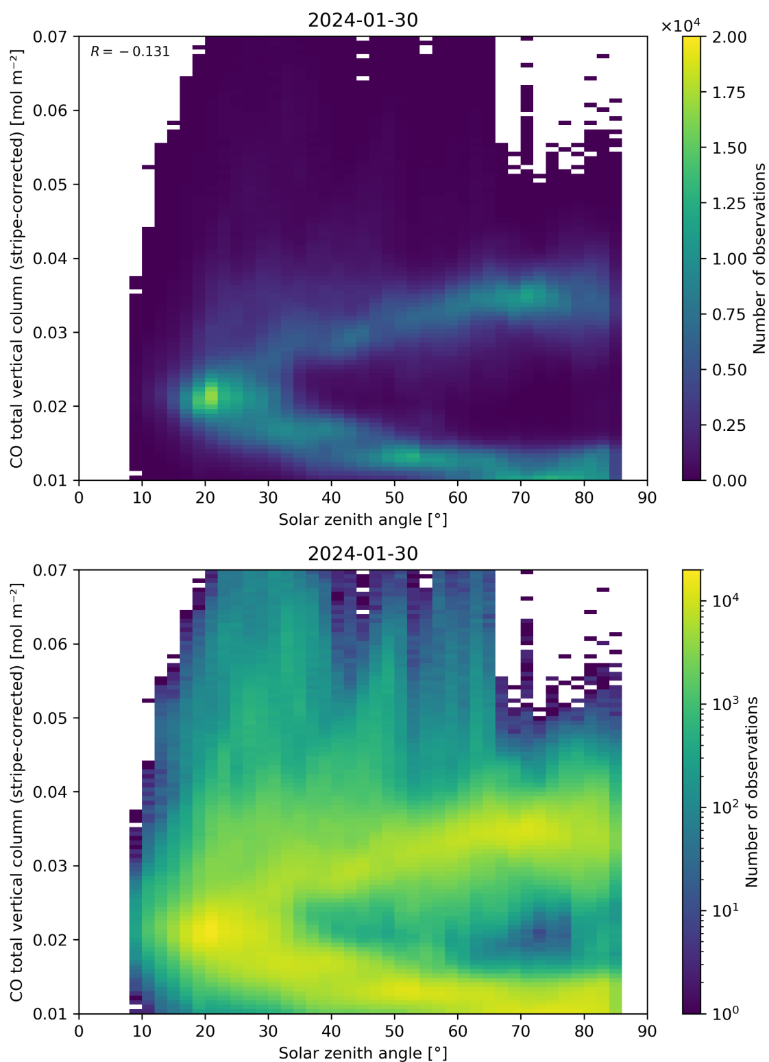
Figure 62: Scatter density plot of “Solar zenith angle” against “CO total vertical column (stripe-corrected)” for 2024-01-29 to 2024-01-31.
