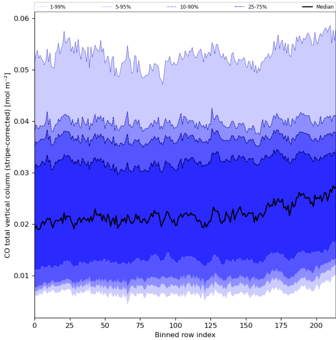
Figure 27: Along track statistics of “CO total vertical column (stripe-corrected)” for 2024-01-29 to 2024-01-31
