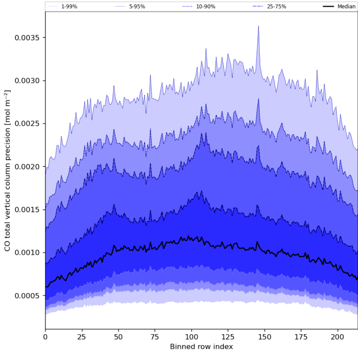
Figure 28: Along track statistics of “CO total vertical column precision” for 2024-01-29 to 2024-01-31
