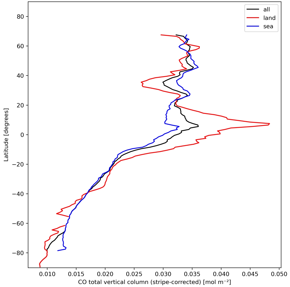
Figure 11: Zonal average of “CO total vertical column (stripe-corrected)” for 2024-01-29 to 2024-01-31.
