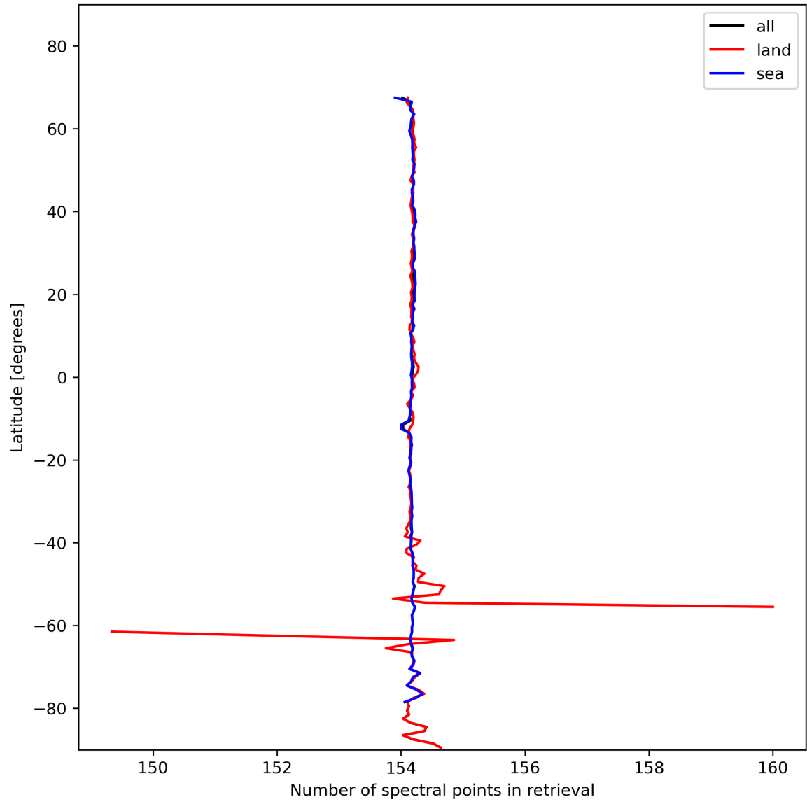
Figure 13: Zonal average of “Number of spectral points in retrieval” for 2024-01-29 to 2024-01-31.
