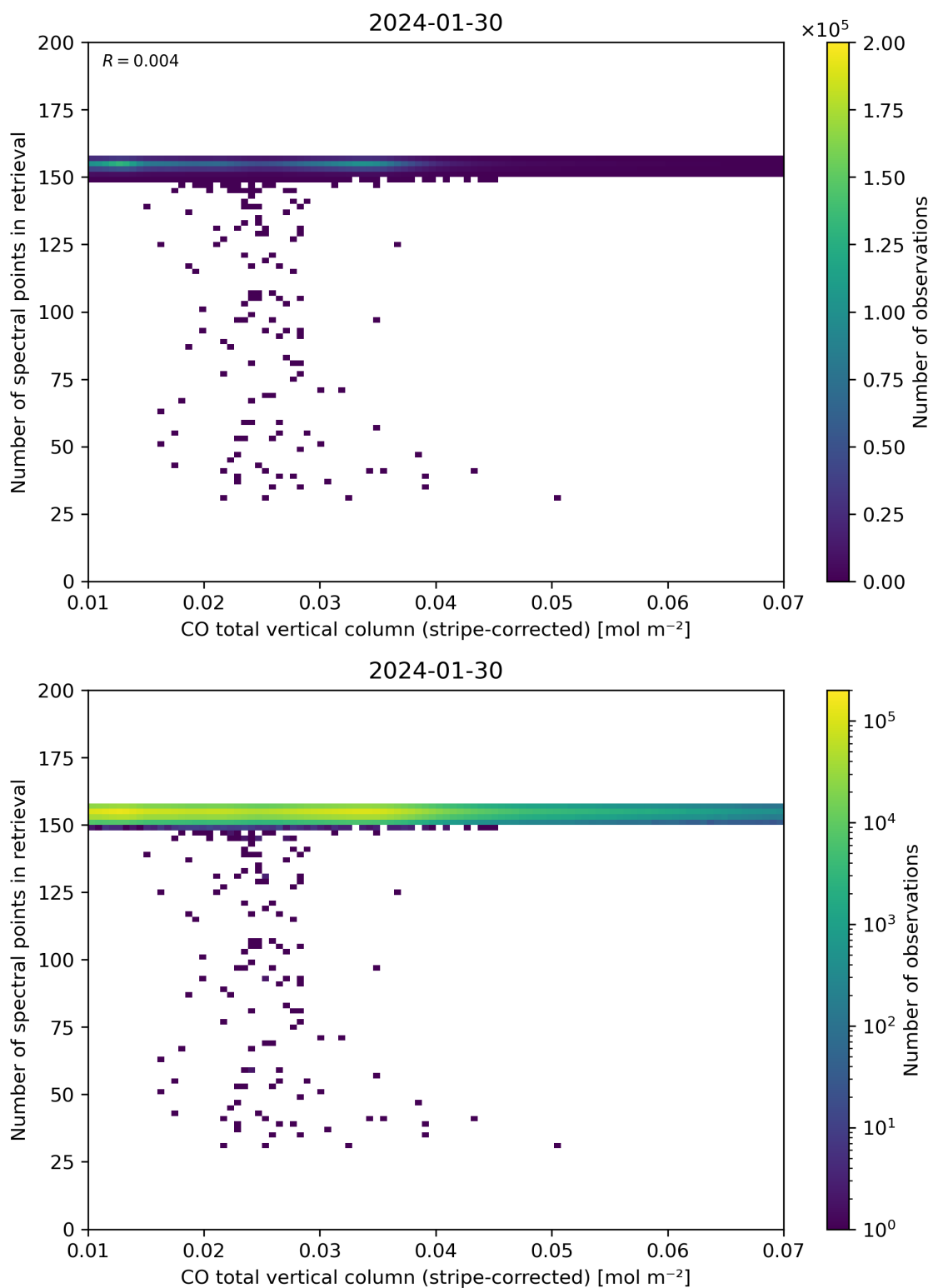
Figure 40: Scatter density plot of “CO total vertical column (stripe-corrected)” against “Number of spectral points in retrieval” for 2024-01-29 to 2024-01-31.
