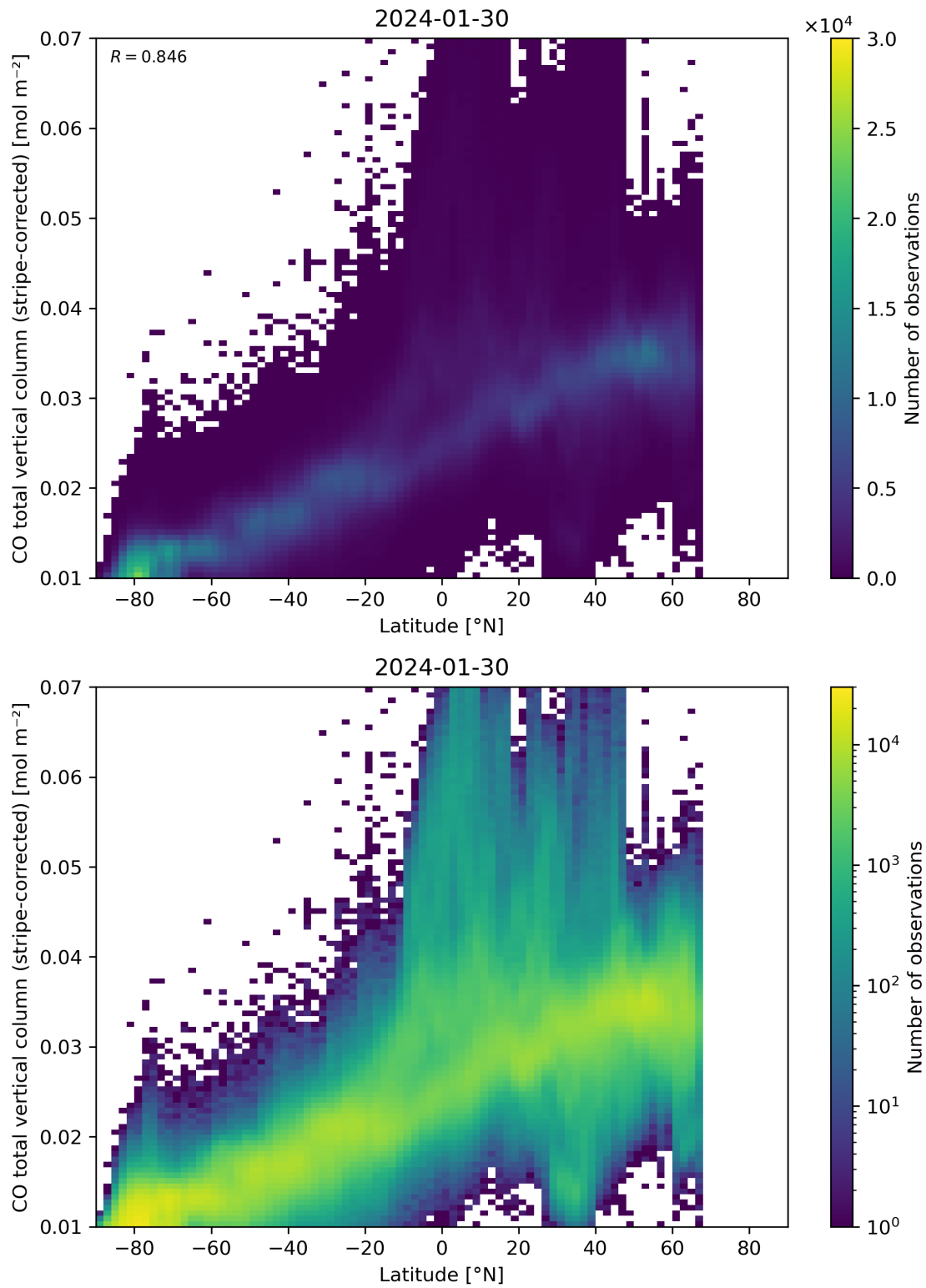
Figure 52: Scatter density plot of “Latitude” against “CO total vertical column (stripe-corrected)” for 2024-01-29 to 2024-01-31.
