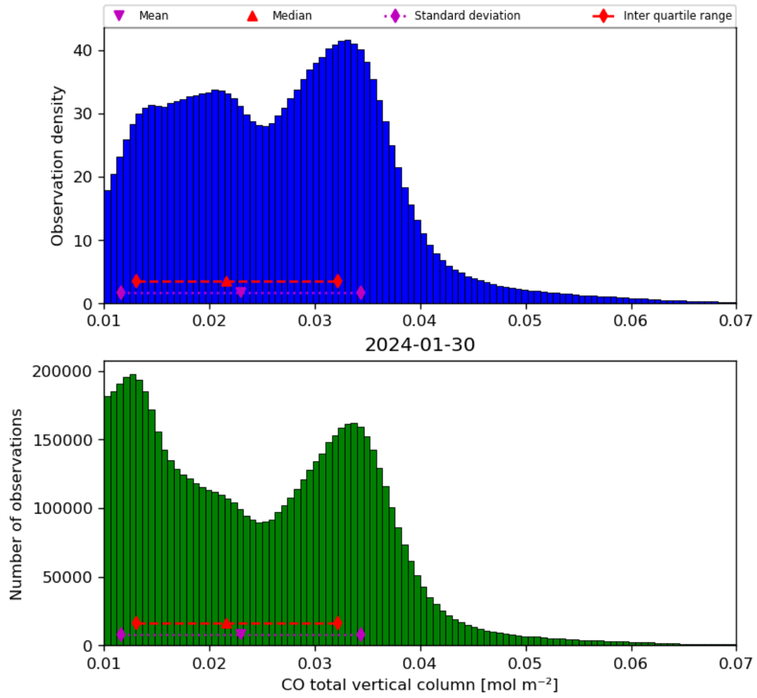
Figure 18: Histogram of “CO total vertical column” for 2024-01-29 to 2024-01-31
