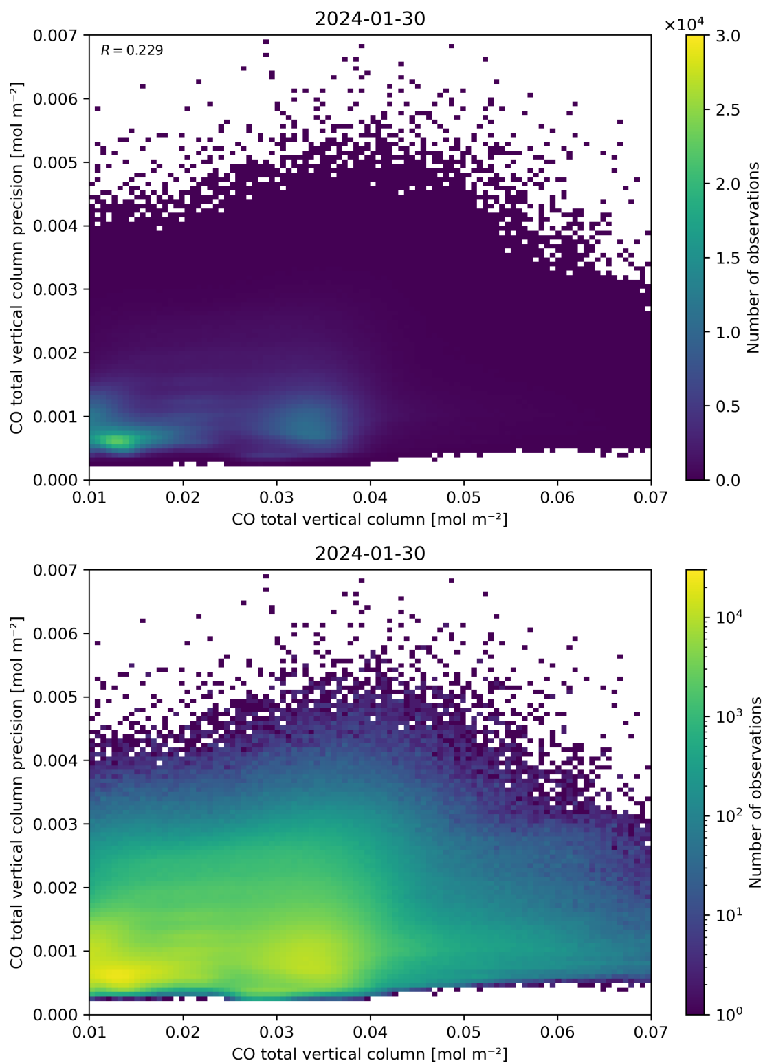
Figure 34: Scatter density plot of “CO total vertical column” against “CO total vertical column precision” for 2024-01-29 to 2024-01-31.
