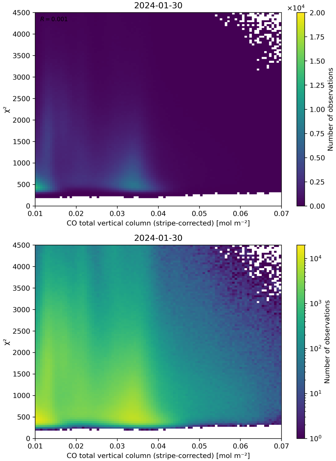
Figure 37: Scatter density plot of “CO total vertical column (stripe-corrected)” against “ \chi^2 ” for 2024-01-29 to 2024-01-31.
