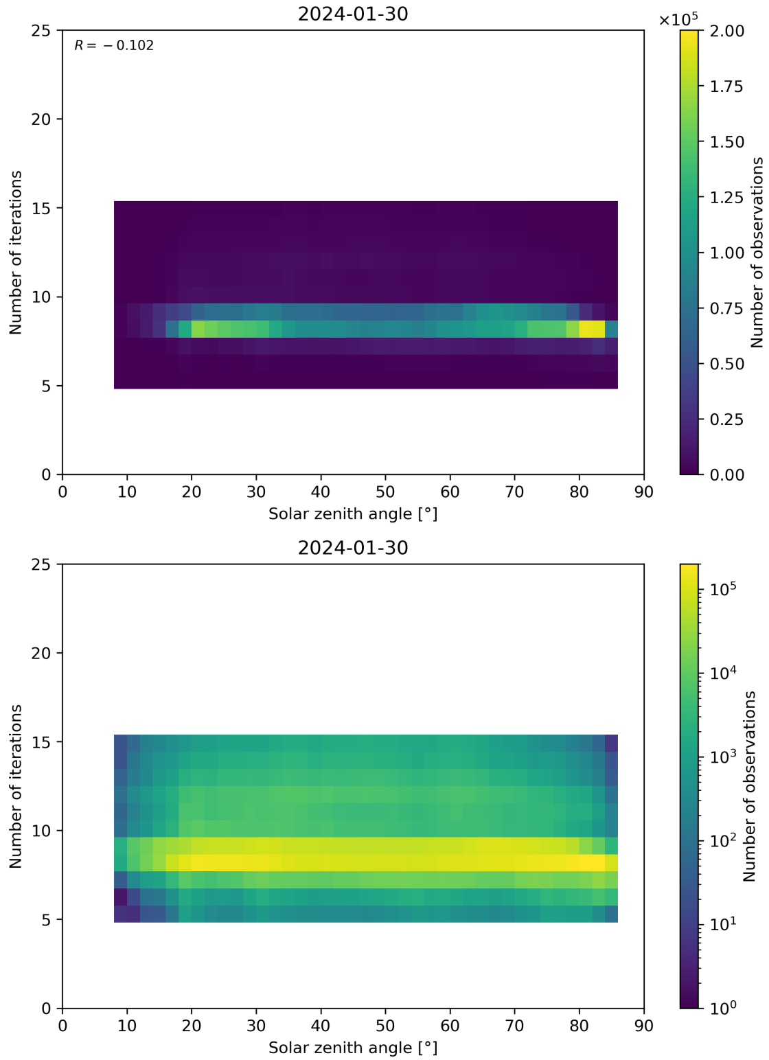
Figure 67: Scatter density plot of “Solar zenith angle” against “Number of iterations” for 2024-01-29 to 2024-01-31.
