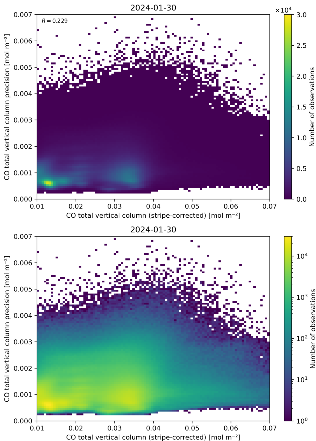
Figure 36: Scatter density plot of “CO total vertical column (stripe-corrected)” against “CO total vertical column precision” for 2024-01-29 to 2024-01-31.
