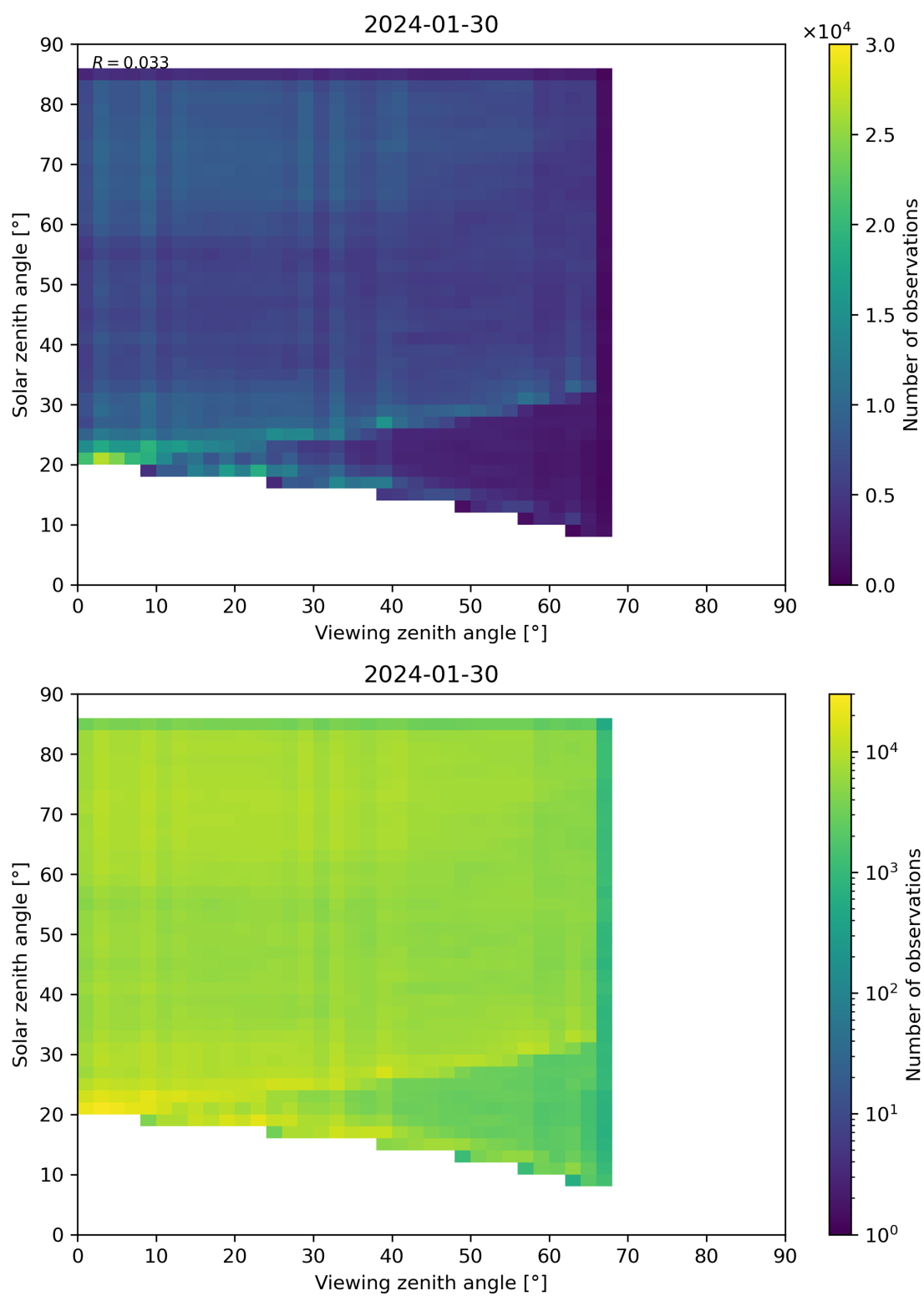
Figure 77: Scatter density plot of “Viewing zenith angle” against “Solar zenith angle” for 2024-01-29 to 2024-01-31.
