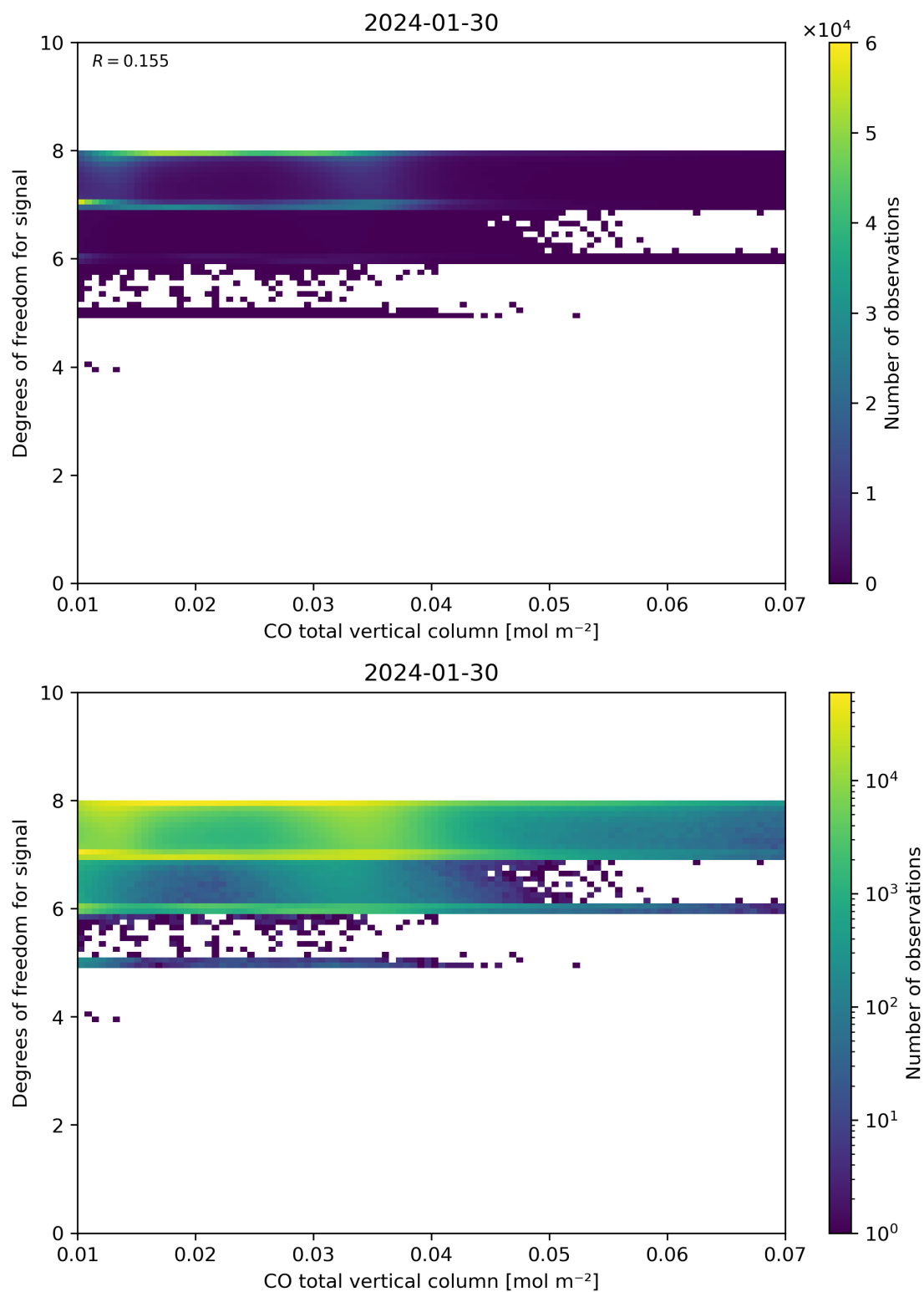
Figure 41: Scatter density plot of “CO total vertical column” against “Degrees of freedom for signal” for 2024-01-29 to 2024-01-31.
