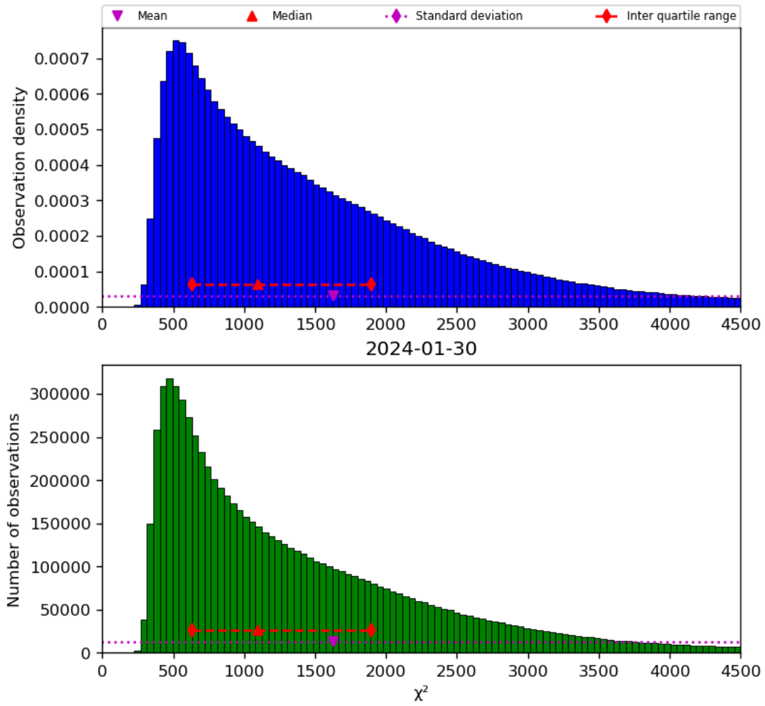
Figure 22: Histogram of “ \chi^2 ” for 2024-01-29 to 2024-01-31
