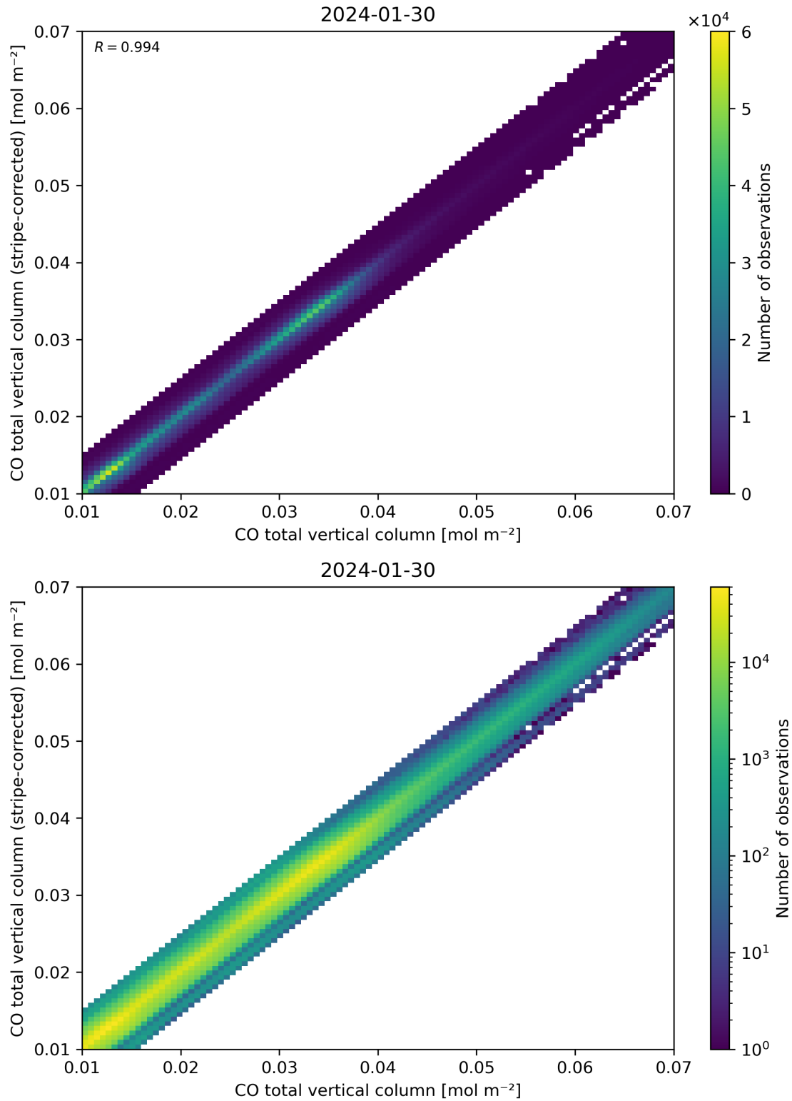
Figure 33: Scatter density plot of “CO total vertical column” against “CO total vertical column (stripe-corrected)” for 2024-01-29 to 2024-01-31.
