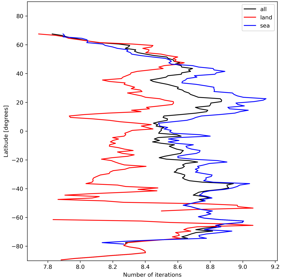
Figure 16: Zonal average of “Number of iterations” for 2024-01-29 to 2024-01-31.
