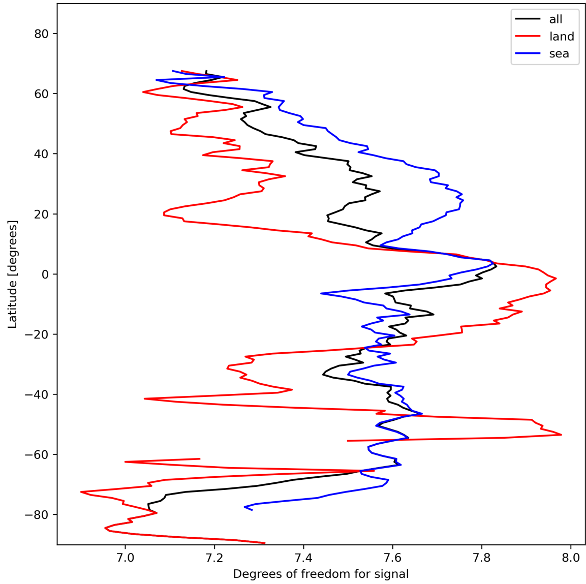
Figure 15: Zonal average of “Degrees of freedom for signal” for 2024-01-29 to 2024-01-31.
