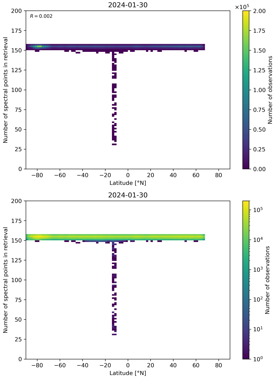
Figure 57: Scatter density plot of “Latitude” against “Number of spectral points in retrieval” for 2024-01-29 to 2024-01-31.
