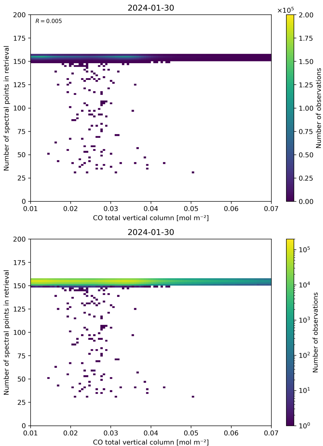
Figure 43: Scatter density plot of “CO total vertical column” against “Number of spectral points in retrieval” for 2024-01-29 to 2024-01-31.
