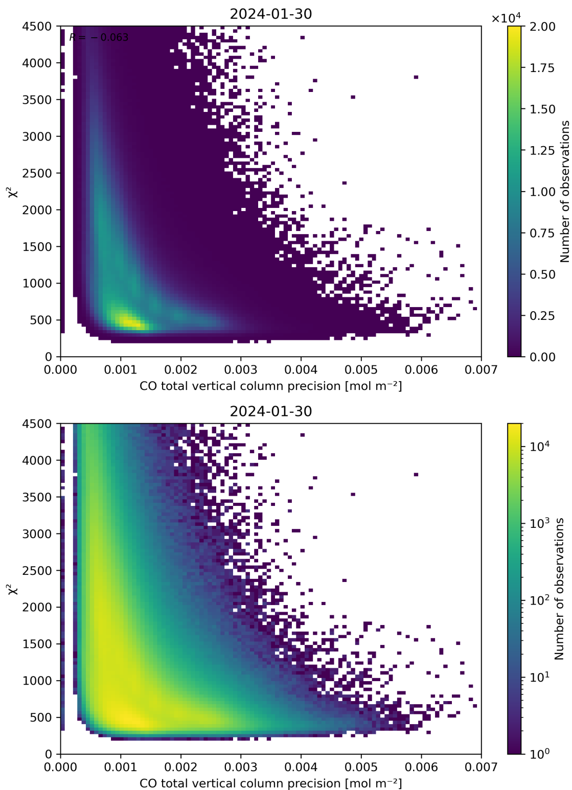
Figure 44: Scatter density plot of “CO total vertical column precision” against “ \chi^2 ” for 2024-01-29 to 2024-01-31.
