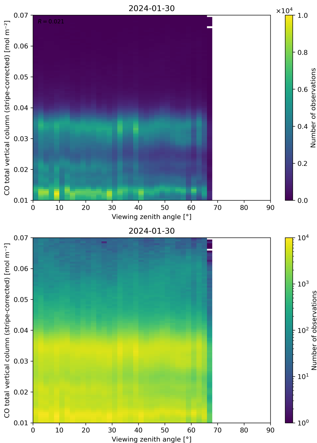
Figure 70: Scatter density plot of “Viewing zenith angle” against “CO total vertical column (stripe-corrected)” for 2024-01-29 to 2024-01-31.
