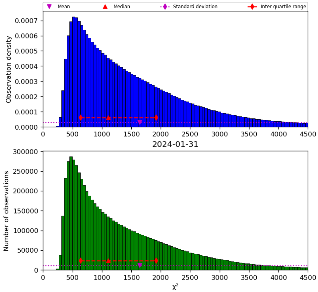
Figure 22: Histogram of “ \chi^2 ” for 2024-01-31 to 2024-02-01
