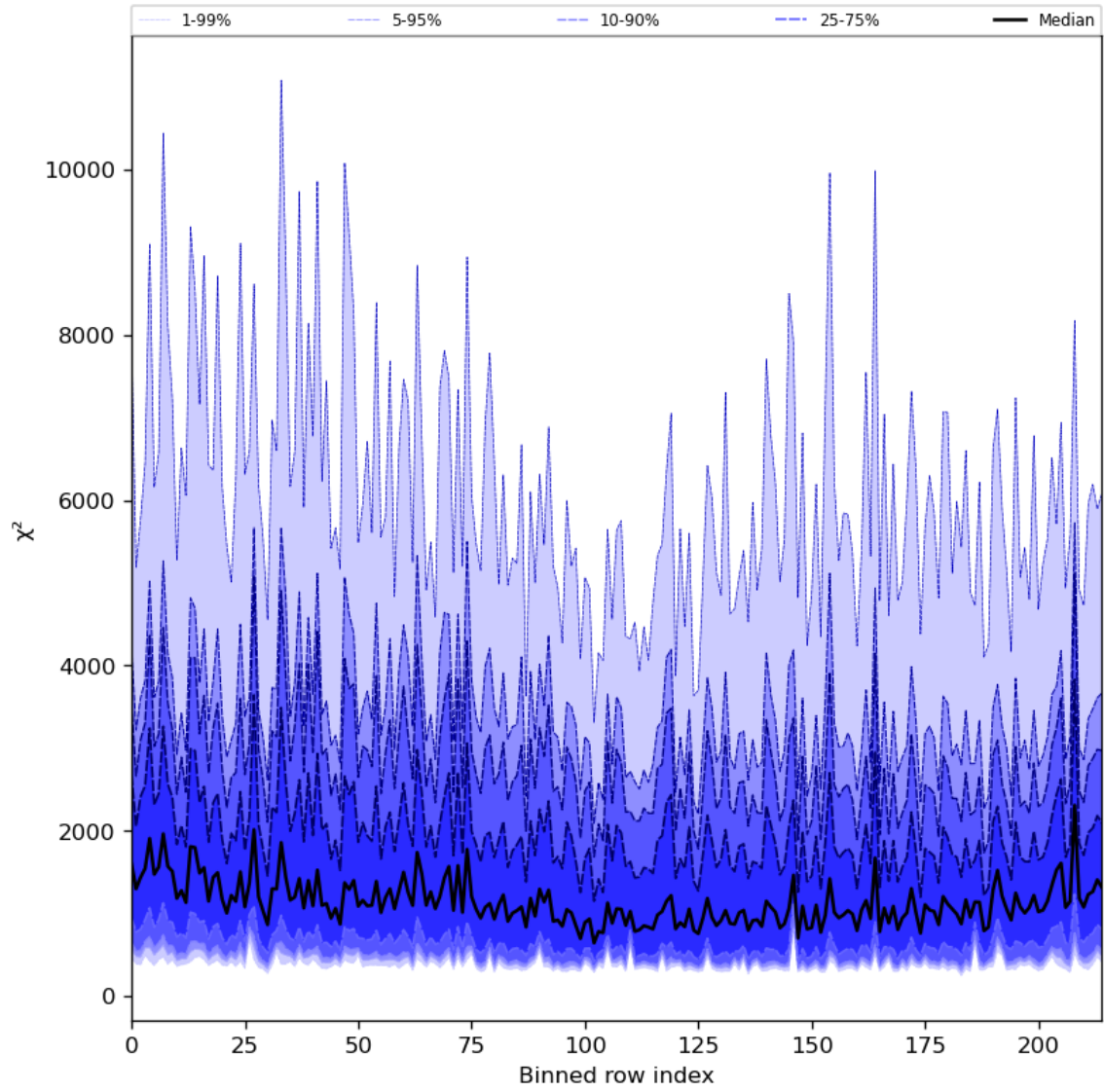
Figure 30: Along track statistics of “ \chi^2 ” for 2024-01-31 to 2024-02-01
