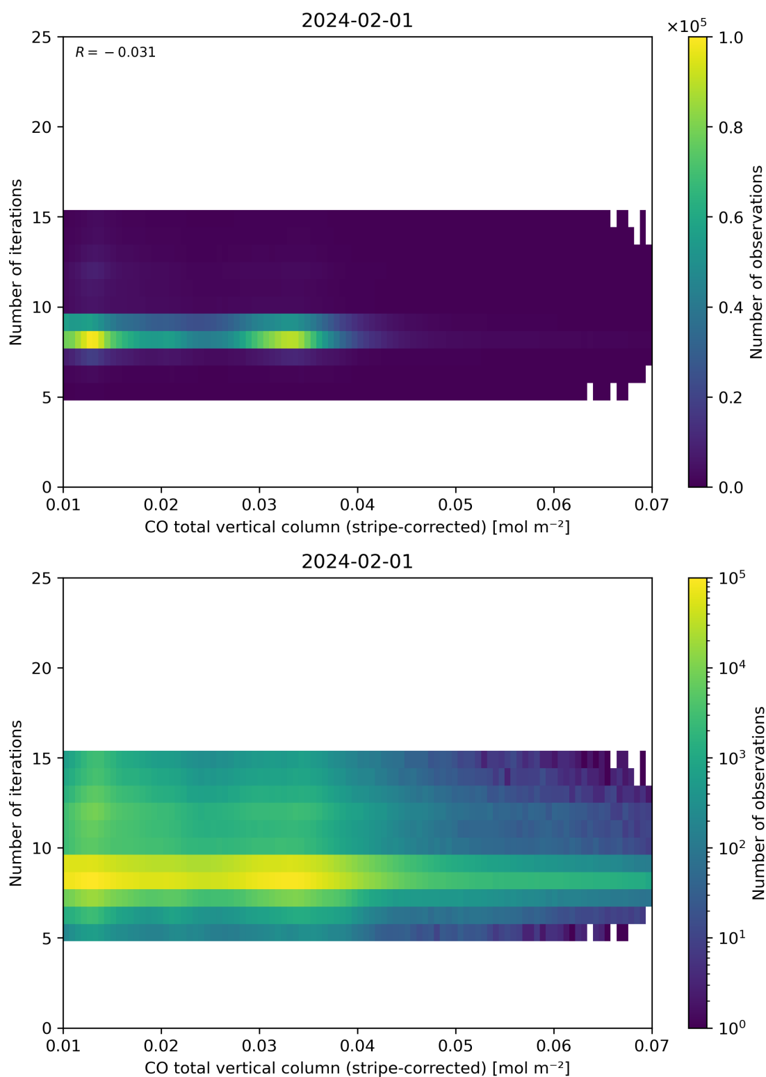
Figure 39: Scatter density plot of “CO total vertical column (stripe-corrected)” against “Number of iterations” for 2024-01-31 to 2024-02-02.
