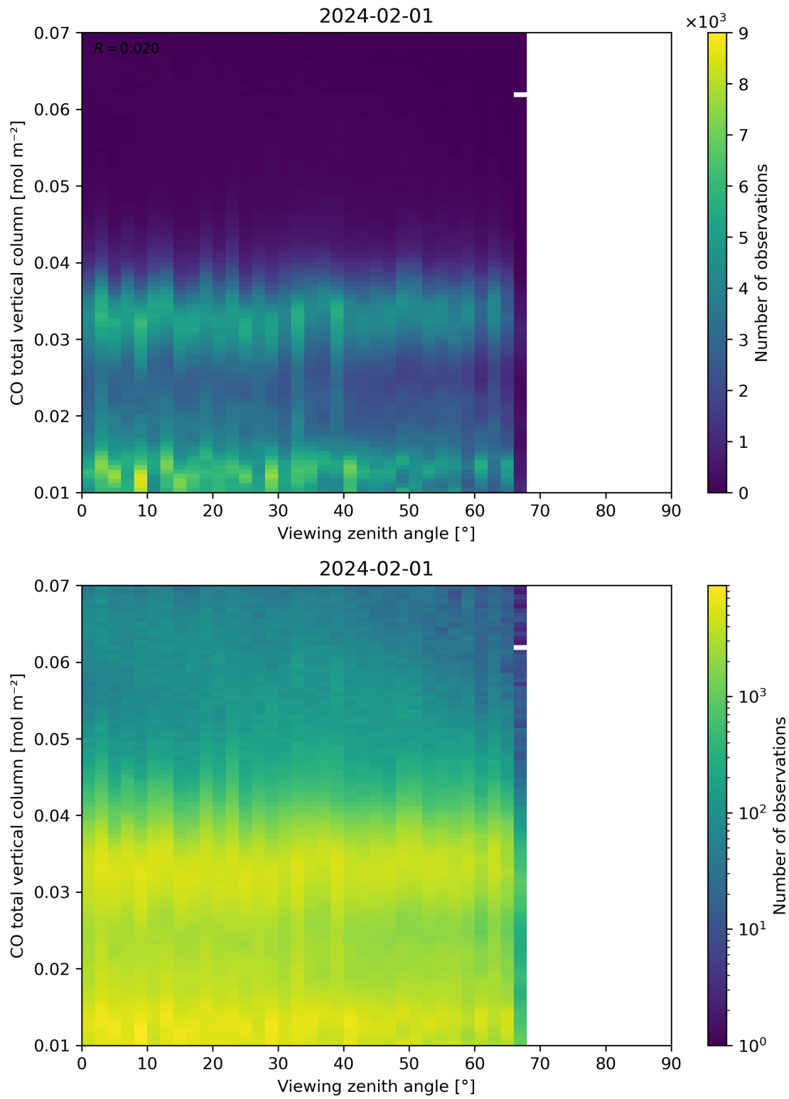
Figure 69: Scatter density plot of “Viewing zenith angle” against “CO total vertical column” for 2024-01-31 to 2024-02-02.
