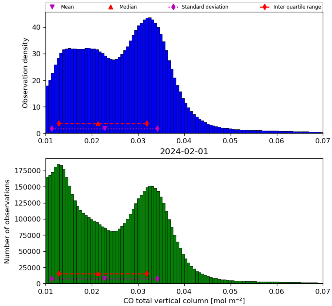
Figure 18: Histogram of “CO total vertical column” for 2024-01-31 to 2024-02-02
