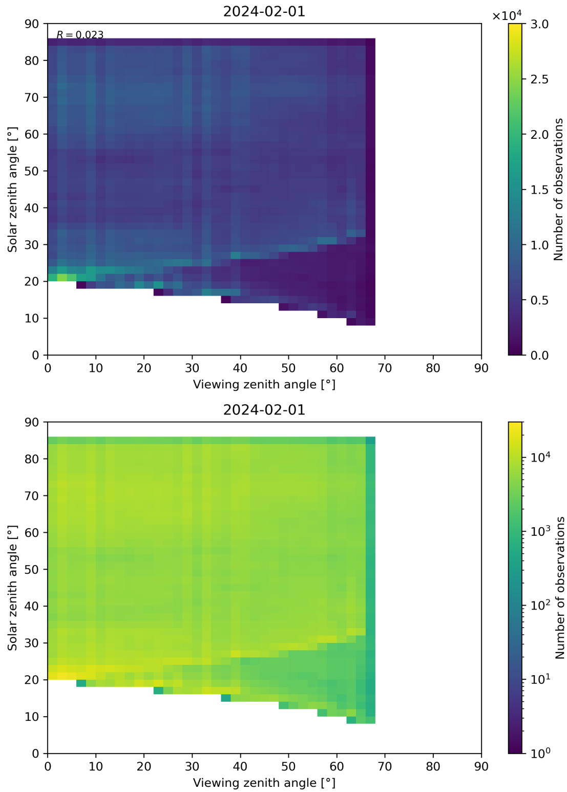
Figure 77: Scatter density plot of “Viewing zenith angle” against “Solar zenith angle” for 2024-01-31 to 2024-02-02.
