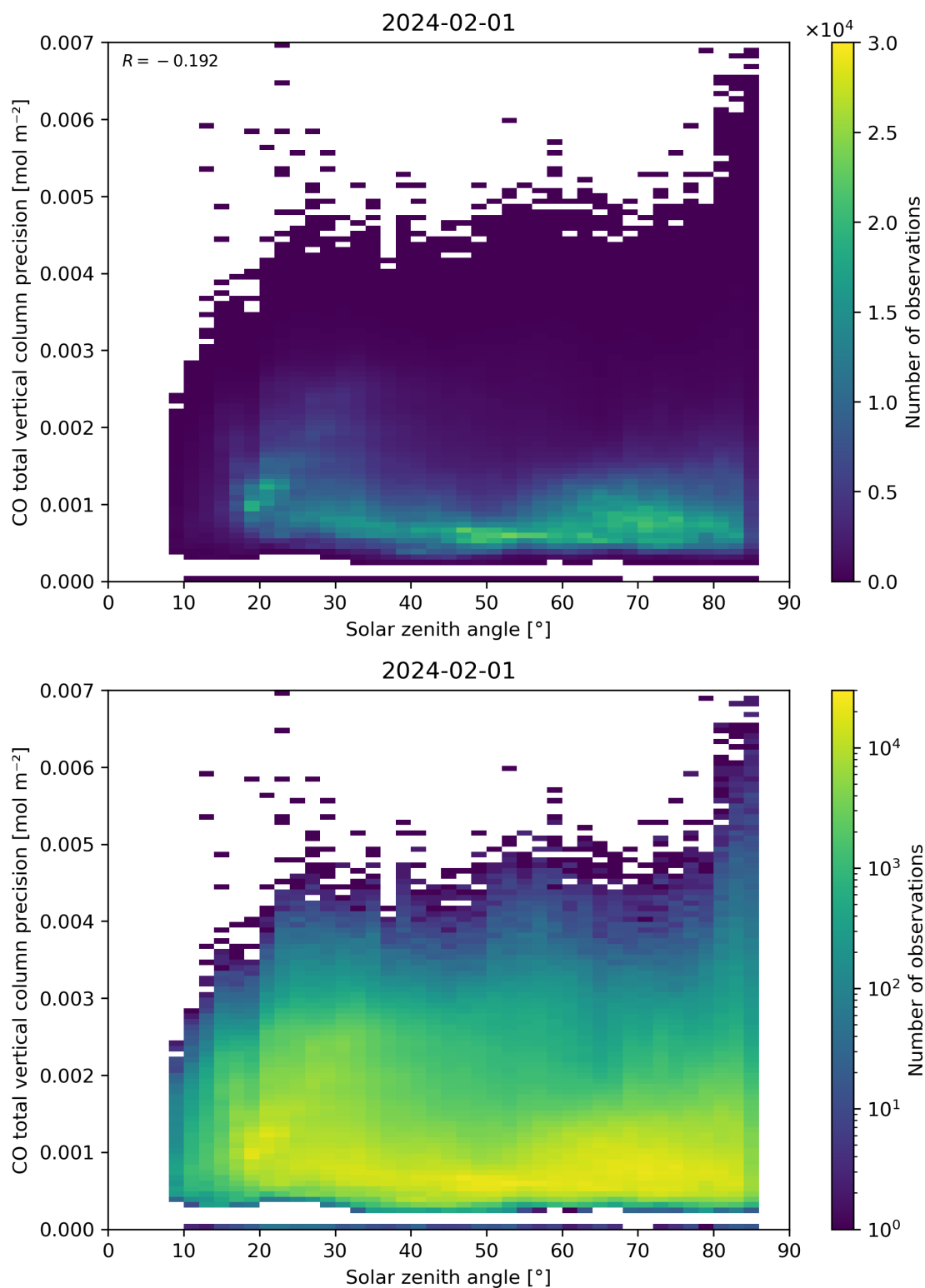
Figure 63: Scatter density plot of “Solar zenith angle” against “CO total vertical column precision” for 2024-01-31 to 2024-02-02.
