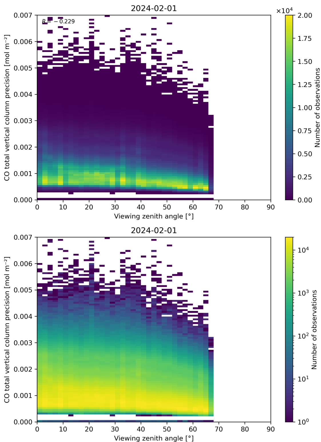
Figure 71: Scatter density plot of “Viewing zenith angle” against “CO total vertical column precision” for 2024-01-31 to 2024-02-02.
