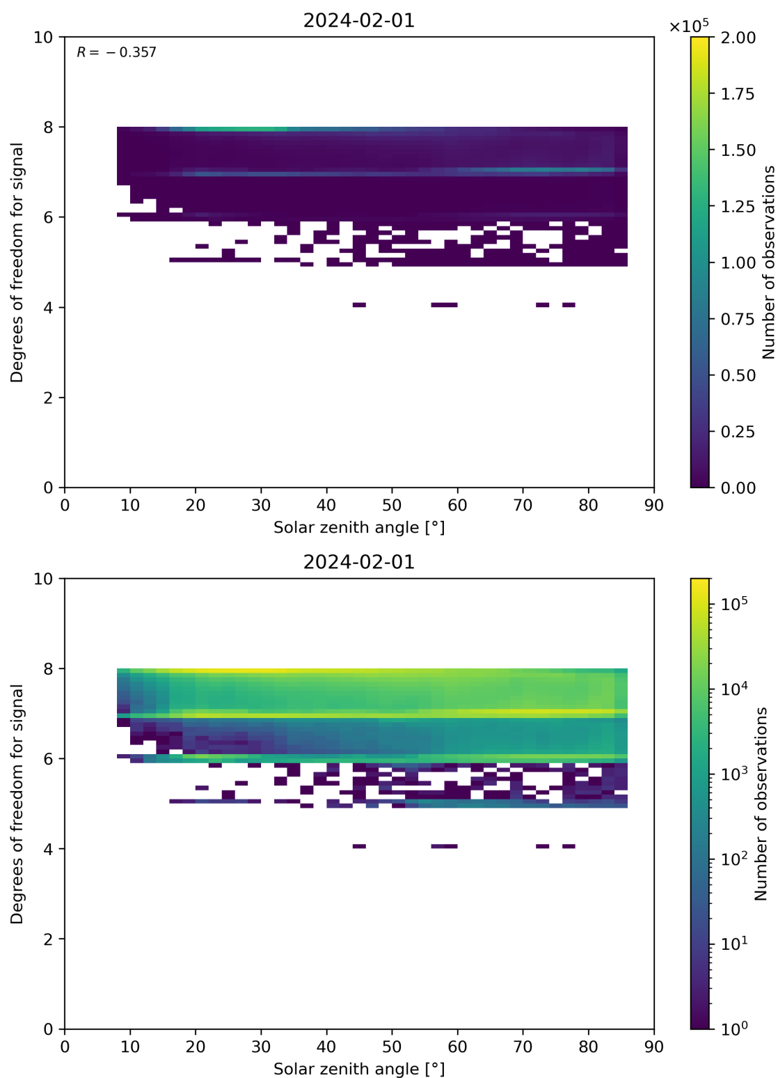
Figure 65: Scatter density plot of “Solar zenith angle” against “Degrees of freedom for signal” for 2024-01-31 to 2024-02-02.
