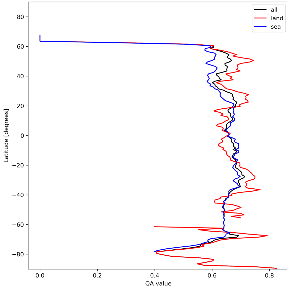
Figure 9: Zonal average of “QA value” for 2024-01-31 to 2024-02-02.
