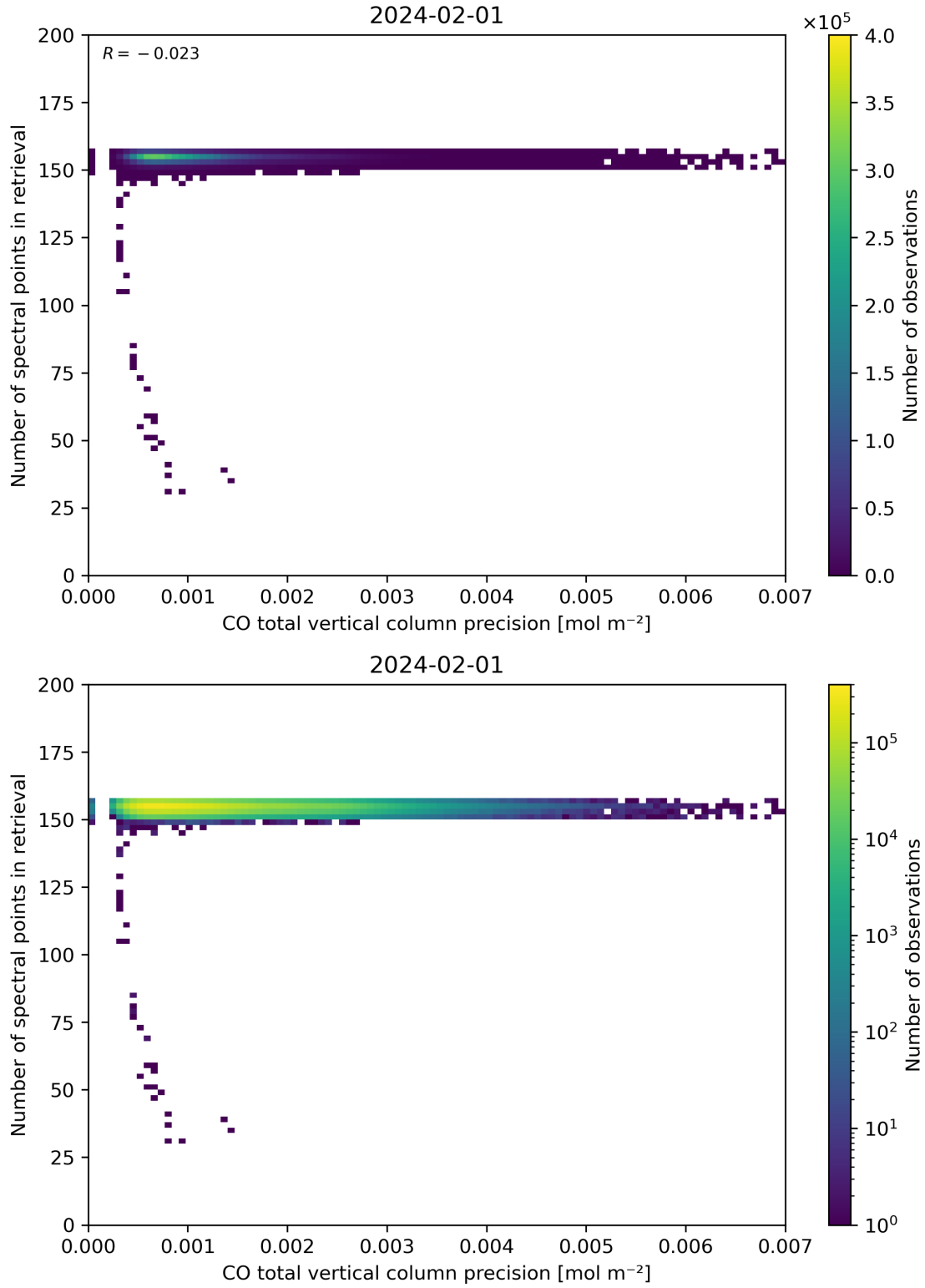
Figure 47: Scatter density plot of “CO total vertical column precision” against “Number of spectral points in retrieval” for 2024-01-31 to 2024-02-02.
