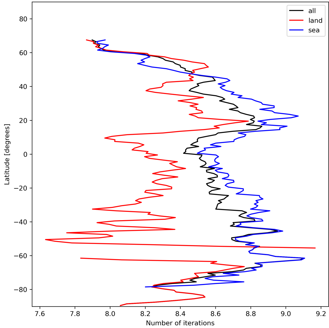
Figure 16: Zonal average of “Number of iterations” for 2024-01-31 to 2024-02-02.
