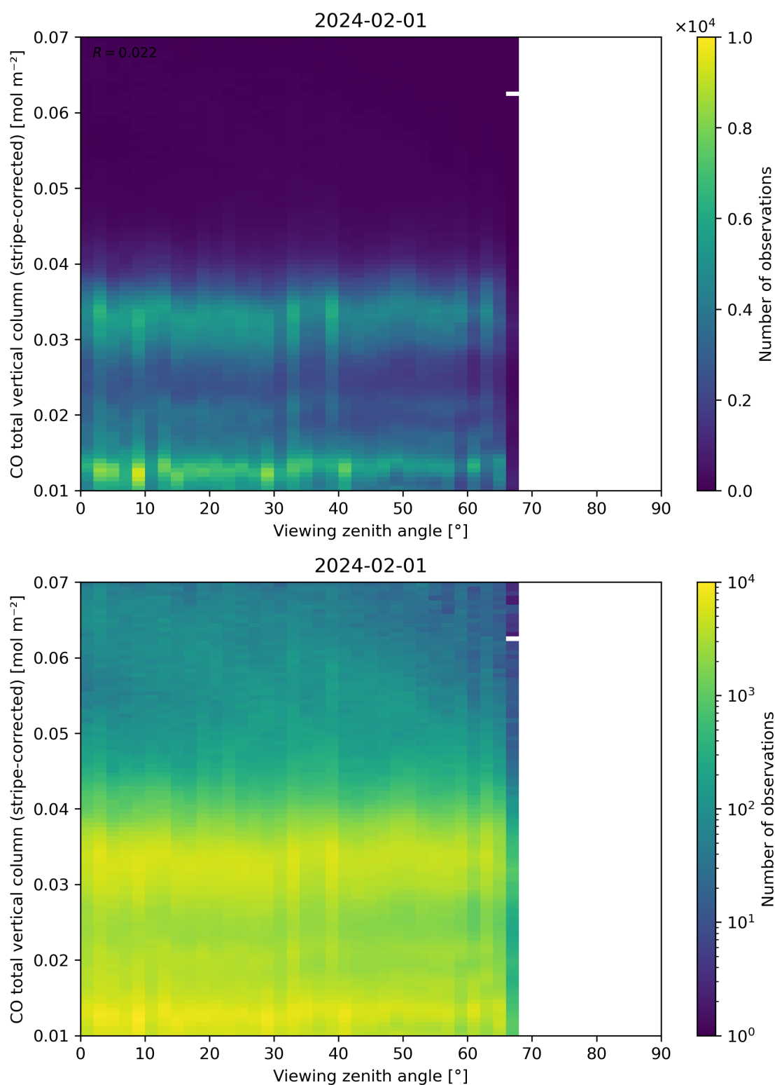
Figure 70: Scatter density plot of “Viewing zenith angle” against “CO total vertical column (stripe-corrected)” for 2024-01-31 to 2024-02-02.
