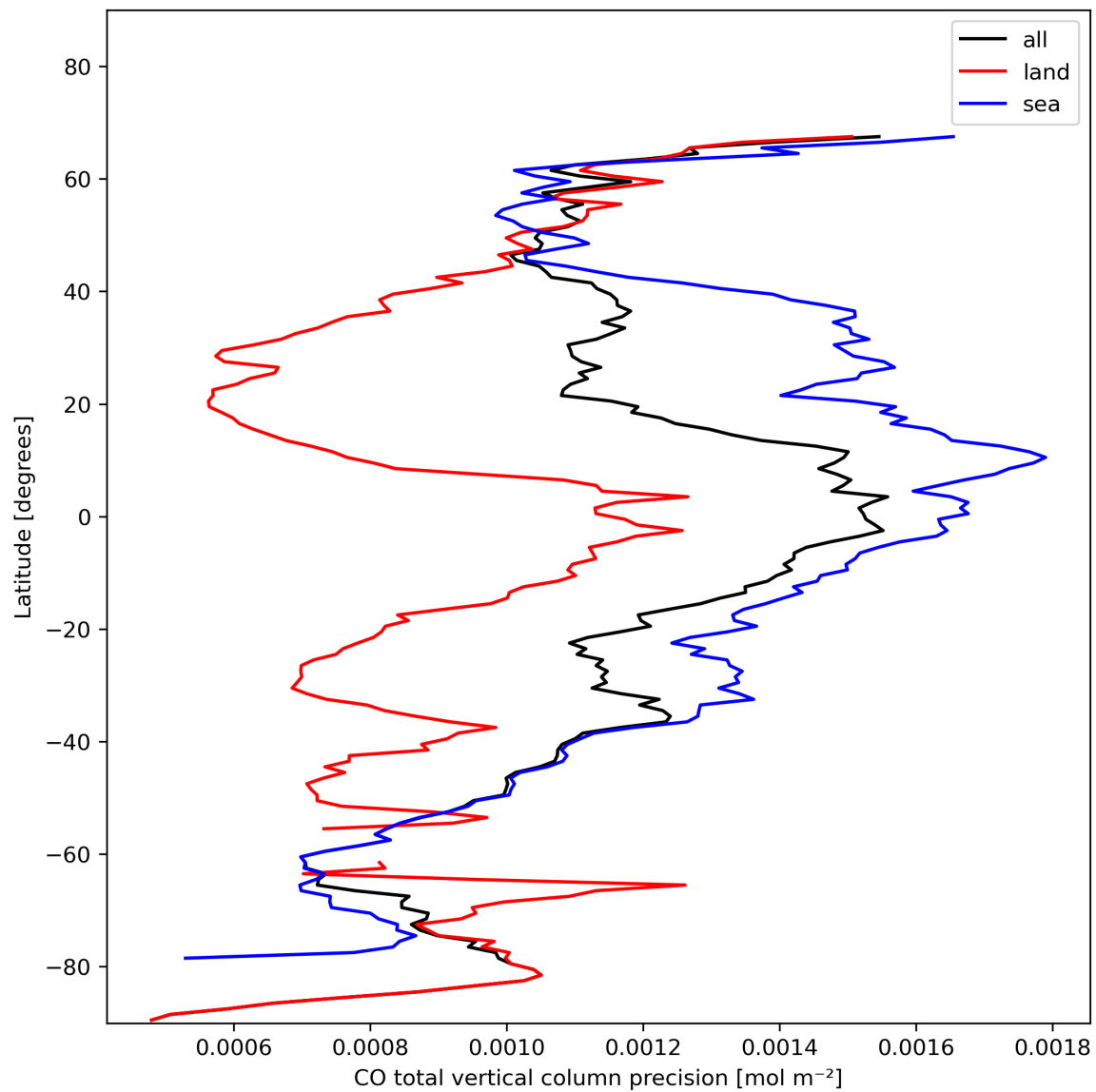
Figure 12: Zonal average of “CO total vertical column precision” for 2024-01-31 to 2024-02-02.
