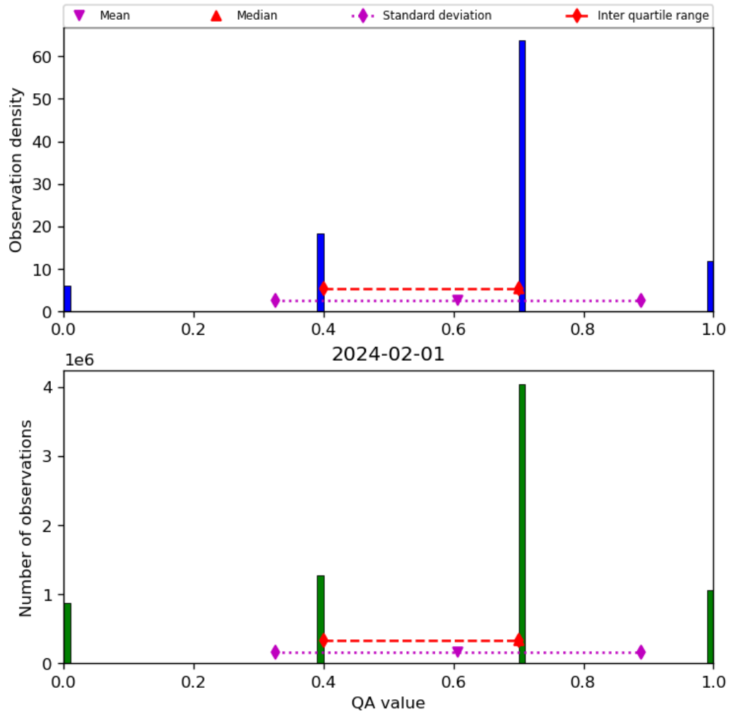
Figure 17: Histogram of “QA value” for 2024-01-31 to 2024-02-02
