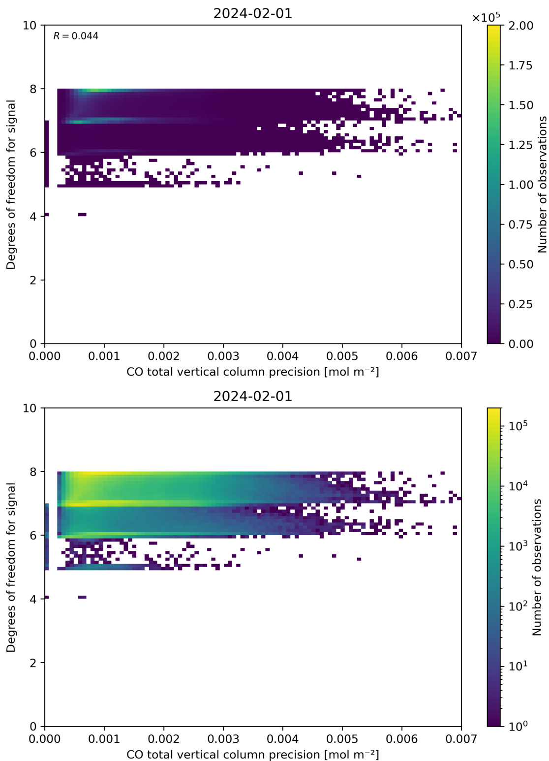
Figure 45: Scatter density plot of “CO total vertical column precision” against “Degrees of freedom for signal” for 2024-01-31 to 2024-02-02.
