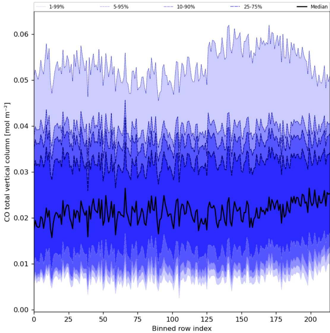
Figure 26: Along track statistics of “CO total vertical column” for 2024-01-31 to 2024-02-02
