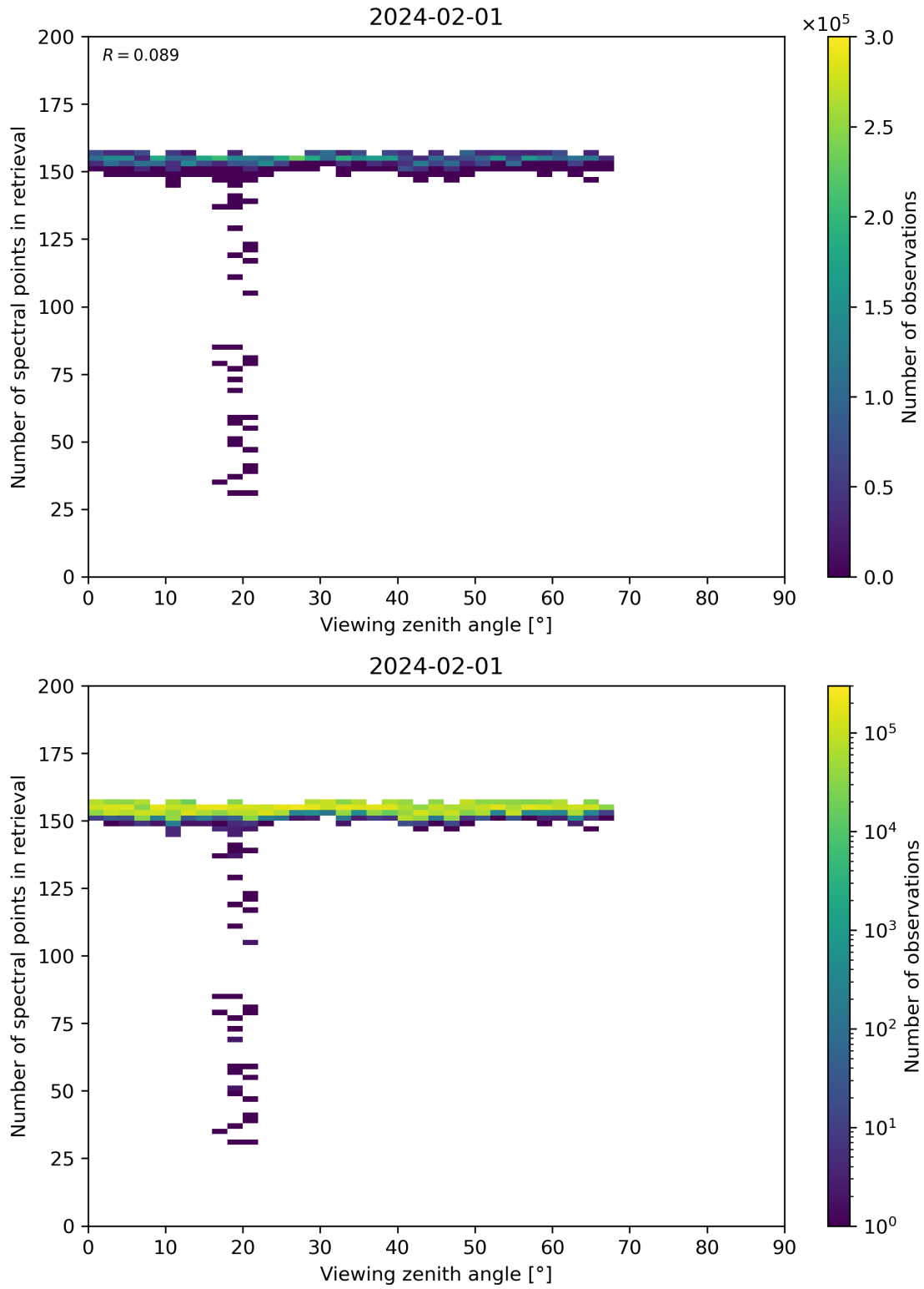
Figure 76: Scatter density plot of “Viewing zenith angle” against “Number of spectral points in retrieval” for 2024-01-31 to 2024-02-02.
