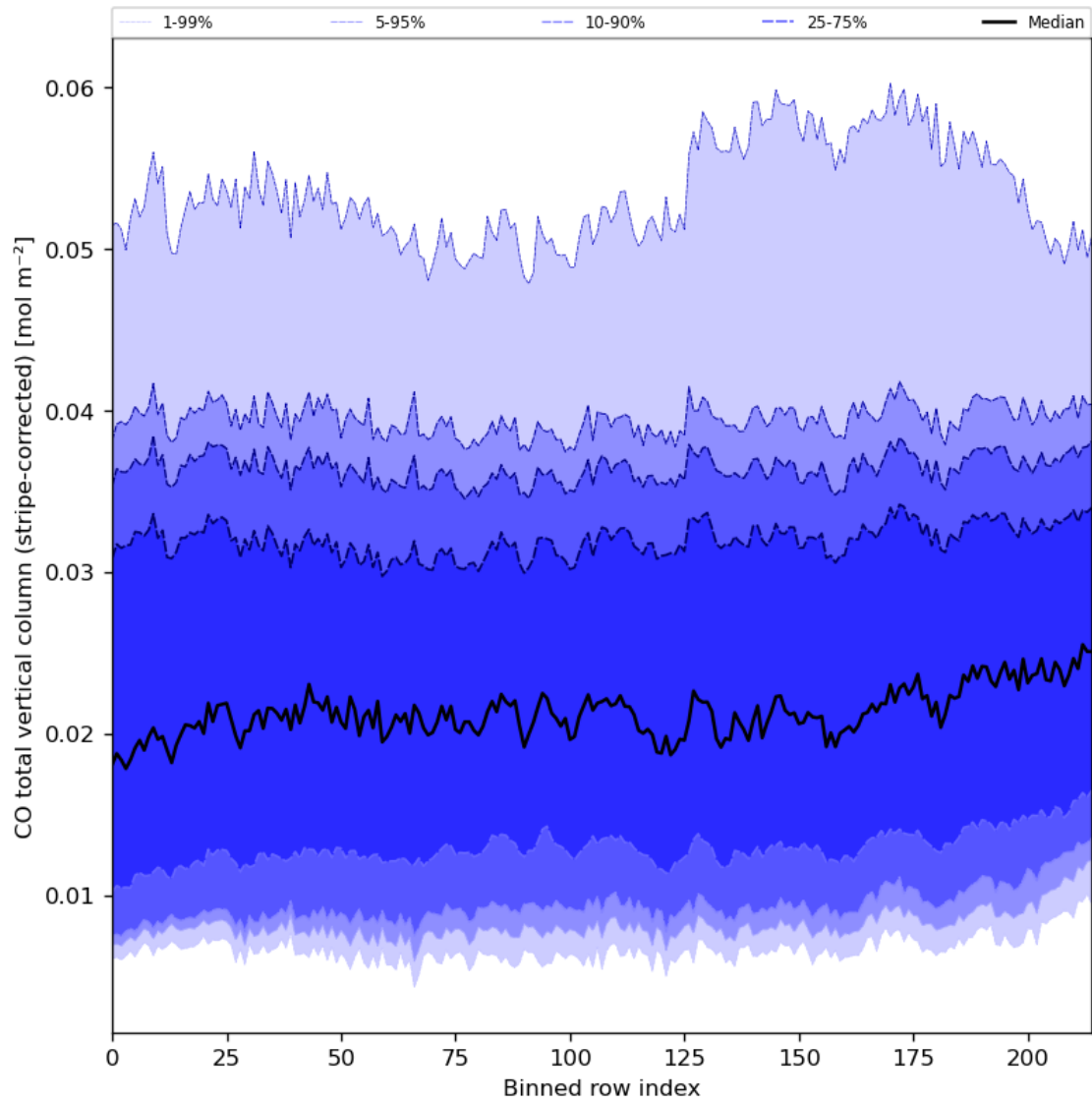
Figure 27: Along track statistics of “CO total vertical column (stripe-corrected)” for 2024-01-31 to 2024-02-02
