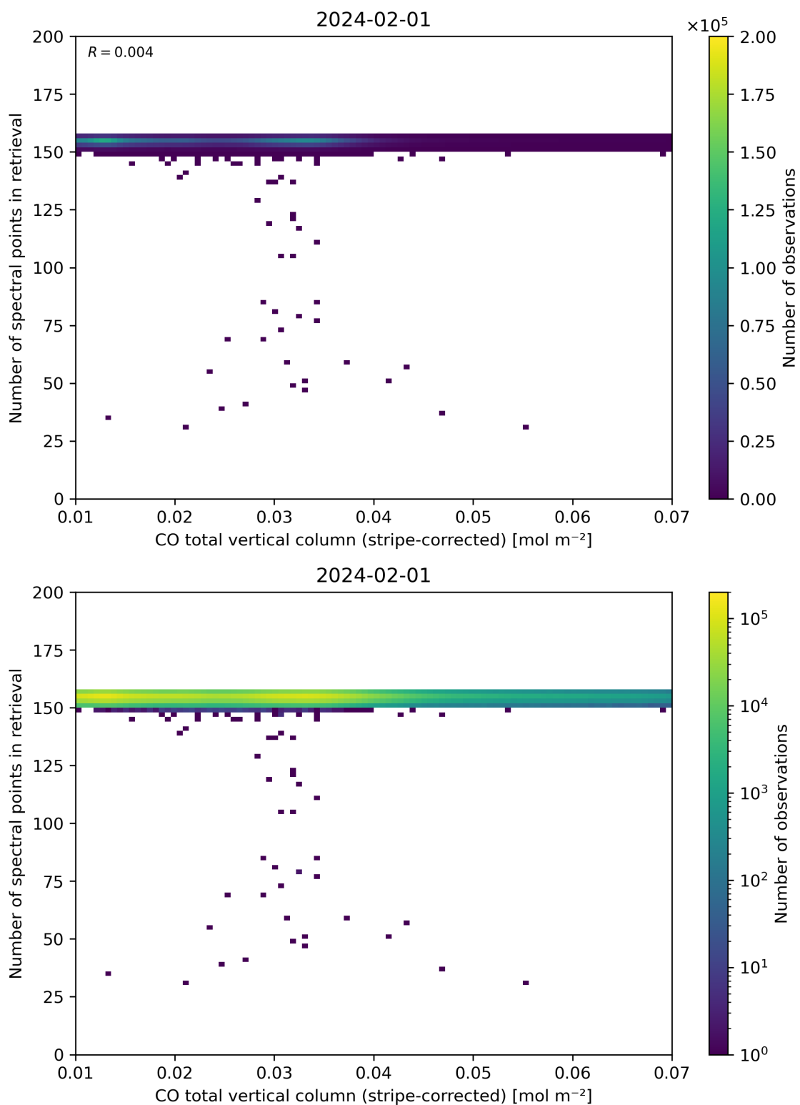
Figure 40: Scatter density plot of “CO total vertical column (stripe-corrected)” against “Number of spectral points in retrieval” for 2024-01-31 to 2024-02-02.
