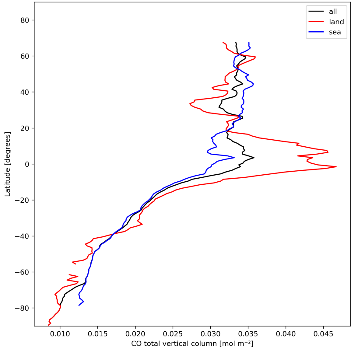
Figure 10: Zonal average of “CO total vertical column” for 2024-01-31 to 2024-02-02.
