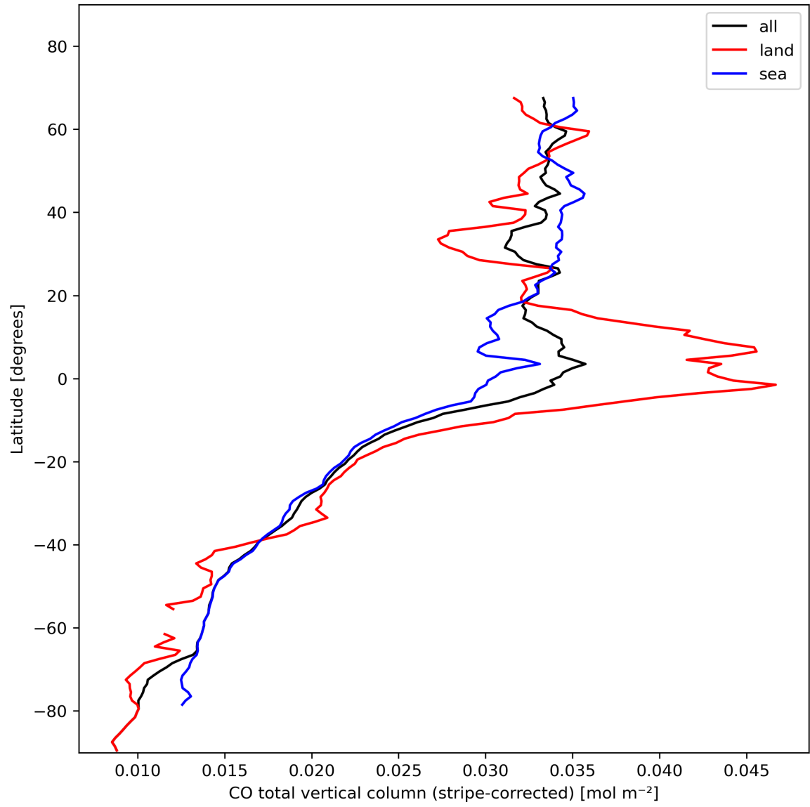
Figure 11: Zonal average of “CO total vertical column (stripe-corrected)” for 2024-01-31 to 2024-02-02.
