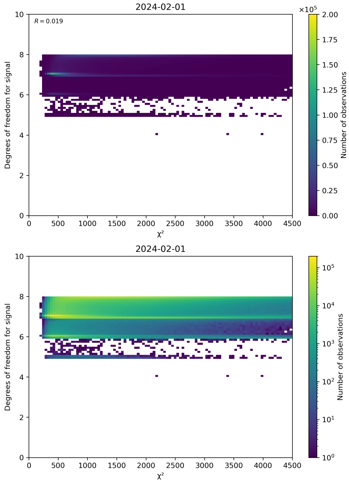
Figure 48: Scatter density plot of “ \chi^2 ” against “Degrees of freedom for signal” for 2024-01-31 to 2024-02-02.
