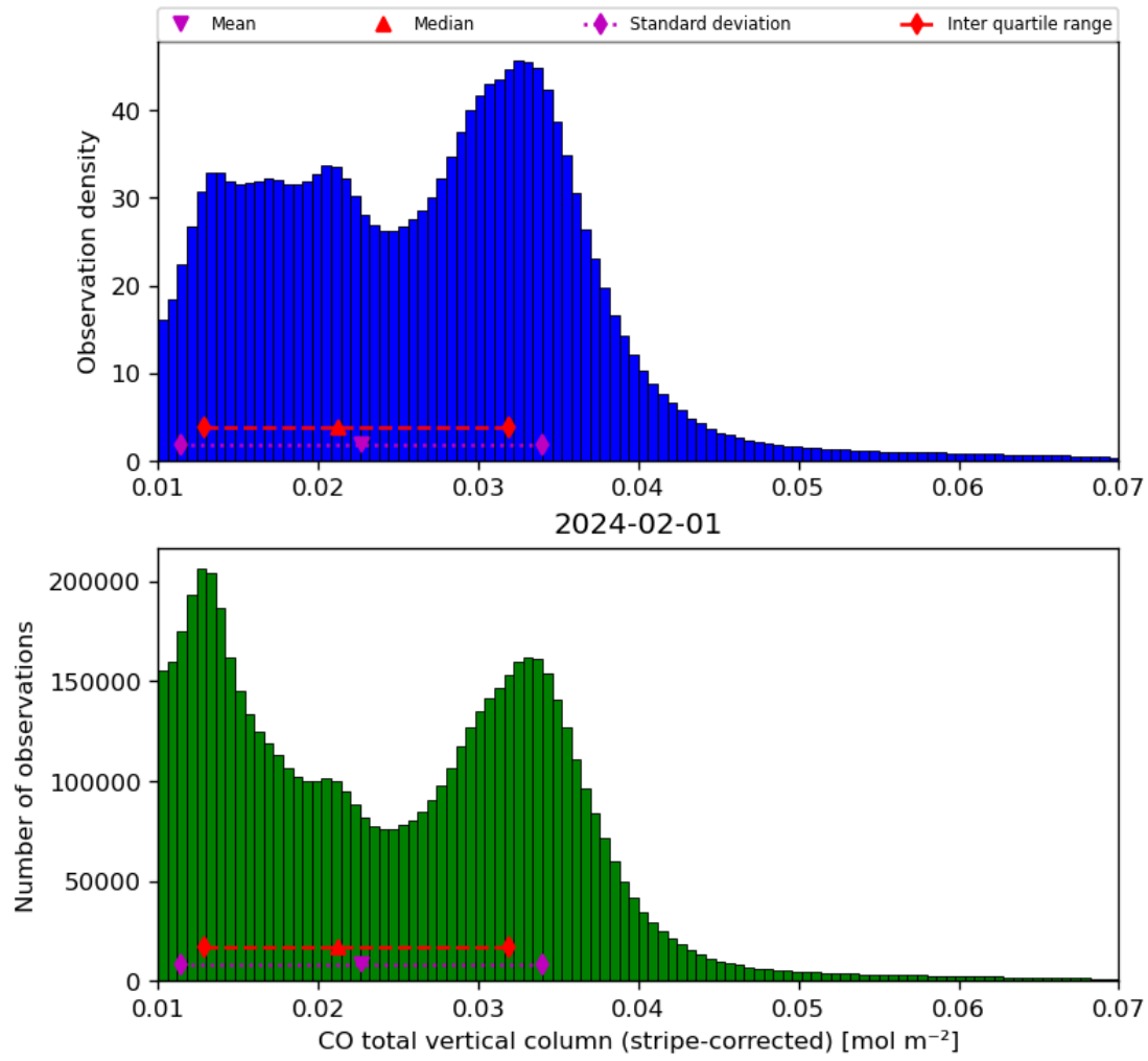
Figure 19: Histogram of “CO total vertical column (stripe-corrected)” for 2024-01-31 to 2024-02-02
