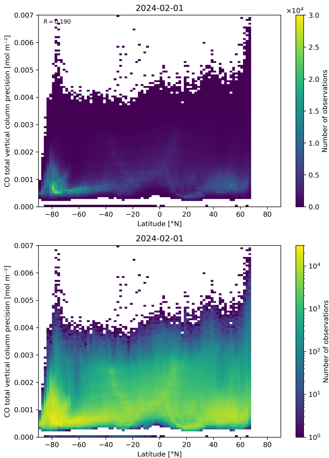
Figure 53: Scatter density plot of “Latitude” against “CO total vertical column precision” for 2024-01-31 to 2024-02-02.
