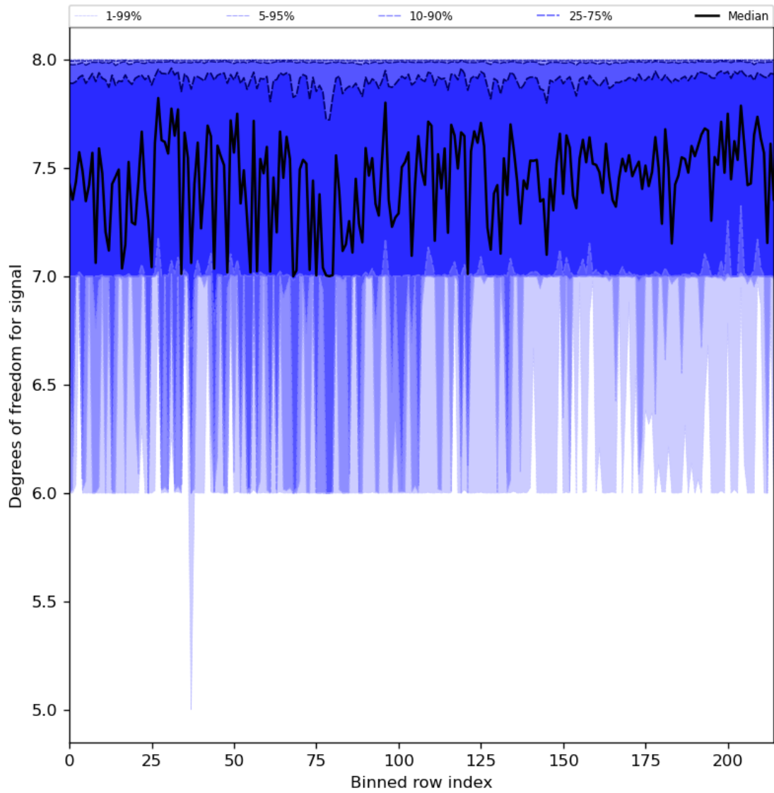
Figure 31: Along track statistics of “Degrees of freedom for signal” for 2024-01-31 to 2024-02-02
