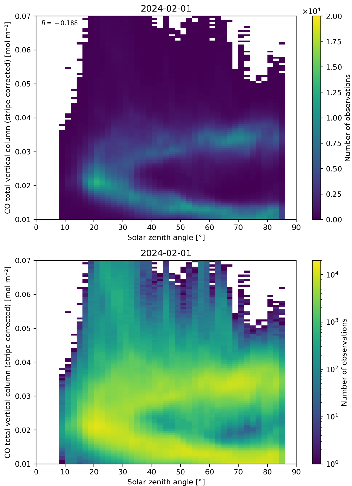
Figure 62: Scatter density plot of “Solar zenith angle” against “CO total vertical column (stripe-corrected)” for 2024-01-31 to 2024-02-02.
