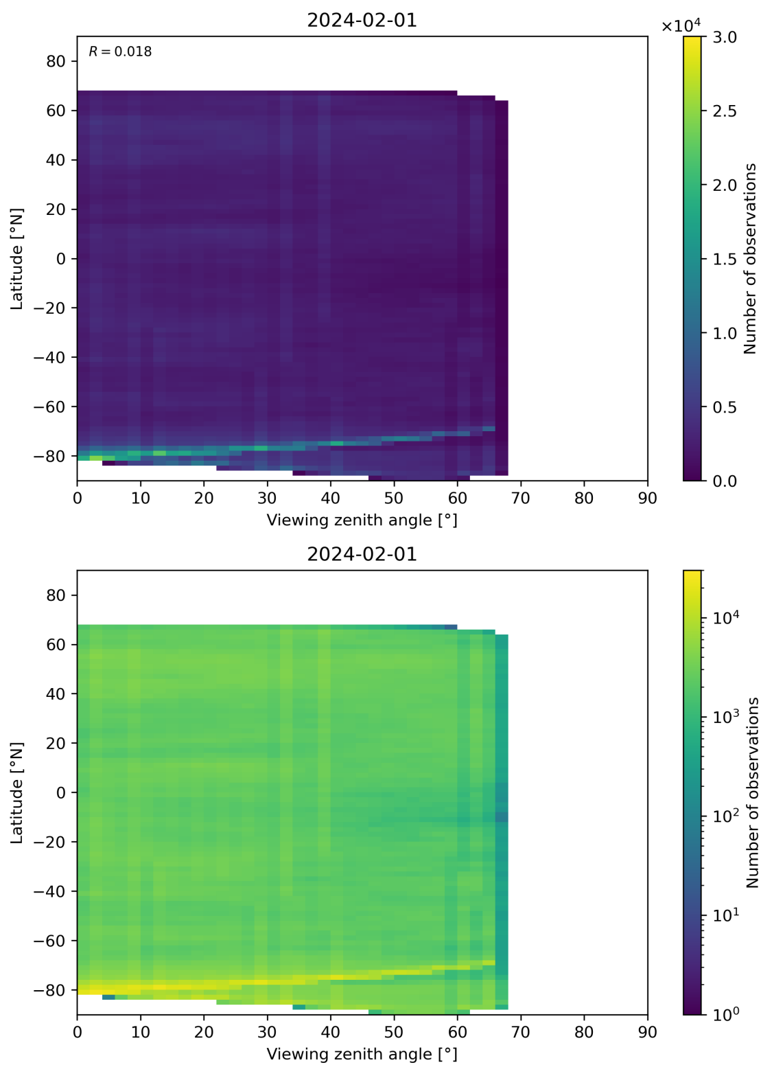
Figure 74: Scatter density plot of “Viewing zenith angle” against “Latitude” for 2024-01-31 to 2024-02-02.
