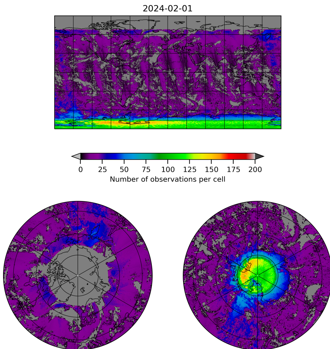
Figure 8: Map of the number of observations for 2024-01-31 to 2024-02-02
