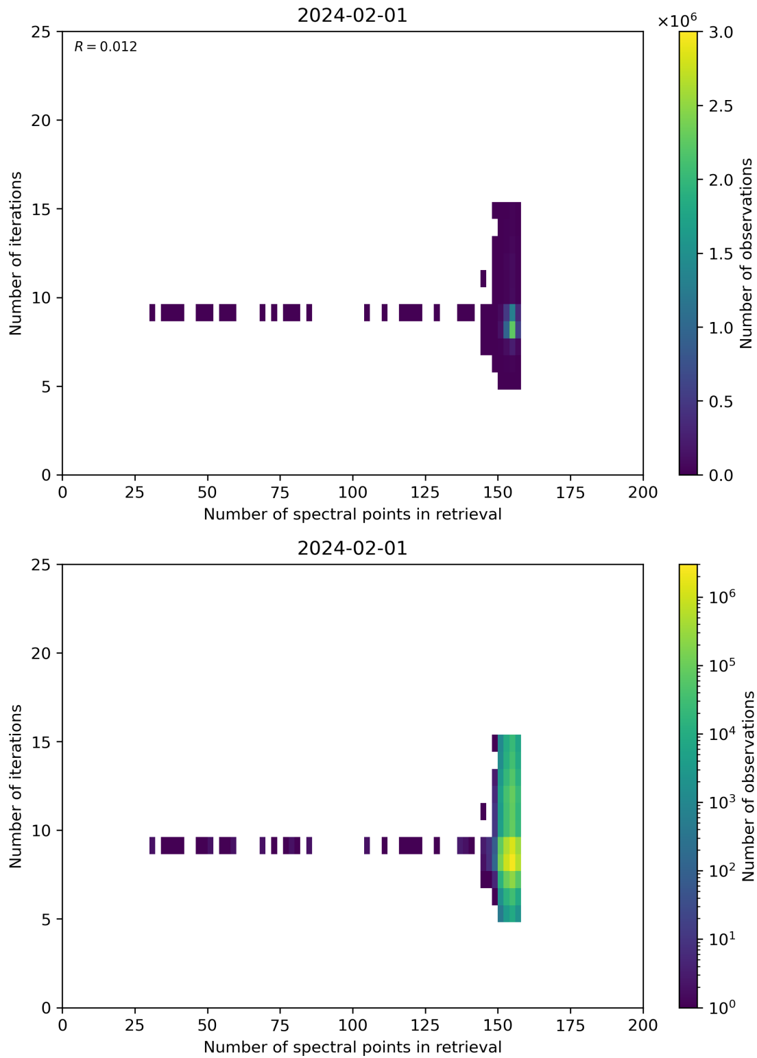
Figure 60: Scatter density plot of “Number of spectral points in retrieval” against “Number of iterations” for 2024-01-31 to 2024-02-02.
