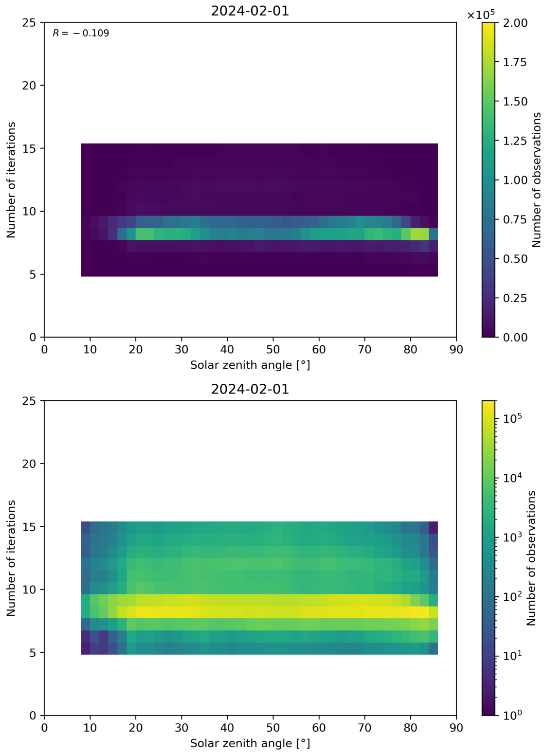
Figure 67: Scatter density plot of “Solar zenith angle” against “Number of iterations” for 2024-01-31 to 2024-02-02.
