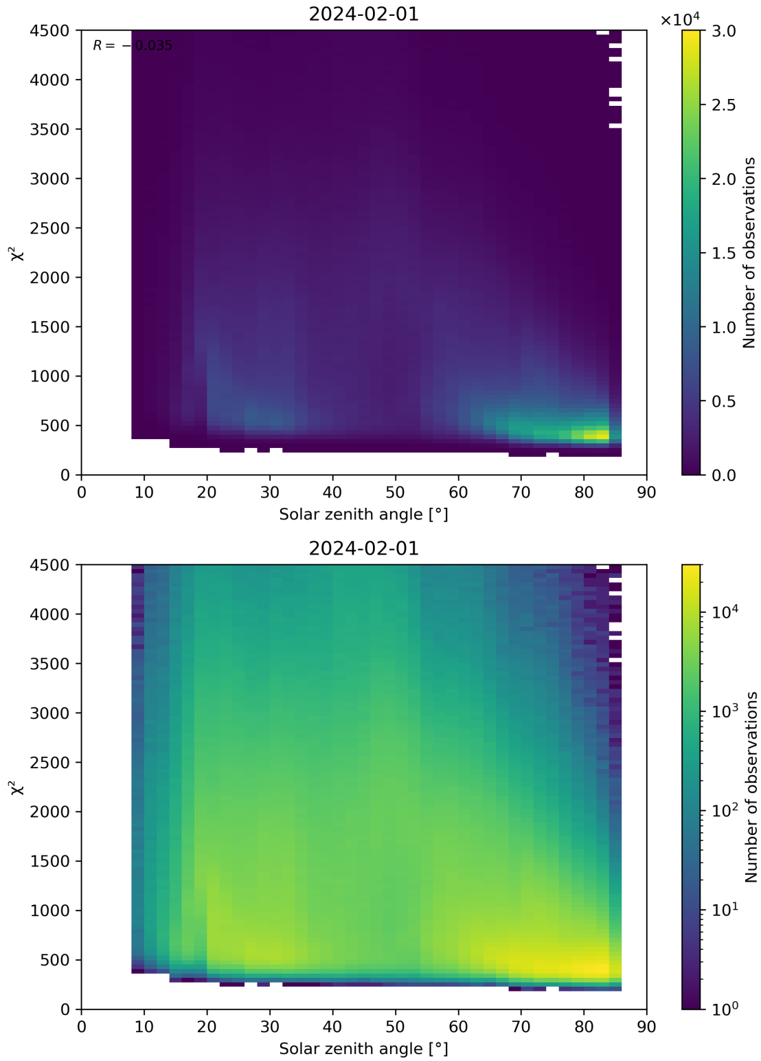
Figure 64: Scatter density plot of “Solar zenith angle” against “ \chi^2 ” for 2024-01-31 to 2024-02-02.
