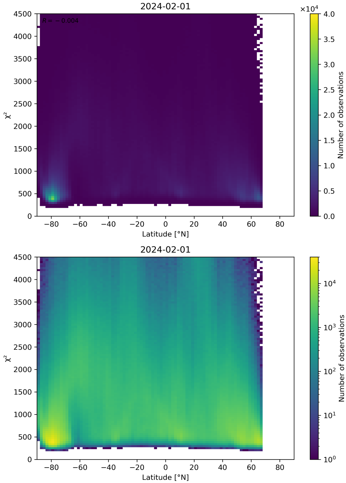
Figure 54: Scatter density plot of “Latitude” against “ \chi^2 ” for 2024-01-31 to 2024-02-02.
