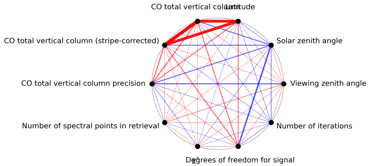
Figure 1: Map of correlation graph for 2024-01-31 to 2024-02-02.
