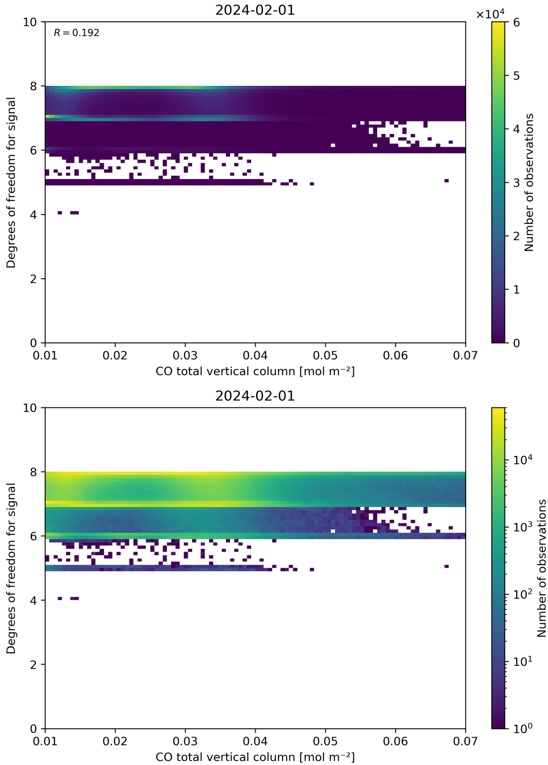
Figure 41: Scatter density plot of “CO total vertical column” against “Degrees of freedom for signal” for 2024-01-31 to 2024-02-02.
