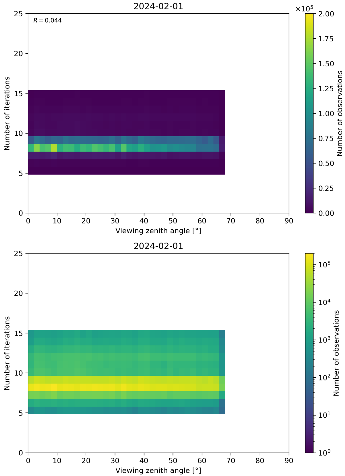
Figure 75: Scatter density plot of “Viewing zenith angle” against “Number of iterations” for 2024-01-31 to 2024-02-02.
