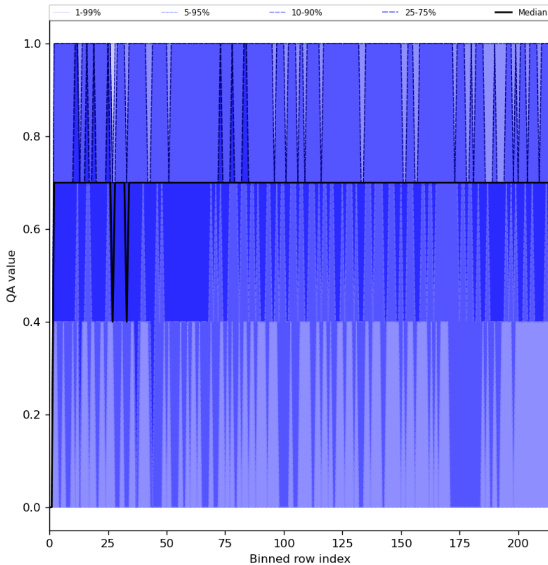
Figure 25: Along track statistics of “QA value” for 2024-01-31 to 2024-02-02
