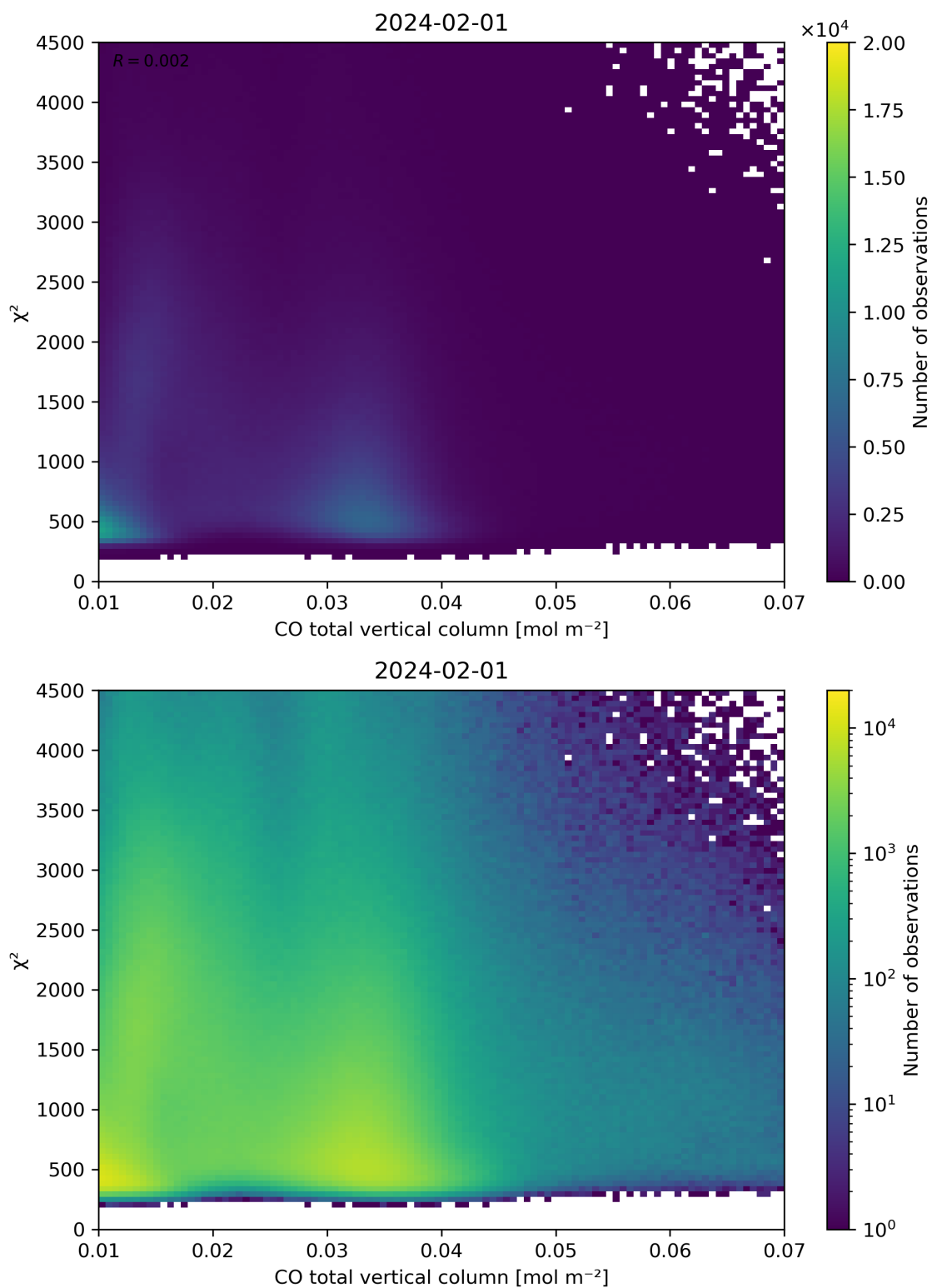
Figure 35: Scatter density plot of “CO total vertical column” against “ \chi^2 ” for 2024-01-31 to 2024-02-02.
