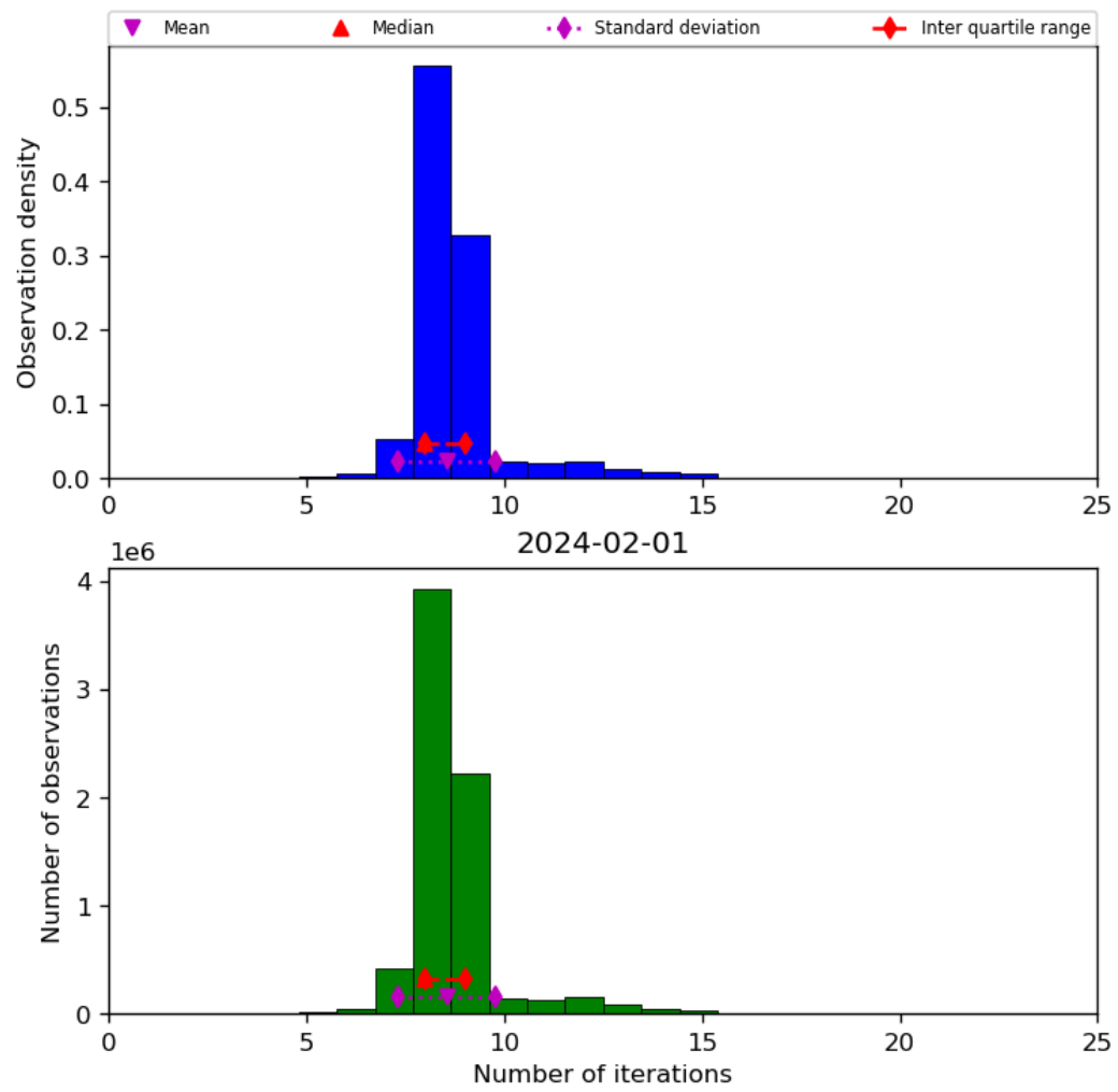
Figure 24: Histogram of “Number of iterations” for 2024-01-31 to 2024-02-02
