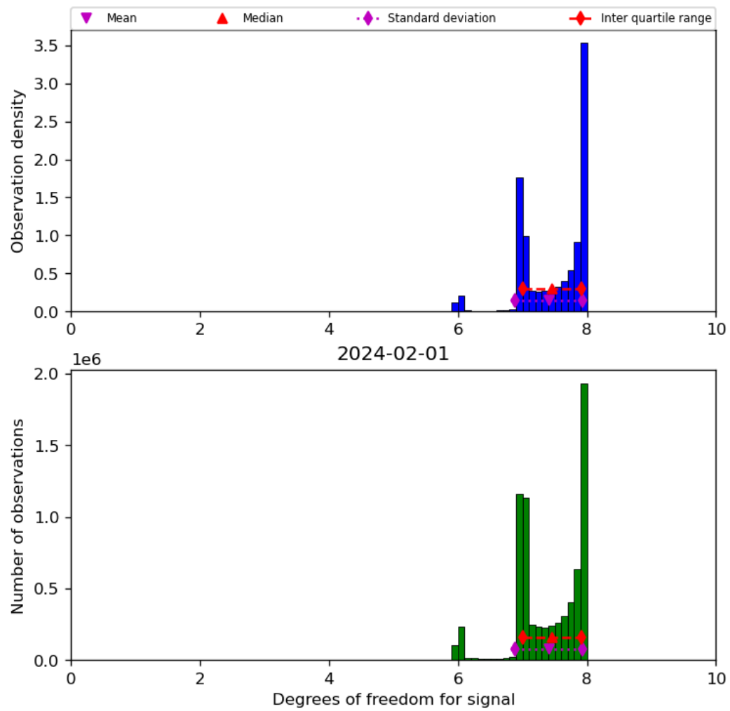
Figure 23: Histogram of “Degrees of freedom for signal” for 2024-01-31 to 2024-02-02
