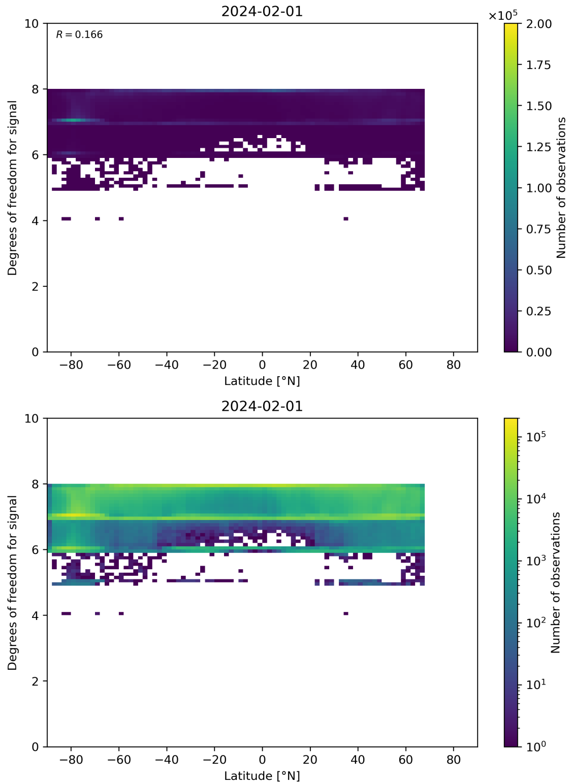
Figure 55: Scatter density plot of “Latitude” against “Degrees of freedom for signal” for 2024-01-31 to 2024-02-02.
