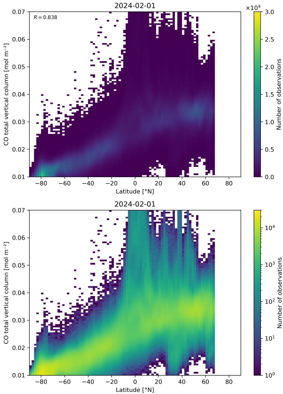
Figure 51: Scatter density plot of “Latitude” against “CO total vertical column” for 2024-01-31 to 2024-02-02.
