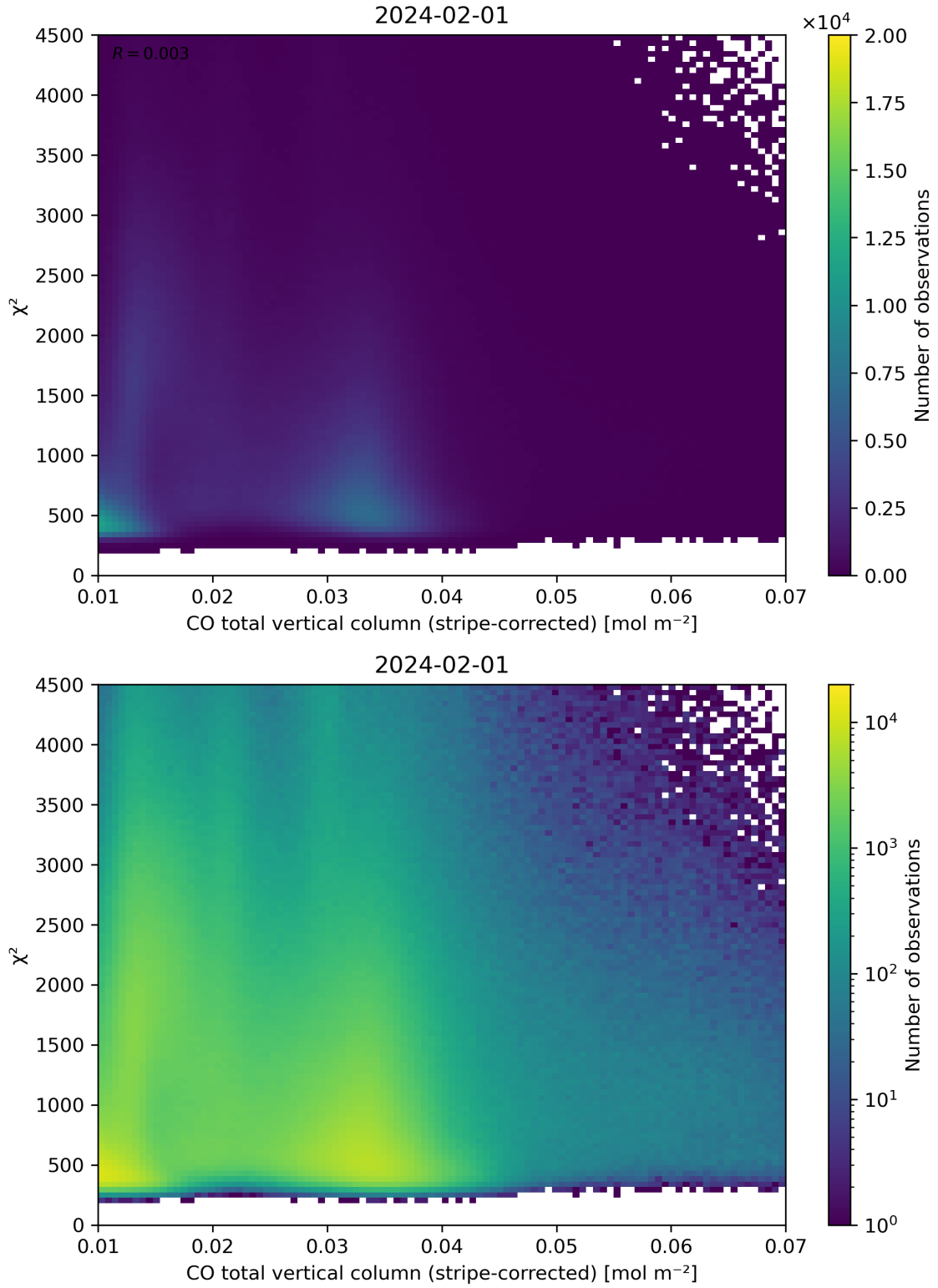
Figure 37: Scatter density plot of “CO total vertical column (stripe-corrected)” against “ \chi^2 ” for 2024-01-31 to 2024-02-02.
