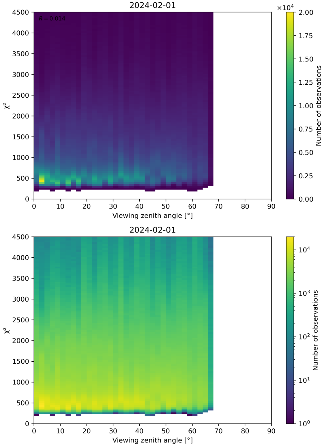
Figure 72: Scatter density plot of “Viewing zenith angle” against “ \chi^2 ” for 2024-01-31 to 2024-02-02.
