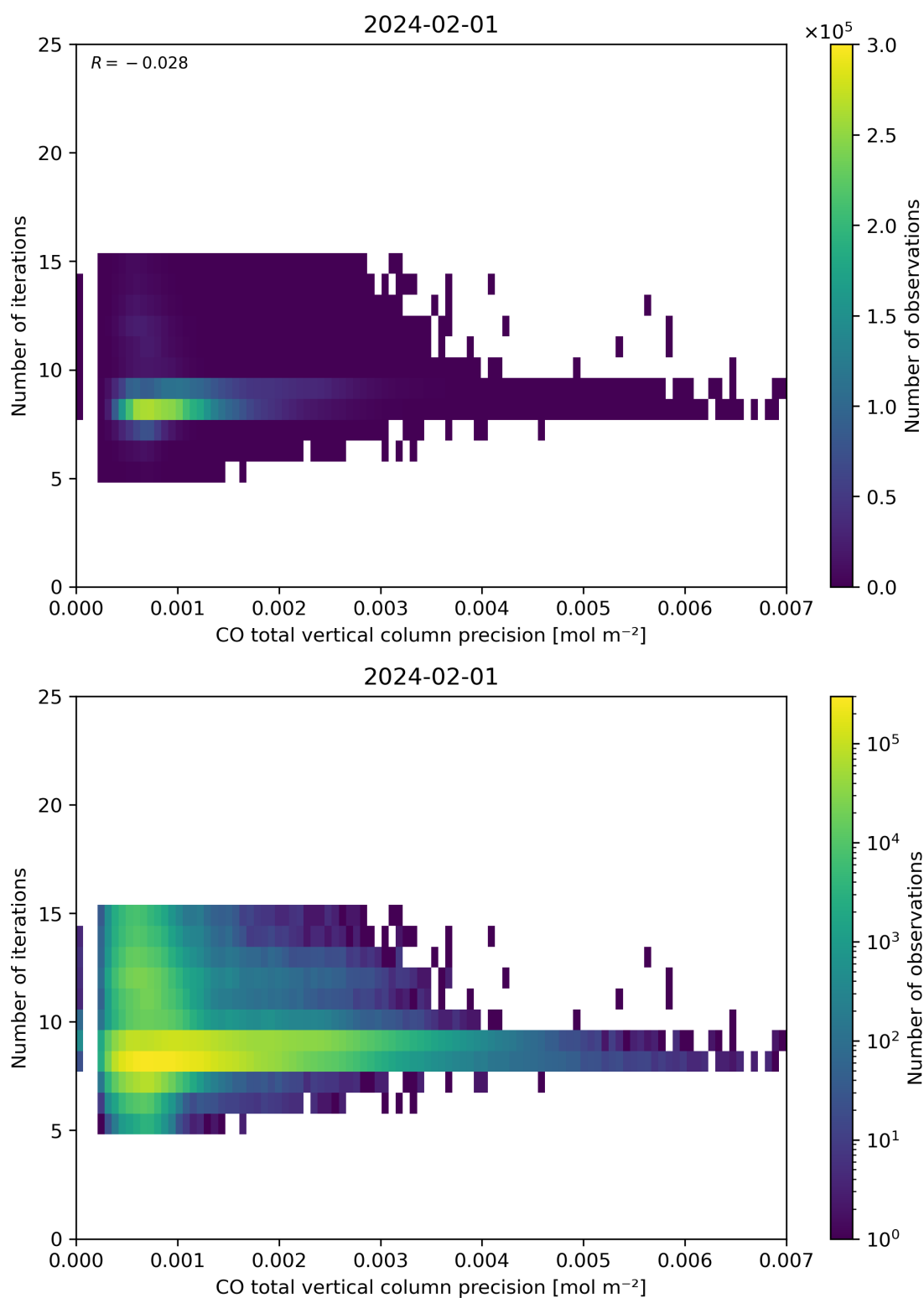
Figure 46: Scatter density plot of “CO total vertical column precision” against “Number of iterations” for 2024-01-31 to 2024-02-02.
