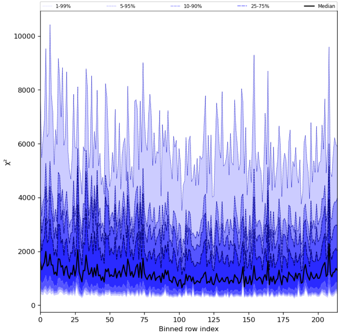
Figure 30: Along track statistics of “ \chi^2 ” for 2024-01-31 to 2024-02-02
