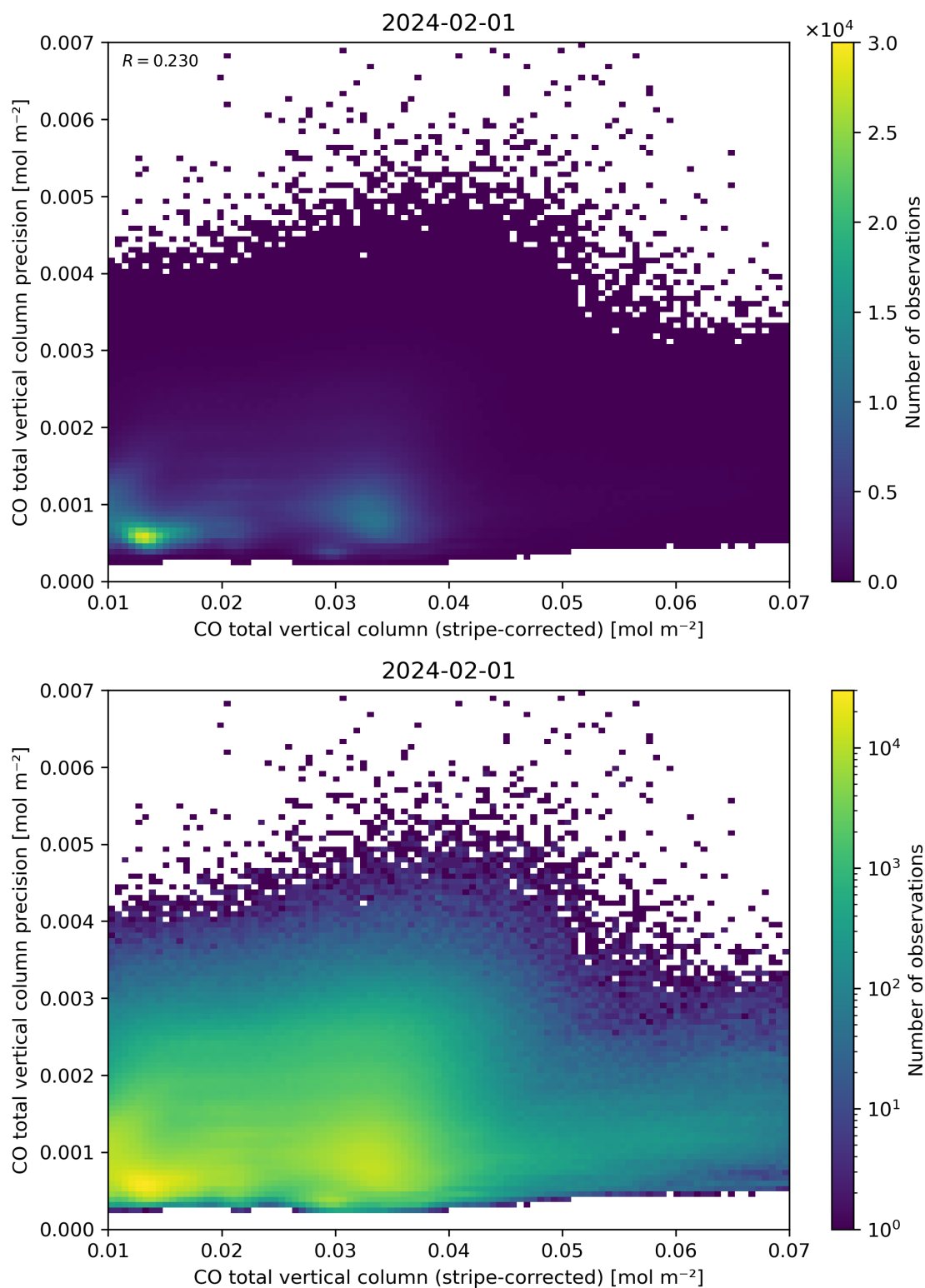
Figure 36: Scatter density plot of “CO total vertical column (stripe-corrected)” against “CO total vertical column precision” for 2024-01-31 to 2024-02-02.
