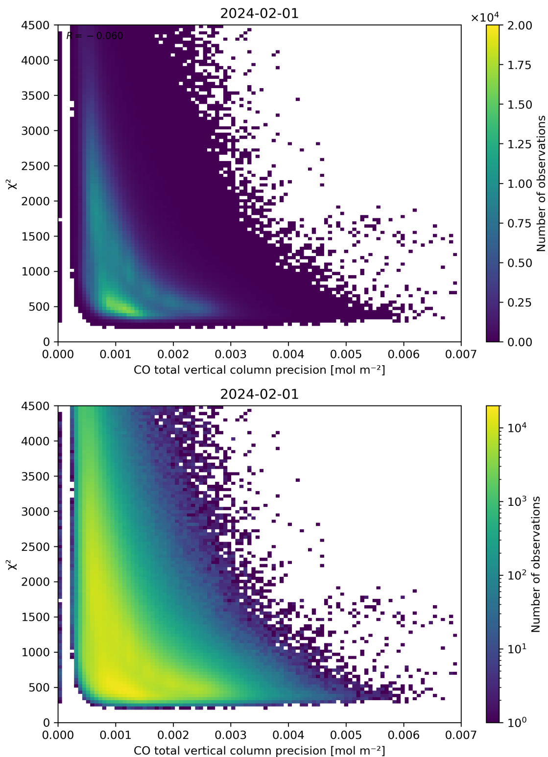
Figure 44: Scatter density plot of “CO total vertical column precision” against “ \chi^2 ” for 2024-01-31 to 2024-02-02.
