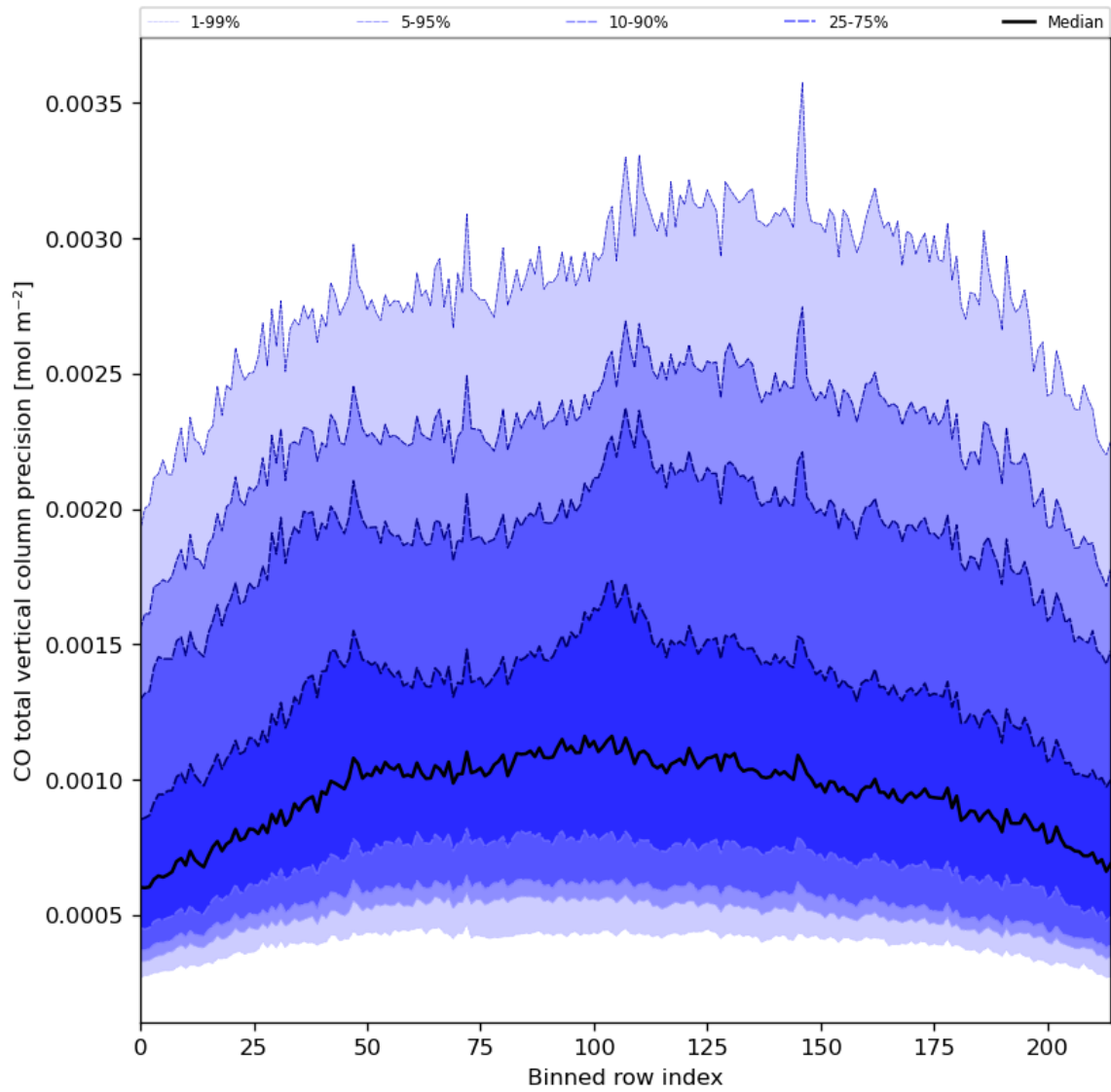
Figure 28: Along track statistics of “CO total vertical column precision” for 2024-01-31 to 2024-02-02
