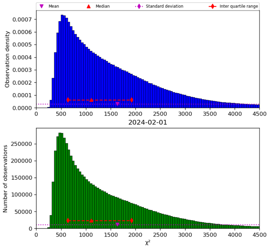
Figure 22: Histogram of " \chi^2 " for 2024-01-31 to 2024-02-02
