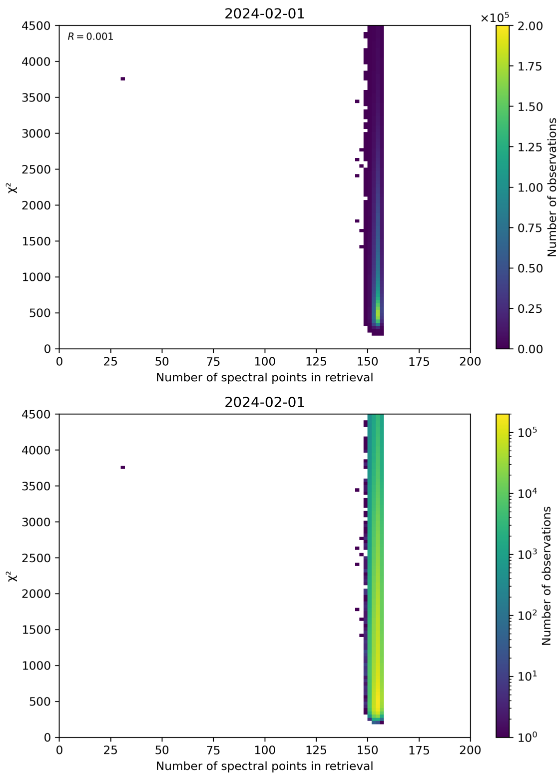
Figure 58: Scatter density plot of “Number of spectral points in retrieval” against “ \chi^2 ” for 2024-01-31 to 2024-02-02.
