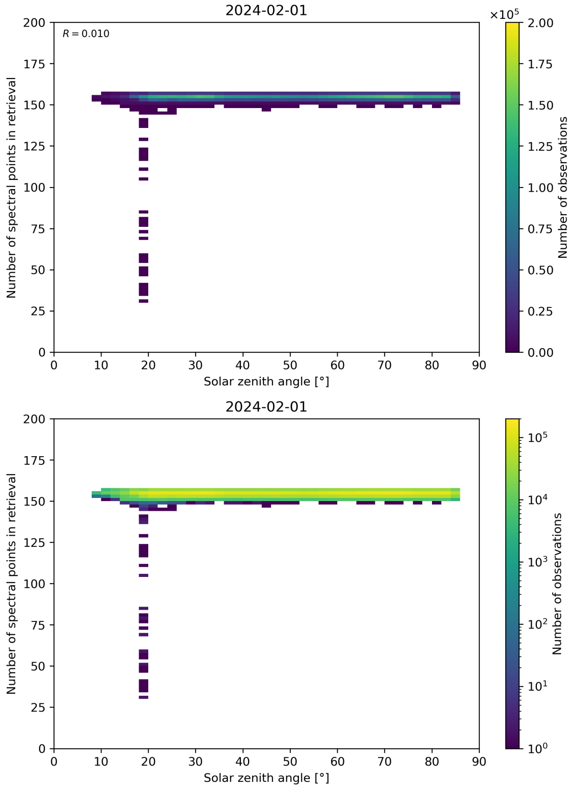
Figure 68: Scatter density plot of “Solar zenith angle” against “Number of spectral points in retrieval” for 2024-01-31 to 2024-02-02.
