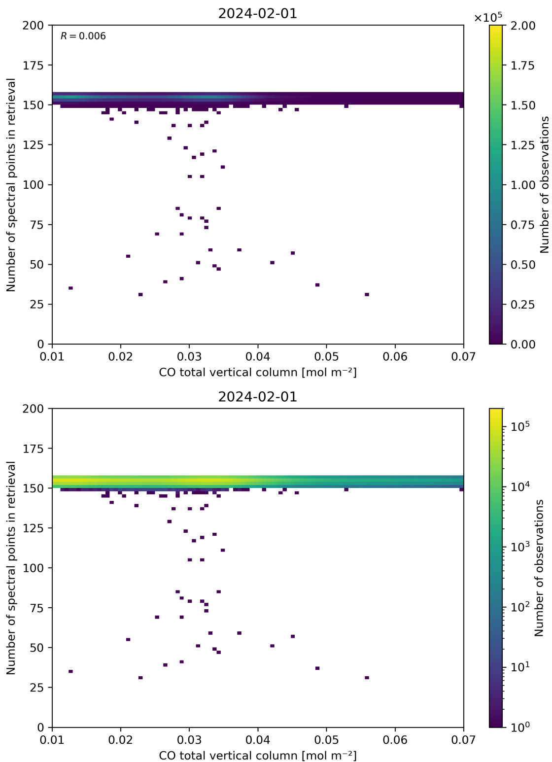
Figure 43: Scatter density plot of “CO total vertical column” against “Number of spectral points in retrieval” for 2024-01-31 to 2024-02-02.
