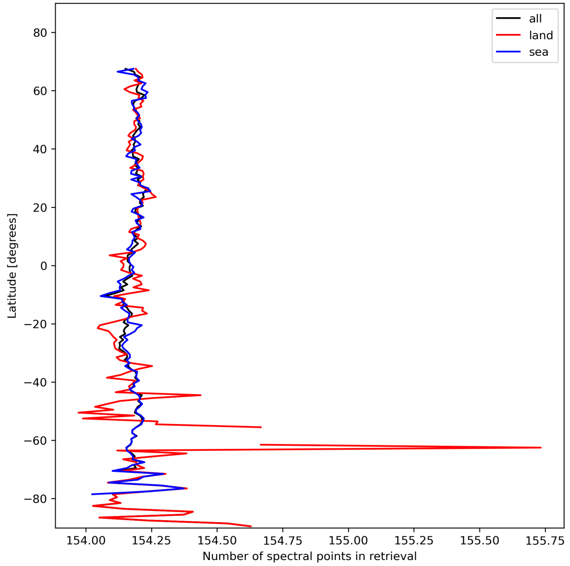
Figure 13: Zonal average of “Number of spectral points in retrieval” for 2024-01-31 to 2024-02-02.
