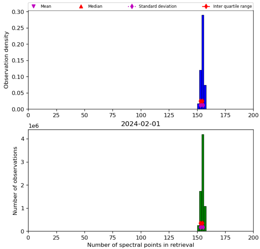
Figure 21: Histogram of “Number of spectral points in retrieval” for 2024-01-31 to 2024-02-02
