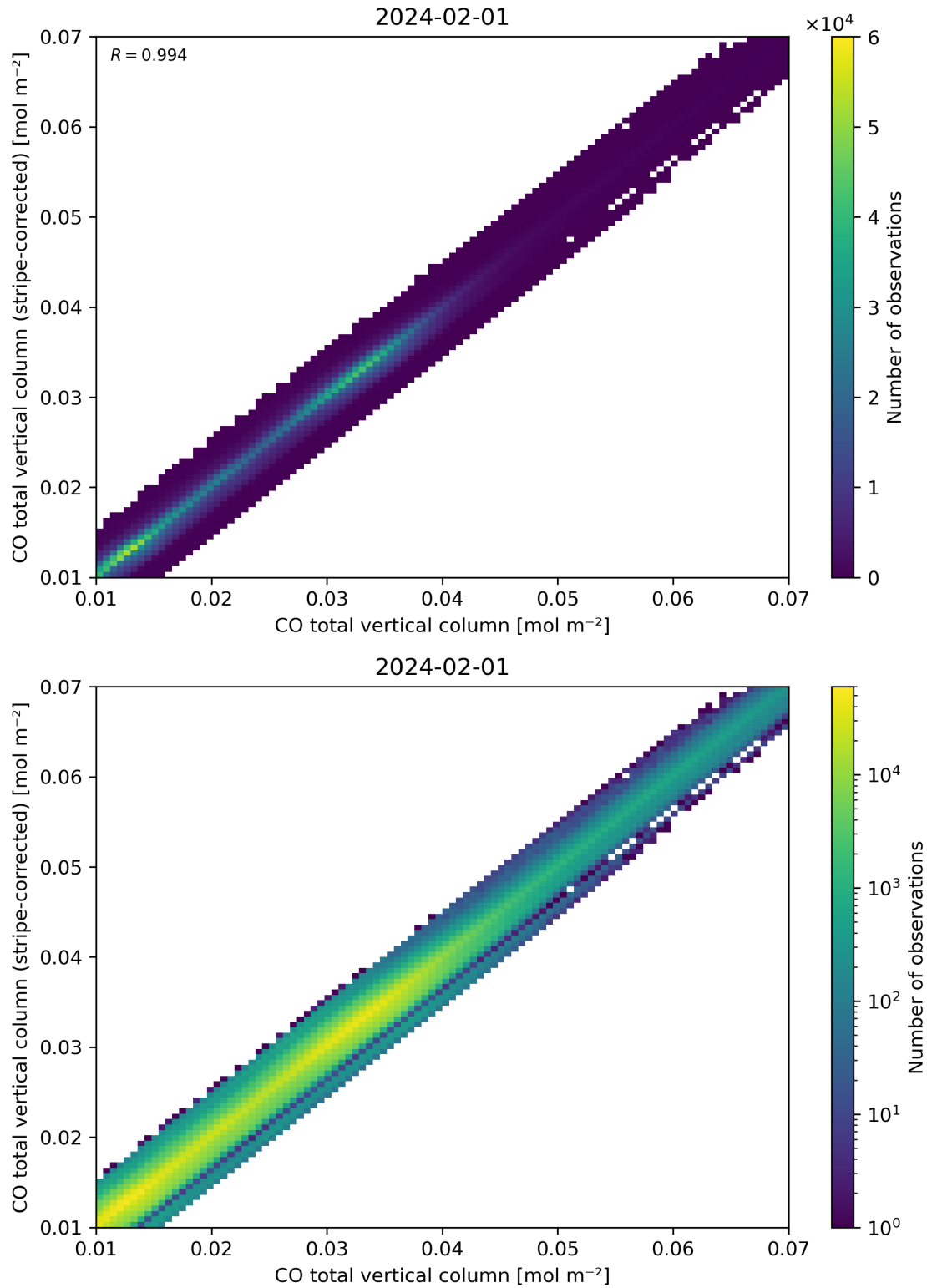
Figure 33: Scatter density plot of “CO total vertical column” against “CO total vertical column (stripe-corrected)” for 2024-01-31 to 2024-02-02.
