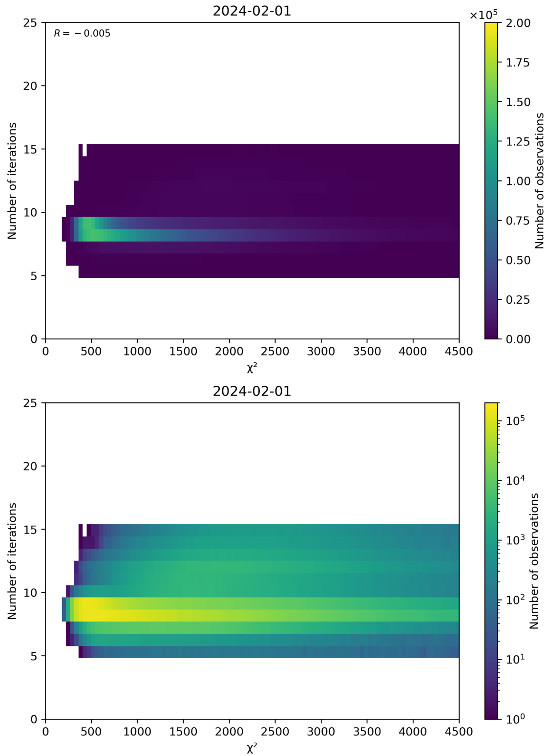
Figure 49: Scatter density plot of “ \chi^2 ” against “Number of iterations” for 2024-01-31 to 2024-02-02.
