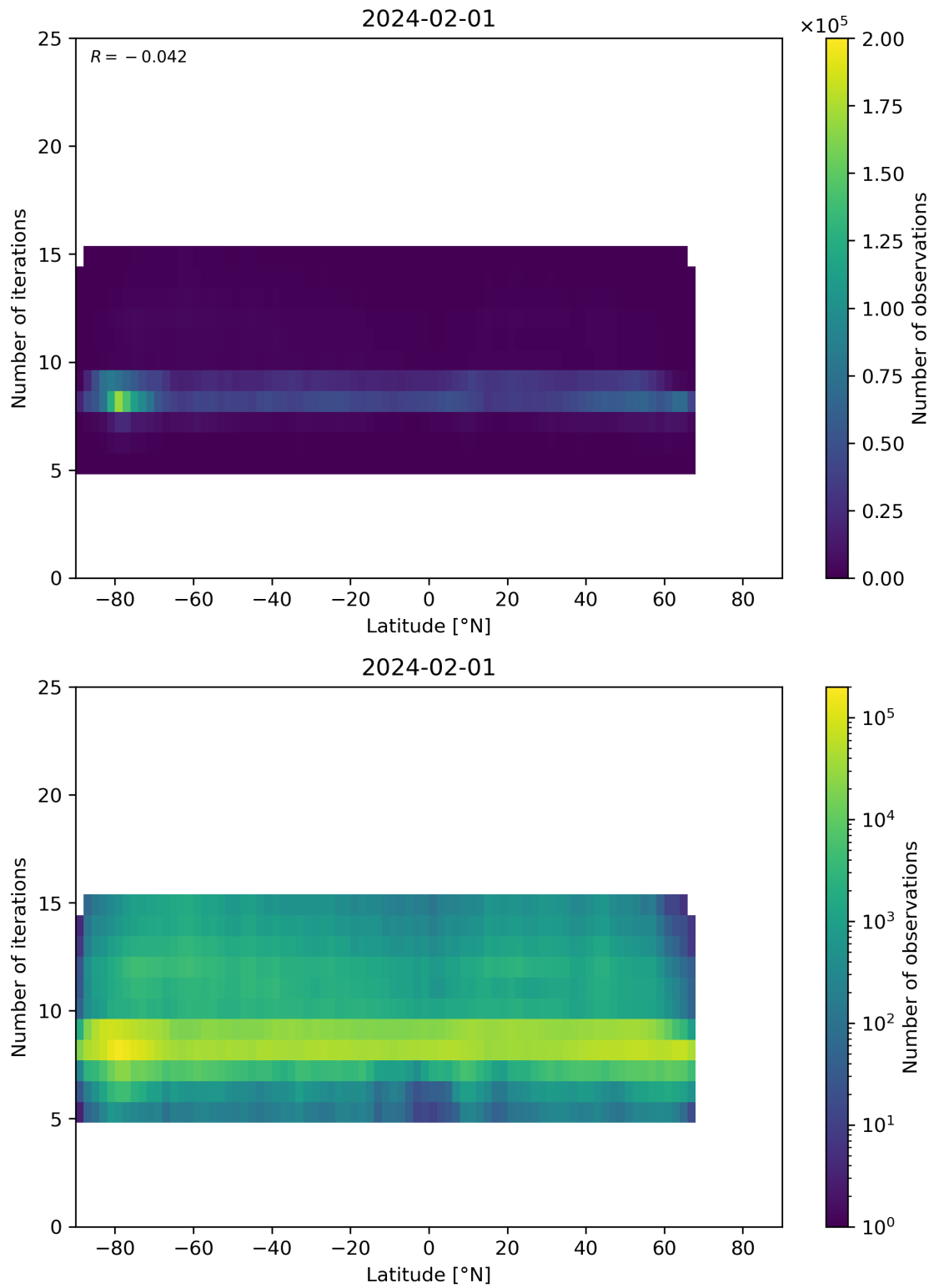
Figure 56: Scatter density plot of “Latitude” against “Number of iterations” for 2024-01-31 to 2024-02-02.
