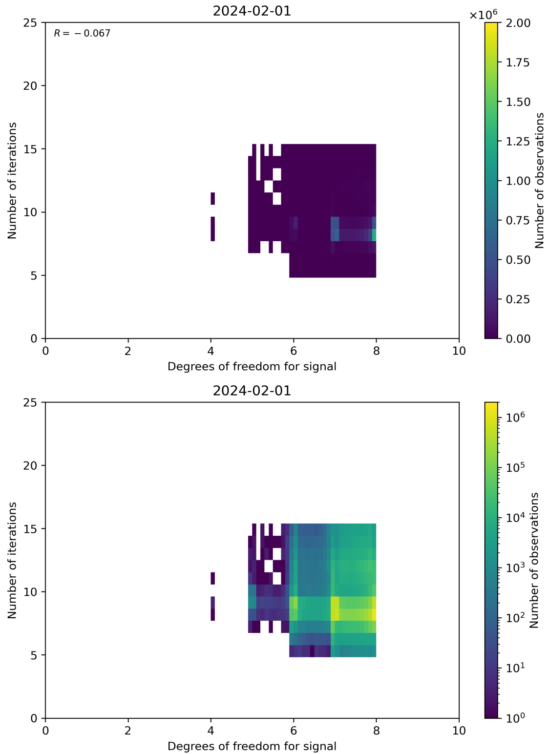
Figure 50: Scatter density plot of “Degrees of freedom for signal” against “Number of iterations” for 2024-01-31 to 2024-02-02.
