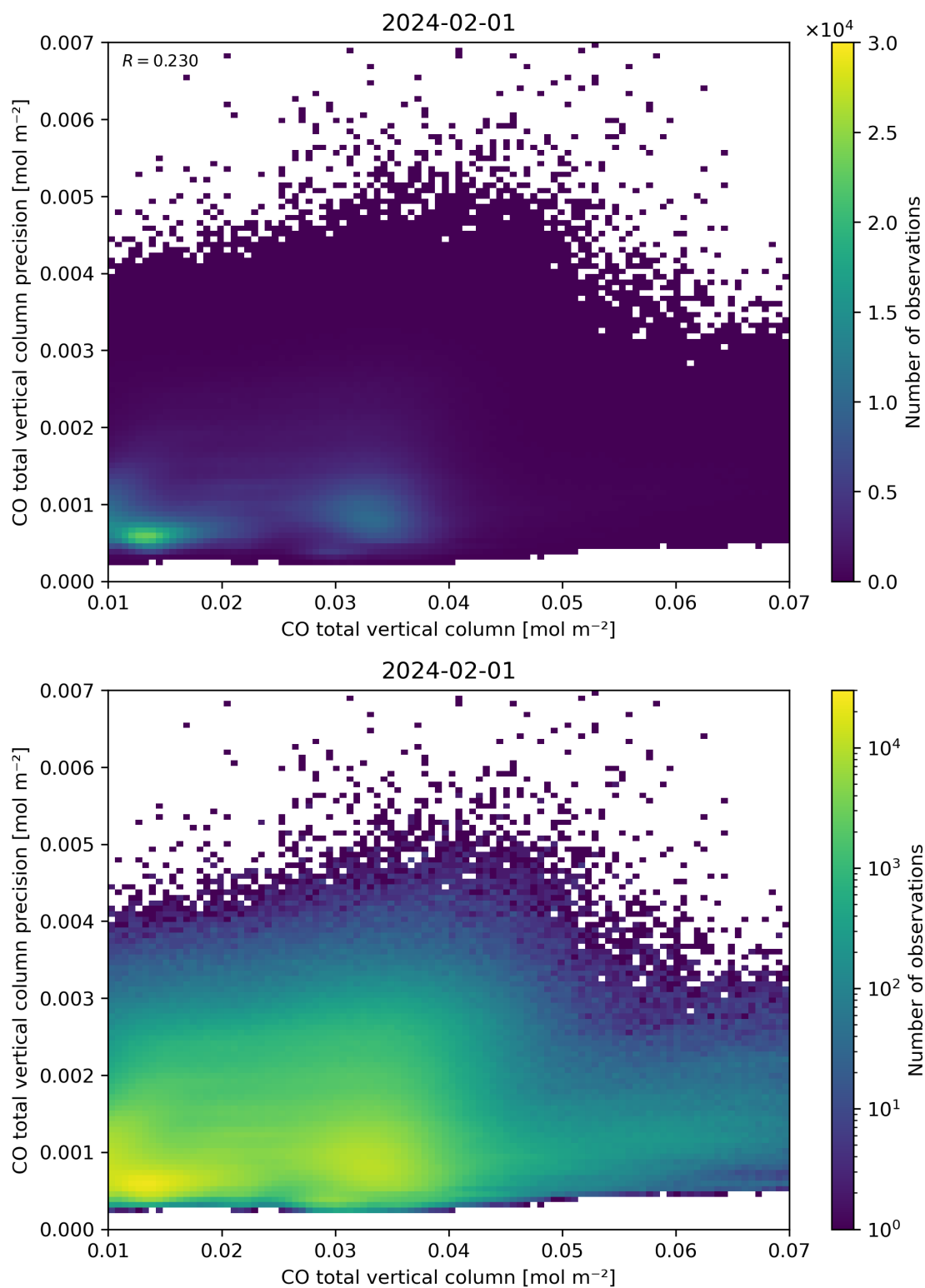
Figure 34: Scatter density plot of “CO total vertical column” against “CO total vertical column precision” for 2024-01-31 to 2024-02-02.
