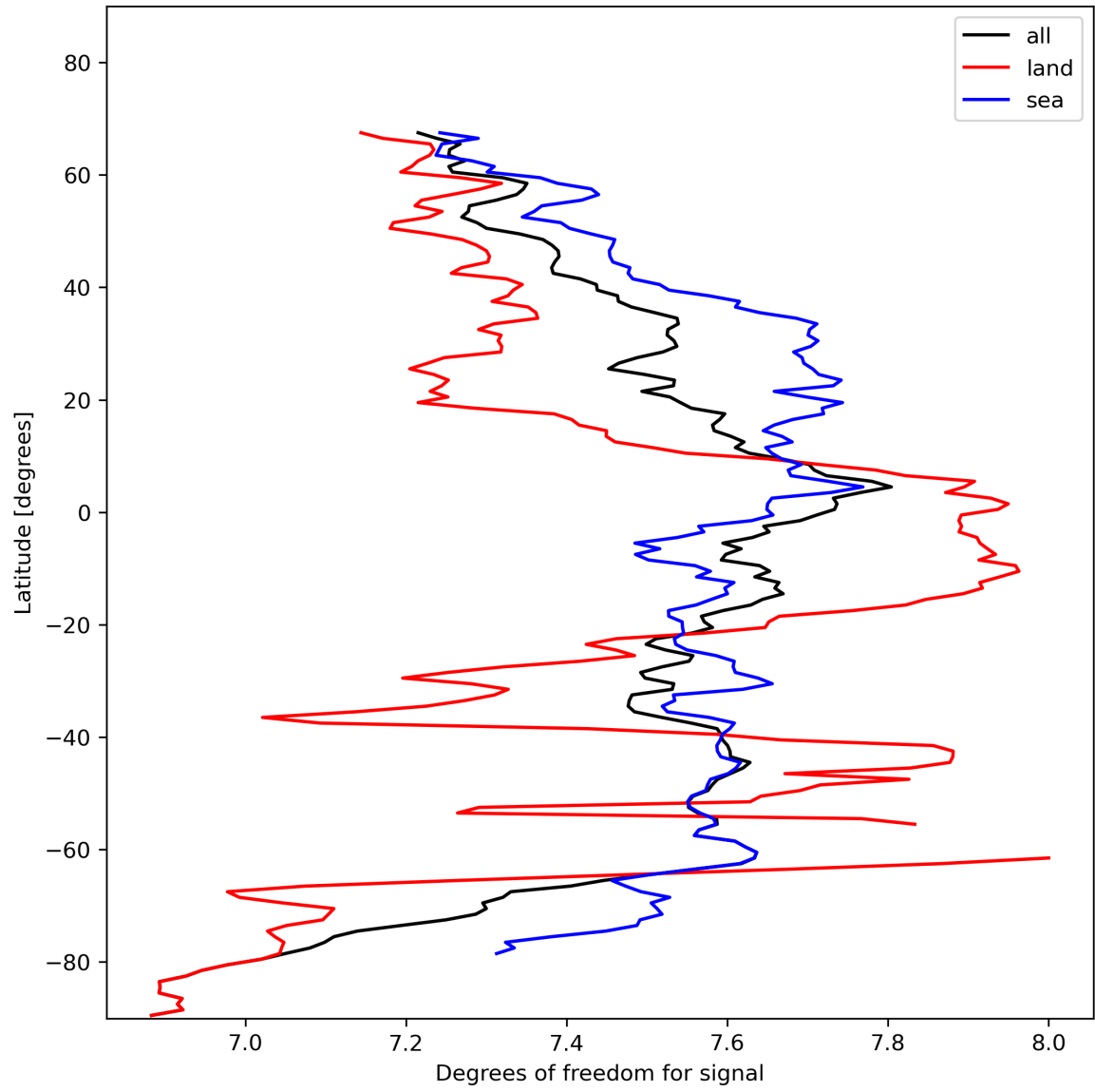
Figure 15: Zonal average of “Degrees of freedom for signal” for 2024-01-31 to 2024-02-02.
