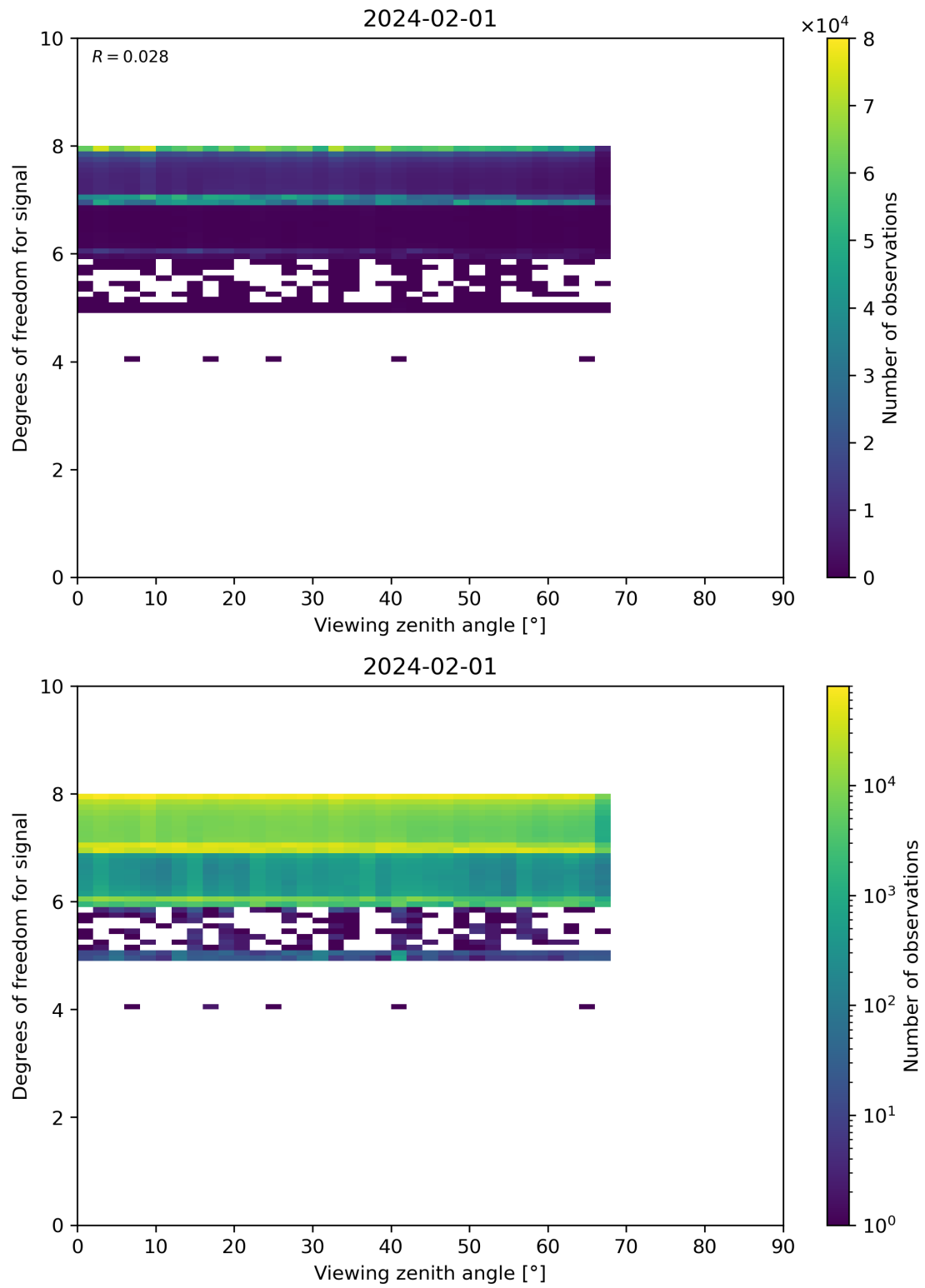
Figure 73: Scatter density plot of “Viewing zenith angle” against “Degrees of freedom for signal” for 2024-01-31 to 2024-02-02.
