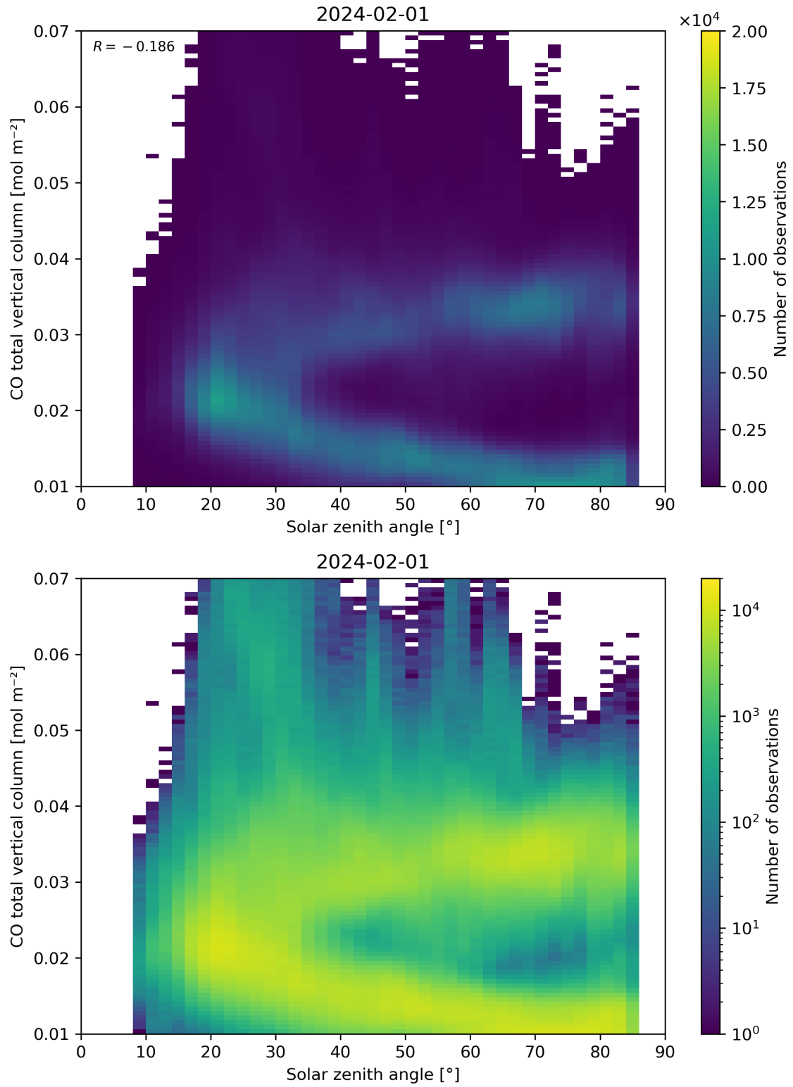
Figure 61: Scatter density plot of “Solar zenith angle” against “CO total vertical column” for 2024-01-31 to 2024-02-02.
