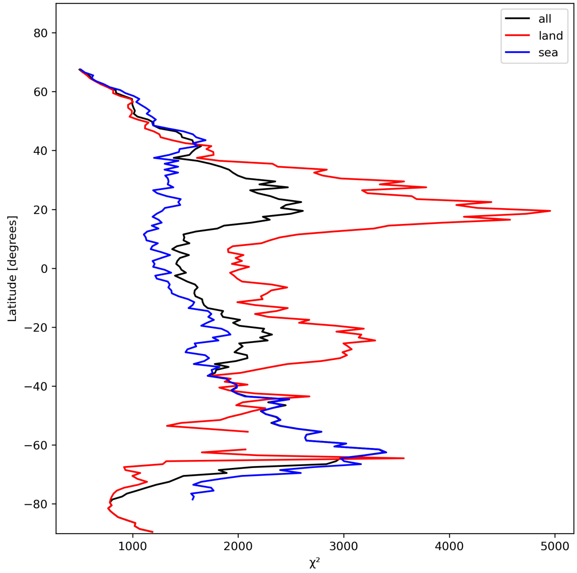
Figure 14: Zonal average of “ \chi^2 ” for 2024-01-31 to 2024-02-02.
