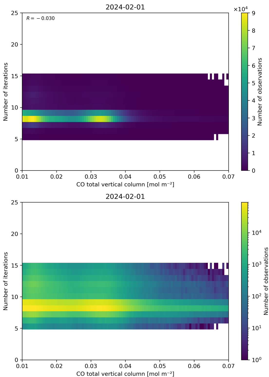
Figure 42: Scatter density plot of “CO total vertical column” against “Number of iterations” for 2024-01-31 to 2024-02-02.
