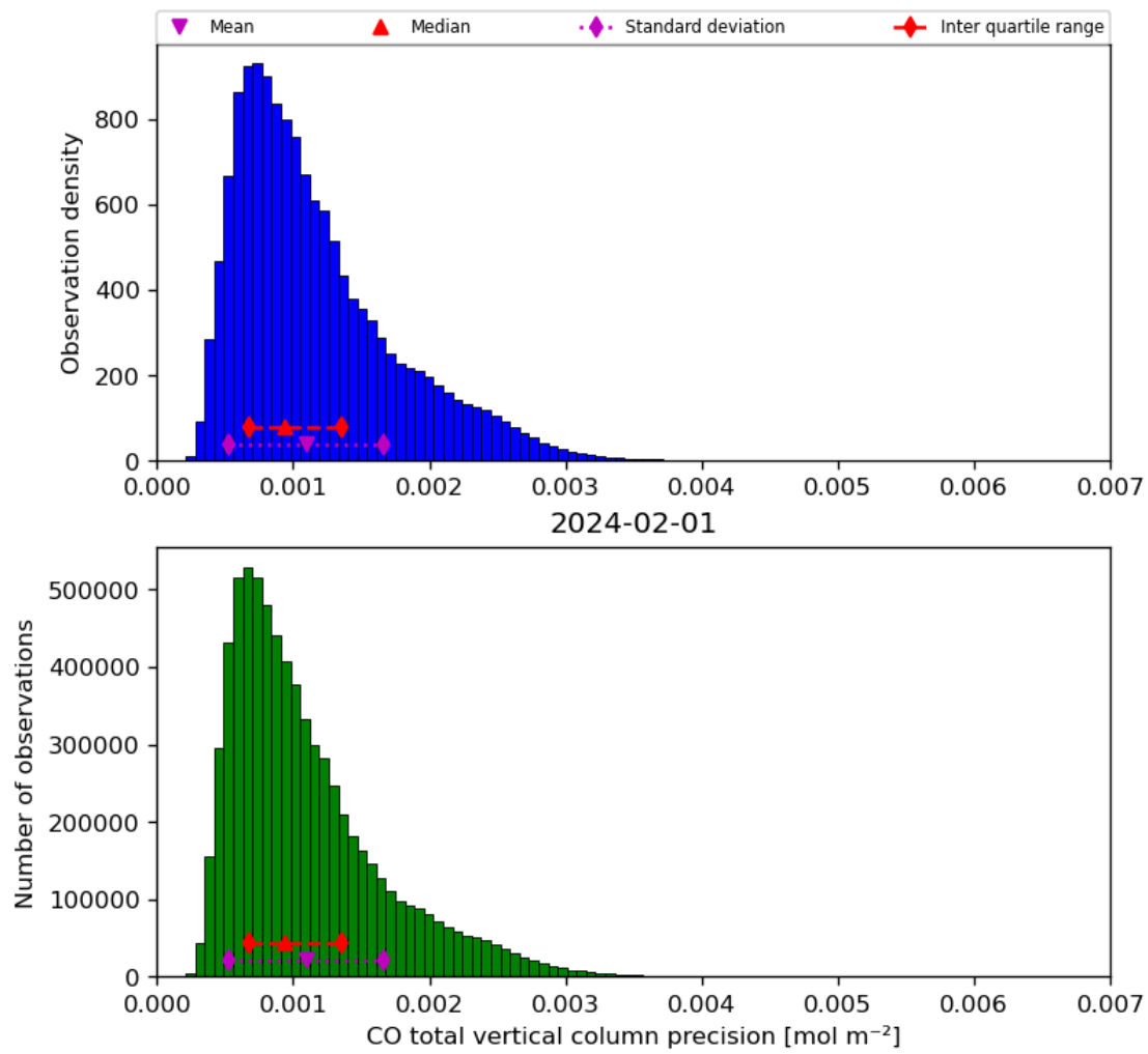
Figure 20: Histogram of “CO total vertical column precision” for 2024-01-31 to 2024-02-02
