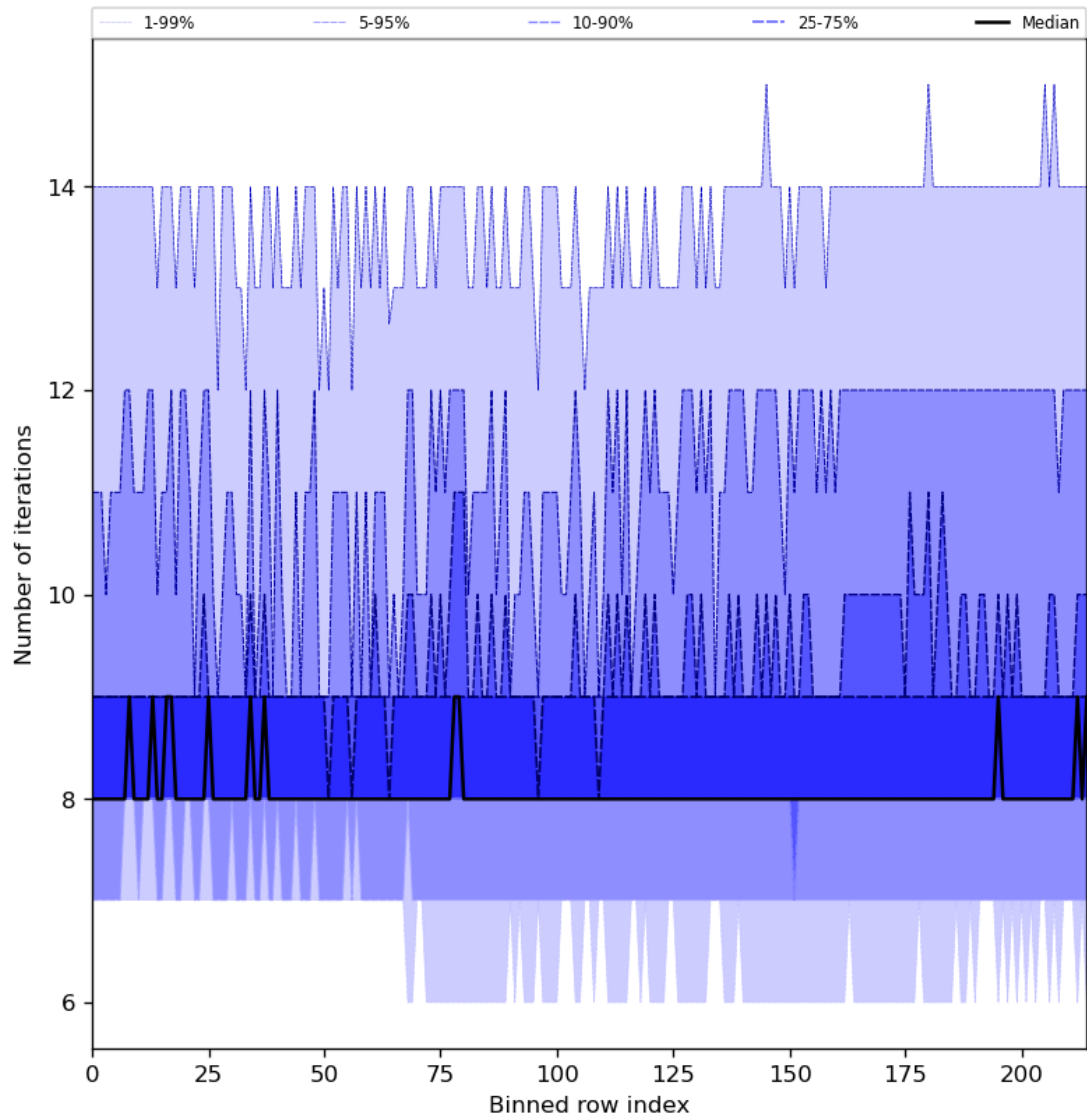
Figure 32: Along track statistics of “Number of iterations” for 2024-01-31 to 2024-02-02
