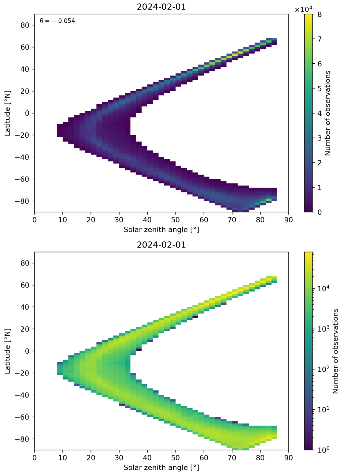
Figure 66: Scatter density plot of “Solar zenith angle” against “Latitude” for 2024-01-31 to 2024-02-02.
