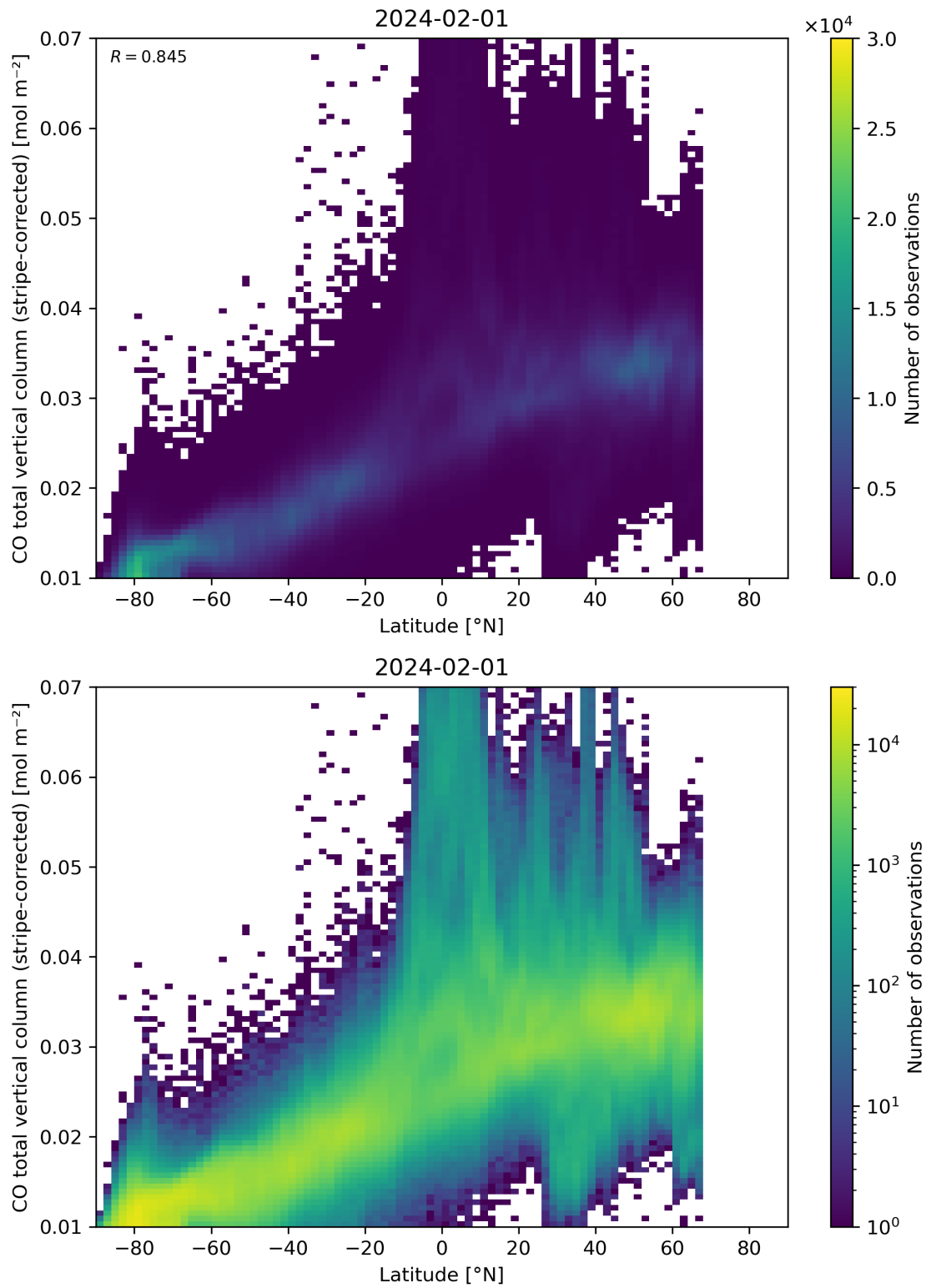
Figure 52: Scatter density plot of “Latitude” against “CO total vertical column (stripe-corrected)” for 2024-01-31 to 2024-02-02.
