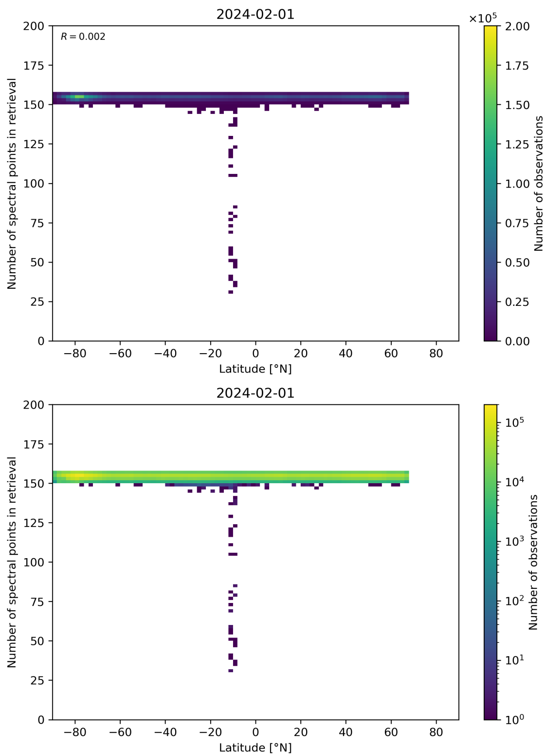
Figure 57: Scatter density plot of “Latitude” against “Number of spectral points in retrieval” for 2024-01-31 to 2024-02-02.
