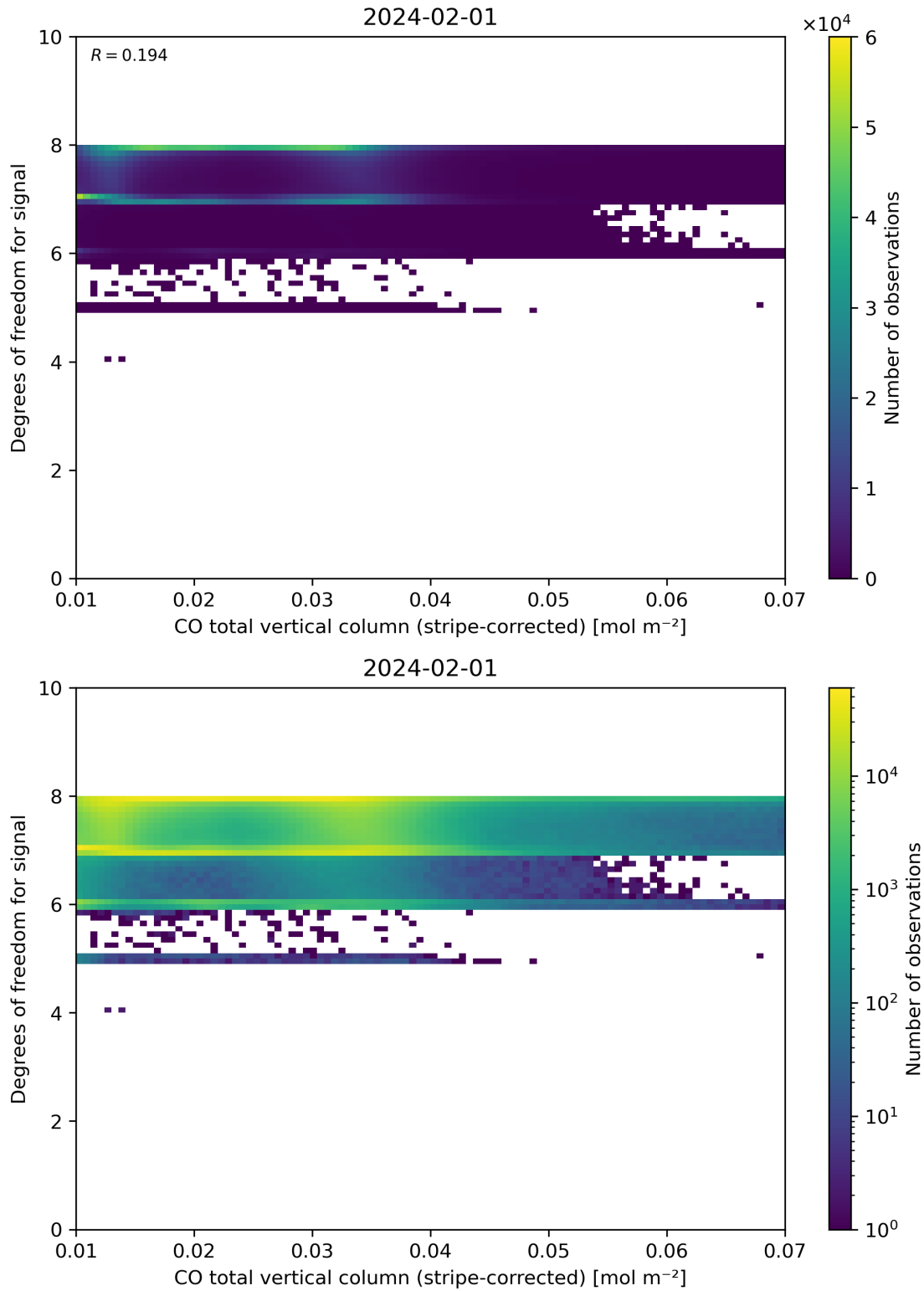
Figure 38: Scatter density plot of “CO total vertical column (stripe-corrected)” against “Degrees of freedom for signal” for 2024-01-31 to 2024-02-02.
