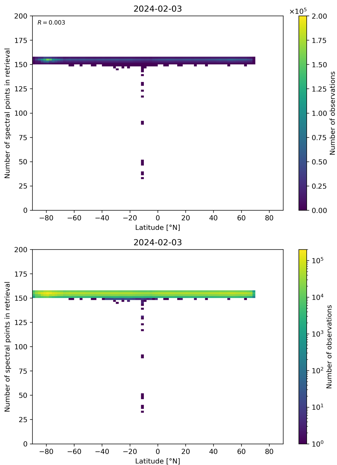
Figure 57: Scatter density plot of “Latitude” against “Number of spectral points in retrieval” for 2024-02-02 to 2024-02-04.
