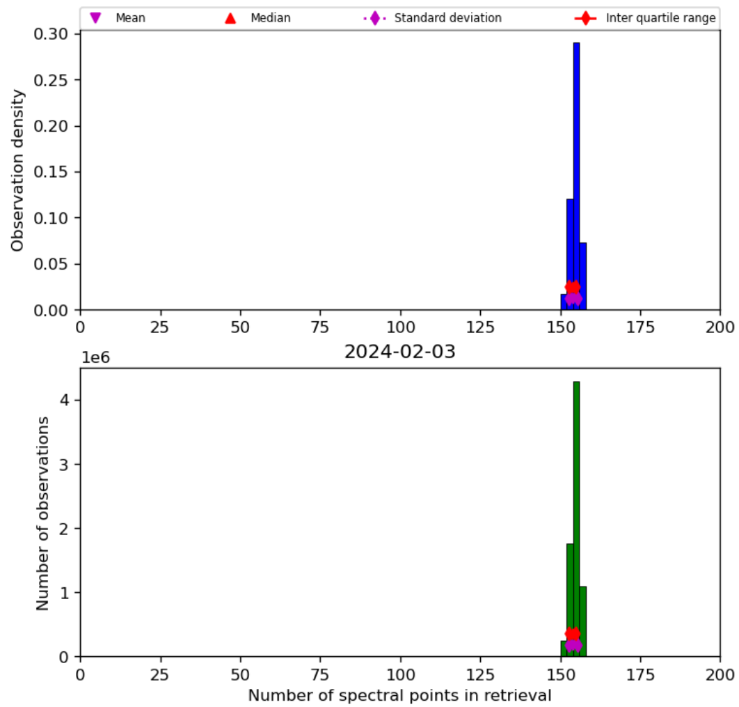
Figure 21: Histogram of “Number of spectral points in retrieval” for 2024-02-02 to 2024-02-04
