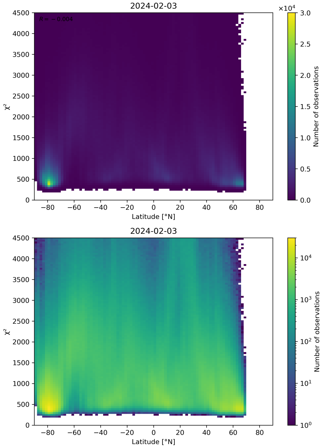
Figure 54: Scatter density plot of “Latitude” against “ \chi^2 ” for 2024-02-02 to 2024-02-04.
