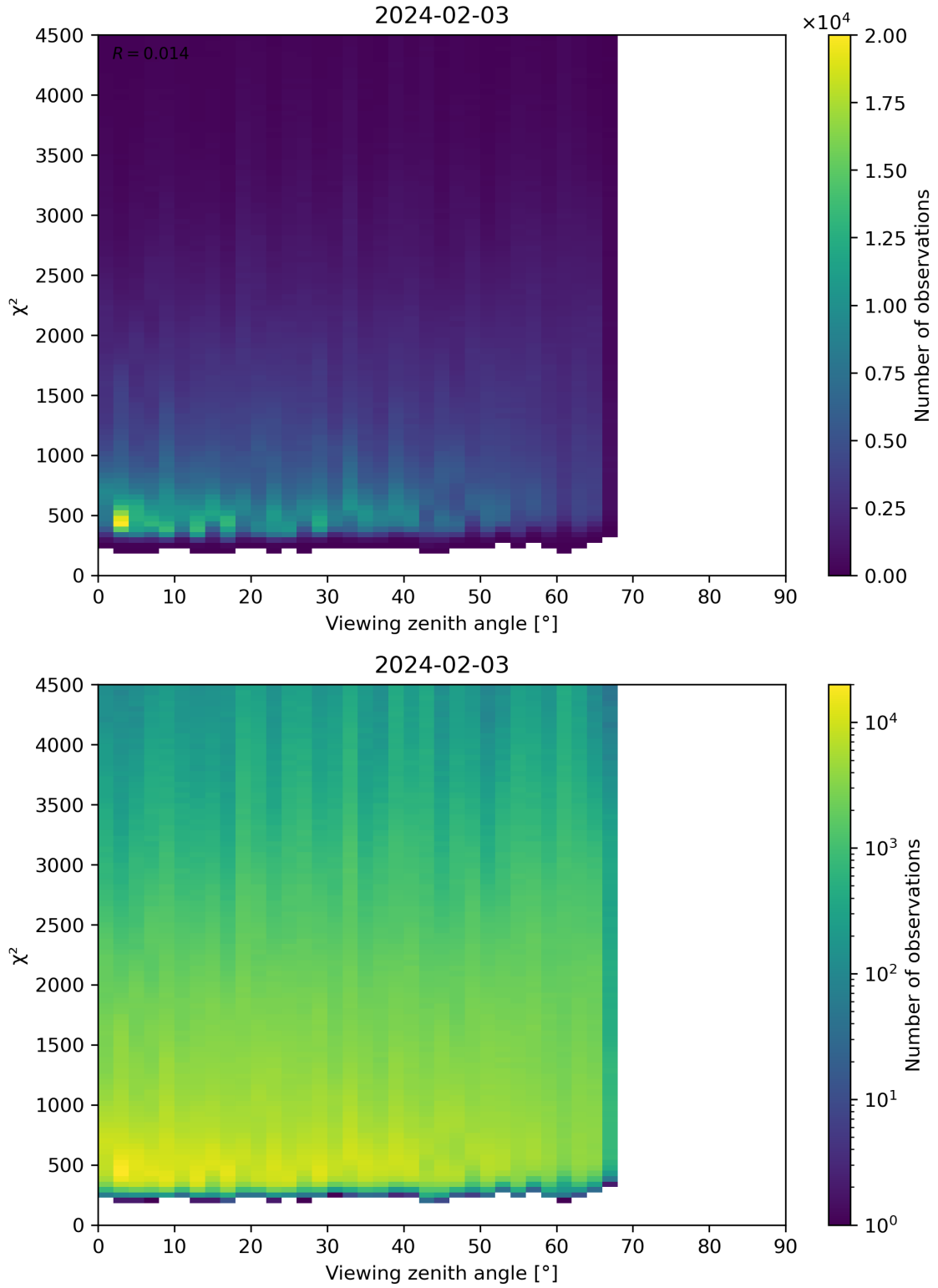
Figure 72: Scatter density plot of “Viewing zenith angle” against “ \chi^2 ” for 2024-02-02 to 2024-02-04.
