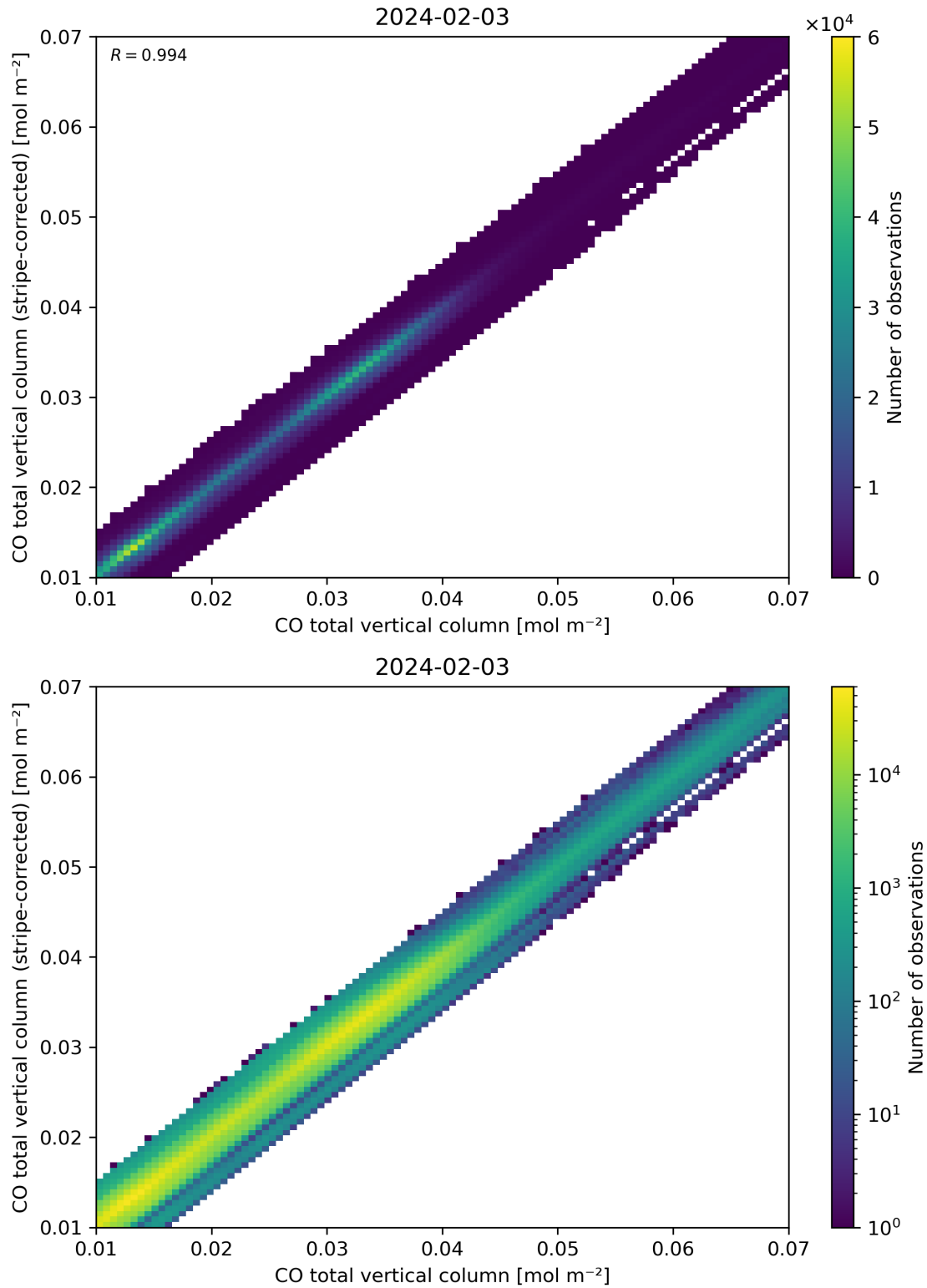
Figure 33: Scatter density plot of “CO total vertical column” against “CO total vertical column (stripe-corrected)” for 2024-02-02 to 2024-02-04.
