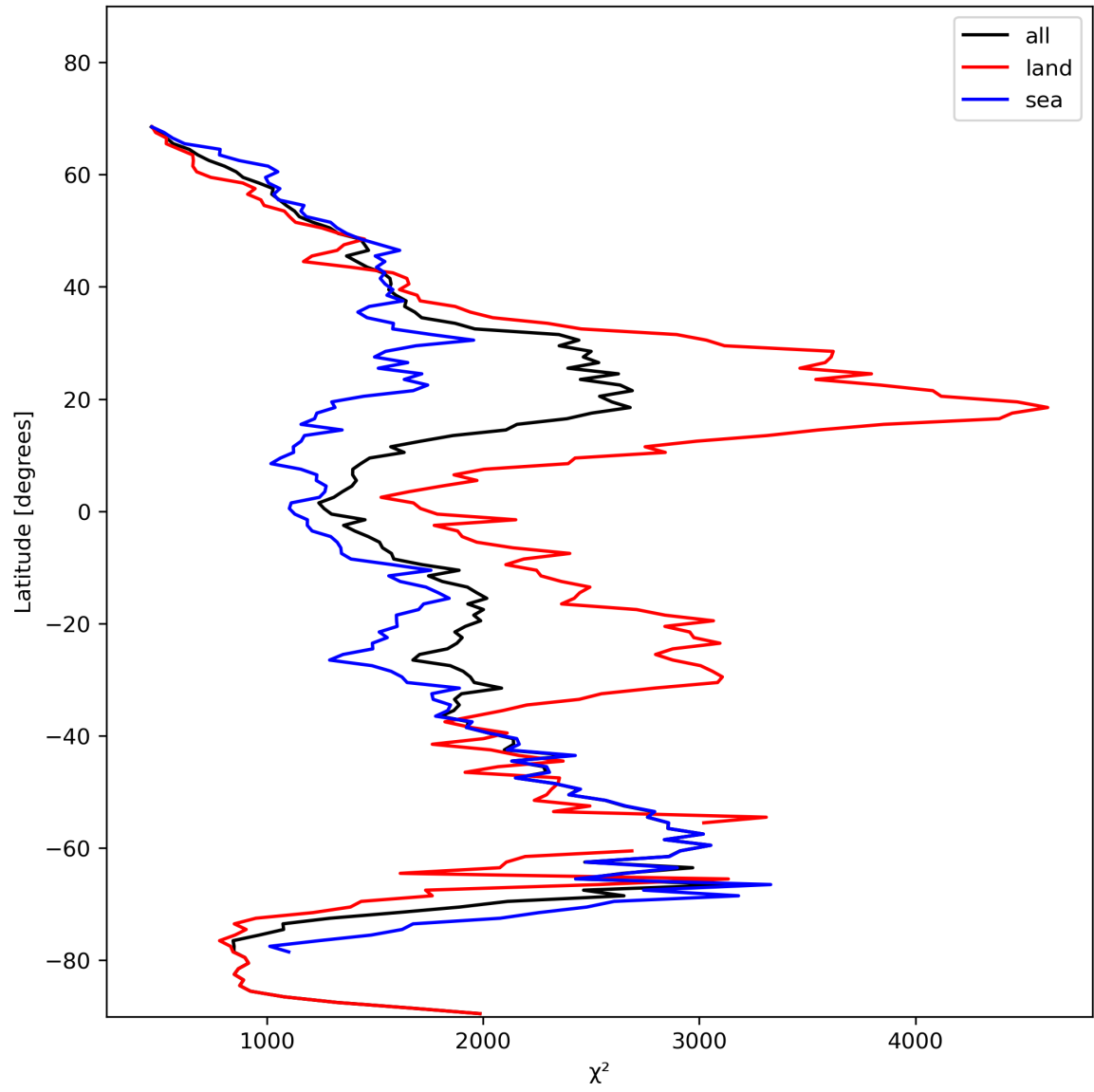
Figure 14: Zonal average of “ \chi^2 ” for 2024-02-02 to 2024-02-04.
