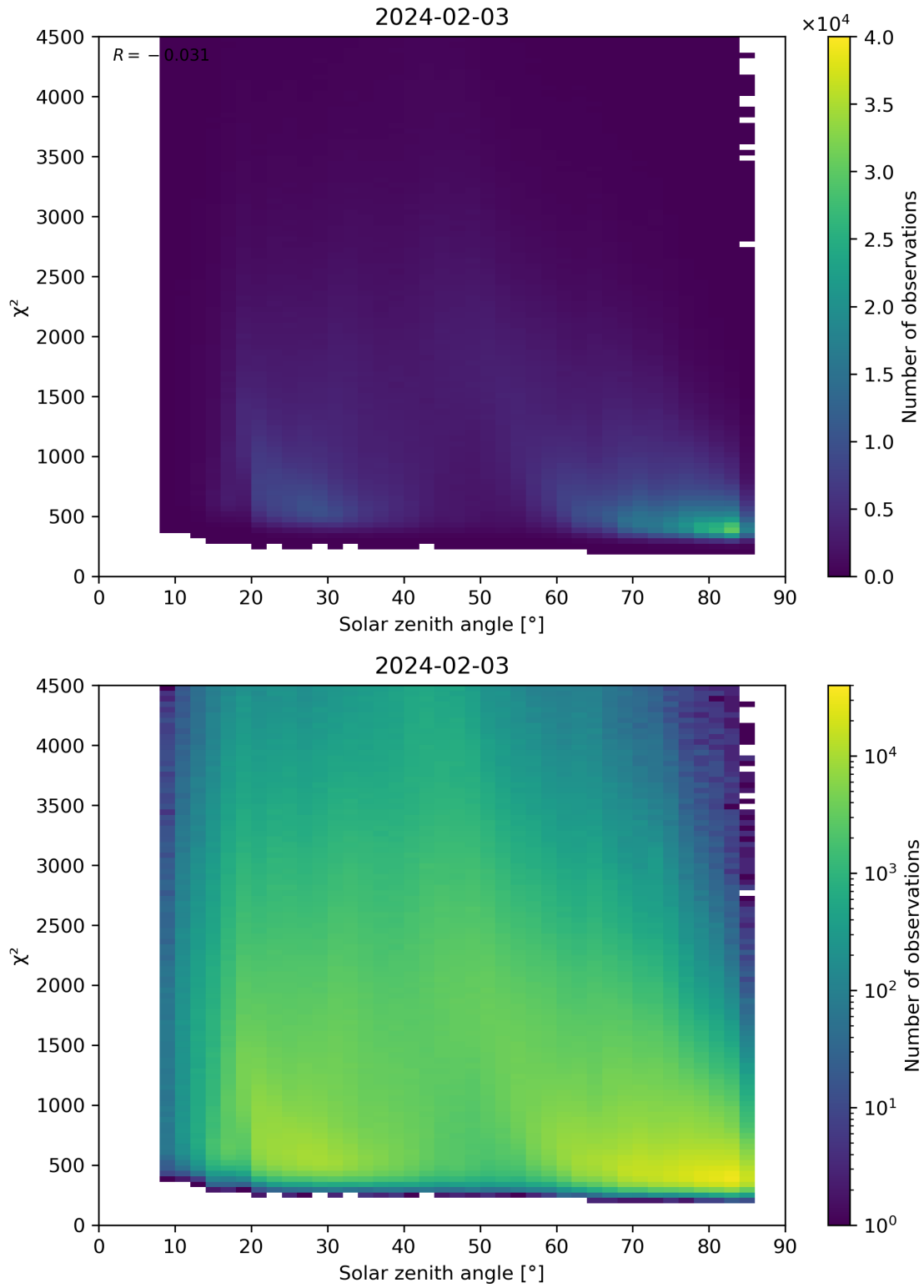
Figure 64: Scatter density plot of “Solar zenith angle” against “ \chi^2 ” for 2024-02-02 to 2024-02-04.
