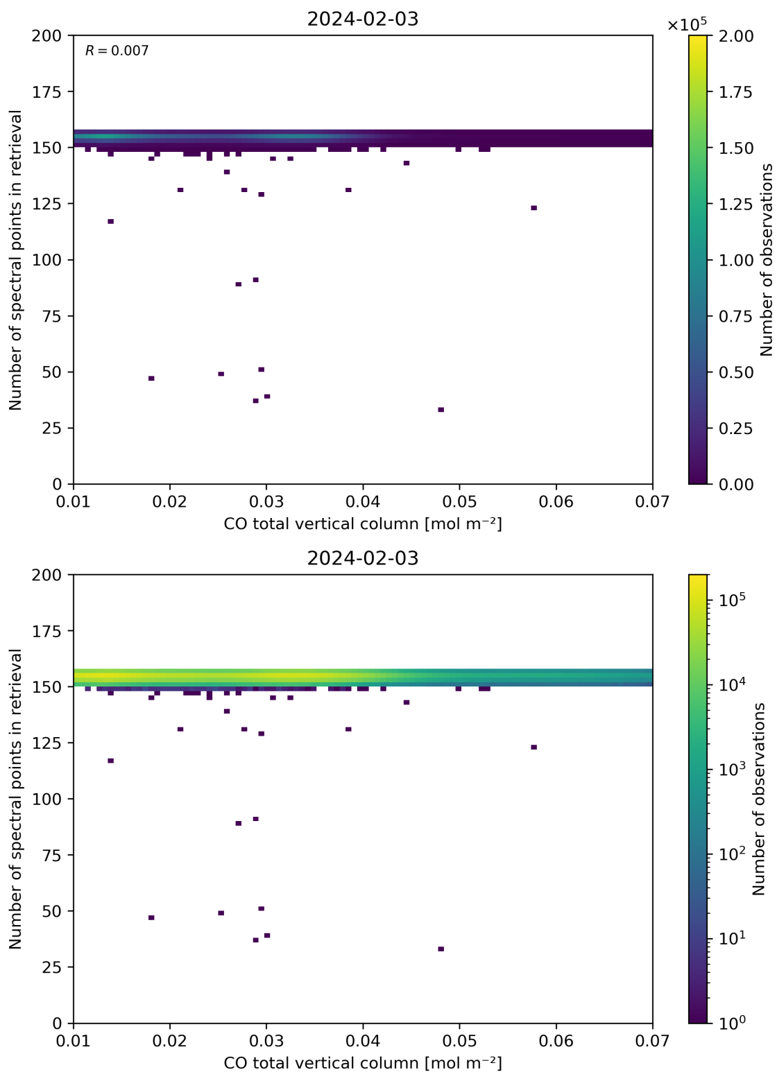
Figure 43: Scatter density plot of “CO total vertical column” against “Number of spectral points in retrieval” for 2024-02-02 to 2024-02-04.
