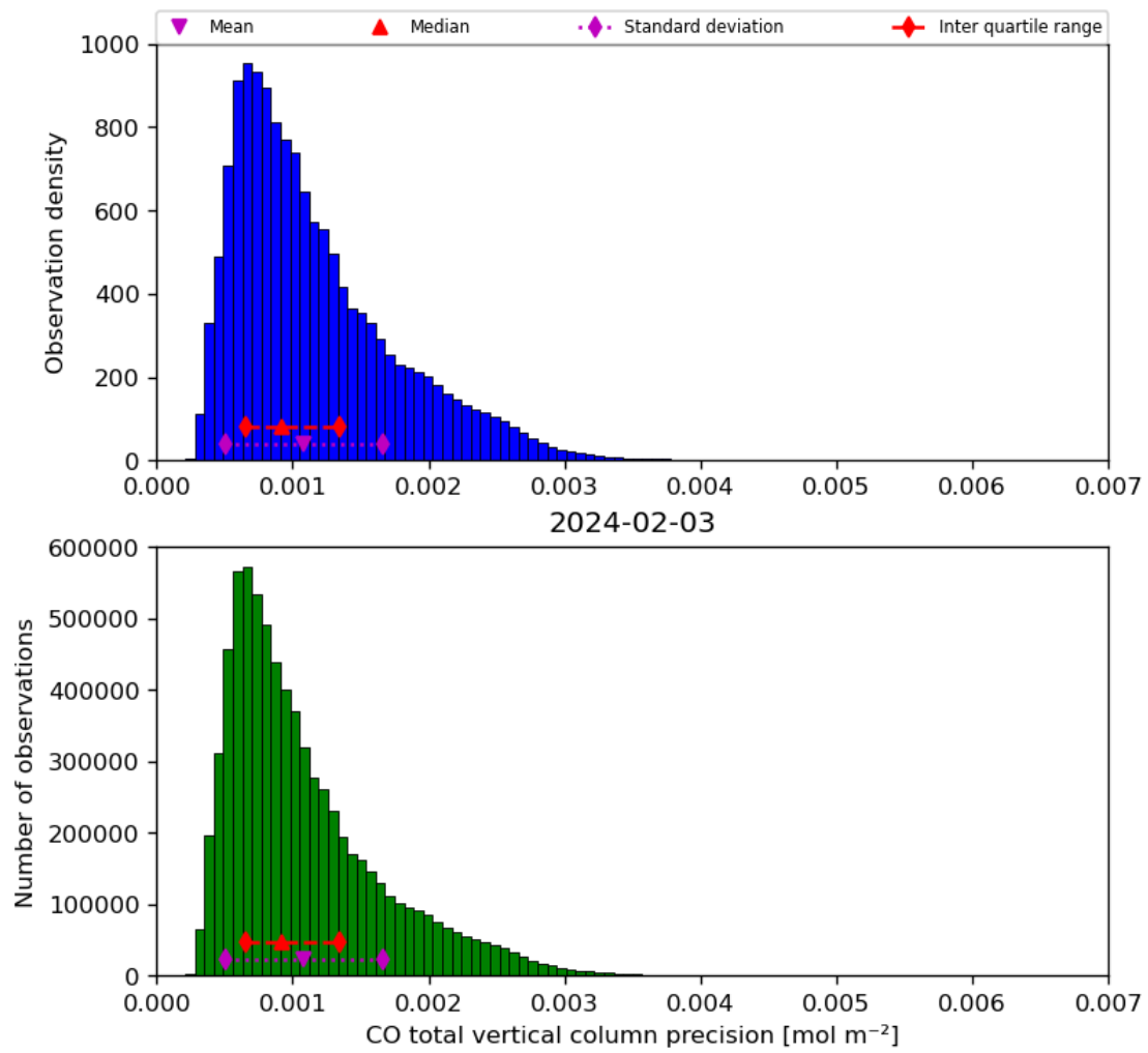
Figure 20: Histogram of “CO total vertical column precision” for 2024-02-02 to 2024-02-04
