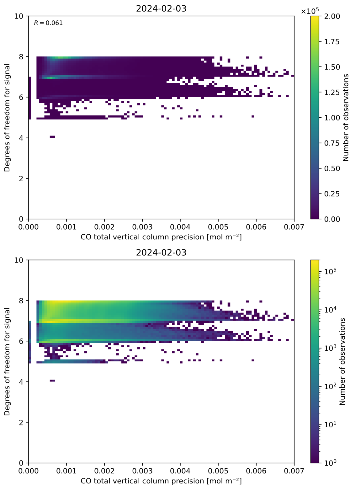
Figure 45: Scatter density plot of “CO total vertical column precision” against “Degrees of freedom for signal” for 2024-02-02 to 2024-02-04.
