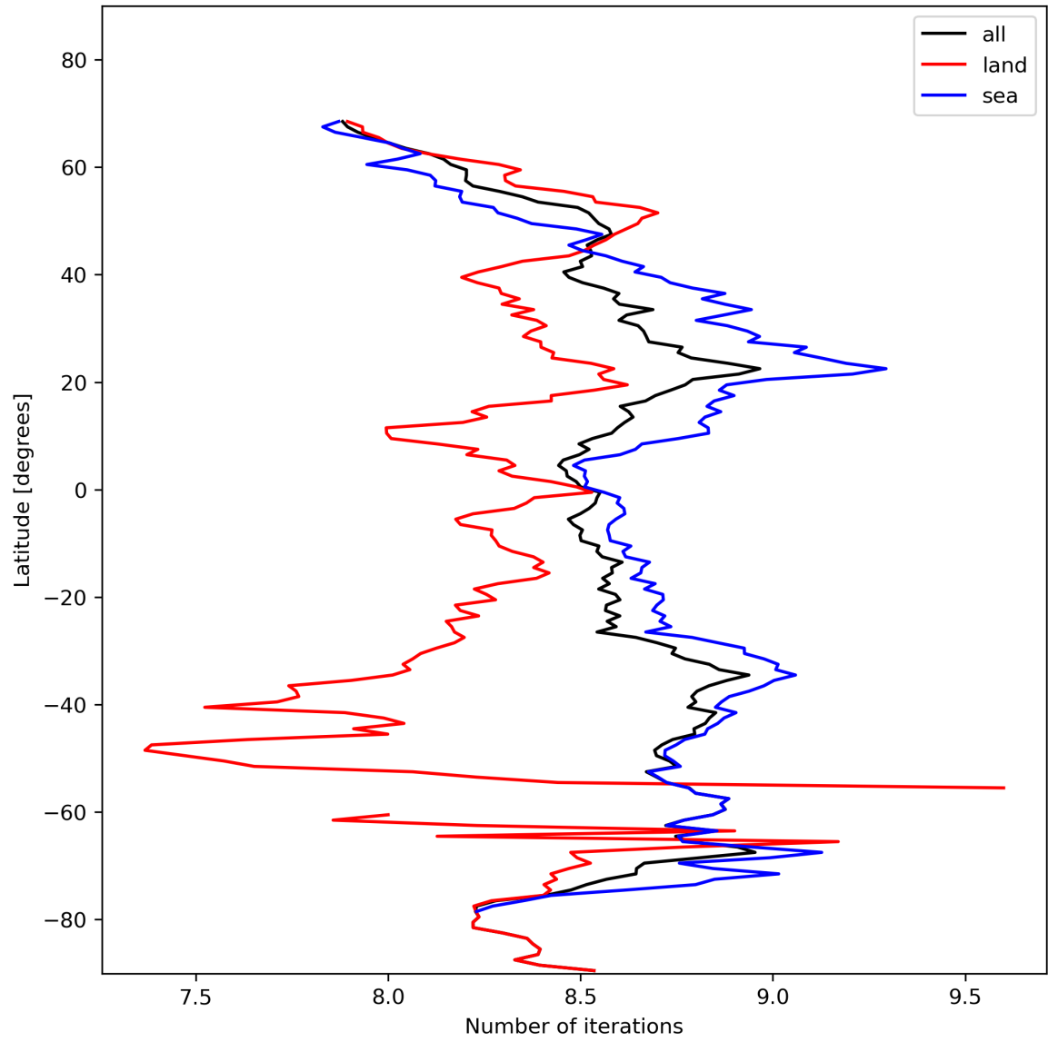
Figure 16: Zonal average of “Number of iterations” for 2024-02-02 to 2024-02-04.
