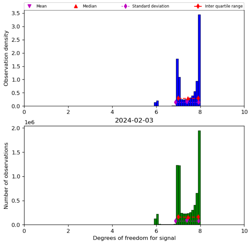
Figure 23: Histogram of “Degrees of freedom for signal” for 2024-02-02 to 2024-02-04
