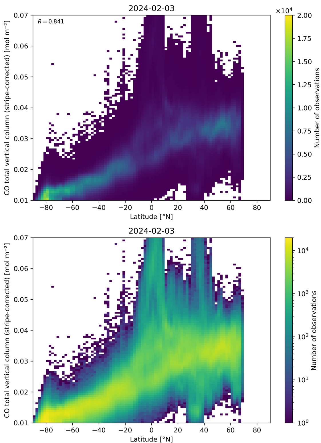
Figure 52: Scatter density plot of “Latitude” against “CO total vertical column (stripe-corrected)” for 2024-02-02 to 2024-02-04.
