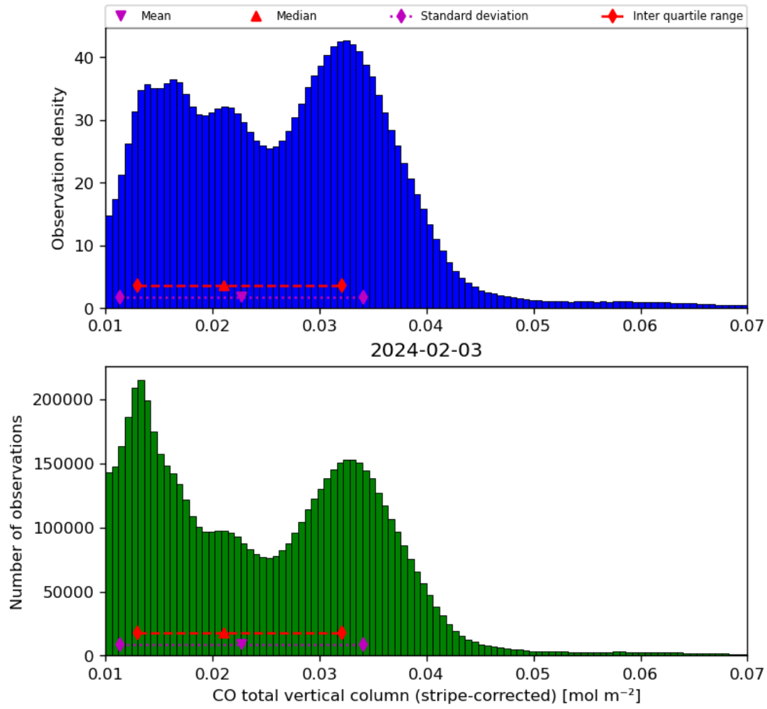
Figure 19: Histogram of “CO total vertical column (stripe-corrected)” for 2024-02-02 to 2024-02-04
