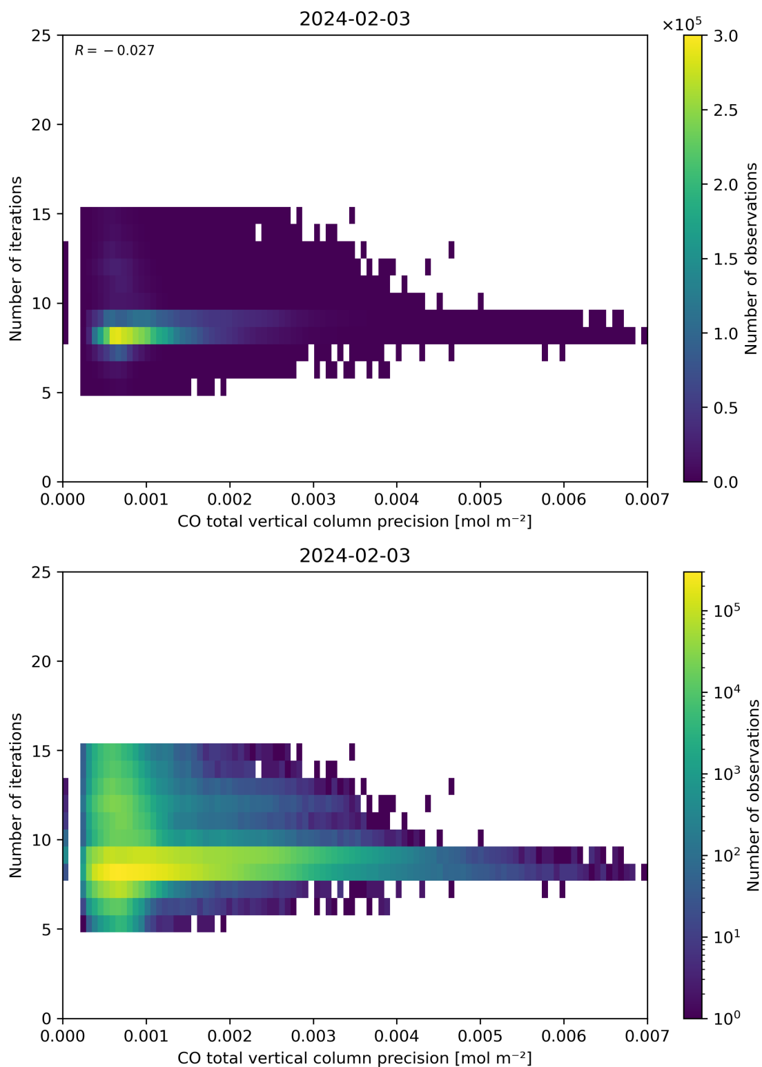
Figure 46: Scatter density plot of “CO total vertical column precision” against “Number of iterations” for 2024-02-02 to 2024-02-04.
