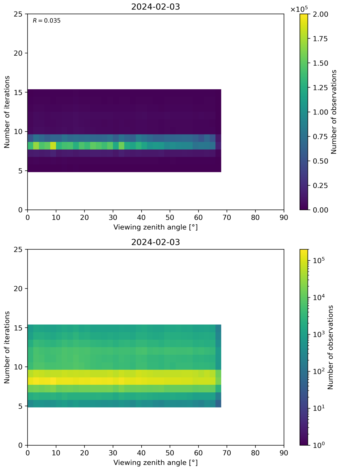
Figure 75: Scatter density plot of “Viewing zenith angle” against “Number of iterations” for 2024-02-02 to 2024-02-04.
