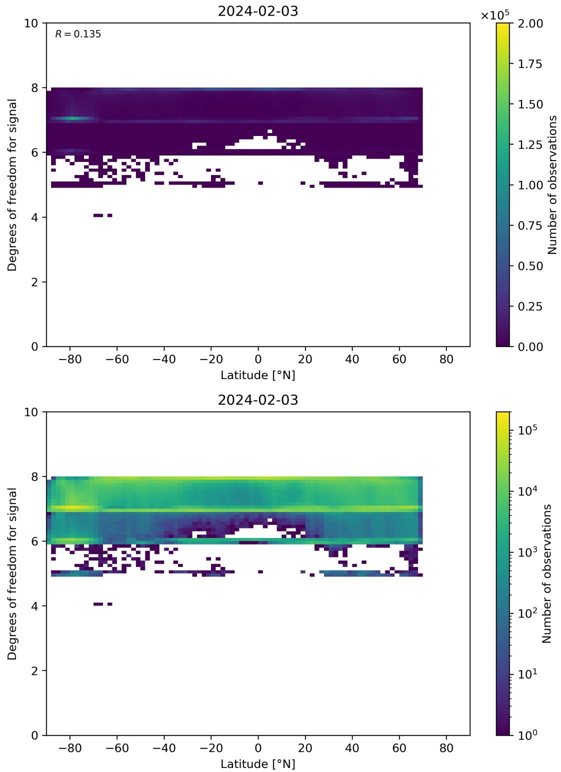
Figure 55: Scatter density plot of “Latitude” against “Degrees of freedom for signal” for 2024-02-02 to 2024-02-04.
