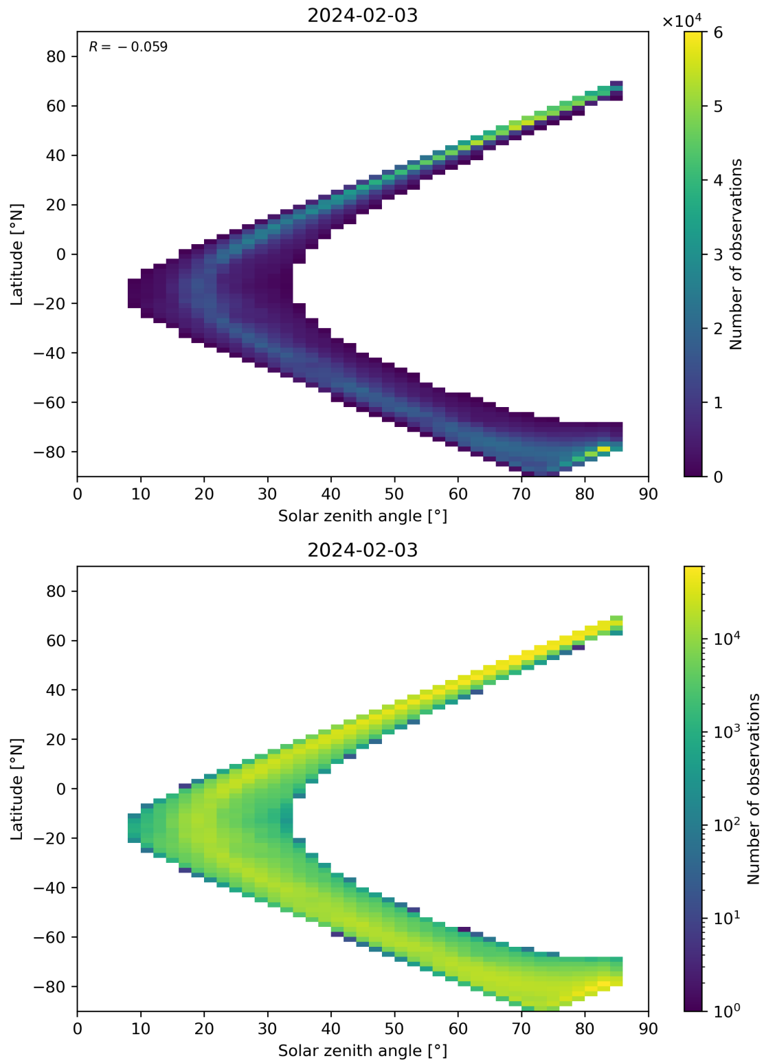
Figure 66: Scatter density plot of “Solar zenith angle” against “Latitude” for 2024-02-02 to 2024-02-04.
