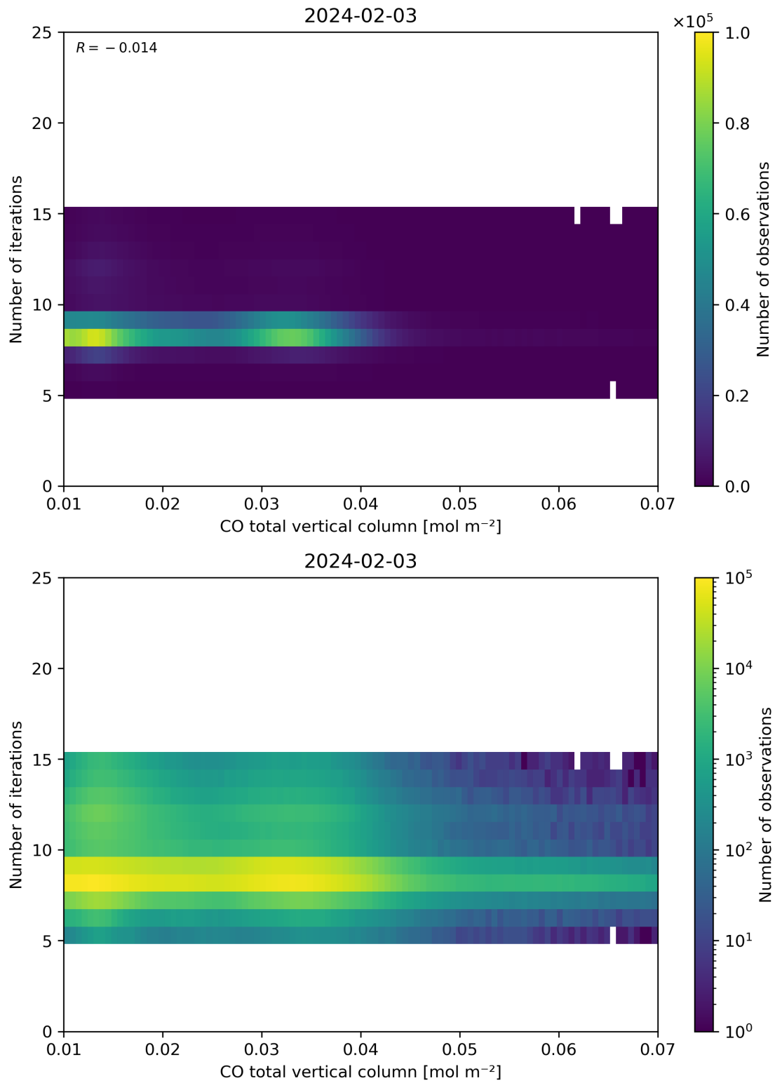
Figure 42: Scatter density plot of “CO total vertical column” against “Number of iterations” for 2024-02-02 to 2024-02-04.
