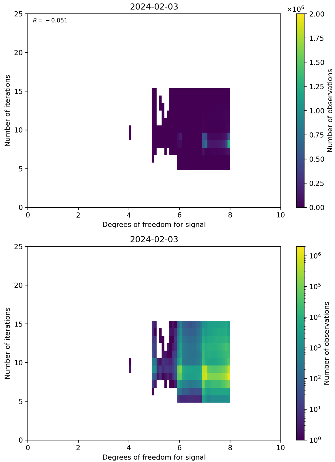
Figure 50: Scatter density plot of “Degrees of freedom for signal” against “Number of iterations” for 2024-02-02 to 2024-02-04.
