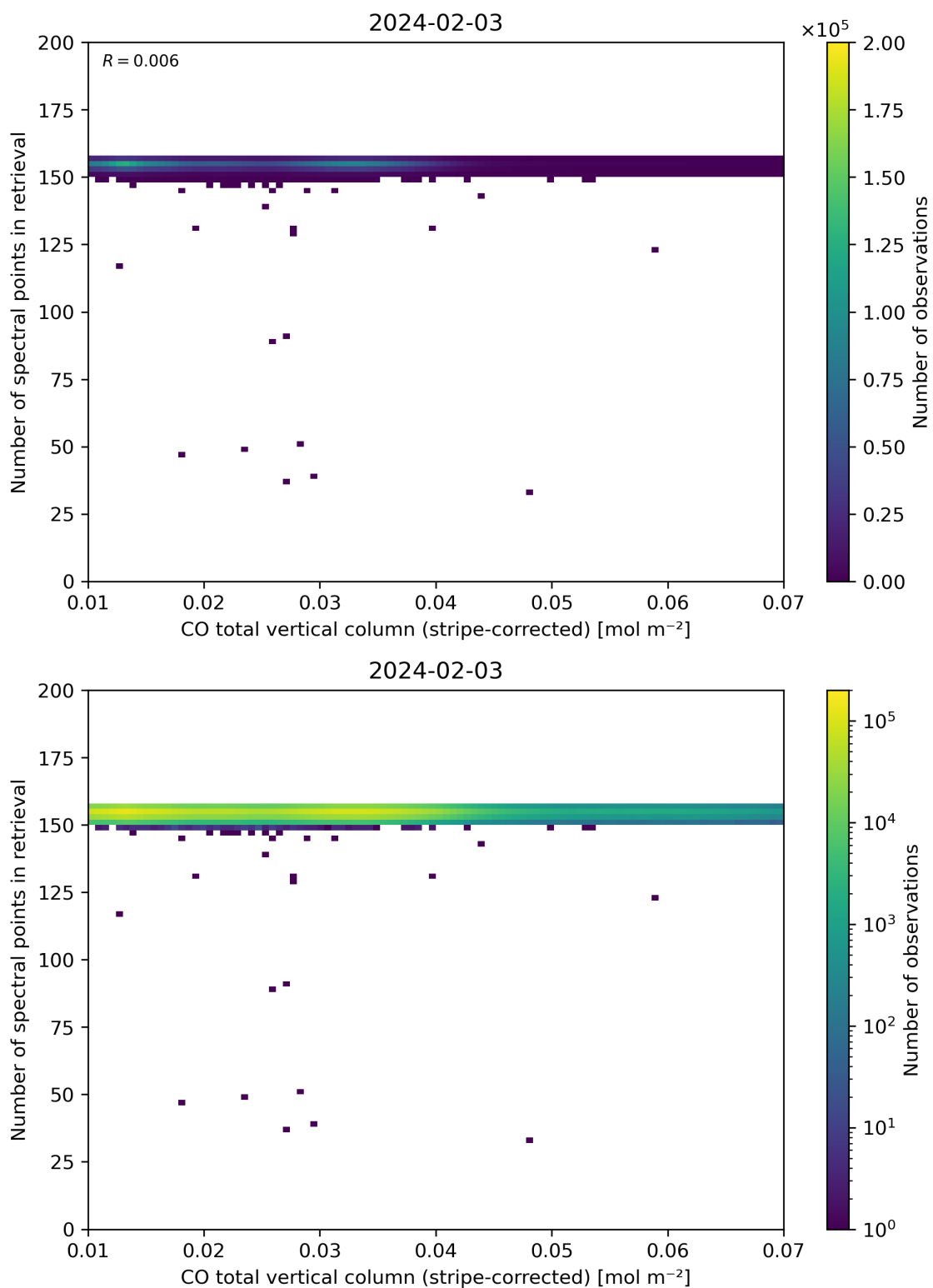
Figure 40: Scatter density plot of “CO total vertical column (stripe-corrected)” against “Number of spectral points in retrieval” for 2024-02-02 to 2024-02-04.
