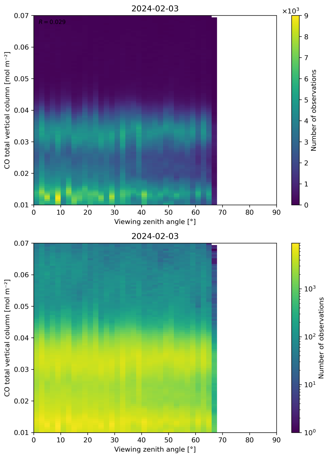
Figure 69: Scatter density plot of “Viewing zenith angle” against “CO total vertical column” for 2024-02-02 to 2024-02-04.
