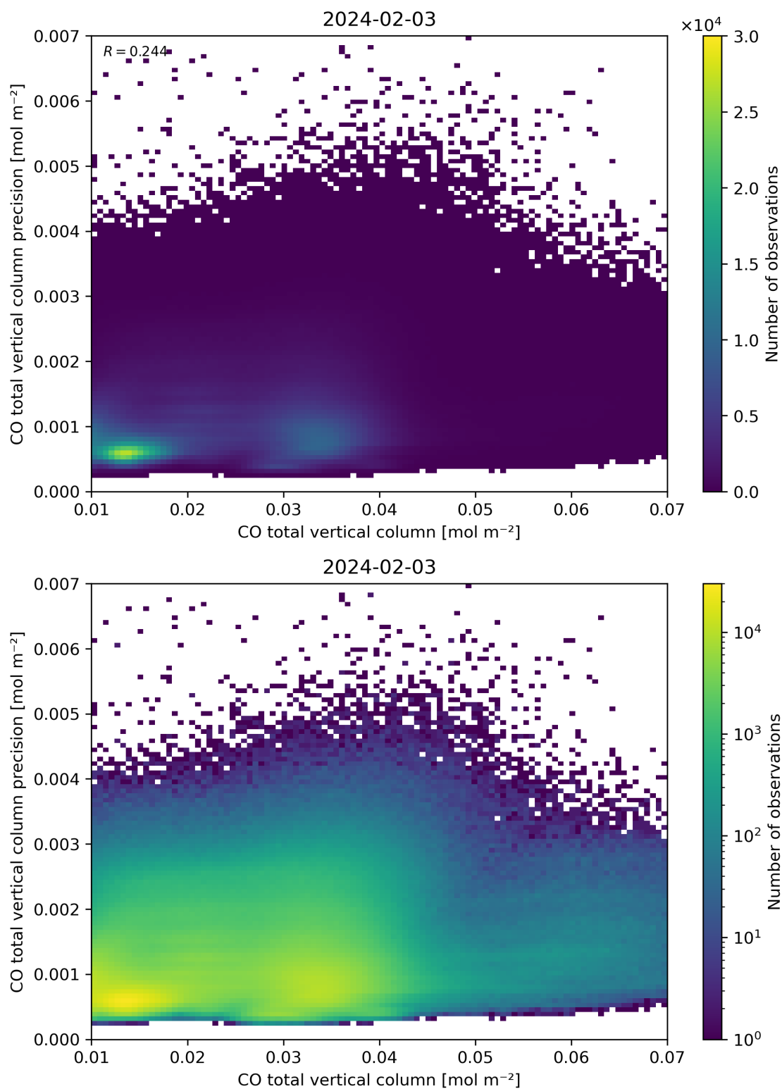
Figure 34: Scatter density plot of “CO total vertical column” against “CO total vertical column precision” for 2024-02-02 to 2024-02-04.
