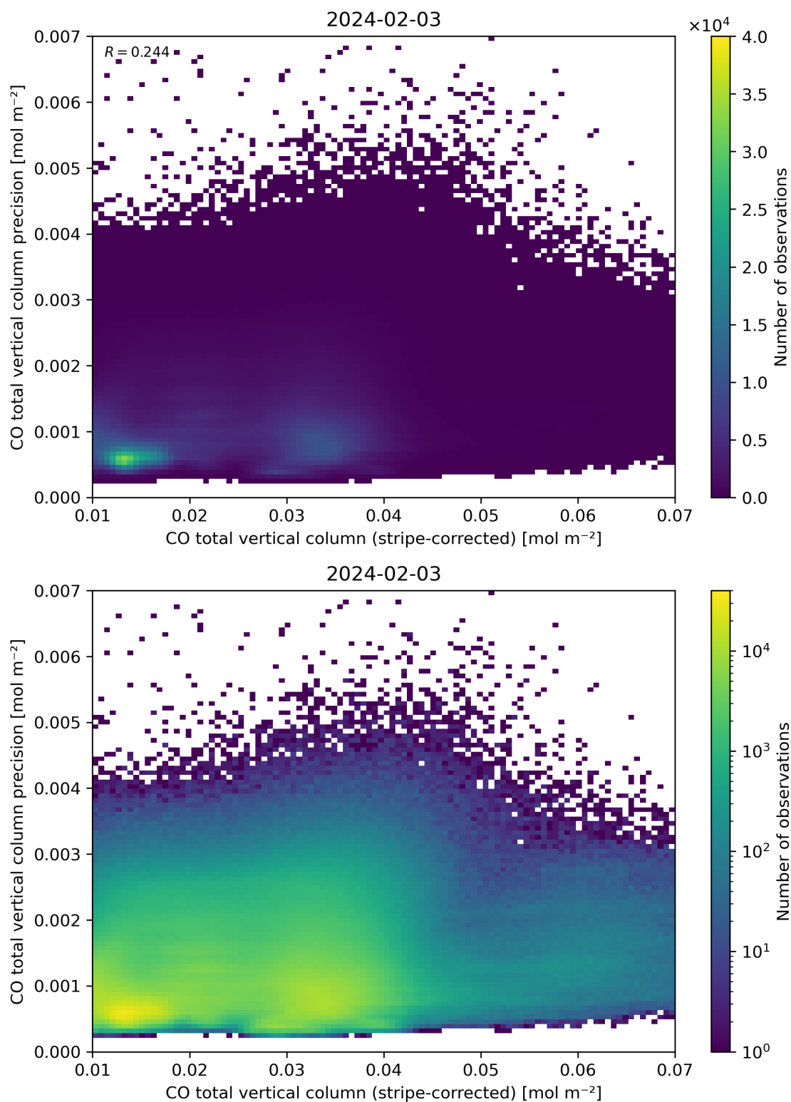
Figure 36: Scatter density plot of “CO total vertical column (stripe-corrected)” against “CO total vertical column precision” for 2024-02-02 to 2024-02-04.
