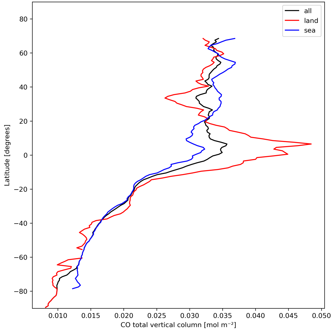
Figure 10: Zonal average of “CO total vertical column” for 2024-02-02 to 2024-02-04.
