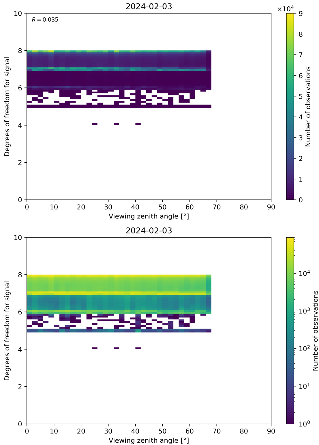
Figure 73: Scatter density plot of “Viewing zenith angle” against “Degrees of freedom for signal” for 2024-02-02 to 2024-02-04.
