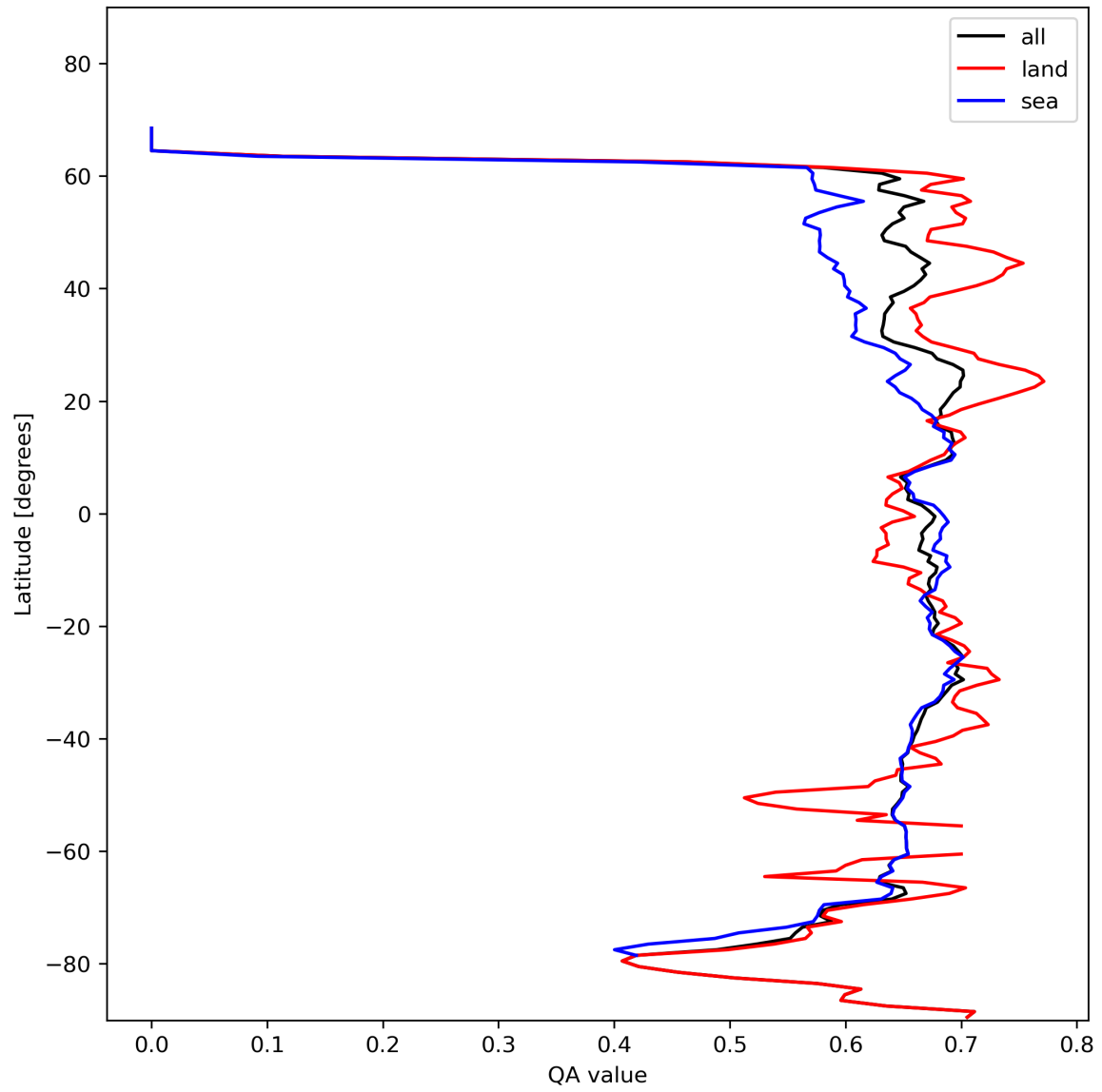
Figure 9: Zonal average of “QA value” for 2024-02-02 to 2024-02-04.
