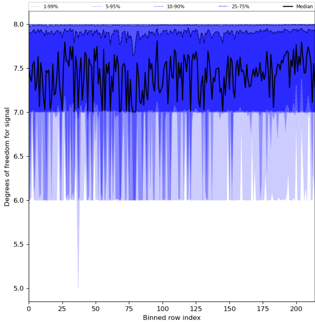
Figure 31: Along track statistics of “Degrees of freedom for signal” for 2024-02-02 to 2024-02-04
