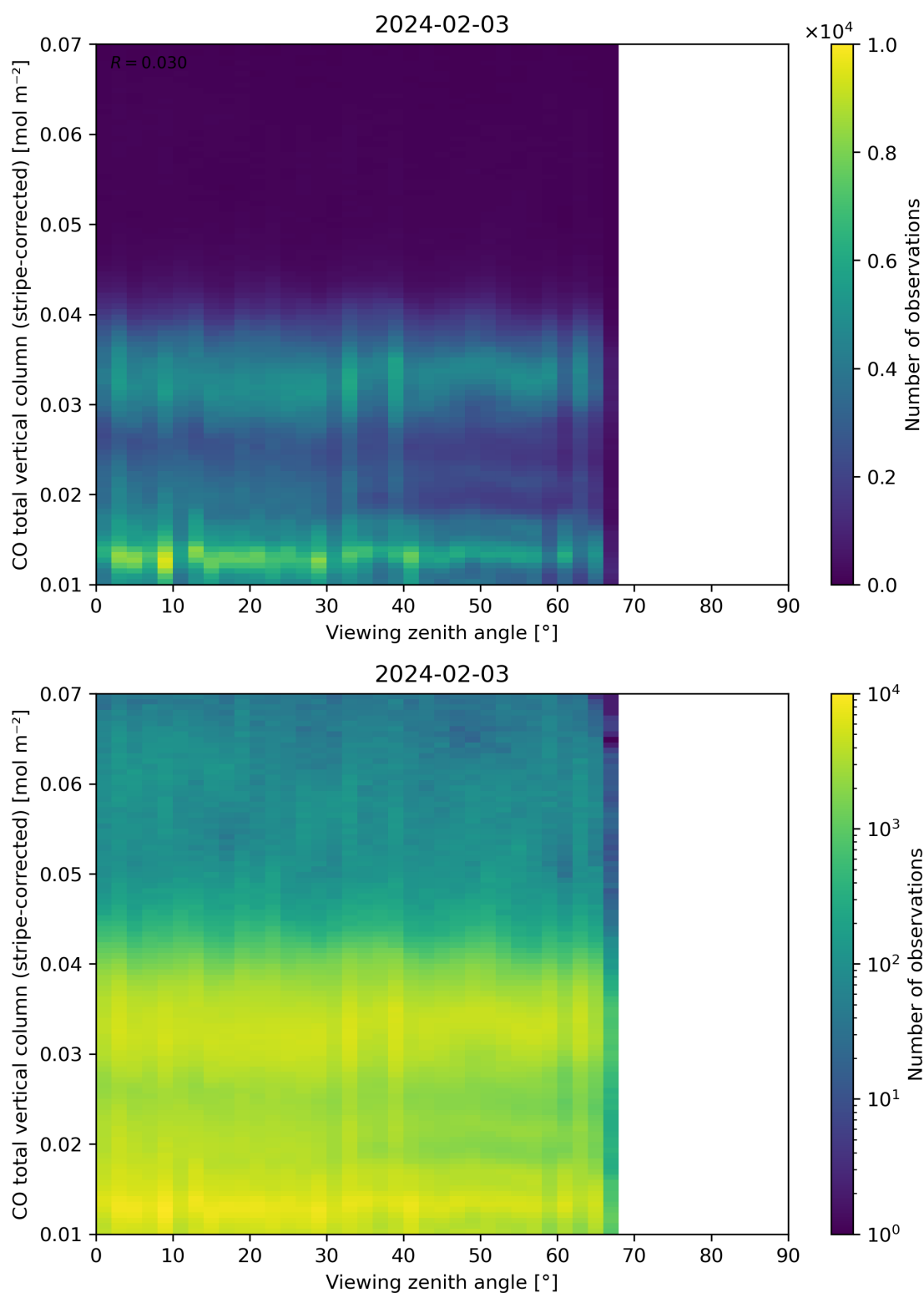
Figure 70: Scatter density plot of “Viewing zenith angle” against “CO total vertical column (stripe-corrected)” for 2024-02-02 to 2024-02-04.
