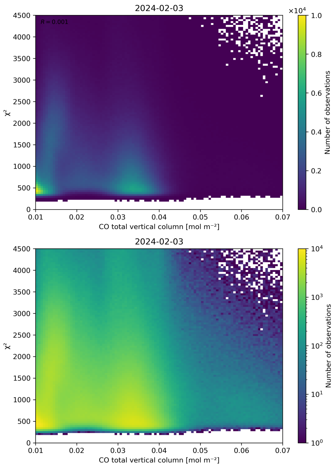
Figure 35: Scatter density plot of “CO total vertical column” against “ \chi^2 ” for 2024-02-02 to 2024-02-04.
