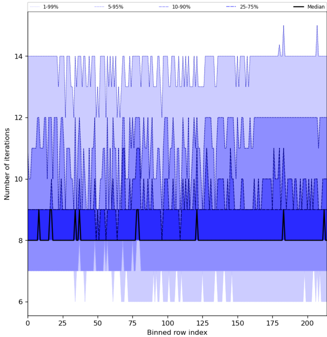
Figure 32: Along track statistics of “Number of iterations” for 2024-02-02 to 2024-02-04
