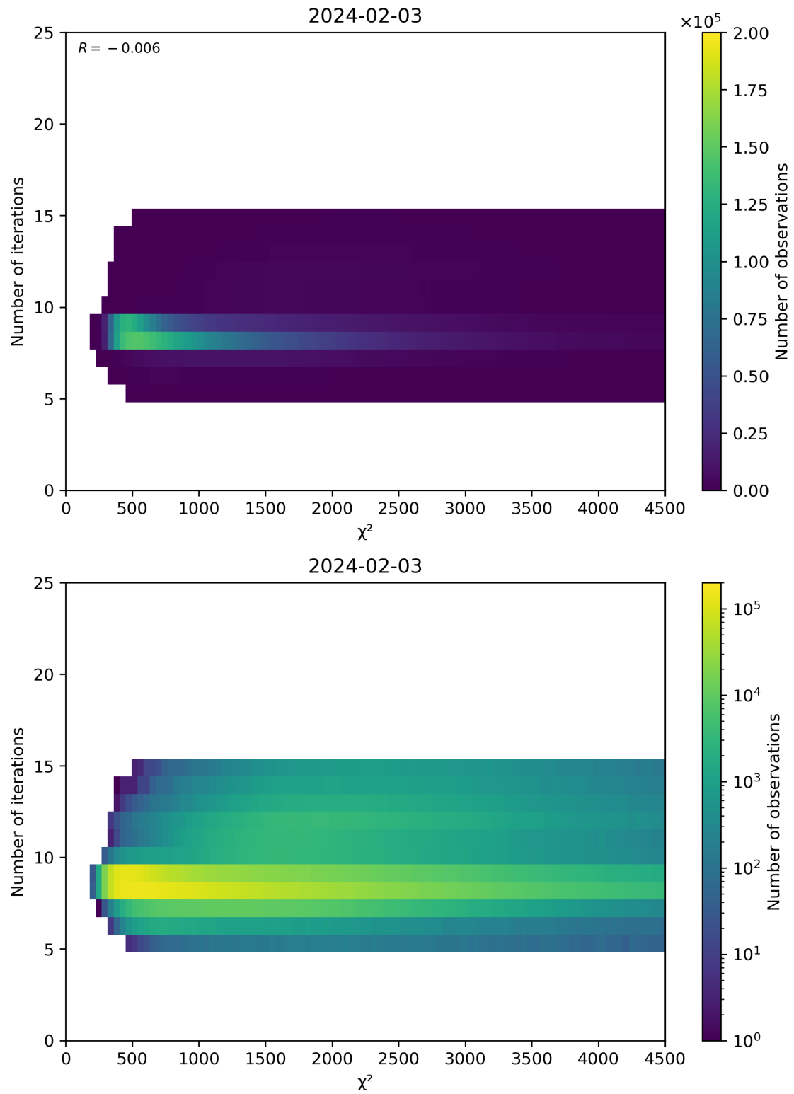
Figure 49: Scatter density plot of “ \chi^2 ” against “Number of iterations” for 2024-02-02 to 2024-02-04.
