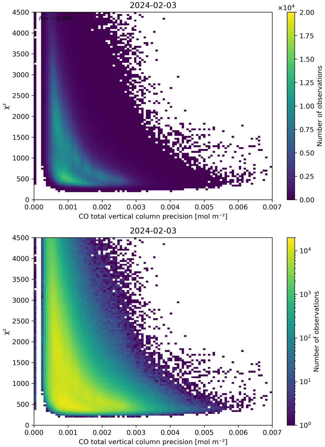
Figure 44: Scatter density plot of “CO total vertical column precision” against “ \chi^2 ” for 2024-02-02 to 2024-02-04.
