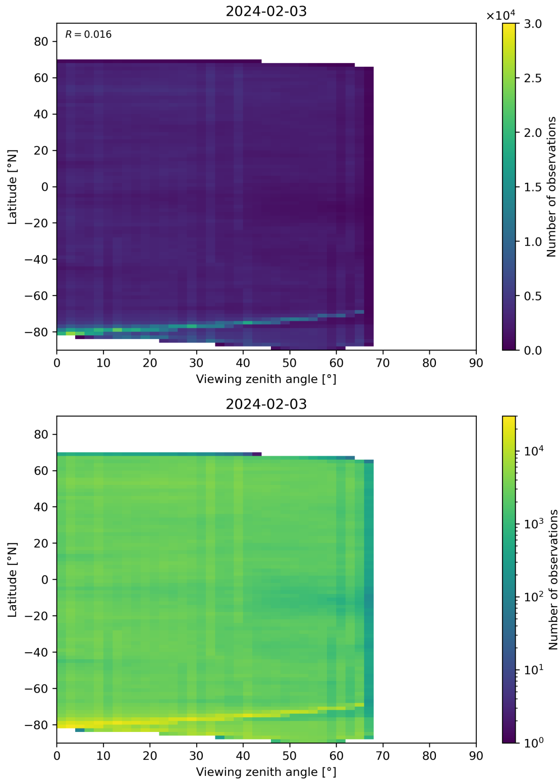
Figure 74: Scatter density plot of “Viewing zenith angle” against “Latitude” for 2024-02-02 to 2024-02-04.
