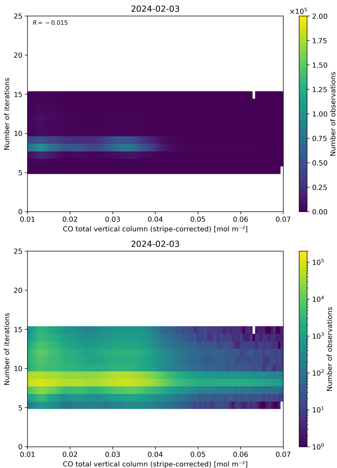
Figure 39: Scatter density plot of “CO total vertical column (stripe-corrected)” against “Number of iterations” for 2024-02-02 to 2024-02-04.
