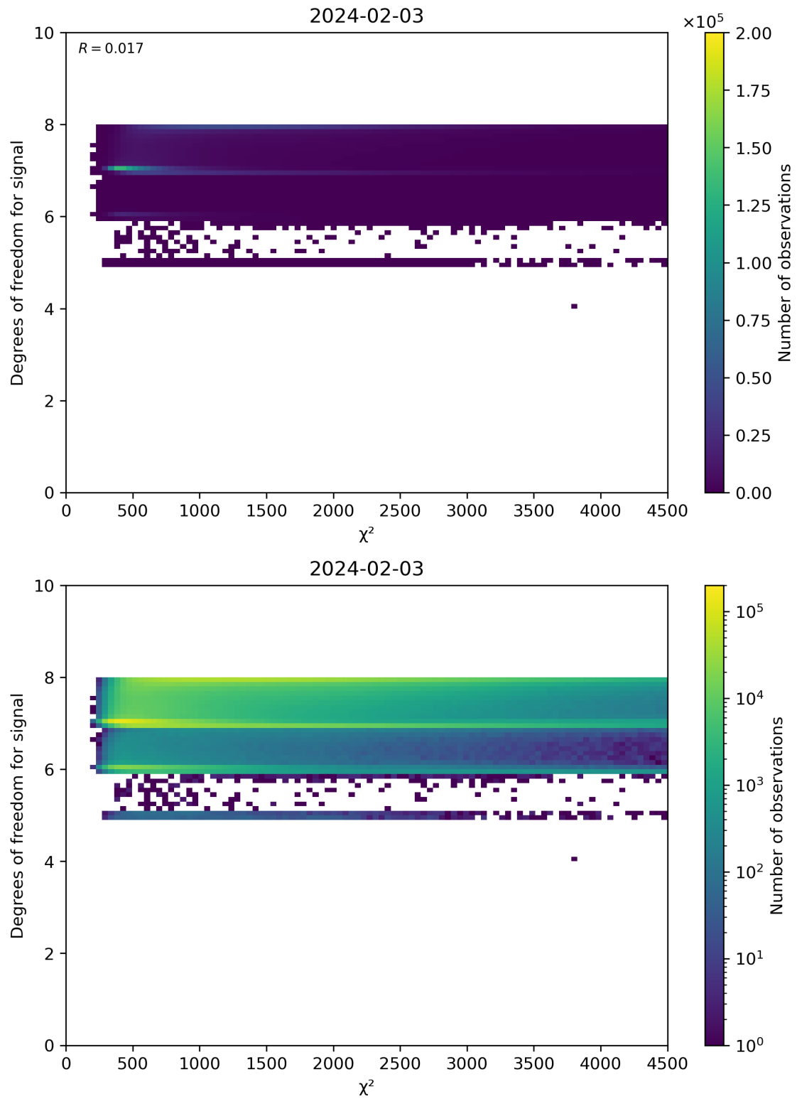
Figure 48: Scatter density plot of “ \chi^2 ” against “Degrees of freedom for signal” for 2024-02-02 to 2024-02-04.
