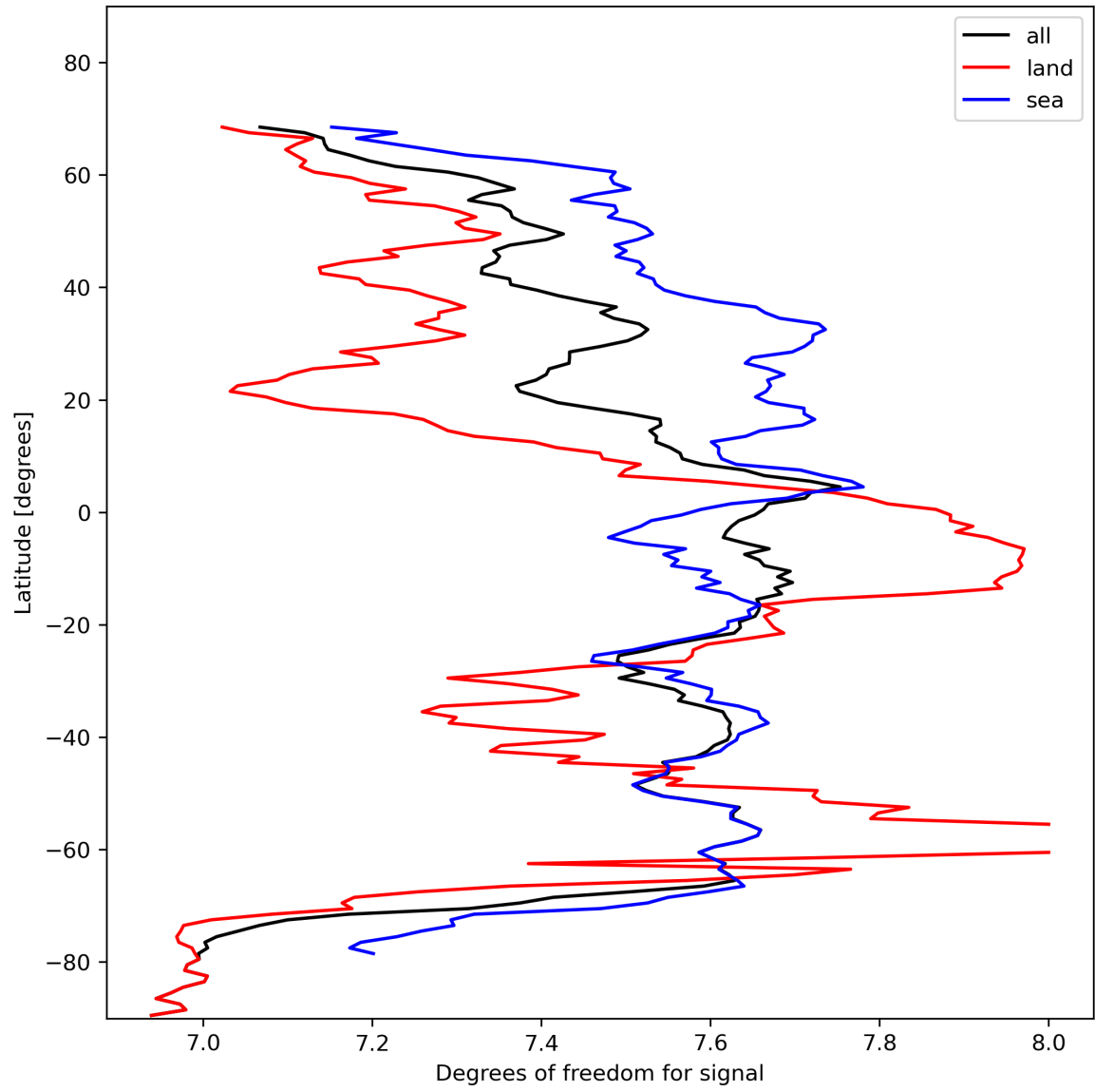
Figure 15: Zonal average of “Degrees of freedom for signal” for 2024-02-02 to 2024-02-04.
