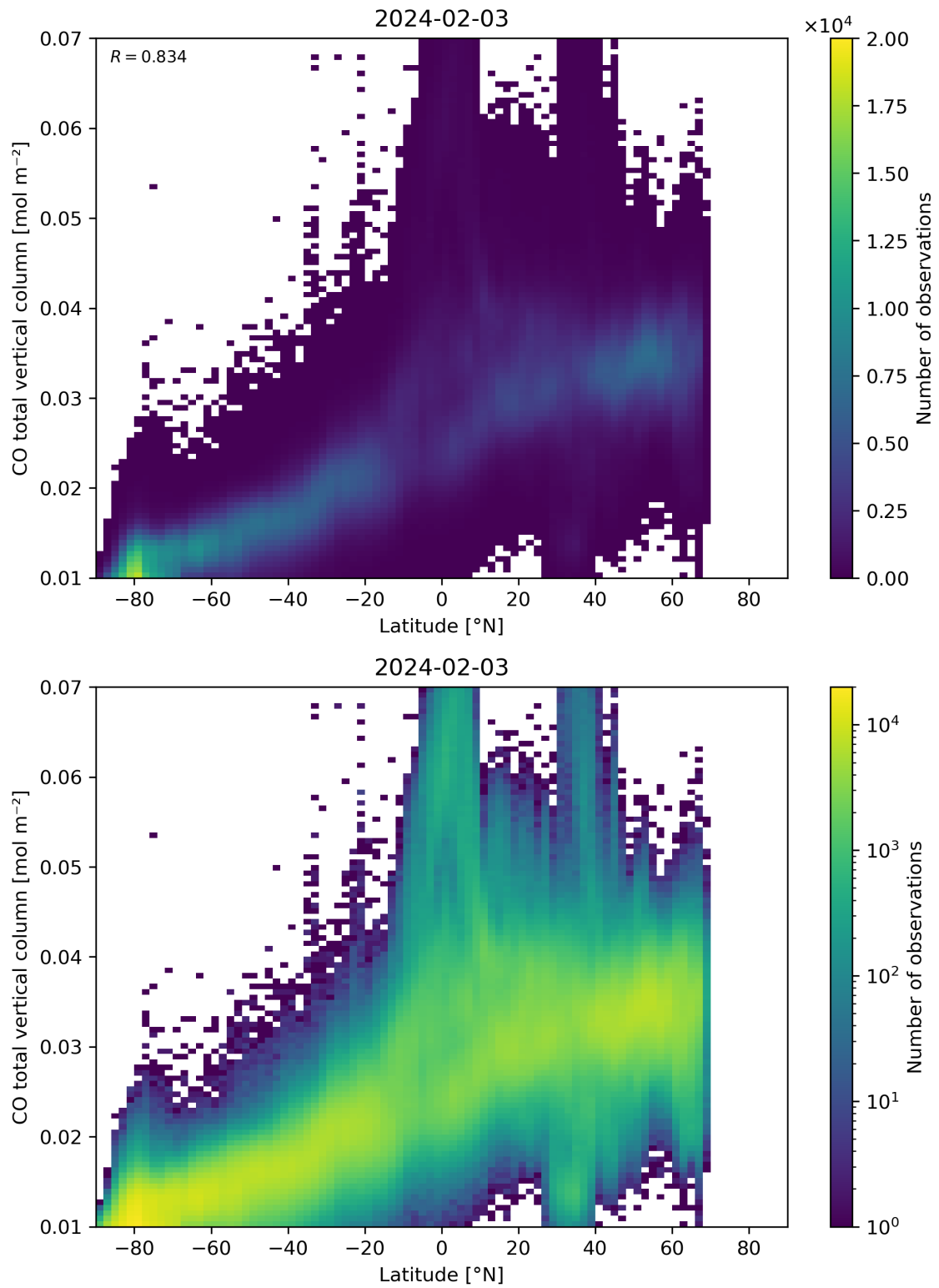
Figure 51: Scatter density plot of “Latitude” against “CO total vertical column” for 2024-02-02 to 2024-02-04.
