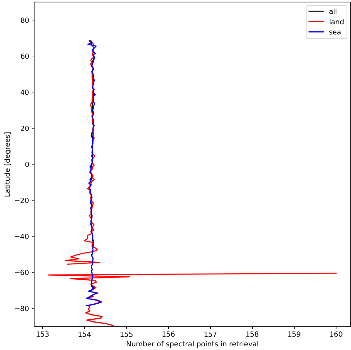
Figure 13: Zonal average of “Number of spectral points in retrieval” for 2024-02-02 to 2024-02-04.
