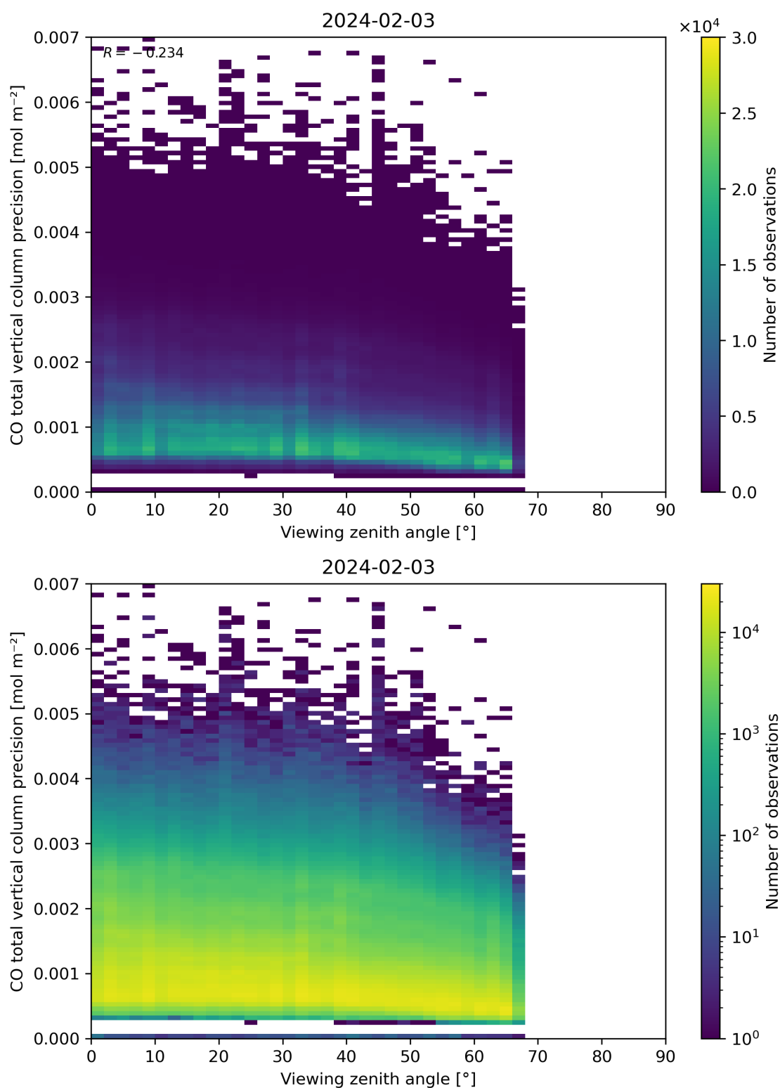
Figure 71: Scatter density plot of “Viewing zenith angle” against “CO total vertical column precision” for 2024-02-02 to 2024-02-04.
