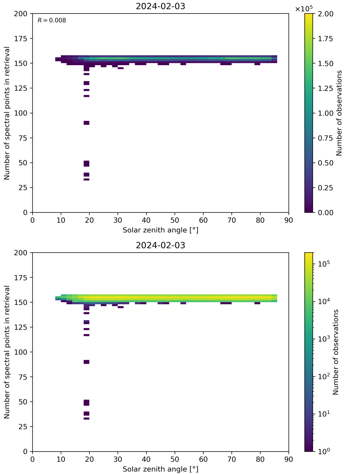
Figure 68: Scatter density plot of “Solar zenith angle” against “Number of spectral points in retrieval” for 2024-02-02 to 2024-02-04.
