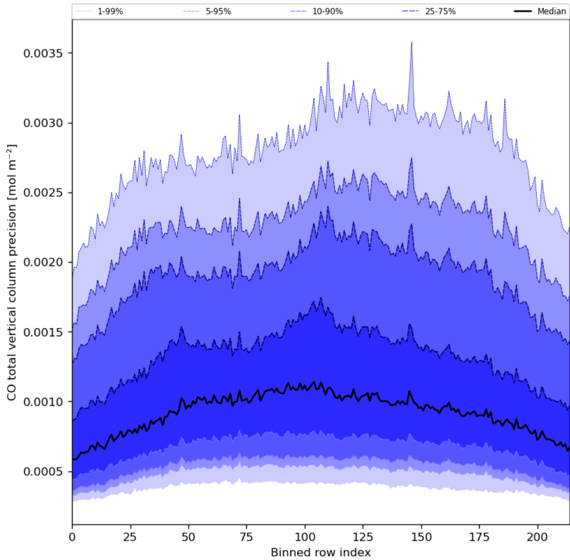
Figure 28: Along track statistics of “CO total vertical column precision” for 2024-02-02 to 2024-02-04
