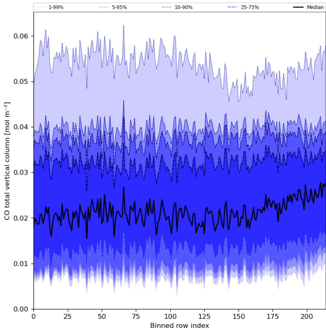
Figure 26: Along track statistics of “CO total vertical column” for 2024-02-02 to 2024-02-04
