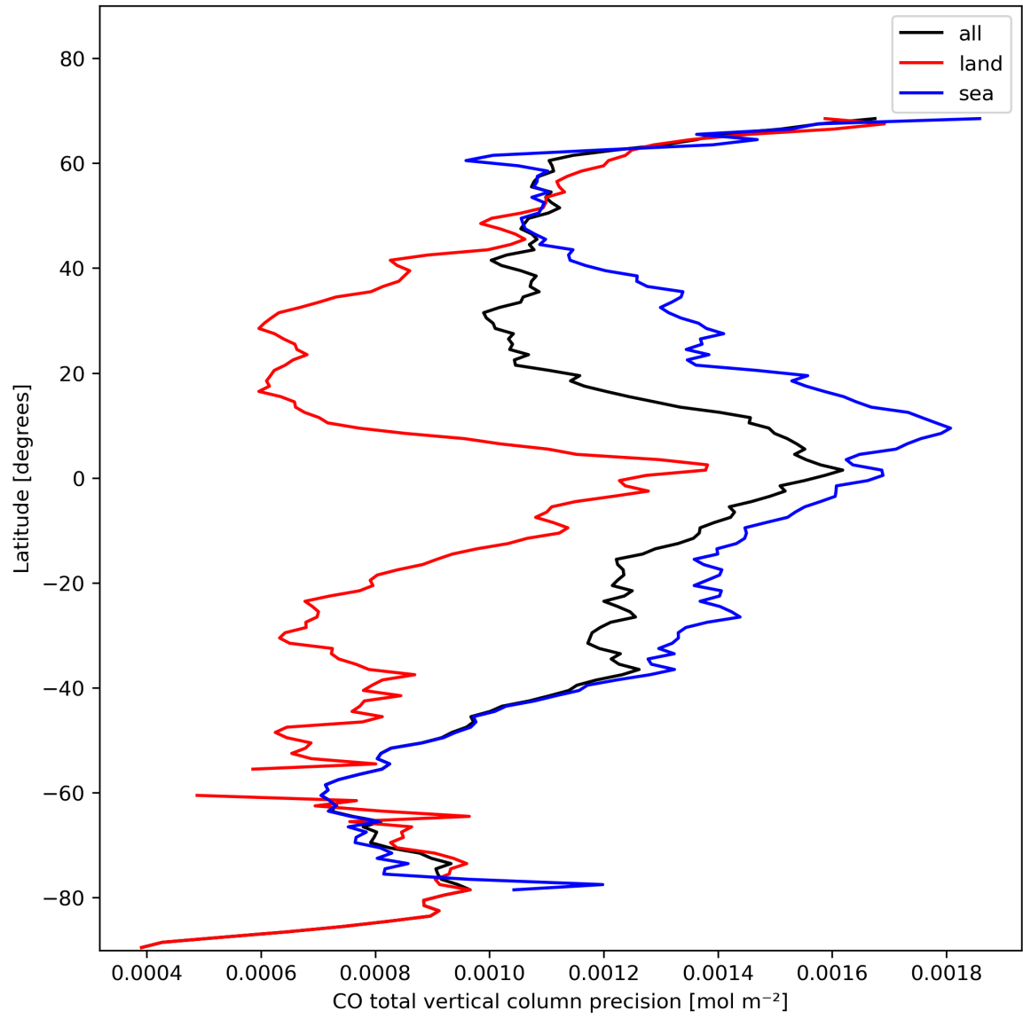
Figure 12: Zonal average of “CO total vertical column precision” for 2024-02-02 to 2024-02-04.
