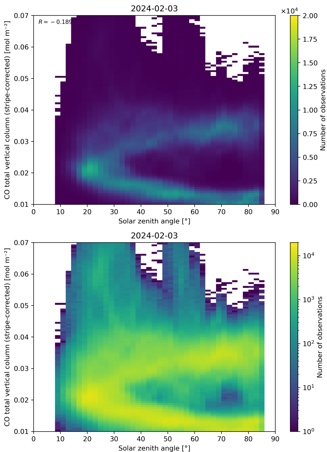
Figure 62: Scatter density plot of “Solar zenith angle” against “CO total vertical column (stripe-corrected)” for 2024-02-02 to 2024-02-04.
