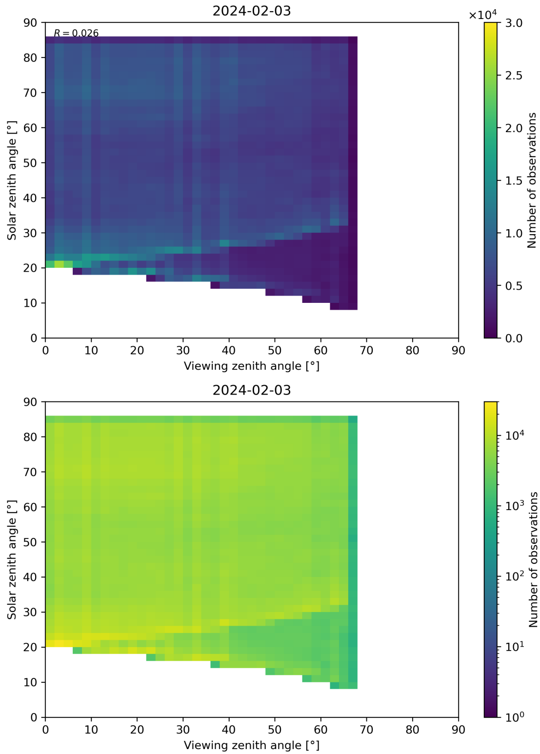
Figure 77: Scatter density plot of “Viewing zenith angle” against “Solar zenith angle” for 2024-02-02 to 2024-02-04.
