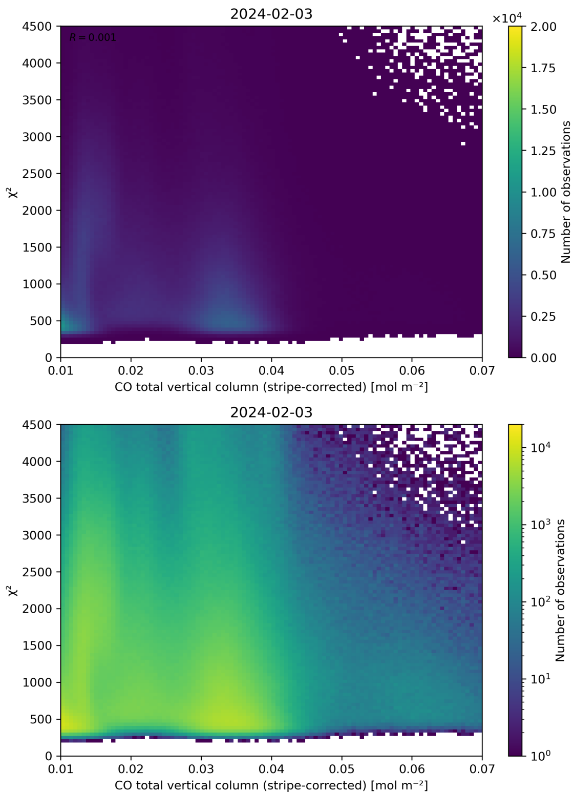
Figure 37: Scatter density plot of “CO total vertical column (stripe-corrected)” against “ \chi^2 ” for 2024-02-02 to 2024-02-04.
