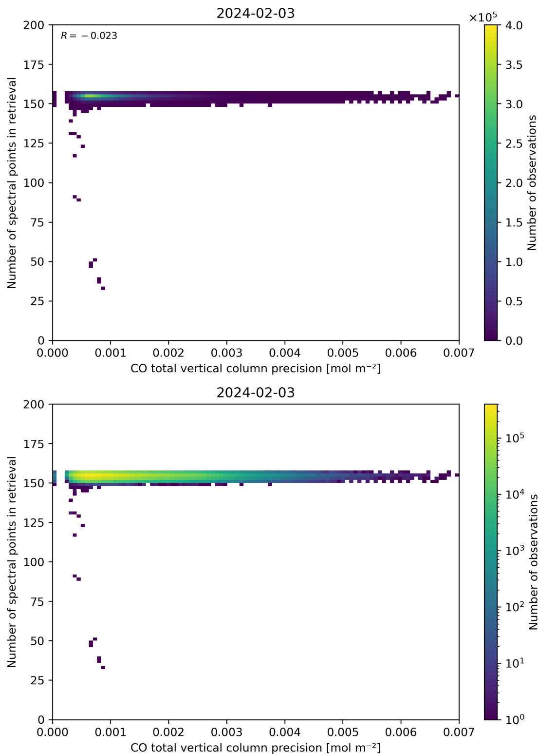
Figure 47: Scatter density plot of “CO total vertical column precision” against “Number of spectral points in retrieval” for 2024-02-02 to 2024-02-04.
