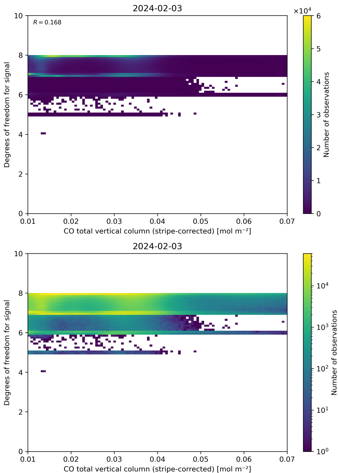
Figure 38: Scatter density plot of “CO total vertical column (stripe-corrected)” against “Degrees of freedom for signal” for 2024-02-02 to 2024-02-04.
