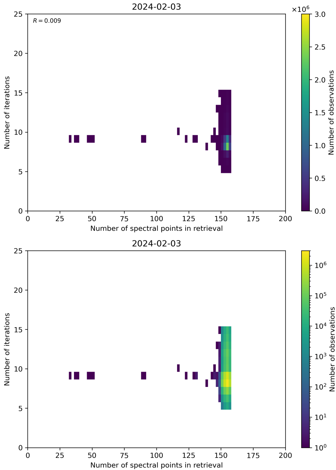
Figure 60: Scatter density plot of “Number of spectral points in retrieval” against “Number of iterations” for 2024-02-02 to 2024-02-04.
