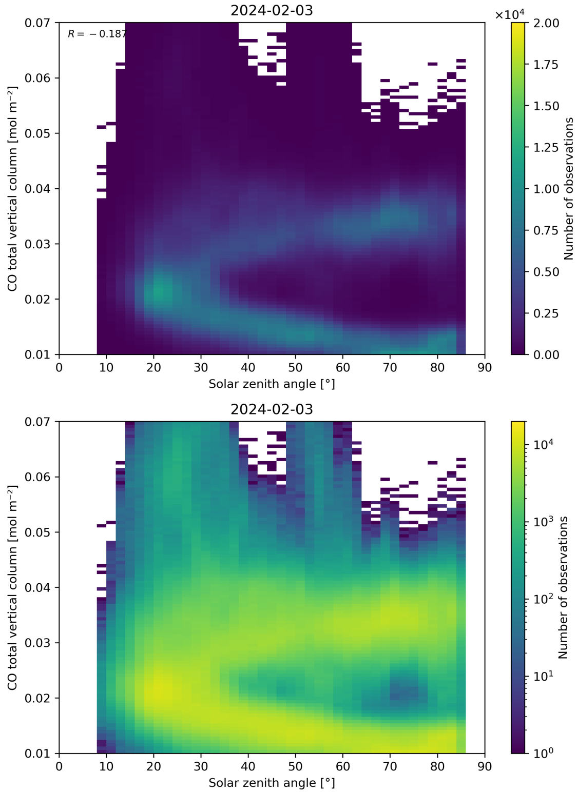
Figure 61: Scatter density plot of “Solar zenith angle” against “CO total vertical column” for 2024-02-02 to 2024-02-04.
