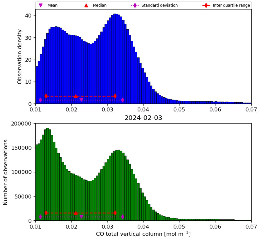
Figure 18: Histogram of “CO total vertical column” for 2024-02-02 to 2024-02-04
