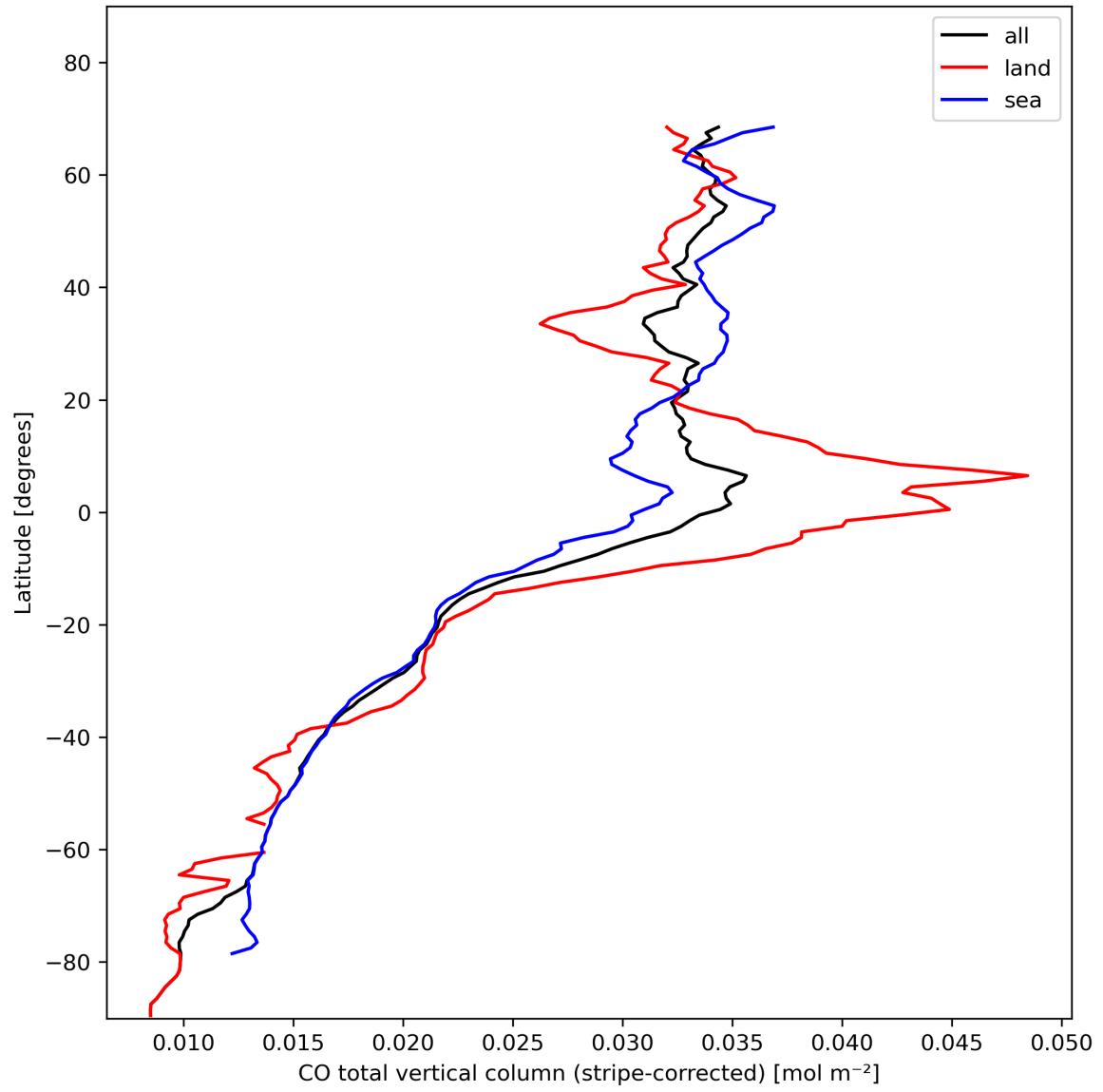
Figure 11: Zonal average of “CO total vertical column (stripe-corrected)” for 2024-02-02 to 2024-02-04.
