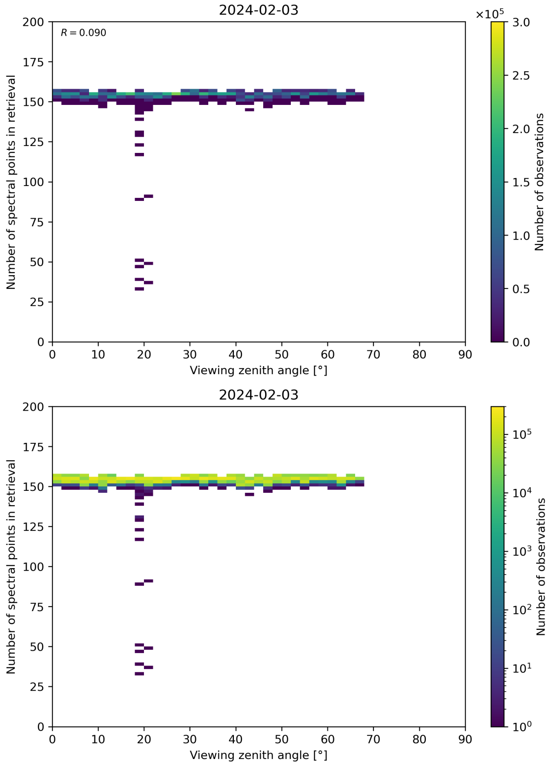
Figure 76: Scatter density plot of “Viewing zenith angle” against “Number of spectral points in retrieval” for 2024-02-02 to 2024-02-04.
