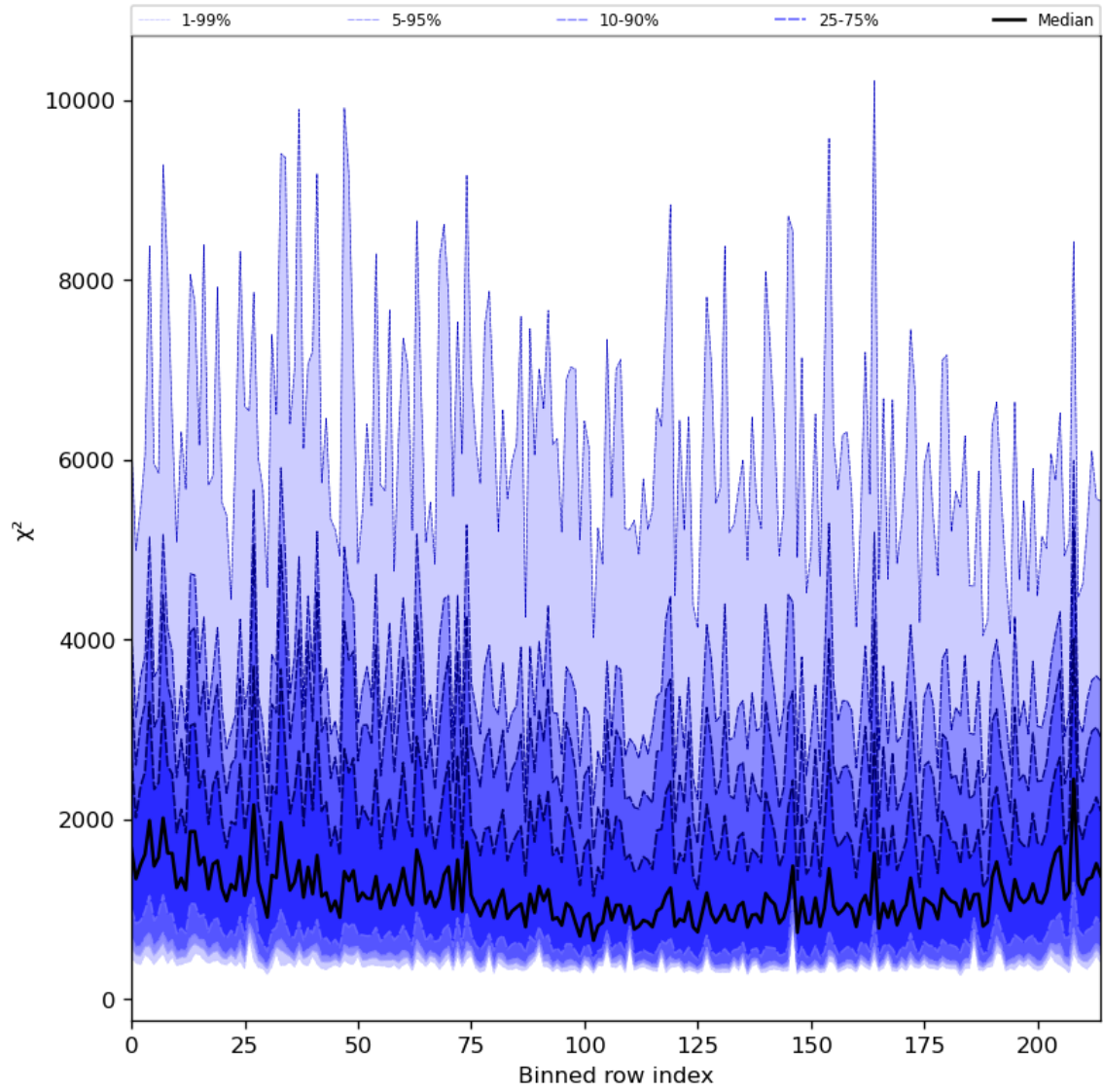
Figure 30: Along track statistics of “ \chi^2 ” for 2024-02-02 to 2024-02-04
