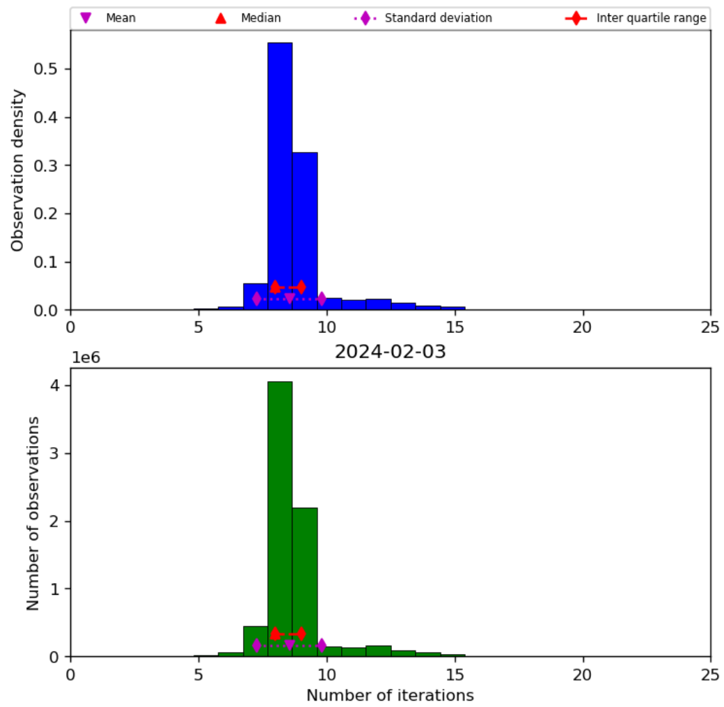
Figure 24: Histogram of “Number of iterations” for 2024-02-02 to 2024-02-04
