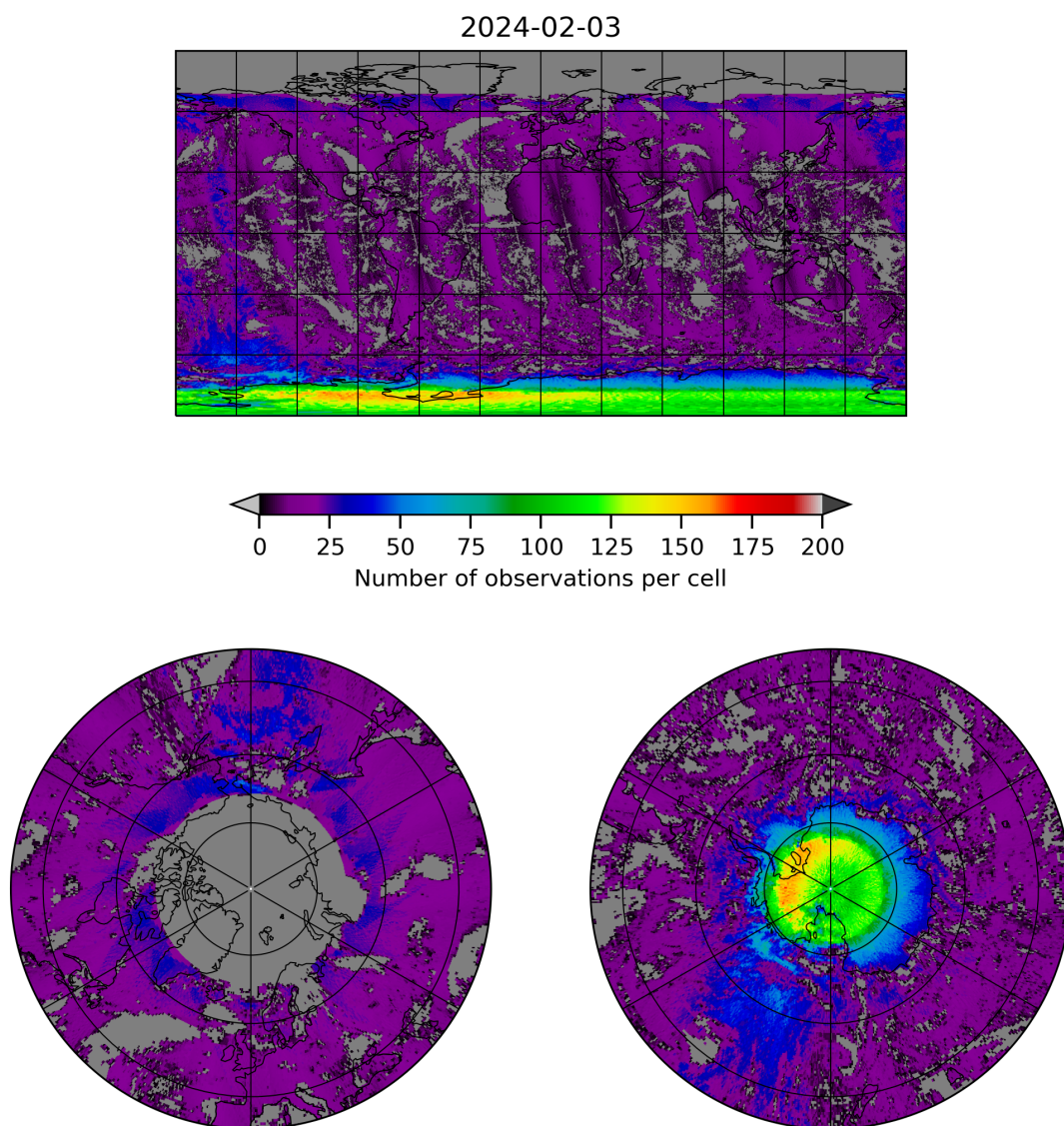
Figure 8: Map of the number of observations for 2024-02-02 to 2024-02-04
