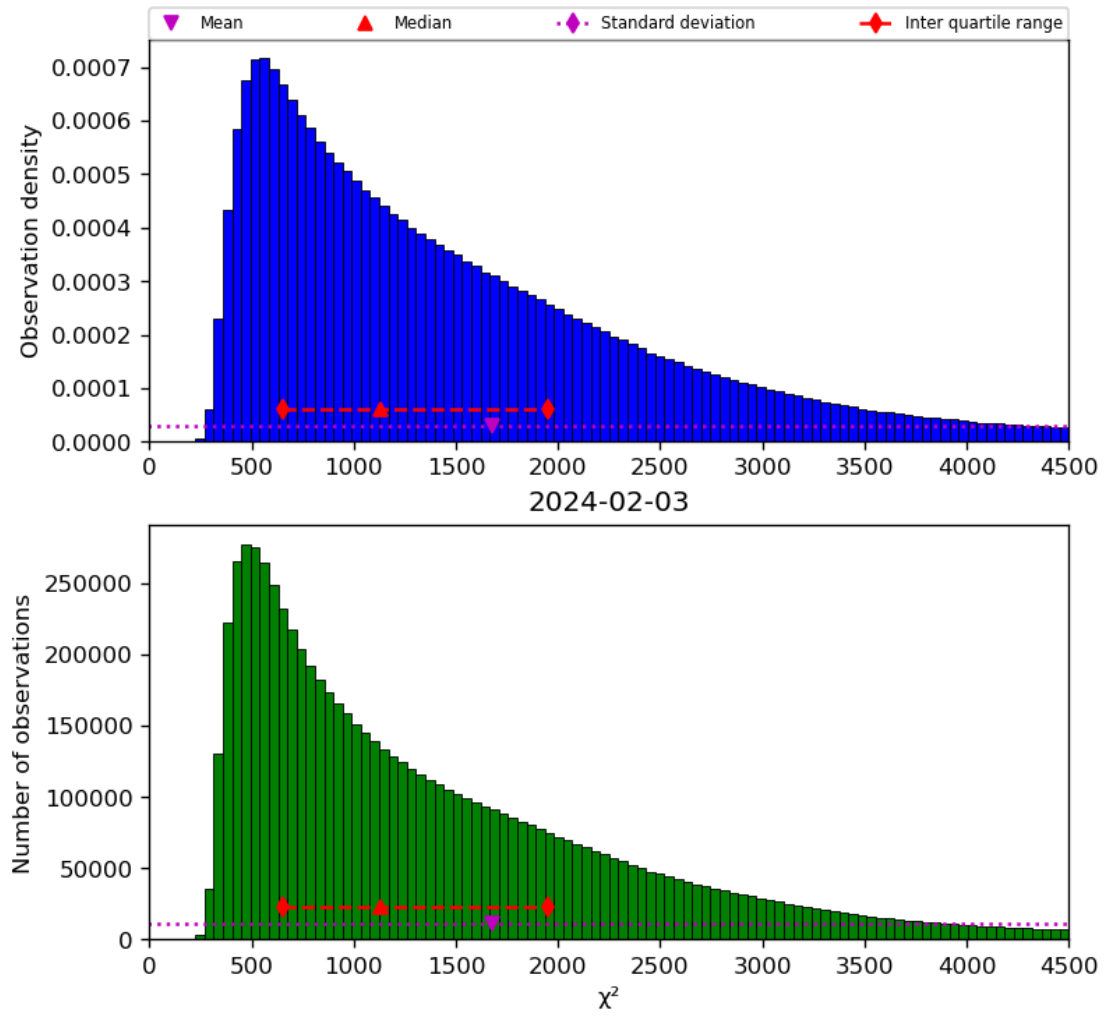
Figure 22: Histogram of “ \chi^2 ” for 2024-02-02 to 2024-02-04
