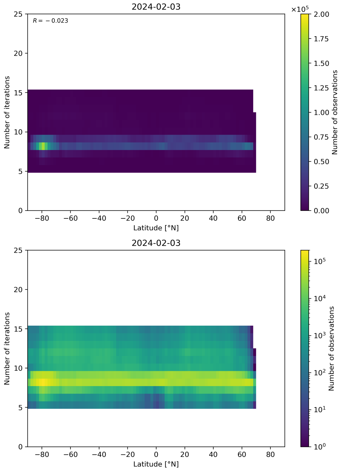
Figure 56: Scatter density plot of “Latitude” against “Number of iterations” for 2024-02-02 to 2024-02-04.
