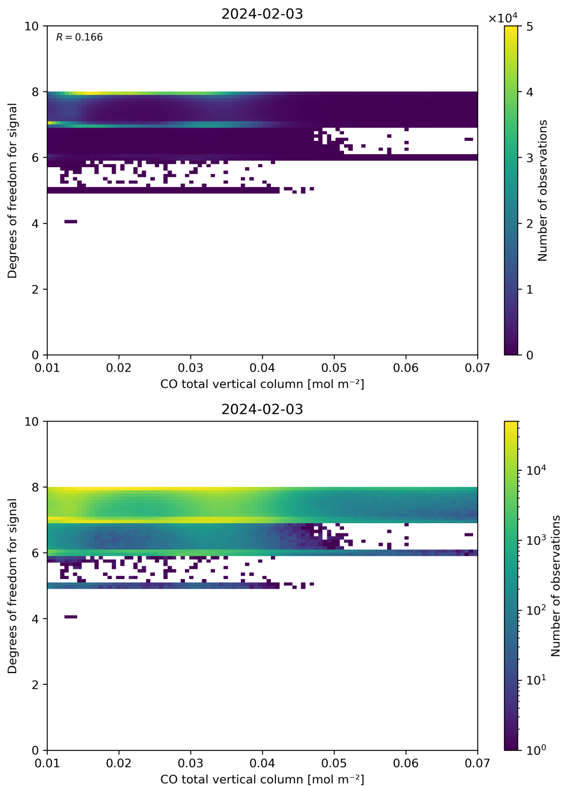
Figure 41: Scatter density plot of “CO total vertical column” against “Degrees of freedom for signal” for 2024-02-02 to 2024-02-04.
