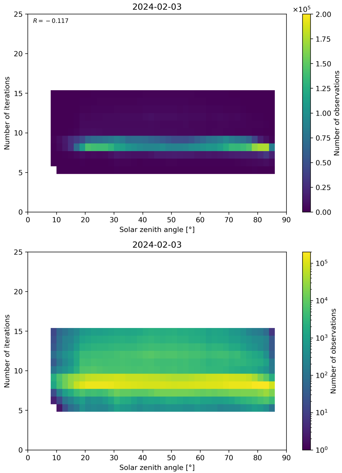
Figure 67: Scatter density plot of “Solar zenith angle” against “Number of iterations” for 2024-02-02 to 2024-02-04.
