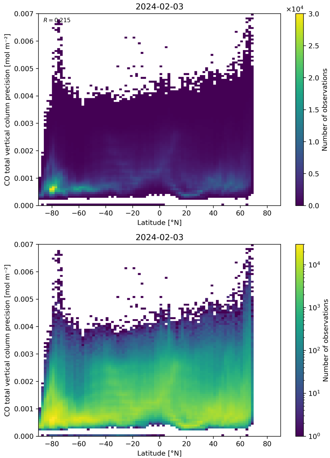
Figure 53: Scatter density plot of “Latitude” against “CO total vertical column precision” for 2024-02-02 to 2024-02-04.
