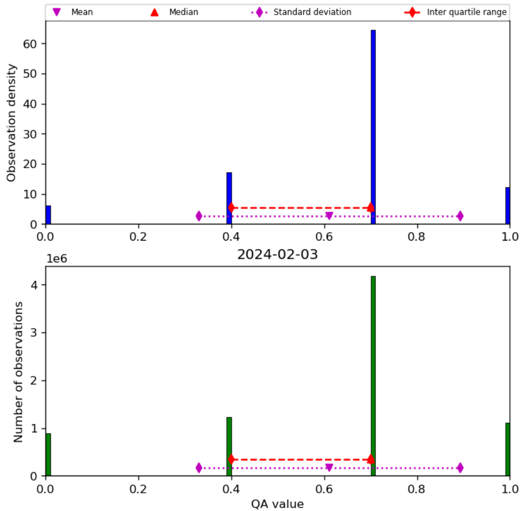
Figure 17: Histogram of “QA value” for 2024-02-02 to 2024-02-04
