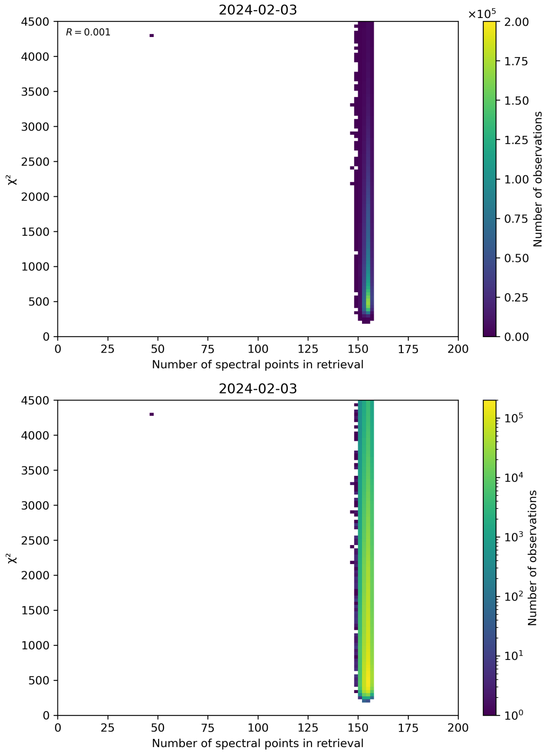
Figure 58: Scatter density plot of “Number of spectral points in retrieval” against “ \chi^2 ” for 2024-02-02 to 2024-02-04.
