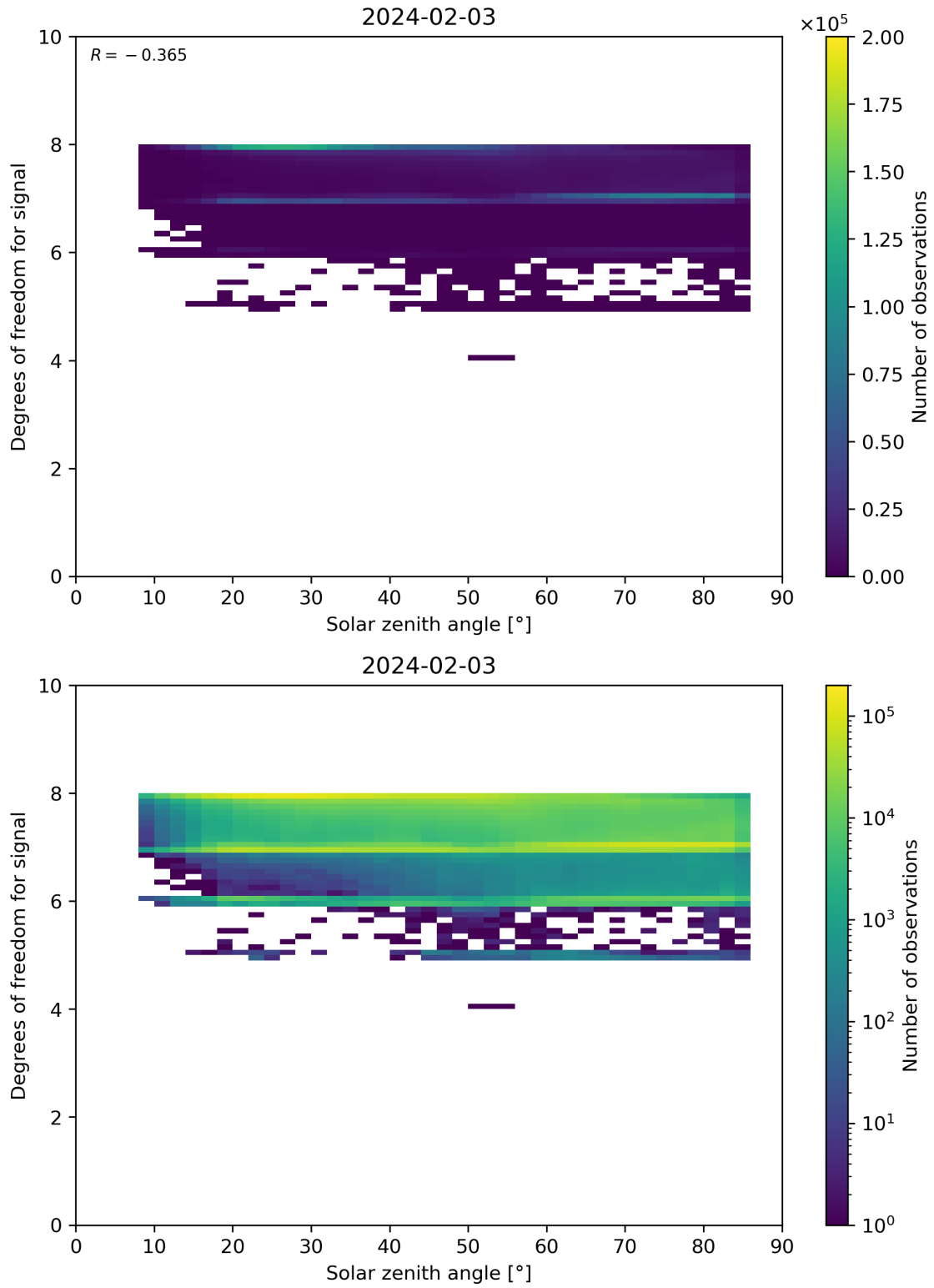
Figure 65: Scatter density plot of “Solar zenith angle” against “Degrees of freedom for signal” for 2024-02-02 to 2024-02-04.
