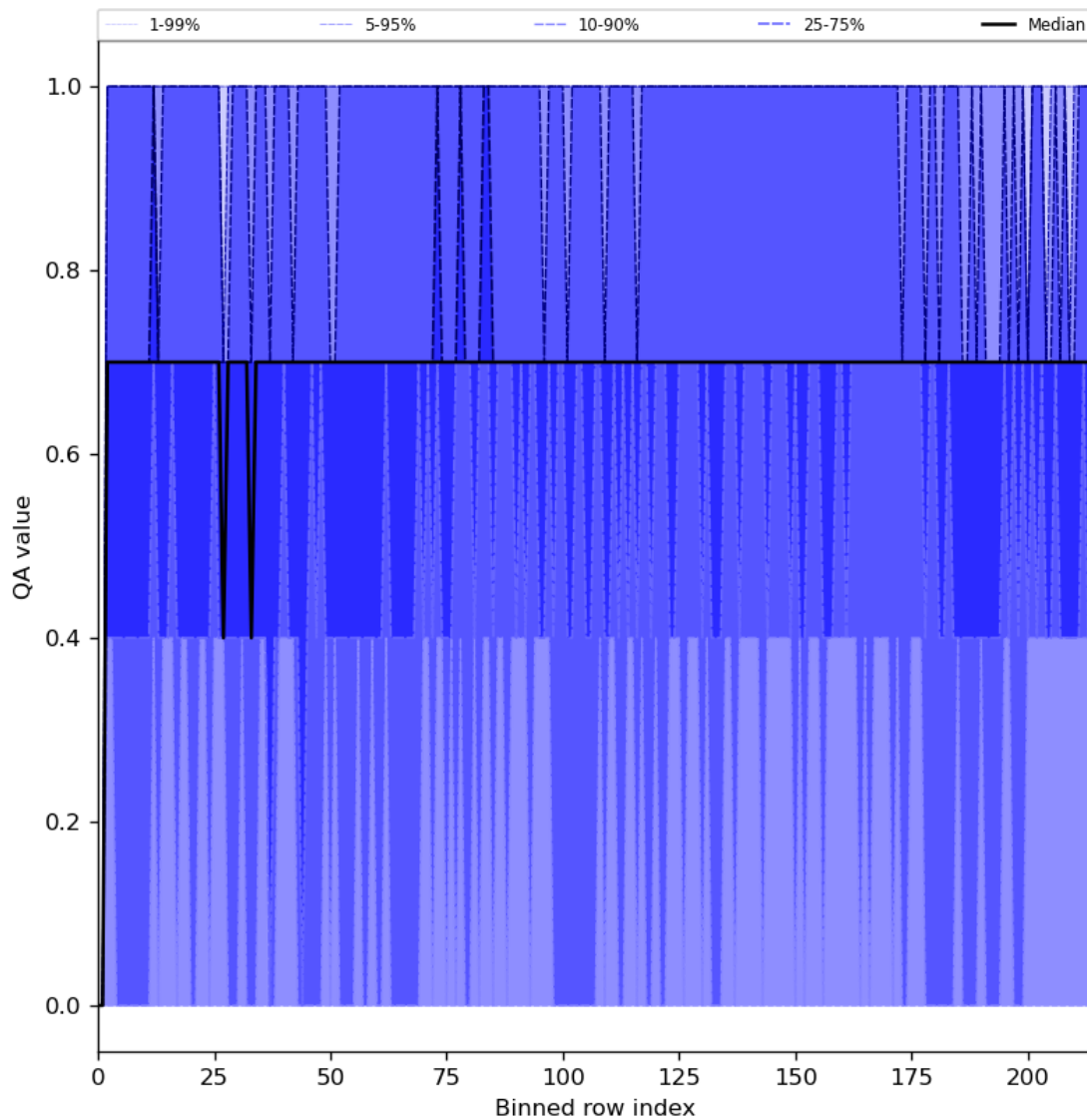
Figure 25: Along track statistics of “QA value” for 2024-02-02 to 2024-02-04
