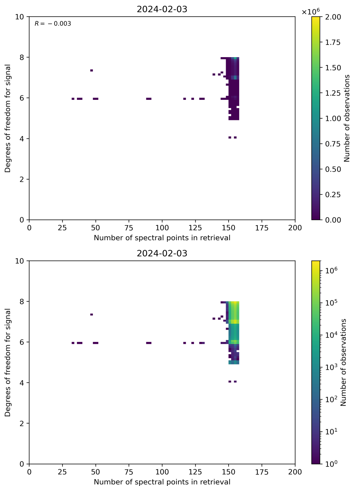
Figure 59: Scatter density plot of “Number of spectral points in retrieval” against “Degrees of freedom for signal” for 2024-02-02 to 2024-02-04.
