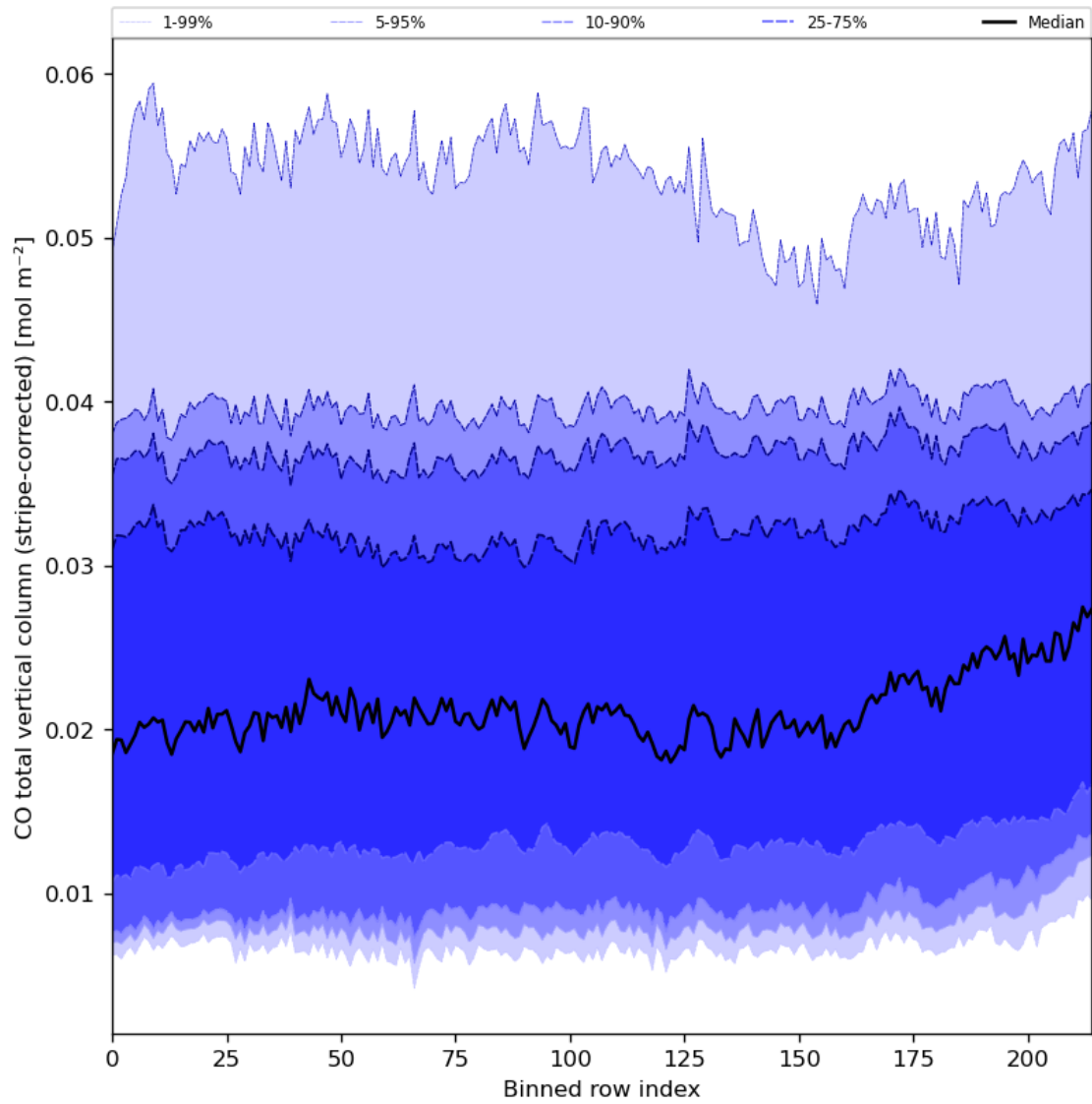
Figure 27: Along track statistics of “CO total vertical column (stripe-corrected)” for 2024-02-02 to 2024-02-04
