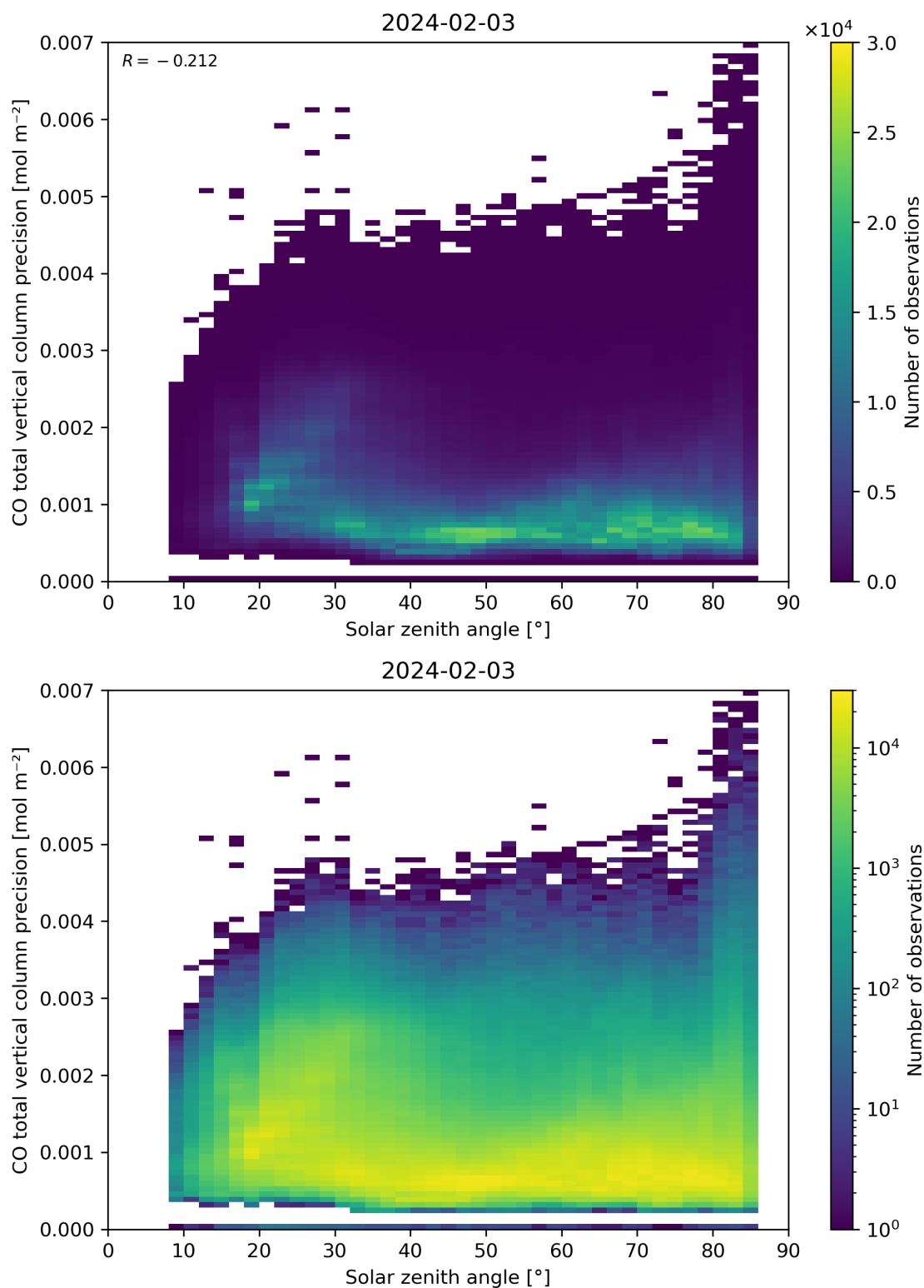
Figure 63: Scatter density plot of “Solar zenith angle” against “CO total vertical column precision” for 2024-02-02 to 2024-02-04.
