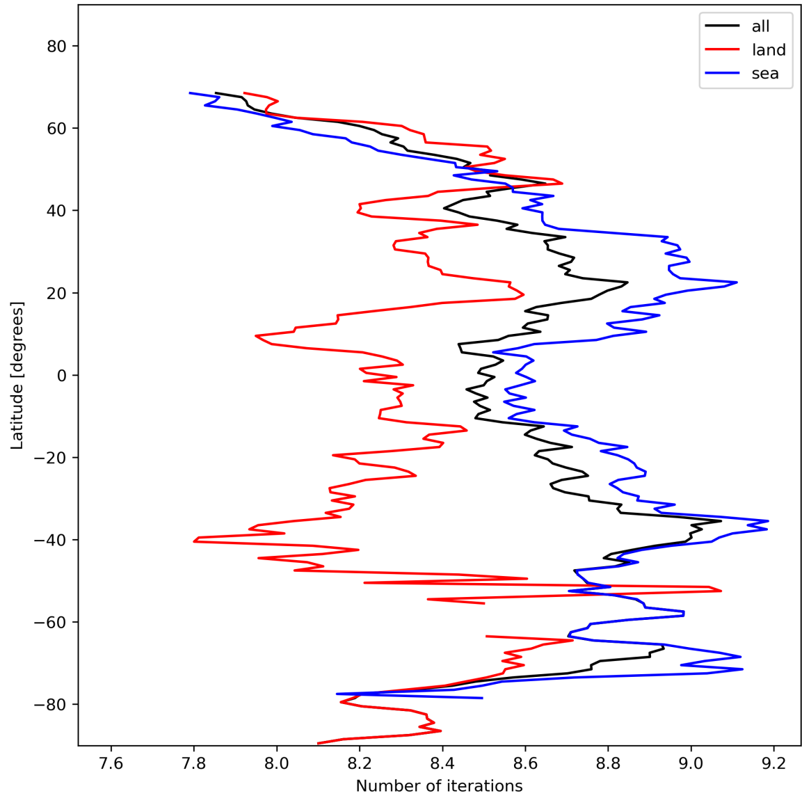
Figure 16: Zonal average of “Number of iterations” for 2024-02-03 to 2024-02-05.
