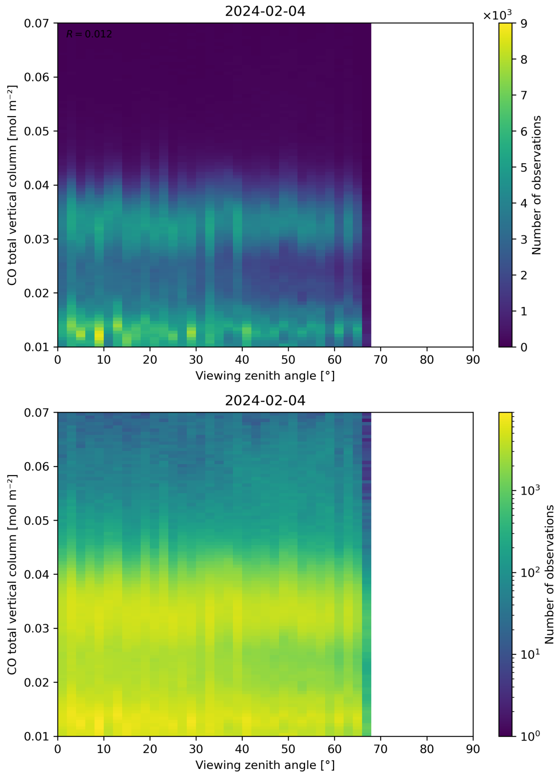
Figure 69: Scatter density plot of “Viewing zenith angle” against “CO total vertical column” for 2024-02-03 to 2024-02-05.
