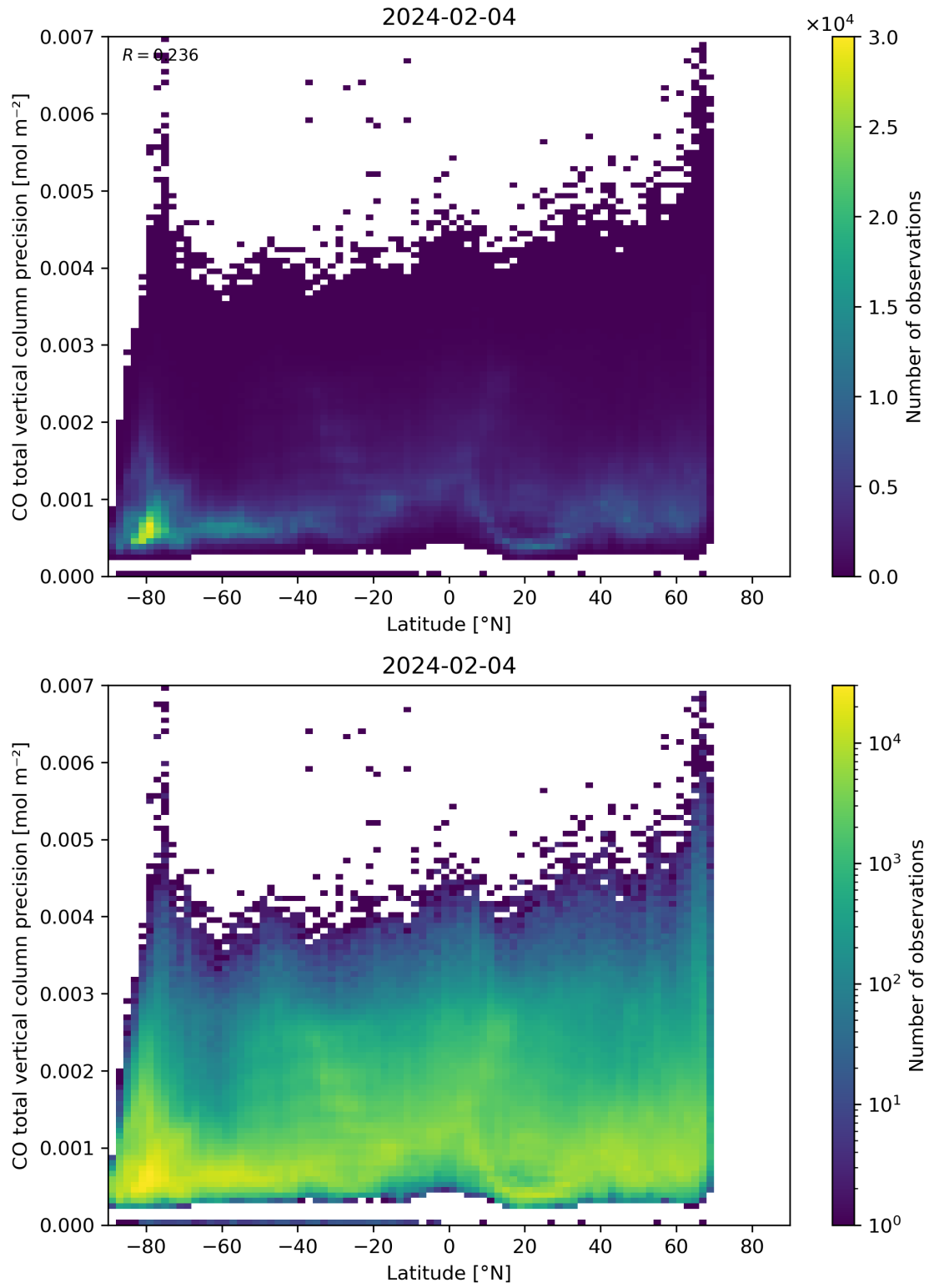
Figure 53: Scatter density plot of “Latitude” against “CO total vertical column precision” for 2024-02-03 to 2024-02-05.
