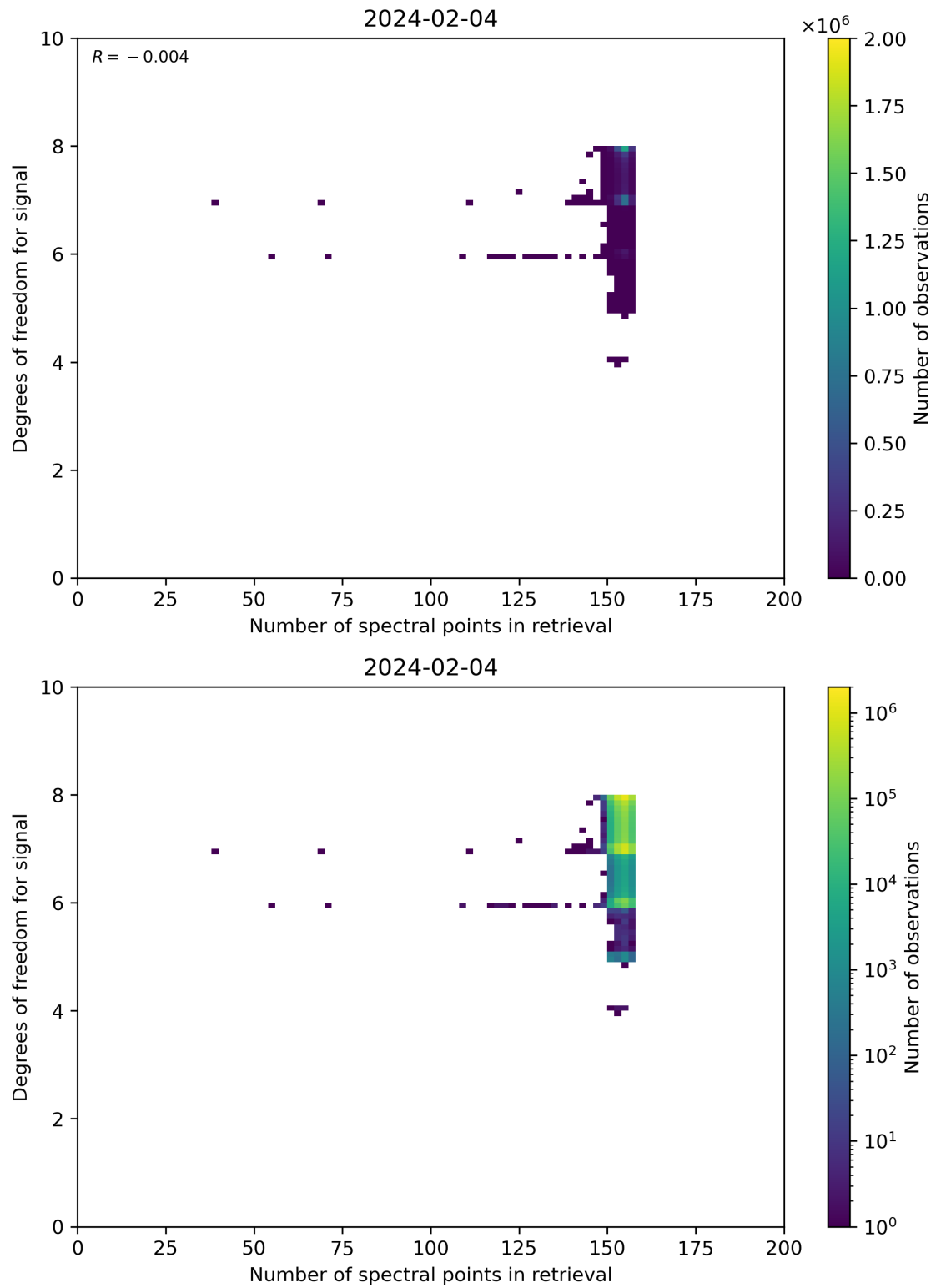
Figure 59: Scatter density plot of “Number of spectral points in retrieval” against “Degrees of freedom for signal” for 2024-02-03 to 2024-02-05.
