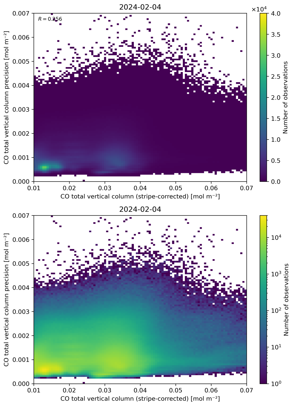
Figure 36: Scatter density plot of “CO total vertical column (stripe-corrected)” against “CO total vertical column precision” for 2024-02-03 to 2024-02-05.
