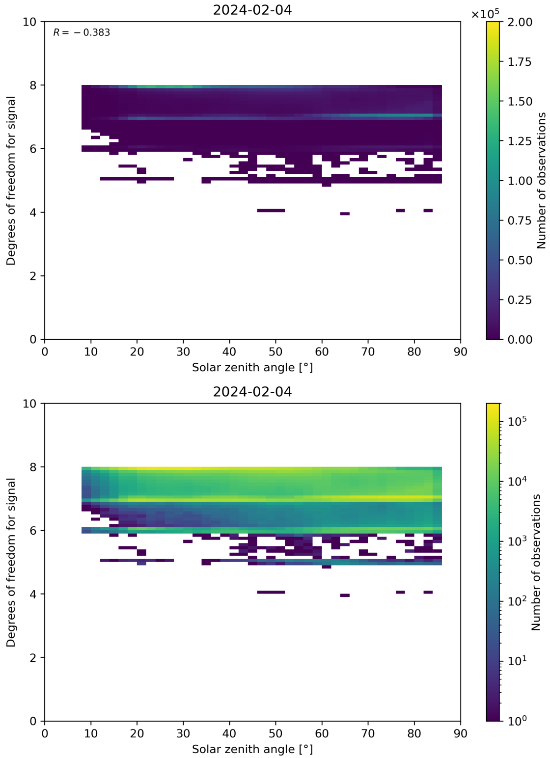
Figure 65: Scatter density plot of “Solar zenith angle” against “Degrees of freedom for signal” for 2024-02-03 to 2024-02-05.
