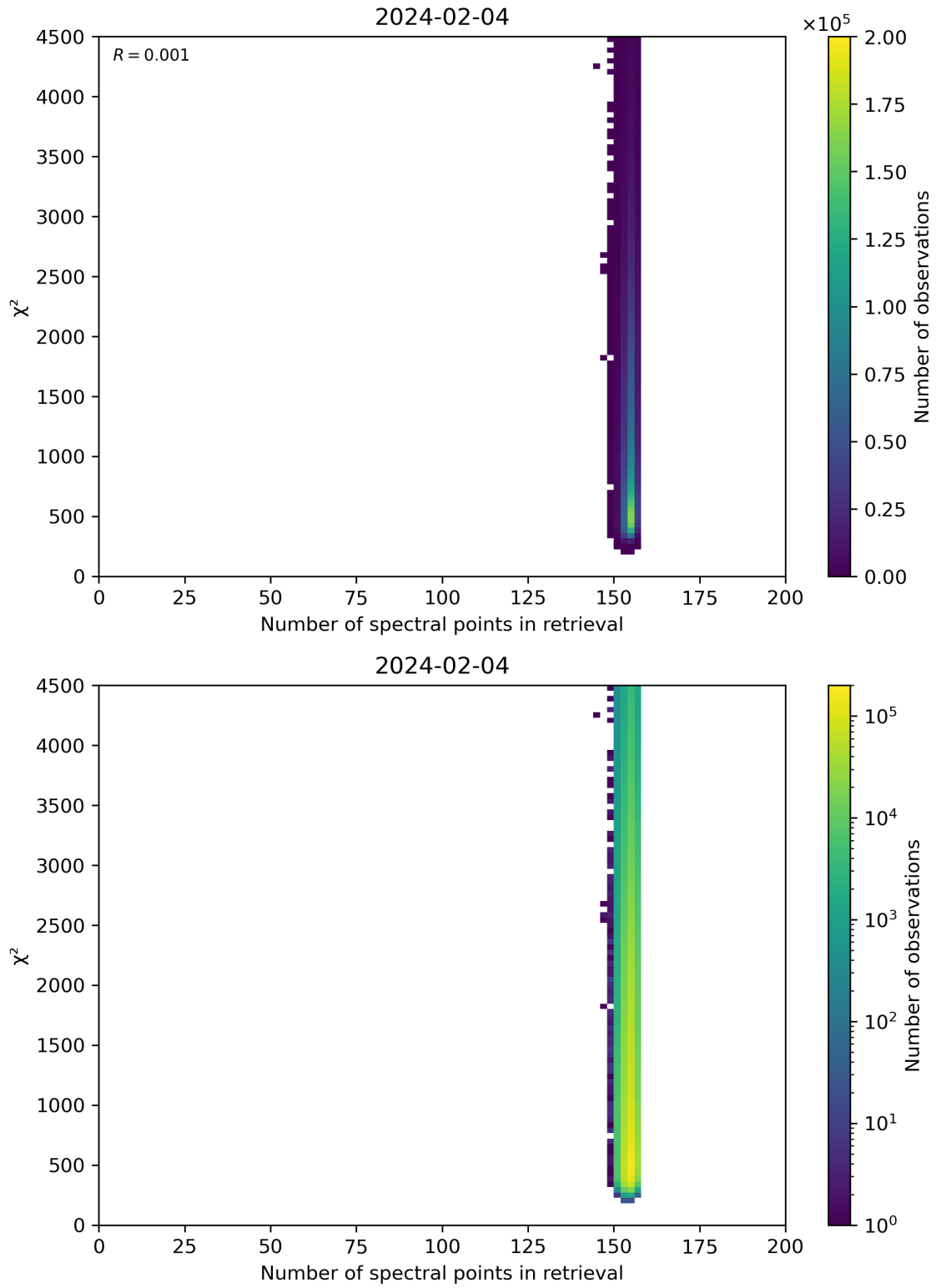
Figure 58: Scatter density plot of “Number of spectral points in retrieval” against “ \chi^2 ” for 2024-02-03 to 2024-02-05.
