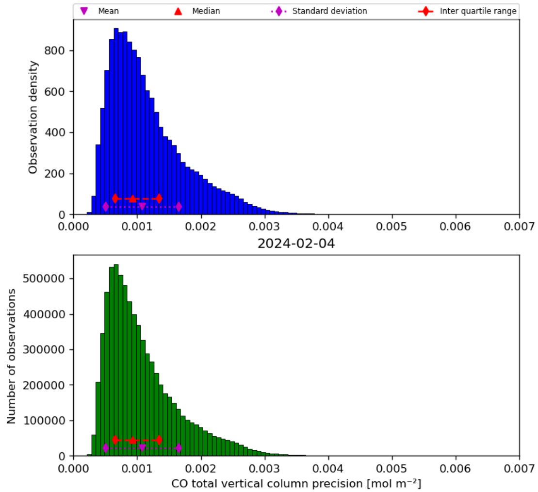
Figure 20: Histogram of “CO total vertical column precision” for 2024-02-03 to 2024-02-05
