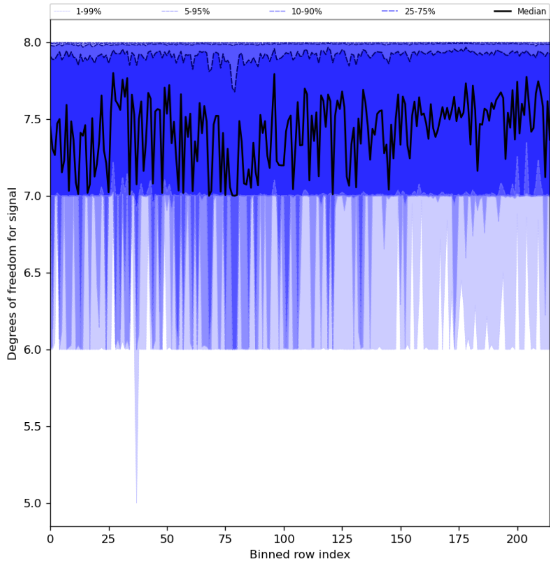
Figure 31: Along track statistics of “Degrees of freedom for signal” for 2024-02-03 to 2024-02-05
