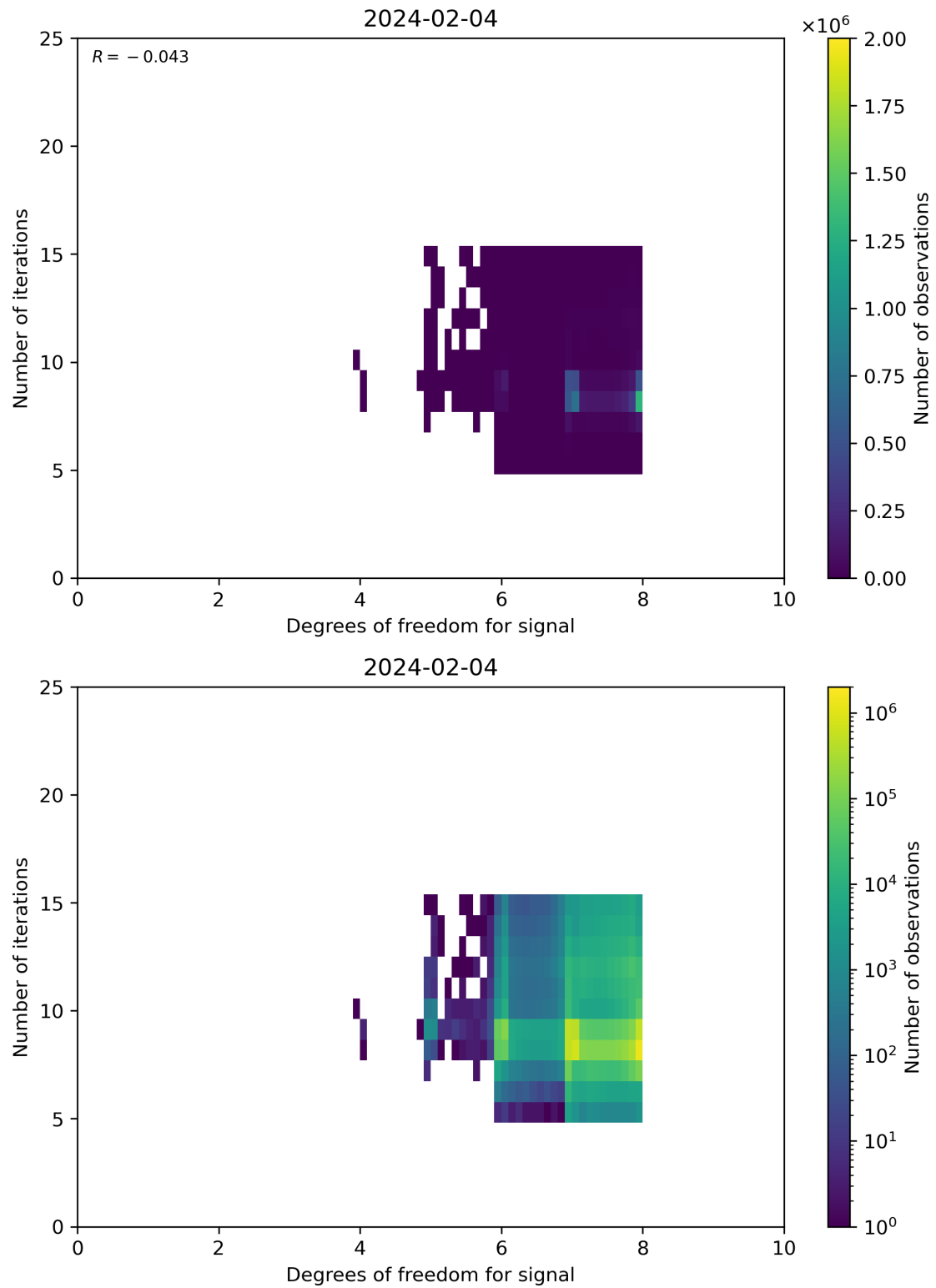
Figure 50: Scatter density plot of “Degrees of freedom for signal” against “Number of iterations” for 2024-02-03 to 2024-02-05.
