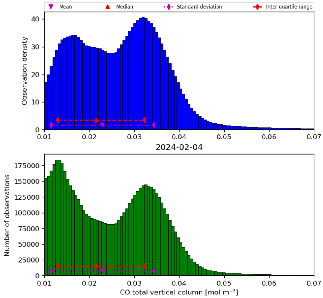
Figure 18: Histogram of “CO total vertical column” for 2024-02-03 to 2024-02-05
