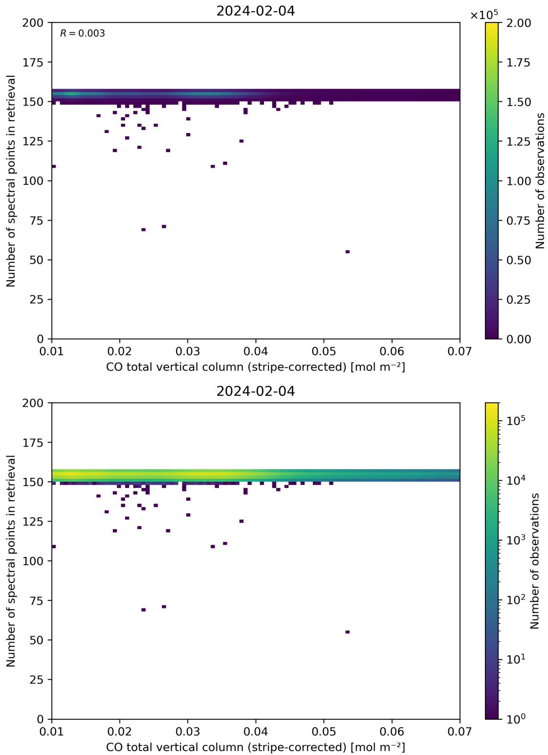
Figure 40: Scatter density plot of “CO total vertical column (stripe-corrected)” against “Number of spectral points in retrieval” for 2024-02-03 to 2024-02-05.
