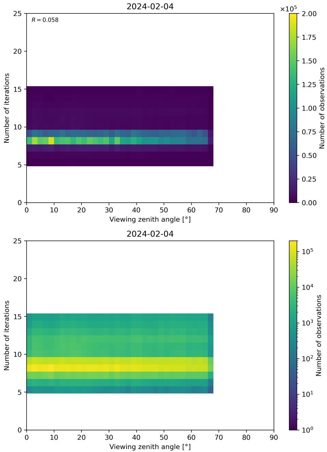
Figure 75: Scatter density plot of “Viewing zenith angle” against “Number of iterations” for 2024-02-03 to 2024-02-05.
