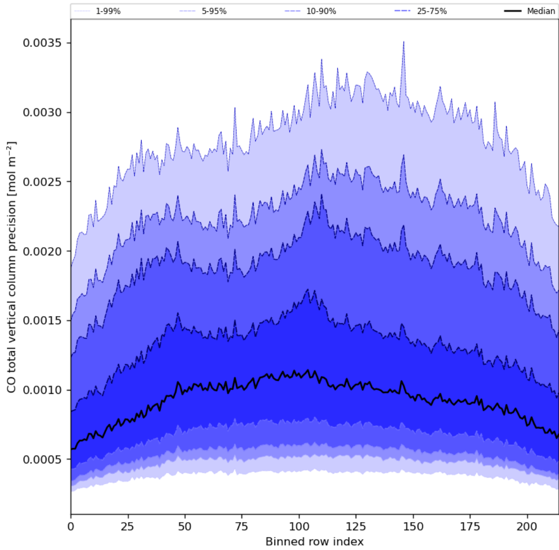
Figure 28: Along track statistics of “CO total vertical column precision” for 2024-02-03 to 2024-02-05
