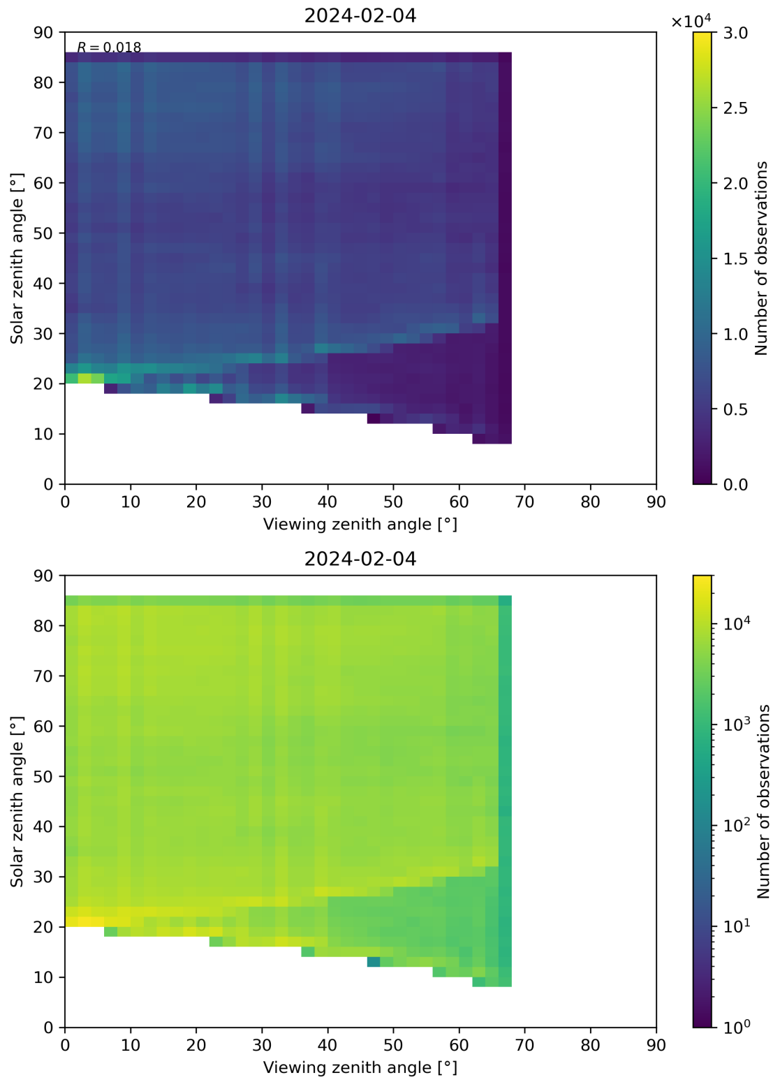
Figure 77: Scatter density plot of “Viewing zenith angle” against “Solar zenith angle” for 2024-02-03 to 2024-02-05.
