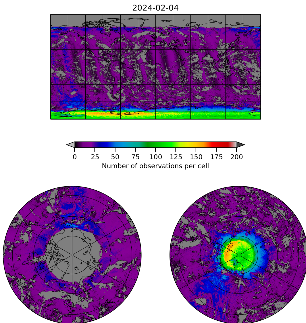
Figure 8: Map of the number of observations for 2024-02-03 to 2024-02-05
