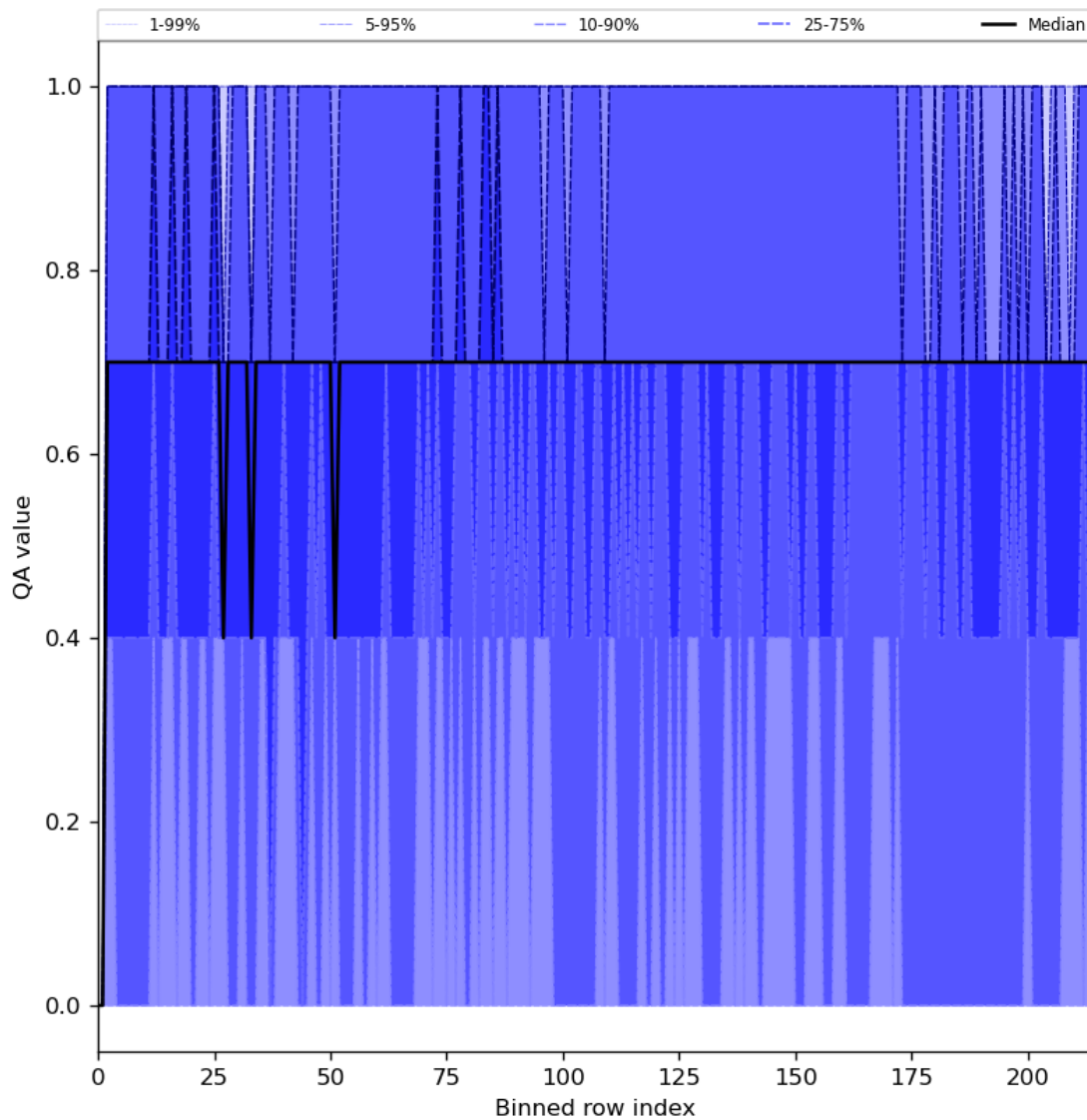
Figure 25: Along track statistics of “QA value” for 2024-02-03 to 2024-02-05
