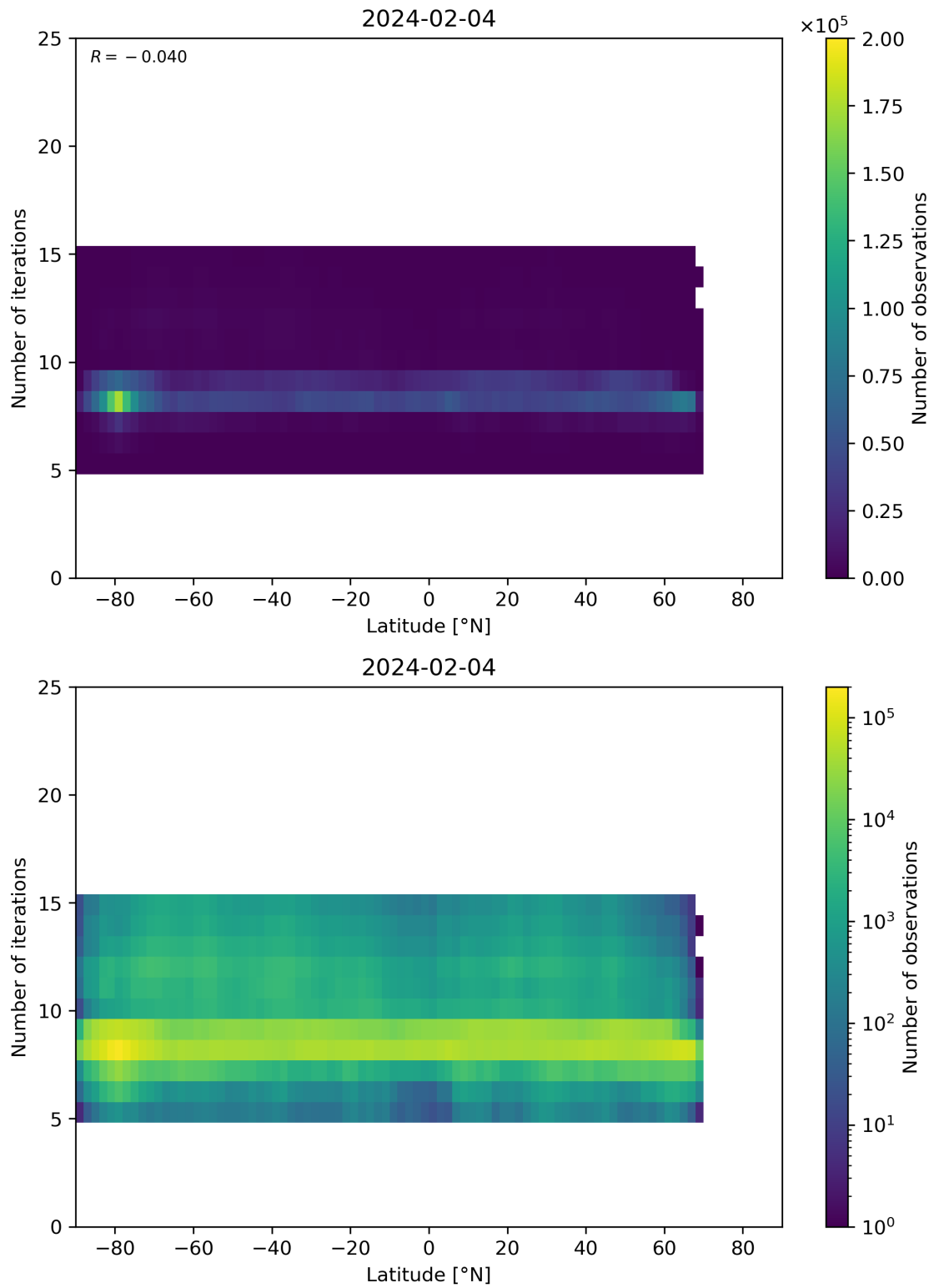
Figure 56: Scatter density plot of “Latitude” against “Number of iterations” for 2024-02-03 to 2024-02-05.
