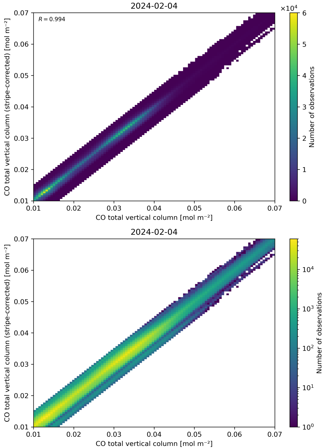
Figure 33: Scatter density plot of “CO total vertical column” against “CO total vertical column (stripe-corrected)” for 2024-02-03 to 2024-02-05.
