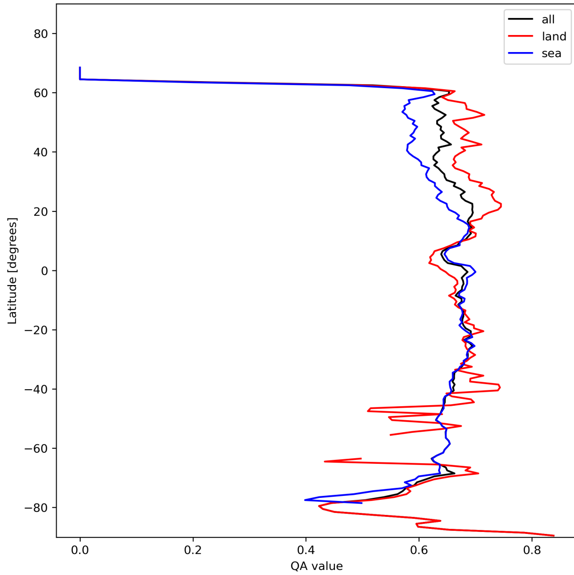
Figure 9: Zonal average of “QA value” for 2024-02-03 to 2024-02-05.
