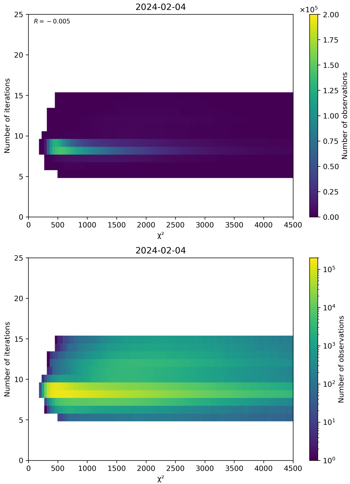
Figure 49: Scatter density plot of “ \chi^2 ” against “Number of iterations” for 2024-02-03 to 2024-02-05.
