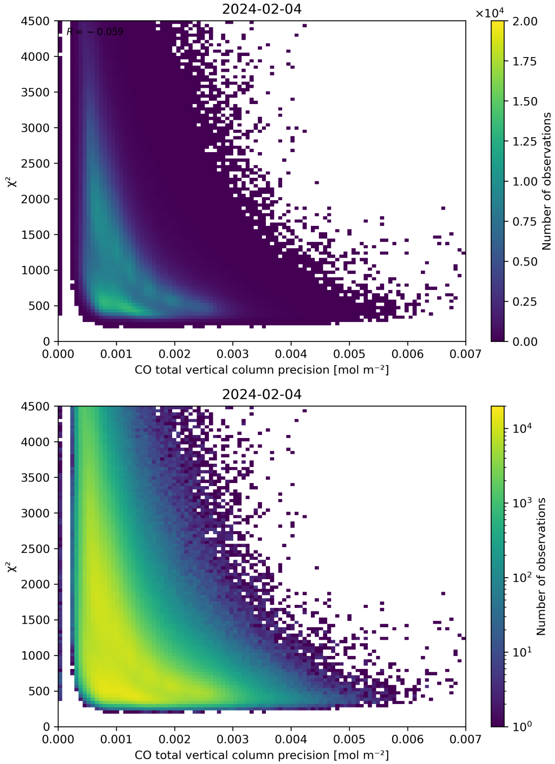
Figure 44: Scatter density plot of “CO total vertical column precision” against “ \chi^2 ” for 2024-02-03 to 2024-02-05.
