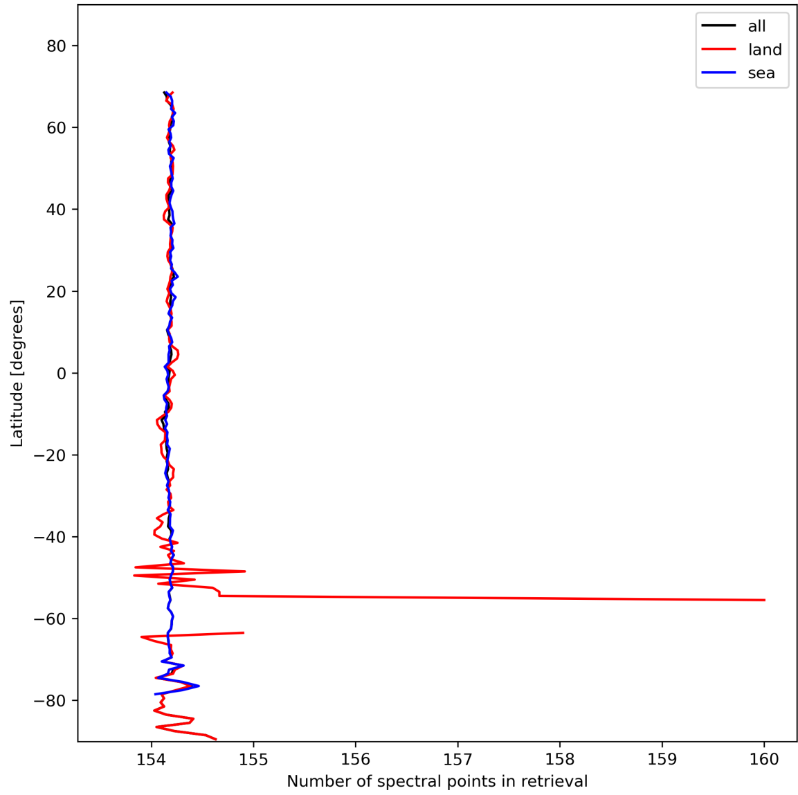
Figure 13: Zonal average of “Number of spectral points in retrieval” for 2024-02-03 to 2024-02-05.
