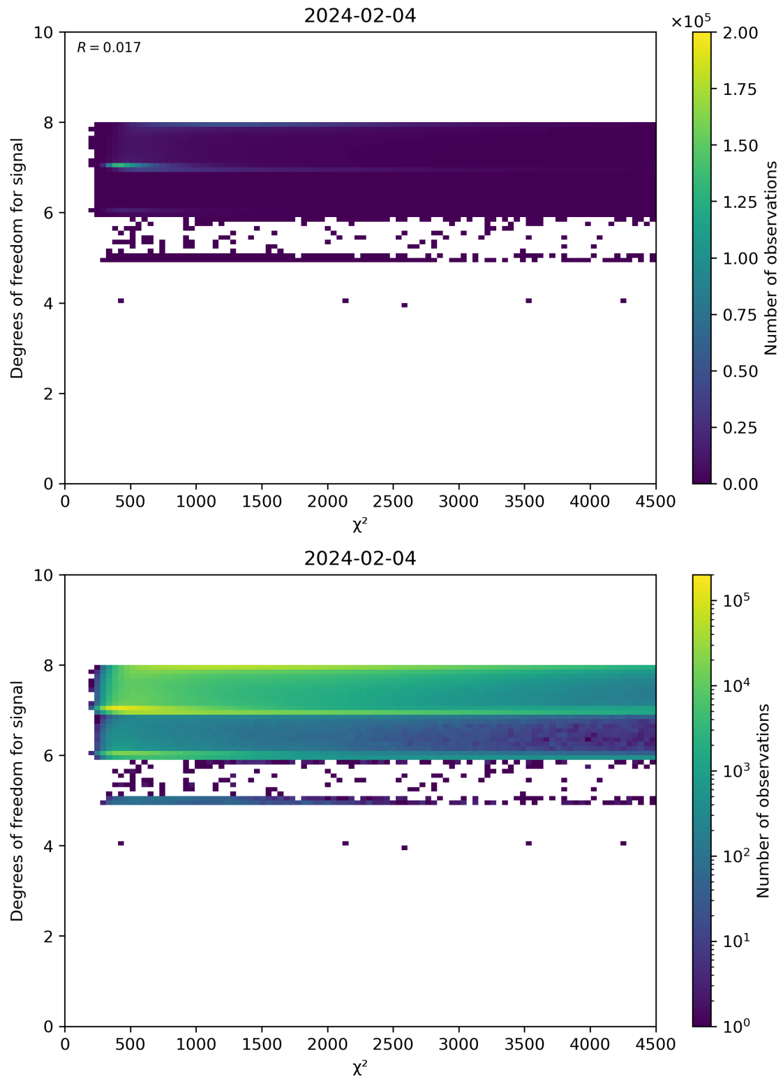
Figure 48: Scatter density plot of “ \chi^2 ” against “Degrees of freedom for signal” for 2024-02-03 to 2024-02-05.
