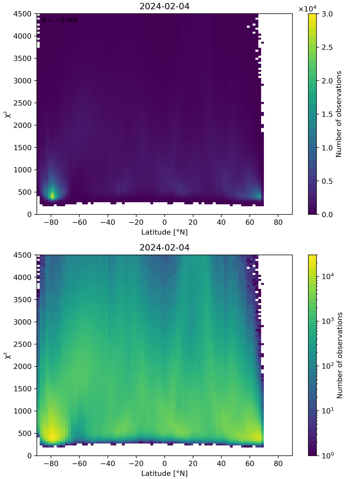
Figure 54: Scatter density plot of “Latitude” against “ \chi^2 ” for 2024-02-03 to 2024-02-05.
