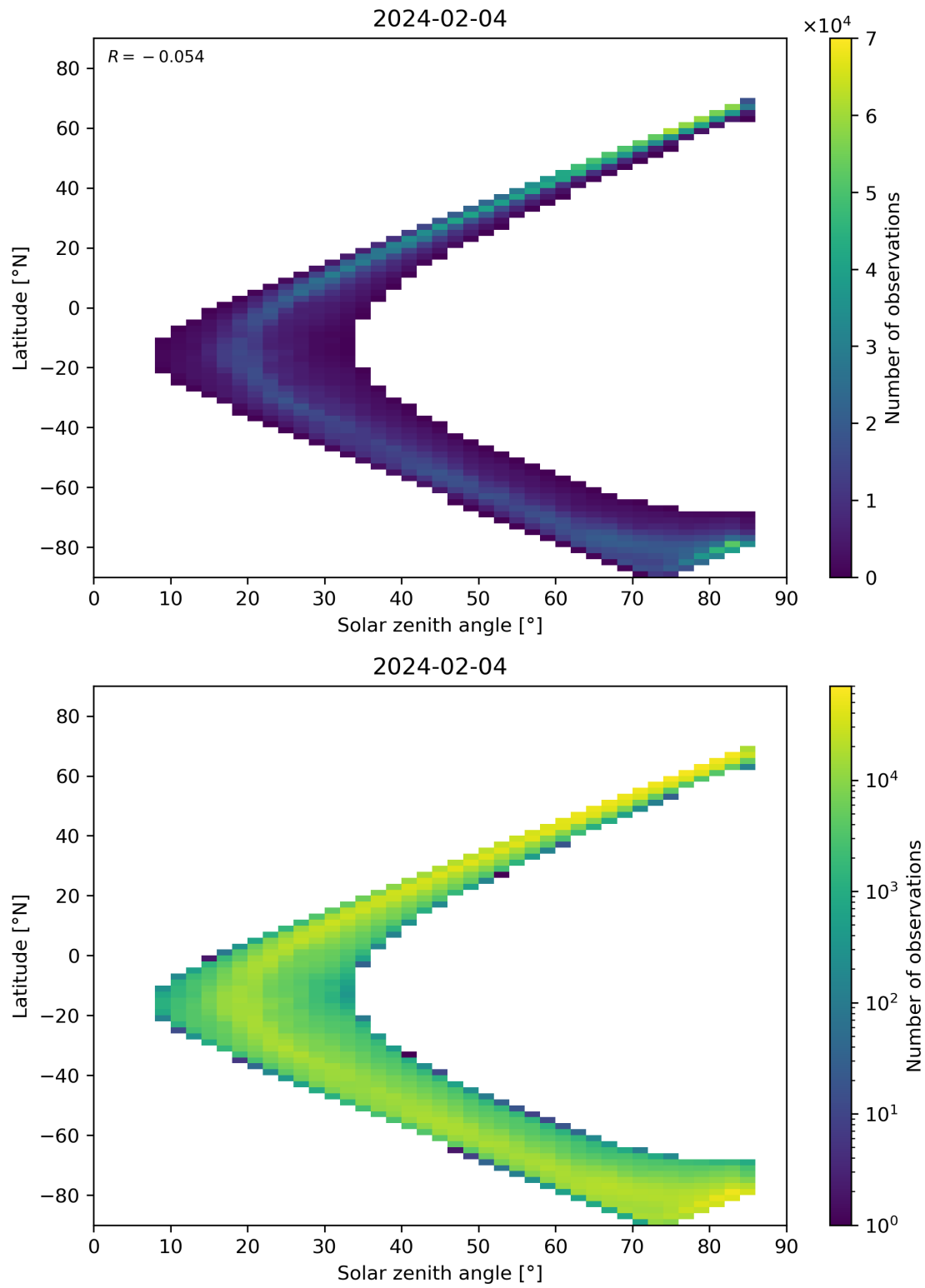
Figure 66: Scatter density plot of “Solar zenith angle” against “Latitude” for 2024-02-03 to 2024-02-05.
