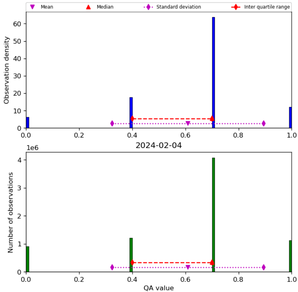
Figure 17: Histogram of “QA value” for 2024-02-03 to 2024-02-05
