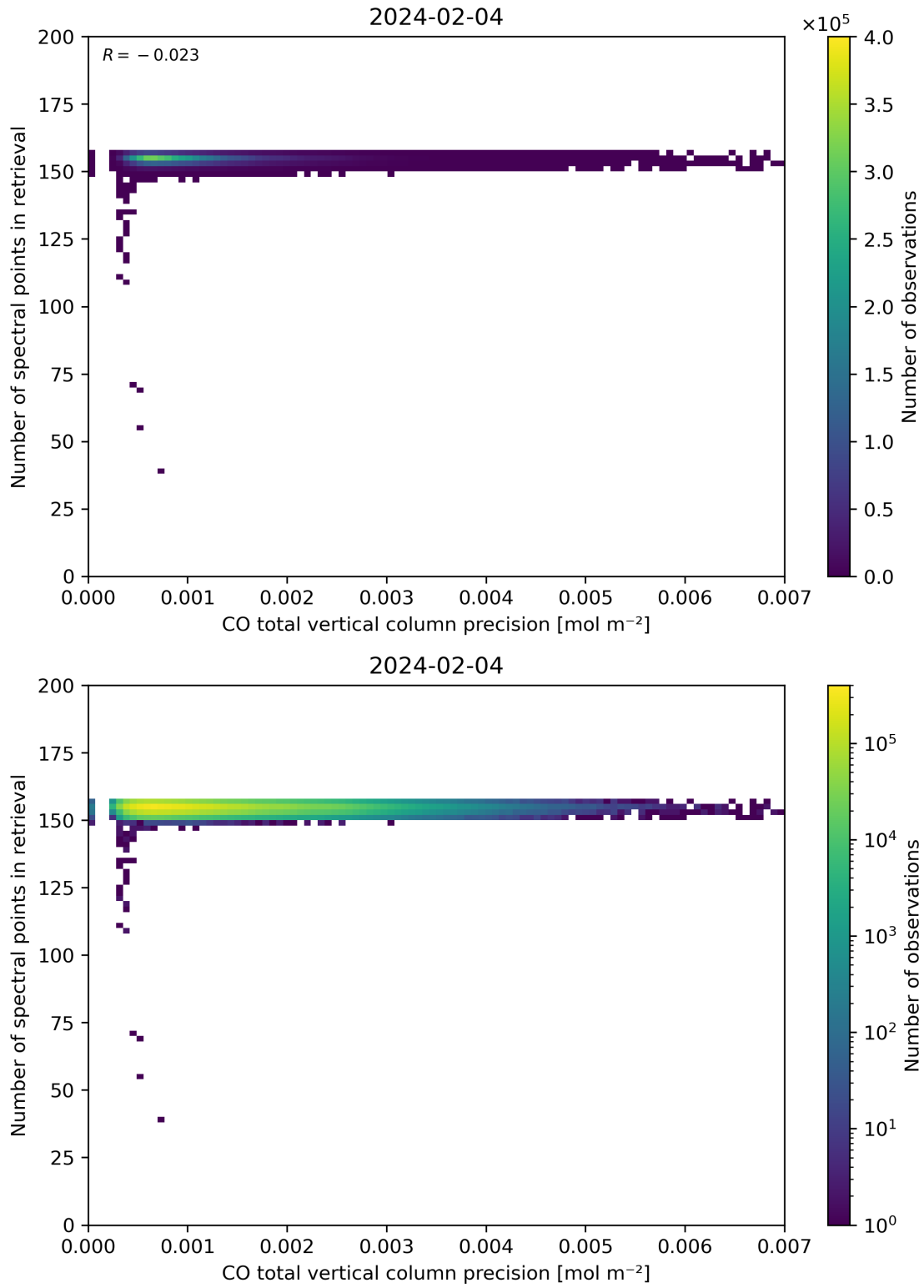
Figure 47: Scatter density plot of “CO total vertical column precision” against “Number of spectral points in retrieval” for 2024-02-03 to 2024-02-05.
