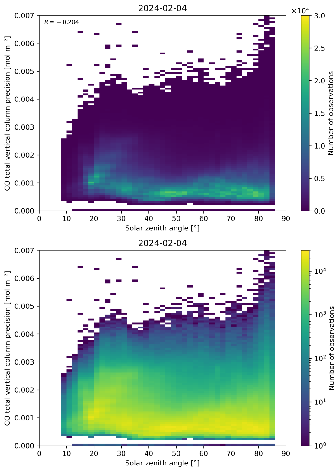
Figure 63: Scatter density plot of “Solar zenith angle” against “CO total vertical column precision” for 2024-02-03 to 2024-02-05.
