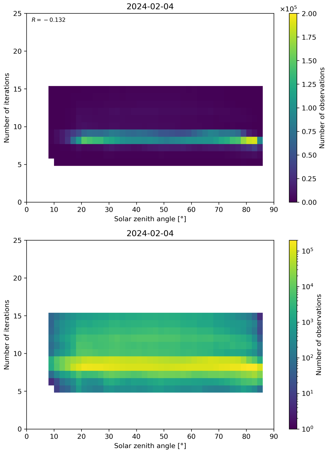
Figure 67: Scatter density plot of “Solar zenith angle” against “Number of iterations” for 2024-02-03 to 2024-02-05.
