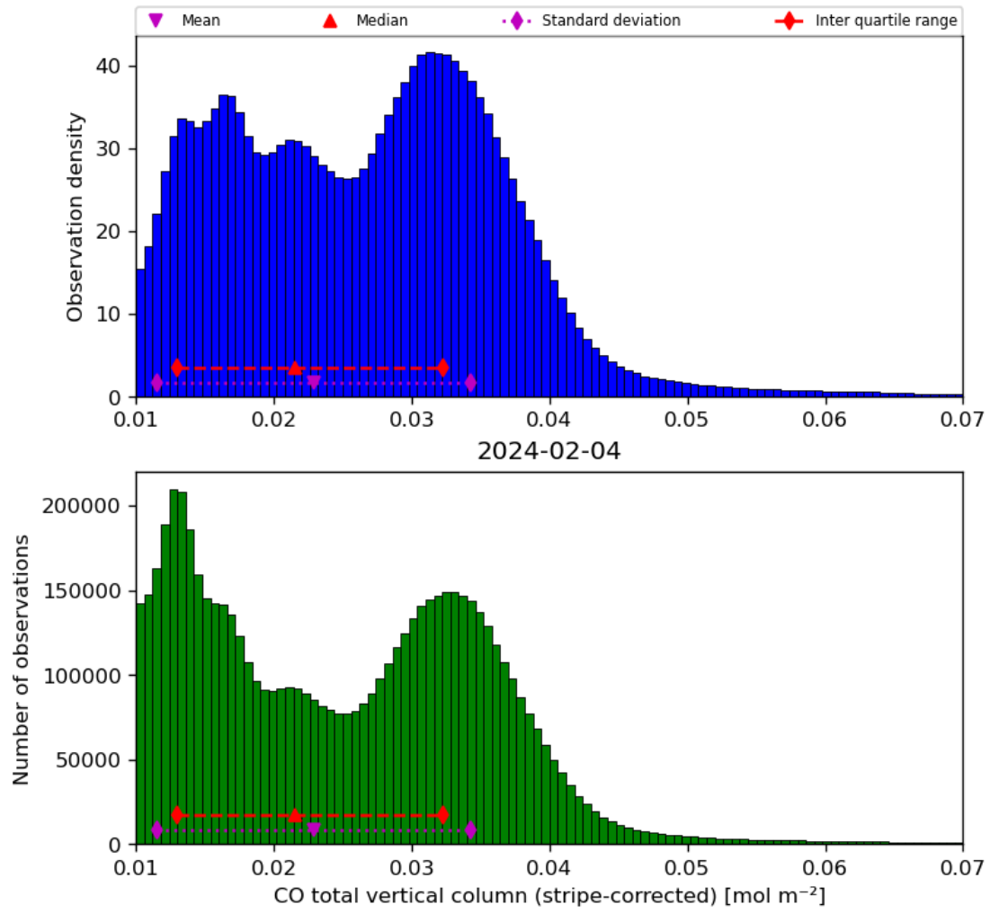
Figure 19: Histogram of “CO total vertical column (stripe-corrected)” for 2024-02-03 to 2024-02-05
