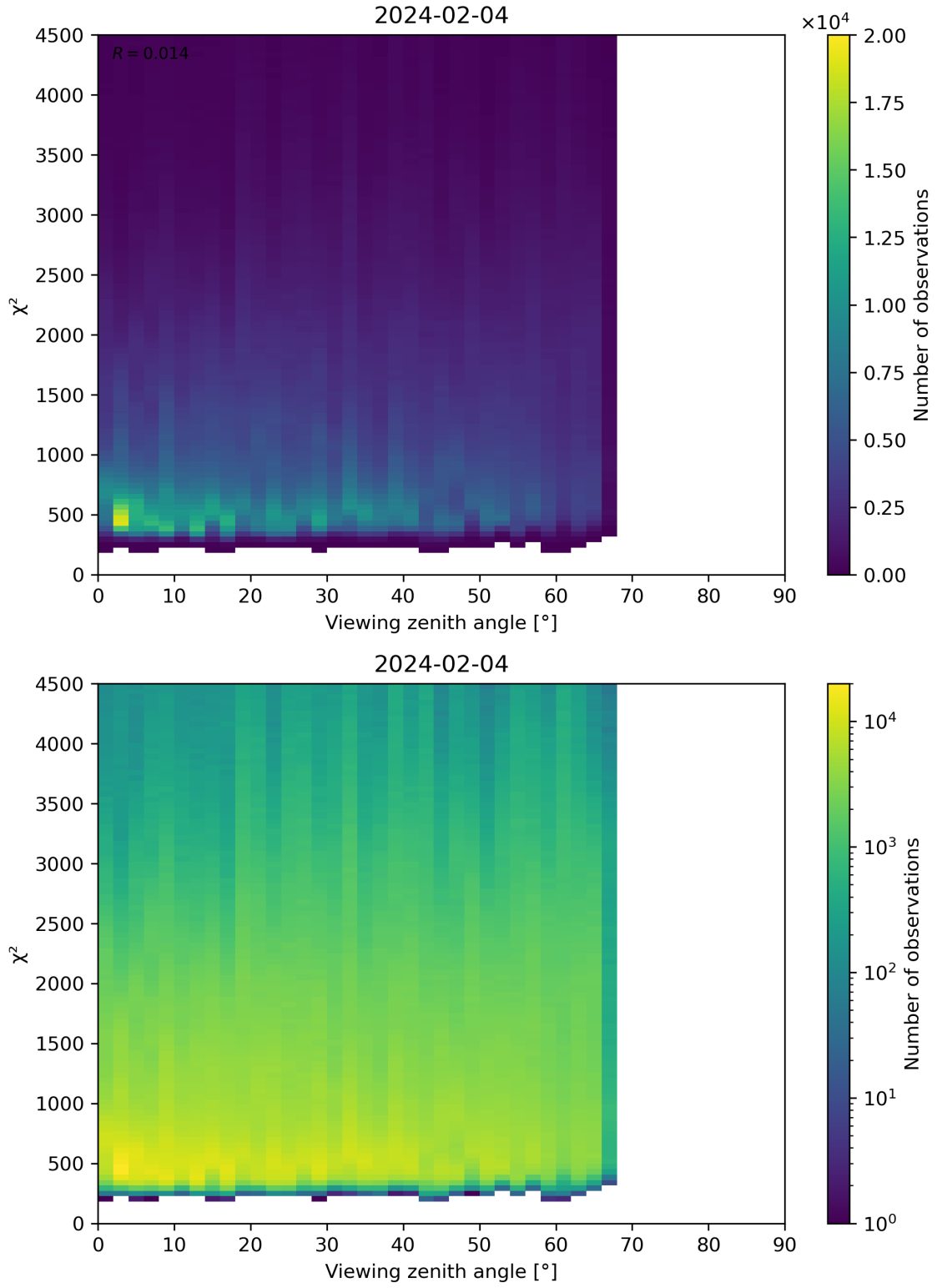
Figure 72: Scatter density plot of “Viewing zenith angle” against “ \chi^2 ” for 2024-02-03 to 2024-02-05.
