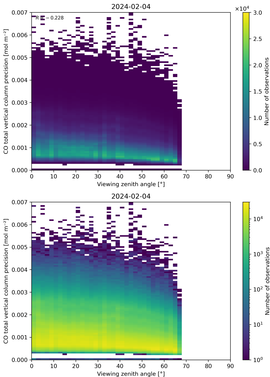
Figure 71: Scatter density plot of “Viewing zenith angle” against “CO total vertical column precision” for 2024-02-03 to 2024-02-05.
