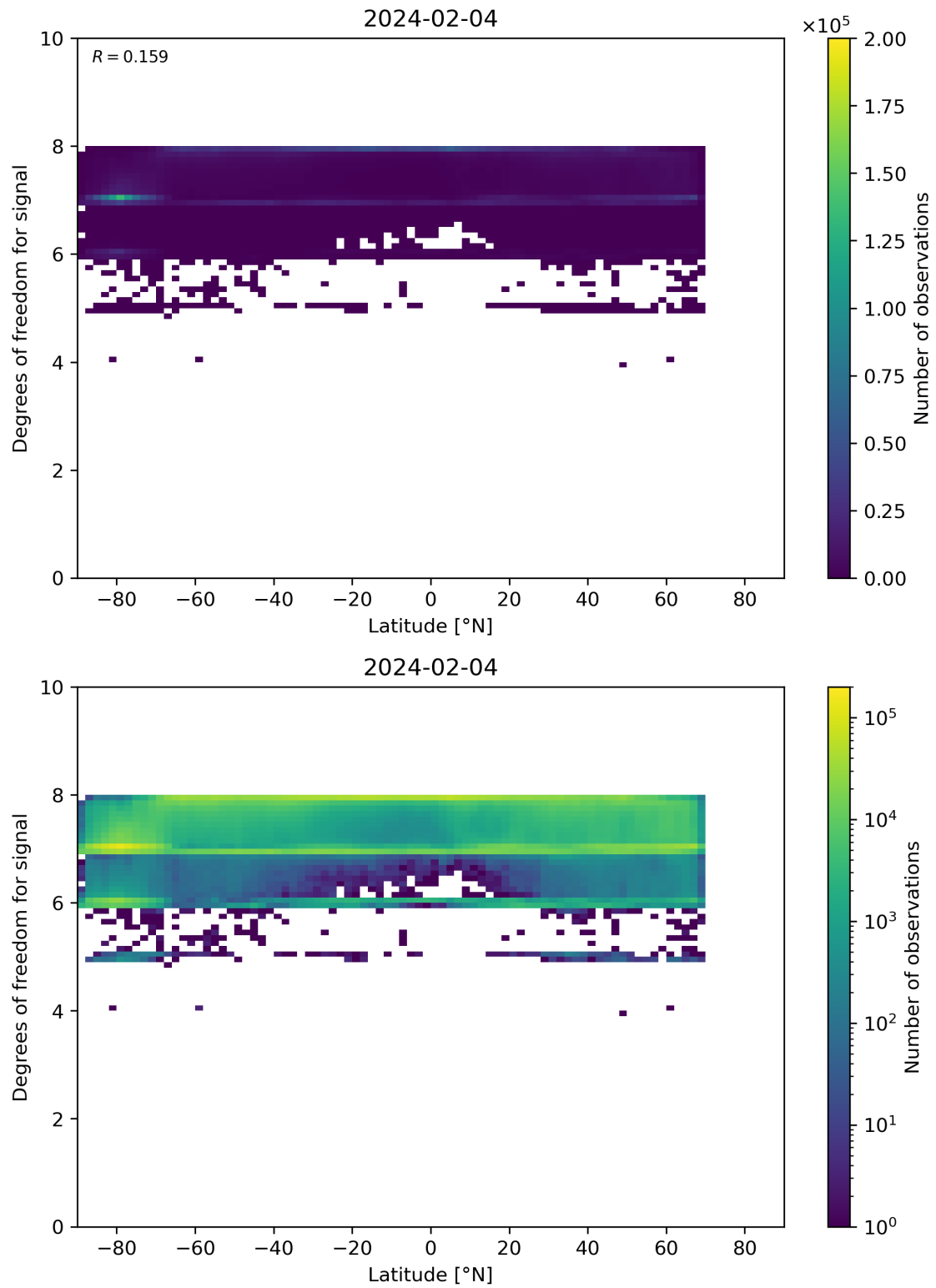
Figure 55: Scatter density plot of “Latitude” against “Degrees of freedom for signal” for 2024-02-03 to 2024-02-05.
