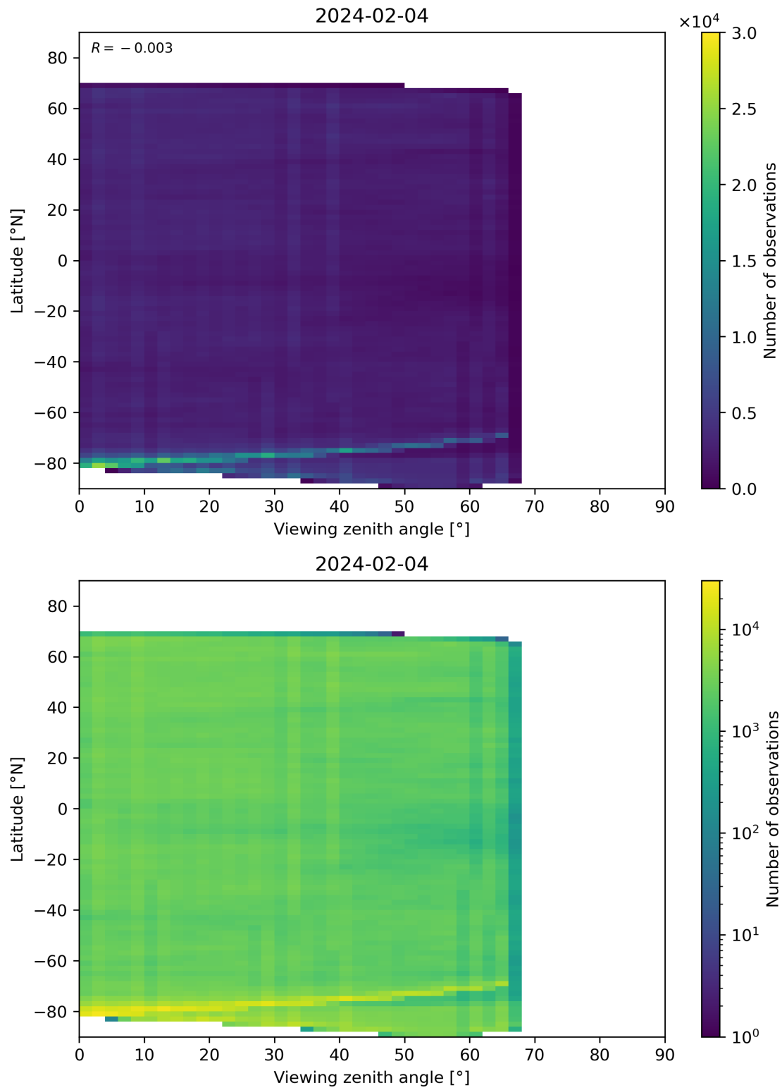
Figure 74: Scatter density plot of “Viewing zenith angle” against “Latitude” for 2024-02-03 to 2024-02-05.
