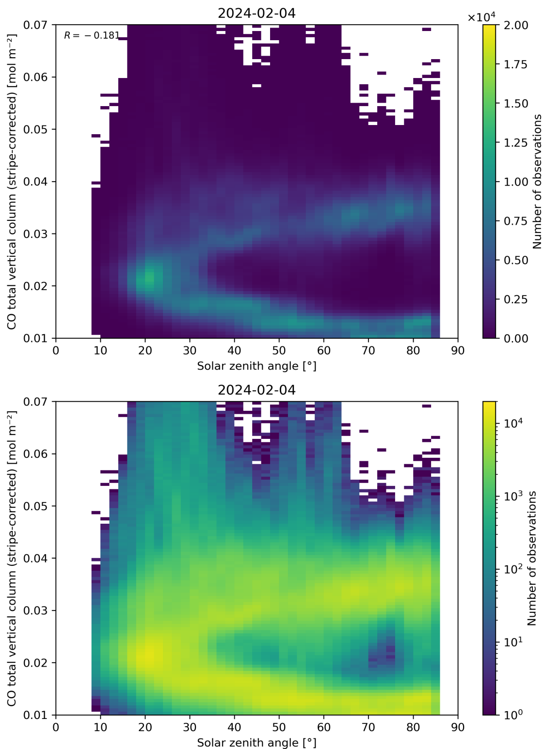
Figure 62: Scatter density plot of “Solar zenith angle” against “CO total vertical column (stripe-corrected)” for 2024-02-03 to 2024-02-05.
