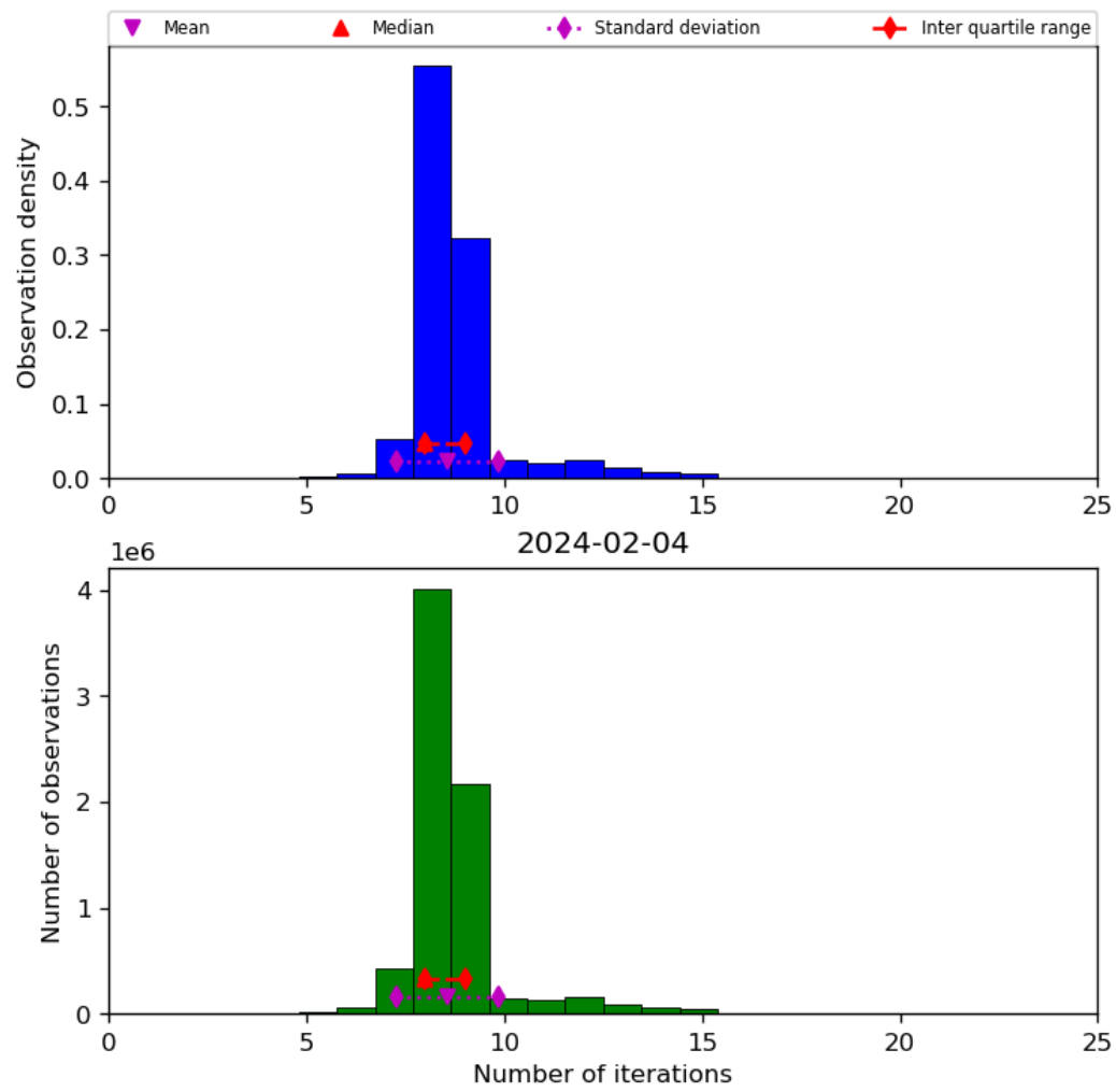
Figure 24: Histogram of “Number of iterations” for 2024-02-03 to 2024-02-05
