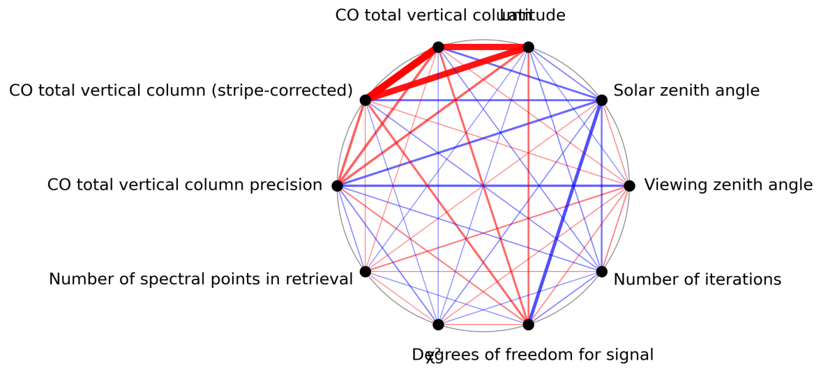
Figure 1: Map of correlation graph for 2024-02-03 to 2024-02-05.
