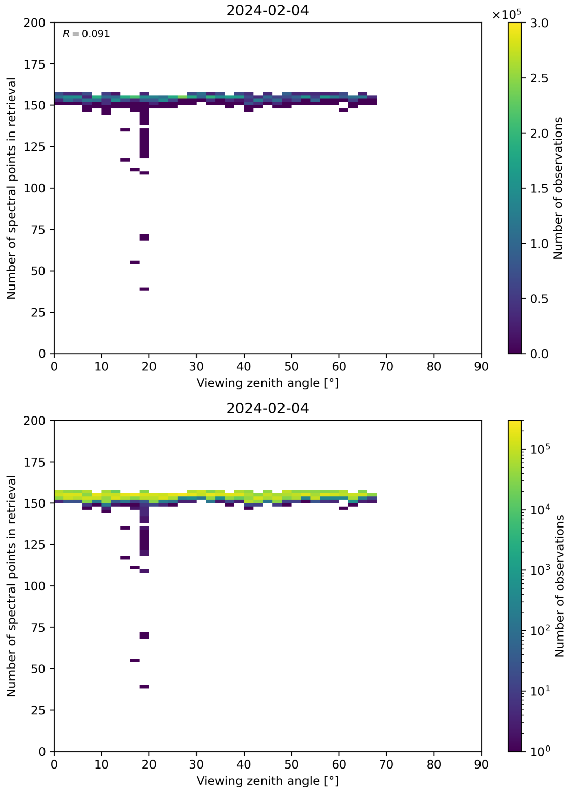
Figure 76: Scatter density plot of “Viewing zenith angle” against “Number of spectral points in retrieval” for 2024-02-03 to 2024-02-05.
