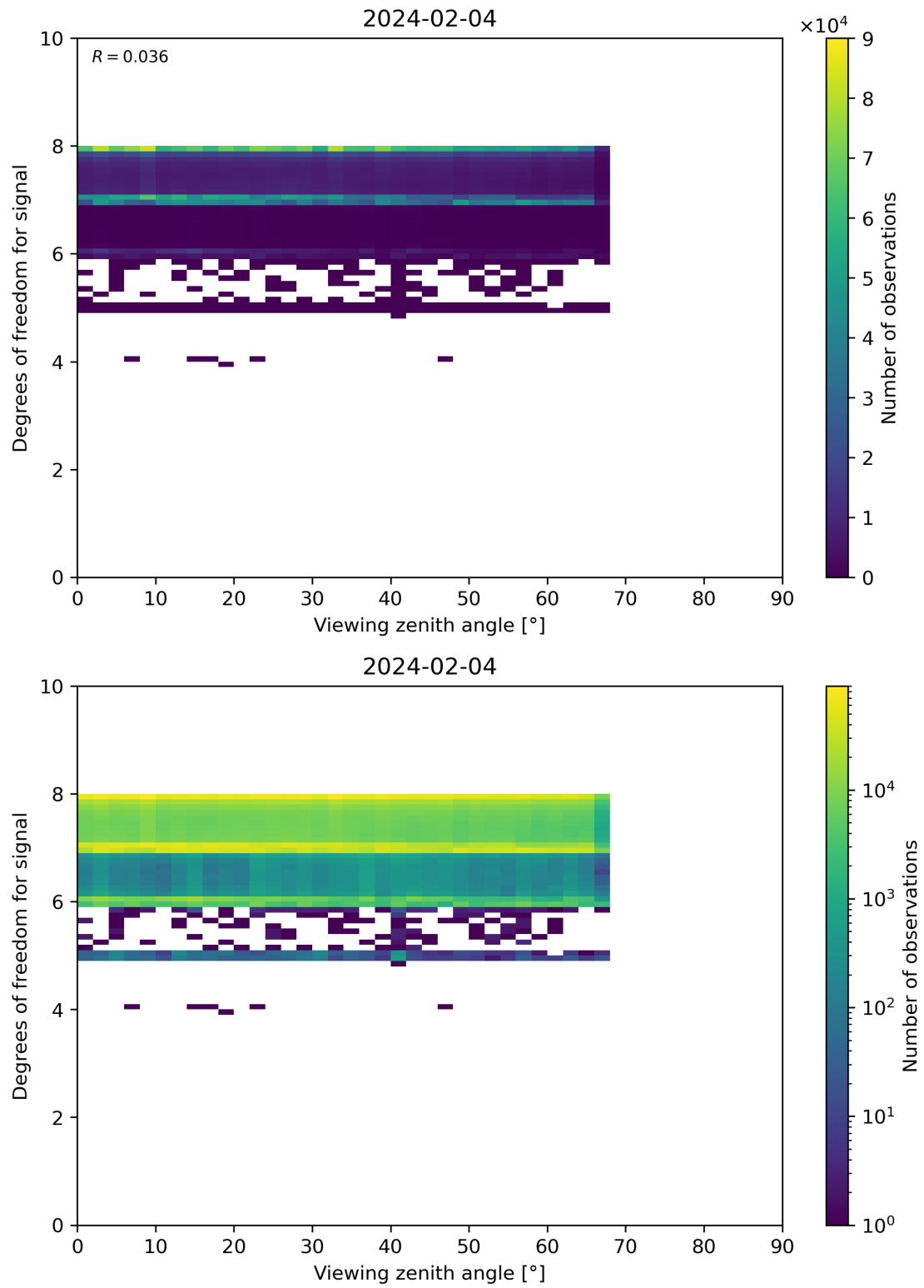
Figure 73: Scatter density plot of “Viewing zenith angle” against “Degrees of freedom for signal” for 2024-02-03 to 2024-02-05.
