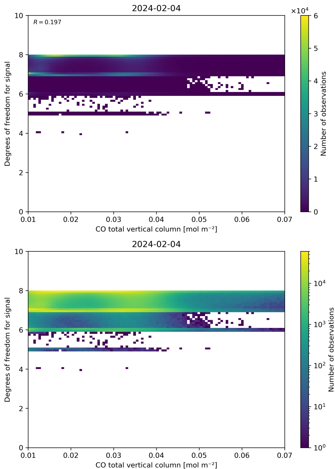
Figure 41: Scatter density plot of “CO total vertical column” against “Degrees of freedom for signal” for 2024-02-03 to 2024-02-05.
