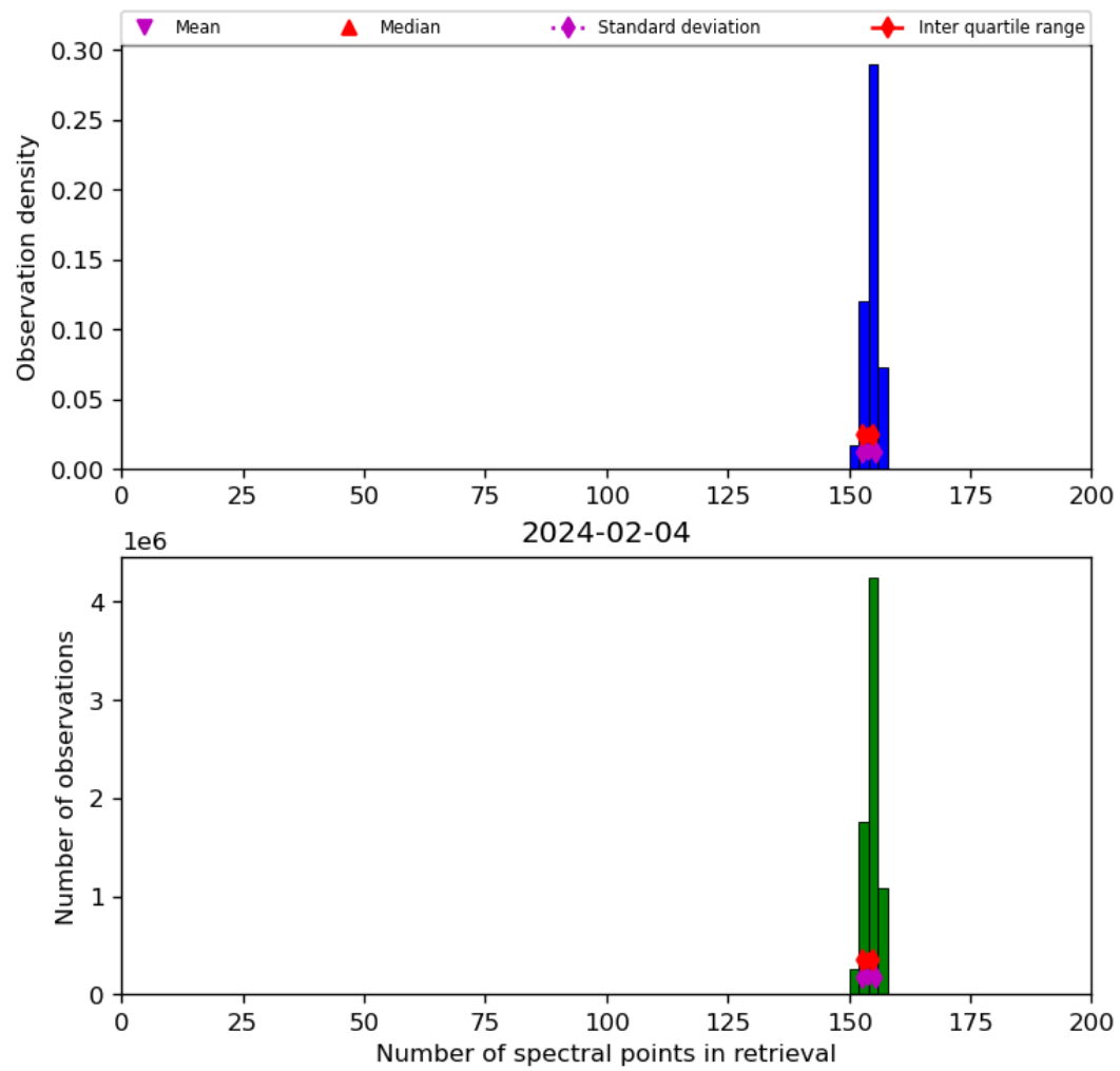
Figure 21: Histogram of “Number of spectral points in retrieval” for 2024-02-03 to 2024-02-05
