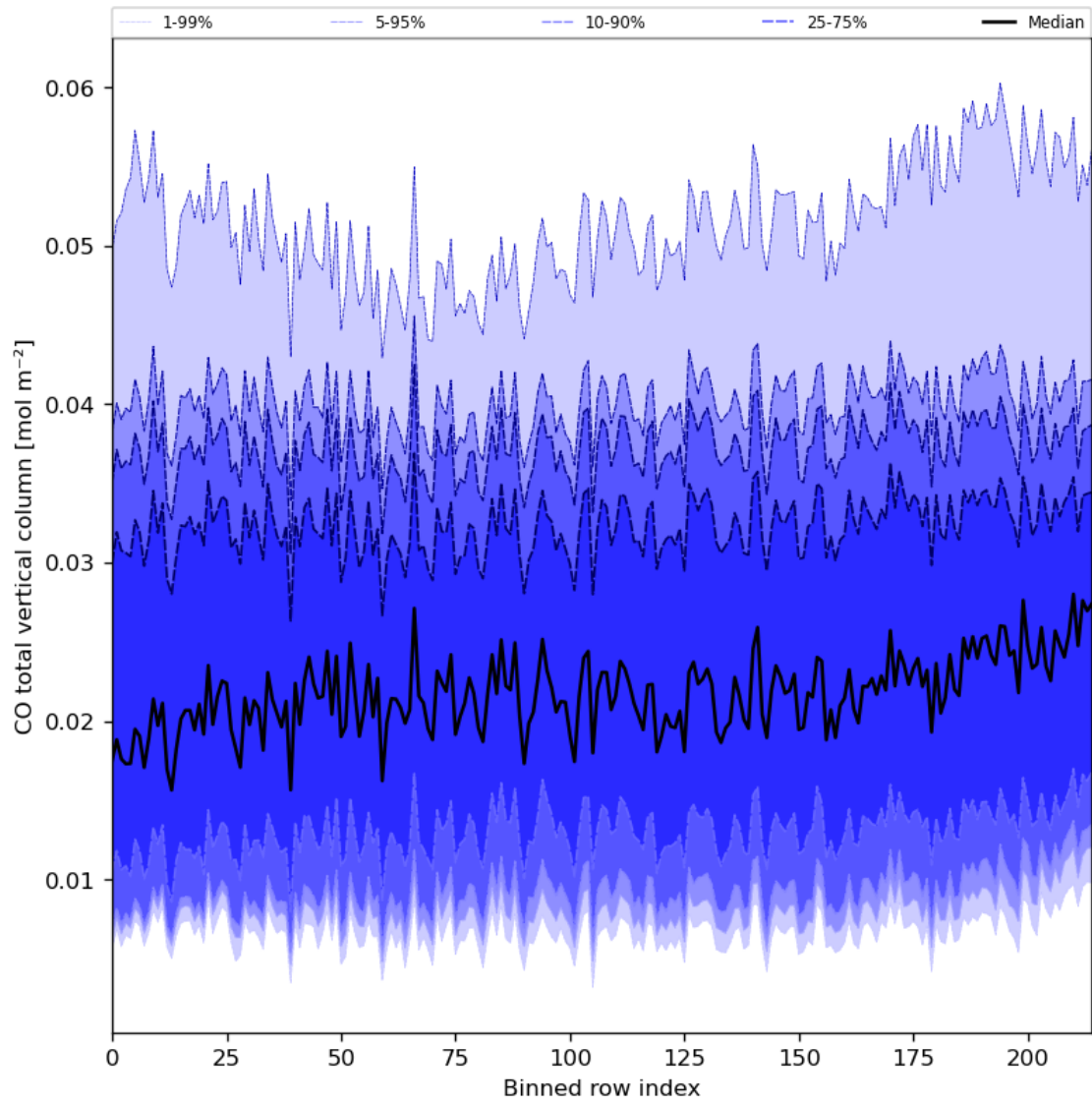
Figure 26: Along track statistics of “CO total vertical column” for 2024-02-03 to 2024-02-05
