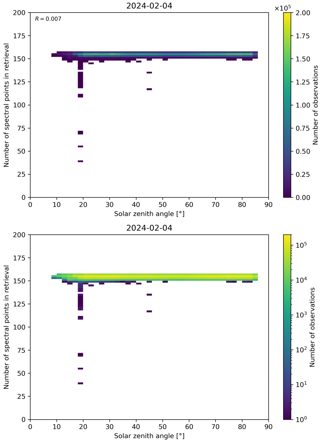
Figure 68: Scatter density plot of “Solar zenith angle” against “Number of spectral points in retrieval” for 2024-02-03 to 2024-02-05.
