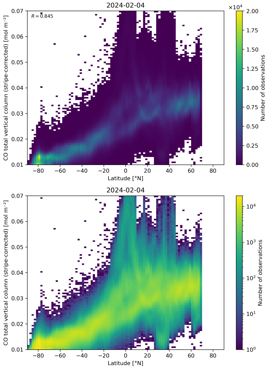
Figure 52: Scatter density plot of “Latitude” against “CO total vertical column (stripe-corrected)” for 2024-02-03 to 2024-02-05.
