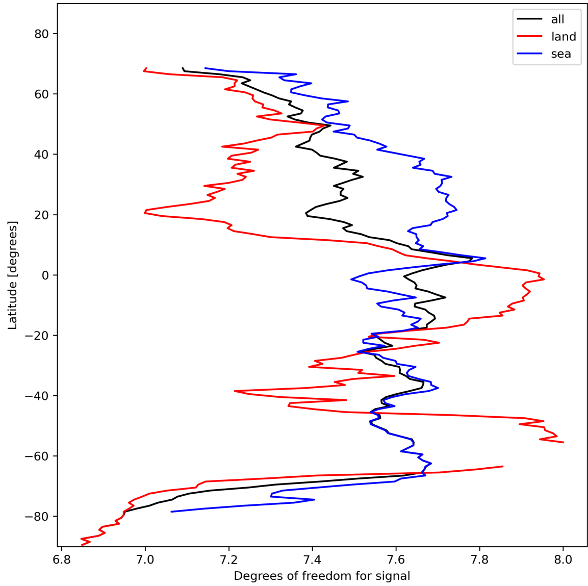
Figure 15: Zonal average of “Degrees of freedom for signal” for 2024-02-03 to 2024-02-05.
