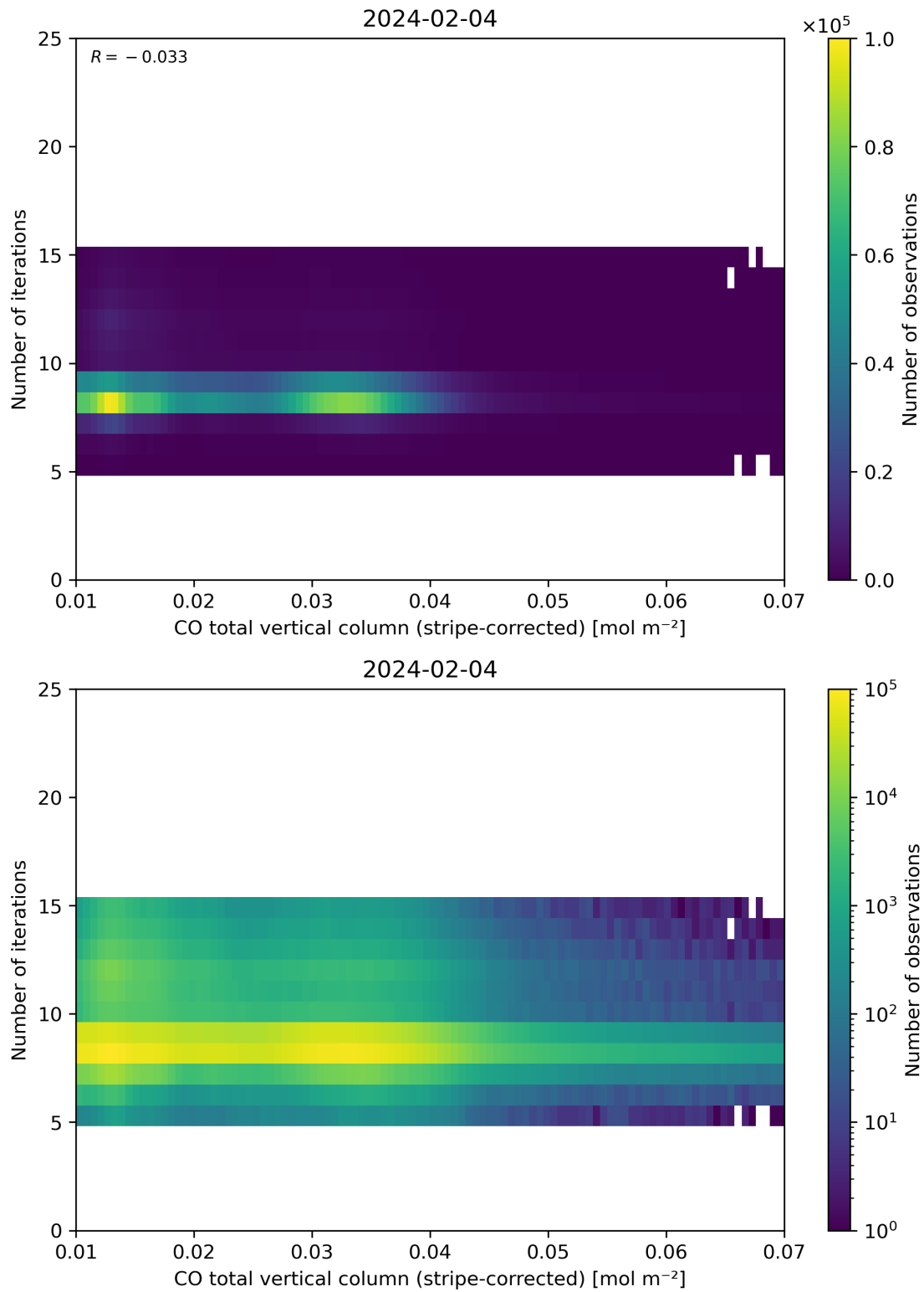
Figure 39: Scatter density plot of “CO total vertical column (stripe-corrected)” against “Number of iterations” for 2024-02-03 to 2024-02-05.
