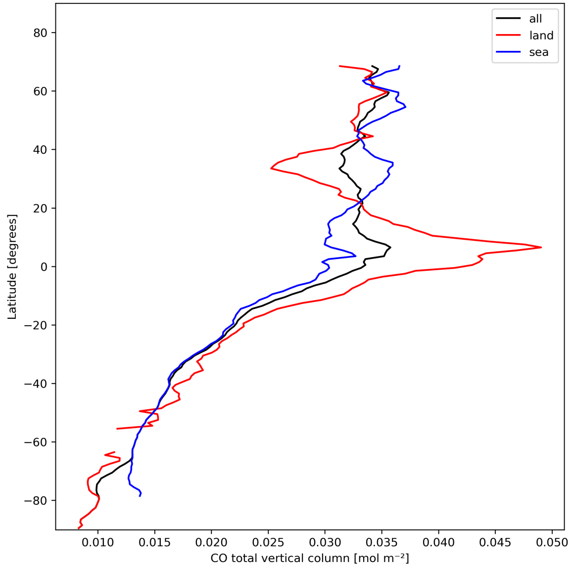
Figure 10: Zonal average of “CO total vertical column” for 2024-02-03 to 2024-02-05.
