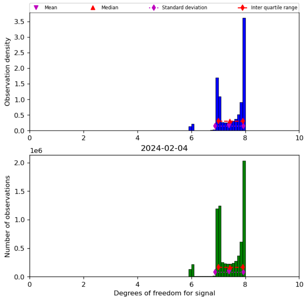
Figure 23: Histogram of “Degrees of freedom for signal” for 2024-02-03 to 2024-02-05
