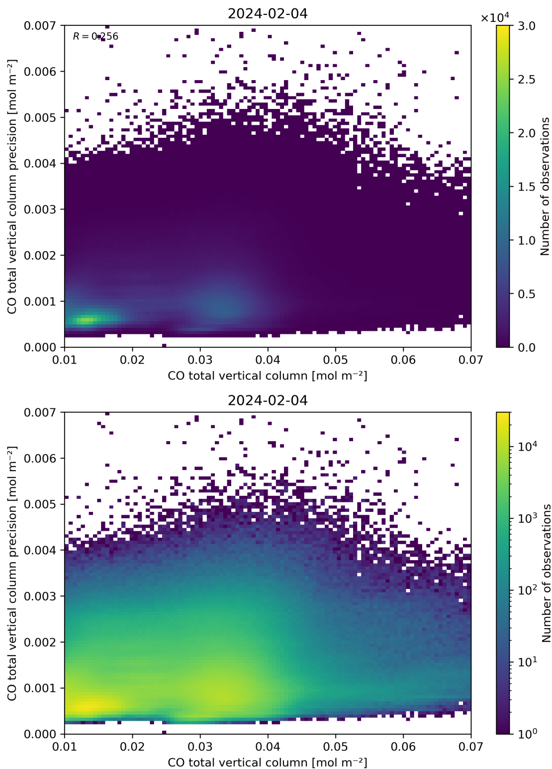
Figure 34: Scatter density plot of “CO total vertical column” against “CO total vertical column precision” for 2024-02-03 to 2024-02-05.
