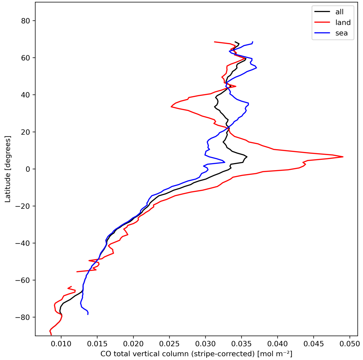
Figure 11: Zonal average of “CO total vertical column (stripe-corrected)” for 2024-02-03 to 2024-02-05.
