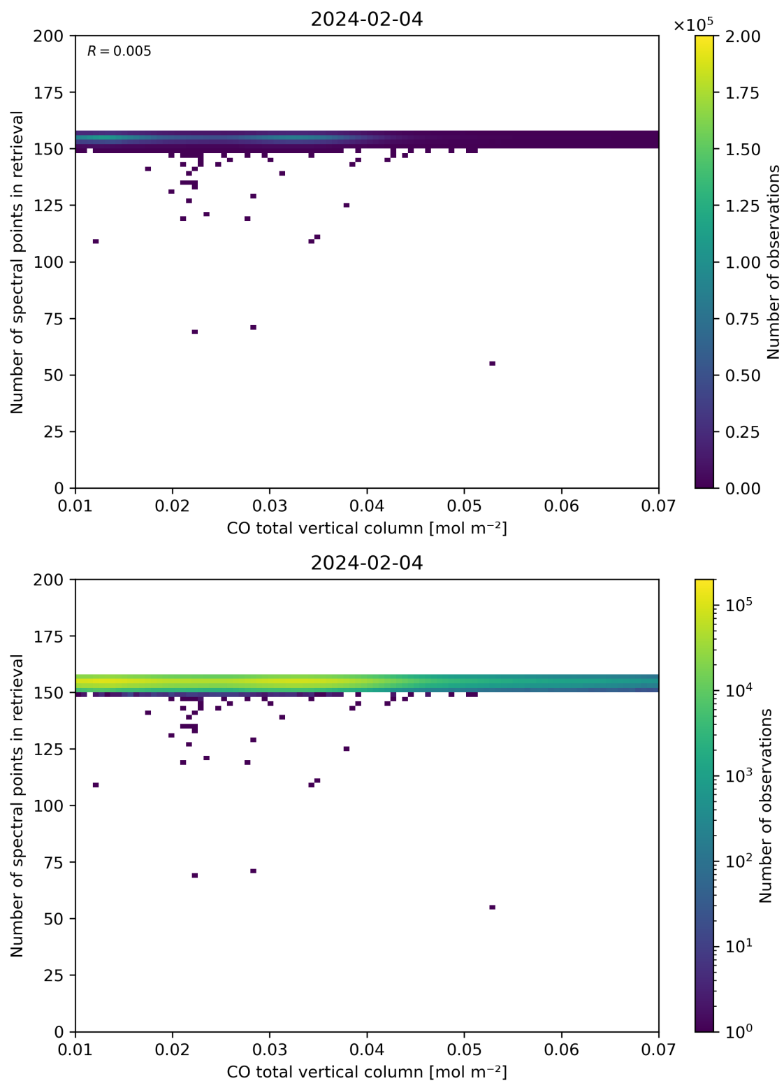
Figure 43: Scatter density plot of “CO total vertical column” against “Number of spectral points in retrieval” for 2024-02-03 to 2024-02-05.
