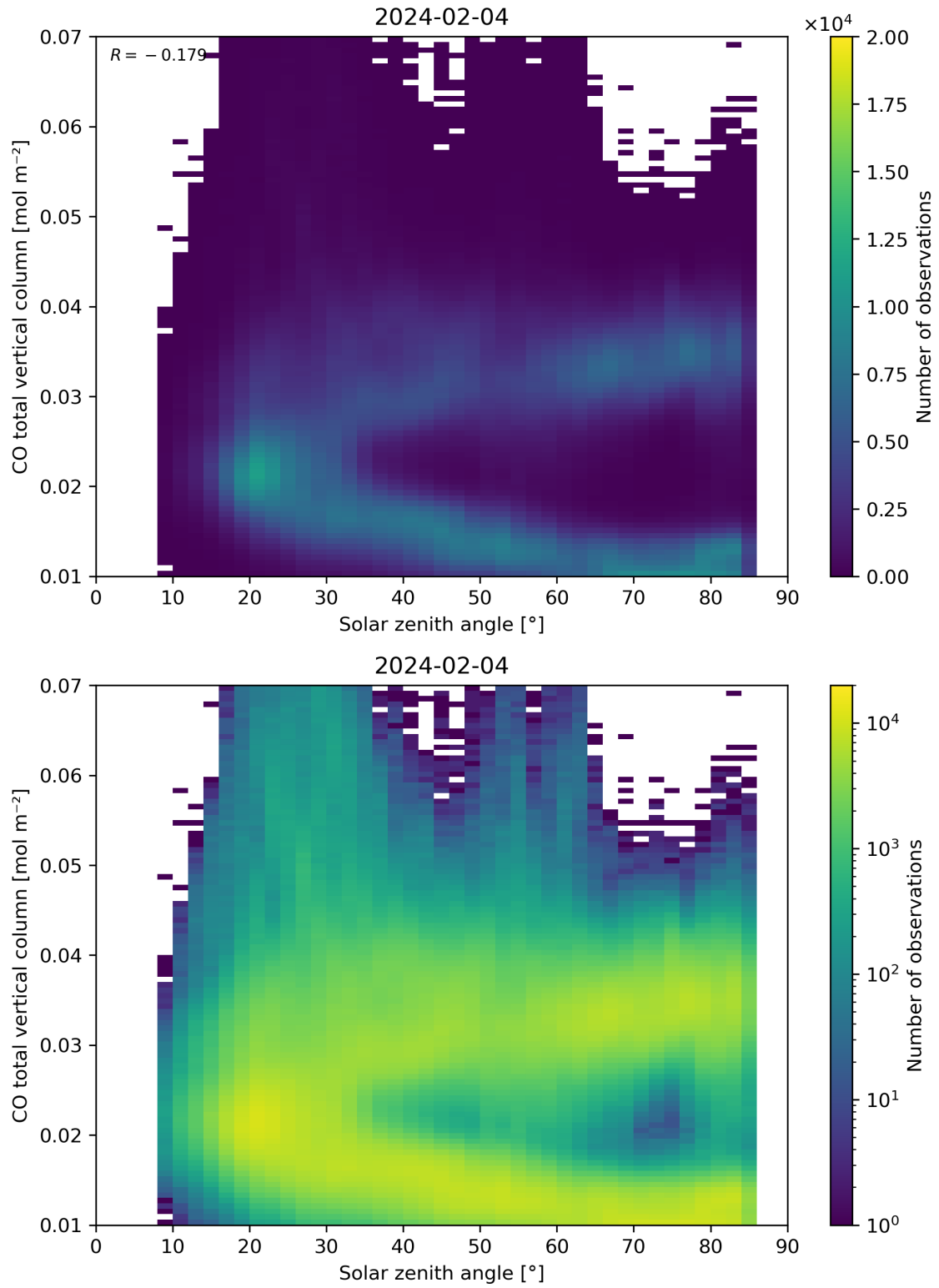
Figure 61: Scatter density plot of “Solar zenith angle” against “CO total vertical column” for 2024-02-03 to 2024-02-05.
