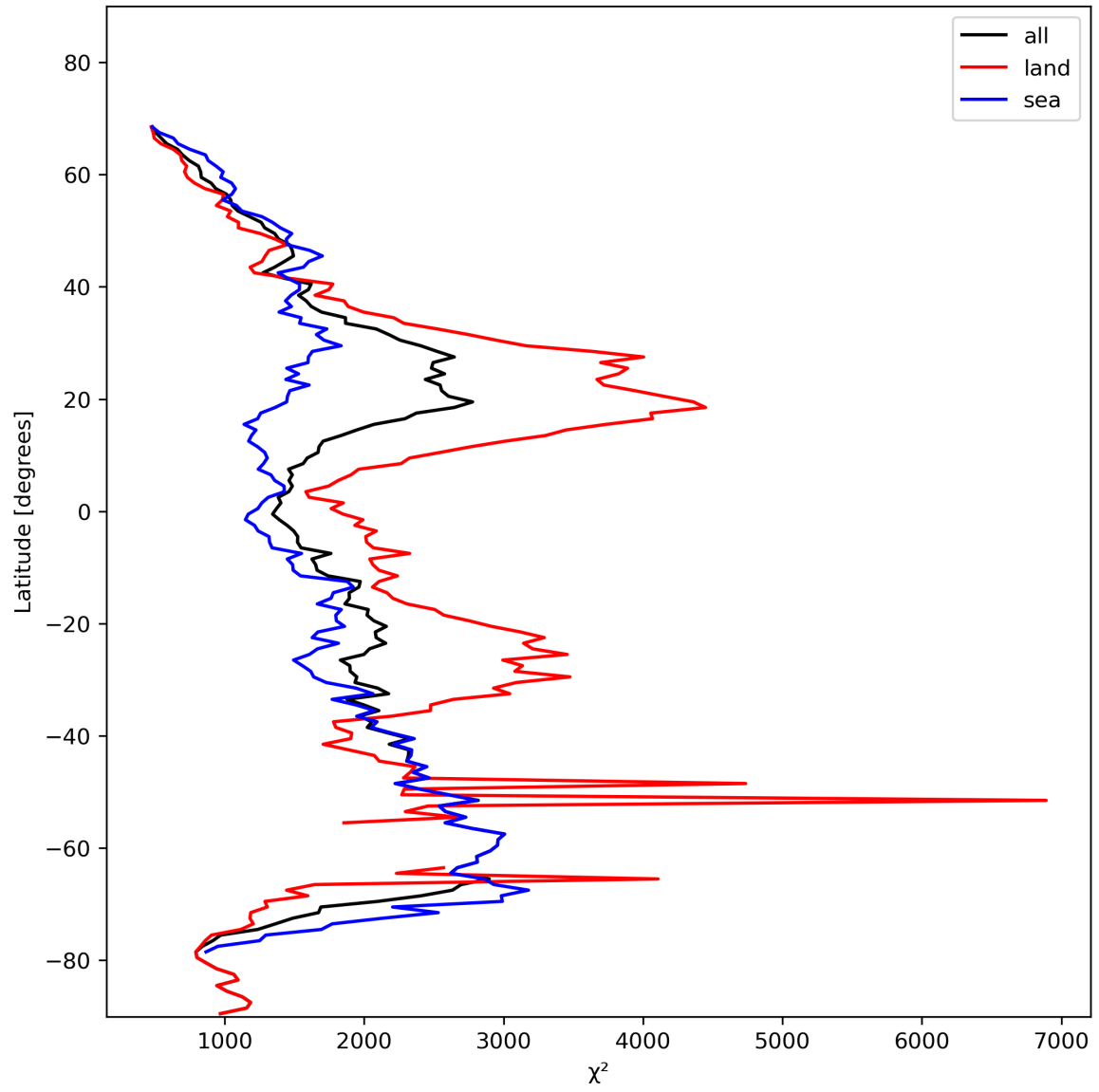
Figure 14: Zonal average of “ \chi^2 ” for 2024-02-03 to 2024-02-05.
