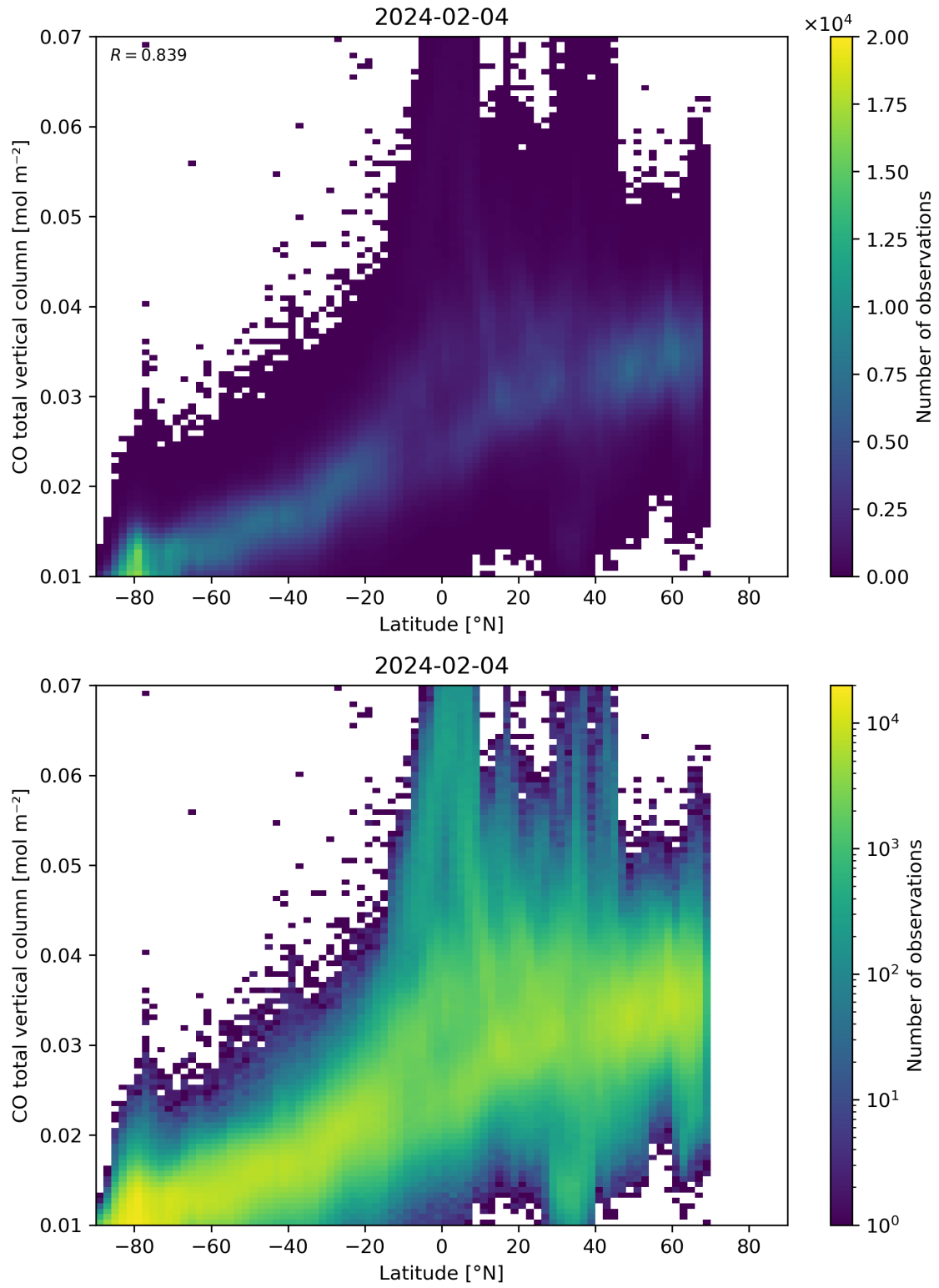
Figure 51: Scatter density plot of “Latitude” against “CO total vertical column” for 2024-02-03 to 2024-02-05.
