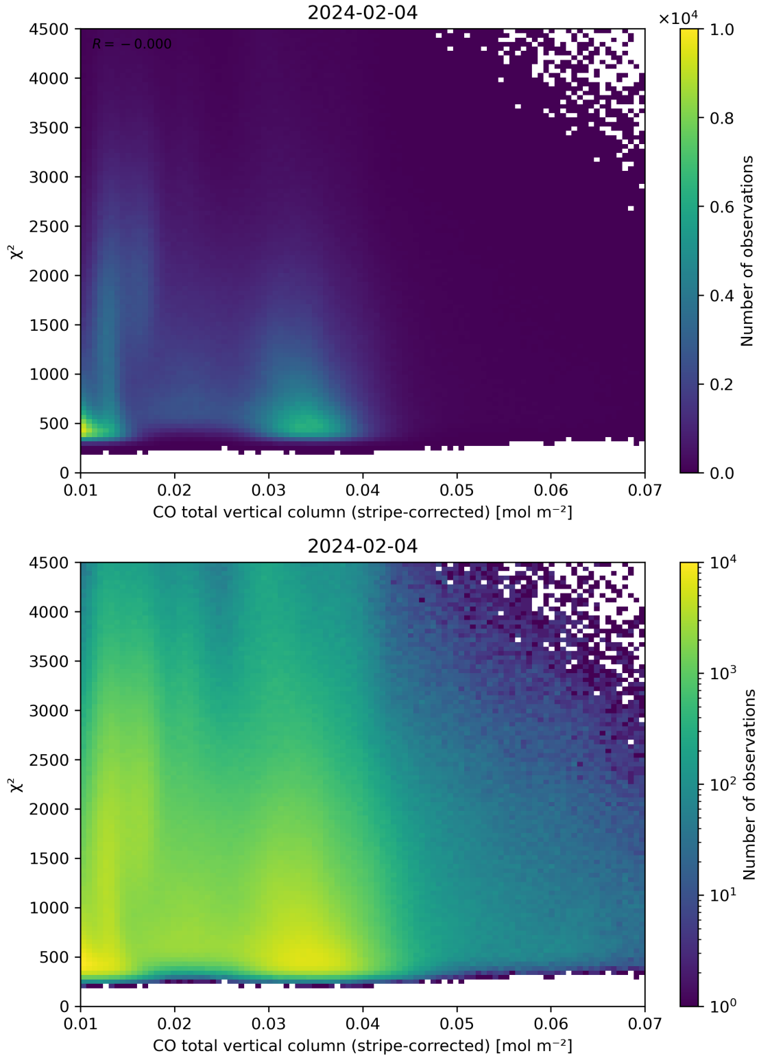
Figure 37: Scatter density plot of “CO total vertical column (stripe-corrected)” against “ \chi^2 ” for 2024-02-03 to 2024-02-05.
