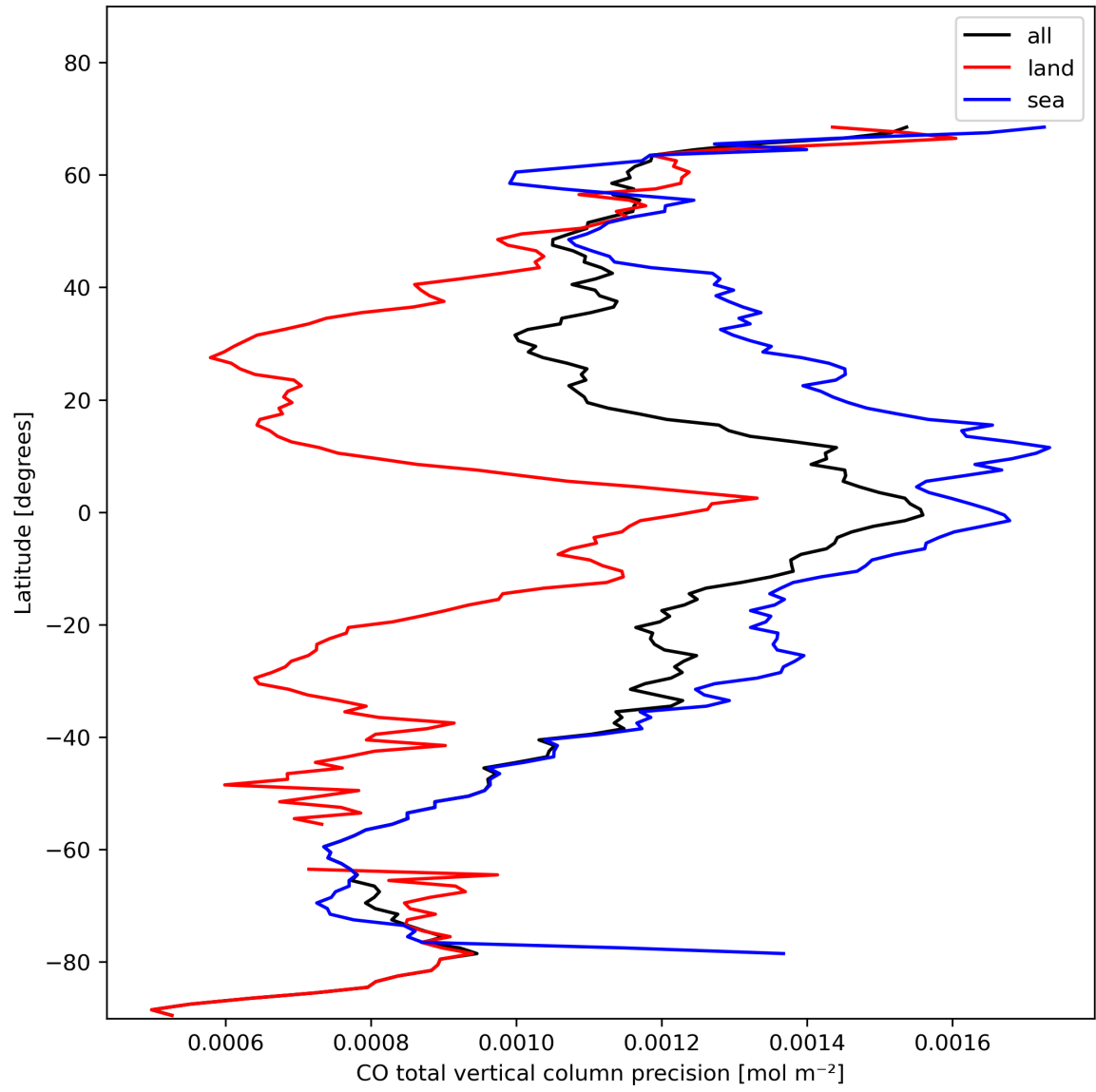
Figure 12: Zonal average of “CO total vertical column precision” for 2024-02-03 to 2024-02-05.
