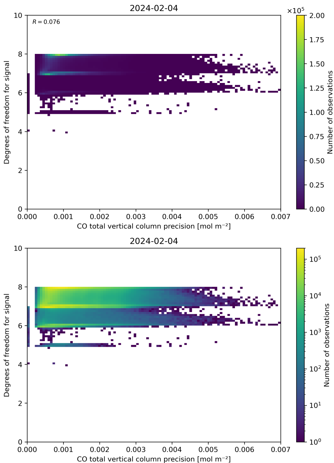
Figure 45: Scatter density plot of “CO total vertical column precision” against “Degrees of freedom for signal” for 2024-02-03 to 2024-02-05.
