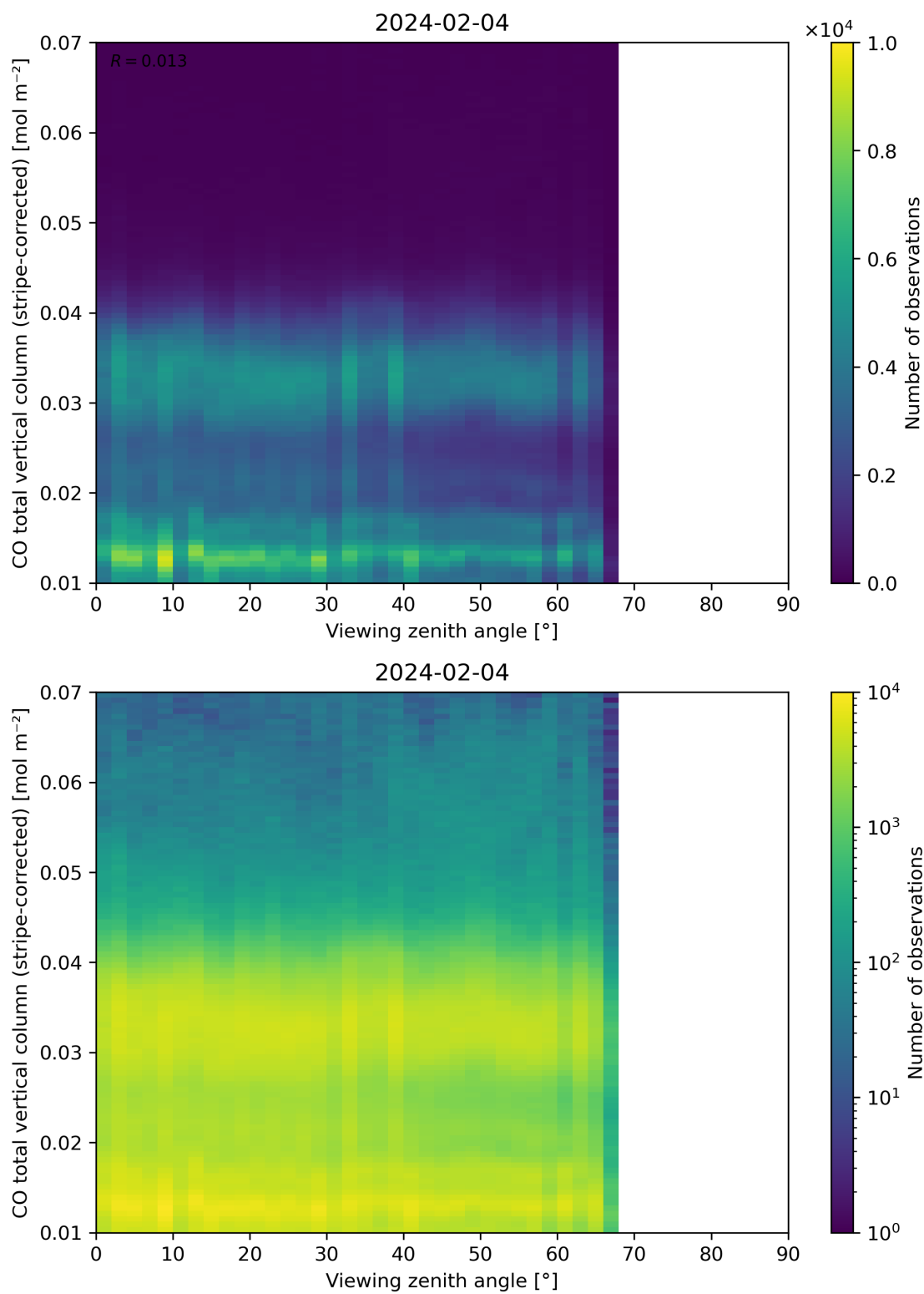
Figure 70: Scatter density plot of “Viewing zenith angle” against “CO total vertical column (stripe-corrected)” for 2024-02-03 to 2024-02-05.
