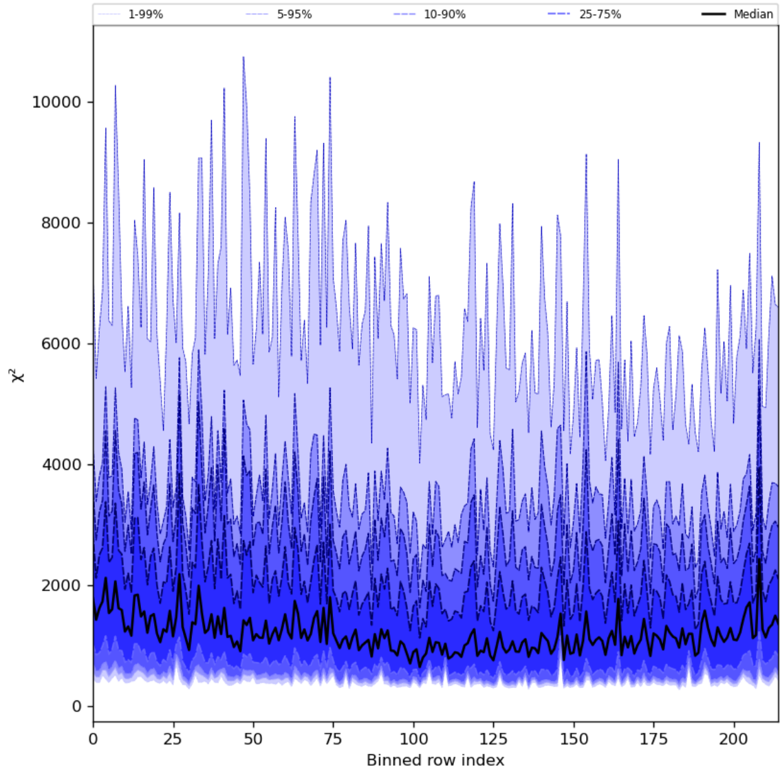
Figure 30: Along track statistics of “ \chi^2 ” for 2024-02-03 to 2024-02-05
