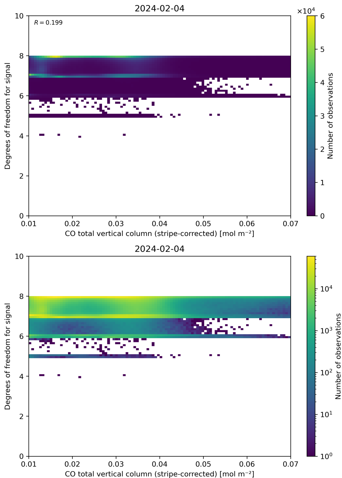
Figure 38: Scatter density plot of “CO total vertical column (stripe-corrected)” against “Degrees of freedom for signal” for 2024-02-03 to 2024-02-05.
