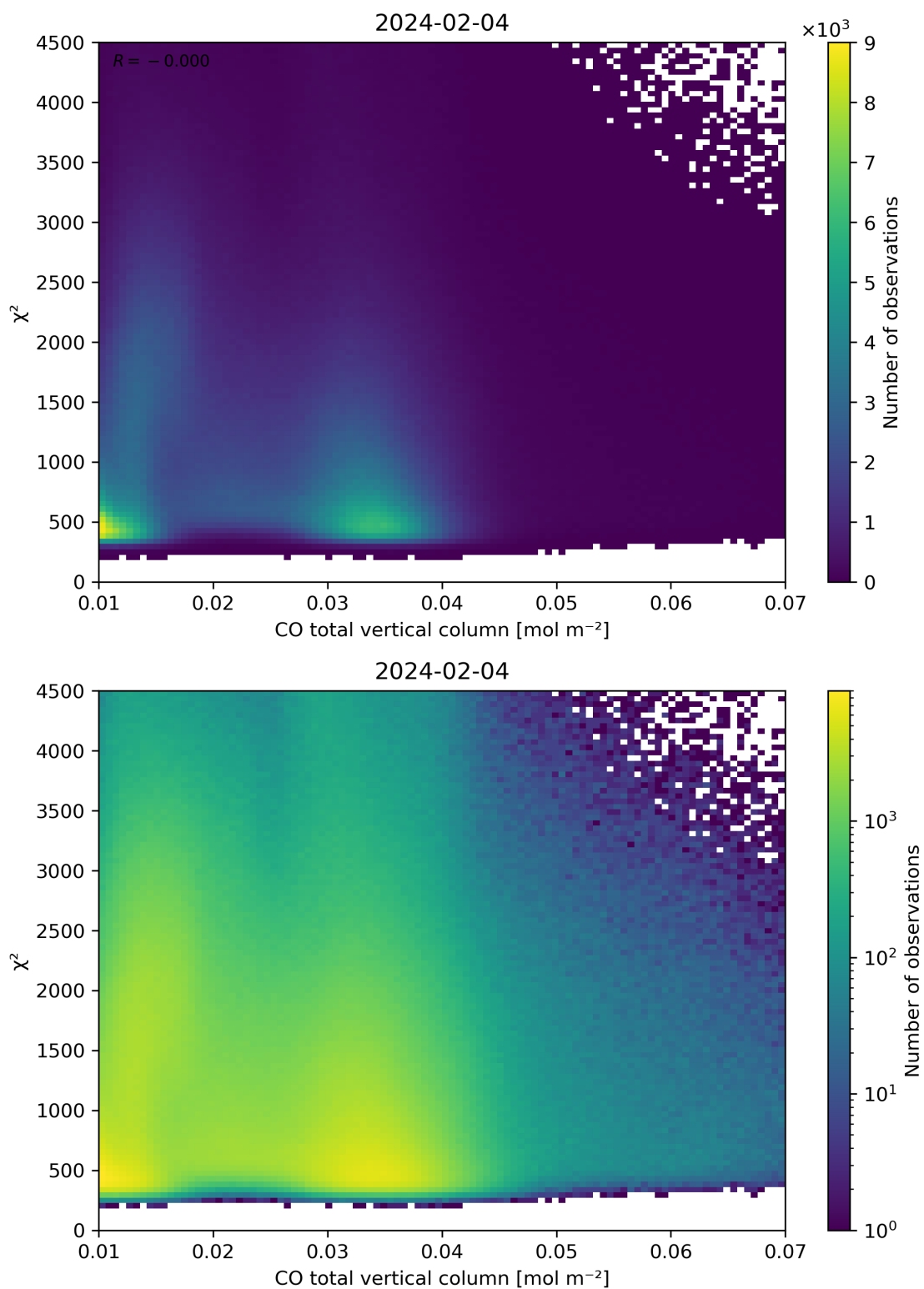
Figure 35: Scatter density plot of “CO total vertical column” against “ \chi^2 ” for 2024-02-03 to 2024-02-05.
