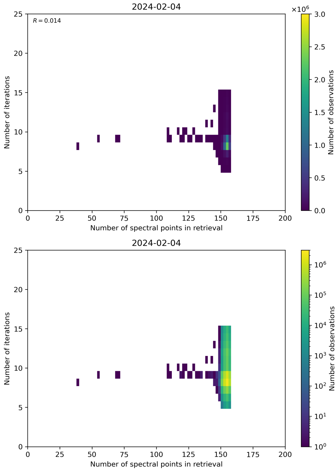
Figure 60: Scatter density plot of “Number of spectral points in retrieval” against “Number of iterations” for 2024-02-03 to 2024-02-05.
