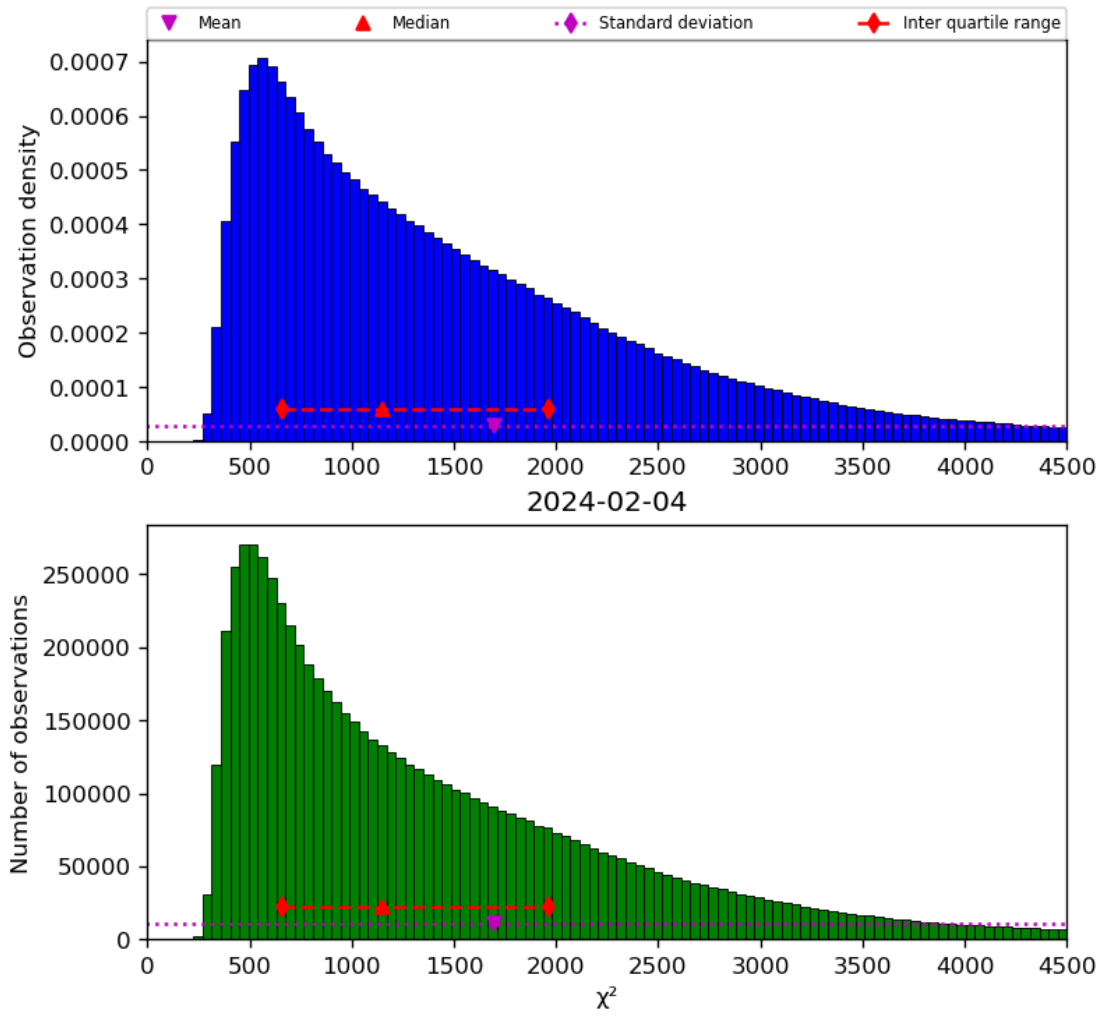
Figure 22: Histogram of “ \chi^2 ” for 2024-02-03 to 2024-02-05
