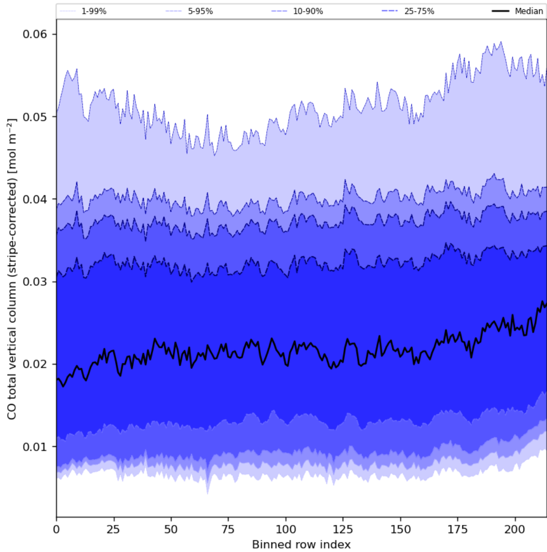
Figure 27: Along track statistics of “CO total vertical column (stripe-corrected)” for 2024-02-03 to 2024-02-05
