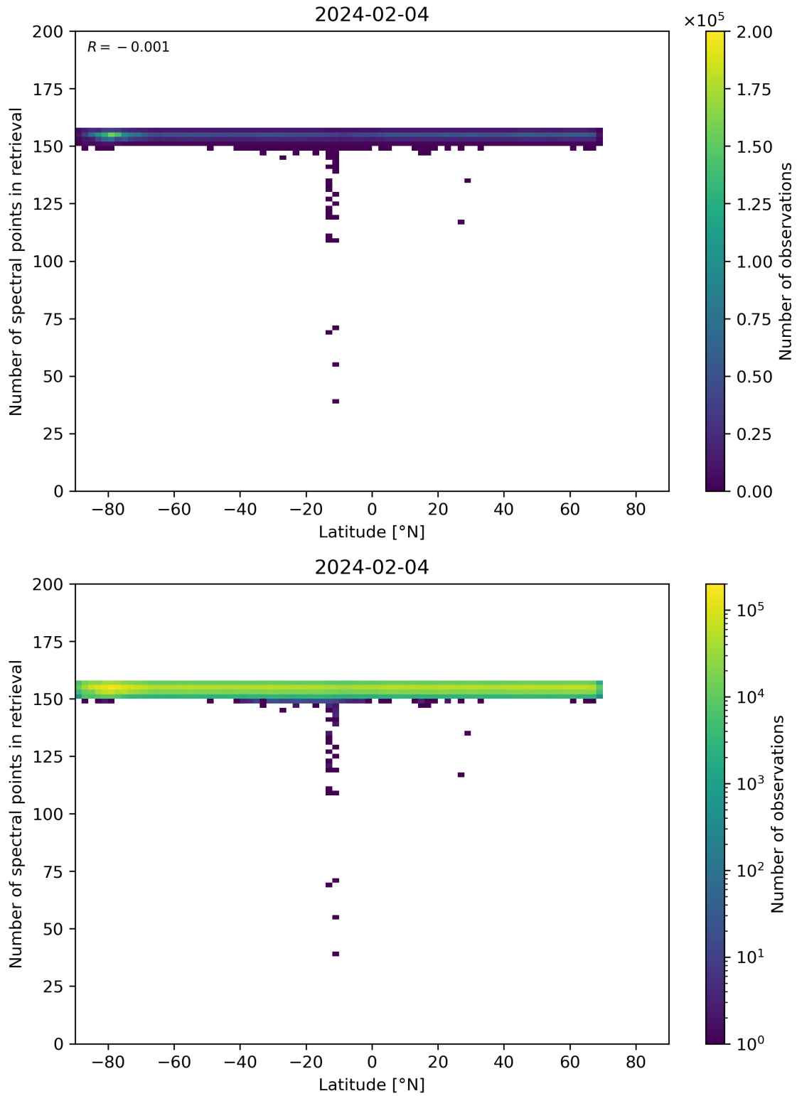
Figure 57: Scatter density plot of “Latitude” against “Number of spectral points in retrieval” for 2024-02-03 to 2024-02-05.
