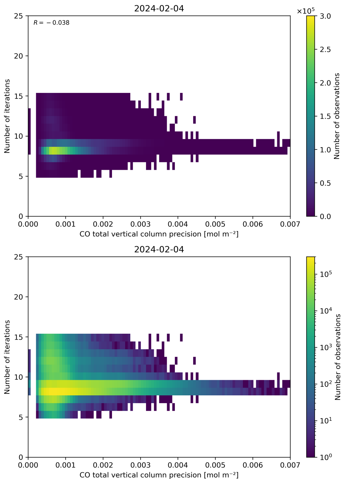
Figure 46: Scatter density plot of “CO total vertical column precision” against “Number of iterations” for 2024-02-03 to 2024-02-05.
