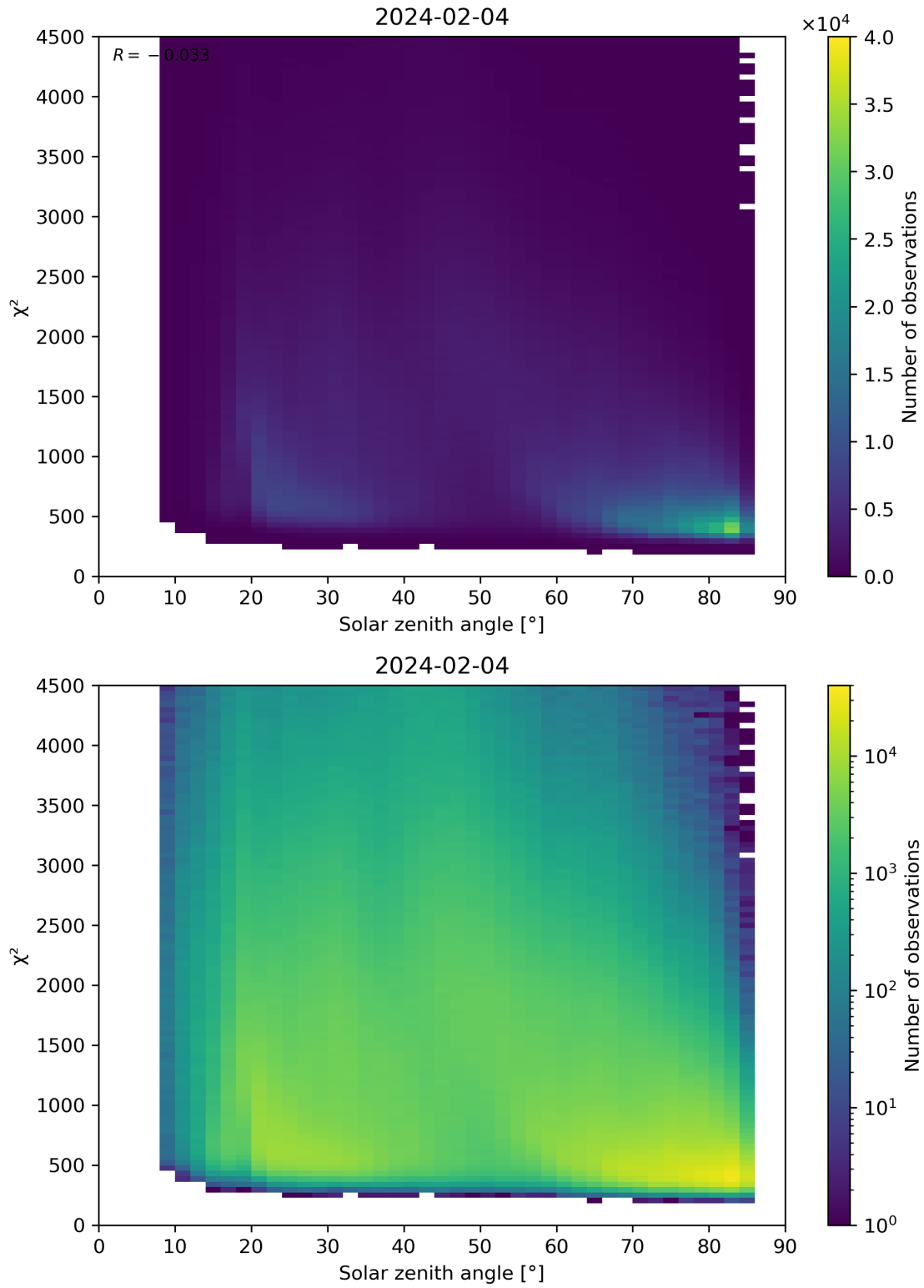
Figure 64: Scatter density plot of “Solar zenith angle” against “ \chi^2 ” for 2024-02-03 to 2024-02-05.
