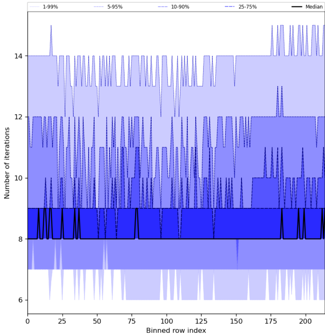
Figure 32: Along track statistics of “Number of iterations” for 2024-02-03 to 2024-02-05
