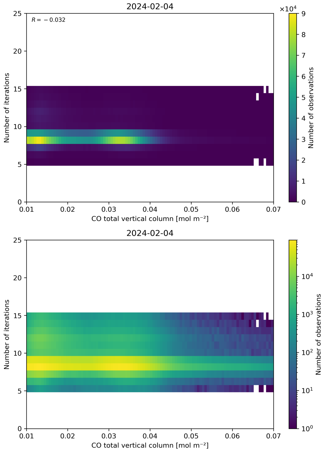
Figure 42: Scatter density plot of “CO total vertical column” against “Number of iterations” for 2024-02-03 to 2024-02-05.
